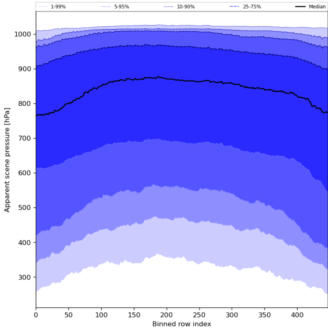
Figure 53: Along track statistics of “Apparent scene pressure” for 2023-12-16 to 2023-12-18
