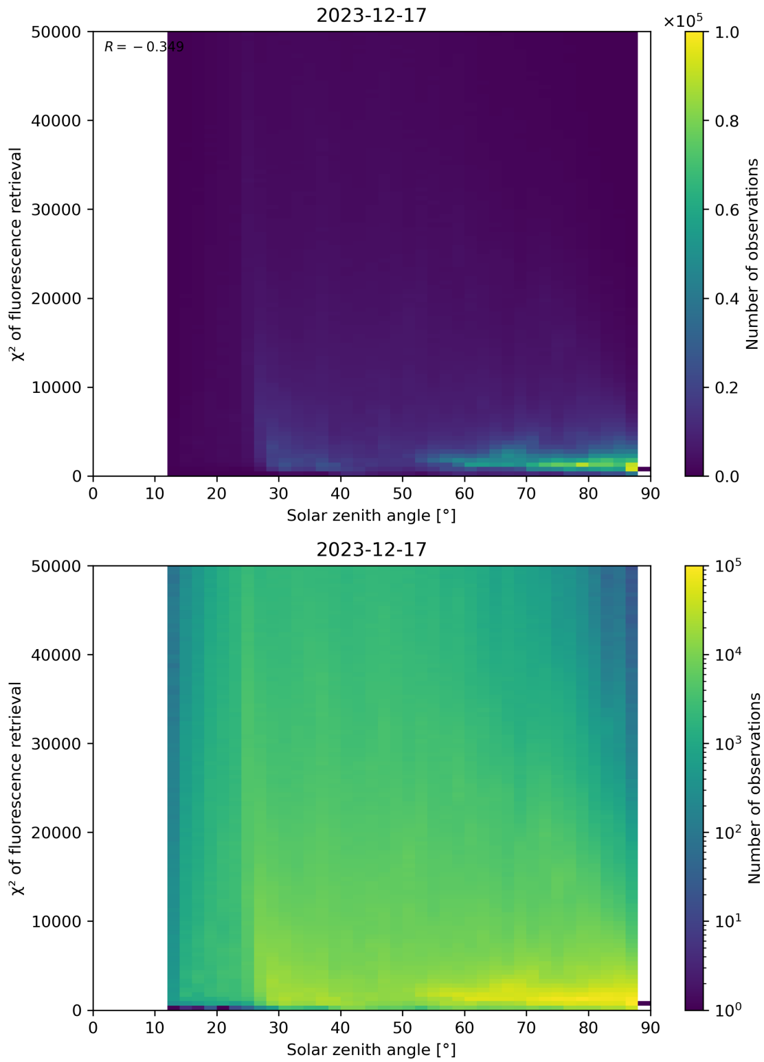
Figure 109: Scatter density plot of “Solar zenith angle” against “ \chi^2 of fluorescence retrieval” for 2023-12-16 to 2023-12-18.
