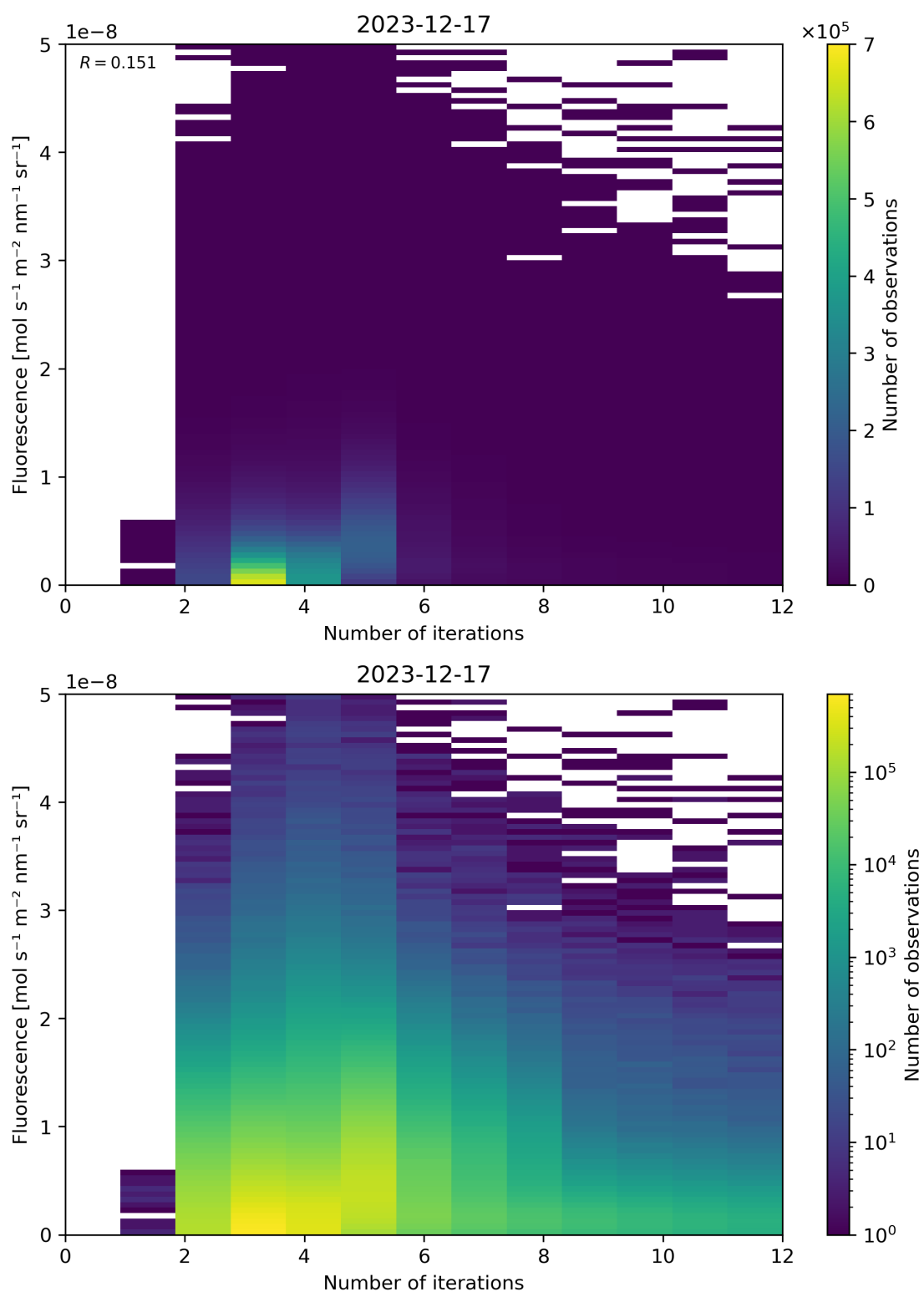
Figure 98: Scatter density plot of “Number of iterations” against “Fluorescence” for 2023-12-16 to 2023-12-18.
