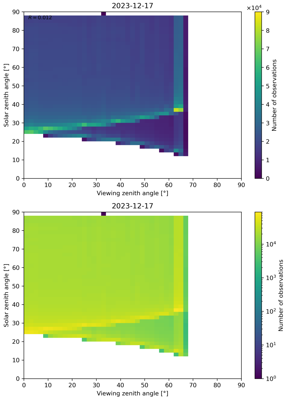
Figure 127: Scatter density plot of “Viewing zenith angle” against “Solar zenith angle” for 2023-12-16 to 2023-12-18.
