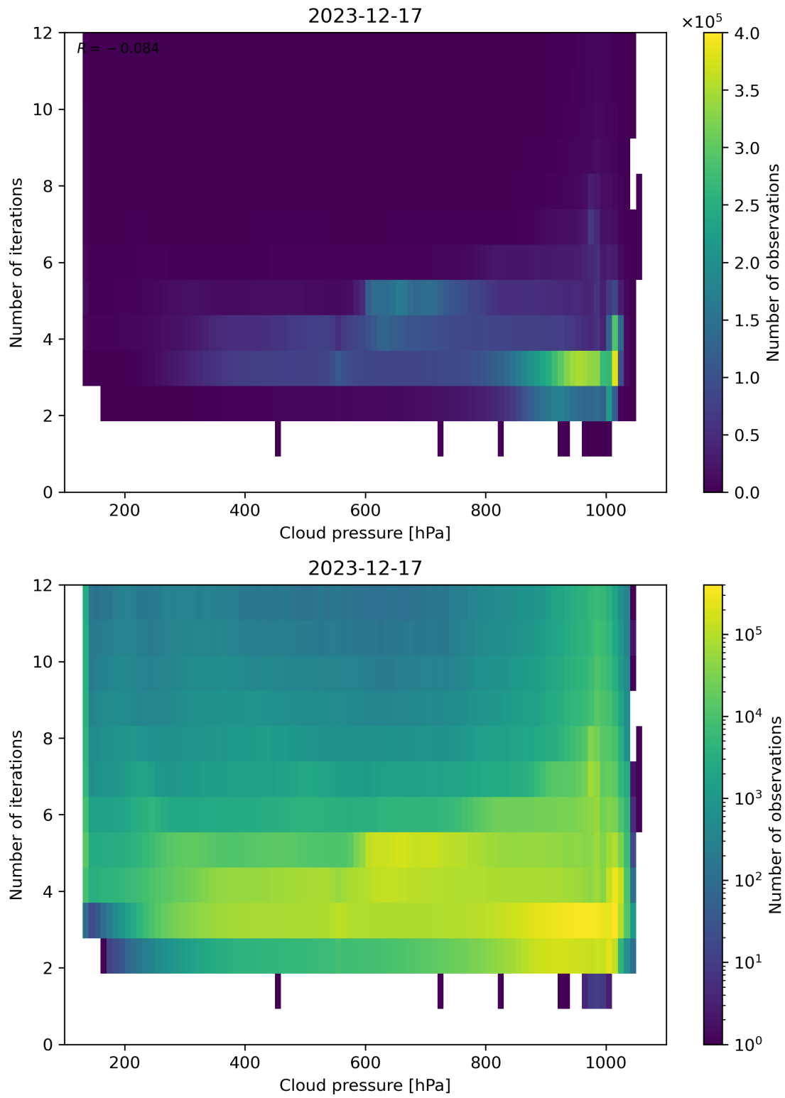
Figure 81: Scatter density plot of “Cloud pressure” against “Number of iterations” for 2023-12-16 to 2023-12-18.
