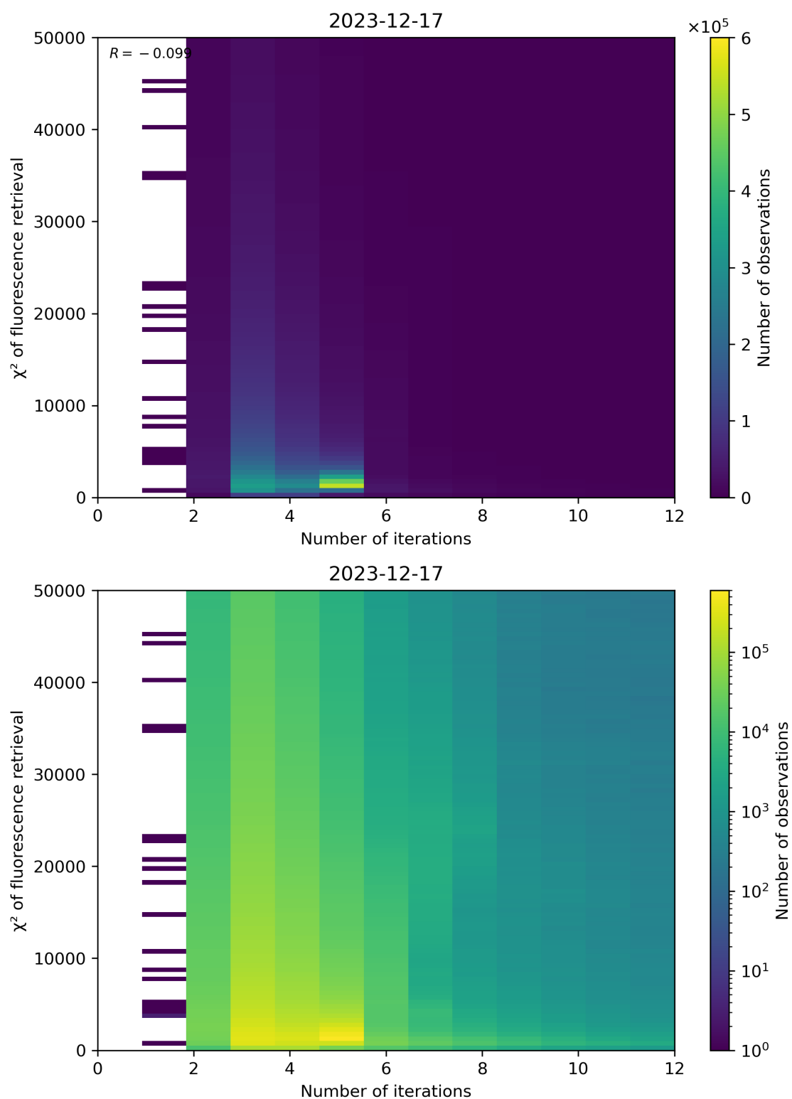
Figure 97: Scatter density plot of “Number of iterations” against “ \chi^2 of fluorescence retrieval” for 2023-12-16 to 2023-12-18.
