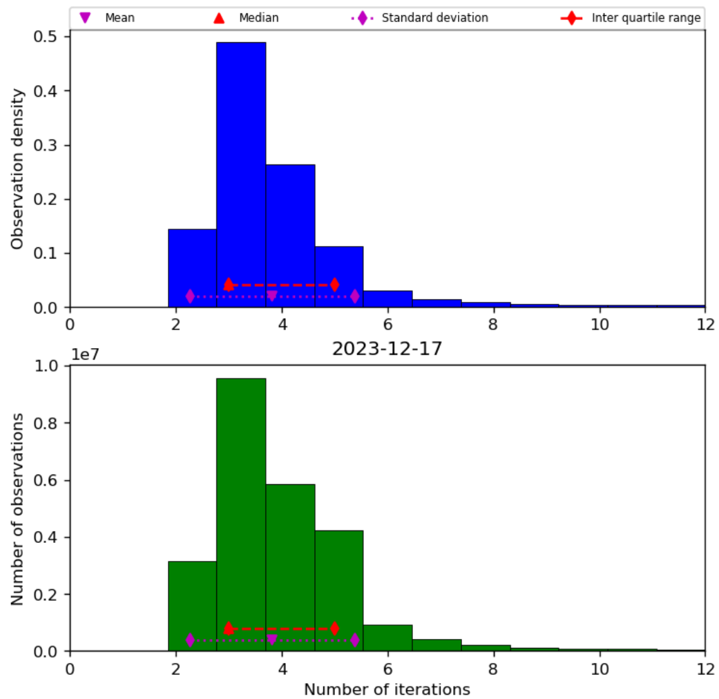
Figure 39: Histogram of “Number of iterations” for 2023-12-16 to 2023-12-18
