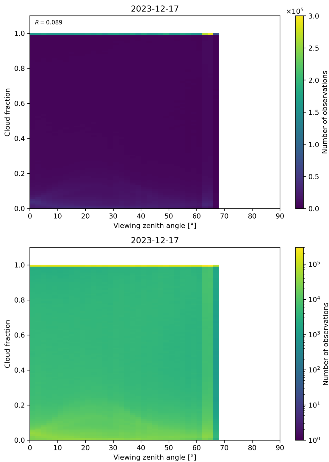
Figure 120: Scatter density plot of “Viewing zenith angle” against “Cloud fraction” for 2023-12-16 to 2023-12-18.
