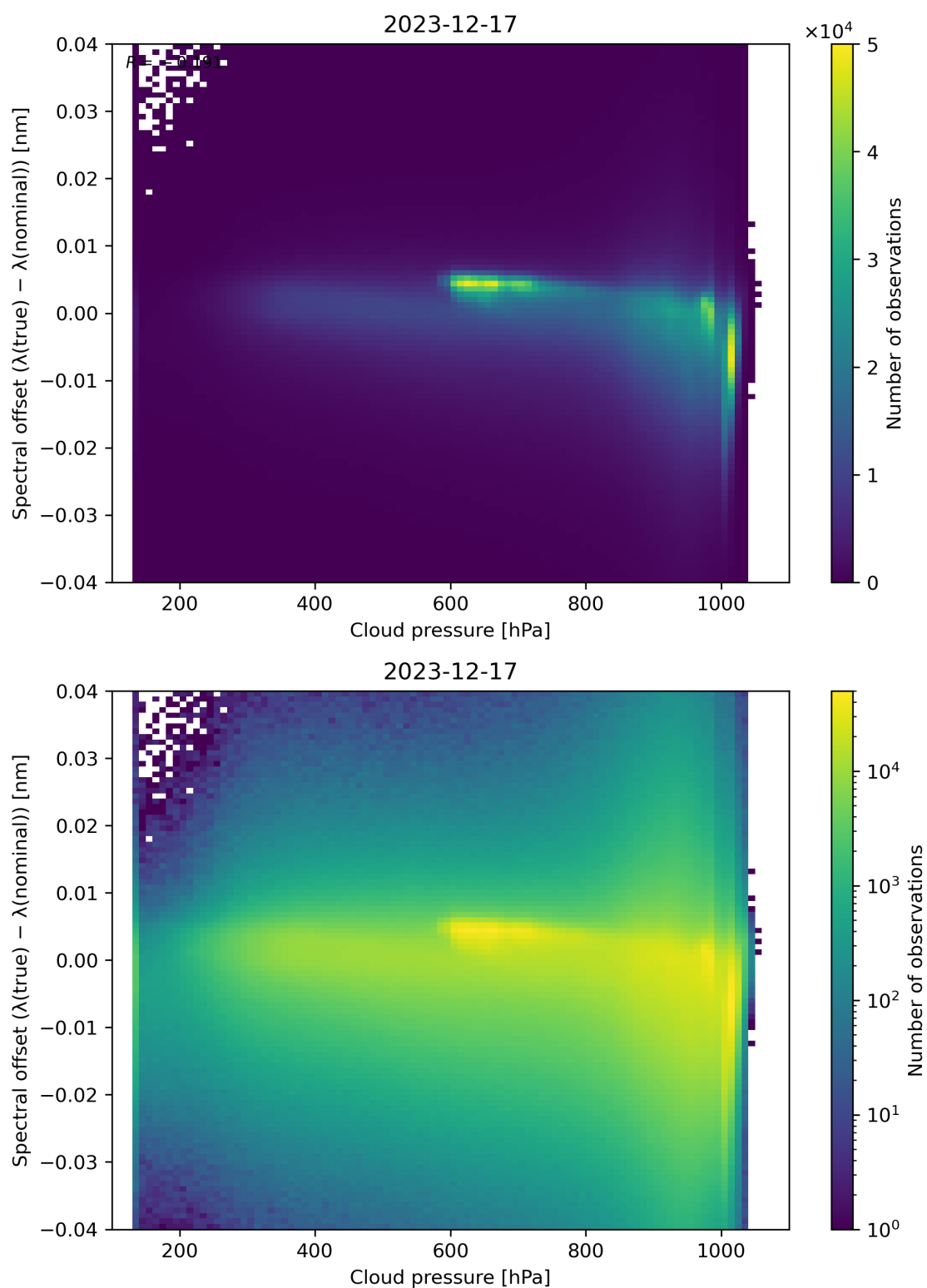
Figure 84: Scatter density plot of “Cloud pressure” against “Spectral offset ( \lambda(\text{true}) - \lambda(\text{nominal}) )” for 2023-12-16 to 2023-12-18.
