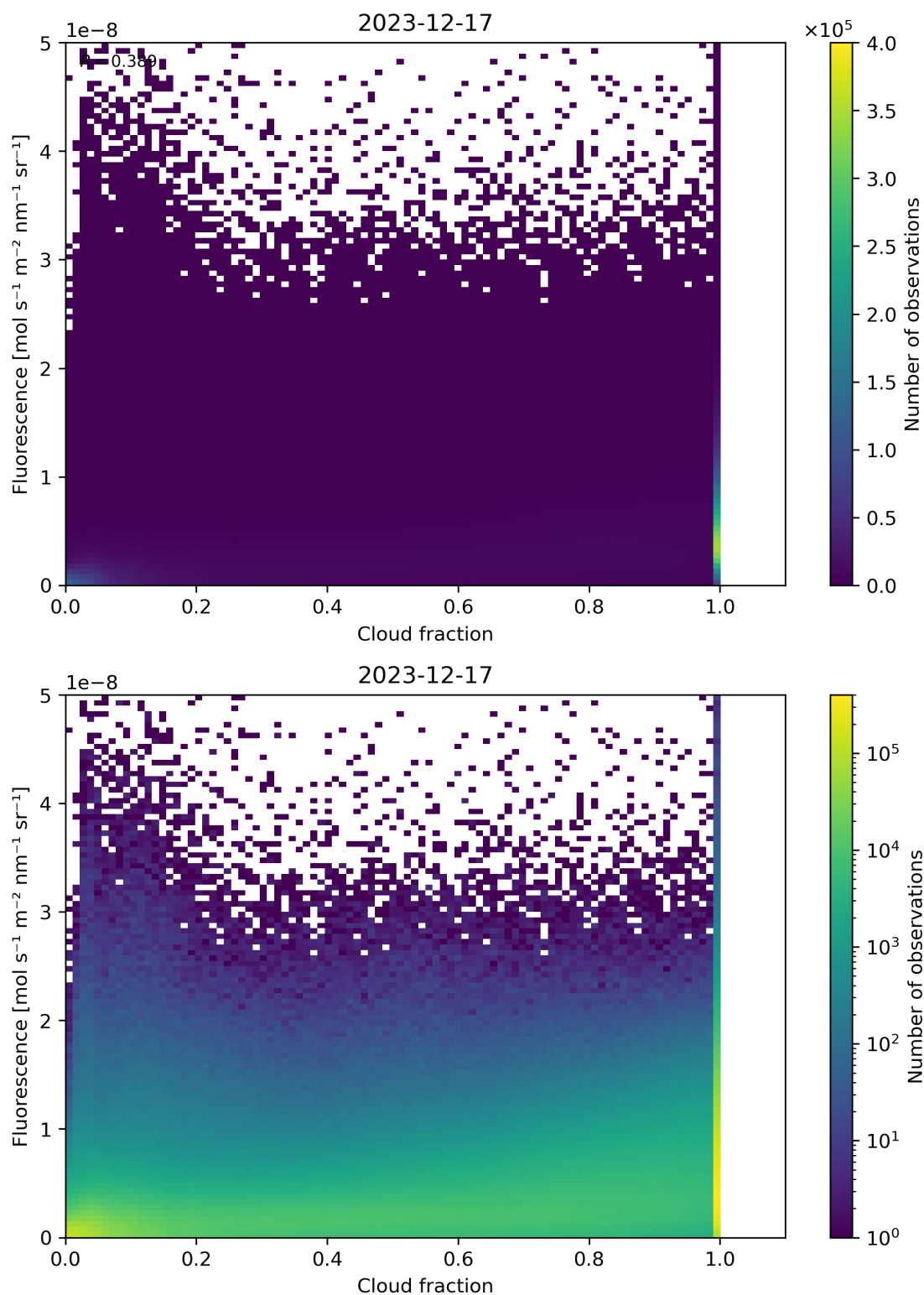
Figure 72: Scatter density plot of “Cloud fraction” against “Fluorescence” for 2023-12-16 to 2023-12-18.
