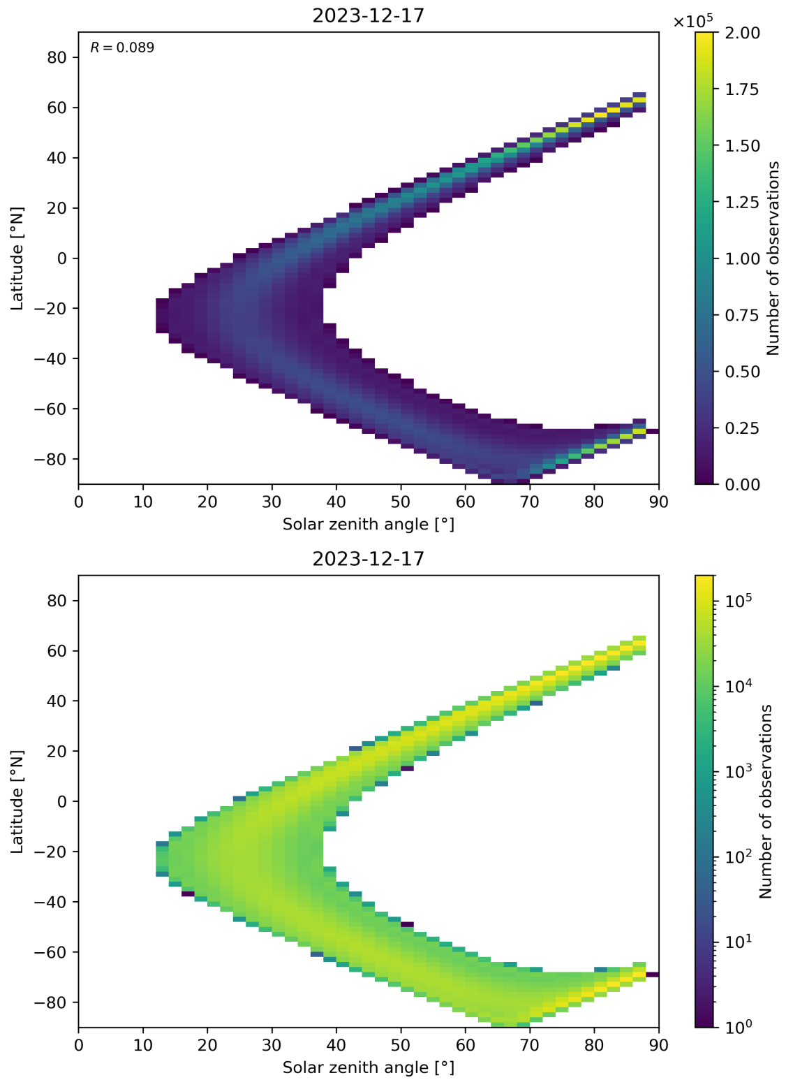
Figure 113: Scatter density plot of “Solar zenith angle” against “Latitude” for 2023-12-16 to 2023-12-18.
