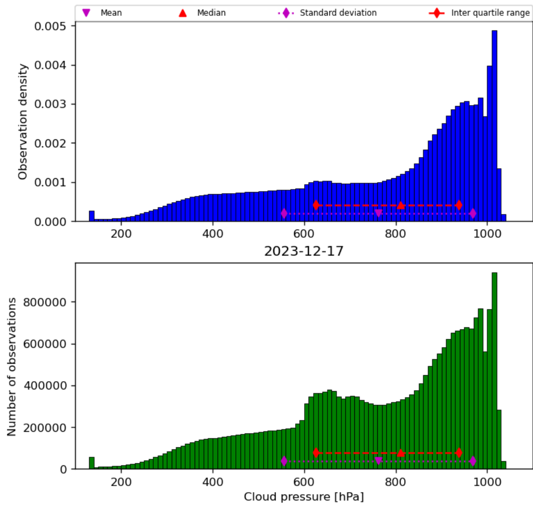
Figure 30: Histogram of “Cloud pressure” for 2023-12-16 to 2023-12-18
