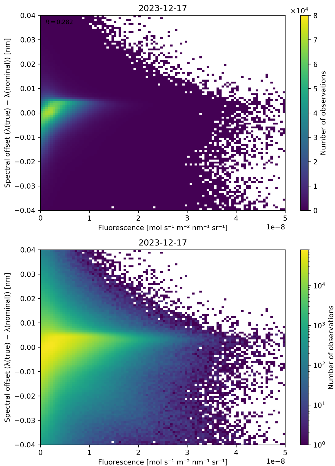
Figure 87: Scatter density plot of “Fluorescence” against “Spectral offset ( \lambda(\text{true}) - \lambda(\text{nominal}) )” for 2023-12-16 to 2023-12-18.
