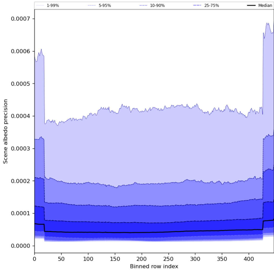
Figure 52: Along track statistics of “Scene albedo precision” for 2023-12-16 to 2023-12-18
