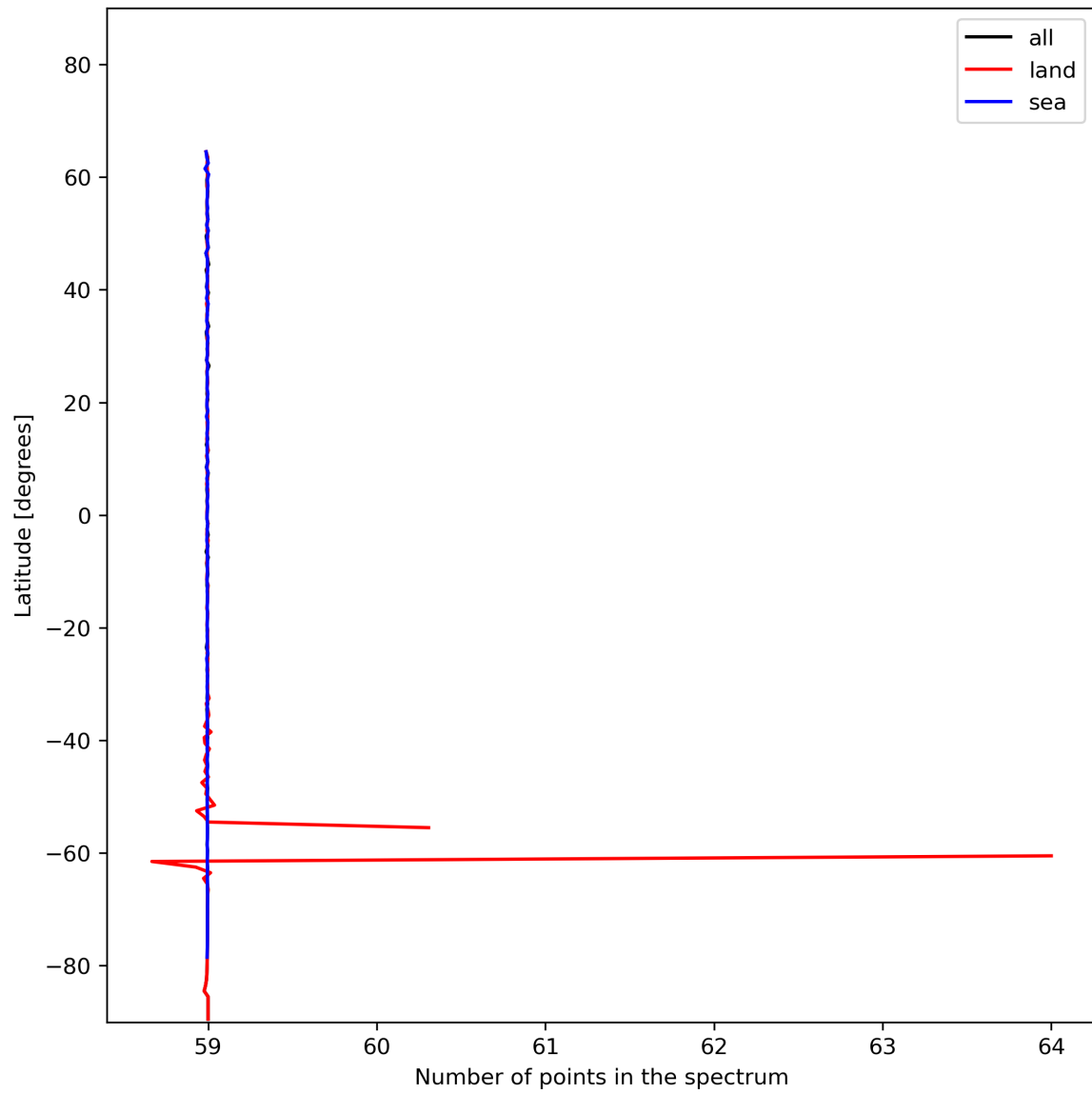
Figure 27: Zonal average of “Number of points in the spectrum” for 2023-12-16 to 2023-12-18.
