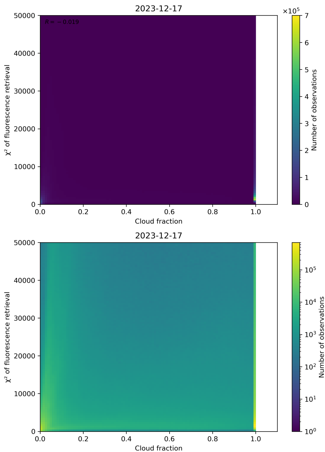
Figure 71: Scatter density plot of “Cloud fraction” against “ \chi^2 of fluorescence retrieval” for 2023-12-16 to 2023-12-18.
