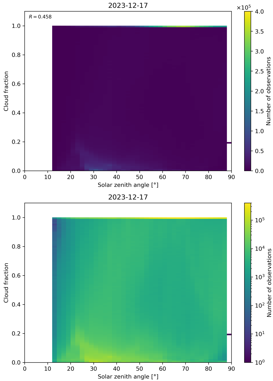
Figure 110: Scatter density plot of “Solar zenith angle” against “Cloud fraction” for 2023-12-16 to 2023-12-18.
