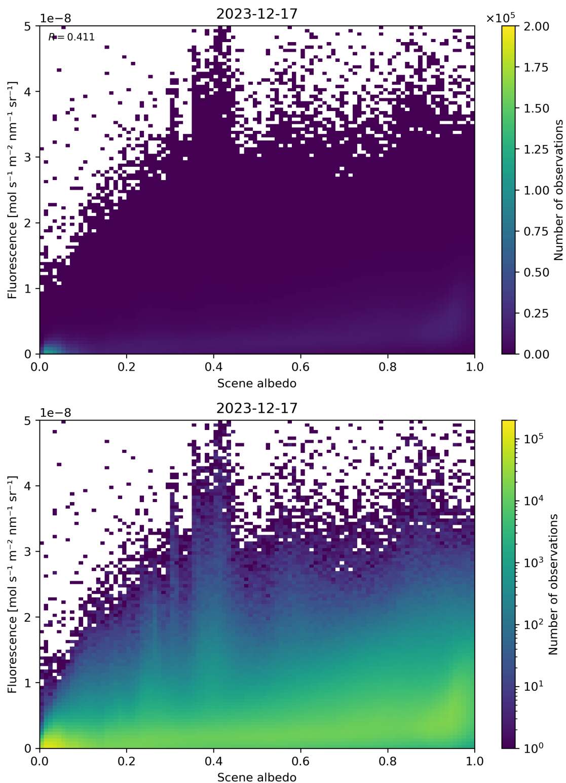
Figure 104: Scatter density plot of “Scene albedo” against “Fluorescence” for 2023-12-16 to 2023-12-18.
