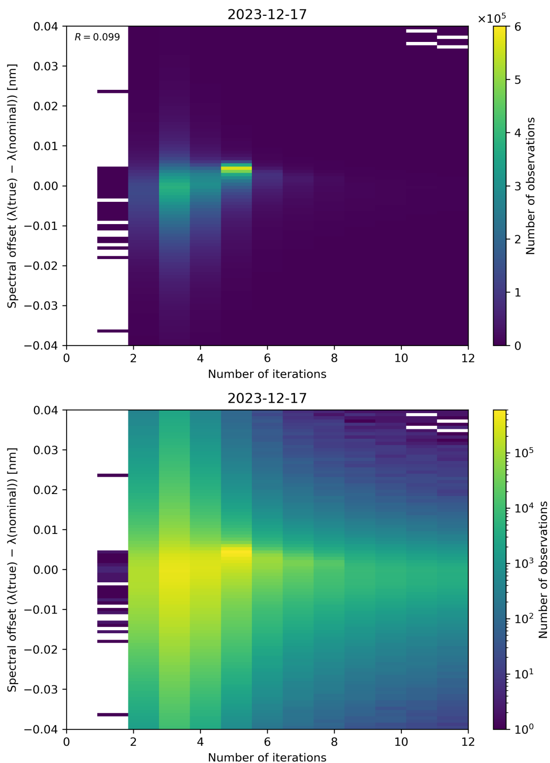
Figure 100: Scatter density plot of “Number of iterations” against “Spectral offset ( \lambda(\text{true}) - \lambda(\text{nominal}) )” for 2023-12-16 to 2023-12-18.
