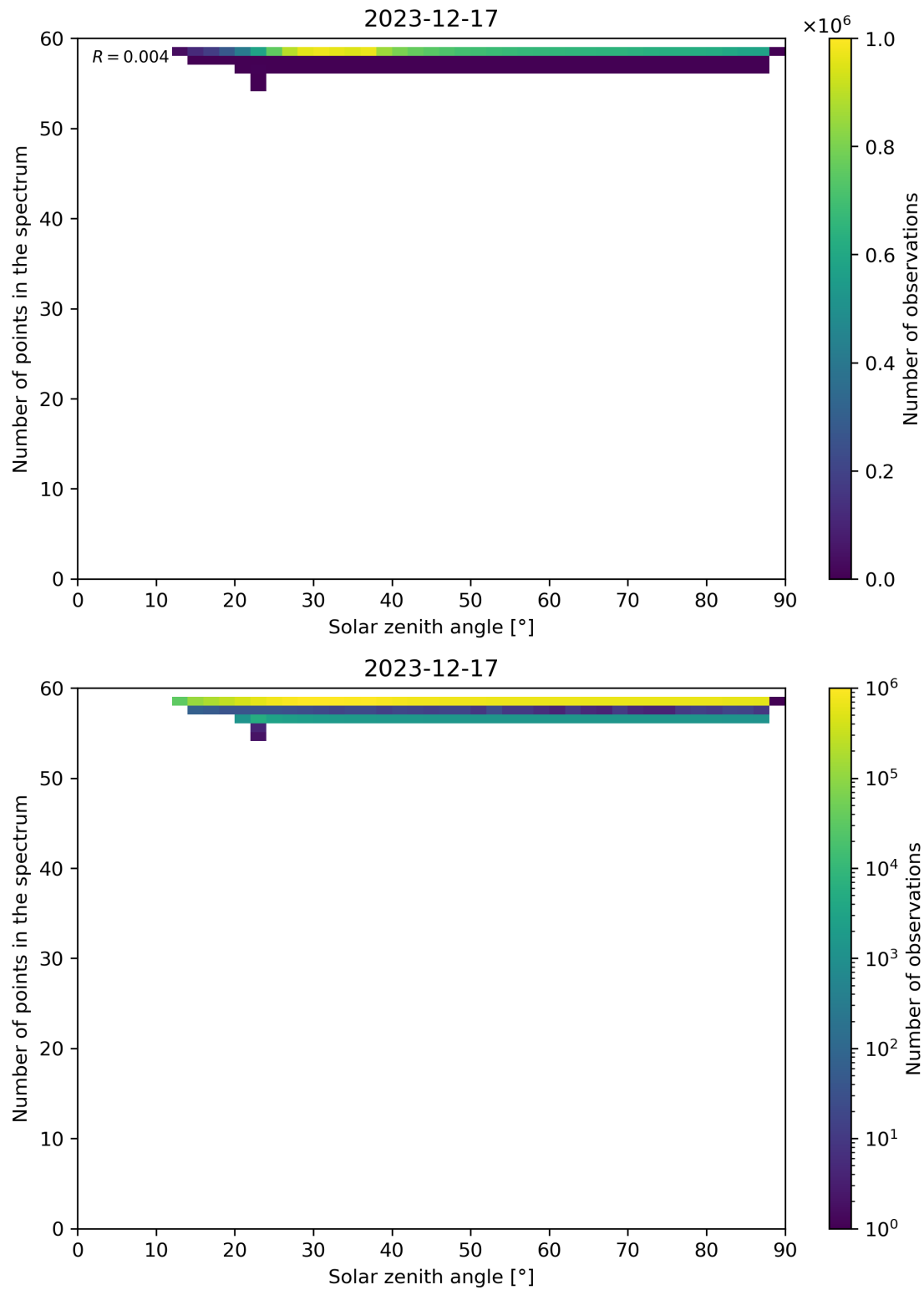
Figure 115: Scatter density plot of “Solar zenith angle” against “Number of points in the spectrum” for 2023-12-16 to 2023-12-18.
