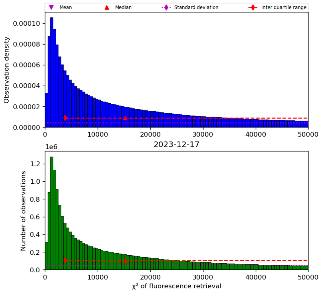
Figure 42: Histogram of “ \chi^2 of fluorescence retrieval” for 2023-12-16 to 2023-12-18
