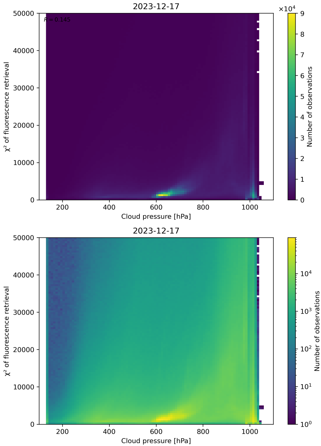
Figure 78: Scatter density plot of “Cloud pressure” against “ \chi^2 of fluorescence retrieval” for 2023-12-16 to 2023-12-18.
