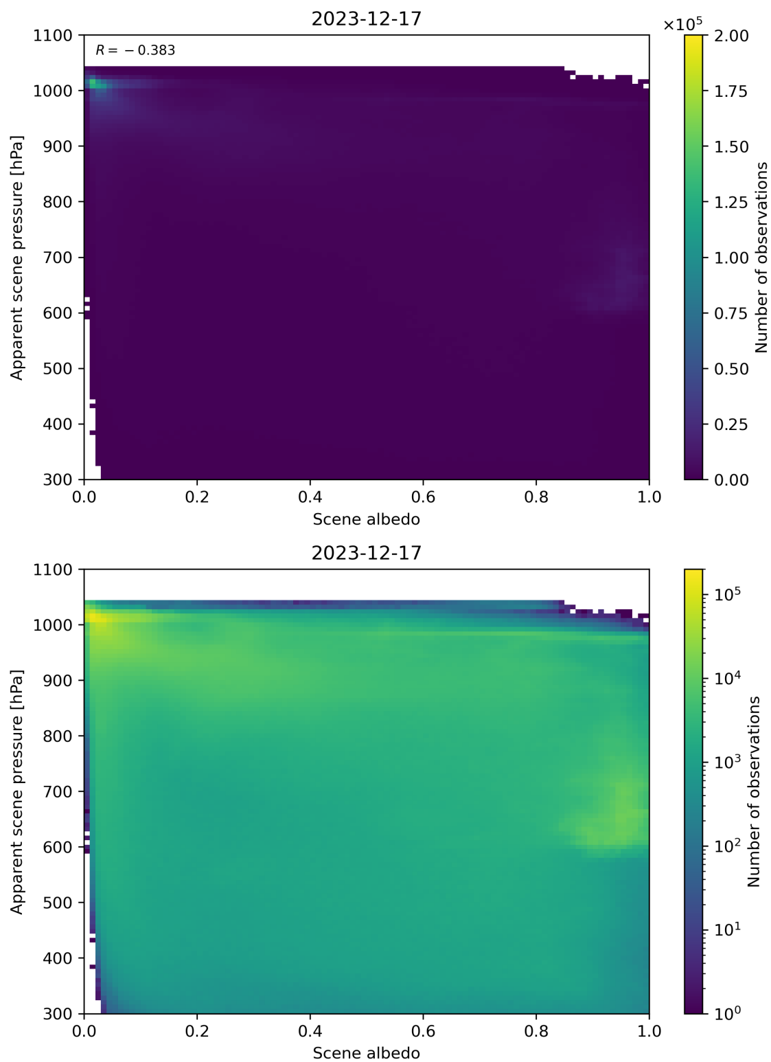
Figure 102: Scatter density plot of “Scene albedo” against “Apparent scene pressure” for 2023-12-16 to 2023-12-18.
