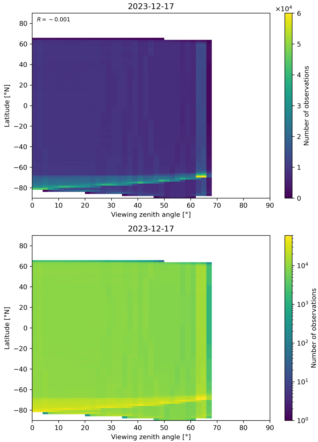
Figure 123: Scatter density plot of “Viewing zenith angle” against “Latitude” for 2023-12-16 to 2023-12-18.
