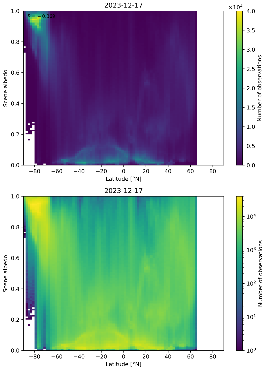
Figure 95: Scatter density plot of “Latitude” against “Scene albedo” for 2023-12-16 to 2023-12-18.
