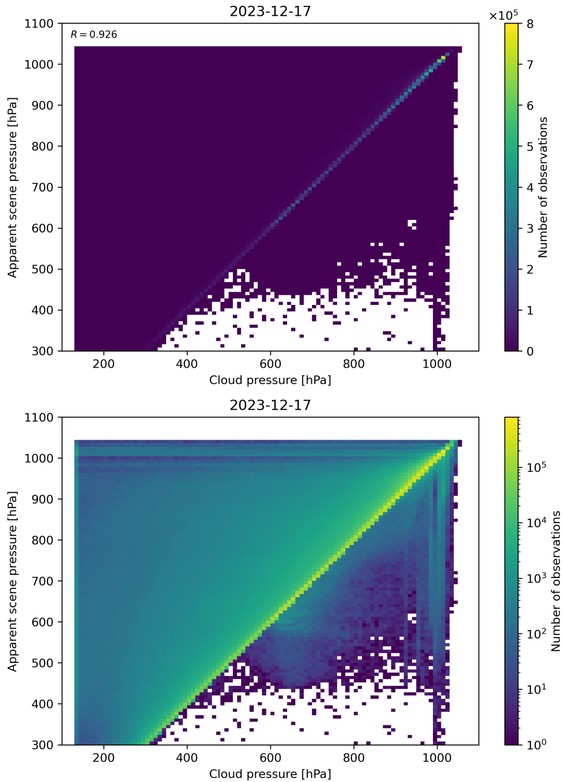
Figure 77: Scatter density plot of “Cloud pressure” against “Apparent scene pressure” for 2023-12-16 to 2023-12-18.
