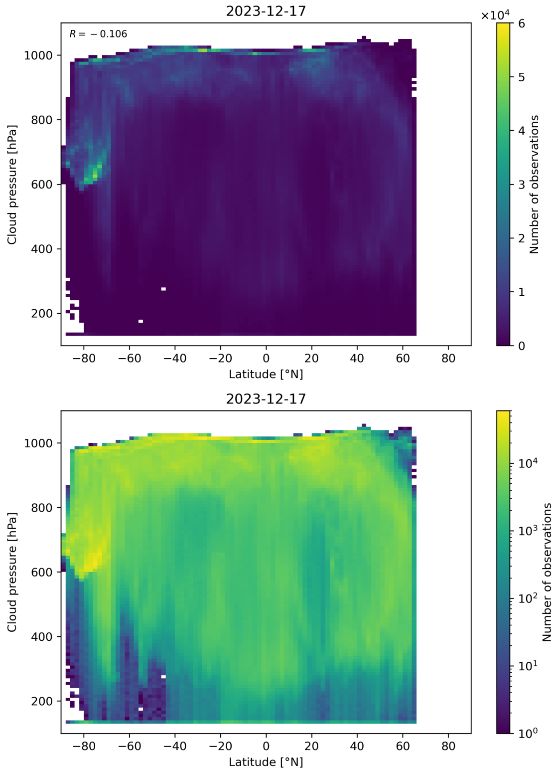
Figure 91: Scatter density plot of “Latitude” against “Cloud pressure” for 2023-12-16 to 2023-12-18.
