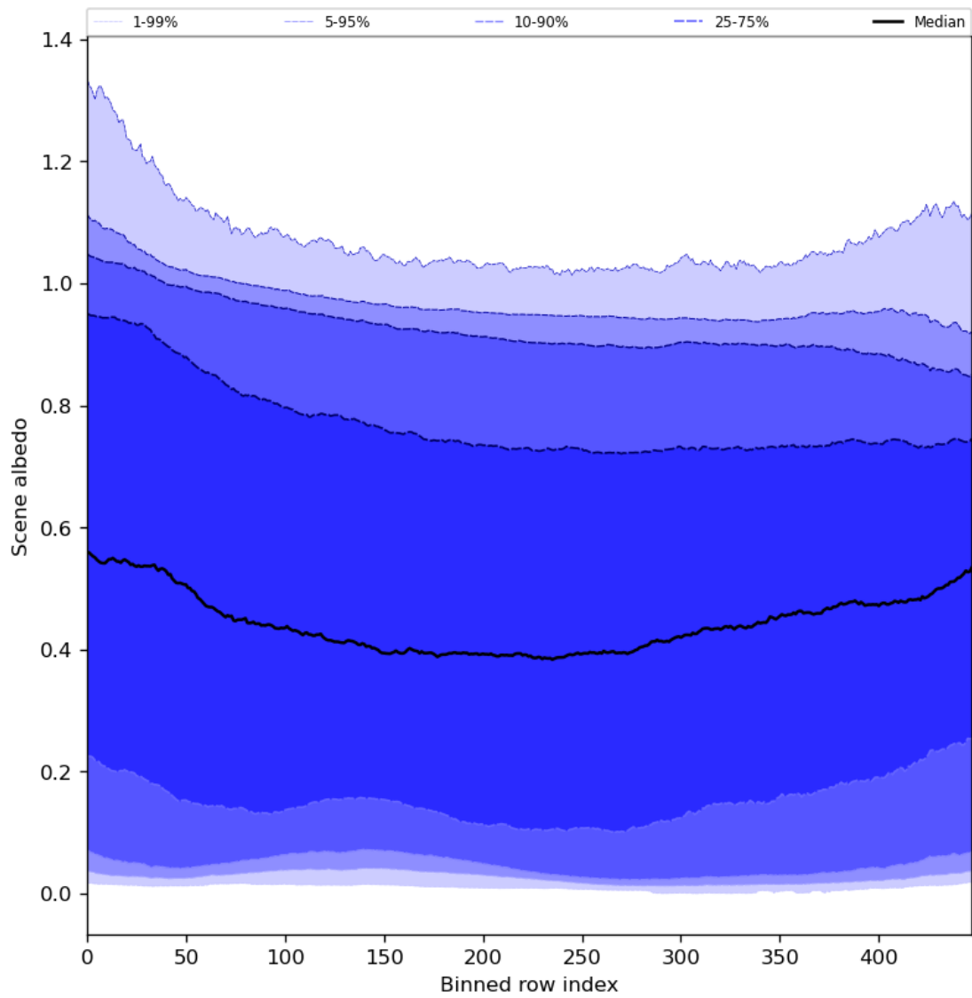
Figure 51: Along track statistics of “Scene albedo” for 2023-12-16 to 2023-12-18
