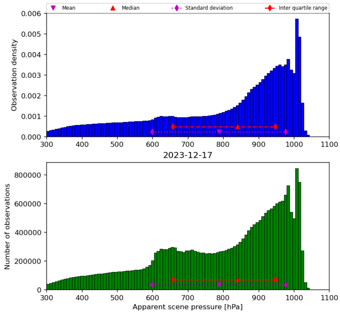
Figure 36: Histogram of “Apparent scene pressure” for 2023-12-16 to 2023-12-18
