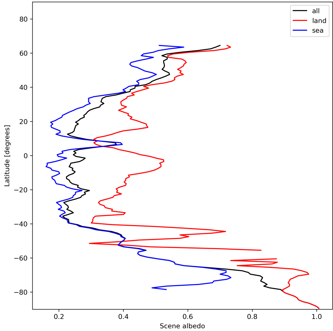
Figure 17: Zonal average of “Scene albedo” for 2023-12-16 to 2023-12-18.
