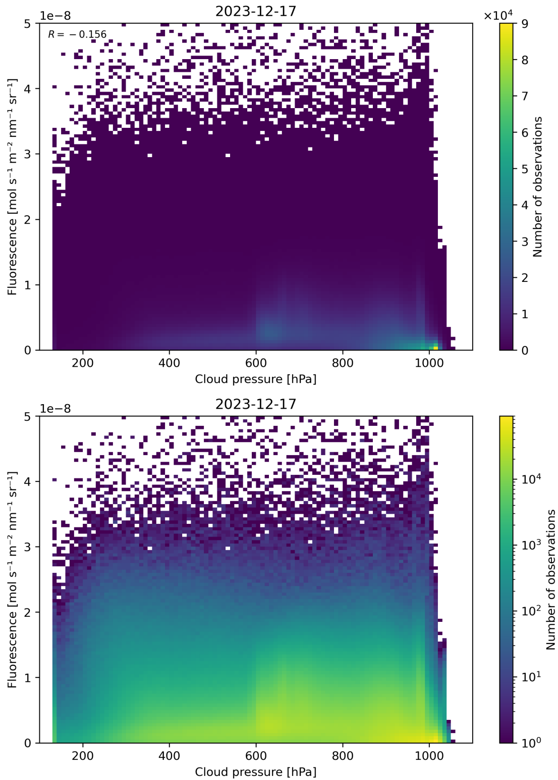
Figure 80: Scatter density plot of “Cloud pressure” against “Fluorescence” for 2023-12-16 to 2023-12-18.
