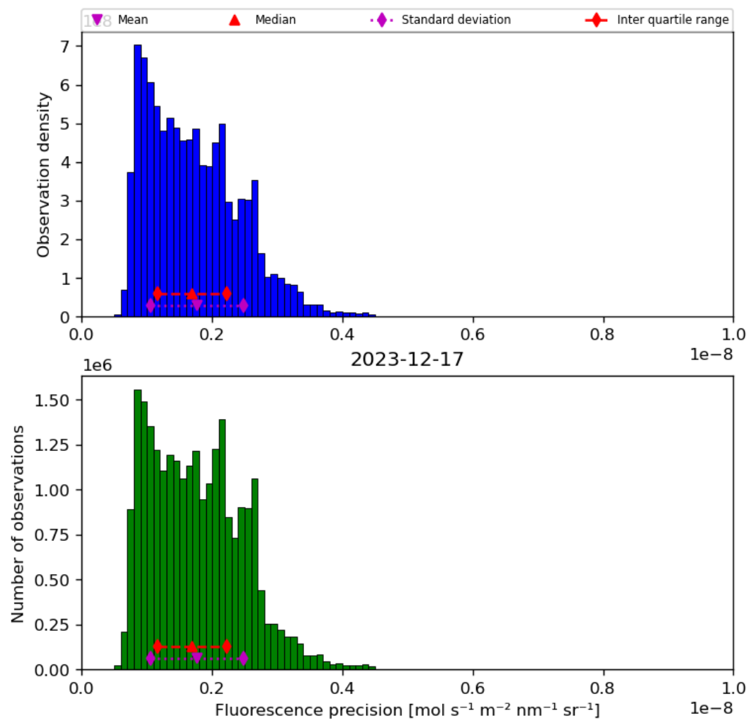
Figure 41: Histogram of “Fluorescence precision” for 2023-12-16 to 2023-12-18
