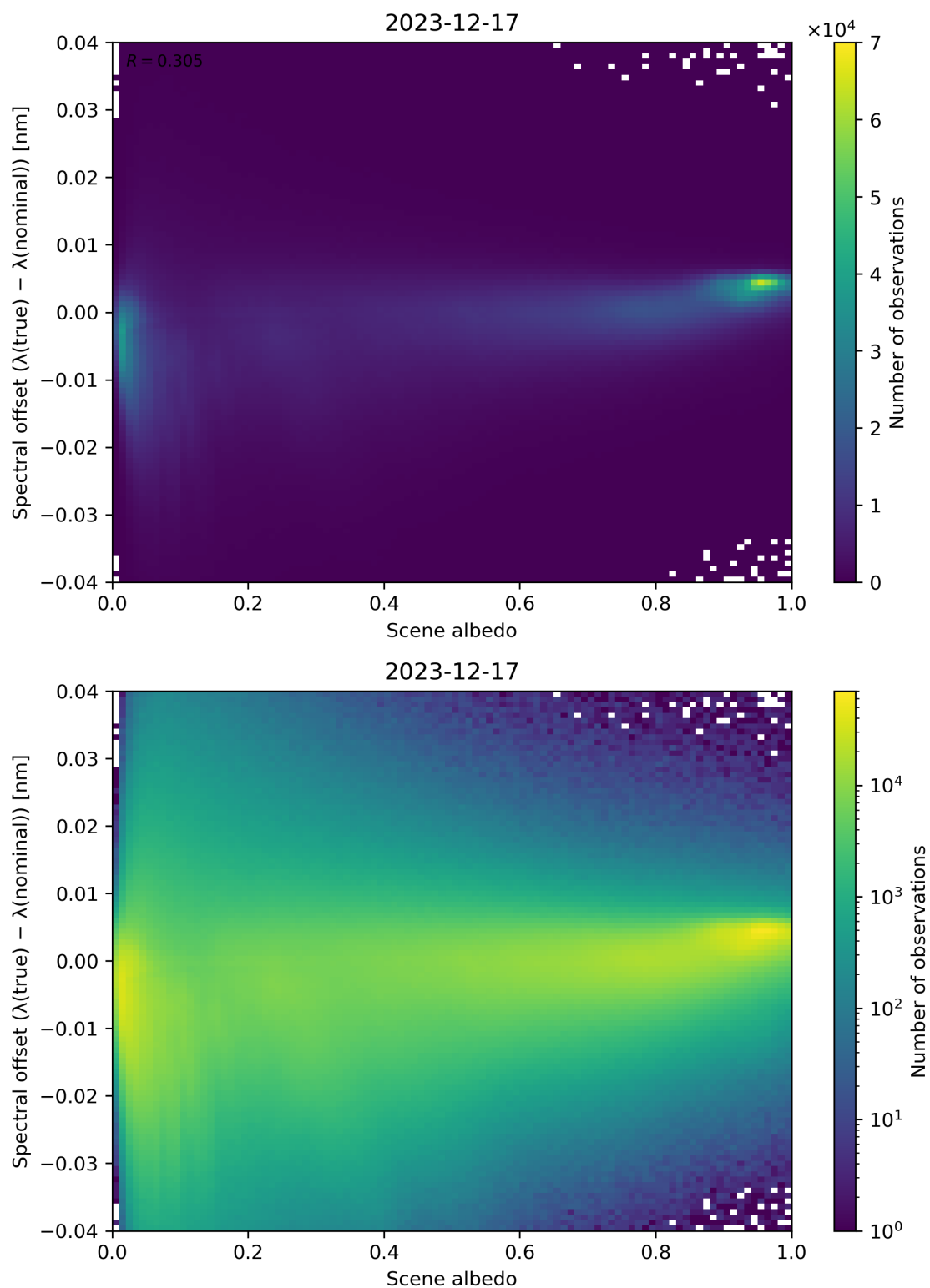
Figure 107: Scatter density plot of “Scene albedo” against “Spectral offset ( \lambda(\text{true}) - \lambda(\text{nominal}) )” for 2023-12-16 to 2023-12-18.
