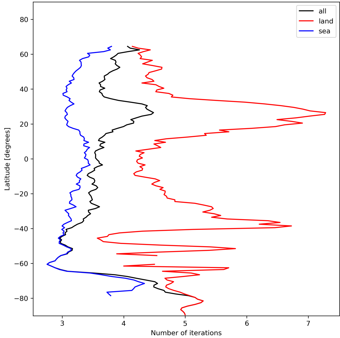
Figure 22: Zonal average of “Number of iterations” for 2023-12-16 to 2023-12-18.
