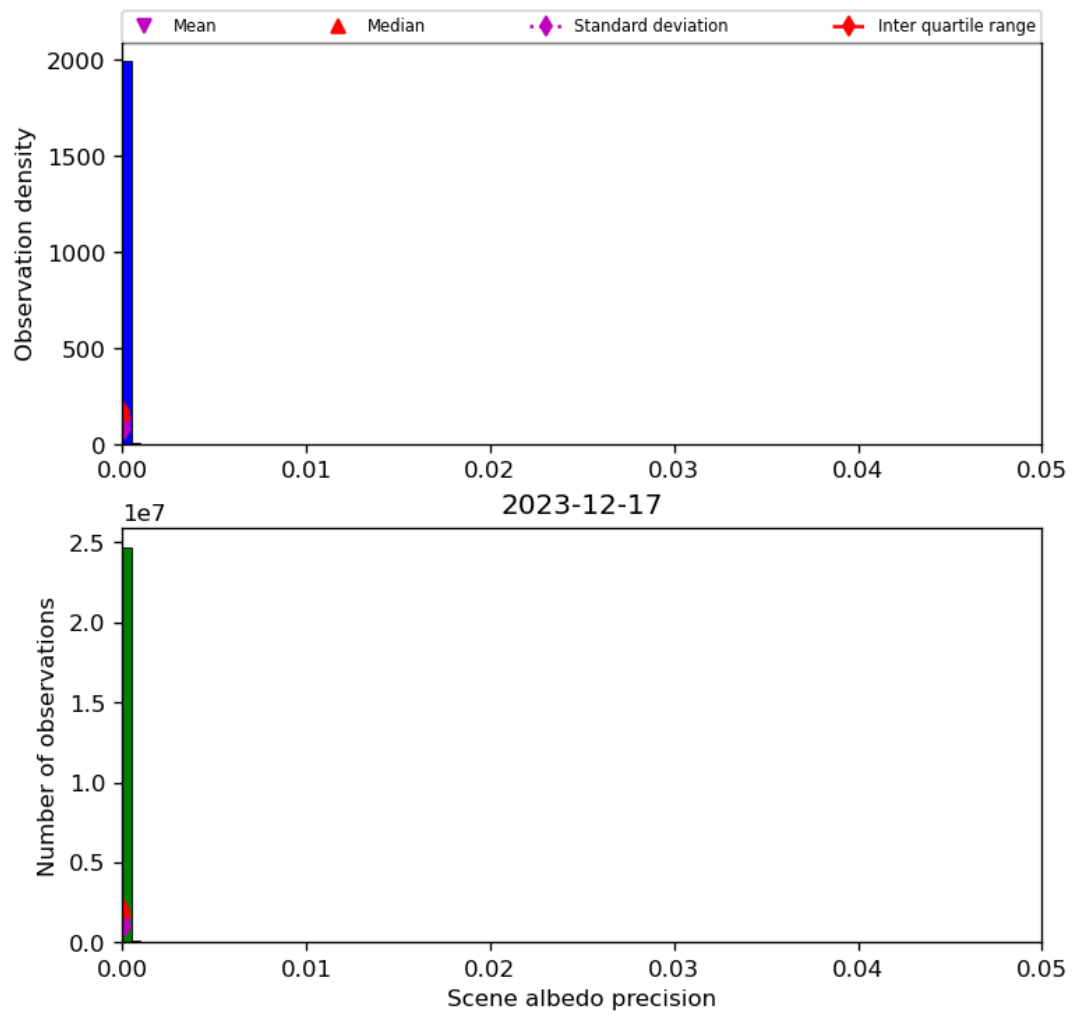
Figure 35: Histogram of “Scene albedo precision” for 2023-12-16 to 2023-12-18
