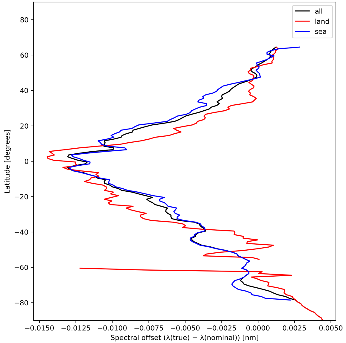
Figure 28: Zonal average of “Spectral offset ( \lambda(\text{true}) - \lambda(\text{nominal}) )” for 2023-12-16 to 2023-12-18.
