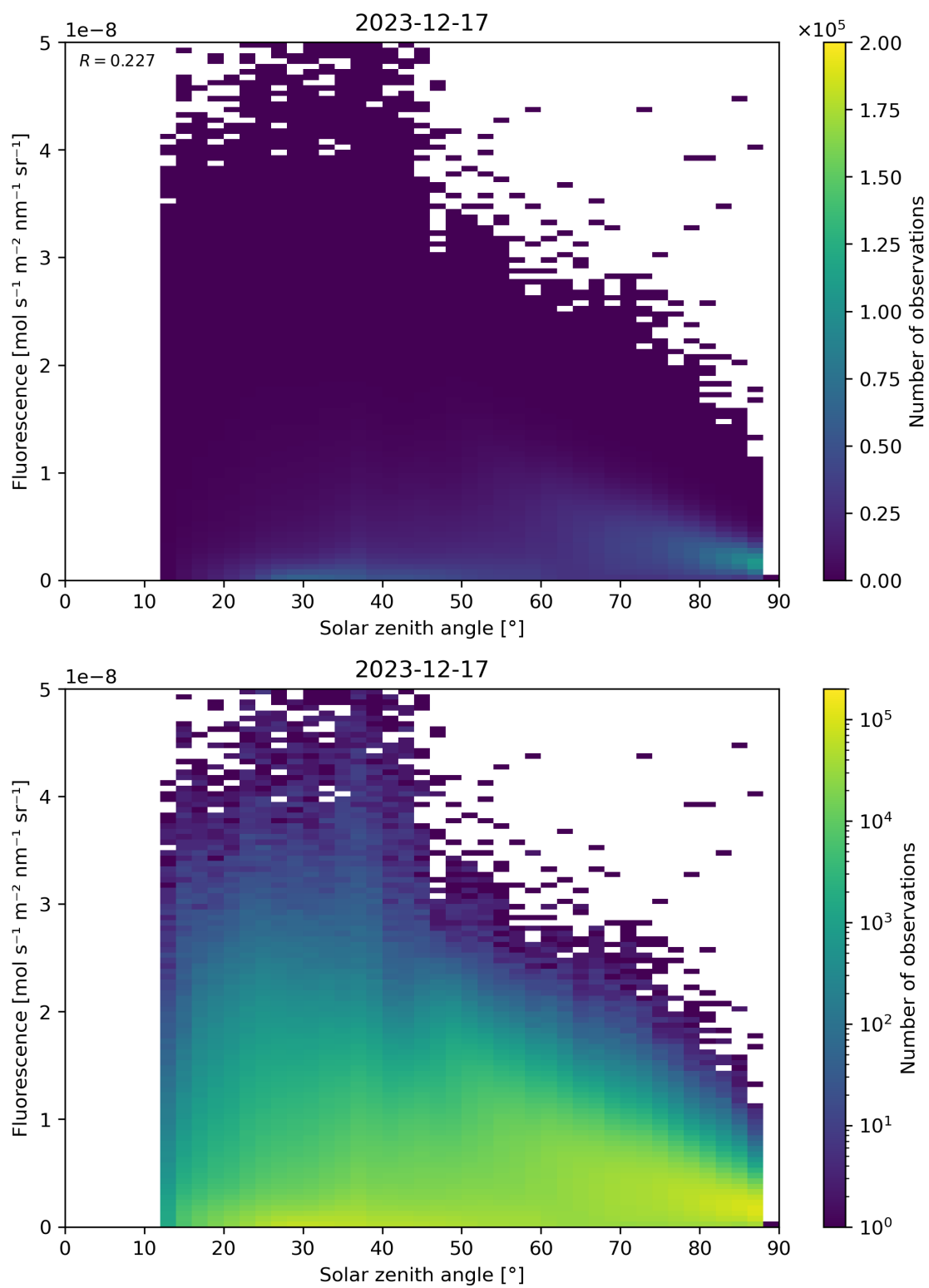
Figure 112: Scatter density plot of “Solar zenith angle” against “Fluorescence” for 2023-12-16 to 2023-12-18.
