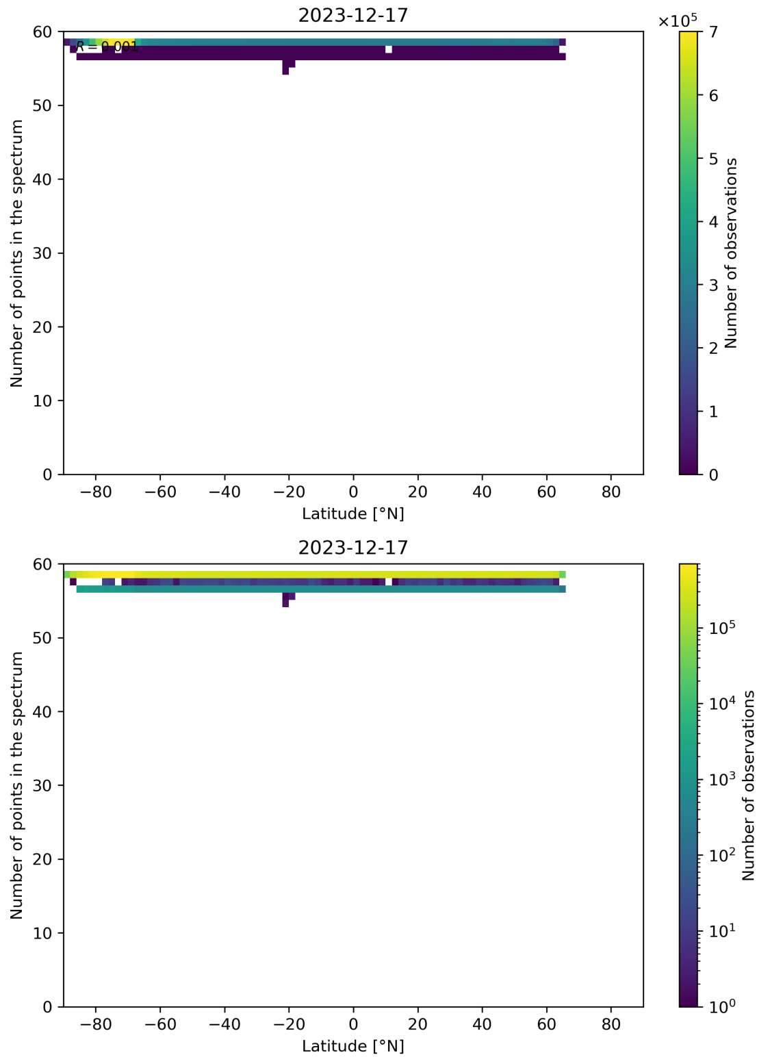
Figure 94: Scatter density plot of “Latitude” against “Number of points in the spectrum” for 2023-12-16 to 2023-12-18.
