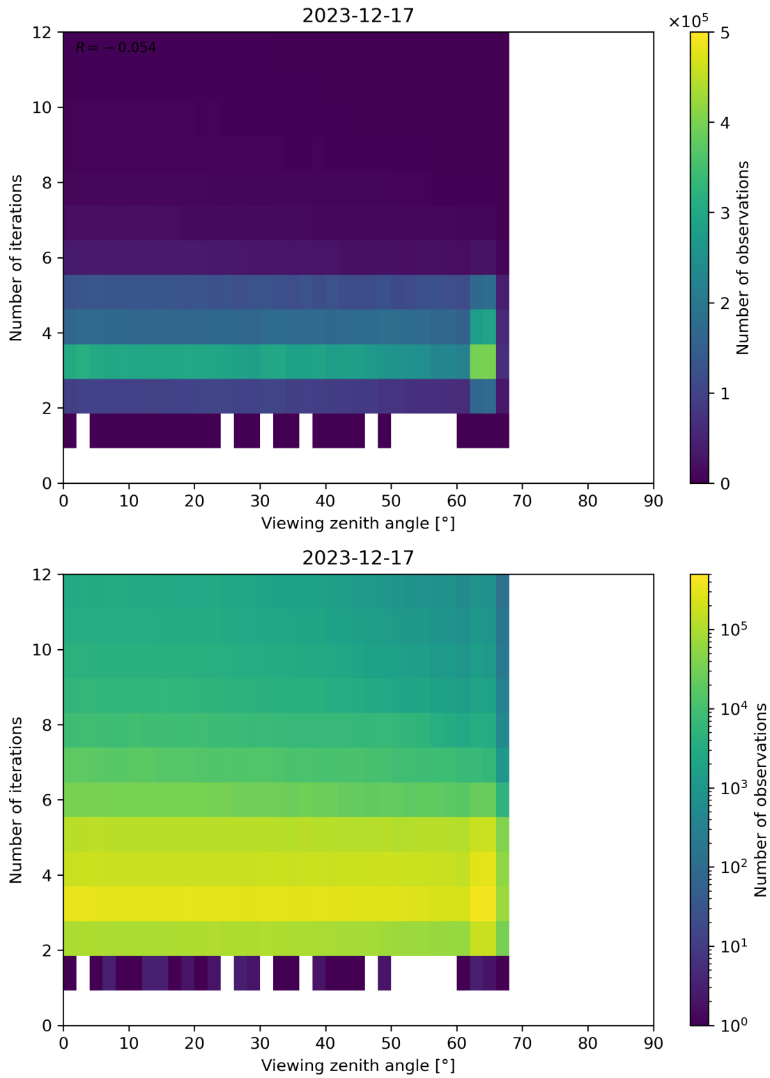
Figure 124: Scatter density plot of “Viewing zenith angle” against “Number of iterations” for 2023-12-16 to 2023-12-18.
