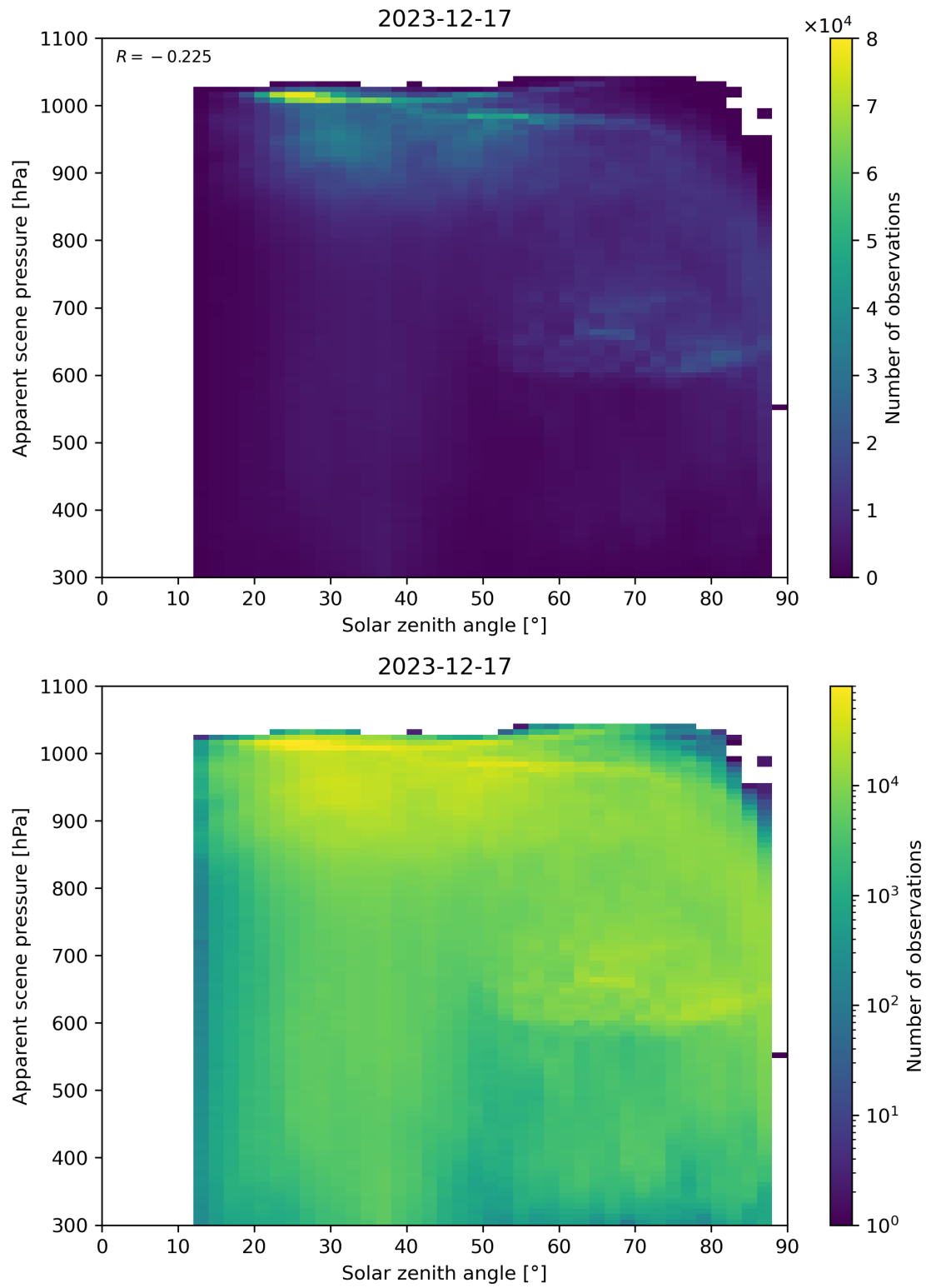
Figure 108: Scatter density plot of “Solar zenith angle” against “Apparent scene pressure” for 2023-12-16 to 2023-12-18.
