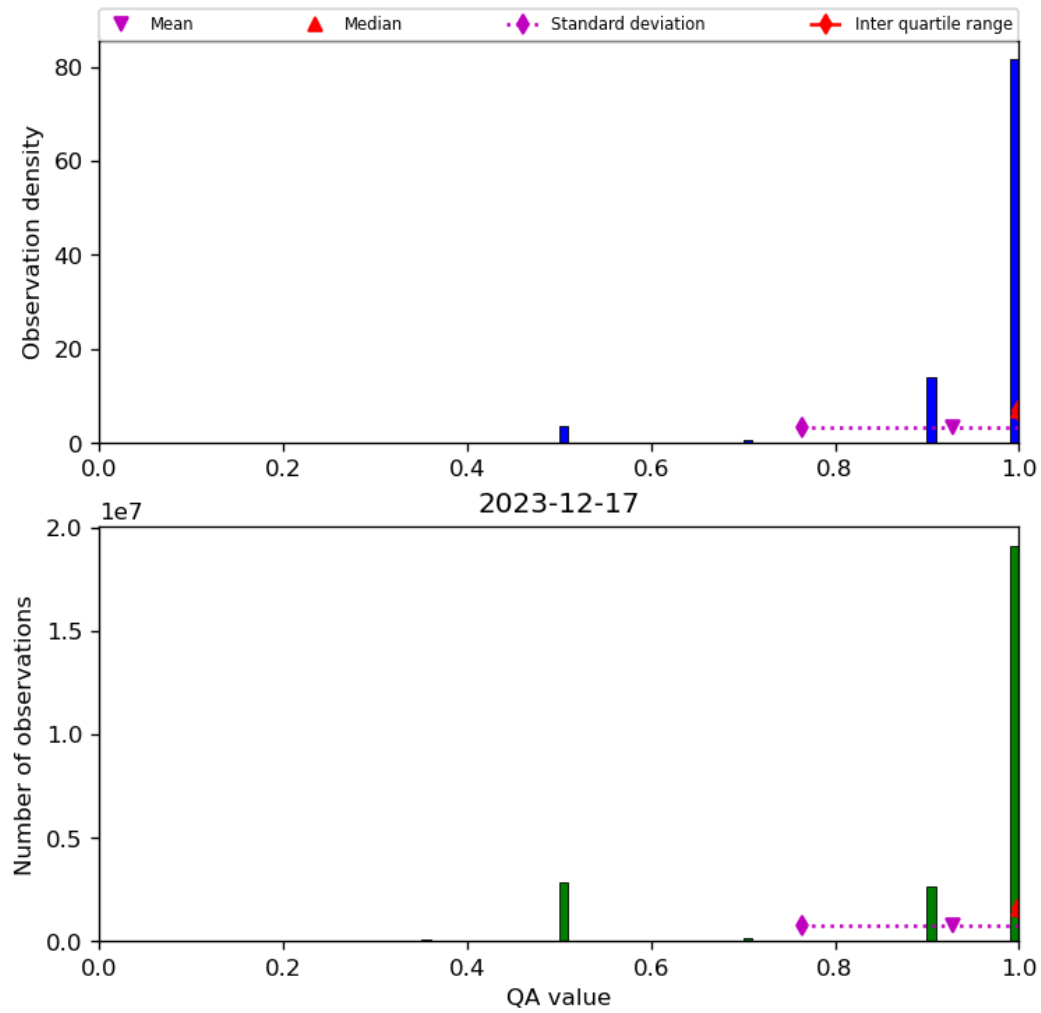
Figure 29: Histogram of “QA value” for 2023-12-16 to 2023-12-18
