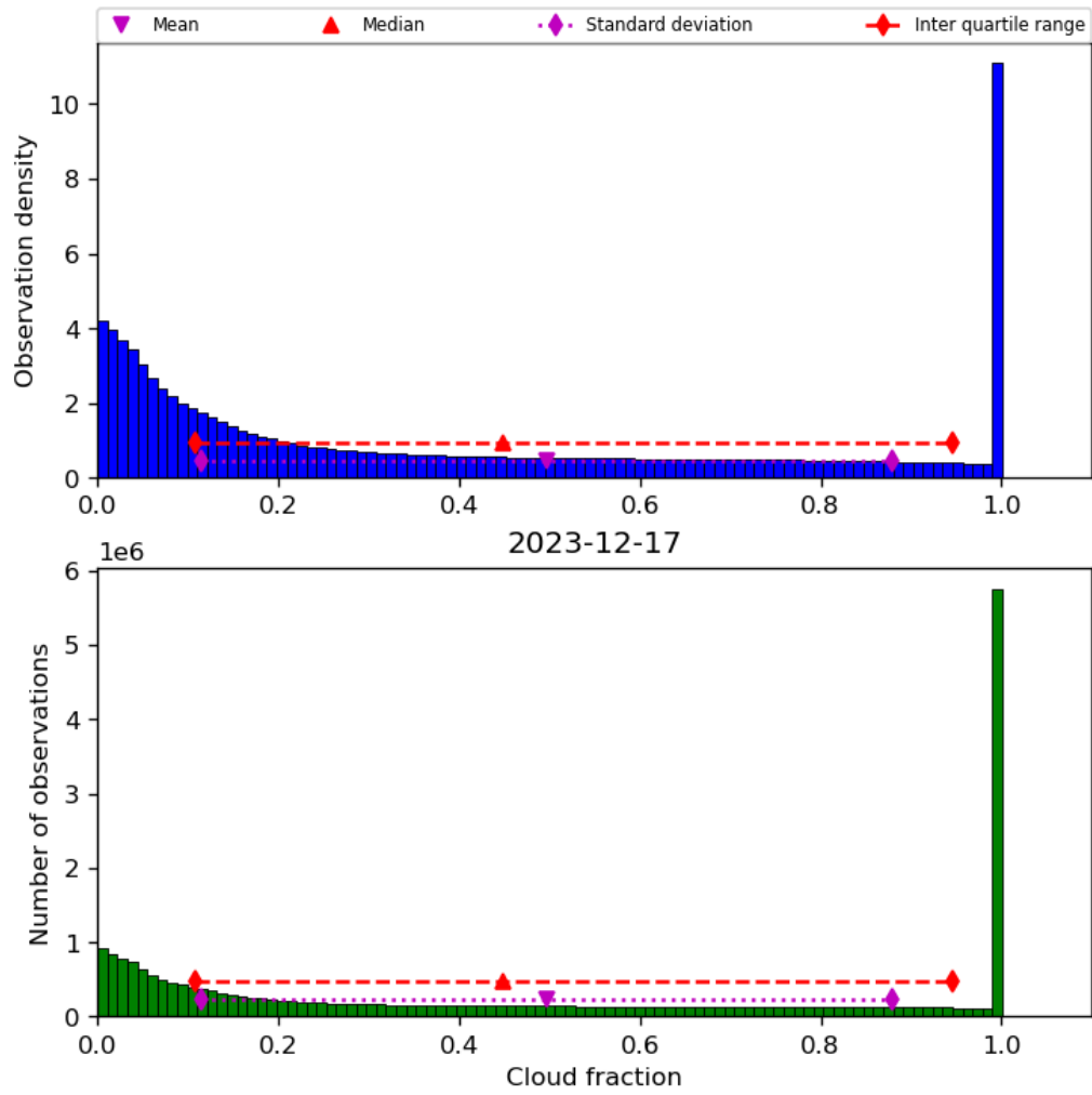
Figure 32: Histogram of “Cloud fraction” for 2023-12-16 to 2023-12-18
