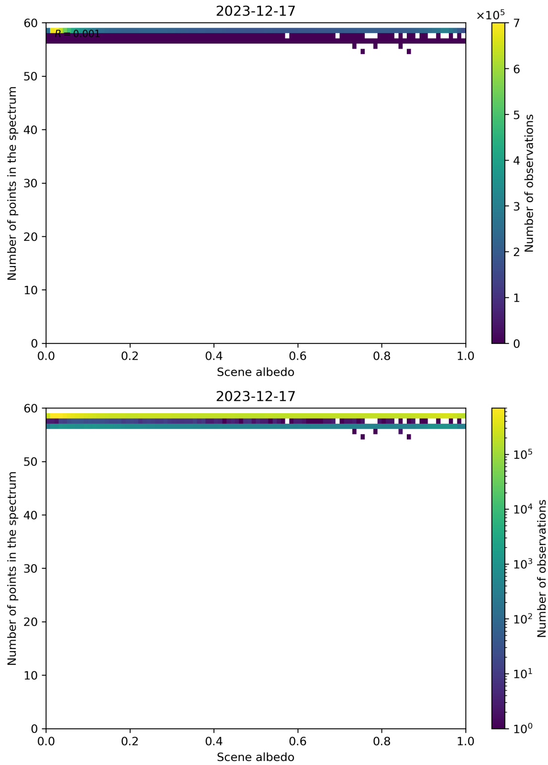
Figure 106: Scatter density plot of “Scene albedo” against “Number of points in the spectrum” for 2023-12-16 to 2023-12-18.
