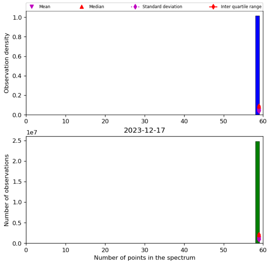
Figure 44: Histogram of “Number of points in the spectrum” for 2023-12-16 to 2023-12-18
