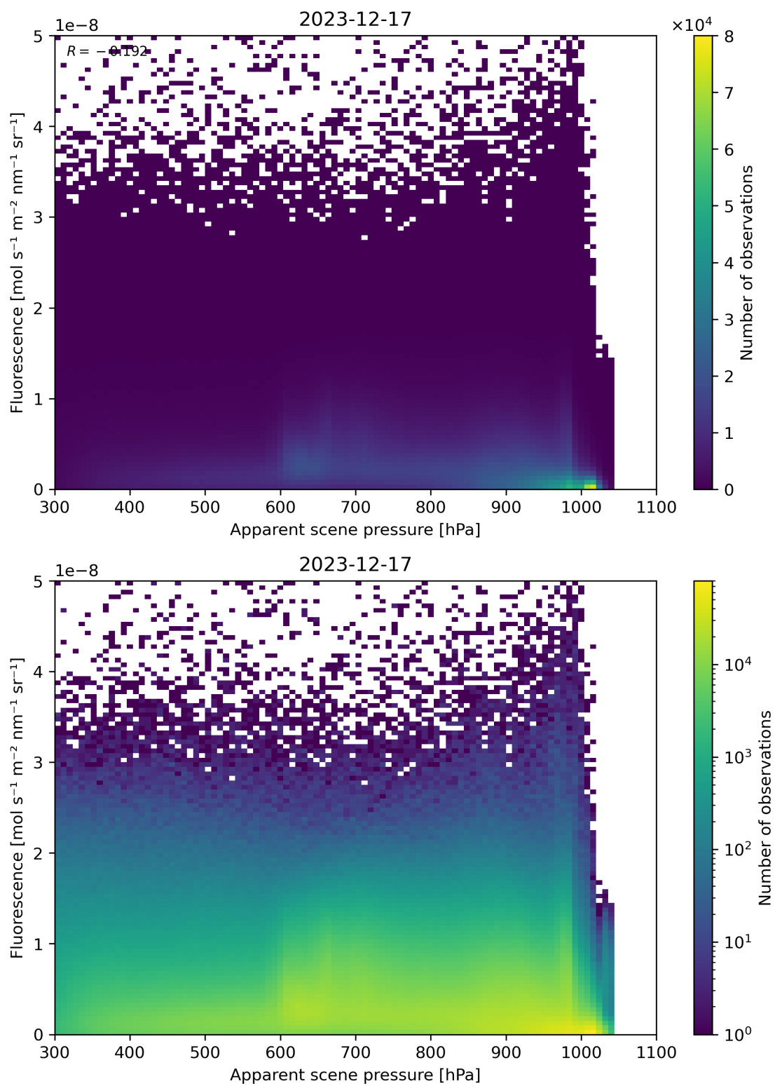
Figure 64: Scatter density plot of “Apparent scene pressure” against “Fluorescence” for 2023-12-16 to 2023-12-18.
