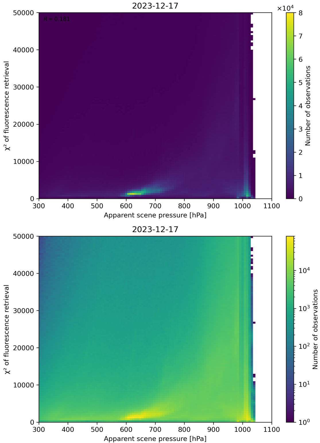
Figure 63: Scatter density plot of “Apparent scene pressure” against “ \chi^2 of fluorescence retrieval” for 2023-12-16 to 2023-12-18.
