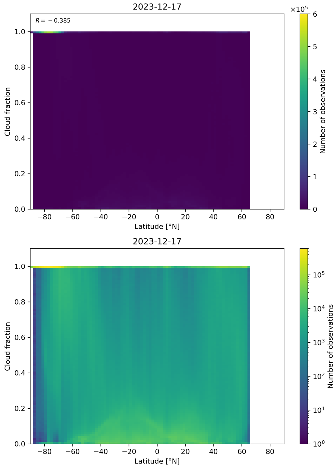
Figure 90: Scatter density plot of “Latitude” against “Cloud fraction” for 2023-12-16 to 2023-12-18.
