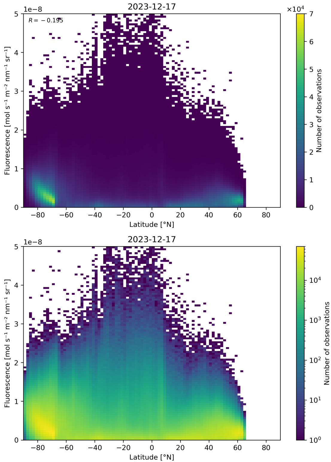
Figure 92: Scatter density plot of “Latitude” against “Fluorescence” for 2023-12-16 to 2023-12-18.
