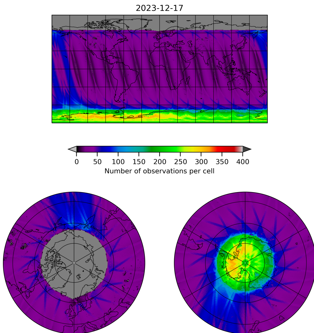
Figure 11: Map of the number of observations for 2023-12-16 to 2023-12-18
