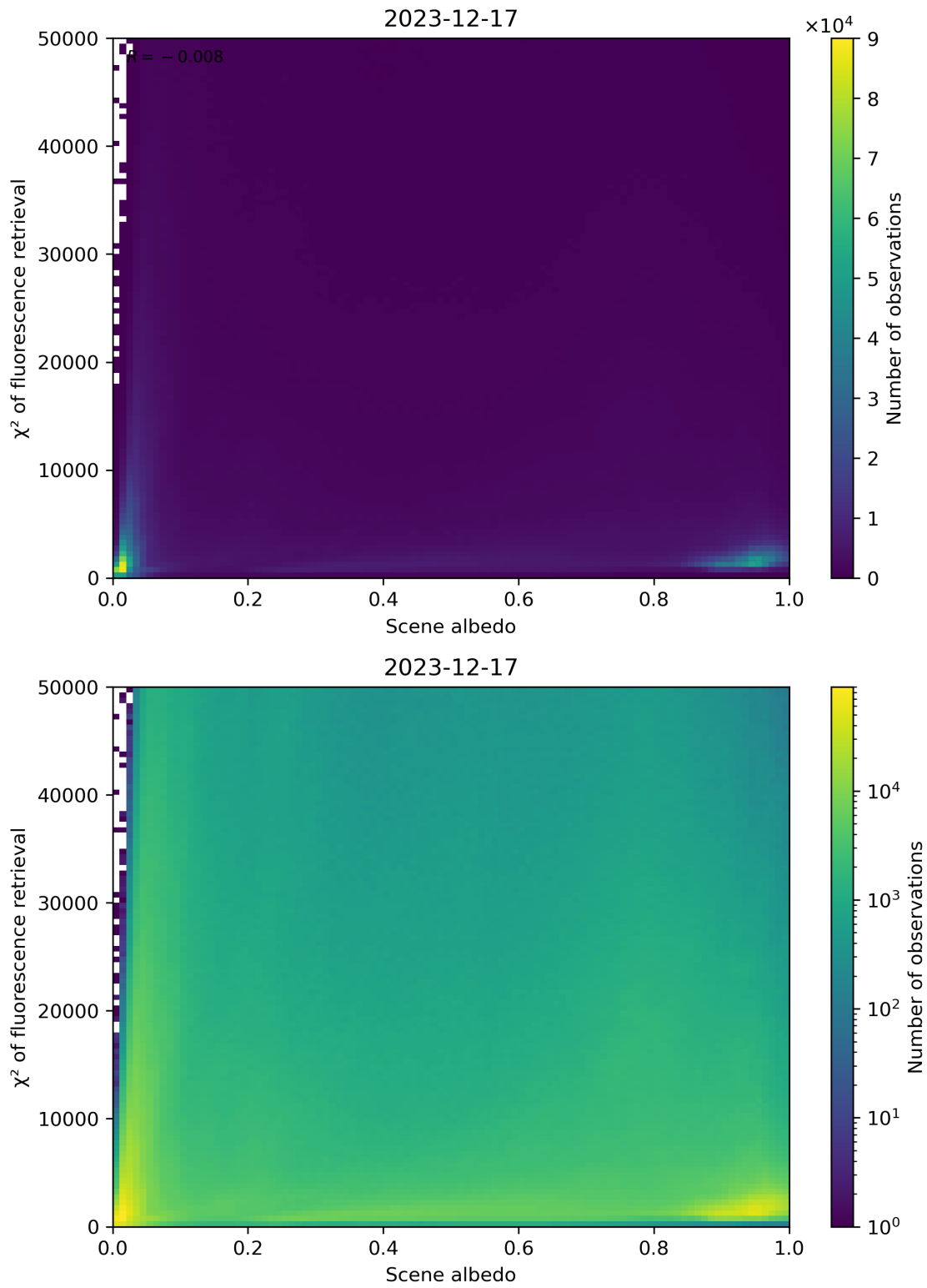
Figure 103: Scatter density plot of “Scene albedo” against “ \chi^2 of fluorescence retrieval” for 2023-12-16 to 2023-12-18.
