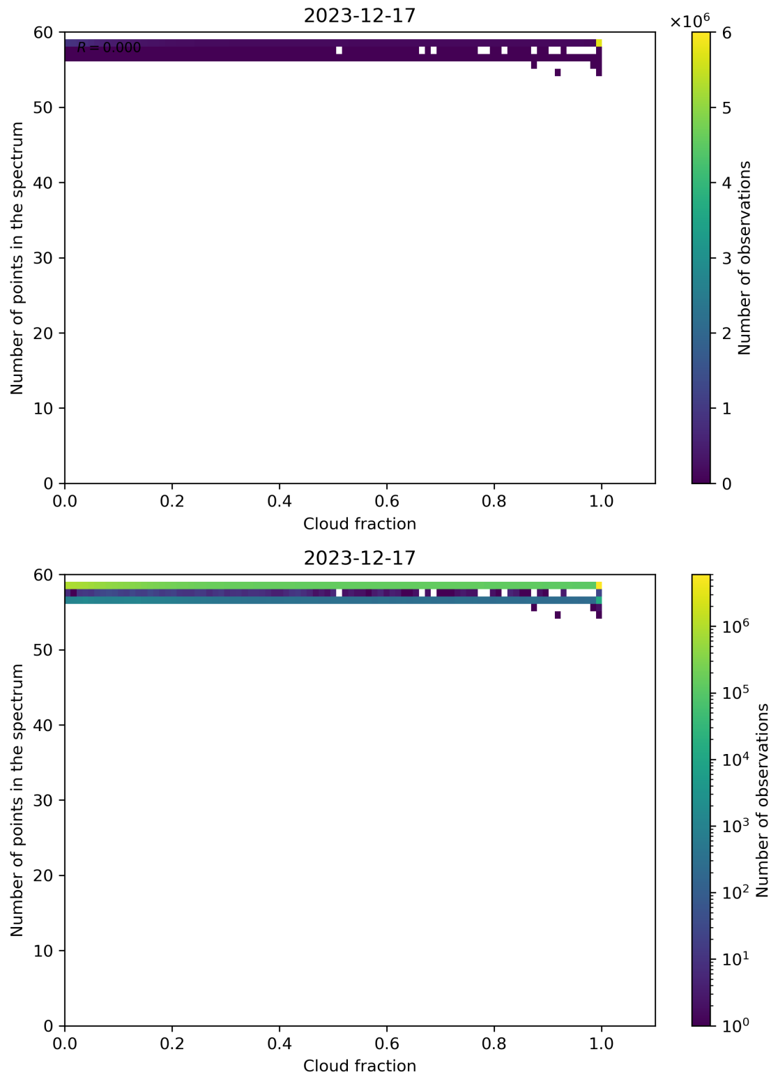
Figure 74: Scatter density plot of “Cloud fraction” against “Number of points in the spectrum” for 2023-12-16 to 2023-12-18.
