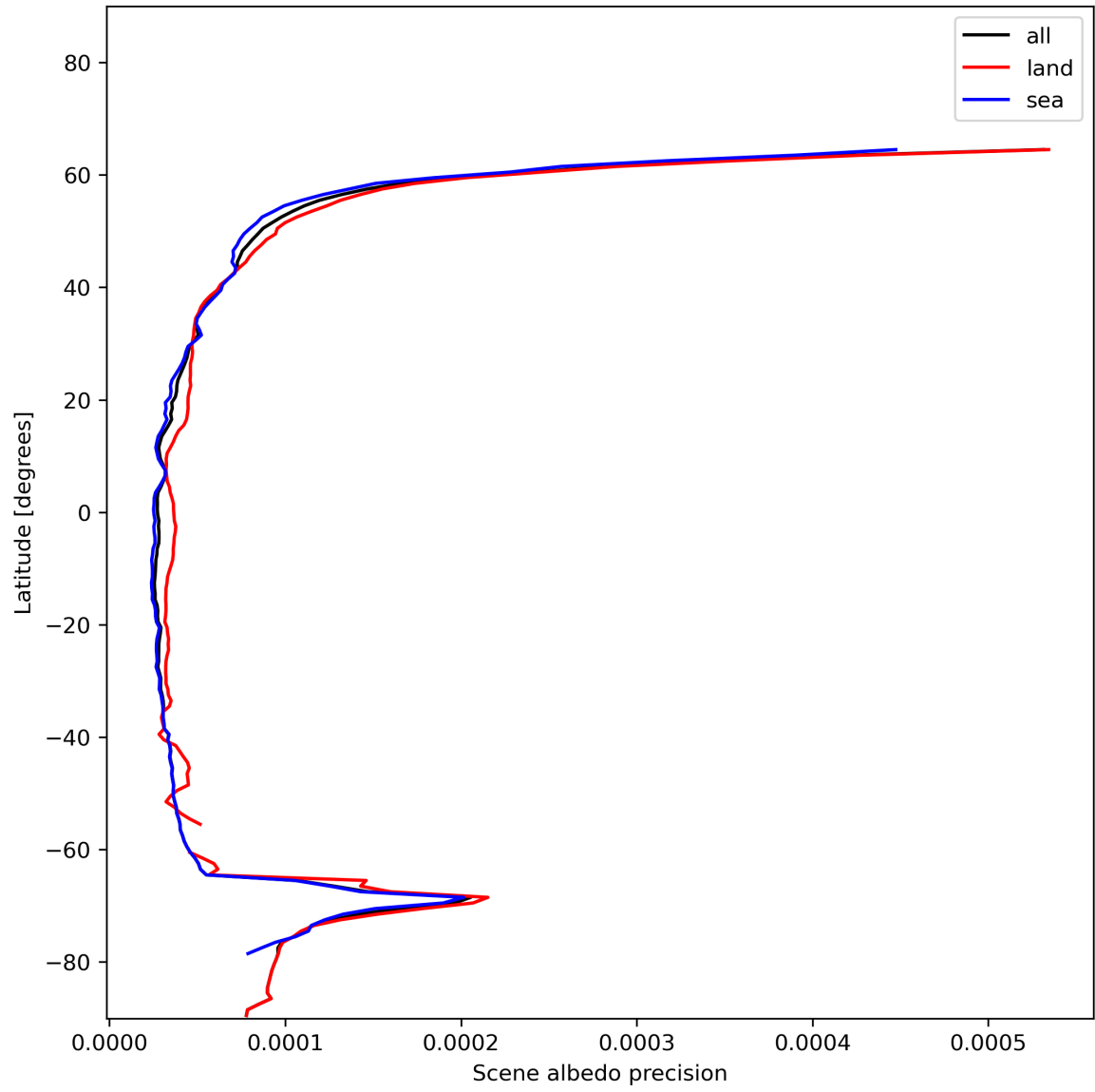
Figure 18: Zonal average of “Scene albedo precision” for 2023-12-16 to 2023-12-18.
