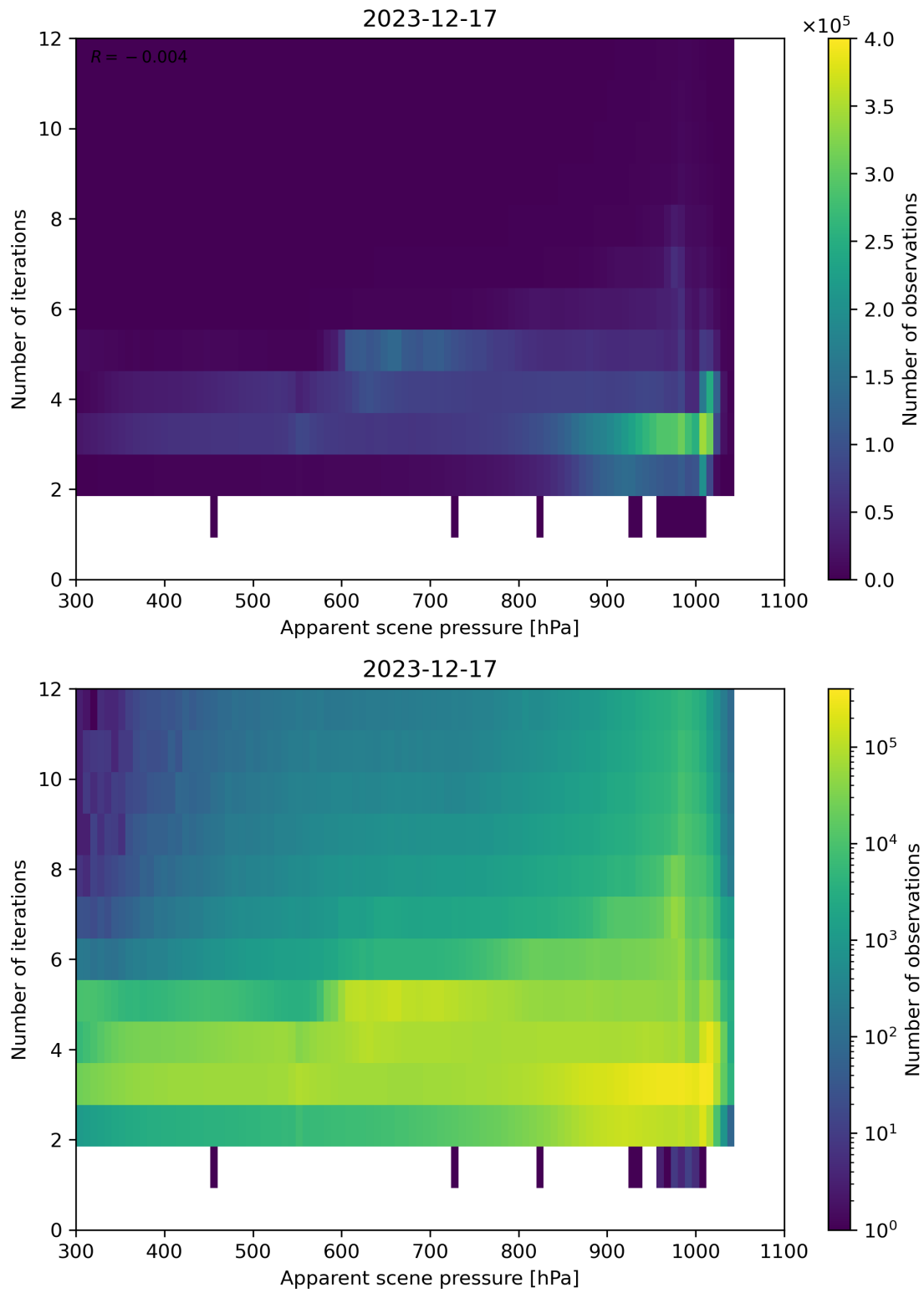
Figure 65: Scatter density plot of “Apparent scene pressure” against “Number of iterations” for 2023-12-16 to 2023-12-18.
