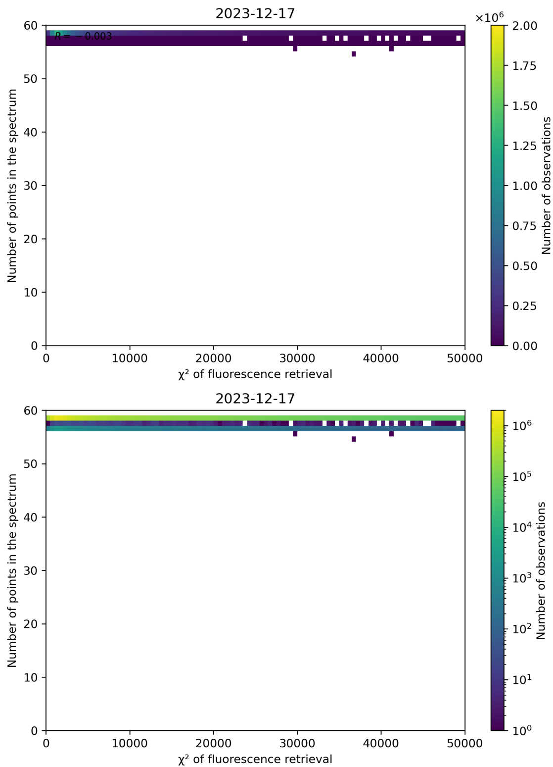
Figure 68: Scatter density plot of " \chi^2 of fluorescence retrieval" against "Number of points in the spectrum" for 2023-12-16 to 2023-12-18.
