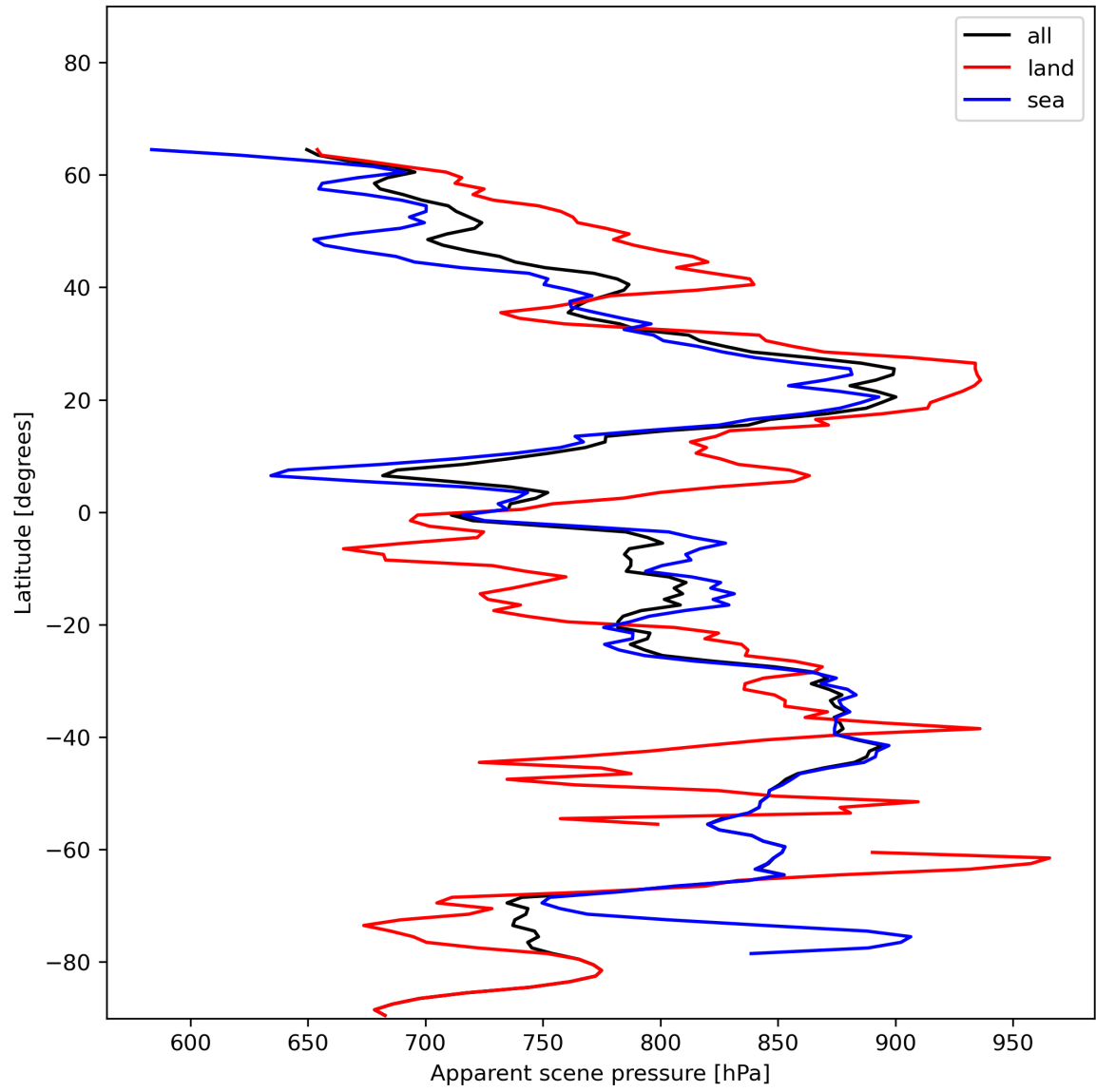
Figure 19: Zonal average of “Apparent scene pressure” for 2023-12-16 to 2023-12-18.
