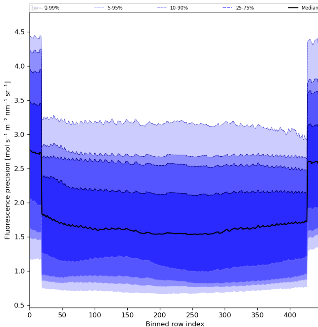
Figure 58: Along track statistics of “Fluorescence precision” for 2023-12-16 to 2023-12-18
