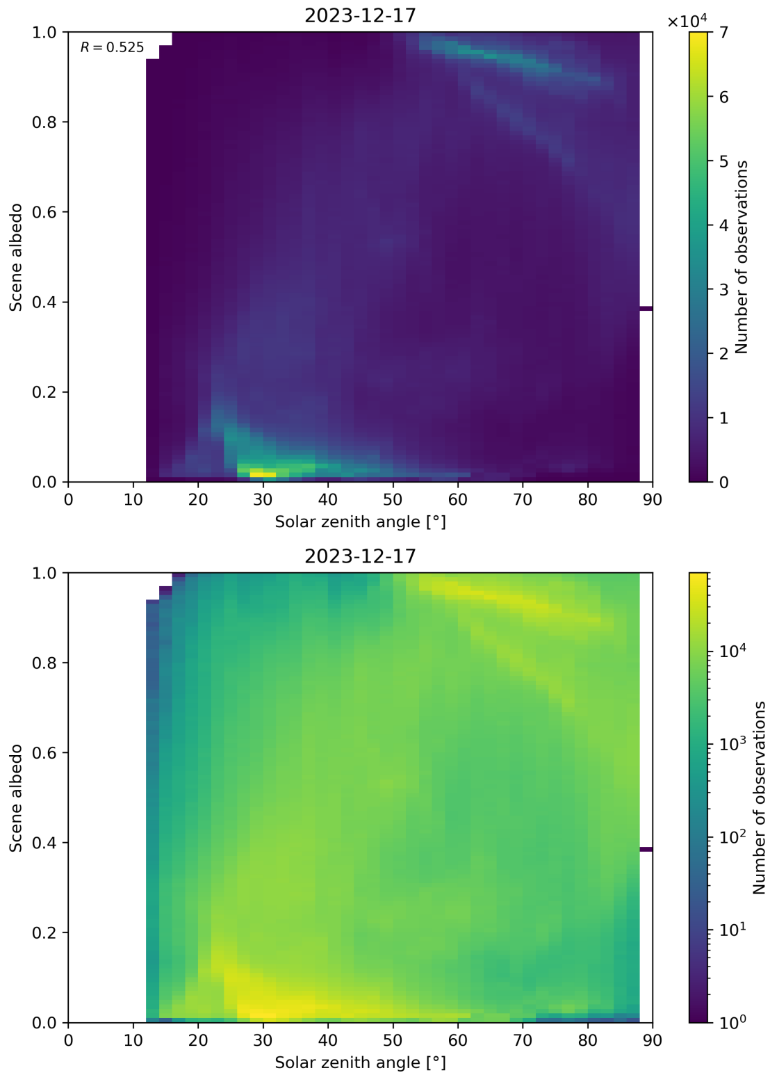
Figure 116: Scatter density plot of “Solar zenith angle” against “Scene albedo” for 2023-12-16 to 2023-12-18.
