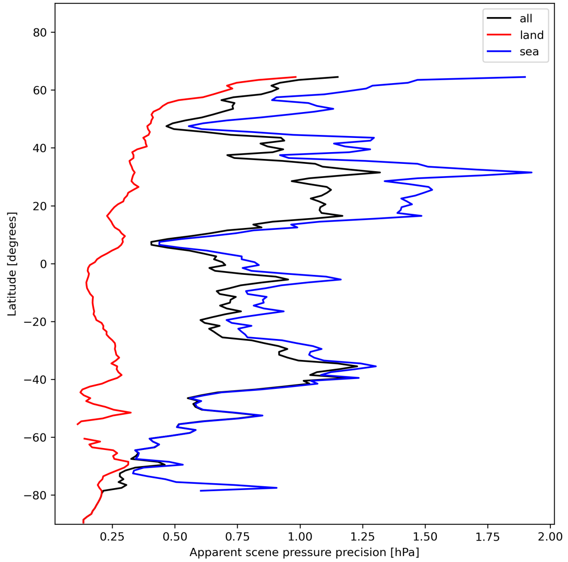
Figure 20: Zonal average of “Apparent scene pressure precision” for 2023-12-16 to 2023-12-18.
