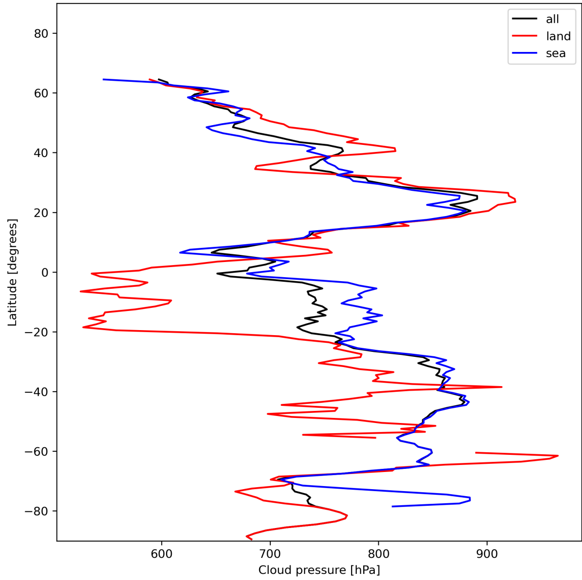
Figure 13: Zonal average of “Cloud pressure” for 2023-12-16 to 2023-12-18.
