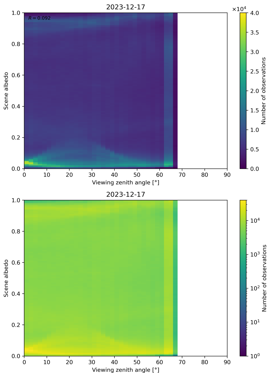
Figure 126: Scatter density plot of “Viewing zenith angle” against “Scene albedo” for 2023-12-16 to 2023-12-18.
