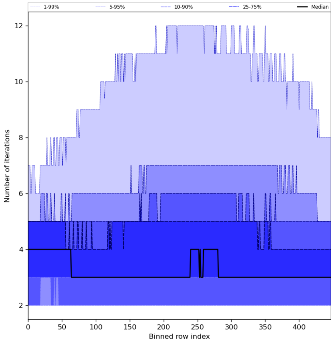
Figure 56: Along track statistics of “Number of iterations” for 2023-12-16 to 2023-12-18
