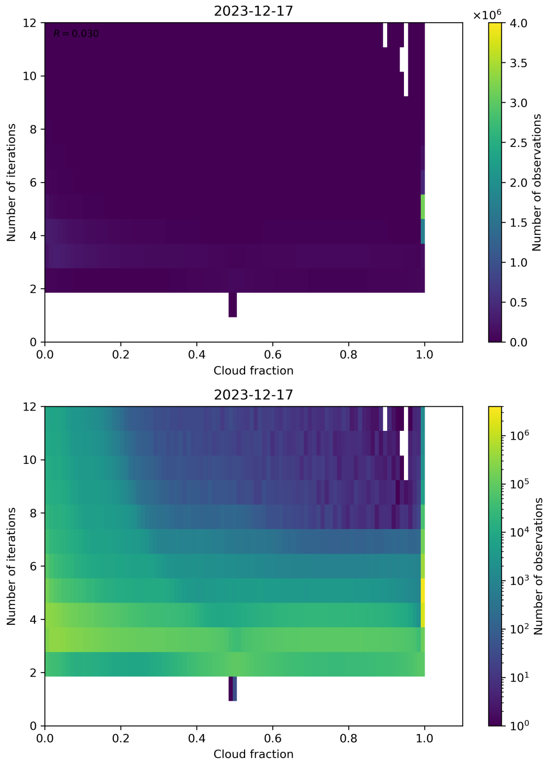
Figure 73: Scatter density plot of “Cloud fraction” against “Number of iterations” for 2023-12-16 to 2023-12-18.
