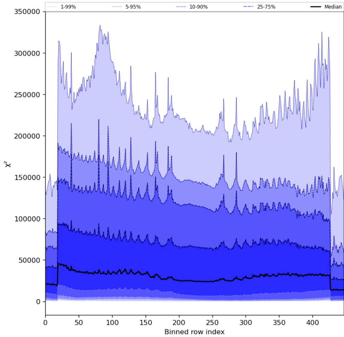
Figure 55: Along track statistics of “ \chi^2 ” for 2023-12-16 to 2023-12-18
