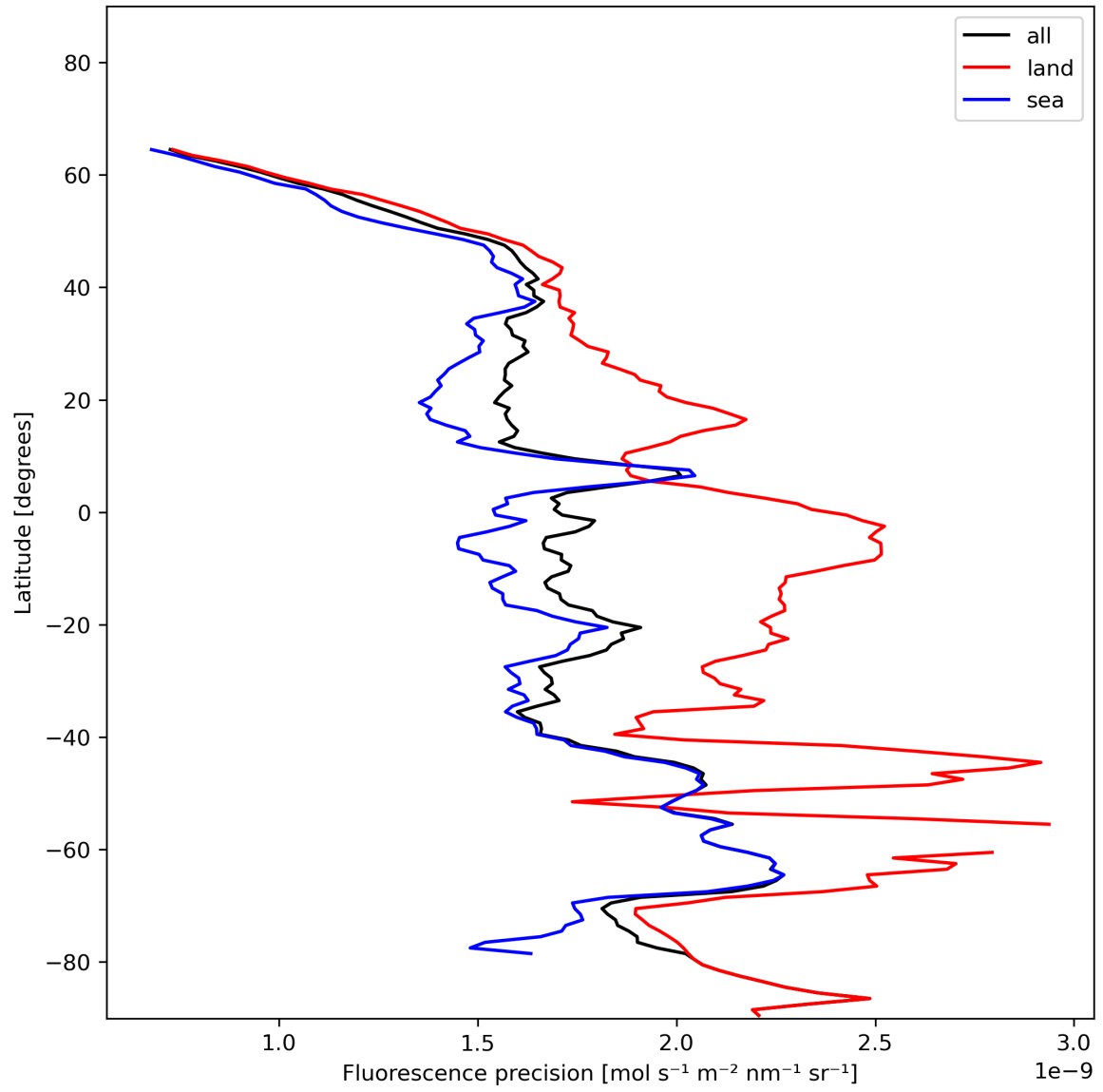
Figure 24: Zonal average of “Fluorescence precision” for 2023-12-16 to 2023-12-18.
