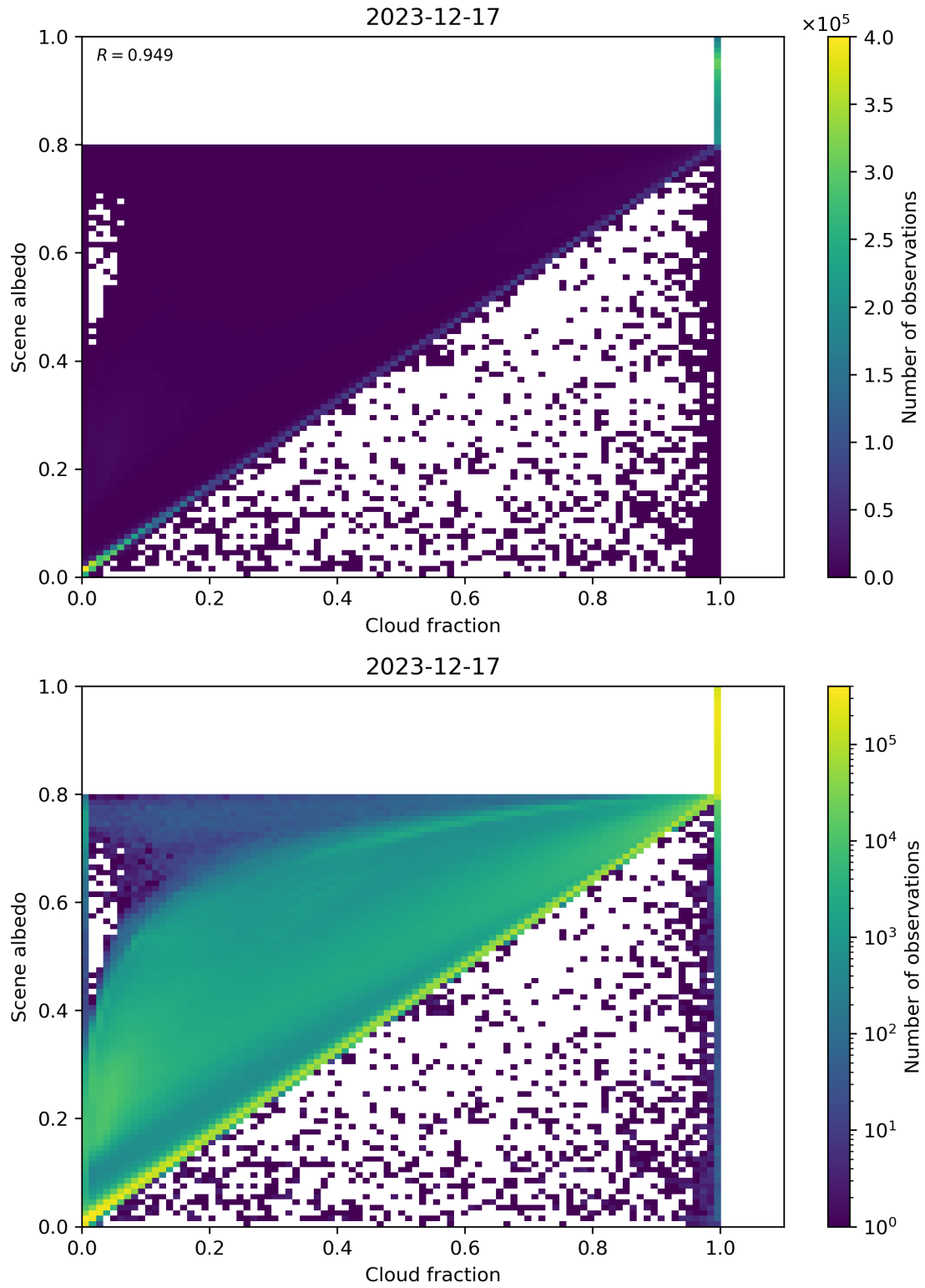
Figure 75: Scatter density plot of “Cloud fraction” against “Scene albedo” for 2023-12-16 to 2023-12-18.
