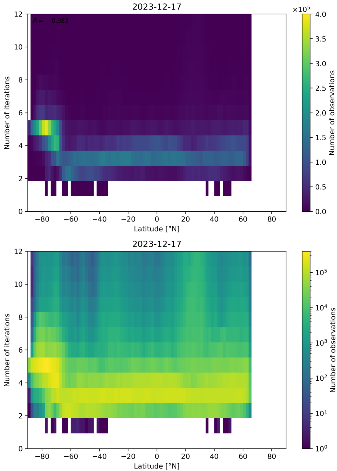
Figure 93: Scatter density plot of “Latitude” against “Number of iterations” for 2023-12-16 to 2023-12-18.
