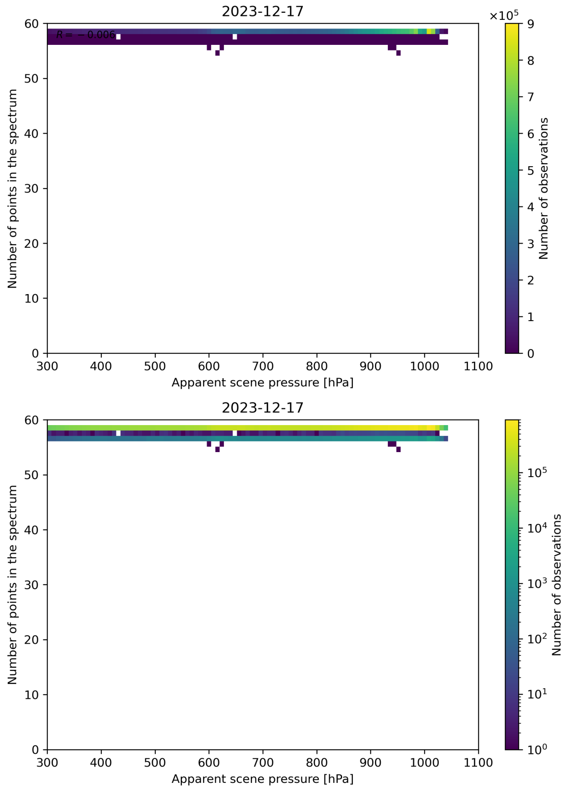
Figure 66: Scatter density plot of “Apparent scene pressure” against “Number of points in the spectrum” for 2023-12-16 to 2023-12-18.
