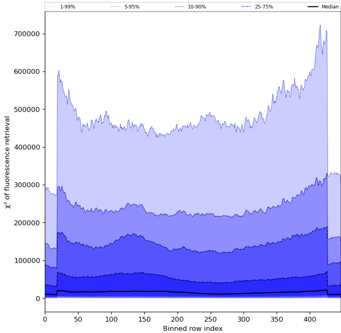
Figure 59: Along track statistics of “ \chi^2 of fluorescence retrieval” for 2023-12-16 to 2023-12-18
