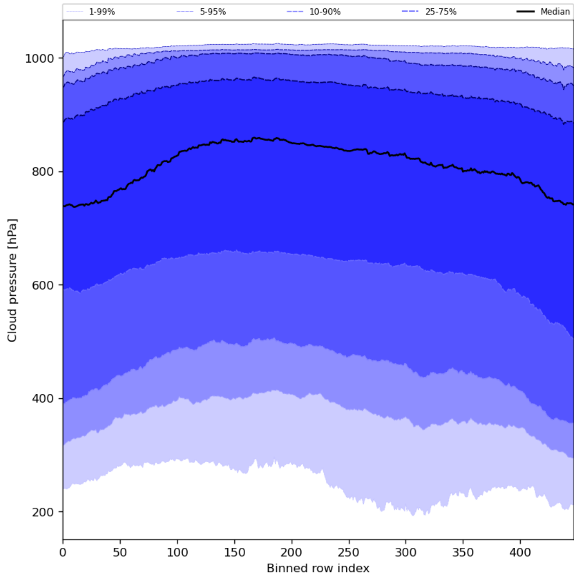
Figure 47: Along track statistics of “Cloud pressure” for 2023-12-16 to 2023-12-18
