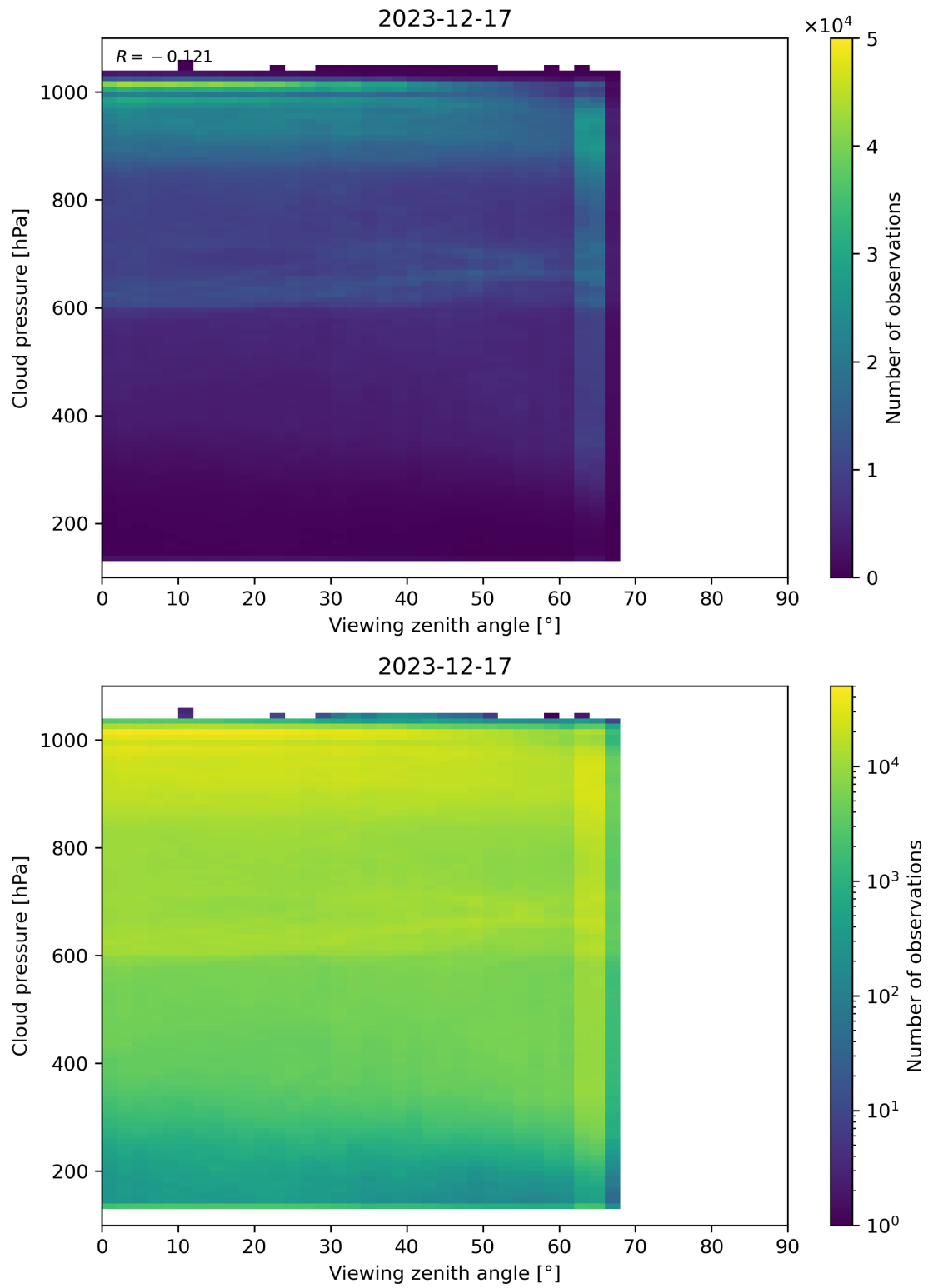
Figure 121: Scatter density plot of “Viewing zenith angle” against “Cloud pressure” for 2023-12-16 to 2023-12-18.
