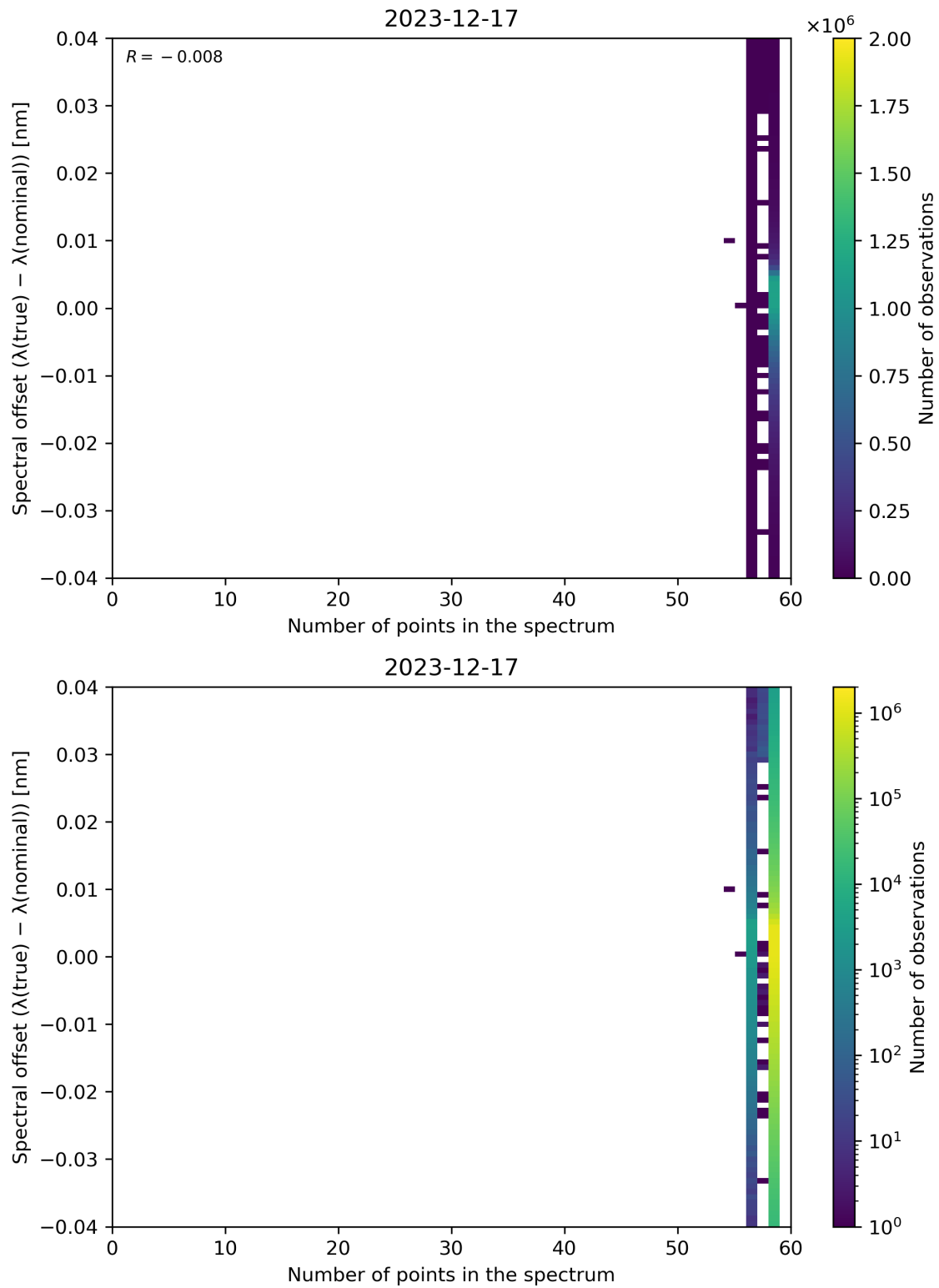
Figure 101: Scatter density plot of “Number of points in the spectrum” against “Spectral offset ( \lambda(\text{true}) - \lambda(\text{nominal}) )” for 2023-12-16 to 2023-12-18.
