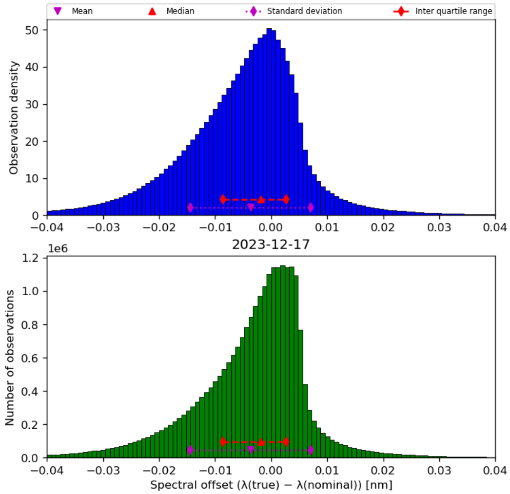
Figure 45: Histogram of “Spectral offset ( \lambda(\text{true}) - \lambda(\text{nominal}) )” for 2023-12-16 to 2023-12-18
