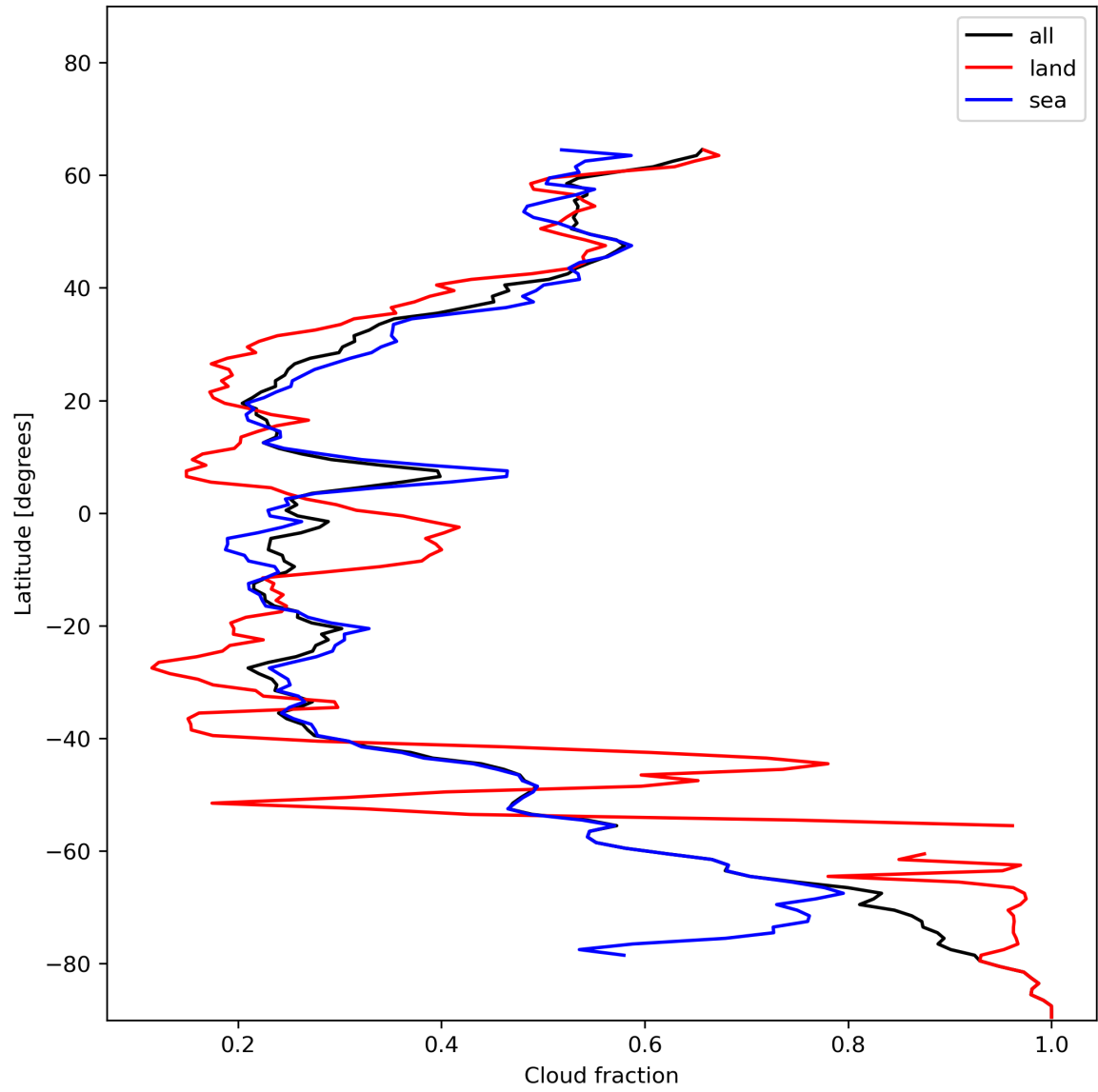
Figure 15: Zonal average of “Cloud fraction” for 2023-12-16 to 2023-12-18.
