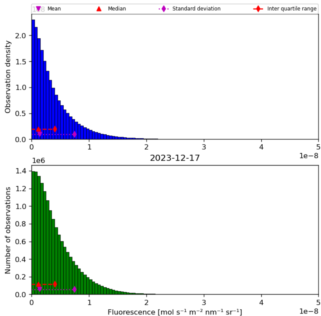
Figure 40: Histogram of “Fluorescence” for 2023-12-16 to 2023-12-18
