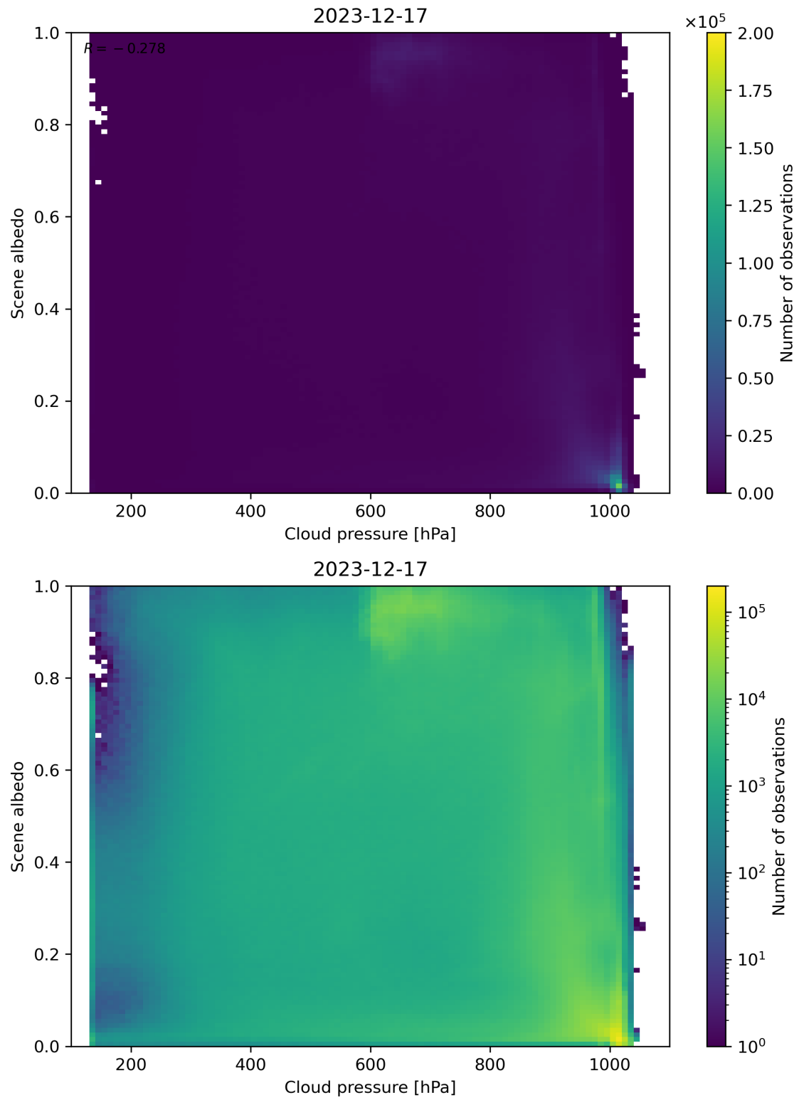
Figure 83: Scatter density plot of “Cloud pressure” against “Scene albedo” for 2023-12-16 to 2023-12-18.
