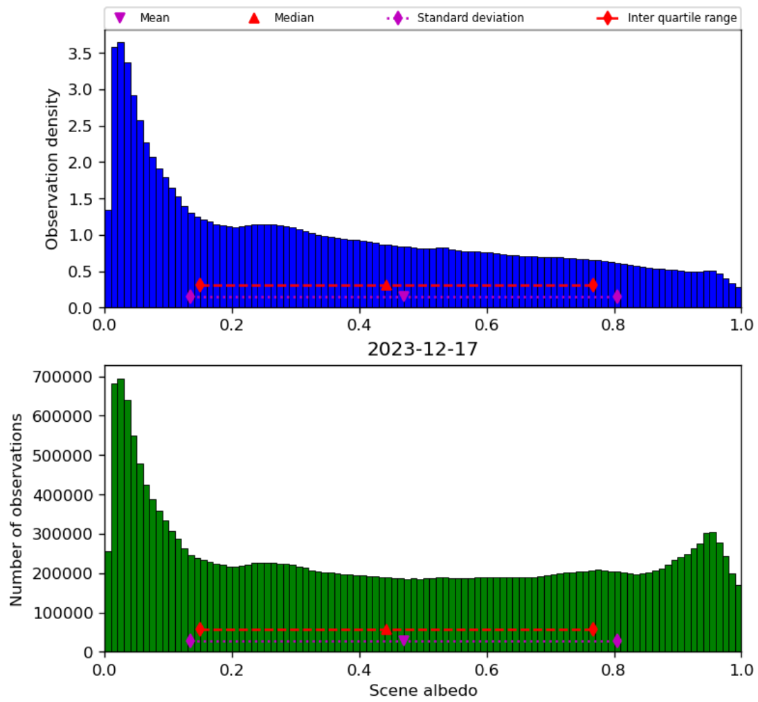
Figure 34: Histogram of “Scene albedo” for 2023-12-16 to 2023-12-18
