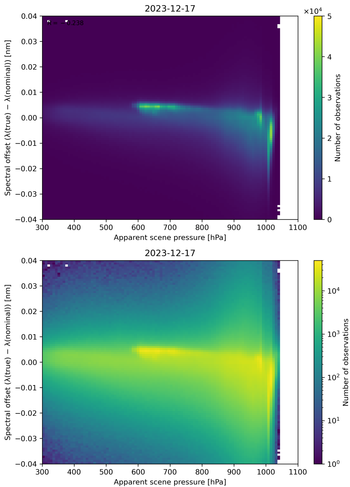
Figure 67: Scatter density plot of “Apparent scene pressure” against “Spectral offset ( \lambda(\text{true}) - \lambda(\text{nominal}) )” for 2023-12-16 to 2023-12-18.
