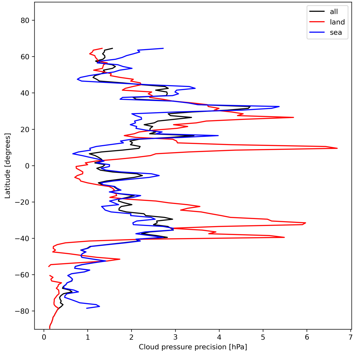
Figure 14: Zonal average of “Cloud pressure precision” for 2023-12-16 to 2023-12-18.
