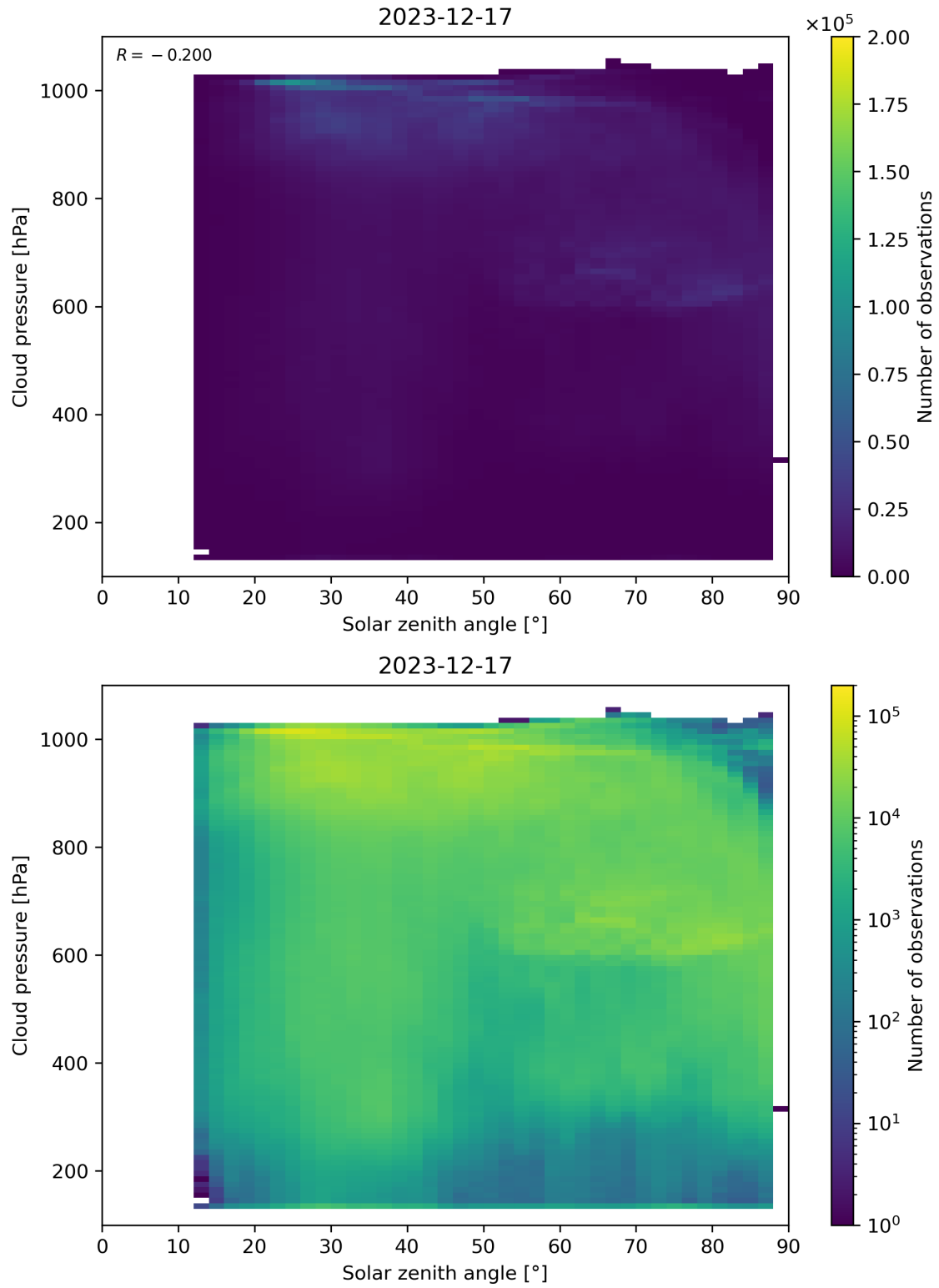
Figure 111: Scatter density plot of “Solar zenith angle” against “Cloud pressure” for 2023-12-16 to 2023-12-18.
