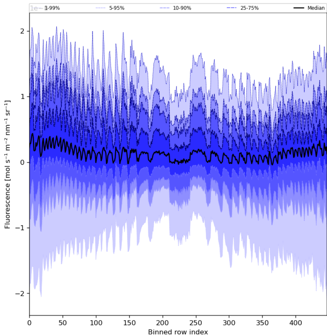
Figure 57: Along track statistics of “Fluorescence” for 2023-12-16 to 2023-12-18
