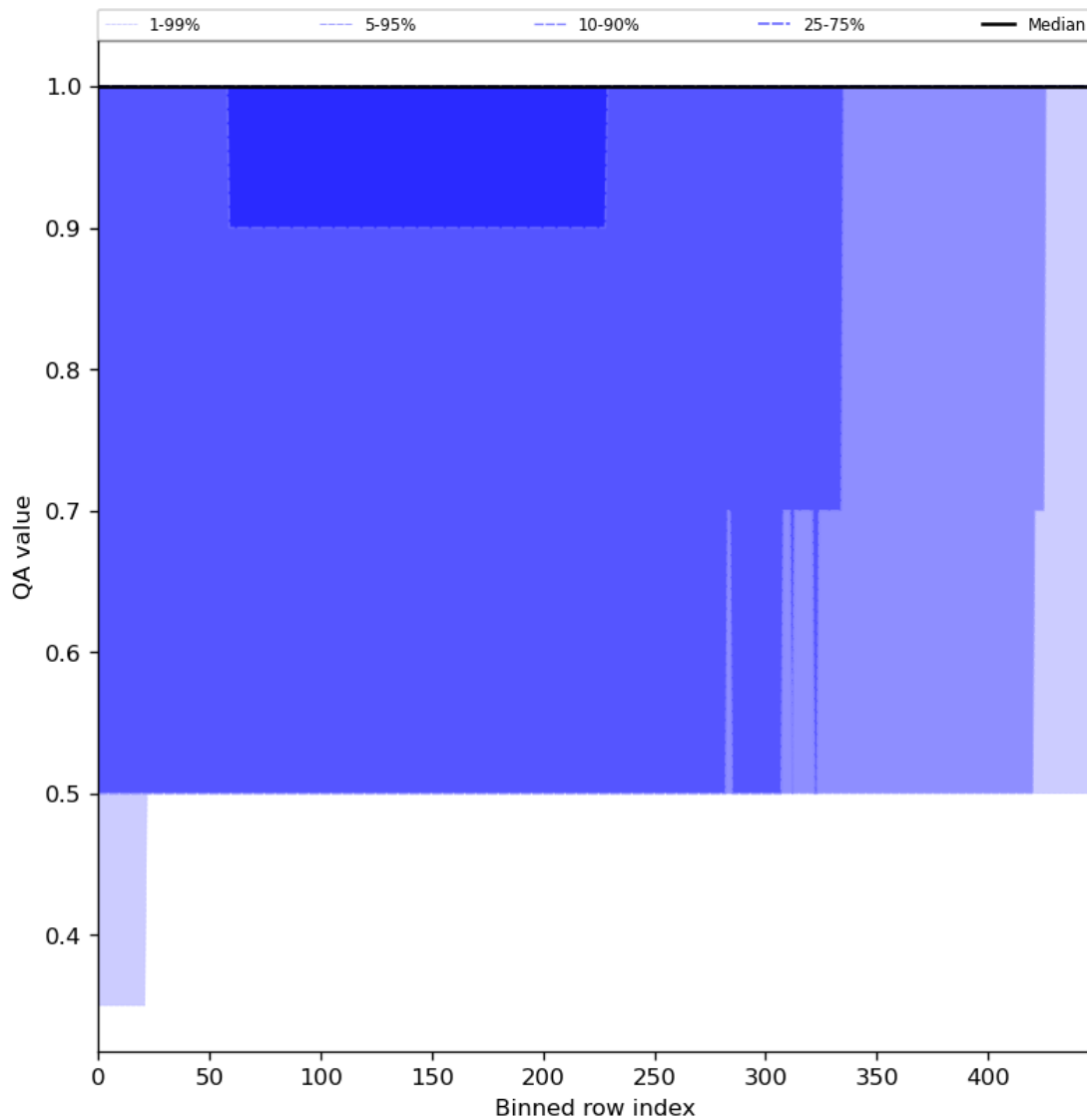
Figure 46: Along track statistics of “QA value” for 2023-12-16 to 2023-12-18
