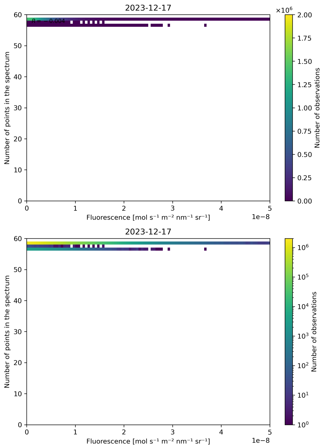
Figure 86: Scatter density plot of “Fluorescence” against “Number of points in the spectrum” for 2023-12-16 to 2023-12-18.
