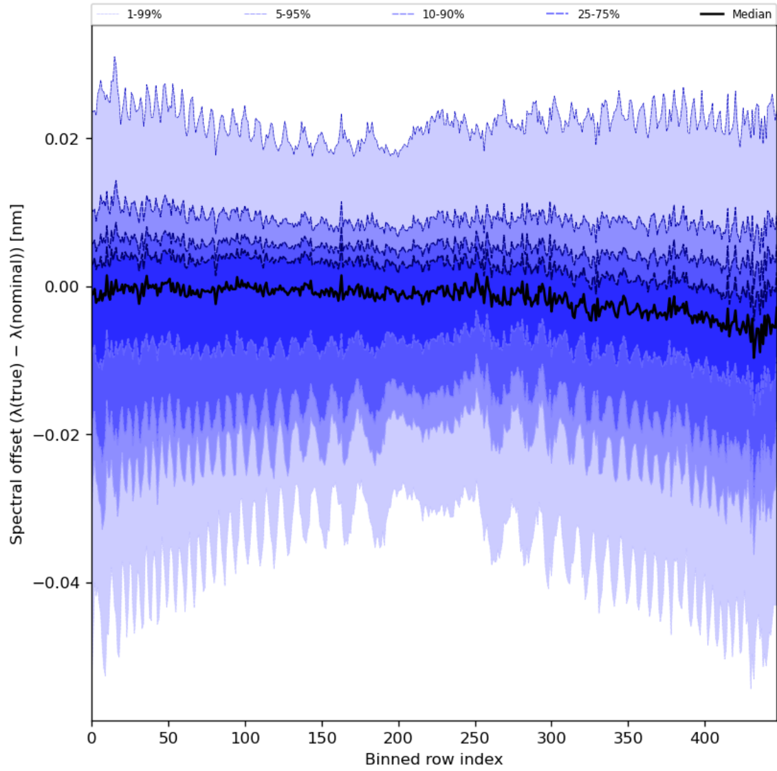
Figure 62: Along track statistics of “Spectral offset ( \lambda(\text{true}) - \lambda(\text{nominal}) )” for 2023-12-16 to 2023-12-18
