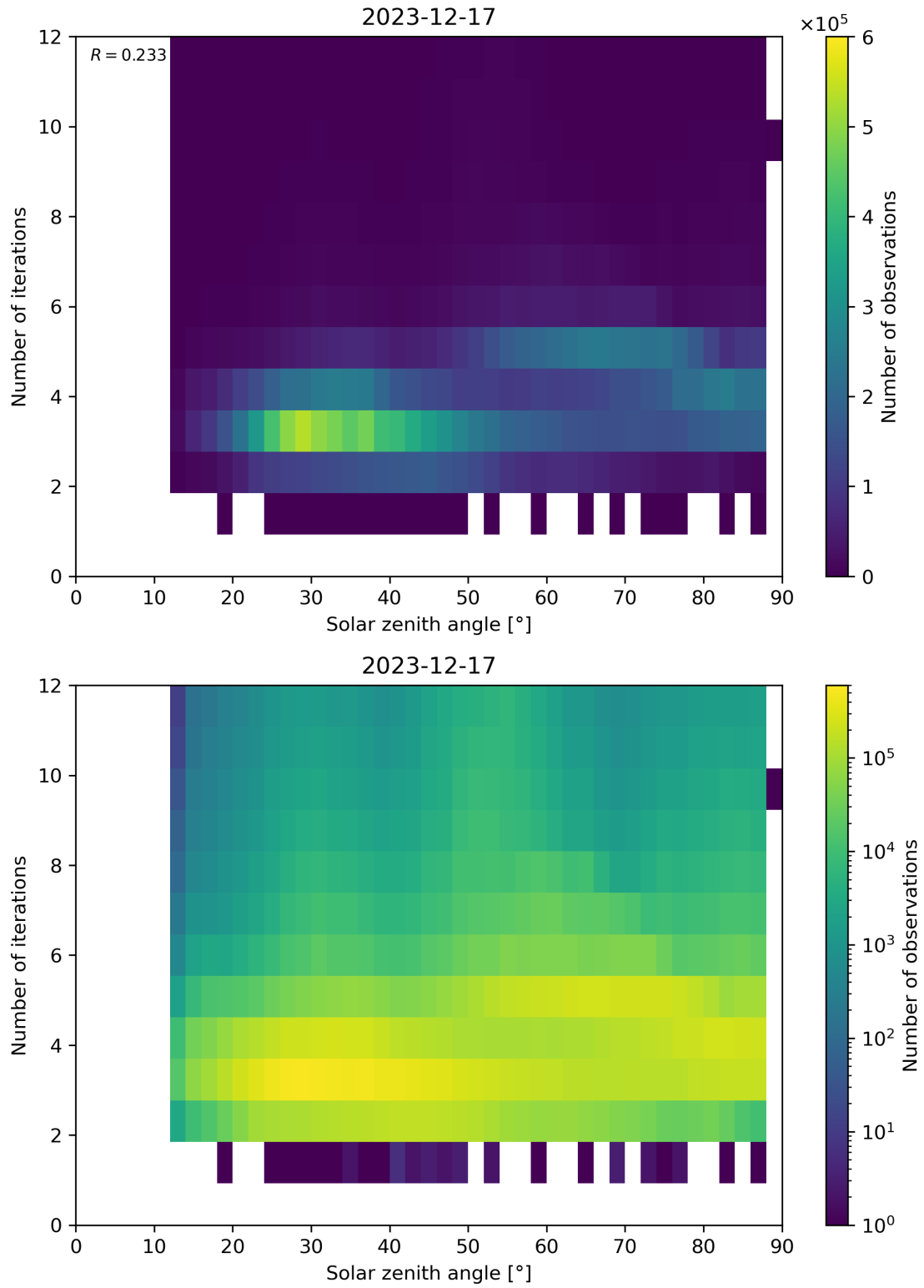
Figure 114: Scatter density plot of “Solar zenith angle” against “Number of iterations” for 2023-12-16 to 2023-12-18.
