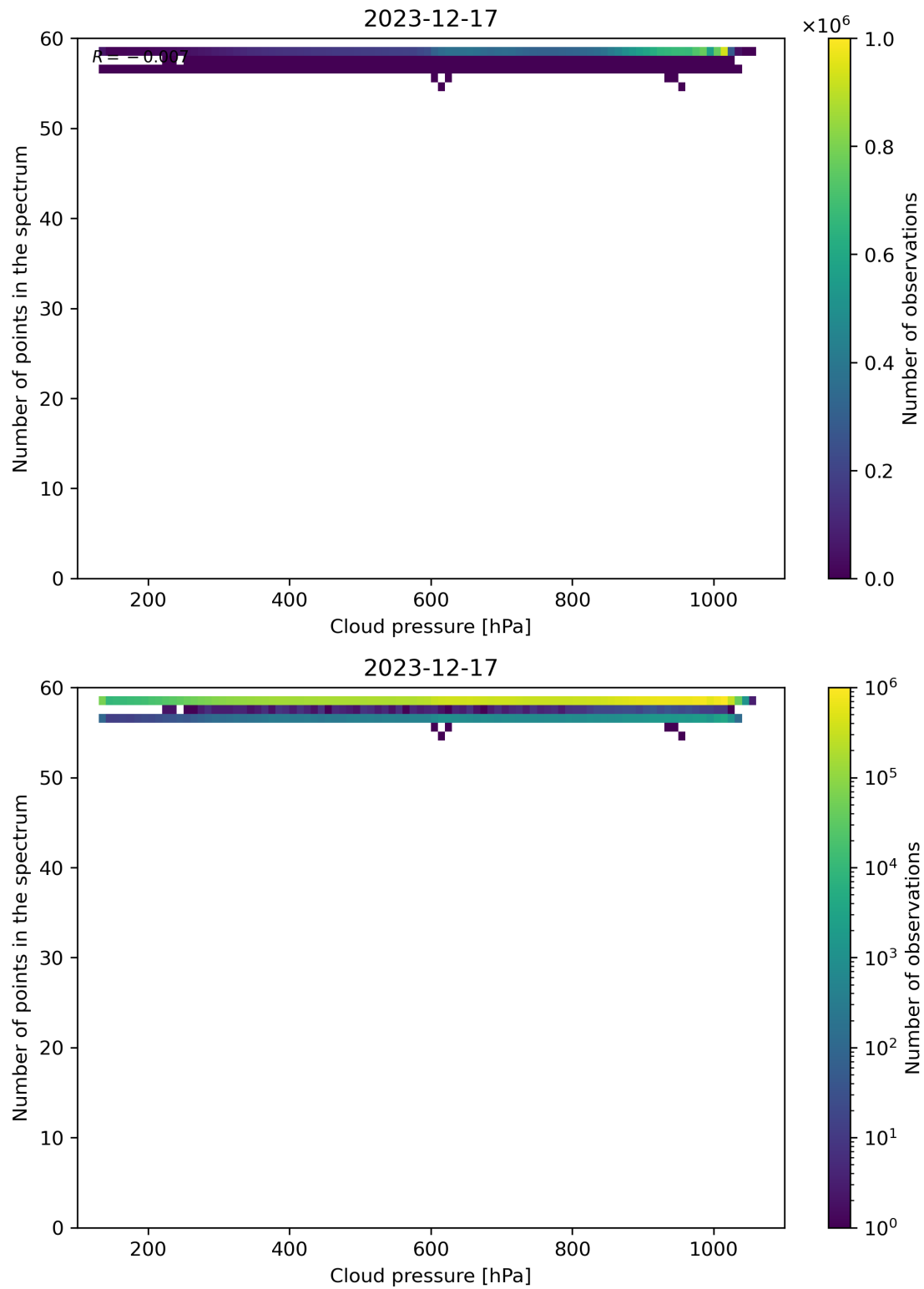
Figure 82: Scatter density plot of “Cloud pressure” against “Number of points in the spectrum” for 2023-12-16 to 2023-12-18.
