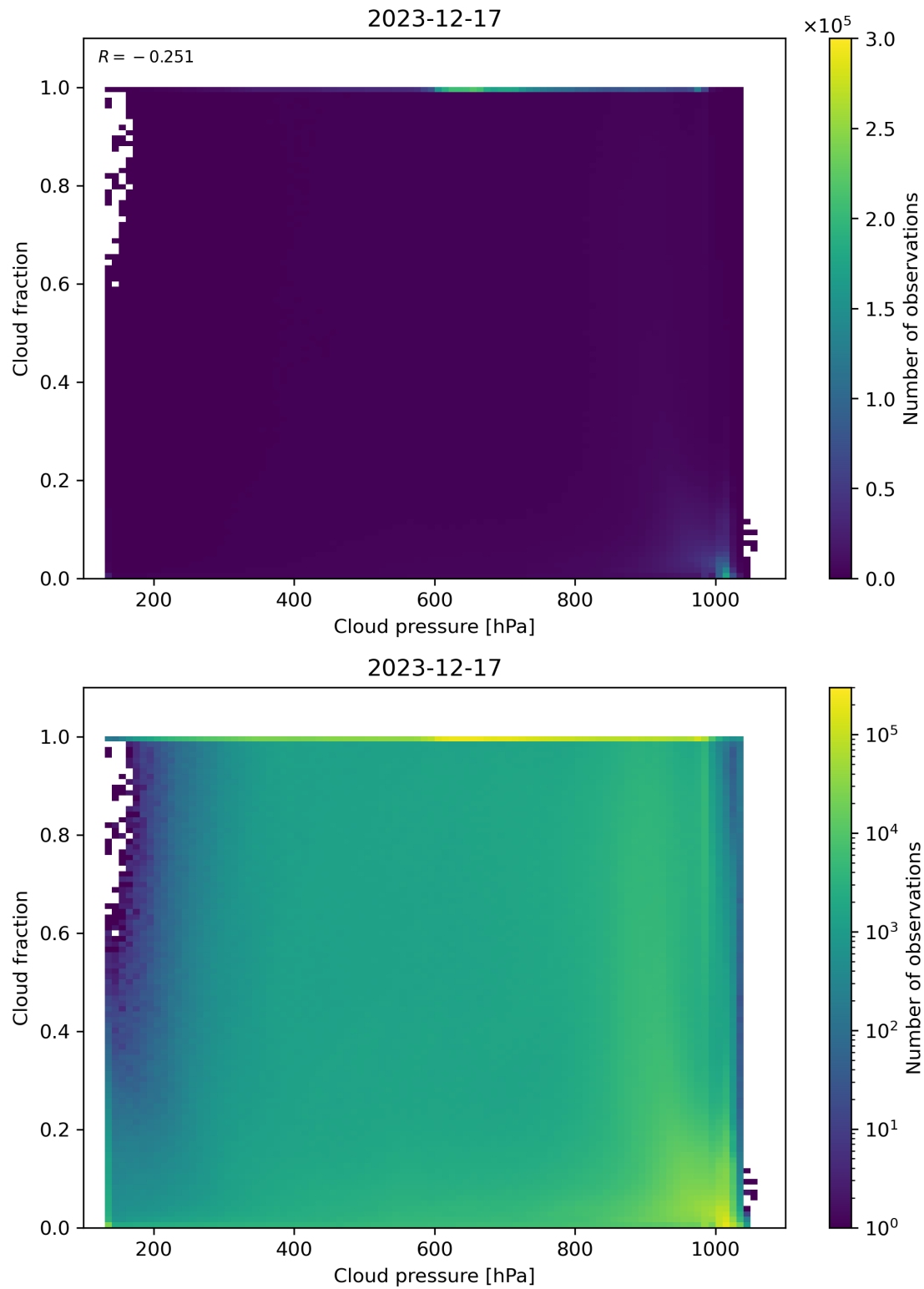
Figure 79: Scatter density plot of “Cloud pressure” against “Cloud fraction” for 2023-12-16 to 2023-12-18.
