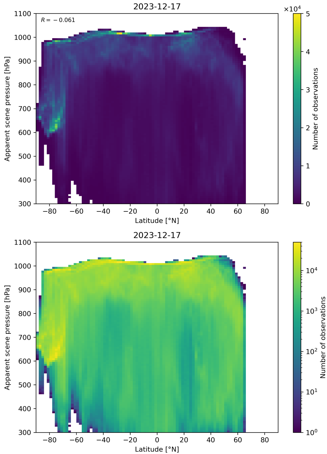
Figure 88: Scatter density plot of “Latitude” against “Apparent scene pressure” for 2023-12-16 to 2023-12-18.
