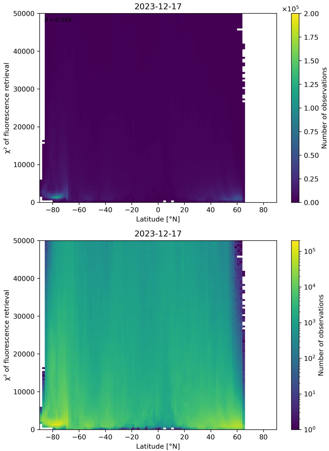
Figure 89: Scatter density plot of “Latitude” against “ \chi^2 of fluorescence retrieval” for 2023-12-16 to 2023-12-18.
