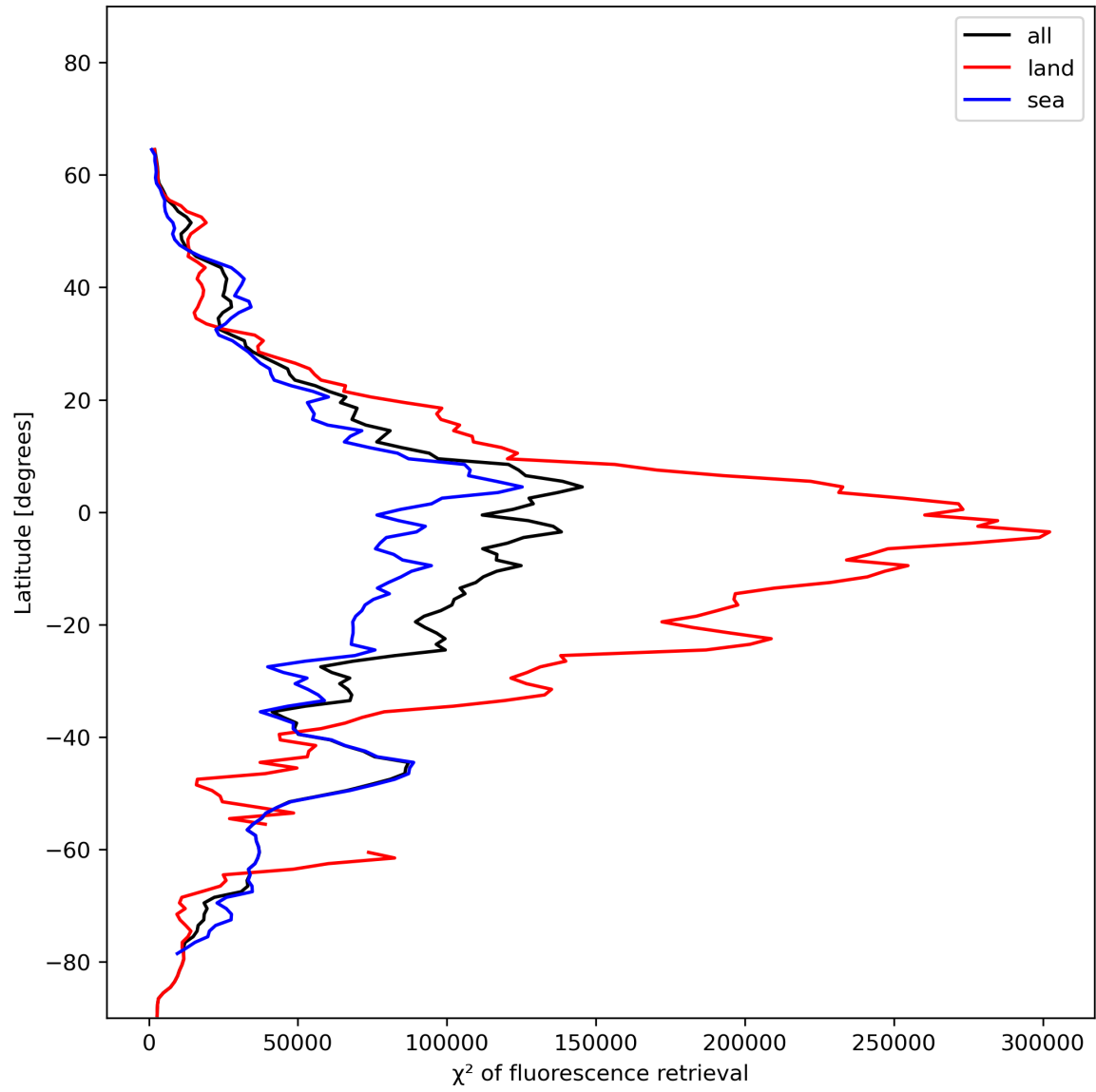
Figure 25: Zonal average of “ \chi^2 of fluorescence retrieval” for 2023-12-16 to 2023-12-18.
