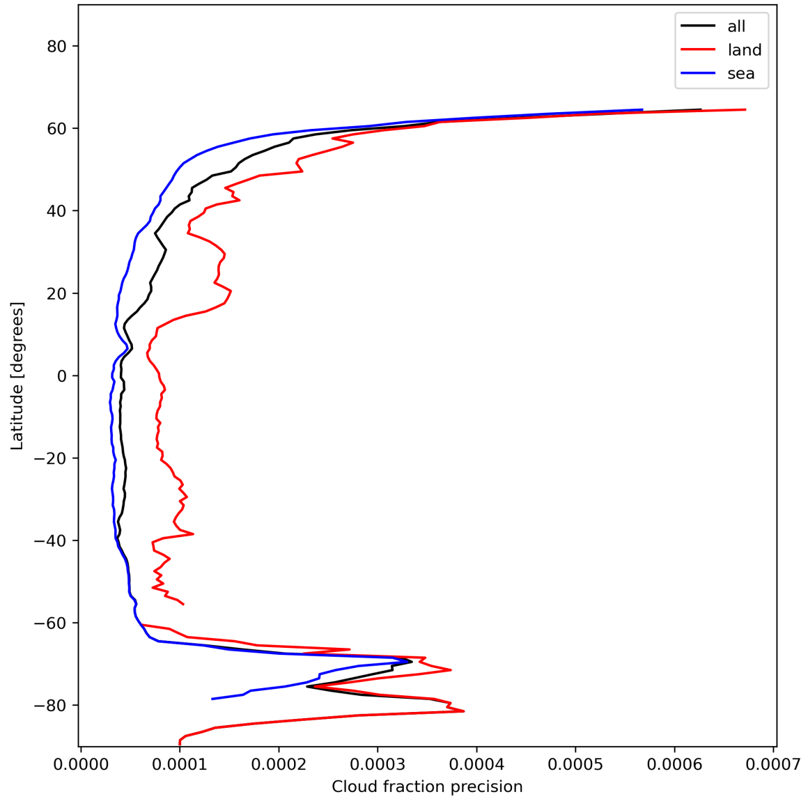
Figure 16: Zonal average of “Cloud fraction precision” for 2023-12-16 to 2023-12-18.
