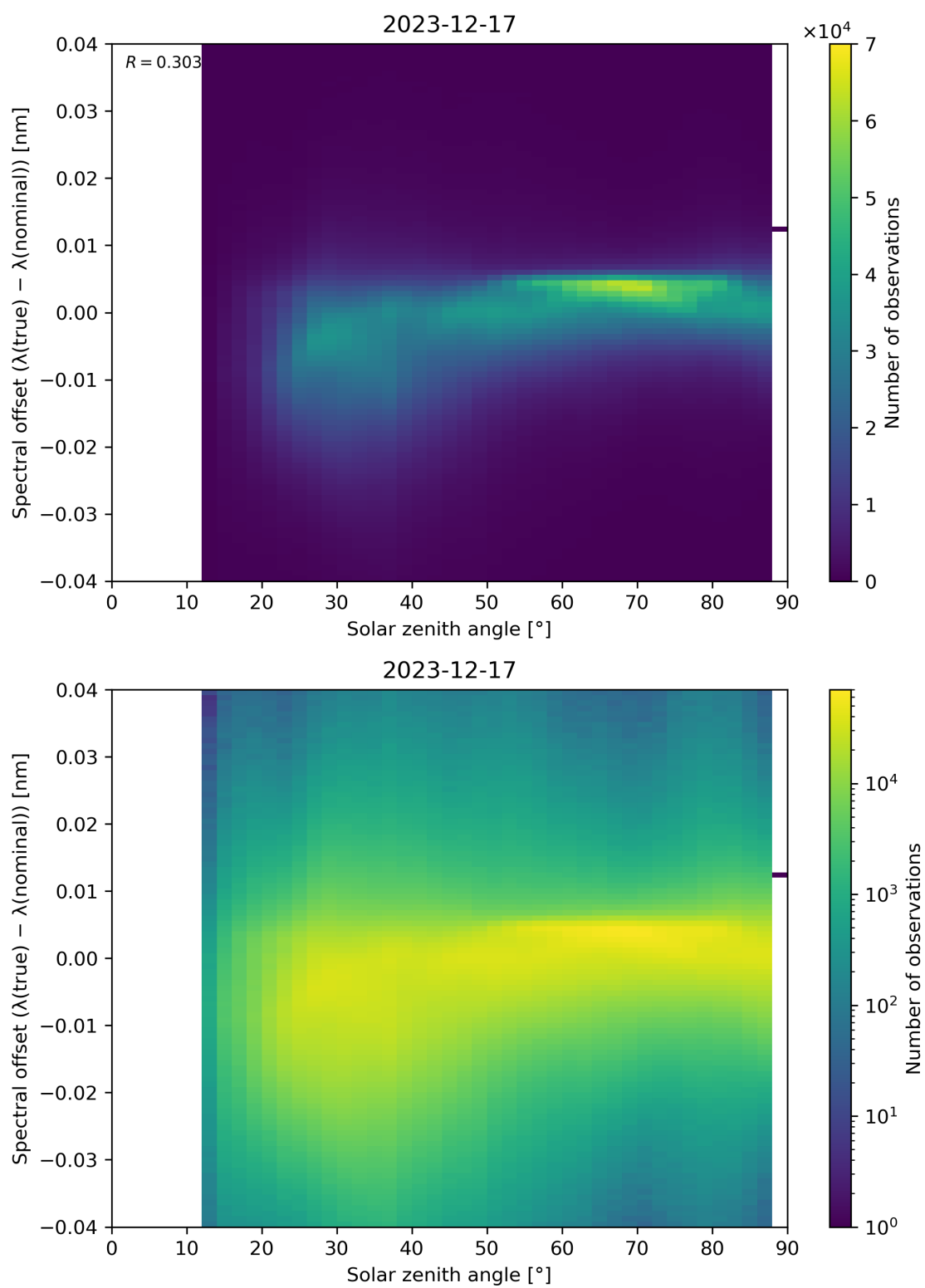
Figure 117: Scatter density plot of “Solar zenith angle” against “Spectral offset ( \lambda(\text{true}) - \lambda(\text{nominal}) )” for 2023-12-16 to 2023-12-18.
