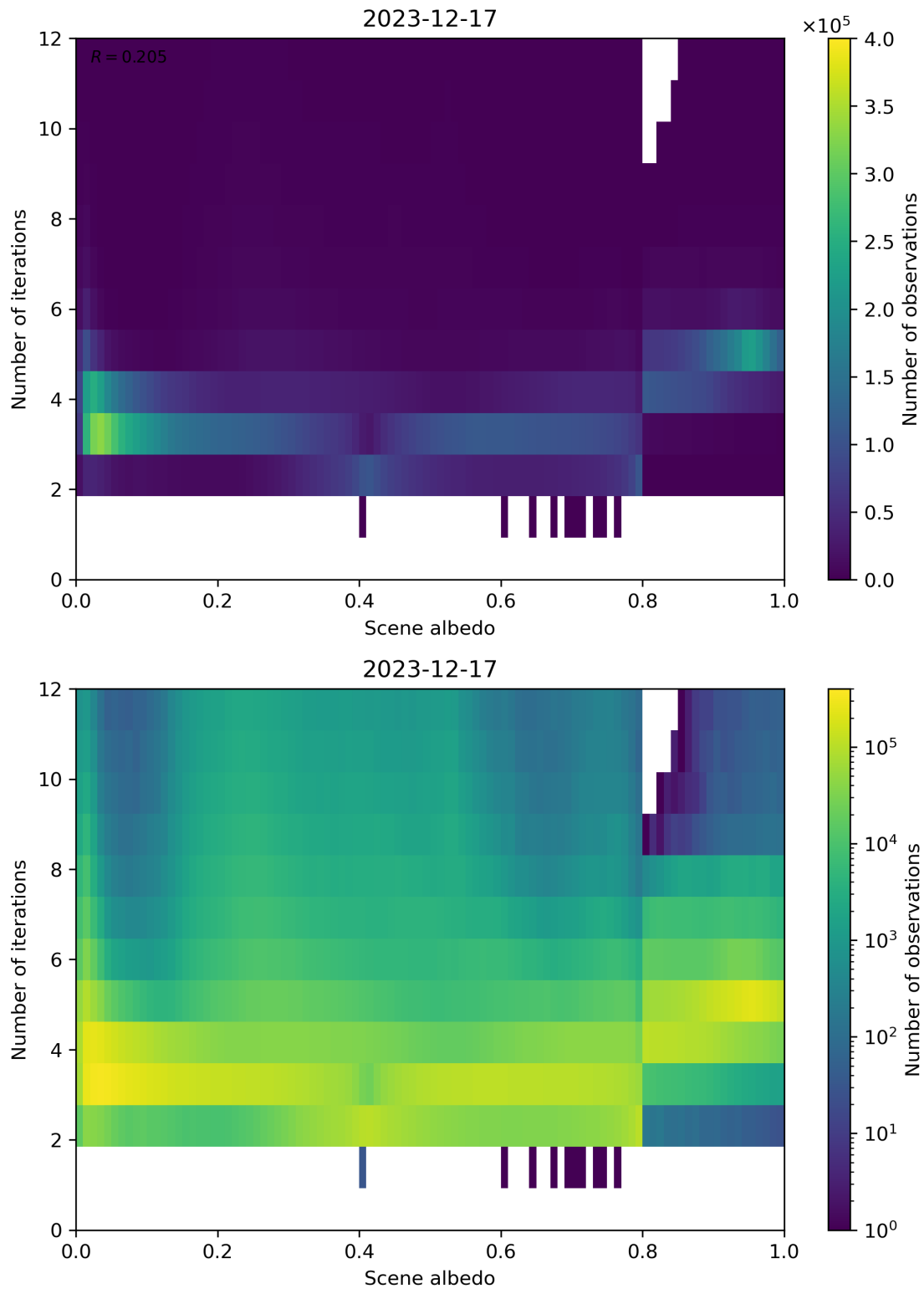
Figure 105: Scatter density plot of “Scene albedo” against “Number of iterations” for 2023-12-16 to 2023-12-18.
