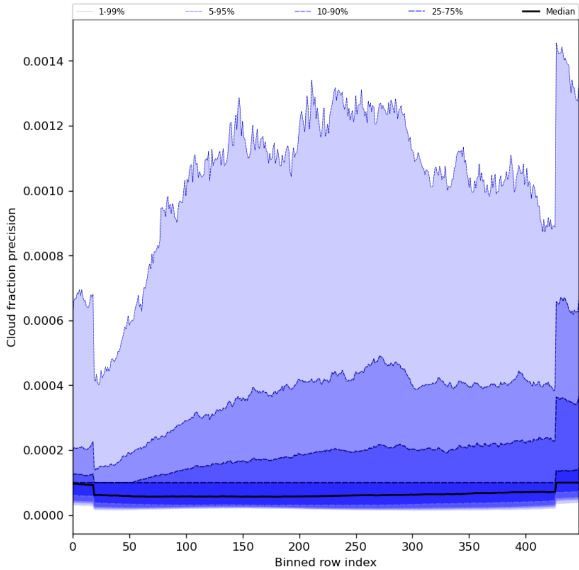
Figure 50: Along track statistics of “Cloud fraction precision” for 2023-12-16 to 2023-12-18
