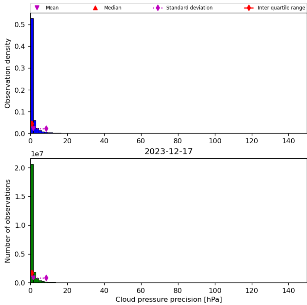
Figure 31: Histogram of “Cloud pressure precision” for 2023-12-16 to 2023-12-18
