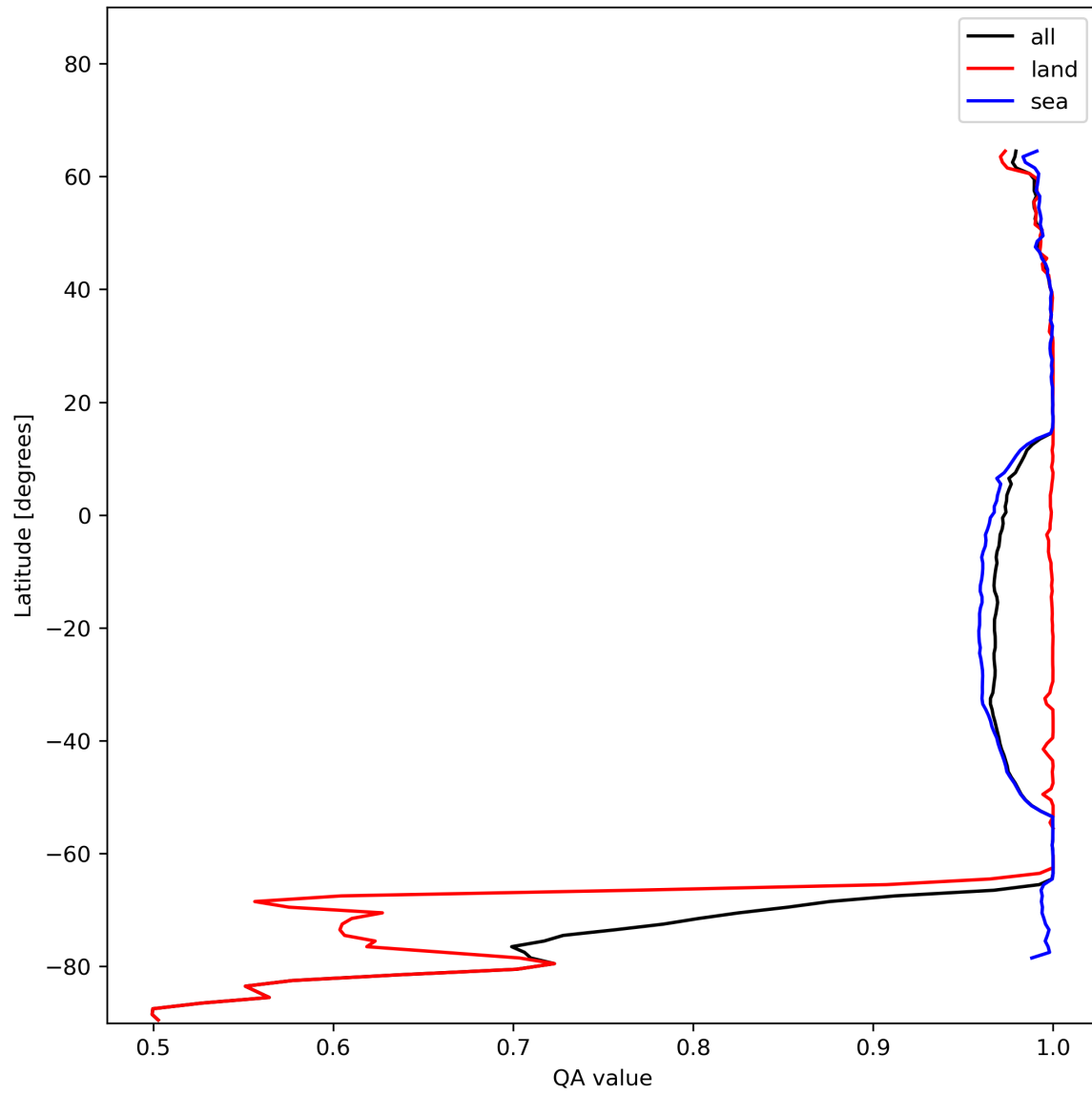
Figure 12: Zonal average of “QA value” for 2023-12-16 to 2023-12-18.
