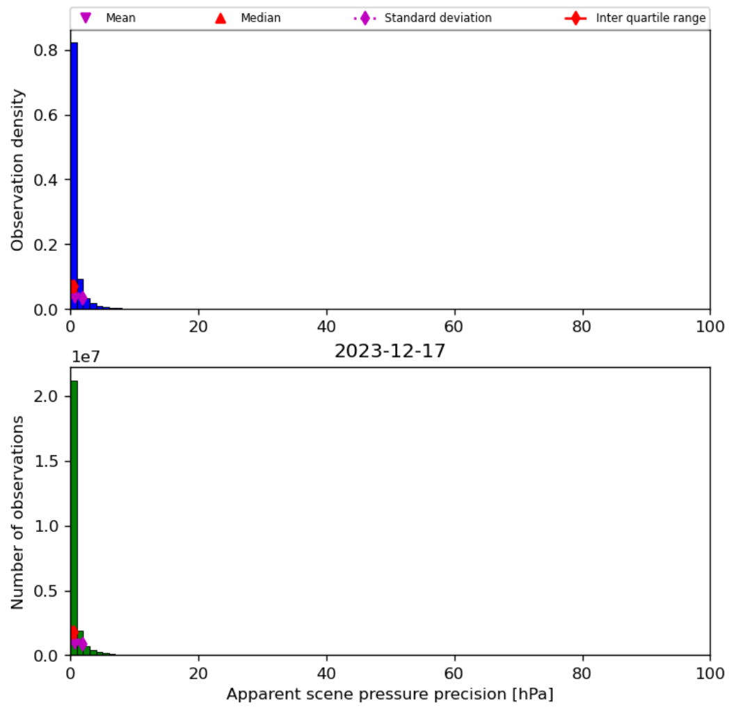
Figure 37: Histogram of “Apparent scene pressure precision” for 2023-12-16 to 2023-12-18
