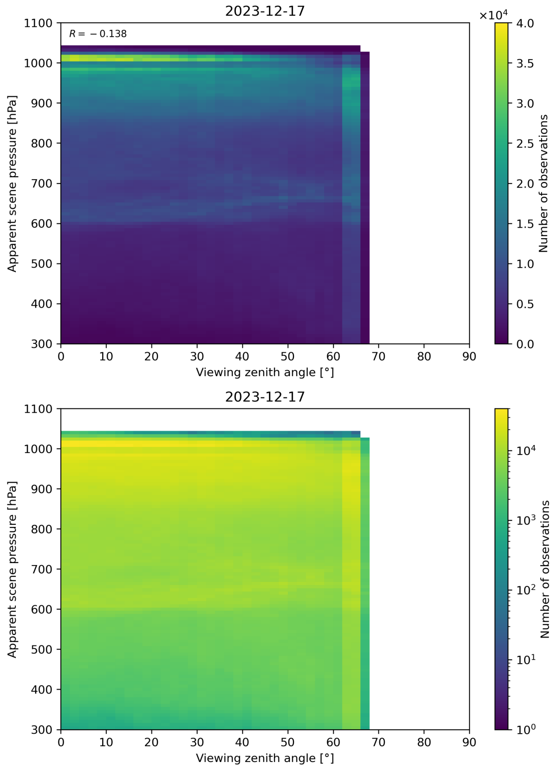
Figure 118: Scatter density plot of “Viewing zenith angle” against “Apparent scene pressure” for 2023-12-16 to 2023-12-18.
