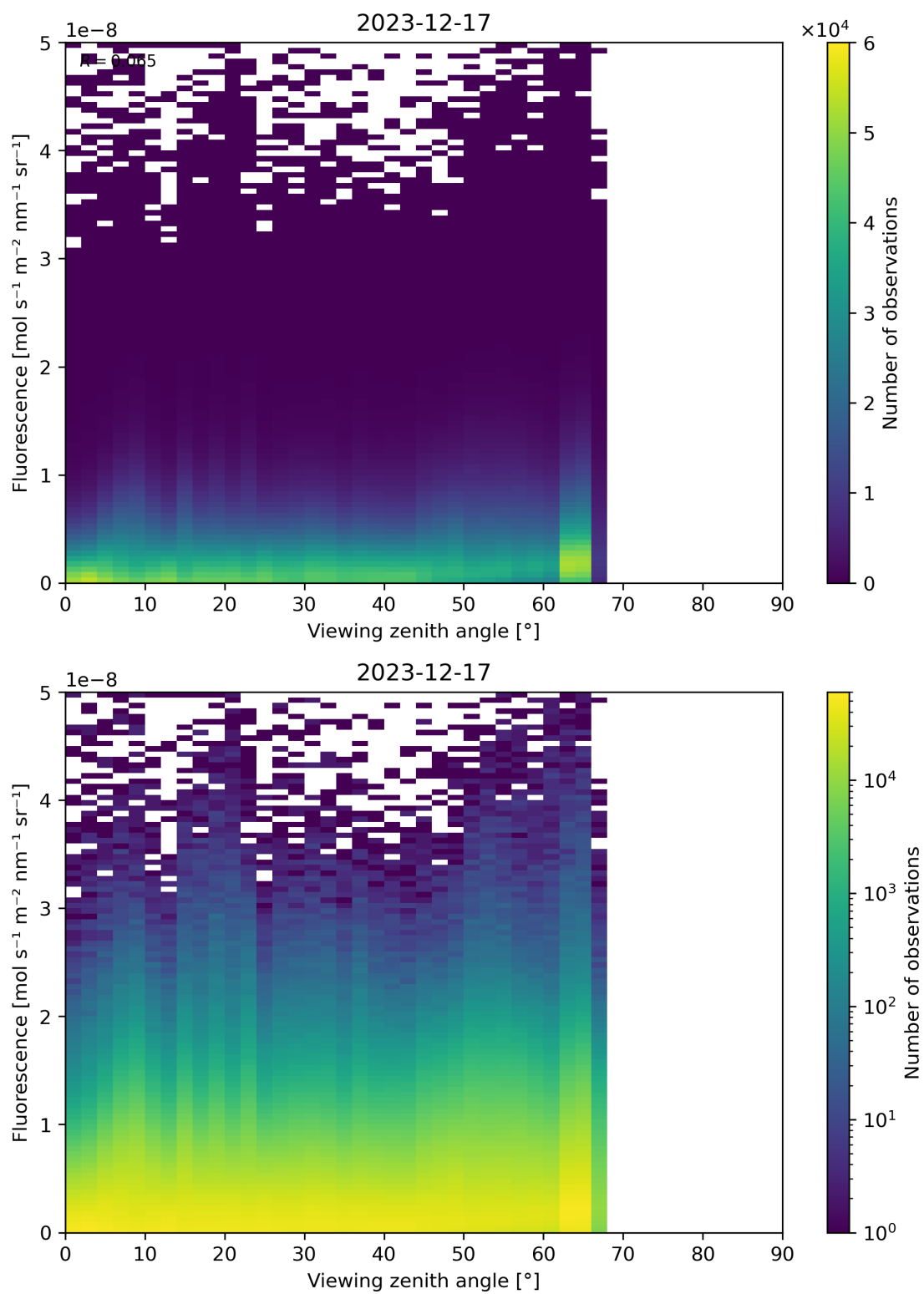
Figure 122: Scatter density plot of “Viewing zenith angle” against “Fluorescence” for 2023-12-16 to 2023-12-18.
