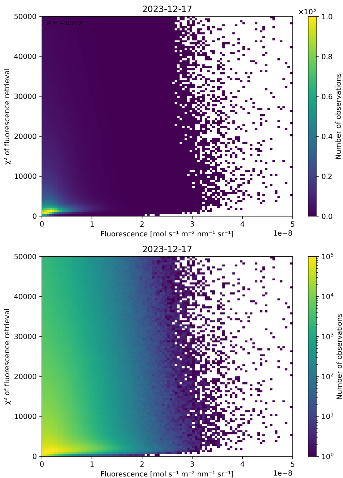
Figure 85: Scatter density plot of “Fluorescence” against “ \chi^2 of fluorescence retrieval” for 2023-12-16 to 2023-12-18.
