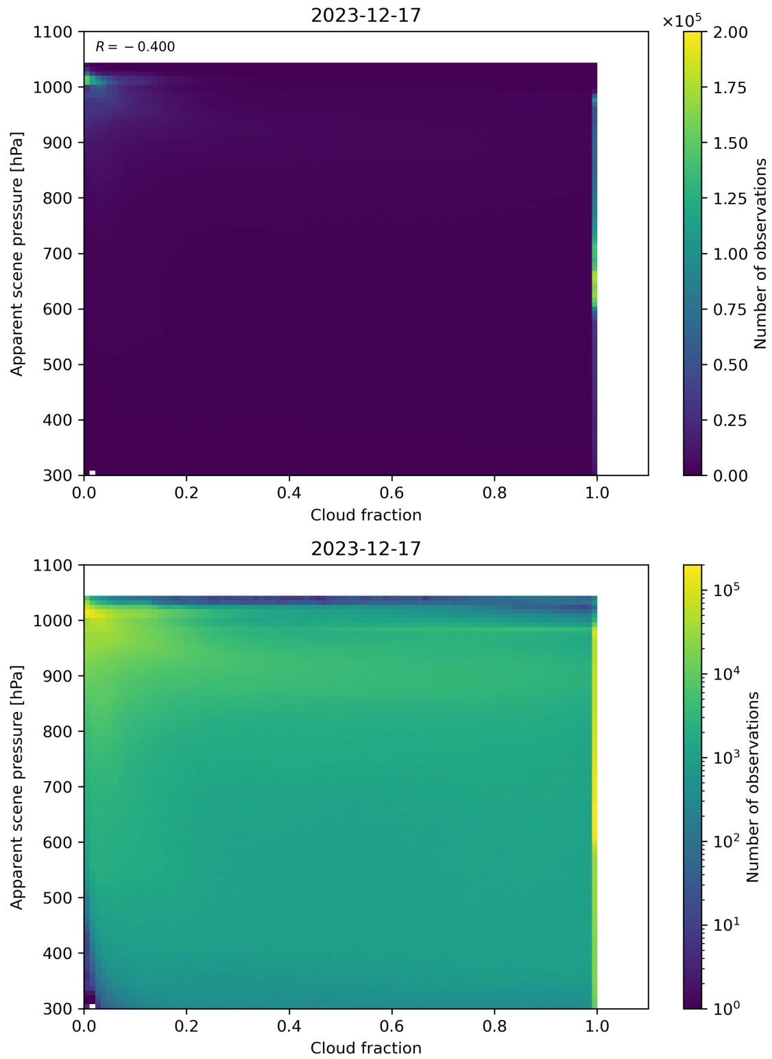
Figure 70: Scatter density plot of “Cloud fraction” against “Apparent scene pressure” for 2023-12-16 to 2023-12-18.
