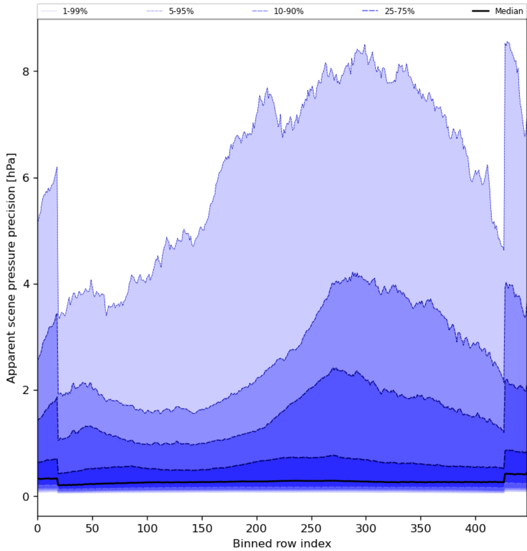
Figure 54: Along track statistics of “Apparent scene pressure precision” for 2023-12-16 to 2023-12-18
