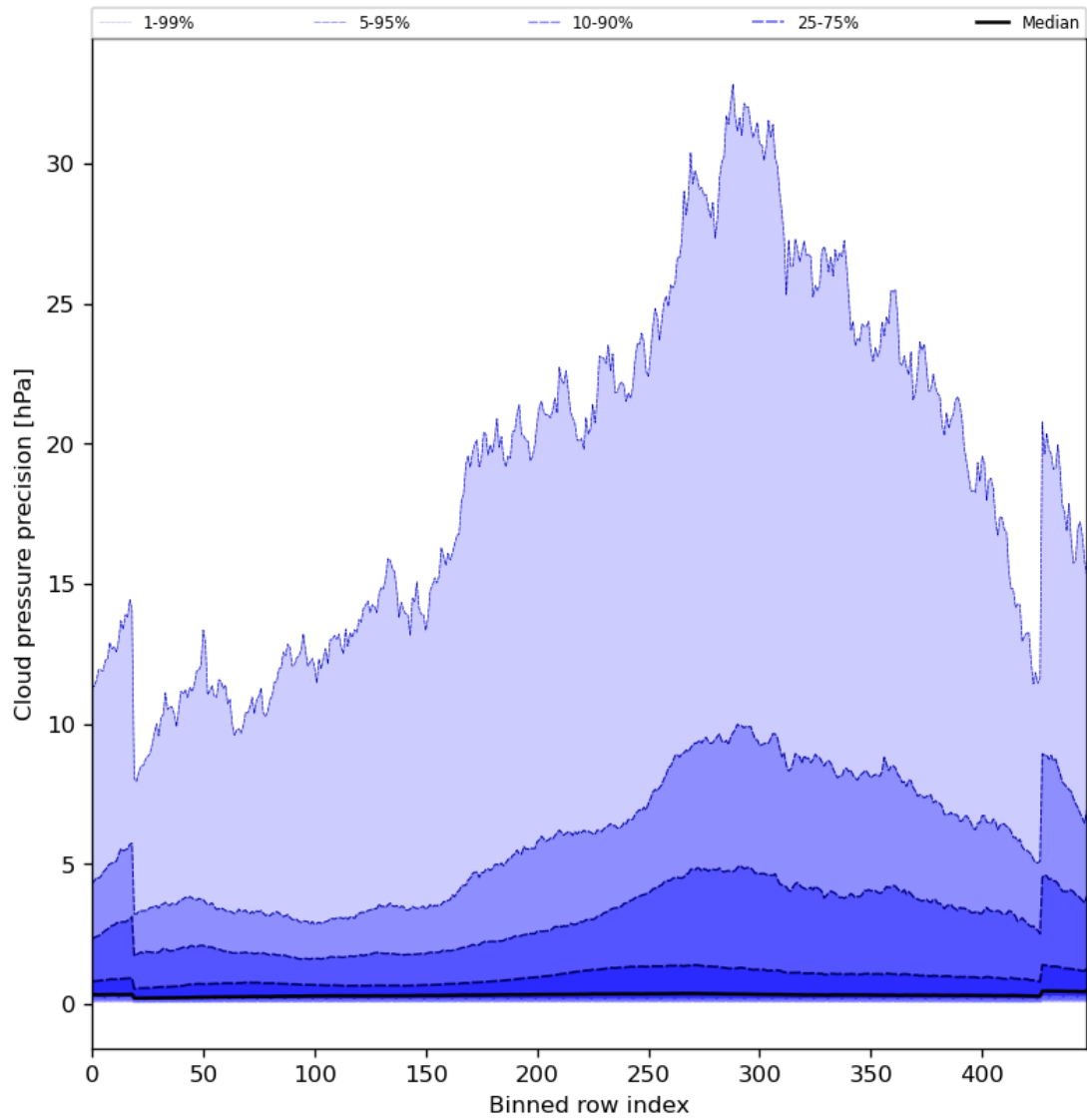
Figure 48: Along track statistics of “Cloud pressure precision” for 2023-12-16 to 2023-12-18
