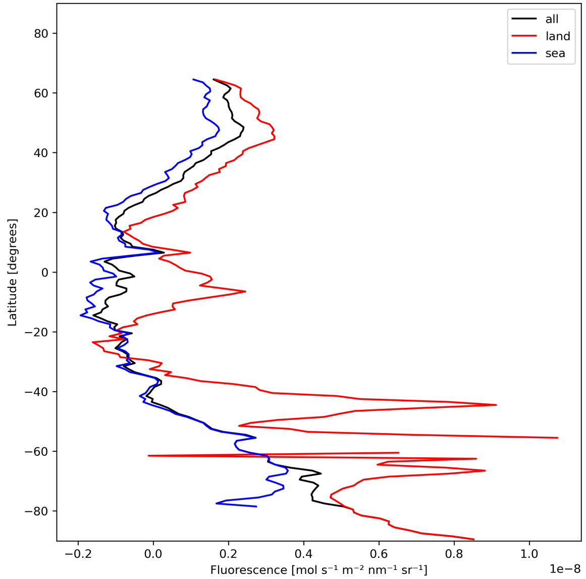
Figure 23: Zonal average of “Fluorescence” for 2023-12-16 to 2023-12-18.
