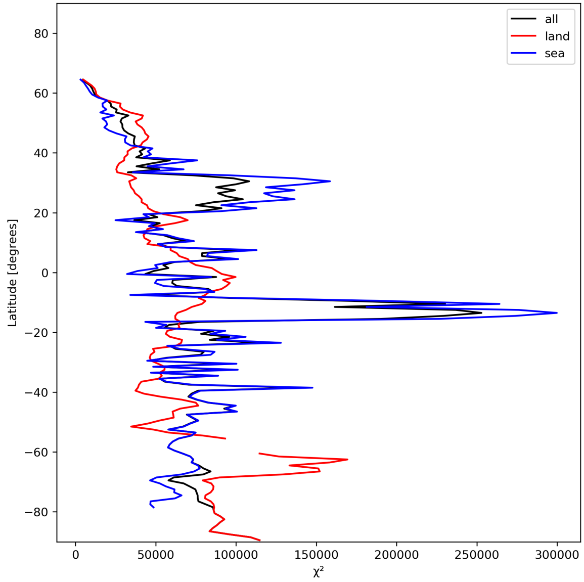
Figure 21: Zonal average of “ \chi^2 ” for 2023-12-16 to 2023-12-18.
