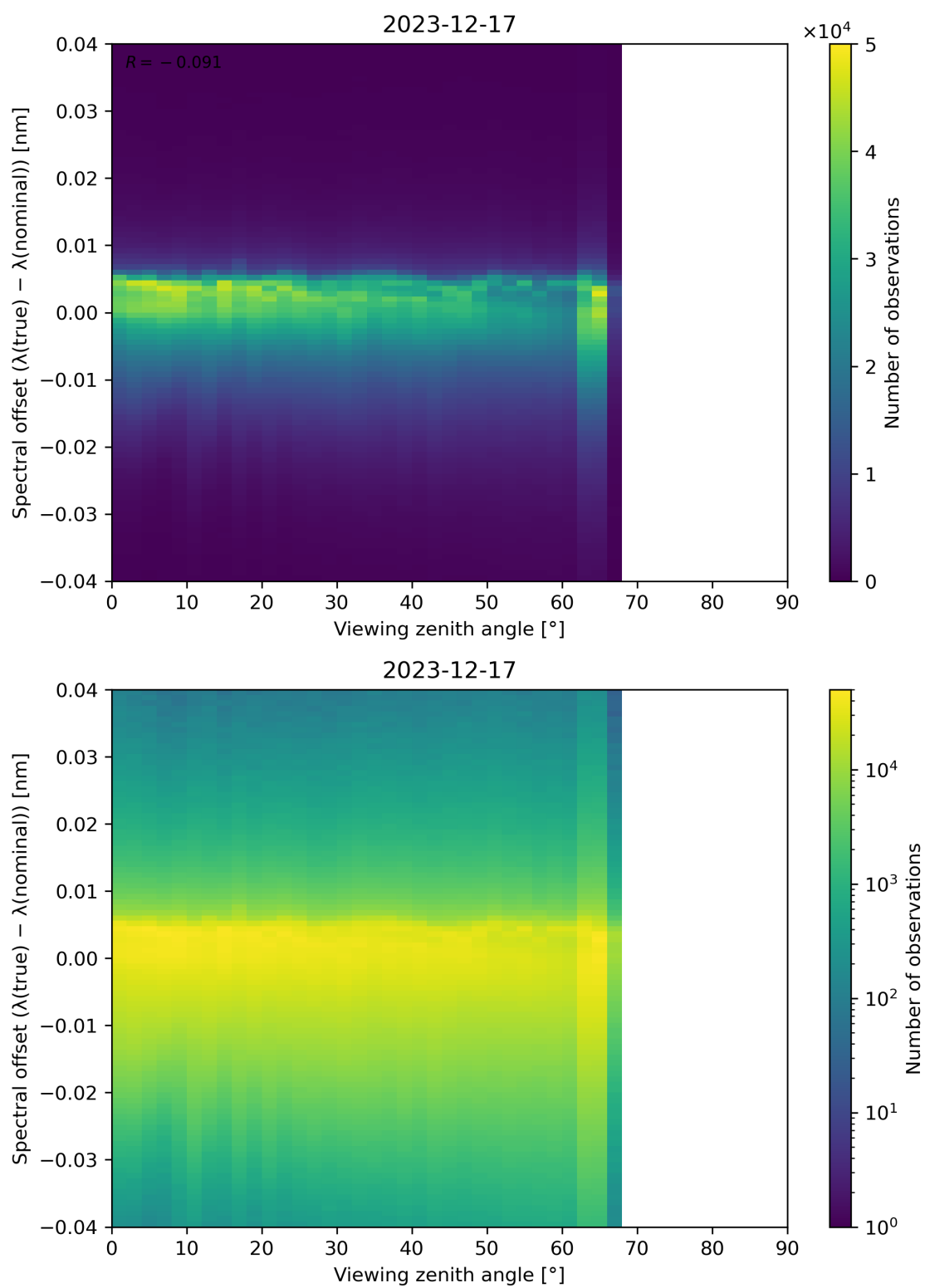
Figure 128: Scatter density plot of “Viewing zenith angle” against “Spectral offset ( \lambda(\text{true}) - \lambda(\text{nominal}) )” for 2023-12-16 to 2023-12-18.
