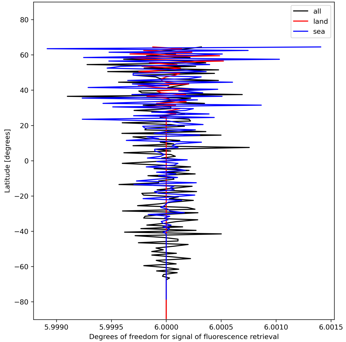
Figure 26: Zonal average of “Degrees of freedom for signal of fluorescence retrieval” for 2023-12-16 to 2023-12-18.
