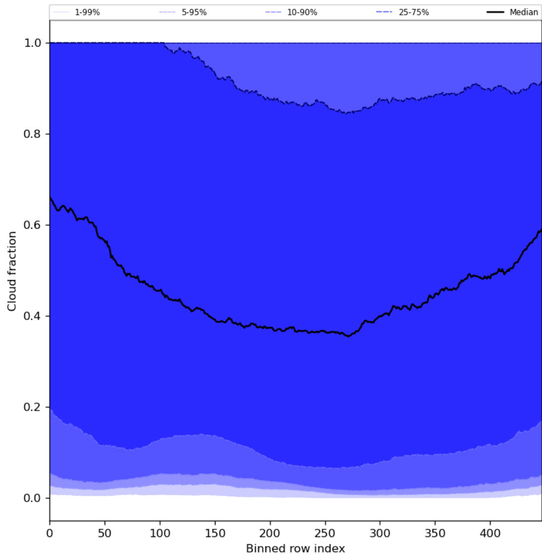
Figure 49: Along track statistics of “Cloud fraction” for 2023-12-16 to 2023-12-18
