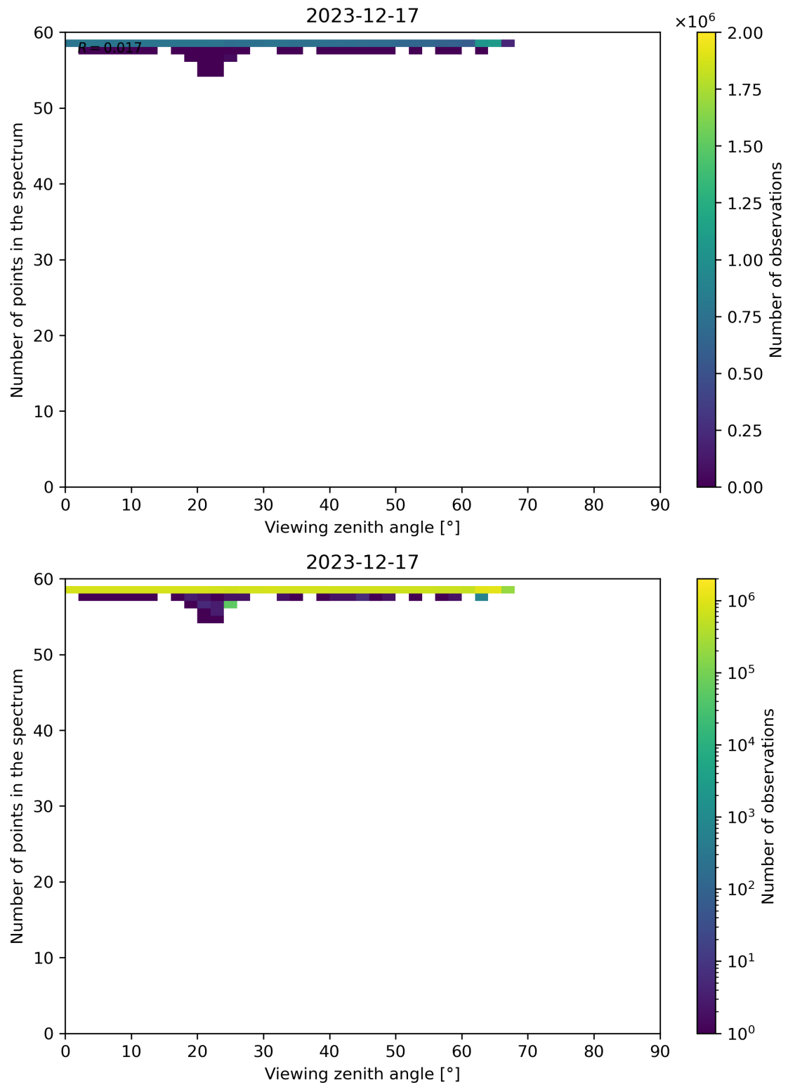
Figure 125: Scatter density plot of “Viewing zenith angle” against “Number of points in the spectrum” for 2023-12-16 to 2023-12-18.
