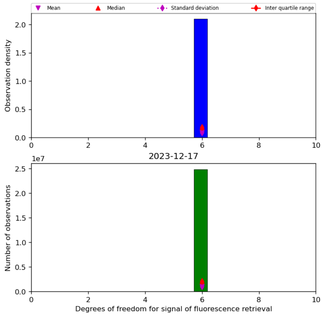
Figure 43: Histogram of “Degrees of freedom for signal of fluorescence retrieval” for 2023-12-16 to 2023-12-18
