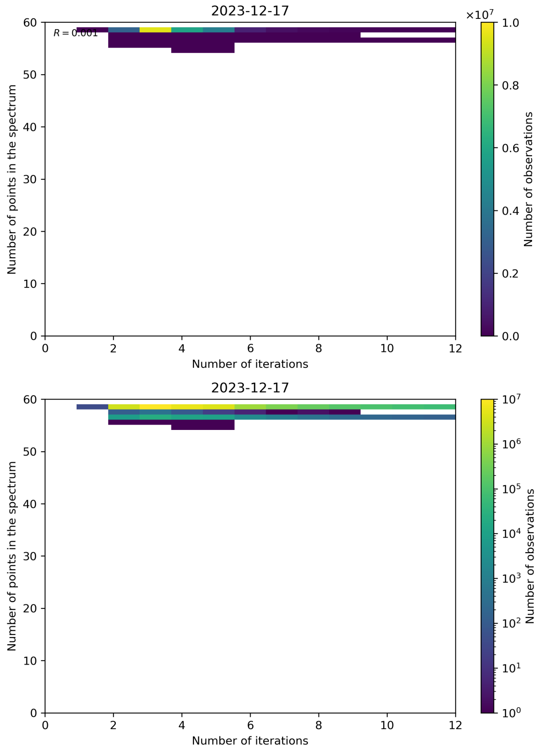
Figure 99: Scatter density plot of “Number of iterations” against “Number of points in the spectrum” for 2023-12-16 to 2023-12-18.
