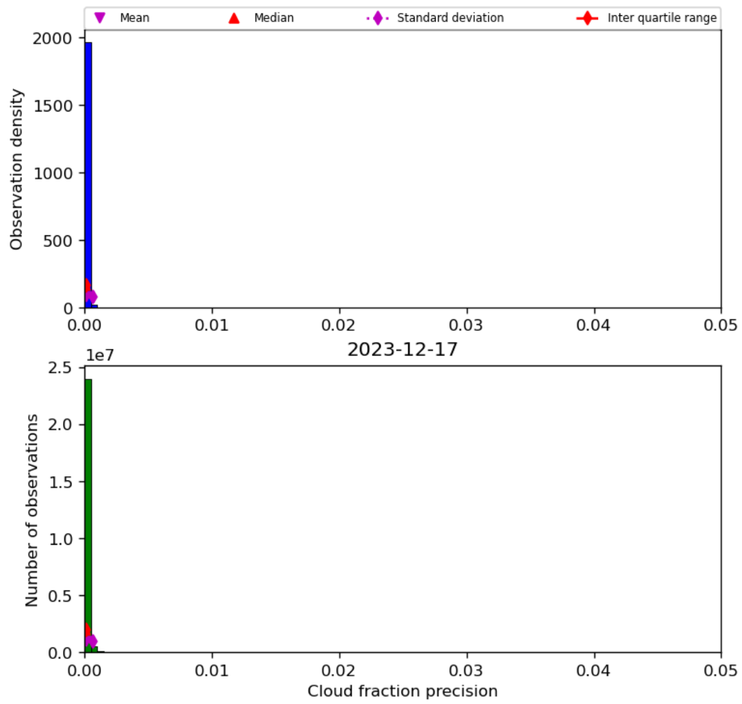
Figure 33: Histogram of “Cloud fraction precision” for 2023-12-16 to 2023-12-18
