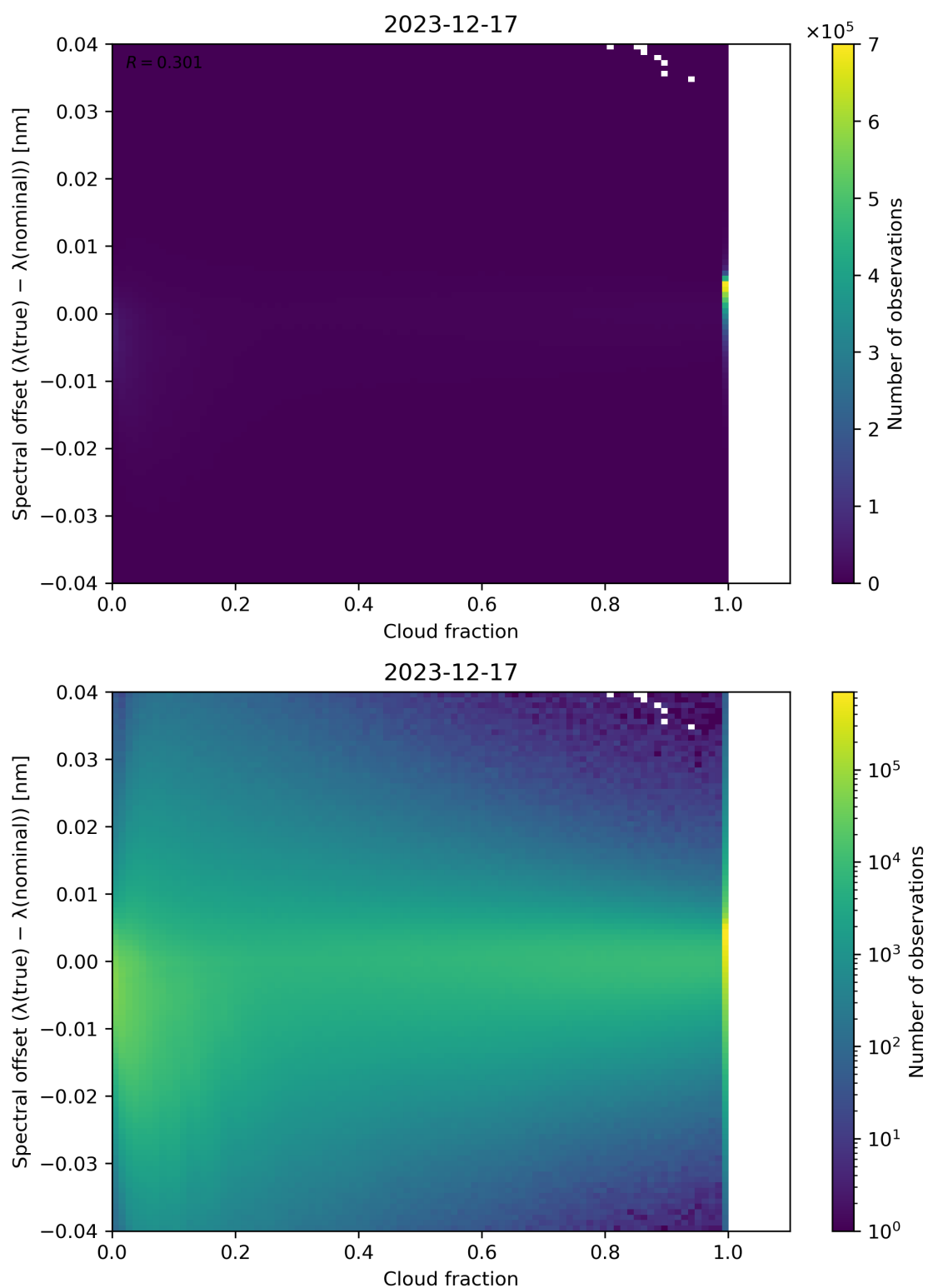
Figure 76: Scatter density plot of “Cloud fraction” against “Spectral offset ( \lambda(\text{true}) - \lambda(\text{nominal}) )” for 2023-12-16 to 2023-12-18.
