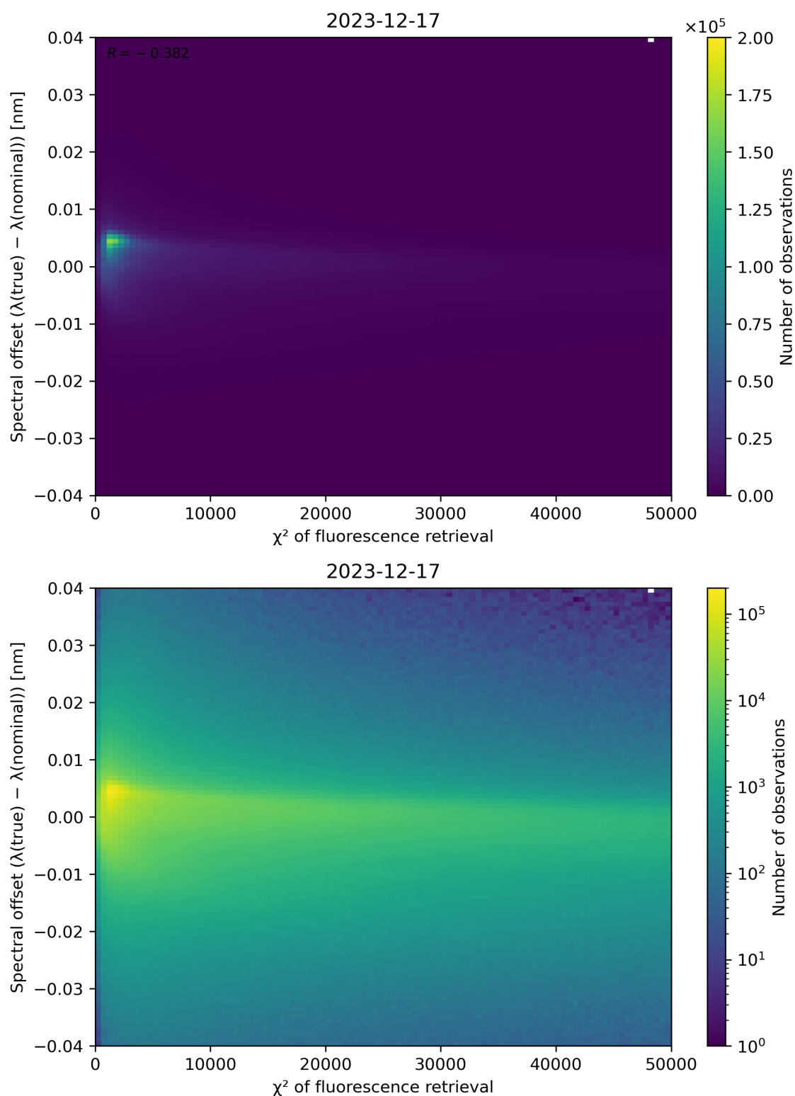
Figure 69: Scatter density plot of " \chi^2 of fluorescence retrieval" against "Spectral offset ( \lambda(\text{true}) - \lambda(\text{nominal}) )" for 2023-12-16 to 2023-12-18.
