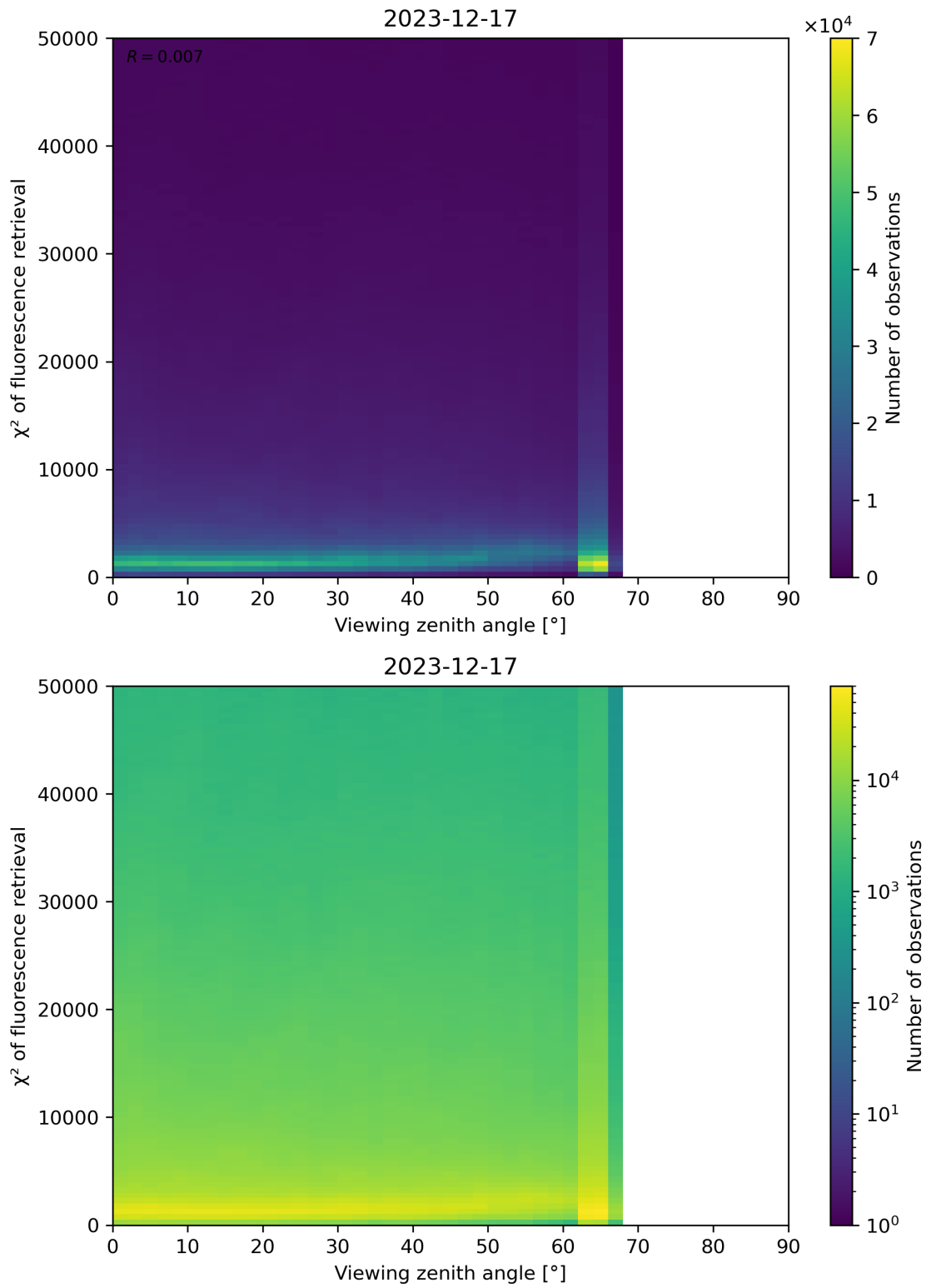
Figure 119: Scatter density plot of “Viewing zenith angle” against “ \chi^2 of fluorescence retrieval” for 2023-12-16 to 2023-12-18.
