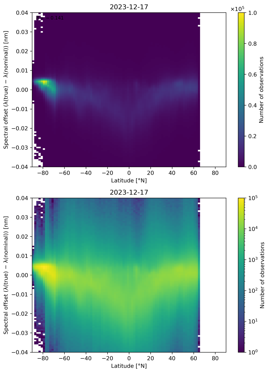
Figure 96: Scatter density plot of “Latitude” against “Spectral offset ( \lambda(\text{true}) - \lambda(\text{nominal}) )” for 2023-12-16 to 2023-12-18.
