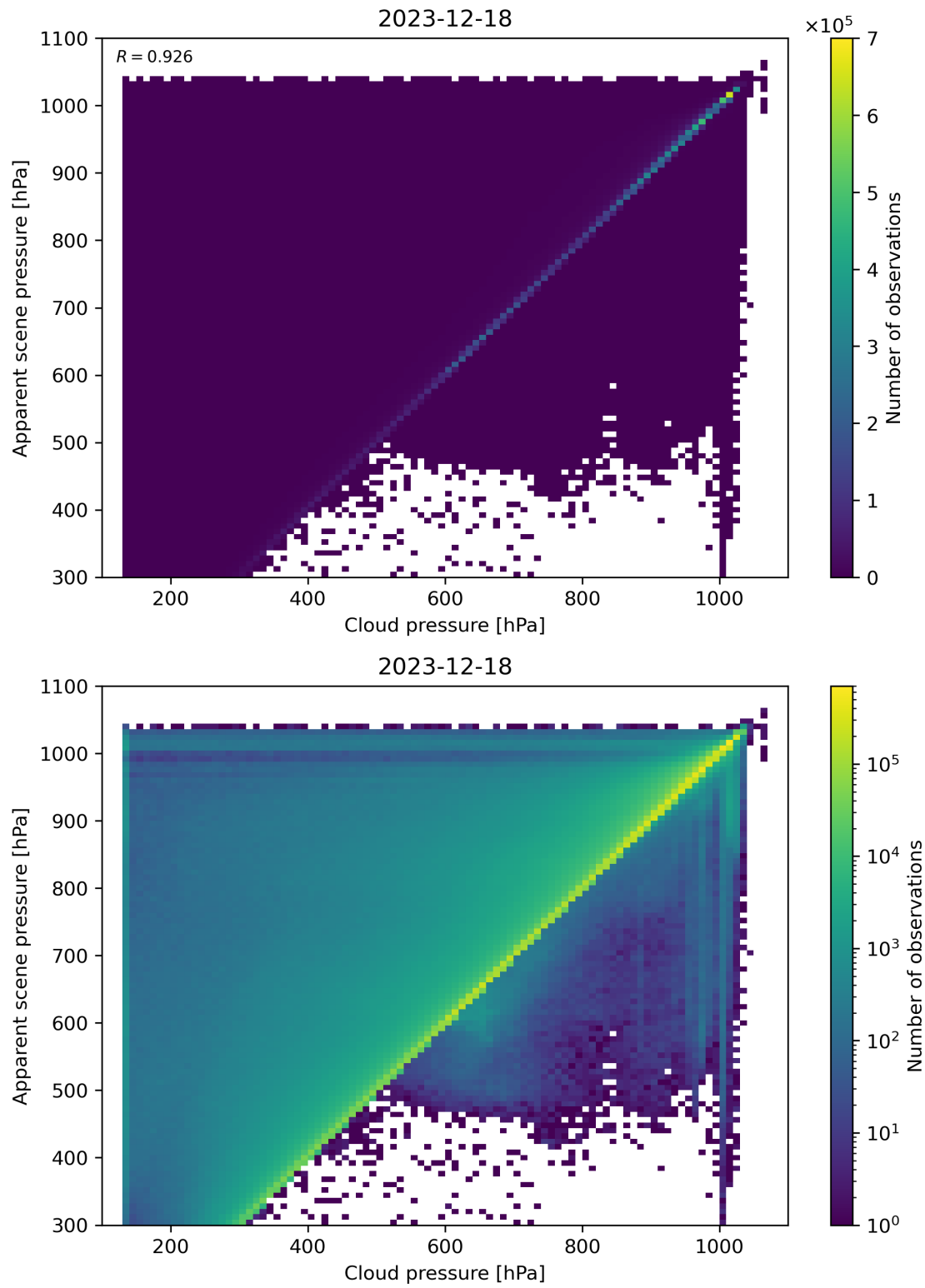
Figure 77: Scatter density plot of “Cloud pressure” against “Apparent scene pressure” for 2023-12-17 to 2023-12-19.
