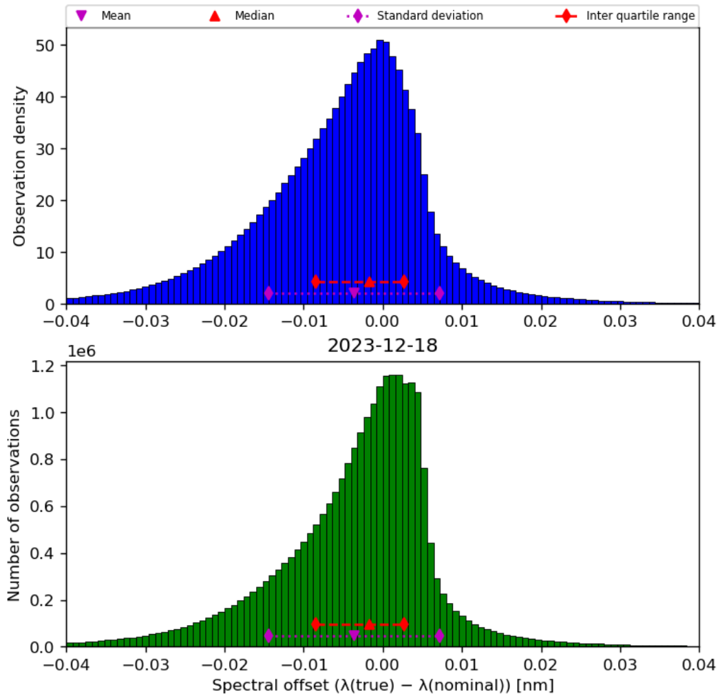
Figure 45: Histogram of “Spectral offset ( \lambda(\text{true}) - \lambda(\text{nominal}) )” for 2023-12-17 to 2023-12-19
