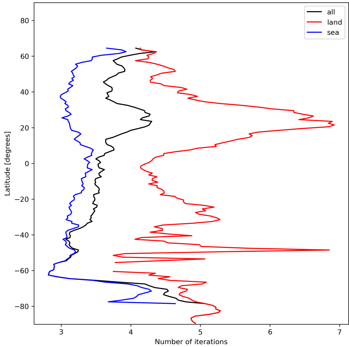
Figure 22: Zonal average of “Number of iterations” for 2023-12-17 to 2023-12-19.
