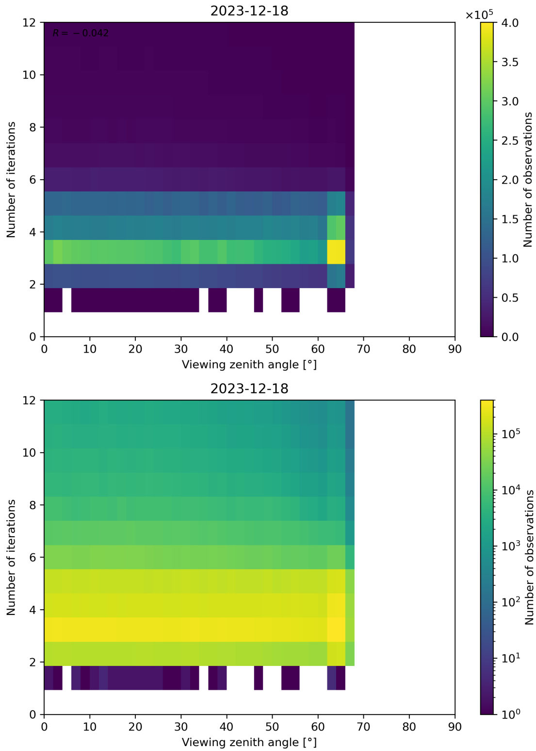
Figure 124: Scatter density plot of “Viewing zenith angle” against “Number of iterations” for 2023-12-17 to 2023-12-19.
