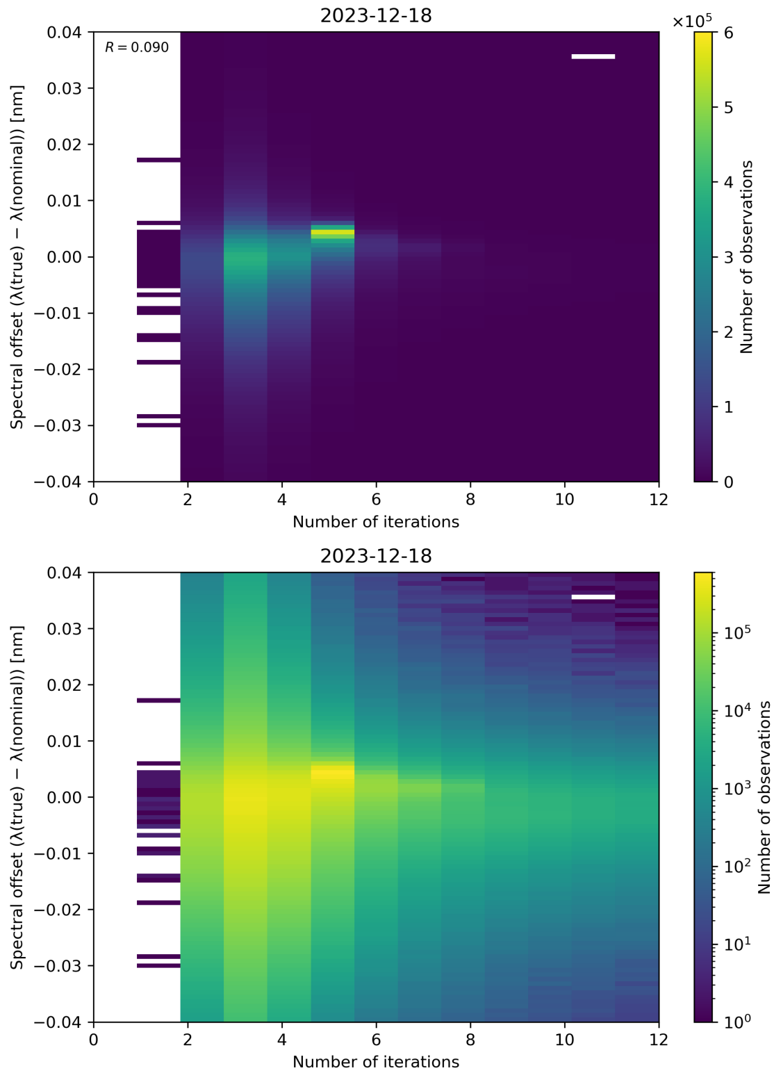
Figure 100: Scatter density plot of “Number of iterations” against “Spectral offset ( \lambda(\text{true}) - \lambda(\text{nominal}) )” for 2023-12-17 to 2023-12-19.
