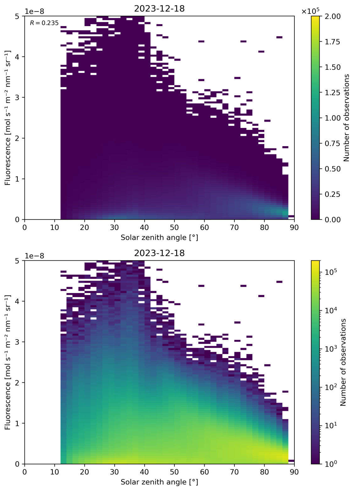
Figure 112: Scatter density plot of “Solar zenith angle” against “Fluorescence” for 2023-12-17 to 2023-12-19.
