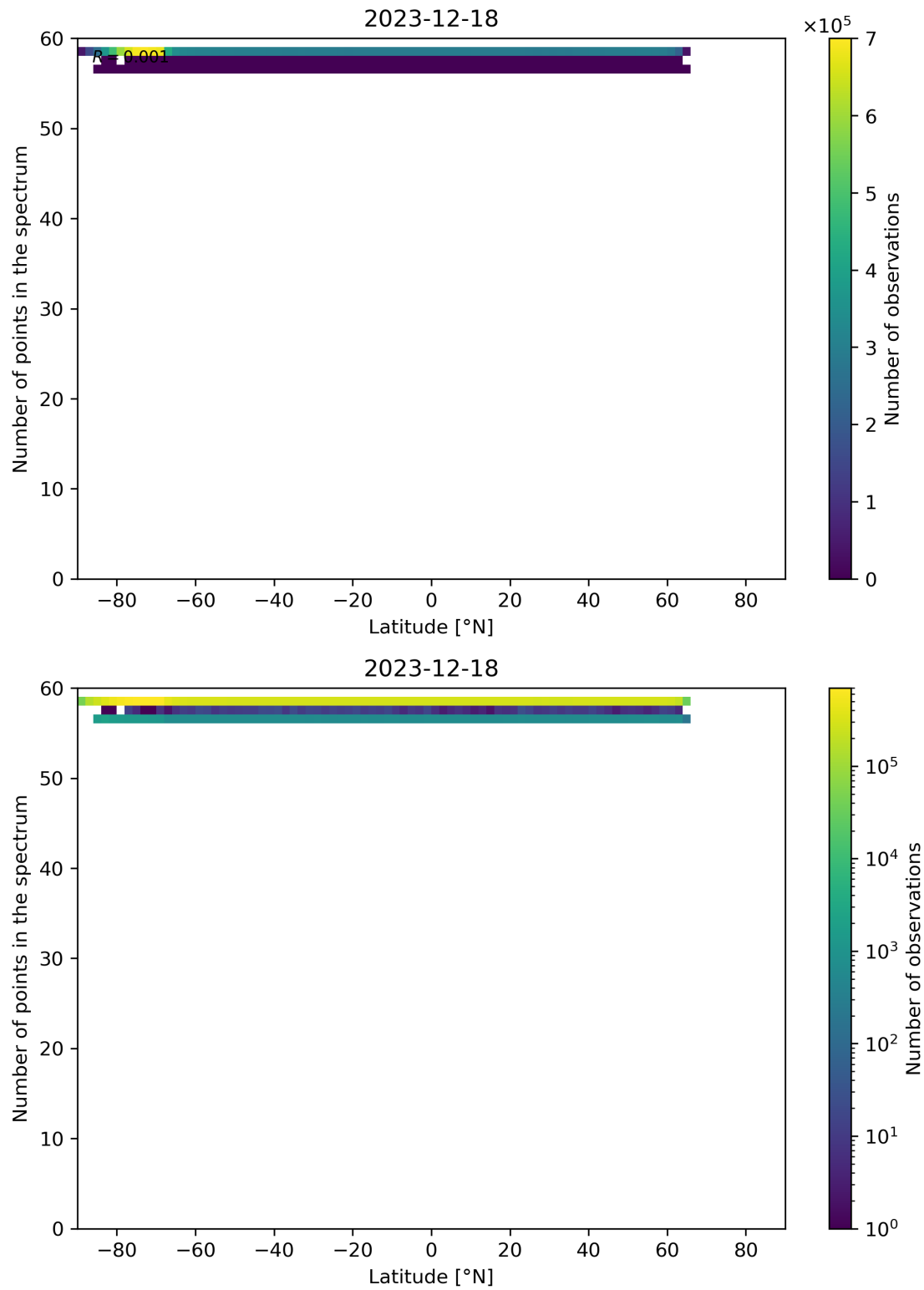
Figure 94: Scatter density plot of “Latitude” against “Number of points in the spectrum” for 2023-12-17 to 2023-12-19.
