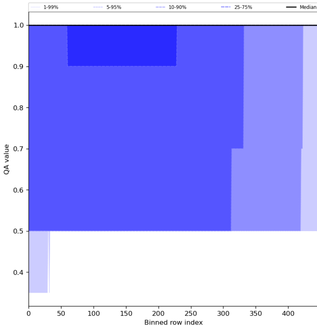
Figure 46: Along track statistics of “QA value” for 2023-12-17 to 2023-12-19
