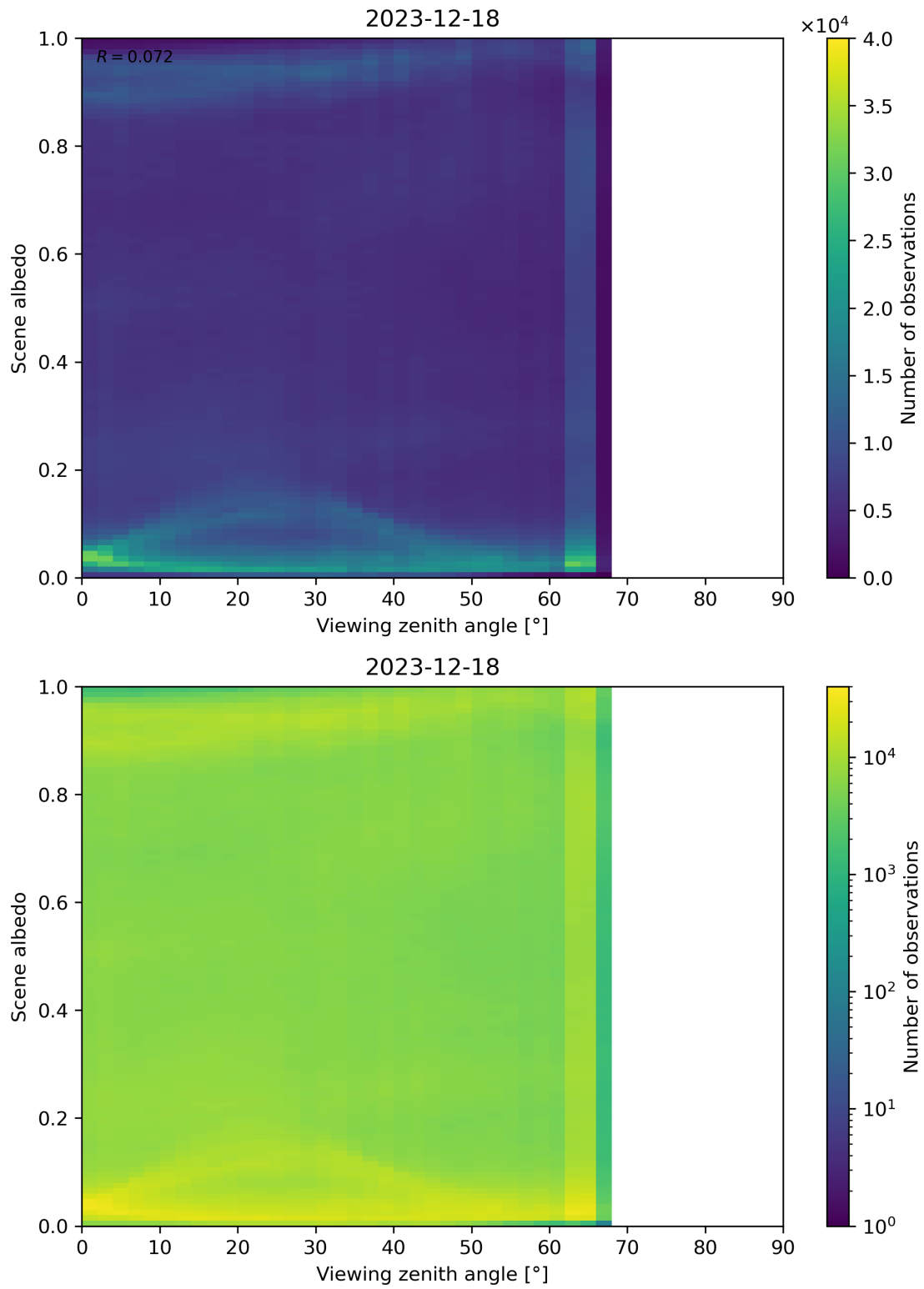
Figure 126: Scatter density plot of “Viewing zenith angle” against “Scene albedo” for 2023-12-17 to 2023-12-19.
