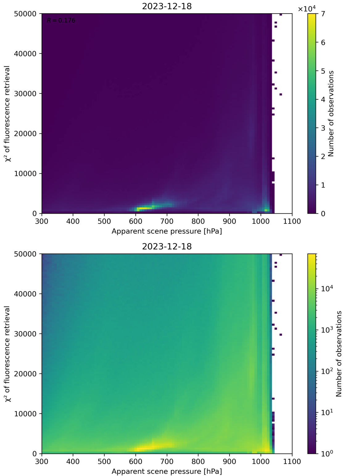
Figure 63: Scatter density plot of “Apparent scene pressure” against “ \chi^2 of fluorescence retrieval” for 2023-12-17 to 2023-12-19.
