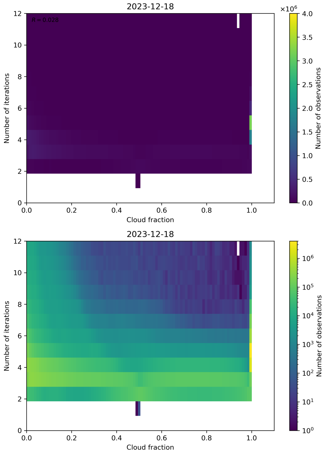
Figure 73: Scatter density plot of “Cloud fraction” against “Number of iterations” for 2023-12-17 to 2023-12-19.
