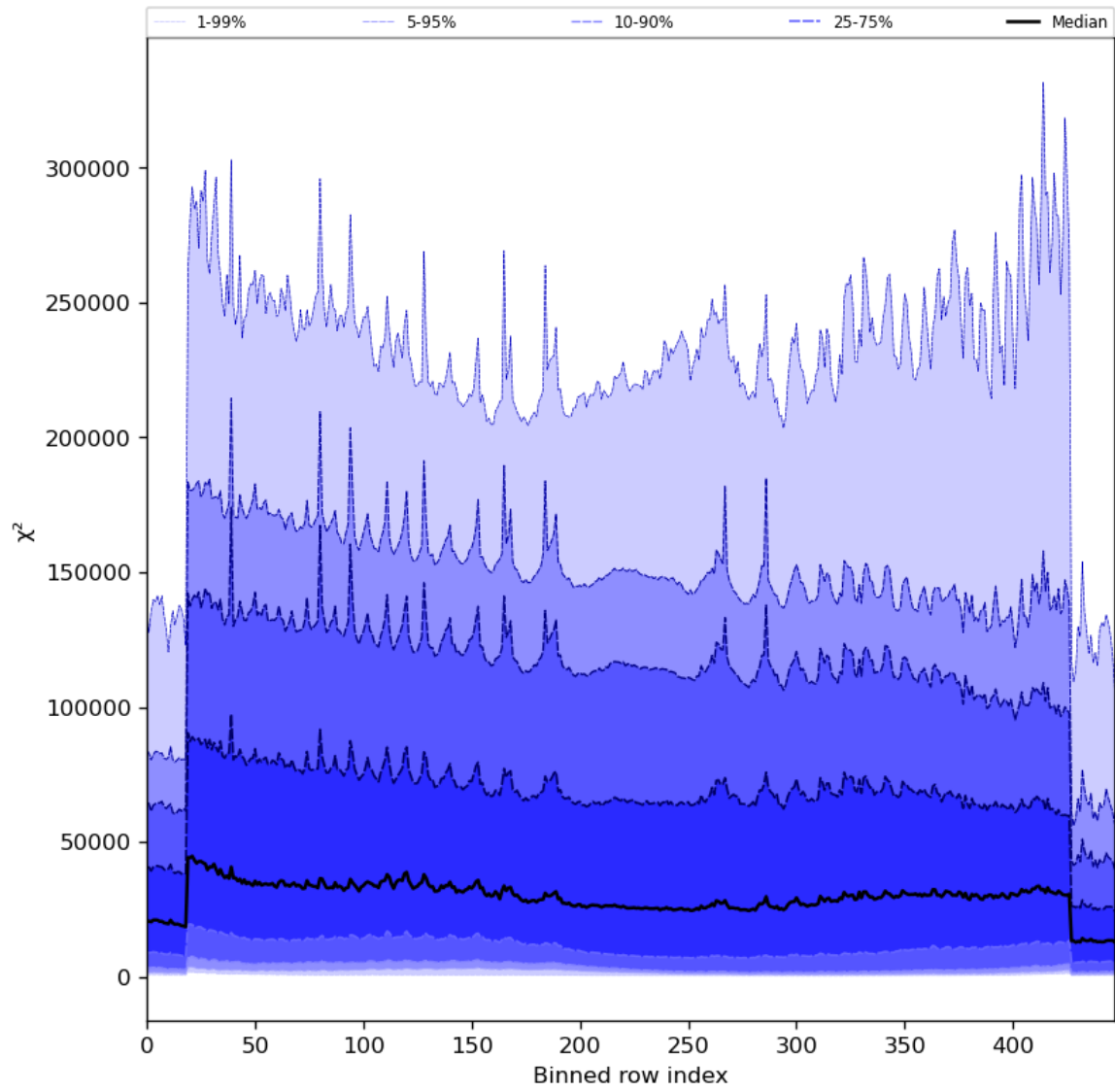
Figure 55: Along track statistics of “ \chi^2 ” for 2023-12-17 to 2023-12-19
