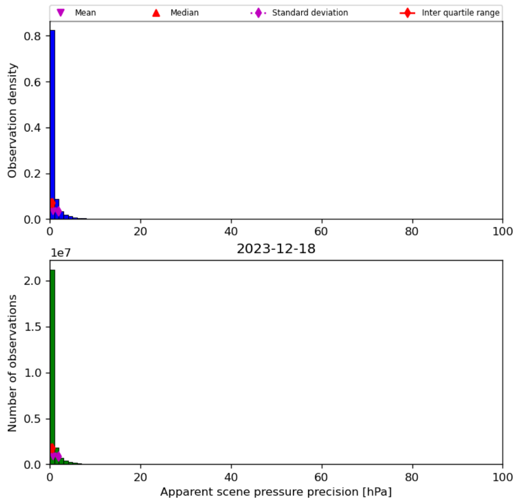
Figure 37: Histogram of “Apparent scene pressure precision” for 2023-12-17 to 2023-12-19
