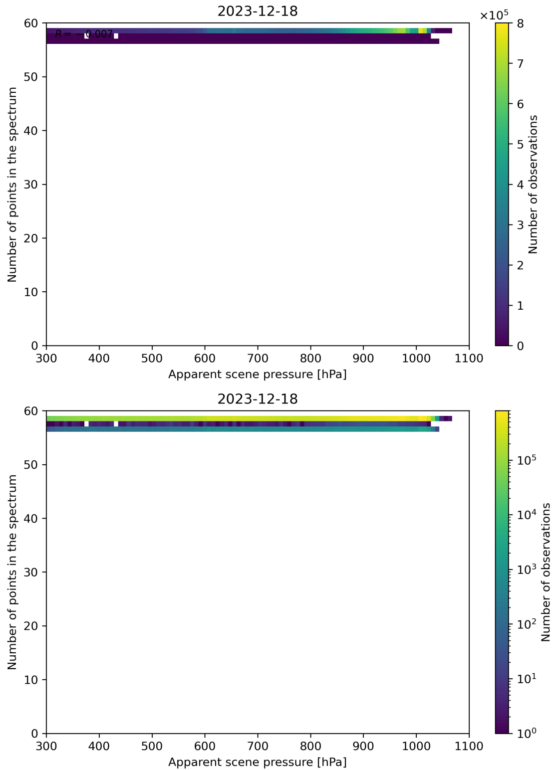
Figure 66: Scatter density plot of “Apparent scene pressure” against “Number of points in the spectrum” for 2023-12-17 to 2023-12-19.
