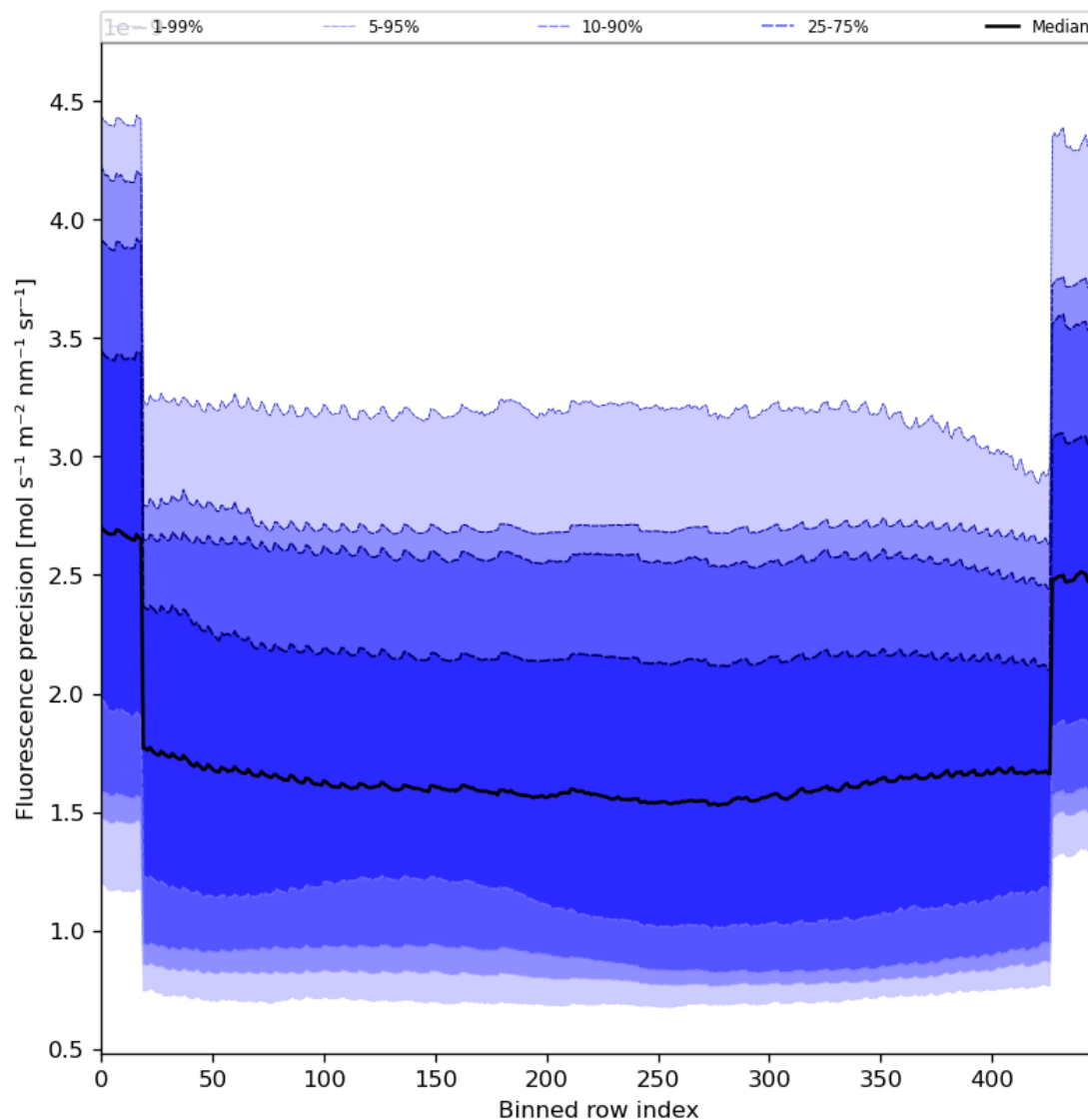
Figure 58: Along track statistics of “Fluorescence precision” for 2023-12-17 to 2023-12-19
