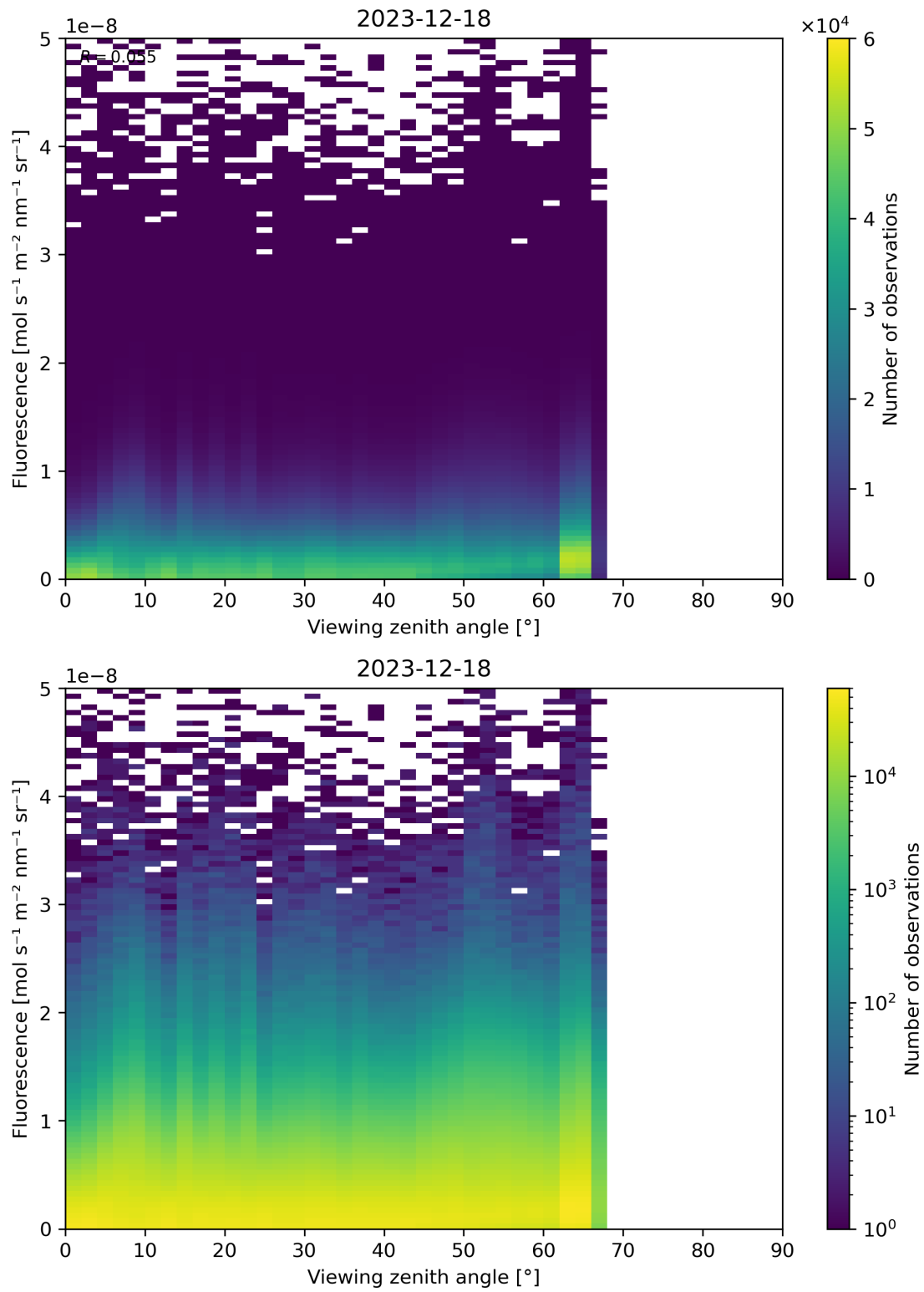
Figure 122: Scatter density plot of “Viewing zenith angle” against “Fluorescence” for 2023-12-17 to 2023-12-19.
