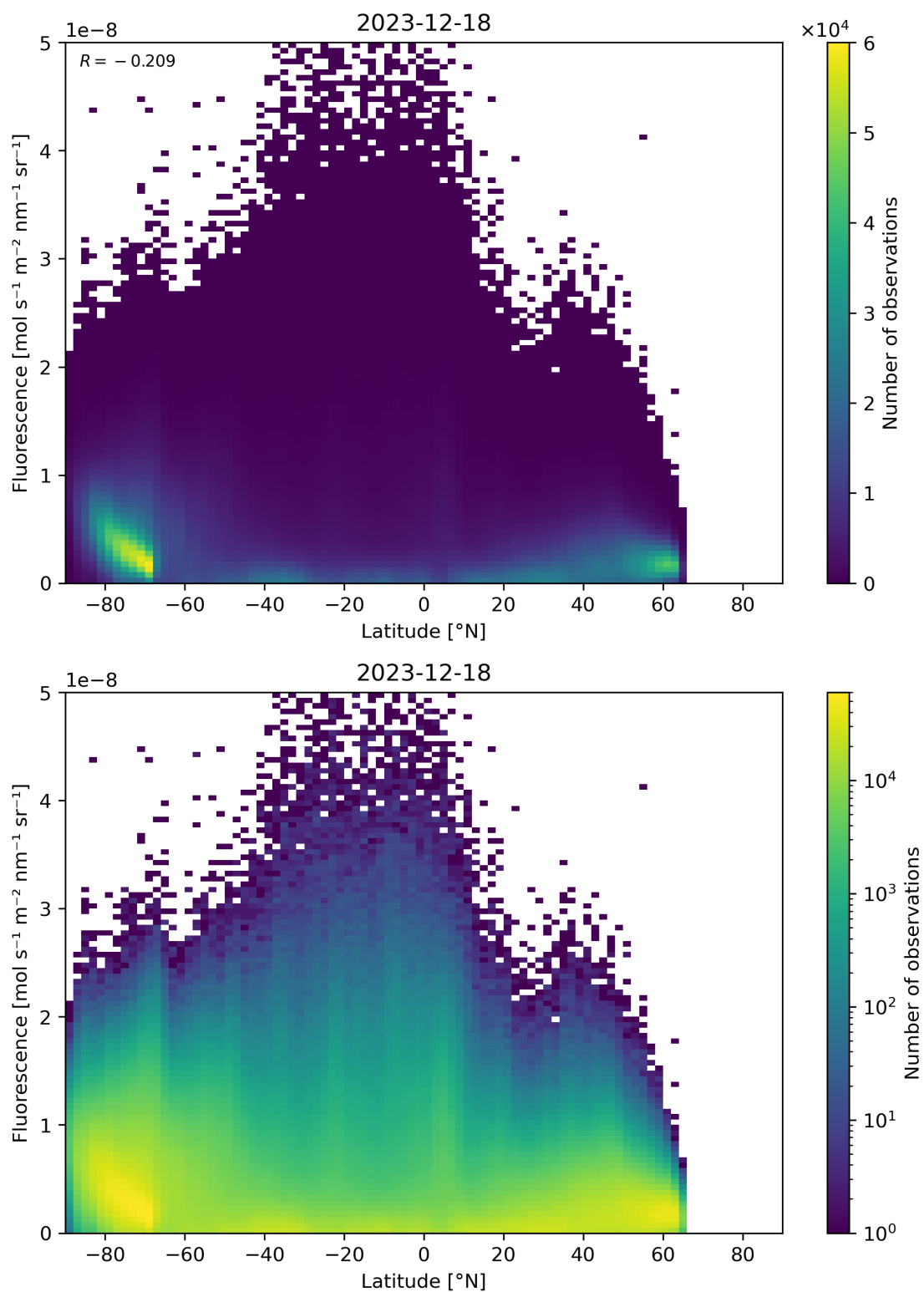
Figure 92: Scatter density plot of “Latitude” against “Fluorescence” for 2023-12-17 to 2023-12-19.
