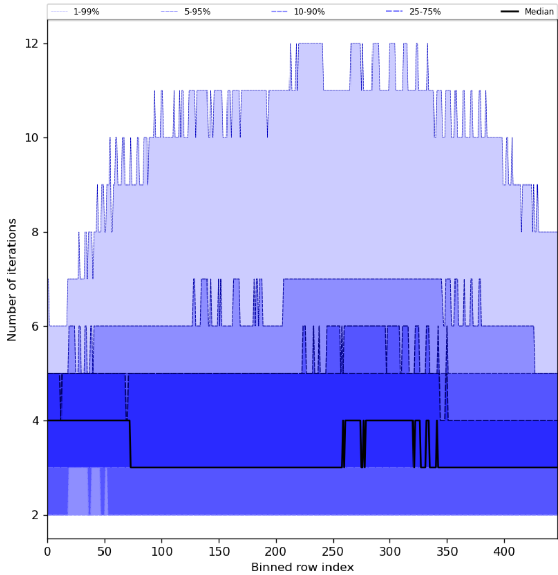
Figure 56: Along track statistics of “Number of iterations” for 2023-12-17 to 2023-12-19
