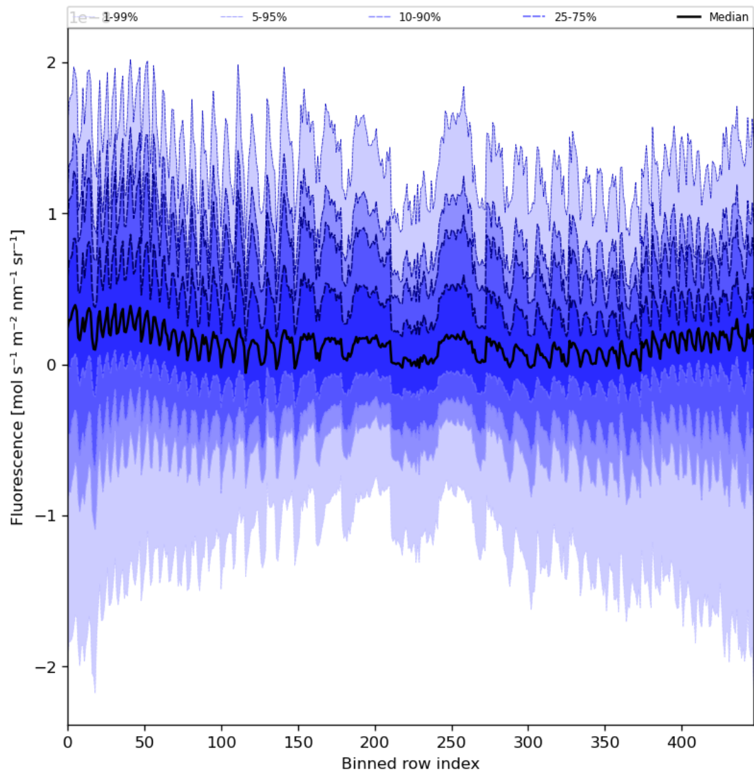
Figure 57: Along track statistics of “Fluorescence” for 2023-12-17 to 2023-12-19
