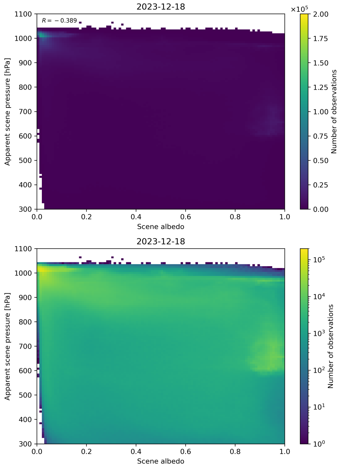
Figure 102: Scatter density plot of “Scene albedo” against “Apparent scene pressure” for 2023-12-17 to 2023-12-19.
