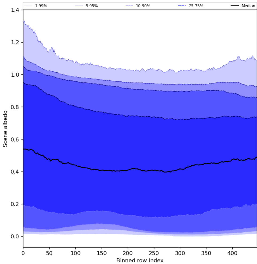
Figure 51: Along track statistics of “Scene albedo” for 2023-12-17 to 2023-12-19
