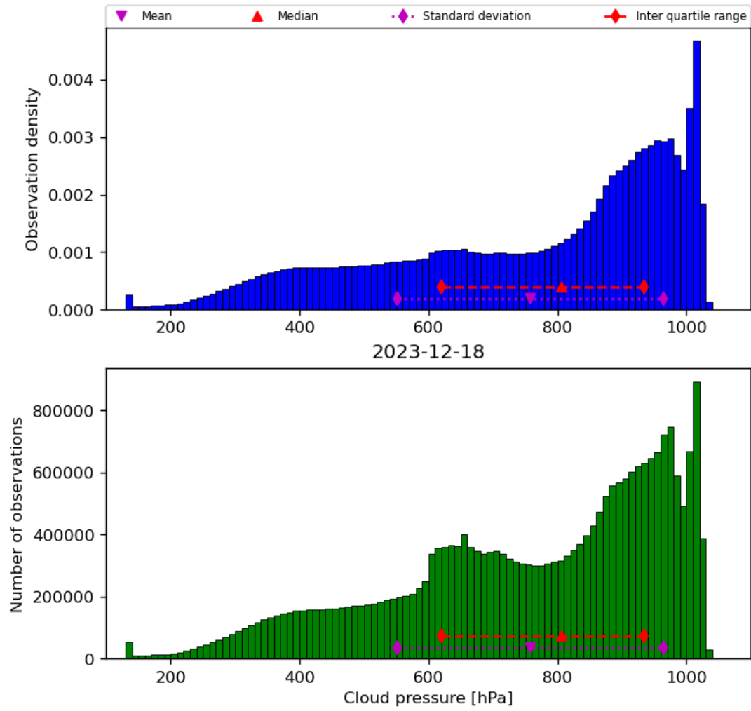
Figure 30: Histogram of “Cloud pressure” for 2023-12-17 to 2023-12-19
