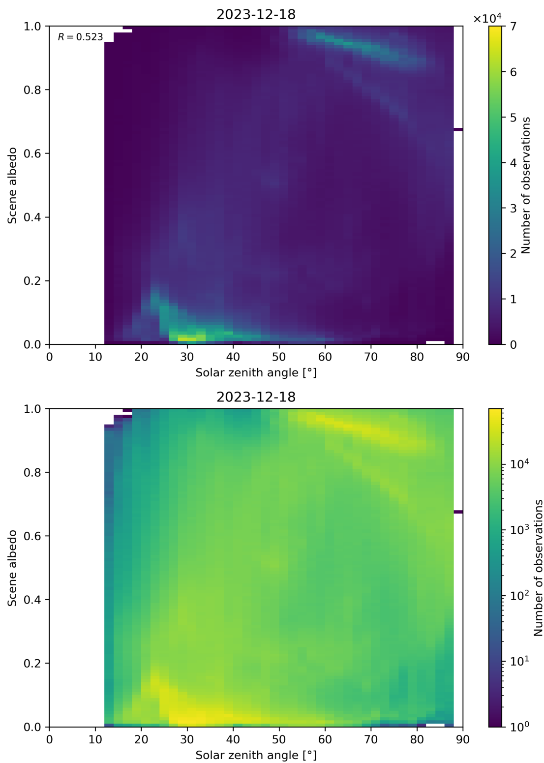
Figure 116: Scatter density plot of “Solar zenith angle” against “Scene albedo” for 2023-12-17 to 2023-12-19.
