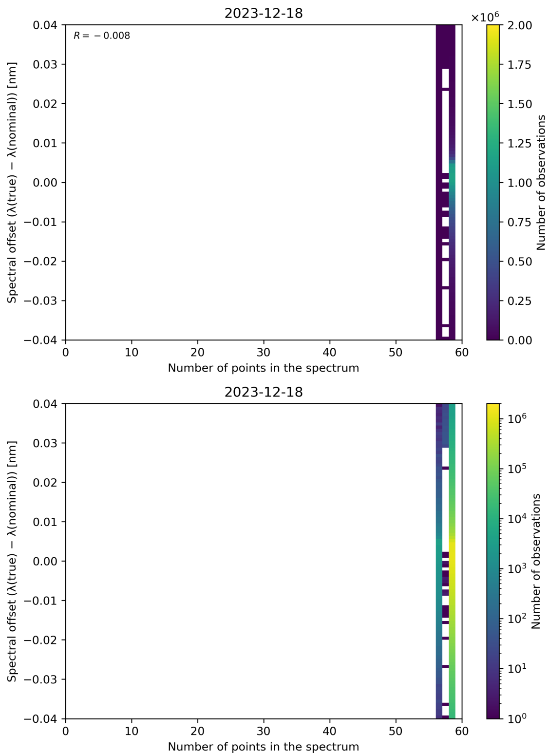
Figure 101: Scatter density plot of “Number of points in the spectrum” against “Spectral offset ( \lambda(\text{true}) - \lambda(\text{nominal}) )” for 2023-12-17 to 2023-12-19.
