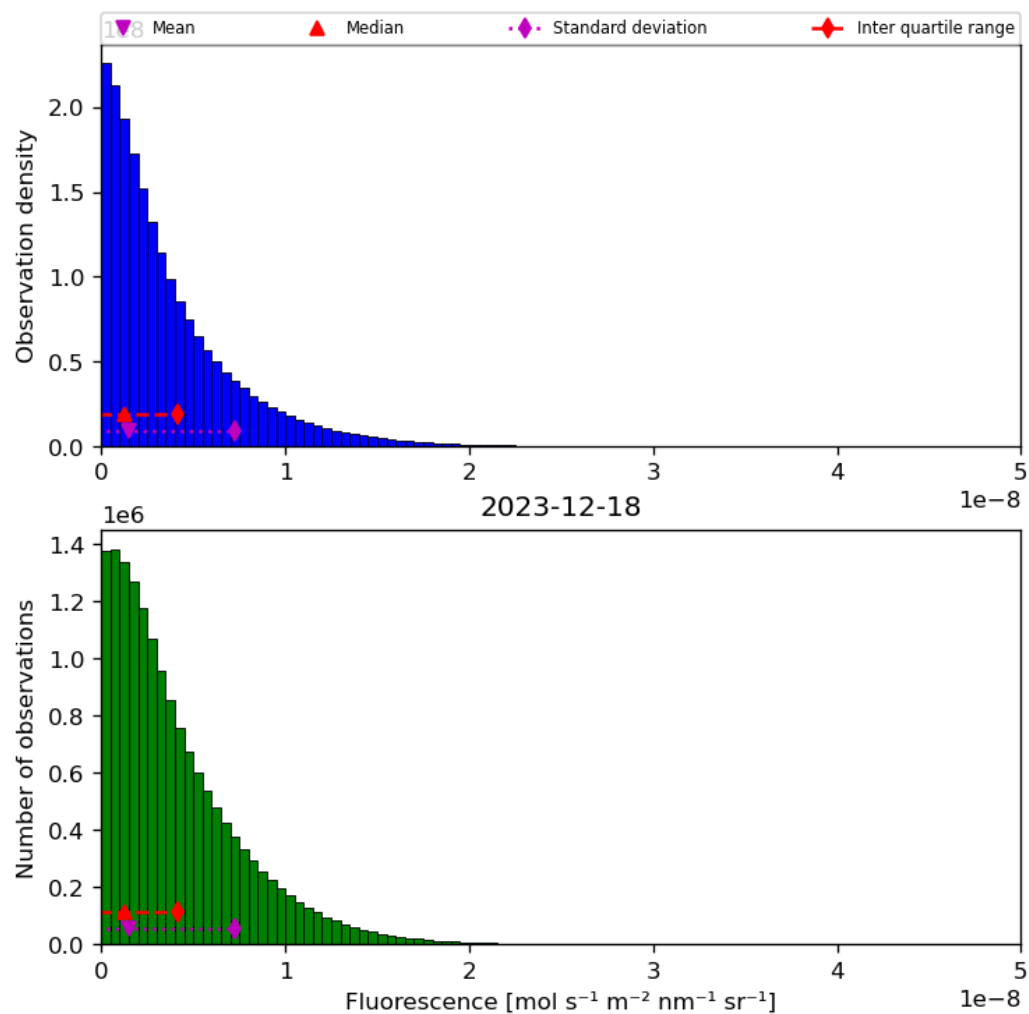
Figure 40: Histogram of “Fluorescence” for 2023-12-17 to 2023-12-19
