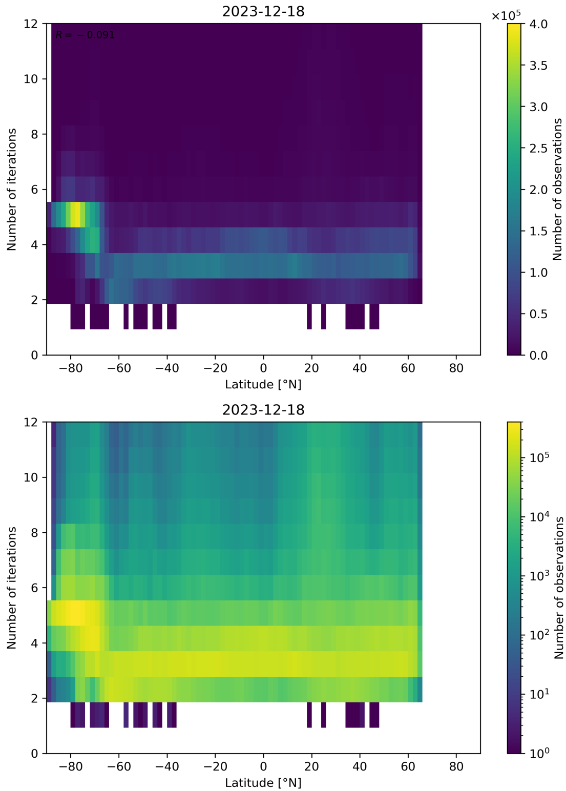
Figure 93: Scatter density plot of “Latitude” against “Number of iterations” for 2023-12-17 to 2023-12-19.
