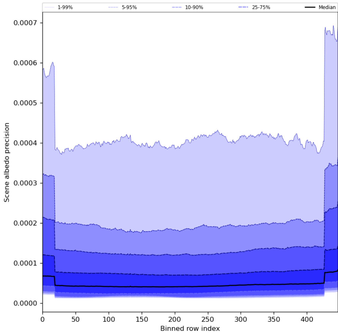
Figure 52: Along track statistics of “Scene albedo precision” for 2023-12-17 to 2023-12-19
