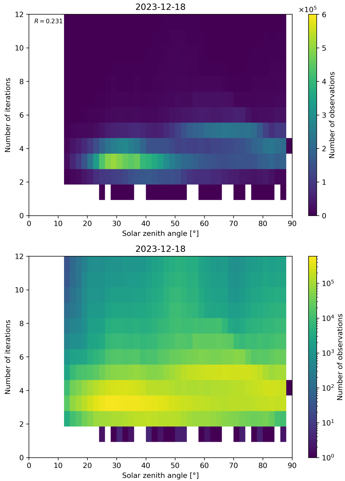
Figure 114: Scatter density plot of “Solar zenith angle” against “Number of iterations” for 2023-12-17 to 2023-12-19.
