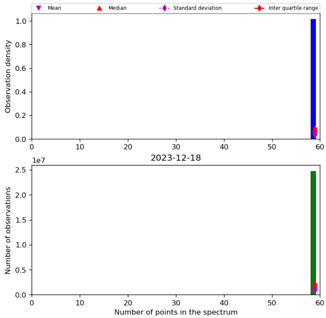
Figure 44: Histogram of “Number of points in the spectrum” for 2023-12-17 to 2023-12-19
