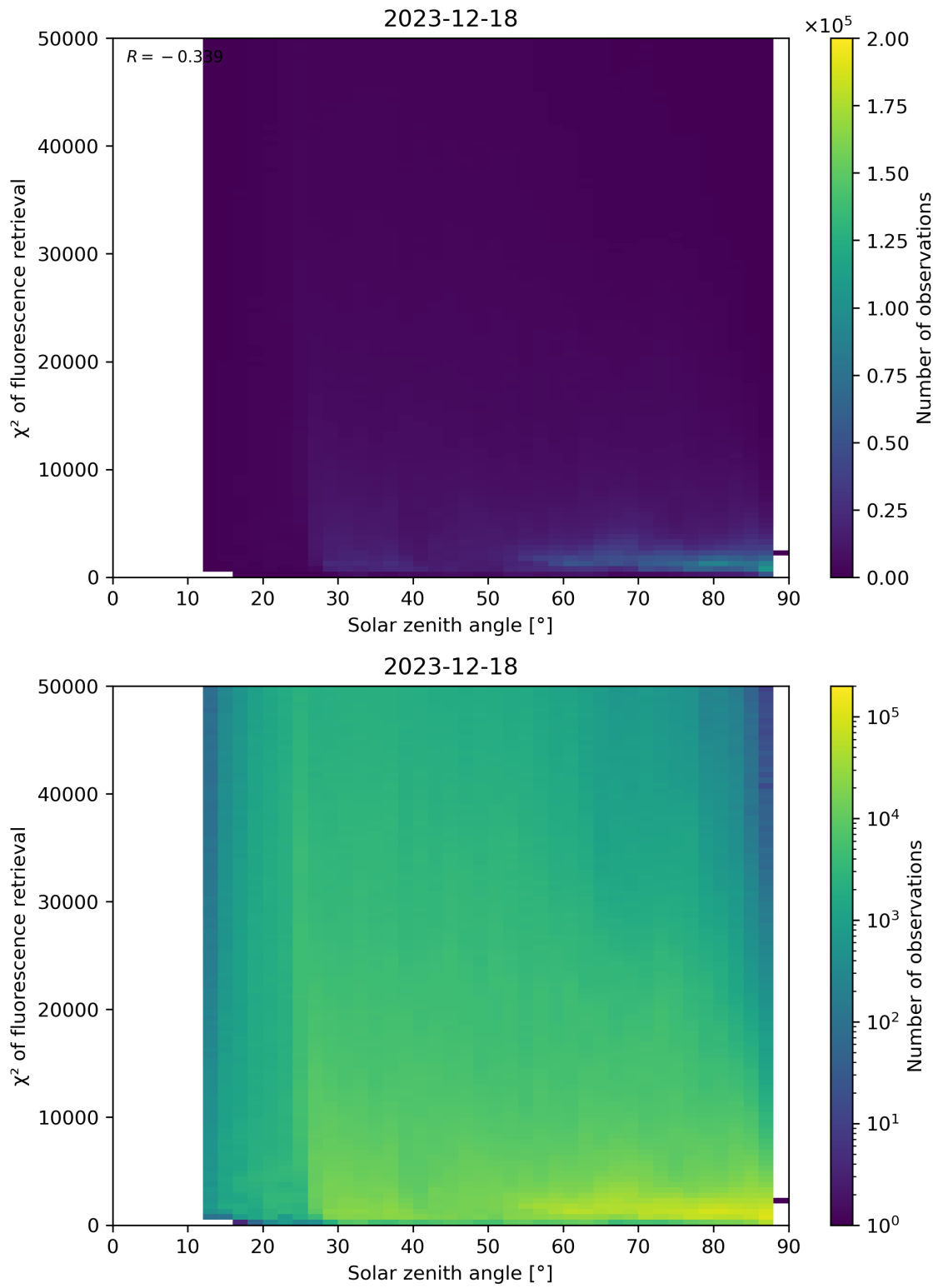
Figure 109: Scatter density plot of “Solar zenith angle” against “ \chi^2 of fluorescence retrieval” for 2023-12-17 to 2023-12-19.
