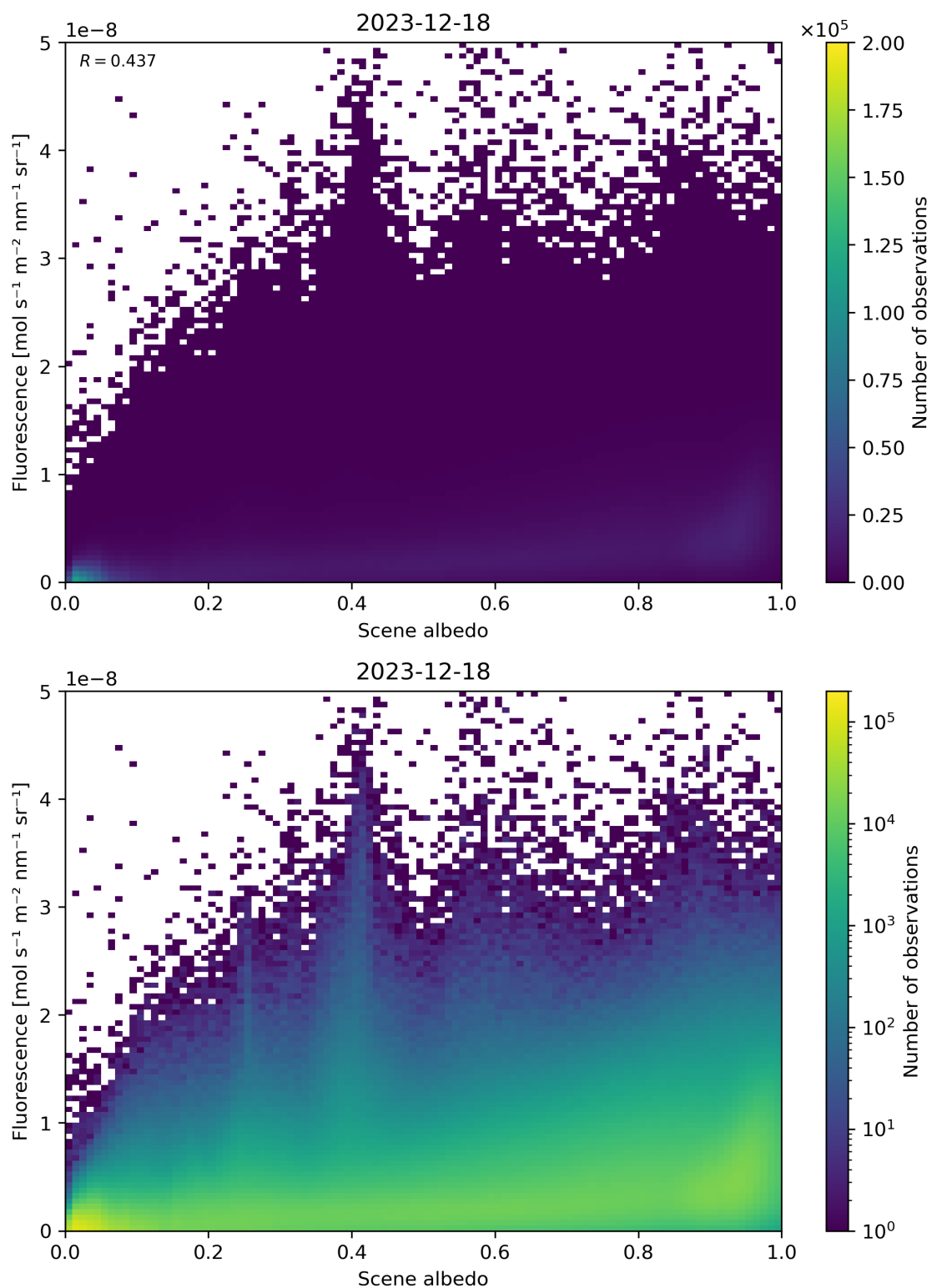
Figure 104: Scatter density plot of “Scene albedo” against “Fluorescence” for 2023-12-17 to 2023-12-19.
