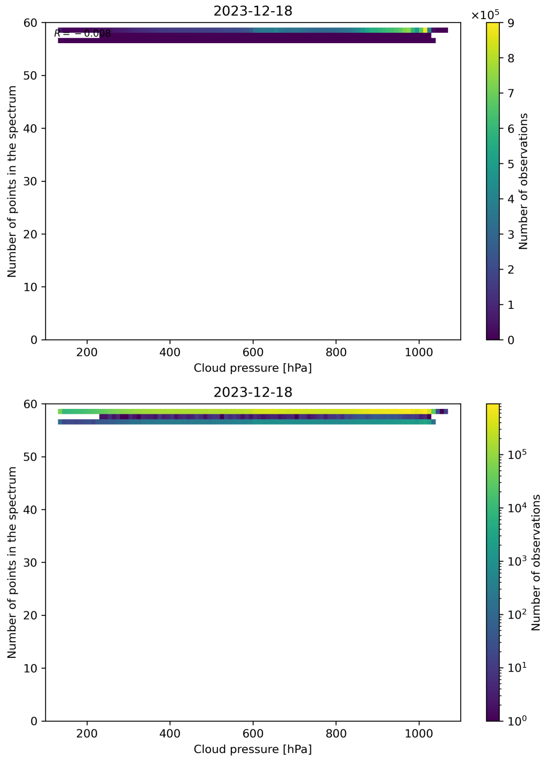
Figure 82: Scatter density plot of “Cloud pressure” against “Number of points in the spectrum” for 2023-12-17 to 2023-12-19.
