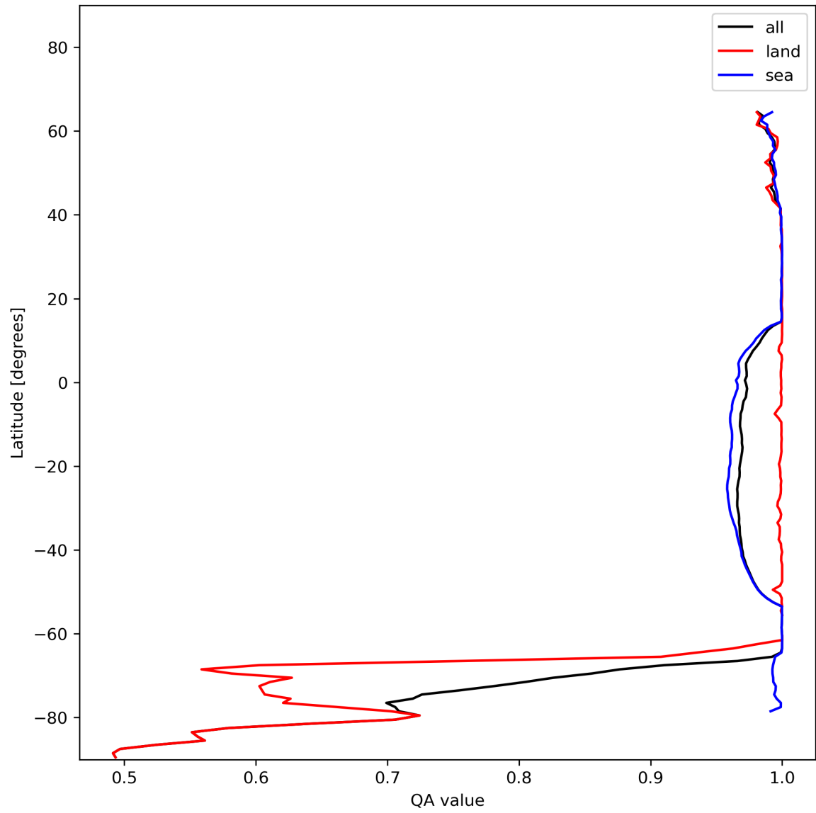
Figure 12: Zonal average of “QA value” for 2023-12-17 to 2023-12-19.
