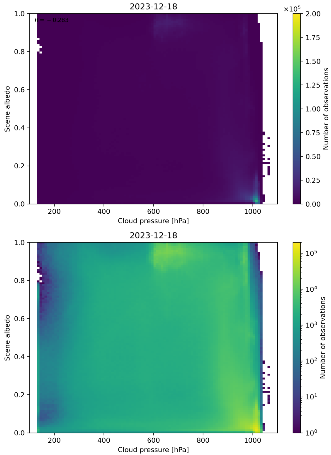
Figure 83: Scatter density plot of “Cloud pressure” against “Scene albedo” for 2023-12-17 to 2023-12-19.
