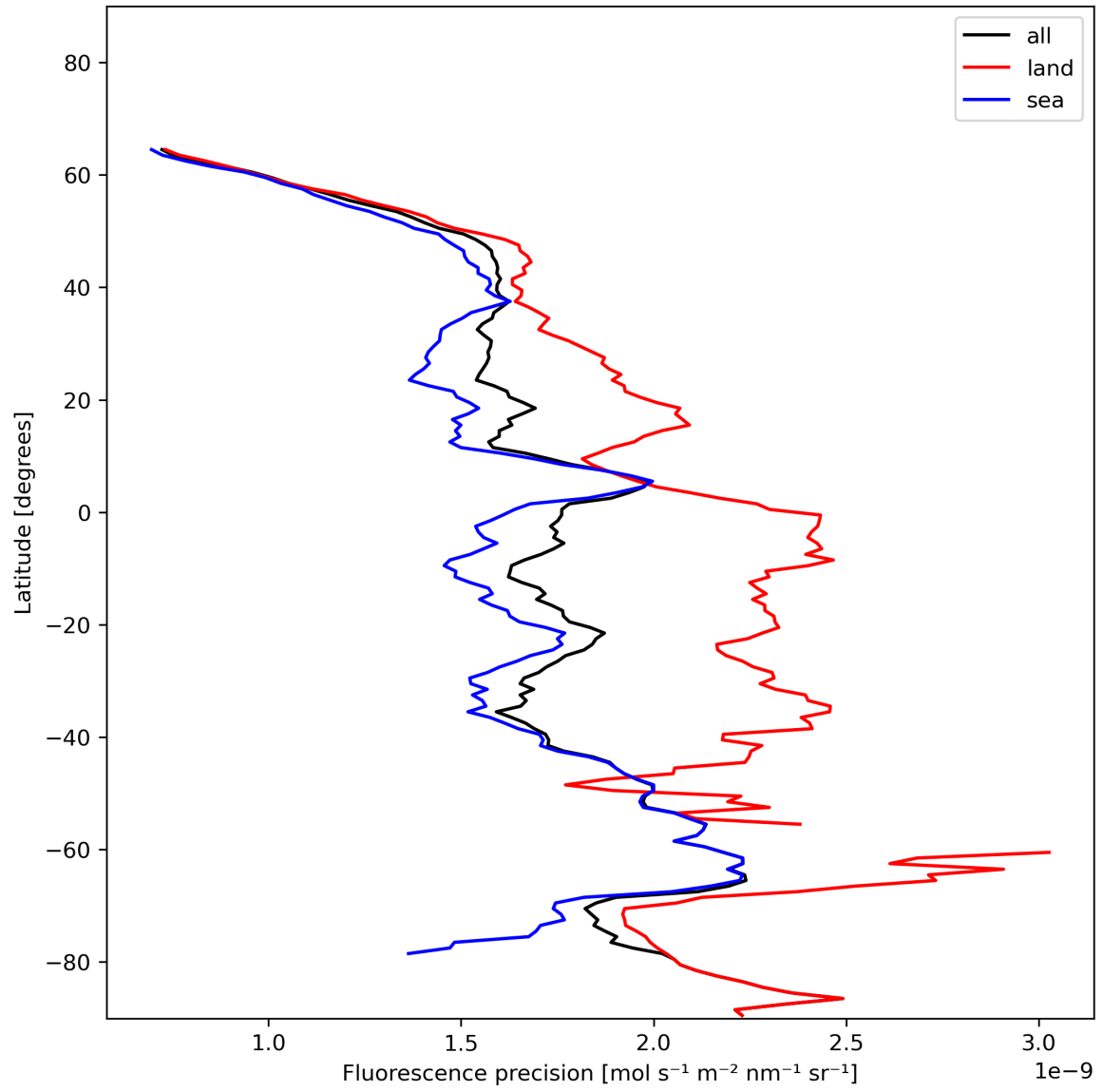
Figure 24: Zonal average of “Fluorescence precision” for 2023-12-17 to 2023-12-19.
