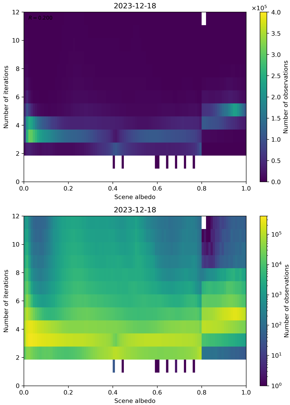
Figure 105: Scatter density plot of “Scene albedo” against “Number of iterations” for 2023-12-17 to 2023-12-19.
