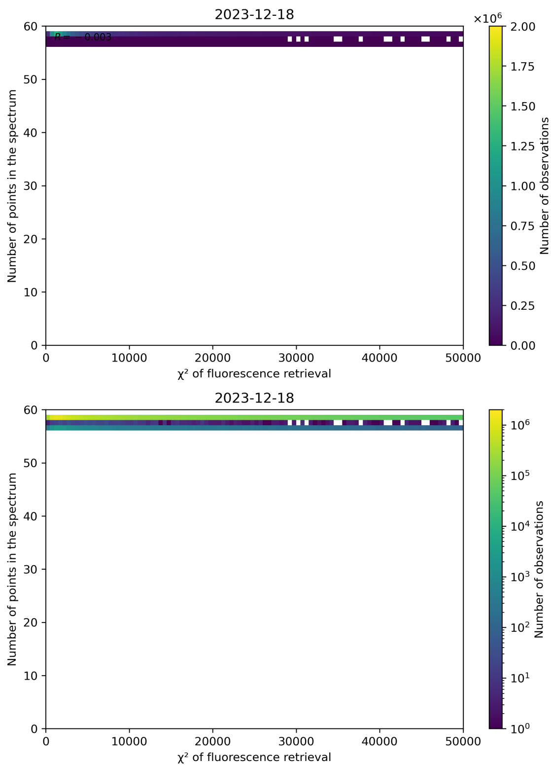
Figure 68: Scatter density plot of " \chi^2 of fluorescence retrieval" against "Number of points in the spectrum" for 2023-12-17 to 2023-12-19.
