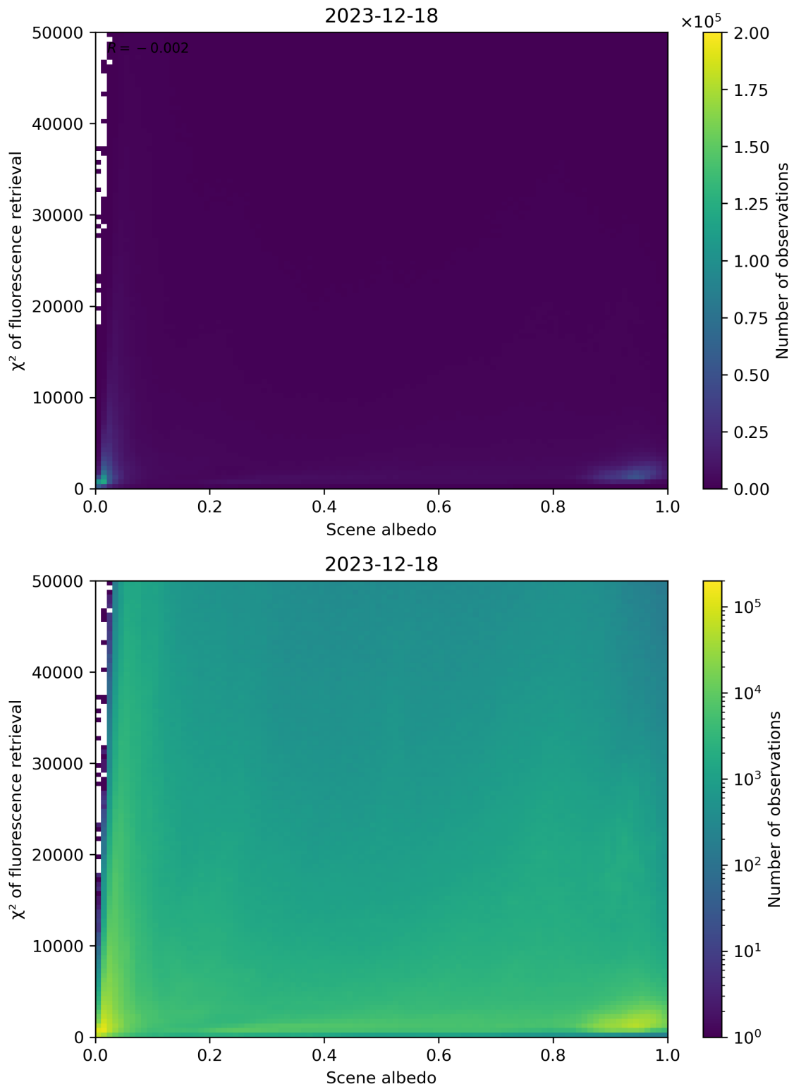
Figure 103: Scatter density plot of “Scene albedo” against “ \chi^2 of fluorescence retrieval” for 2023-12-17 to 2023-12-19.
