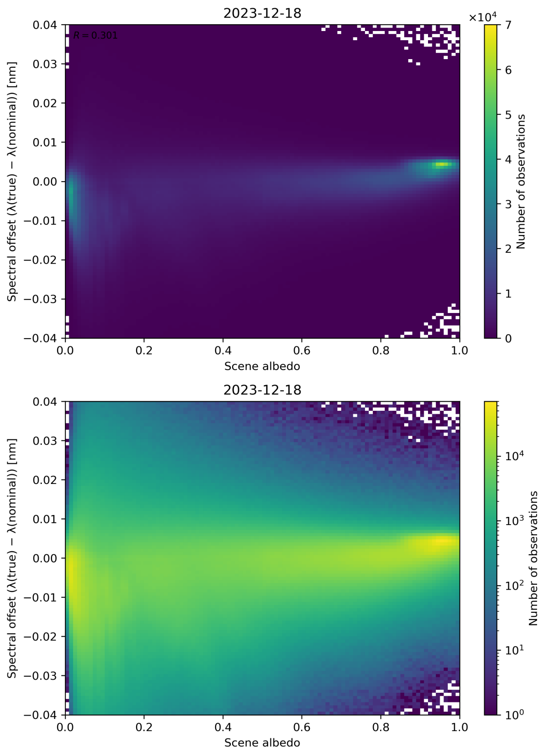
Figure 107: Scatter density plot of “Scene albedo” against “Spectral offset ( \lambda(\text{true}) - \lambda(\text{nominal}) )” for 2023-12-17 to 2023-12-19.
