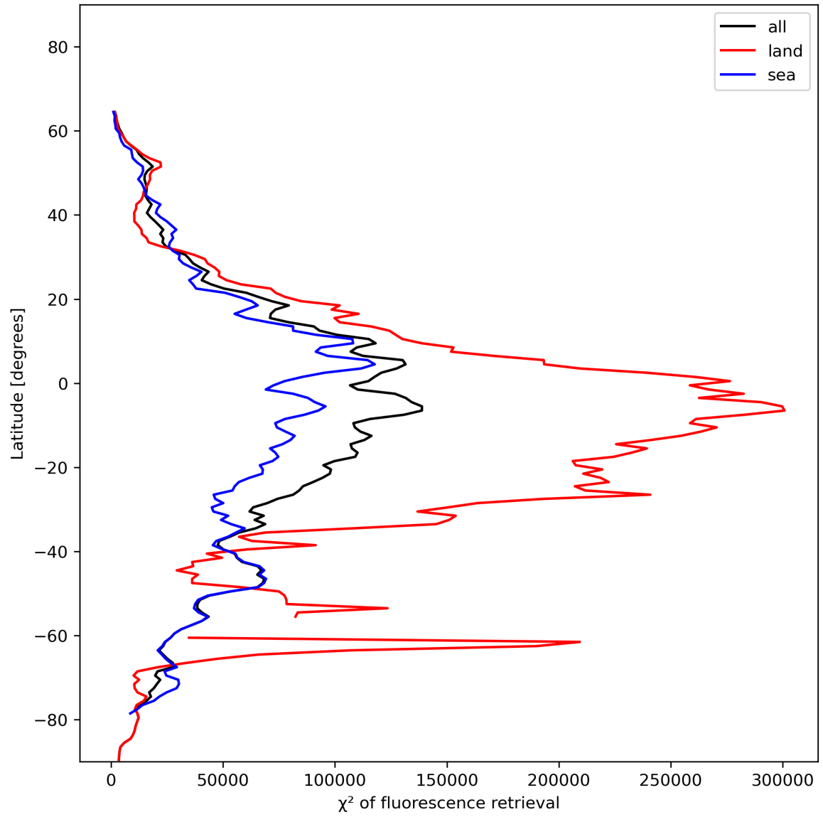
Figure 25: Zonal average of “ \chi^2 of fluorescence retrieval” for 2023-12-17 to 2023-12-19.
