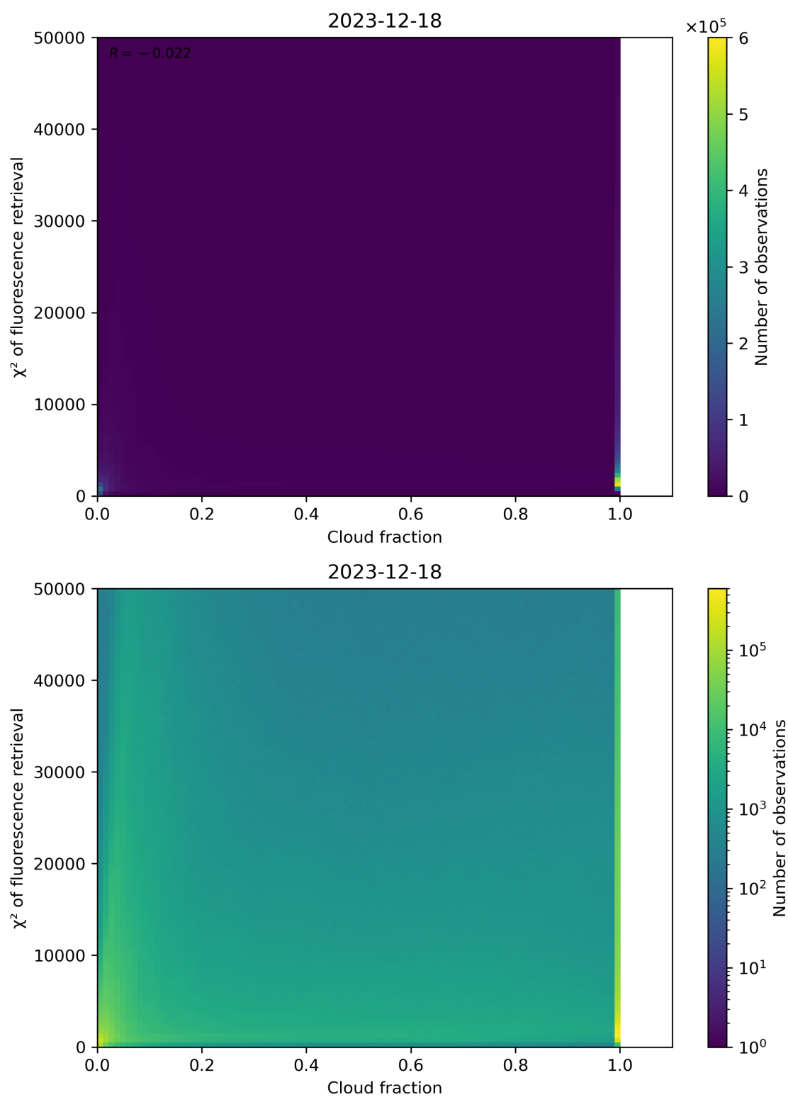
Figure 71: Scatter density plot of “Cloud fraction” against “ \chi^2 of fluorescence retrieval” for 2023-12-17 to 2023-12-19.
