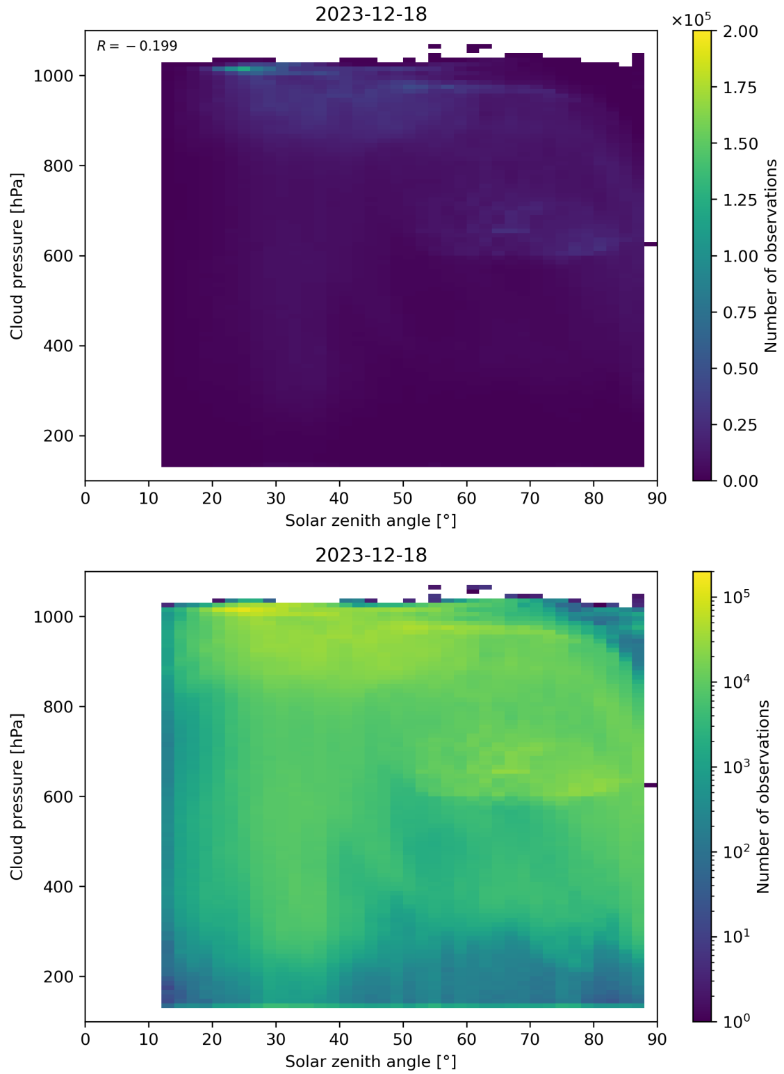
Figure 111: Scatter density plot of “Solar zenith angle” against “Cloud pressure” for 2023-12-17 to 2023-12-19.
