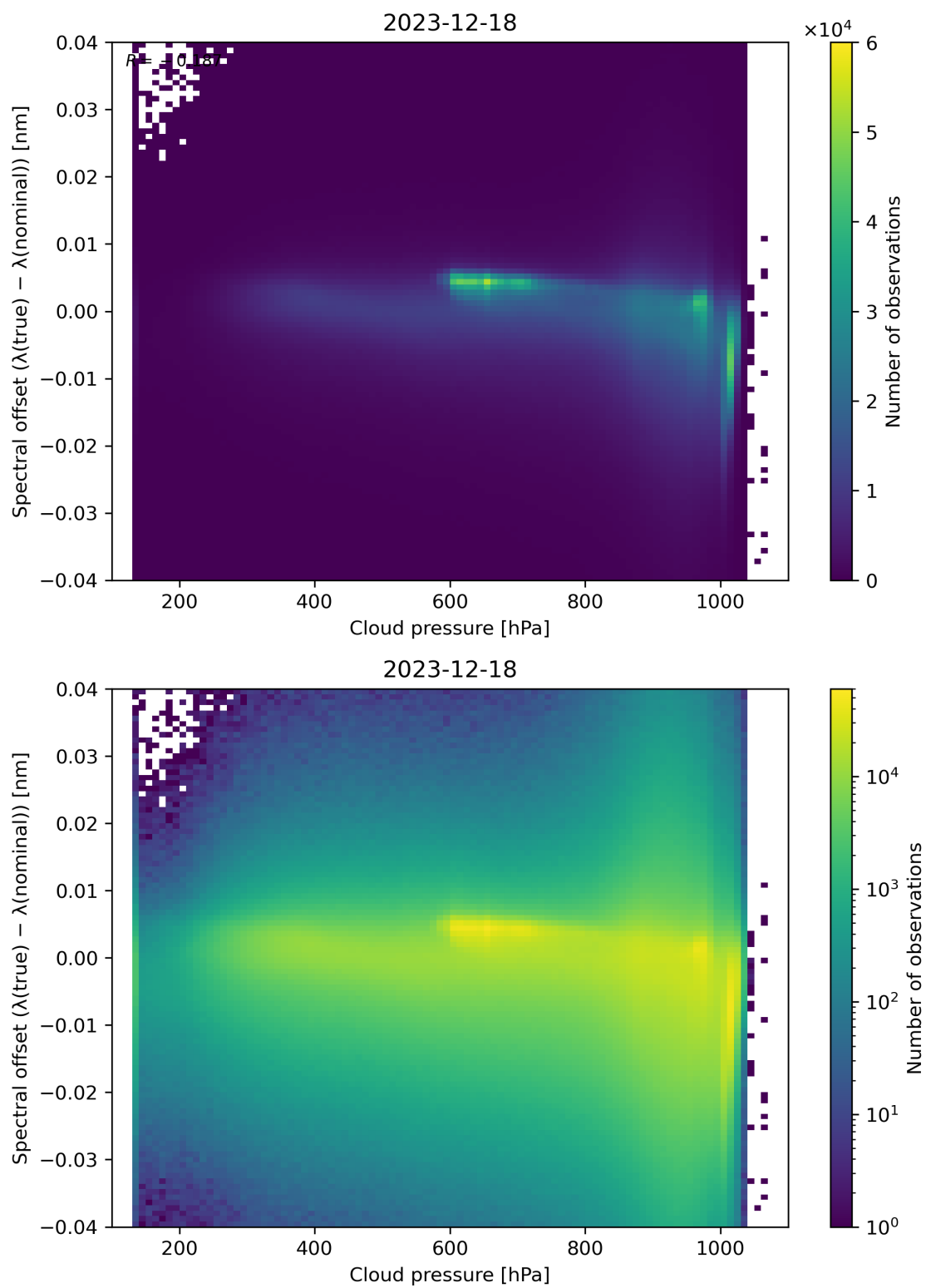
Figure 84: Scatter density plot of “Cloud pressure” against “Spectral offset ( \lambda(\text{true}) - \lambda(\text{nominal}) )” for 2023-12-17 to 2023-12-19.
