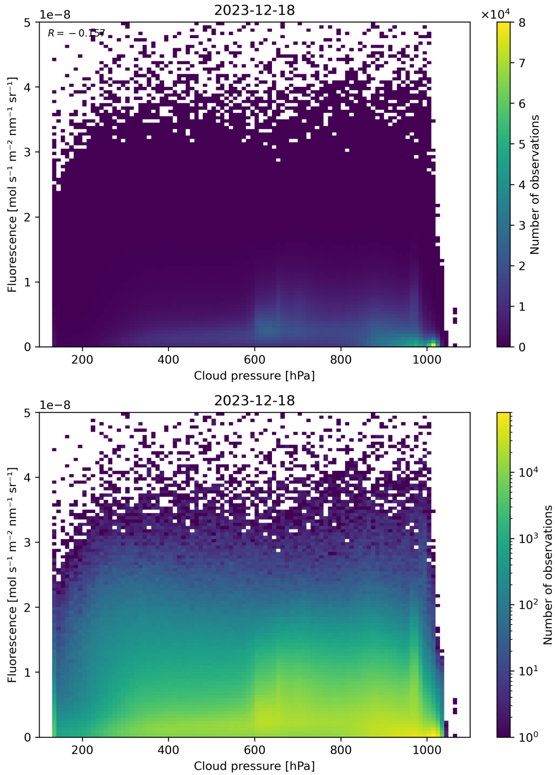
Figure 80: Scatter density plot of “Cloud pressure” against “Fluorescence” for 2023-12-17 to 2023-12-19.
