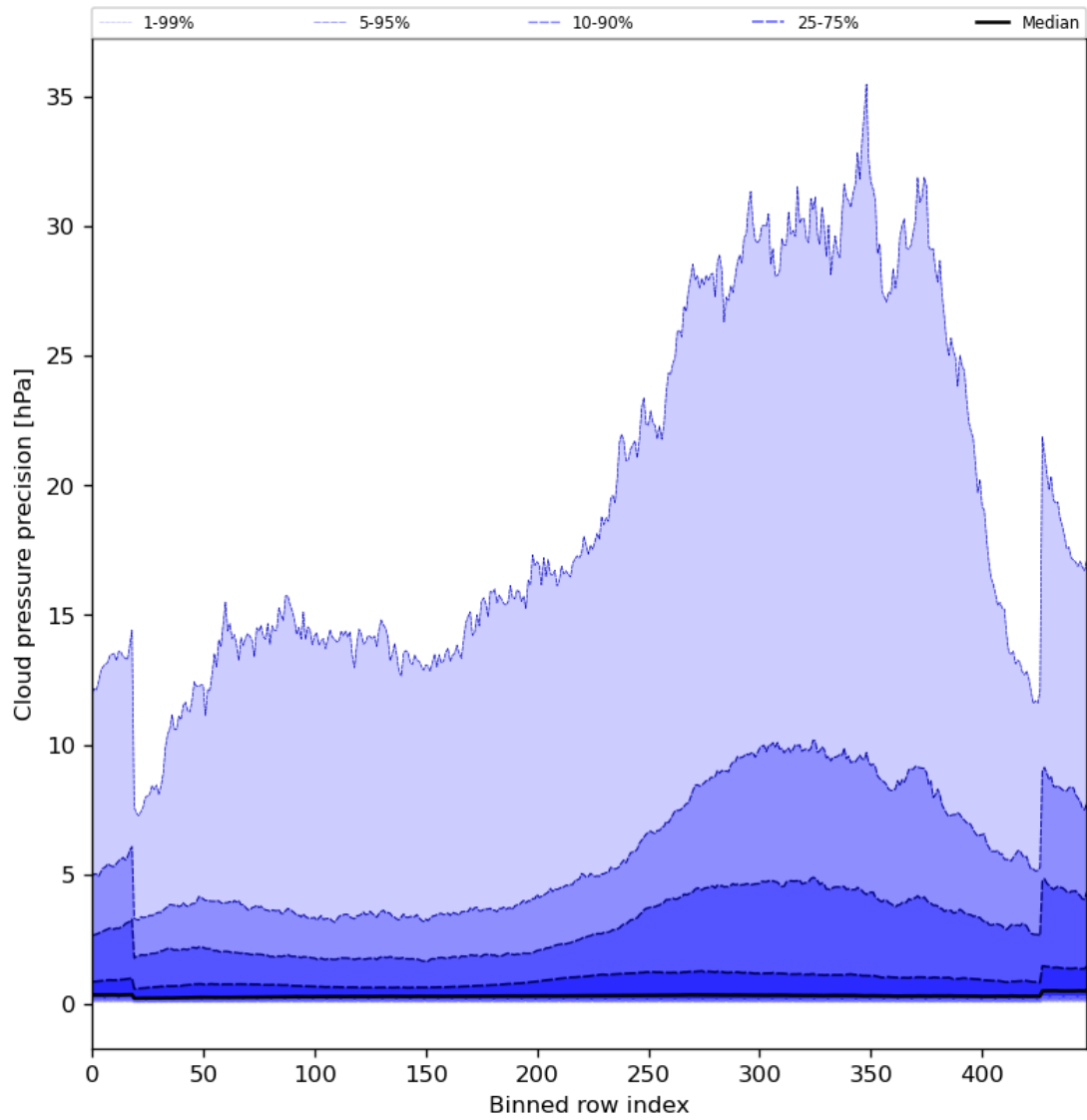
Figure 48: Along track statistics of “Cloud pressure precision” for 2023-12-17 to 2023-12-19
