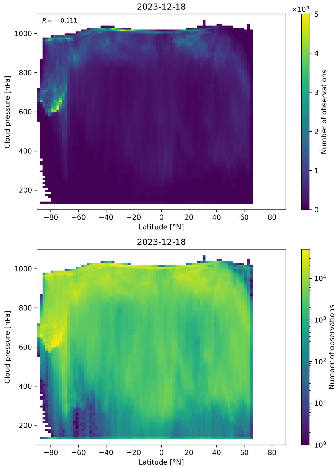
Figure 91: Scatter density plot of “Latitude” against “Cloud pressure” for 2023-12-17 to 2023-12-19.
