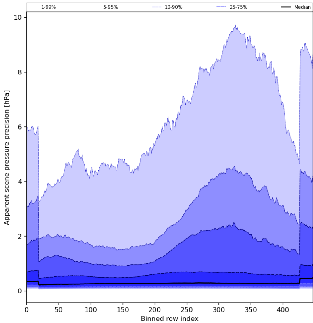
Figure 54: Along track statistics of “Apparent scene pressure precision” for 2023-12-17 to 2023-12-19
