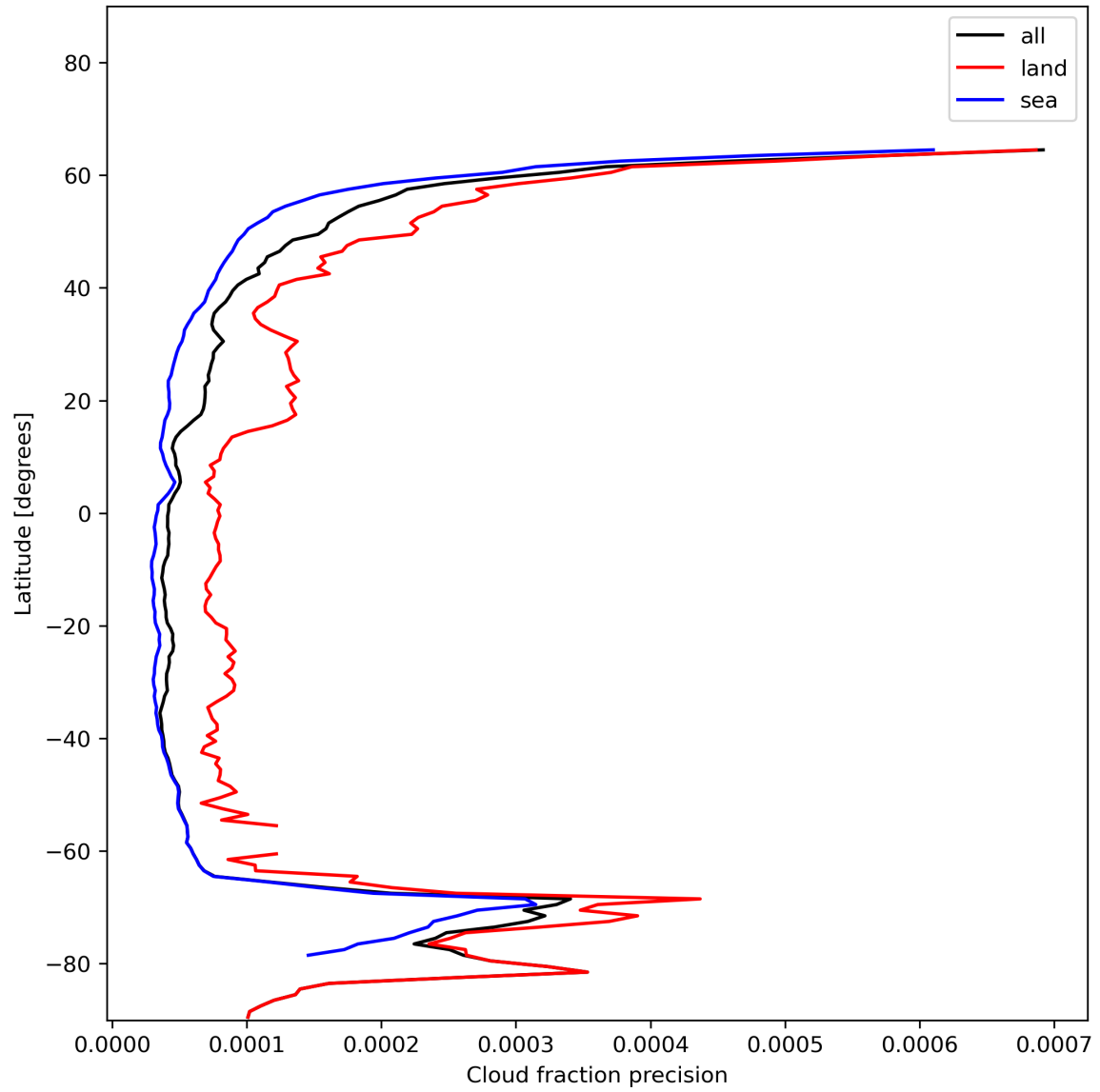
Figure 16: Zonal average of “Cloud fraction precision” for 2023-12-17 to 2023-12-19.
