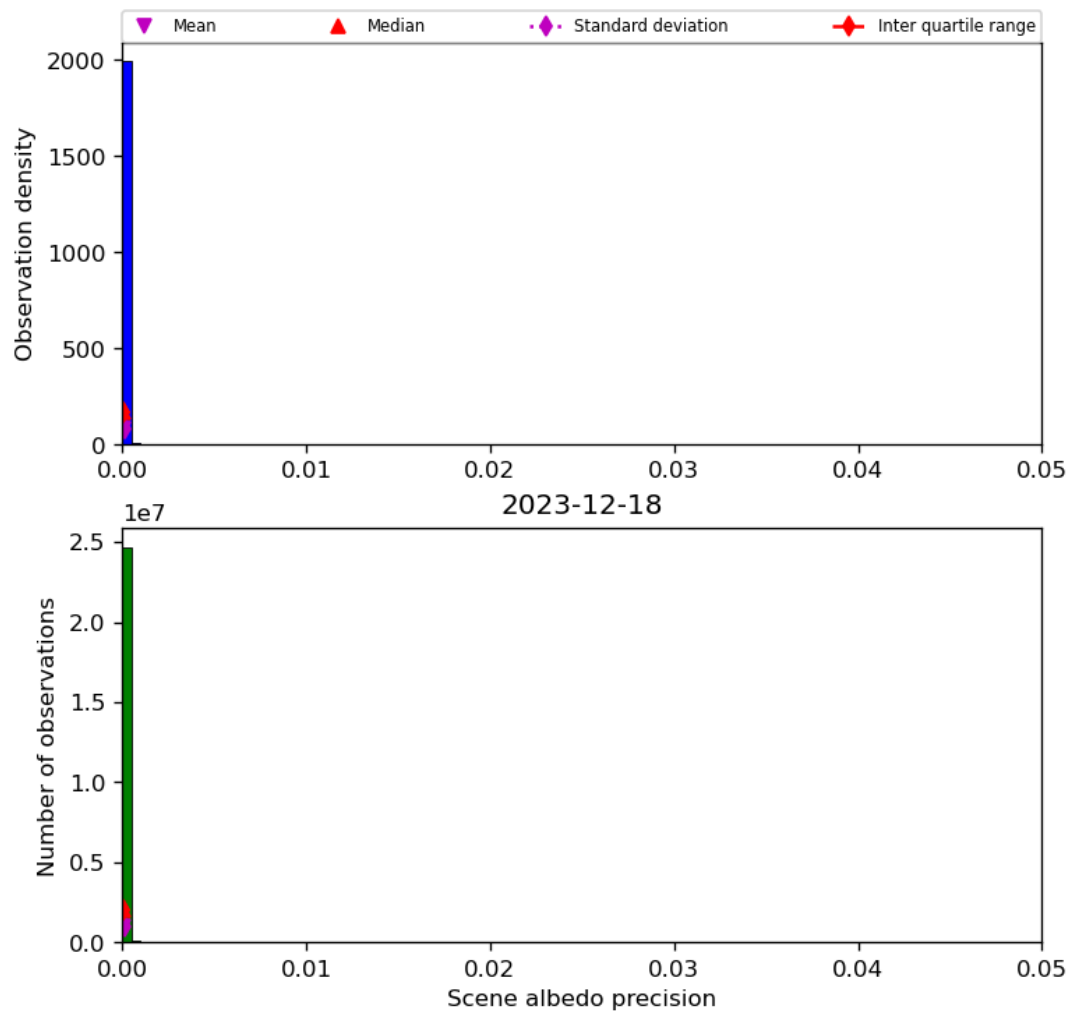
Figure 35: Histogram of “Scene albedo precision” for 2023-12-17 to 2023-12-19
