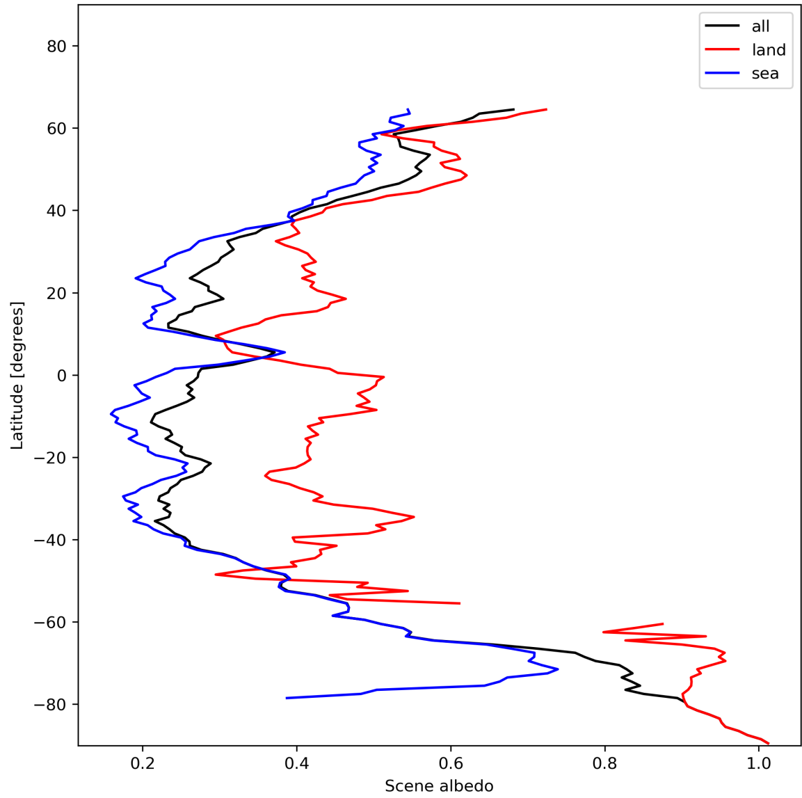
Figure 17: Zonal average of “Scene albedo” for 2023-12-17 to 2023-12-19.
