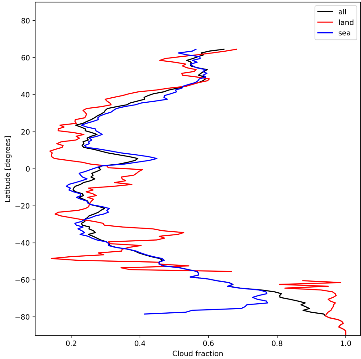
Figure 15: Zonal average of “Cloud fraction” for 2023-12-17 to 2023-12-19.
