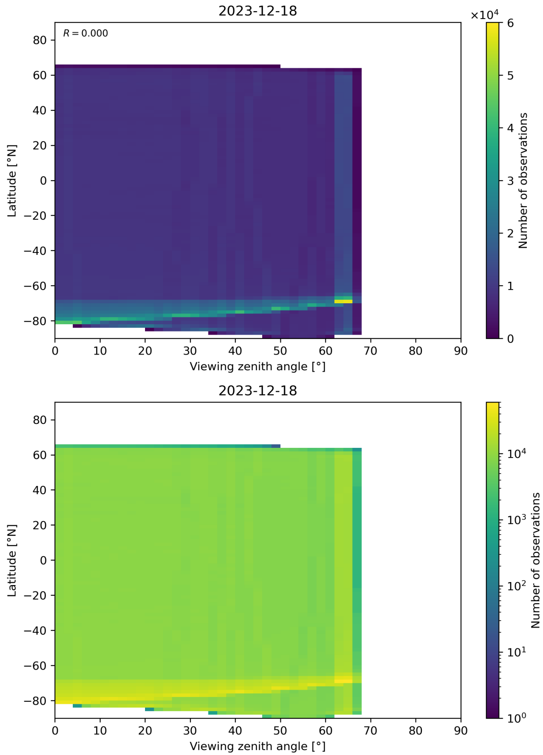
Figure 123: Scatter density plot of “Viewing zenith angle” against “Latitude” for 2023-12-17 to 2023-12-19.
