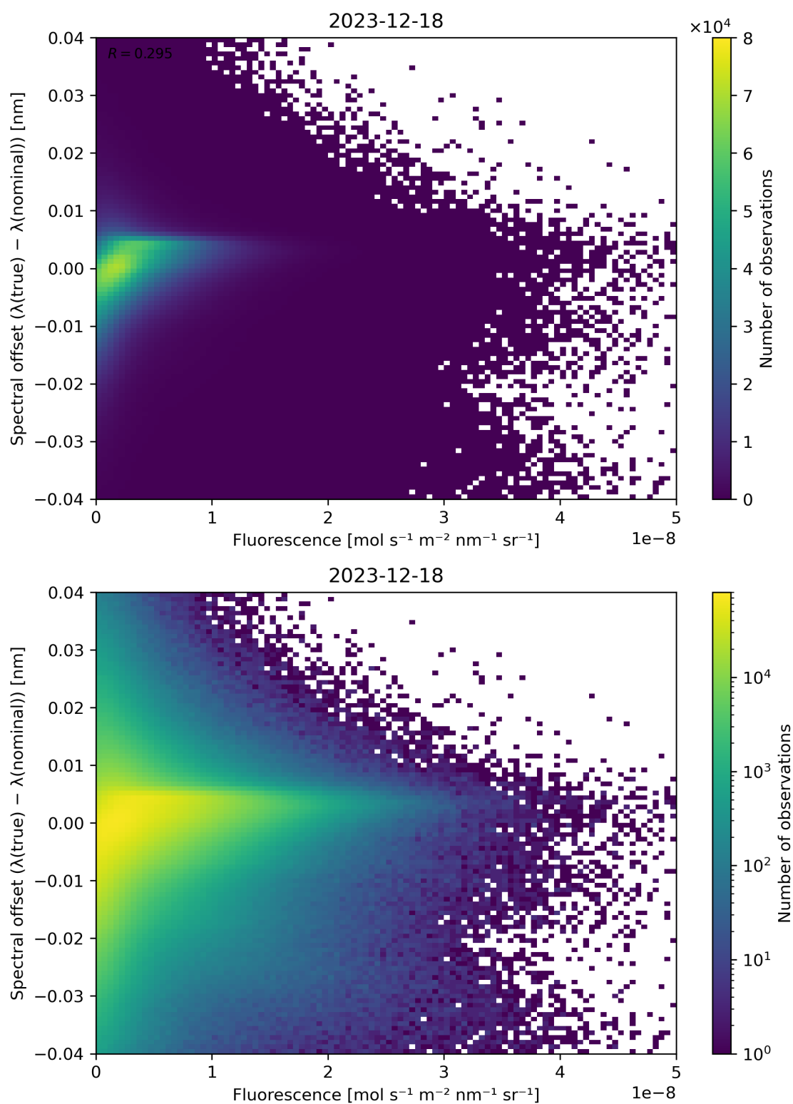
Figure 87: Scatter density plot of “Fluorescence” against “Spectral offset ( \lambda(\text{true}) - \lambda(\text{nominal}) )” for 2023-12-17 to 2023-12-19.
