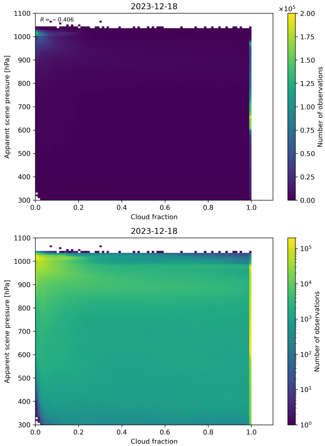
Figure 70: Scatter density plot of “Cloud fraction” against “Apparent scene pressure” for 2023-12-17 to 2023-12-19.
