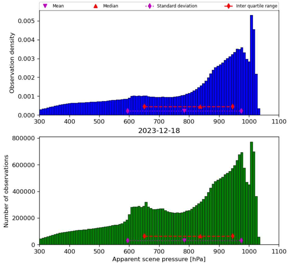
Figure 36: Histogram of “Apparent scene pressure” for 2023-12-17 to 2023-12-19
