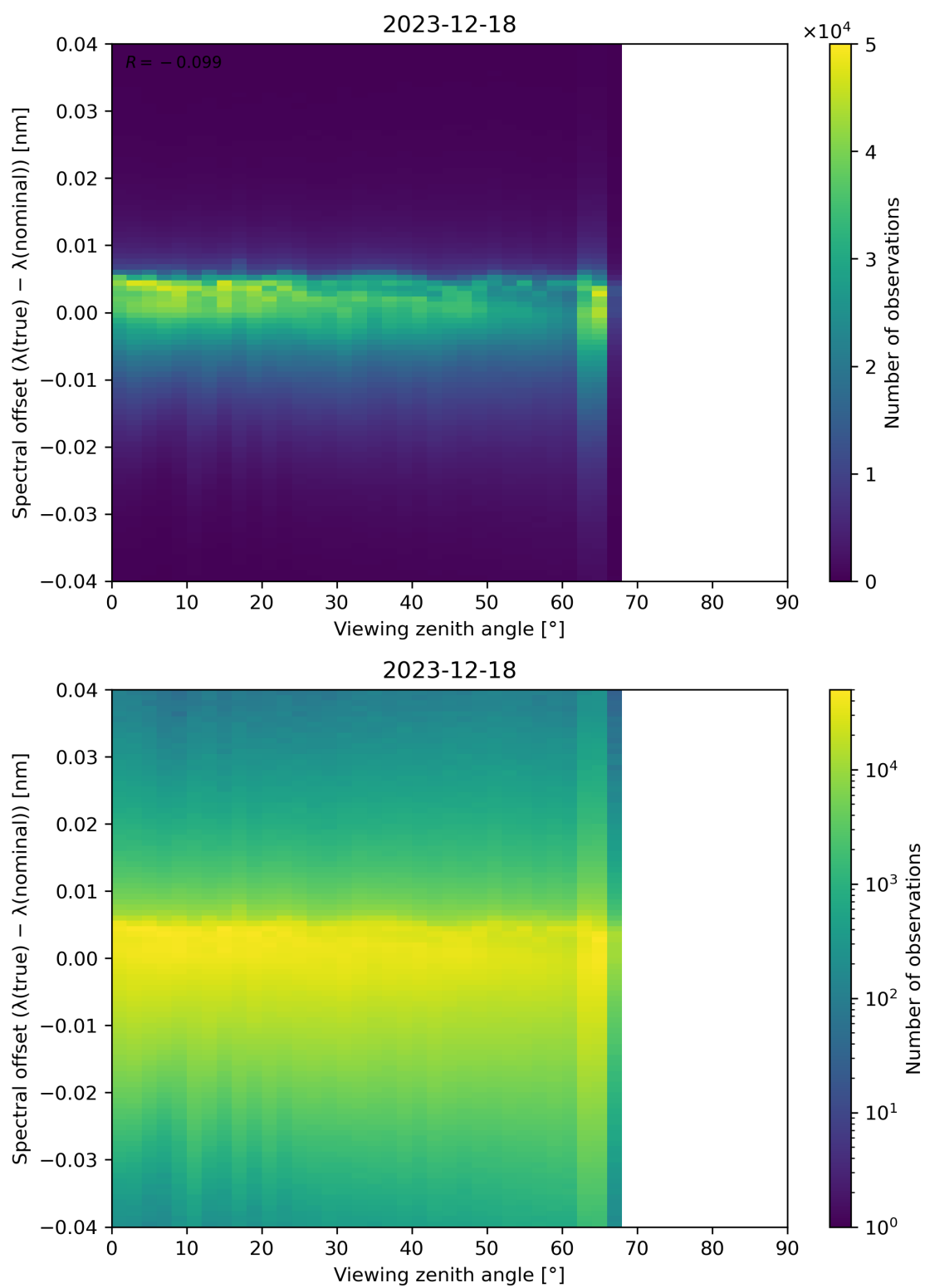
Figure 128: Scatter density plot of “Viewing zenith angle” against “Spectral offset ( \lambda(\text{true}) - \lambda(\text{nominal}) )” for 2023-12-17 to 2023-12-19.
