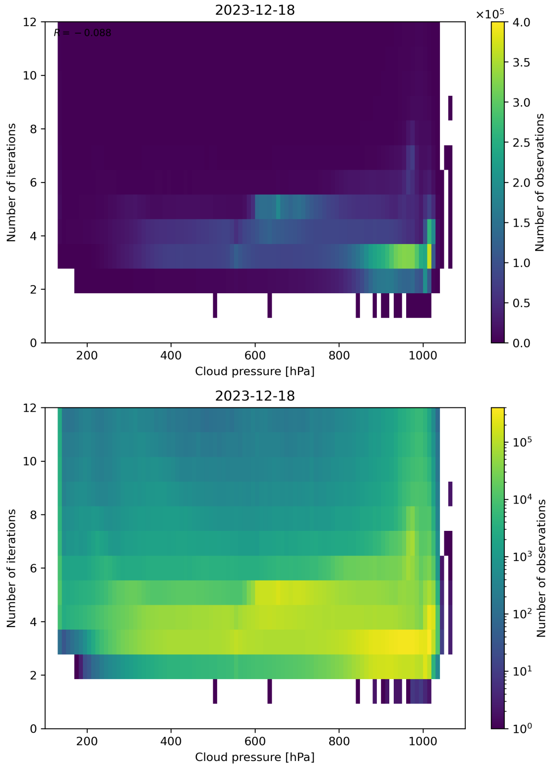
Figure 81: Scatter density plot of “Cloud pressure” against “Number of iterations” for 2023-12-17 to 2023-12-19.
