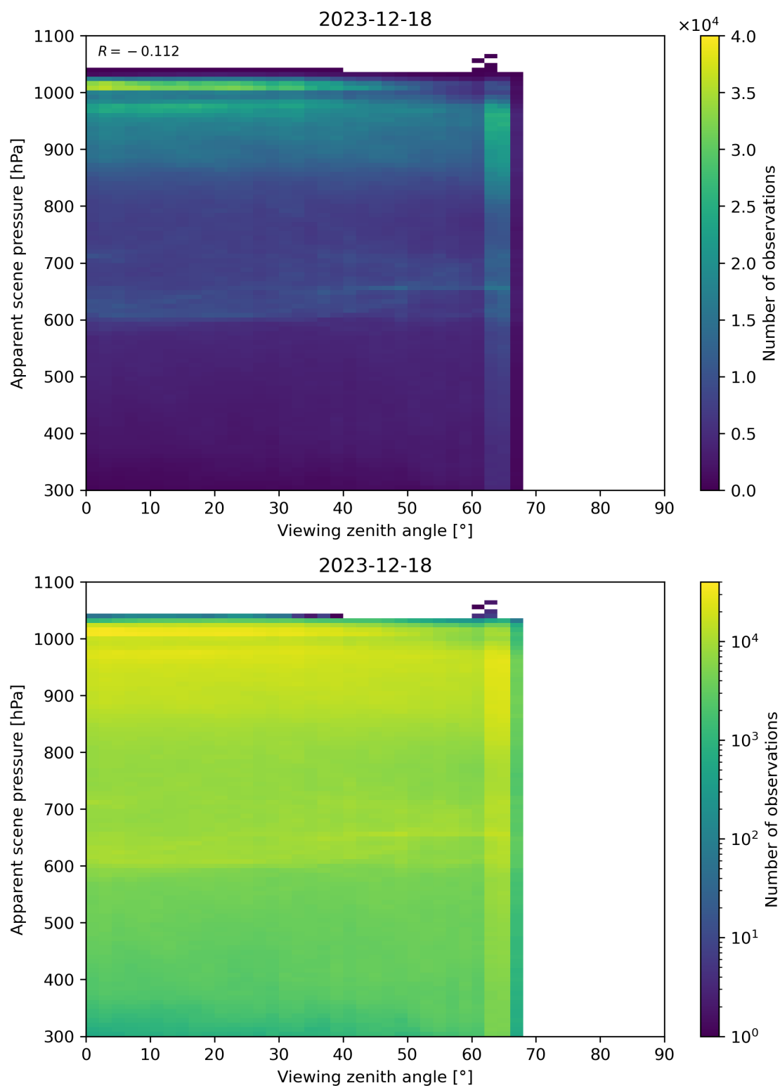
Figure 118: Scatter density plot of “Viewing zenith angle” against “Apparent scene pressure” for 2023-12-17 to 2023-12-19.
