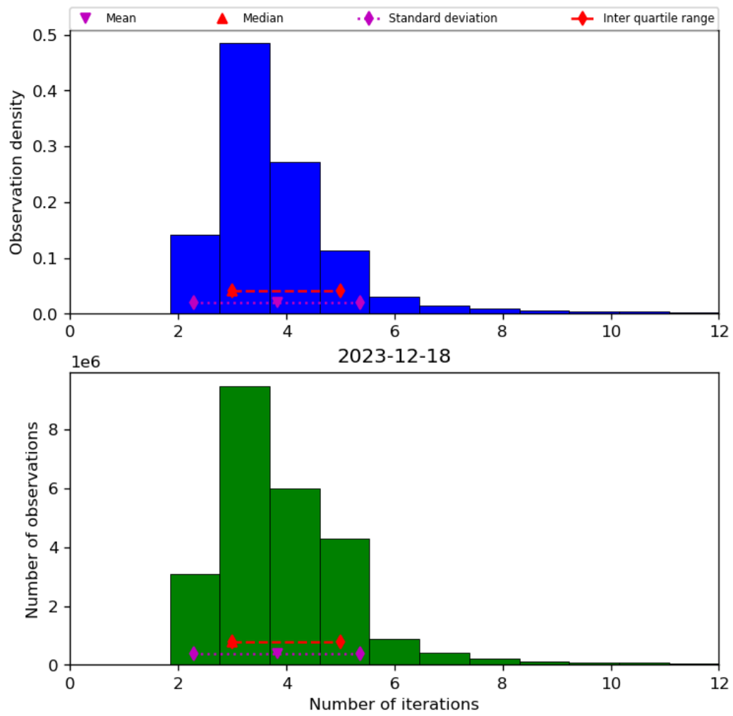
Figure 39: Histogram of “Number of iterations” for 2023-12-17 to 2023-12-19
