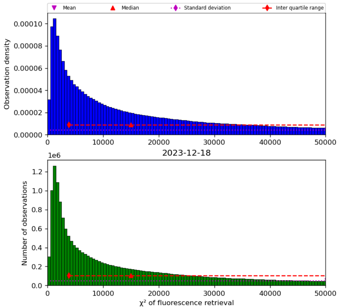
Figure 42: Histogram of “ \chi^2 of fluorescence retrieval” for 2023-12-17 to 2023-12-19
