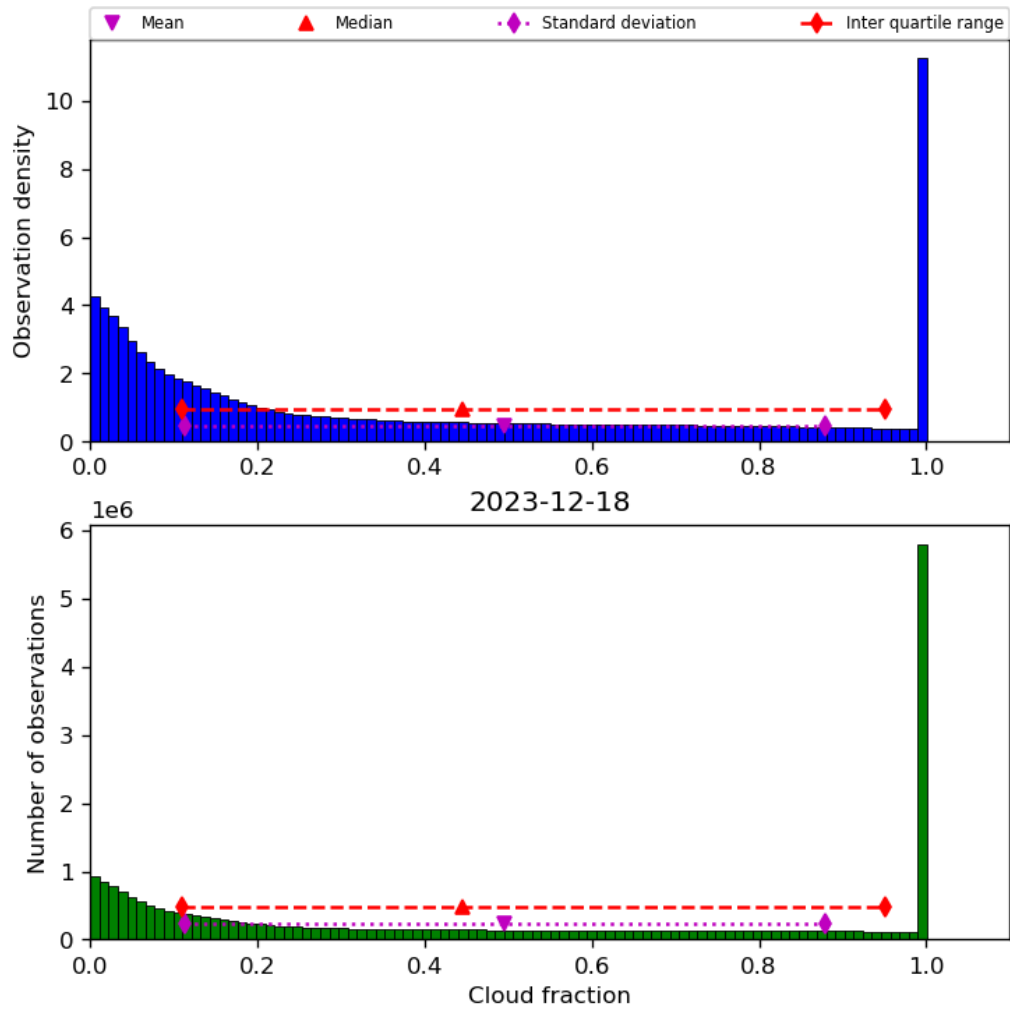
Figure 32: Histogram of “Cloud fraction” for 2023-12-17 to 2023-12-19
