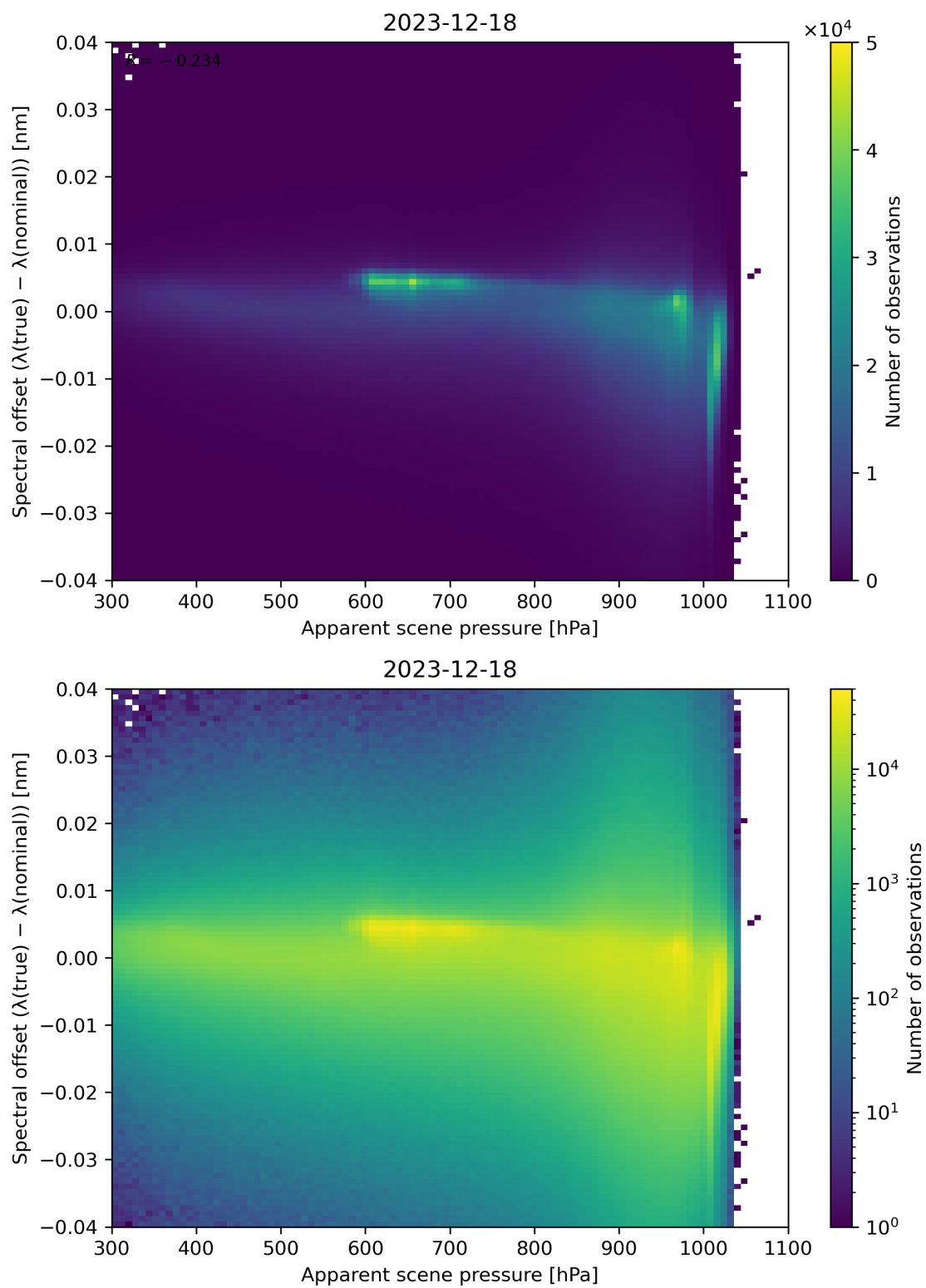
Figure 67: Scatter density plot of “Apparent scene pressure” against “Spectral offset ( \lambda(\text{true}) - \lambda(\text{nominal}) )” for 2023-12-17 to 2023-12-19.
