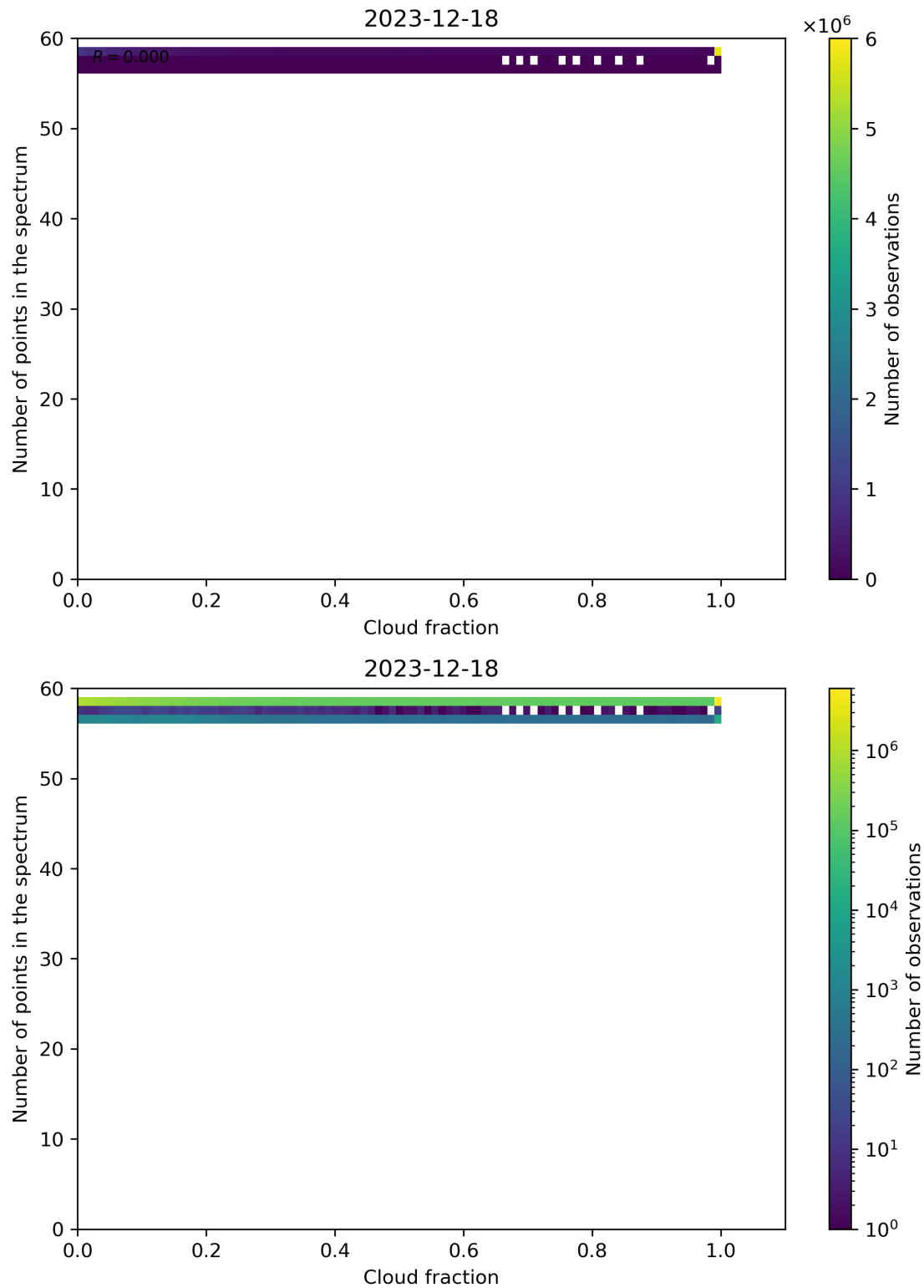
Figure 74: Scatter density plot of “Cloud fraction” against “Number of points in the spectrum” for 2023-12-17 to 2023-12-19.
