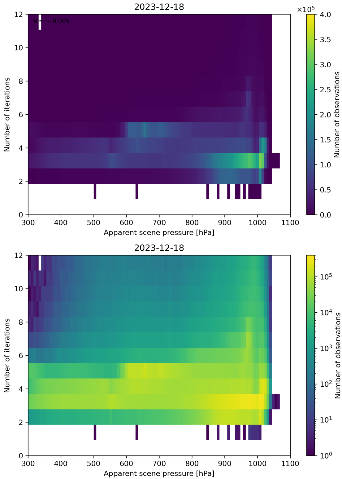
Figure 65: Scatter density plot of “Apparent scene pressure” against “Number of iterations” for 2023-12-17 to 2023-12-19.
