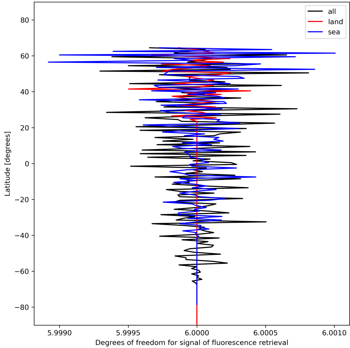
Figure 26: Zonal average of “Degrees of freedom for signal of fluorescence retrieval” for 2023-12-17 to 2023-12-19.
