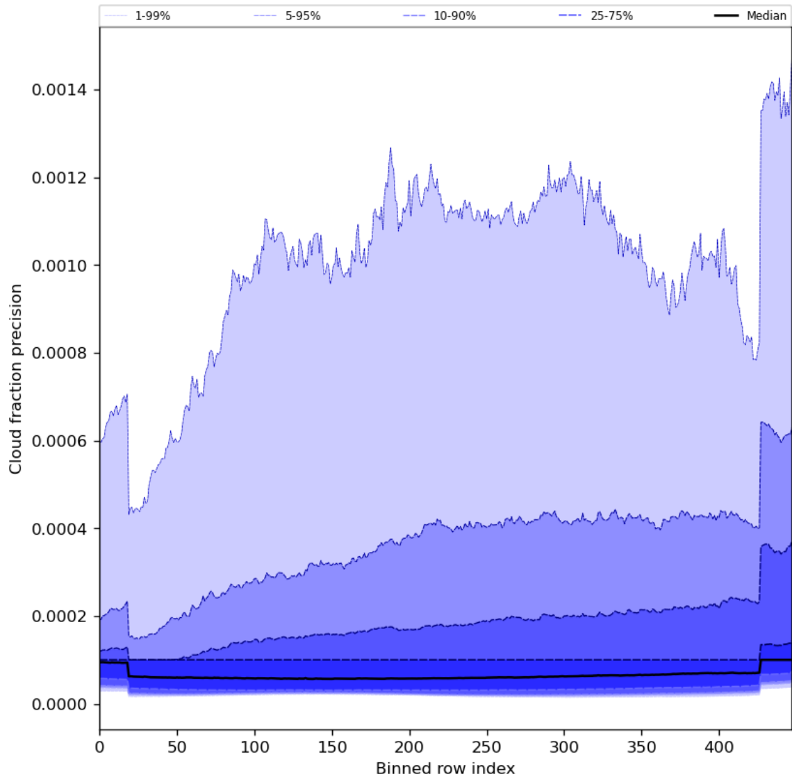
Figure 50: Along track statistics of “Cloud fraction precision” for 2023-12-17 to 2023-12-19
