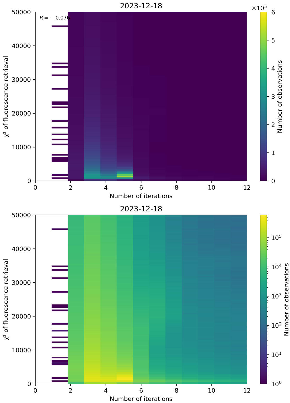
Figure 97: Scatter density plot of “Number of iterations” against “ \chi^2 of fluorescence retrieval” for 2023-12-17 to 2023-12-19.
