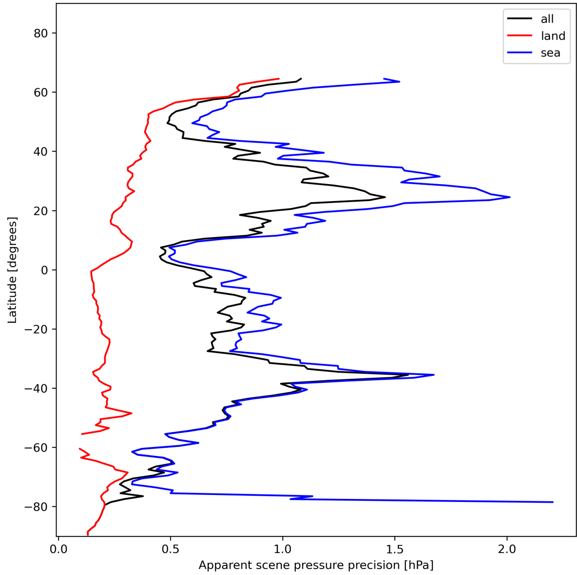
Figure 20: Zonal average of “Apparent scene pressure precision” for 2023-12-17 to 2023-12-19.
