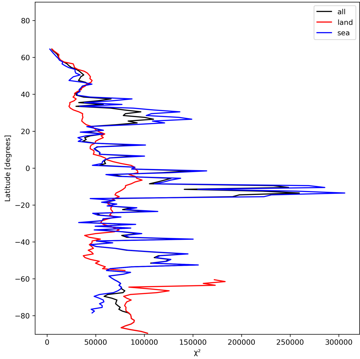
Figure 21: Zonal average of “ \chi^2 ” for 2023-12-17 to 2023-12-19.
