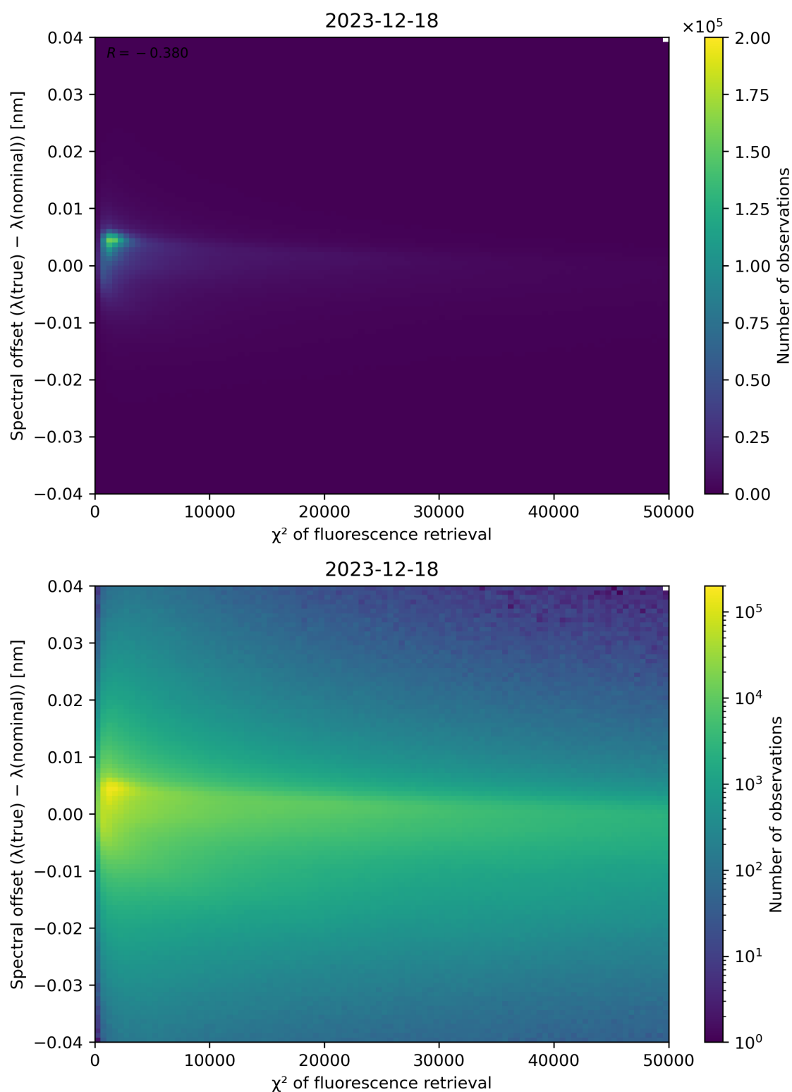
Figure 69: Scatter density plot of " \chi^2 of fluorescence retrieval" against "Spectral offset ( \lambda(\text{true}) - \lambda(\text{nominal}) )" for 2023-12-17 to 2023-12-19.
