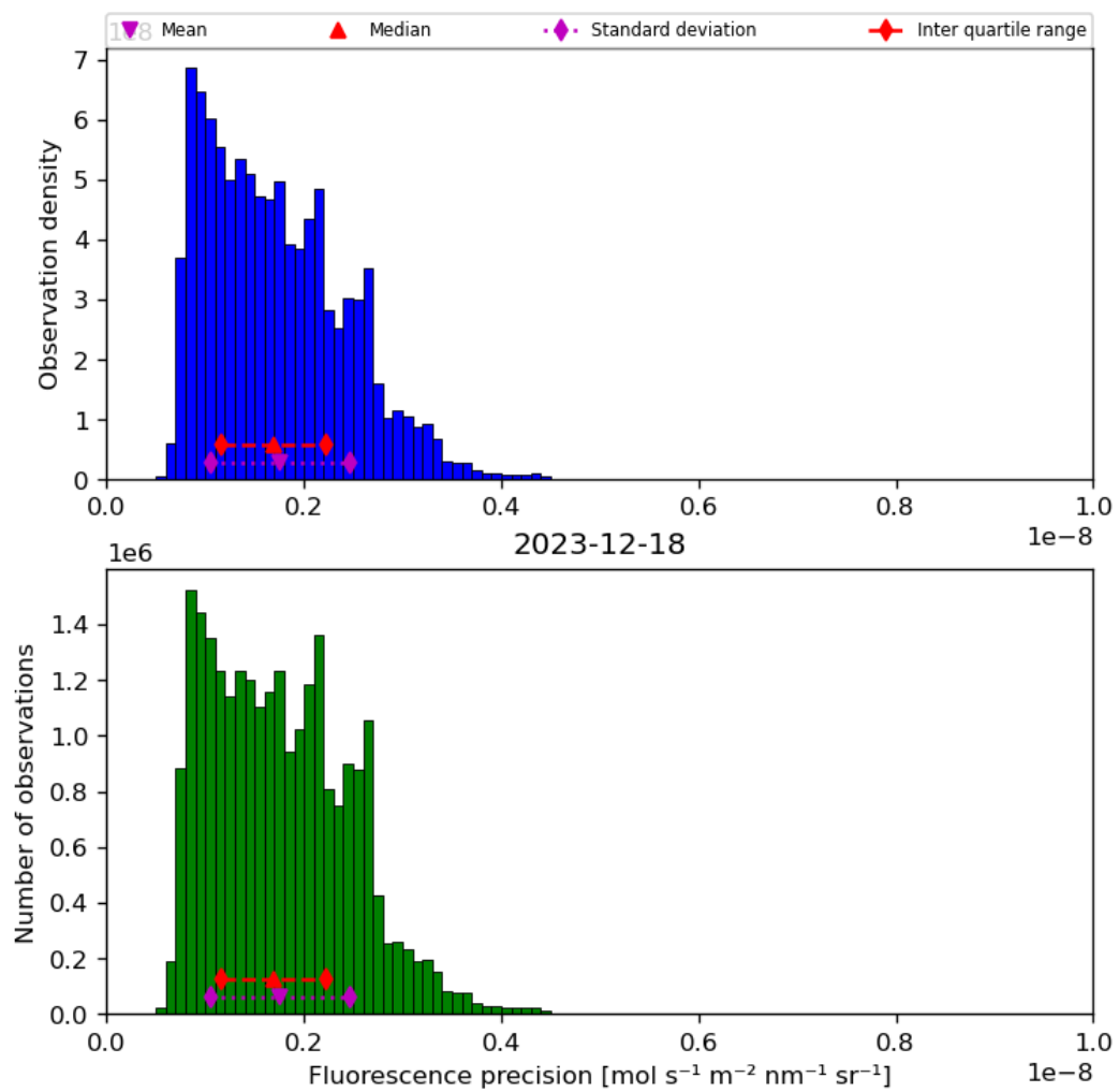
Figure 41: Histogram of “Fluorescence precision” for 2023-12-17 to 2023-12-19
