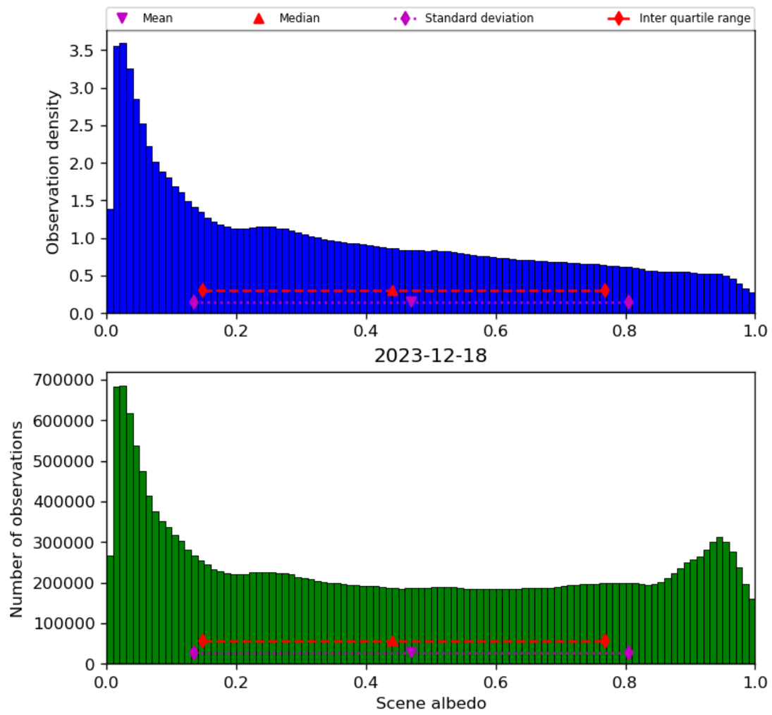
Figure 34: Histogram of “Scene albedo” for 2023-12-17 to 2023-12-19
