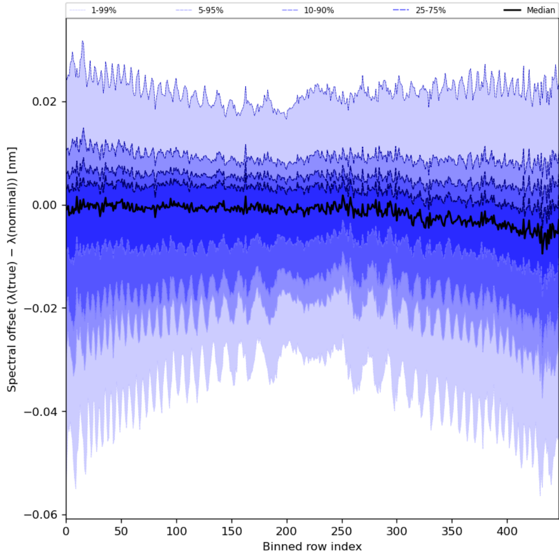
Figure 62: Along track statistics of “Spectral offset ( \lambda(\text{true}) - \lambda(\text{nominal}) )” for 2023-12-17 to 2023-12-19
