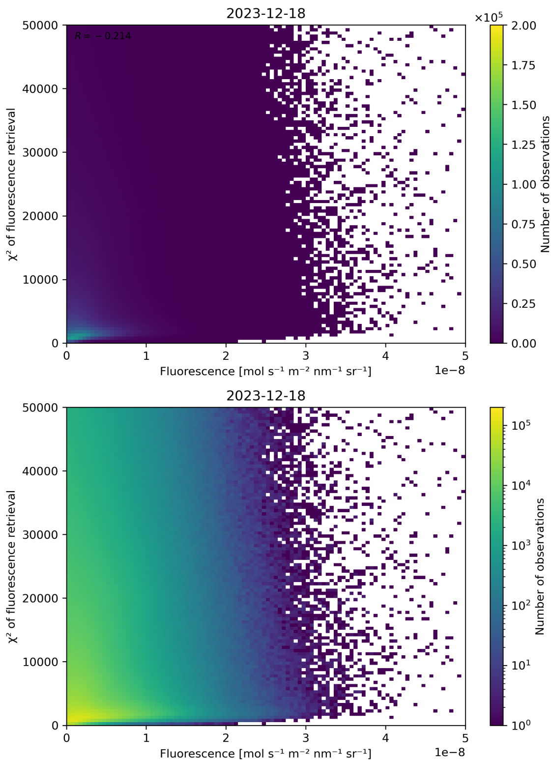
Figure 85: Scatter density plot of “Fluorescence” against “ \chi^2 of fluorescence retrieval” for 2023-12-17 to 2023-12-19.
