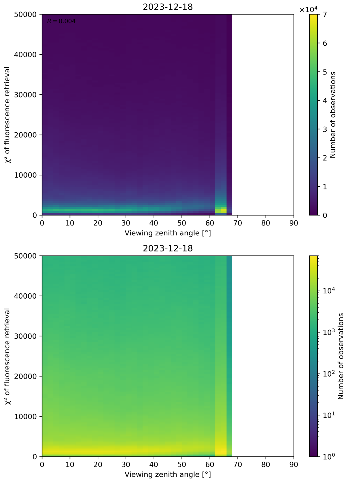
Figure 119: Scatter density plot of “Viewing zenith angle” against “ \chi^2 of fluorescence retrieval” for 2023-12-17 to 2023-12-19.
