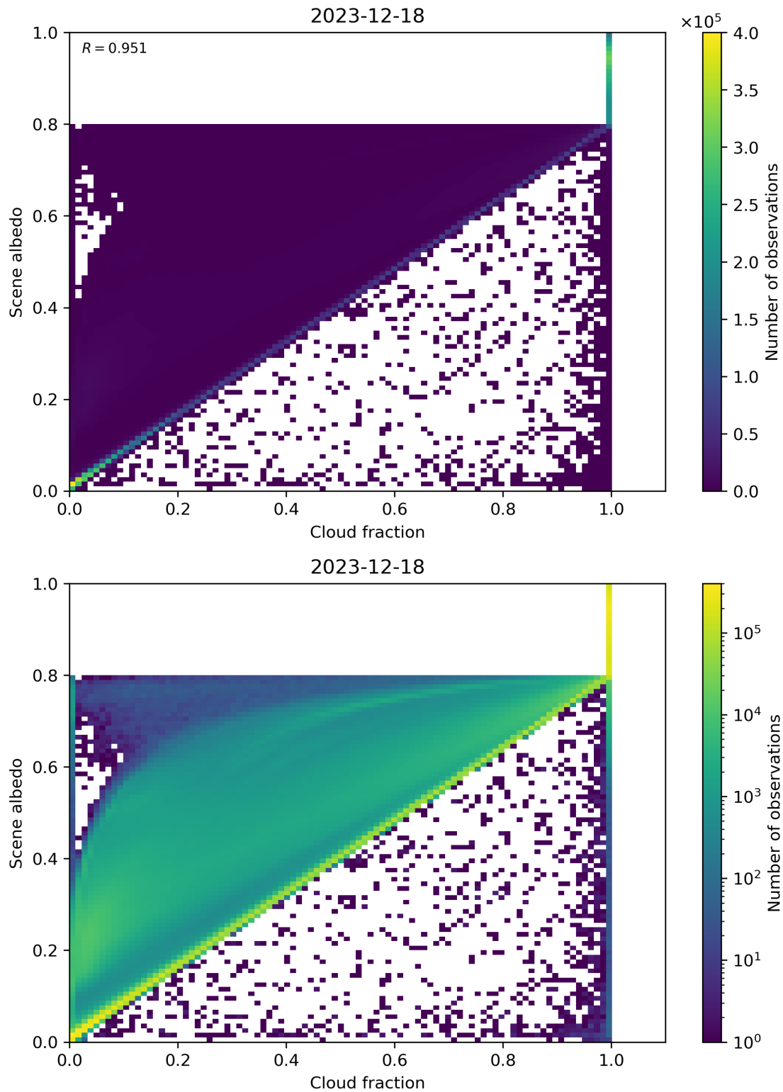
Figure 75: Scatter density plot of “Cloud fraction” against “Scene albedo” for 2023-12-17 to 2023-12-19.
