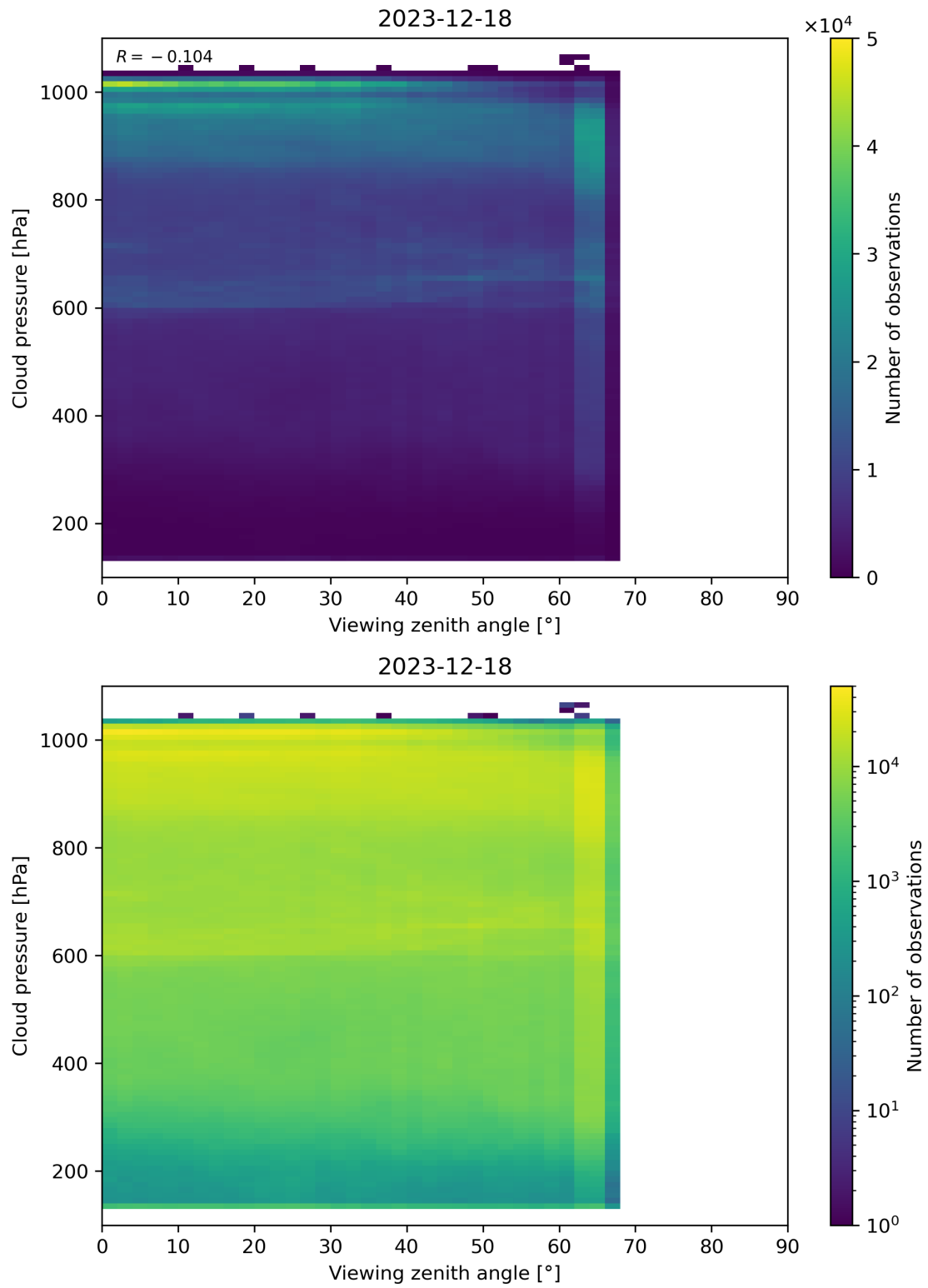
Figure 121: Scatter density plot of “Viewing zenith angle” against “Cloud pressure” for 2023-12-17 to 2023-12-19.
