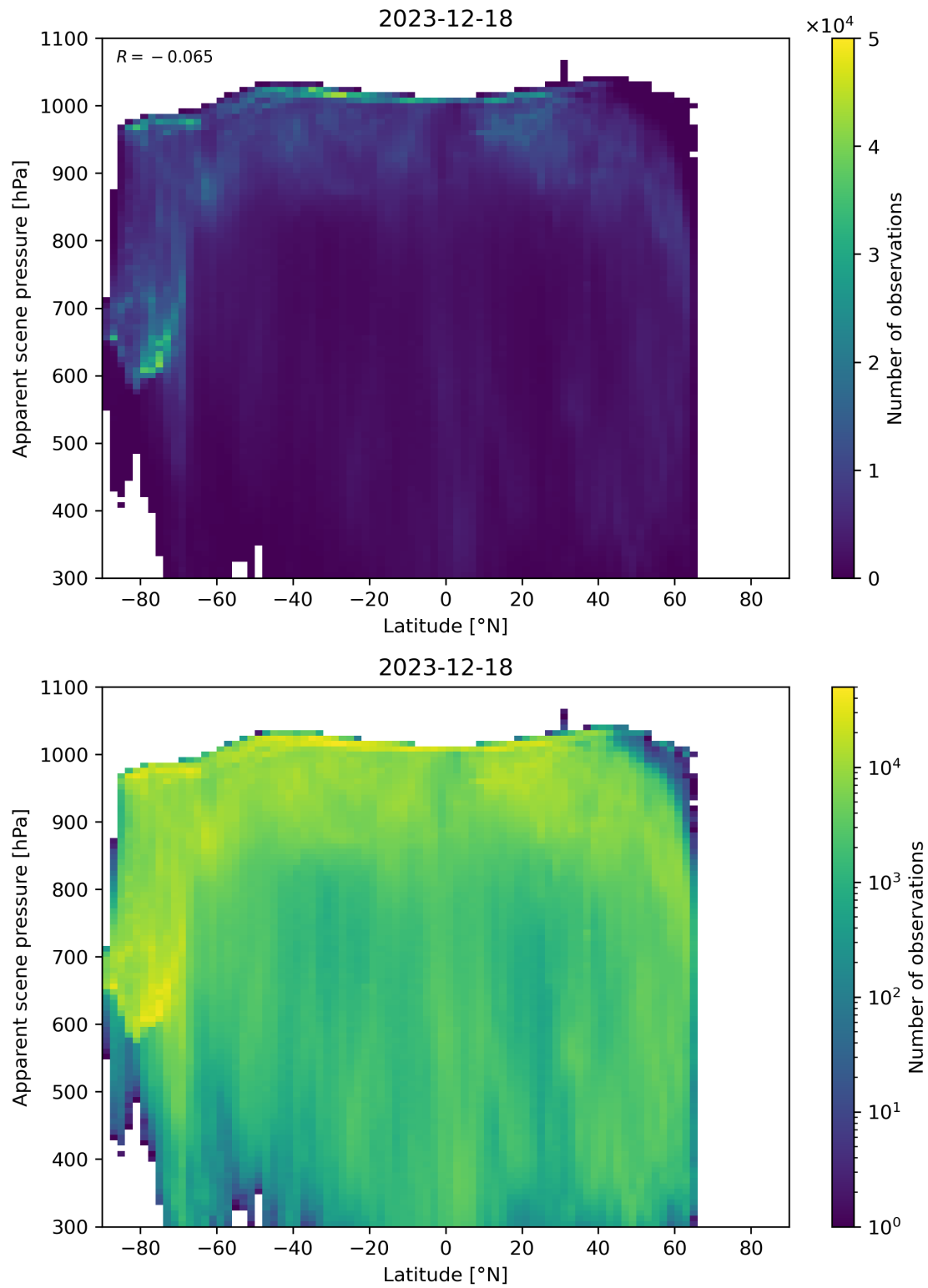
Figure 88: Scatter density plot of “Latitude” against “Apparent scene pressure” for 2023-12-17 to 2023-12-19.
