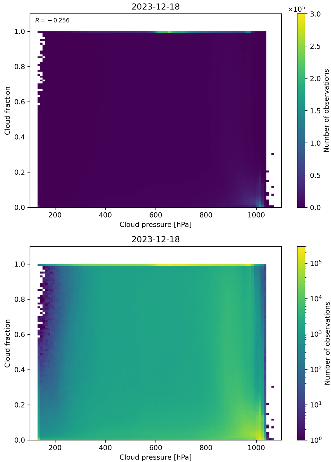
Figure 79: Scatter density plot of “Cloud pressure” against “Cloud fraction” for 2023-12-17 to 2023-12-19.
