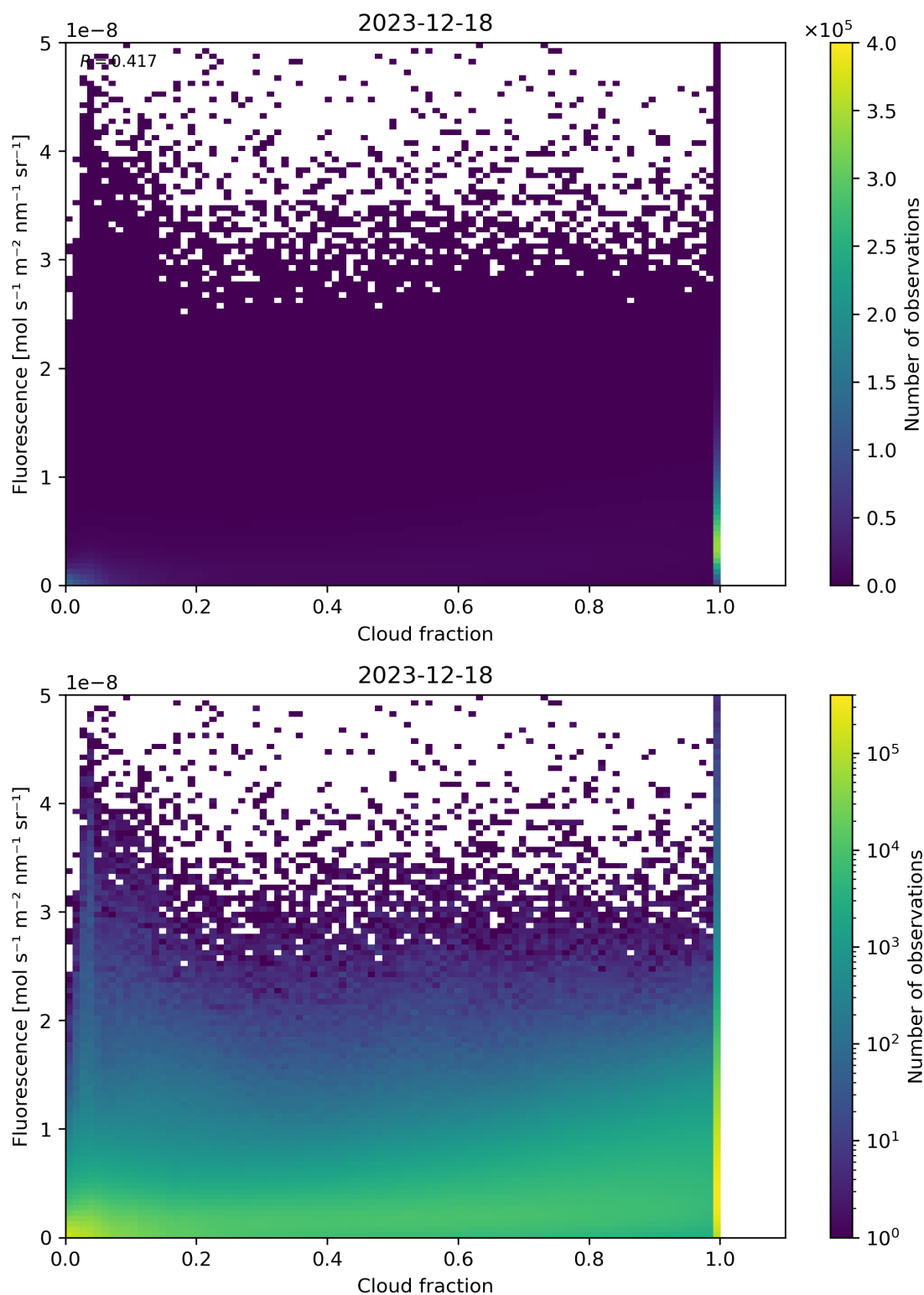
Figure 72: Scatter density plot of “Cloud fraction” against “Fluorescence” for 2023-12-17 to 2023-12-19.
