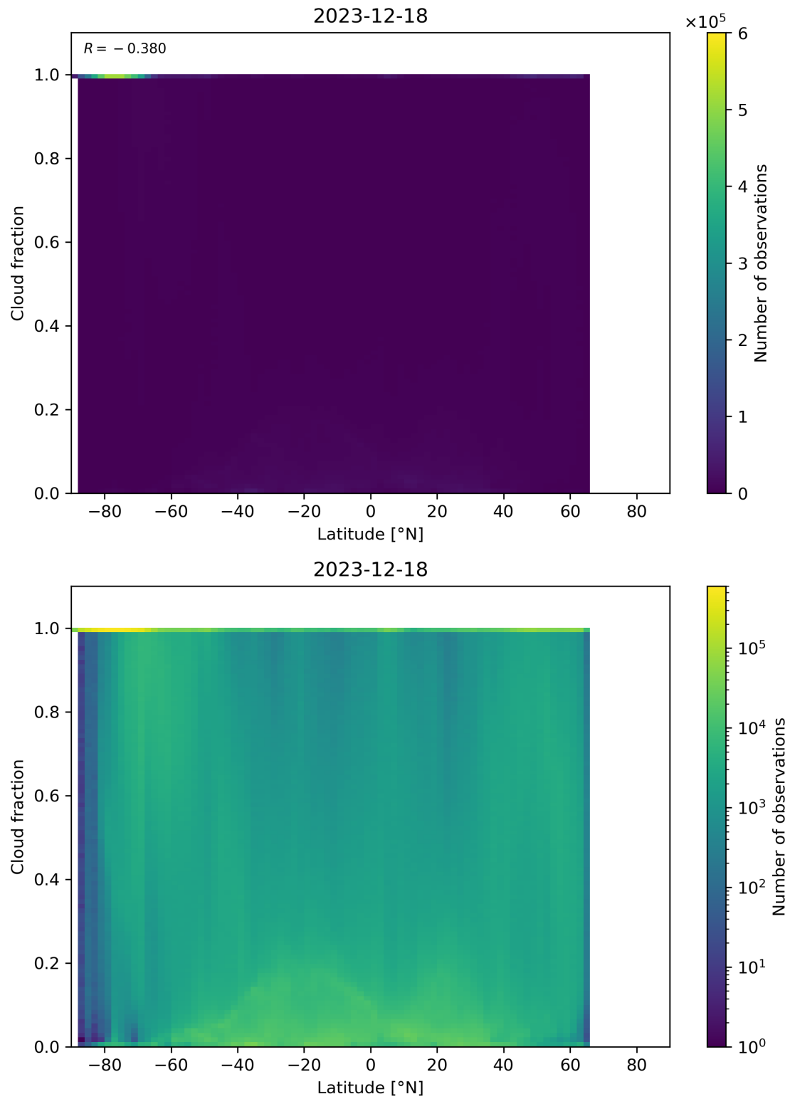
Figure 90: Scatter density plot of “Latitude” against “Cloud fraction” for 2023-12-17 to 2023-12-19.
