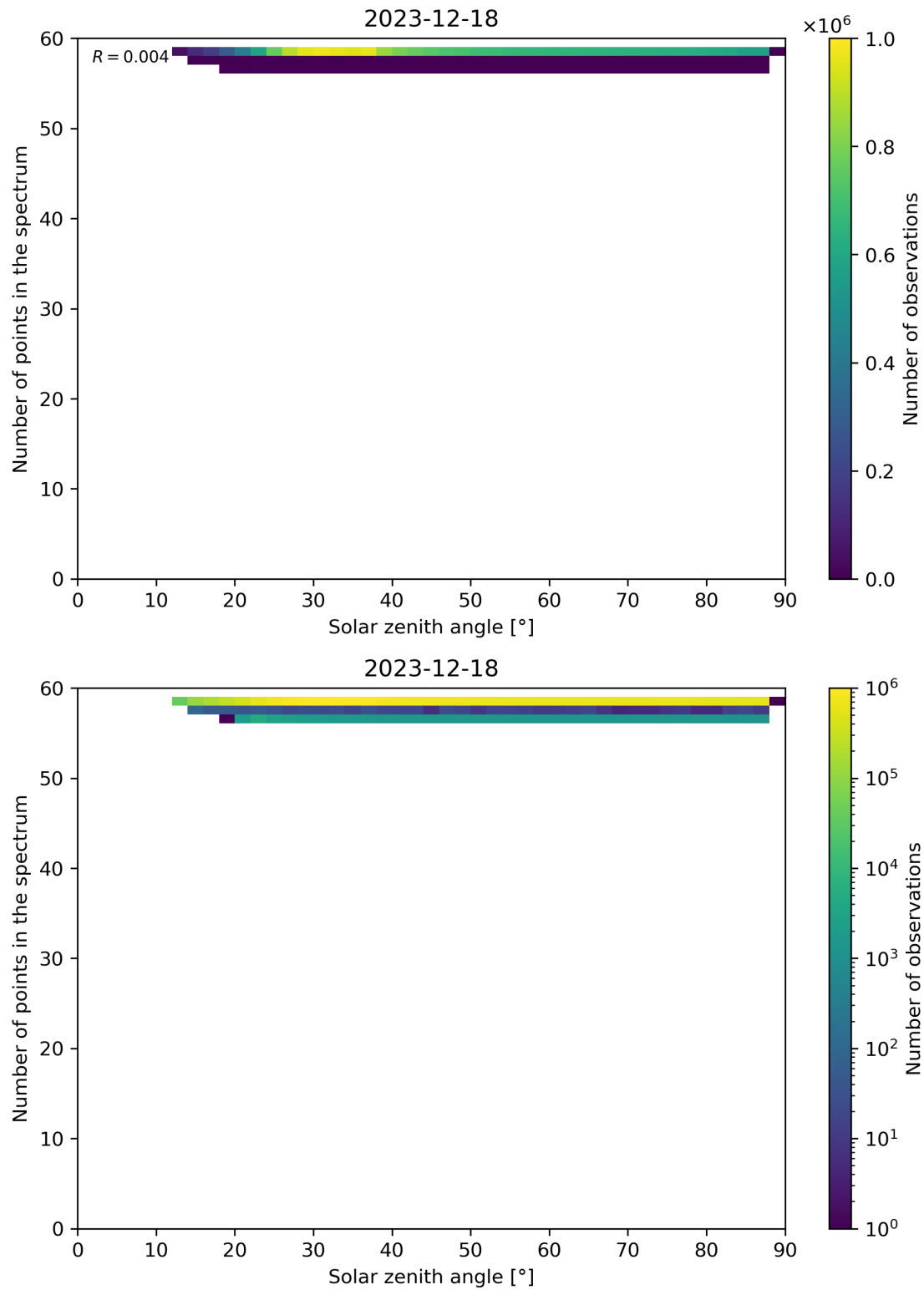
Figure 115: Scatter density plot of “Solar zenith angle” against “Number of points in the spectrum” for 2023-12-17 to 2023-12-19.
