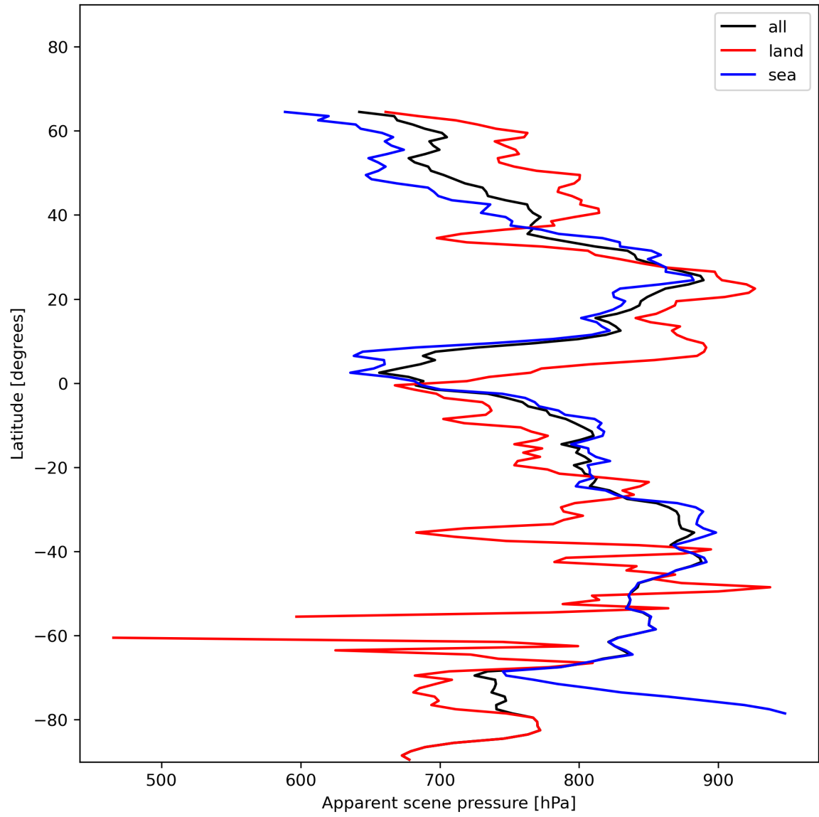
Figure 19: Zonal average of “Apparent scene pressure” for 2023-12-17 to 2023-12-19.
