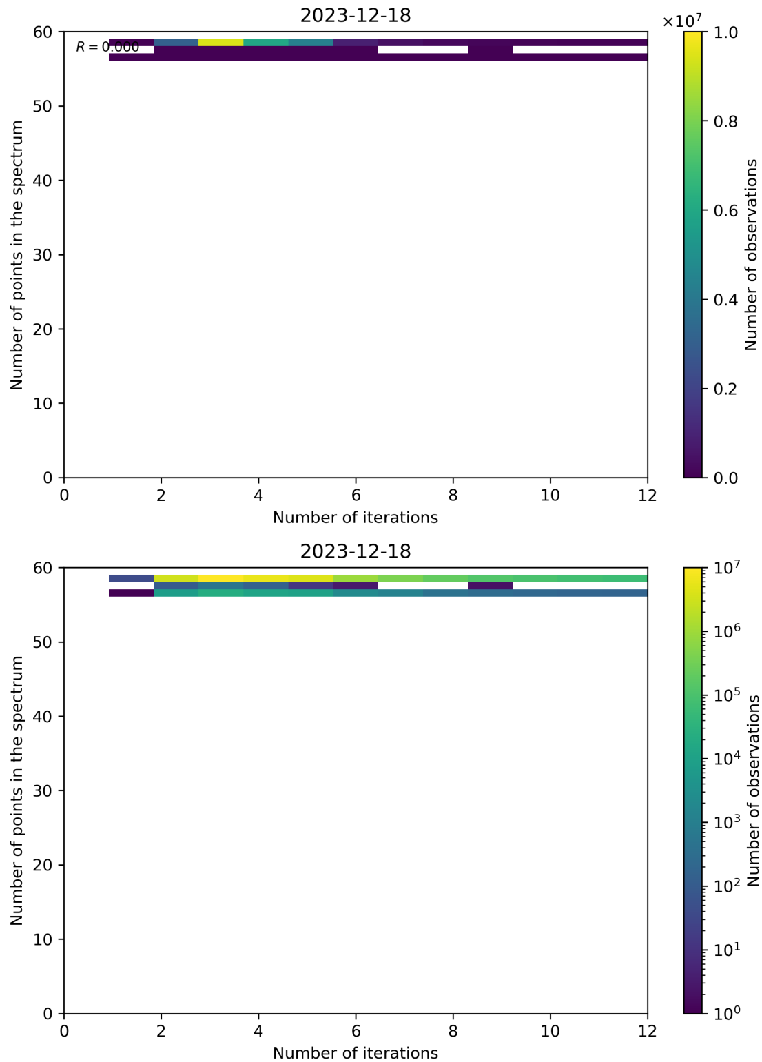
Figure 99: Scatter density plot of “Number of iterations” against “Number of points in the spectrum” for 2023-12-17 to 2023-12-19.
