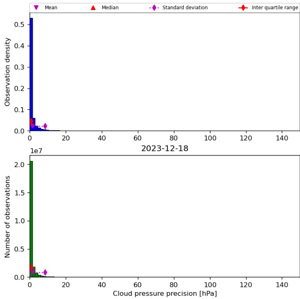
Figure 31: Histogram of “Cloud pressure precision” for 2023-12-17 to 2023-12-19
