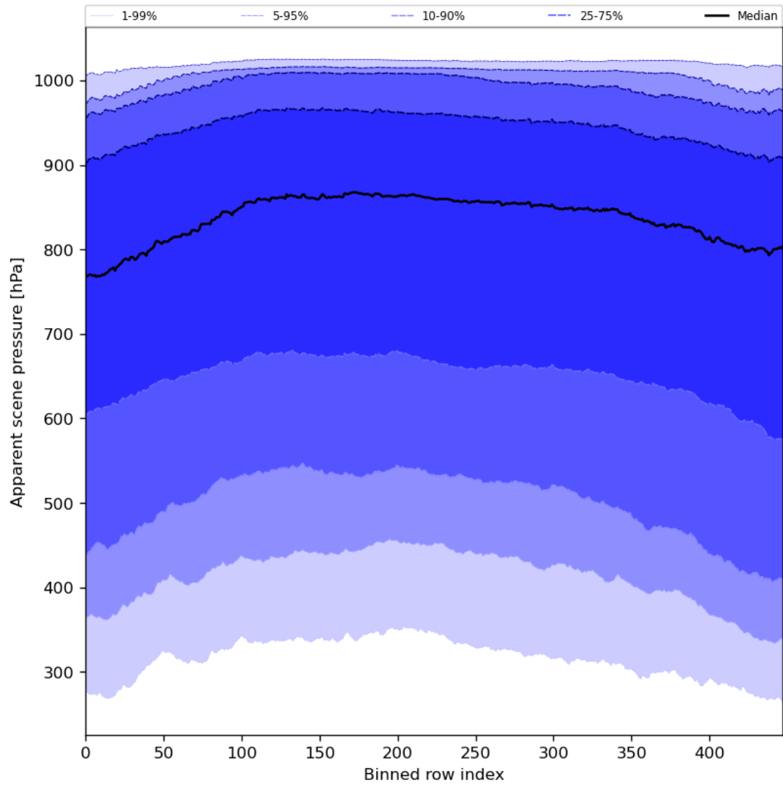
Figure 53: Along track statistics of “Apparent scene pressure” for 2023-12-17 to 2023-12-19
