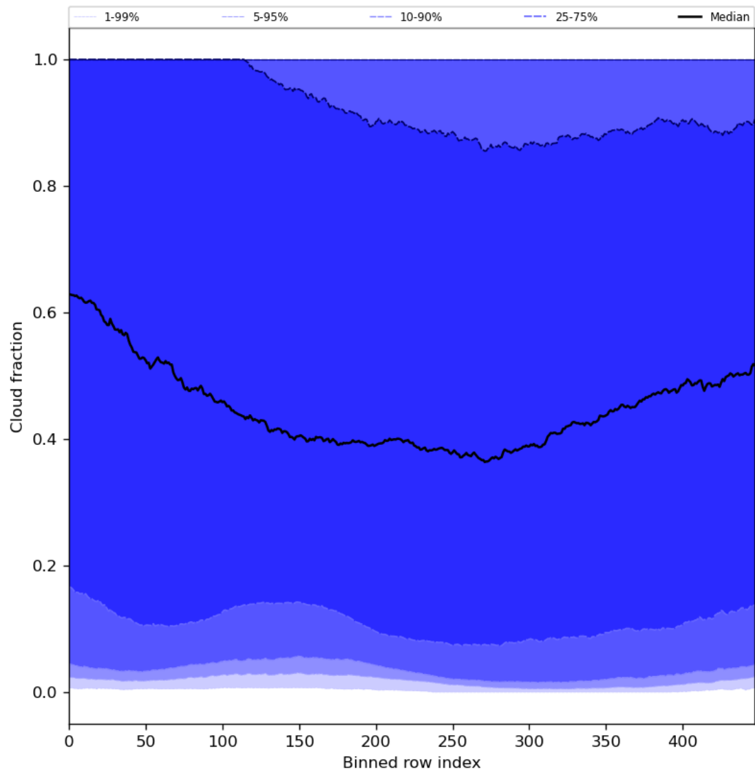
Figure 49: Along track statistics of “Cloud fraction” for 2023-12-17 to 2023-12-19
