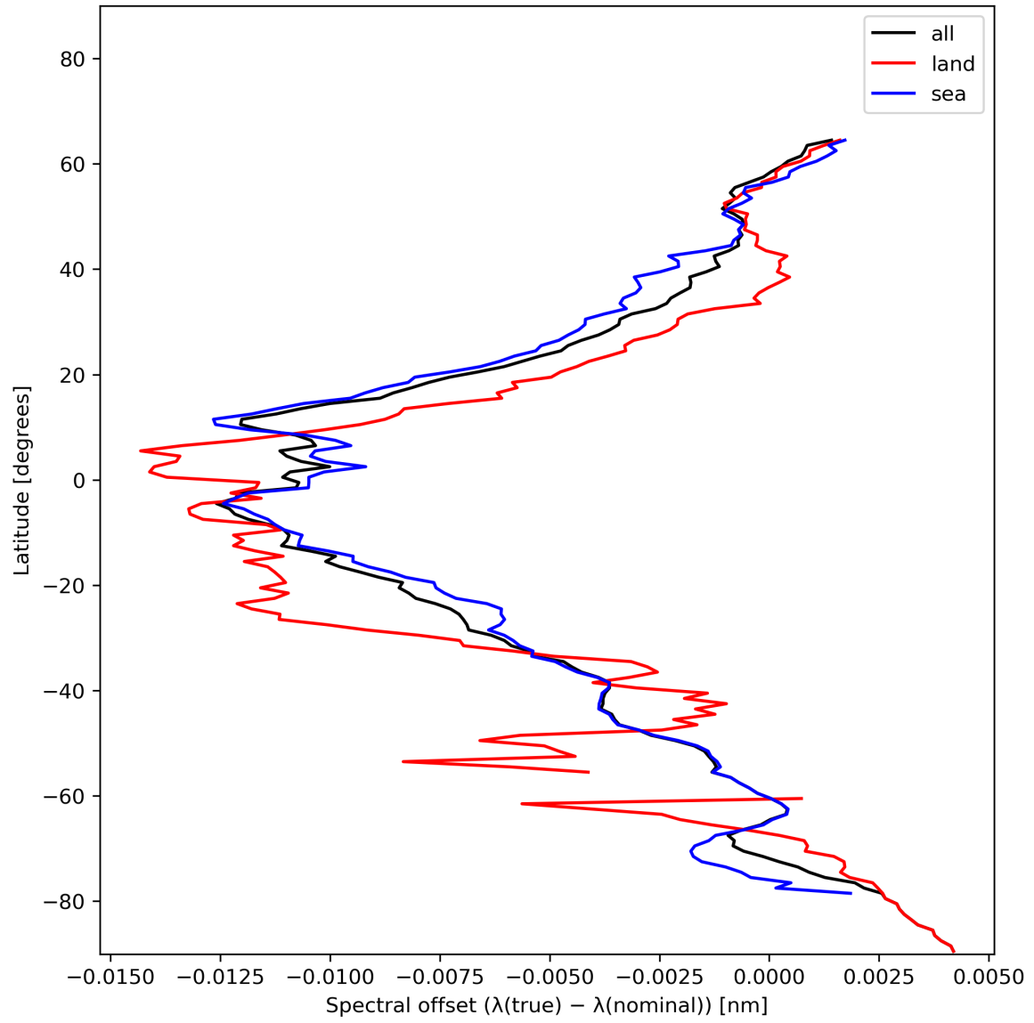
Figure 28: Zonal average of “Spectral offset ( \lambda(\text{true}) - \lambda(\text{nominal}) )” for 2023-12-17 to 2023-12-19.
