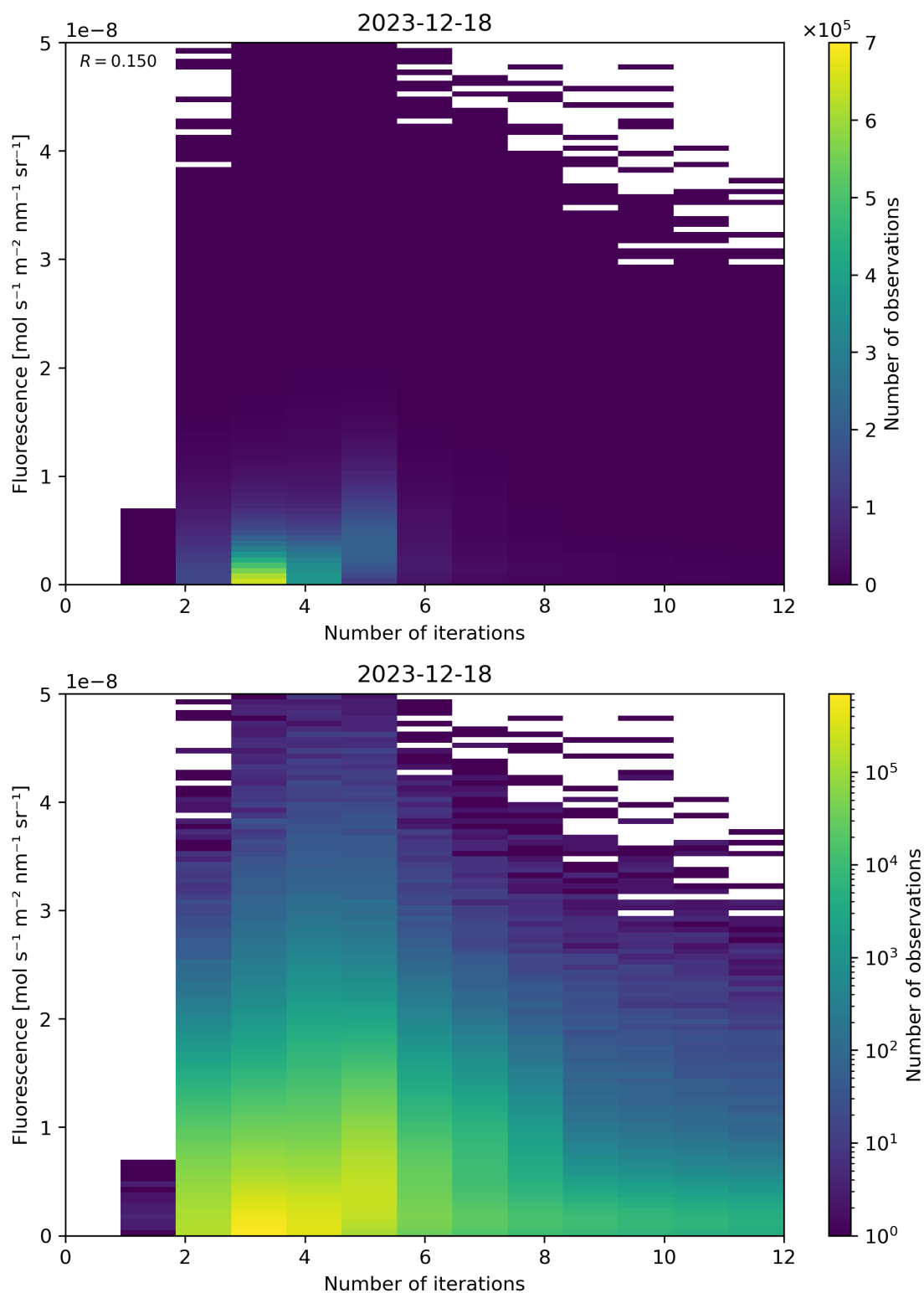
Figure 98: Scatter density plot of “Number of iterations” against “Fluorescence” for 2023-12-17 to 2023-12-19.
