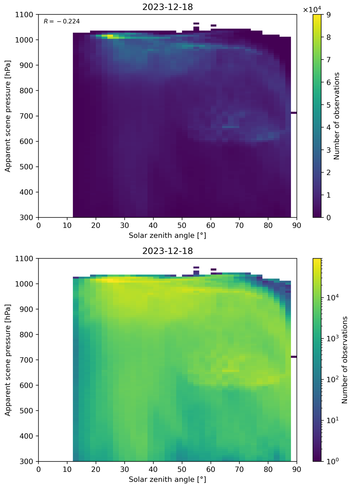
Figure 108: Scatter density plot of “Solar zenith angle” against “Apparent scene pressure” for 2023-12-17 to 2023-12-19.
