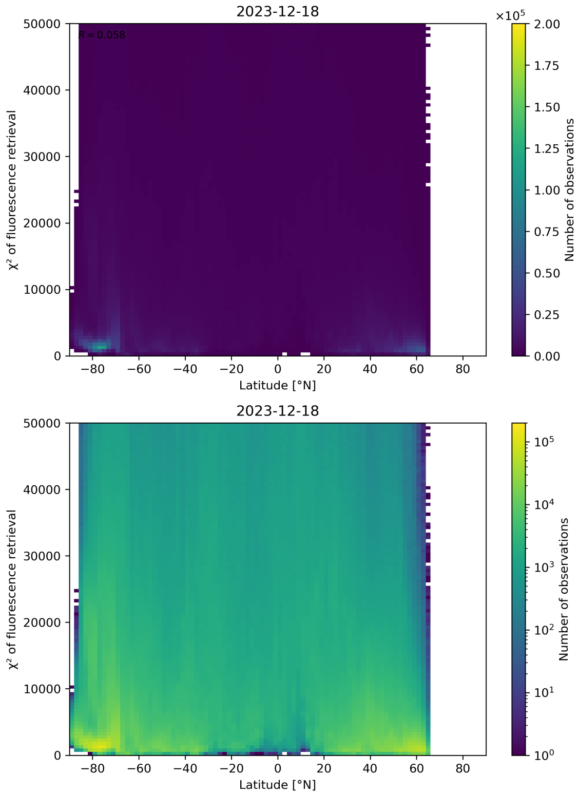
Figure 89: Scatter density plot of “Latitude” against “ \chi^2 of fluorescence retrieval” for 2023-12-17 to 2023-12-19.
