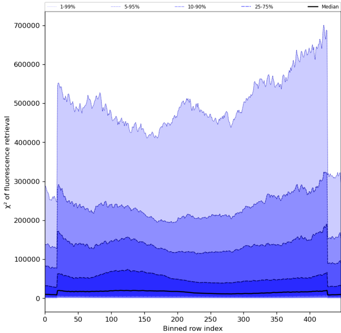
Figure 59: Along track statistics of “ \chi^2 of fluorescence retrieval” for 2023-12-17 to 2023-12-19
