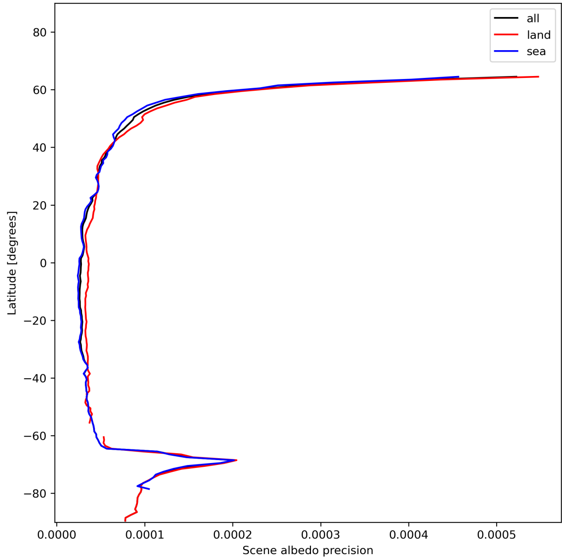
Figure 18: Zonal average of “Scene albedo precision” for 2023-12-17 to 2023-12-19.
