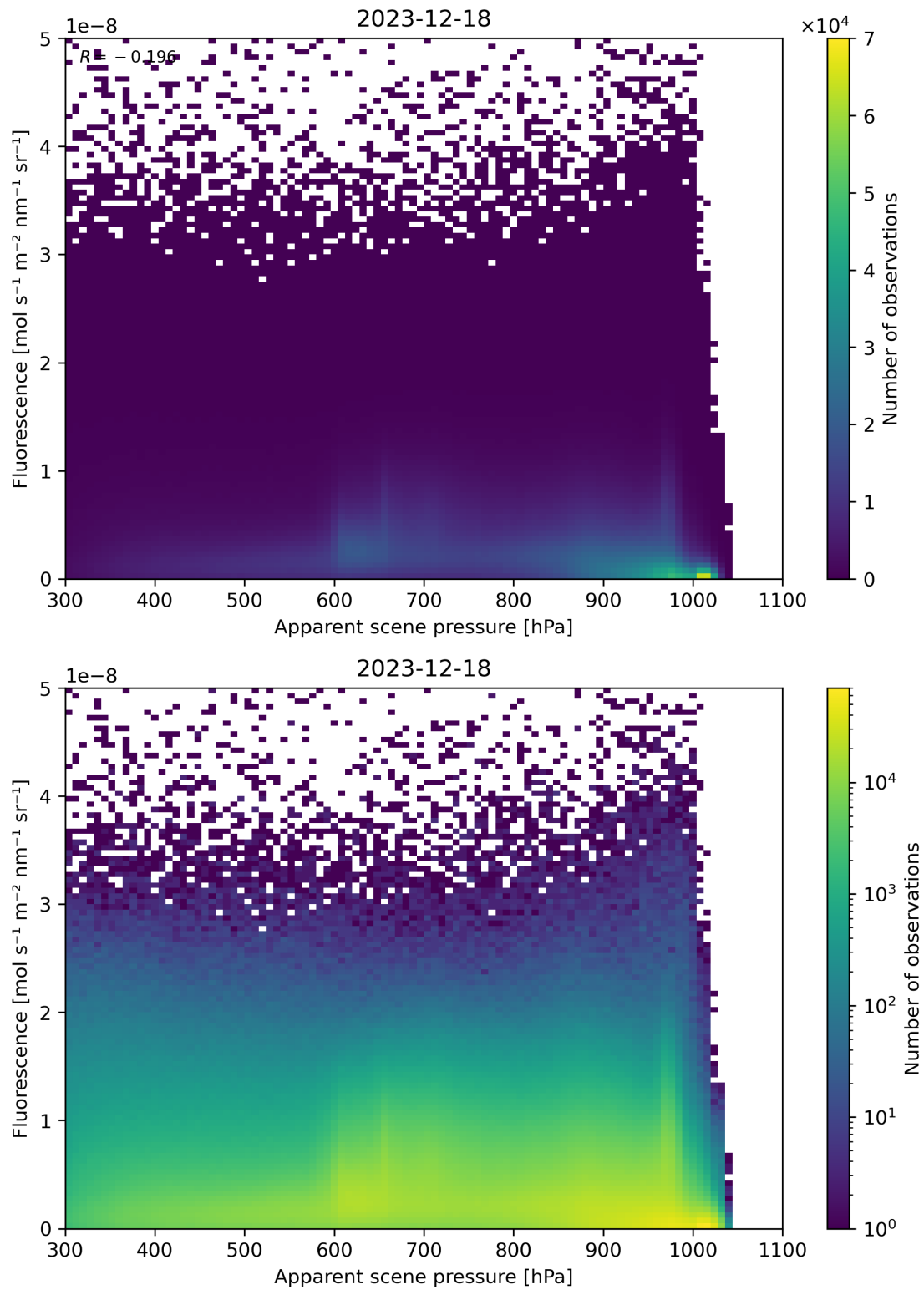
Figure 64: Scatter density plot of “Apparent scene pressure” against “Fluorescence” for 2023-12-17 to 2023-12-19.
