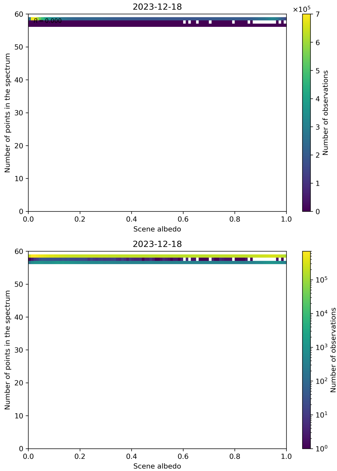
Figure 106: Scatter density plot of “Scene albedo” against “Number of points in the spectrum” for 2023-12-17 to 2023-12-19.
