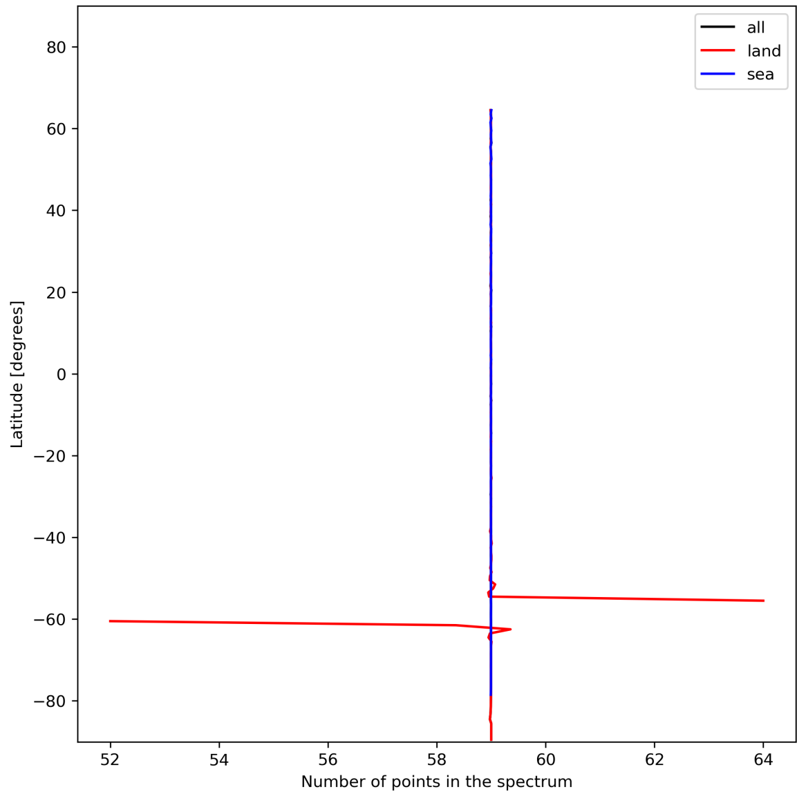
Figure 27: Zonal average of “Number of points in the spectrum” for 2023-12-17 to 2023-12-19.
