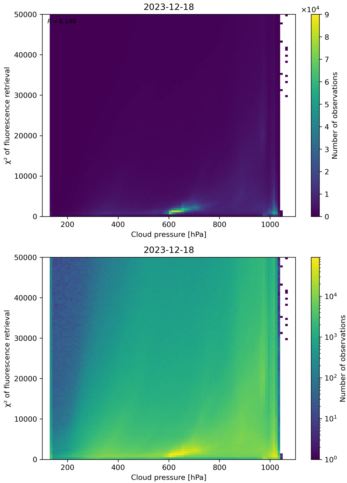
Figure 78: Scatter density plot of “Cloud pressure” against “ \chi^2 of fluorescence retrieval” for 2023-12-17 to 2023-12-19.
