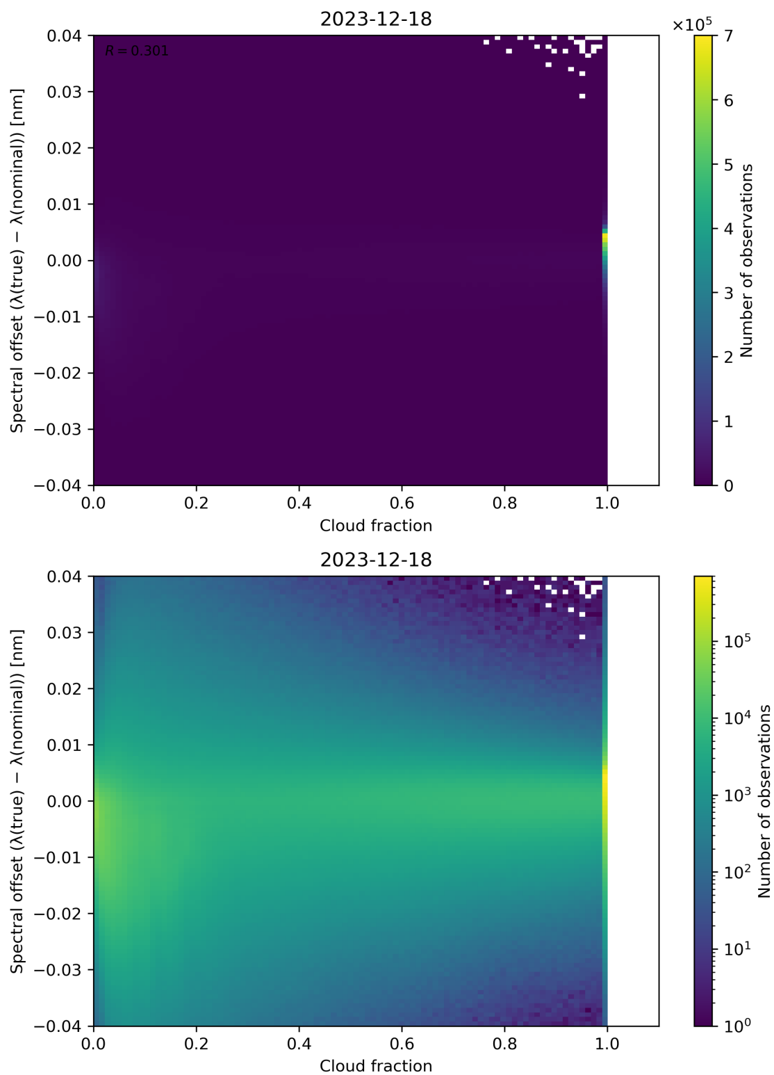
Figure 76: Scatter density plot of “Cloud fraction” against “Spectral offset ( \lambda(\text{true}) - \lambda(\text{nominal}) )” for 2023-12-17 to 2023-12-19.
