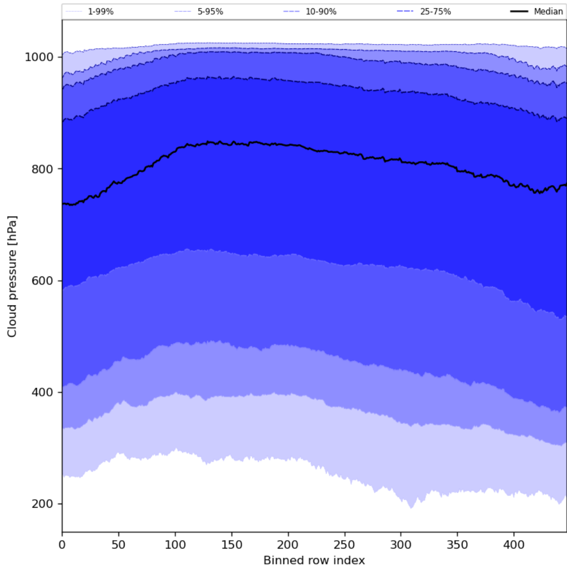
Figure 47: Along track statistics of “Cloud pressure” for 2023-12-17 to 2023-12-19
