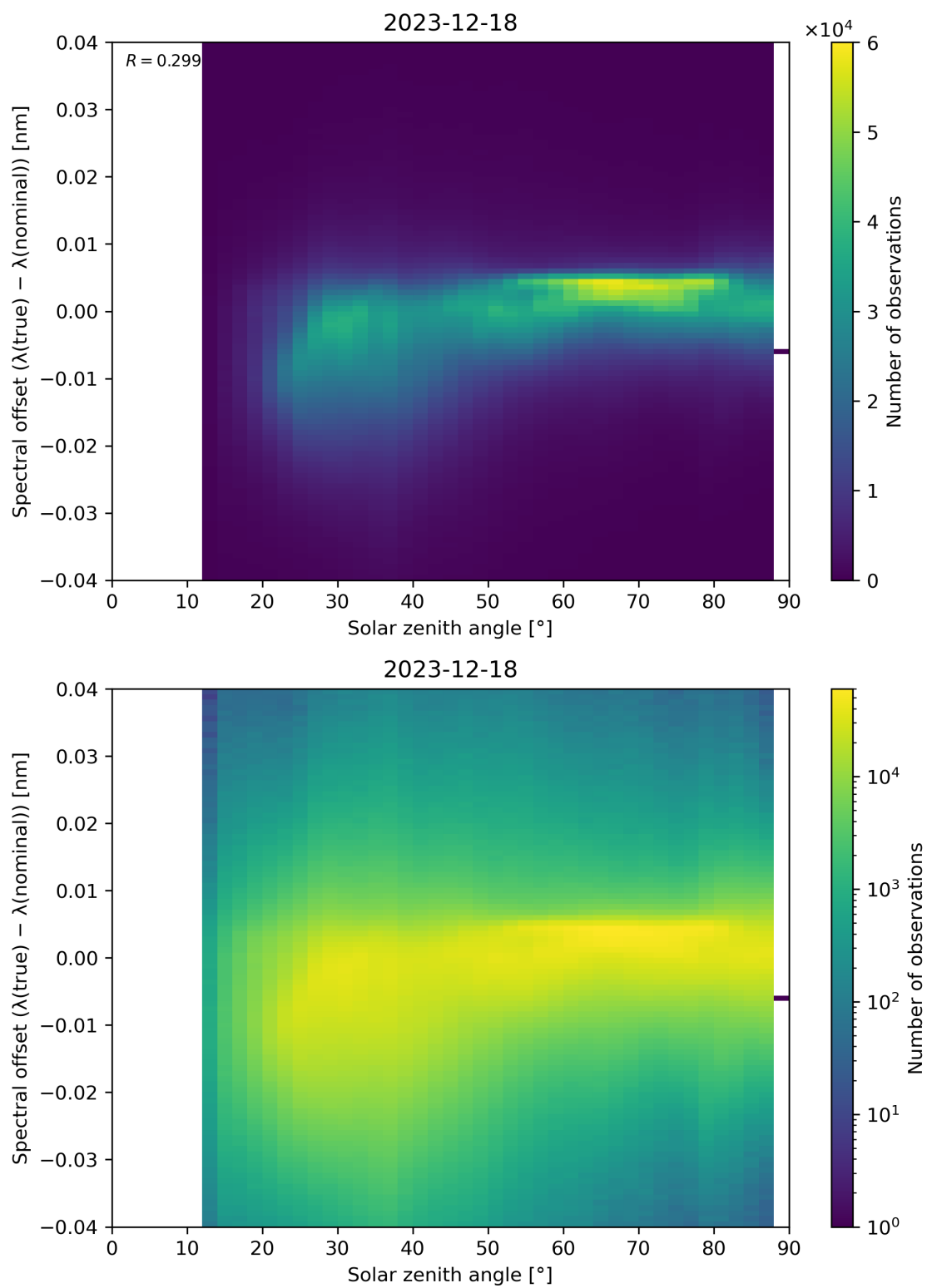
Figure 117: Scatter density plot of “Solar zenith angle” against “Spectral offset ( \lambda(\text{true}) - \lambda(\text{nominal}) )” for 2023-12-17 to 2023-12-19.
