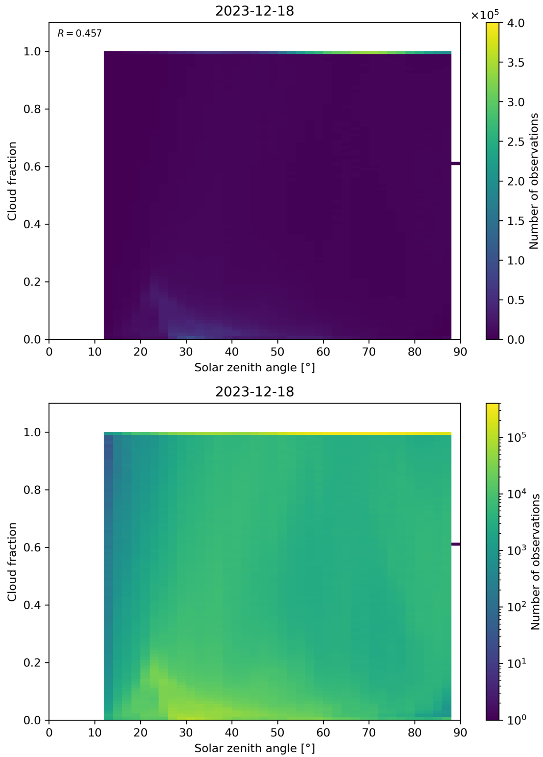
Figure 110: Scatter density plot of “Solar zenith angle” against “Cloud fraction” for 2023-12-17 to 2023-12-19.
