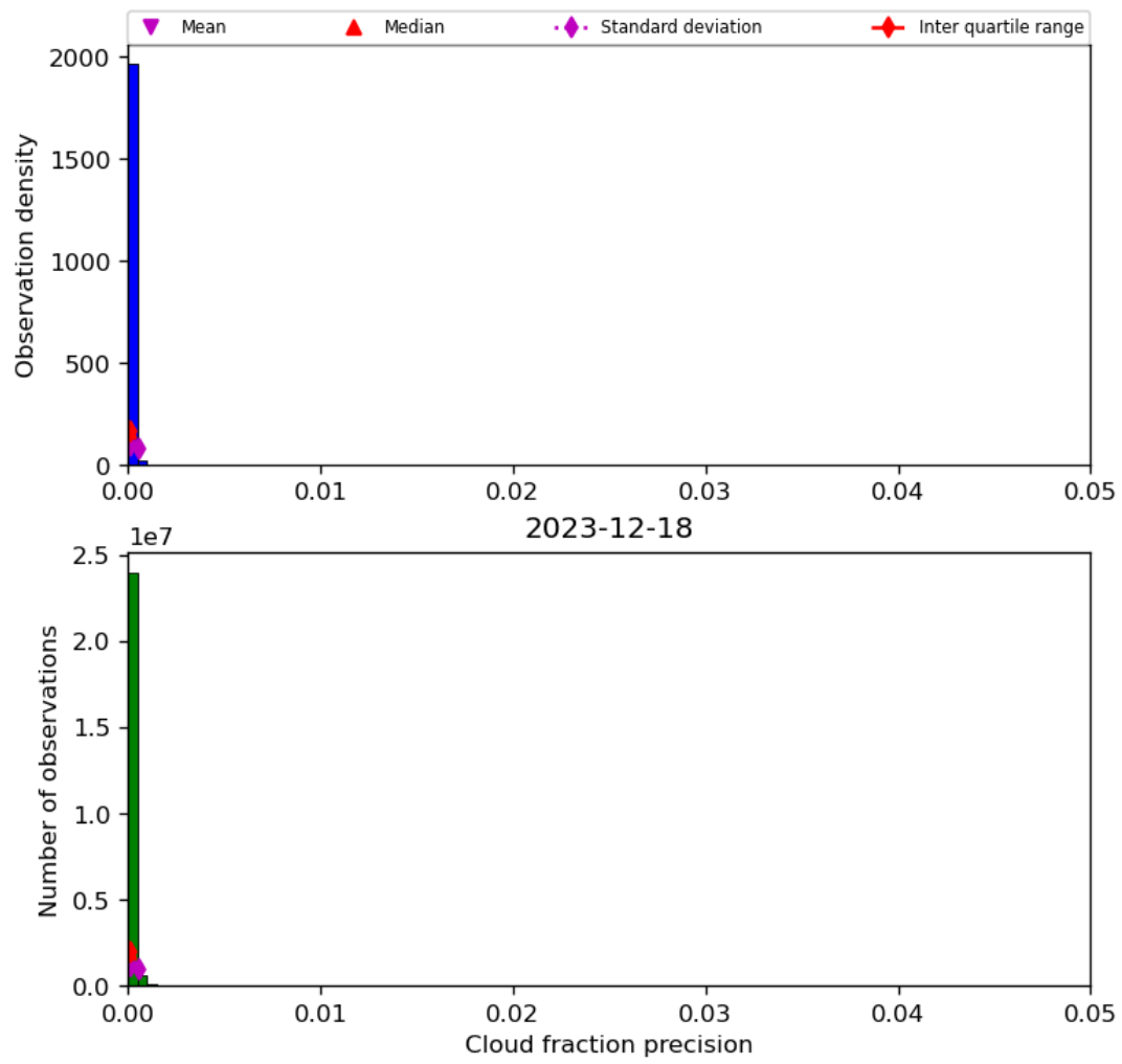
Figure 33: Histogram of “Cloud fraction precision” for 2023-12-17 to 2023-12-19
