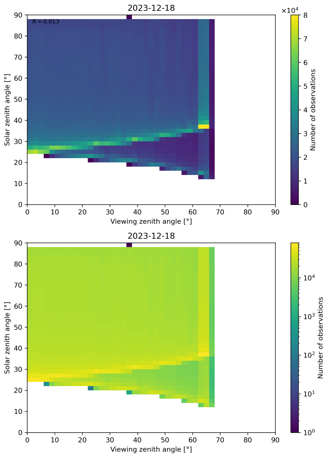
Figure 127: Scatter density plot of “Viewing zenith angle” against “Solar zenith angle” for 2023-12-17 to 2023-12-19.
