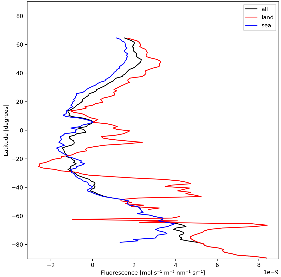
Figure 23: Zonal average of “Fluorescence” for 2023-12-17 to 2023-12-19.
