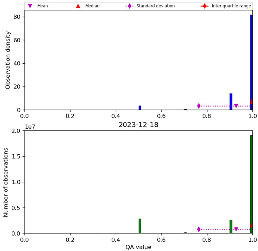
Figure 29: Histogram of “QA value” for 2023-12-17 to 2023-12-19
