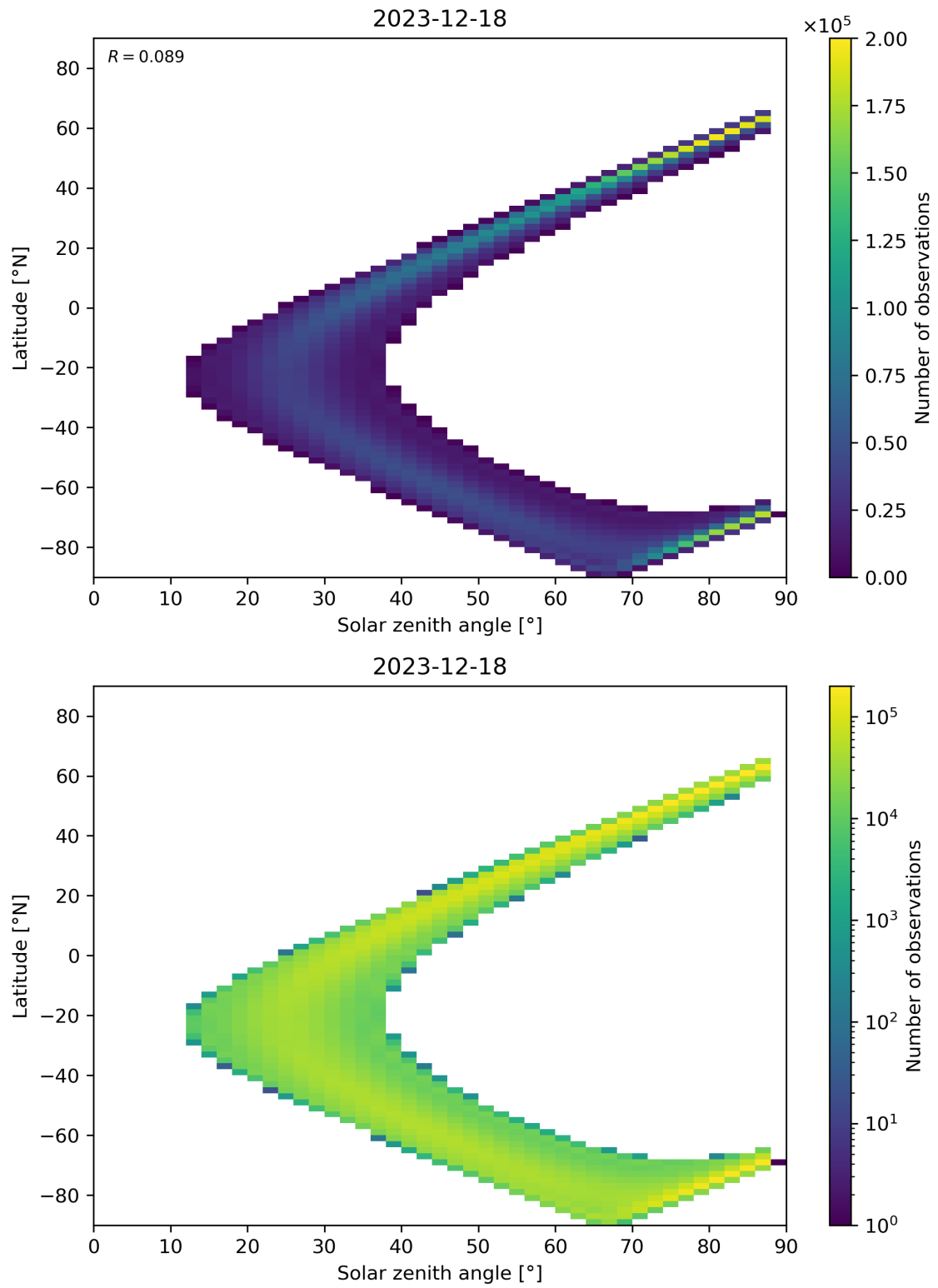
Figure 113: Scatter density plot of “Solar zenith angle” against “Latitude” for 2023-12-17 to 2023-12-19.
