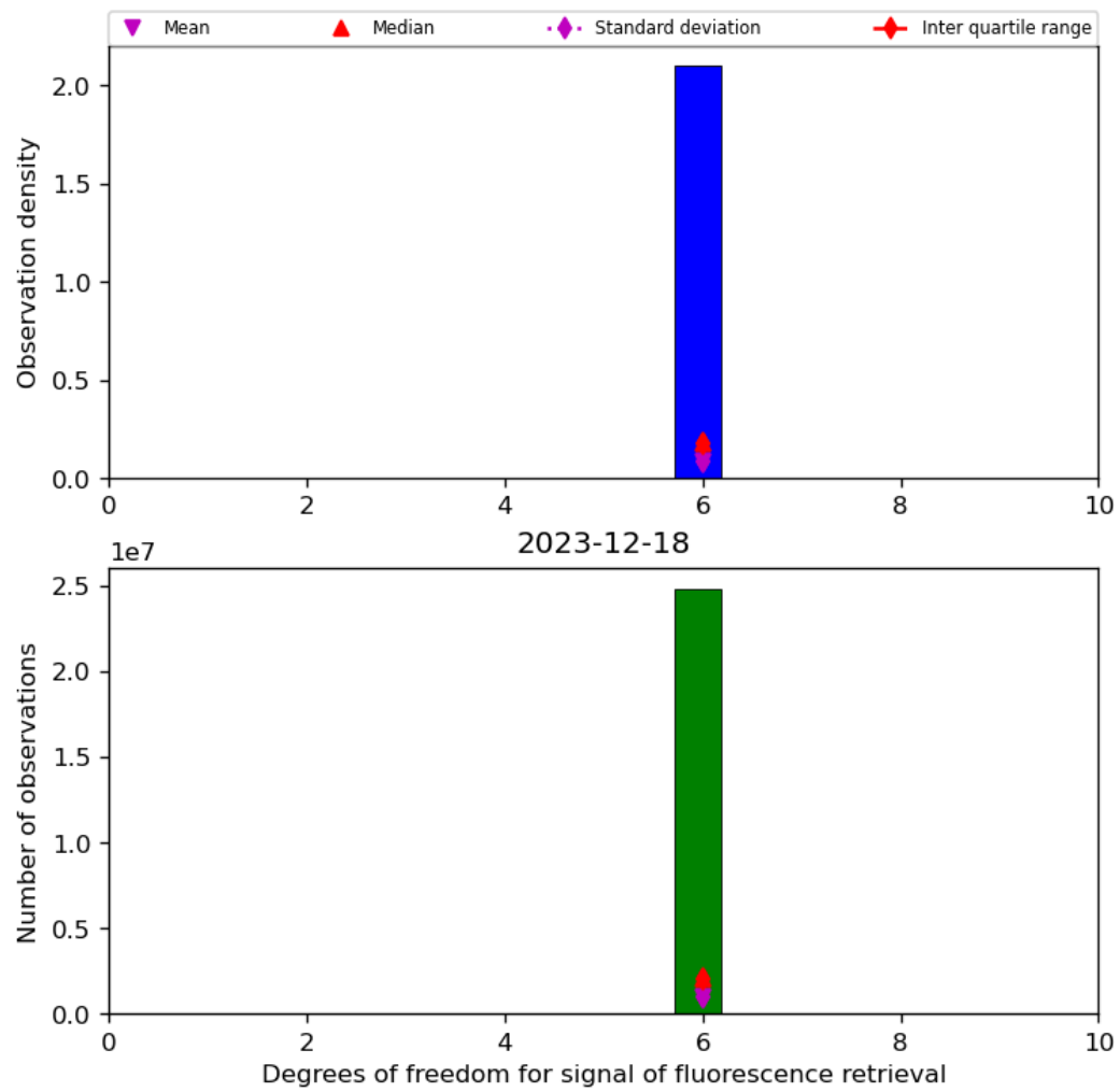
Figure 43: Histogram of “Degrees of freedom for signal of fluorescence retrieval” for 2023-12-17 to 2023-12-19
