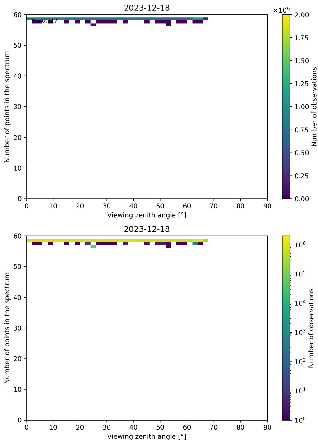
Figure 125: Scatter density plot of “Viewing zenith angle” against “Number of points in the spectrum” for 2023-12-17 to 2023-12-19.
