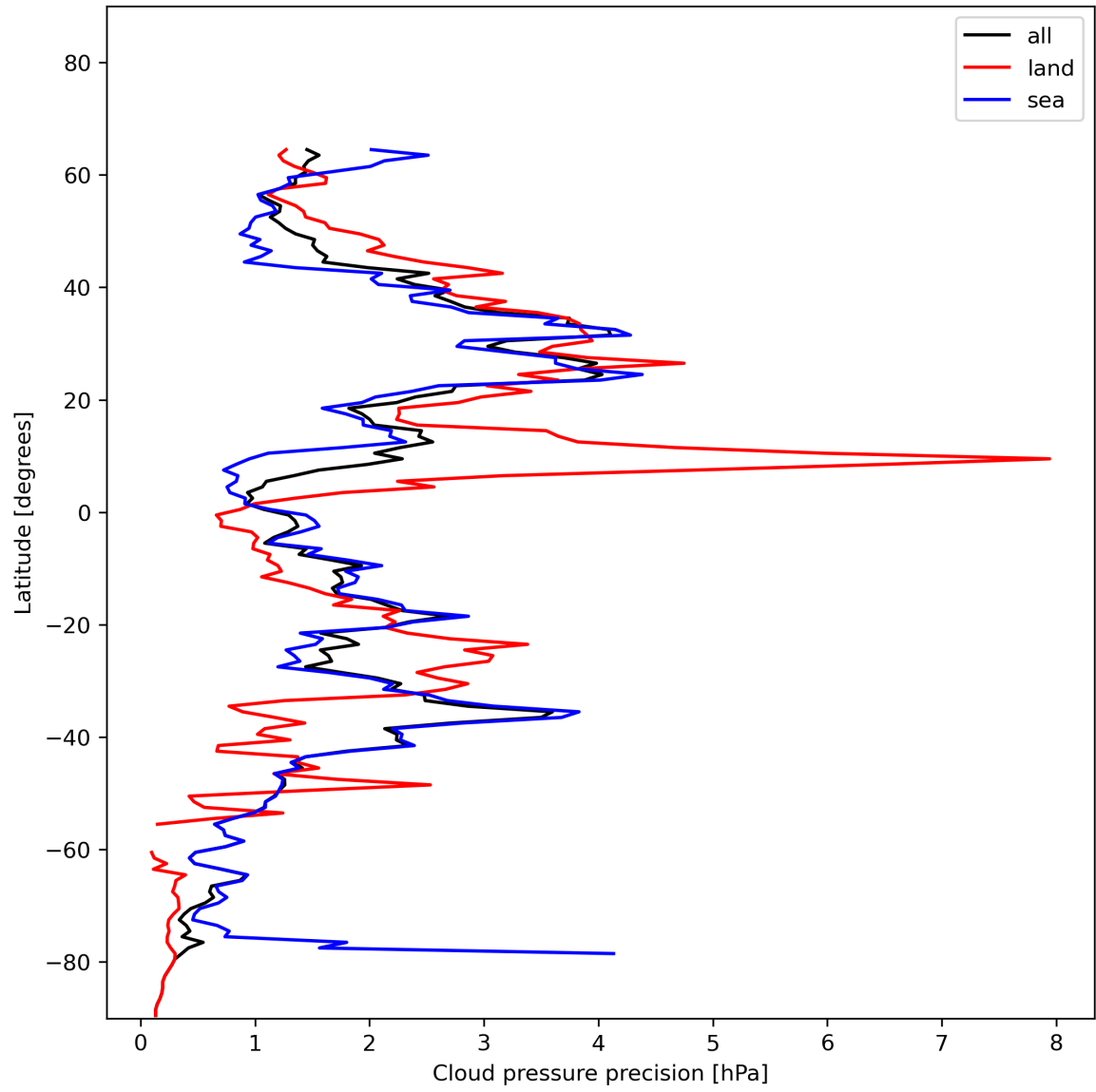
Figure 14: Zonal average of “Cloud pressure precision” for 2023-12-17 to 2023-12-19.
