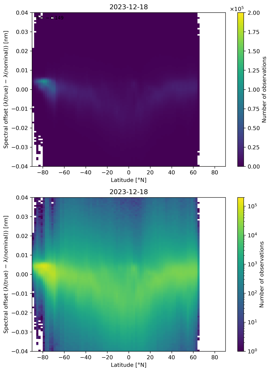
Figure 96: Scatter density plot of “Latitude” against “Spectral offset ( \lambda(\text{true}) - \lambda(\text{nominal}) )” for 2023-12-17 to 2023-12-19.
