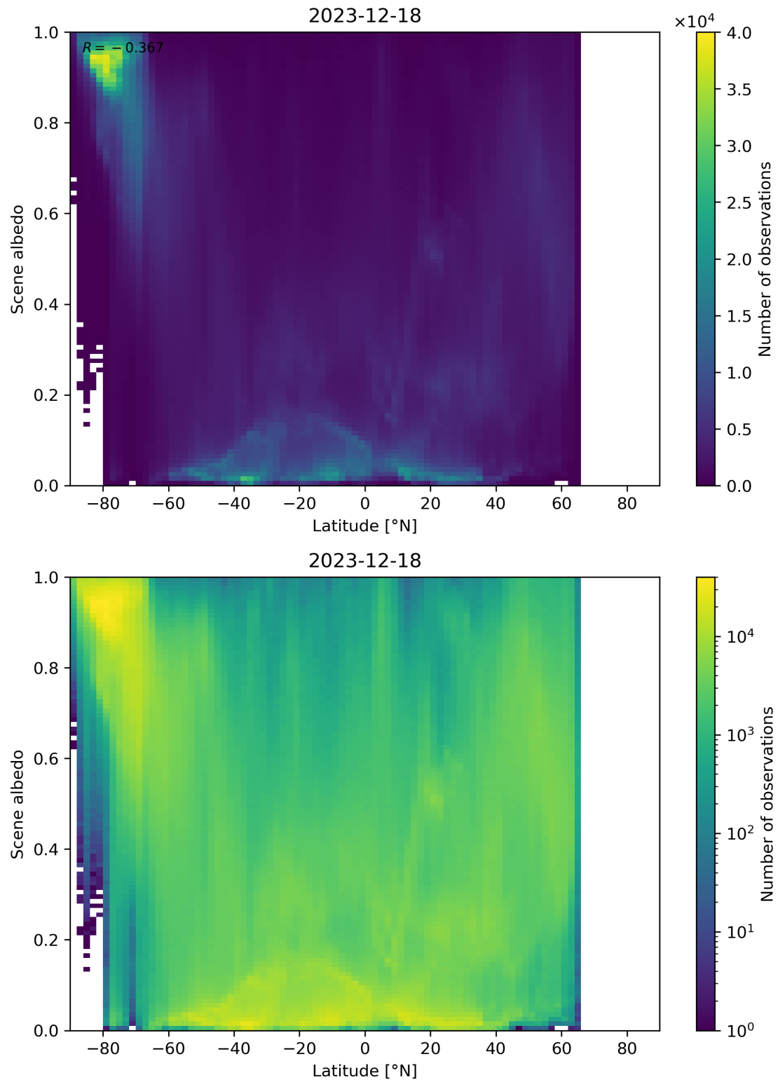
Figure 95: Scatter density plot of “Latitude” against “Scene albedo” for 2023-12-17 to 2023-12-19.
