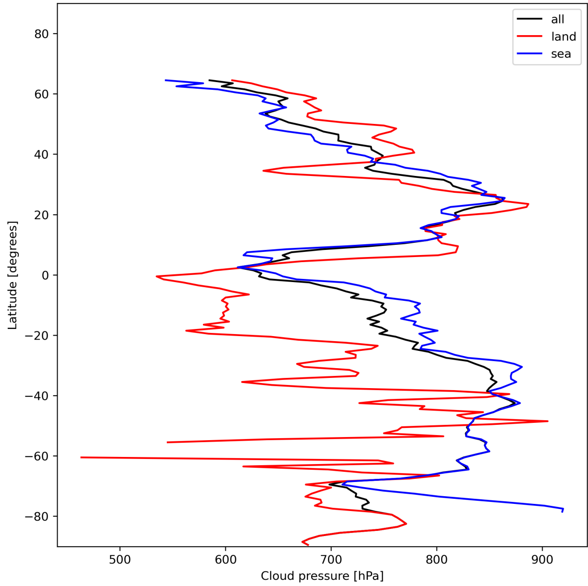
Figure 13: Zonal average of “Cloud pressure” for 2023-12-17 to 2023-12-19.
