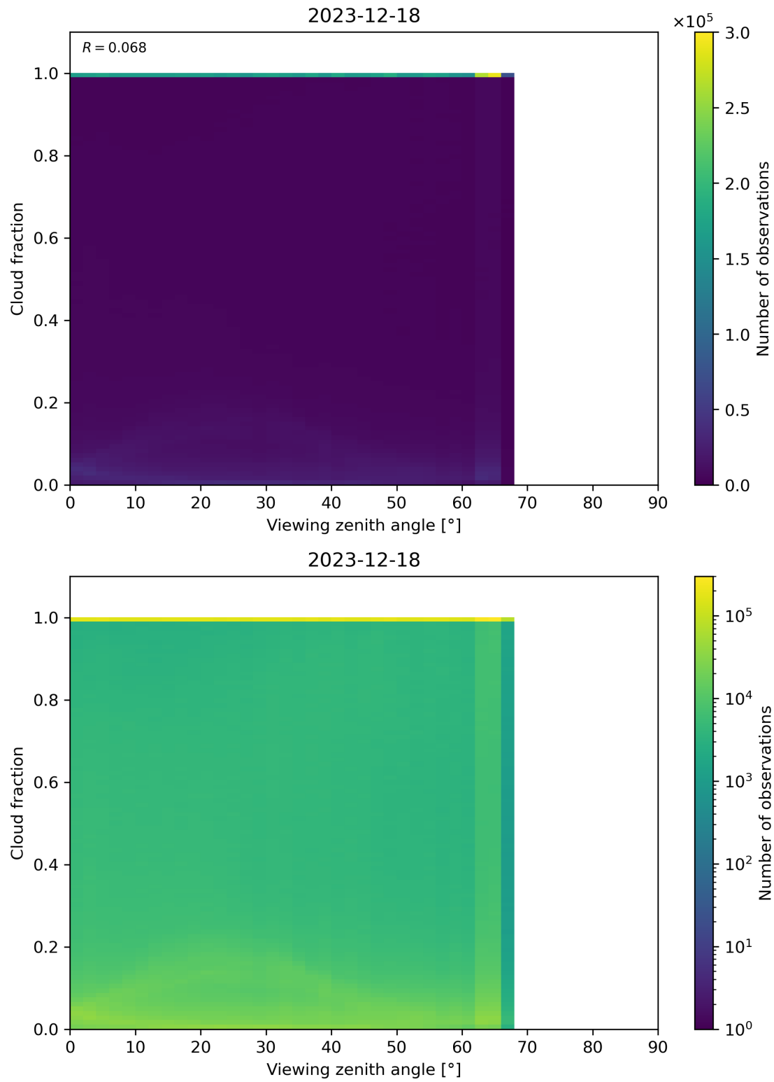
Figure 120: Scatter density plot of “Viewing zenith angle” against “Cloud fraction” for 2023-12-17 to 2023-12-19.
