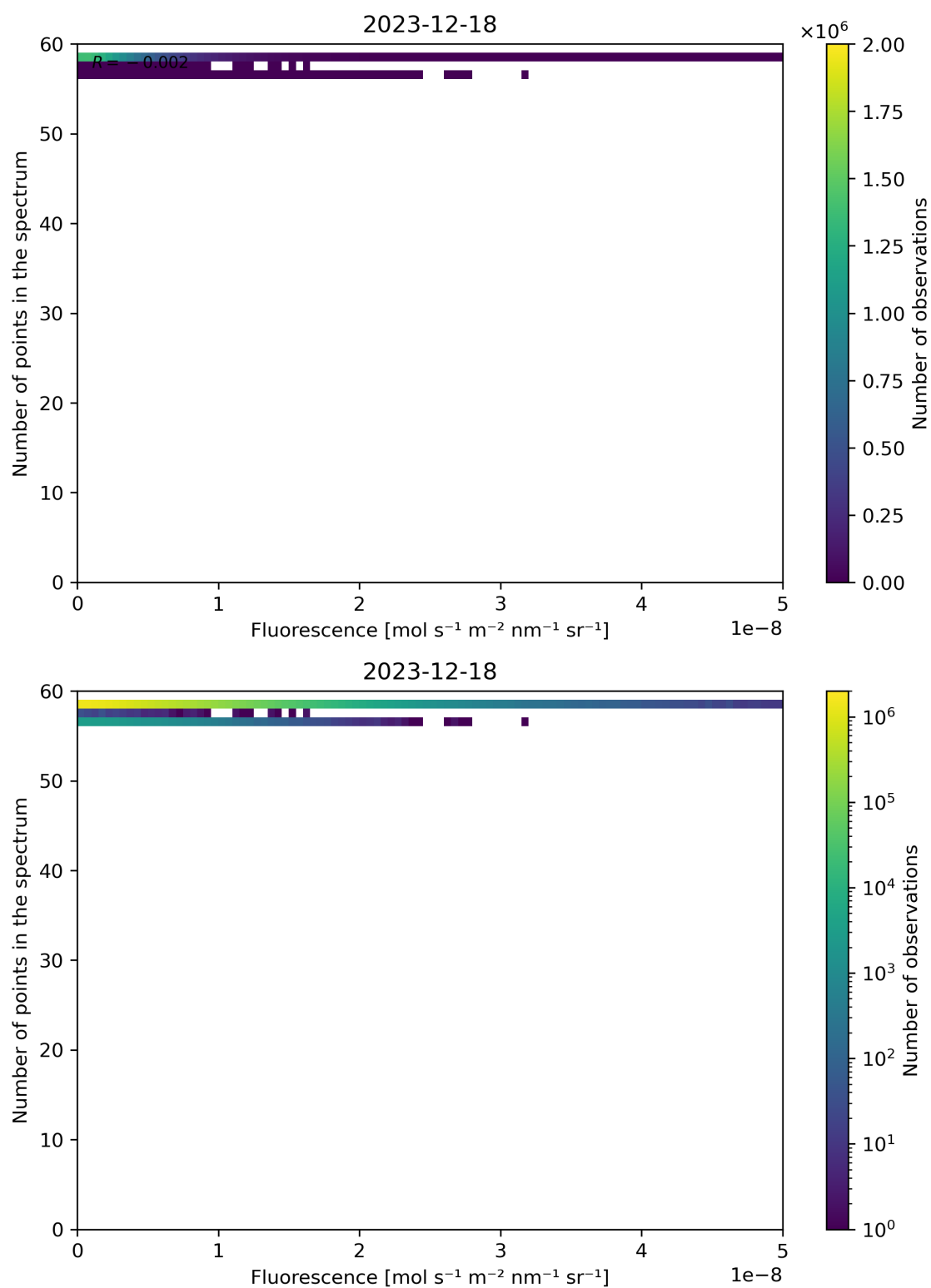
Figure 86: Scatter density plot of “Fluorescence” against “Number of points in the spectrum” for 2023-12-17 to 2023-12-19.
