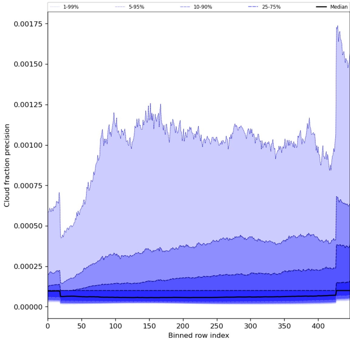
Figure 50: Along track statistics of “Cloud fraction precision” for 2023-12-20 to 2023-12-21
