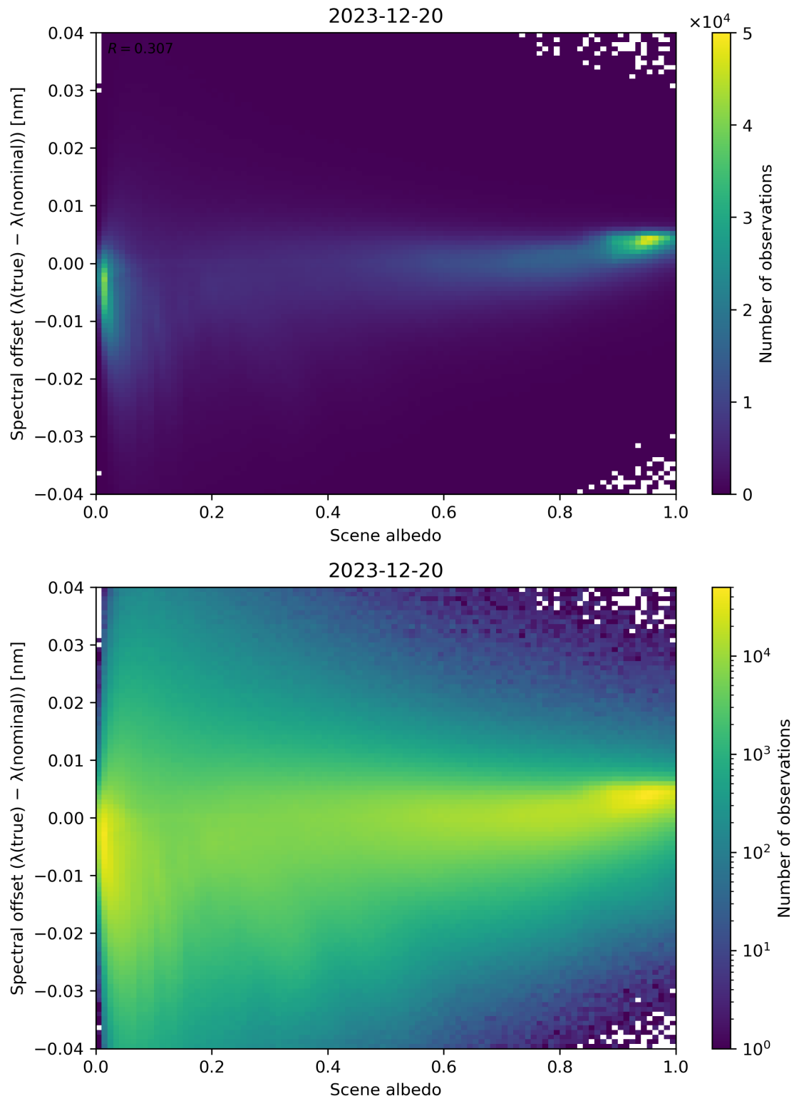
Figure 107: Scatter density plot of “Scene albedo” against “Spectral offset ( \lambda(\text{true}) - \lambda(\text{nominal}) )” for 2023-12-20 to 2023-12-21.
