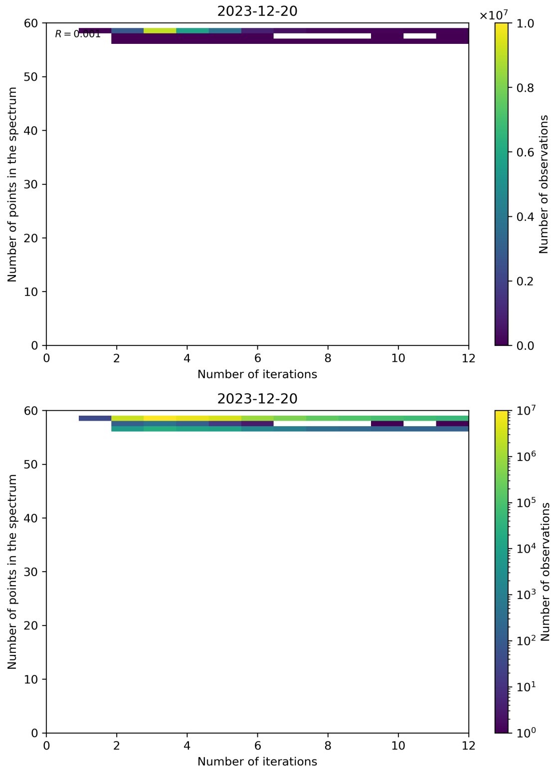
Figure 99: Scatter density plot of “Number of iterations” against “Number of points in the spectrum” for 2023-12-20 to 2023-12-21.
