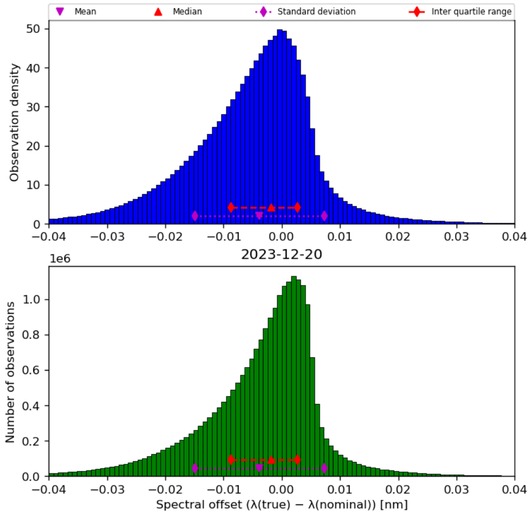
Figure 45: Histogram of “Spectral offset ( \lambda(\text{true}) - \lambda(\text{nominal}) )” for 2023-12-20 to 2023-12-21
