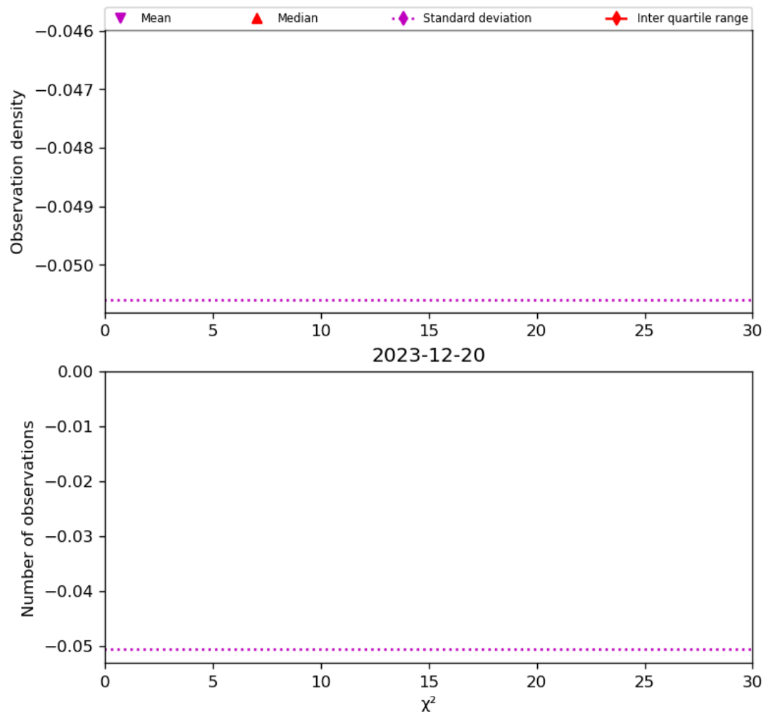
Figure 38: Histogram of “ \chi^2 ” for 2023-12-20 to 2023-12-21
