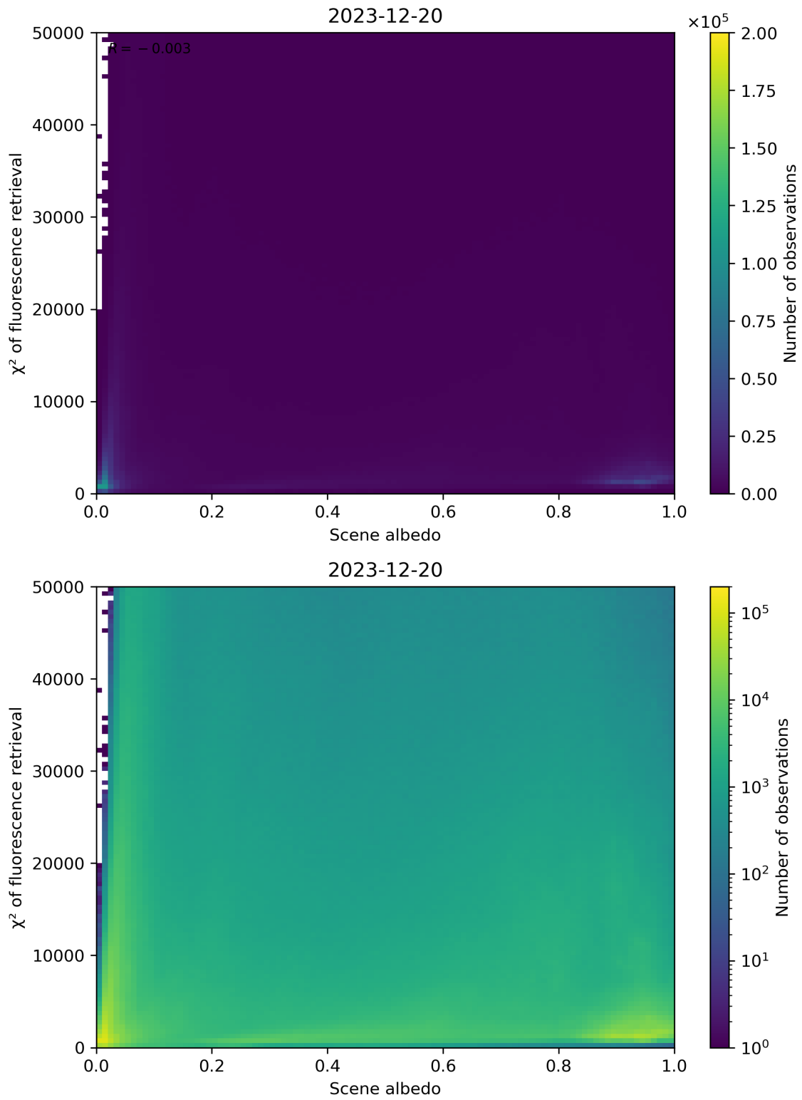
Figure 103: Scatter density plot of “Scene albedo” against “ \chi^2 of fluorescence retrieval” for 2023-12-20 to 2023-12-21.
