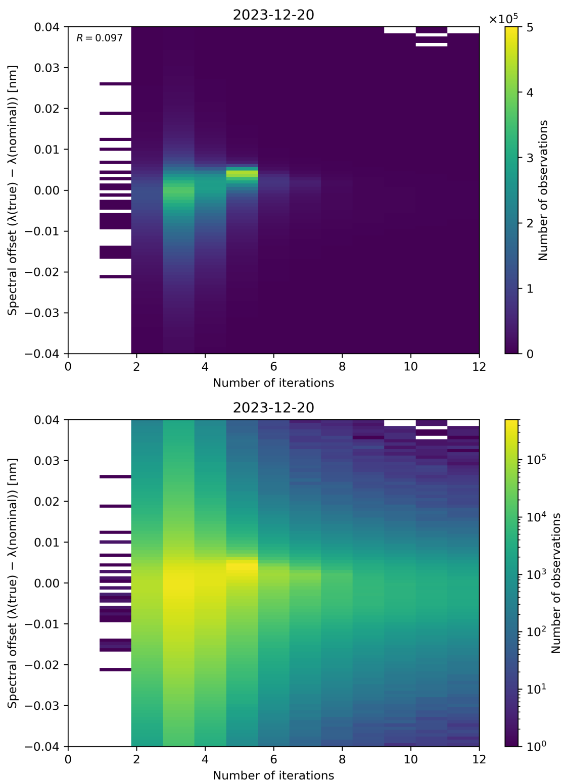
Figure 100: Scatter density plot of “Number of iterations” against “Spectral offset ( \lambda(\text{true}) - \lambda(\text{nominal}) )” for 2023-12-20 to 2023-12-21.
