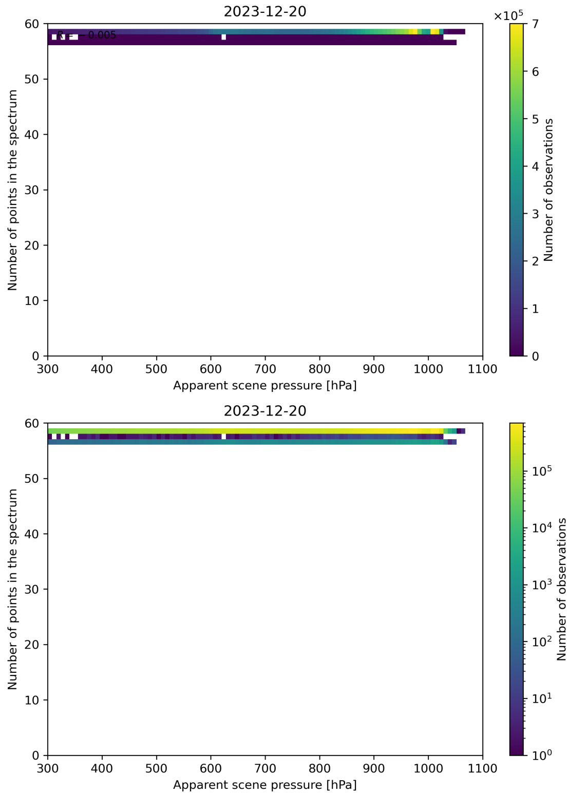
Figure 66: Scatter density plot of “Apparent scene pressure” against “Number of points in the spectrum” for 2023-12-20 to 2023-12-21.
