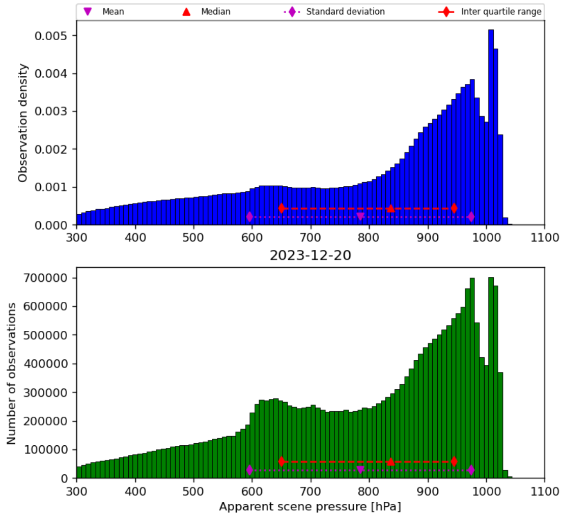
Figure 36: Histogram of “Apparent scene pressure” for 2023-12-20 to 2023-12-21
