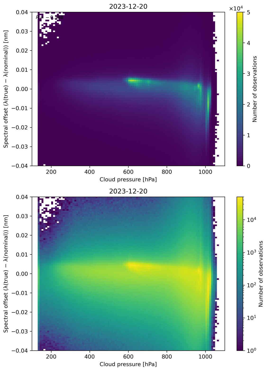
Figure 84: Scatter density plot of “Cloud pressure” against “Spectral offset ( \lambda(\text{true}) - \lambda(\text{nominal}) )” for 2023-12-20 to 2023-12-21.
