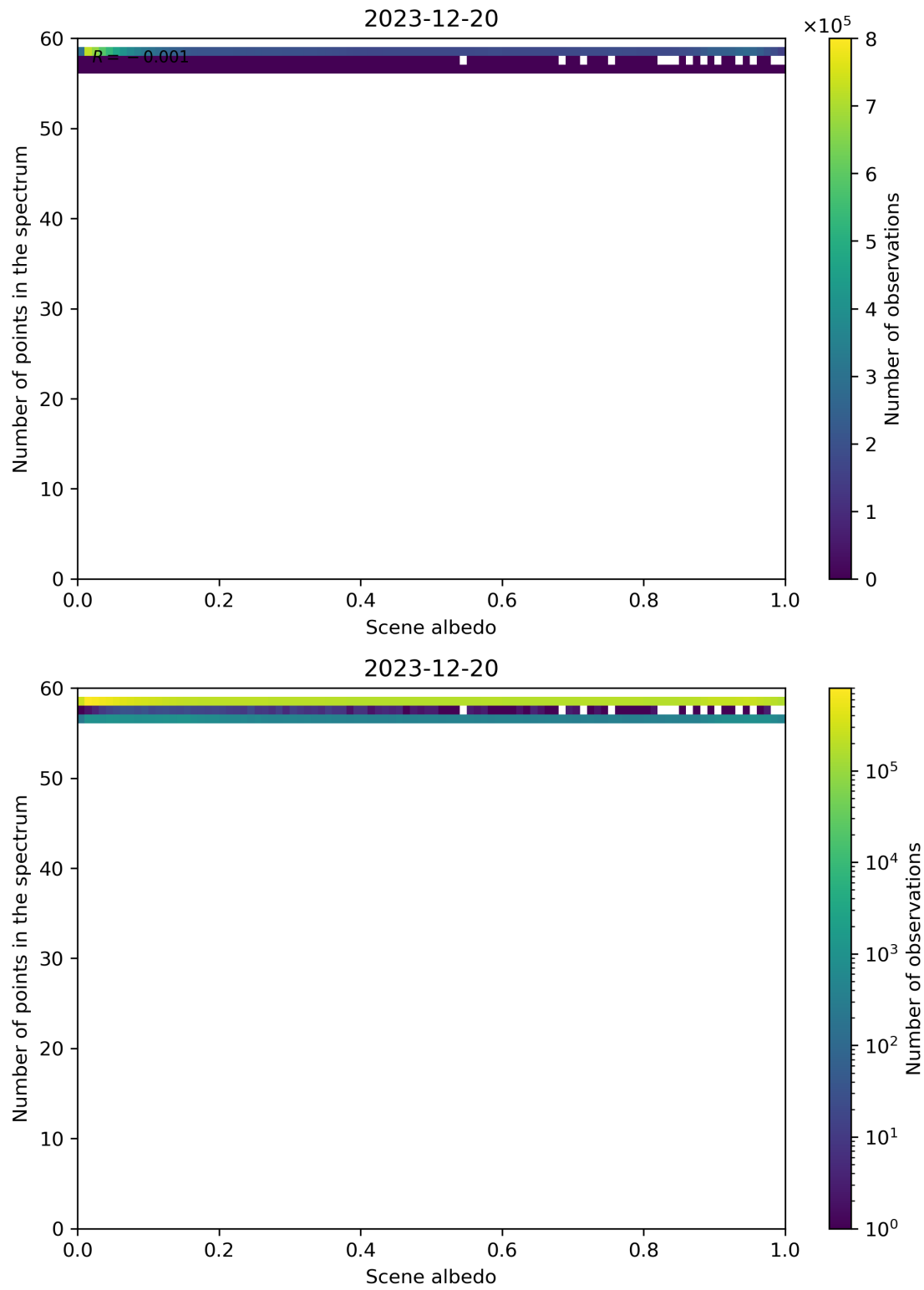
Figure 106: Scatter density plot of “Scene albedo” against “Number of points in the spectrum” for 2023-12-20 to 2023-12-21.
