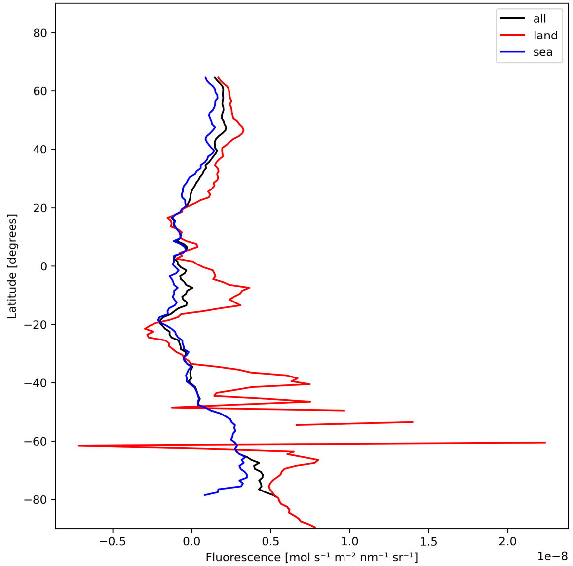
Figure 23: Zonal average of “Fluorescence” for 2023-12-20 to 2023-12-21.
