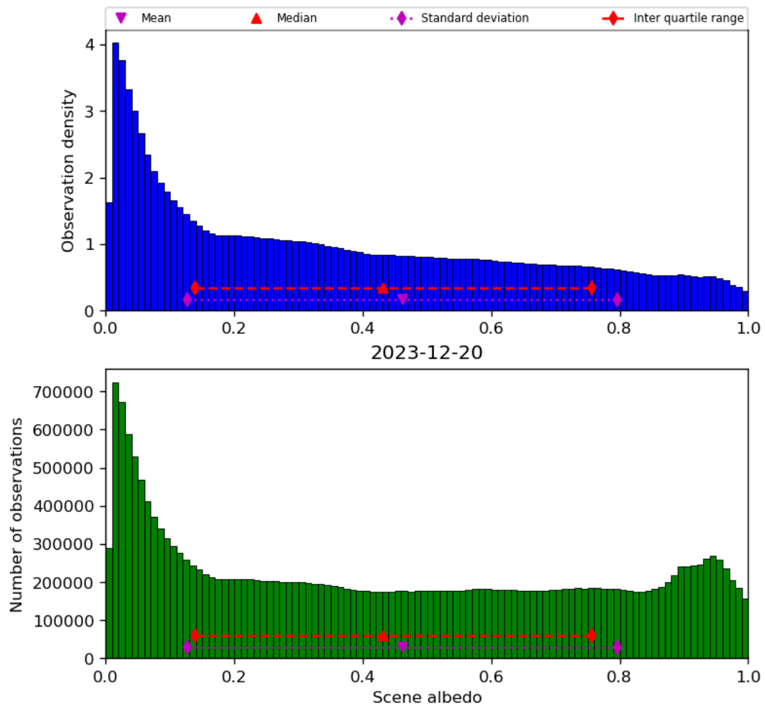
Figure 34: Histogram of “Scene albedo” for 2023-12-20 to 2023-12-21
