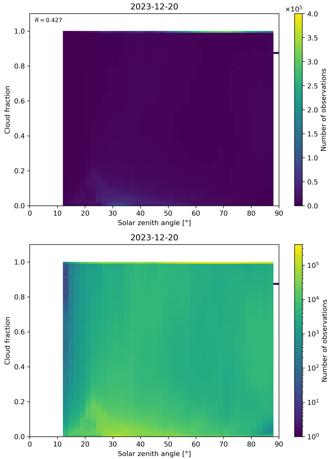
Figure 110: Scatter density plot of “Solar zenith angle” against “Cloud fraction” for 2023-12-20 to 2023-12-21.
