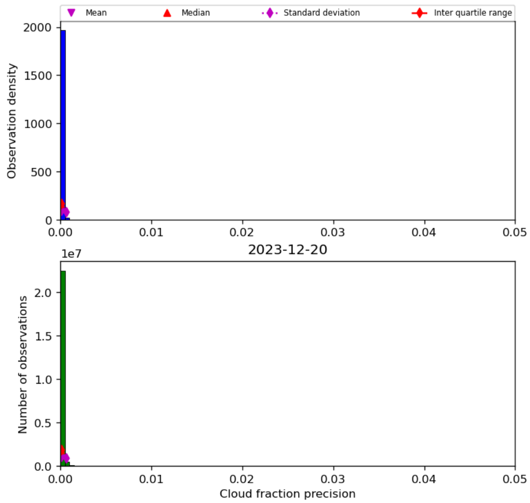
Figure 33: Histogram of “Cloud fraction precision” for 2023-12-20 to 2023-12-21
