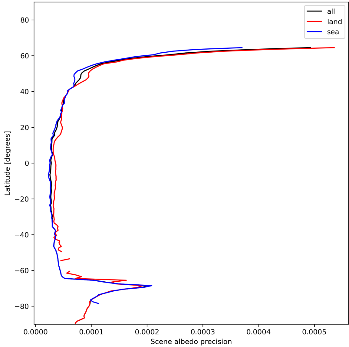
Figure 18: Zonal average of “Scene albedo precision” for 2023-12-20 to 2023-12-21.
