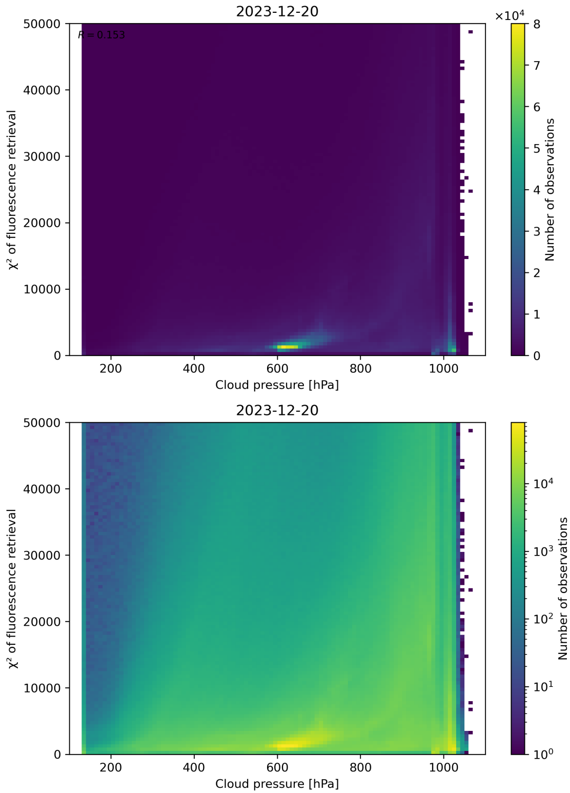
Figure 78: Scatter density plot of “Cloud pressure” against “ \chi^2 of fluorescence retrieval” for 2023-12-20 to 2023-12-21.
