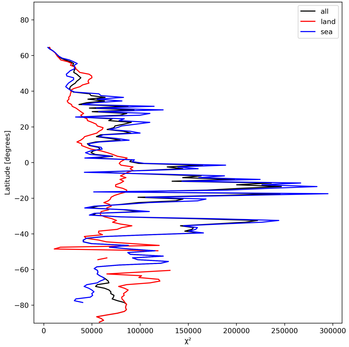
Figure 21: Zonal average of “ \chi^2 ” for 2023-12-20 to 2023-12-21.
