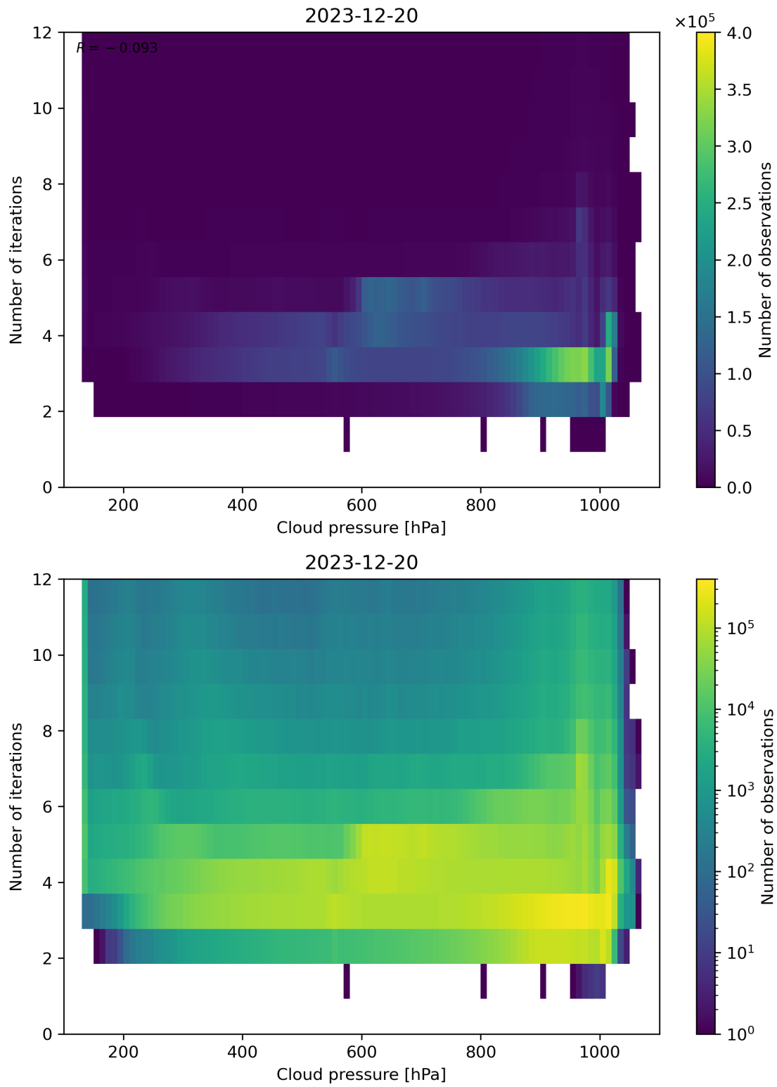
Figure 81: Scatter density plot of “Cloud pressure” against “Number of iterations” for 2023-12-20 to 2023-12-21.
