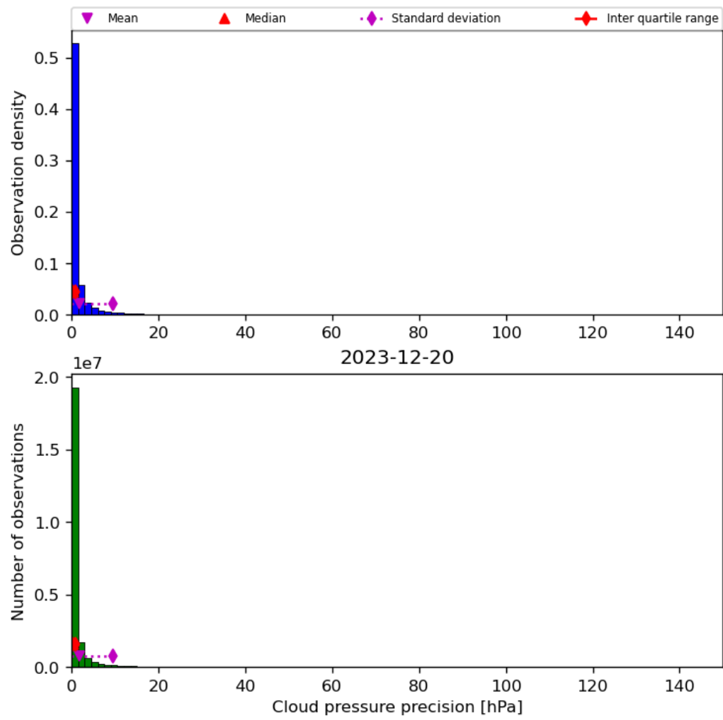
Figure 31: Histogram of “Cloud pressure precision” for 2023-12-20 to 2023-12-21
