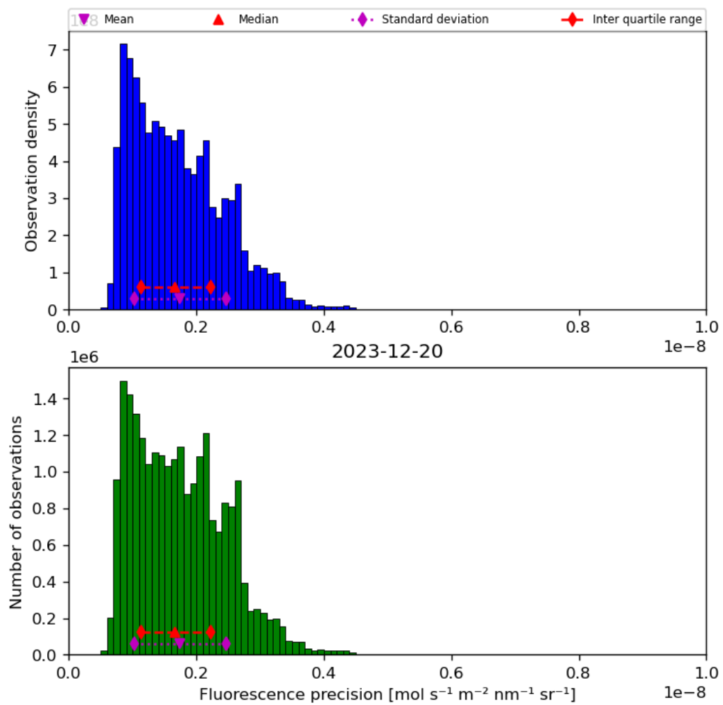
Figure 41: Histogram of “Fluorescence precision” for 2023-12-20 to 2023-12-21
