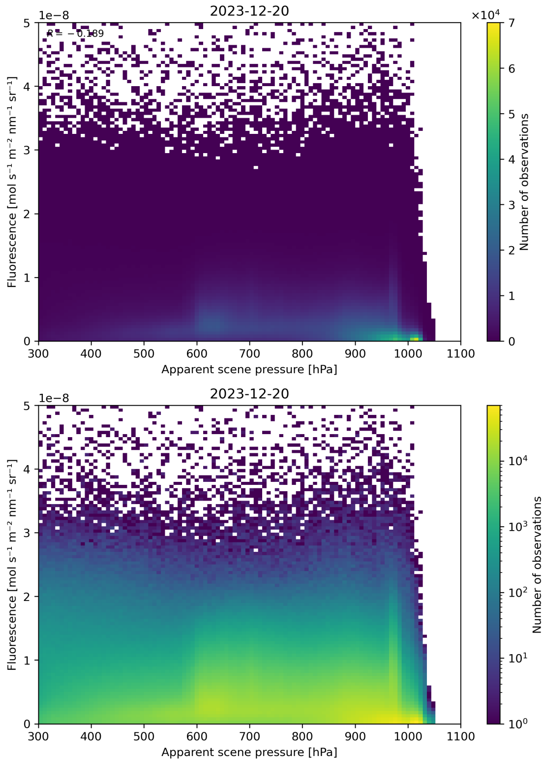
Figure 64: Scatter density plot of “Apparent scene pressure” against “Fluorescence” for 2023-12-20 to 2023-12-21.
