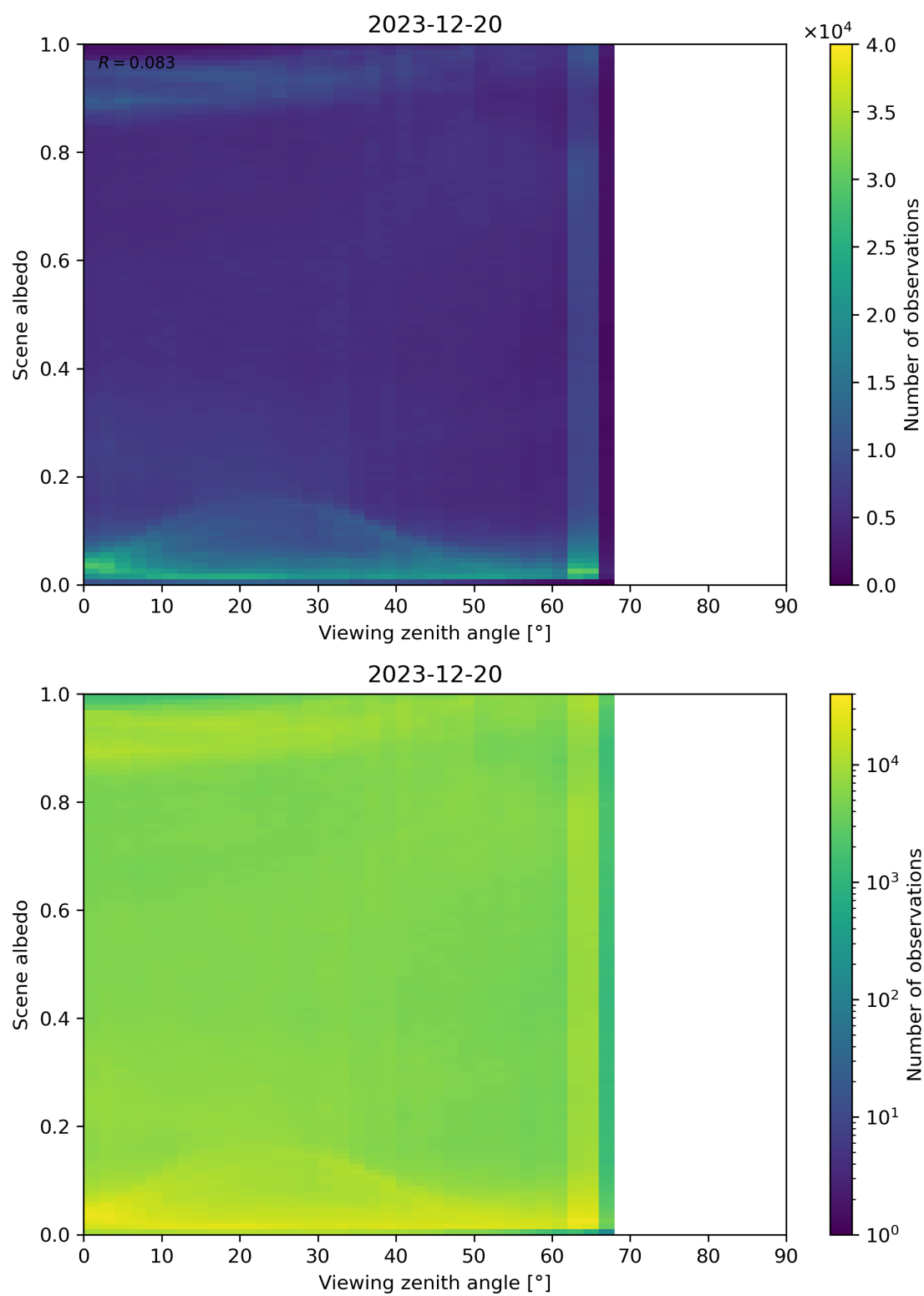
Figure 126: Scatter density plot of “Viewing zenith angle” against “Scene albedo” for 2023-12-20 to 2023-12-21.
