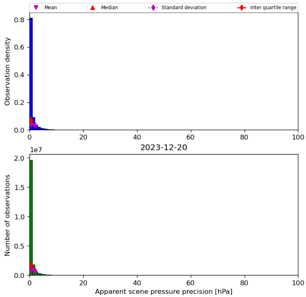
Figure 37: Histogram of “Apparent scene pressure precision” for 2023-12-20 to 2023-12-21
