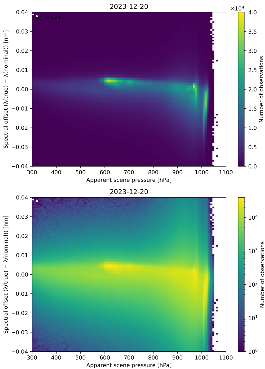
Figure 67: Scatter density plot of “Apparent scene pressure” against “Spectral offset ( \lambda(\text{true}) - \lambda(\text{nominal}) )” for 2023-12-20 to 2023-12-21.
