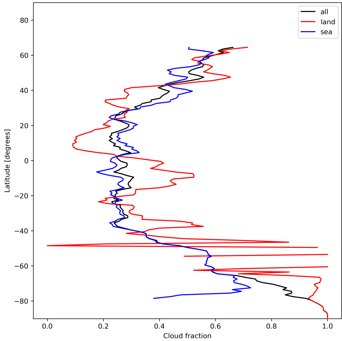
Figure 15: Zonal average of “Cloud fraction” for 2023-12-20 to 2023-12-21.
