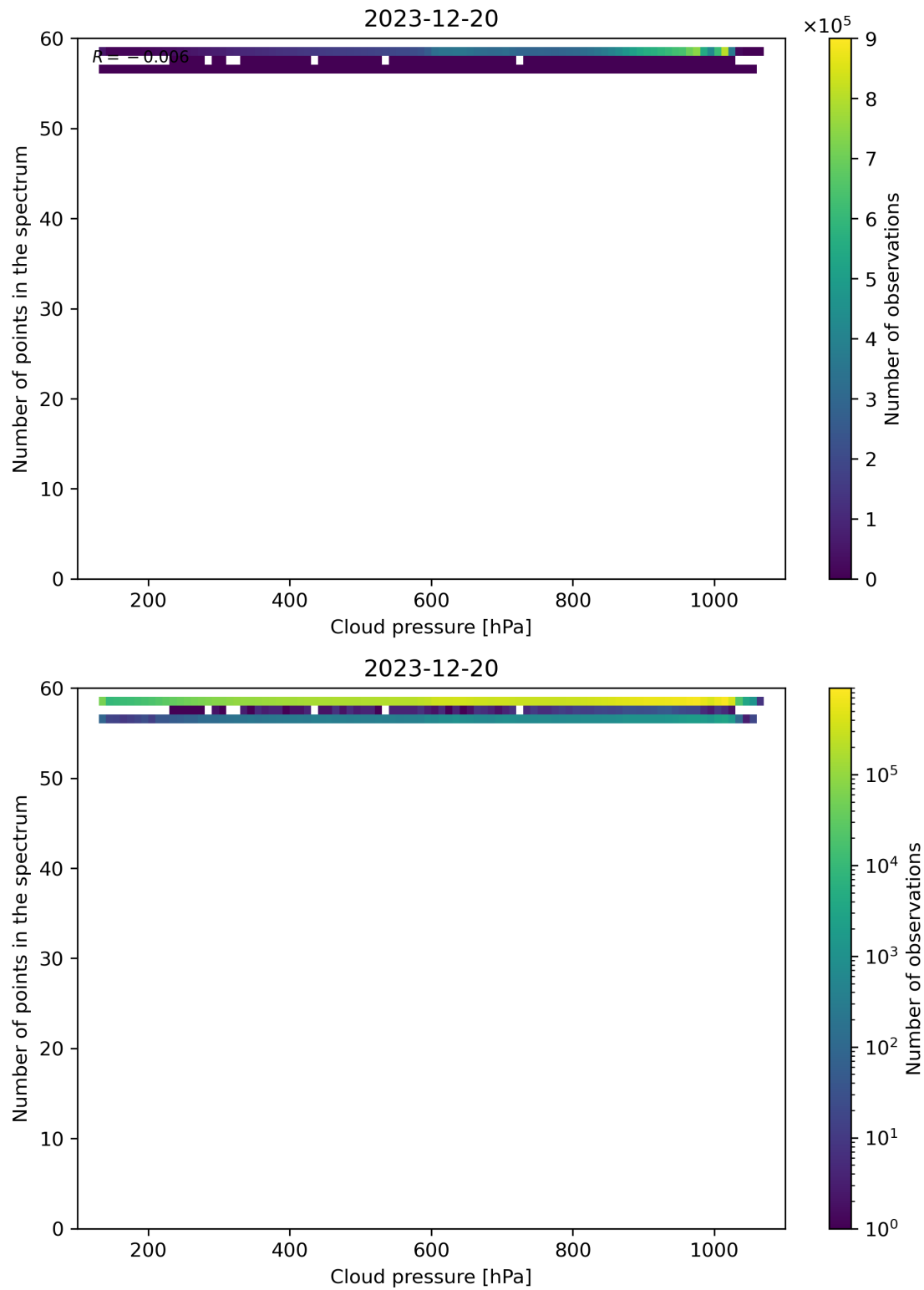
Figure 82: Scatter density plot of “Cloud pressure” against “Number of points in the spectrum” for 2023-12-20 to 2023-12-21.
