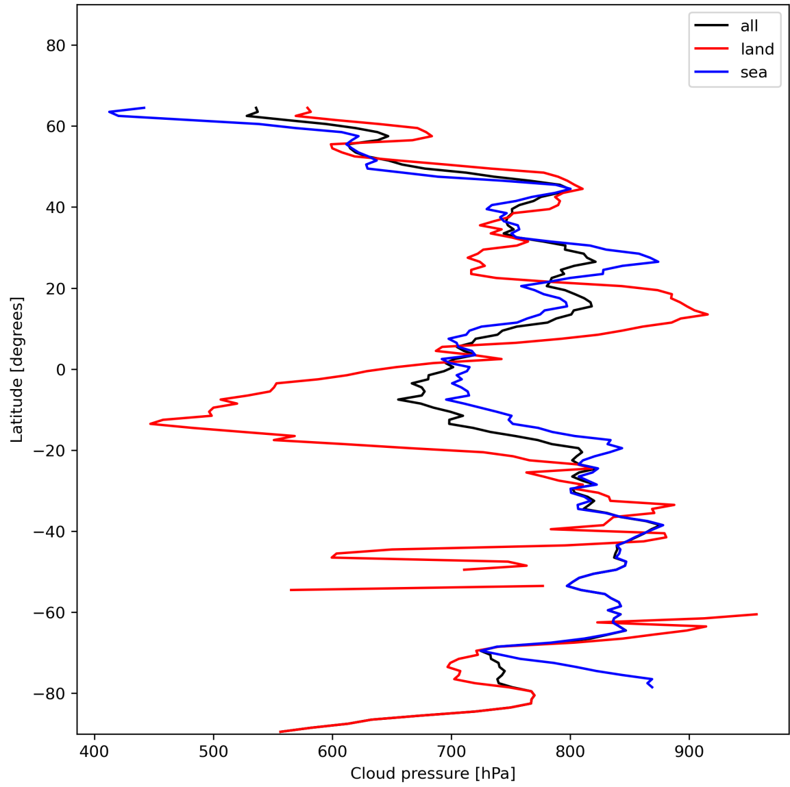
Figure 13: Zonal average of “Cloud pressure” for 2023-12-20 to 2023-12-21.
