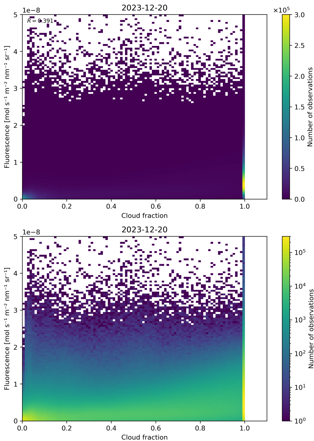
Figure 72: Scatter density plot of “Cloud fraction” against “Fluorescence” for 2023-12-20 to 2023-12-21.
