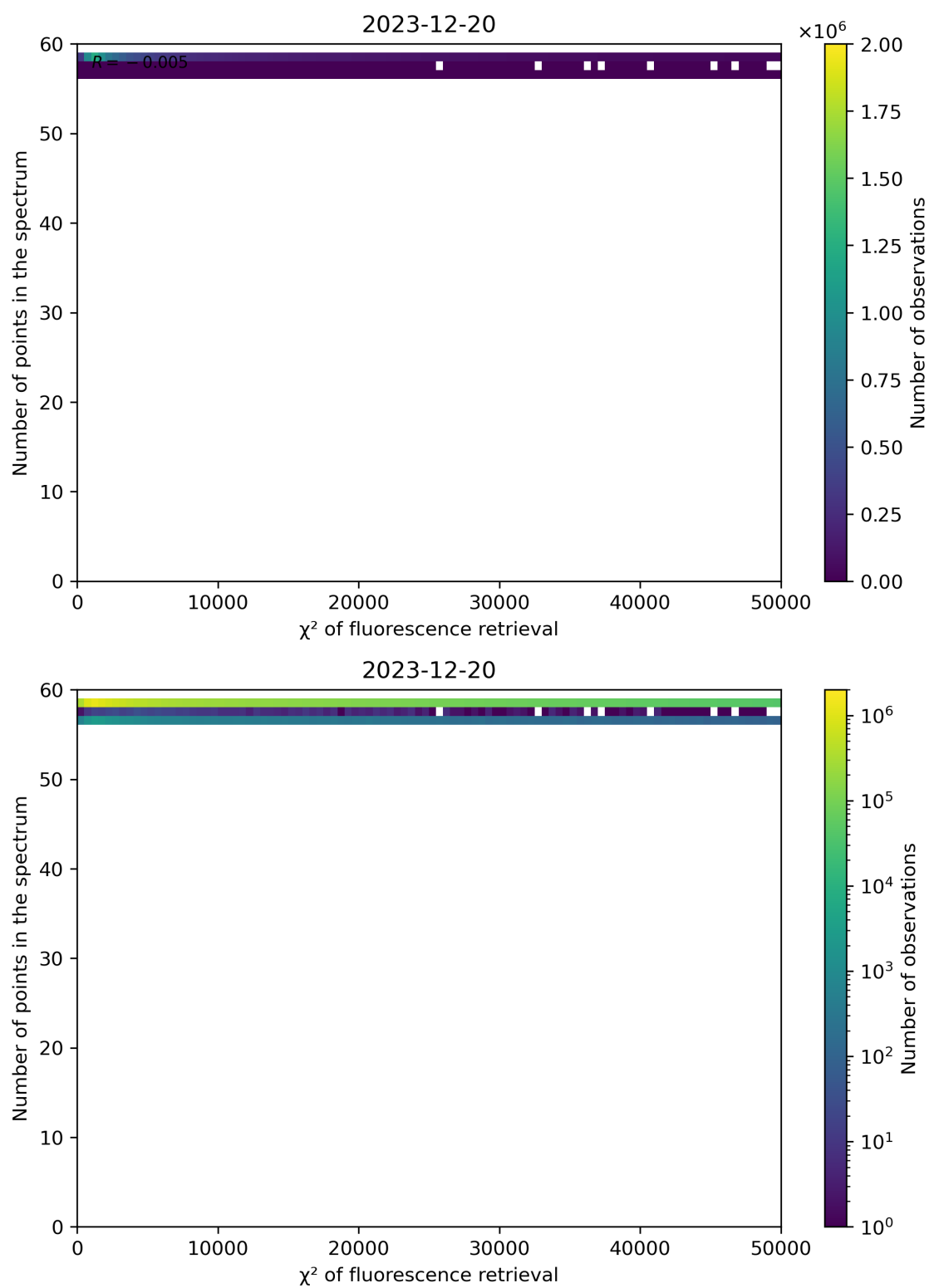
Figure 68: Scatter density plot of " \chi^2 of fluorescence retrieval" against "Number of points in the spectrum" for 2023-12-20 to 2023-12-21.
