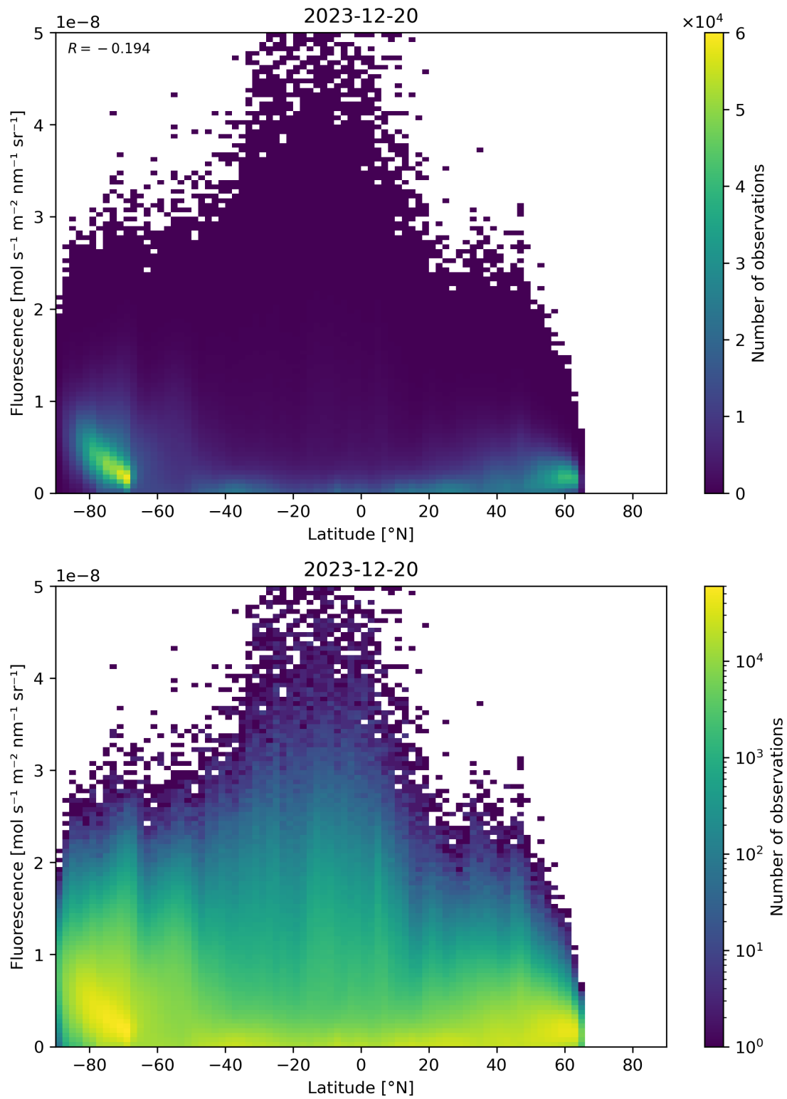
Figure 92: Scatter density plot of “Latitude” against “Fluorescence” for 2023-12-20 to 2023-12-21.
