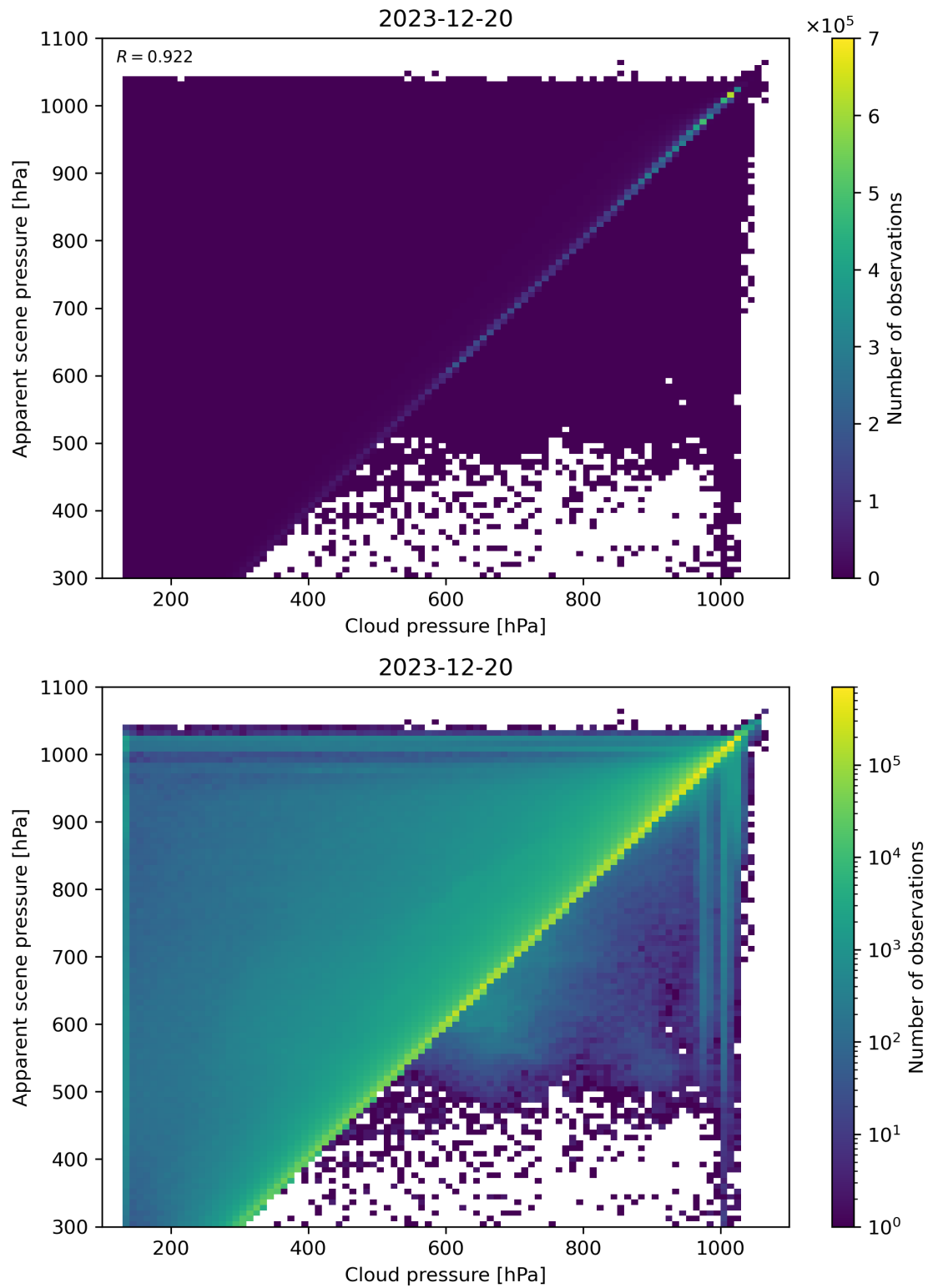
Figure 77: Scatter density plot of “Cloud pressure” against “Apparent scene pressure” for 2023-12-20 to 2023-12-21.
