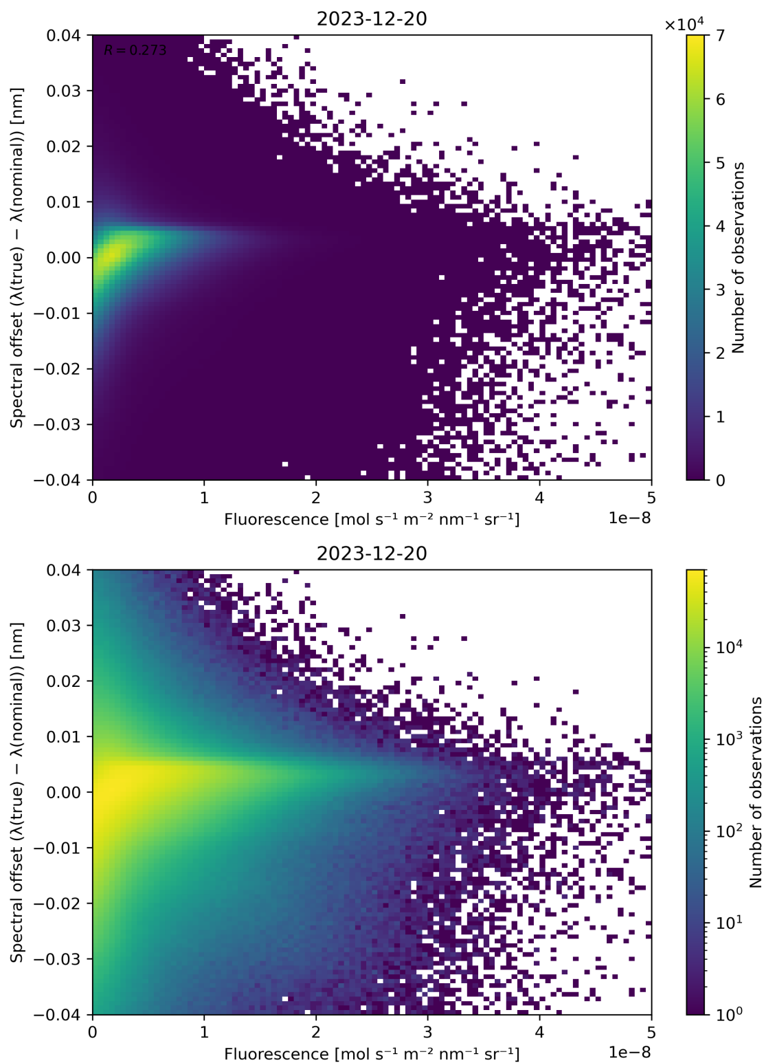
Figure 87: Scatter density plot of “Fluorescence” against “Spectral offset ( \lambda(\text{true}) - \lambda(\text{nominal}) )” for 2023-12-20 to 2023-12-21.
