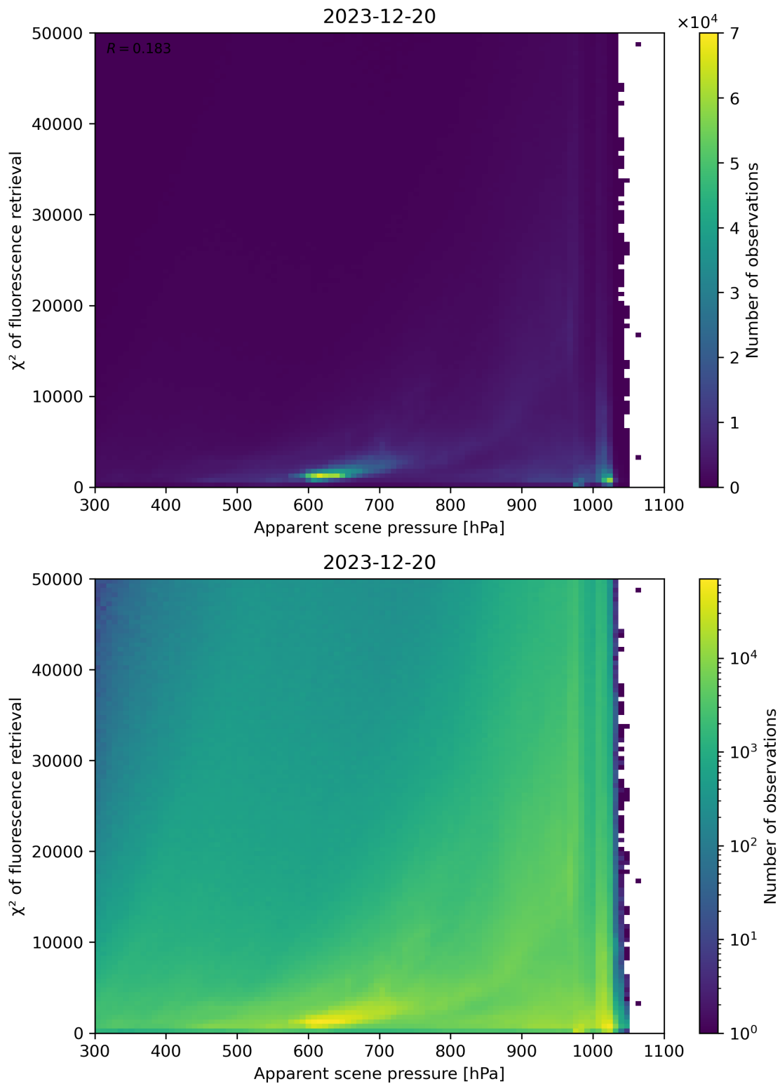
Figure 63: Scatter density plot of “Apparent scene pressure” against “ \chi^2 of fluorescence retrieval” for 2023-12-20 to 2023-12-21.
