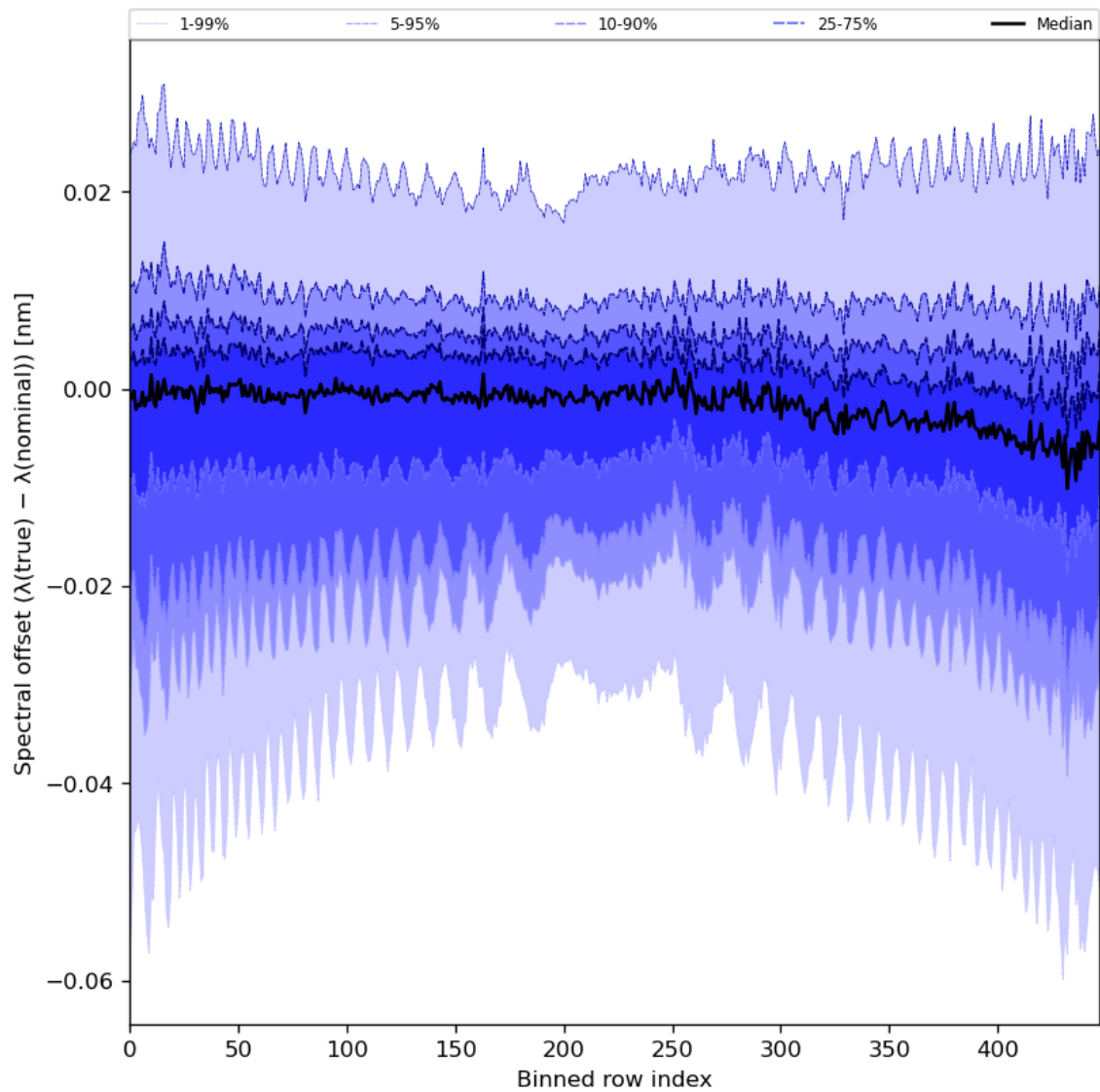
Figure 62: Along track statistics of “Spectral offset ( \lambda(\text{true}) - \lambda(\text{nominal}) )” for 2023-12-20 to 2023-12-21
