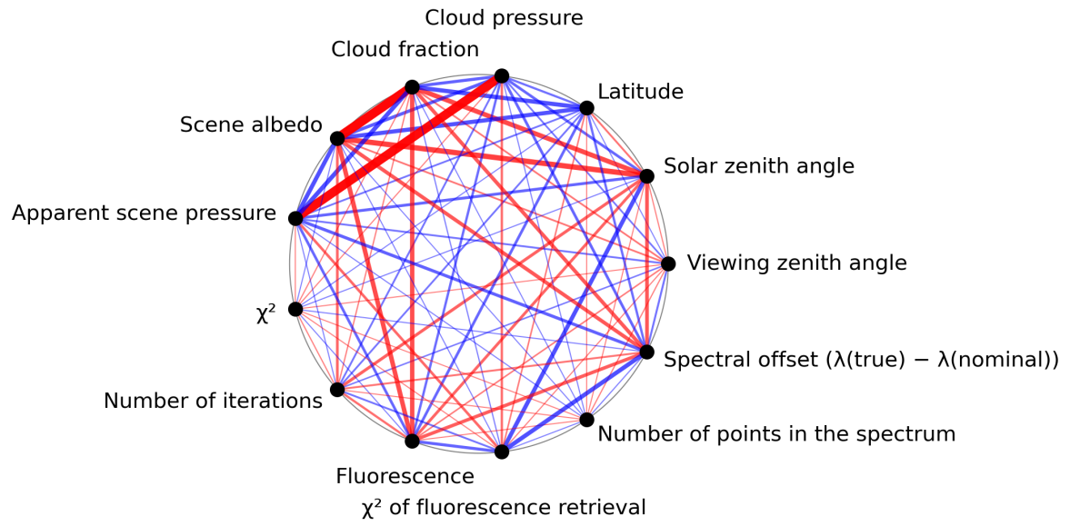
Figure 1: Map of correlation graph for 2023-12-20 to 2023-12-21.
