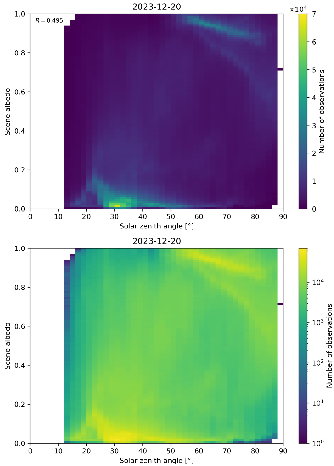
Figure 116: Scatter density plot of “Solar zenith angle” against “Scene albedo” for 2023-12-20 to 2023-12-21.
