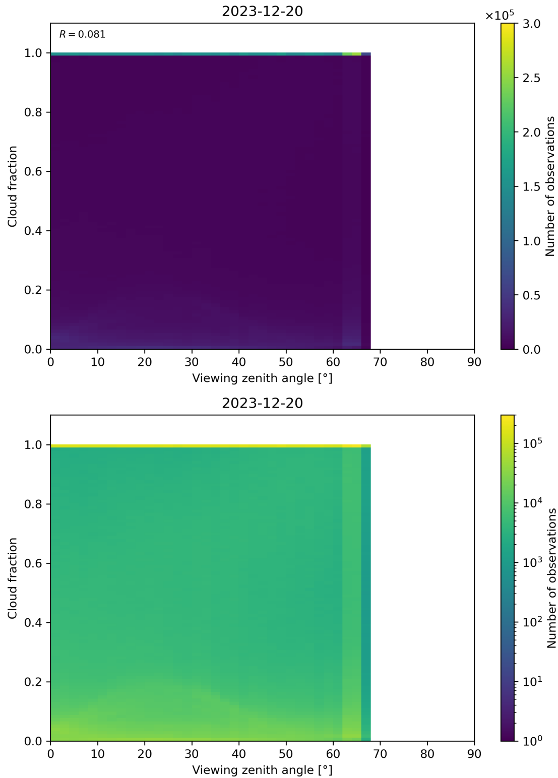
Figure 120: Scatter density plot of “Viewing zenith angle” against “Cloud fraction” for 2023-12-20 to 2023-12-21.
