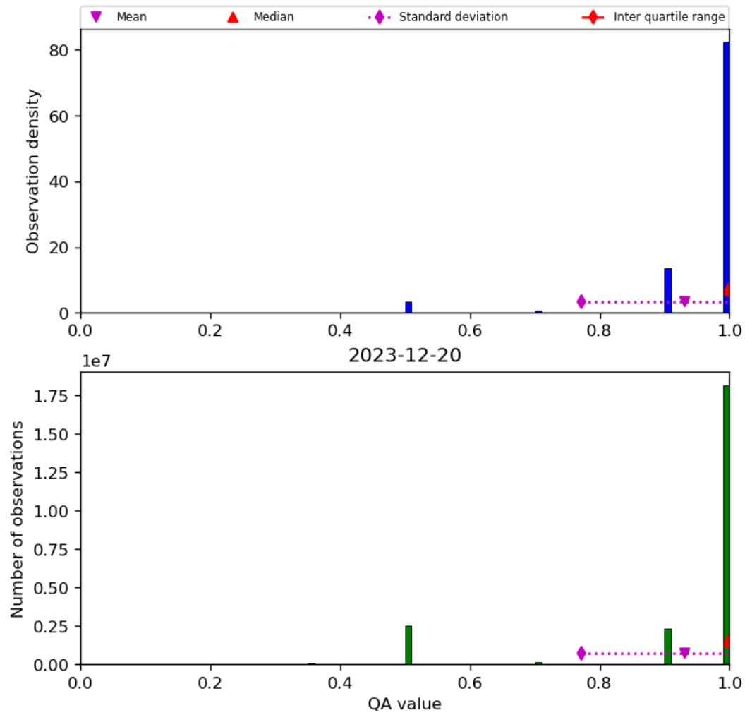
Figure 29: Histogram of “QA value” for 2023-12-20 to 2023-12-21
