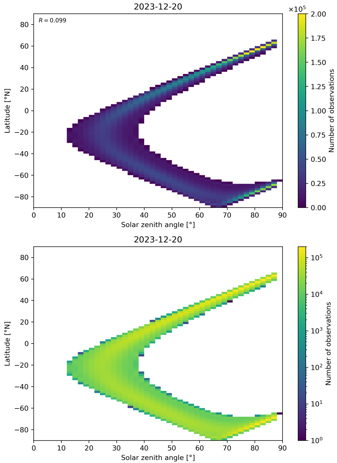
Figure 113: Scatter density plot of “Solar zenith angle” against “Latitude” for 2023-12-20 to 2023-12-21.
