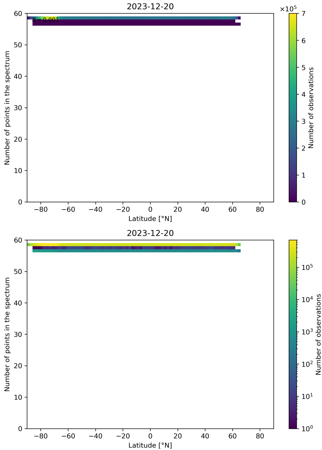
Figure 94: Scatter density plot of “Latitude” against “Number of points in the spectrum” for 2023-12-20 to 2023-12-21.
