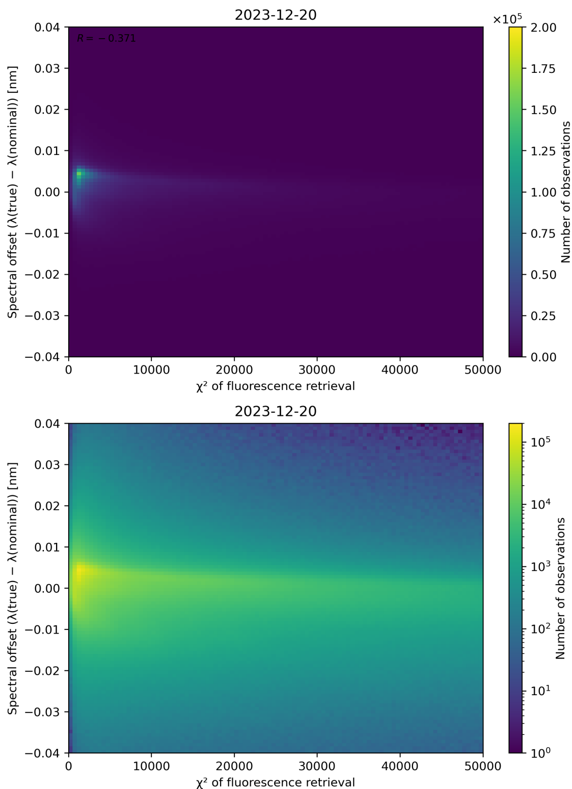
Figure 69: Scatter density plot of “ \chi^2 of fluorescence retrieval” against “Spectral offset ( \lambda(\text{true}) - \lambda(\text{nominal}) )” for 2023-12-20 to 2023-12-21.
