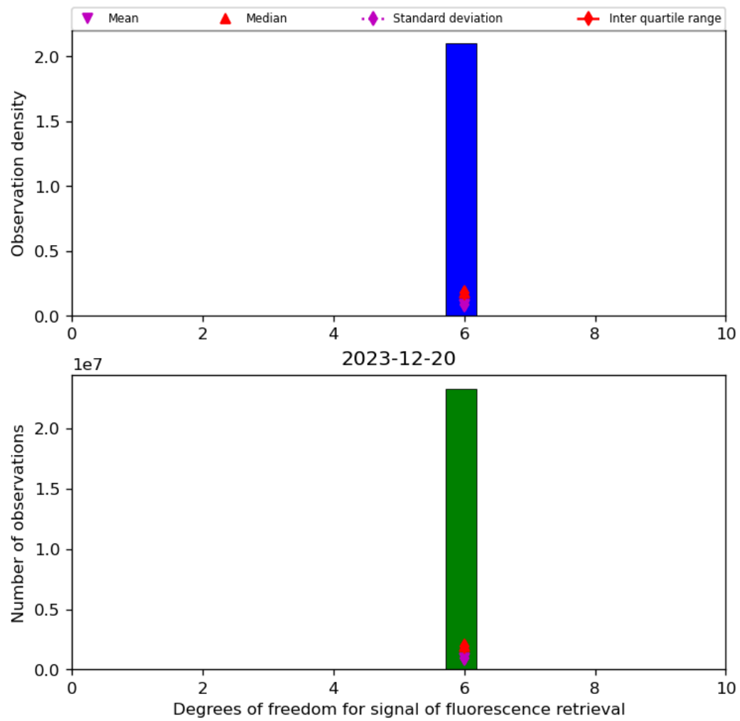
Figure 43: Histogram of “Degrees of freedom for signal of fluorescence retrieval” for 2023-12-20 to 2023-12-21
