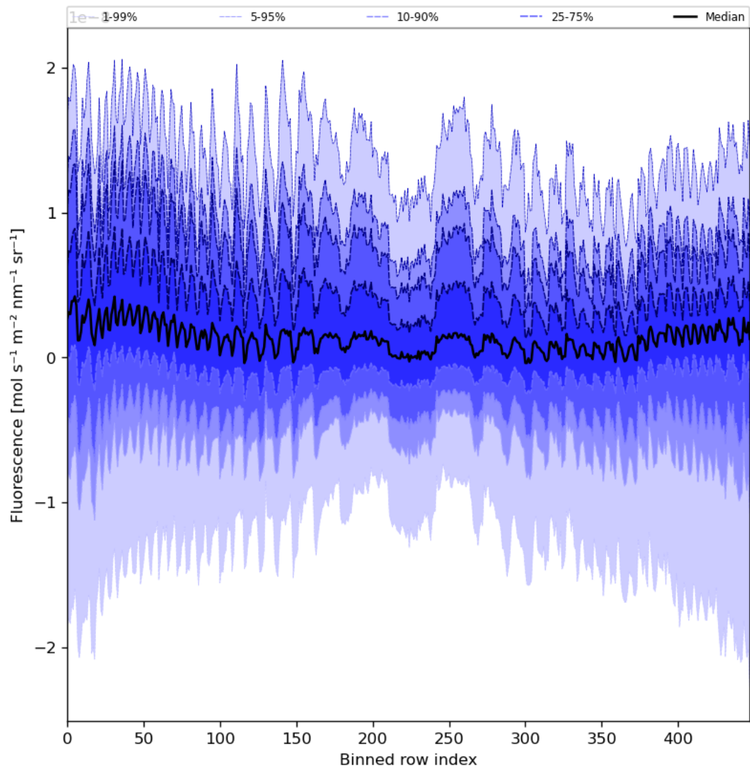
Figure 57: Along track statistics of “Fluorescence” for 2023-12-20 to 2023-12-21
