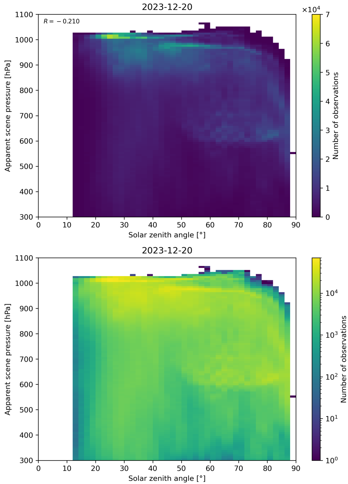
Figure 108: Scatter density plot of “Solar zenith angle” against “Apparent scene pressure” for 2023-12-20 to 2023-12-21.
