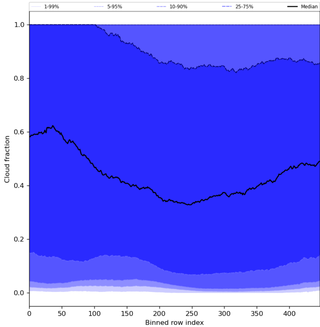
Figure 49: Along track statistics of “Cloud fraction” for 2023-12-20 to 2023-12-21
