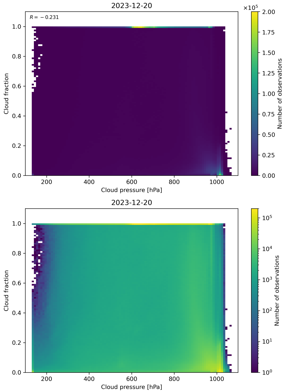
Figure 79: Scatter density plot of “Cloud pressure” against “Cloud fraction” for 2023-12-20 to 2023-12-21.
