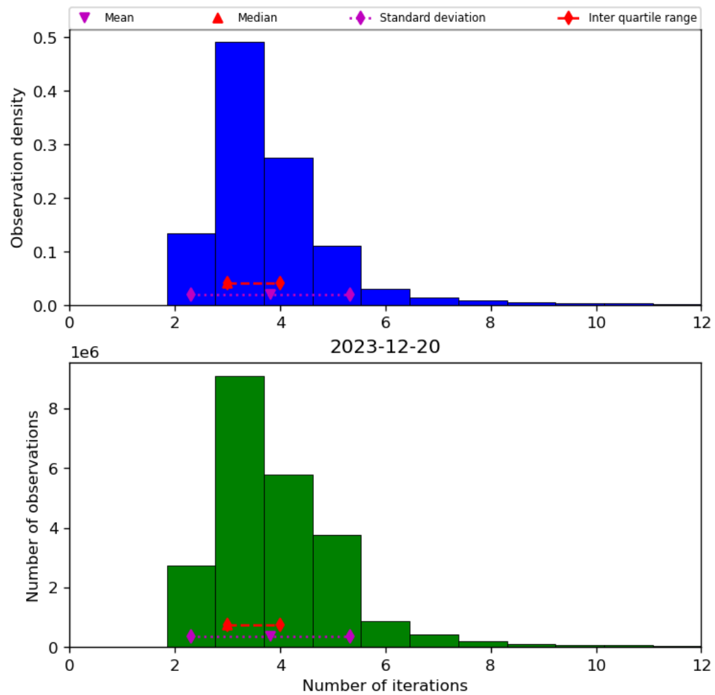
Figure 39: Histogram of “Number of iterations” for 2023-12-20 to 2023-12-21
