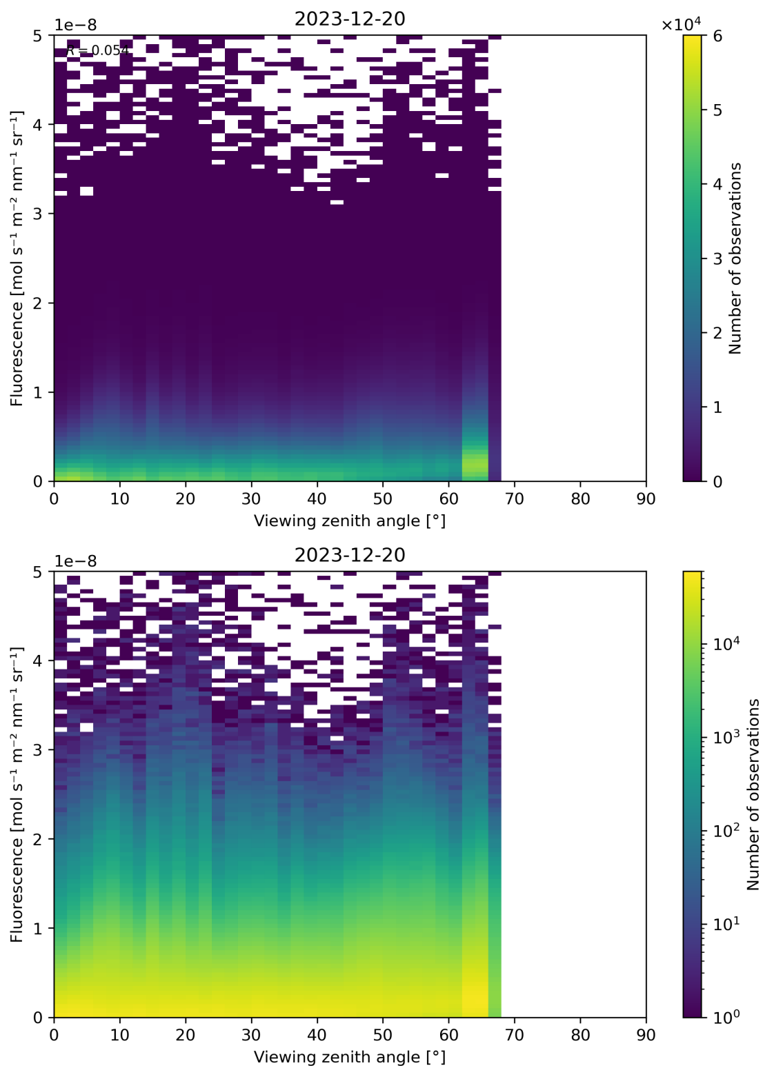
Figure 122: Scatter density plot of “Viewing zenith angle” against “Fluorescence” for 2023-12-20 to 2023-12-21.
