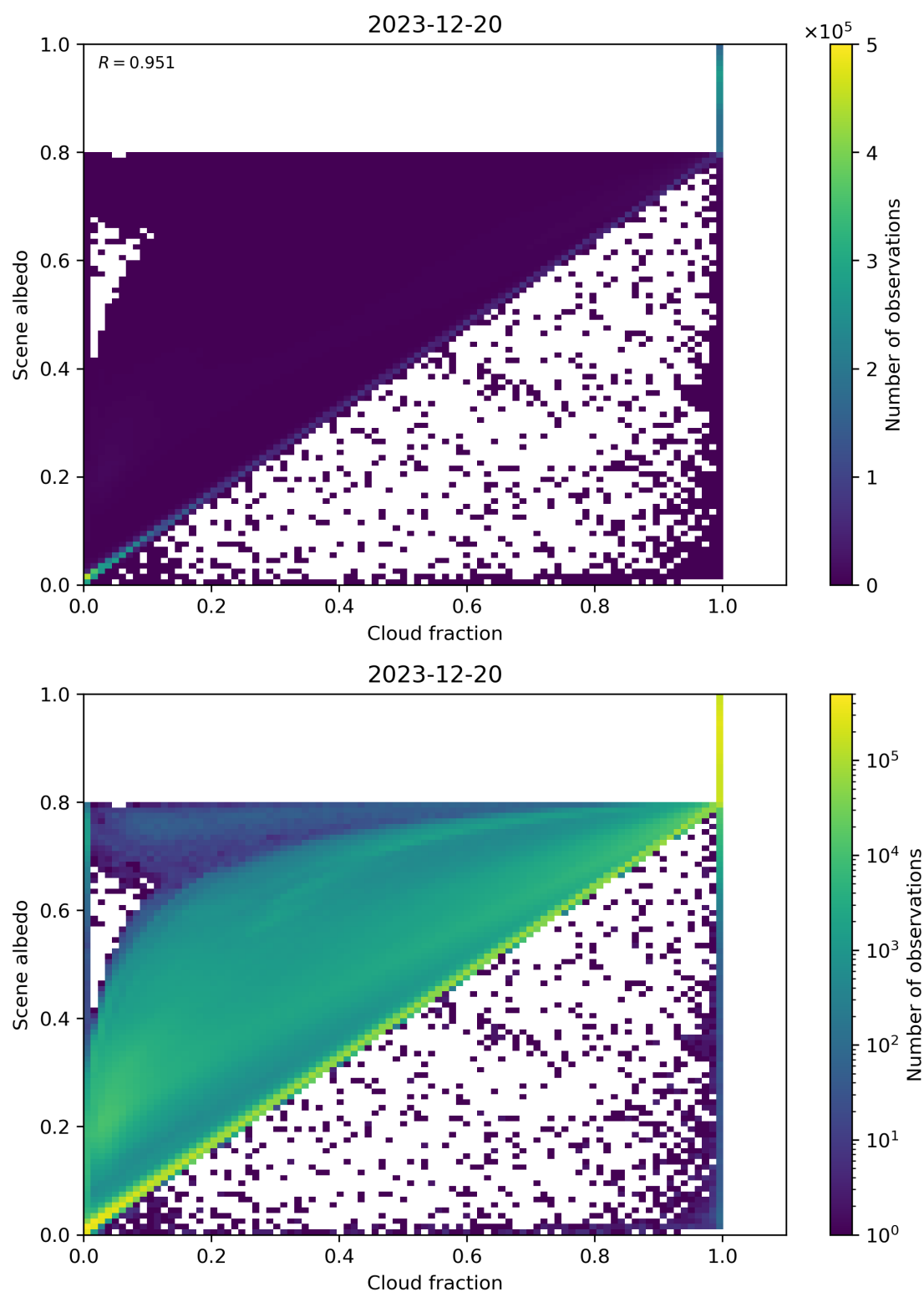
Figure 75: Scatter density plot of “Cloud fraction” against “Scene albedo” for 2023-12-20 to 2023-12-21.
