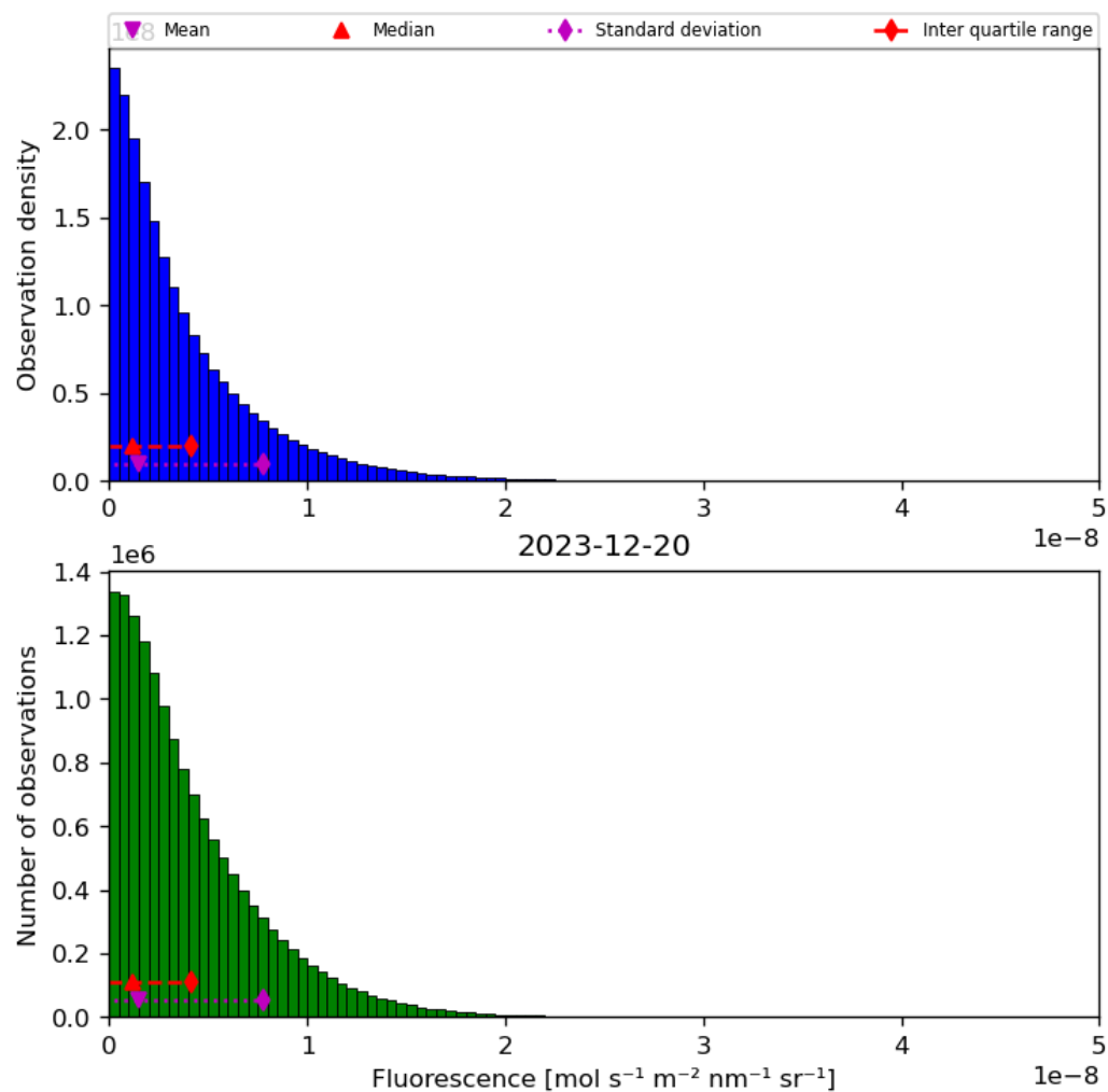
Figure 40: Histogram of “Fluorescence” for 2023-12-20 to 2023-12-21
