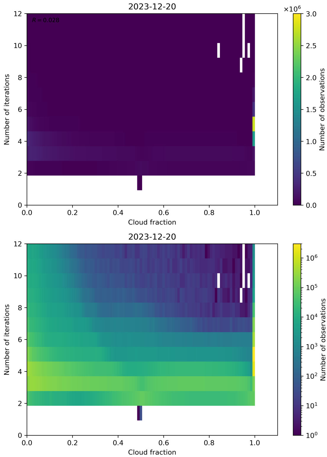
Figure 73: Scatter density plot of “Cloud fraction” against “Number of iterations” for 2023-12-20 to 2023-12-21.
