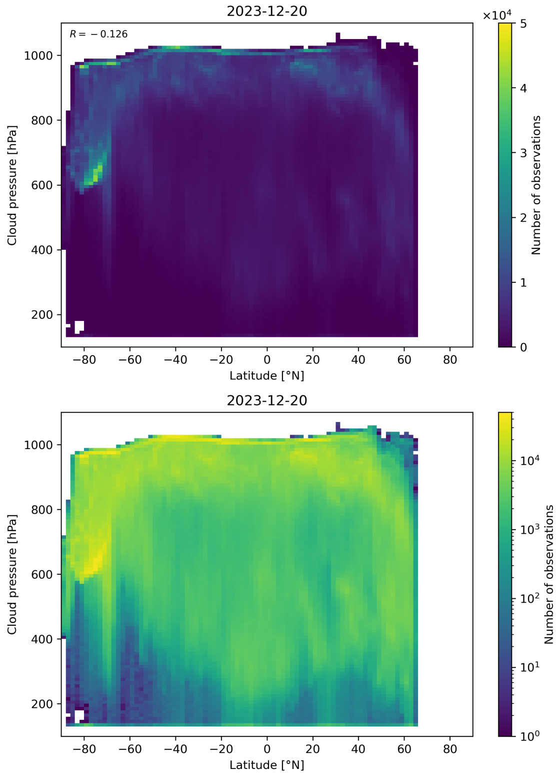
Figure 91: Scatter density plot of “Latitude” against “Cloud pressure” for 2023-12-20 to 2023-12-21.
