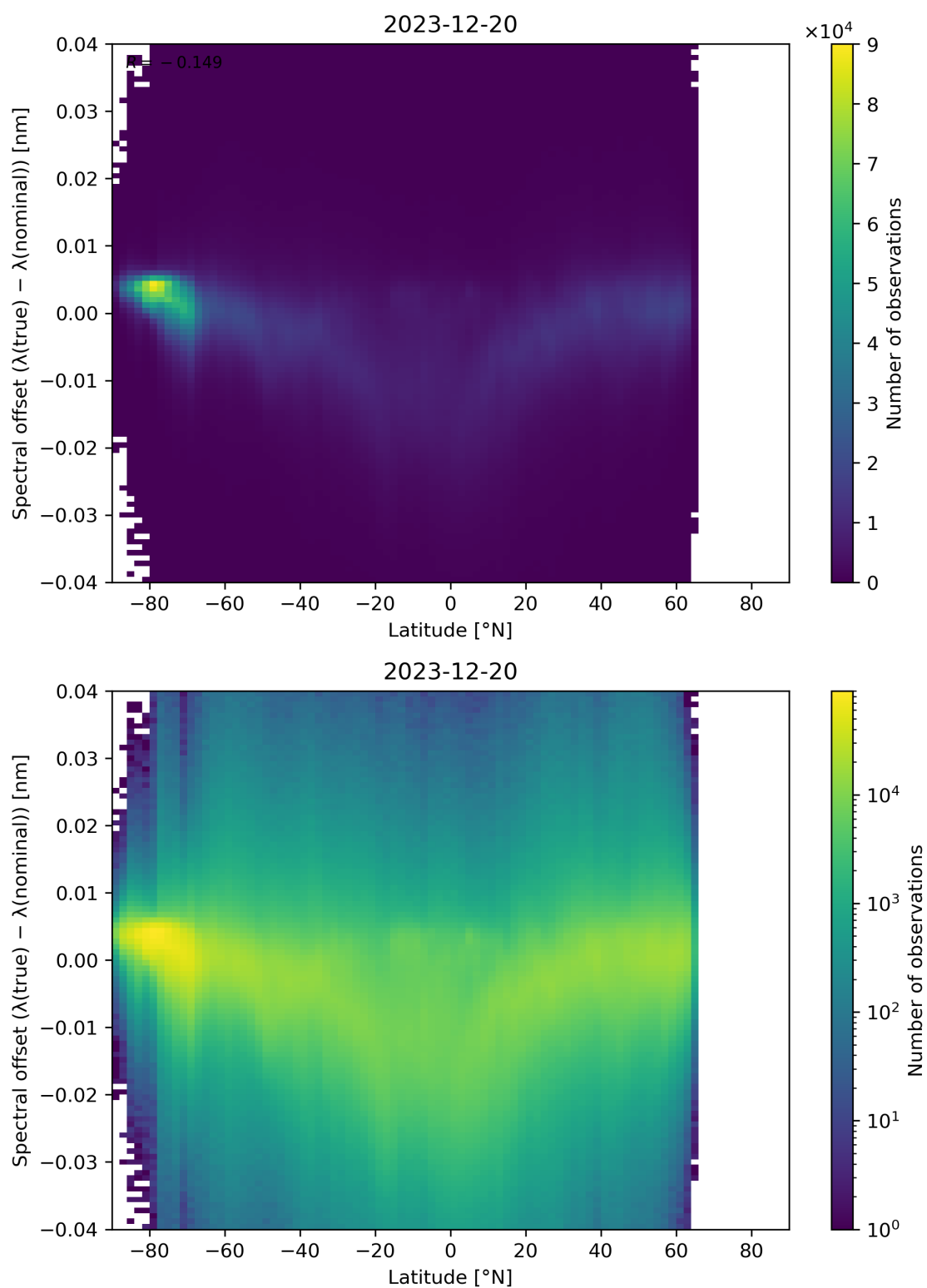
Figure 96: Scatter density plot of “Latitude” against “Spectral offset ( \lambda(\text{true}) - \lambda(\text{nominal}) )” for 2023-12-20 to 2023-12-21.
