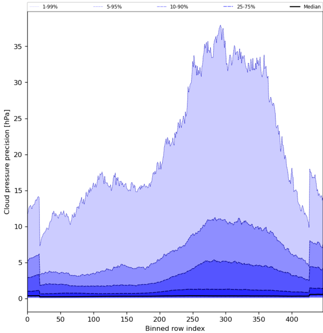
Figure 48: Along track statistics of “Cloud pressure precision” for 2023-12-20 to 2023-12-21
