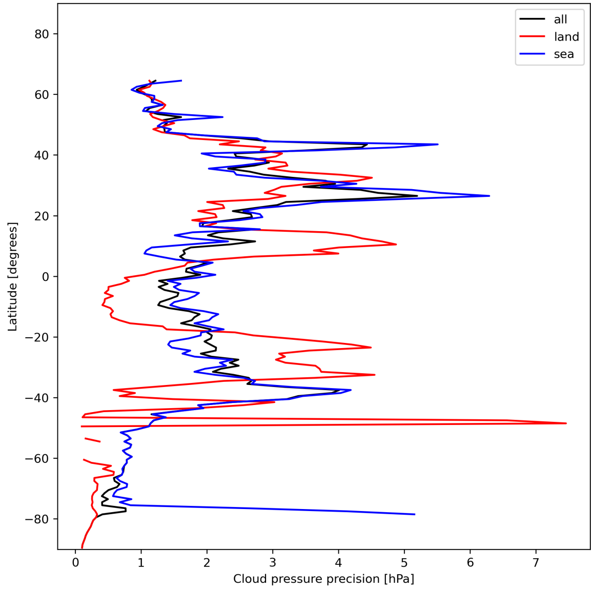
Figure 14: Zonal average of “Cloud pressure precision” for 2023-12-20 to 2023-12-21.
