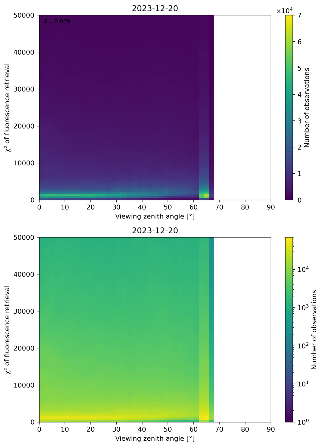
Figure 119: Scatter density plot of “Viewing zenith angle” against “ \chi^2 of fluorescence retrieval” for 2023-12-20 to 2023-12-21.
