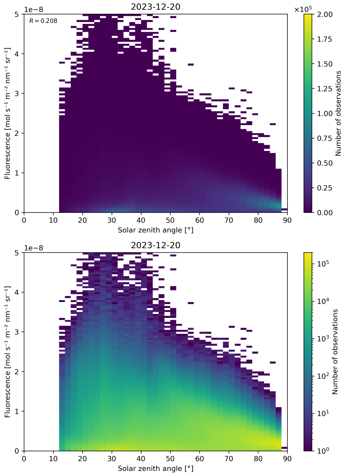
Figure 112: Scatter density plot of “Solar zenith angle” against “Fluorescence” for 2023-12-20 to 2023-12-21.
