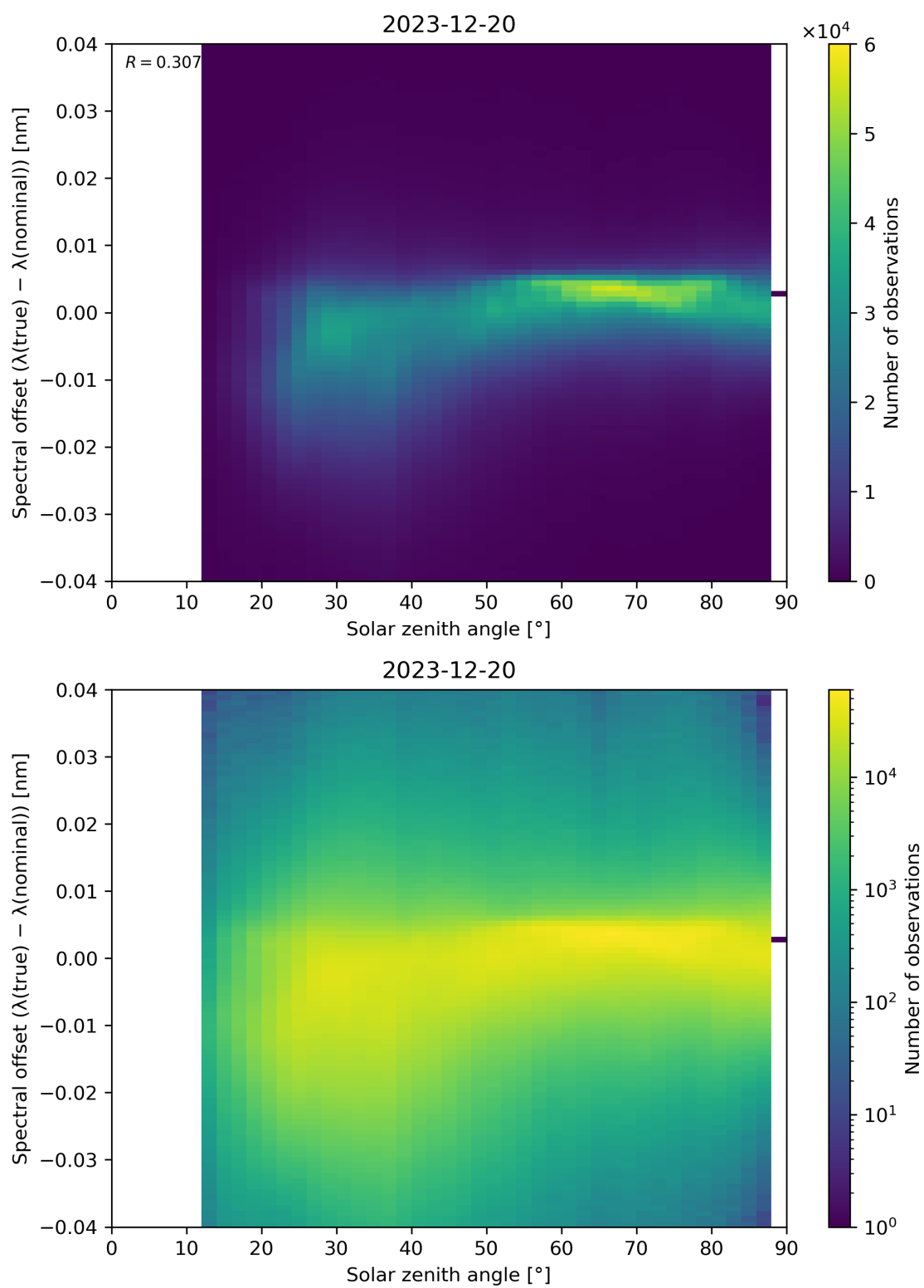
Figure 117: Scatter density plot of “Solar zenith angle” against “Spectral offset ( \lambda(\text{true}) - \lambda(\text{nominal}) )” for 2023-12-20 to 2023-12-21.
