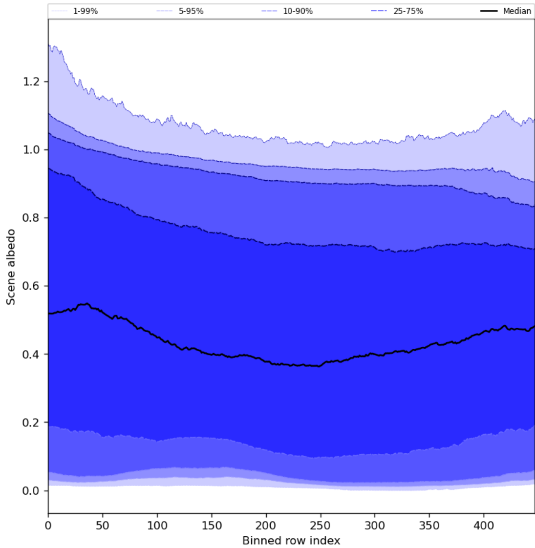
Figure 51: Along track statistics of “Scene albedo” for 2023-12-20 to 2023-12-21
