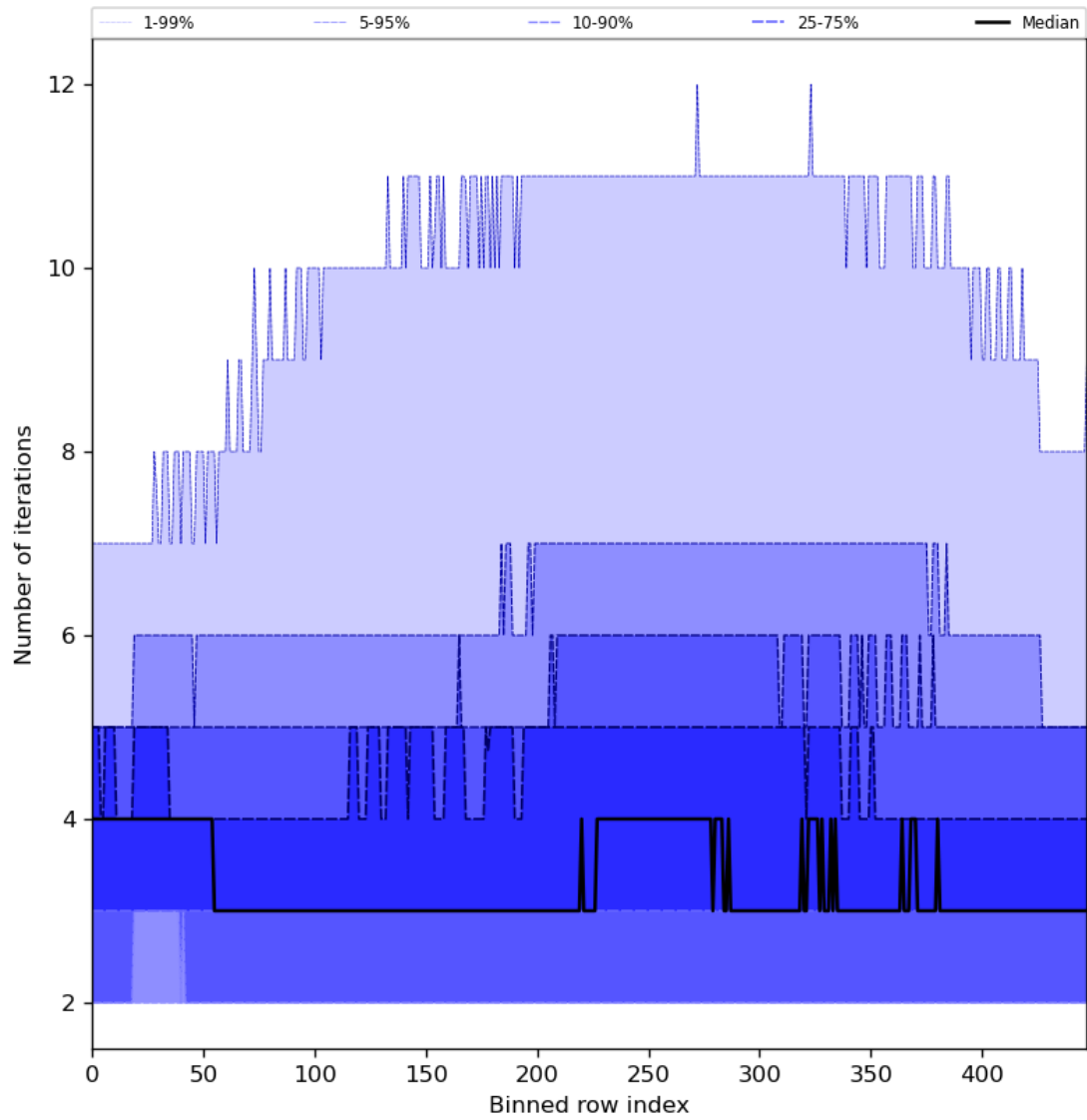
Figure 56: Along track statistics of “Number of iterations” for 2023-12-20 to 2023-12-21
