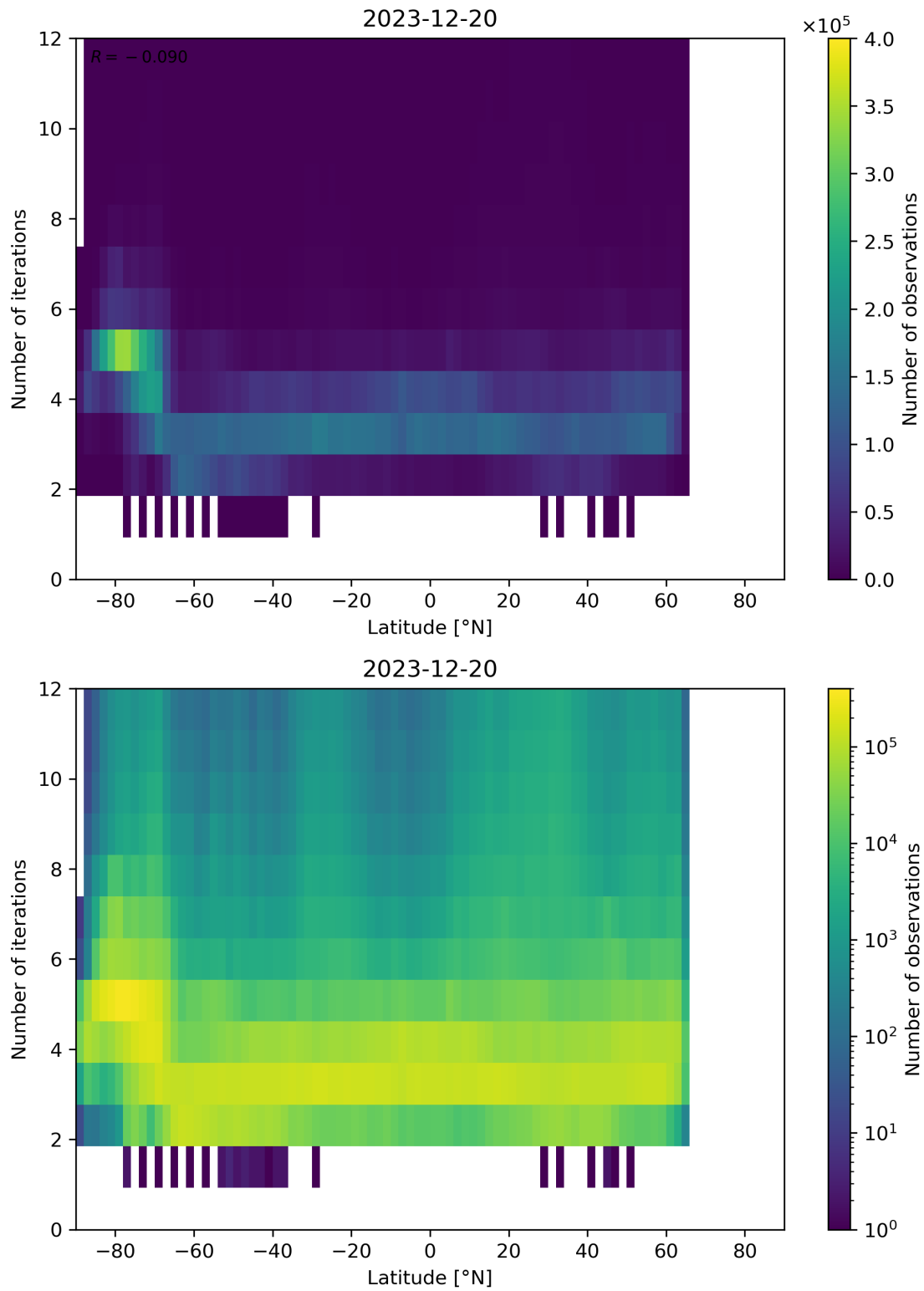
Figure 93: Scatter density plot of “Latitude” against “Number of iterations” for 2023-12-20 to 2023-12-21.
