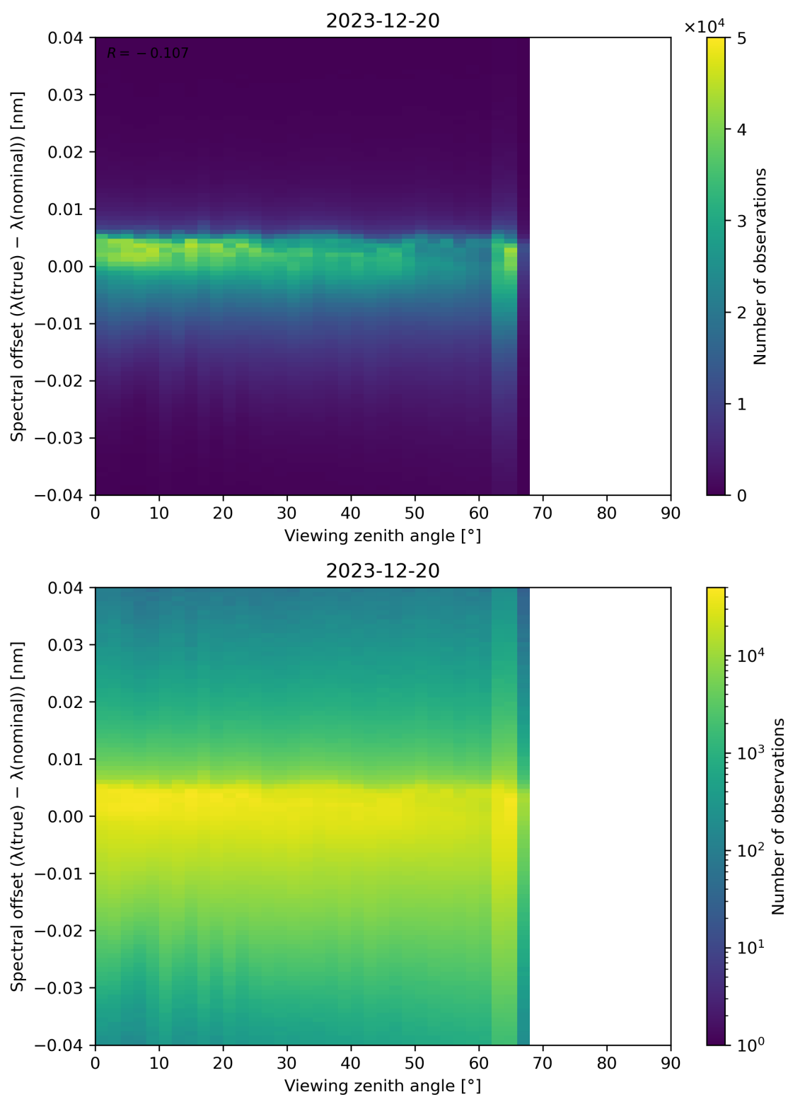
Figure 128: Scatter density plot of “Viewing zenith angle” against “Spectral offset ( \lambda(\text{true}) - \lambda(\text{nominal}) )” for 2023-12-20 to 2023-12-21.
