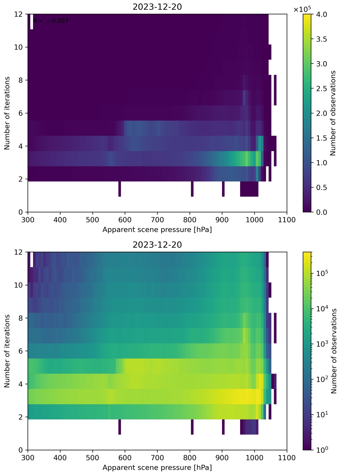
Figure 65: Scatter density plot of “Apparent scene pressure” against “Number of iterations” for 2023-12-20 to 2023-12-21.
