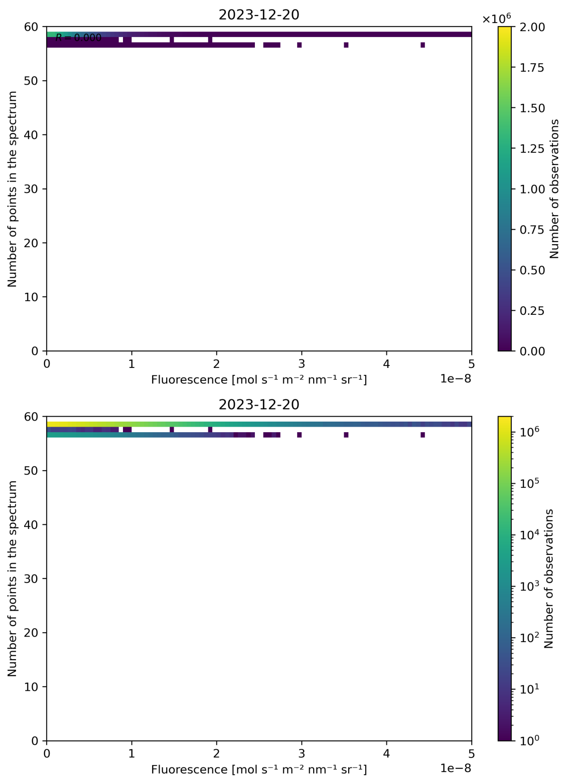
Figure 86: Scatter density plot of “Fluorescence” against “Number of points in the spectrum” for 2023-12-20 to 2023-12-21.
