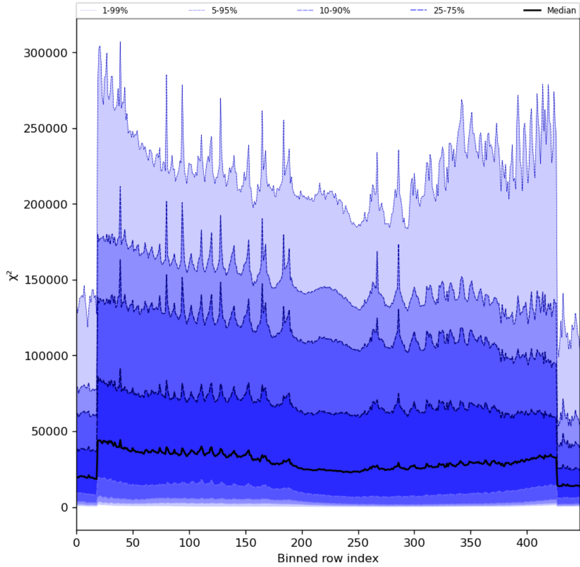
Figure 55: Along track statistics of “ \chi^2 ” for 2023-12-20 to 2023-12-21
