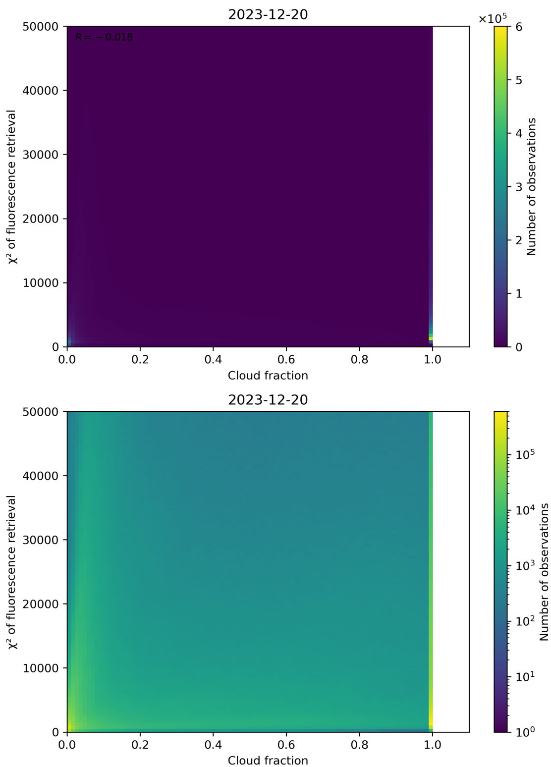
Figure 71: Scatter density plot of “Cloud fraction” against “ \chi^2 of fluorescence retrieval” for 2023-12-20 to 2023-12-21.
