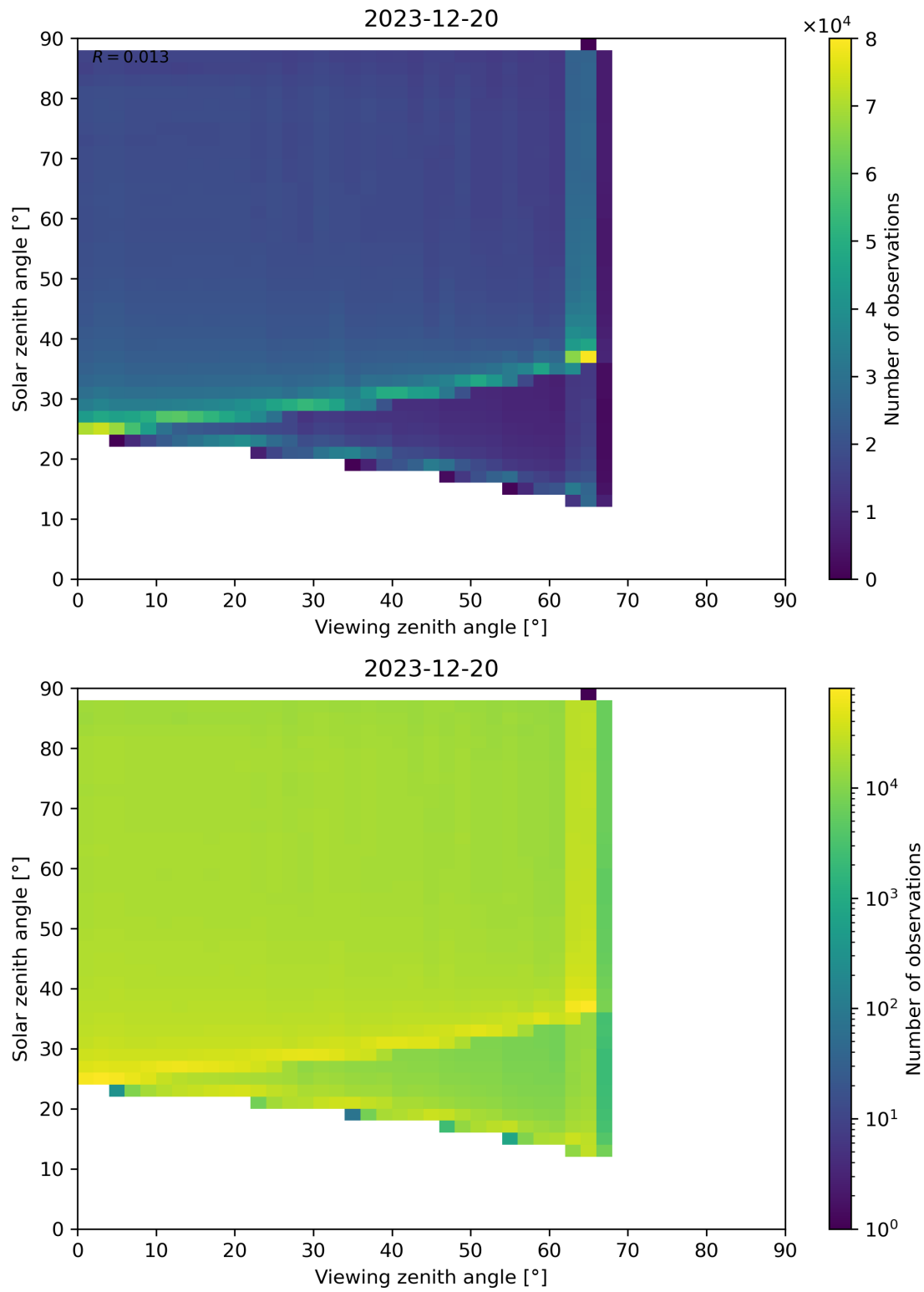
Figure 127: Scatter density plot of “Viewing zenith angle” against “Solar zenith angle” for 2023-12-20 to 2023-12-21.
