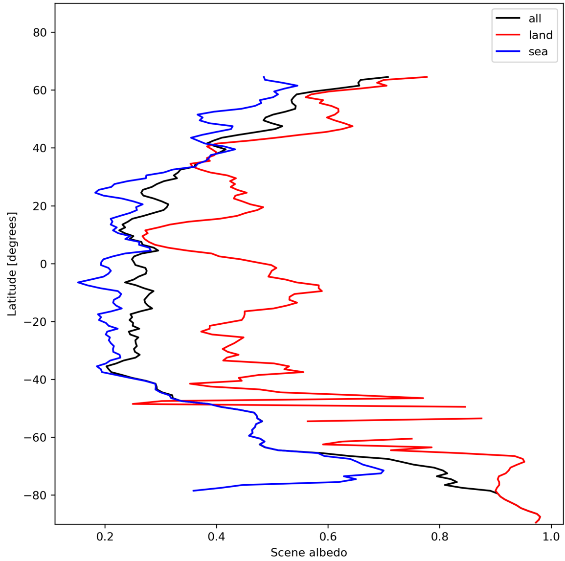
Figure 17: Zonal average of “Scene albedo” for 2023-12-20 to 2023-12-21.
