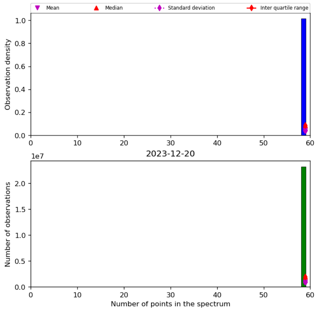
Figure 44: Histogram of “Number of points in the spectrum” for 2023-12-20 to 2023-12-21
