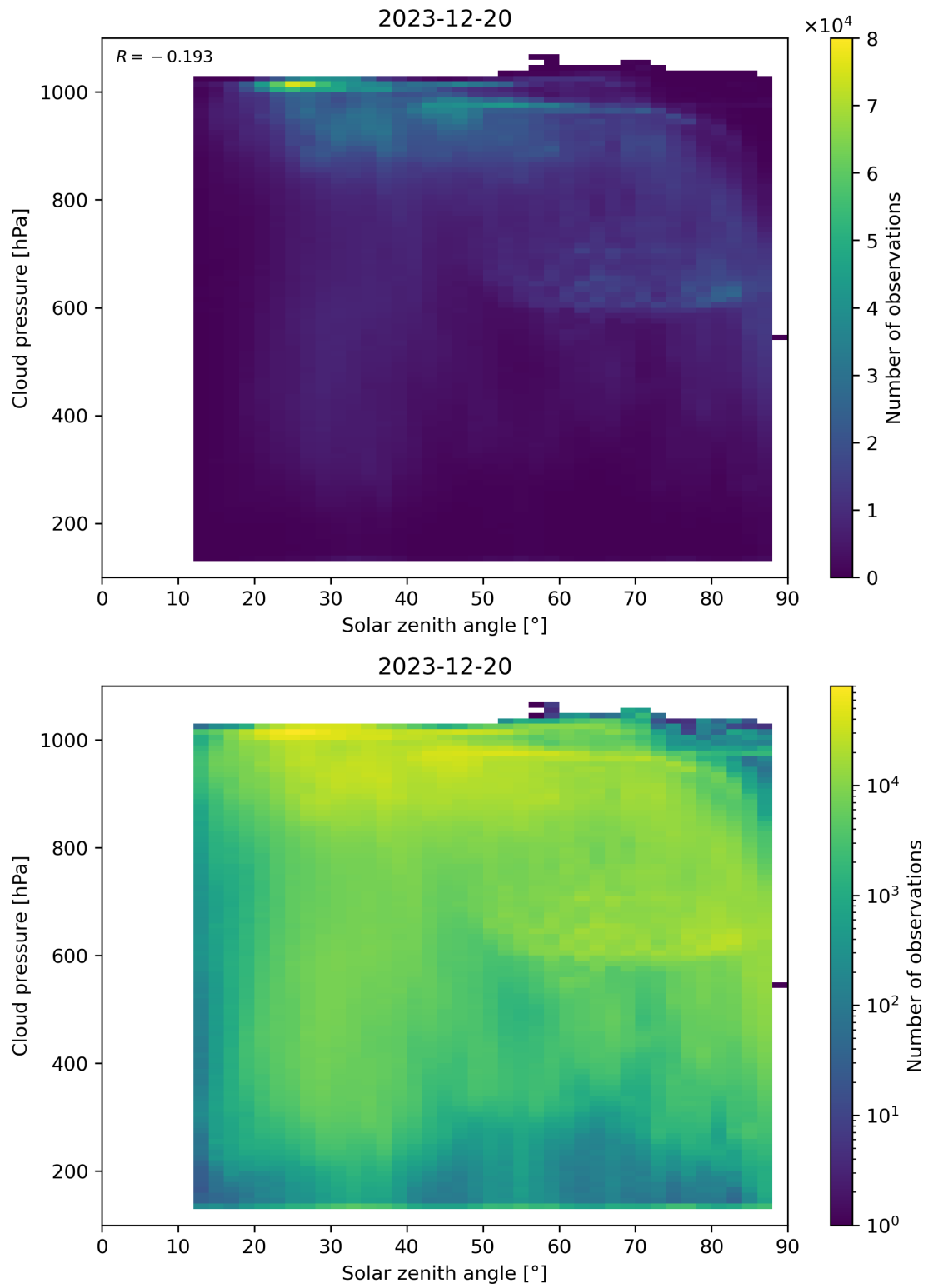
Figure 111: Scatter density plot of “Solar zenith angle” against “Cloud pressure” for 2023-12-20 to 2023-12-21.
