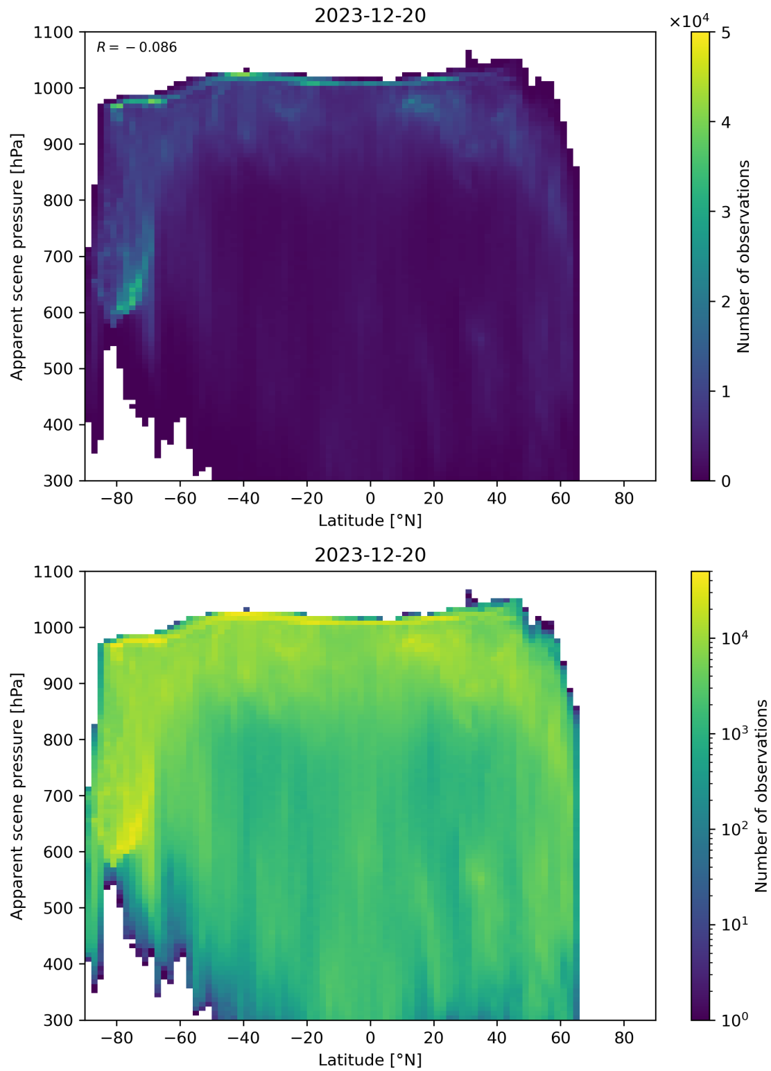
Figure 88: Scatter density plot of “Latitude” against “Apparent scene pressure” for 2023-12-20 to 2023-12-21.
