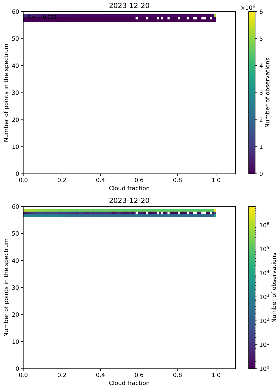
Figure 74: Scatter density plot of “Cloud fraction” against “Number of points in the spectrum” for 2023-12-20 to 2023-12-21.
