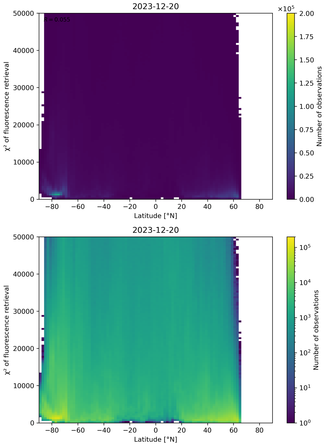
Figure 89: Scatter density plot of “Latitude” against “ \chi^2 of fluorescence retrieval” for 2023-12-20 to 2023-12-21.
