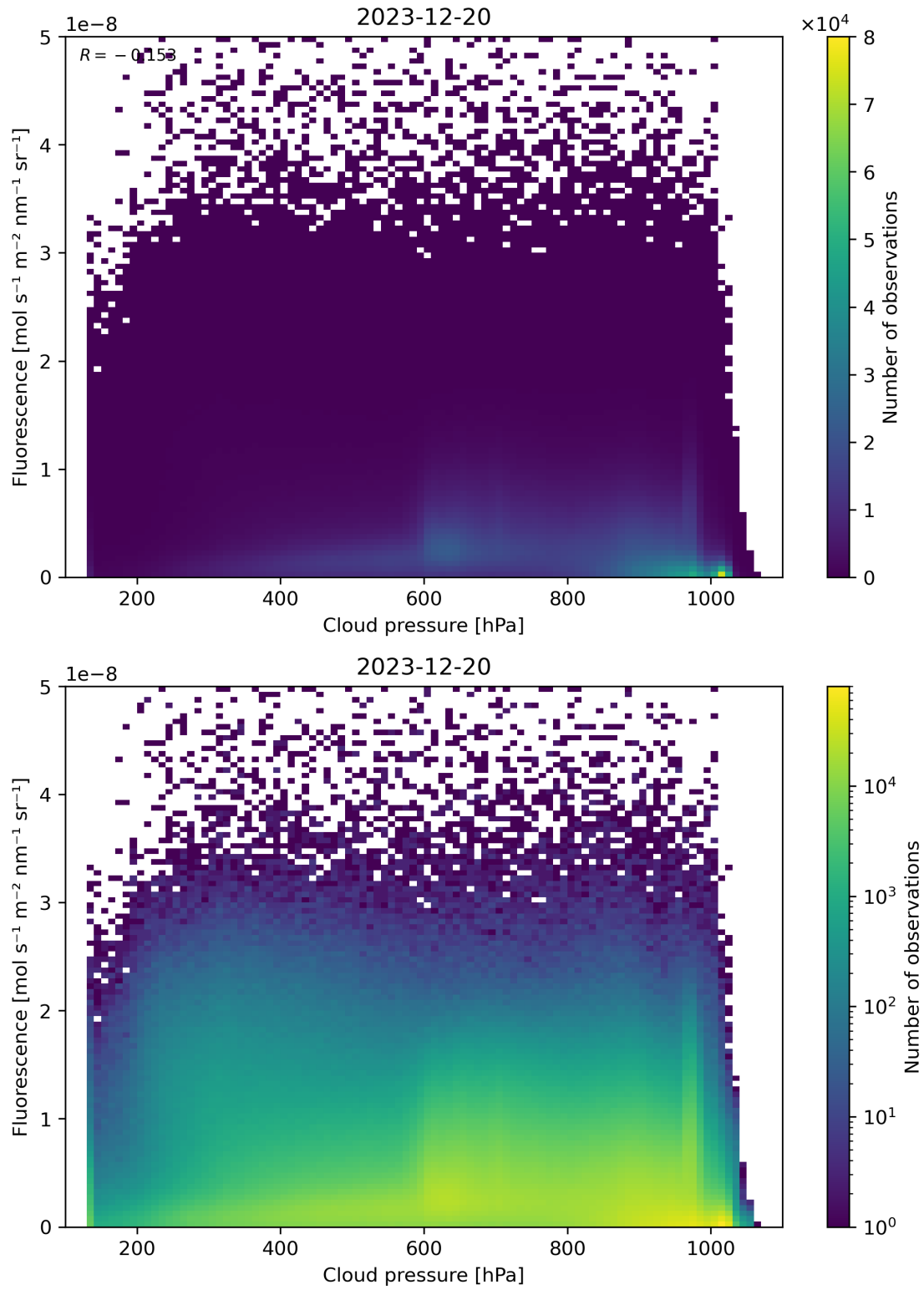
Figure 80: Scatter density plot of “Cloud pressure” against “Fluorescence” for 2023-12-20 to 2023-12-21.
