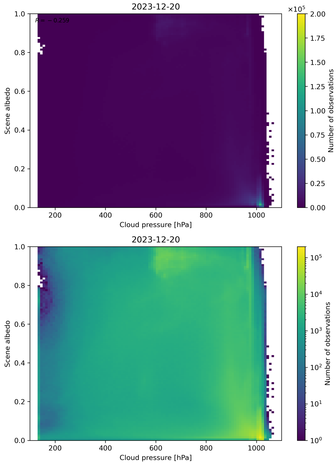
Figure 83: Scatter density plot of “Cloud pressure” against “Scene albedo” for 2023-12-20 to 2023-12-21.
