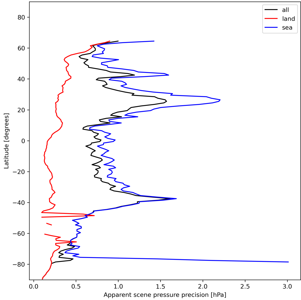
Figure 20: Zonal average of “Apparent scene pressure precision” for 2023-12-20 to 2023-12-21.
