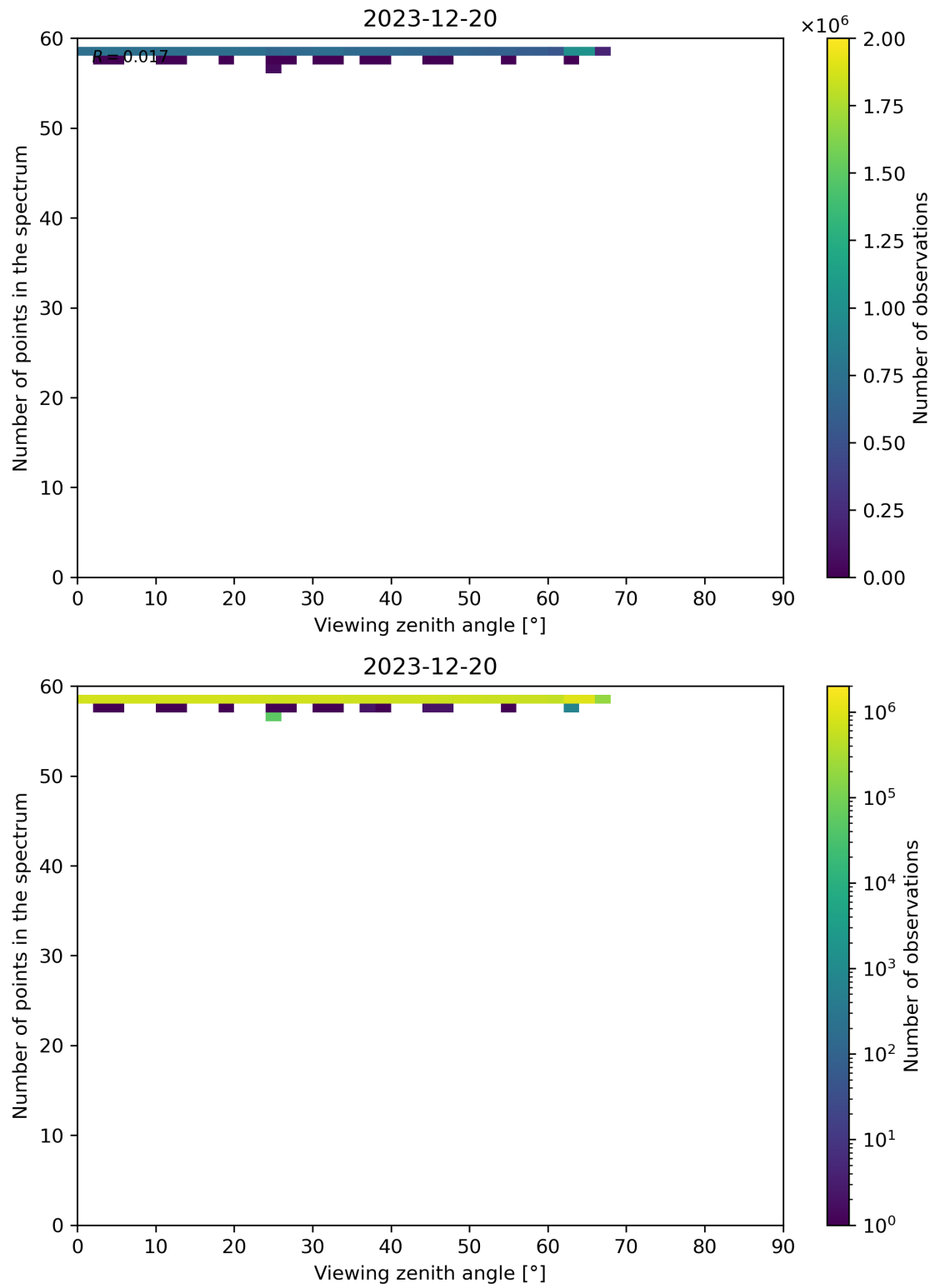
Figure 125: Scatter density plot of “Viewing zenith angle” against “Number of points in the spectrum” for 2023-12-20 to 2023-12-21.
