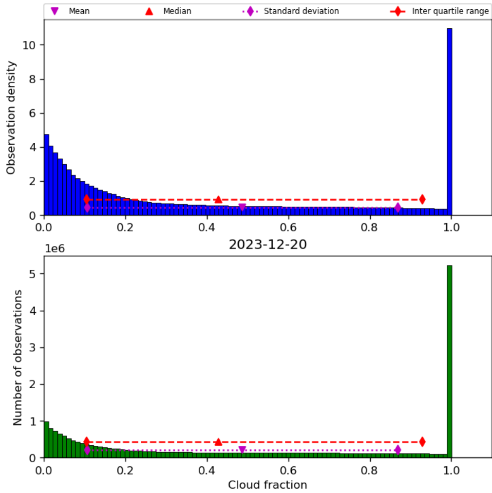
Figure 32: Histogram of “Cloud fraction” for 2023-12-20 to 2023-12-21
