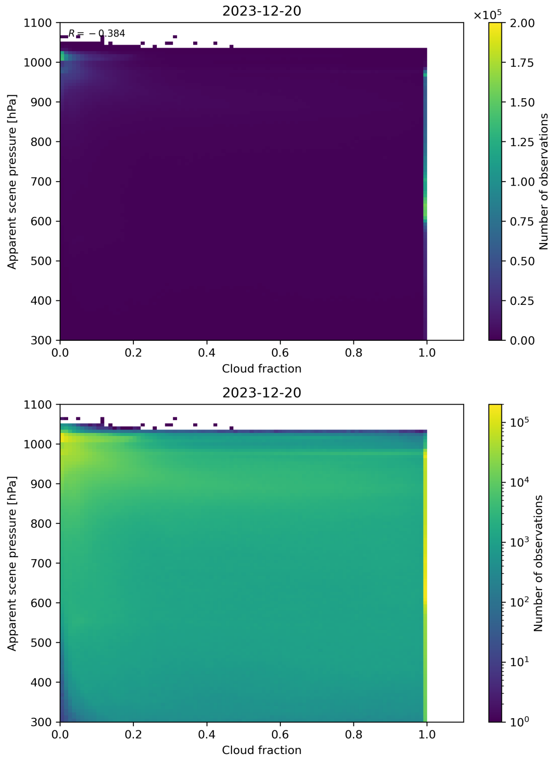
Figure 70: Scatter density plot of “Cloud fraction” against “Apparent scene pressure” for 2023-12-20 to 2023-12-21.
