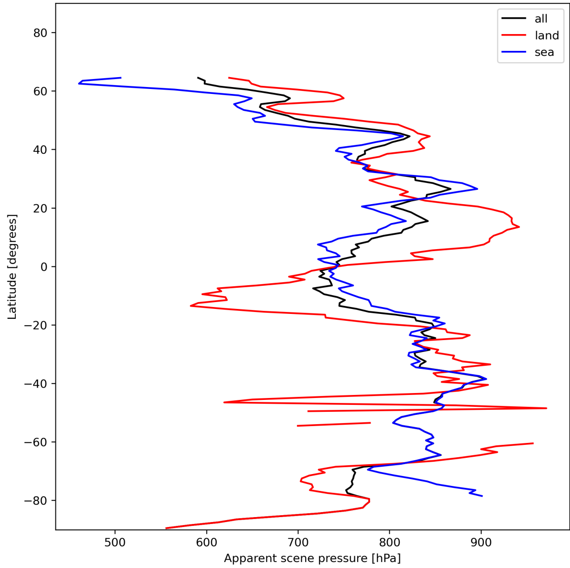
Figure 19: Zonal average of “Apparent scene pressure” for 2023-12-20 to 2023-12-21.
