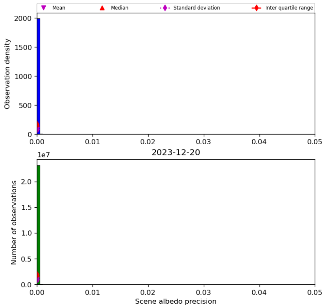
Figure 35: Histogram of “Scene albedo precision” for 2023-12-20 to 2023-12-21
