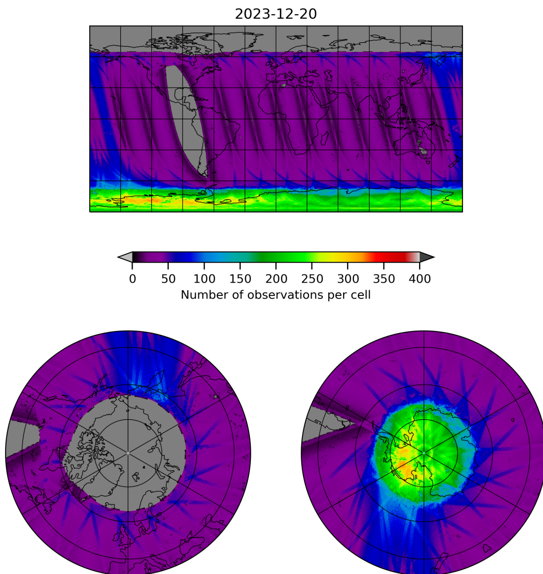
Figure 11: Map of the number of observations for 2023-12-20 to 2023-12-21
