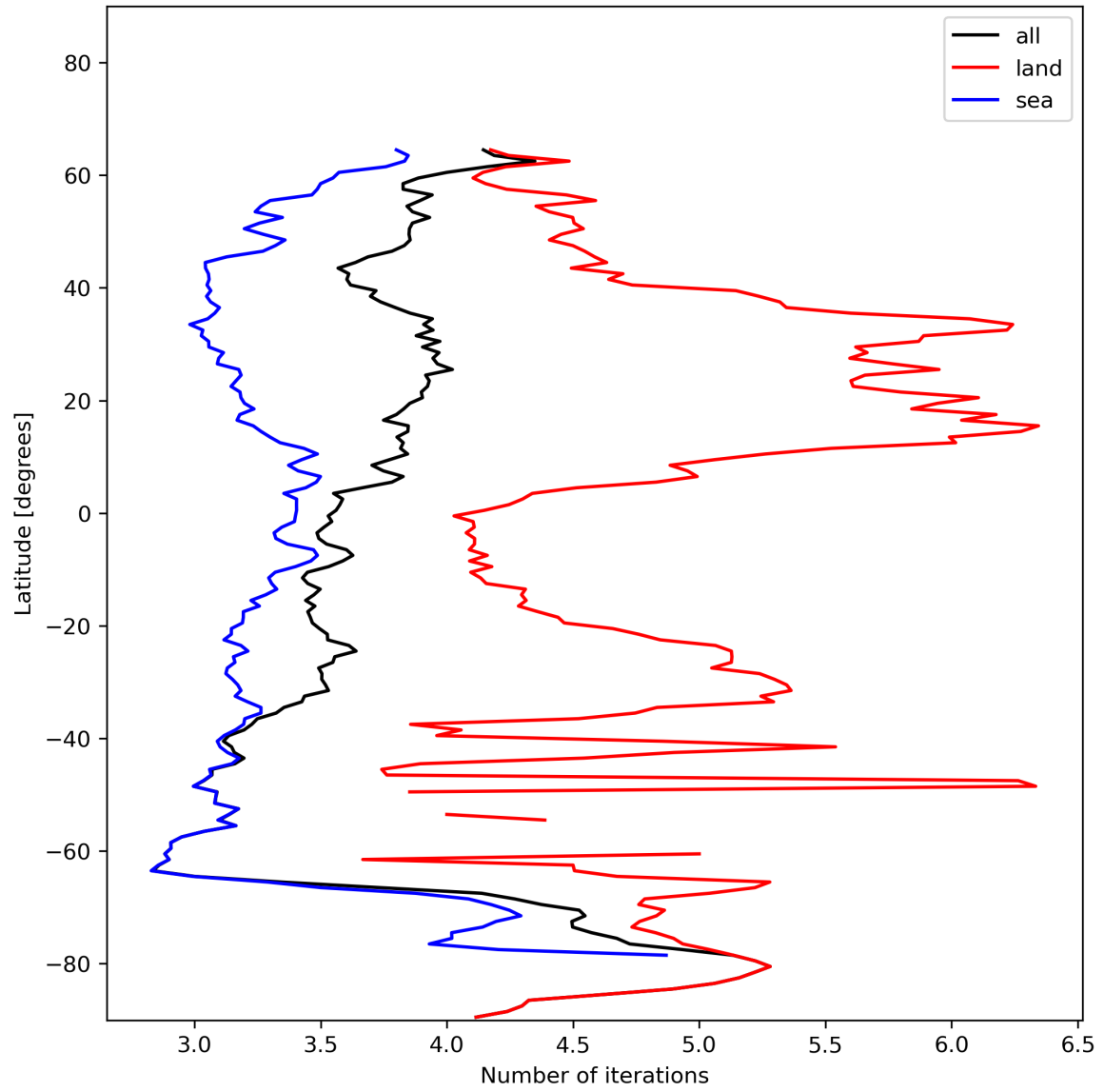
Figure 22: Zonal average of “Number of iterations” for 2023-12-20 to 2023-12-21.
