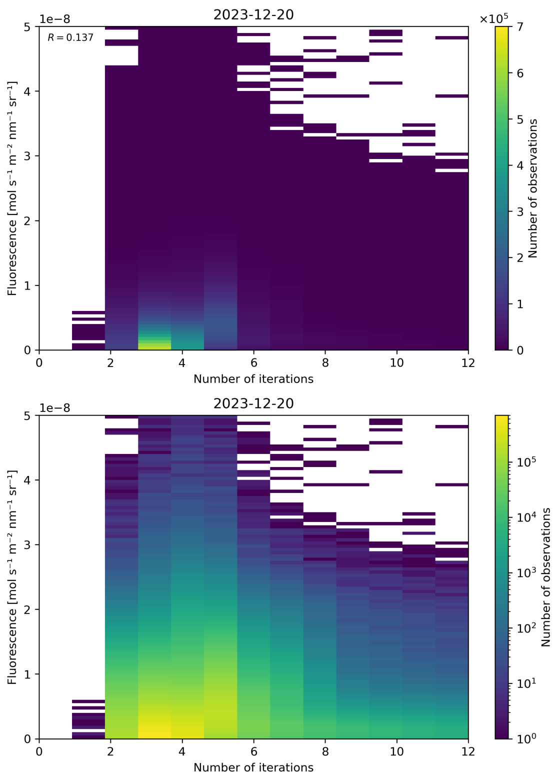
Figure 98: Scatter density plot of “Number of iterations” against “Fluorescence” for 2023-12-20 to 2023-12-21.
