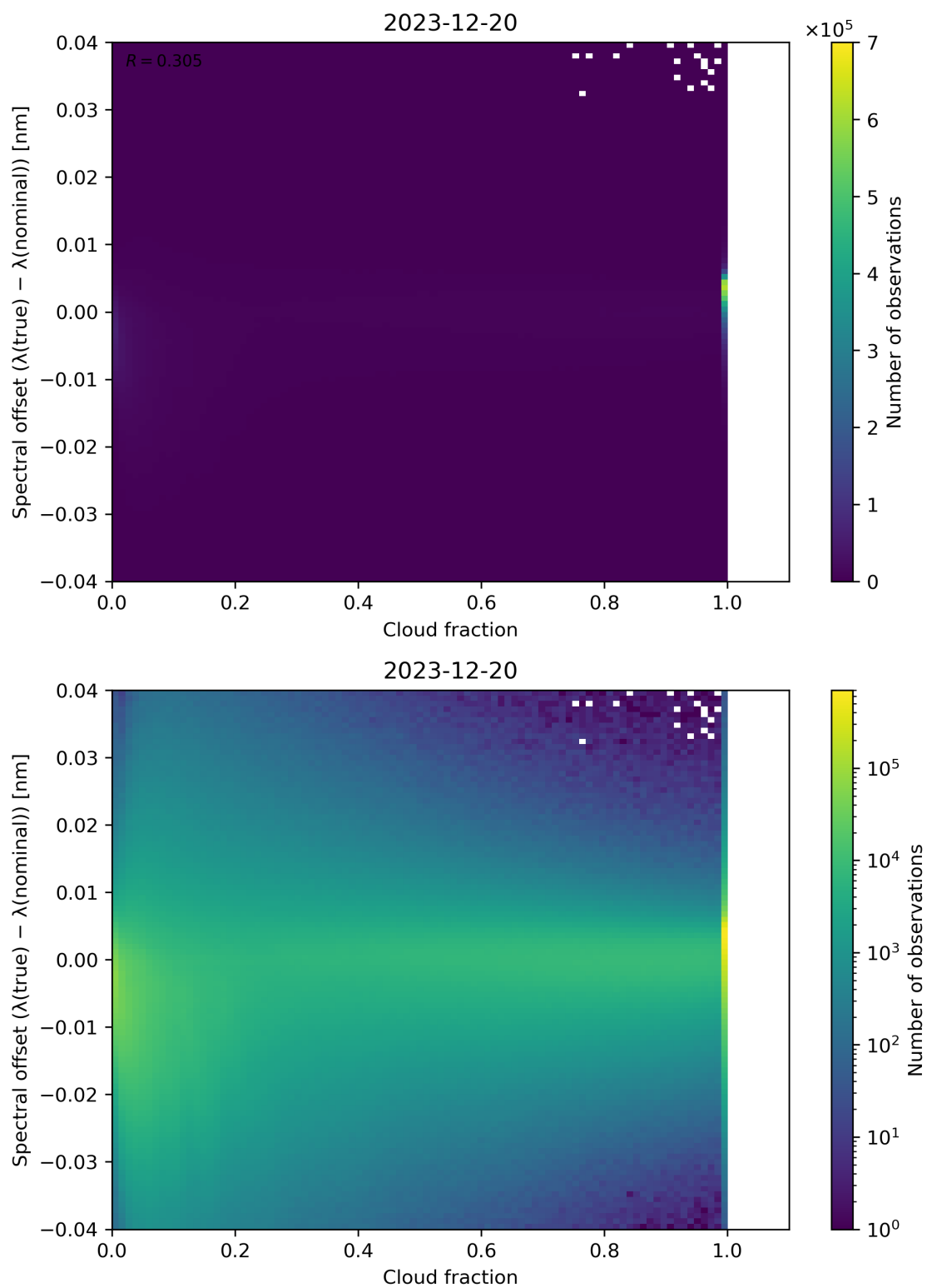
Figure 76: Scatter density plot of “Cloud fraction” against “Spectral offset ( \lambda(\text{true}) - \lambda(\text{nominal}) )” for 2023-12-20 to 2023-12-21.
