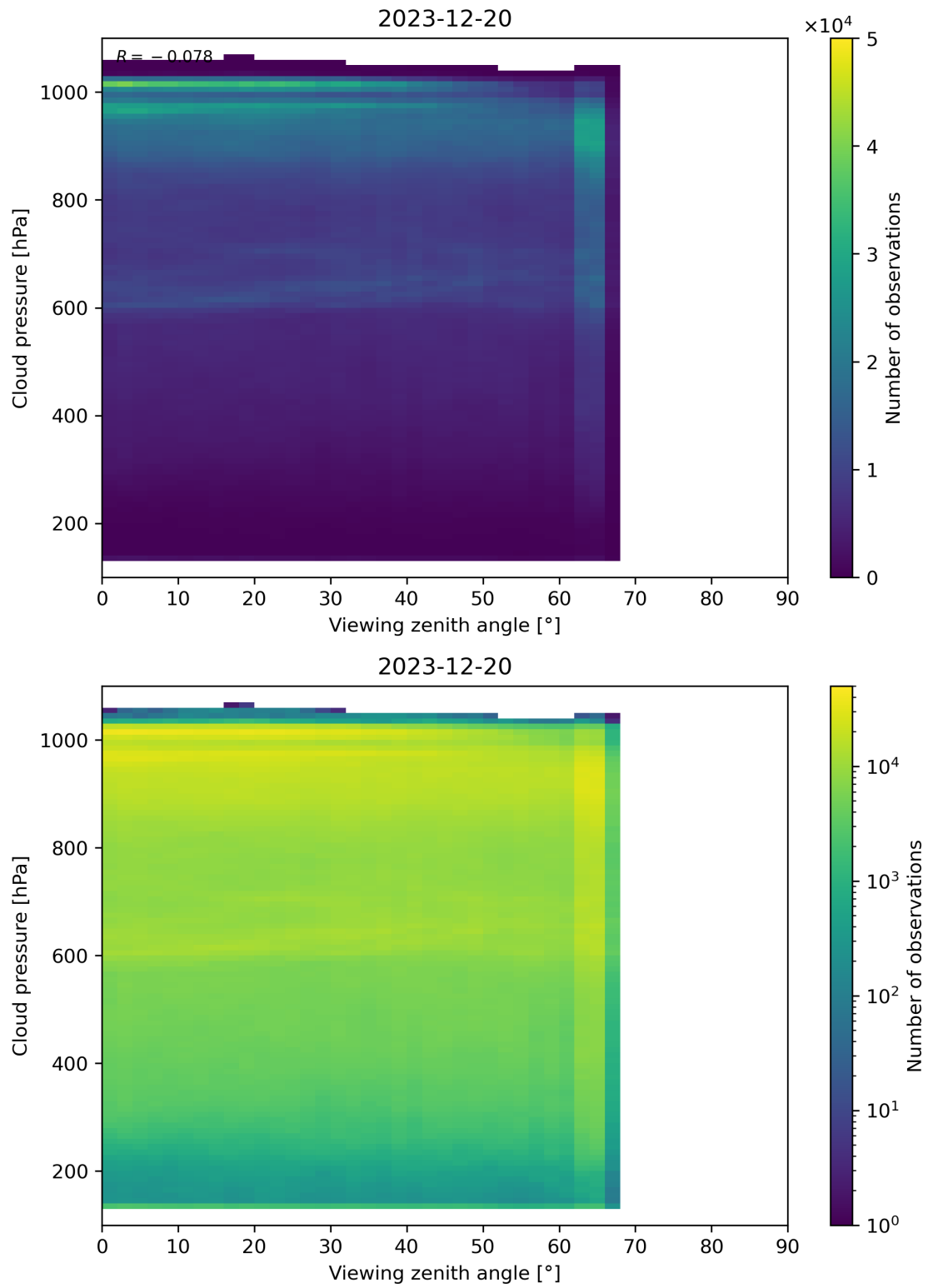
Figure 121: Scatter density plot of “Viewing zenith angle” against “Cloud pressure” for 2023-12-20 to 2023-12-21.
