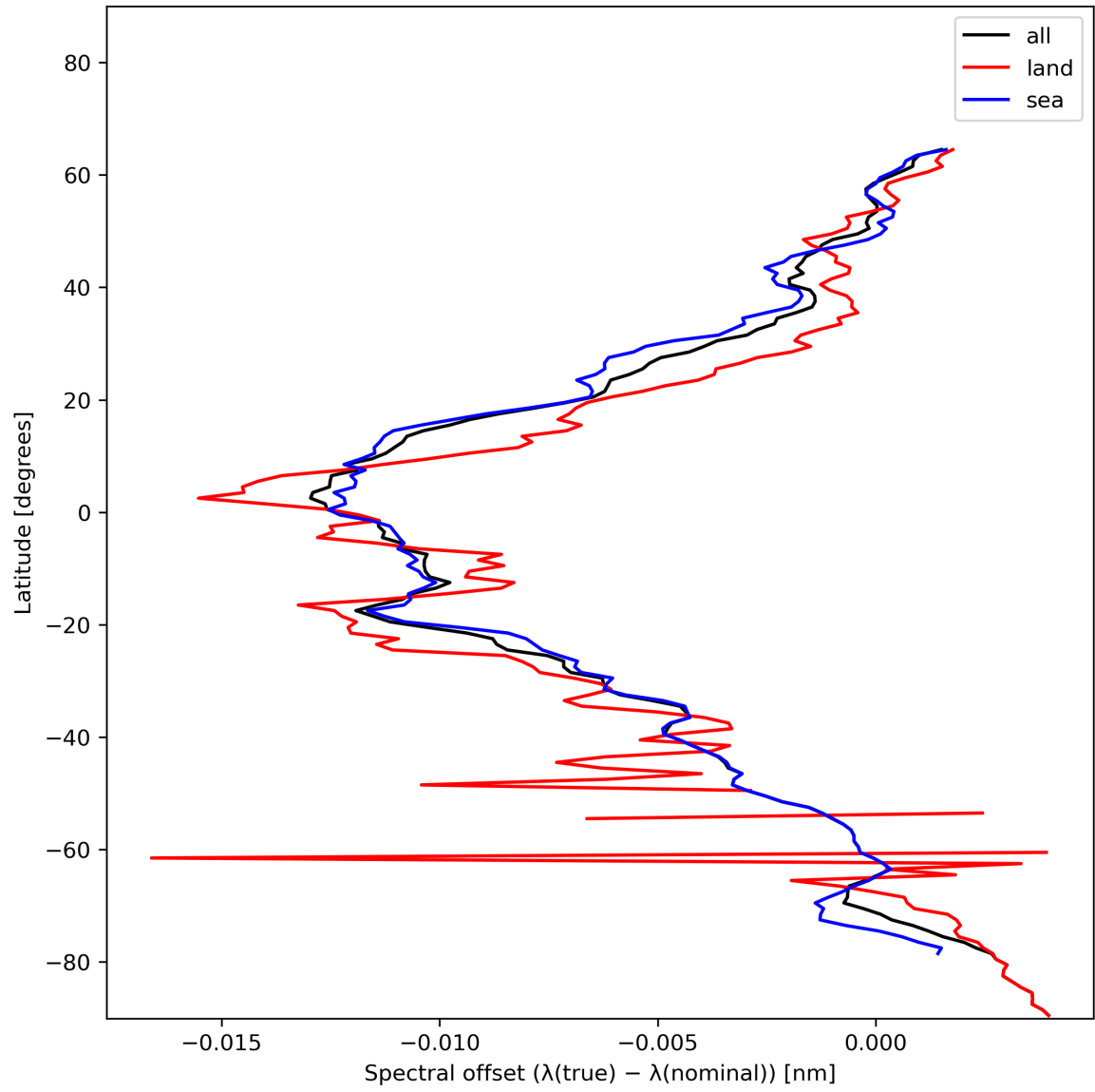
Figure 28: Zonal average of “Spectral offset ( \lambda(\text{true}) - \lambda(\text{nominal}) )” for 2023-12-20 to 2023-12-21.
