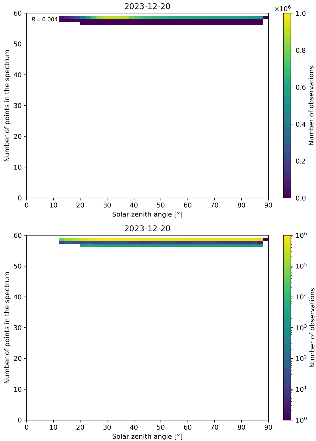
Figure 115: Scatter density plot of “Solar zenith angle” against “Number of points in the spectrum” for 2023-12-20 to 2023-12-21.
