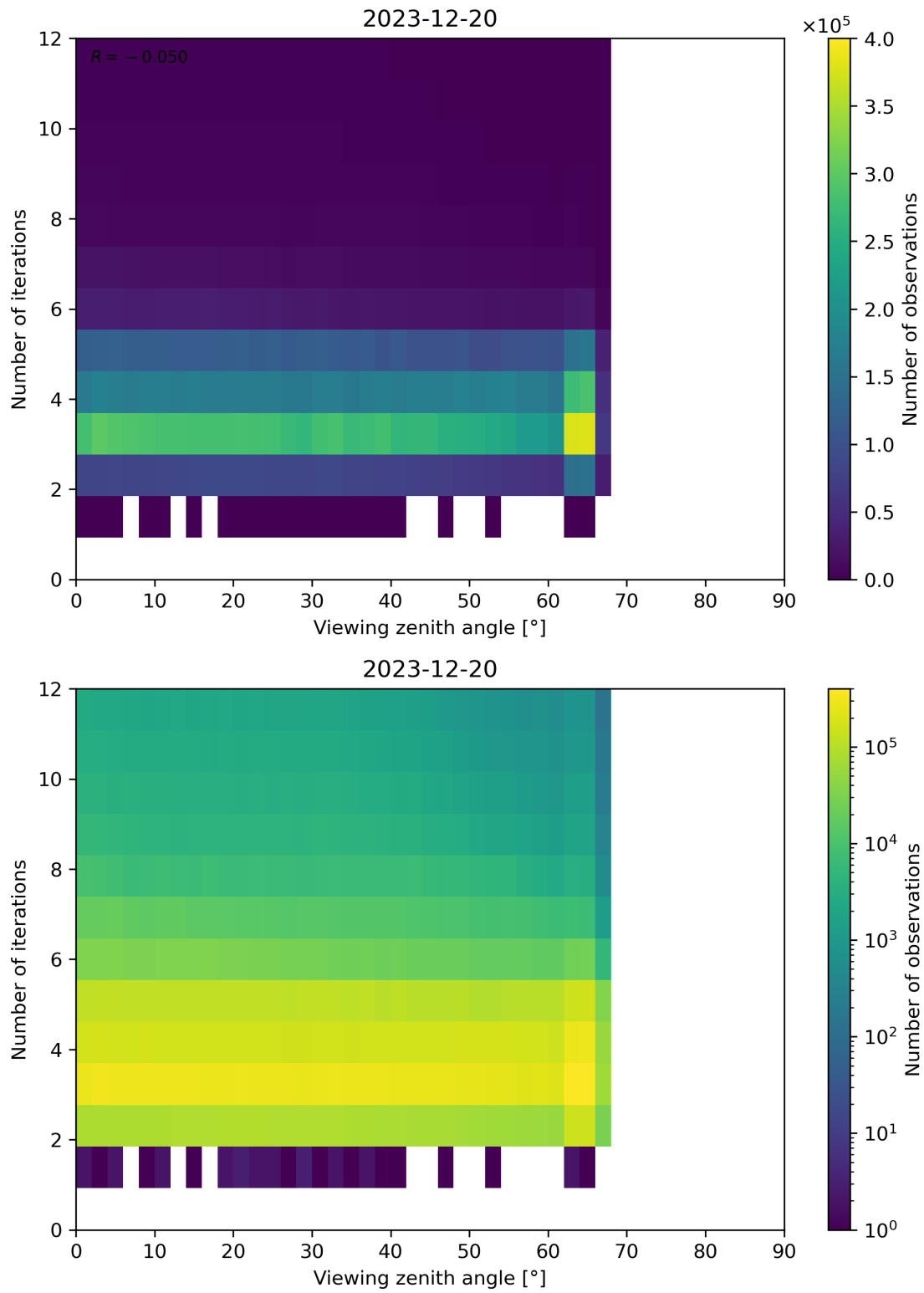
Figure 124: Scatter density plot of “Viewing zenith angle” against “Number of iterations” for 2023-12-20 to 2023-12-21.
