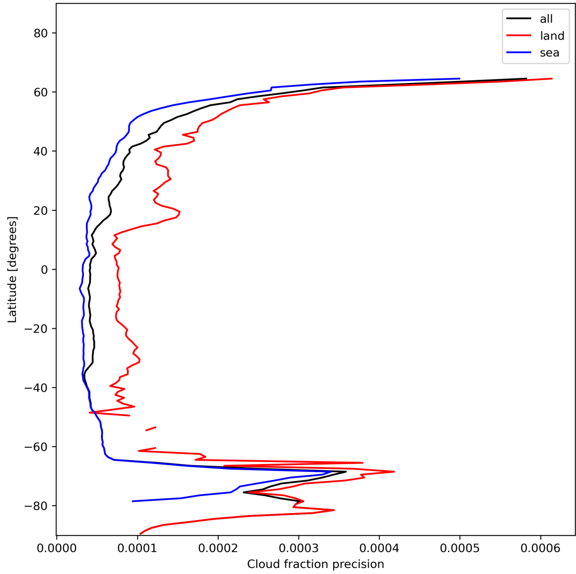
Figure 16: Zonal average of “Cloud fraction precision” for 2023-12-20 to 2023-12-21.
