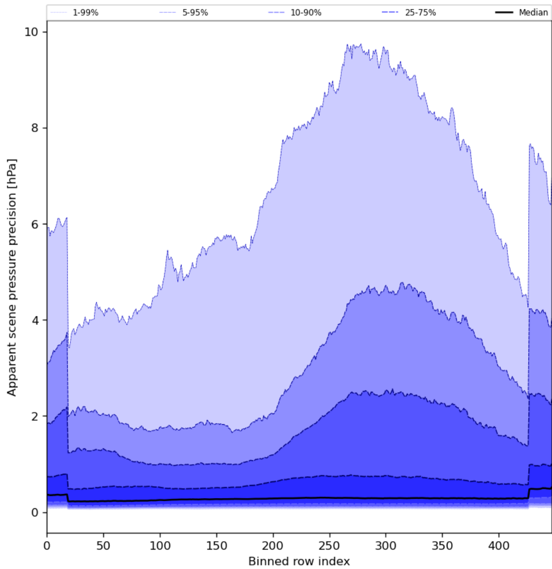
Figure 54: Along track statistics of “Apparent scene pressure precision” for 2023-12-20 to 2023-12-21
