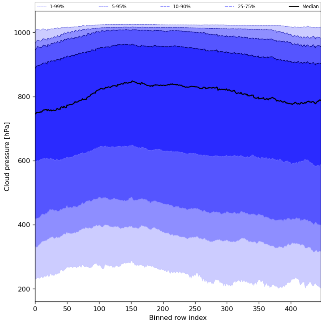
Figure 47: Along track statistics of “Cloud pressure” for 2023-12-20 to 2023-12-21
