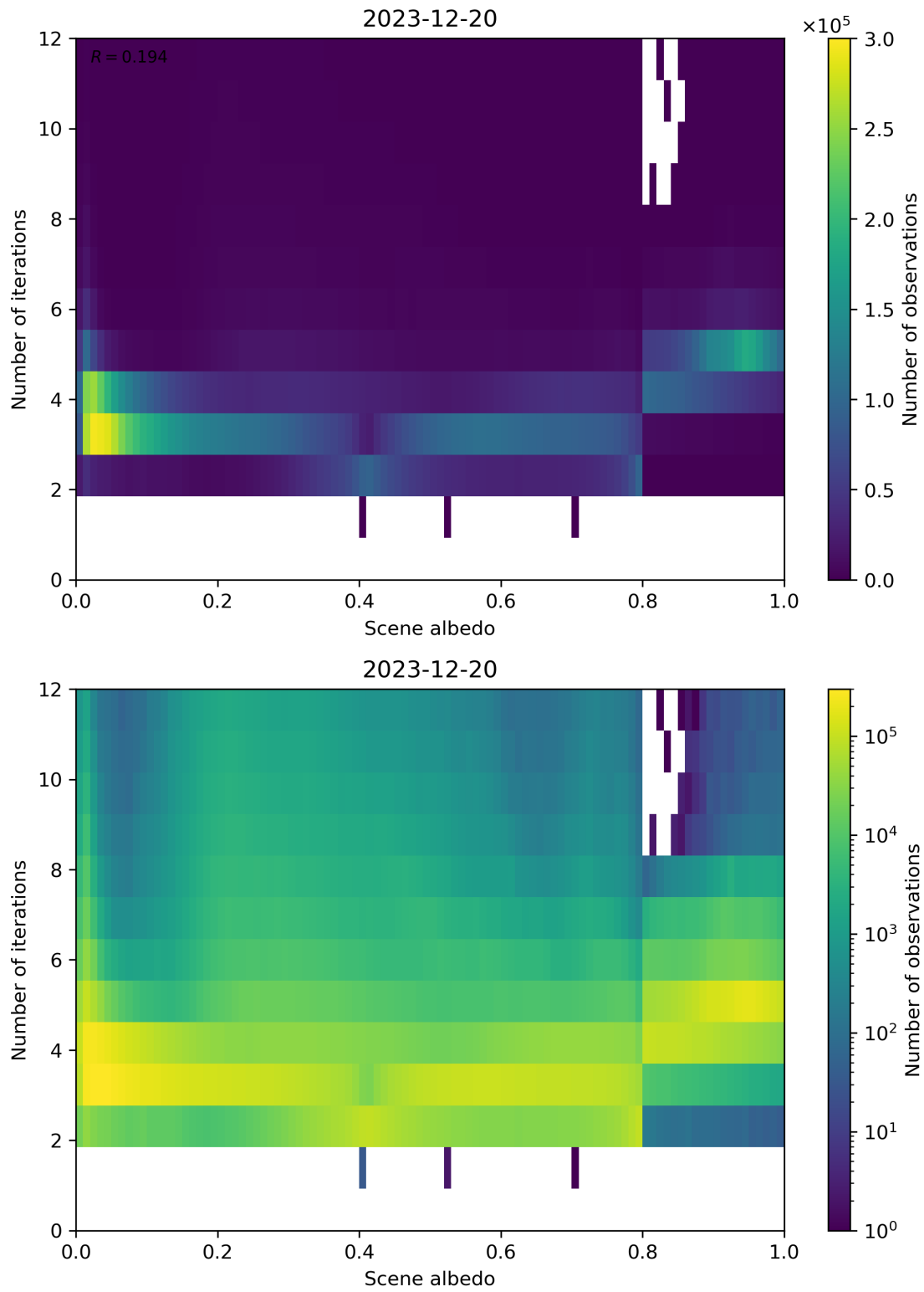
Figure 105: Scatter density plot of “Scene albedo” against “Number of iterations” for 2023-12-20 to 2023-12-21.
