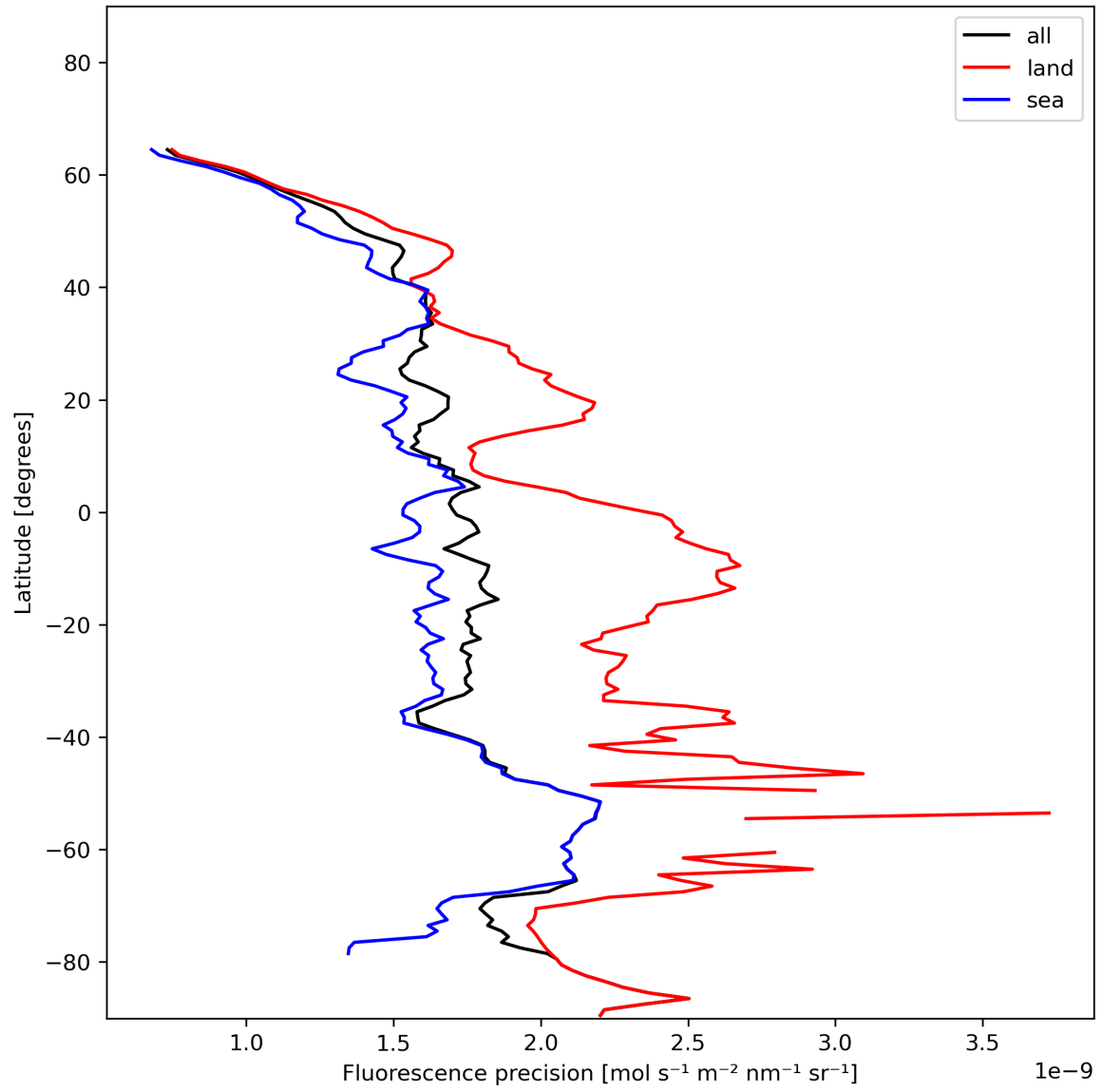
Figure 24: Zonal average of “Fluorescence precision” for 2023-12-20 to 2023-12-21.
