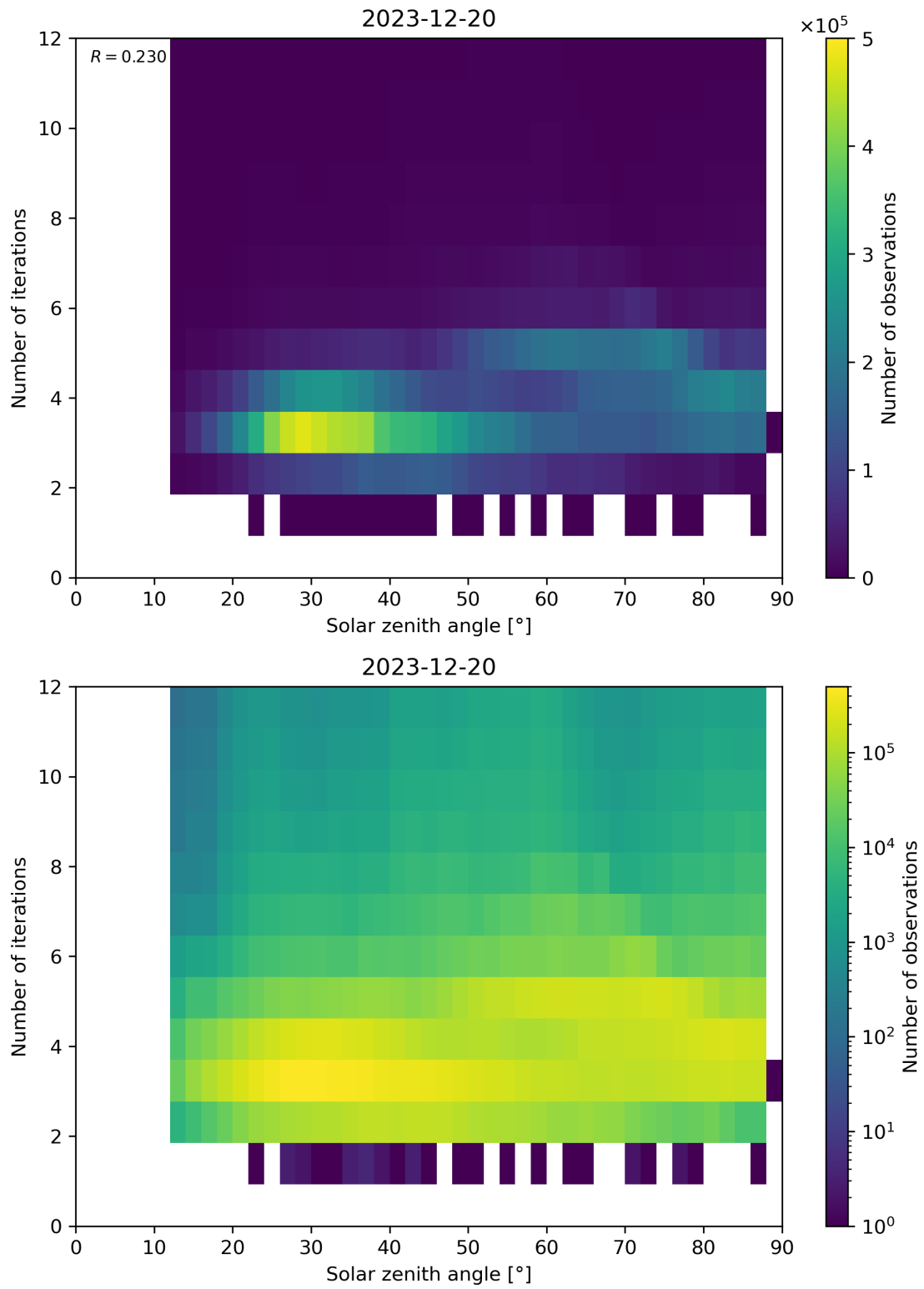
Figure 114: Scatter density plot of “Solar zenith angle” against “Number of iterations” for 2023-12-20 to 2023-12-21.
