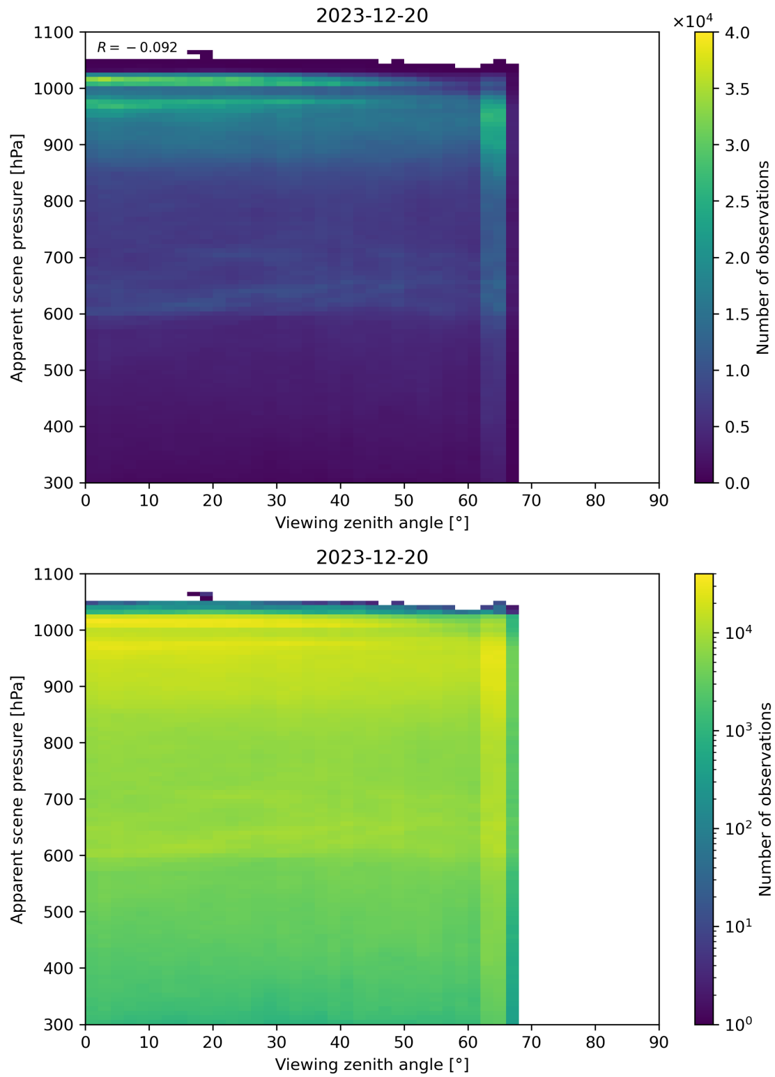
Figure 118: Scatter density plot of “Viewing zenith angle” against “Apparent scene pressure” for 2023-12-20 to 2023-12-21.
