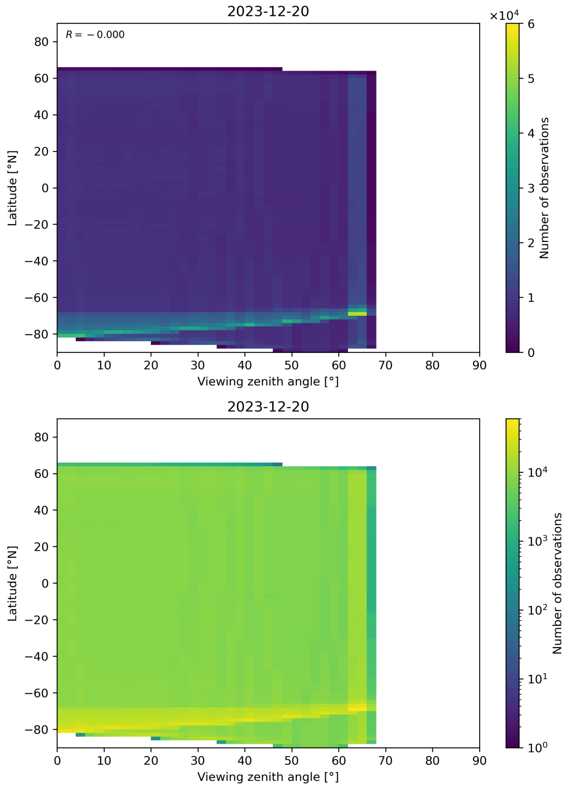
Figure 123: Scatter density plot of “Viewing zenith angle” against “Latitude” for 2023-12-20 to 2023-12-21.
