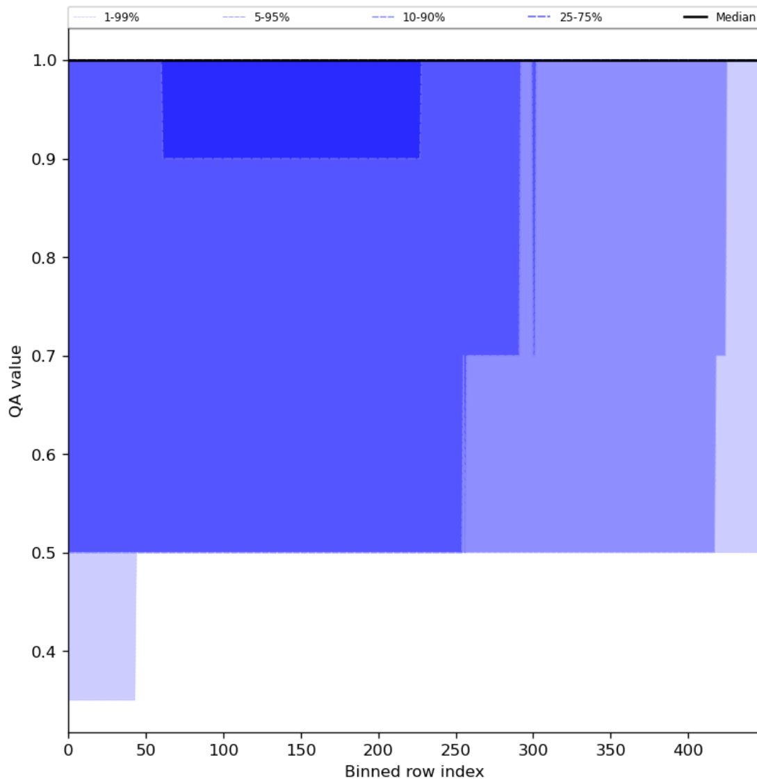
Figure 46: Along track statistics of “QA value” for 2023-12-20 to 2023-12-21
