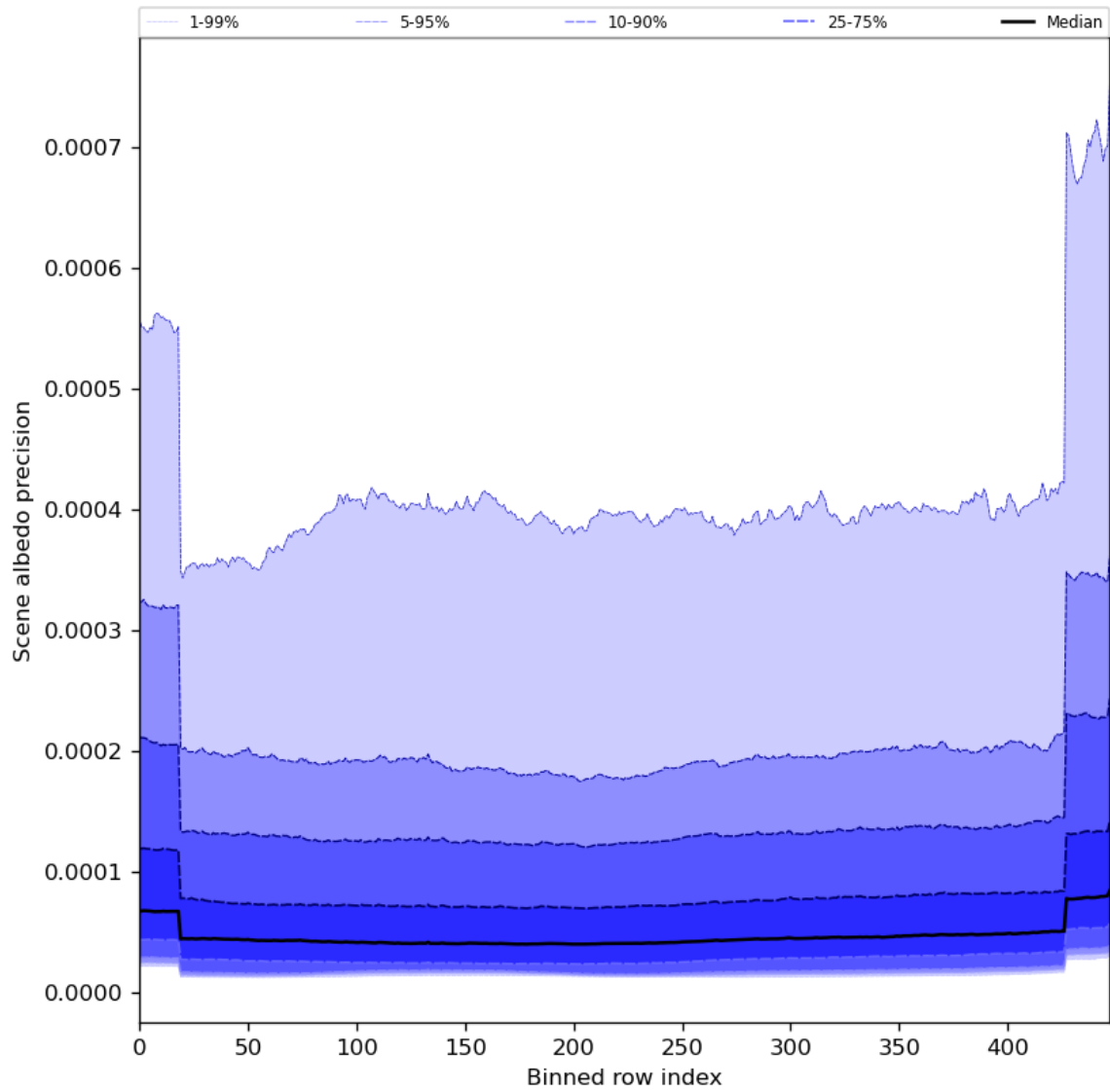
Figure 52: Along track statistics of “Scene albedo precision” for 2023-12-20 to 2023-12-21
