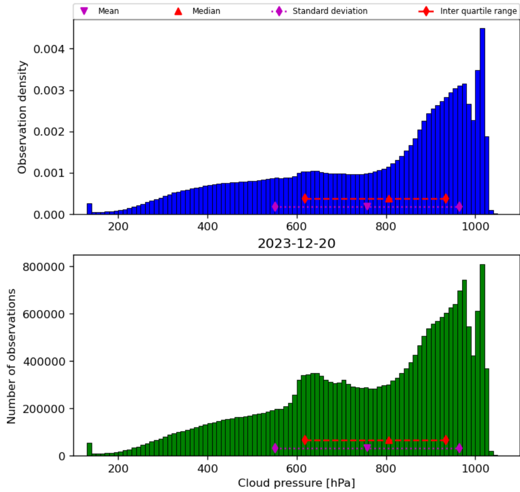
Figure 30: Histogram of “Cloud pressure” for 2023-12-20 to 2023-12-21
