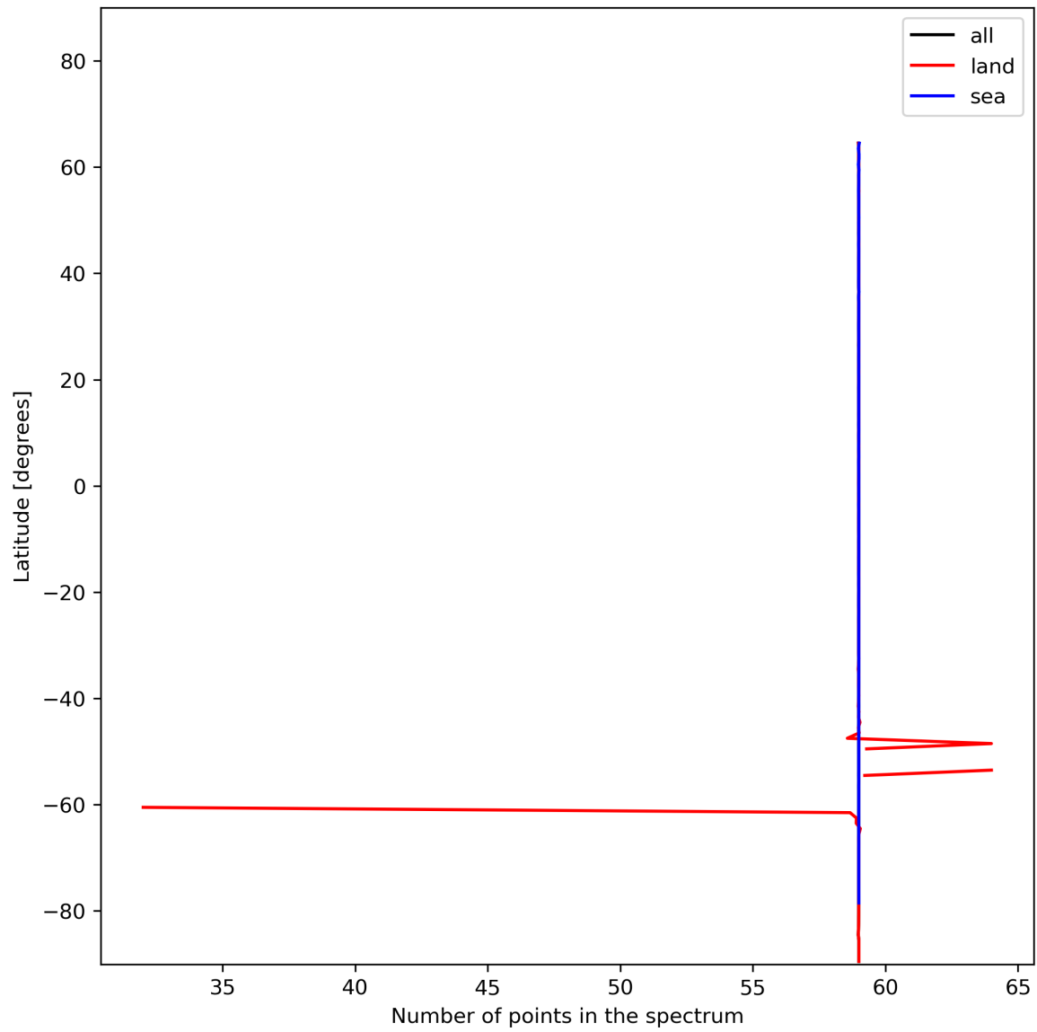
Figure 27: Zonal average of “Number of points in the spectrum” for 2023-12-20 to 2023-12-21.
