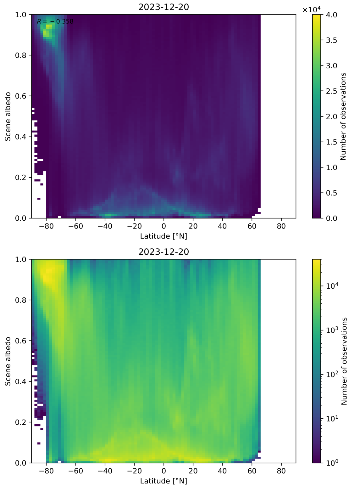
Figure 95: Scatter density plot of “Latitude” against “Scene albedo” for 2023-12-20 to 2023-12-21.
