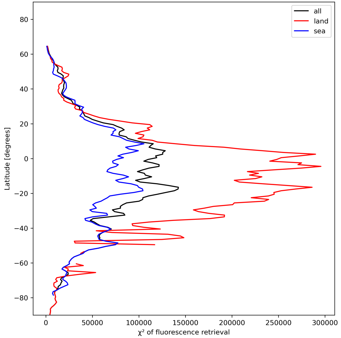
Figure 25: Zonal average of “ \chi^2 of fluorescence retrieval” for 2023-12-20 to 2023-12-21.
