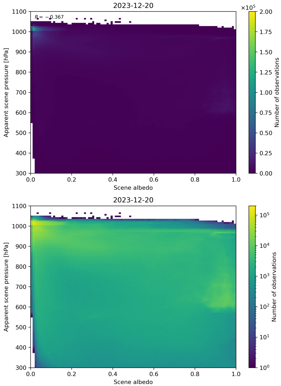
Figure 102: Scatter density plot of “Scene albedo” against “Apparent scene pressure” for 2023-12-20 to 2023-12-21.
