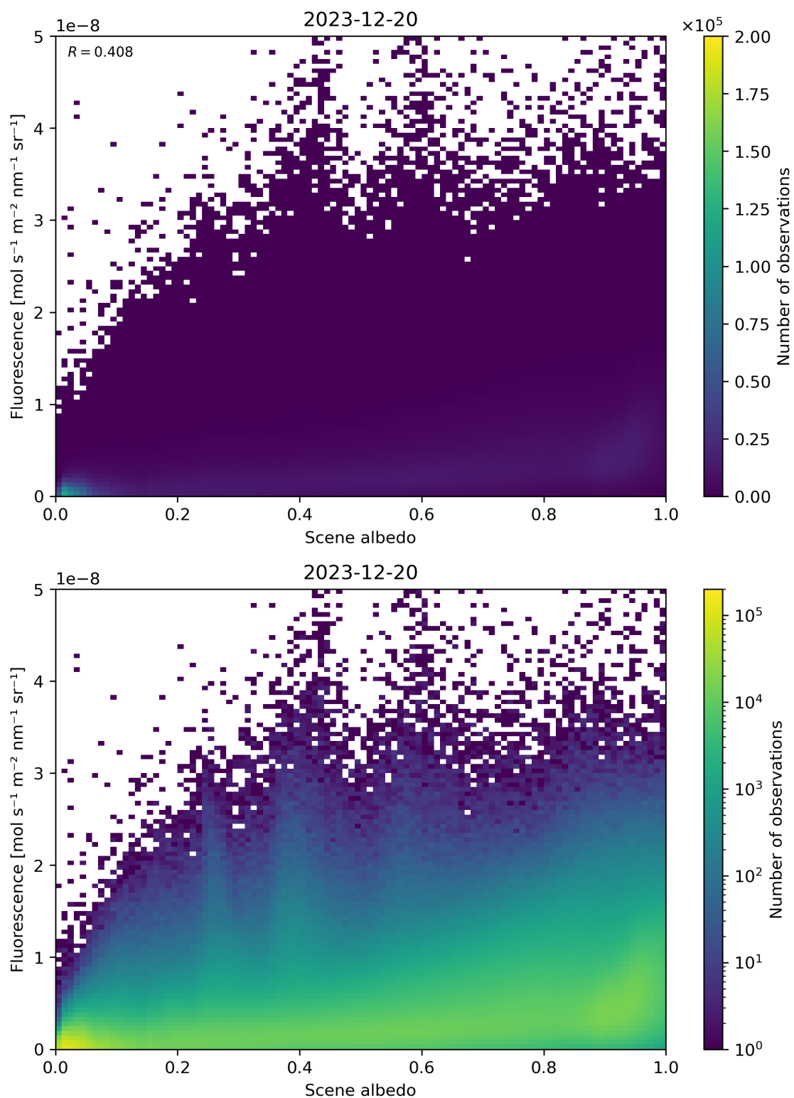
Figure 104: Scatter density plot of “Scene albedo” against “Fluorescence” for 2023-12-20 to 2023-12-21.
