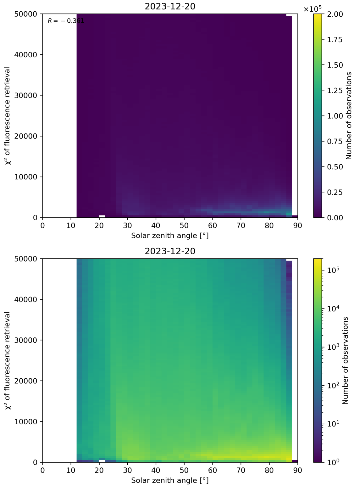
Figure 109: Scatter density plot of “Solar zenith angle” against “ \chi^2 of fluorescence retrieval” for 2023-12-20 to 2023-12-21.
