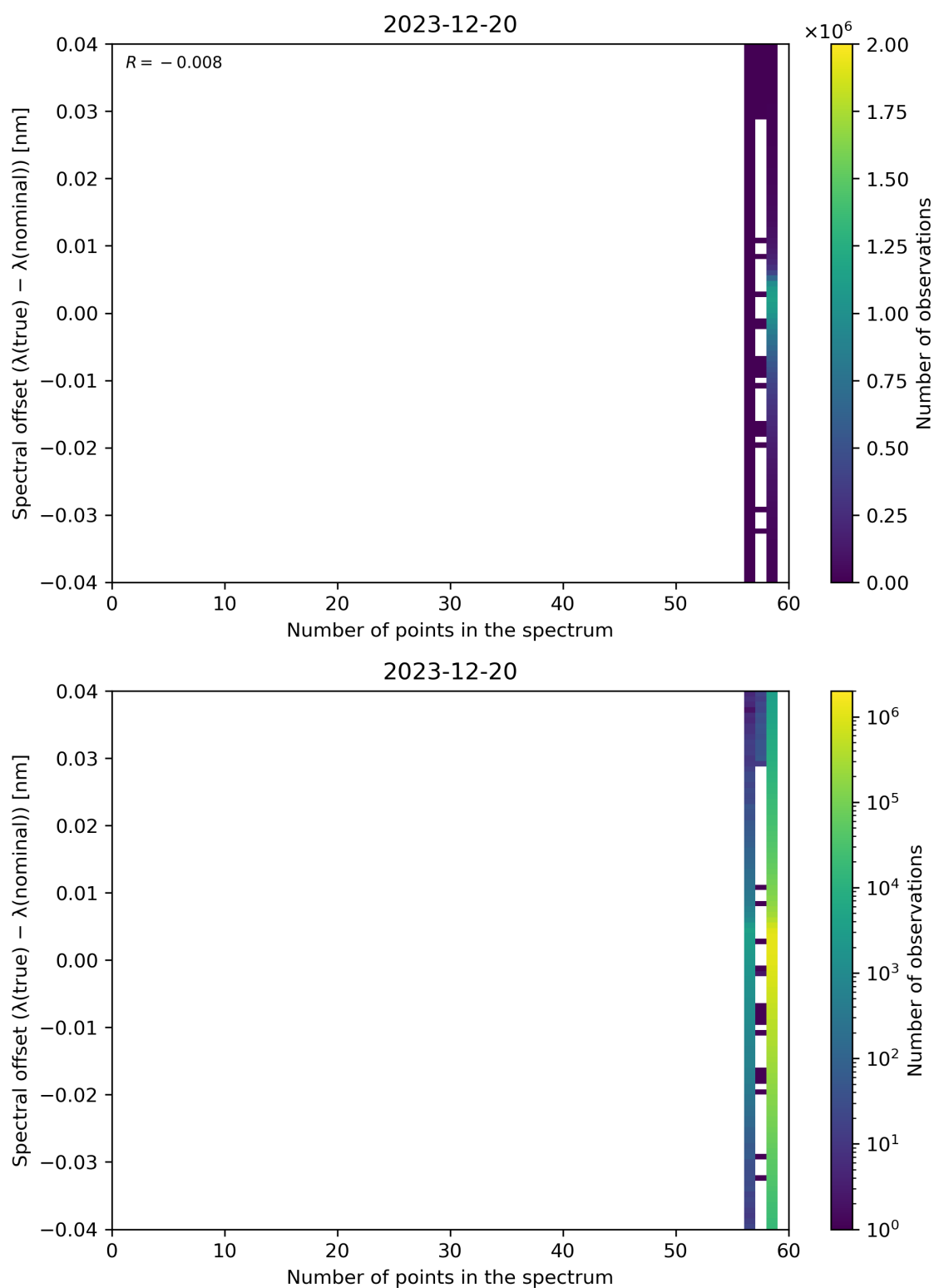
Figure 101: Scatter density plot of “Number of points in the spectrum” against “Spectral offset ( \lambda(\text{true}) - \lambda(\text{nominal}) )” for 2023-12-20 to 2023-12-21.
