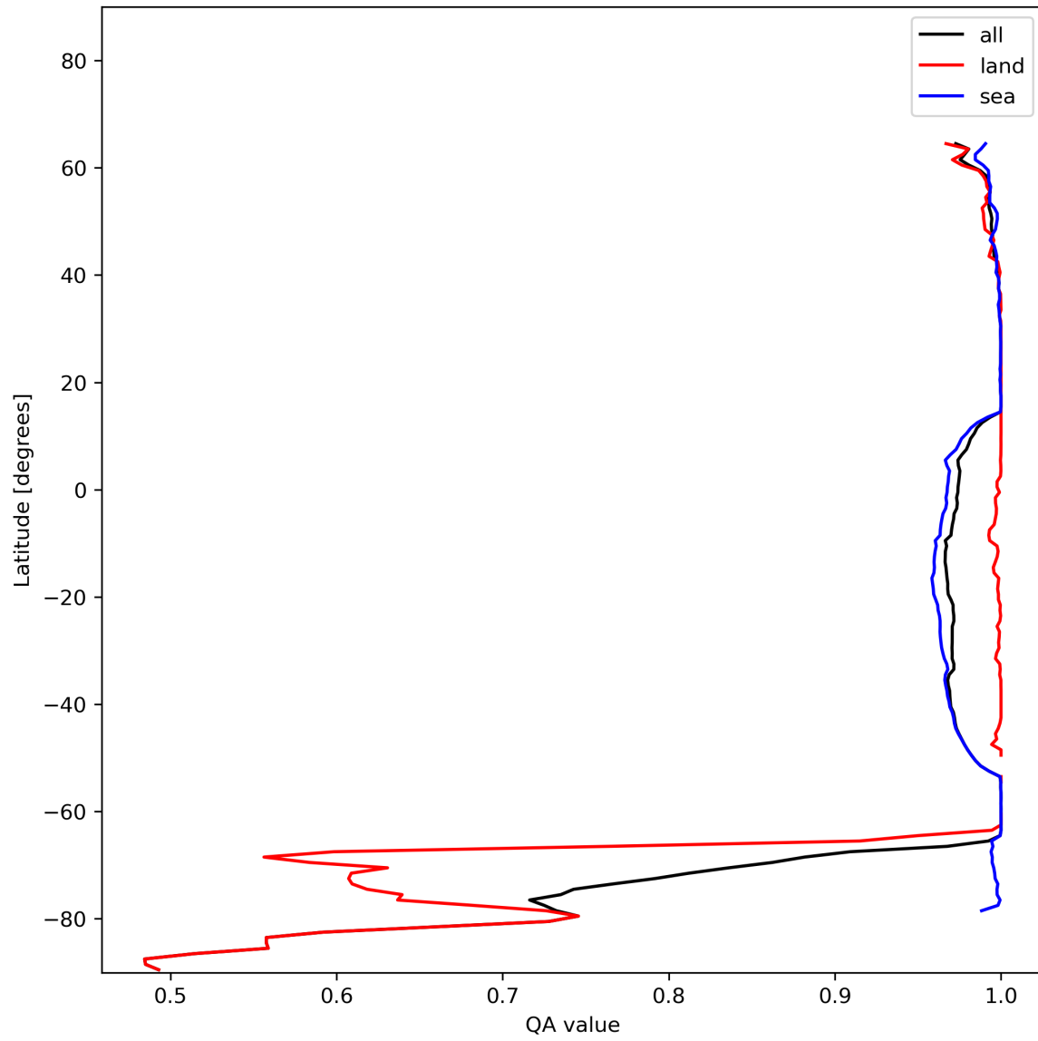
Figure 12: Zonal average of “QA value” for 2023-12-20 to 2023-12-21.
