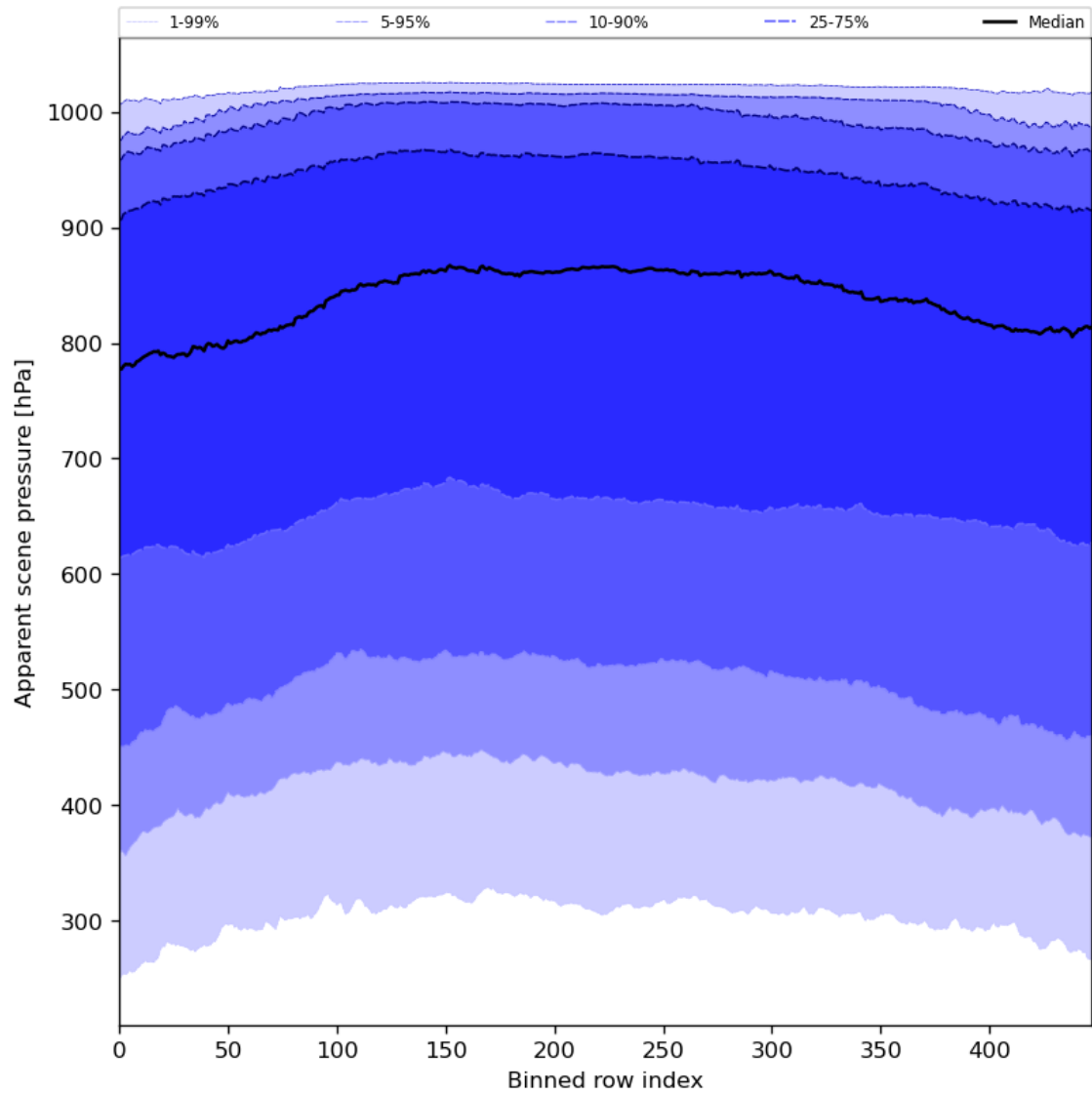
Figure 53: Along track statistics of “Apparent scene pressure” for 2023-12-20 to 2023-12-21
