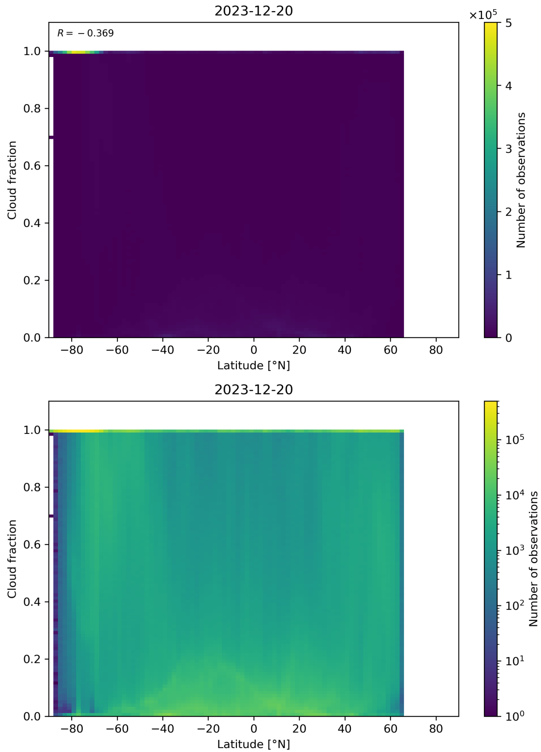
Figure 90: Scatter density plot of “Latitude” against “Cloud fraction” for 2023-12-20 to 2023-12-21.
