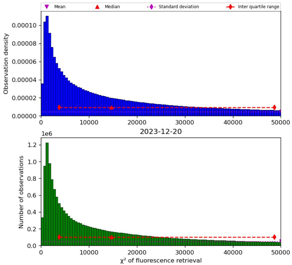
Figure 42: Histogram of “ \chi^2 of fluorescence retrieval” for 2023-12-20 to 2023-12-21
