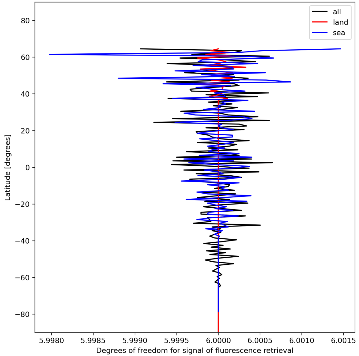
Figure 26: Zonal average of “Degrees of freedom for signal of fluorescence retrieval” for 2023-12-20 to 2023-12-21.
