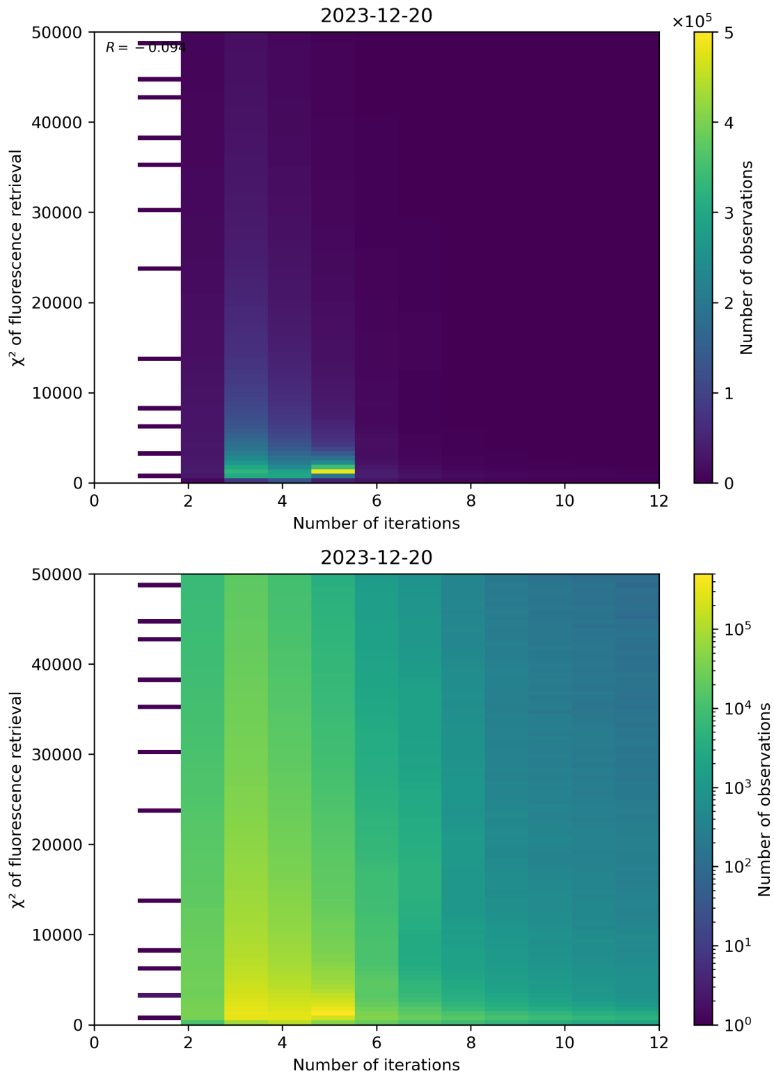
Figure 97: Scatter density plot of “Number of iterations” against “ \chi^2 of fluorescence retrieval” for 2023-12-20 to 2023-12-21.
