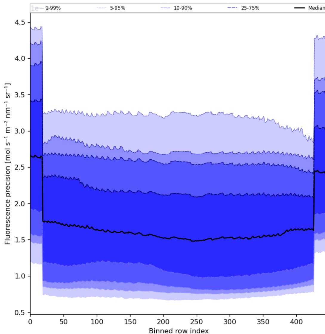
Figure 58: Along track statistics of “Fluorescence precision” for 2023-12-20 to 2023-12-21
