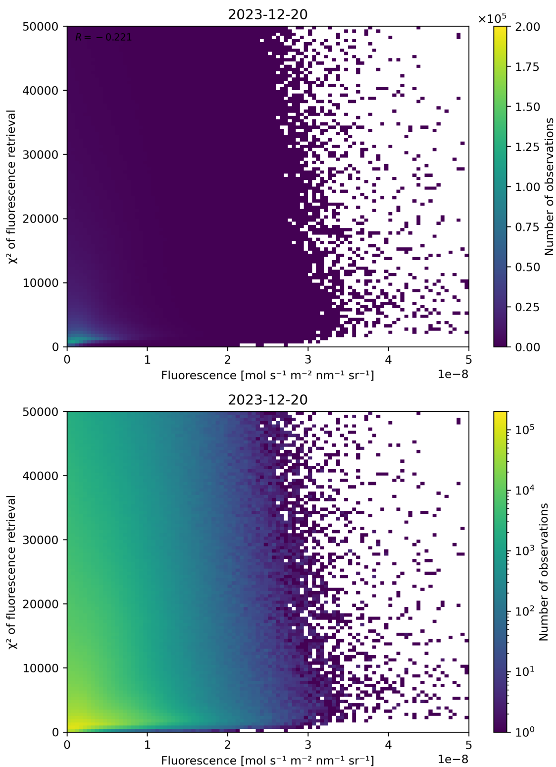
Figure 85: Scatter density plot of “Fluorescence” against “ \chi^2 of fluorescence retrieval” for 2023-12-20 to 2023-12-21.
