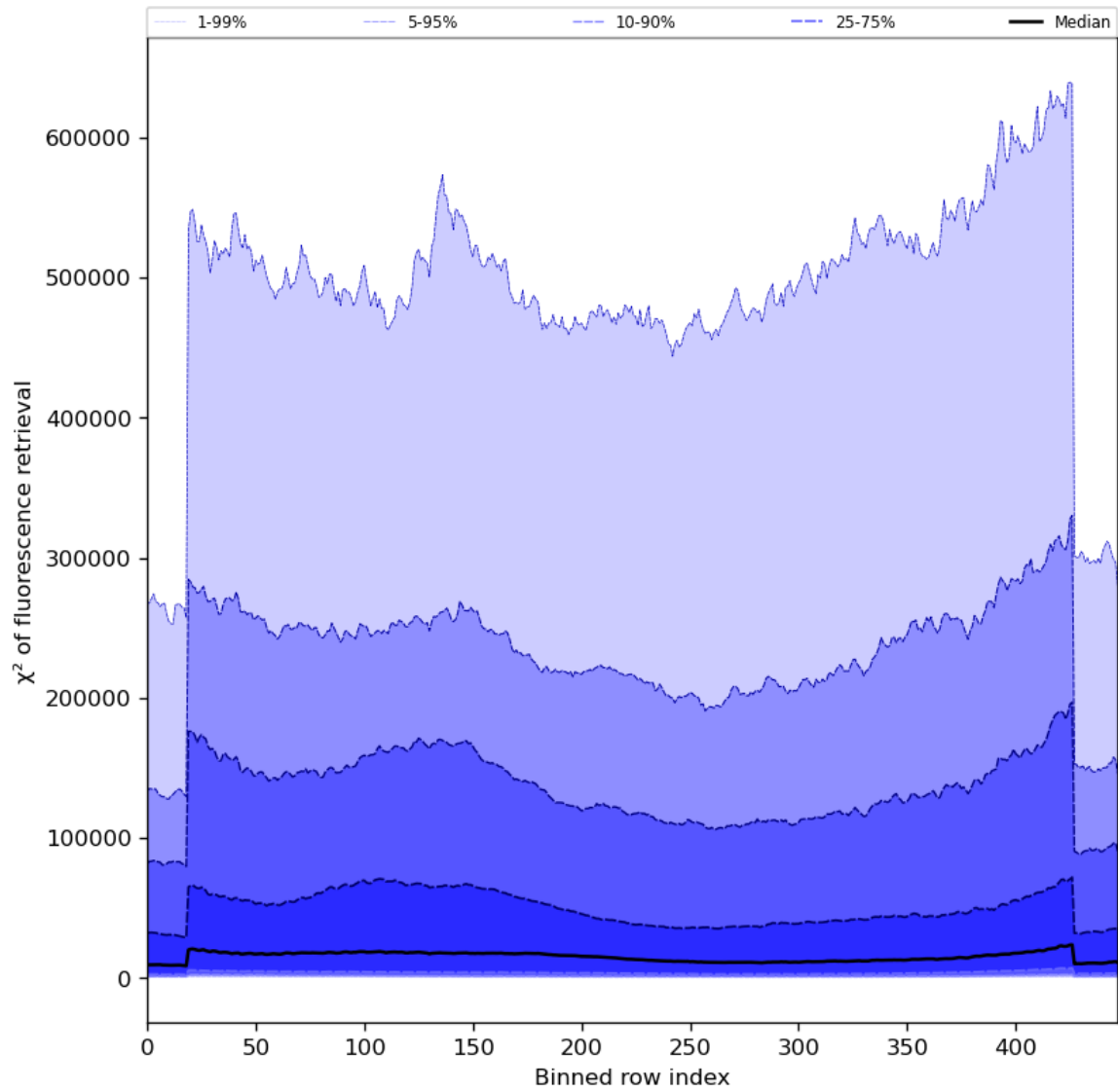
Figure 59: Along track statistics of “ \chi^2 of fluorescence retrieval” for 2023-12-20 to 2023-12-21
