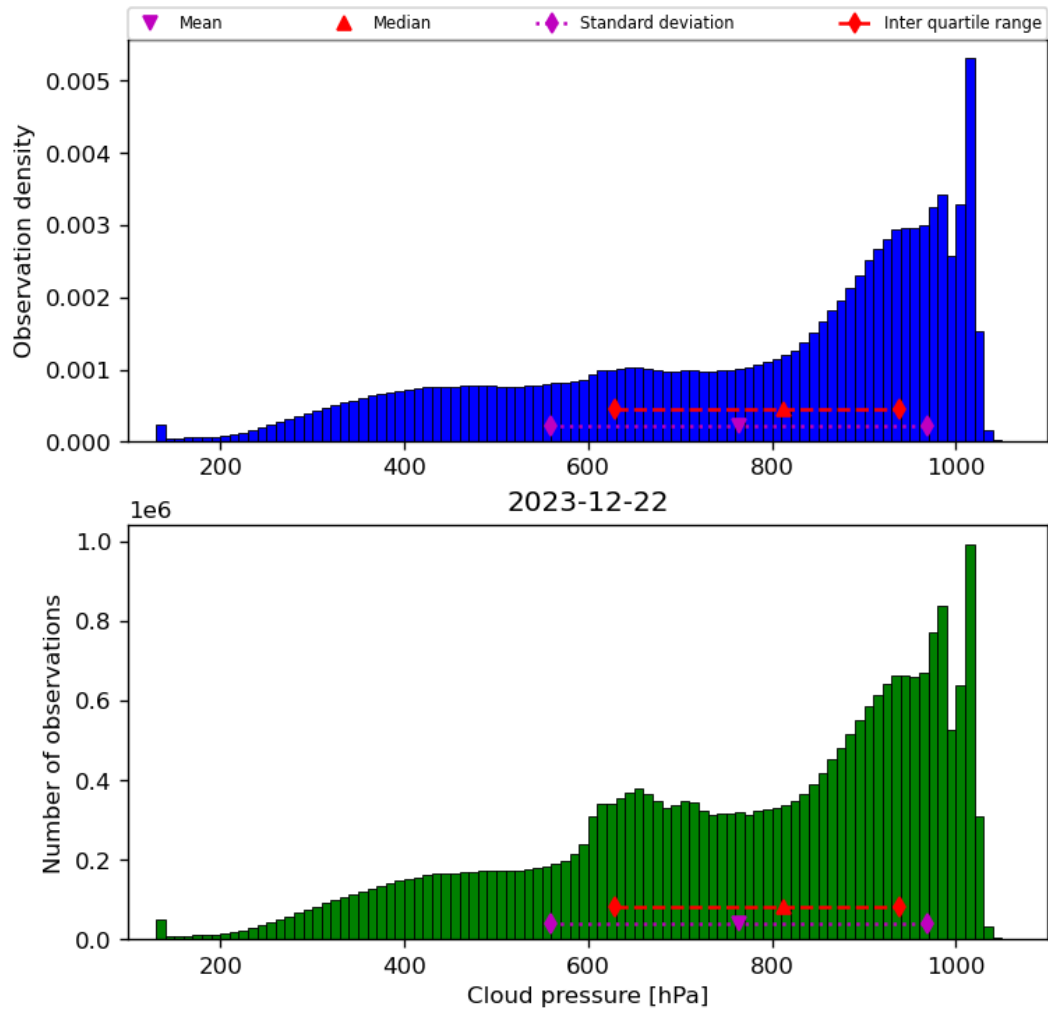
Figure 30: Histogram of “Cloud pressure” for 2023-12-21 to 2023-12-23
