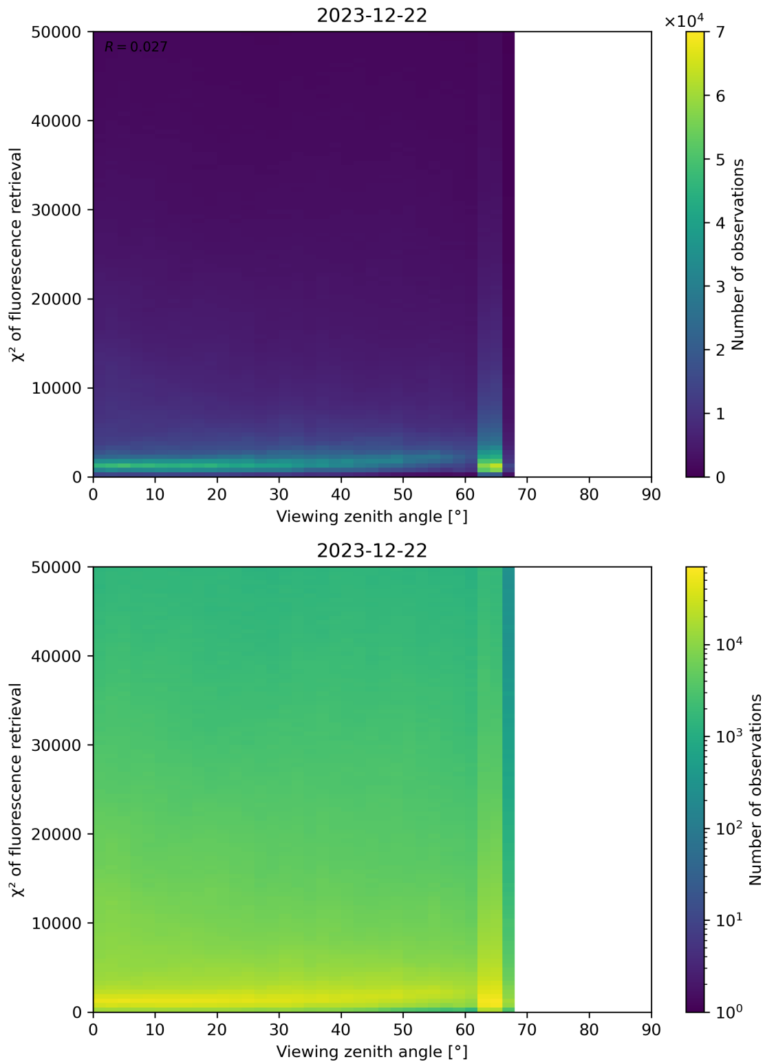
Figure 119: Scatter density plot of “Viewing zenith angle” against “ \chi^2 of fluorescence retrieval” for 2023-12-21 to 2023-12-23.
