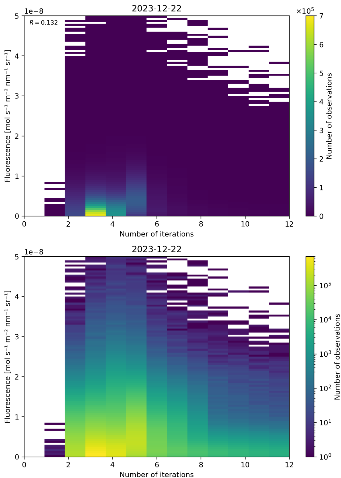
Figure 98: Scatter density plot of “Number of iterations” against “Fluorescence” for 2023-12-21 to 2023-12-23.
