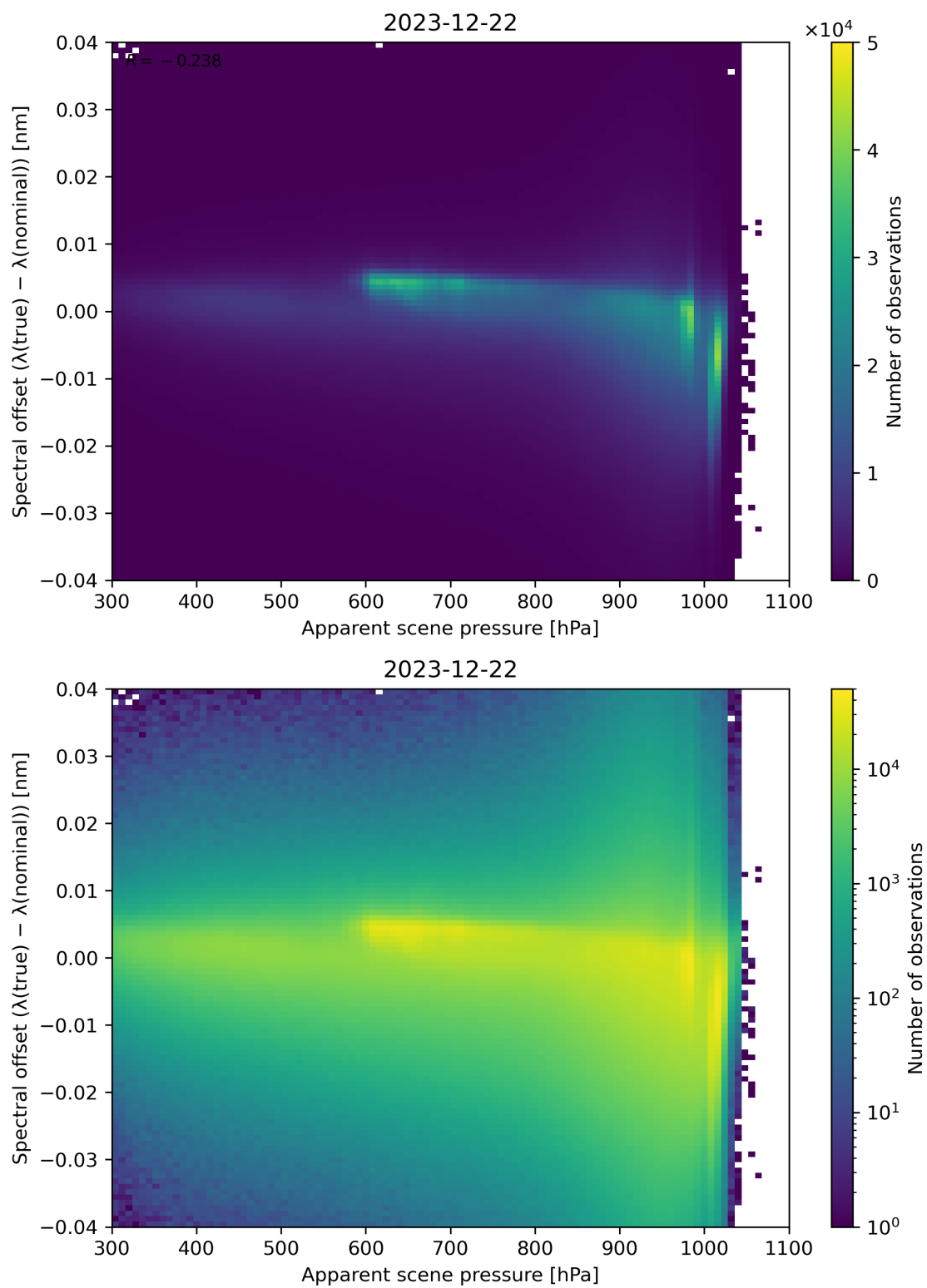
Figure 67: Scatter density plot of “Apparent scene pressure” against “Spectral offset ( \lambda(\text{true}) - \lambda(\text{nominal}) )” for 2023-12-21 to 2023-12-23.
