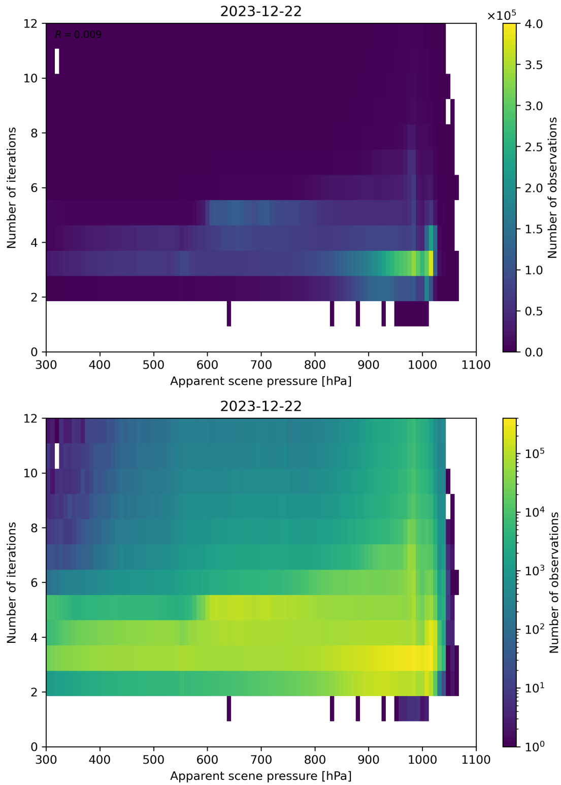
Figure 65: Scatter density plot of “Apparent scene pressure” against “Number of iterations” for 2023-12-21 to 2023-12-23.
