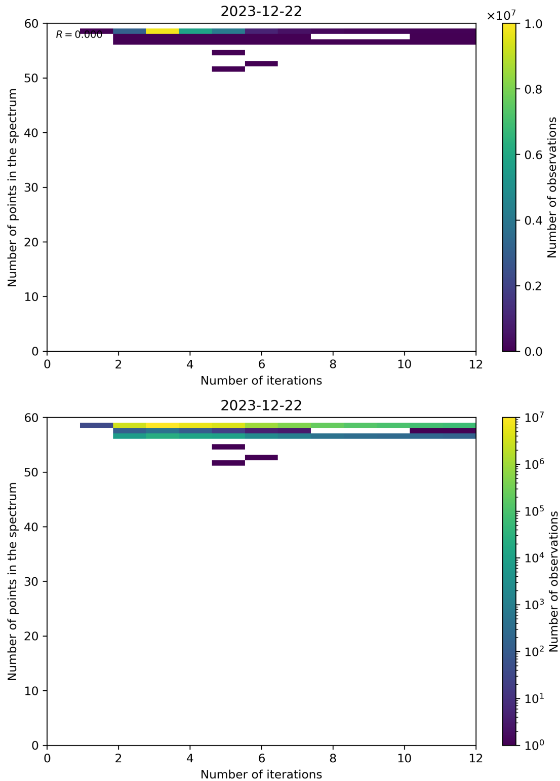
Figure 99: Scatter density plot of “Number of iterations” against “Number of points in the spectrum” for 2023-12-21 to 2023-12-23.
