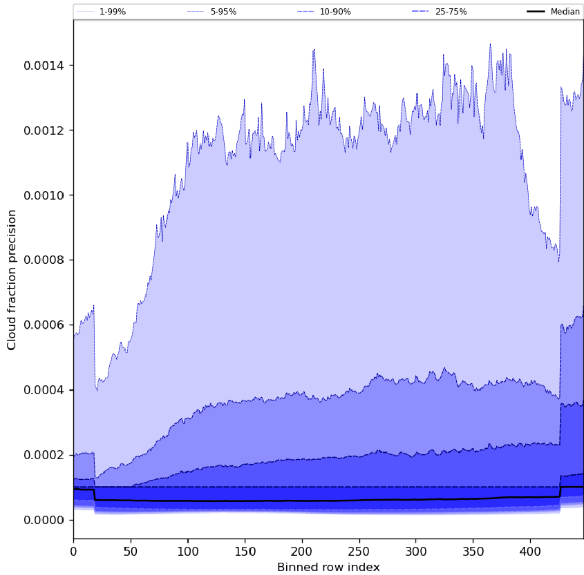
Figure 50: Along track statistics of “Cloud fraction precision” for 2023-12-21 to 2023-12-23
