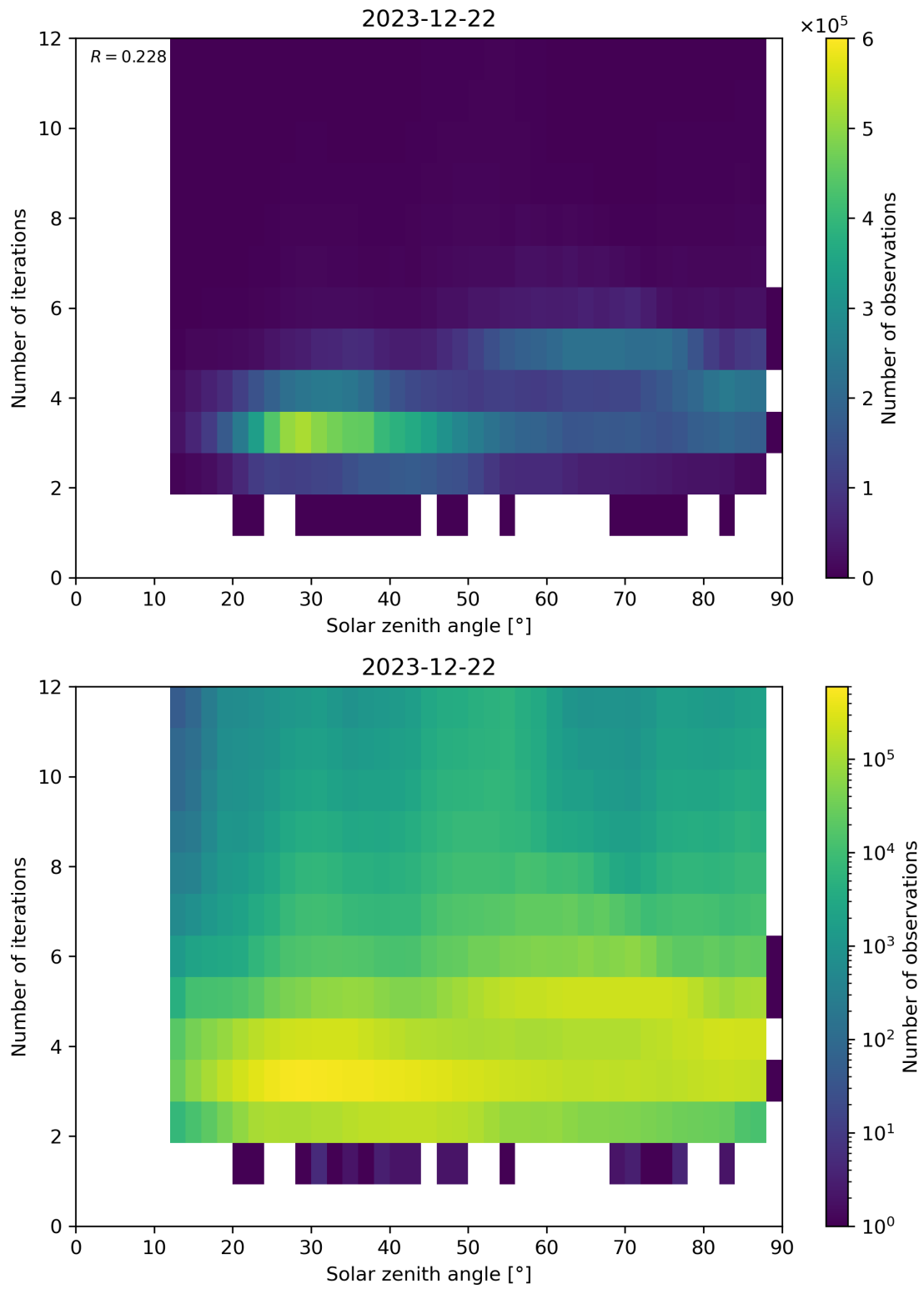
Figure 114: Scatter density plot of “Solar zenith angle” against “Number of iterations” for 2023-12-21 to 2023-12-23.
