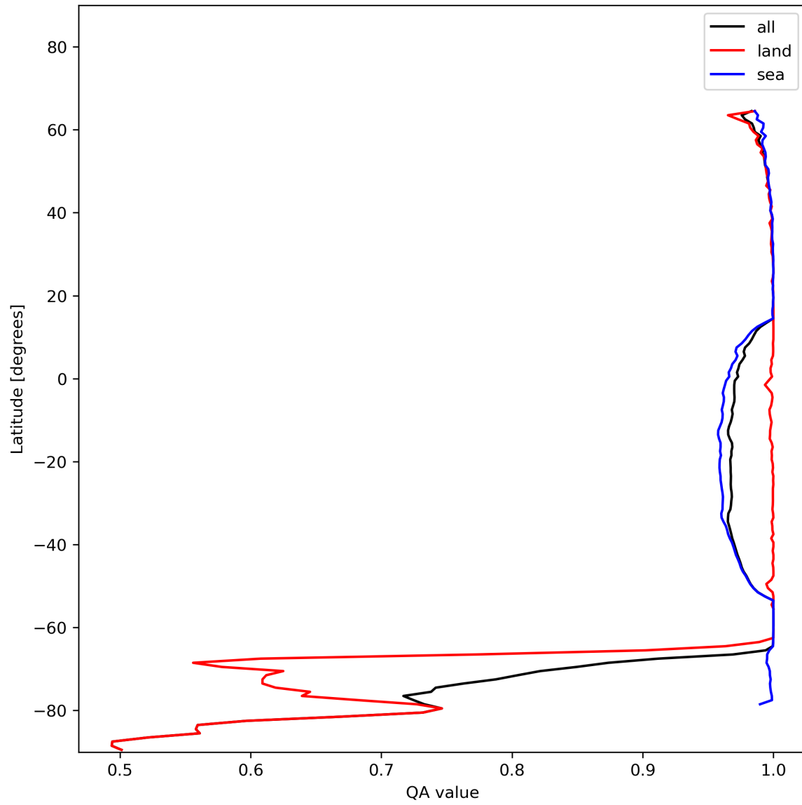
Figure 12: Zonal average of “QA value” for 2023-12-21 to 2023-12-23.
