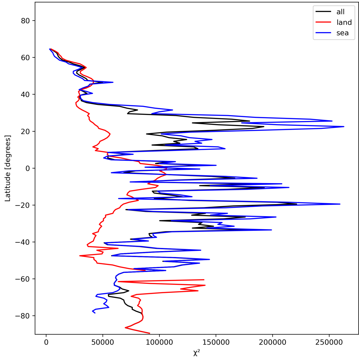
Figure 21: Zonal average of “ \chi^2 ” for 2023-12-21 to 2023-12-23.
