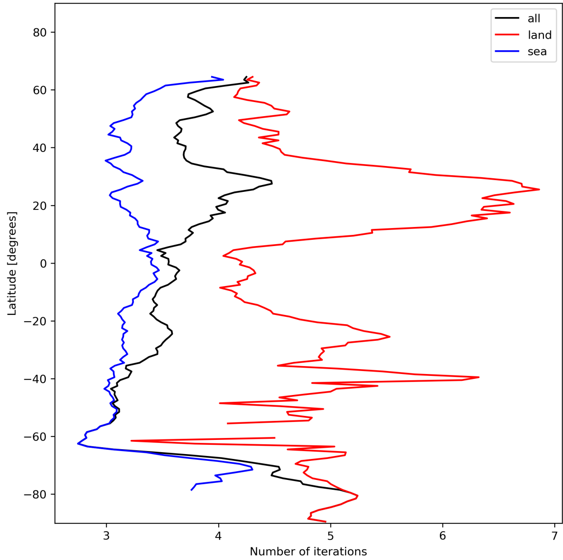
Figure 22: Zonal average of “Number of iterations” for 2023-12-21 to 2023-12-23.
