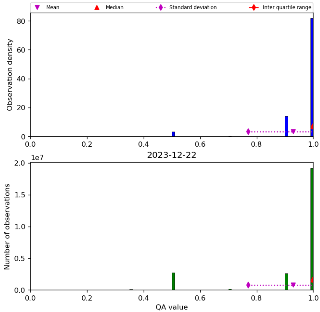
Figure 29: Histogram of “QA value” for 2023-12-21 to 2023-12-23
