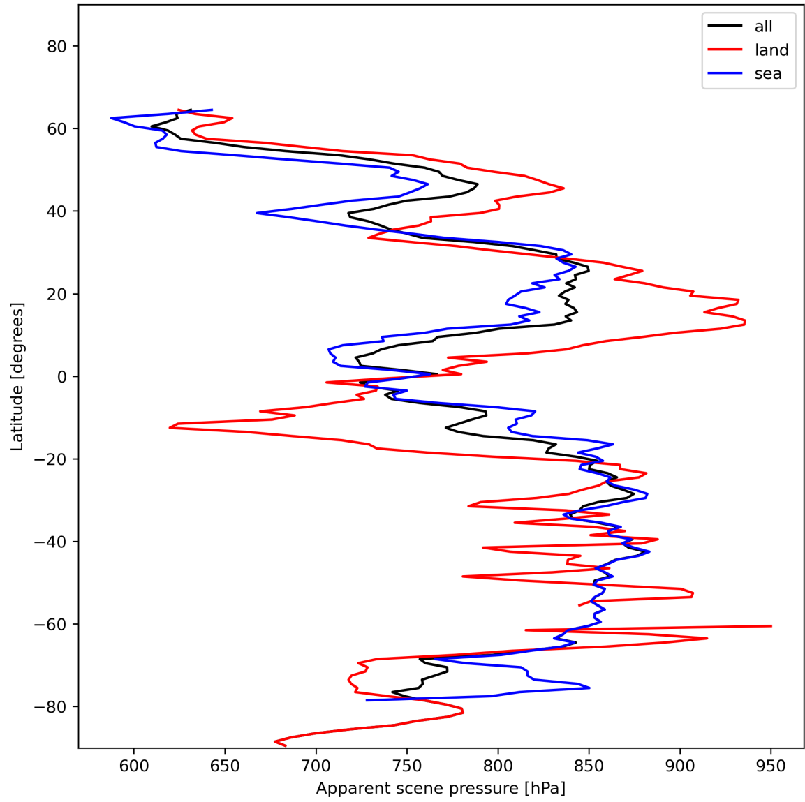
Figure 19: Zonal average of “Apparent scene pressure” for 2023-12-21 to 2023-12-23.
