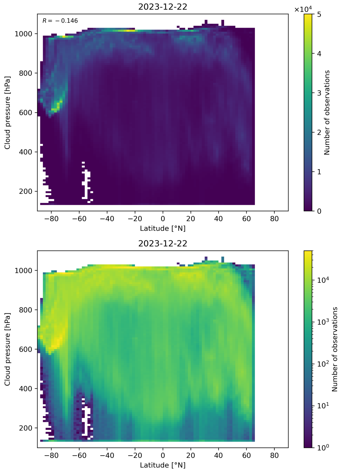
Figure 91: Scatter density plot of “Latitude” against “Cloud pressure” for 2023-12-21 to 2023-12-23.
