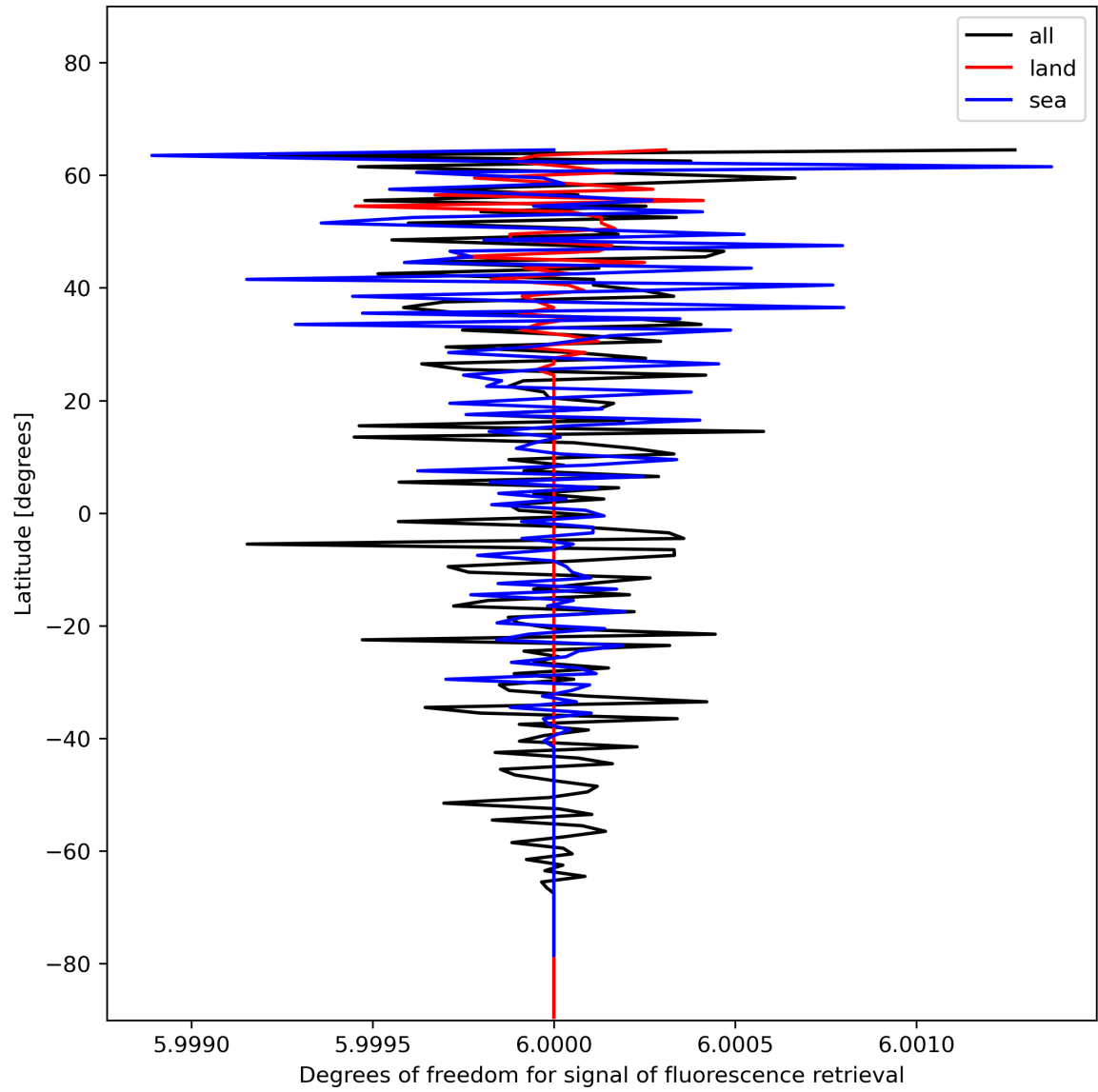
Figure 26: Zonal average of “Degrees of freedom for signal of fluorescence retrieval” for 2023-12-21 to 2023-12-23.
