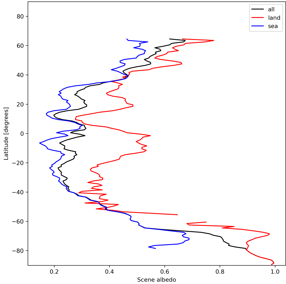
Figure 17: Zonal average of “Scene albedo” for 2023-12-21 to 2023-12-23.
