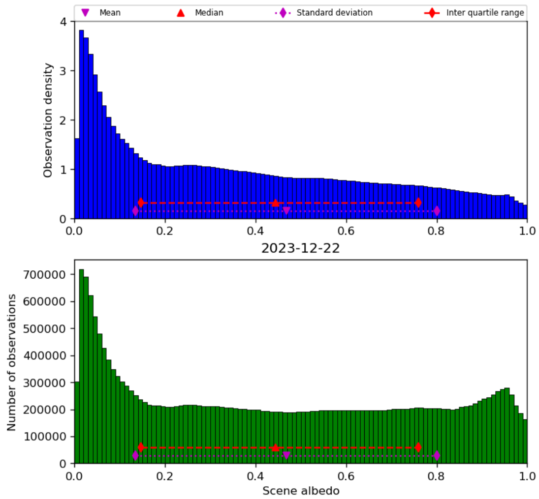
Figure 34: Histogram of “Scene albedo” for 2023-12-21 to 2023-12-23
