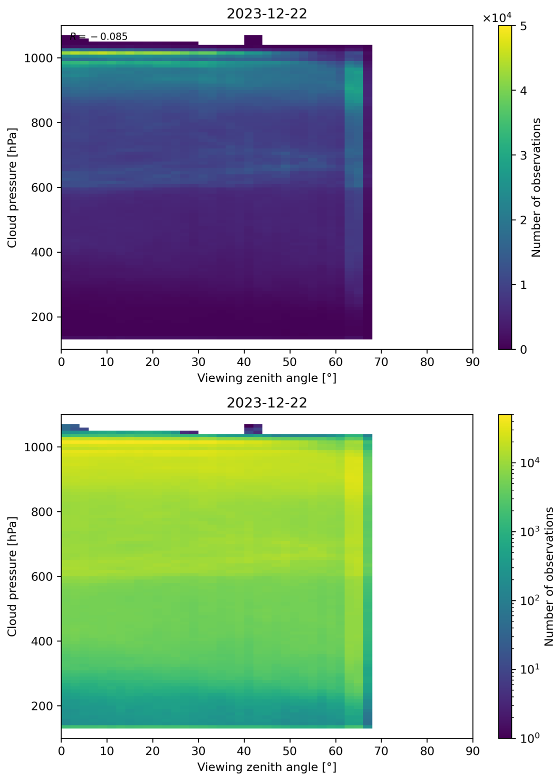
Figure 121: Scatter density plot of “Viewing zenith angle” against “Cloud pressure” for 2023-12-21 to 2023-12-23.
