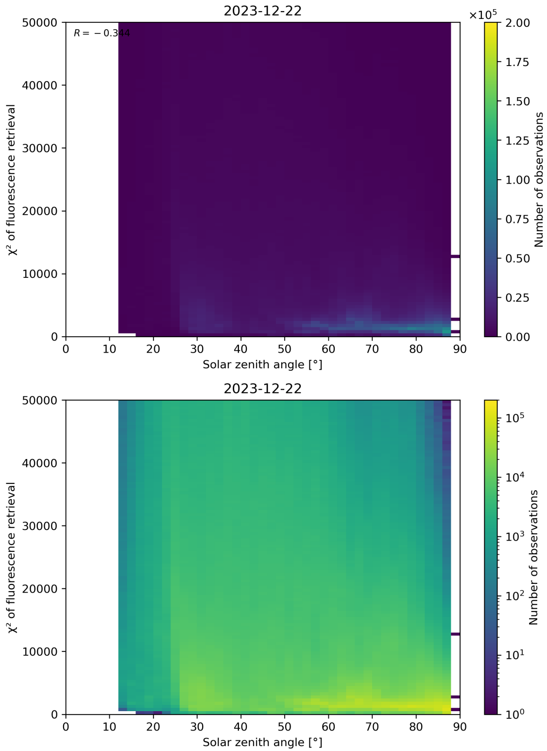
Figure 109: Scatter density plot of “Solar zenith angle” against “ \chi^2 of fluorescence retrieval” for 2023-12-21 to 2023-12-23.
