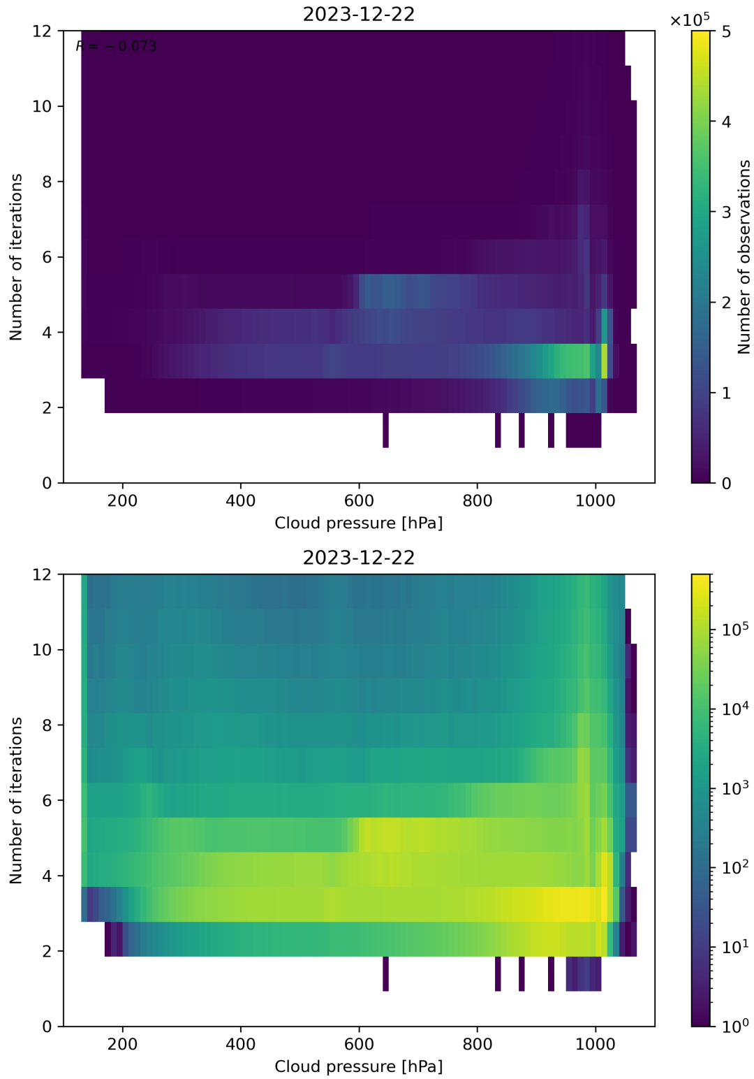
Figure 81: Scatter density plot of “Cloud pressure” against “Number of iterations” for 2023-12-21 to 2023-12-23.
