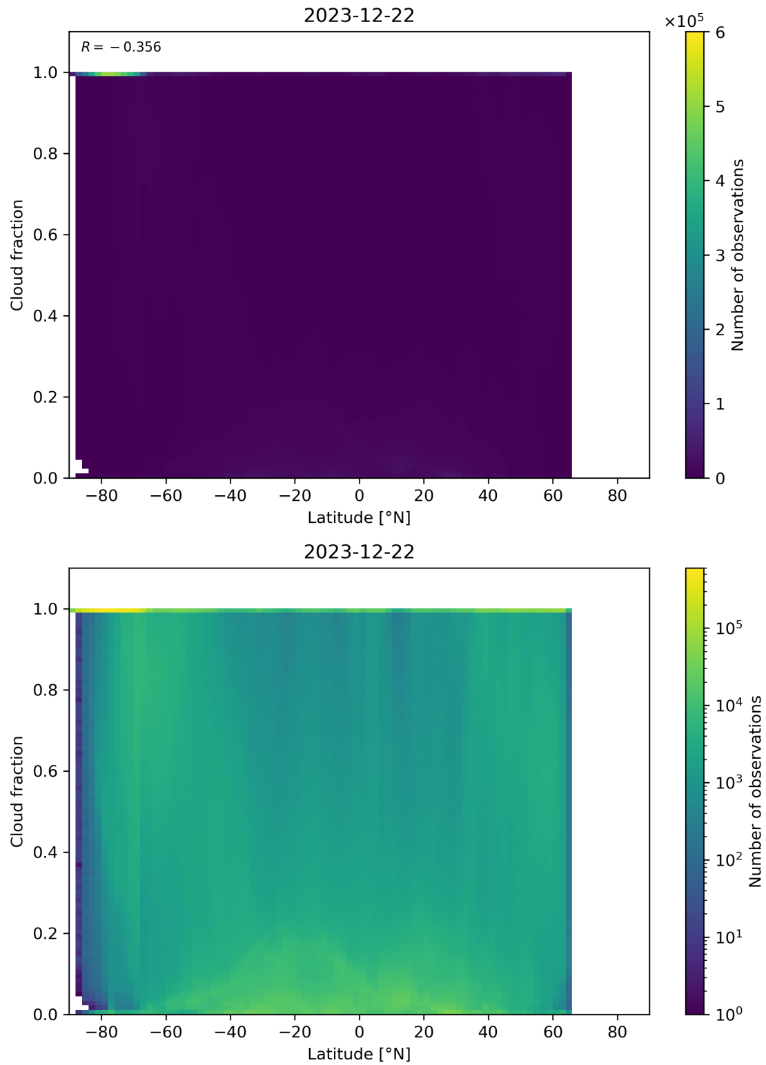
Figure 90: Scatter density plot of “Latitude” against “Cloud fraction” for 2023-12-21 to 2023-12-23.
