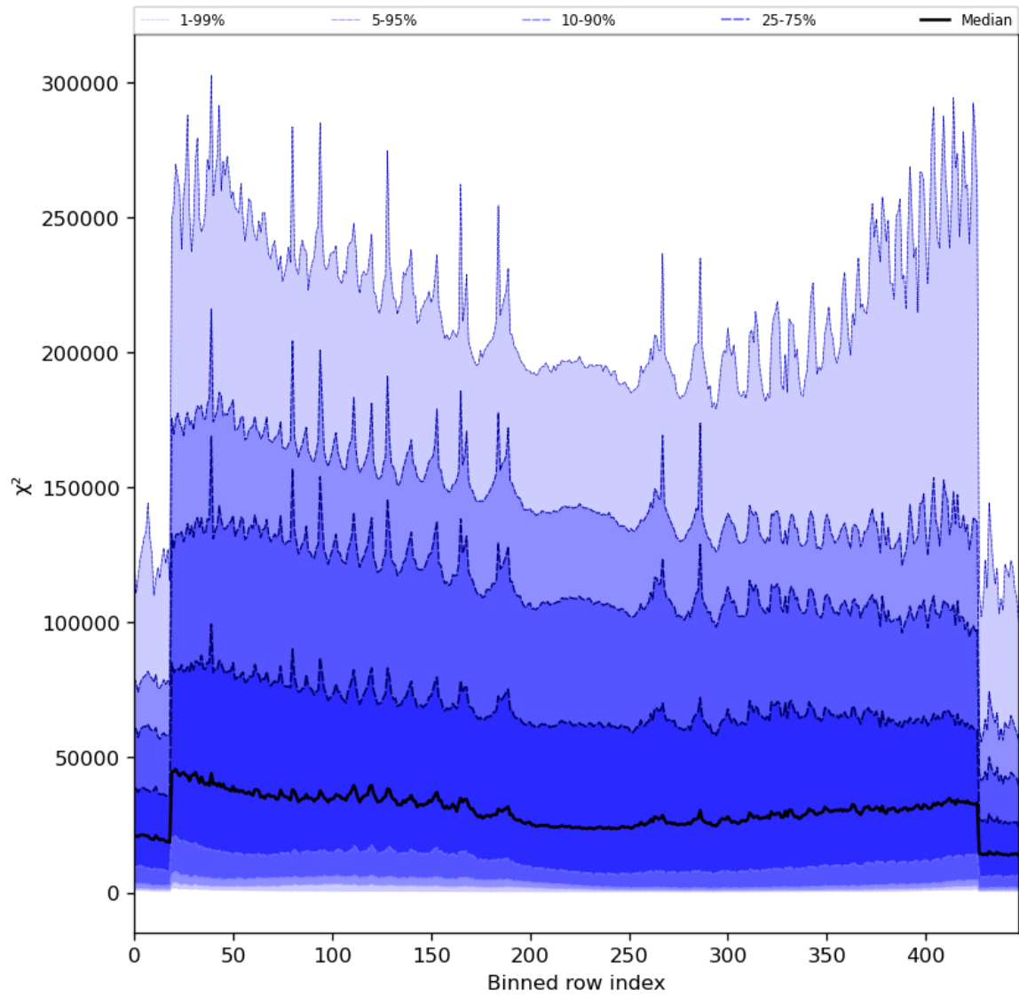
Figure 55: Along track statistics of “ \chi^2 ” for 2023-12-21 to 2023-12-23
