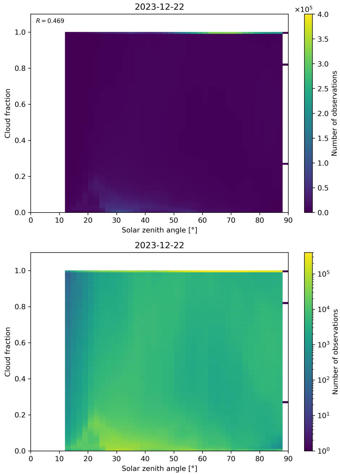
Figure 110: Scatter density plot of “Solar zenith angle” against “Cloud fraction” for 2023-12-21 to 2023-12-23.
