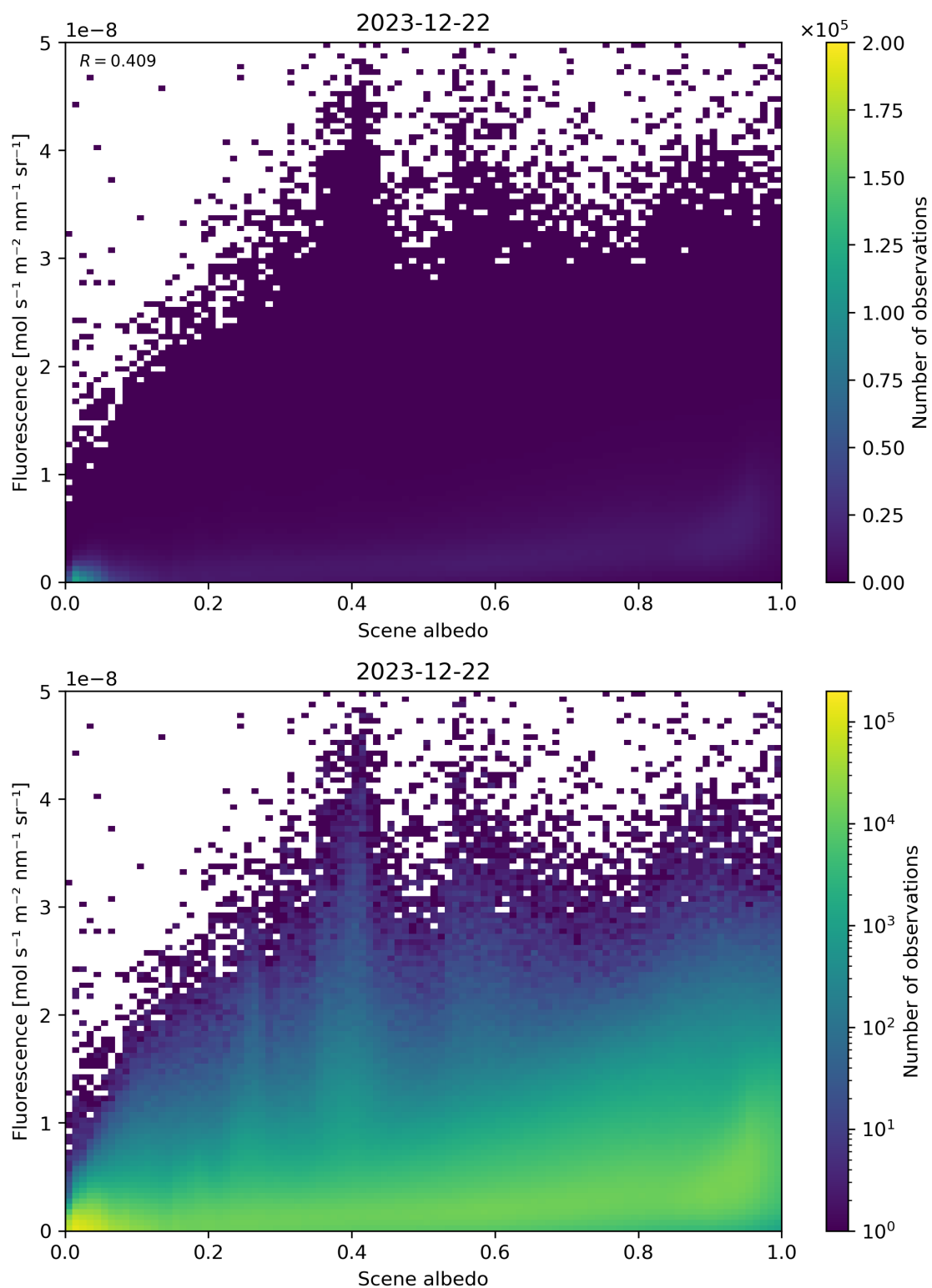
Figure 104: Scatter density plot of “Scene albedo” against “Fluorescence” for 2023-12-21 to 2023-12-23.
