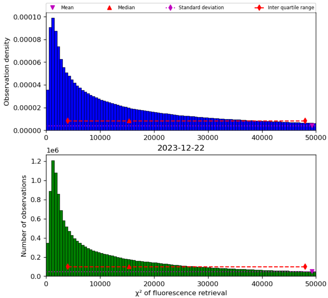
Figure 42: Histogram of “ \chi^2 of fluorescence retrieval” for 2023-12-21 to 2023-12-23
