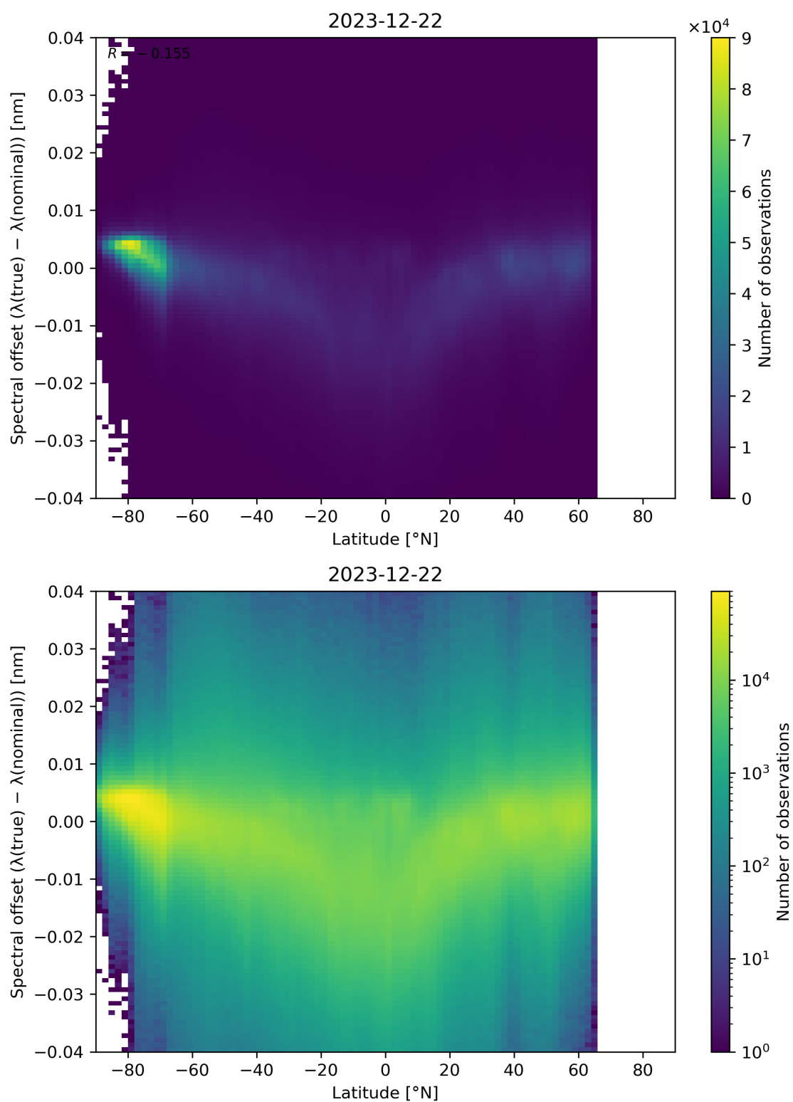
Figure 96: Scatter density plot of “Latitude” against “Spectral offset ( \lambda(\text{true}) - \lambda(\text{nominal}) )” for 2023-12-21 to 2023-12-23.
