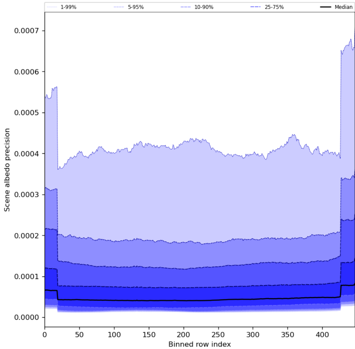
Figure 52: Along track statistics of “Scene albedo precision” for 2023-12-21 to 2023-12-23
