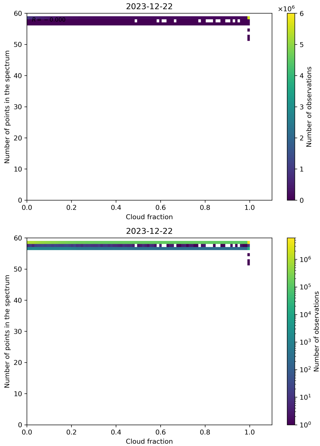
Figure 74: Scatter density plot of “Cloud fraction” against “Number of points in the spectrum” for 2023-12-21 to 2023-12-23.
