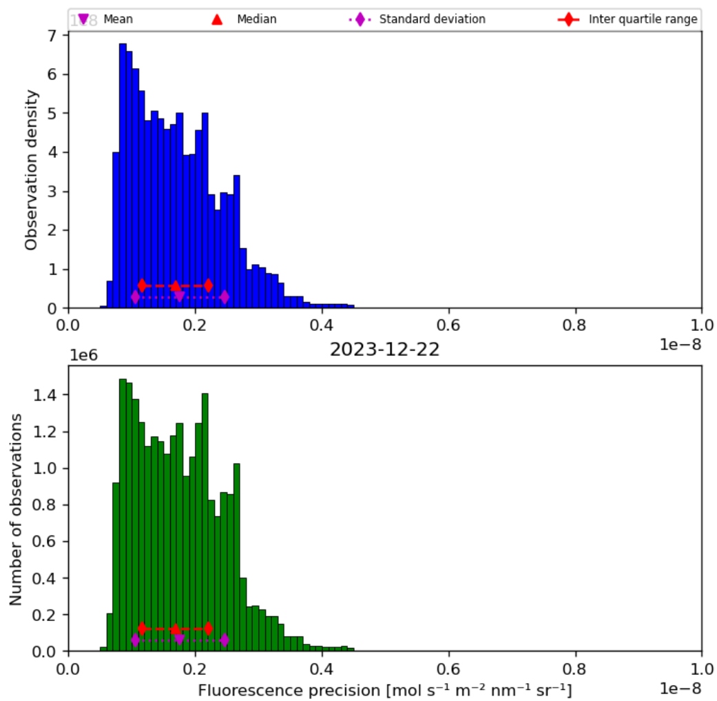
Figure 41: Histogram of “Fluorescence precision” for 2023-12-21 to 2023-12-23
