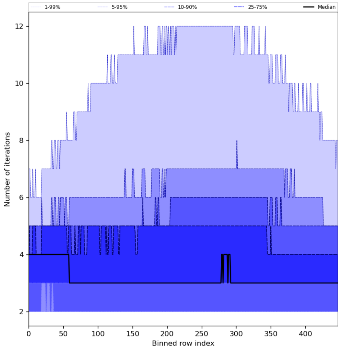
Figure 56: Along track statistics of “Number of iterations” for 2023-12-21 to 2023-12-23
