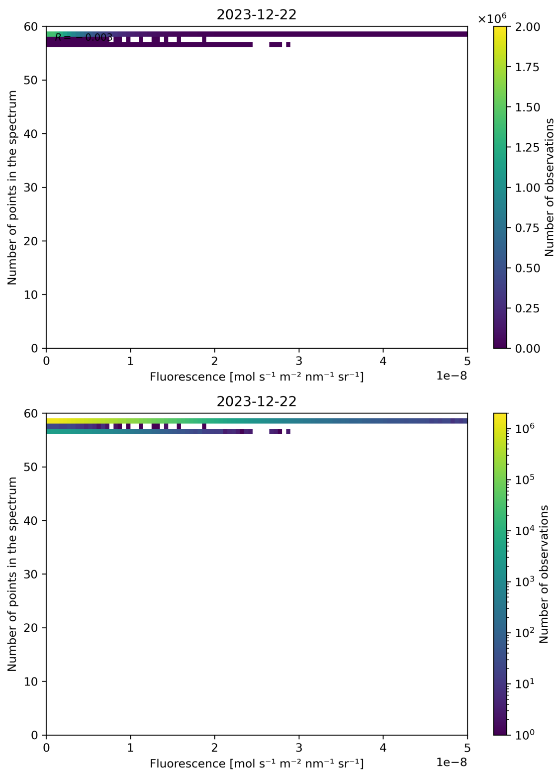
Figure 86: Scatter density plot of “Fluorescence” against “Number of points in the spectrum” for 2023-12-21 to 2023-12-23.
