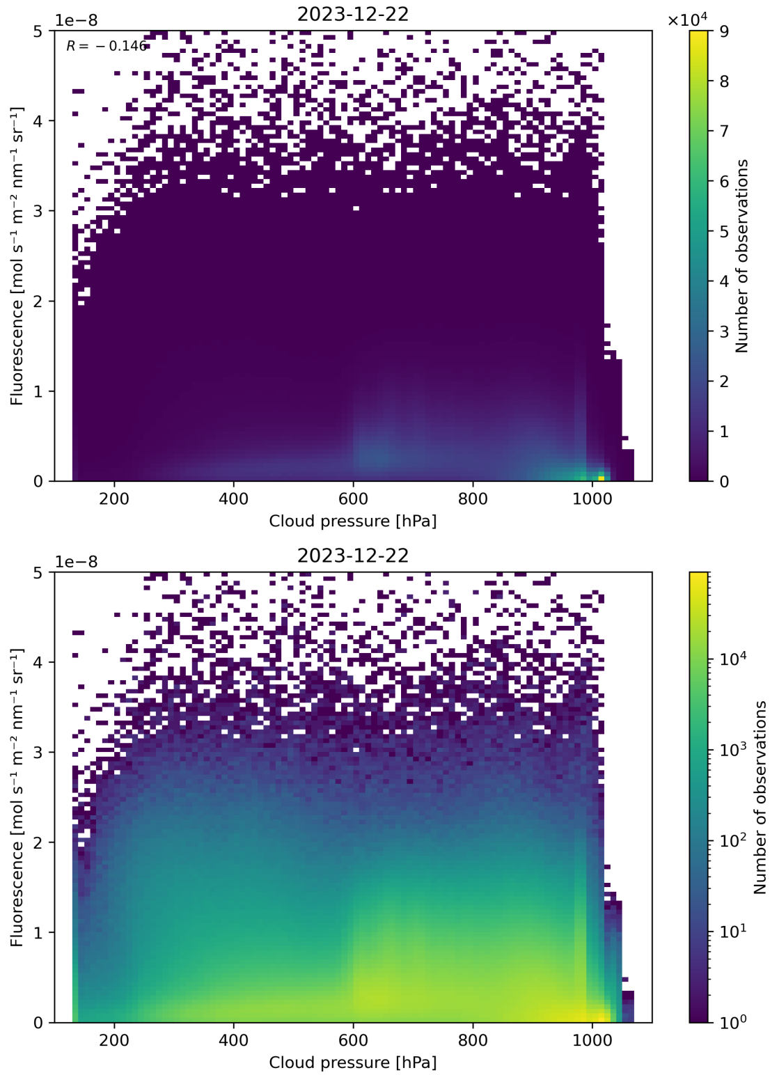
Figure 80: Scatter density plot of “Cloud pressure” against “Fluorescence” for 2023-12-21 to 2023-12-23.
