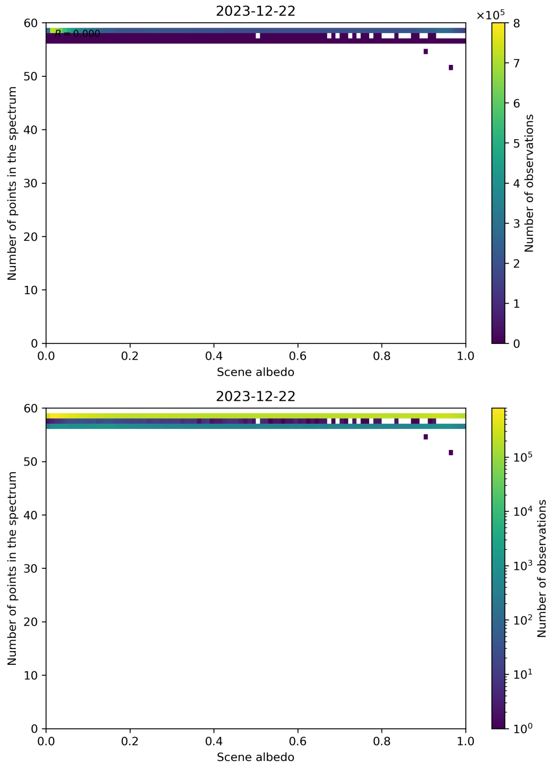
Figure 106: Scatter density plot of “Scene albedo” against “Number of points in the spectrum” for 2023-12-21 to 2023-12-23.
