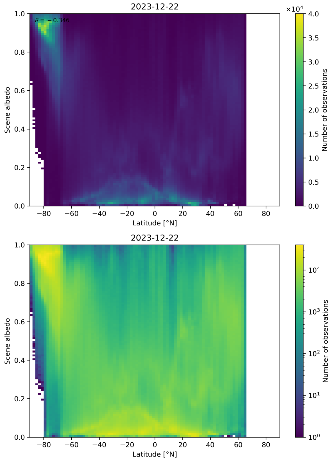
Figure 95: Scatter density plot of “Latitude” against “Scene albedo” for 2023-12-21 to 2023-12-23.
