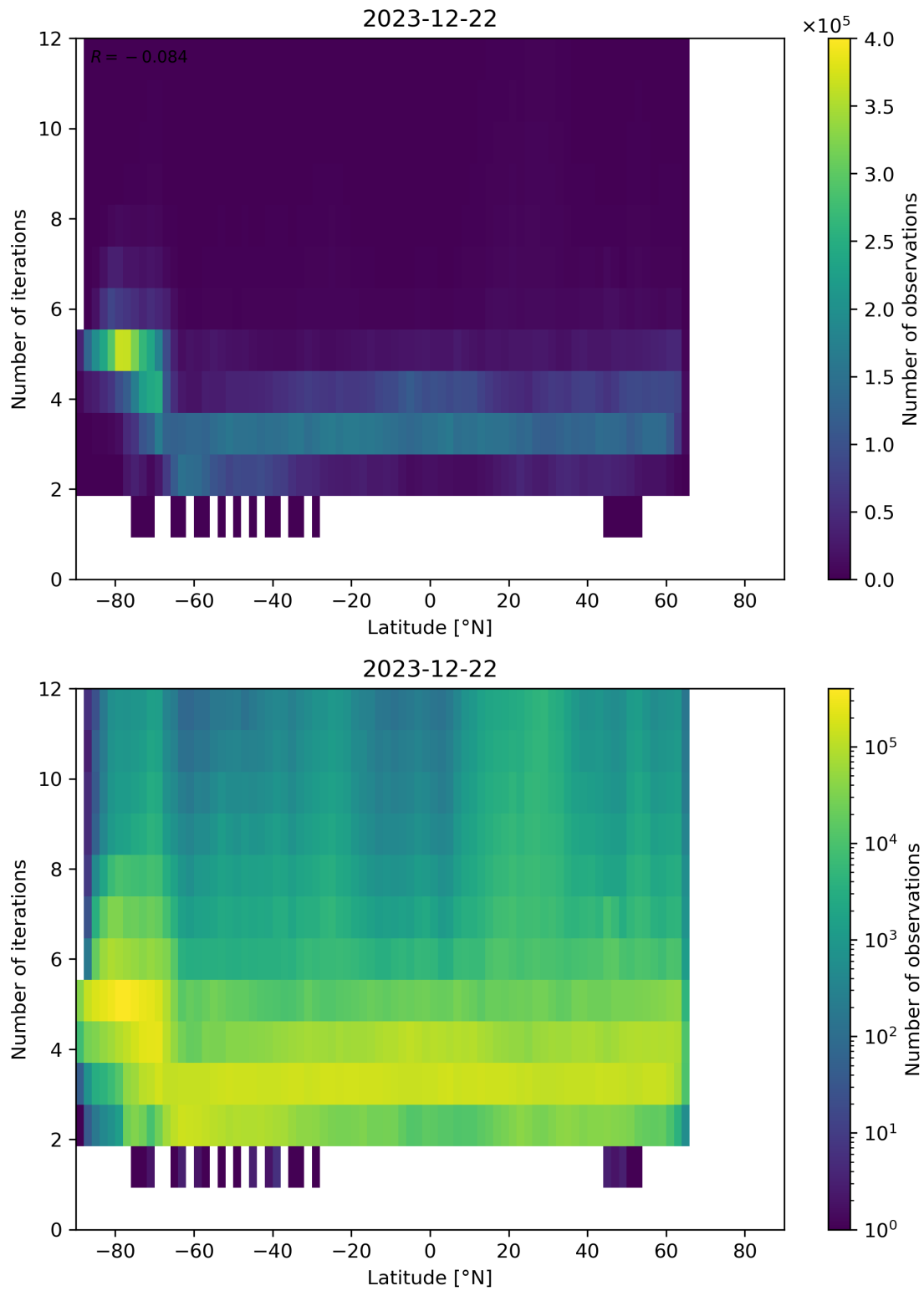
Figure 93: Scatter density plot of “Latitude” against “Number of iterations” for 2023-12-21 to 2023-12-23.
