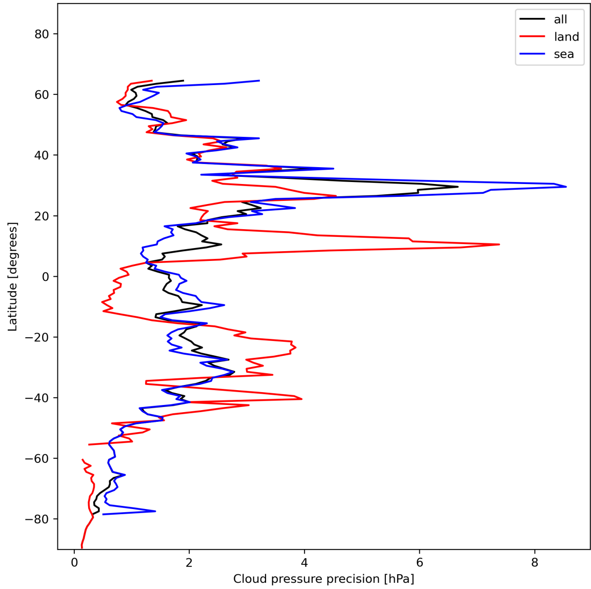
Figure 14: Zonal average of “Cloud pressure precision” for 2023-12-21 to 2023-12-23.
