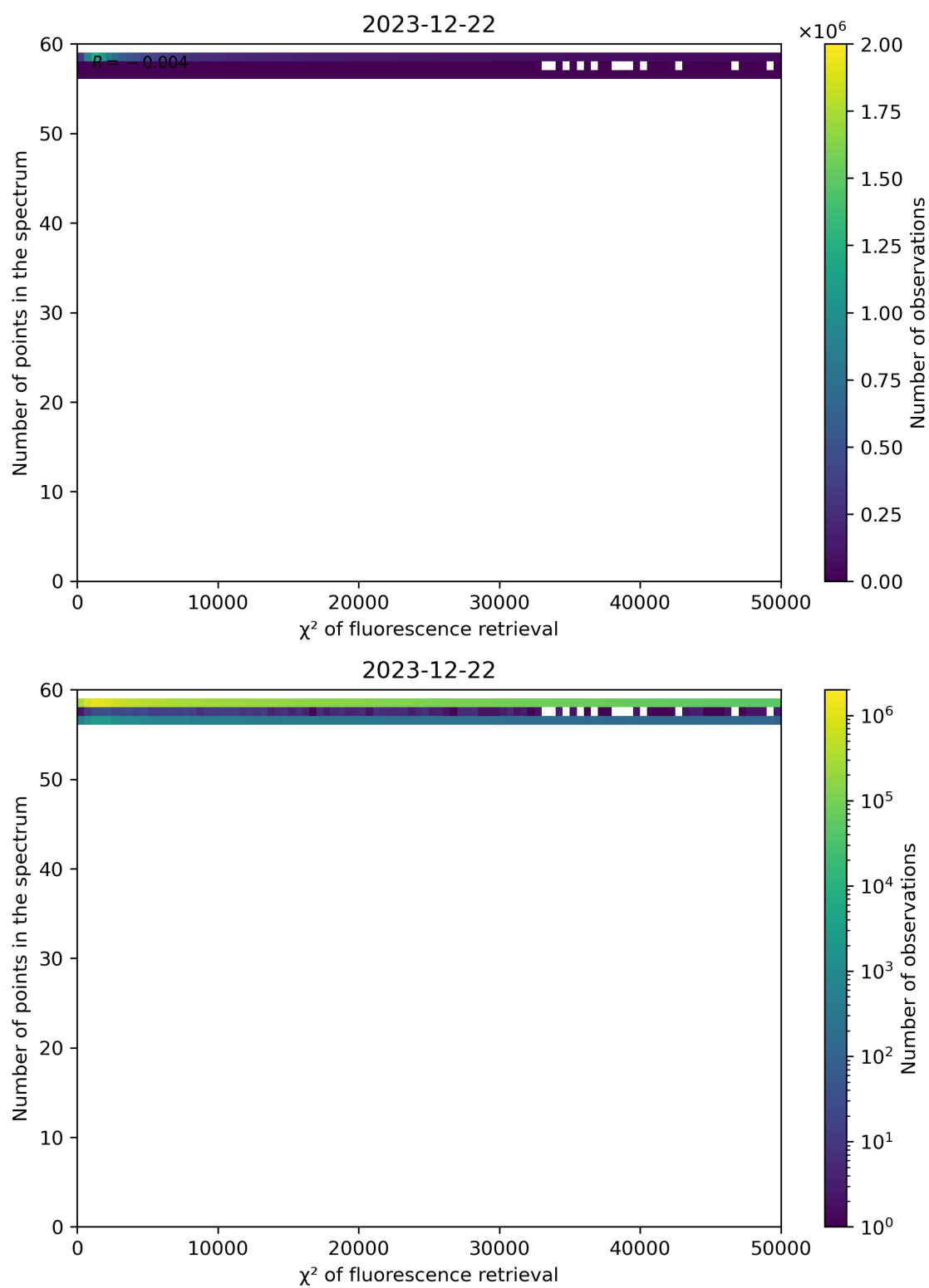
Figure 68: Scatter density plot of " \chi^2 of fluorescence retrieval" against "Number of points in the spectrum" for 2023-12-21 to 2023-12-23.
