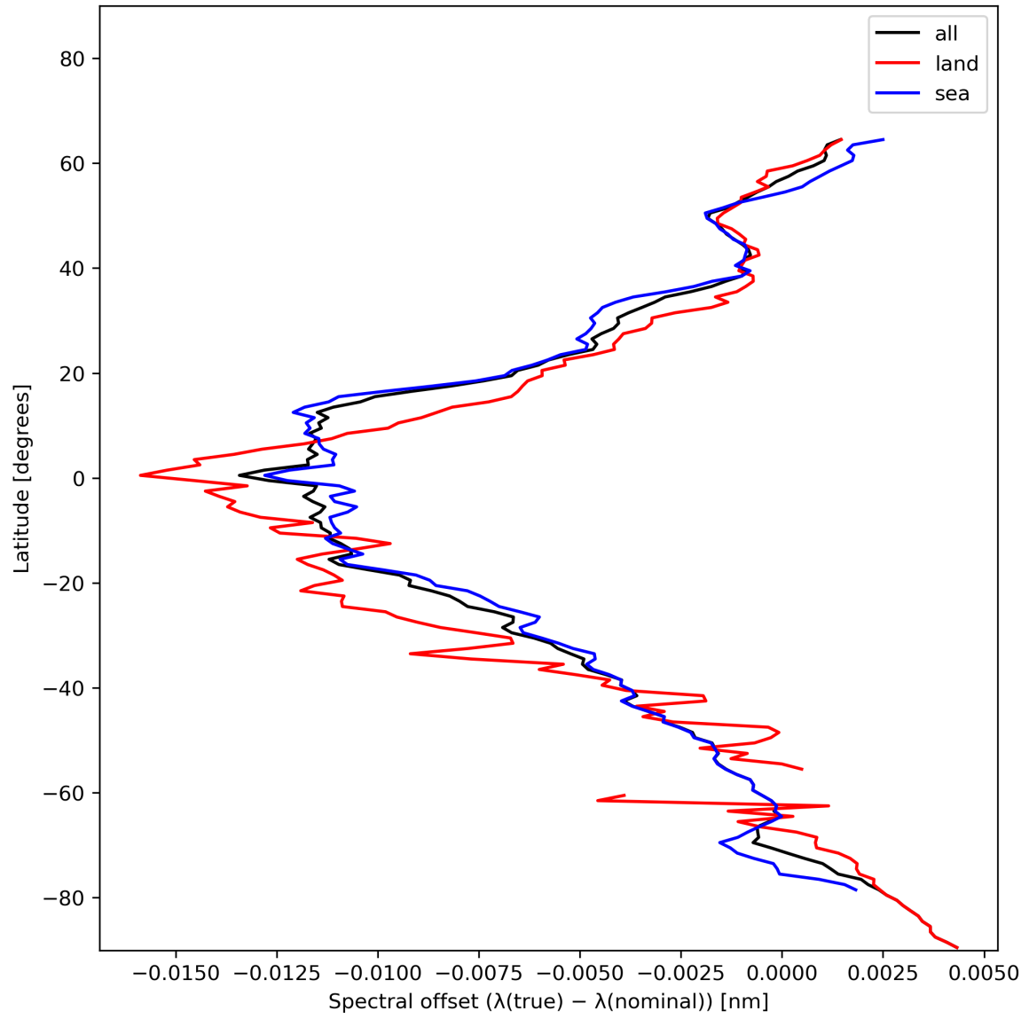
Figure 28: Zonal average of “Spectral offset ( \lambda(\text{true}) - \lambda(\text{nominal}) )” for 2023-12-21 to 2023-12-23.
