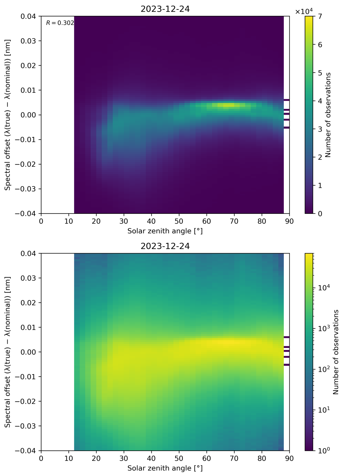
Figure 117: Scatter density plot of “Solar zenith angle” against “Spectral offset ( \lambda(\text{true}) - \lambda(\text{nominal}) )” for 2023-12-23 to 2023-12-25.
