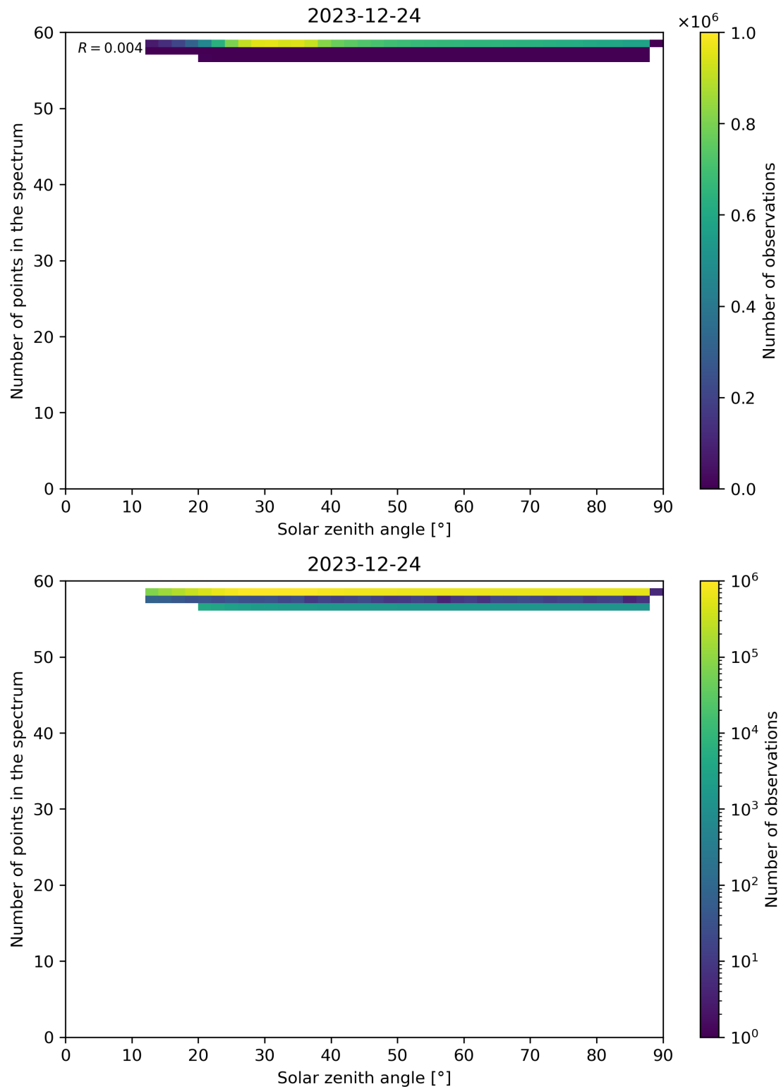
Figure 115: Scatter density plot of “Solar zenith angle” against “Number of points in the spectrum” for 2023-12-23 to 2023-12-25.
