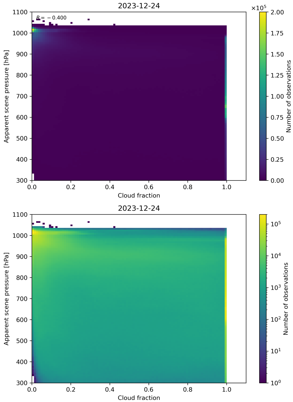
Figure 70: Scatter density plot of “Cloud fraction” against “Apparent scene pressure” for 2023-12-23 to 2023-12-25.
