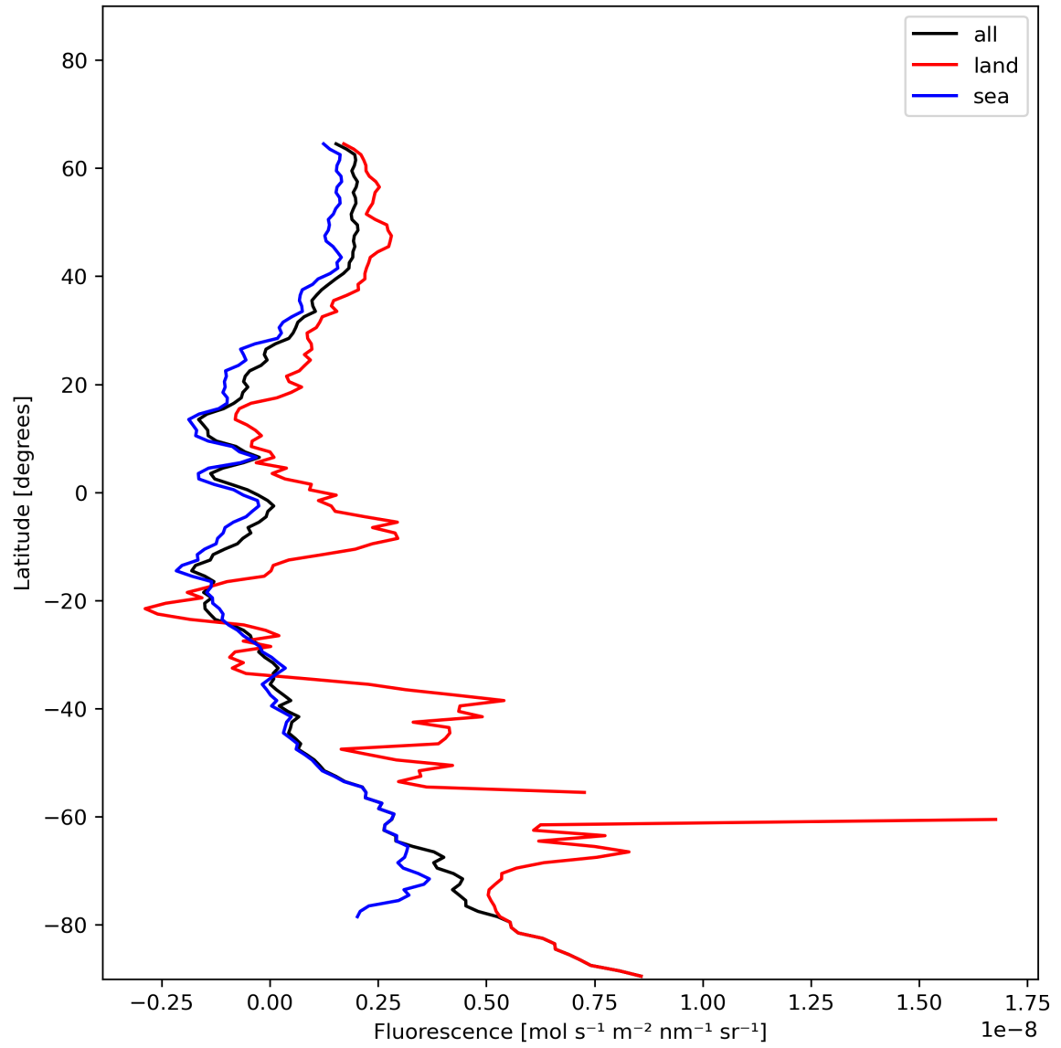
Figure 23: Zonal average of “Fluorescence” for 2023-12-23 to 2023-12-25.
