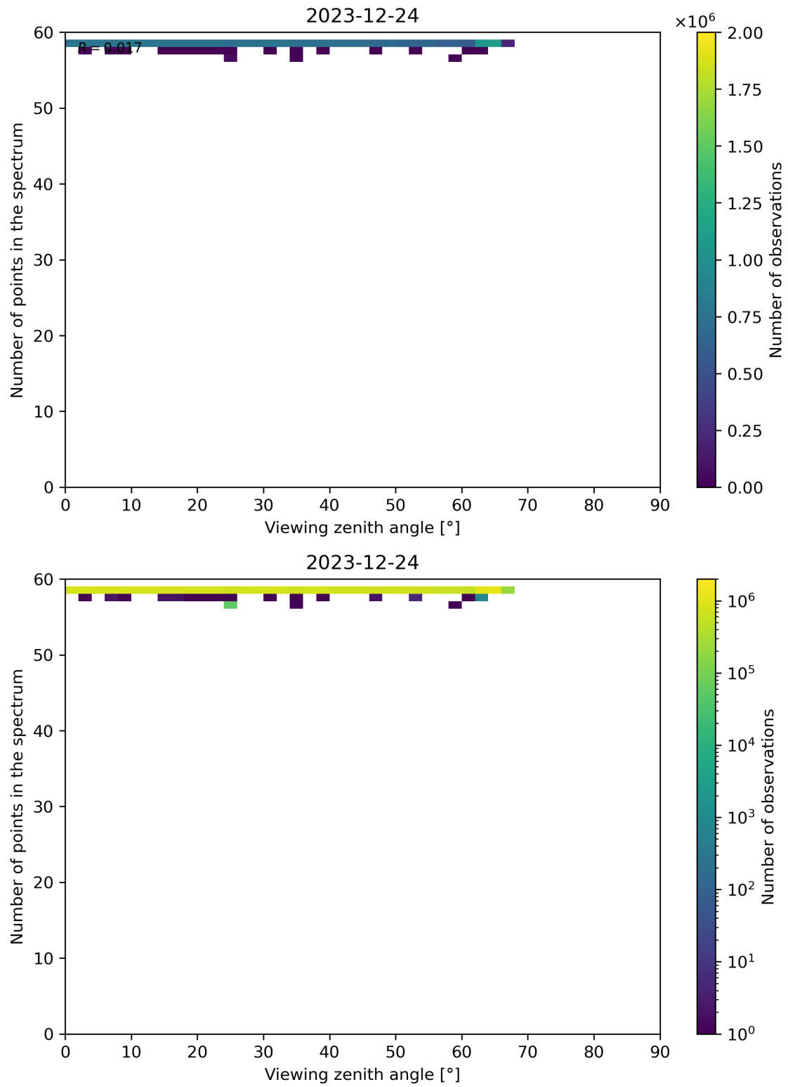
Figure 125: Scatter density plot of “Viewing zenith angle” against “Number of points in the spectrum” for 2023-12-23 to 2023-12-25.
