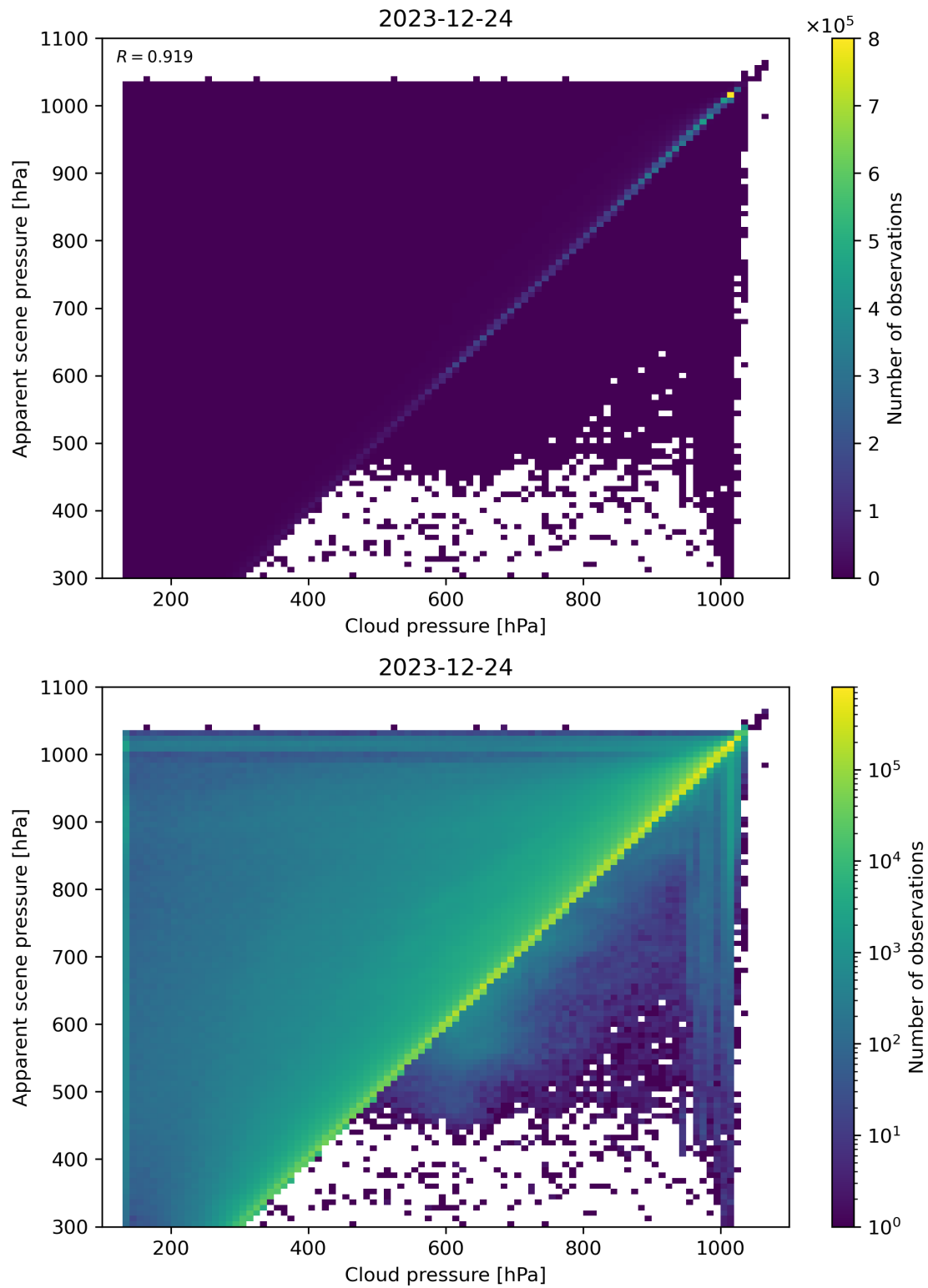
Figure 77: Scatter density plot of “Cloud pressure” against “Apparent scene pressure” for 2023-12-23 to 2023-12-25.
