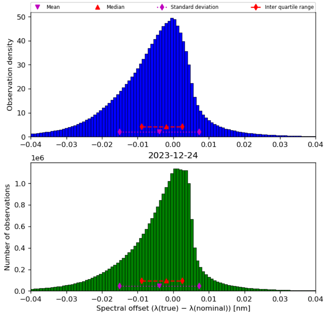
Figure 45: Histogram of “Spectral offset ( \lambda(\text{true}) - \lambda(\text{nominal}) )” for 2023-12-23 to 2023-12-25
