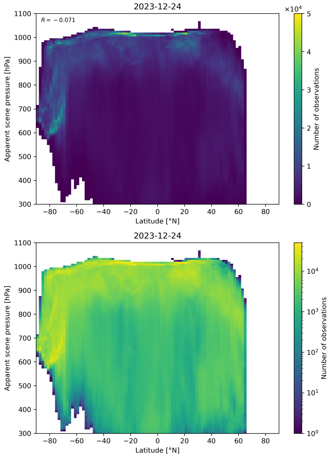
Figure 88: Scatter density plot of “Latitude” against “Apparent scene pressure” for 2023-12-23 to 2023-12-25.
