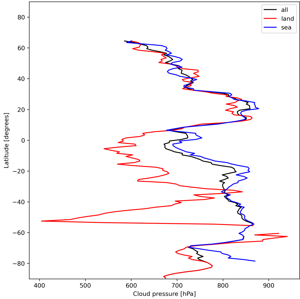
Figure 13: Zonal average of “Cloud pressure” for 2023-12-23 to 2023-12-25.
