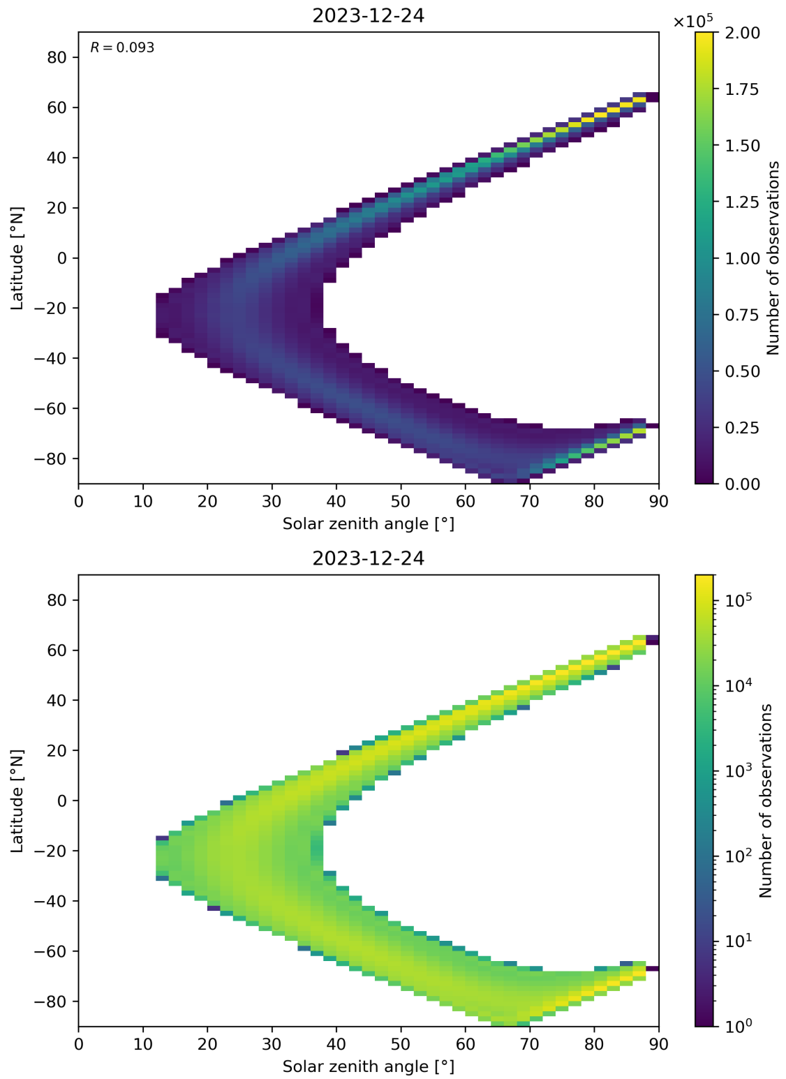
Figure 113: Scatter density plot of “Solar zenith angle” against “Latitude” for 2023-12-23 to 2023-12-25.
