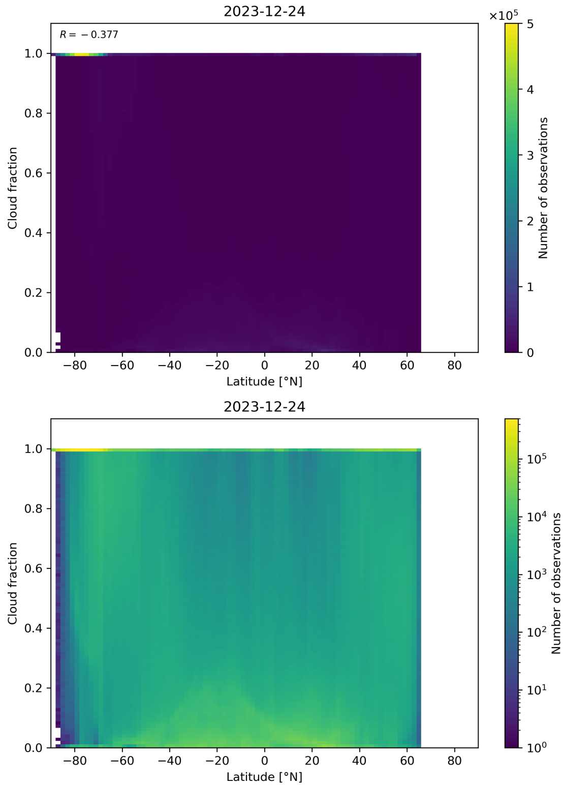
Figure 90: Scatter density plot of “Latitude” against “Cloud fraction” for 2023-12-23 to 2023-12-25.
