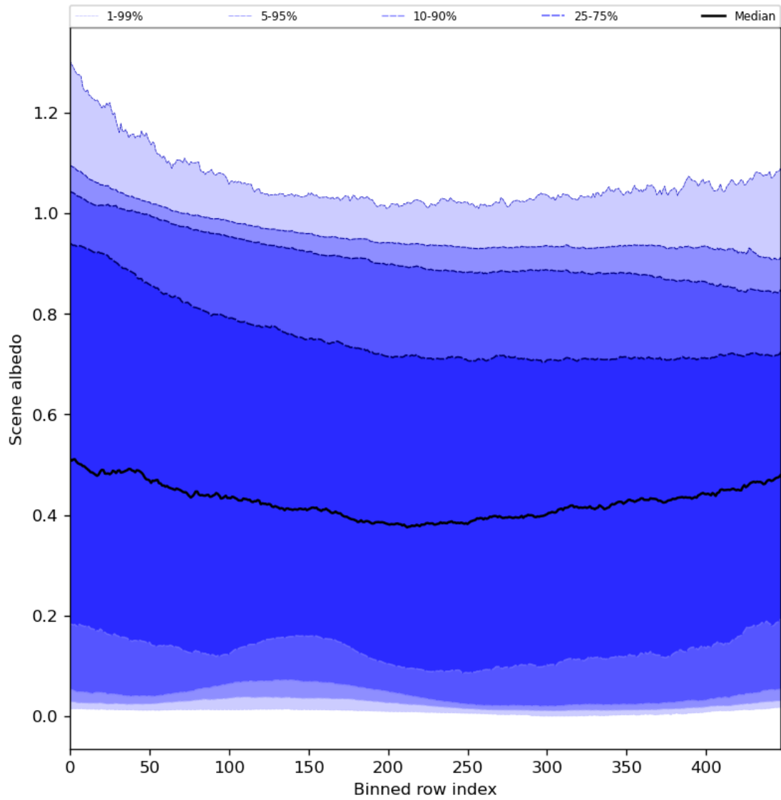
Figure 51: Along track statistics of “Scene albedo” for 2023-12-23 to 2023-12-25
