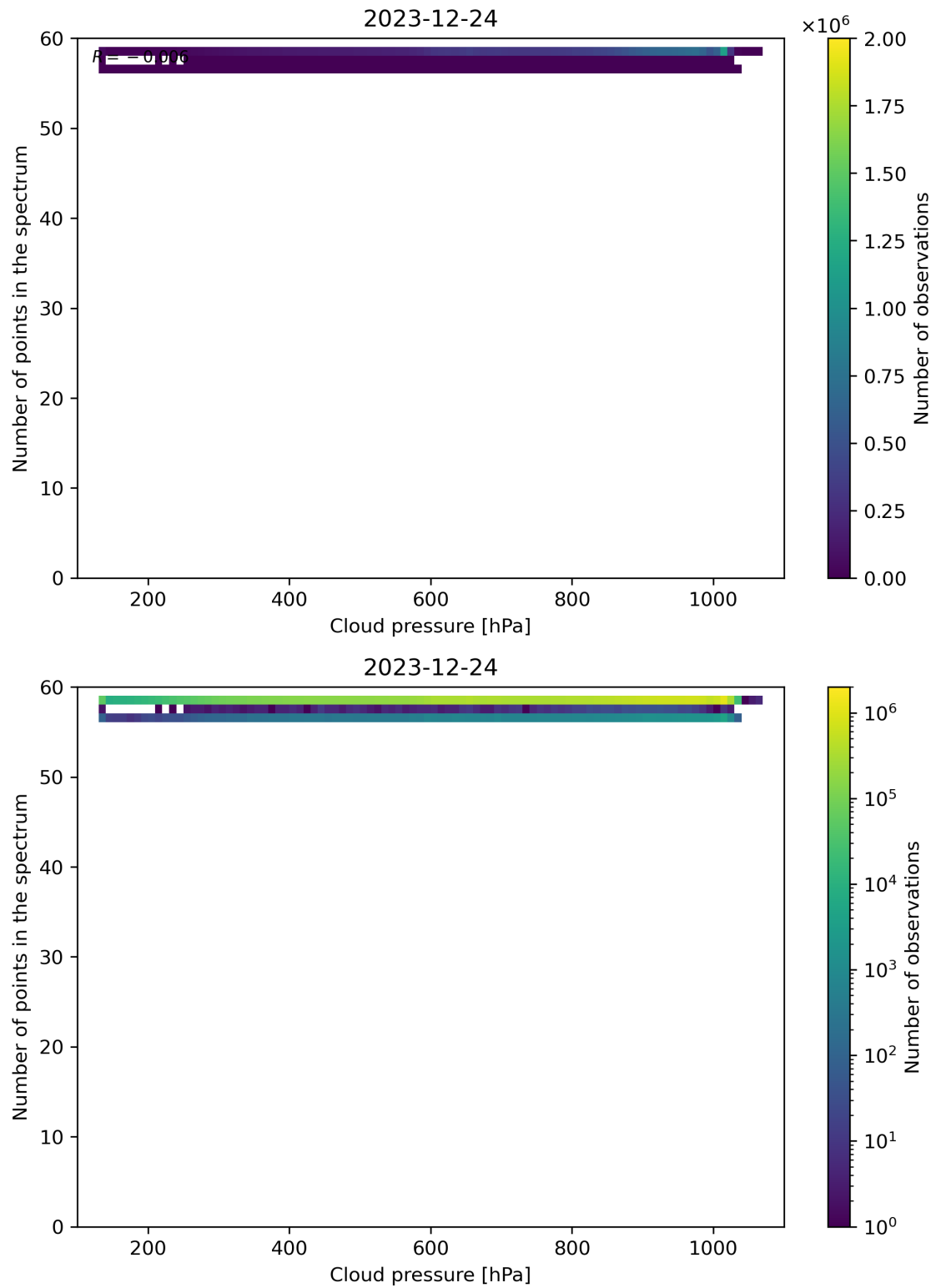
Figure 82: Scatter density plot of “Cloud pressure” against “Number of points in the spectrum” for 2023-12-23 to 2023-12-25.
