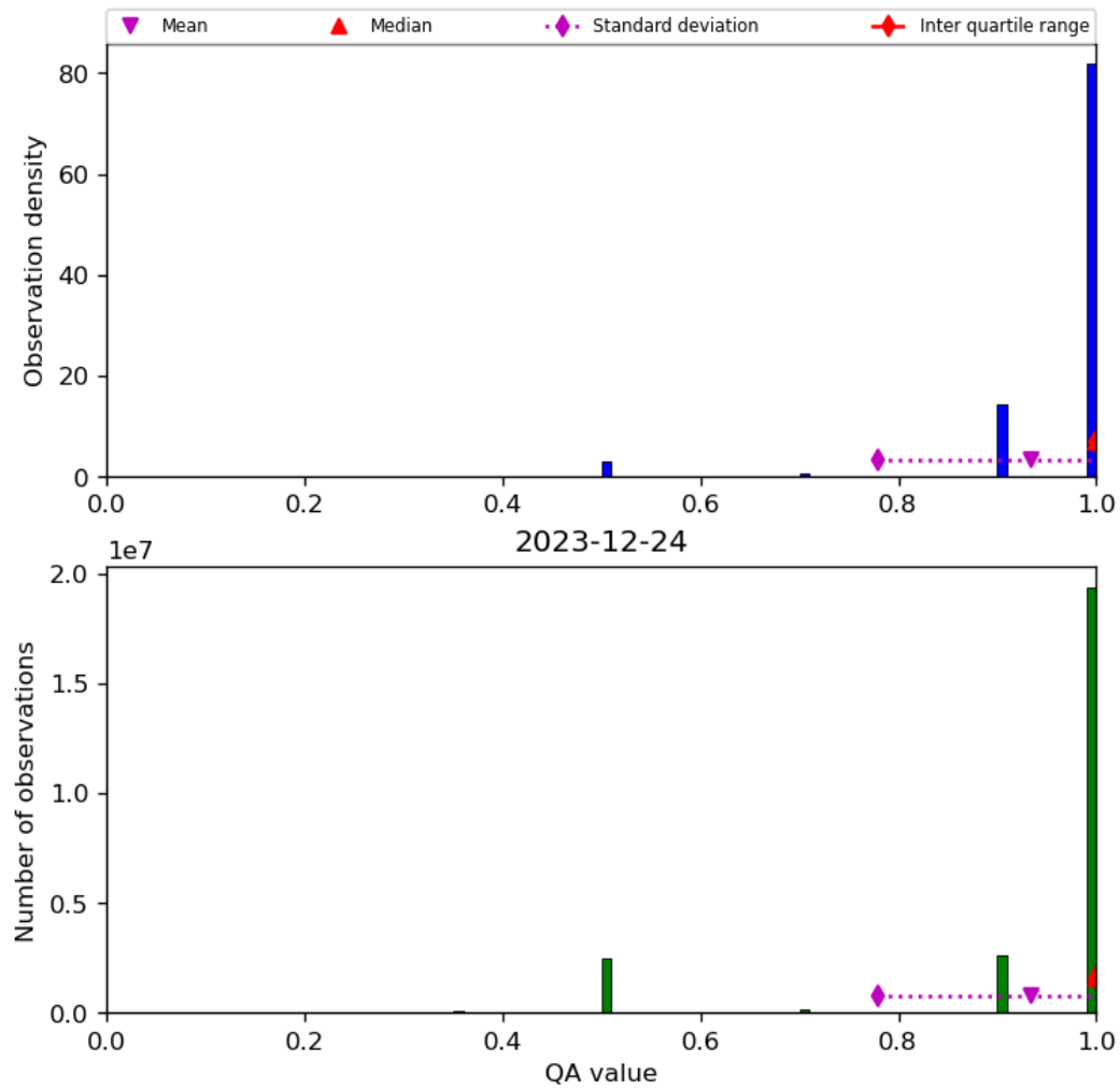
Figure 29: Histogram of “QA value” for 2023-12-23 to 2023-12-25
