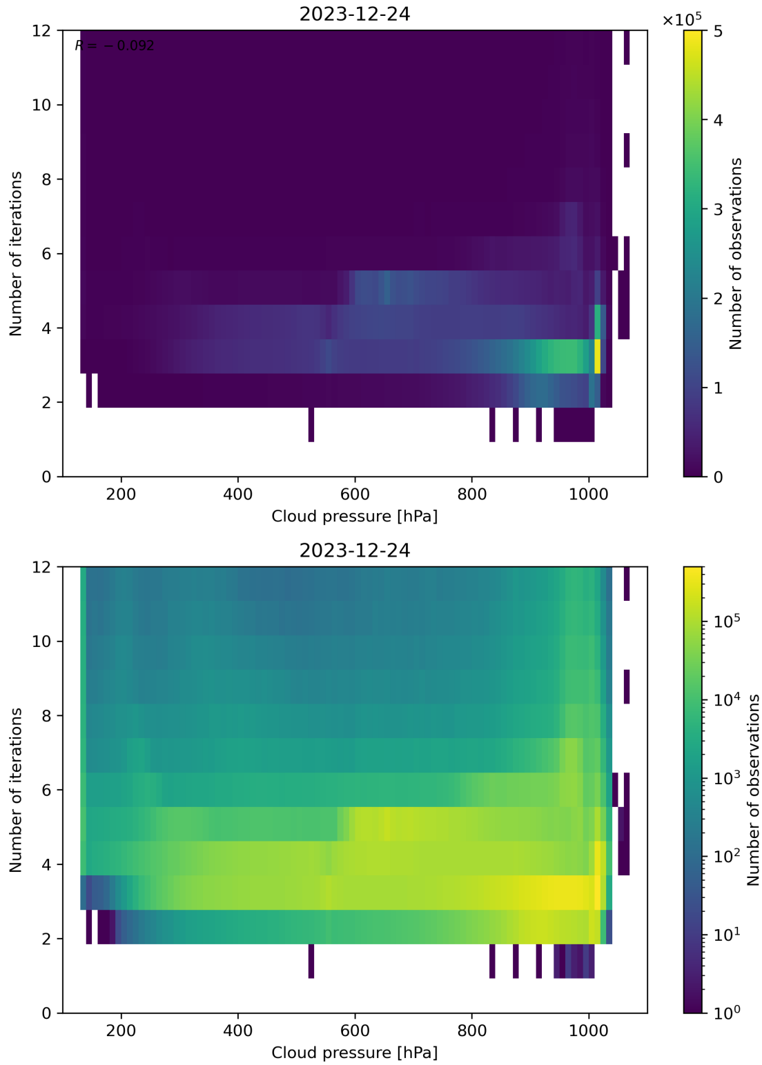
Figure 81: Scatter density plot of “Cloud pressure” against “Number of iterations” for 2023-12-23 to 2023-12-25.
