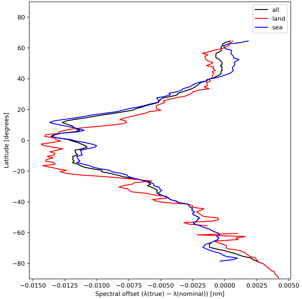
Figure 28: Zonal average of “Spectral offset ( \lambda(\text{true}) - \lambda(\text{nominal}) )” for 2023-12-23 to 2023-12-25.
