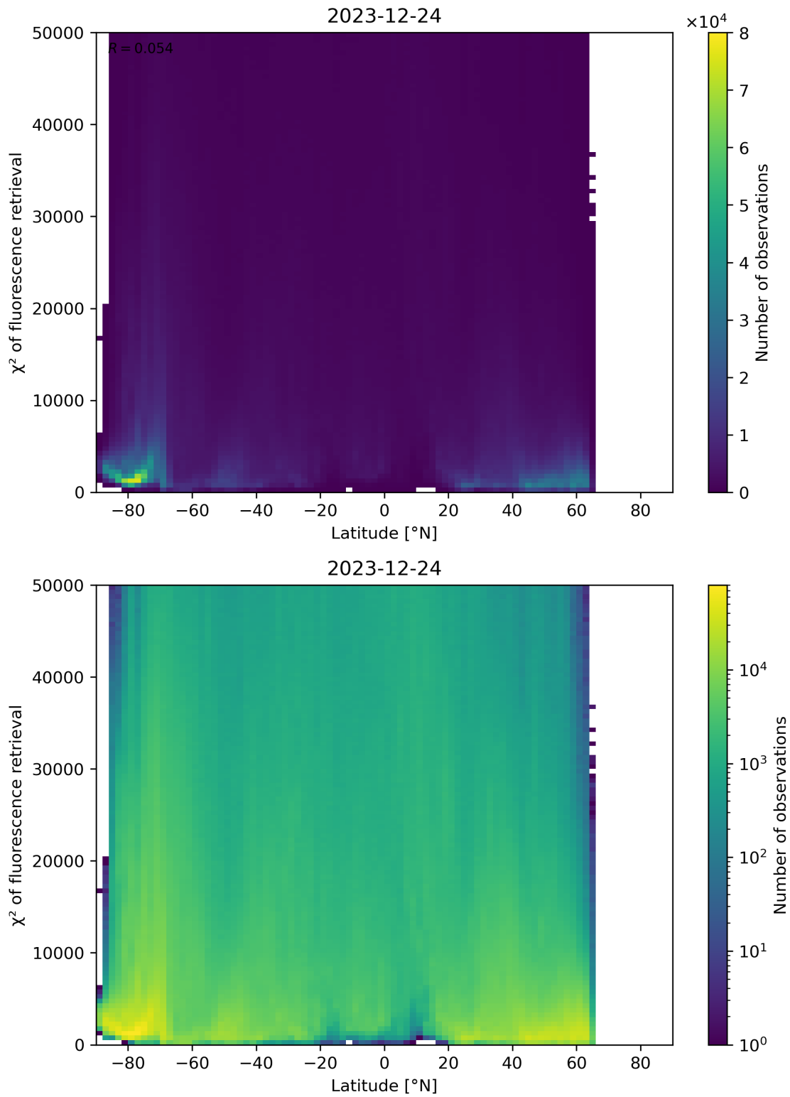
Figure 89: Scatter density plot of “Latitude” against “ \chi^2 of fluorescence retrieval” for 2023-12-23 to 2023-12-25.
