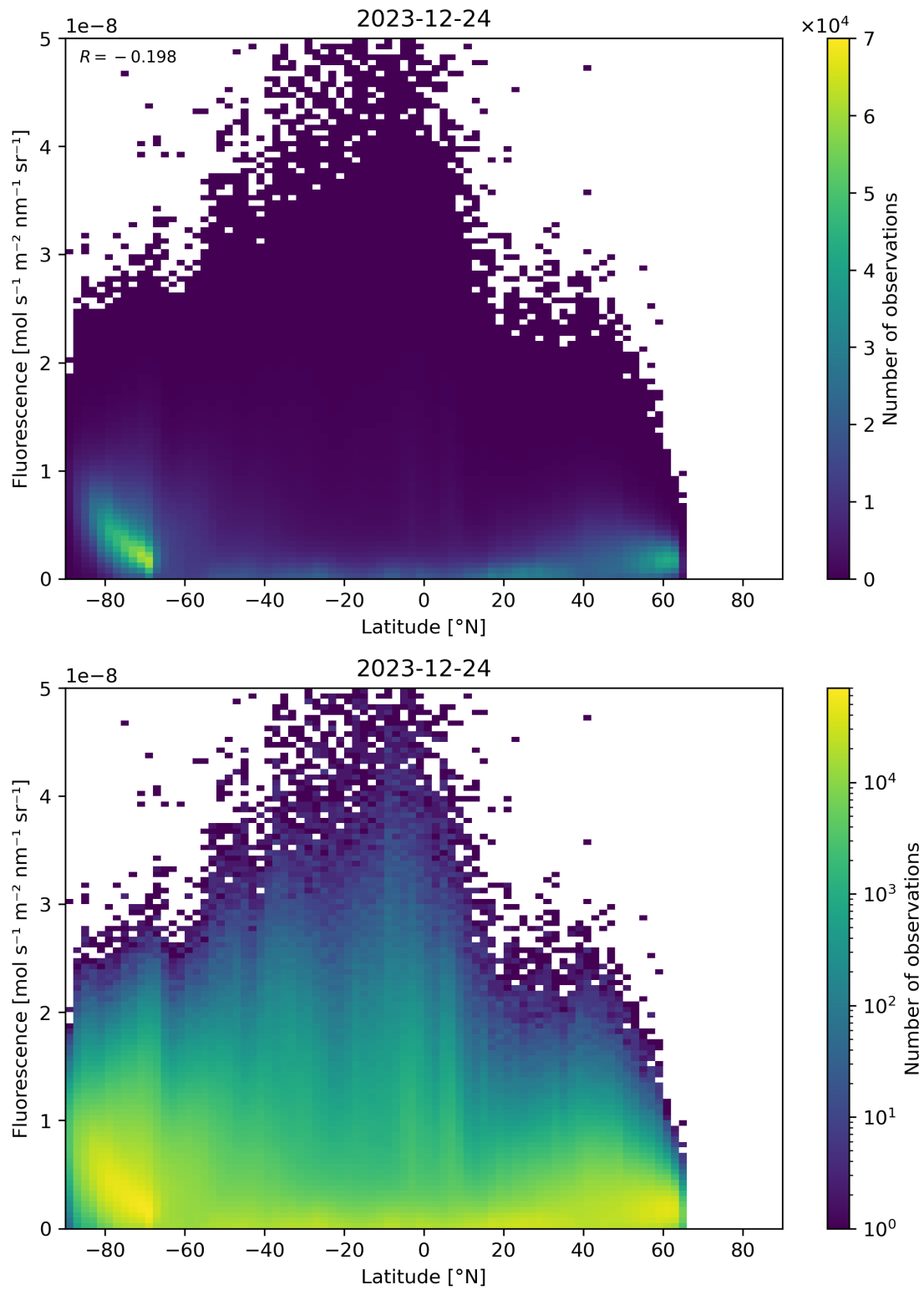
Figure 92: Scatter density plot of “Latitude” against “Fluorescence” for 2023-12-23 to 2023-12-25.
