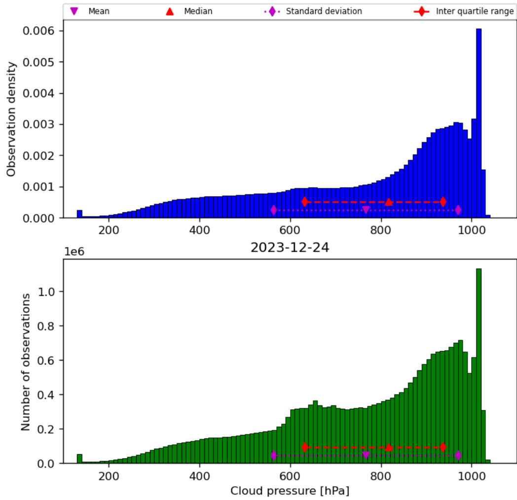
Figure 30: Histogram of “Cloud pressure” for 2023-12-23 to 2023-12-25
