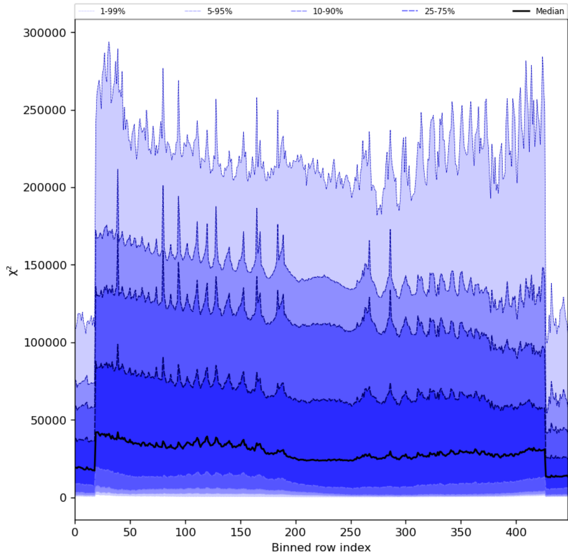
Figure 55: Along track statistics of “ \chi^2 ” for 2023-12-23 to 2023-12-25
