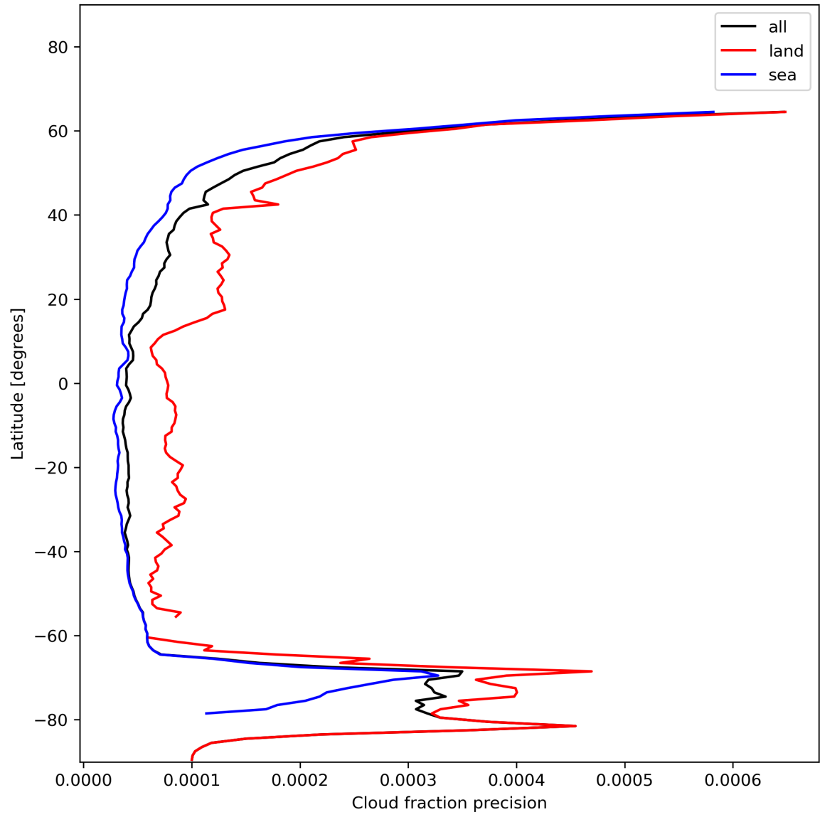
Figure 16: Zonal average of “Cloud fraction precision” for 2023-12-23 to 2023-12-25.
