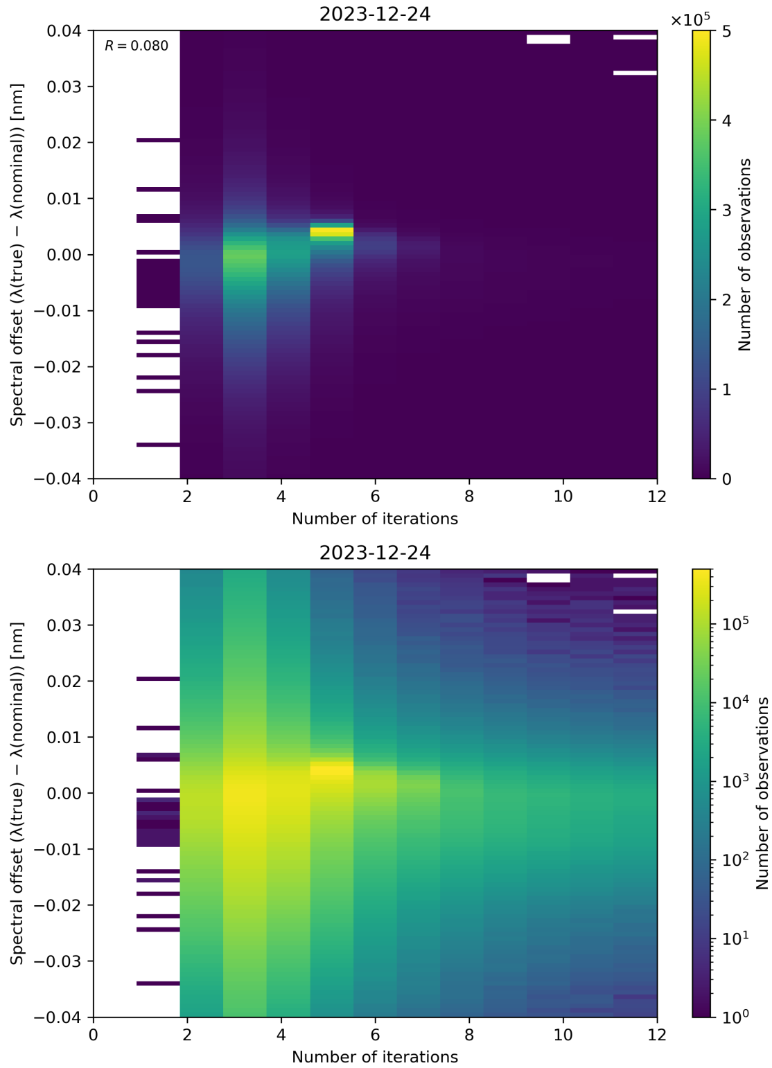
Figure 100: Scatter density plot of “Number of iterations” against “Spectral offset ( \lambda(\text{true}) - \lambda(\text{nominal}) )” for 2023-12-23 to 2023-12-25.
