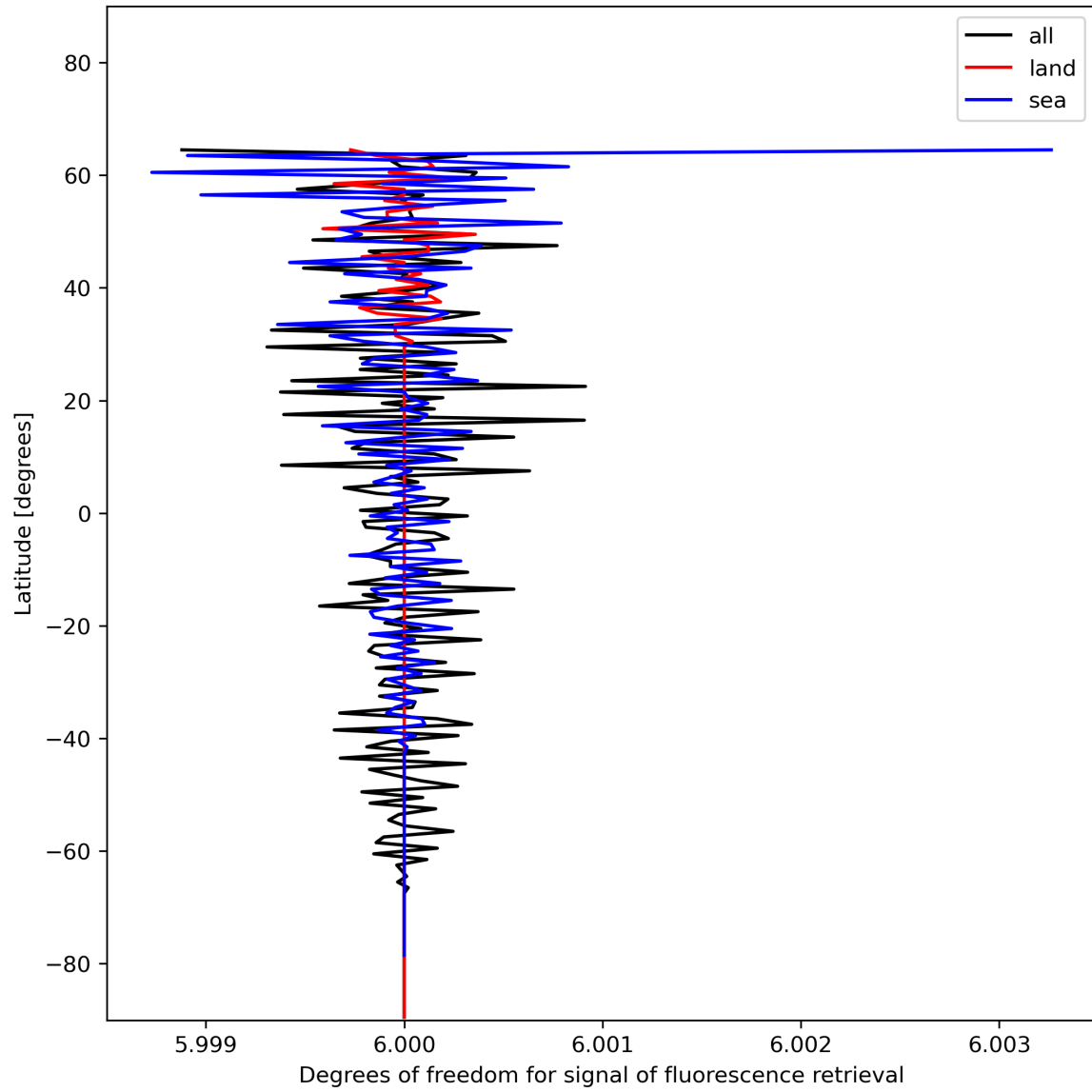
Figure 26: Zonal average of “Degrees of freedom for signal of fluorescence retrieval” for 2023-12-23 to 2023-12-25.
