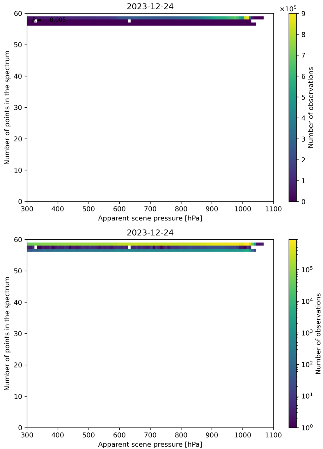
Figure 66: Scatter density plot of “Apparent scene pressure” against “Number of points in the spectrum” for 2023-12-23 to 2023-12-25.
