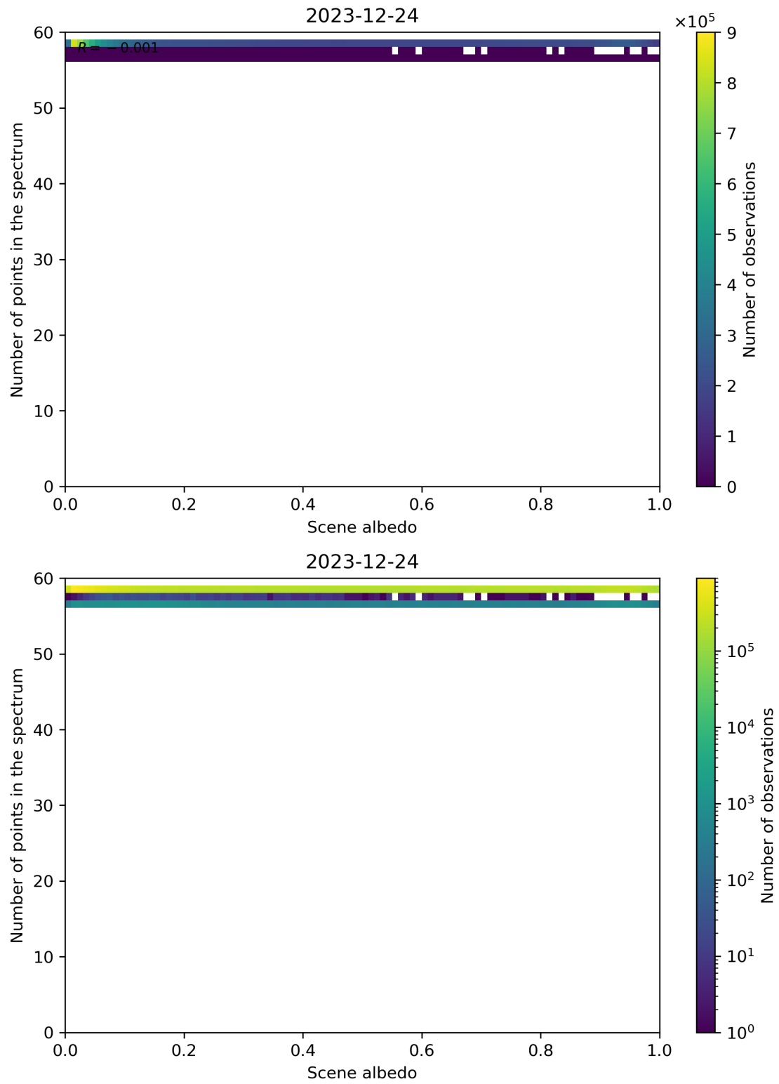
Figure 106: Scatter density plot of “Scene albedo” against “Number of points in the spectrum” for 2023-12-23 to 2023-12-25.
