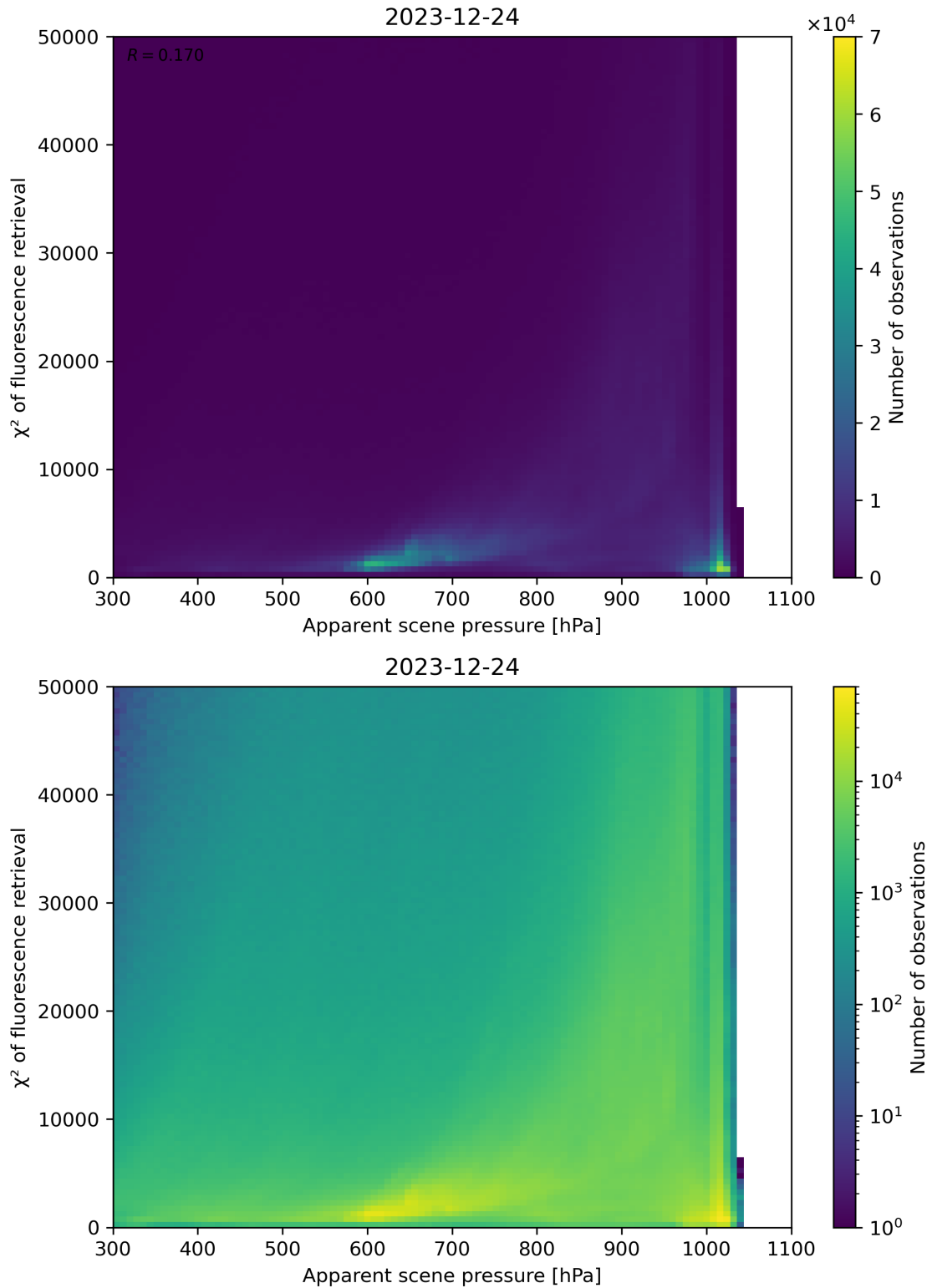
Figure 63: Scatter density plot of “Apparent scene pressure” against “ \chi^2 of fluorescence retrieval” for 2023-12-23 to 2023-12-25.
