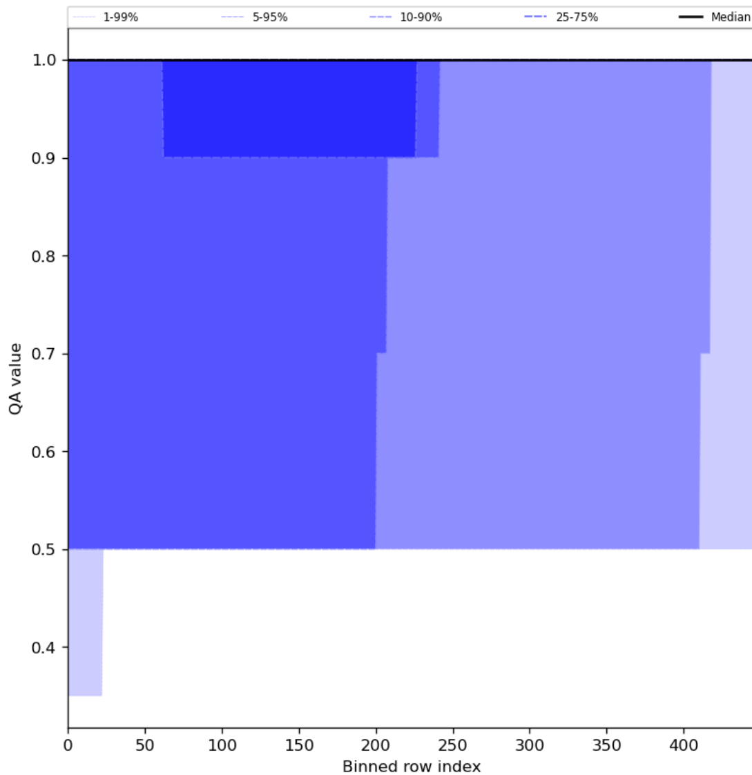
Figure 46: Along track statistics of “QA value” for 2023-12-23 to 2023-12-25
