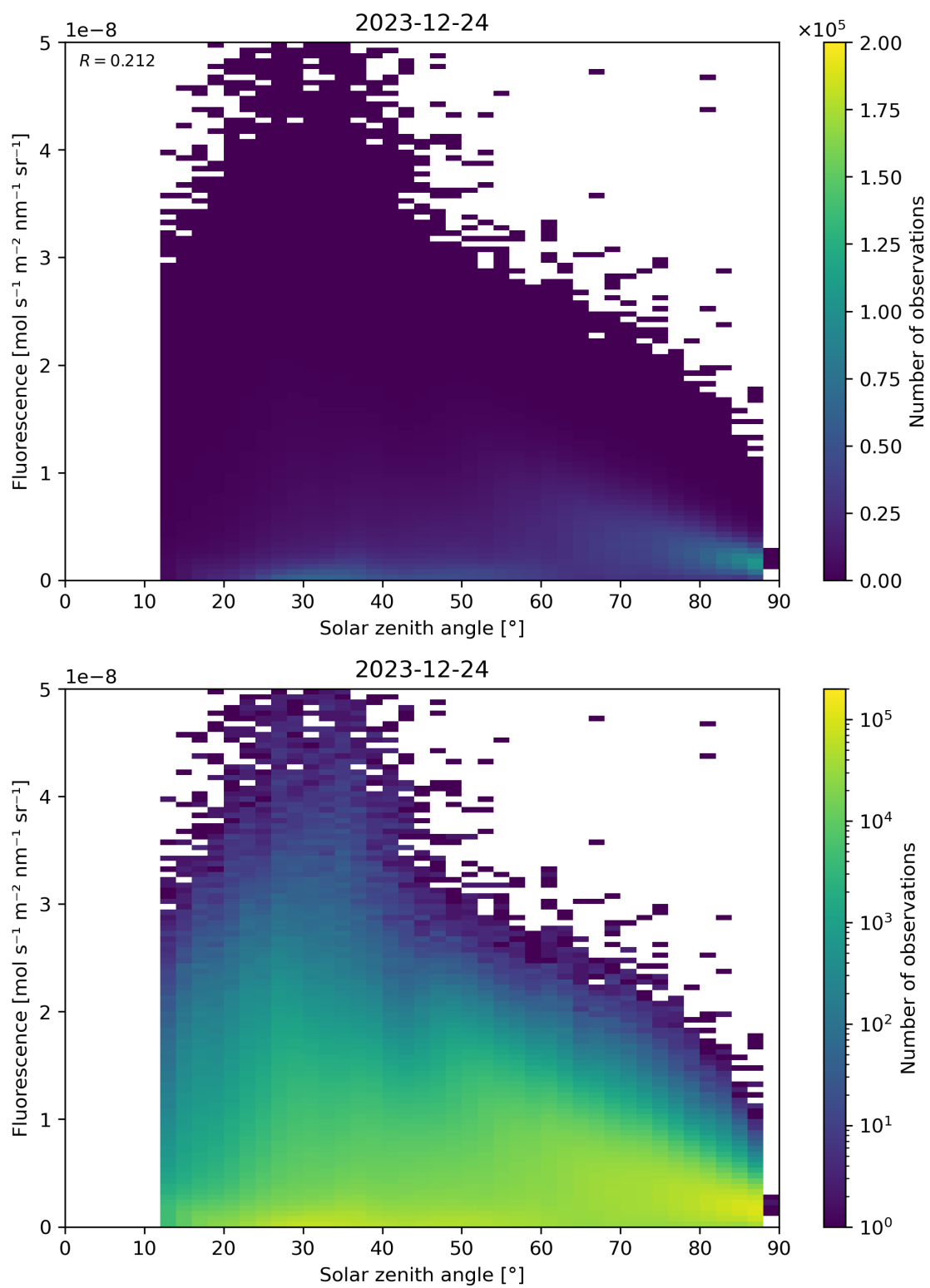
Figure 112: Scatter density plot of “Solar zenith angle” against “Fluorescence” for 2023-12-23 to 2023-12-25.
