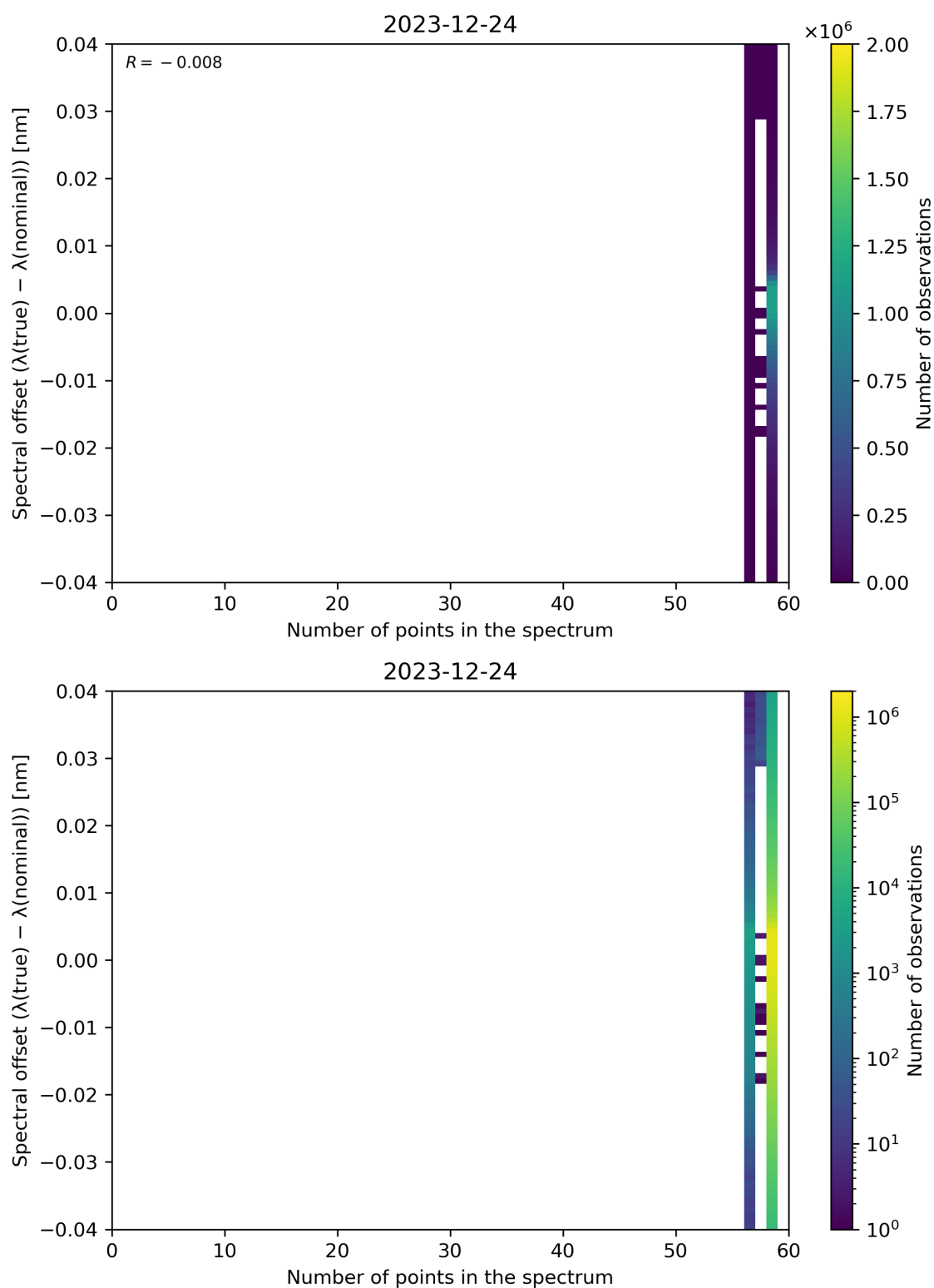
Figure 101: Scatter density plot of “Number of points in the spectrum” against “Spectral offset ( \lambda(\text{true}) - \lambda(\text{nominal}) )” for 2023-12-23 to 2023-12-25.
