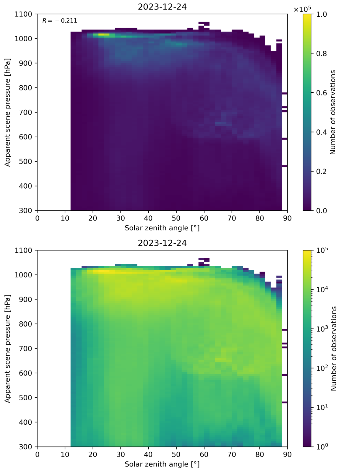
Figure 108: Scatter density plot of “Solar zenith angle” against “Apparent scene pressure” for 2023-12-23 to 2023-12-25.
