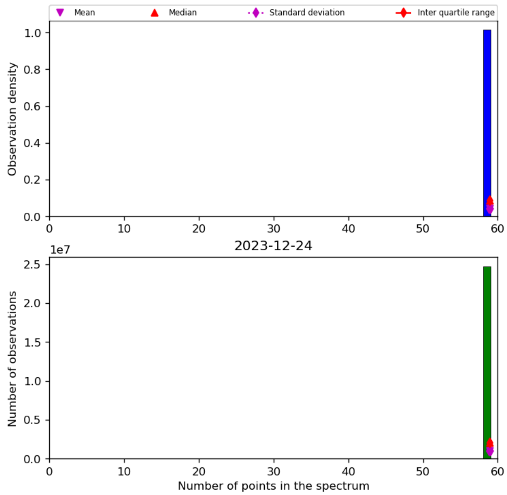
Figure 44: Histogram of “Number of points in the spectrum” for 2023-12-23 to 2023-12-25
