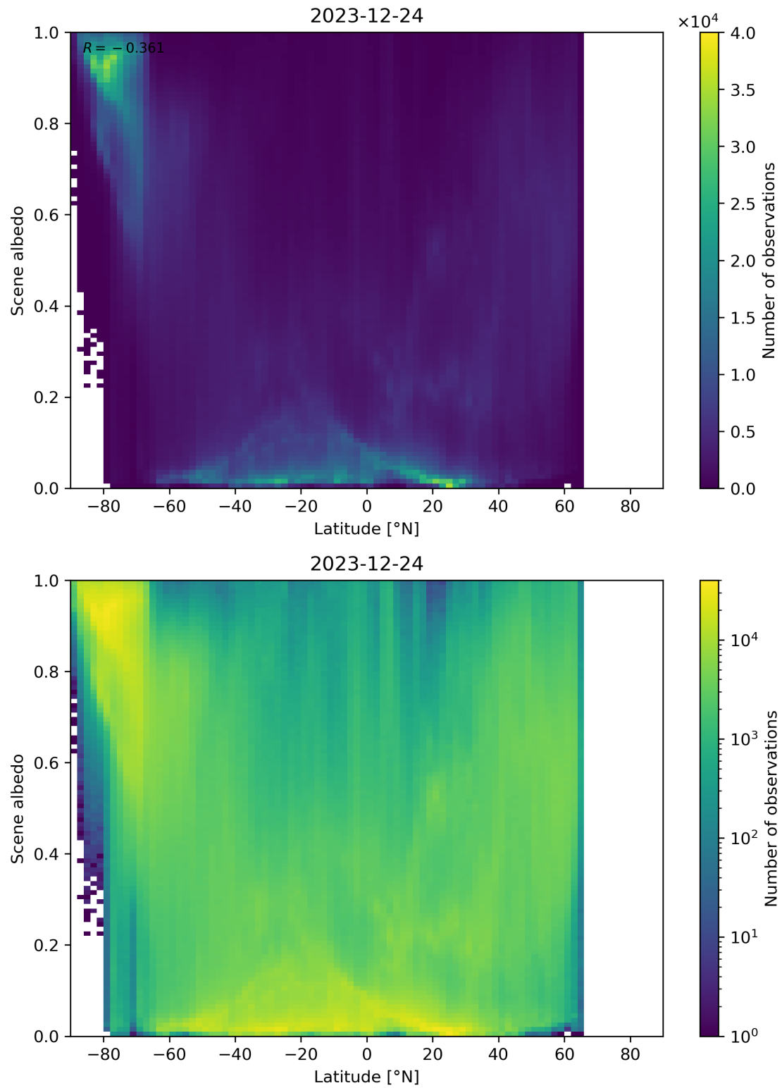
Figure 95: Scatter density plot of “Latitude” against “Scene albedo” for 2023-12-23 to 2023-12-25.
