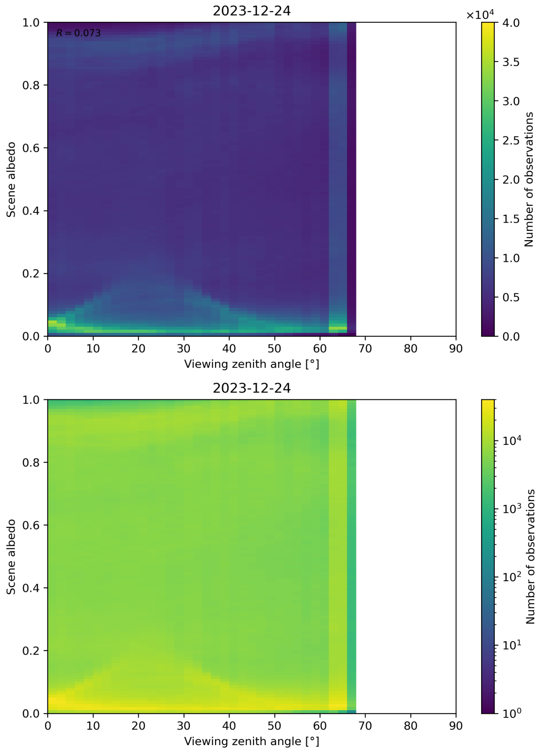
Figure 126: Scatter density plot of “Viewing zenith angle” against “Scene albedo” for 2023-12-23 to 2023-12-25.
