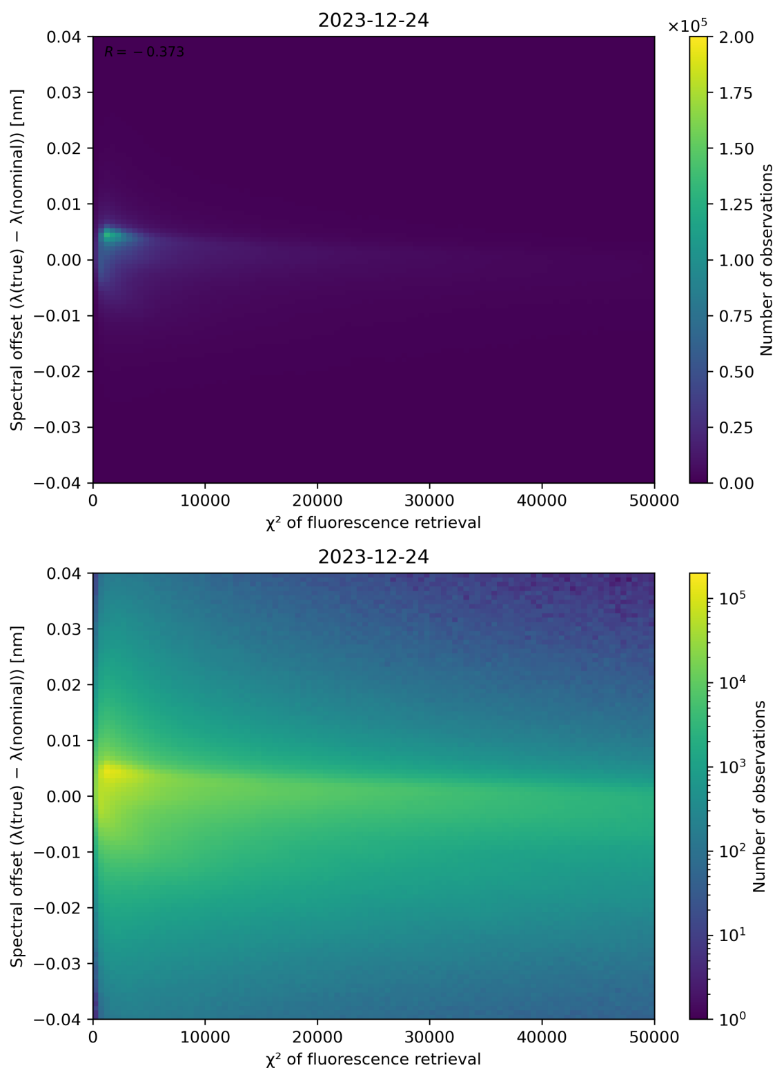
Figure 69: Scatter density plot of " \chi^2 of fluorescence retrieval" against "Spectral offset ( \lambda(\text{true}) - \lambda(\text{nominal}) )" for 2023-12-23 to 2023-12-25.
