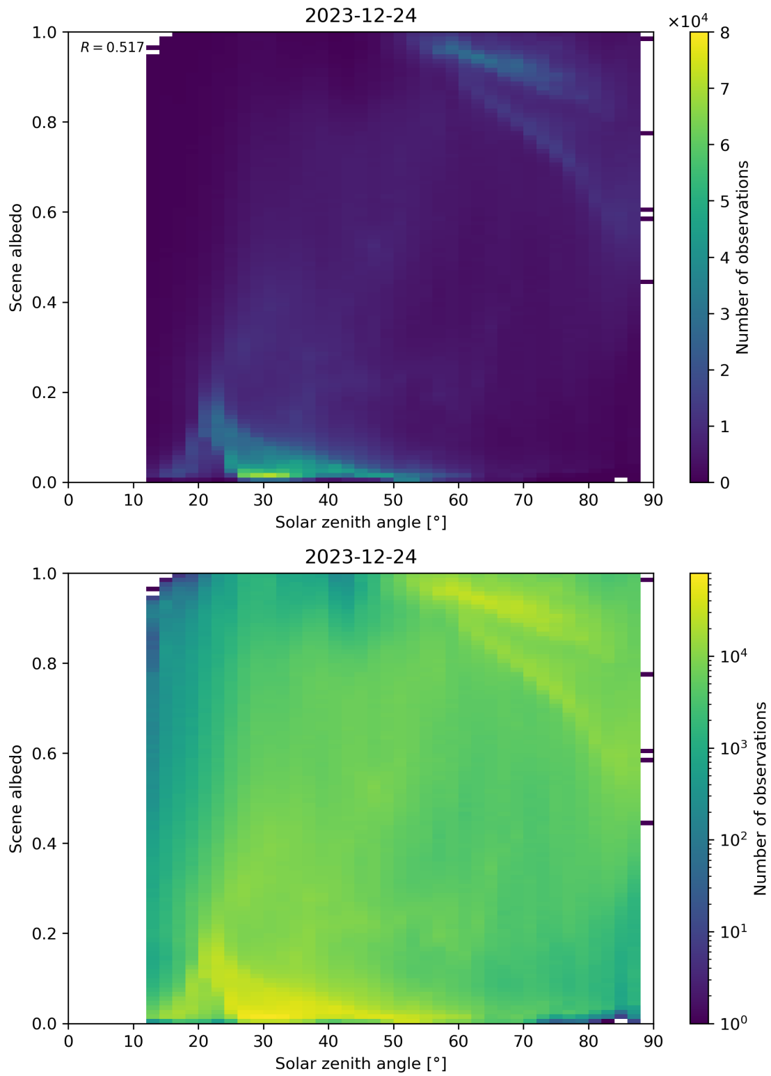
Figure 116: Scatter density plot of “Solar zenith angle” against “Scene albedo” for 2023-12-23 to 2023-12-25.
