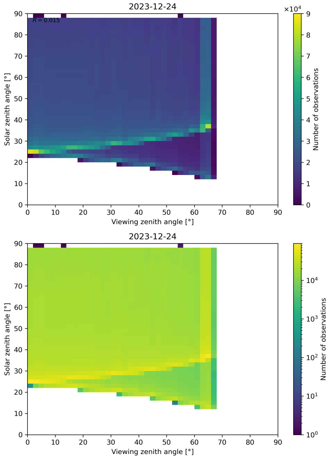
Figure 127: Scatter density plot of “Viewing zenith angle” against “Solar zenith angle” for 2023-12-23 to 2023-12-25.
