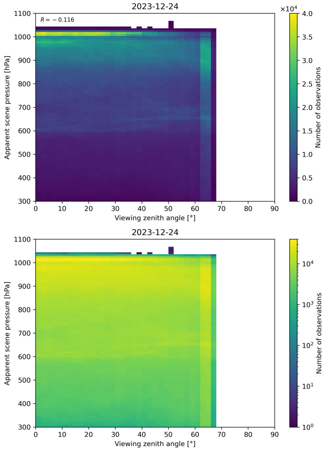
Figure 118: Scatter density plot of “Viewing zenith angle” against “Apparent scene pressure” for 2023-12-23 to 2023-12-25.
