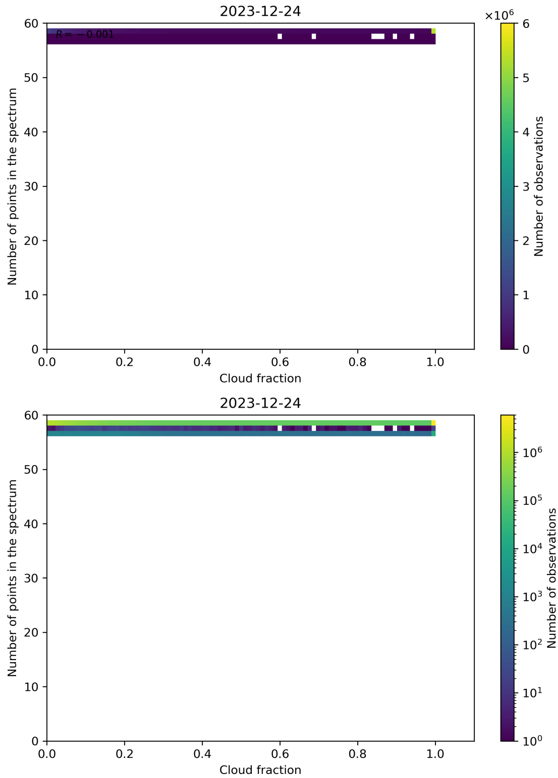
Figure 74: Scatter density plot of “Cloud fraction” against “Number of points in the spectrum” for 2023-12-23 to 2023-12-25.
