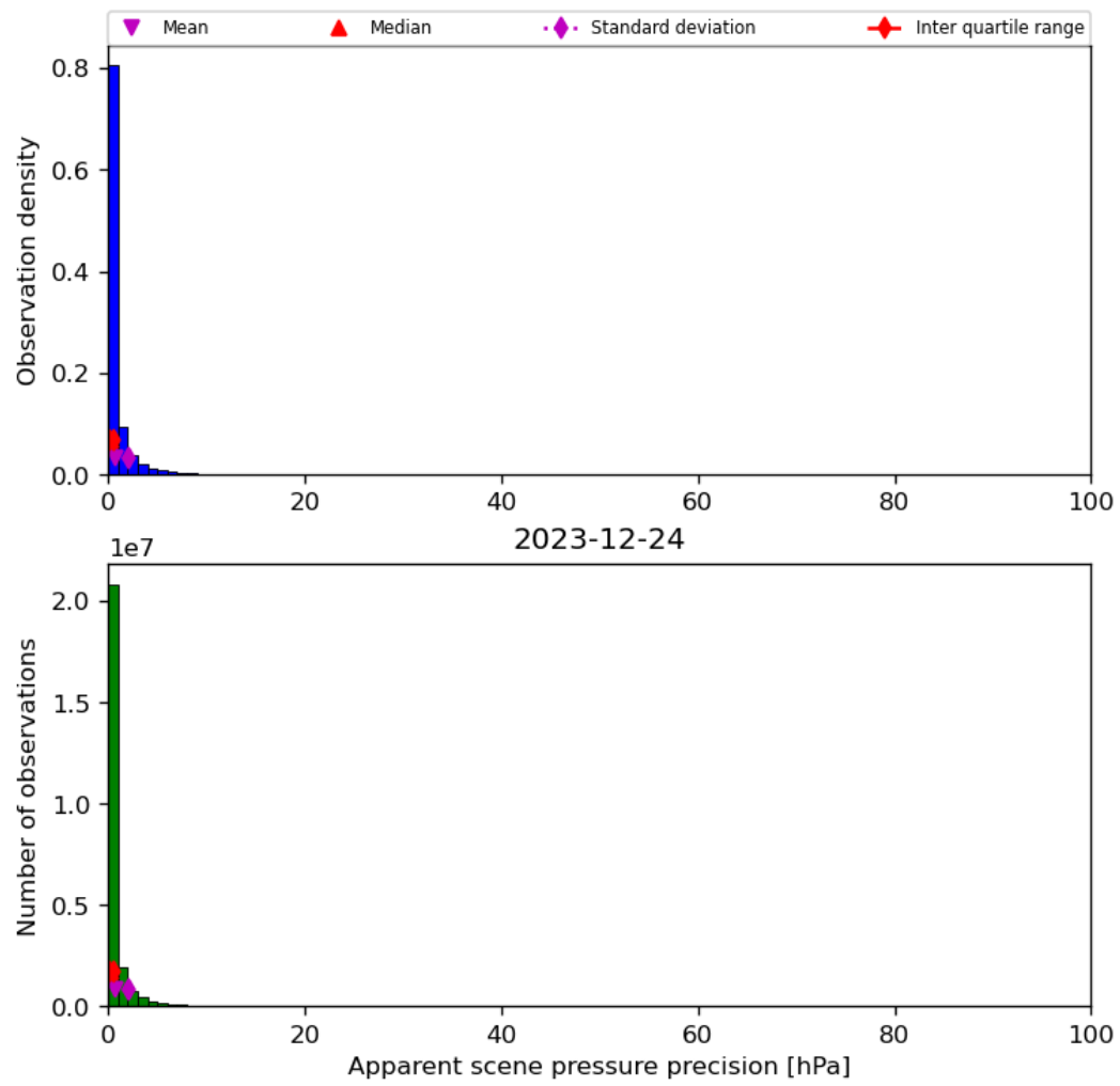
Figure 37: Histogram of “Apparent scene pressure precision” for 2023-12-23 to 2023-12-25
