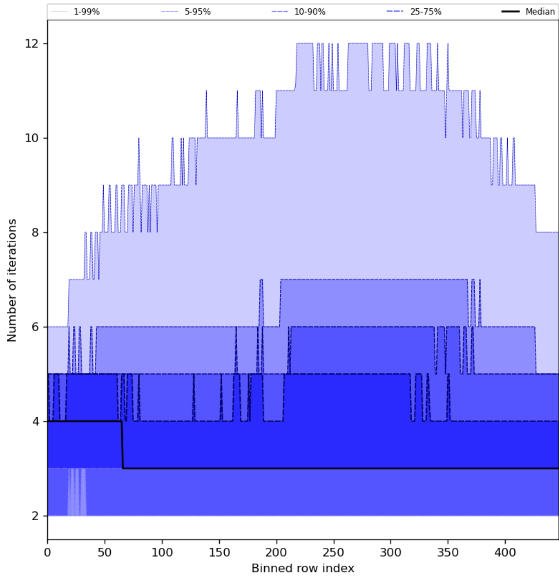
Figure 56: Along track statistics of “Number of iterations” for 2023-12-23 to 2023-12-25
