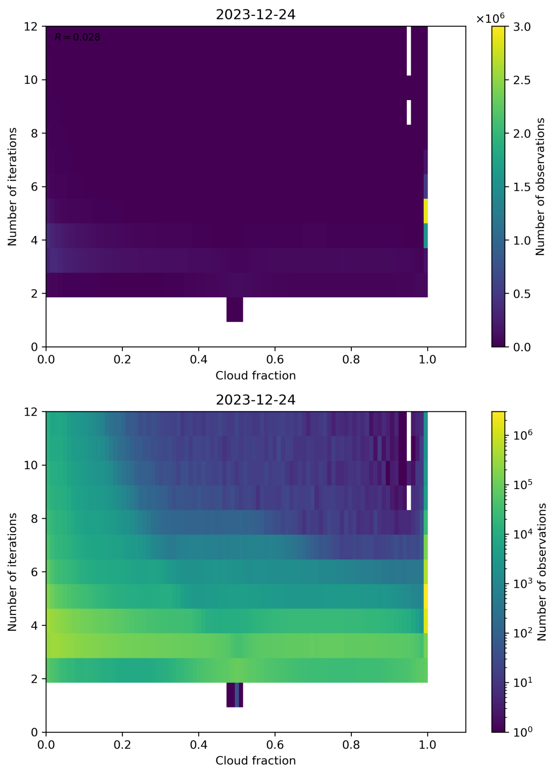
Figure 73: Scatter density plot of “Cloud fraction” against “Number of iterations” for 2023-12-23 to 2023-12-25.
