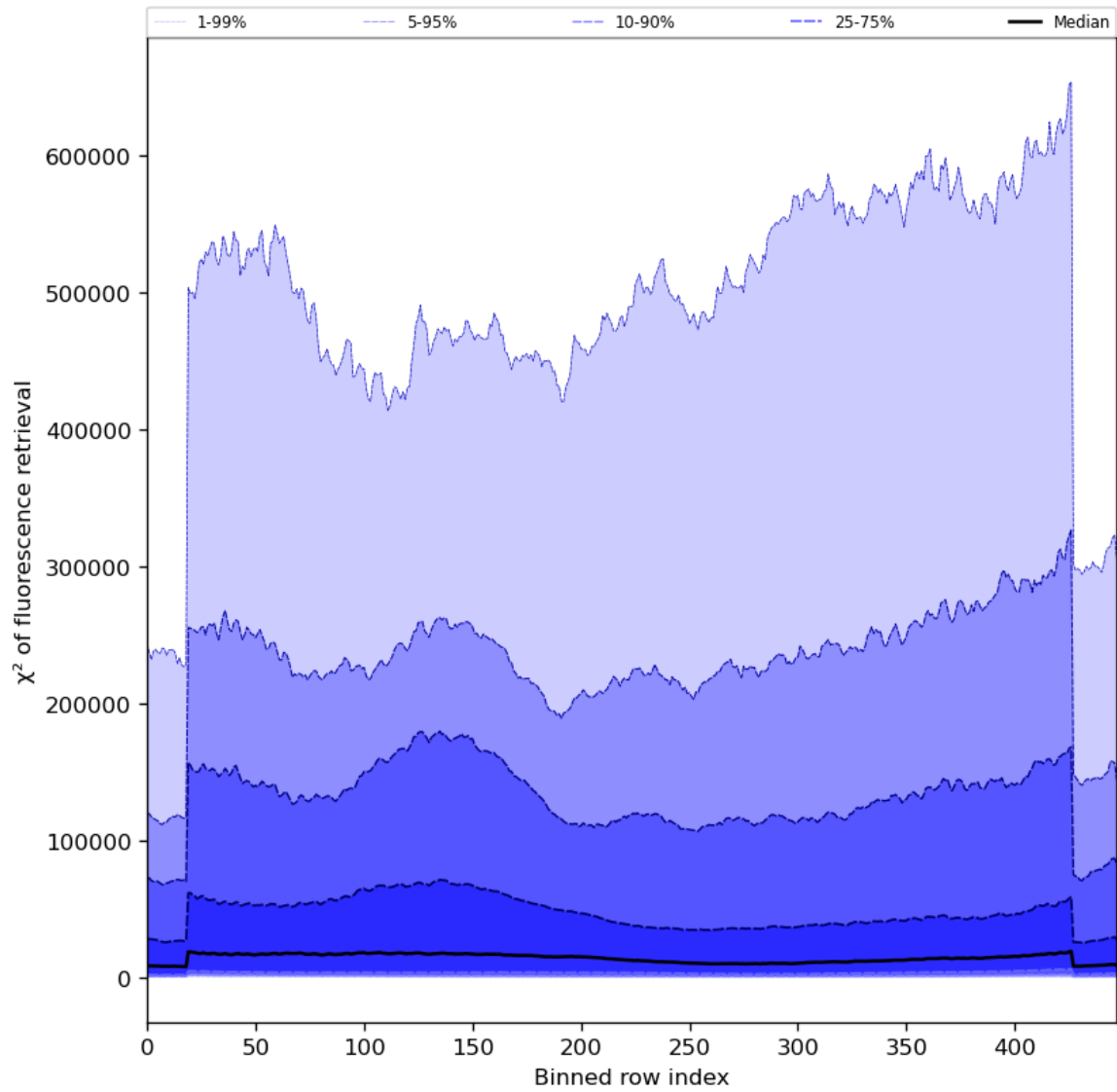
Figure 59: Along track statistics of “ \chi^2 of fluorescence retrieval” for 2023-12-23 to 2023-12-25
