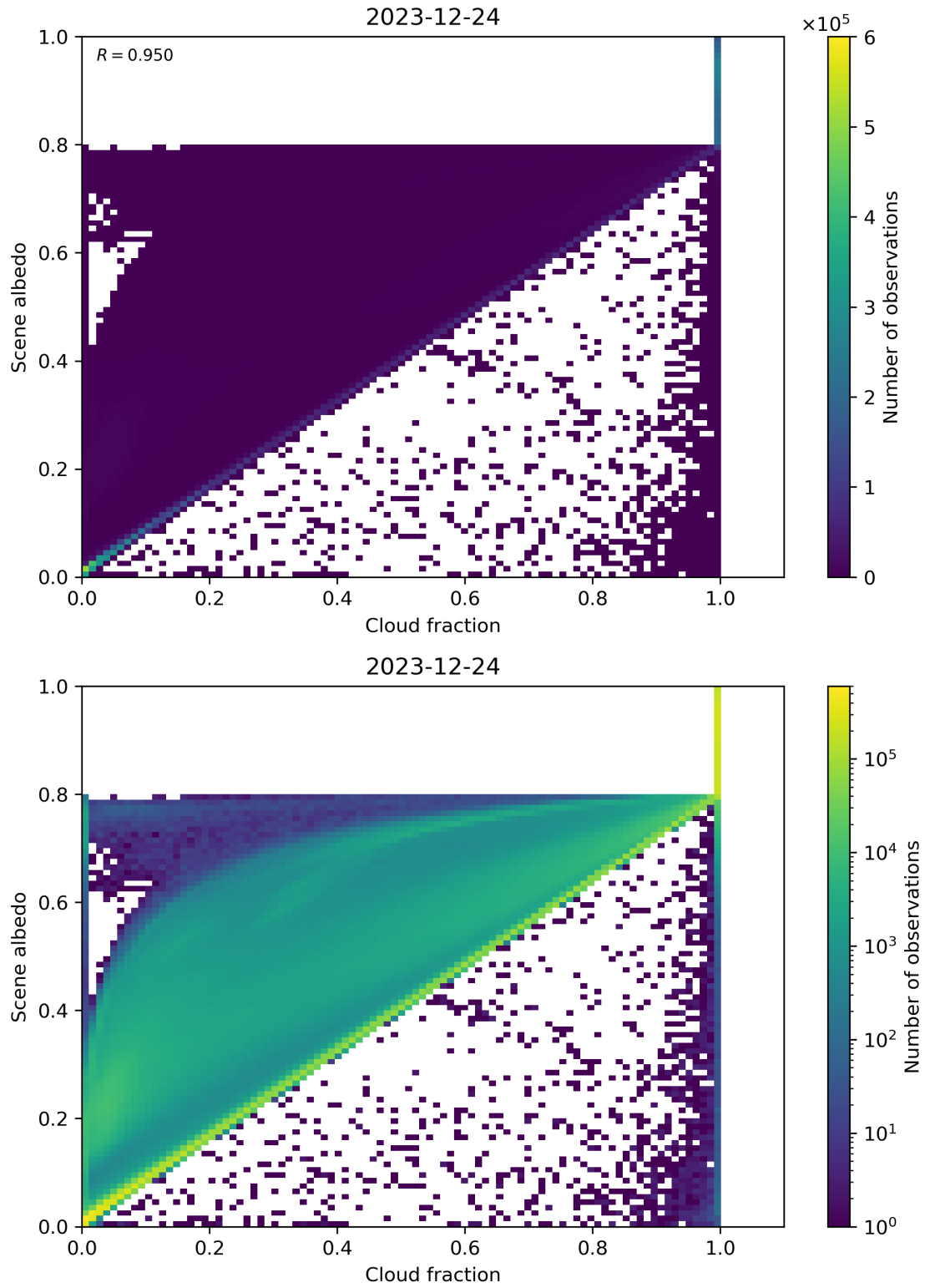
Figure 75: Scatter density plot of “Cloud fraction” against “Scene albedo” for 2023-12-23 to 2023-12-25.
