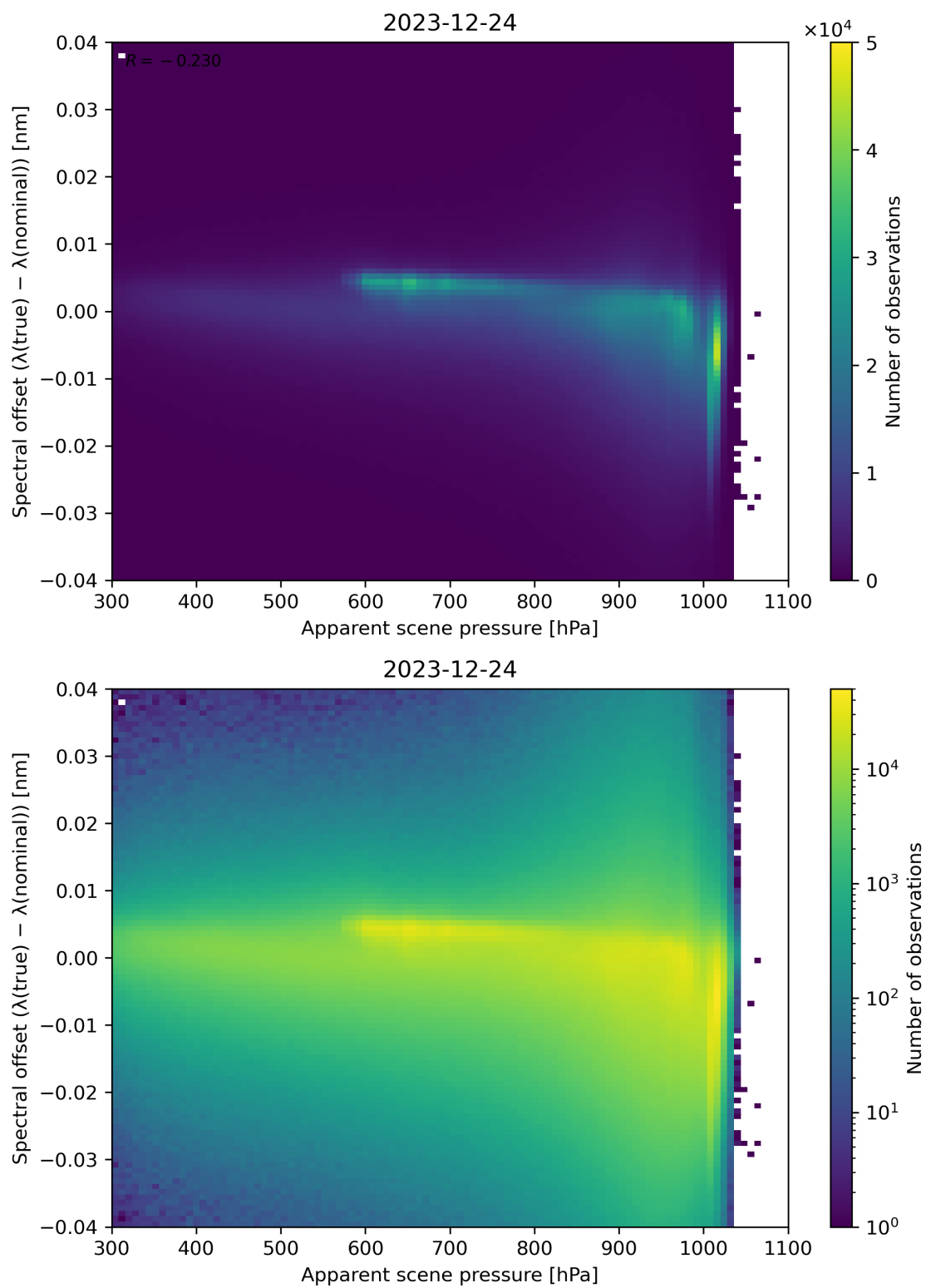
Figure 67: Scatter density plot of “Apparent scene pressure” against “Spectral offset ( \lambda(\text{true}) - \lambda(\text{nominal}) )” for 2023-12-23 to 2023-12-25.
