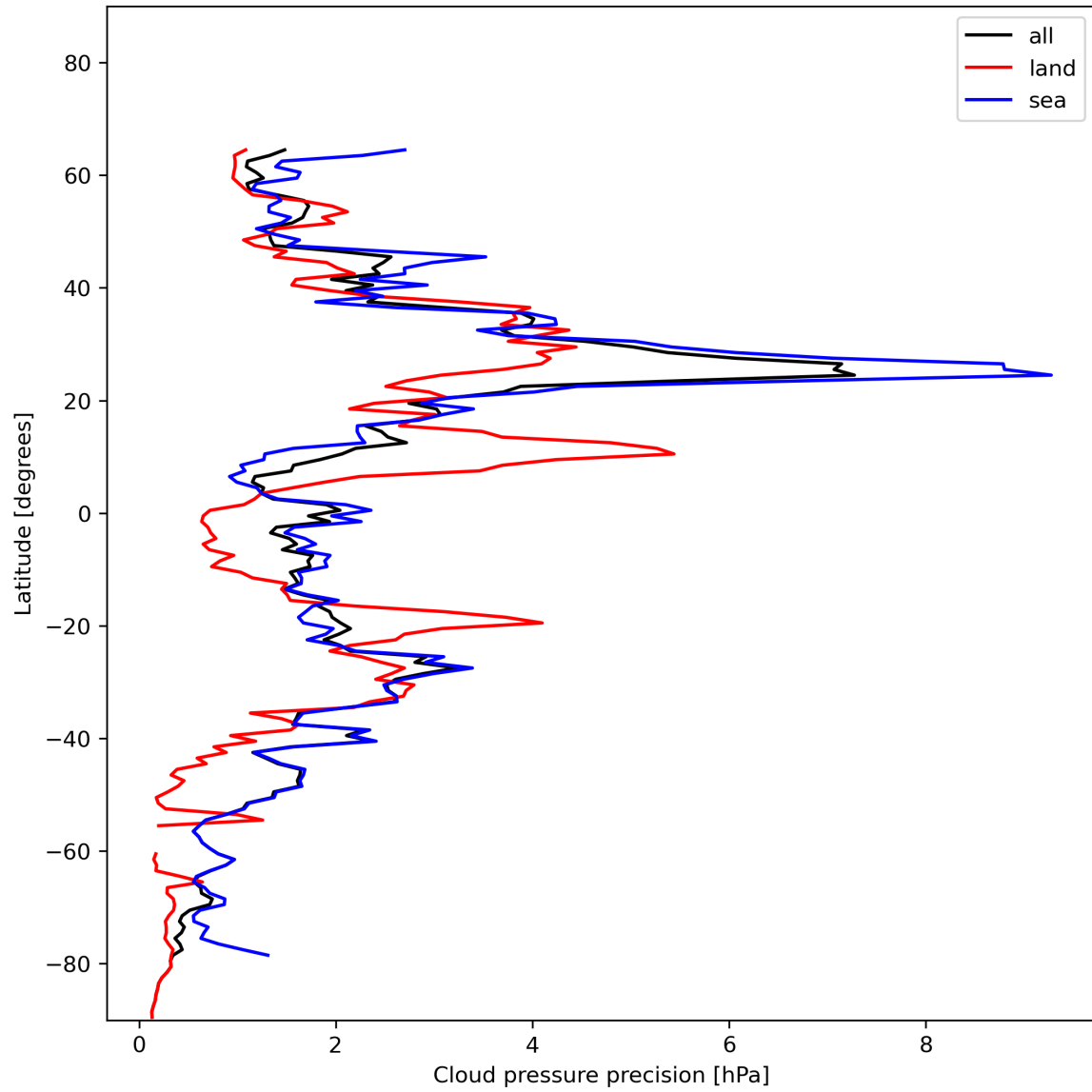
Figure 14: Zonal average of “Cloud pressure precision” for 2023-12-23 to 2023-12-25.
