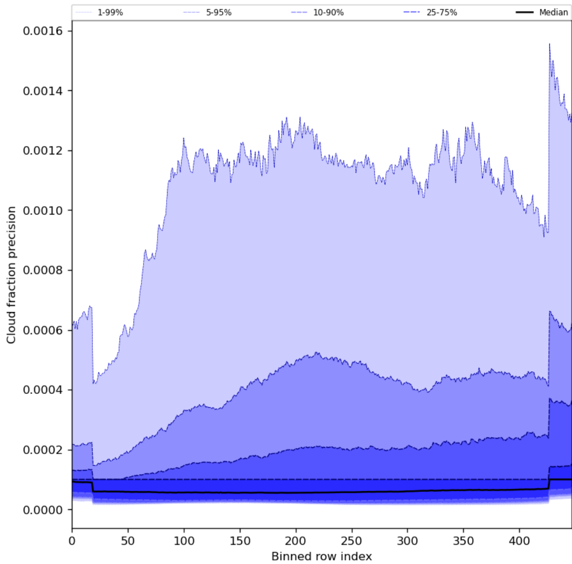
Figure 50: Along track statistics of “Cloud fraction precision” for 2023-12-23 to 2023-12-25
