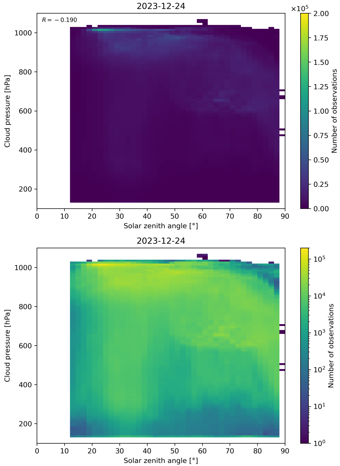
Figure 111: Scatter density plot of “Solar zenith angle” against “Cloud pressure” for 2023-12-23 to 2023-12-25.
