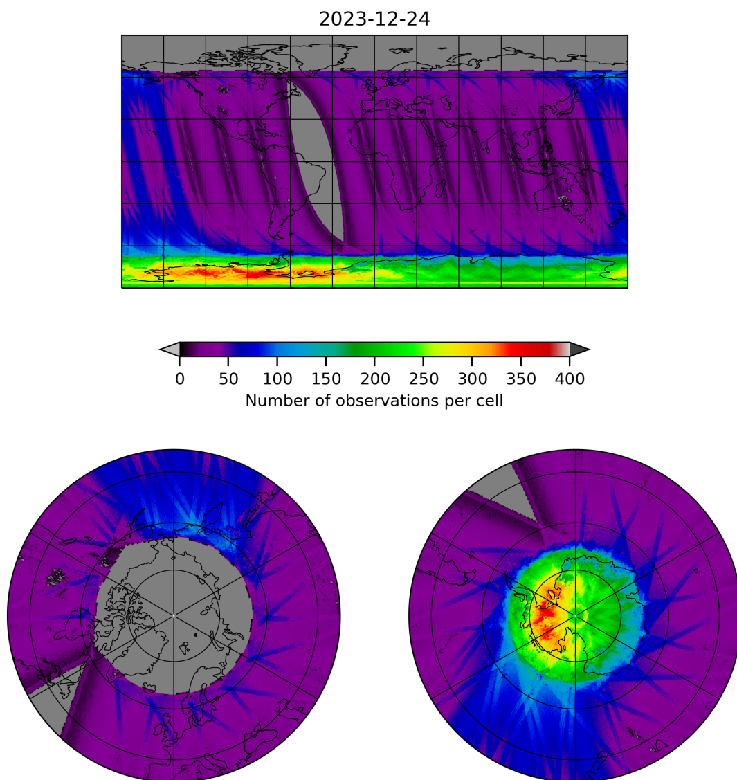
Figure 11: Map of the number of observations for 2023-12-23 to 2023-12-25
