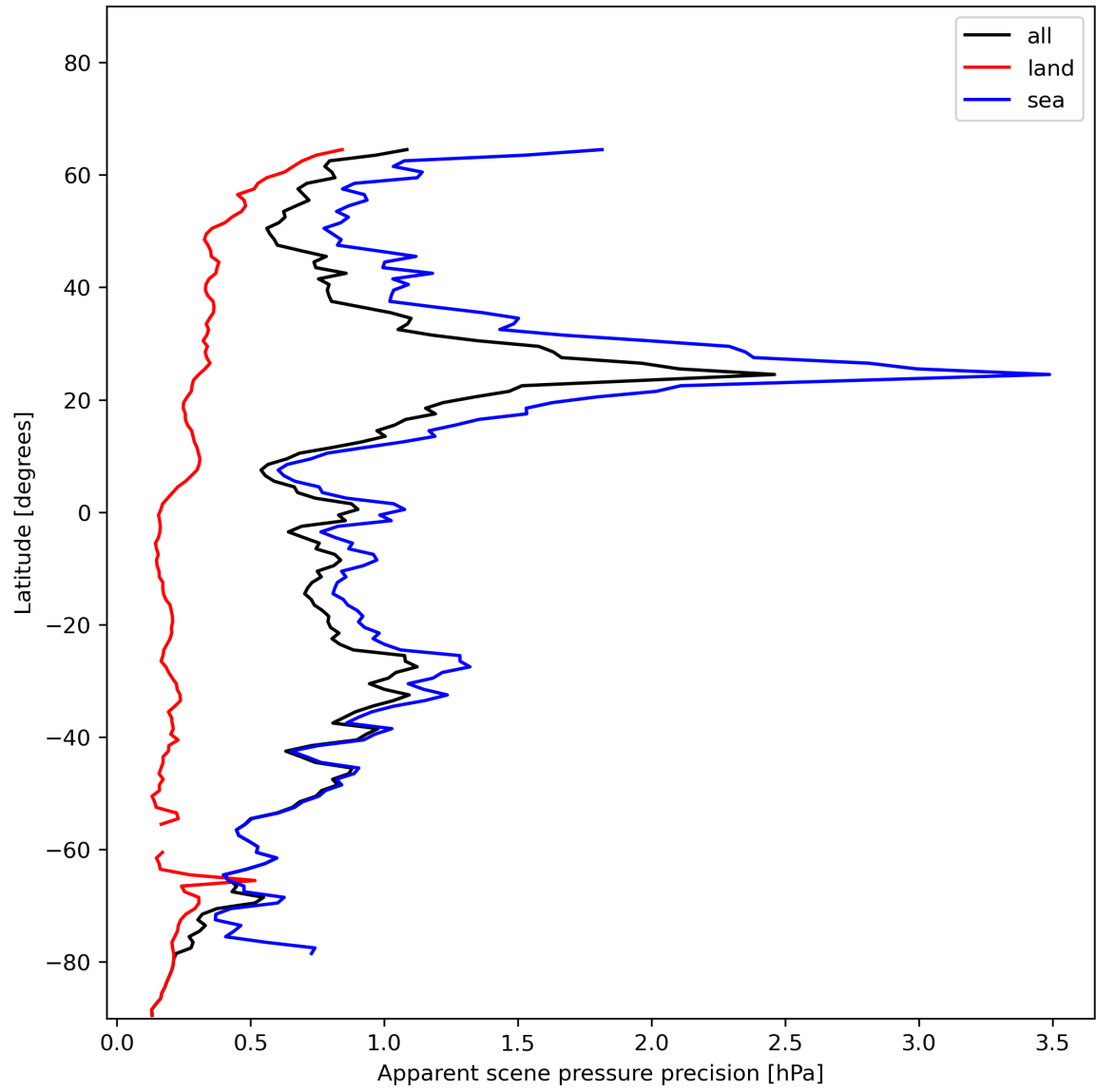
Figure 20: Zonal average of “Apparent scene pressure precision” for 2023-12-23 to 2023-12-25.
