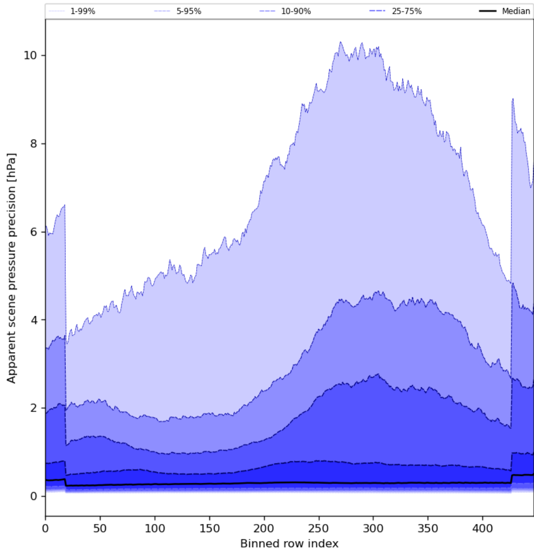
Figure 54: Along track statistics of “Apparent scene pressure precision” for 2023-12-23 to 2023-12-25
