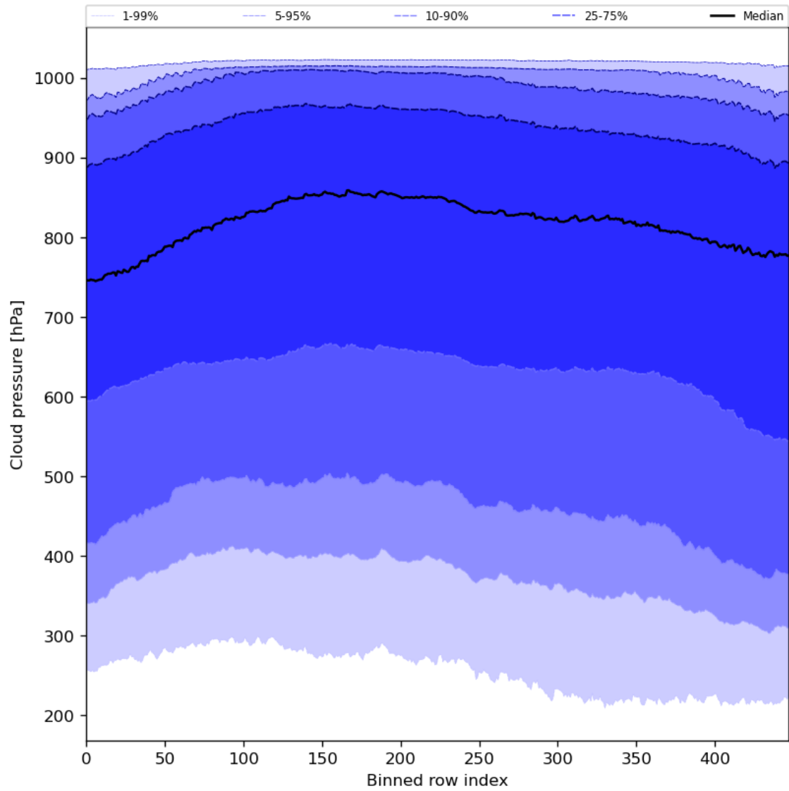
Figure 47: Along track statistics of “Cloud pressure” for 2023-12-23 to 2023-12-25
