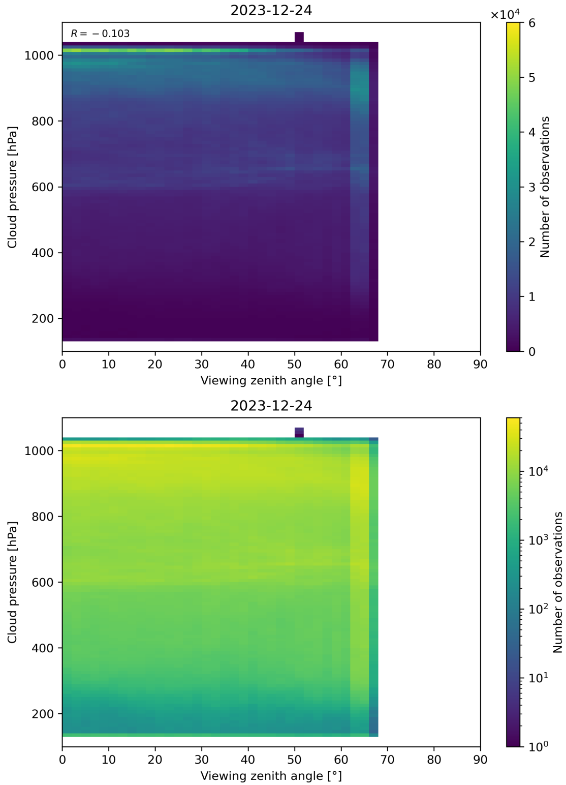
Figure 121: Scatter density plot of “Viewing zenith angle” against “Cloud pressure” for 2023-12-23 to 2023-12-25.
