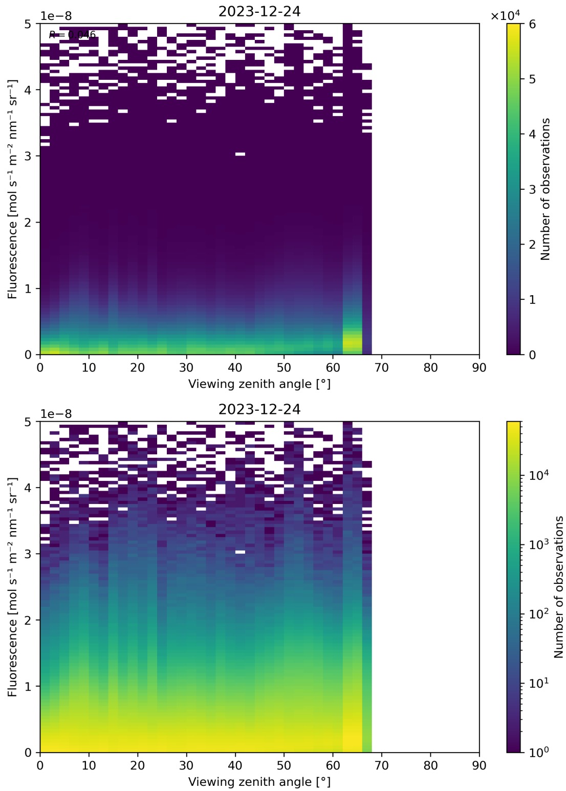
Figure 122: Scatter density plot of “Viewing zenith angle” against “Fluorescence” for 2023-12-23 to 2023-12-25.
