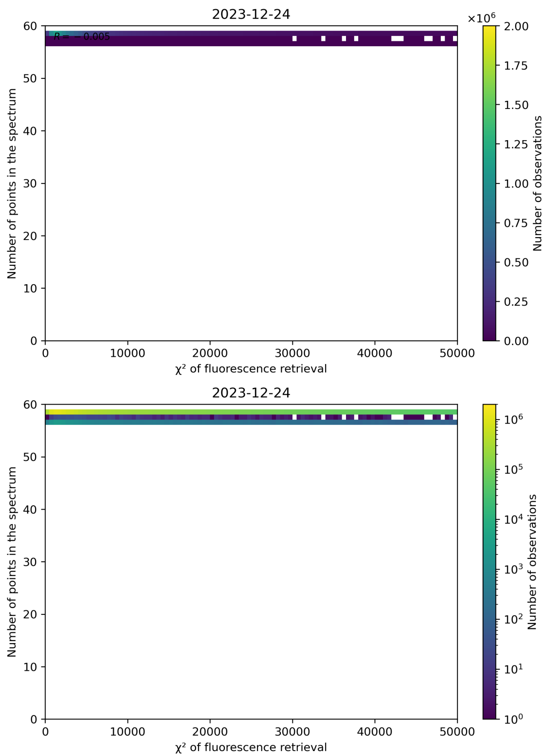
Figure 68: Scatter density plot of “ \chi^2 of fluorescence retrieval” against “Number of points in the spectrum” for 2023-12-23 to 2023-12-25.
