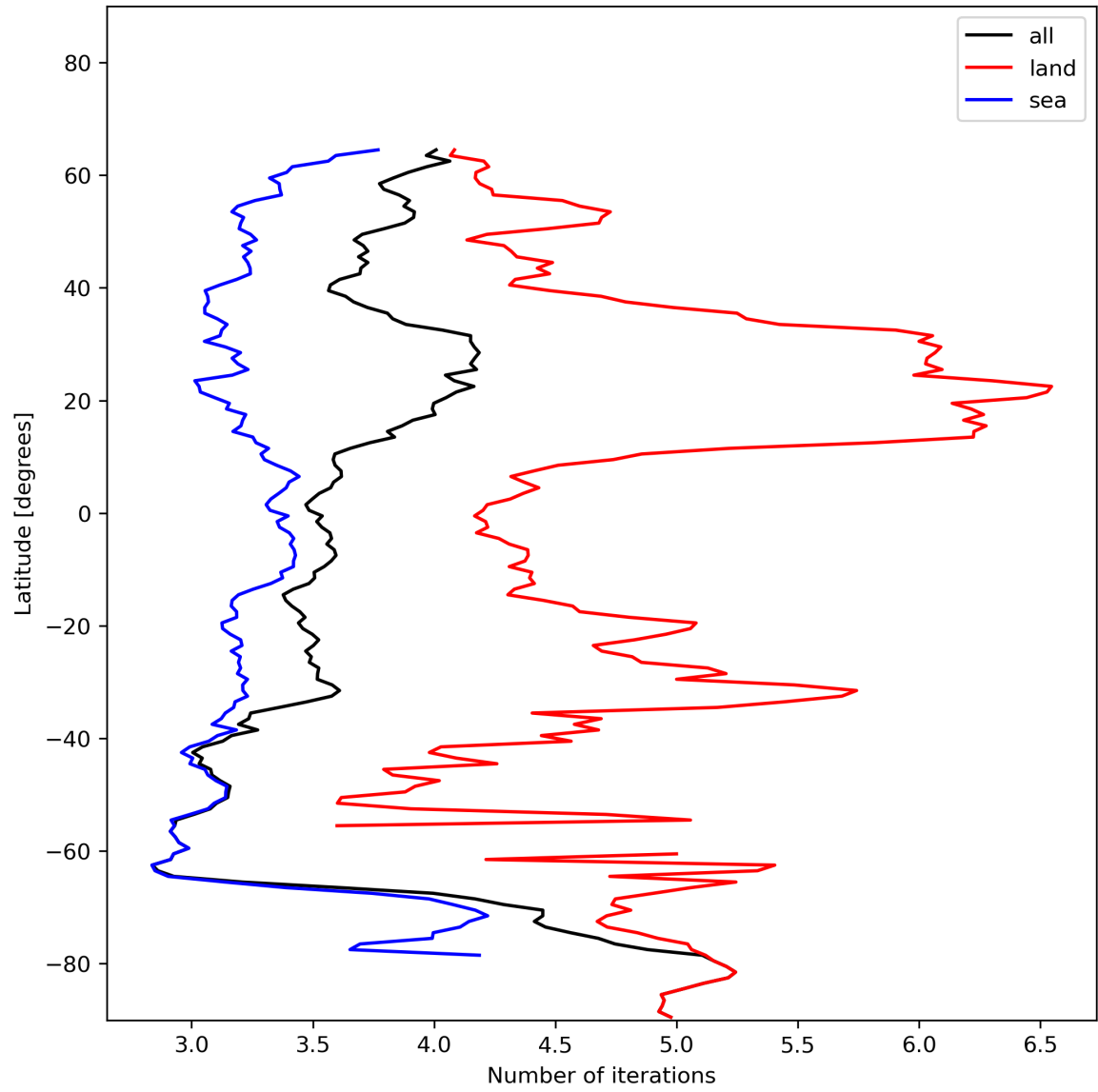
Figure 22: Zonal average of “Number of iterations” for 2023-12-23 to 2023-12-25.
