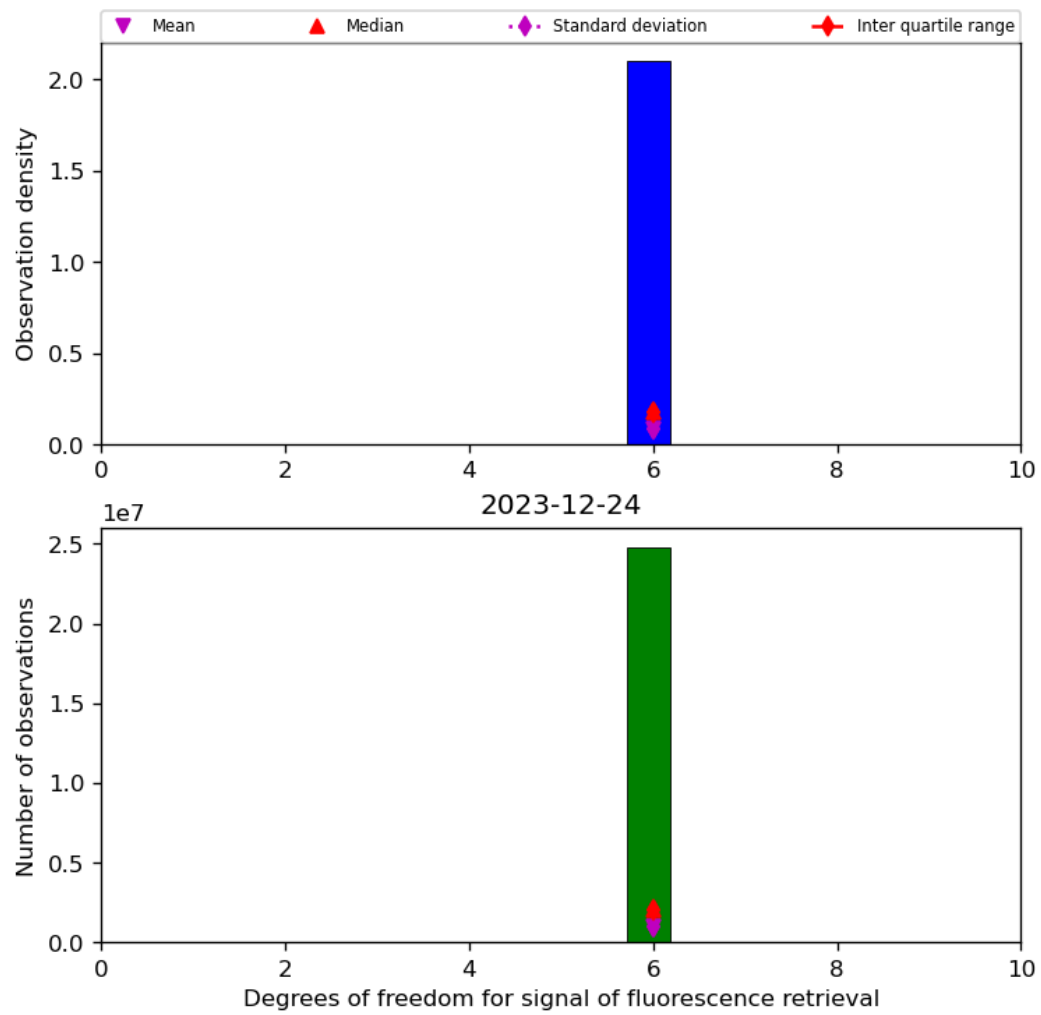
Figure 43: Histogram of “Degrees of freedom for signal of fluorescence retrieval” for 2023-12-23 to 2023-12-25
