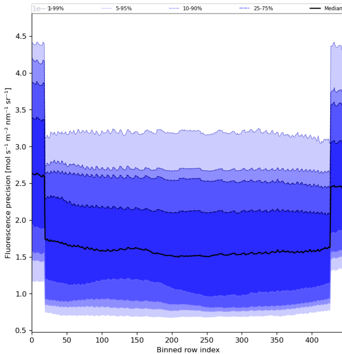
Figure 58: Along track statistics of “Fluorescence precision” for 2023-12-23 to 2023-12-25
