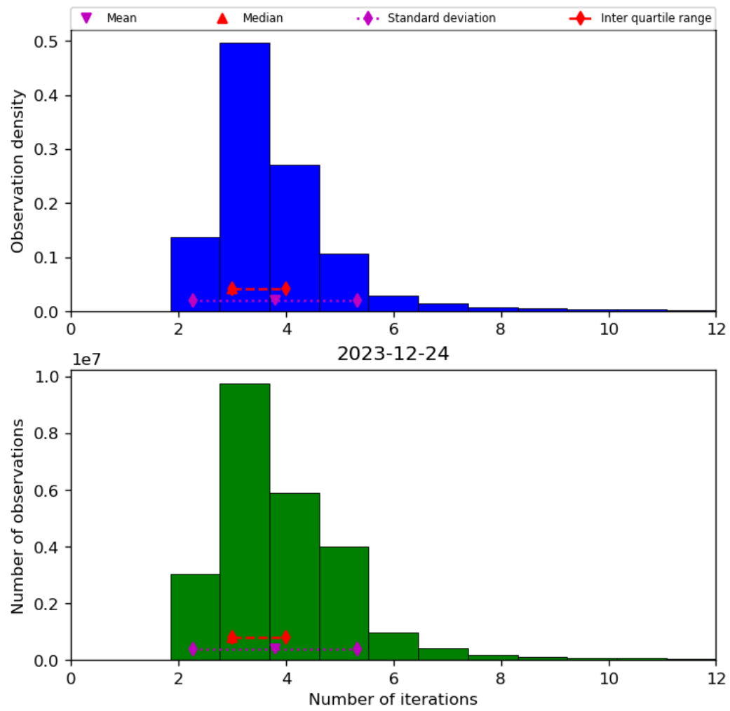
Figure 39: Histogram of “Number of iterations” for 2023-12-23 to 2023-12-25
