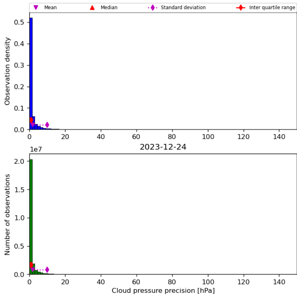
Figure 31: Histogram of “Cloud pressure precision” for 2023-12-23 to 2023-12-25
