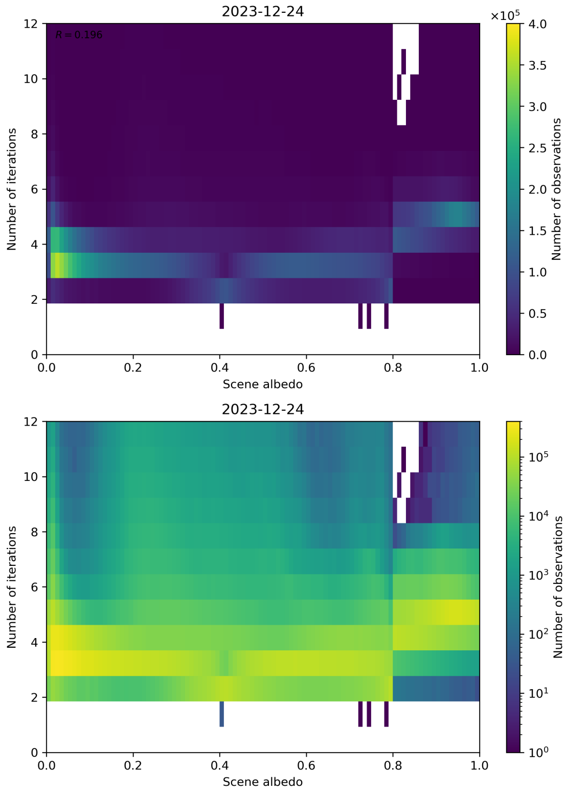
Figure 105: Scatter density plot of “Scene albedo” against “Number of iterations” for 2023-12-23 to 2023-12-25.
