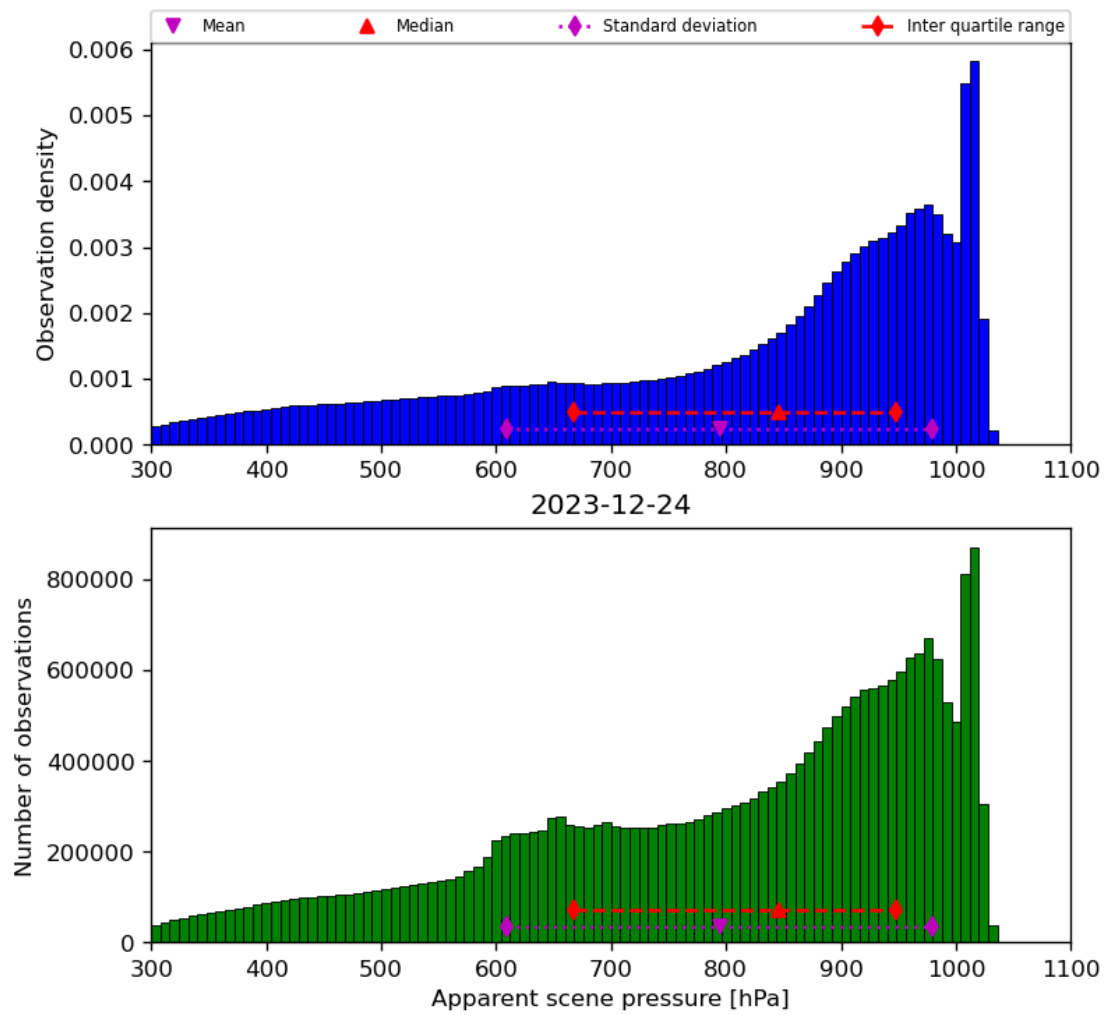
Figure 36: Histogram of “Apparent scene pressure” for 2023-12-23 to 2023-12-25
