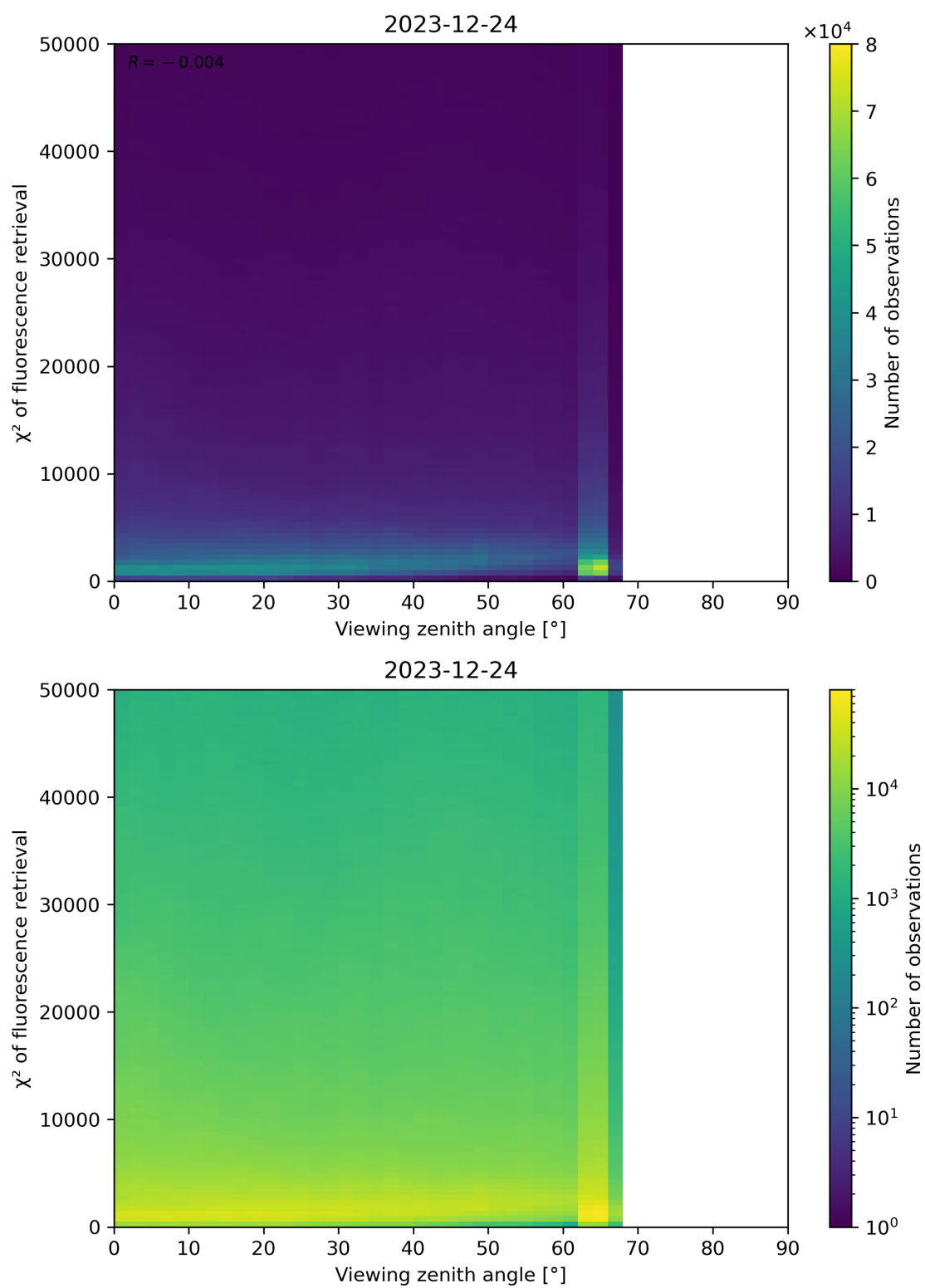
Figure 119: Scatter density plot of “Viewing zenith angle” against “ \chi^2 of fluorescence retrieval” for 2023-12-23 to 2023-12-25.
