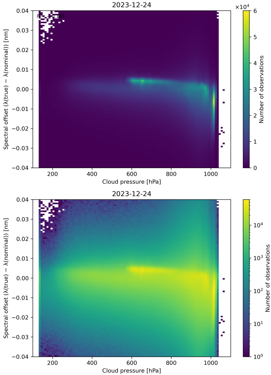
Figure 84: Scatter density plot of “Cloud pressure” against “Spectral offset ( \lambda(\text{true}) - \lambda(\text{nominal}) )” for 2023-12-23 to 2023-12-25.
