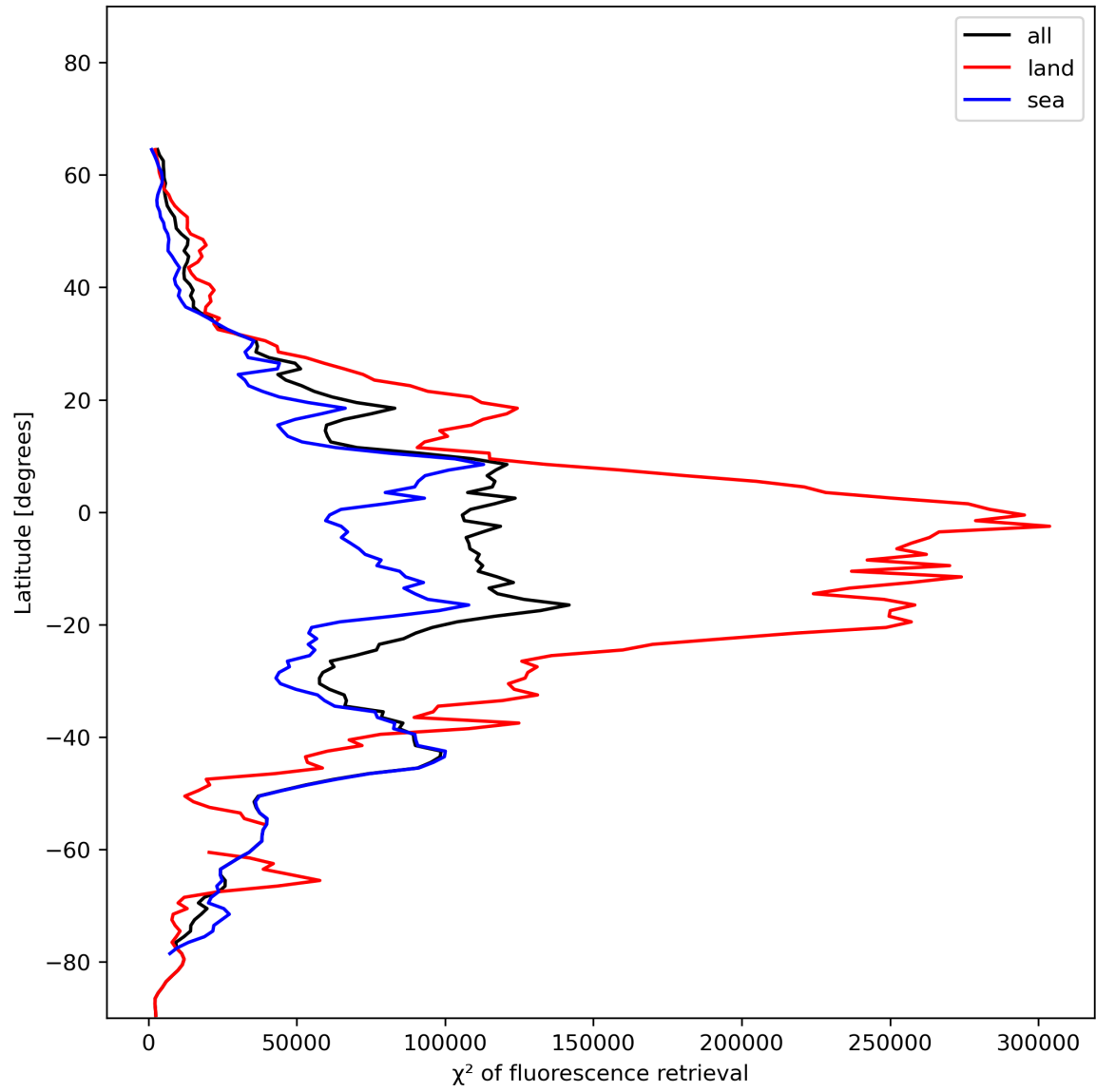
Figure 25: Zonal average of “ \chi^2 of fluorescence retrieval” for 2023-12-26 to 2023-12-28.
