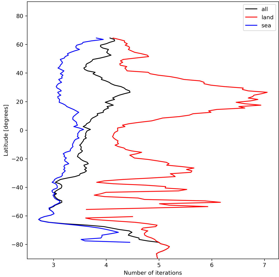
Figure 22: Zonal average of “Number of iterations” for 2023-12-26 to 2023-12-28.
