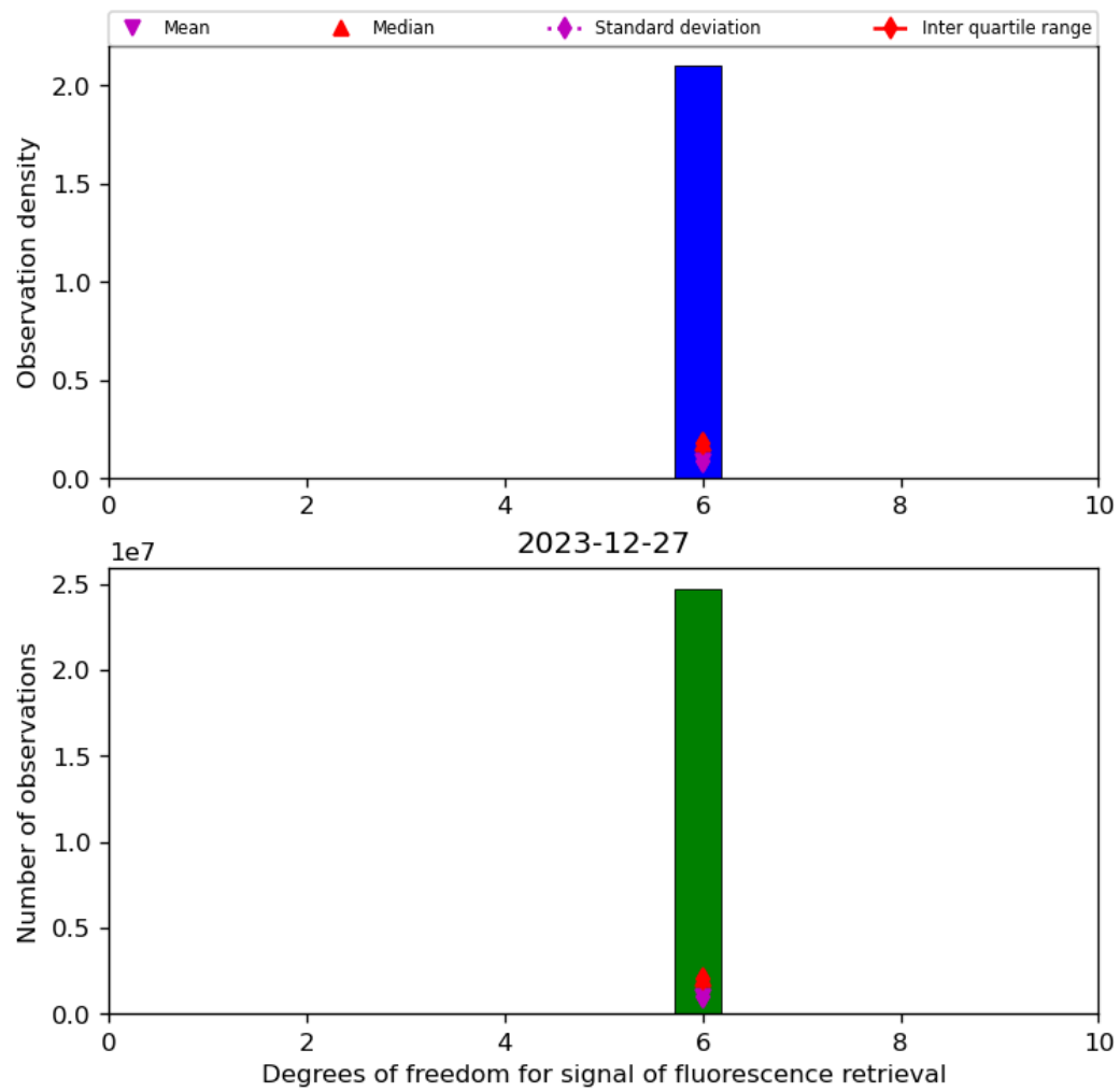
Figure 43: Histogram of “Degrees of freedom for signal of fluorescence retrieval” for 2023-12-26 to 2023-12-28
