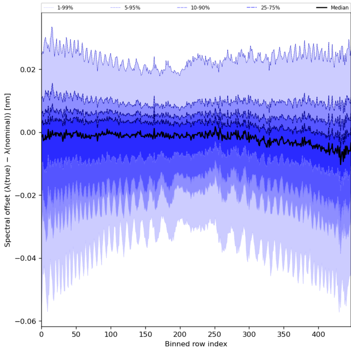
Figure 62: Along track statistics of “Spectral offset ( \lambda(\text{true}) - \lambda(\text{nominal}) )” for 2023-12-26 to 2023-12-28
