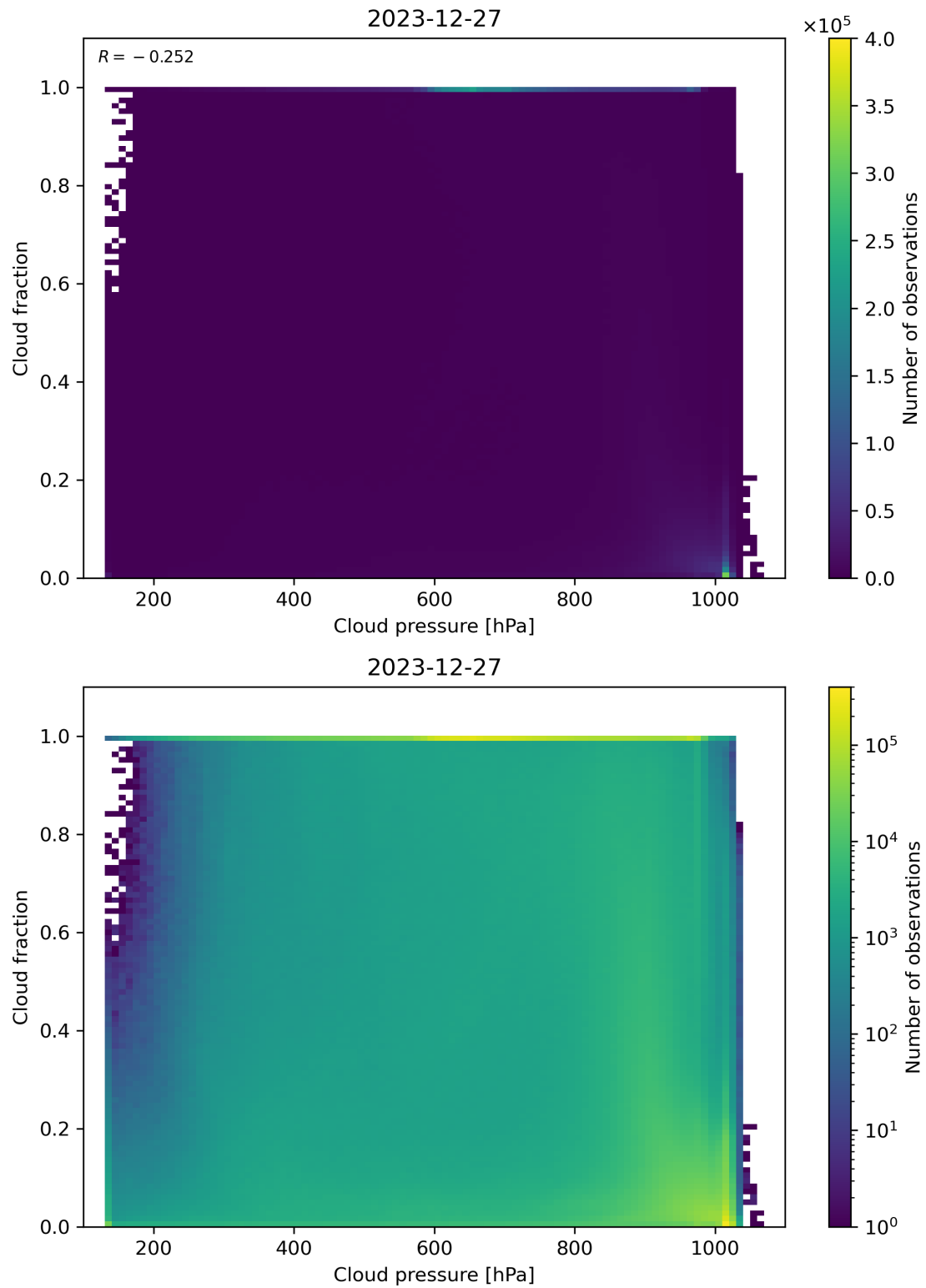
Figure 79: Scatter density plot of “Cloud pressure” against “Cloud fraction” for 2023-12-26 to 2023-12-28.
