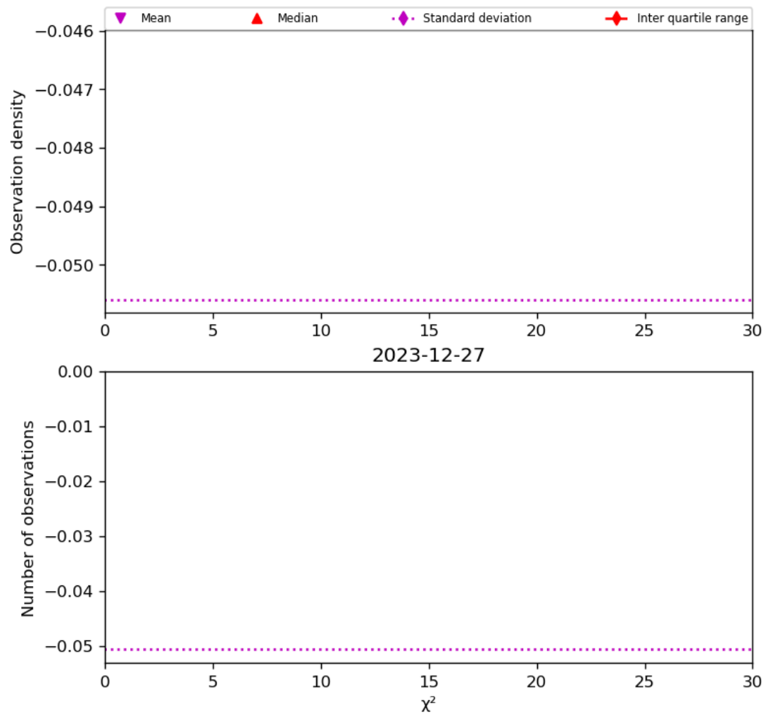
Figure 38: Histogram of “ \chi^2 ” for 2023-12-26 to 2023-12-28
