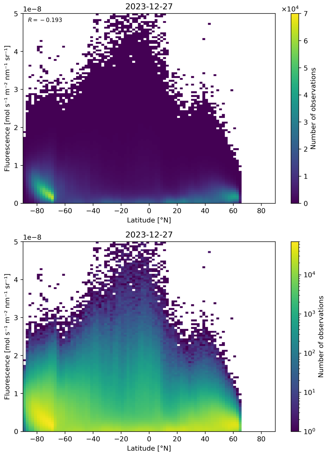
Figure 92: Scatter density plot of “Latitude” against “Fluorescence” for 2023-12-26 to 2023-12-28.
