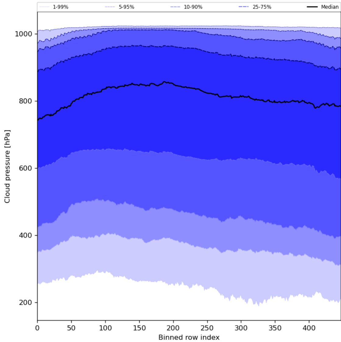
Figure 47: Along track statistics of “Cloud pressure” for 2023-12-26 to 2023-12-28
