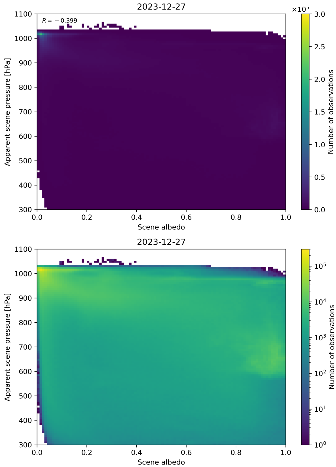
Figure 102: Scatter density plot of “Scene albedo” against “Apparent scene pressure” for 2023-12-26 to 2023-12-28.
