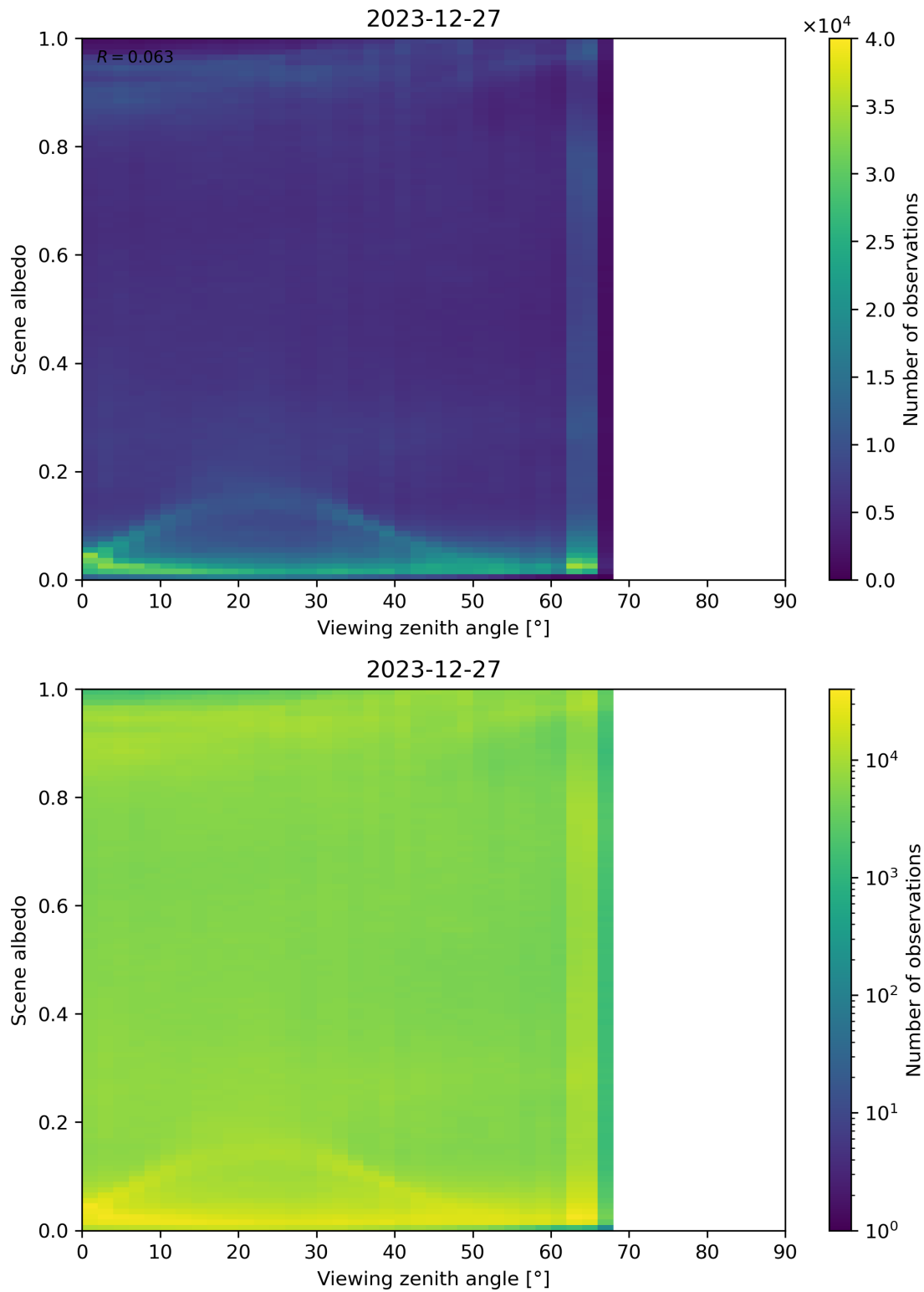
Figure 126: Scatter density plot of “Viewing zenith angle” against “Scene albedo” for 2023-12-26 to 2023-12-28.
