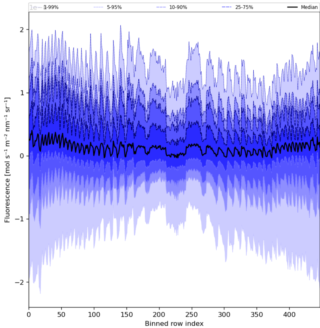
Figure 57: Along track statistics of “Fluorescence” for 2023-12-26 to 2023-12-28
