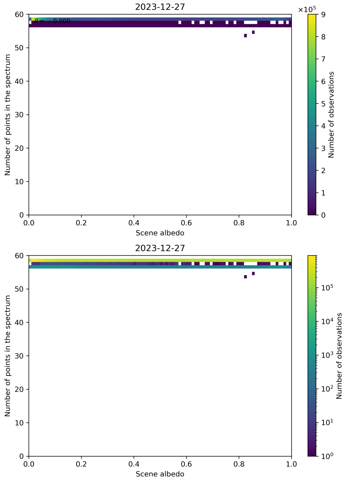
Figure 106: Scatter density plot of “Scene albedo” against “Number of points in the spectrum” for 2023-12-26 to 2023-12-28.
