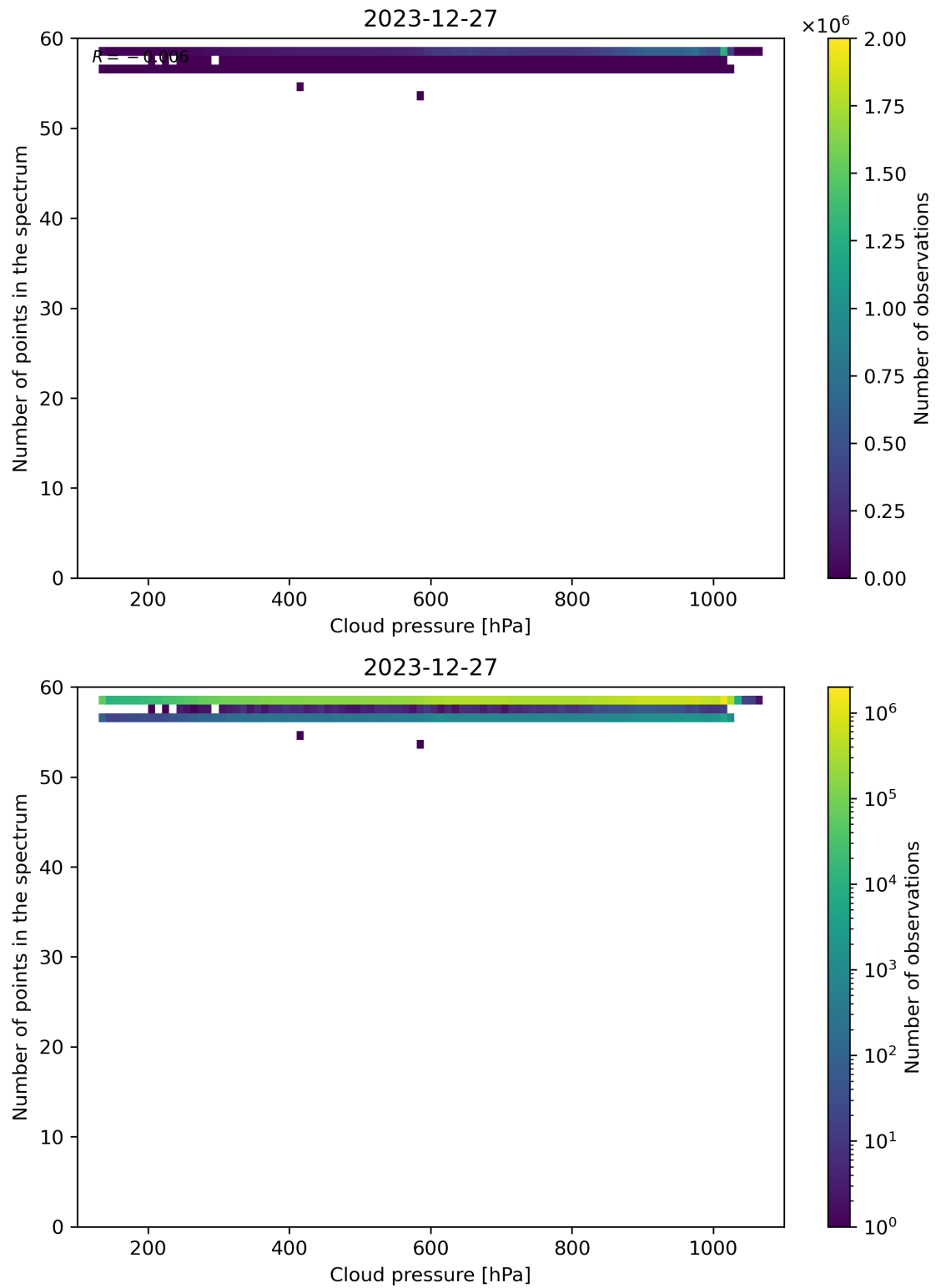
Figure 82: Scatter density plot of “Cloud pressure” against “Number of points in the spectrum” for 2023-12-26 to 2023-12-28.
