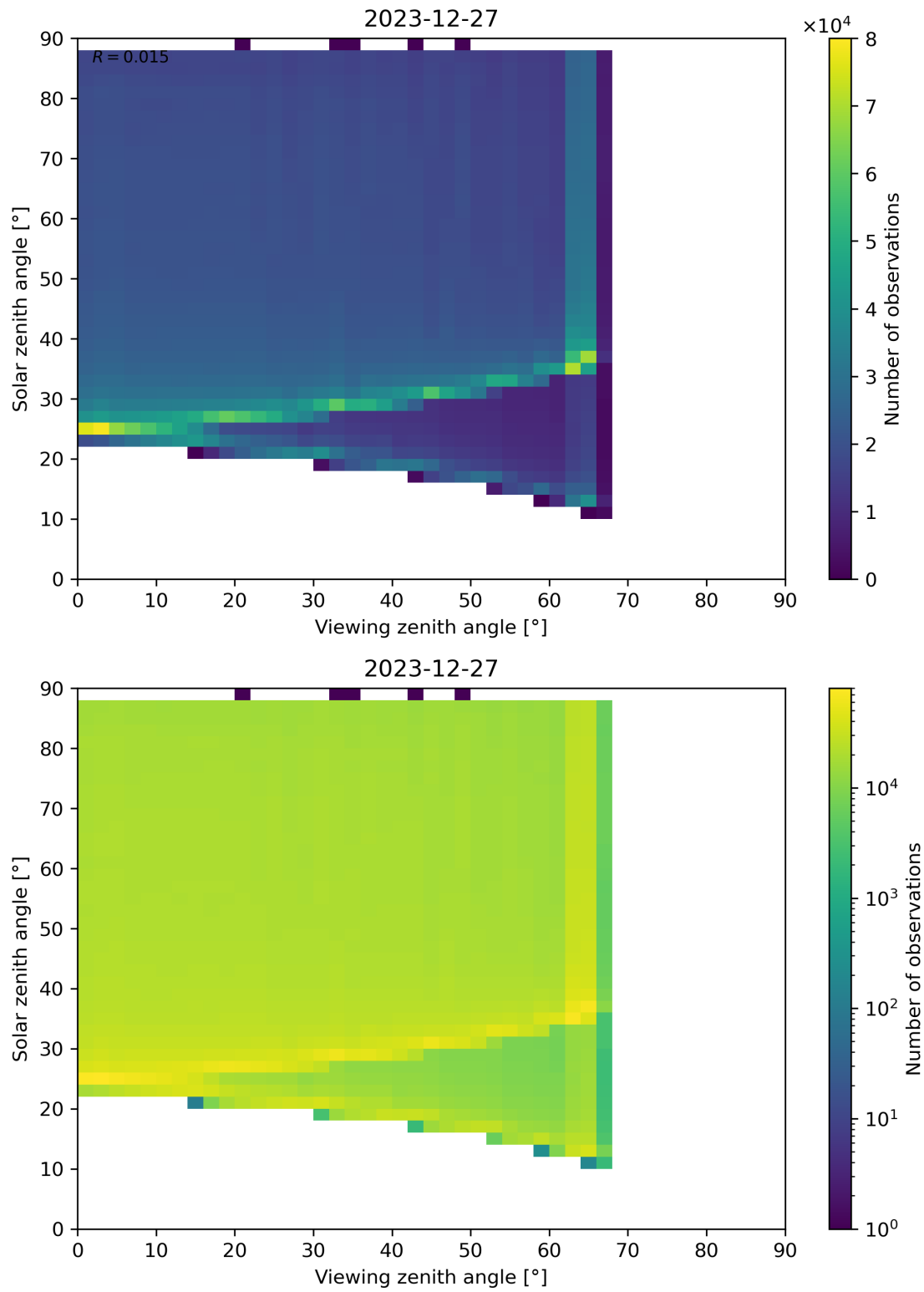
Figure 127: Scatter density plot of “Viewing zenith angle” against “Solar zenith angle” for 2023-12-26 to 2023-12-28.
