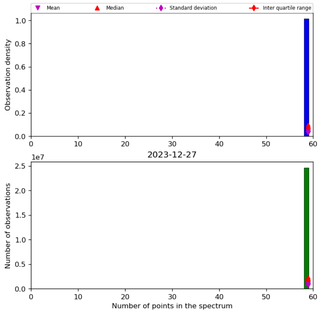
Figure 44: Histogram of “Number of points in the spectrum” for 2023-12-26 to 2023-12-28
