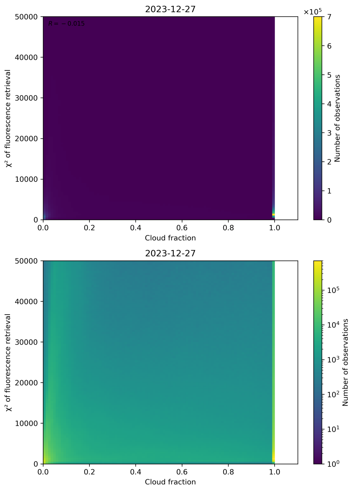
Figure 71: Scatter density plot of “Cloud fraction” against “ \chi^2 of fluorescence retrieval” for 2023-12-26 to 2023-12-28.
