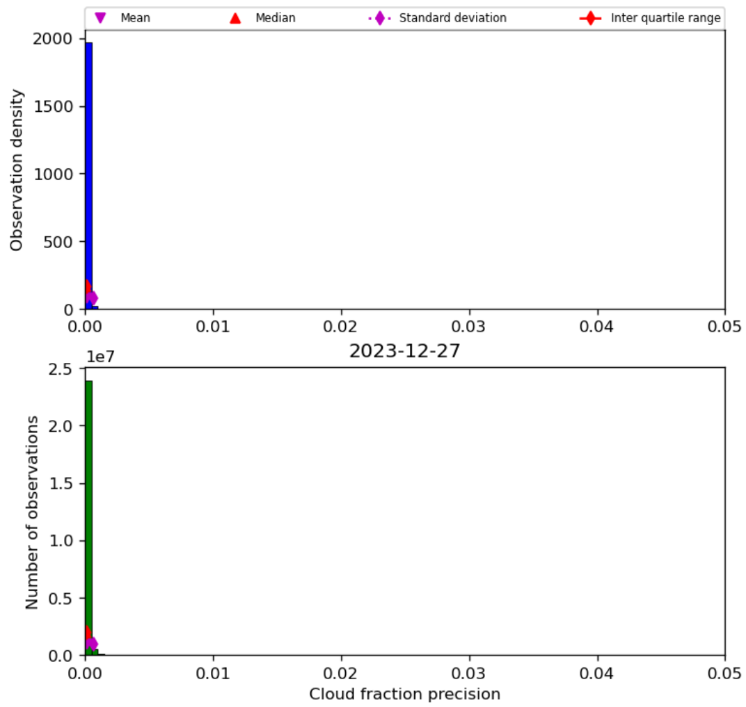
Figure 33: Histogram of “Cloud fraction precision” for 2023-12-26 to 2023-12-28
