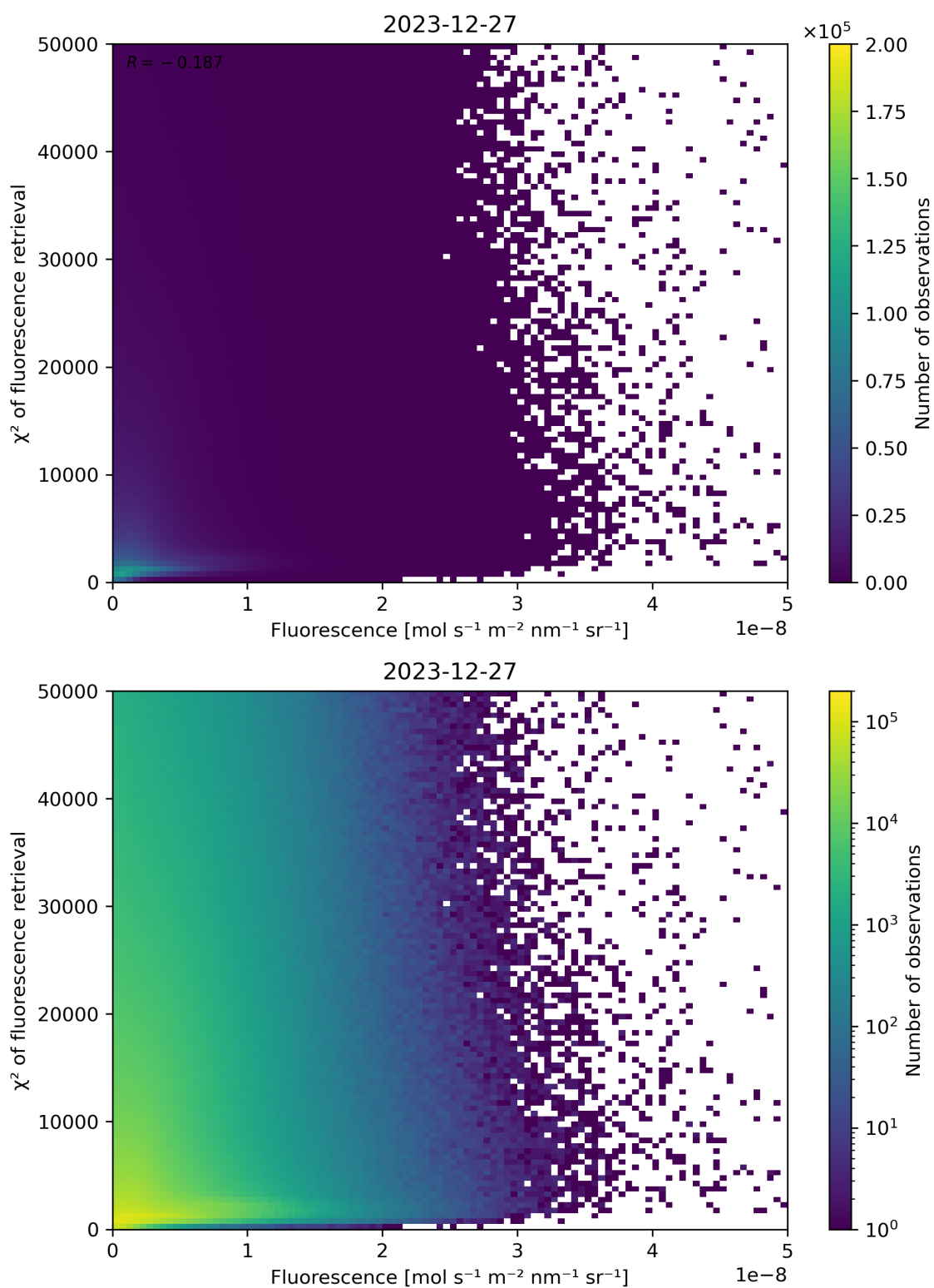
Figure 85: Scatter density plot of “Fluorescence” against “ \chi^2 of fluorescence retrieval” for 2023-12-26 to 2023-12-28.
