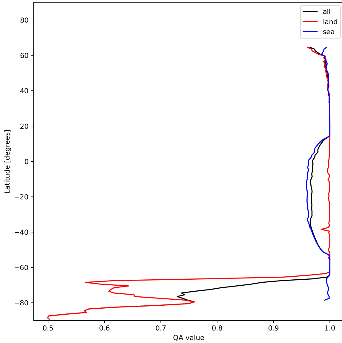
Figure 12: Zonal average of “QA value” for 2023-12-26 to 2023-12-28.
