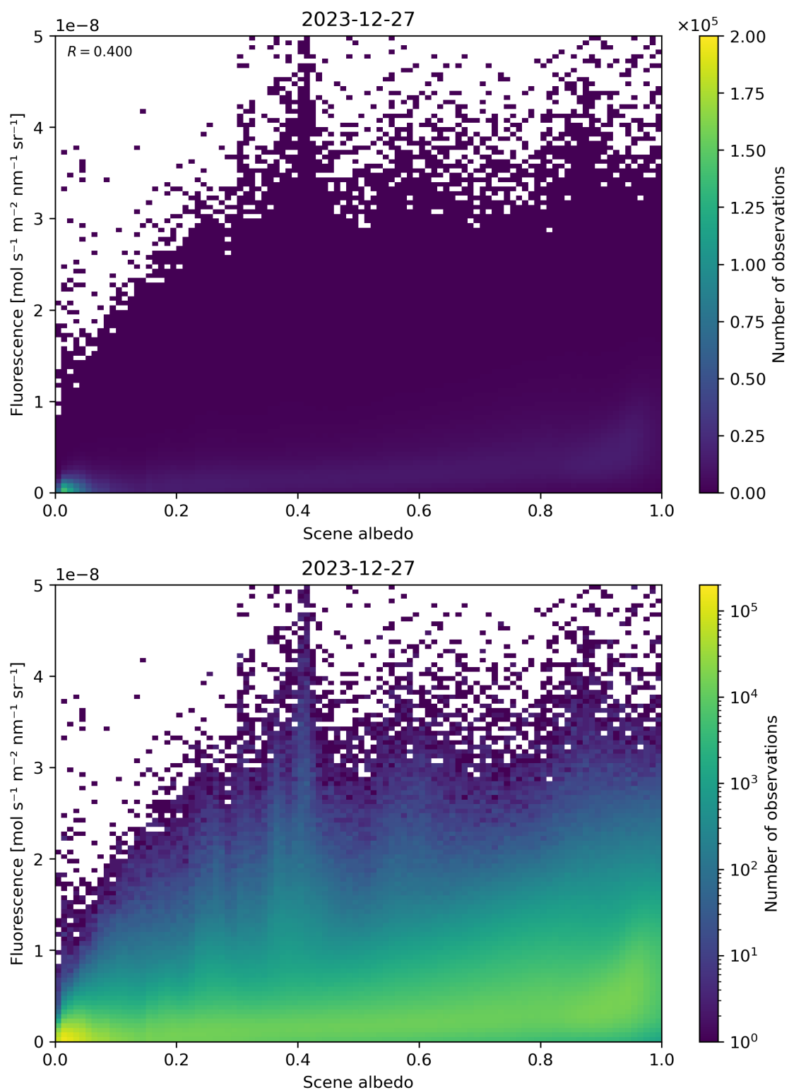
Figure 104: Scatter density plot of “Scene albedo” against “Fluorescence” for 2023-12-26 to 2023-12-28.
