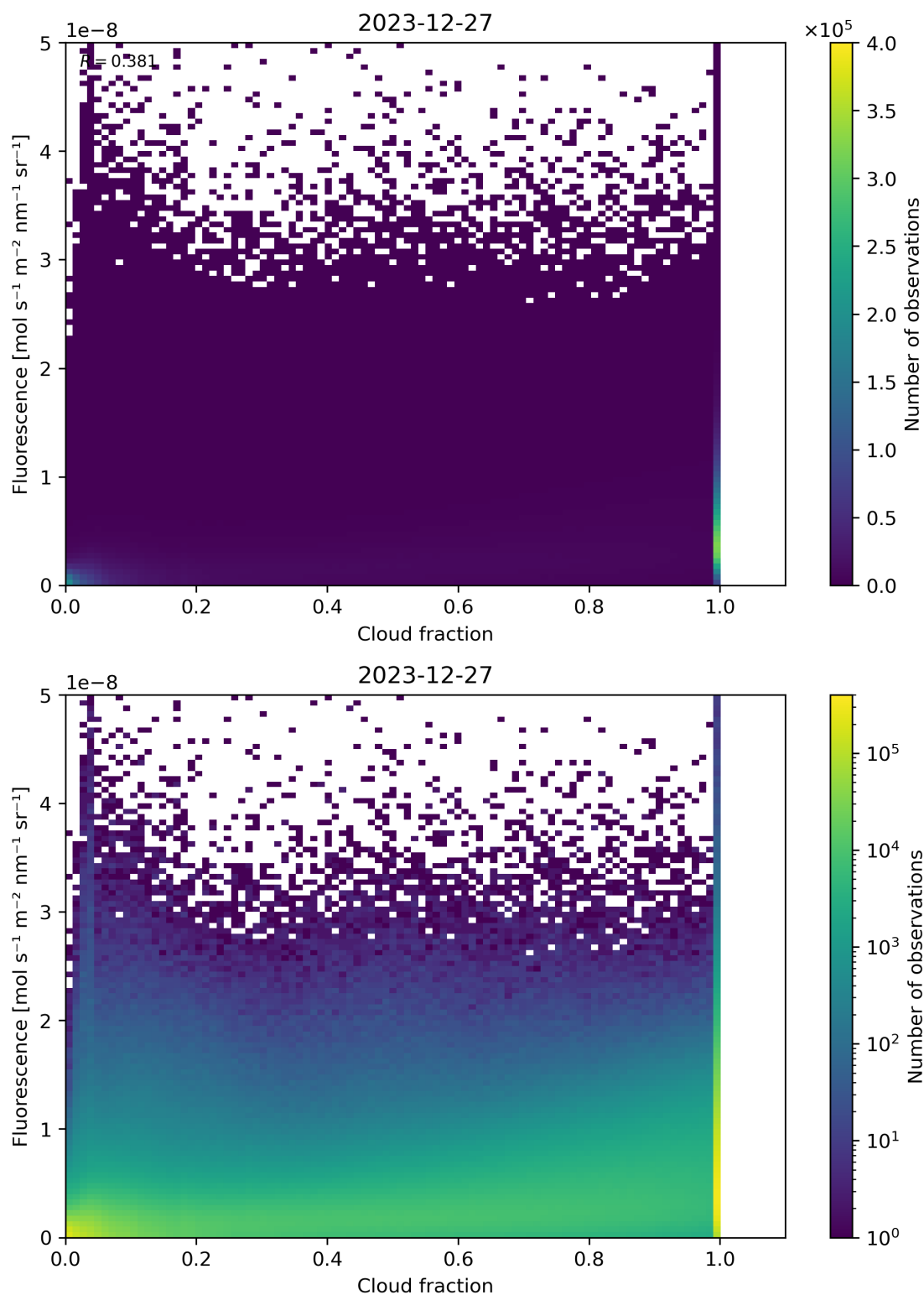
Figure 72: Scatter density plot of “Cloud fraction” against “Fluorescence” for 2023-12-26 to 2023-12-28.
