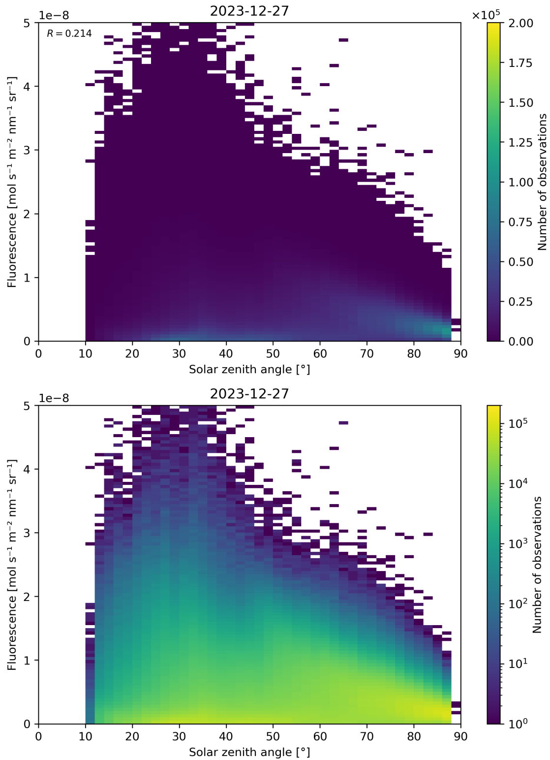
Figure 112: Scatter density plot of “Solar zenith angle” against “Fluorescence” for 2023-12-26 to 2023-12-28.
