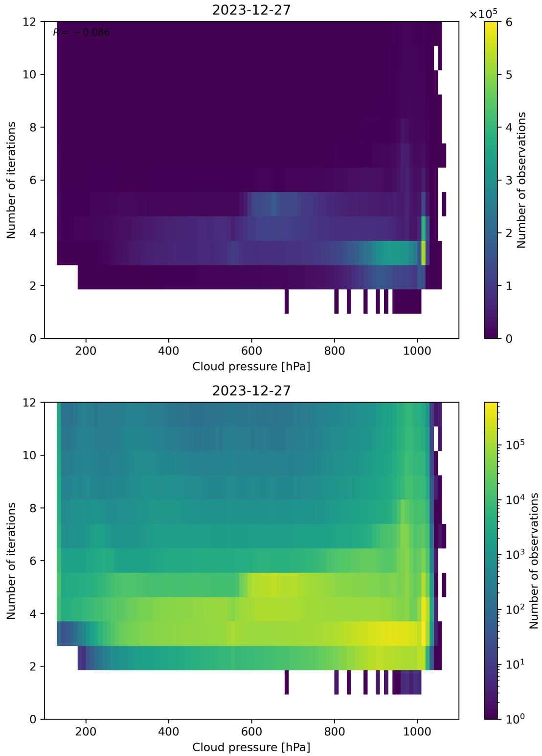
Figure 81: Scatter density plot of “Cloud pressure” against “Number of iterations” for 2023-12-26 to 2023-12-28.
