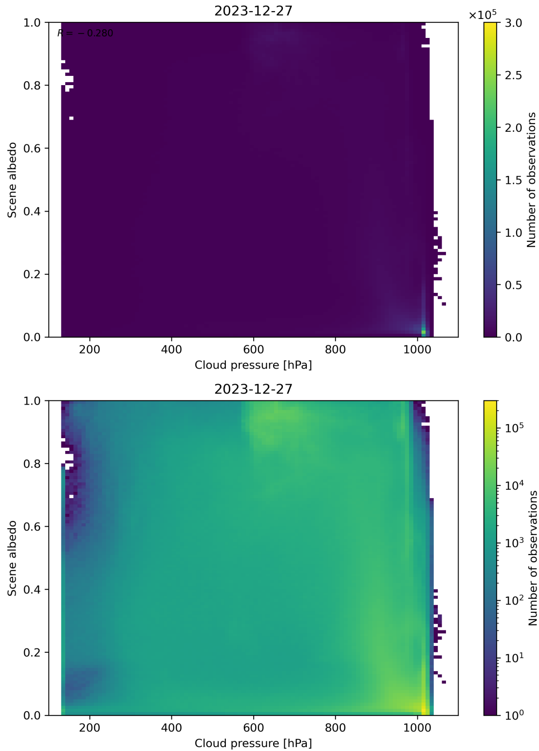
Figure 83: Scatter density plot of “Cloud pressure” against “Scene albedo” for 2023-12-26 to 2023-12-28.
