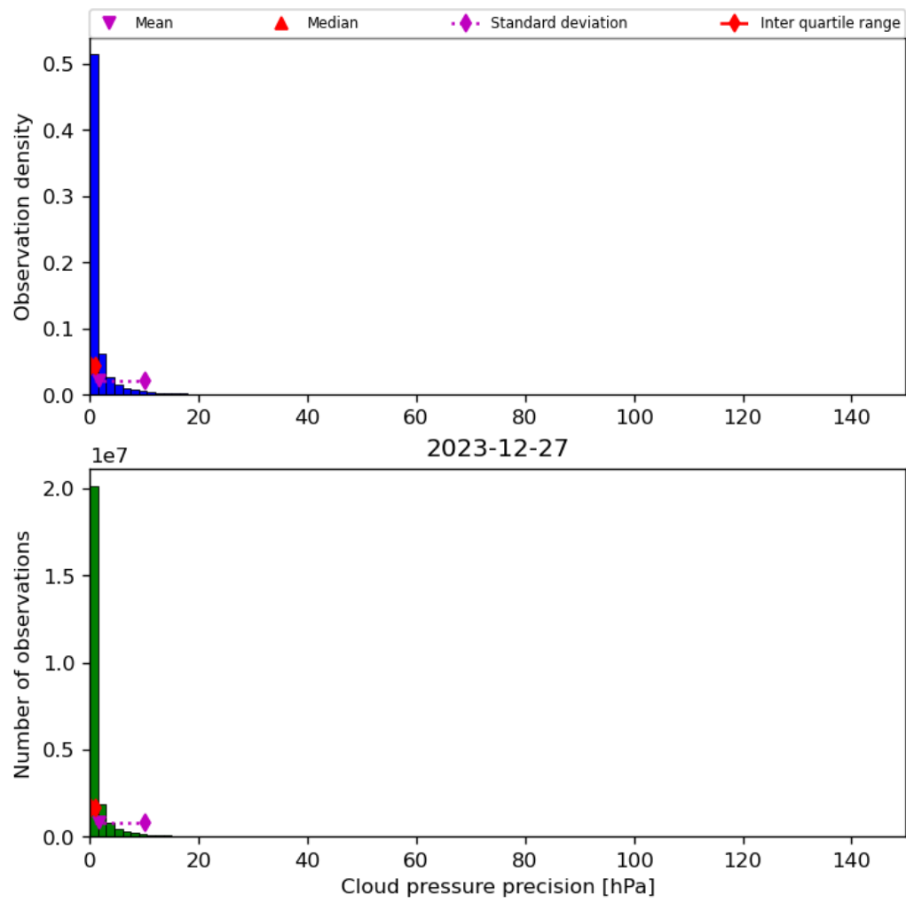
Figure 31: Histogram of “Cloud pressure precision” for 2023-12-26 to 2023-12-28
