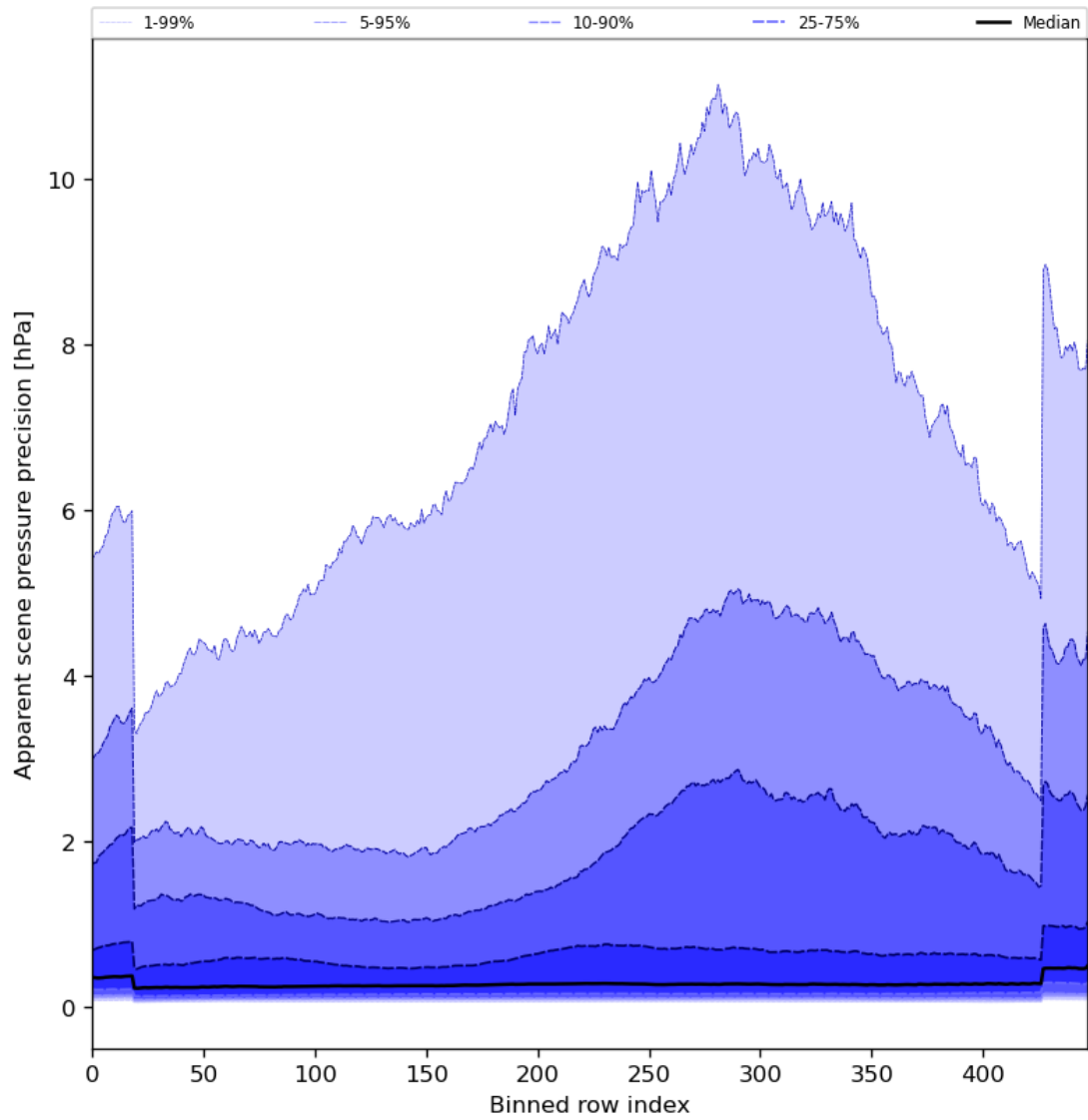
Figure 54: Along track statistics of “Apparent scene pressure precision” for 2023-12-26 to 2023-12-28
