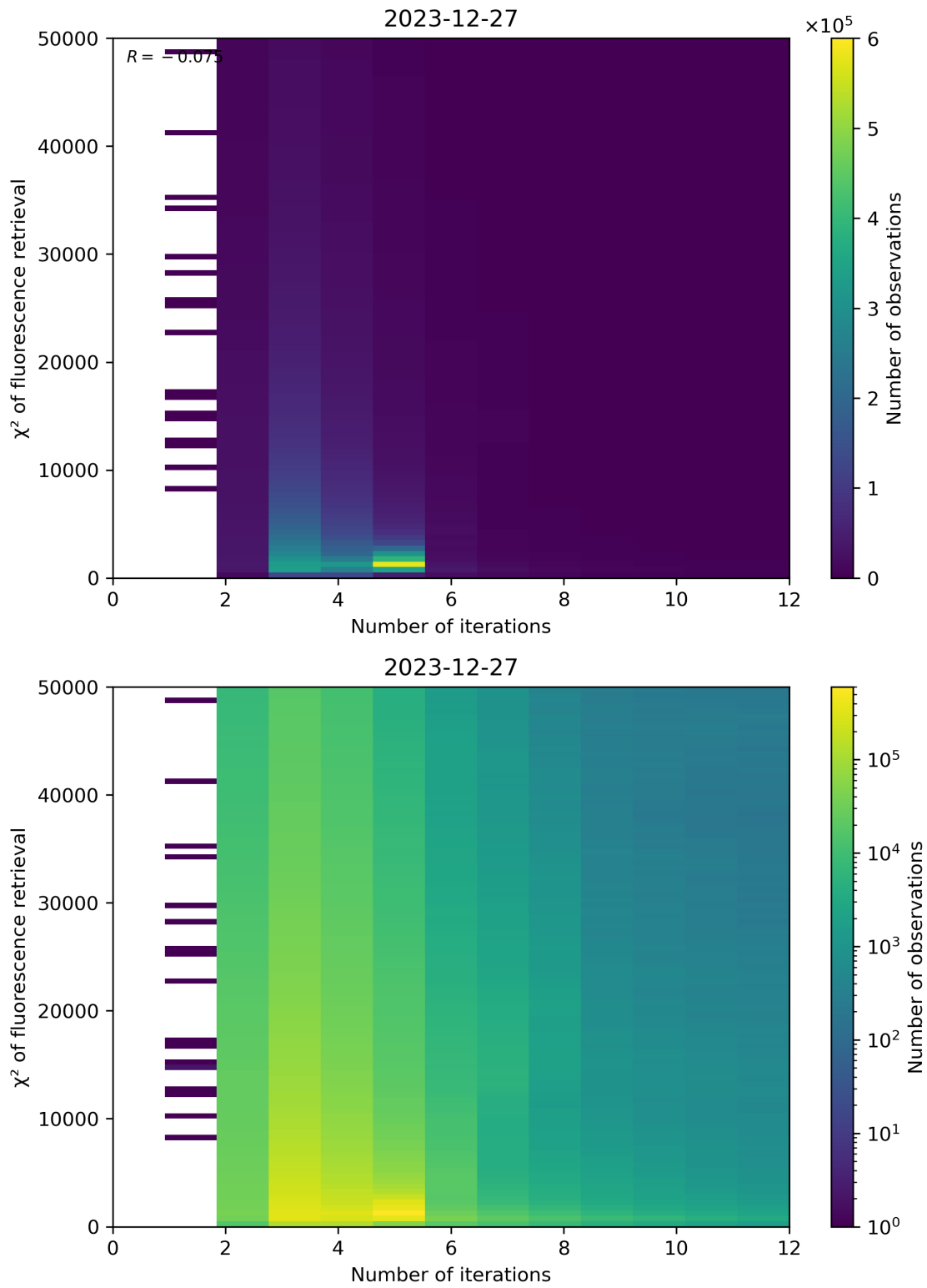
Figure 97: Scatter density plot of “Number of iterations” against “ \chi^2 of fluorescence retrieval” for 2023-12-26 to 2023-12-28.
