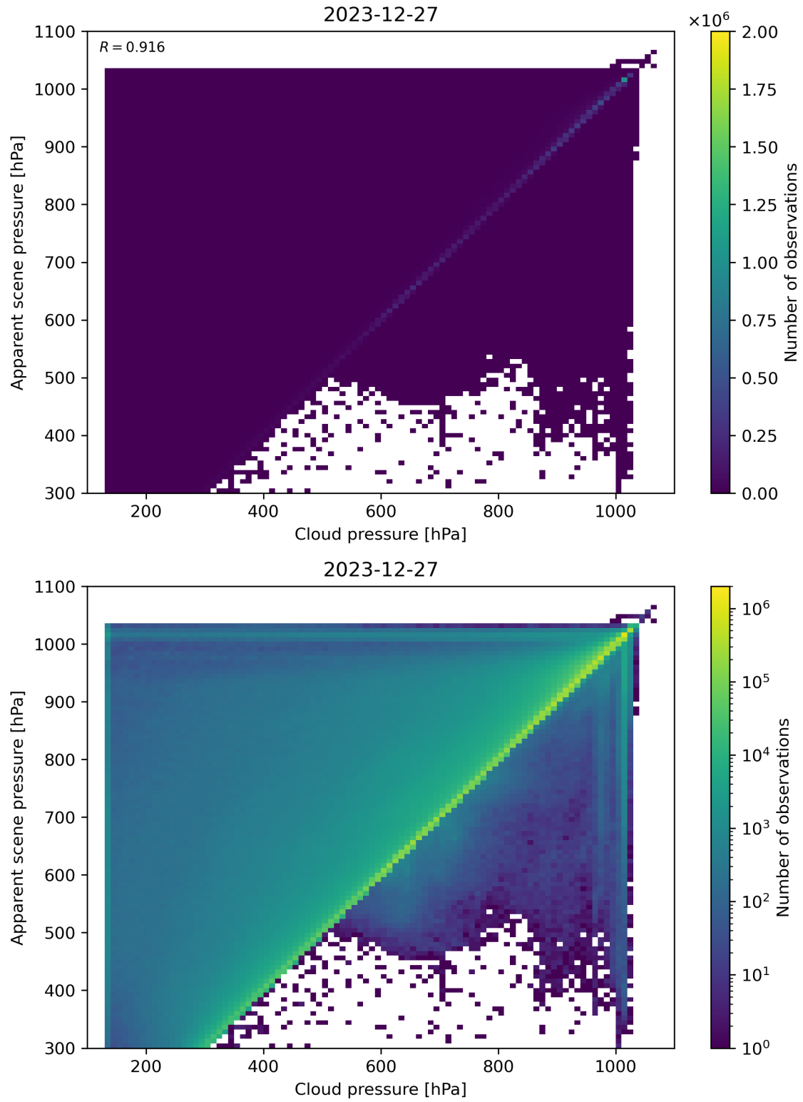
Figure 77: Scatter density plot of “Cloud pressure” against “Apparent scene pressure” for 2023-12-26 to 2023-12-28.
