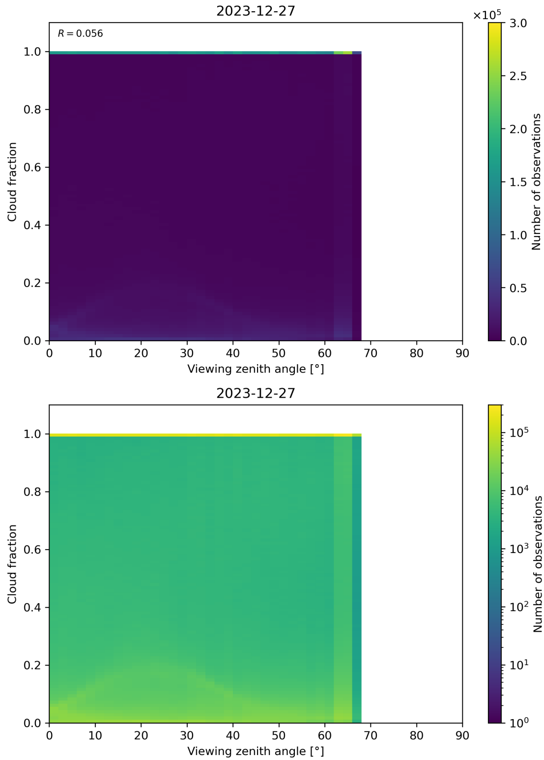
Figure 120: Scatter density plot of “Viewing zenith angle” against “Cloud fraction” for 2023-12-26 to 2023-12-28.
