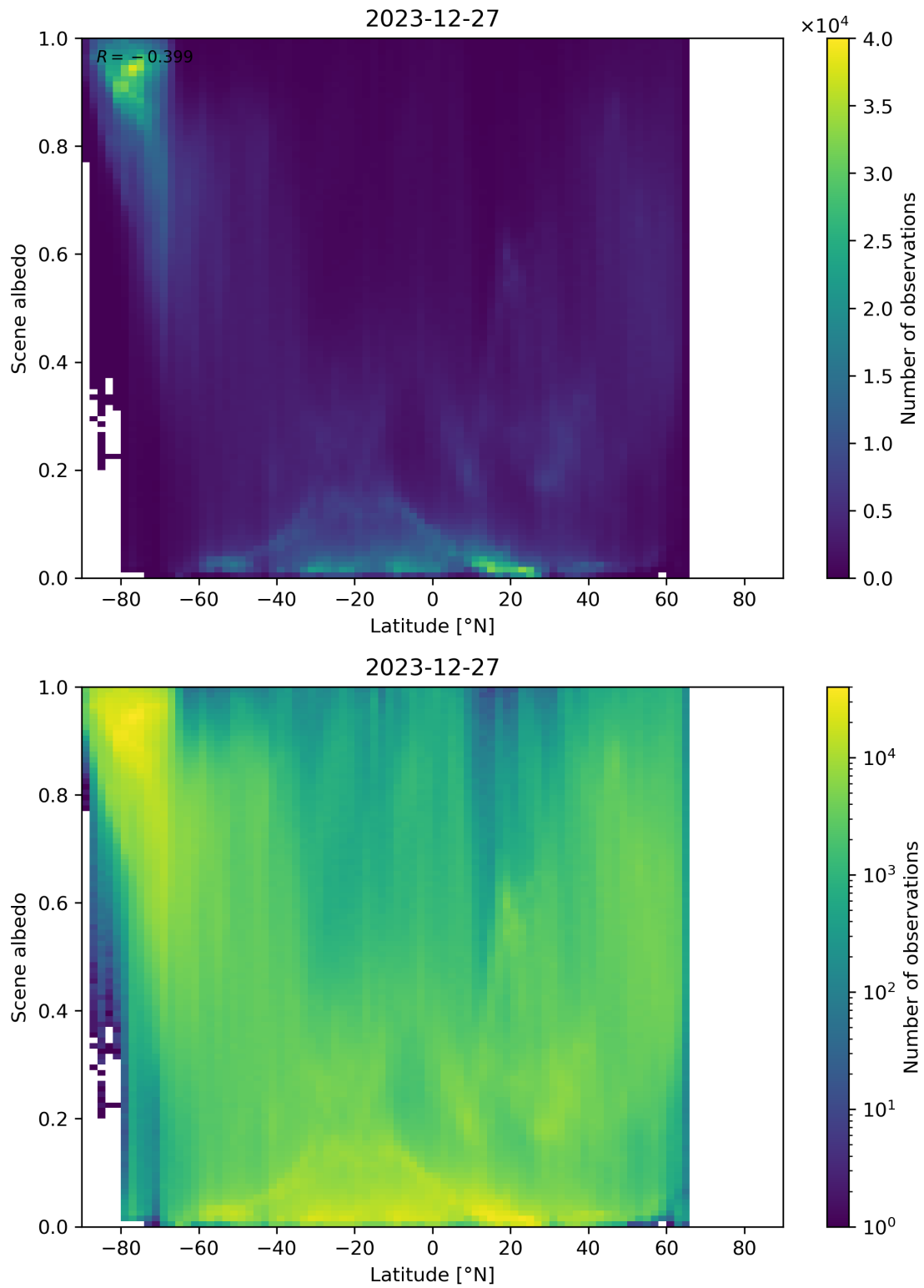
Figure 95: Scatter density plot of “Latitude” against “Scene albedo” for 2023-12-26 to 2023-12-28.
