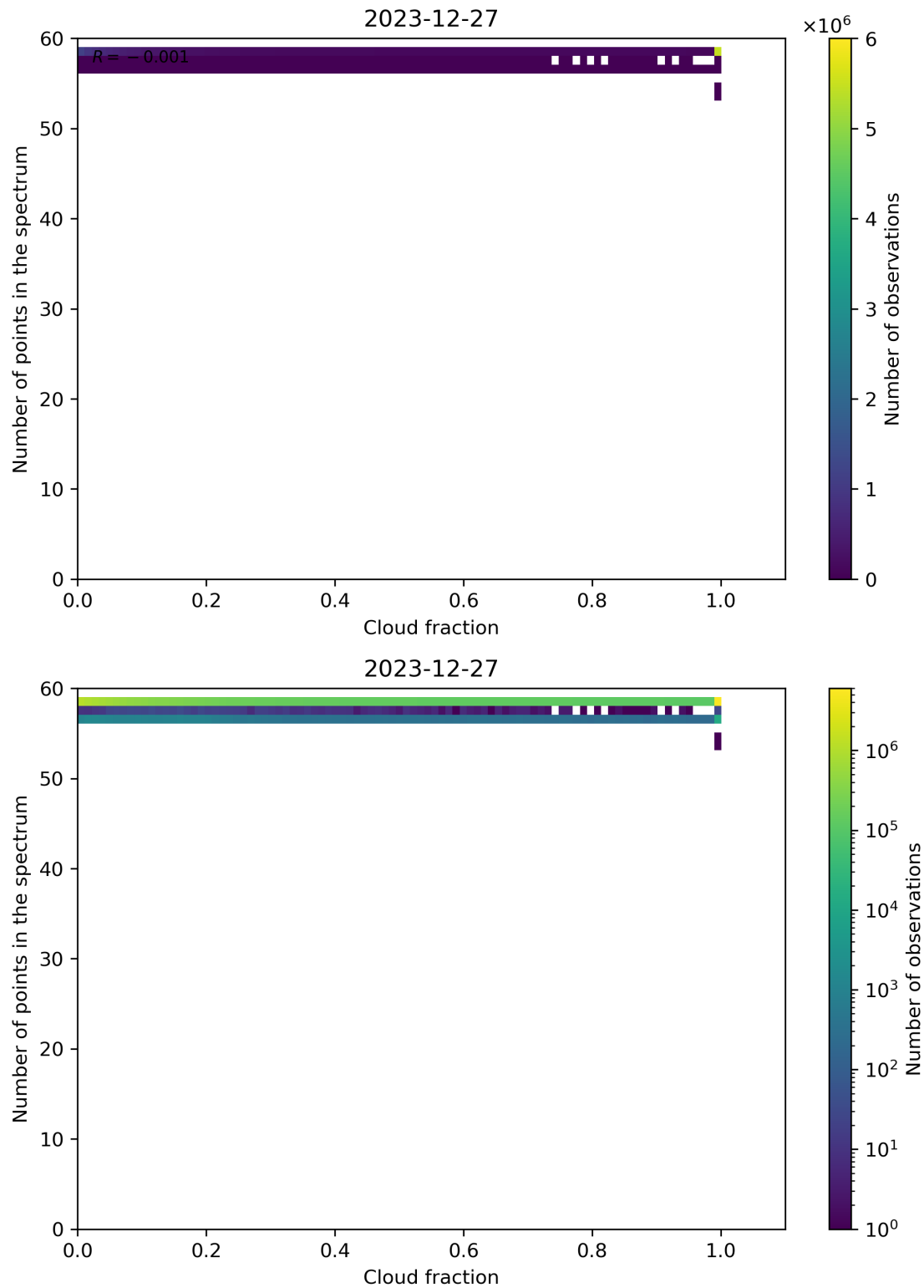
Figure 74: Scatter density plot of “Cloud fraction” against “Number of points in the spectrum” for 2023-12-26 to 2023-12-28.
