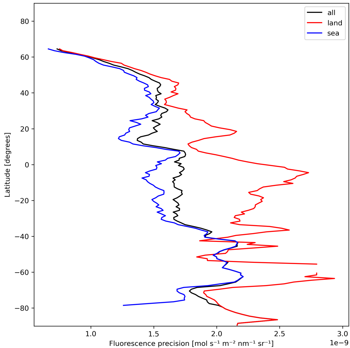
Figure 24: Zonal average of “Fluorescence precision” for 2023-12-26 to 2023-12-28.
