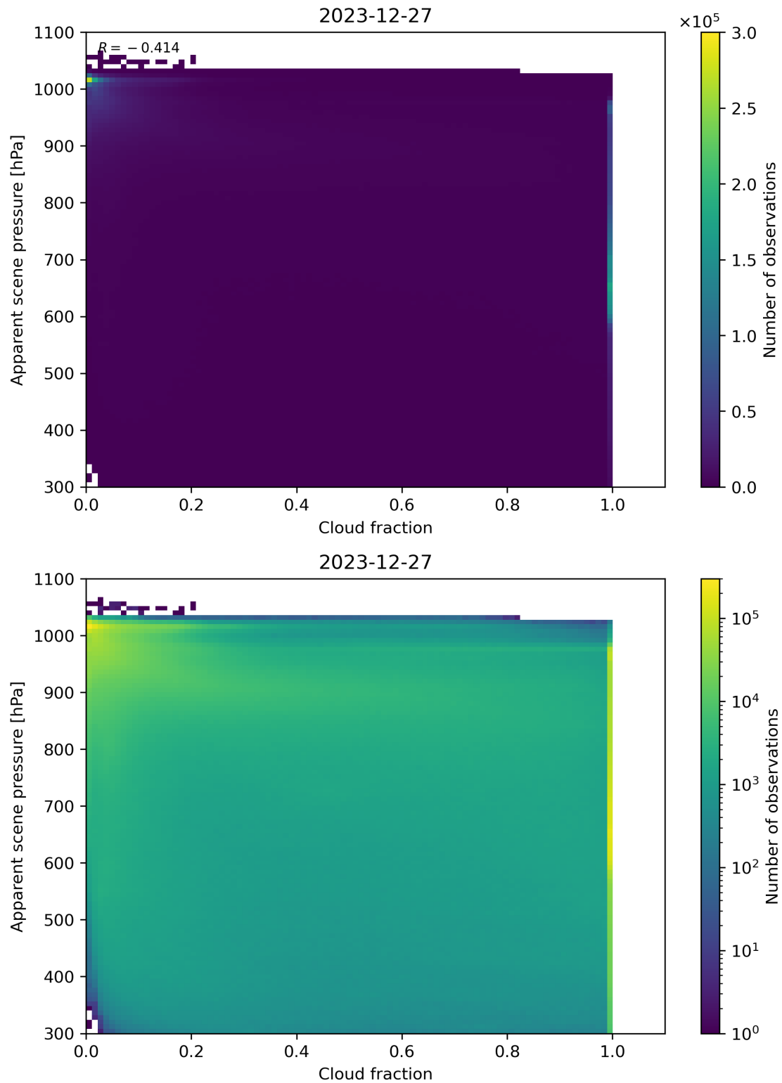
Figure 70: Scatter density plot of “Cloud fraction” against “Apparent scene pressure” for 2023-12-26 to 2023-12-28.
