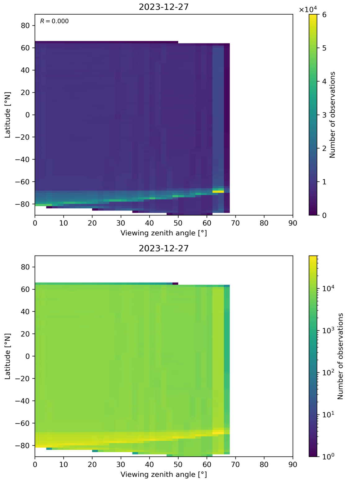
Figure 123: Scatter density plot of “Viewing zenith angle” against “Latitude” for 2023-12-26 to 2023-12-28.
