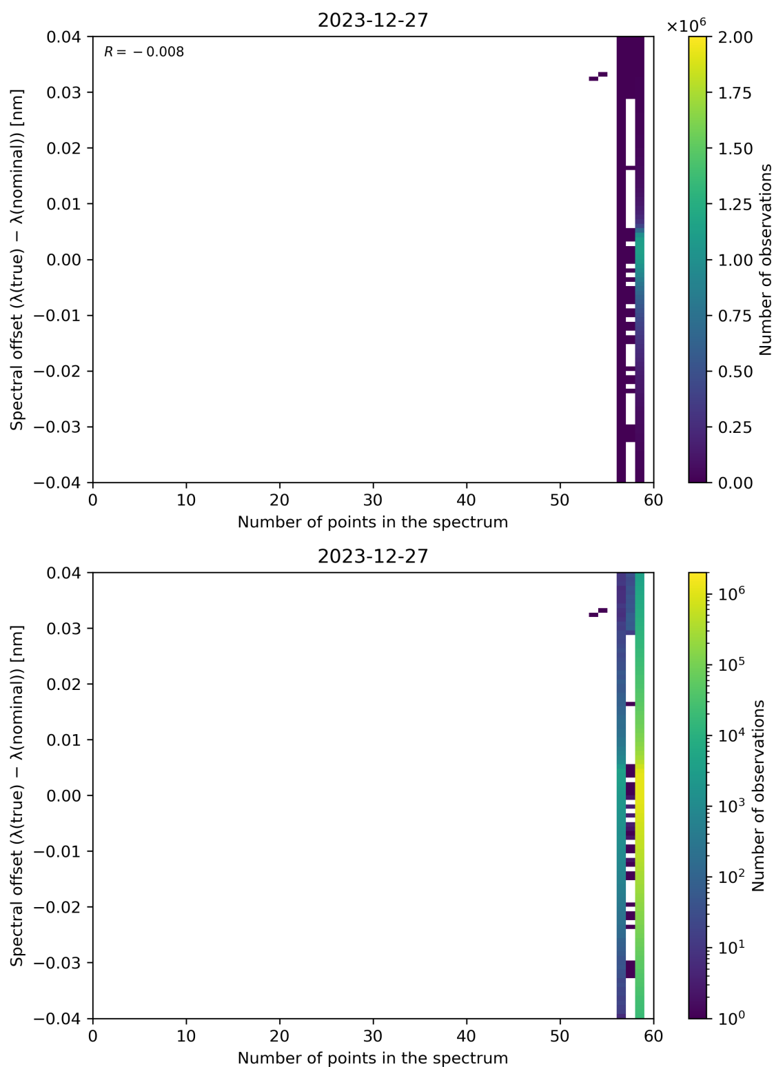
Figure 101: Scatter density plot of “Number of points in the spectrum” against “Spectral offset ( \lambda(\text{true}) - \lambda(\text{nominal}) )” for 2023-12-26 to 2023-12-28.
