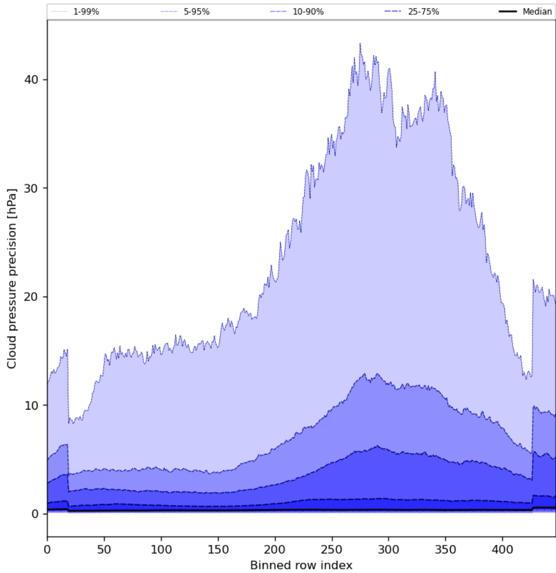
Figure 48: Along track statistics of “Cloud pressure precision” for 2023-12-26 to 2023-12-28
