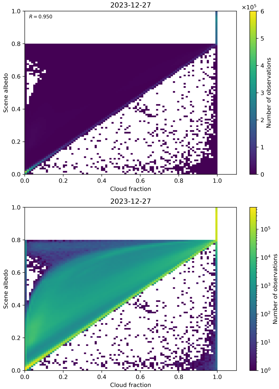
Figure 75: Scatter density plot of “Cloud fraction” against “Scene albedo” for 2023-12-26 to 2023-12-28.
