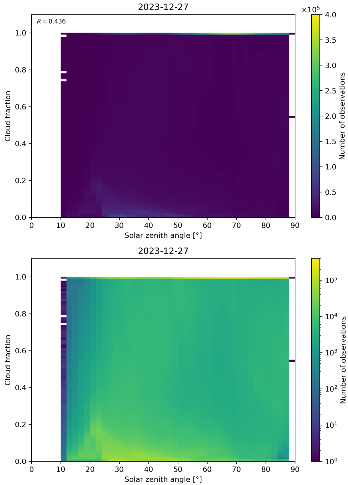
Figure 110: Scatter density plot of “Solar zenith angle” against “Cloud fraction” for 2023-12-26 to 2023-12-28.
