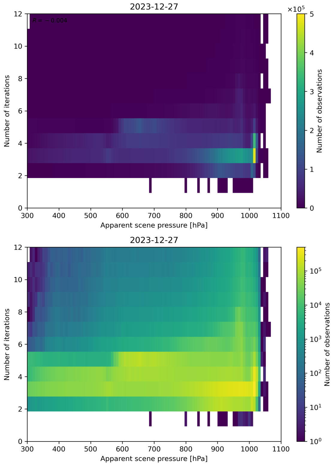
Figure 65: Scatter density plot of “Apparent scene pressure” against “Number of iterations” for 2023-12-26 to 2023-12-28.
