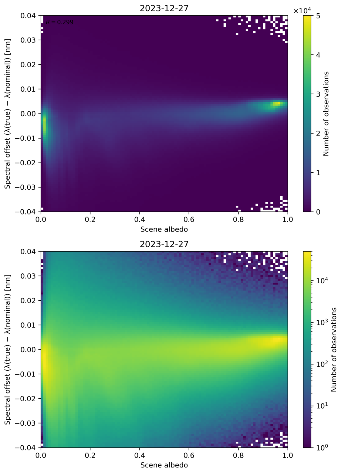
Figure 107: Scatter density plot of “Scene albedo” against “Spectral offset ( \lambda(\text{true}) - \lambda(\text{nominal}) )” for 2023-12-26 to 2023-12-28.
