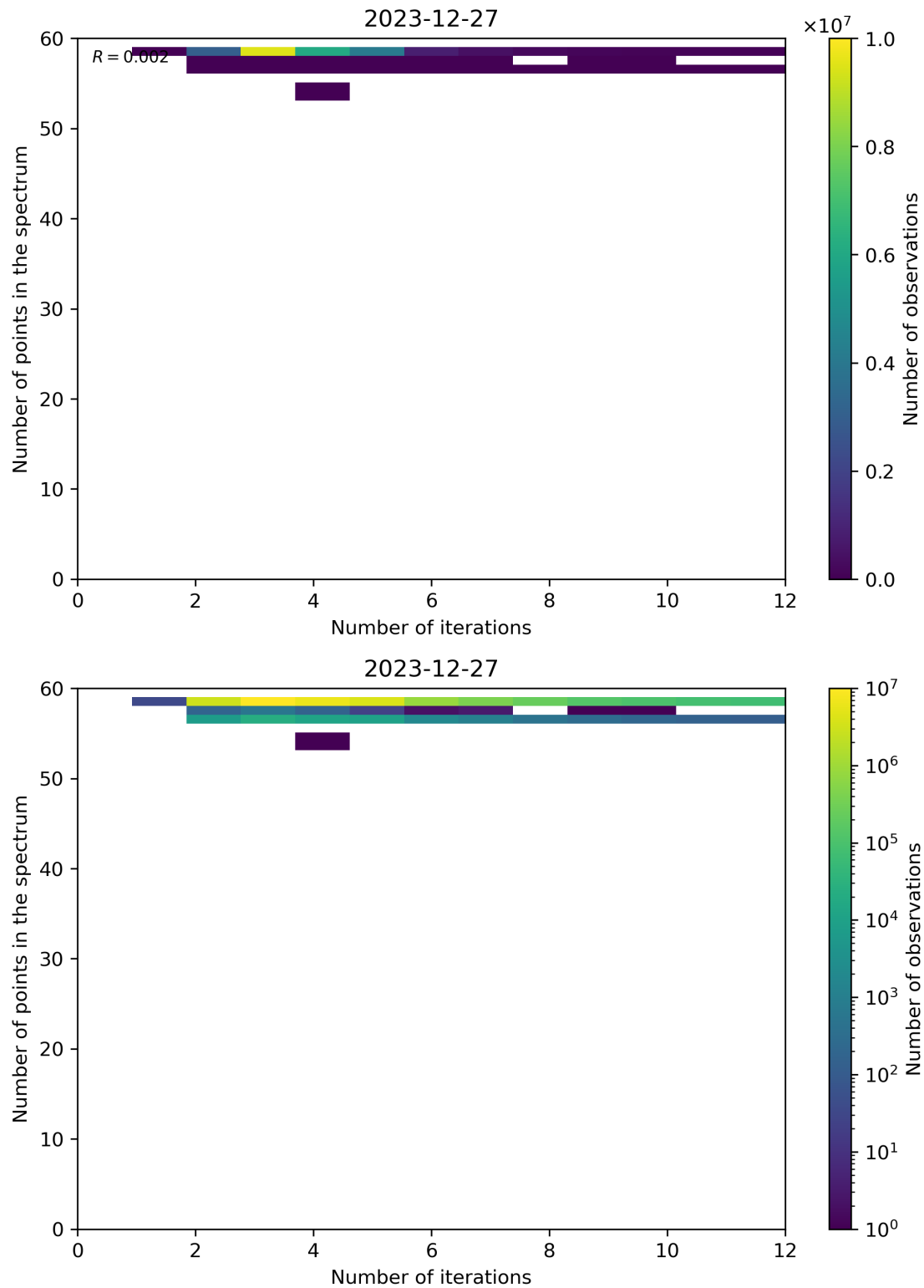
Figure 99: Scatter density plot of “Number of iterations” against “Number of points in the spectrum” for 2023-12-26 to 2023-12-28.
