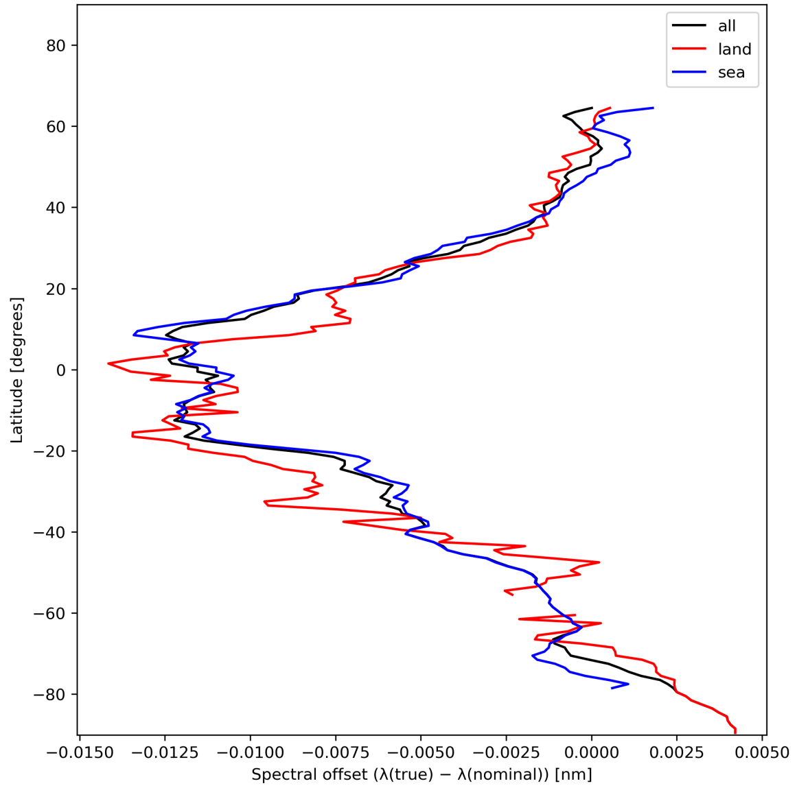
Figure 28: Zonal average of “Spectral offset ( \lambda(\text{true}) - \lambda(\text{nominal}) )” for 2023-12-26 to 2023-12-28.
