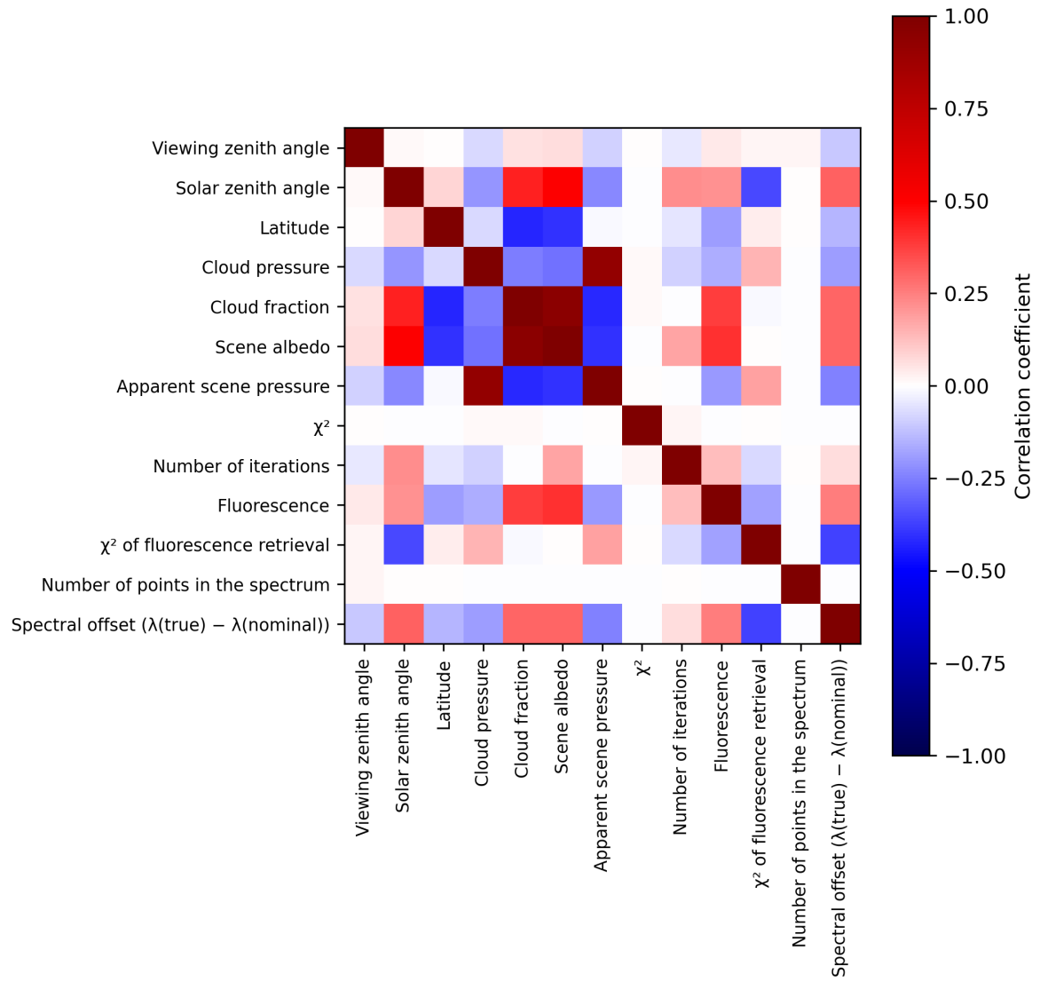
Figure 2: Map of correlation matrix for 2023-12-26 to 2023-12-28.
