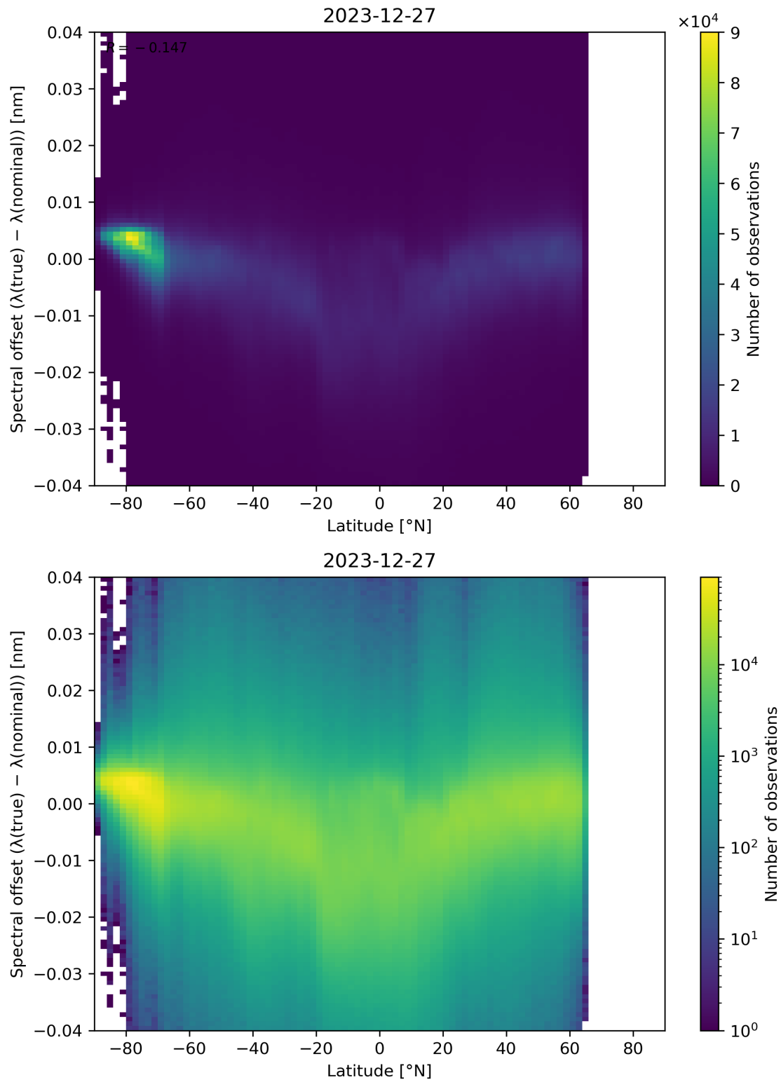
Figure 96: Scatter density plot of “Latitude” against “Spectral offset ( \lambda(\text{true}) - \lambda(\text{nominal}) )” for 2023-12-26 to 2023-12-28.
