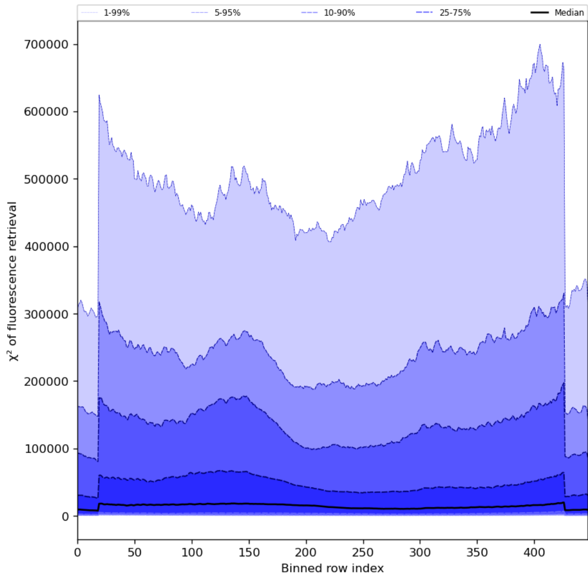
Figure 59: Along track statistics of “ \chi^2 of fluorescence retrieval” for 2023-12-26 to 2023-12-28
