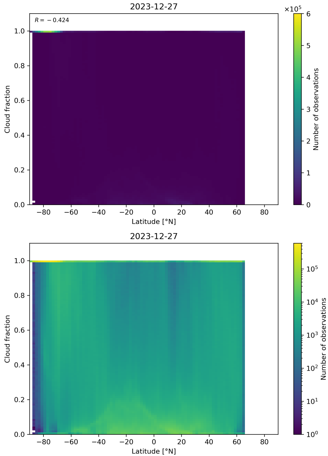
Figure 90: Scatter density plot of “Latitude” against “Cloud fraction” for 2023-12-26 to 2023-12-28.
