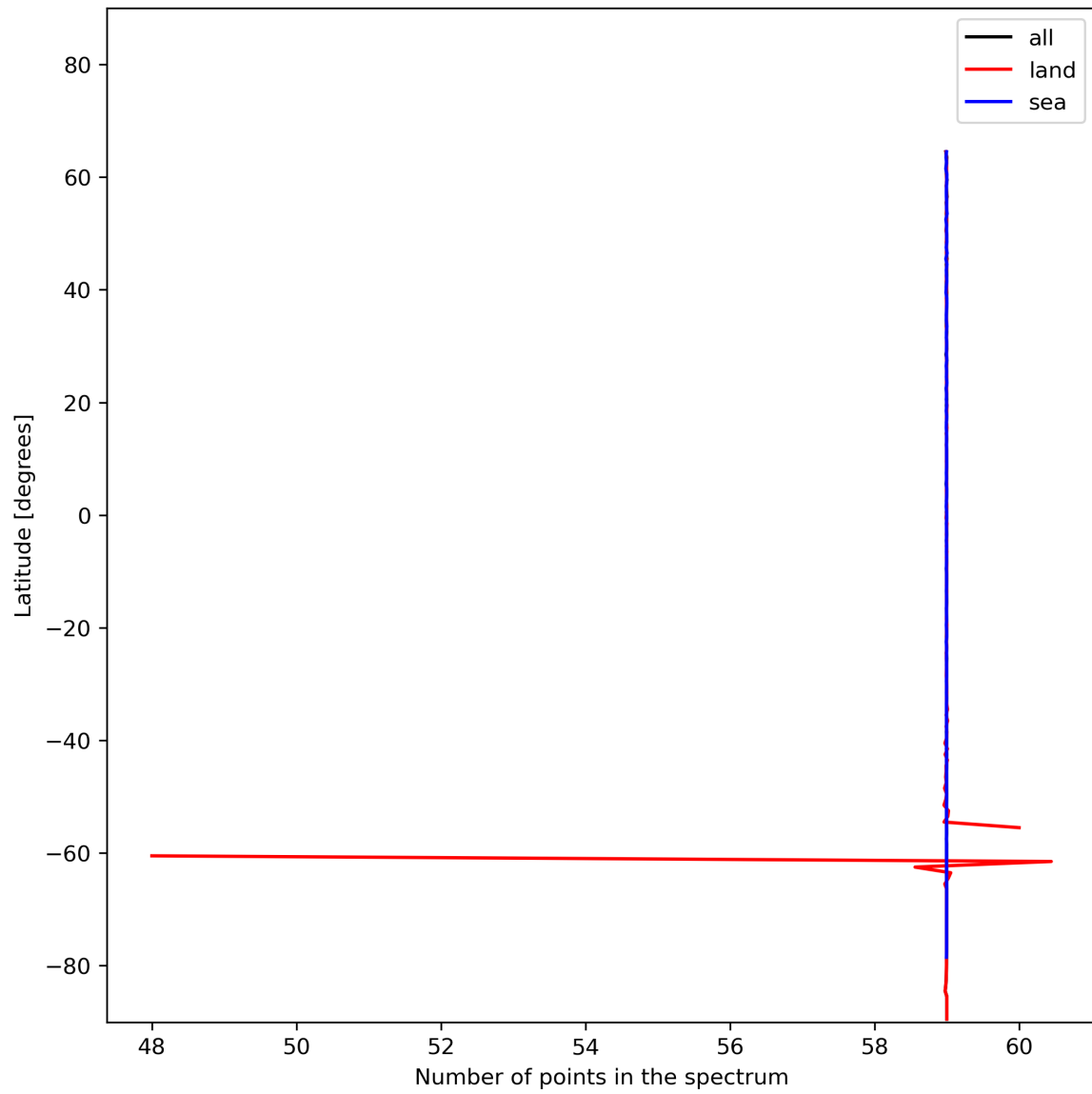
Figure 27: Zonal average of “Number of points in the spectrum” for 2023-12-26 to 2023-12-28.
