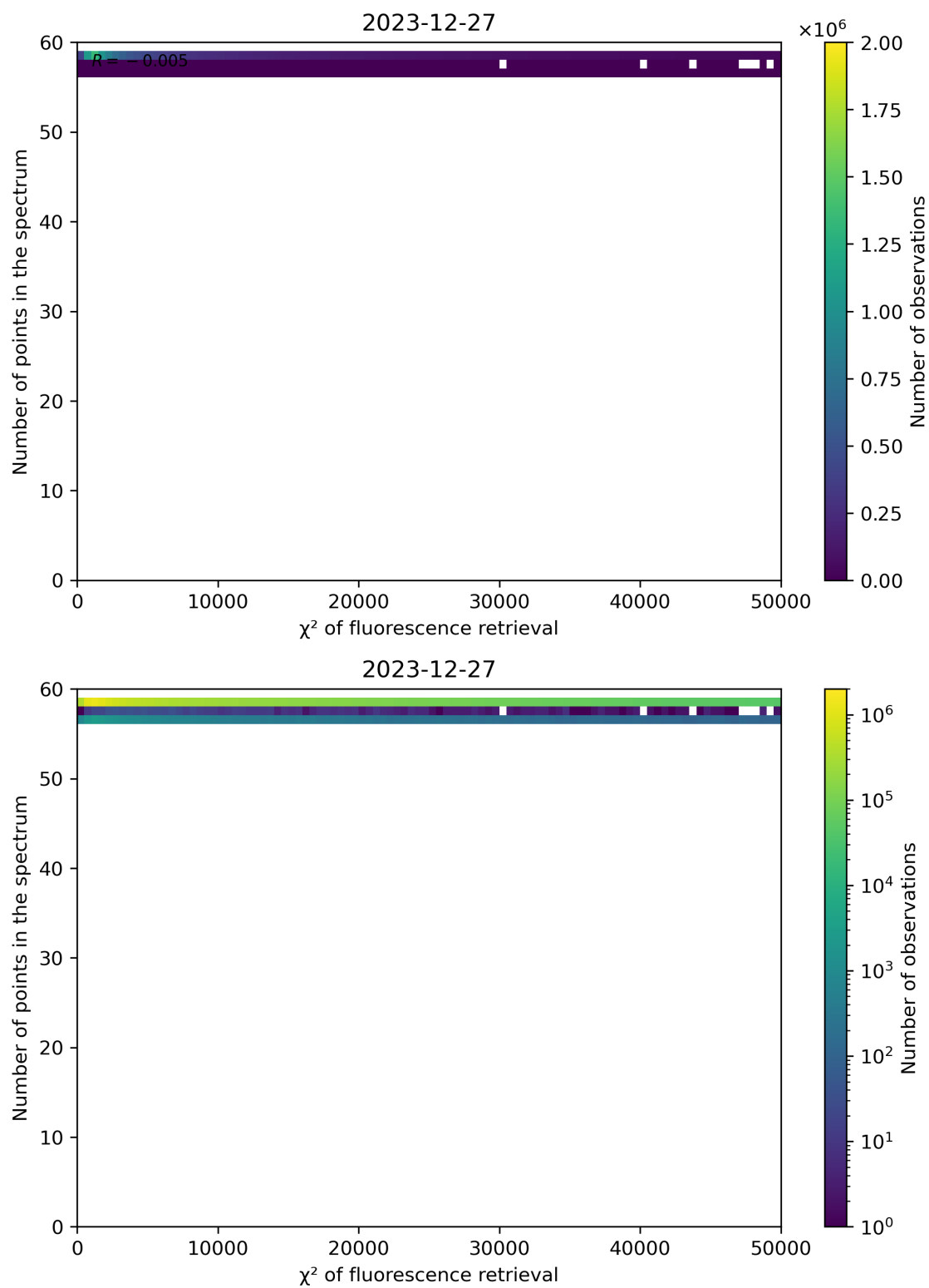
Figure 68: Scatter density plot of “ \chi^2 of fluorescence retrieval” against “Number of points in the spectrum” for 2023-12-26 to 2023-12-28.
