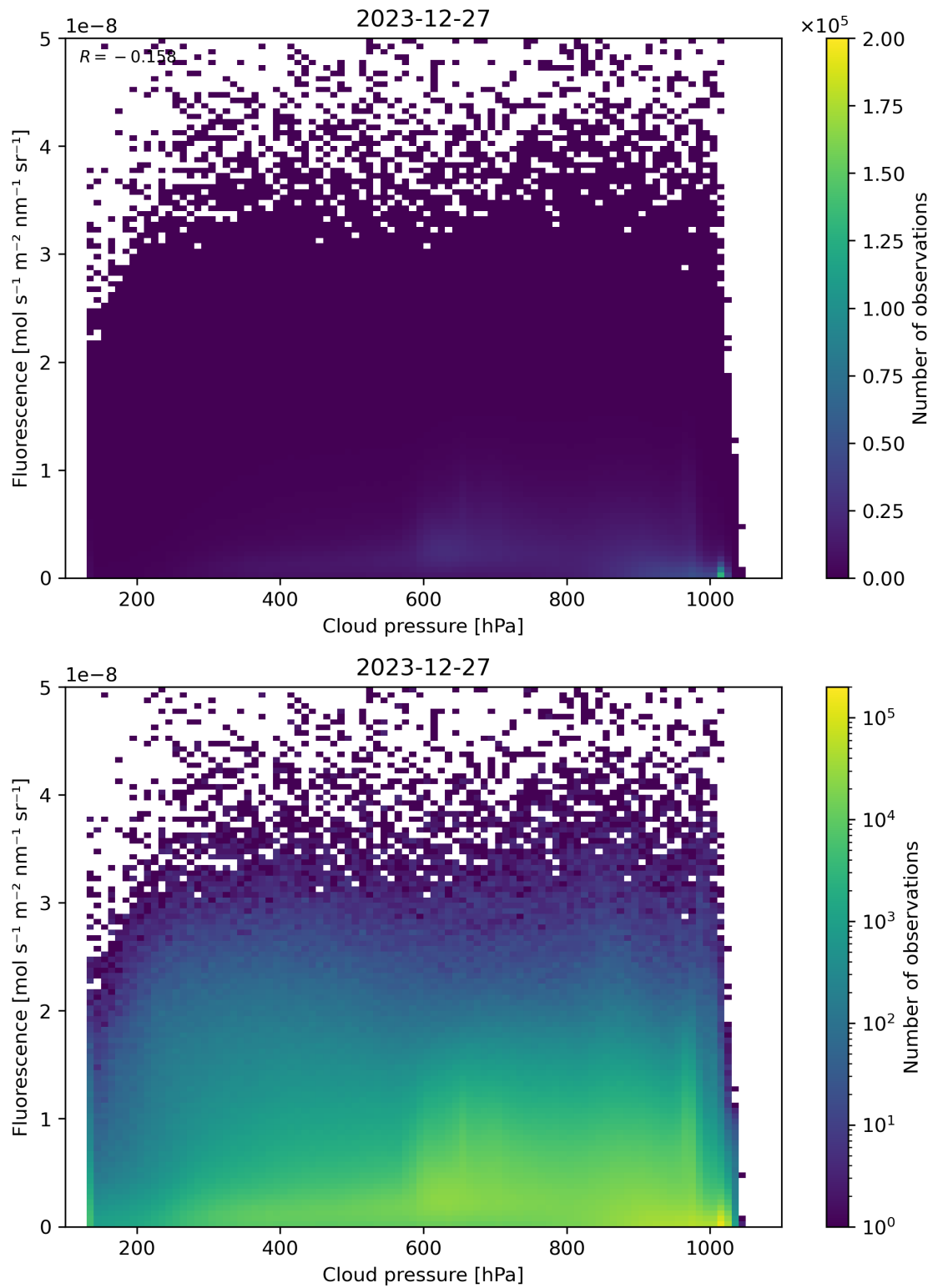
Figure 80: Scatter density plot of “Cloud pressure” against “Fluorescence” for 2023-12-26 to 2023-12-28.
