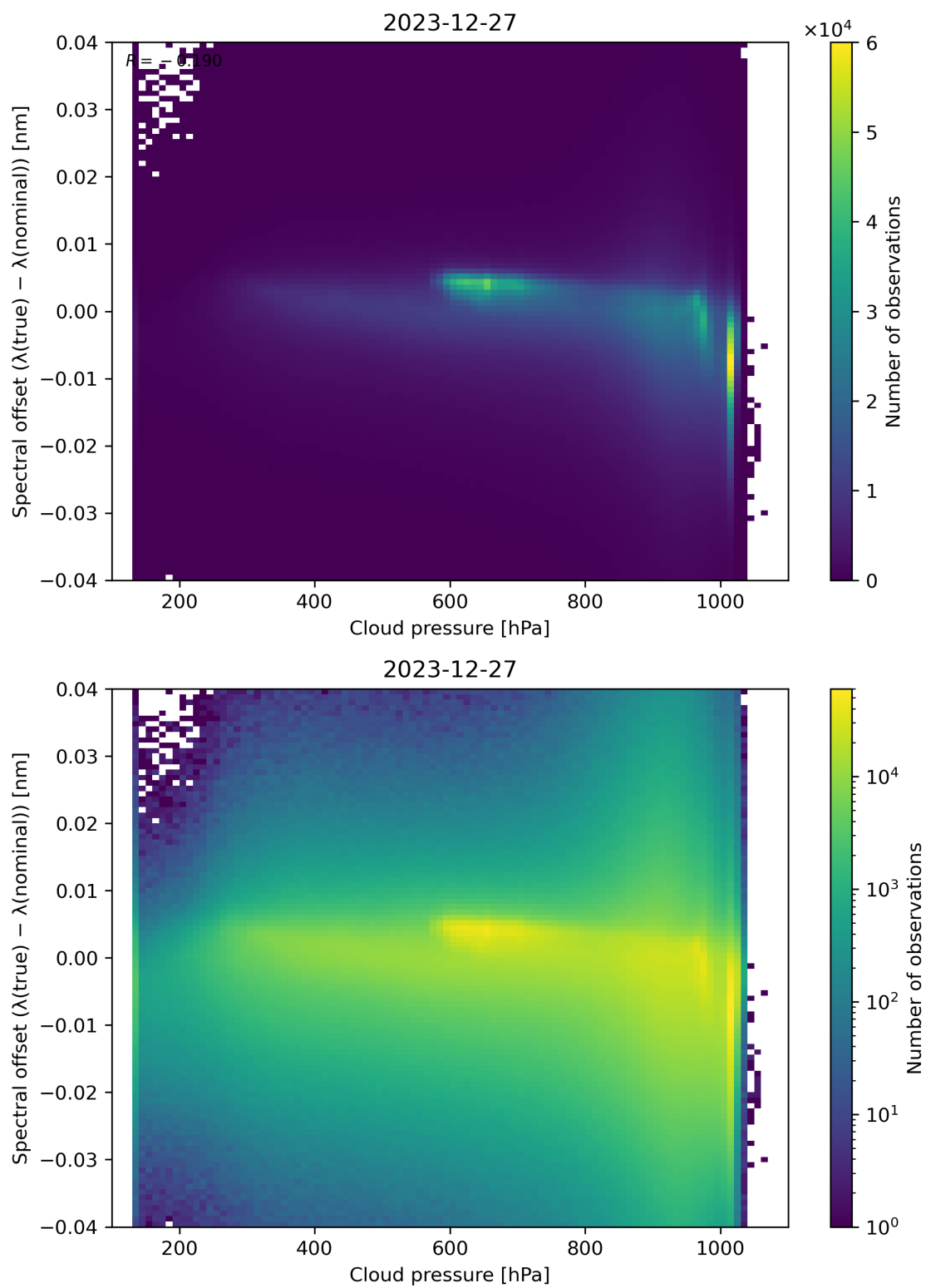
Figure 84: Scatter density plot of “Cloud pressure” against “Spectral offset ( \lambda(\text{true}) - \lambda(\text{nominal}) )” for 2023-12-26 to 2023-12-28.
