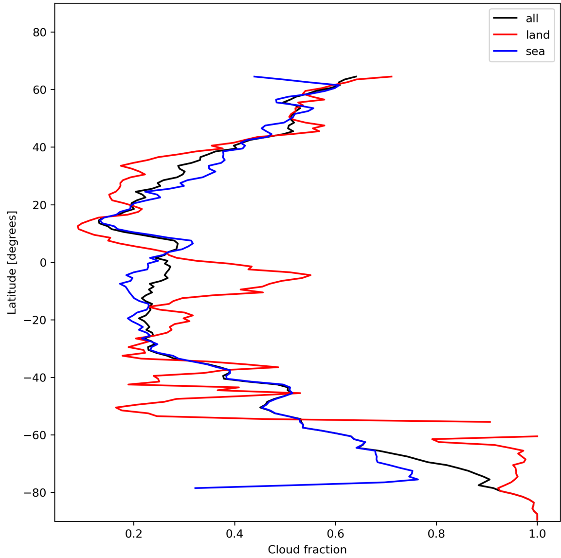
Figure 15: Zonal average of “Cloud fraction” for 2023-12-26 to 2023-12-28.
