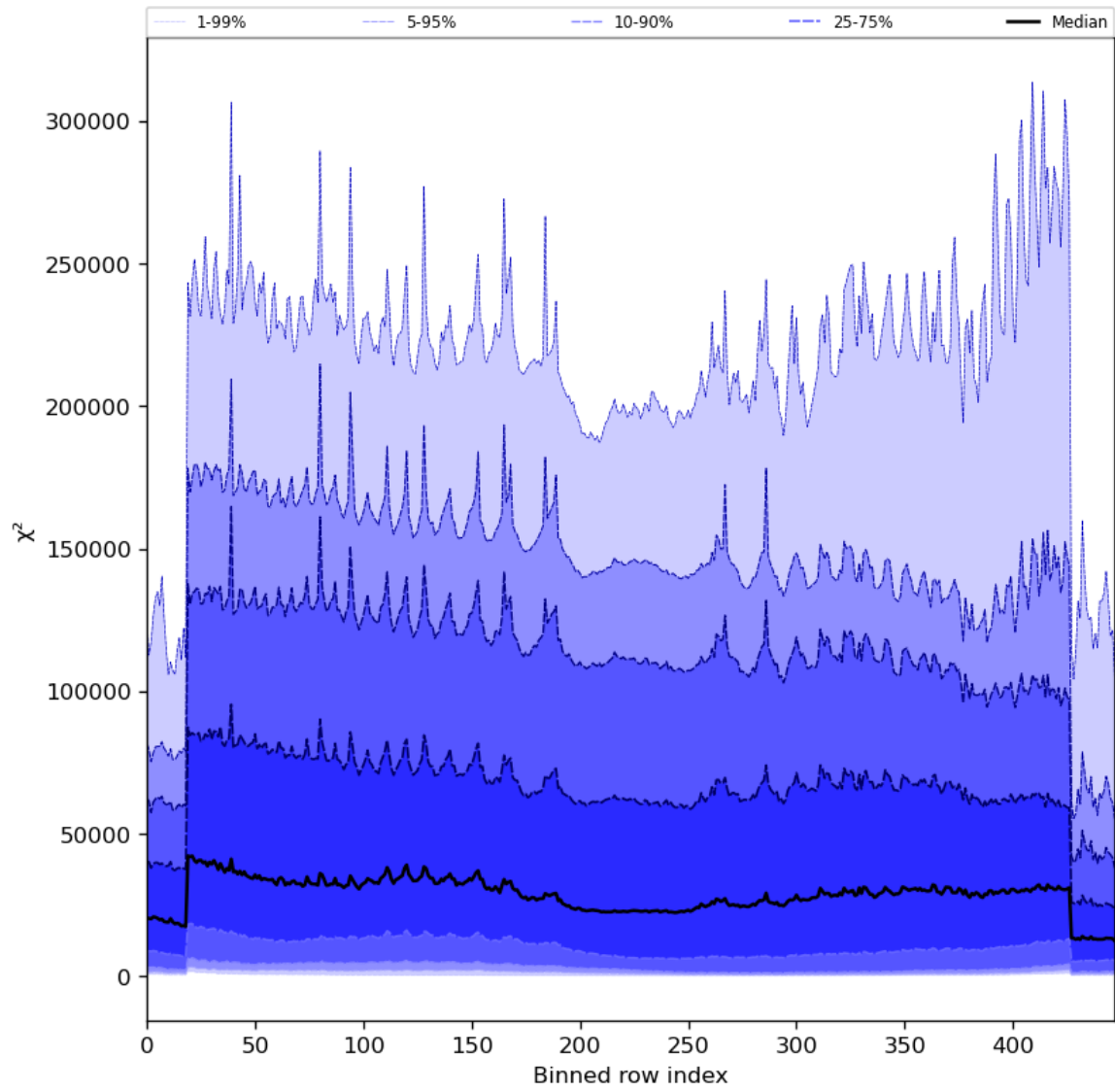
Figure 55: Along track statistics of “ \chi^2 ” for 2023-12-26 to 2023-12-28
