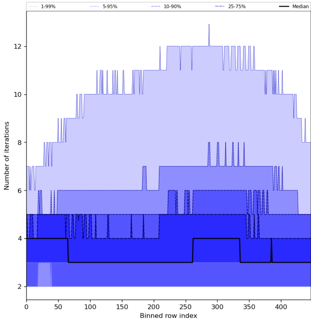
Figure 56: Along track statistics of “Number of iterations” for 2023-12-26 to 2023-12-28
