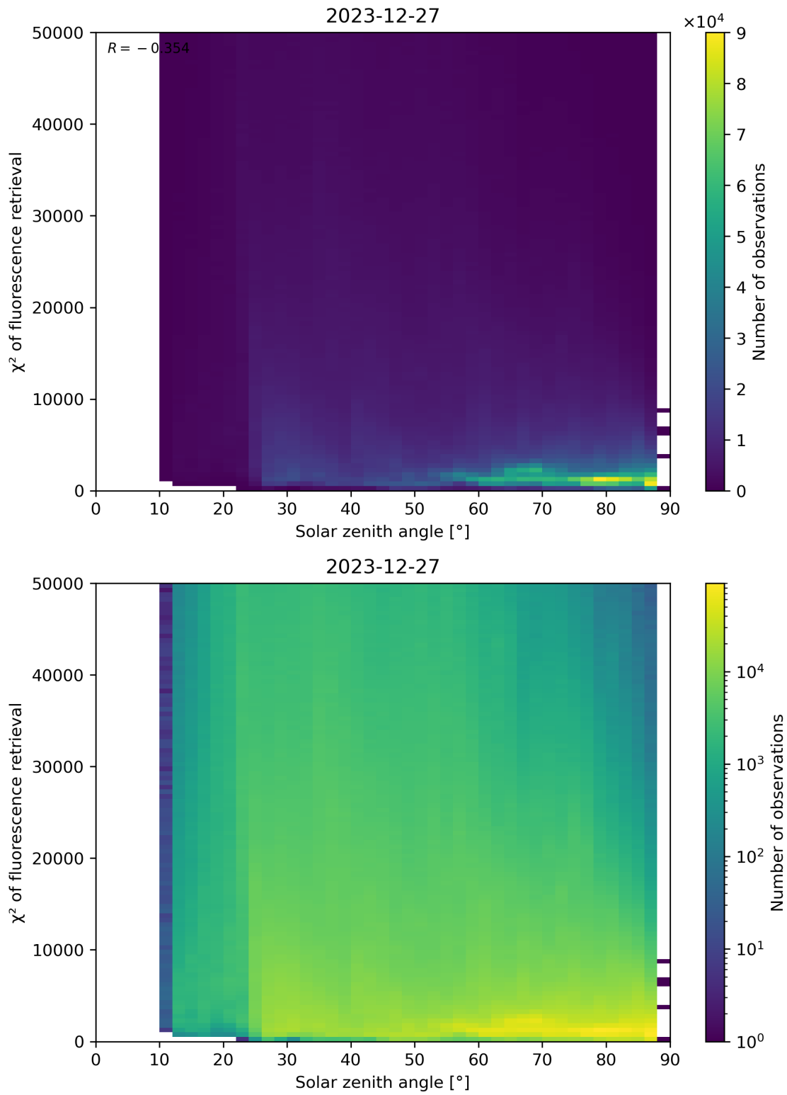
Figure 109: Scatter density plot of “Solar zenith angle” against “ \chi^2 of fluorescence retrieval” for 2023-12-26 to 2023-12-28.
