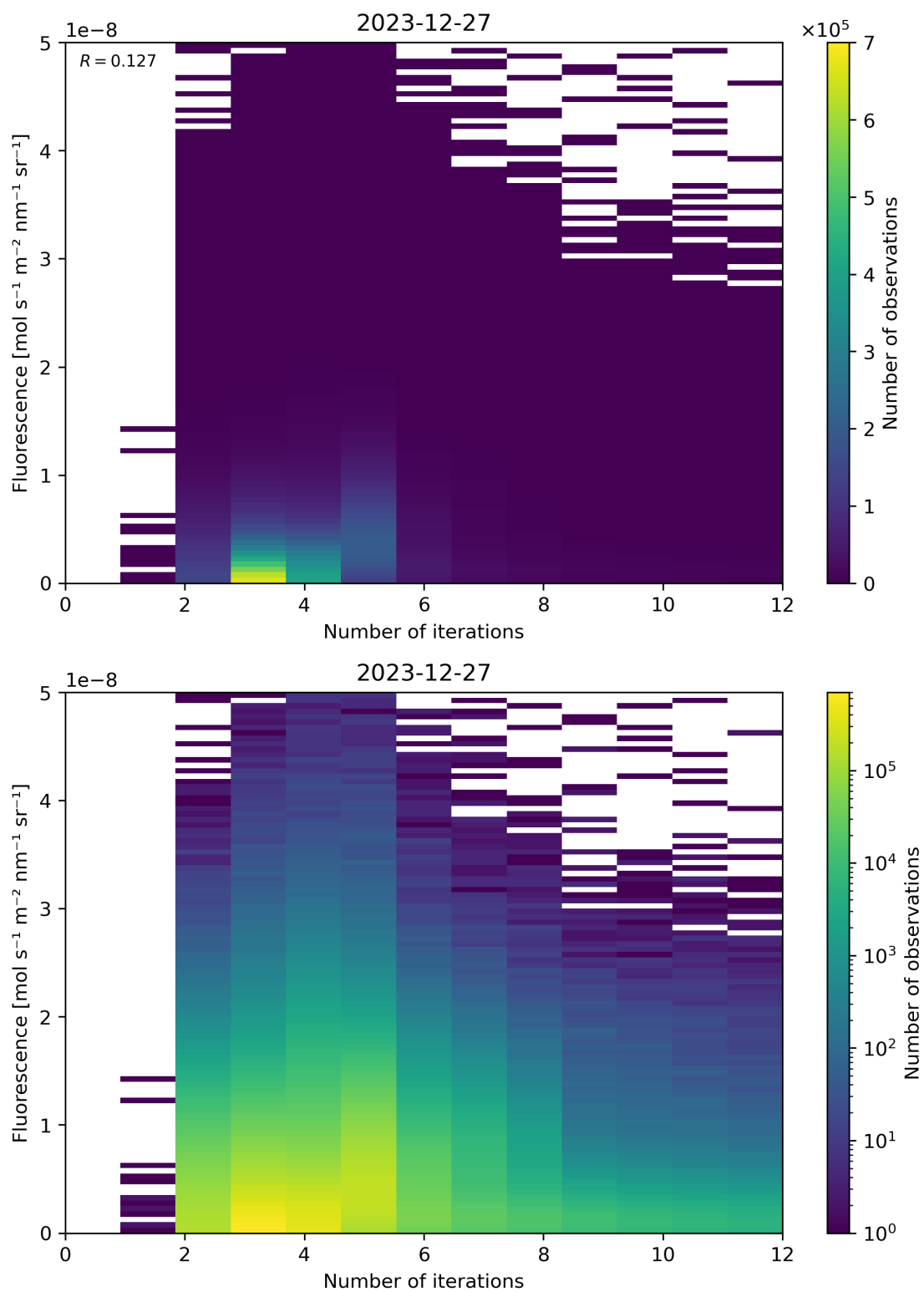
Figure 98: Scatter density plot of “Number of iterations” against “Fluorescence” for 2023-12-26 to 2023-12-28.
