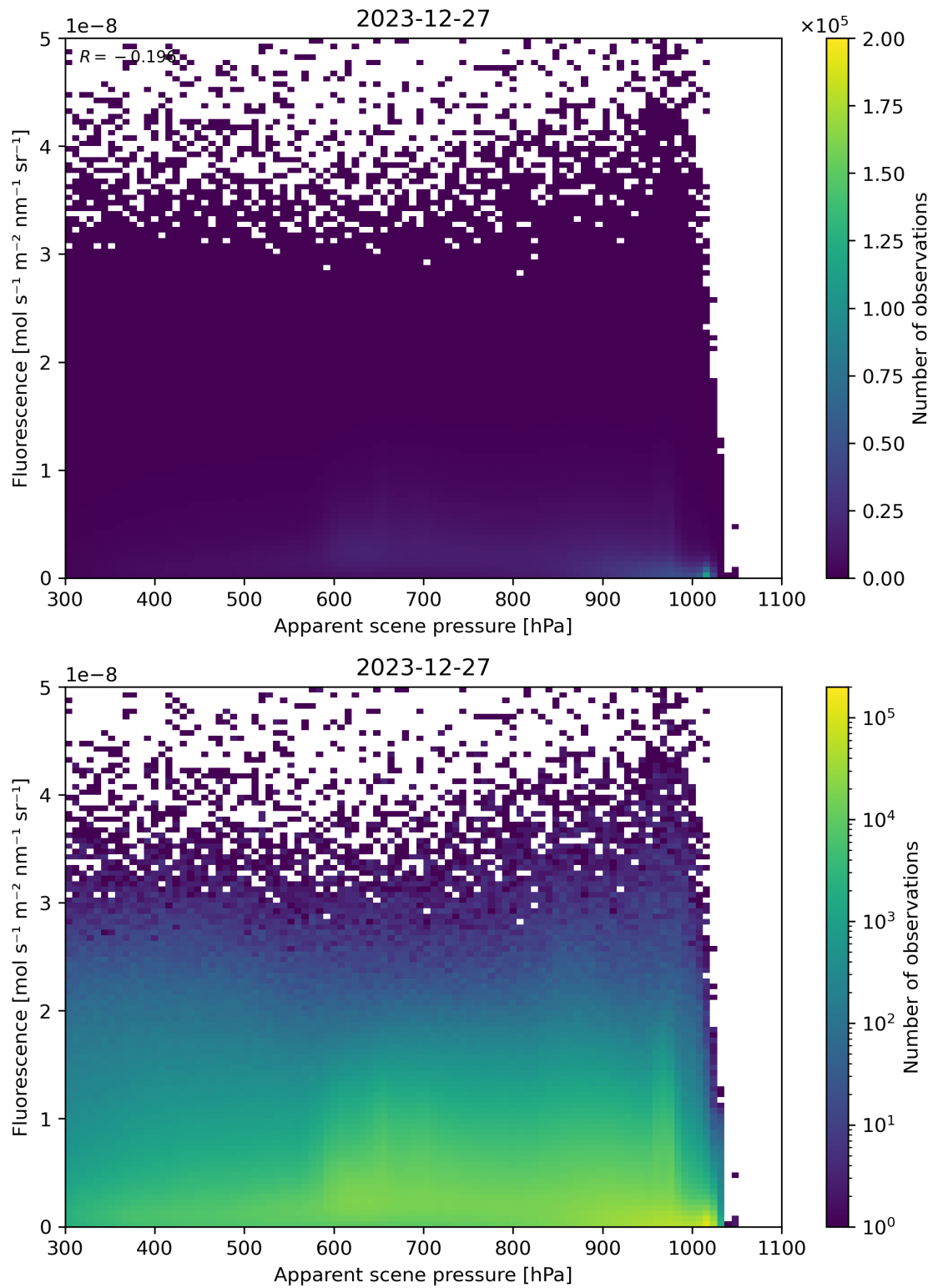
Figure 64: Scatter density plot of “Apparent scene pressure” against “Fluorescence” for 2023-12-26 to 2023-12-28.
