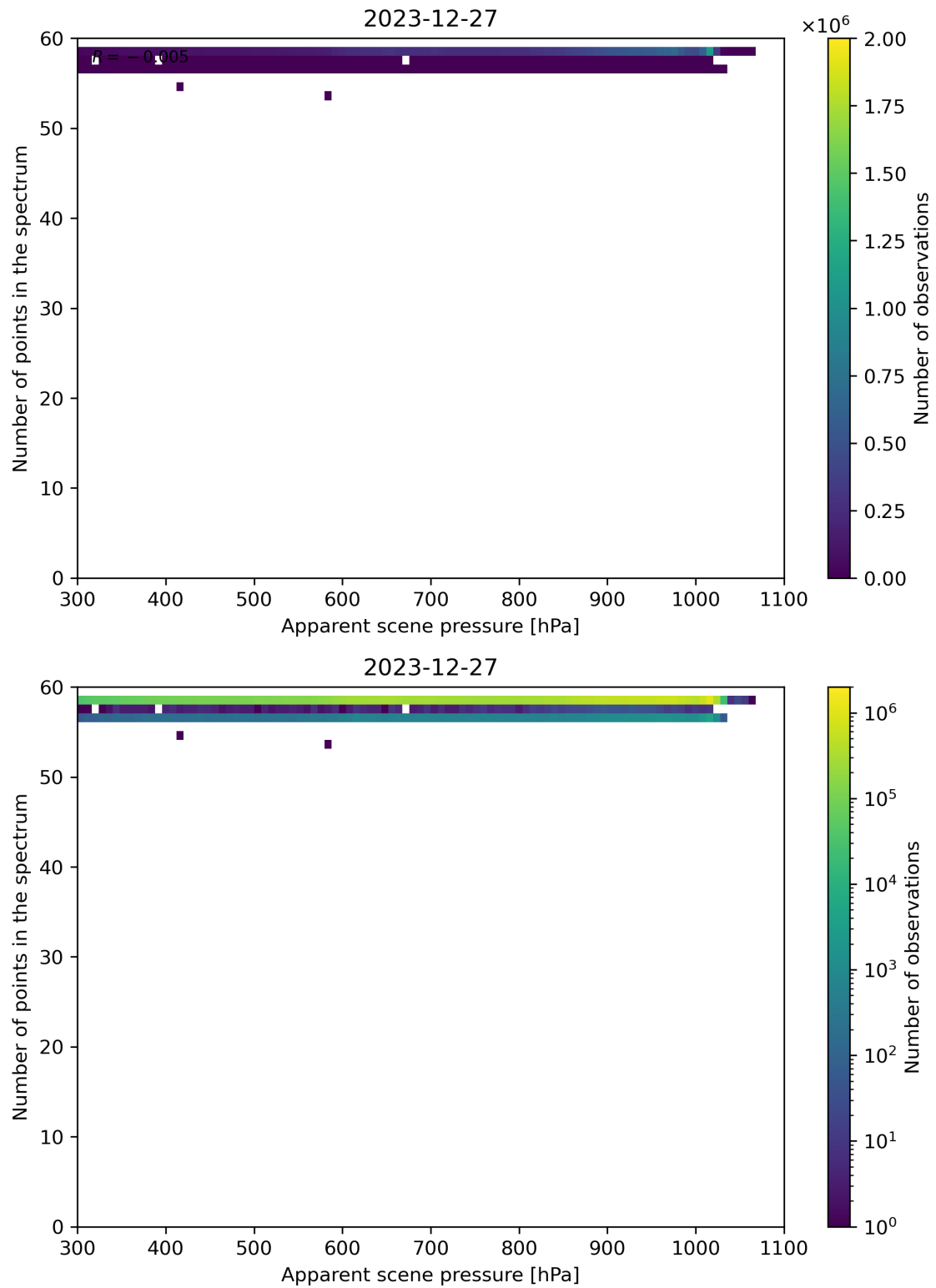
Figure 66: Scatter density plot of “Apparent scene pressure” against “Number of points in the spectrum” for 2023-12-26 to 2023-12-28.
