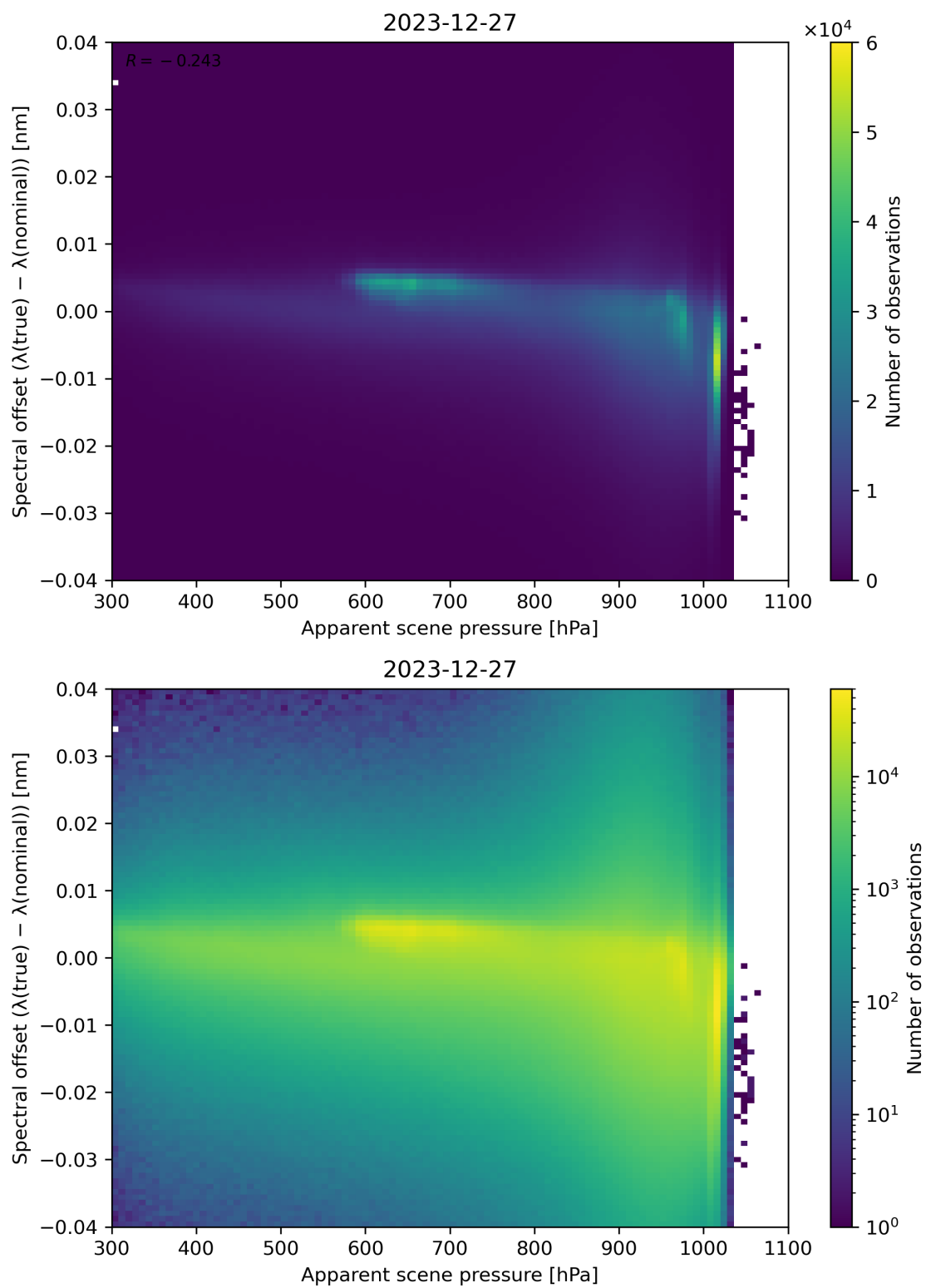
Figure 67: Scatter density plot of “Apparent scene pressure” against “Spectral offset ( \lambda(\text{true}) - \lambda(\text{nominal}) )” for 2023-12-26 to 2023-12-28.
