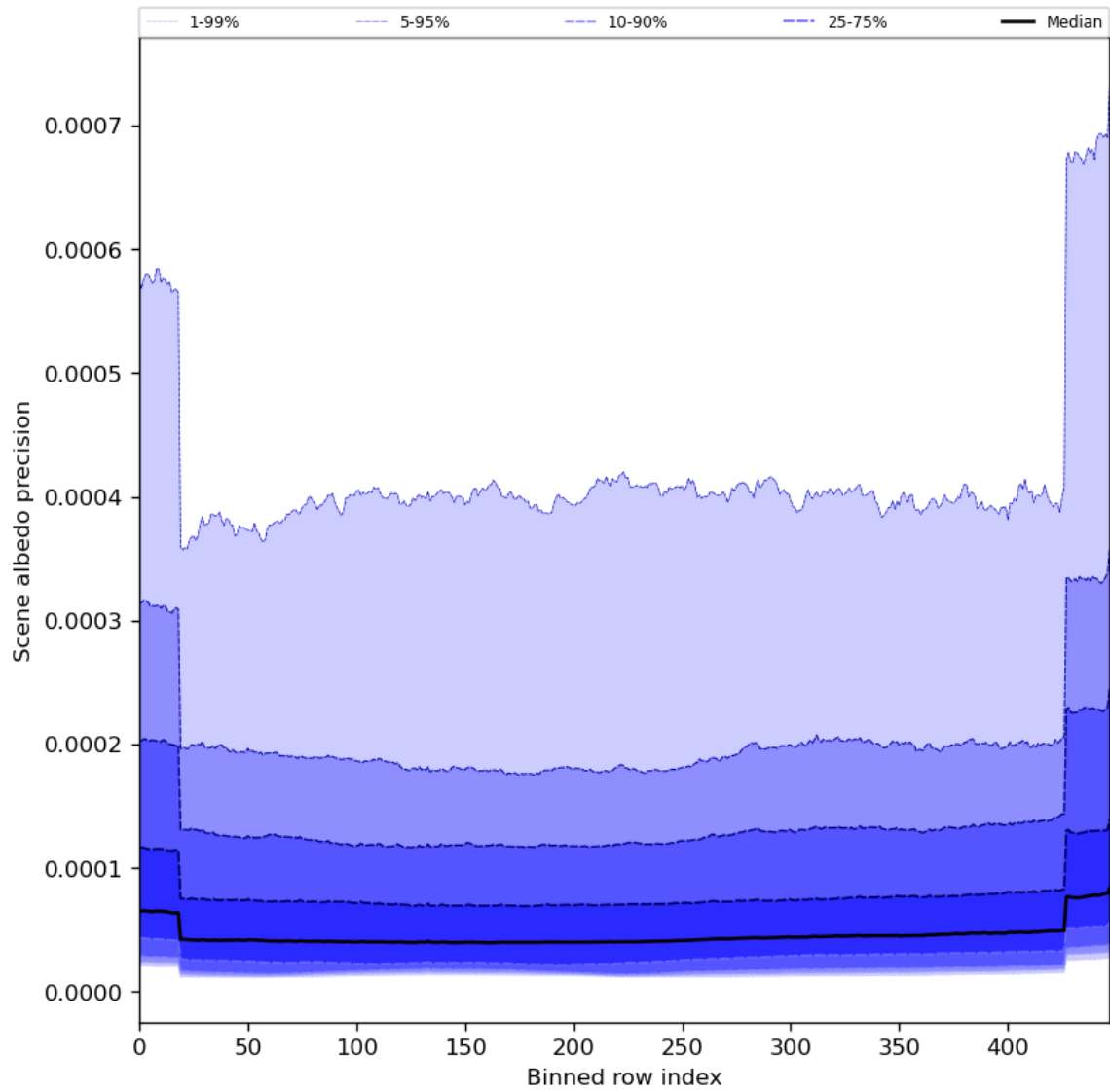
Figure 52: Along track statistics of “Scene albedo precision” for 2023-12-26 to 2023-12-28
