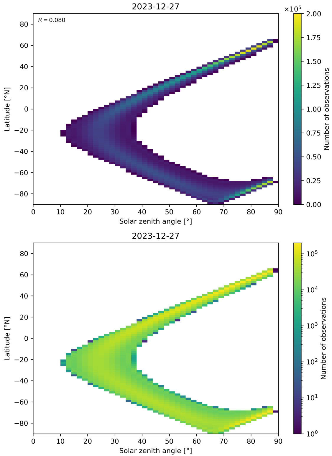
Figure 113: Scatter density plot of “Solar zenith angle” against “Latitude” for 2023-12-26 to 2023-12-28.
