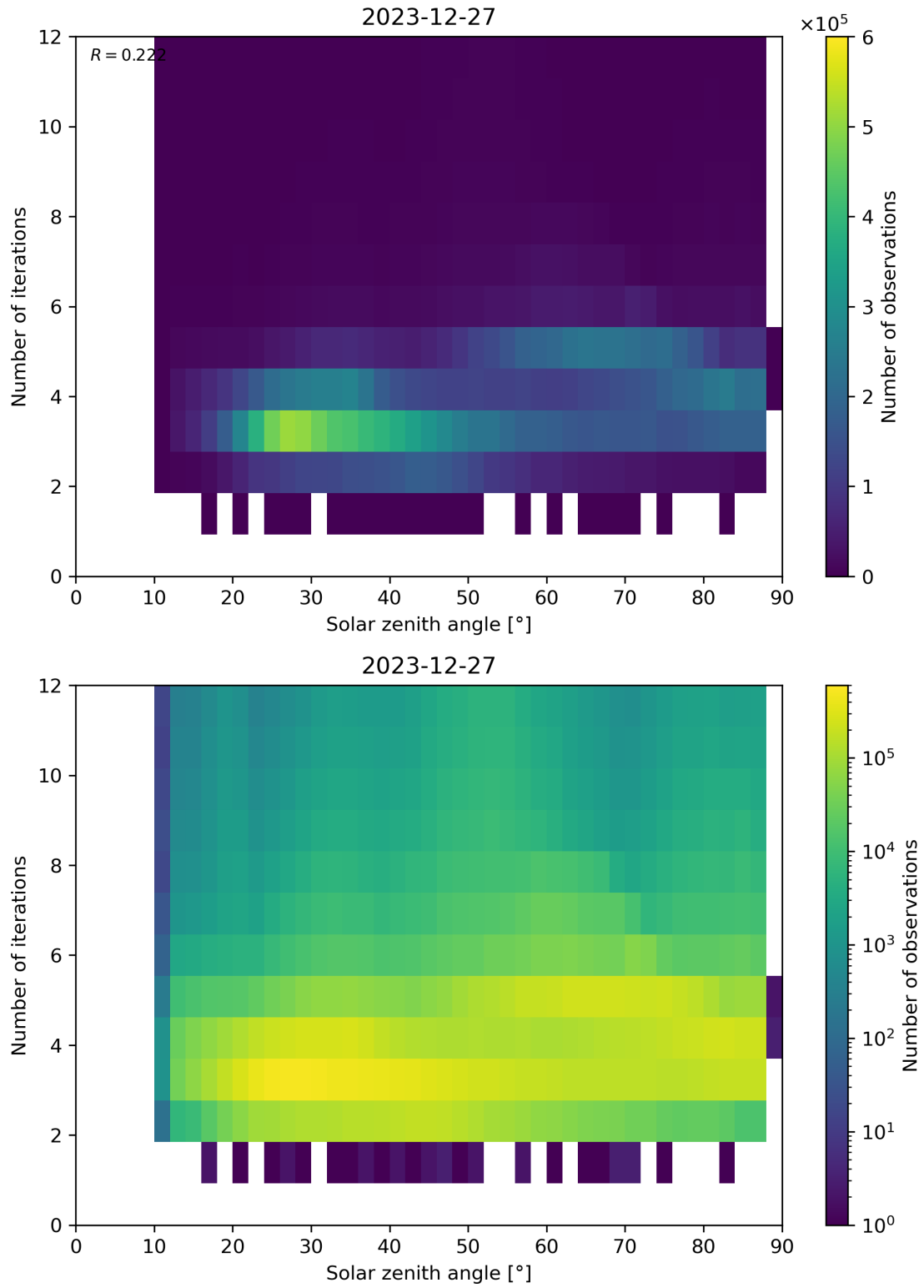
Figure 114: Scatter density plot of “Solar zenith angle” against “Number of iterations” for 2023-12-26 to 2023-12-28.
