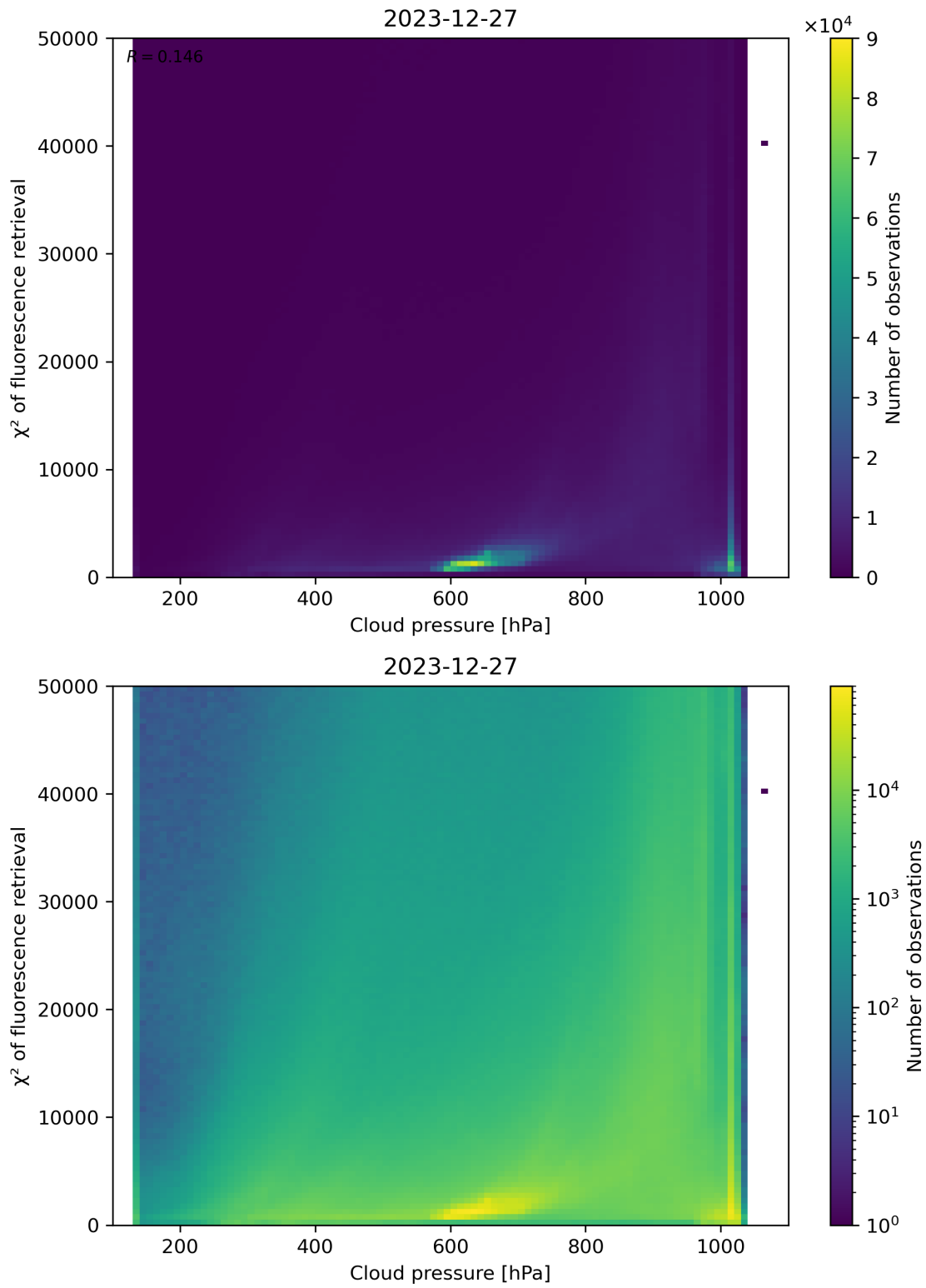
Figure 78: Scatter density plot of “Cloud pressure” against “ \chi^2 of fluorescence retrieval” for 2023-12-26 to 2023-12-28.
