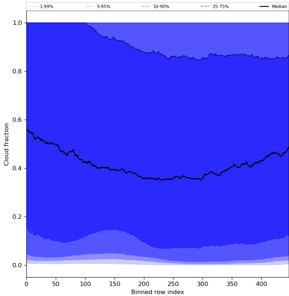
Figure 49: Along track statistics of “Cloud fraction” for 2023-12-26 to 2023-12-28
