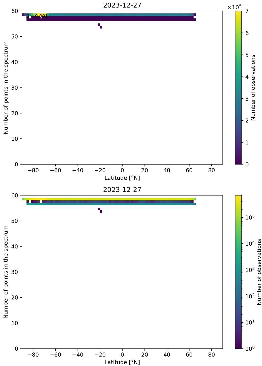
Figure 94: Scatter density plot of “Latitude” against “Number of points in the spectrum” for 2023-12-26 to 2023-12-28.
