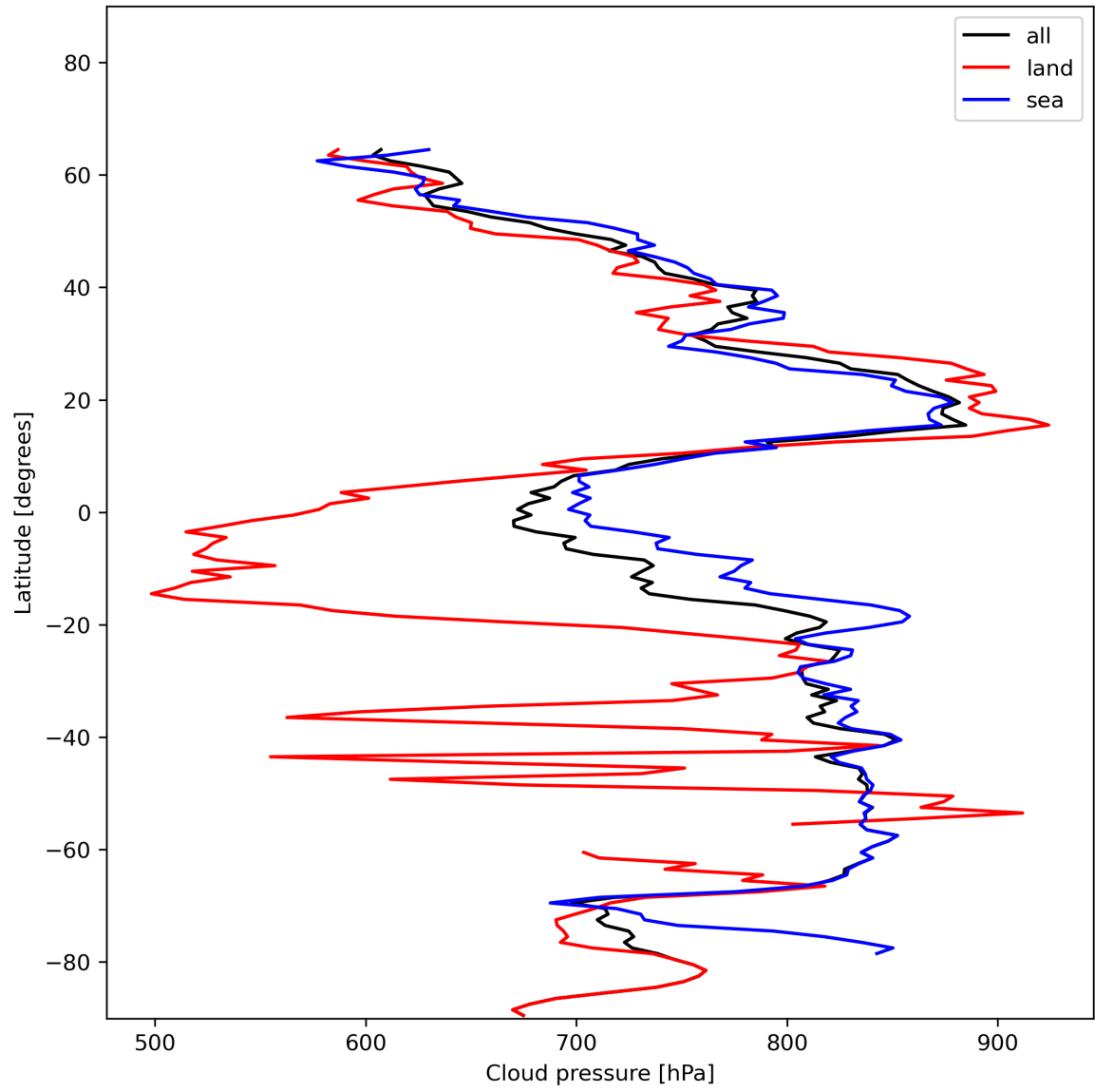
Figure 13: Zonal average of “Cloud pressure” for 2023-12-26 to 2023-12-28.
