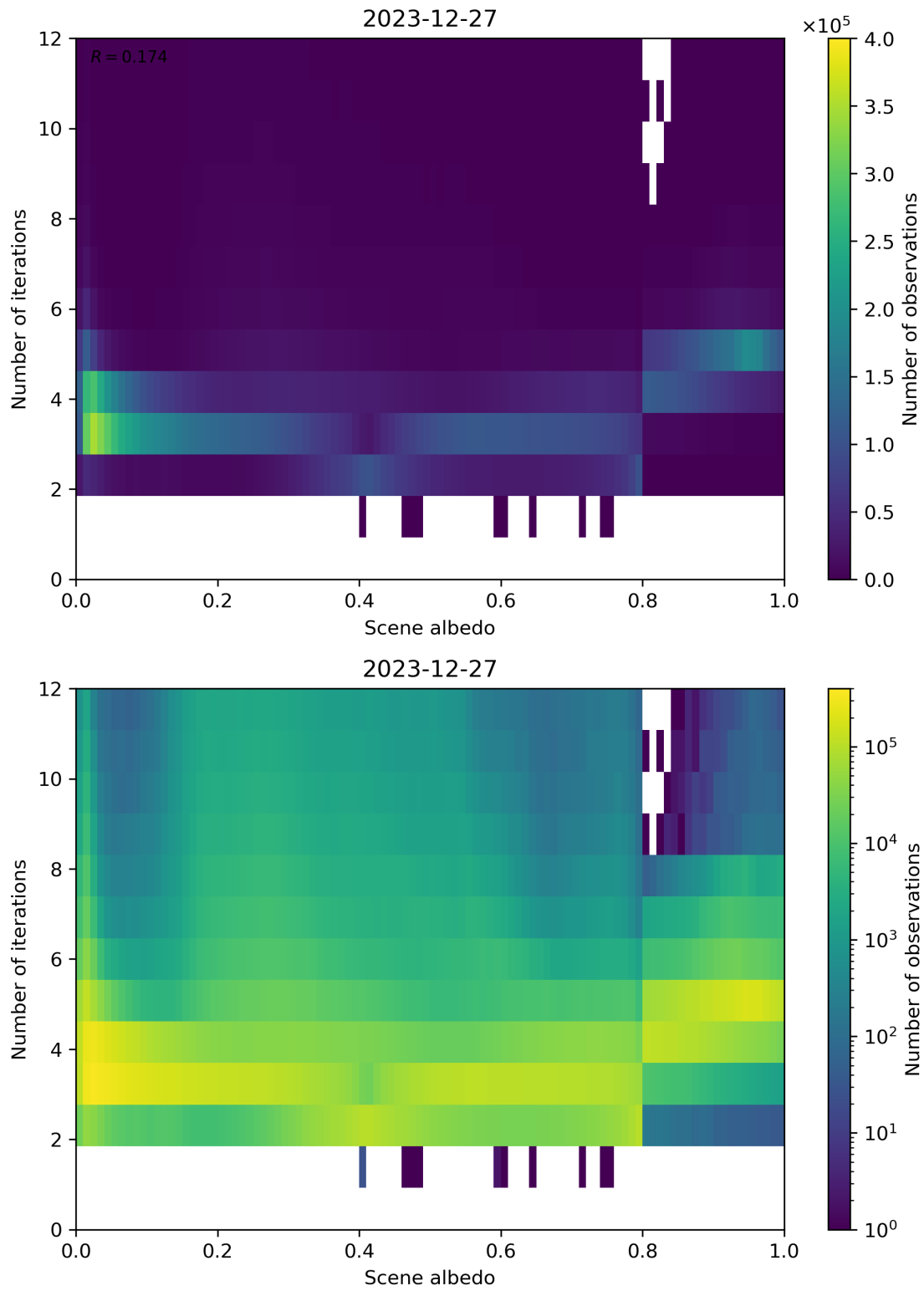
Figure 105: Scatter density plot of “Scene albedo” against “Number of iterations” for 2023-12-26 to 2023-12-28.
