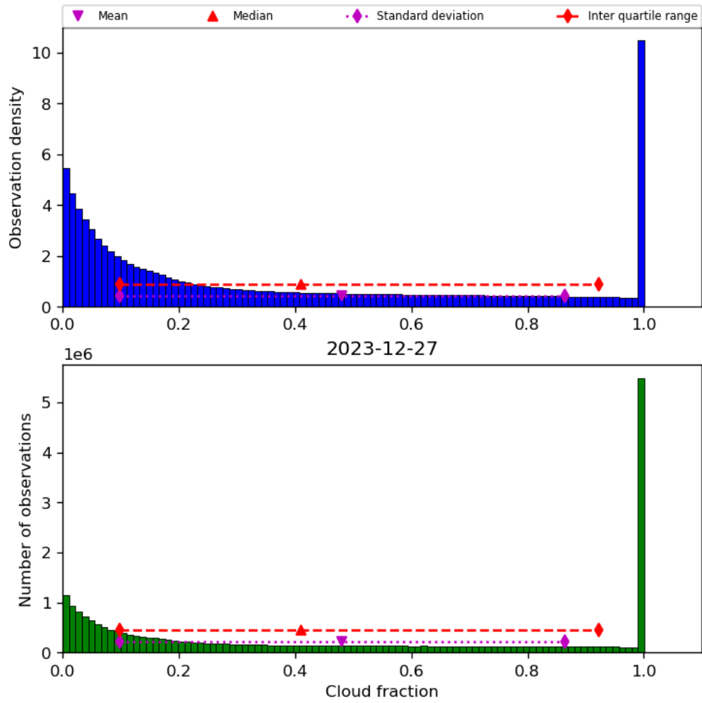
Figure 32: Histogram of “Cloud fraction” for 2023-12-26 to 2023-12-28
