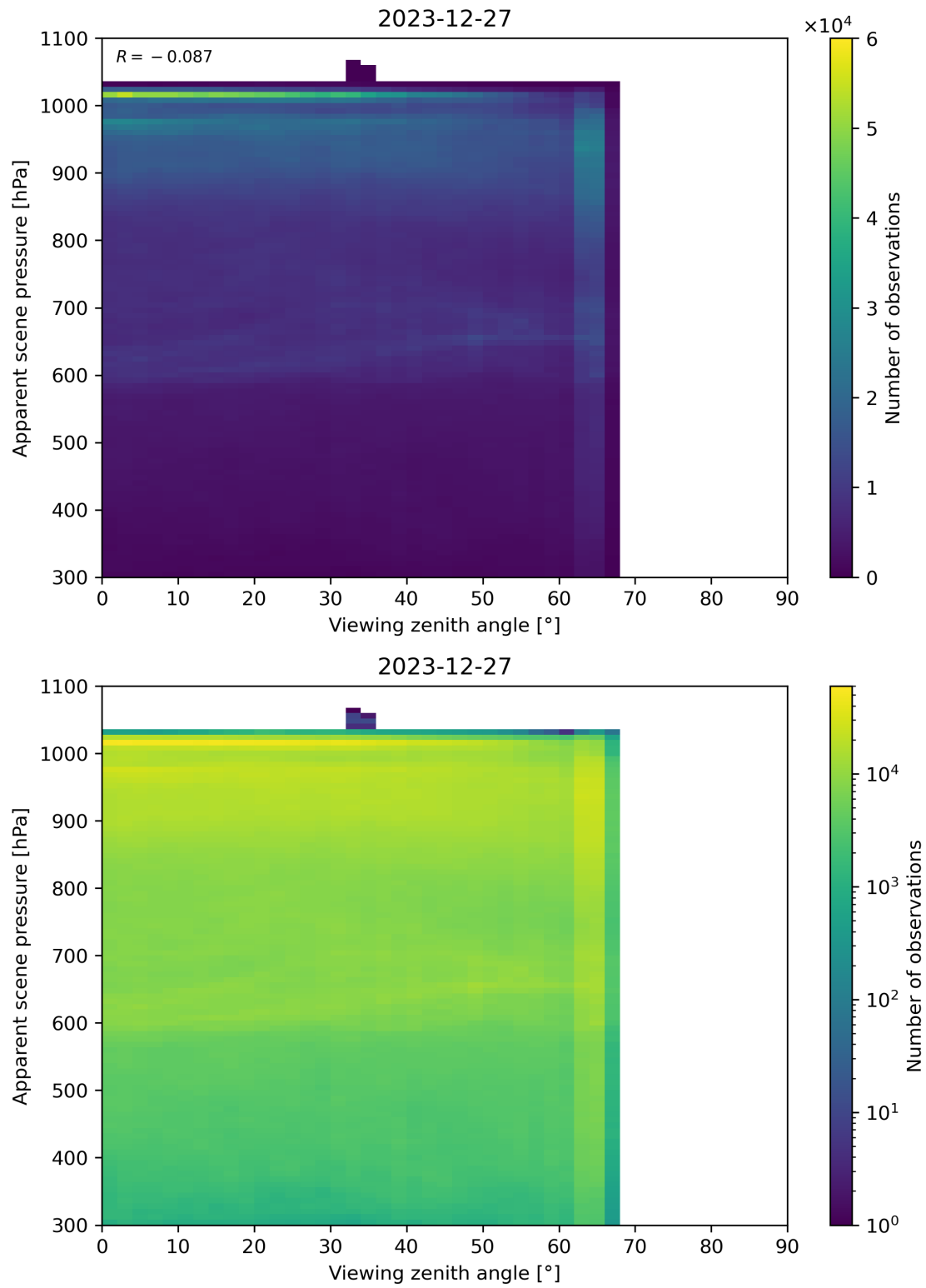
Figure 118: Scatter density plot of “Viewing zenith angle” against “Apparent scene pressure” for 2023-12-26 to 2023-12-28.
