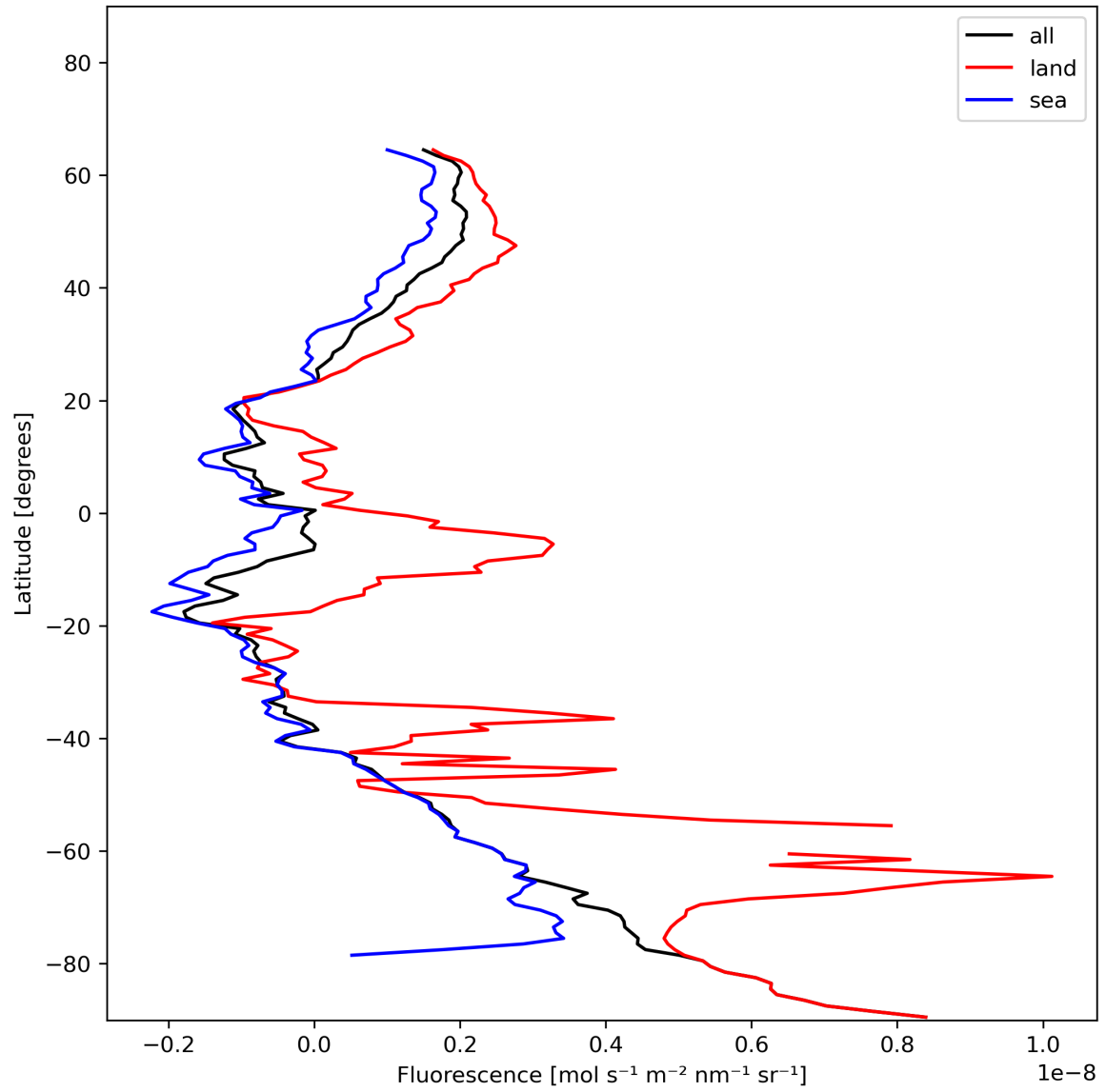
Figure 23: Zonal average of “Fluorescence” for 2023-12-26 to 2023-12-28.
