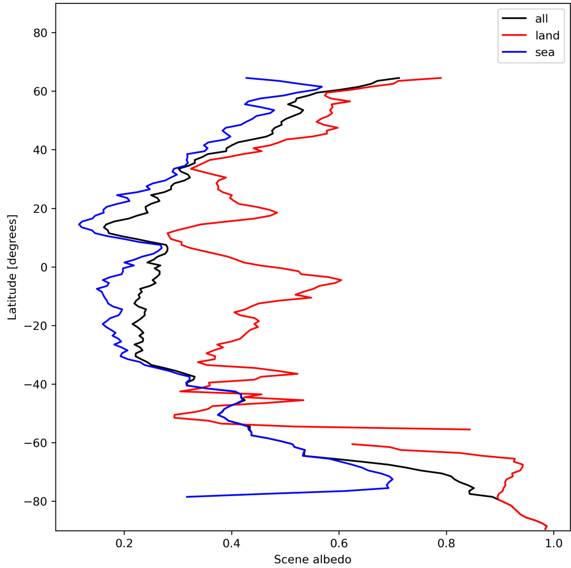
Figure 17: Zonal average of “Scene albedo” for 2023-12-26 to 2023-12-28.
