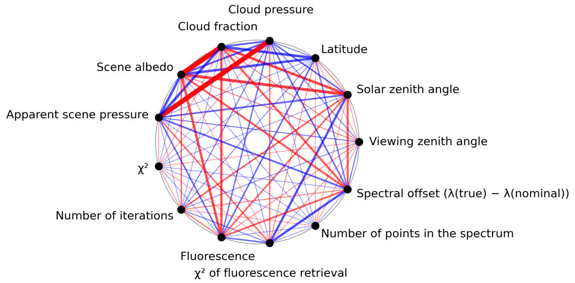
Figure 1: Map of correlation graph for 2023-12-26 to 2023-12-28.
