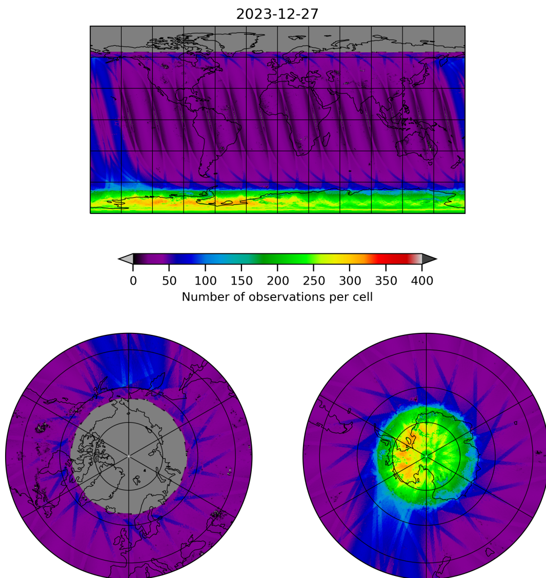
Figure 11: Map of the number of observations for 2023-12-26 to 2023-12-28
