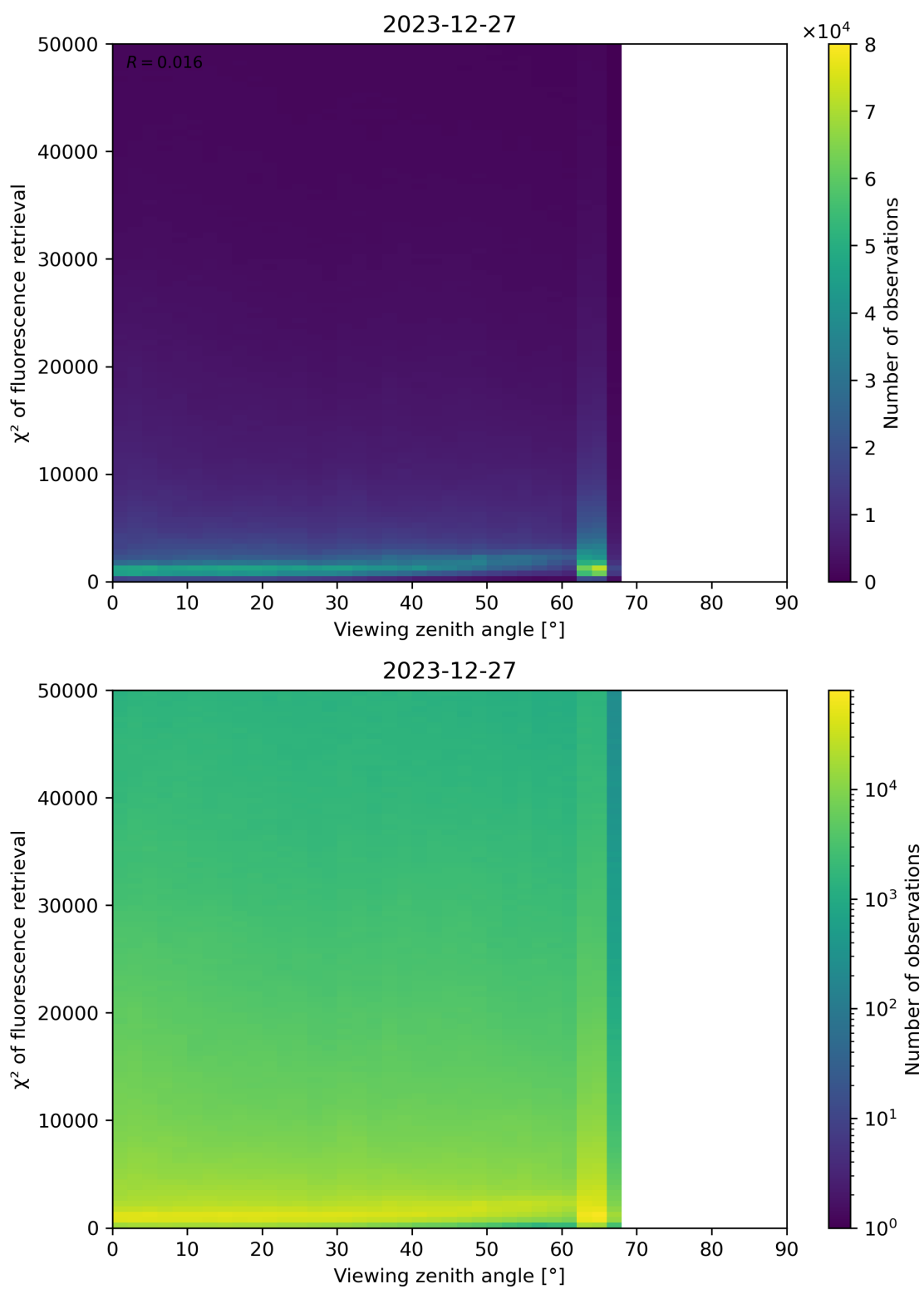
Figure 119: Scatter density plot of “Viewing zenith angle” against “ \chi^2 of fluorescence retrieval” for 2023-12-26 to 2023-12-28.
