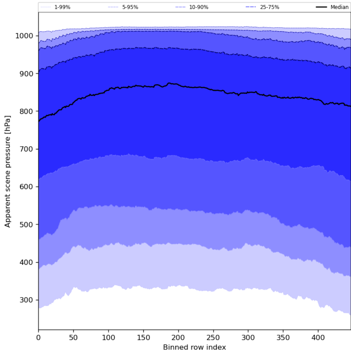
Figure 53: Along track statistics of “Apparent scene pressure” for 2023-12-26 to 2023-12-28
