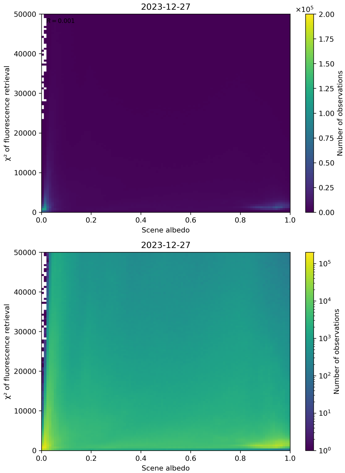
Figure 103: Scatter density plot of “Scene albedo” against “ \chi^2 of fluorescence retrieval” for 2023-12-26 to 2023-12-28.
