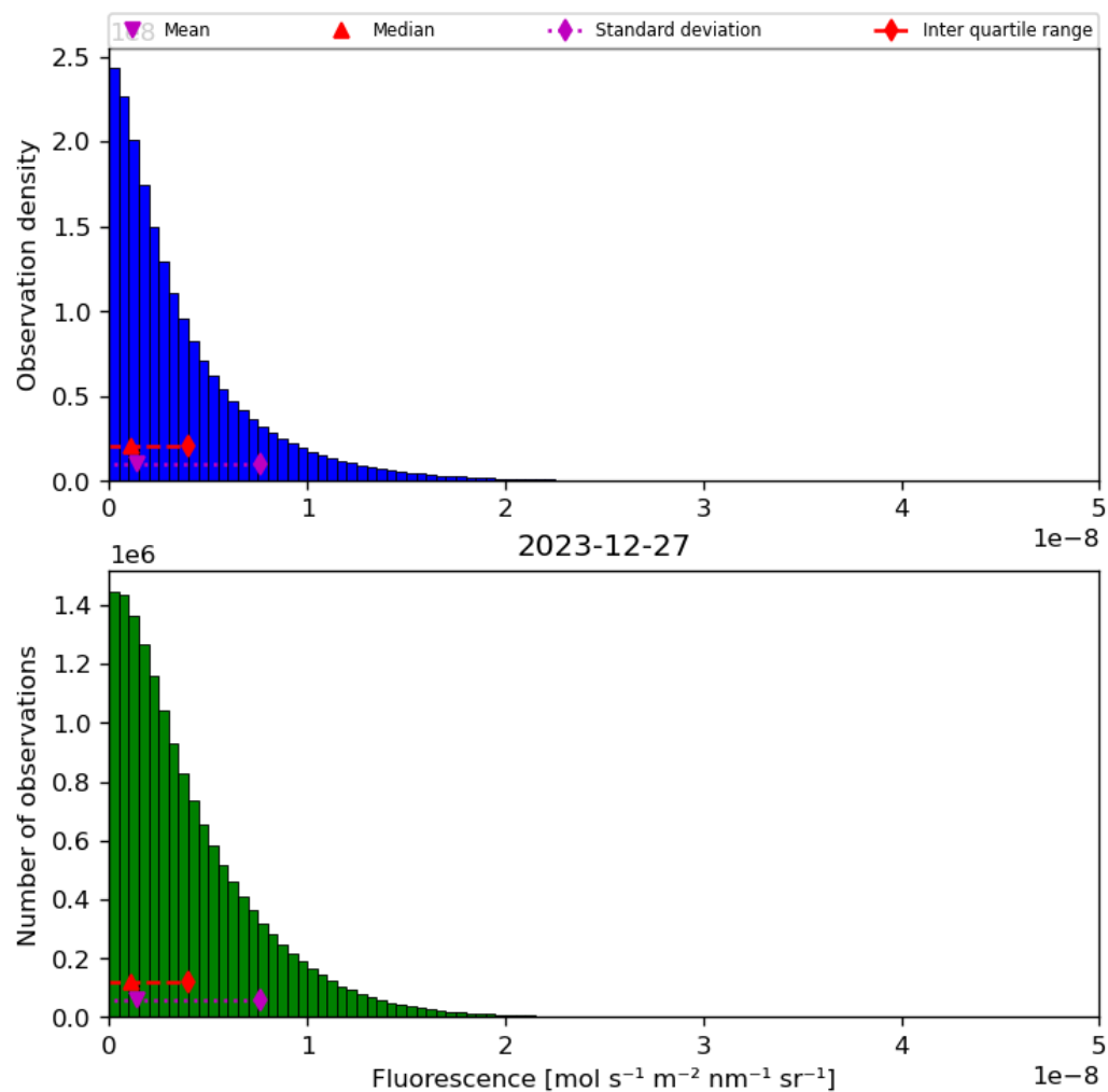
Figure 40: Histogram of “Fluorescence” for 2023-12-26 to 2023-12-28
