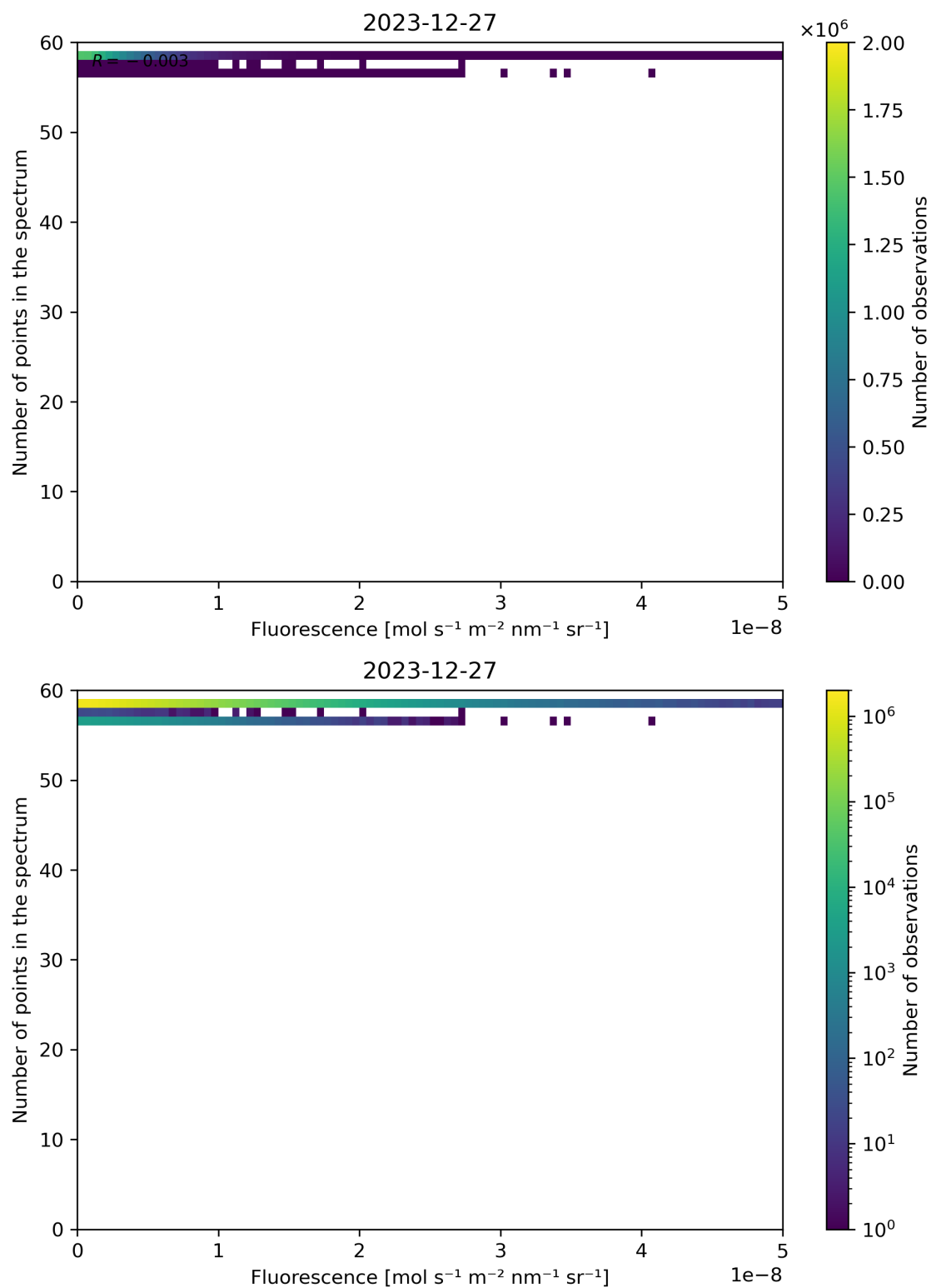
Figure 86: Scatter density plot of “Fluorescence” against “Number of points in the spectrum” for 2023-12-26 to 2023-12-28.
