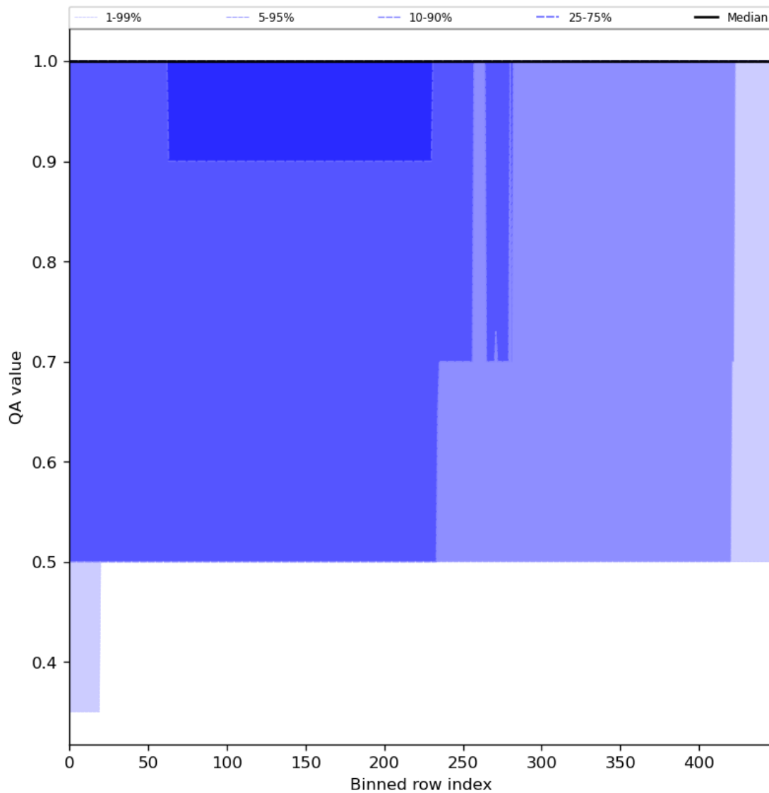
Figure 46: Along track statistics of “QA value” for 2023-12-26 to 2023-12-28
