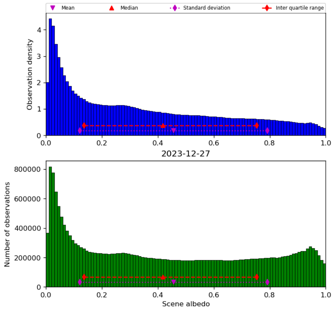
Figure 34: Histogram of “Scene albedo” for 2023-12-26 to 2023-12-28
