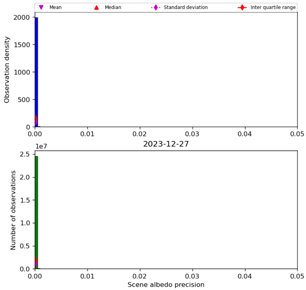
Figure 35: Histogram of “Scene albedo precision” for 2023-12-26 to 2023-12-28
