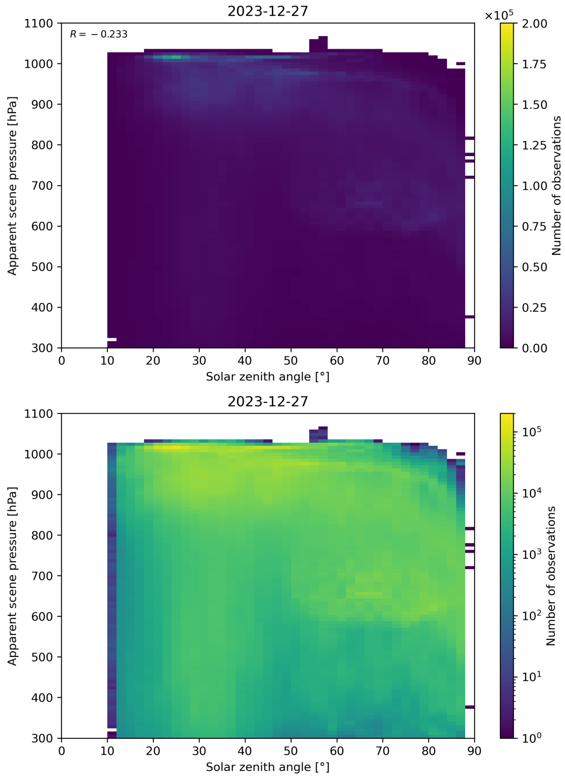
Figure 108: Scatter density plot of “Solar zenith angle” against “Apparent scene pressure” for 2023-12-26 to 2023-12-28.
