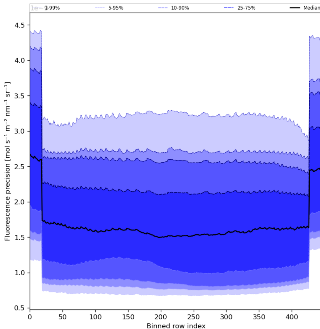
Figure 58: Along track statistics of “Fluorescence precision” for 2023-12-26 to 2023-12-28
