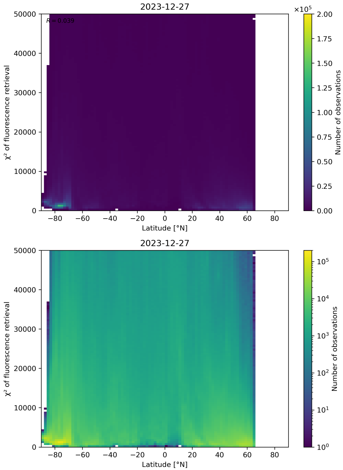
Figure 89: Scatter density plot of “Latitude” against “ \chi^2 of fluorescence retrieval” for 2023-12-26 to 2023-12-28.
