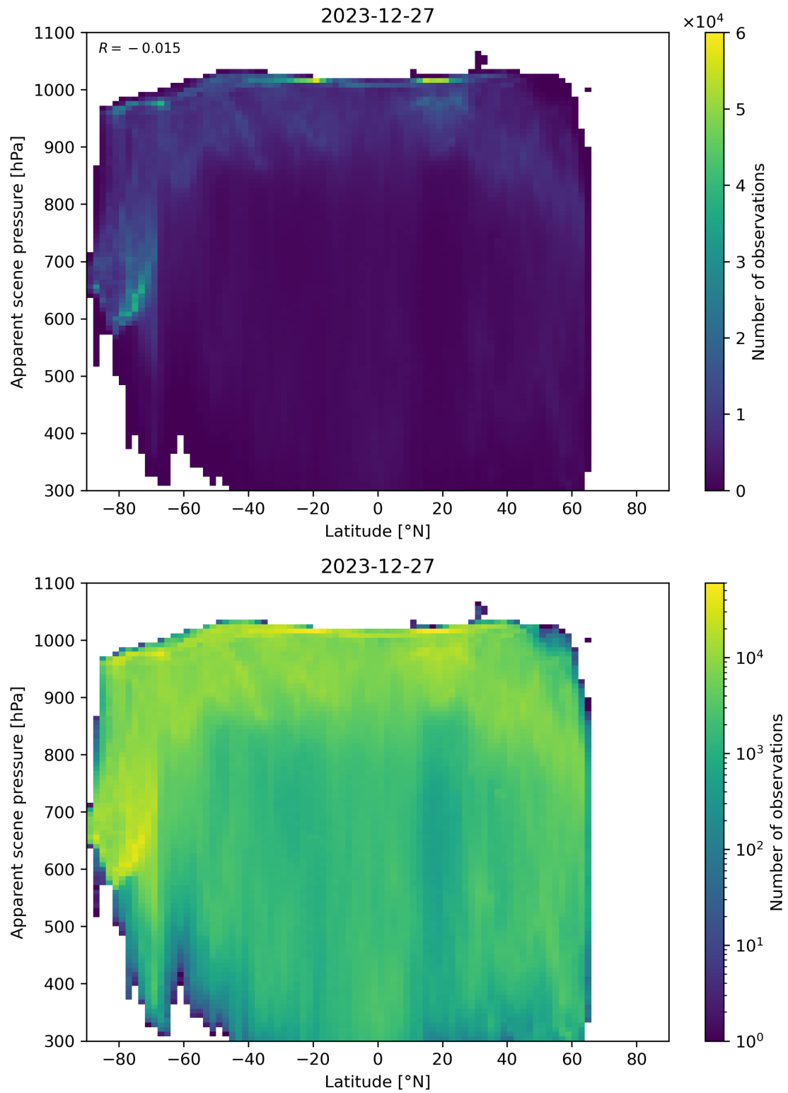
Figure 88: Scatter density plot of “Latitude” against “Apparent scene pressure” for 2023-12-26 to 2023-12-28.
