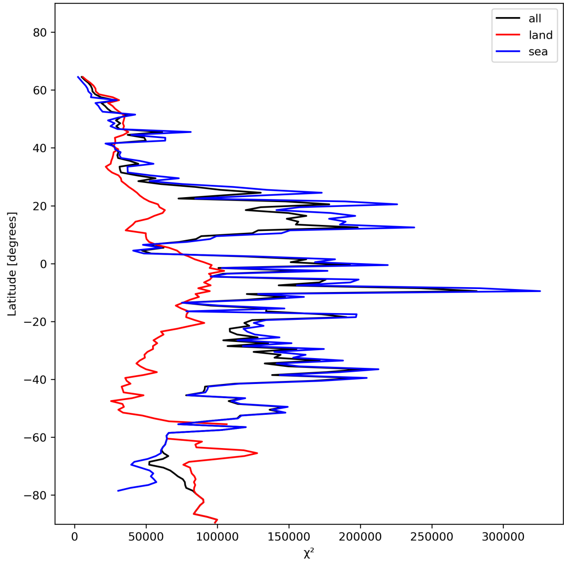
Figure 21: Zonal average of “ \chi^2 ” for 2023-12-26 to 2023-12-28.
