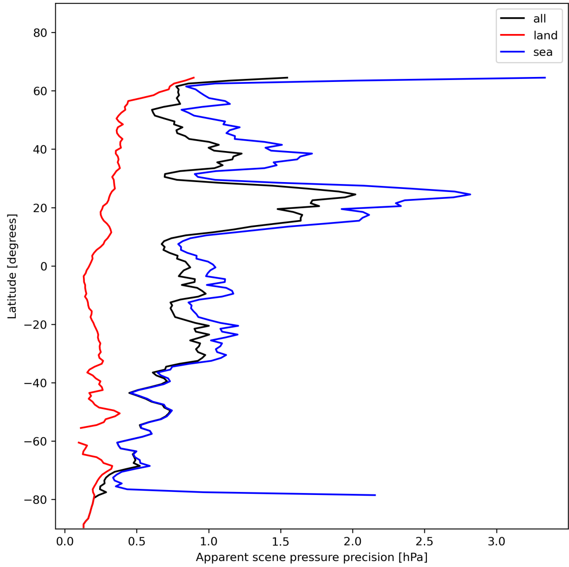
Figure 20: Zonal average of “Apparent scene pressure precision” for 2023-12-26 to 2023-12-28.
