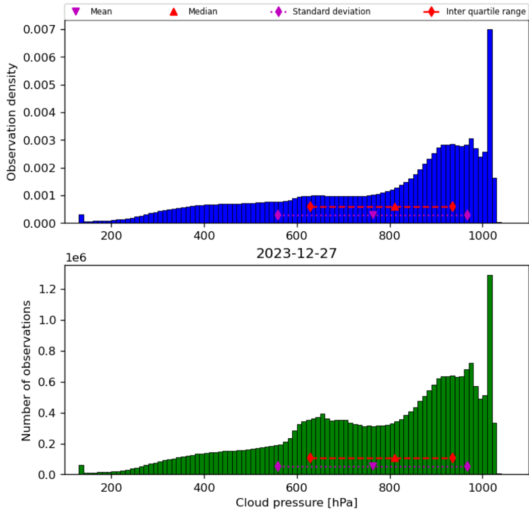
Figure 30: Histogram of “Cloud pressure” for 2023-12-26 to 2023-12-28
