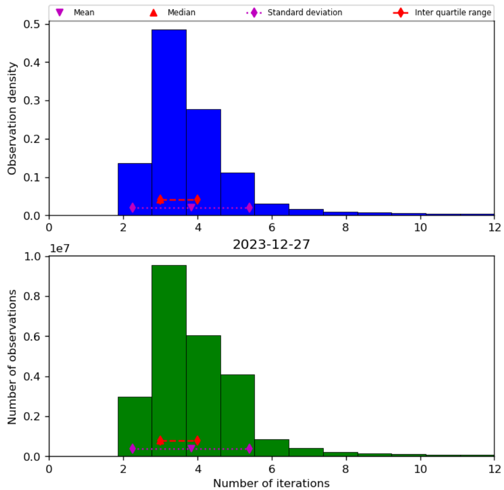
Figure 39: Histogram of “Number of iterations” for 2023-12-26 to 2023-12-28
