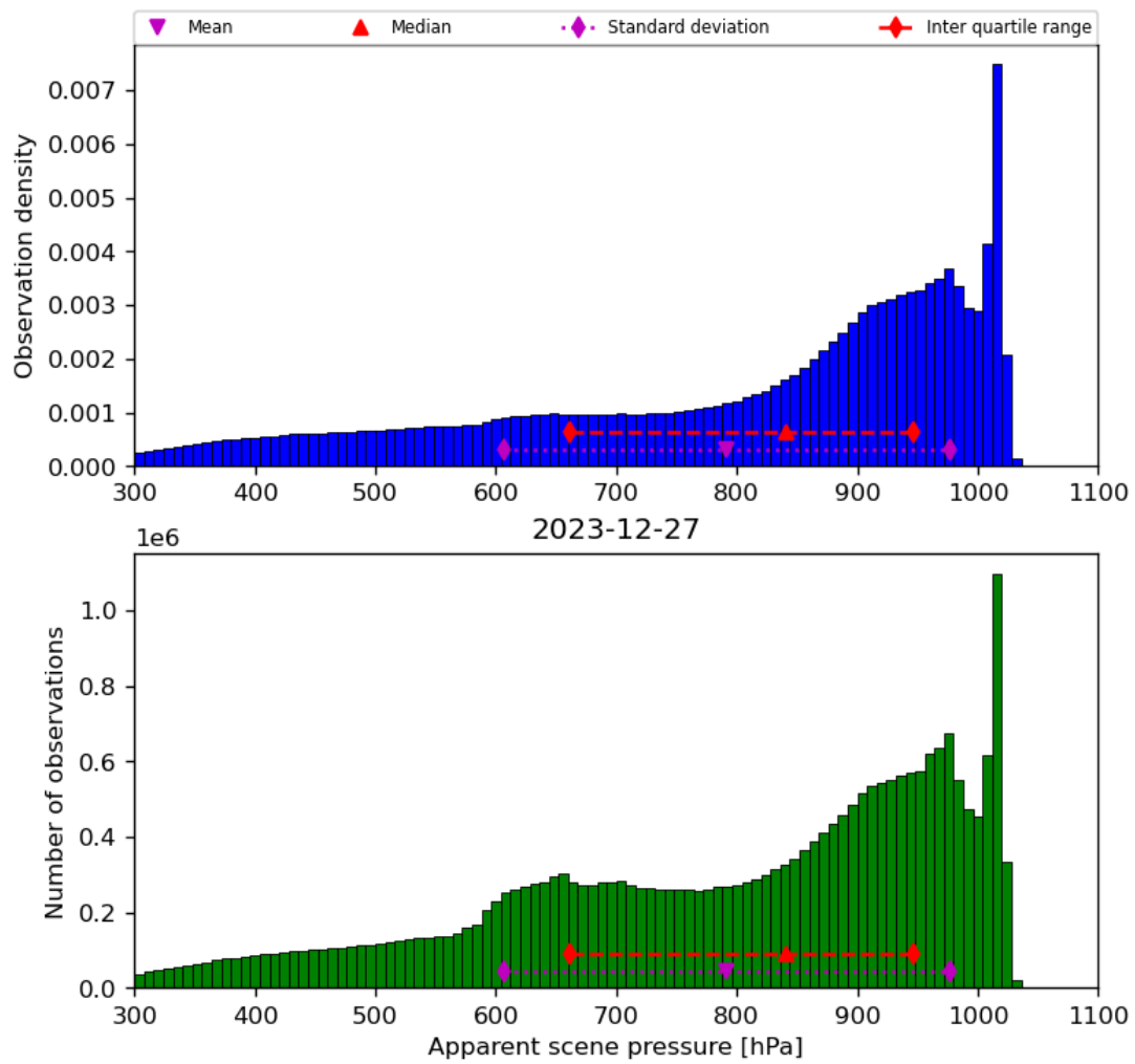
Figure 36: Histogram of “Apparent scene pressure” for 2023-12-26 to 2023-12-28
