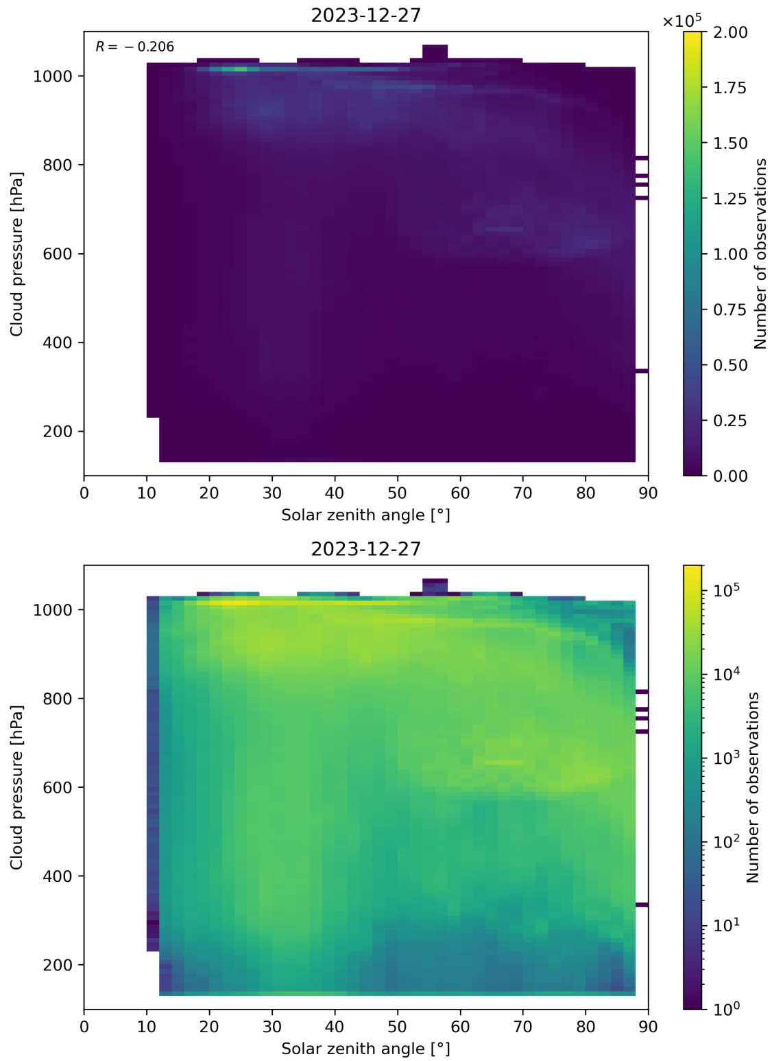
Figure 111: Scatter density plot of “Solar zenith angle” against “Cloud pressure” for 2023-12-26 to 2023-12-28.
