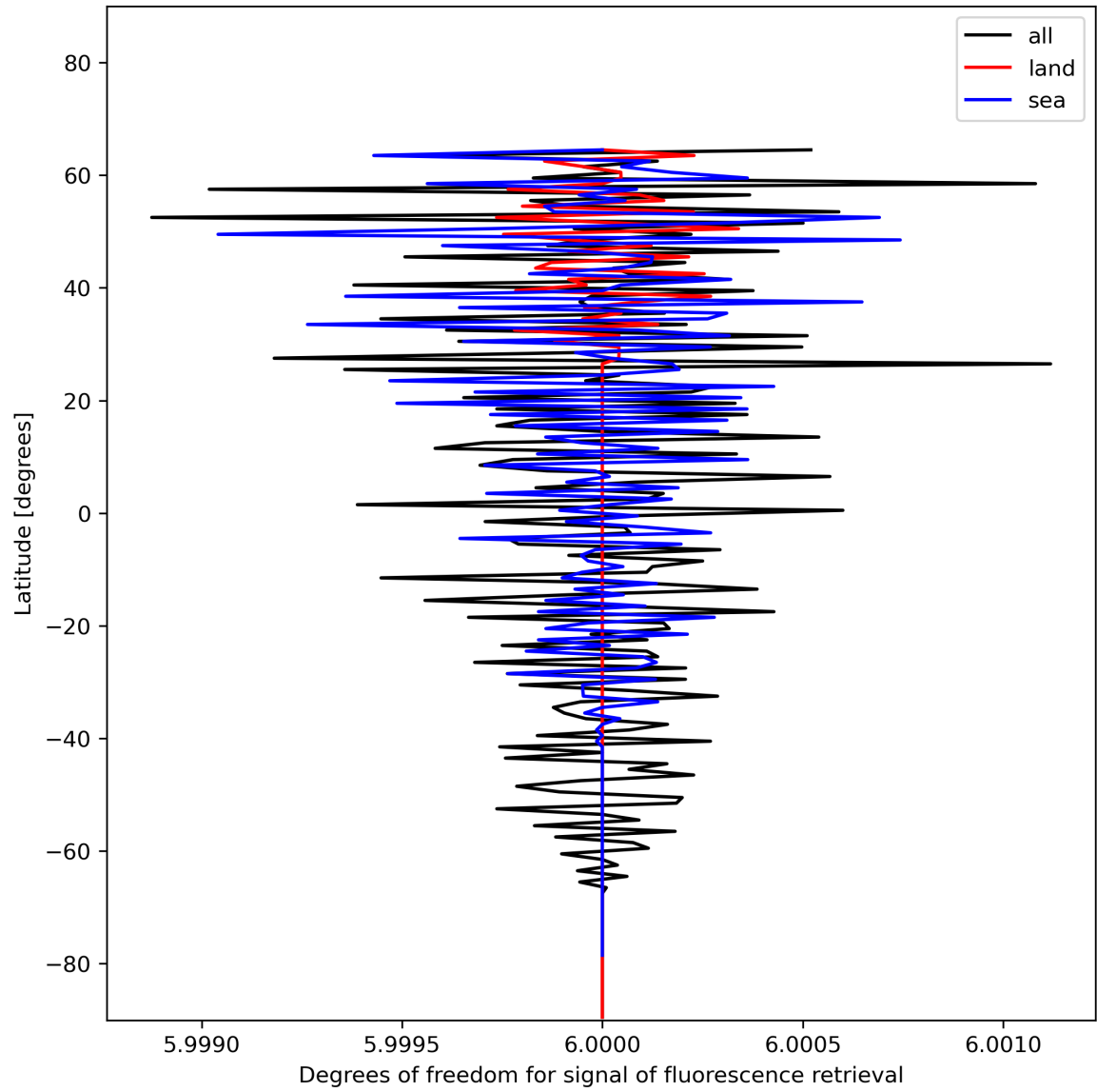
Figure 26: Zonal average of “Degrees of freedom for signal of fluorescence retrieval” for 2023-12-26 to 2023-12-28.
