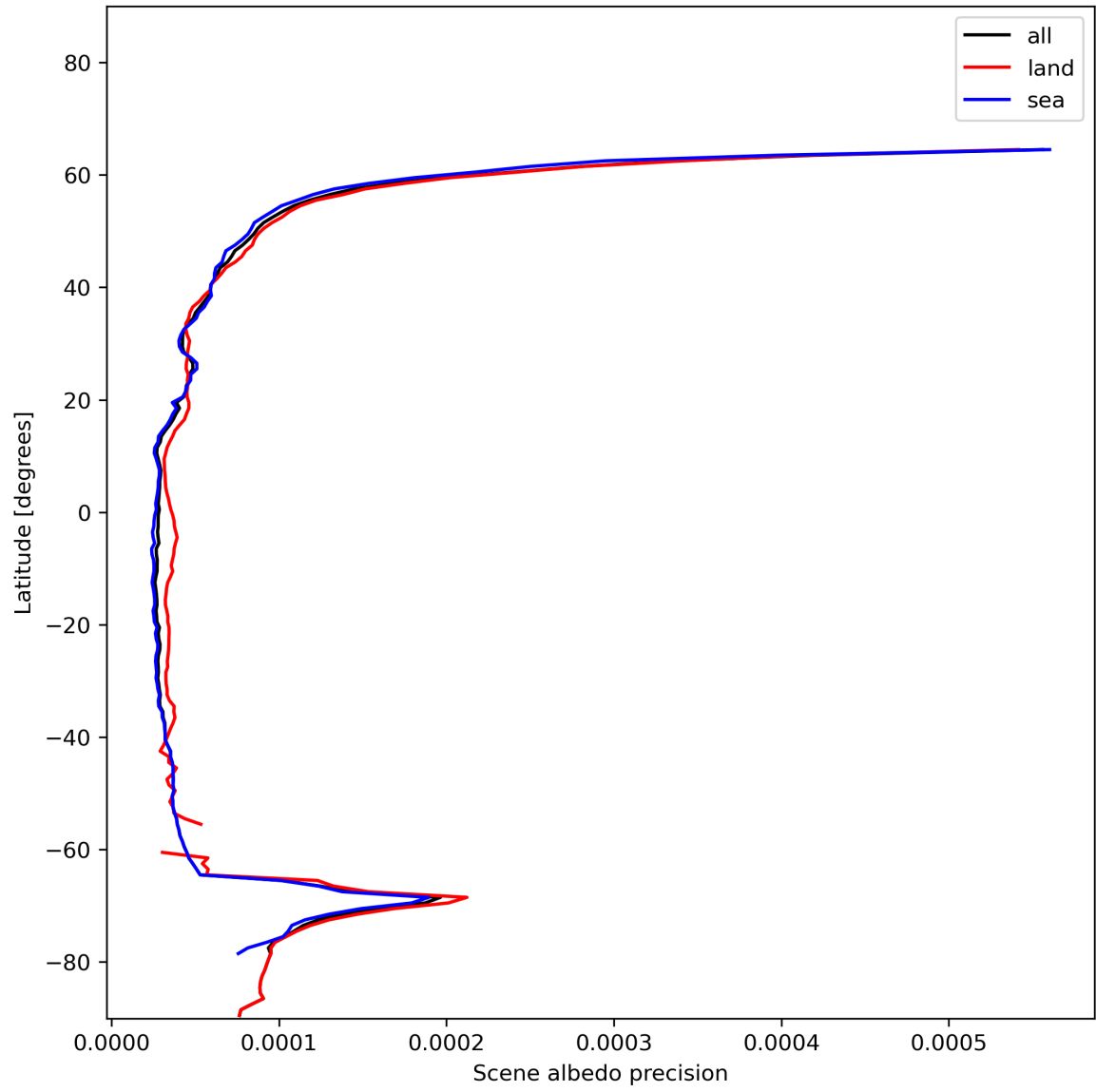
Figure 18: Zonal average of “Scene albedo precision” for 2023-12-26 to 2023-12-28.
