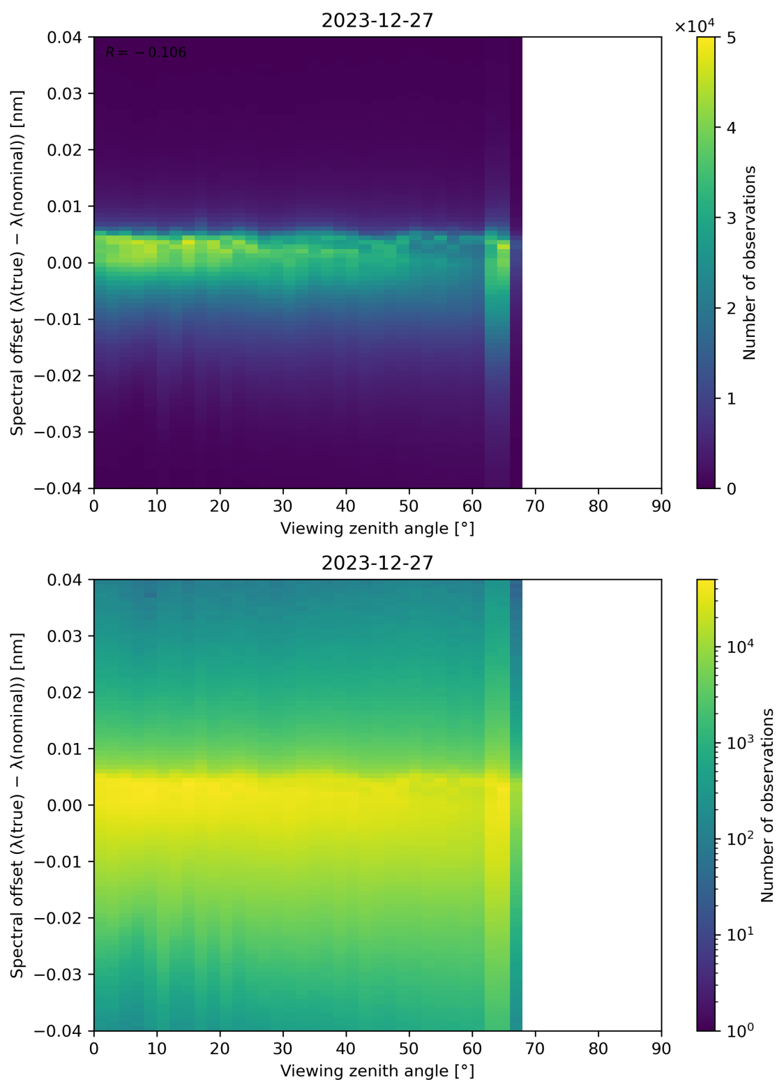
Figure 128: Scatter density plot of “Viewing zenith angle” against “Spectral offset ( \lambda(\text{true}) - \lambda(\text{nominal}) )” for 2023-12-26 to 2023-12-28.
