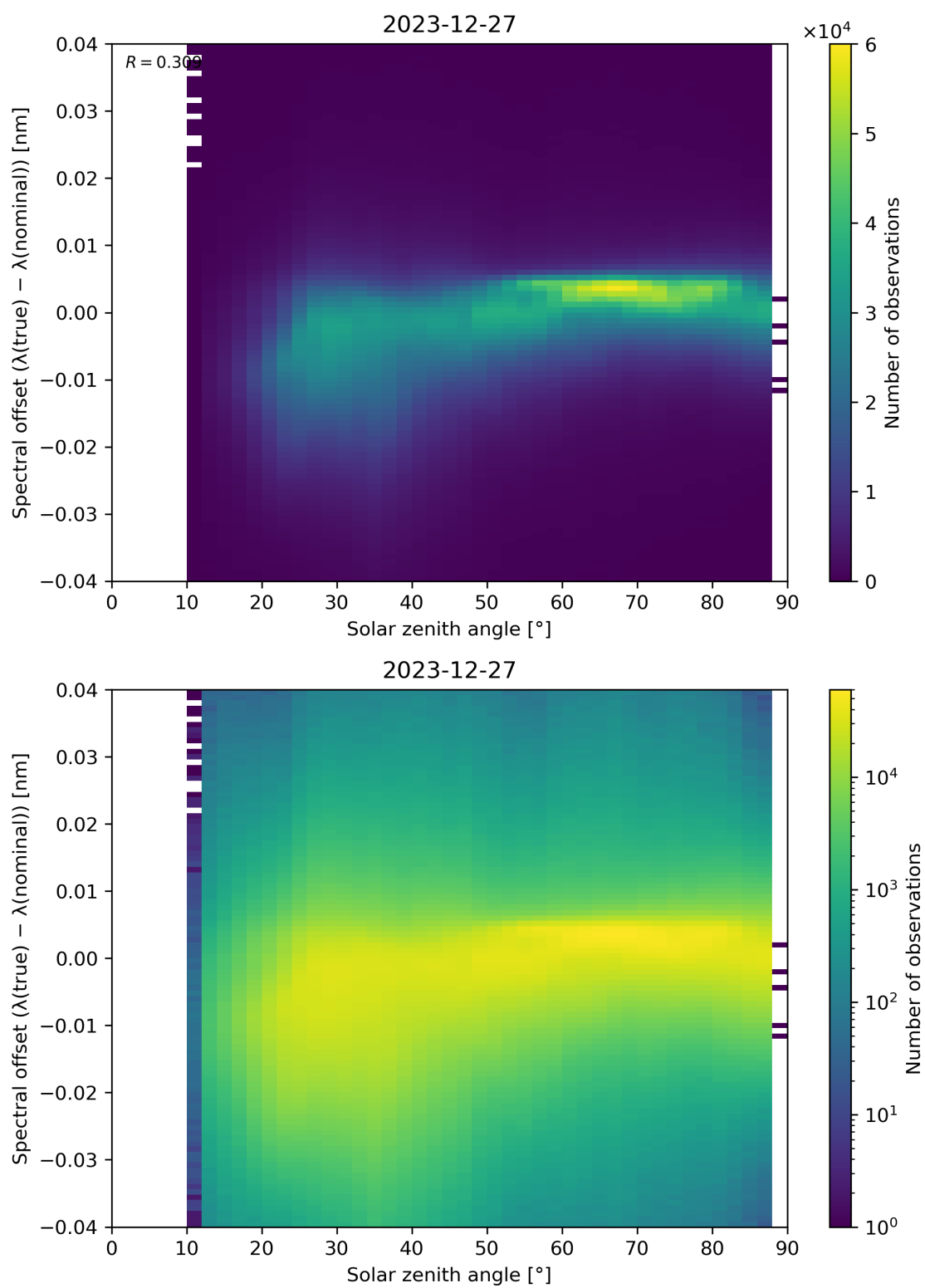
Figure 117: Scatter density plot of “Solar zenith angle” against “Spectral offset ( \lambda(\text{true}) - \lambda(\text{nominal}) )” for 2023-12-26 to 2023-12-28.
