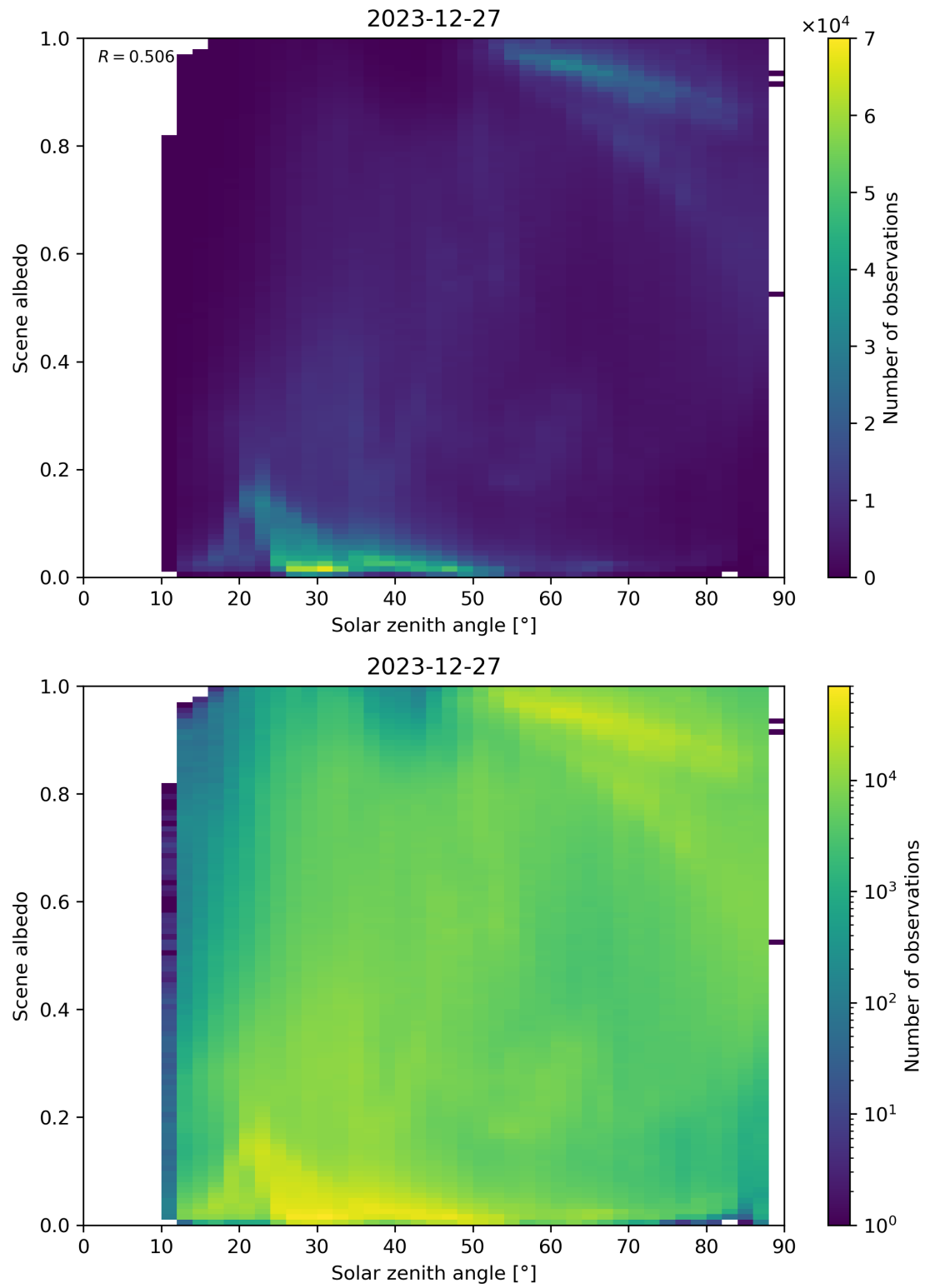
Figure 116: Scatter density plot of “Solar zenith angle” against “Scene albedo” for 2023-12-26 to 2023-12-28.
