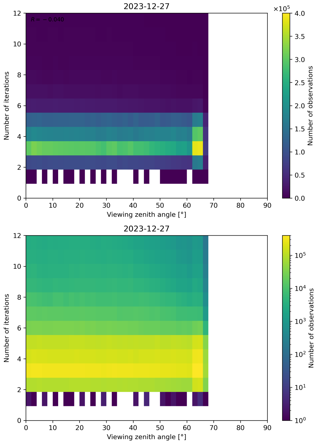
Figure 124: Scatter density plot of “Viewing zenith angle” against “Number of iterations” for 2023-12-26 to 2023-12-28.
