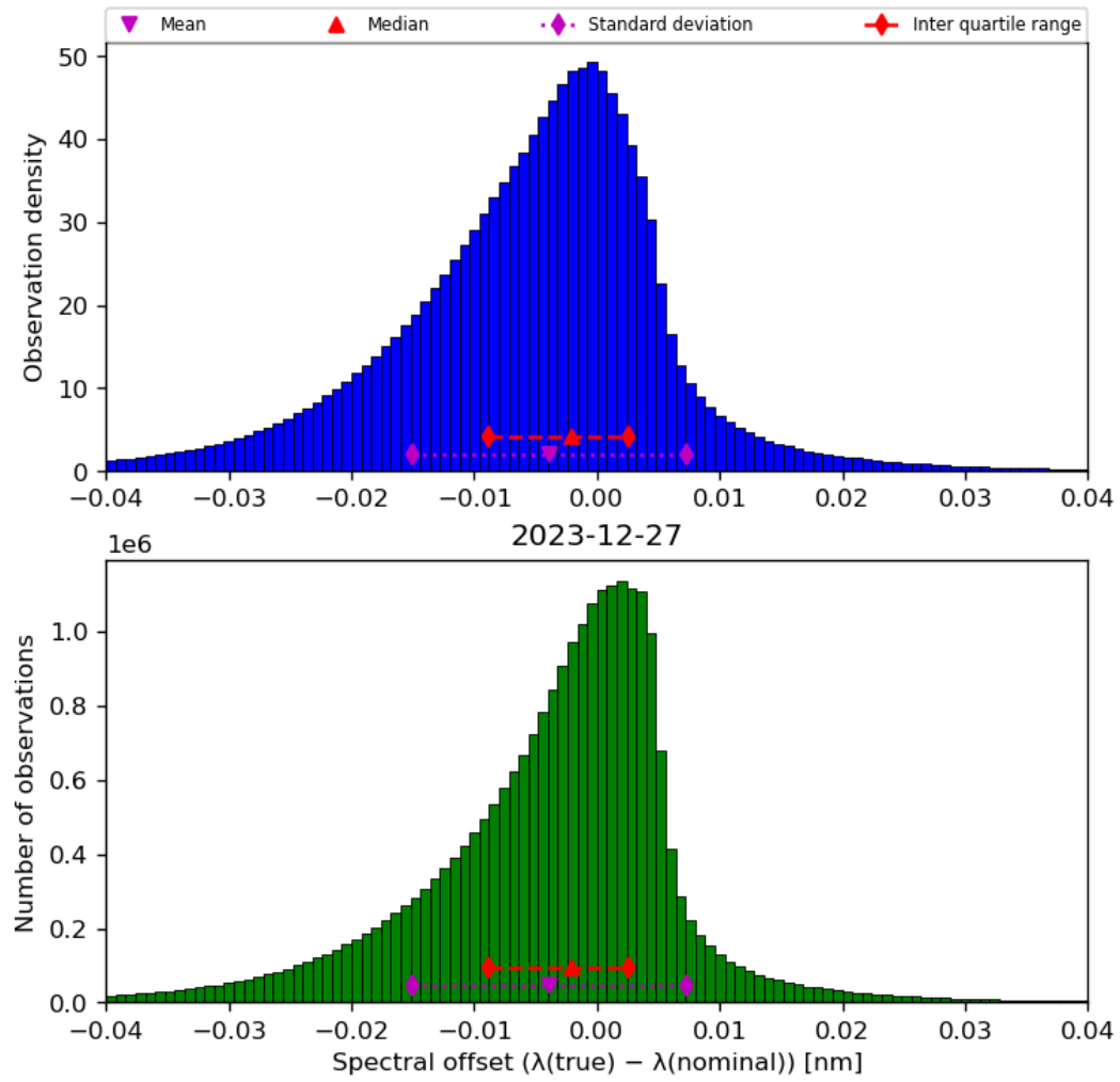
Figure 45: Histogram of “Spectral offset ( \lambda(\text{true}) - \lambda(\text{nominal}) )” for 2023-12-26 to 2023-12-28
