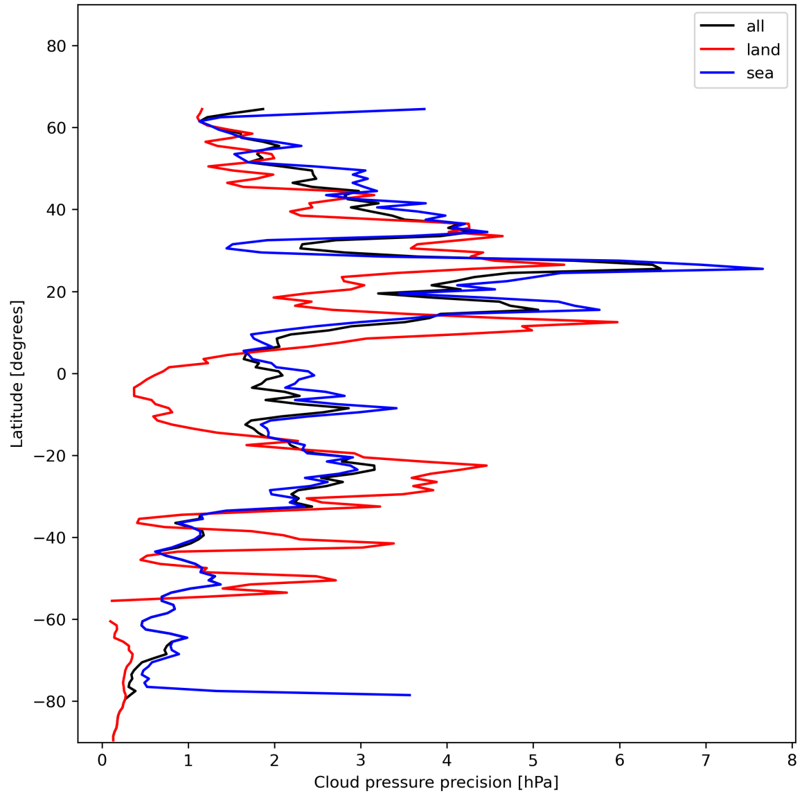
Figure 14: Zonal average of “Cloud pressure precision” for 2023-12-26 to 2023-12-28.
