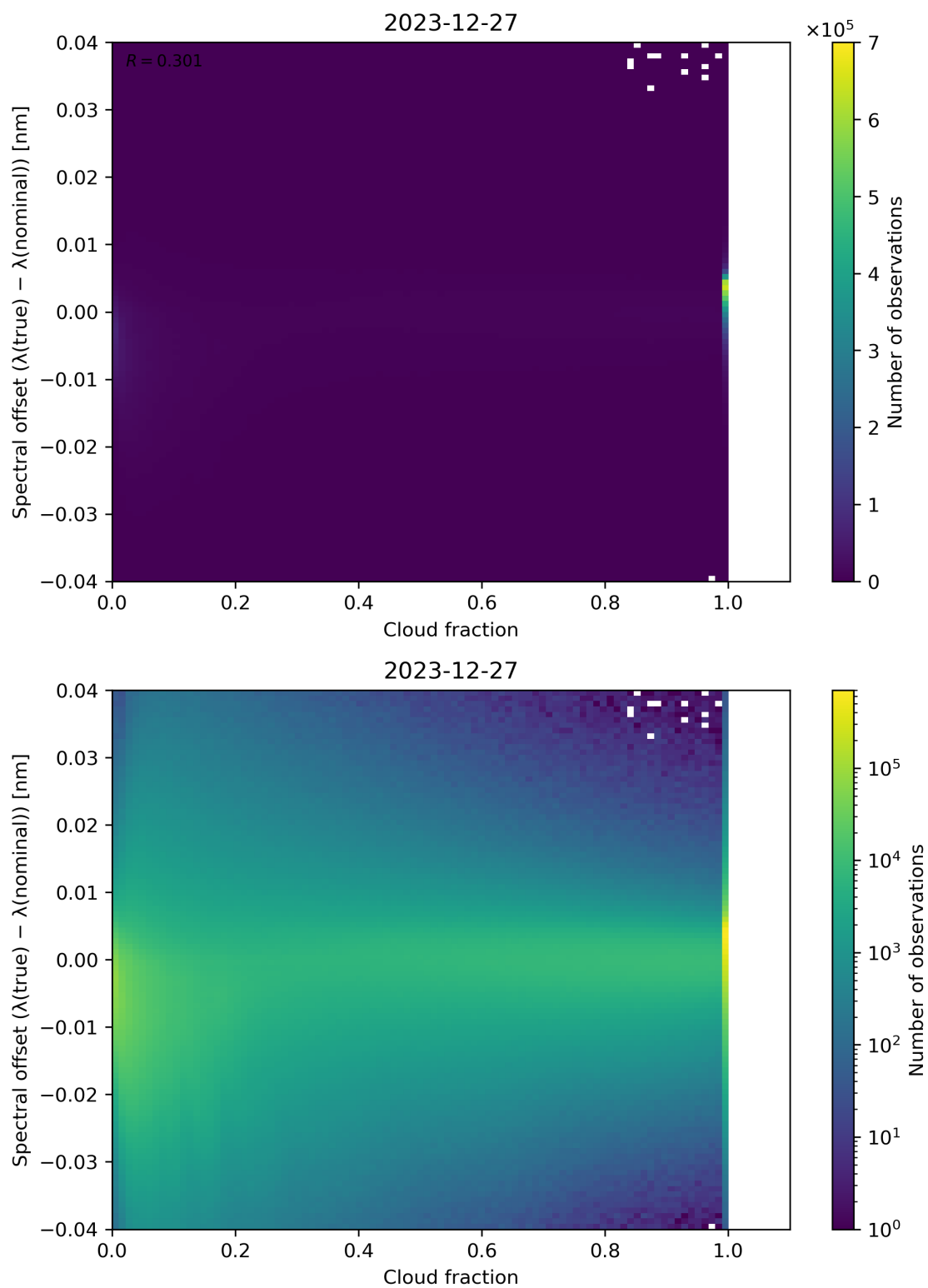
Figure 76: Scatter density plot of “Cloud fraction” against “Spectral offset ( \lambda(\text{true}) - \lambda(\text{nominal}) )” for 2023-12-26 to 2023-12-28.
