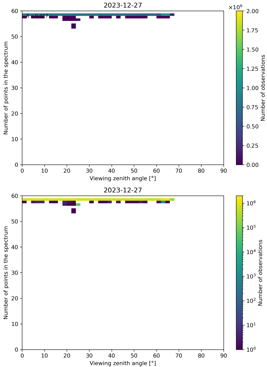
Figure 125: Scatter density plot of “Viewing zenith angle” against “Number of points in the spectrum” for 2023-12-26 to 2023-12-28.
