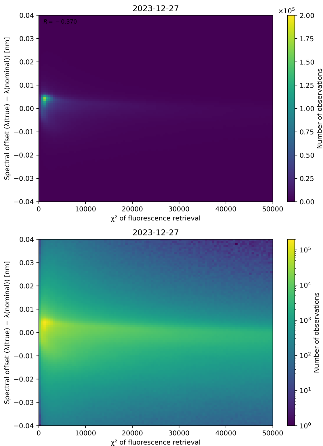
Figure 69: Scatter density plot of " \chi^2 of fluorescence retrieval" against "Spectral offset ( \lambda(\text{true}) - \lambda(\text{nominal})) " for 2023-12-26 to 2023-12-28.
