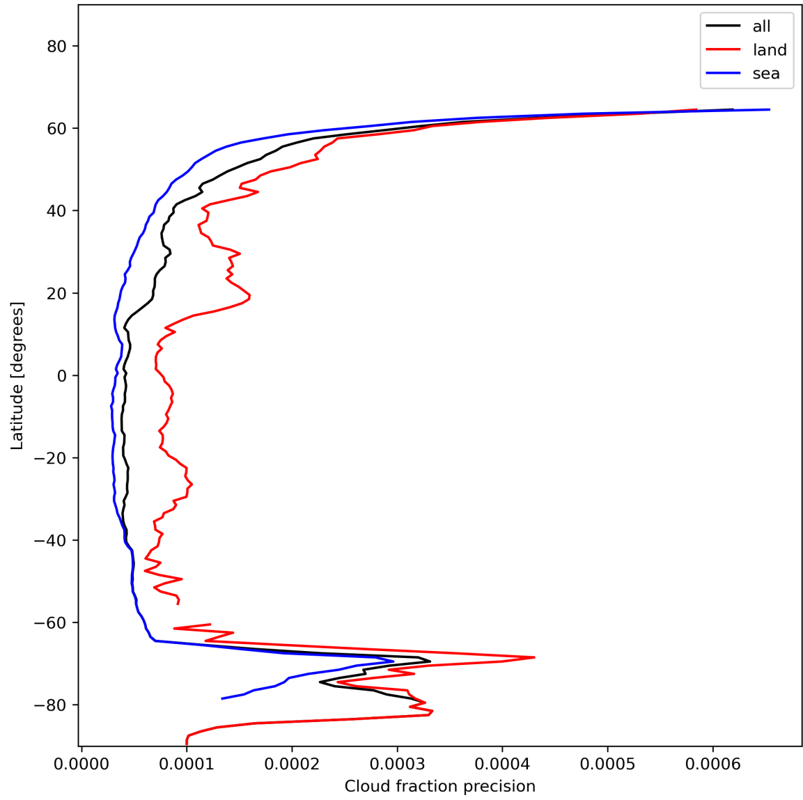
Figure 16: Zonal average of “Cloud fraction precision” for 2023-12-26 to 2023-12-28.
