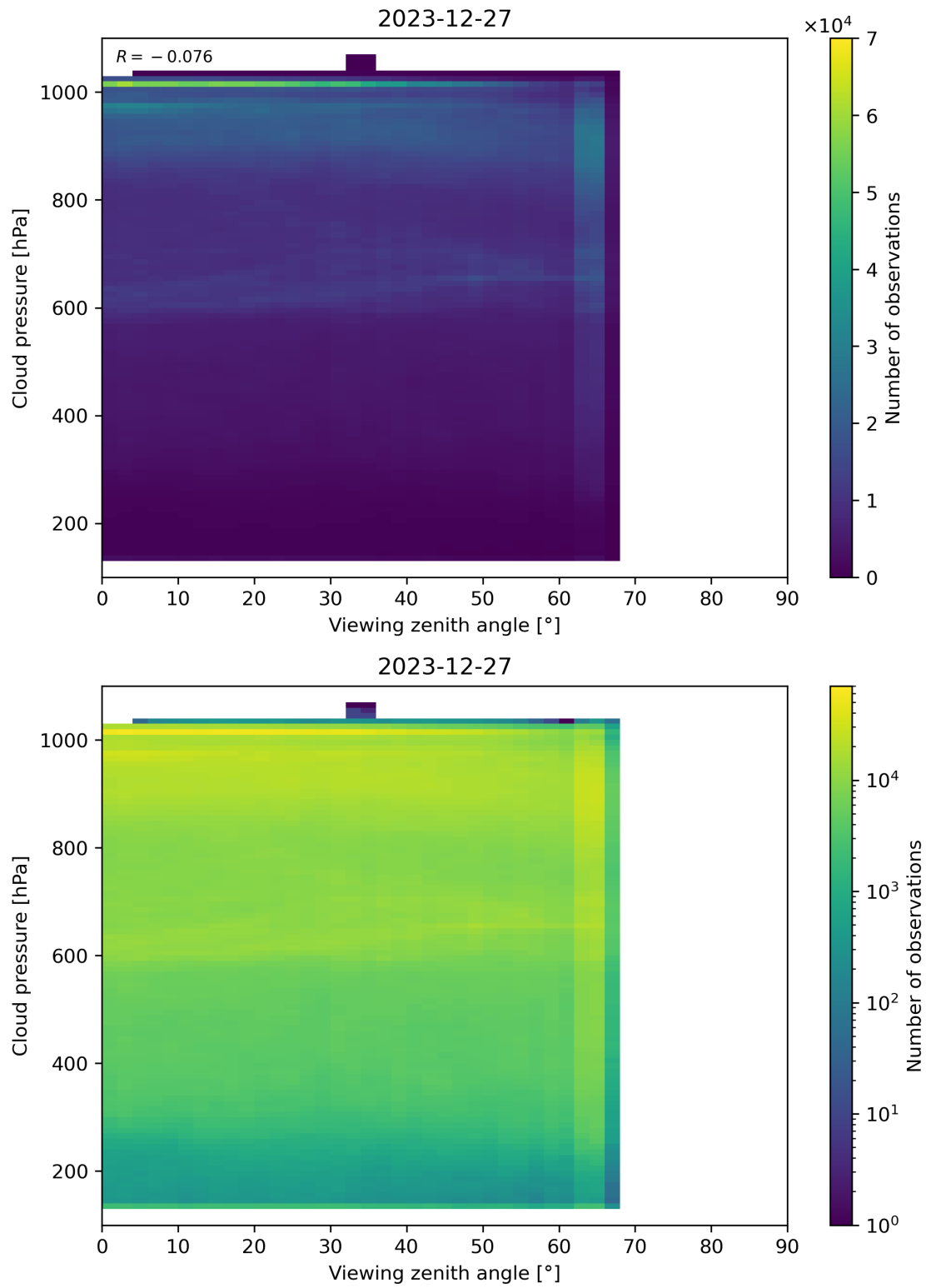
Figure 121: Scatter density plot of “Viewing zenith angle” against “Cloud pressure” for 2023-12-26 to 2023-12-28.
