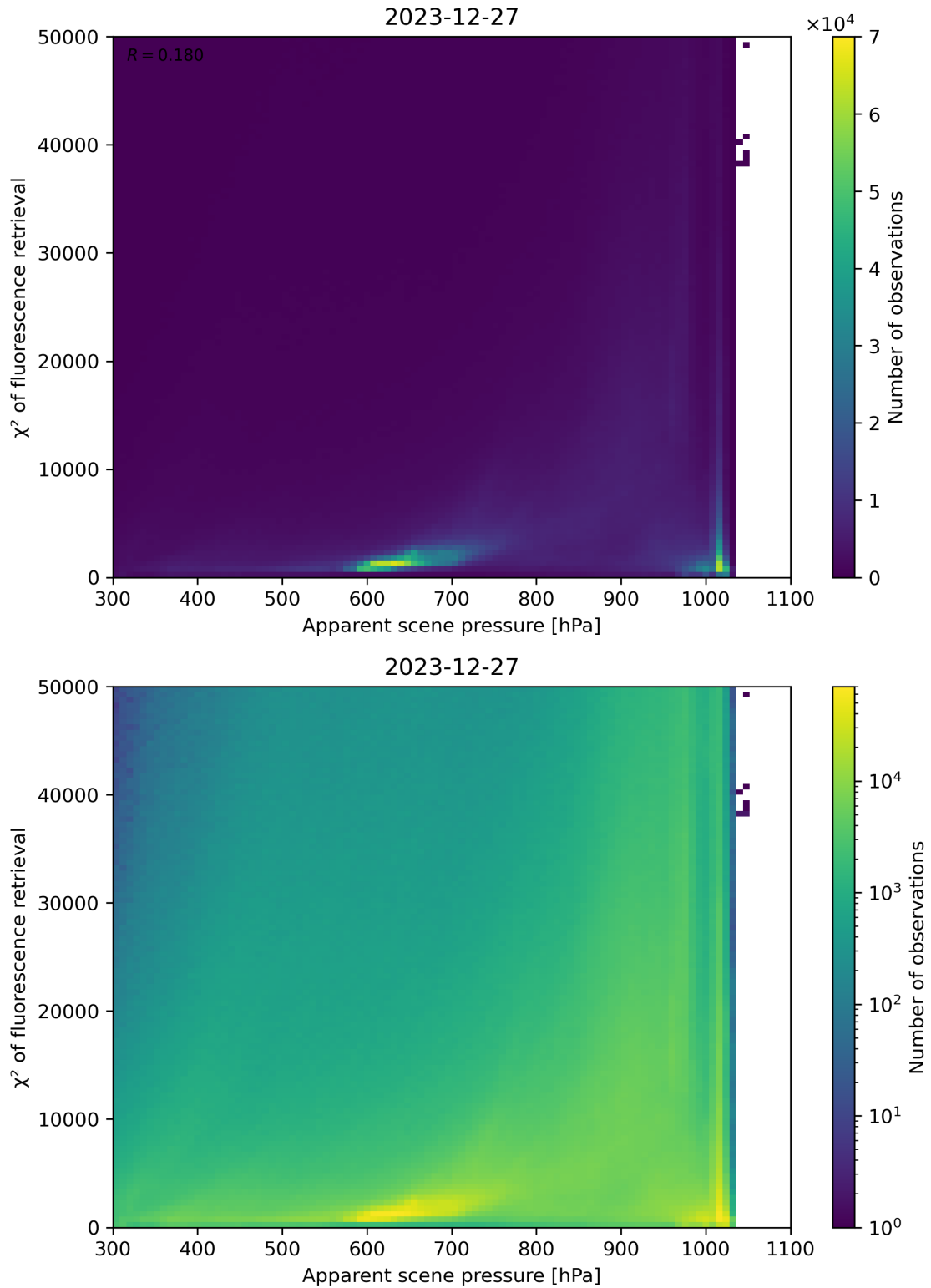
Figure 63: Scatter density plot of “Apparent scene pressure” against “ \chi^2 of fluorescence retrieval” for 2023-12-26 to 2023-12-28.
