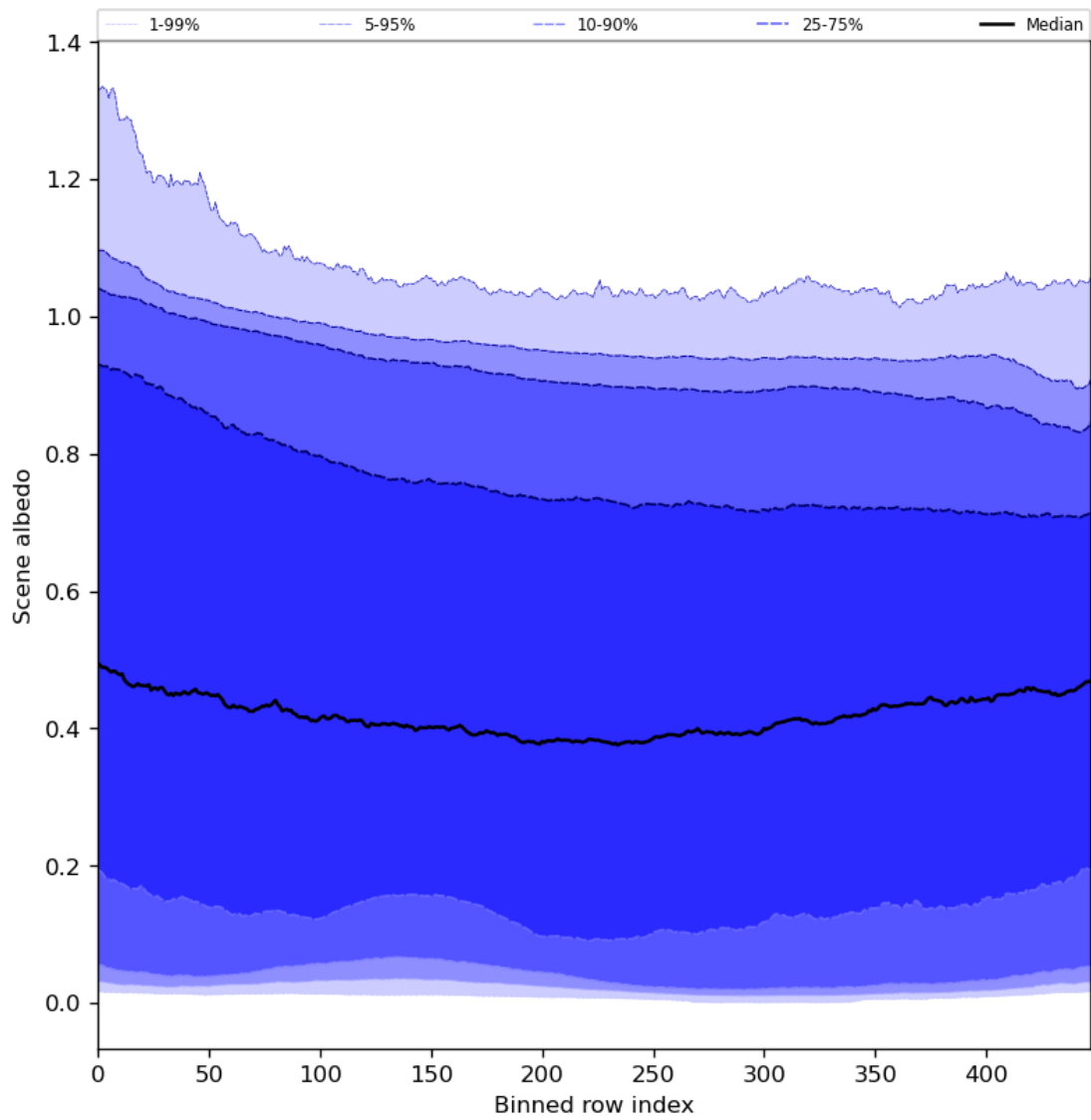
Figure 51: Along track statistics of “Scene albedo” for 2023-12-26 to 2023-12-28
