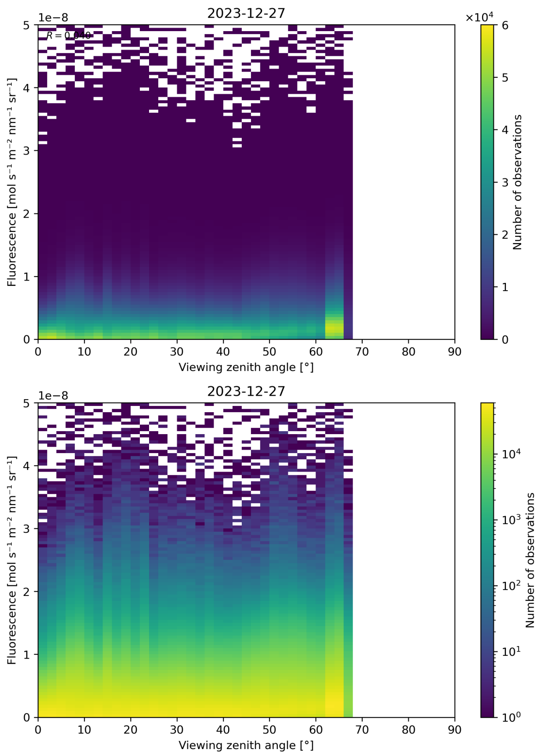
Figure 122: Scatter density plot of “Viewing zenith angle” against “Fluorescence” for 2023-12-26 to 2023-12-28.
