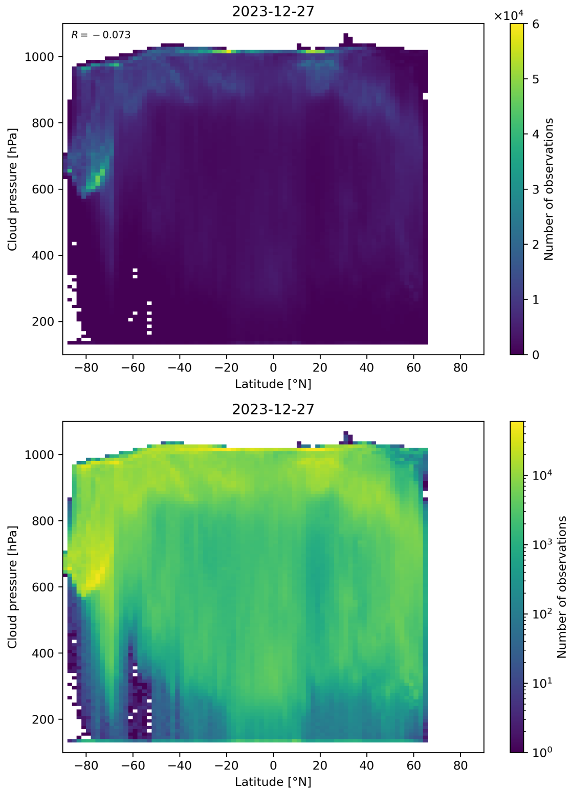
Figure 91: Scatter density plot of “Latitude” against “Cloud pressure” for 2023-12-26 to 2023-12-28.
