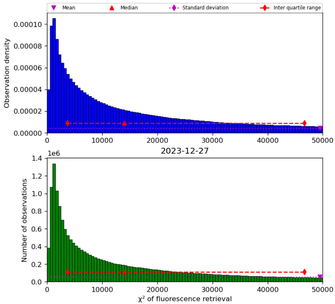
Figure 42: Histogram of “ \chi^2 of fluorescence retrieval” for 2023-12-26 to 2023-12-28
