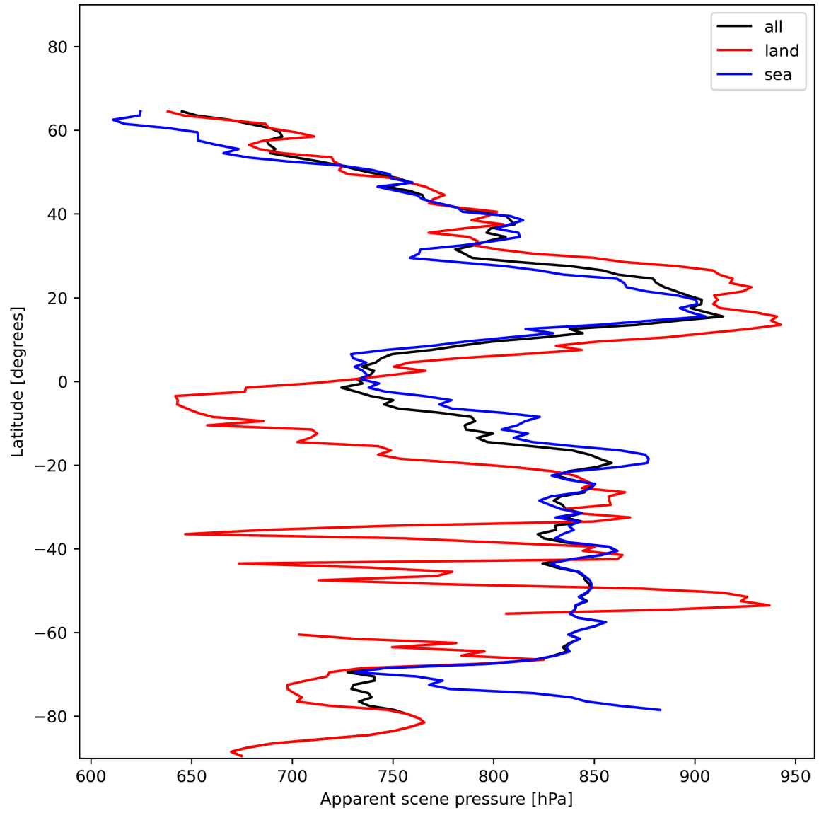
Figure 19: Zonal average of “Apparent scene pressure” for 2023-12-26 to 2023-12-28.
