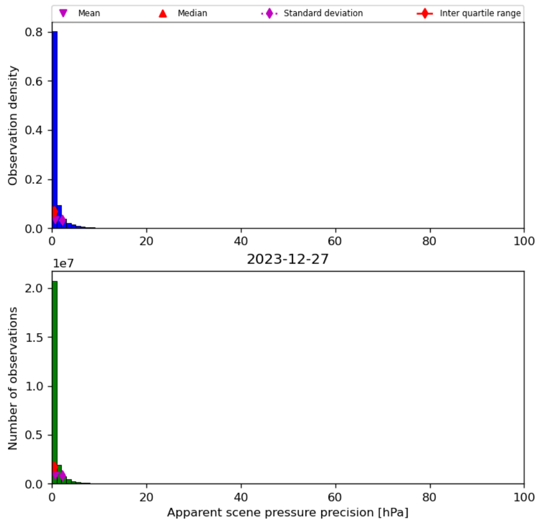
Figure 37: Histogram of “Apparent scene pressure precision” for 2023-12-26 to 2023-12-28
