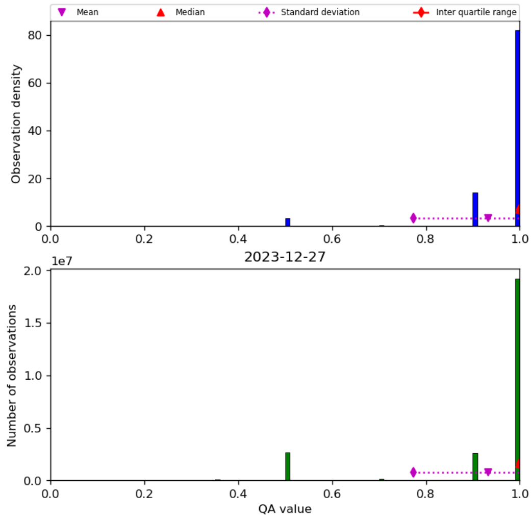
Figure 29: Histogram of “QA value” for 2023-12-26 to 2023-12-28
