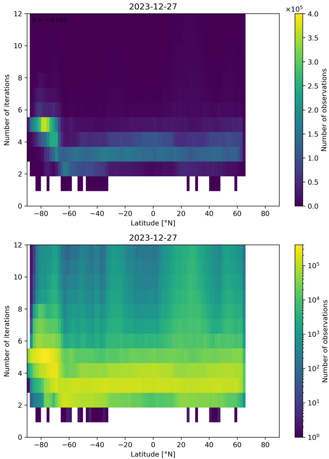
Figure 93: Scatter density plot of “Latitude” against “Number of iterations” for 2023-12-26 to 2023-12-28.
