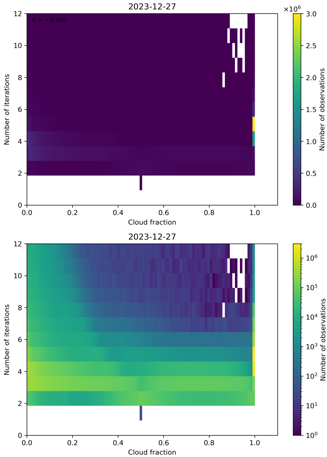
Figure 73: Scatter density plot of “Cloud fraction” against “Number of iterations” for 2023-12-26 to 2023-12-28.
