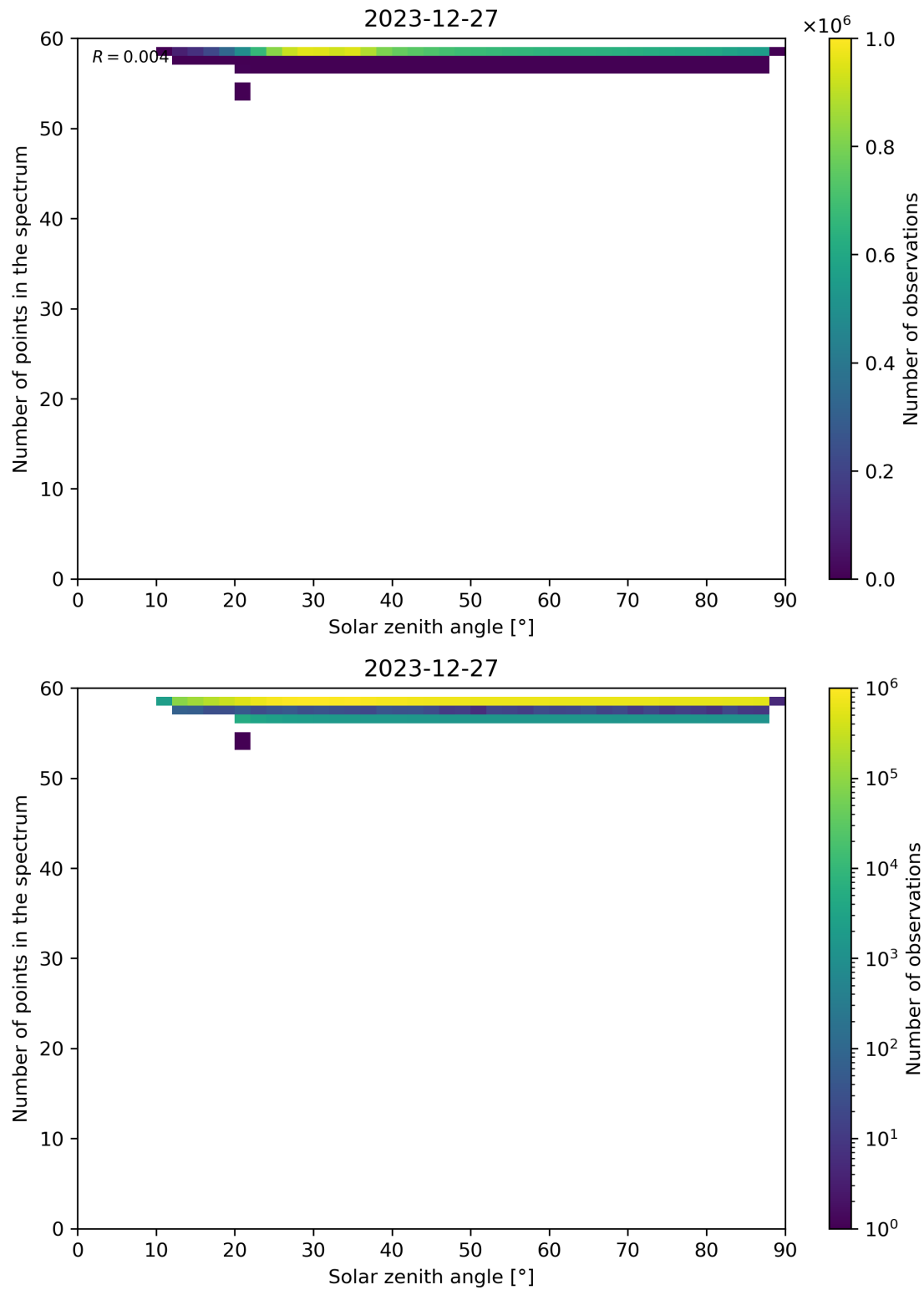
Figure 115: Scatter density plot of “Solar zenith angle” against “Number of points in the spectrum” for 2023-12-26 to 2023-12-28.
