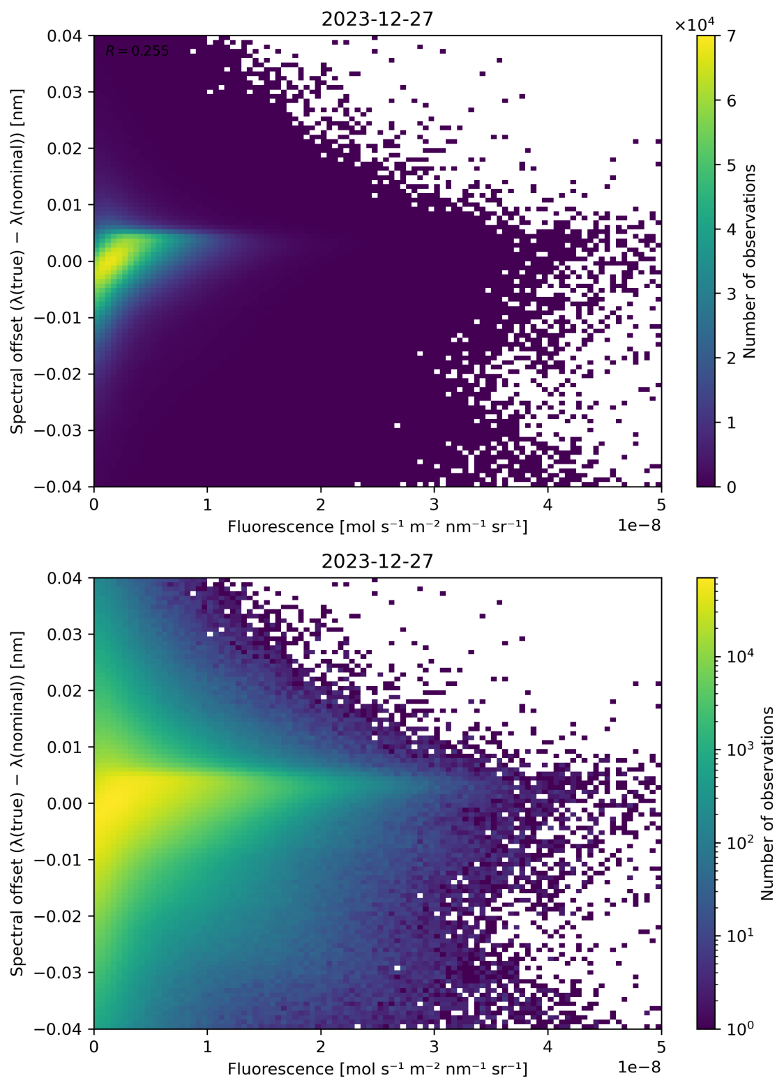
Figure 87: Scatter density plot of “Fluorescence” against “Spectral offset ( \lambda(\text{true}) - \lambda(\text{nominal}) )” for 2023-12-26 to 2023-12-28.
