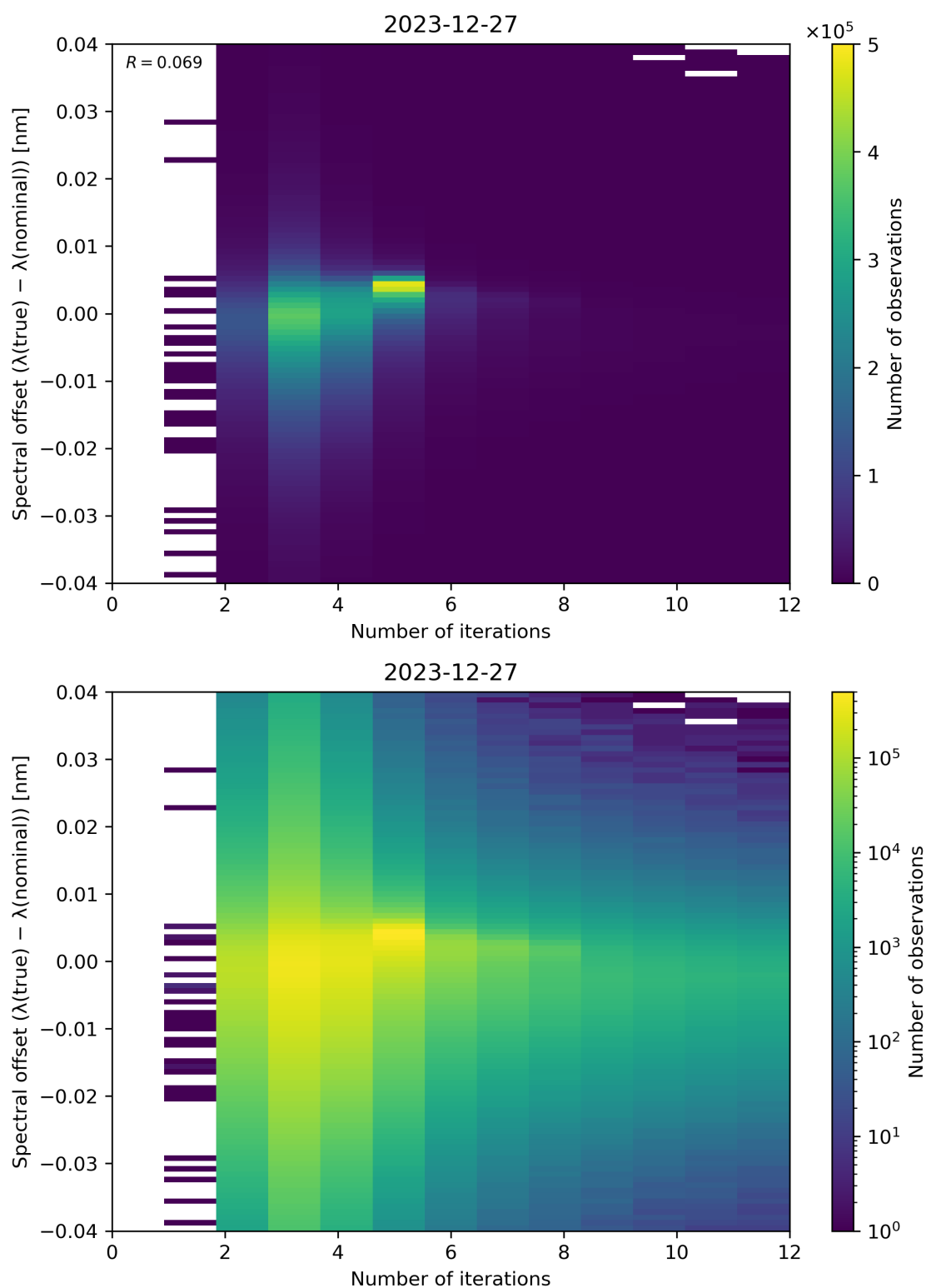
Figure 100: Scatter density plot of “Number of iterations” against “Spectral offset ( \lambda(\text{true}) - \lambda(\text{nominal}) )” for 2023-12-26 to 2023-12-28.
