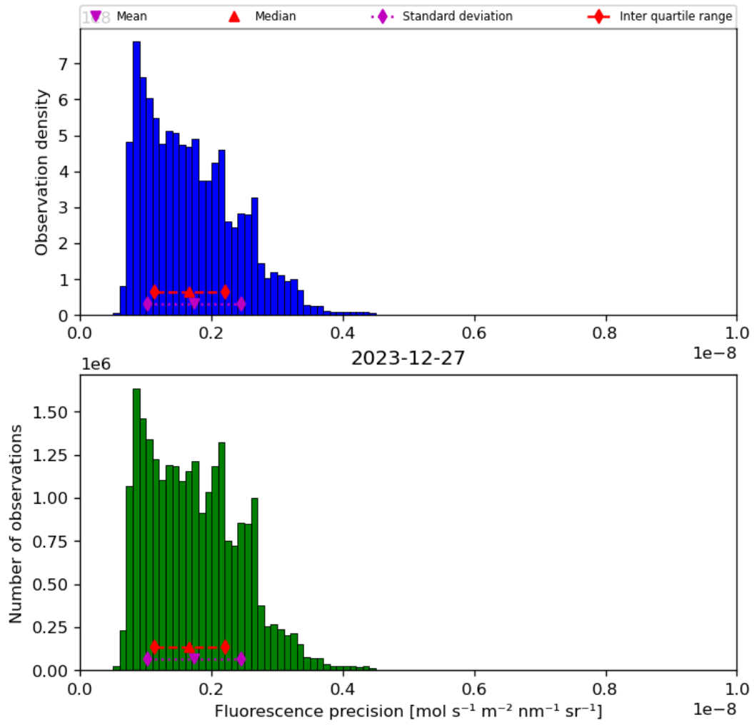
Figure 41: Histogram of “Fluorescence precision” for 2023-12-26 to 2023-12-28
