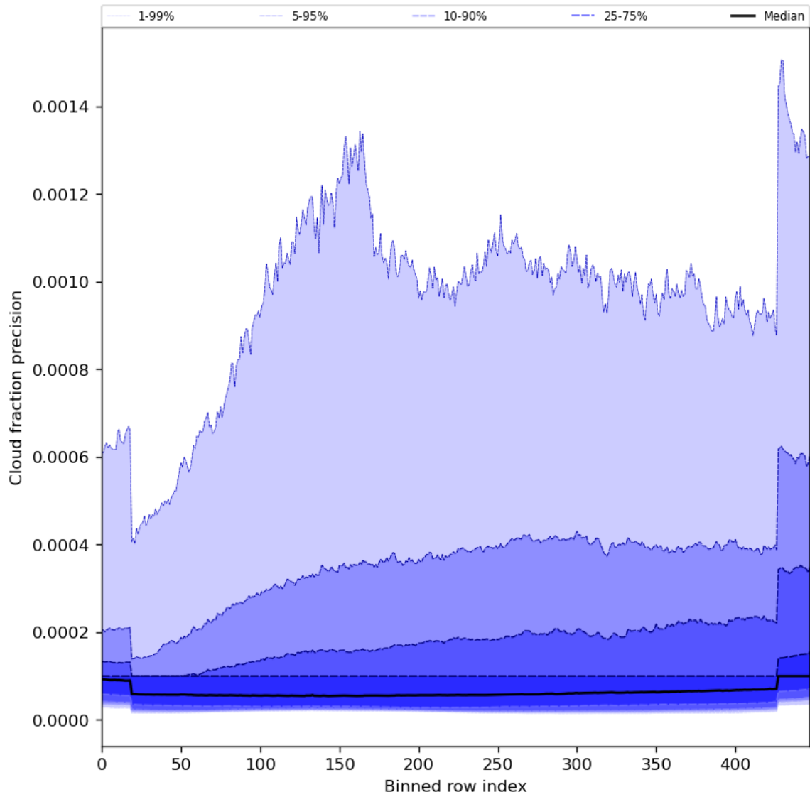
Figure 50: Along track statistics of “Cloud fraction precision” for 2023-12-26 to 2023-12-28
