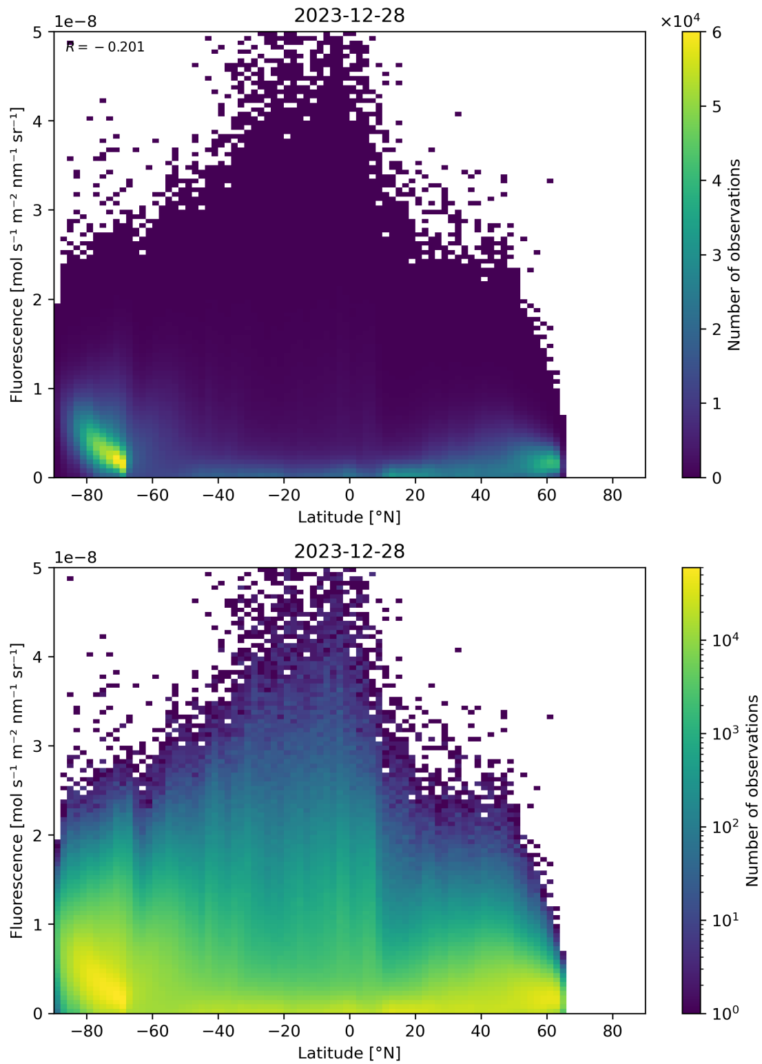
Figure 92: Scatter density plot of “Latitude” against “Fluorescence” for 2023-12-27 to 2023-12-29.
