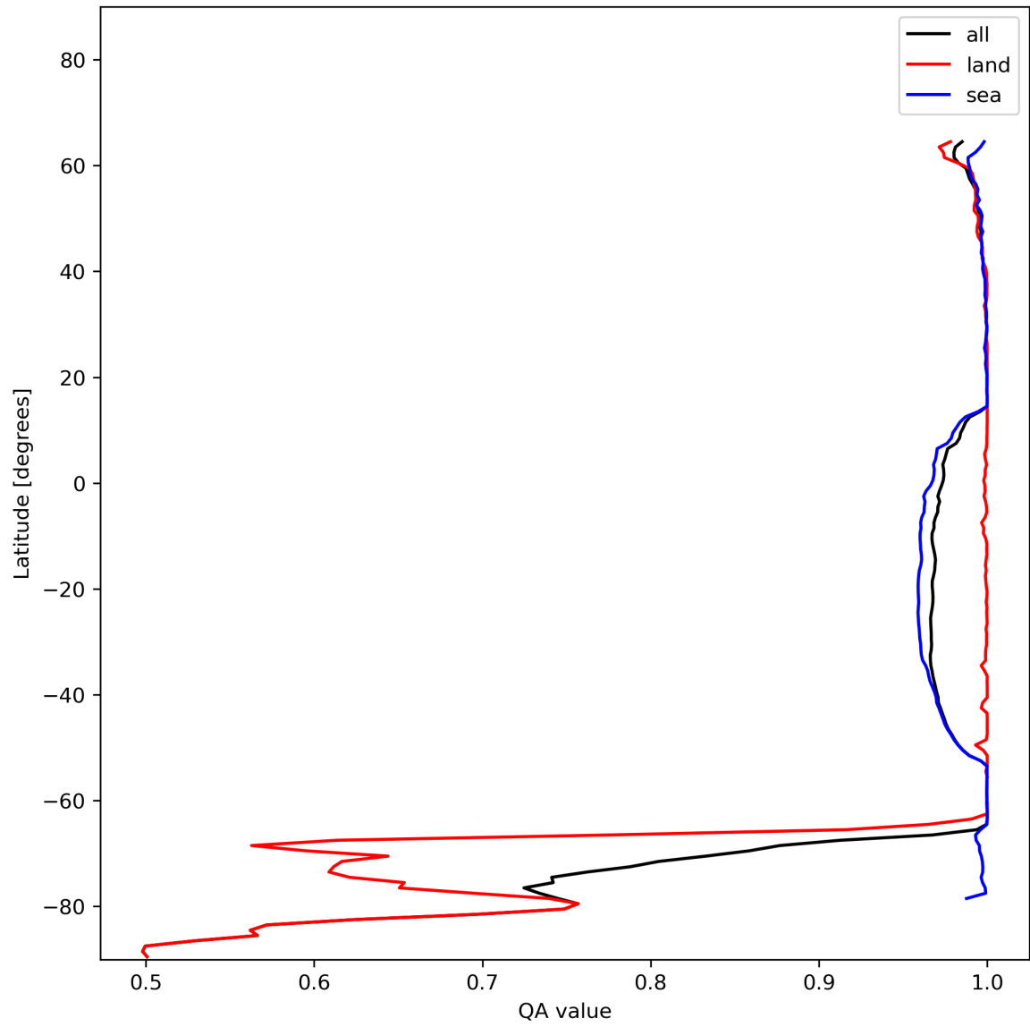
Figure 12: Zonal average of “QA value” for 2023-12-27 to 2023-12-29.
