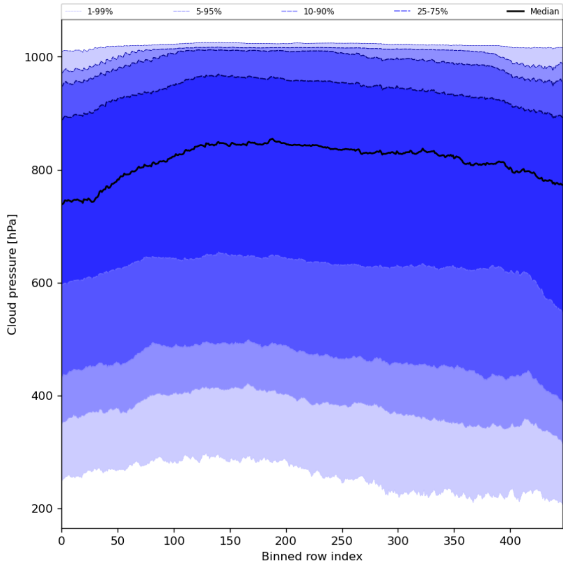
Figure 47: Along track statistics of “Cloud pressure” for 2023-12-27 to 2023-12-29
