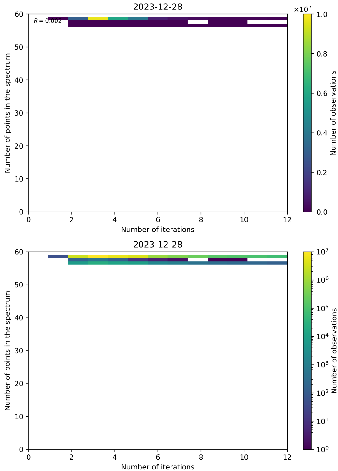
Figure 99: Scatter density plot of “Number of iterations” against “Number of points in the spectrum” for 2023-12-27 to 2023-12-29.
