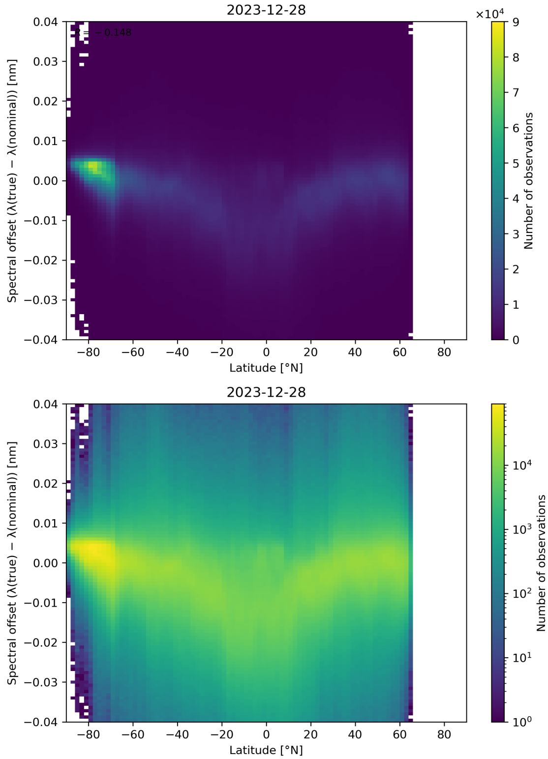
Figure 96: Scatter density plot of “Latitude” against “Spectral offset ( \lambda(\text{true}) - \lambda(\text{nominal}) )” for 2023-12-27 to 2023-12-29.
