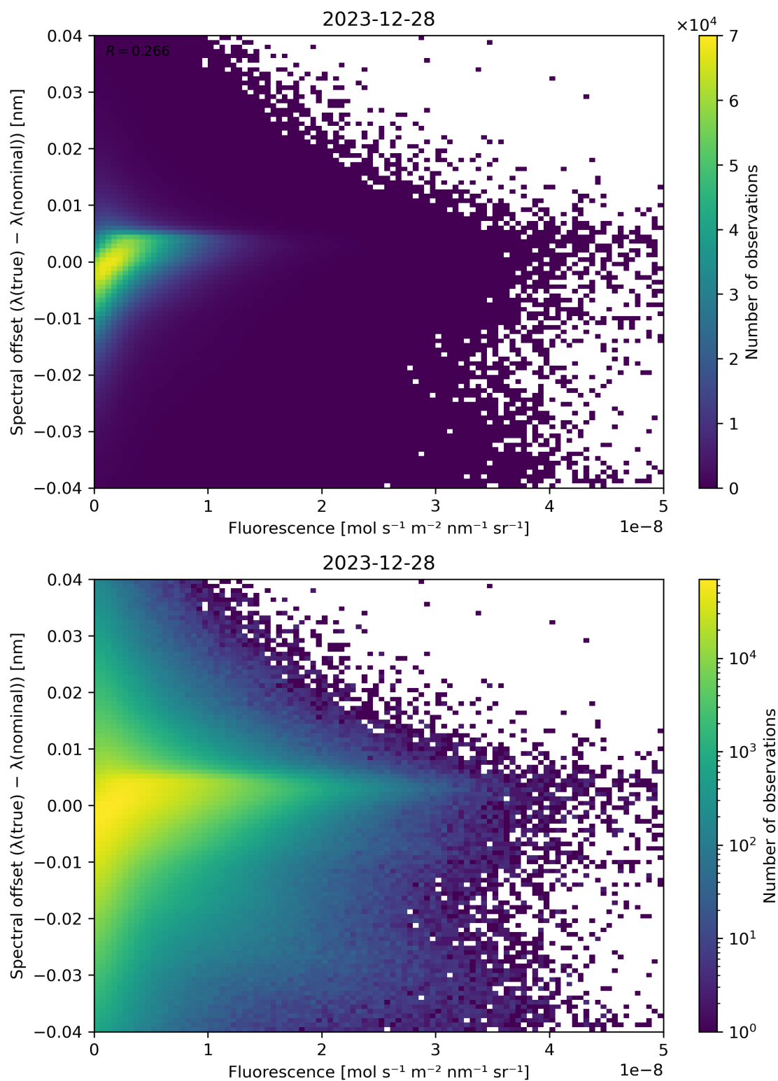
Figure 87: Scatter density plot of “Fluorescence” against “Spectral offset ( \lambda(\text{true}) - \lambda(\text{nominal}) )” for 2023-12-27 to 2023-12-29.
