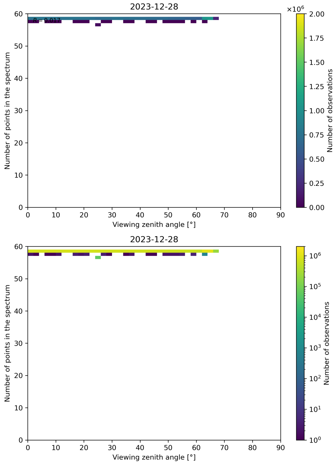
Figure 125: Scatter density plot of “Viewing zenith angle” against “Number of points in the spectrum” for 2023-12-27 to 2023-12-29.
