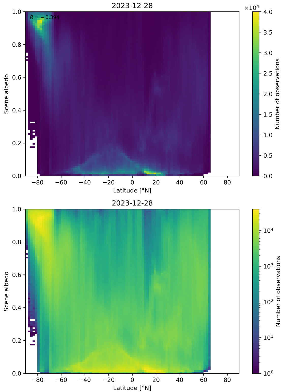
Figure 95: Scatter density plot of “Latitude” against “Scene albedo” for 2023-12-27 to 2023-12-29.
