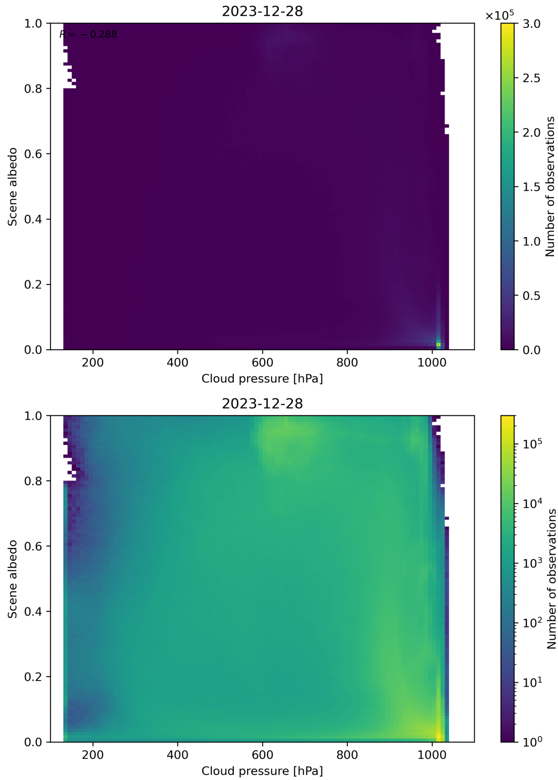
Figure 83: Scatter density plot of “Cloud pressure” against “Scene albedo” for 2023-12-27 to 2023-12-29.
