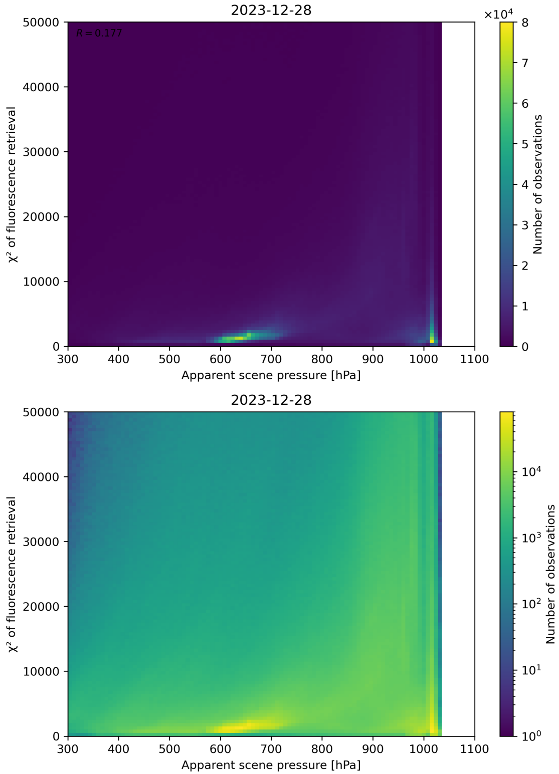
Figure 63: Scatter density plot of “Apparent scene pressure” against “ \chi^2 of fluorescence retrieval” for 2023-12-27 to 2023-12-29.
