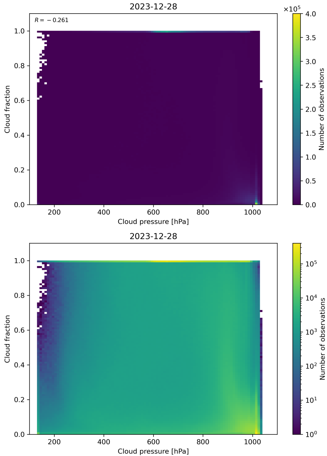
Figure 79: Scatter density plot of “Cloud pressure” against “Cloud fraction” for 2023-12-27 to 2023-12-29.
