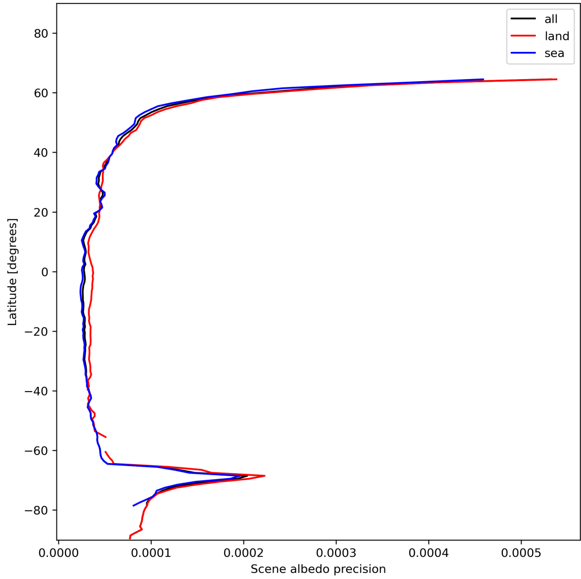
Figure 18: Zonal average of “Scene albedo precision” for 2023-12-27 to 2023-12-29.
