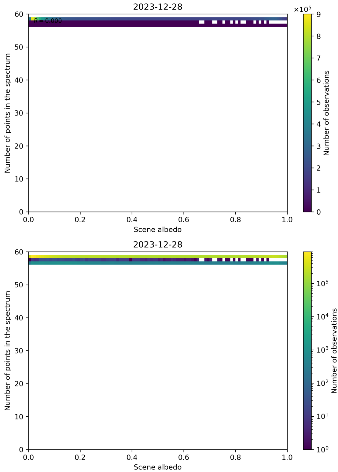
Figure 106: Scatter density plot of “Scene albedo” against “Number of points in the spectrum” for 2023-12-27 to 2023-12-29.
