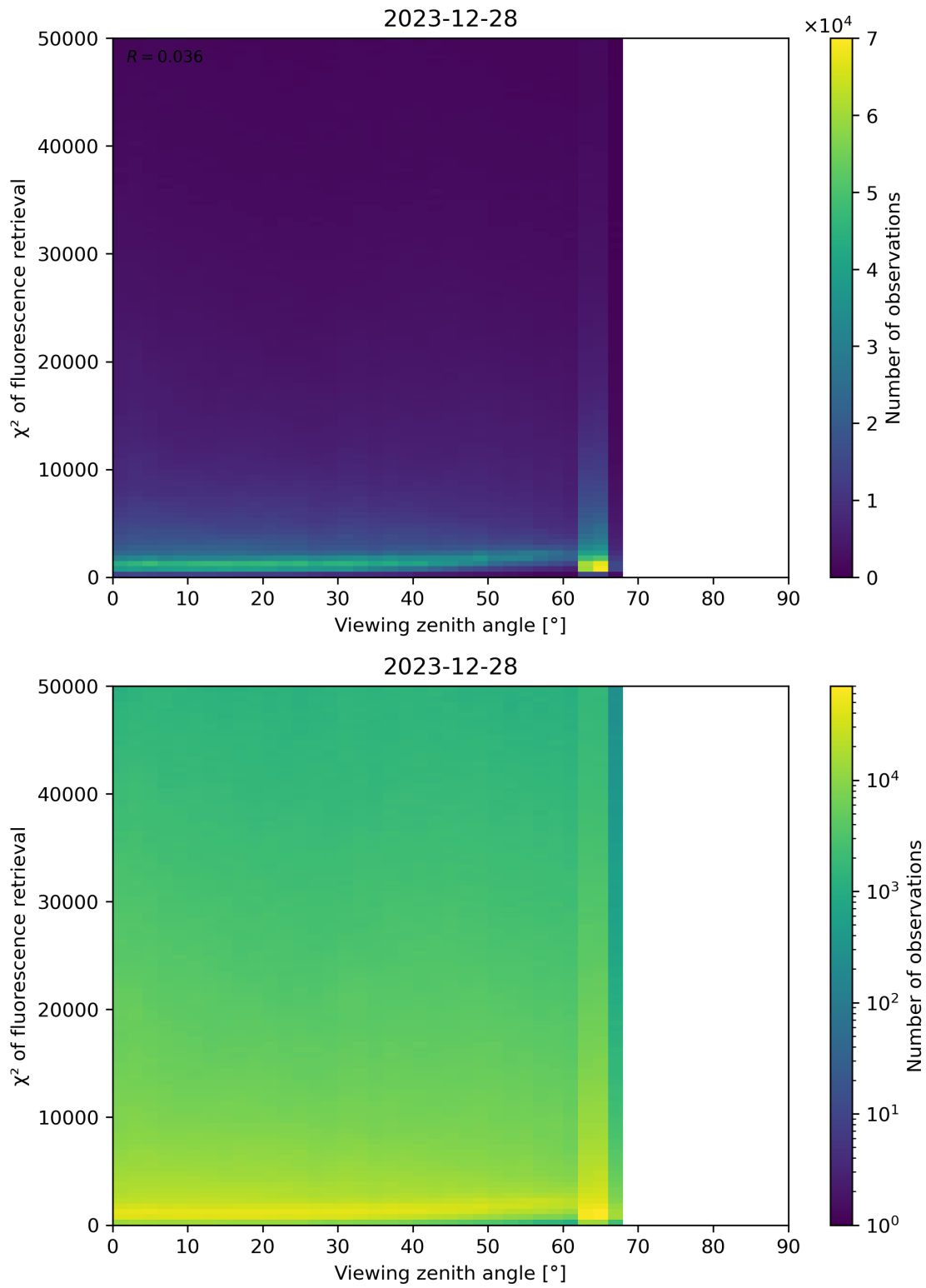
Figure 119: Scatter density plot of “Viewing zenith angle” against “ \chi^2 of fluorescence retrieval” for 2023-12-27 to 2023-12-29.
