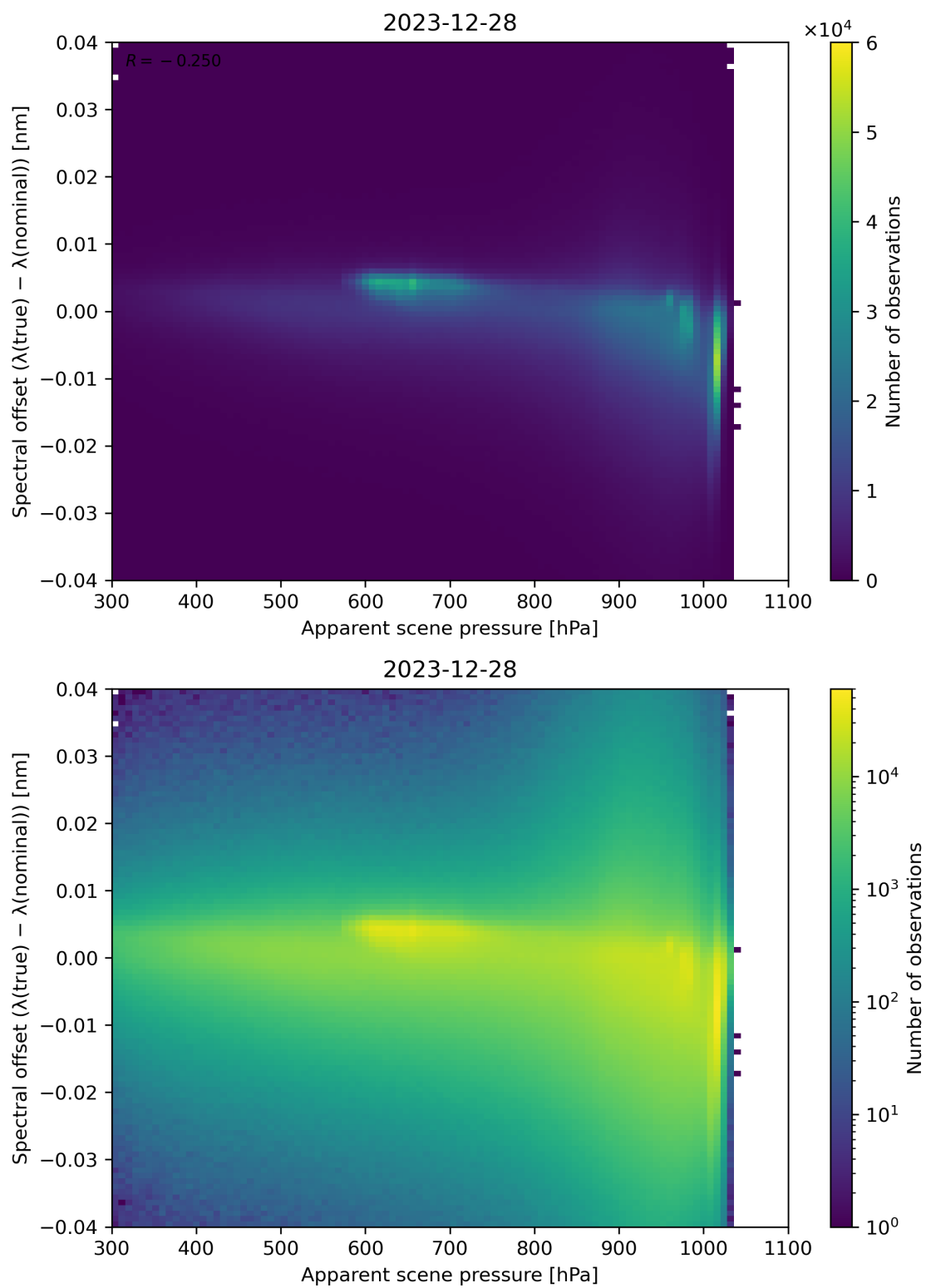
Figure 67: Scatter density plot of “Apparent scene pressure” against “Spectral offset ( \lambda(\text{true}) - \lambda(\text{nominal}) )” for 2023-12-27 to 2023-12-29.
