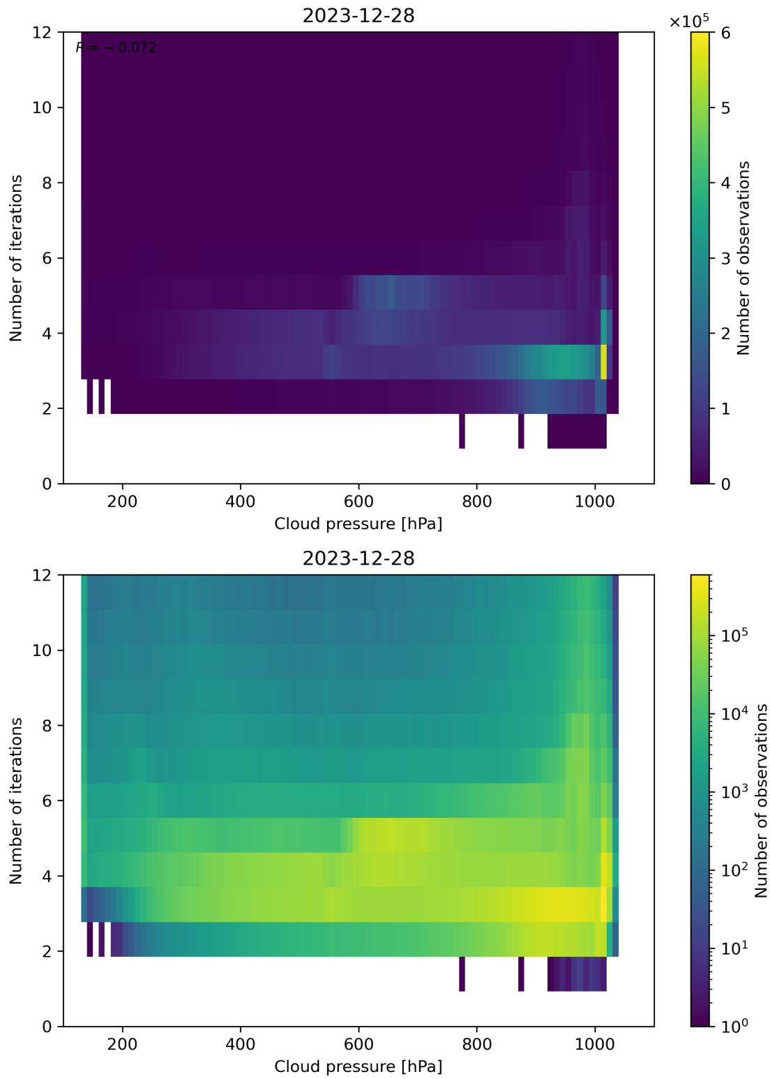
Figure 81: Scatter density plot of “Cloud pressure” against “Number of iterations” for 2023-12-27 to 2023-12-29.
