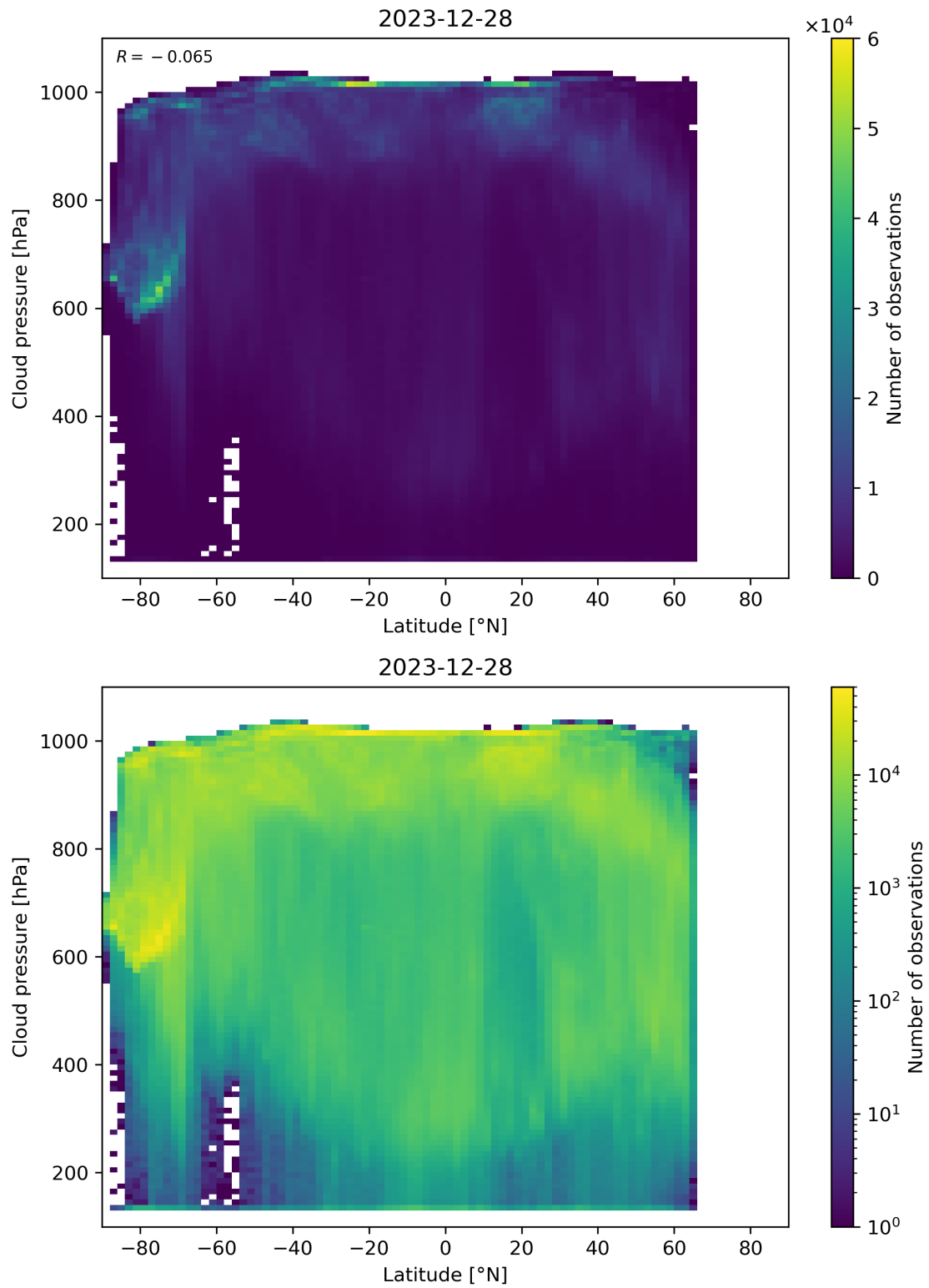
Figure 91: Scatter density plot of “Latitude” against “Cloud pressure” for 2023-12-27 to 2023-12-29.
