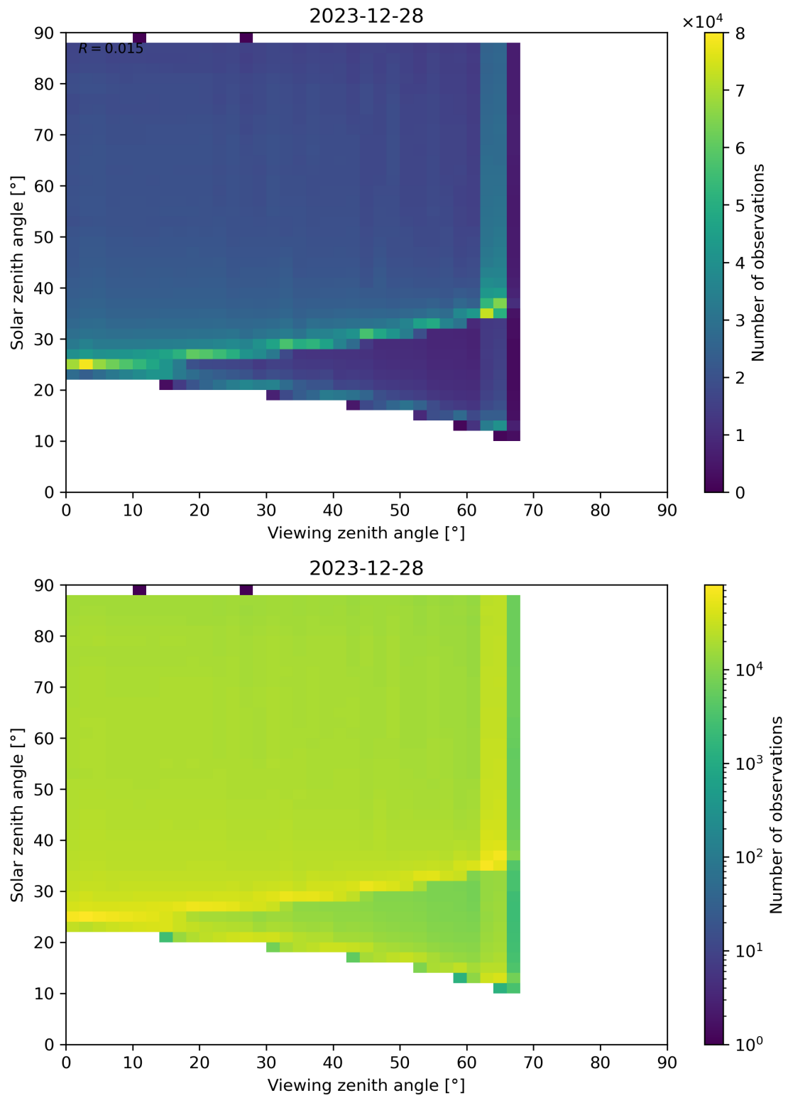
Figure 127: Scatter density plot of “Viewing zenith angle” against “Solar zenith angle” for 2023-12-27 to 2023-12-29.
