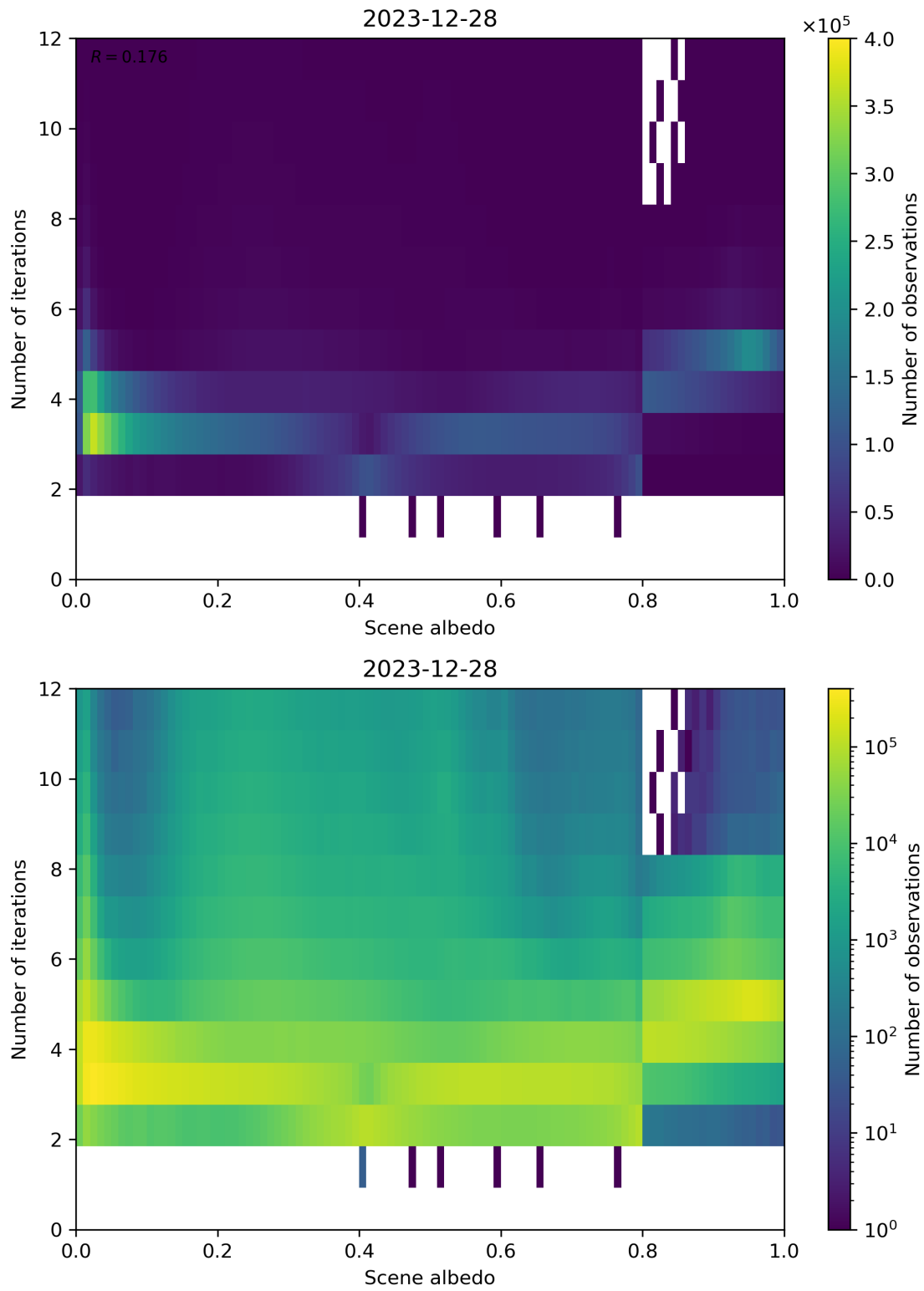
Figure 105: Scatter density plot of “Scene albedo” against “Number of iterations” for 2023-12-27 to 2023-12-29.
