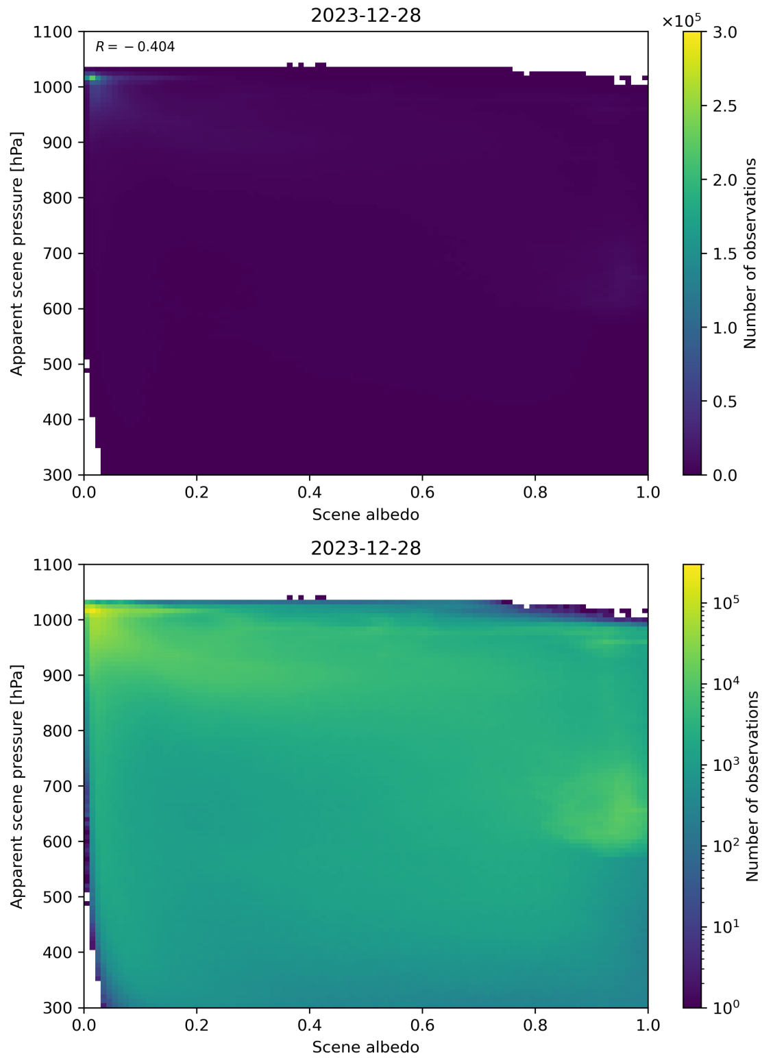
Figure 102: Scatter density plot of “Scene albedo” against “Apparent scene pressure” for 2023-12-27 to 2023-12-29.
