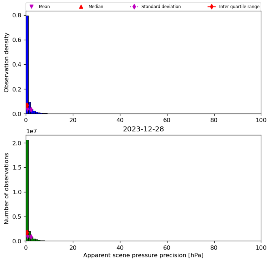
Figure 37: Histogram of “Apparent scene pressure precision” for 2023-12-27 to 2023-12-29
