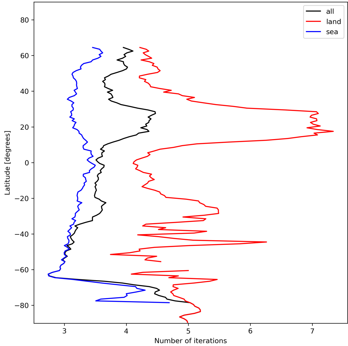
Figure 22: Zonal average of “Number of iterations” for 2023-12-27 to 2023-12-29.
