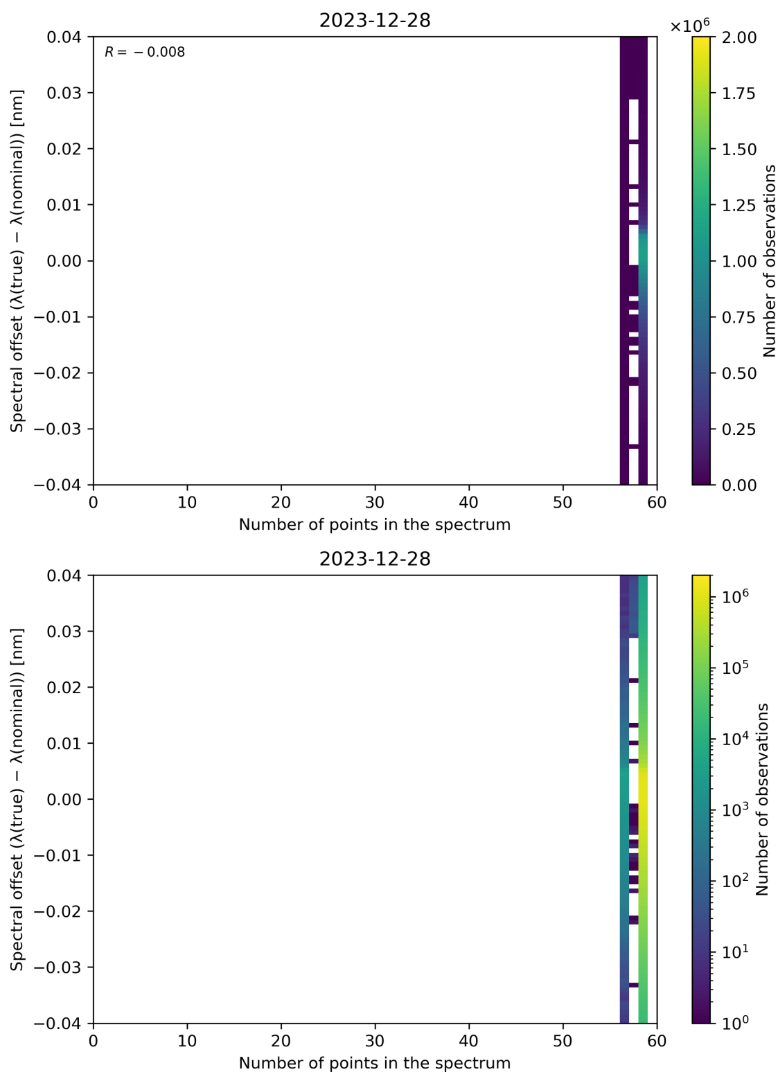
Figure 101: Scatter density plot of “Number of points in the spectrum” against “Spectral offset ( \lambda(\text{true}) - \lambda(\text{nominal}) )” for 2023-12-27 to 2023-12-29.
