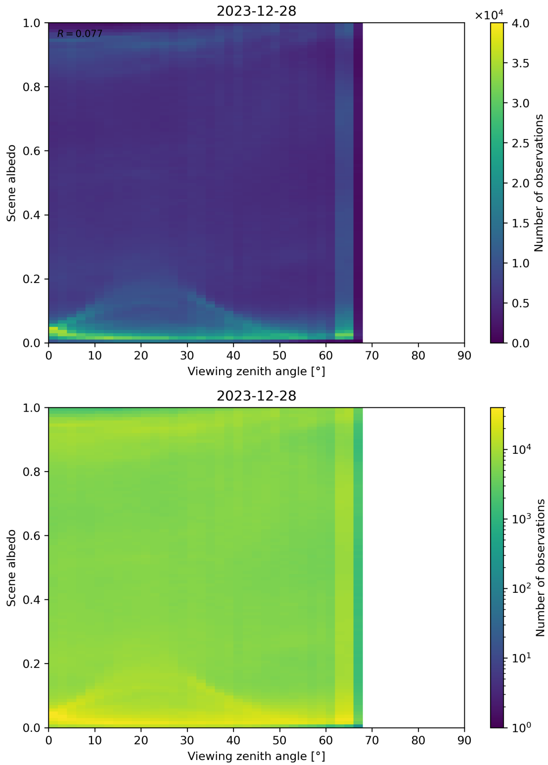
Figure 126: Scatter density plot of “Viewing zenith angle” against “Scene albedo” for 2023-12-27 to 2023-12-29.
