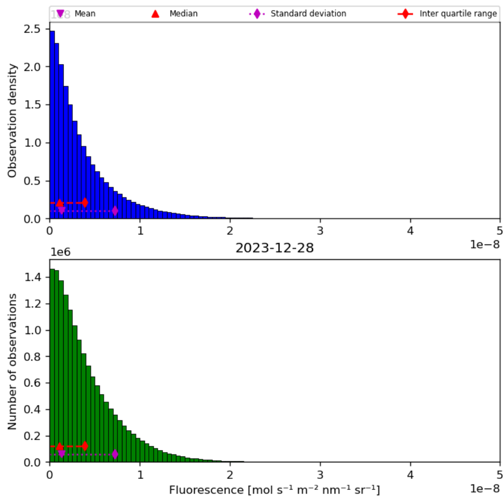
Figure 40: Histogram of “Fluorescence” for 2023-12-27 to 2023-12-29
