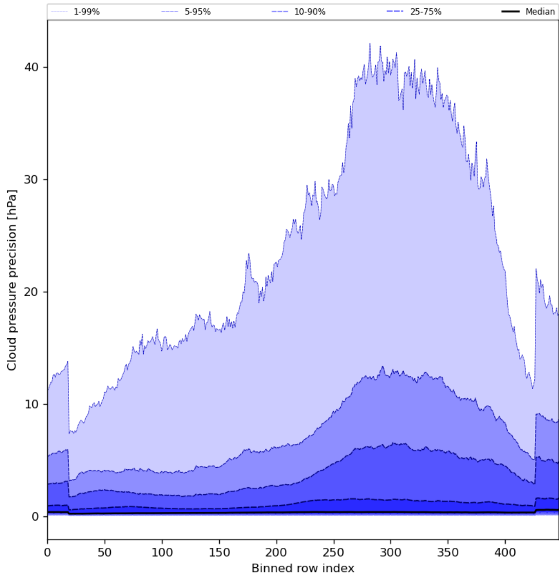
Figure 48: Along track statistics of “Cloud pressure precision” for 2023-12-27 to 2023-12-29
