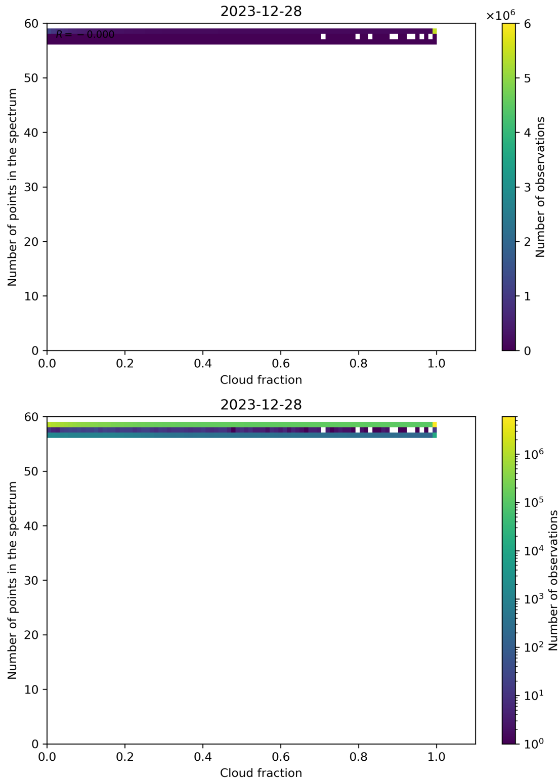
Figure 74: Scatter density plot of “Cloud fraction” against “Number of points in the spectrum” for 2023-12-27 to 2023-12-29.
