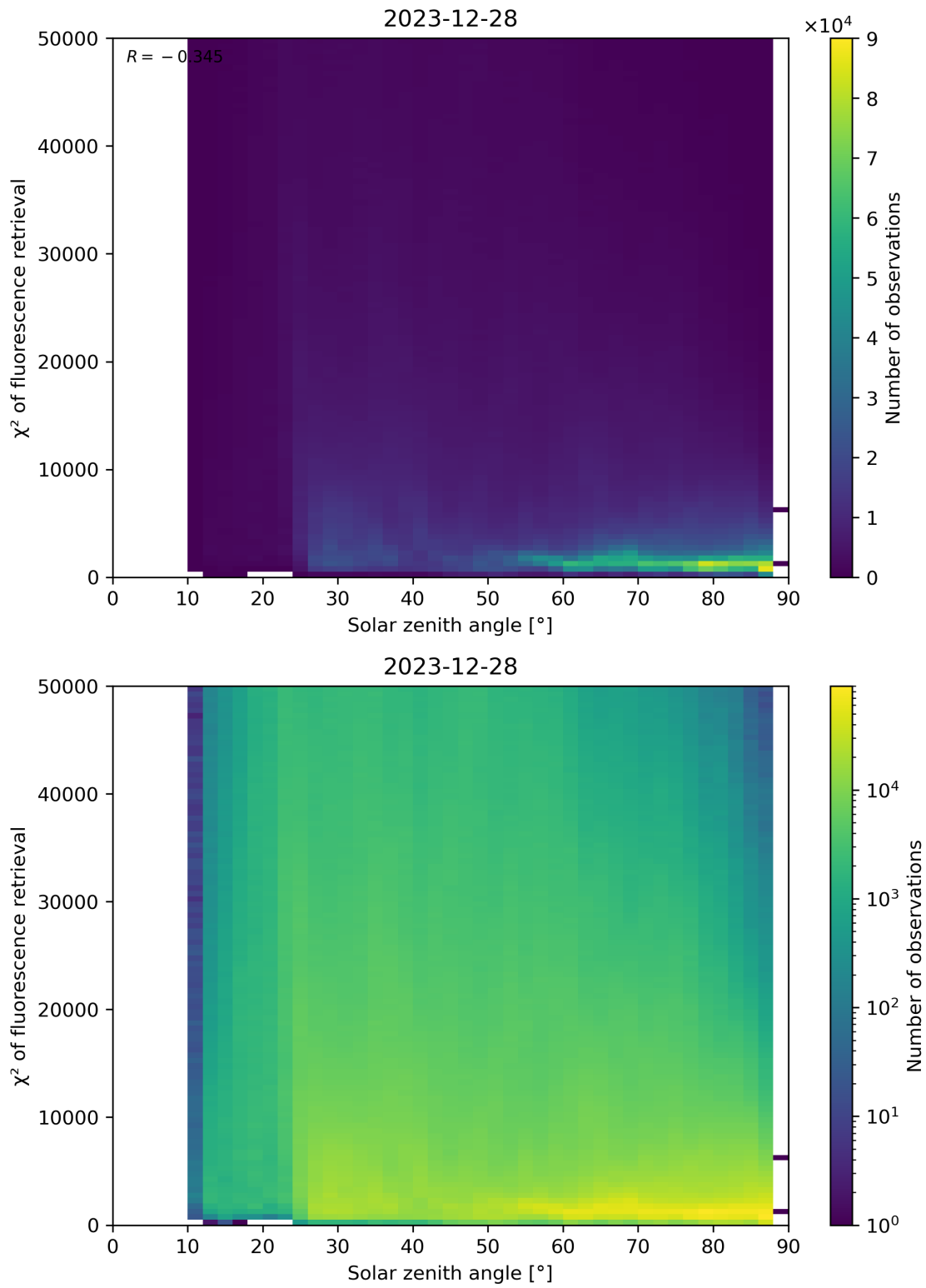
Figure 109: Scatter density plot of “Solar zenith angle” against “ \chi^2 of fluorescence retrieval” for 2023-12-27 to 2023-12-29.
