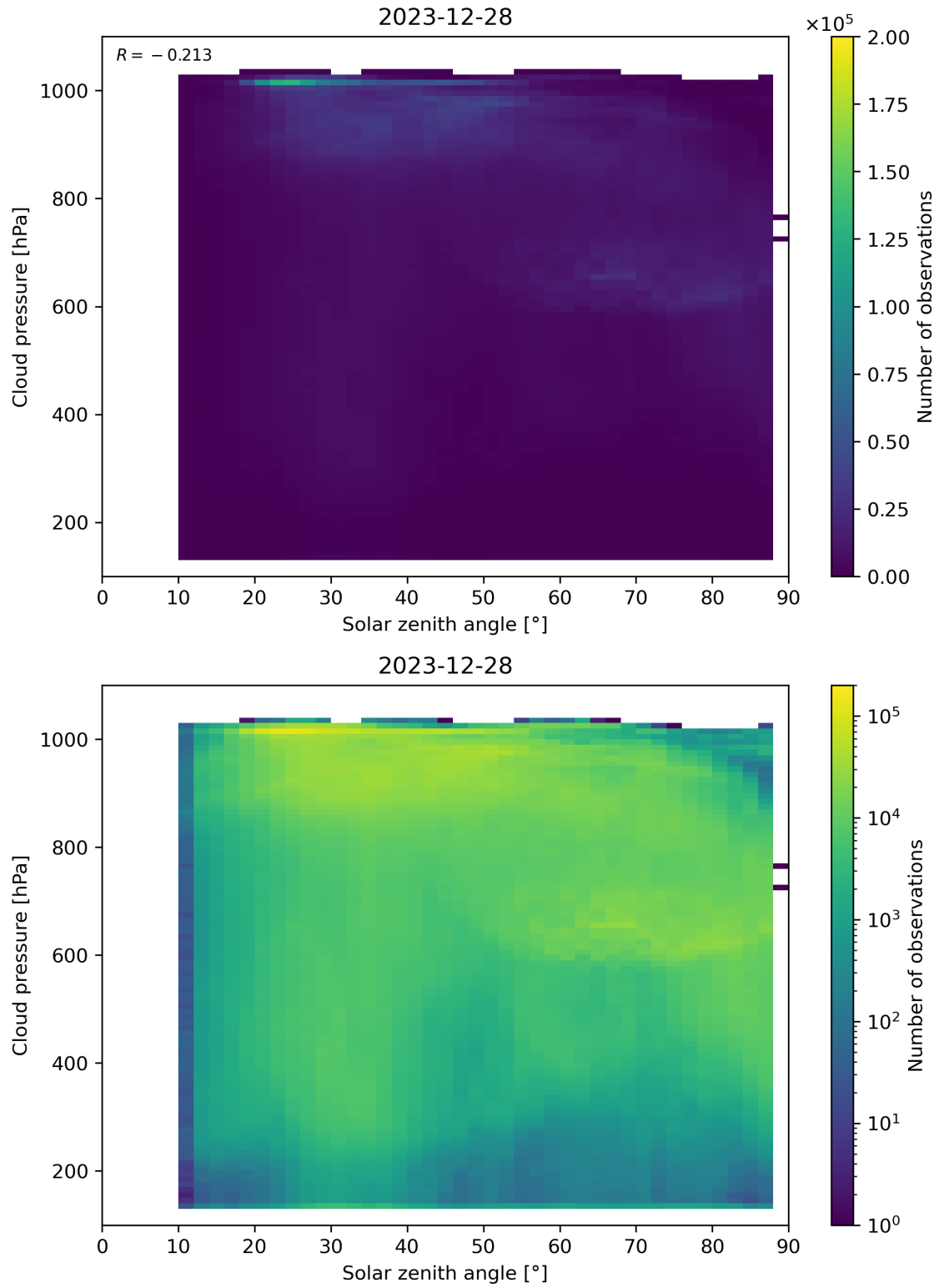
Figure 111: Scatter density plot of “Solar zenith angle” against “Cloud pressure” for 2023-12-27 to 2023-12-29.
