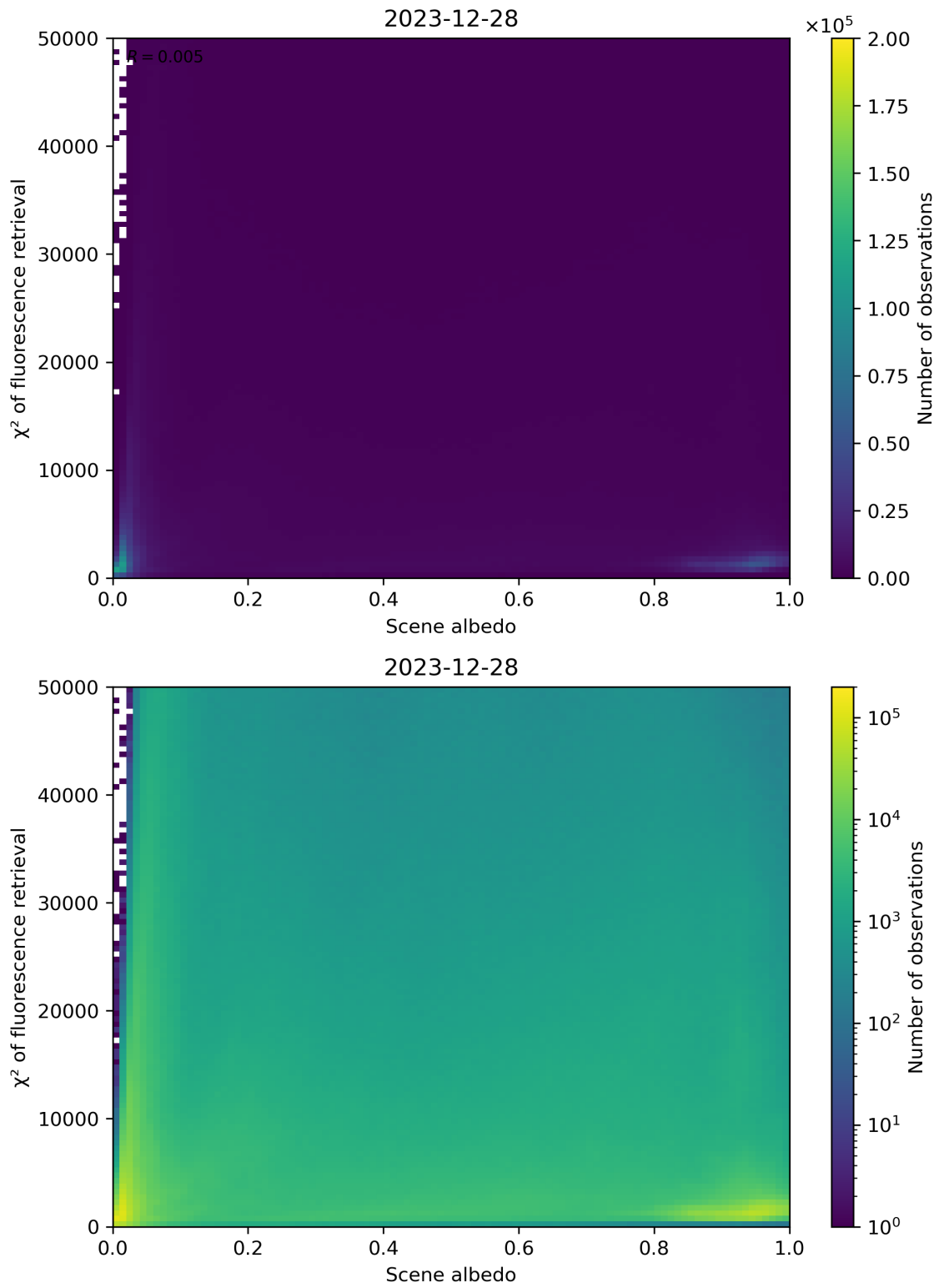
Figure 103: Scatter density plot of “Scene albedo” against “ \chi^2 of fluorescence retrieval” for 2023-12-27 to 2023-12-29.
