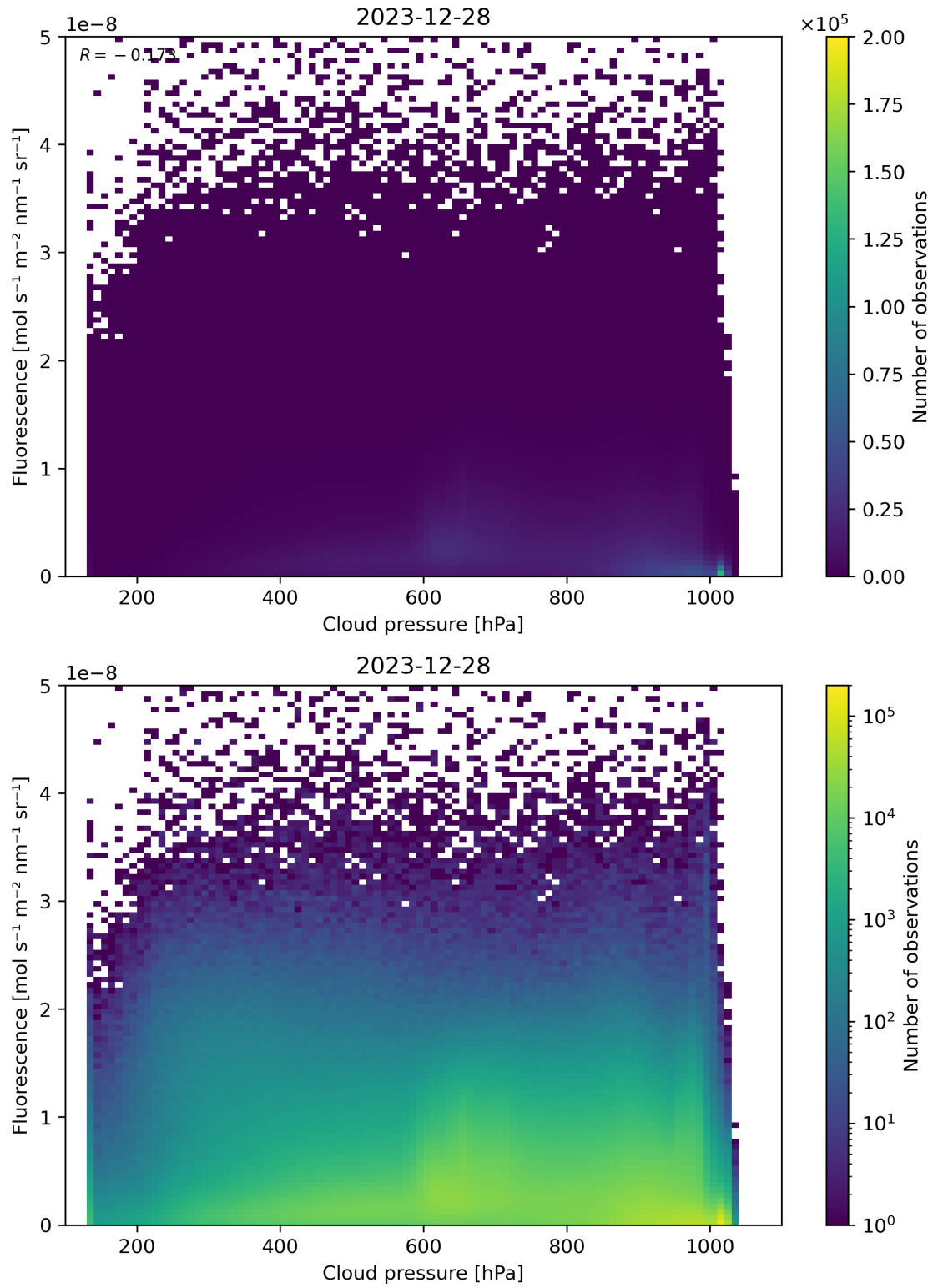
Figure 80: Scatter density plot of “Cloud pressure” against “Fluorescence” for 2023-12-27 to 2023-12-29.
