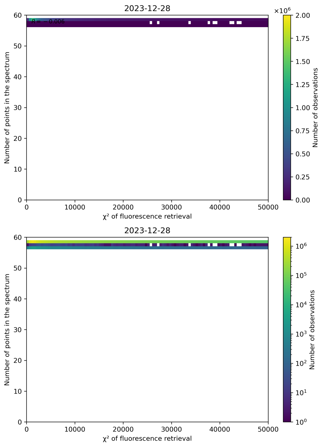
Figure 68: Scatter density plot of " \chi^2 of fluorescence retrieval" against "Number of points in the spectrum" for 2023-12-27 to 2023-12-29.
