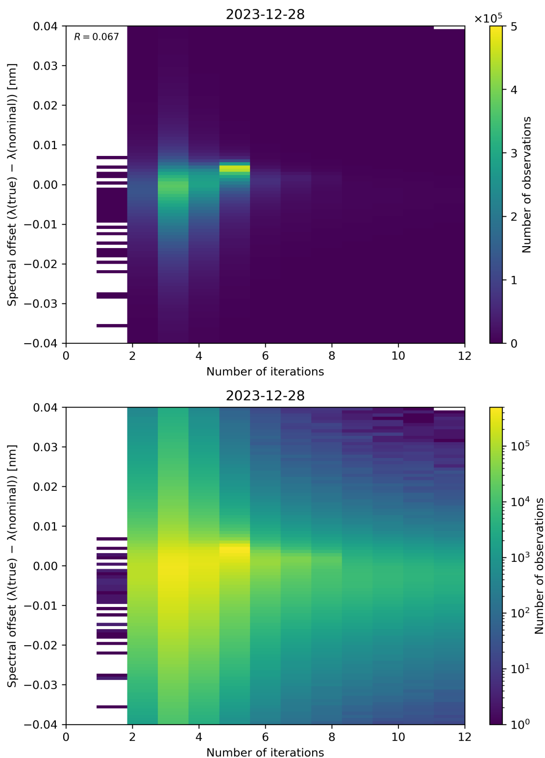
Figure 100: Scatter density plot of “Number of iterations” against “Spectral offset ( \lambda(\text{true}) - \lambda(\text{nominal}) )” for 2023-12-27 to 2023-12-29.
