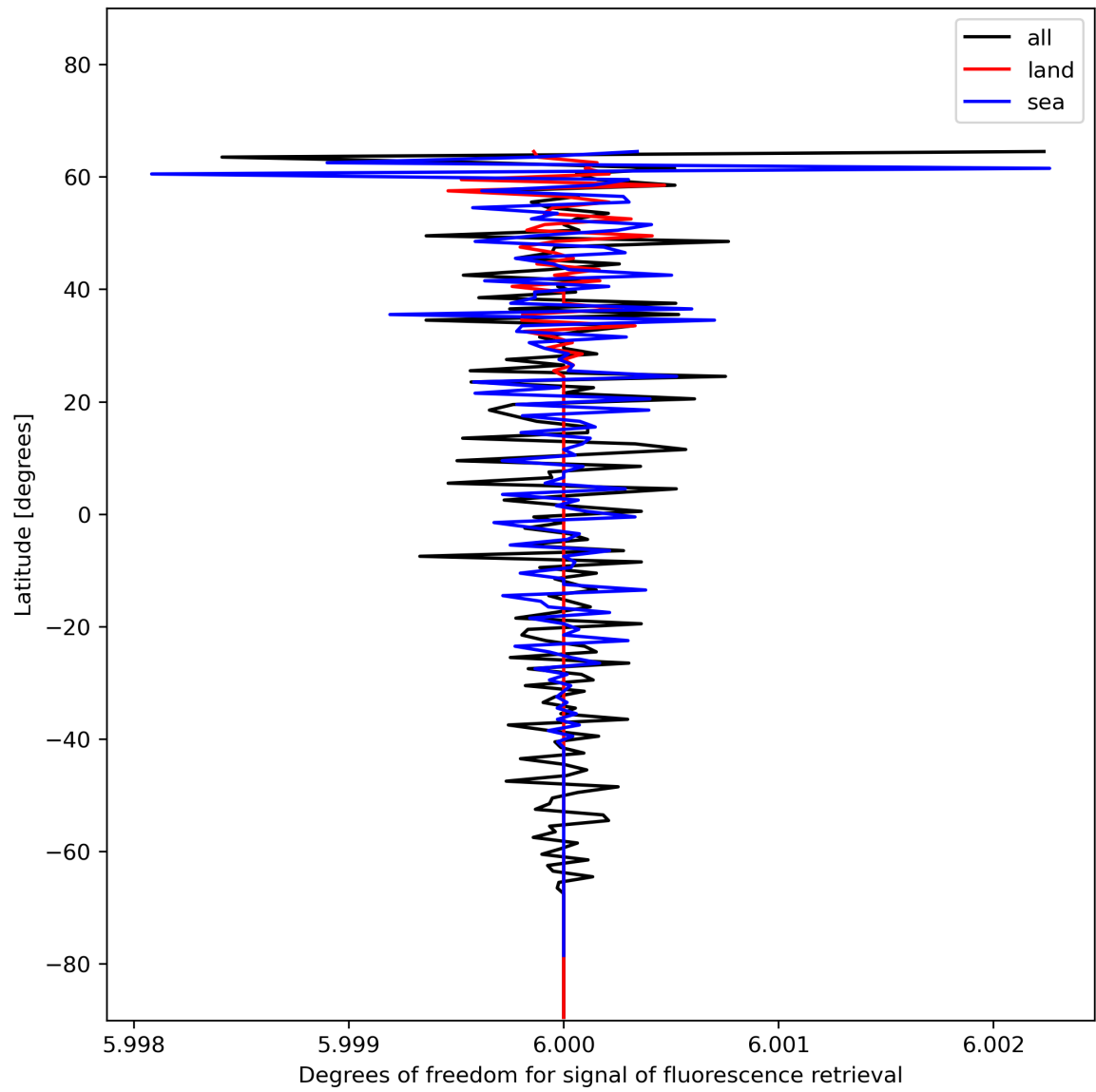
Figure 26: Zonal average of “Degrees of freedom for signal of fluorescence retrieval” for 2023-12-27 to 2023-12-29.
