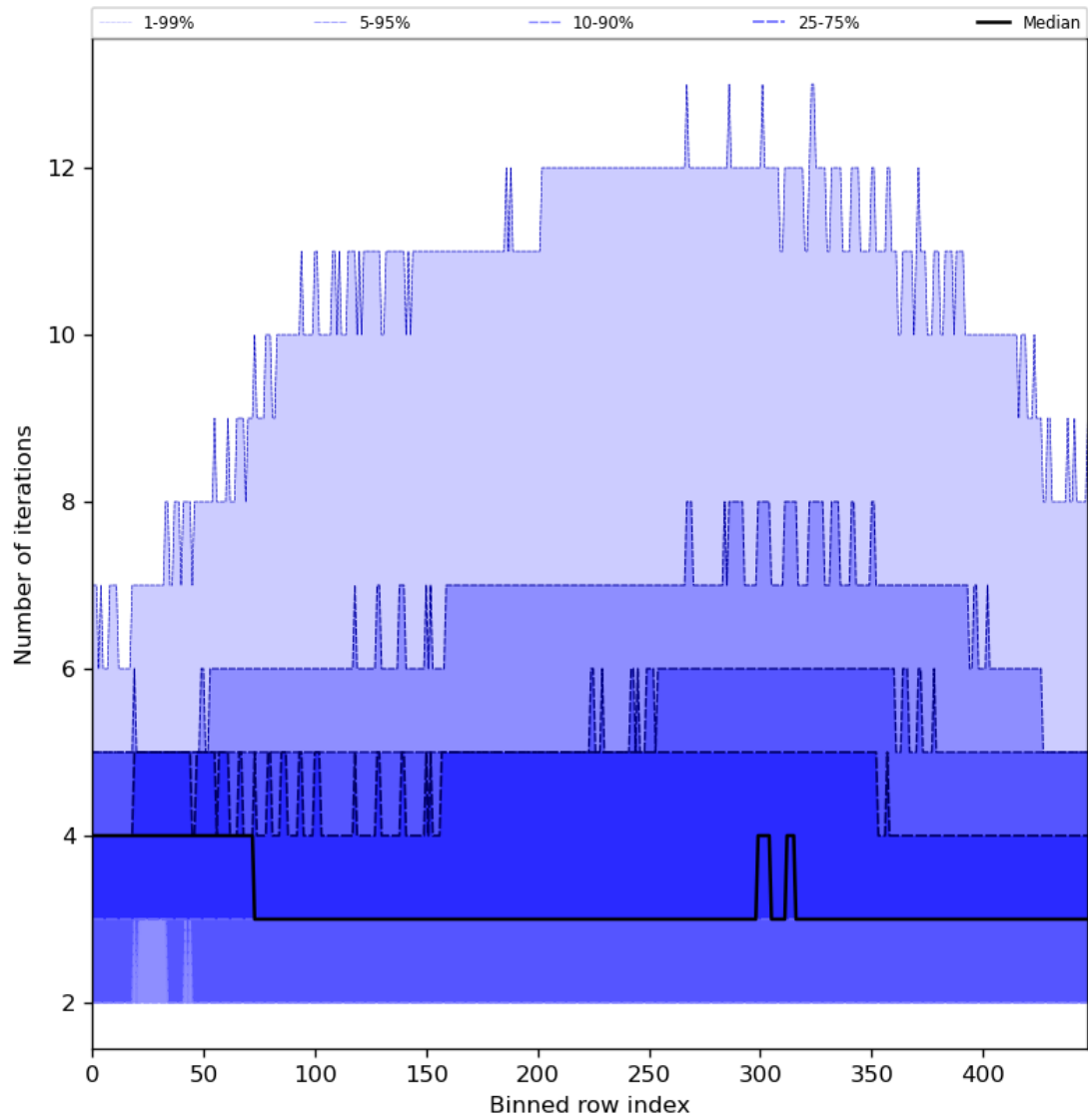
Figure 56: Along track statistics of “Number of iterations” for 2023-12-27 to 2023-12-29
