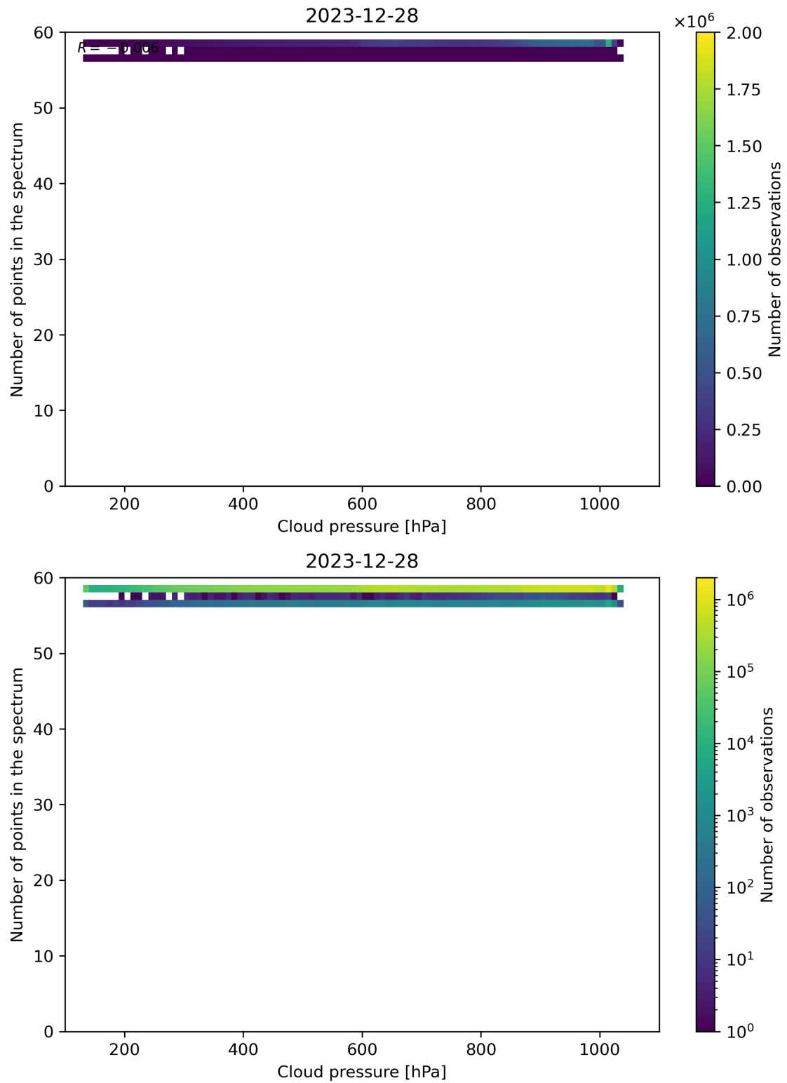
Figure 82: Scatter density plot of “Cloud pressure” against “Number of points in the spectrum” for 2023-12-27 to 2023-12-29.
