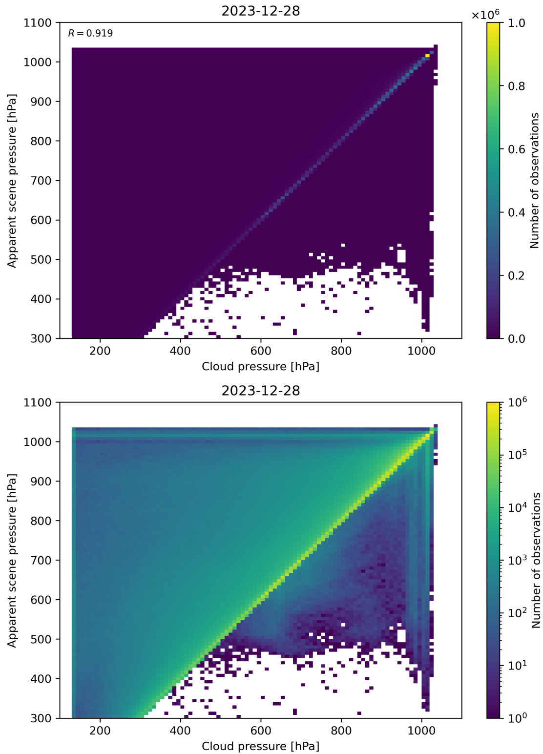
Figure 77: Scatter density plot of “Cloud pressure” against “Apparent scene pressure” for 2023-12-27 to 2023-12-29.
