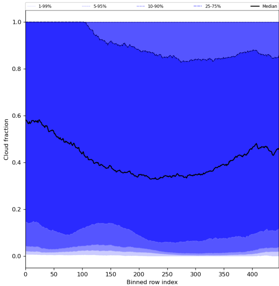
Figure 49: Along track statistics of “Cloud fraction” for 2023-12-27 to 2023-12-29
