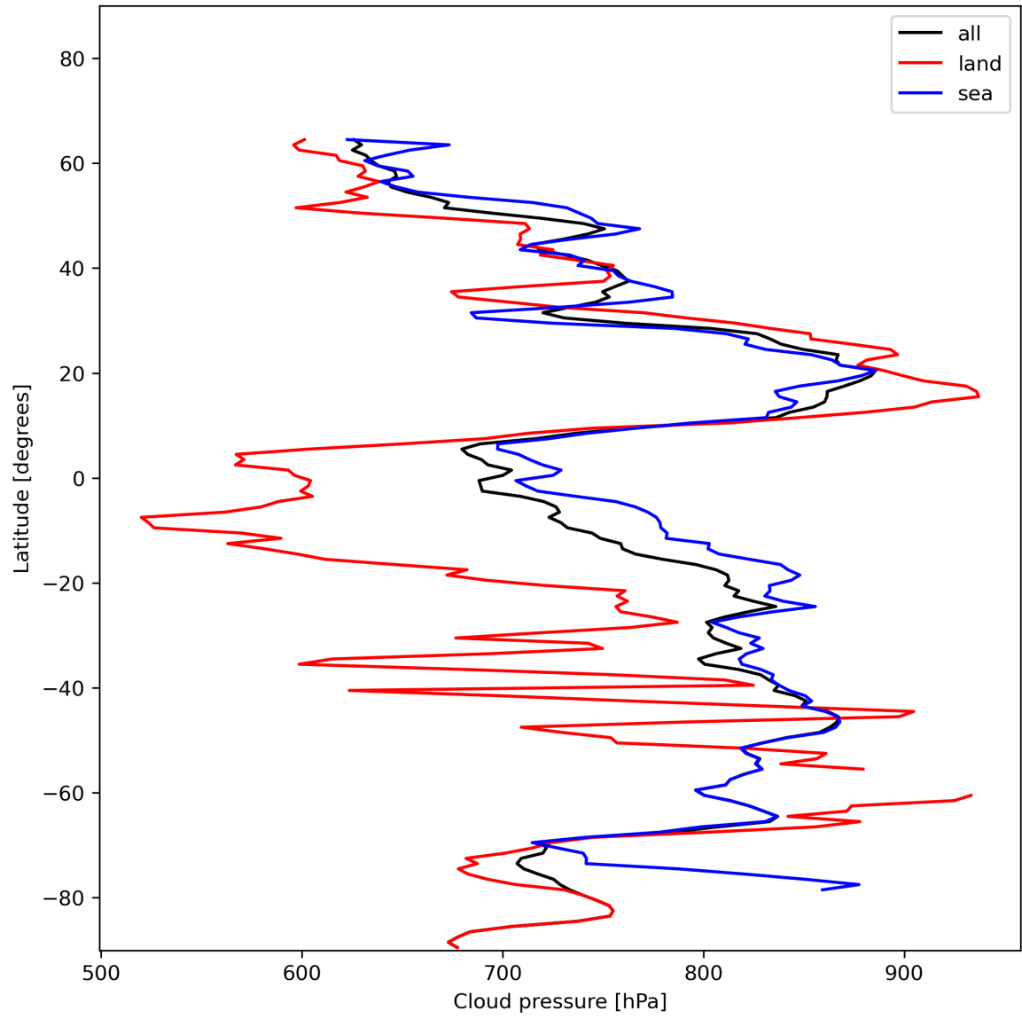
Figure 13: Zonal average of “Cloud pressure” for 2023-12-27 to 2023-12-29.
