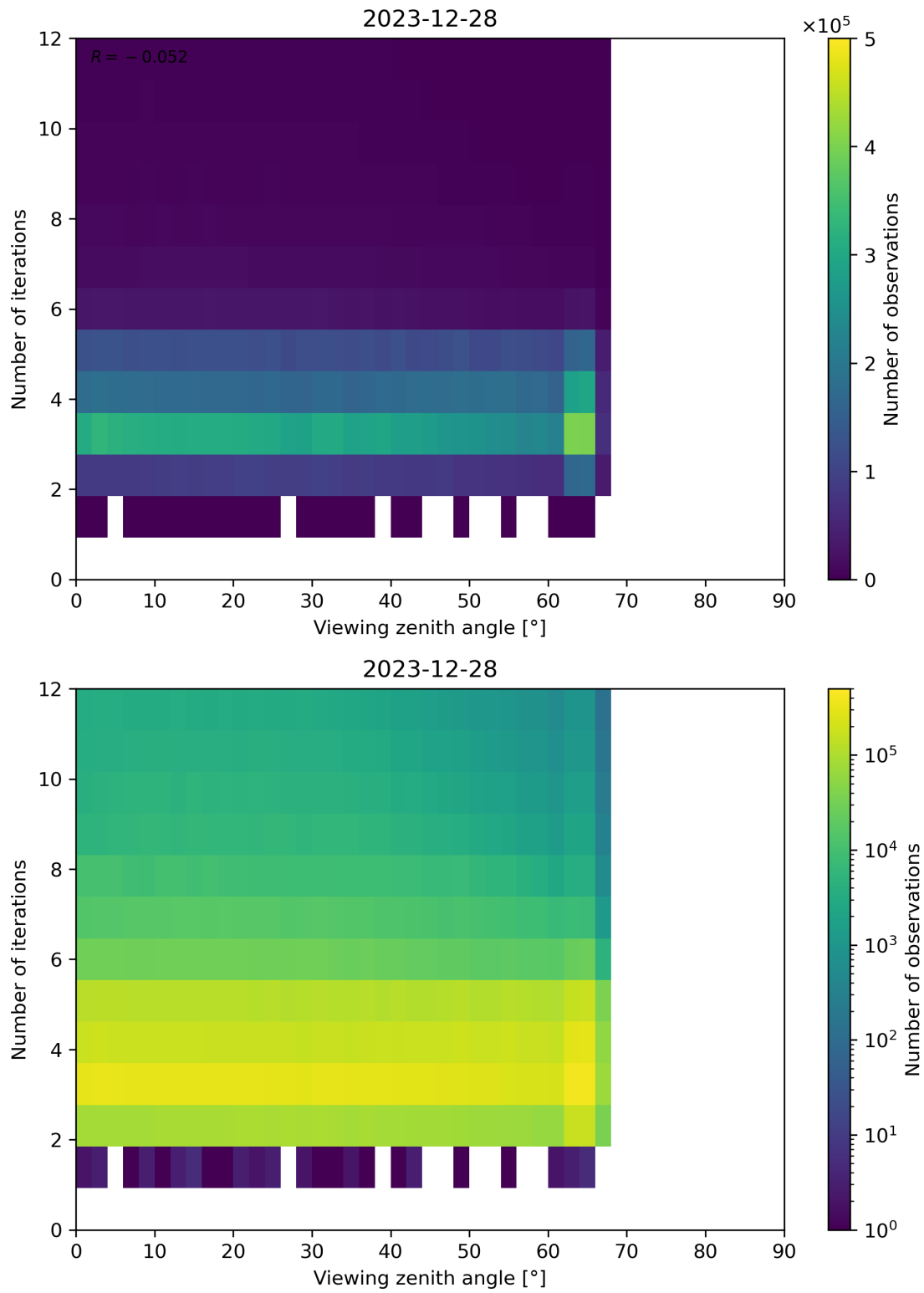
Figure 124: Scatter density plot of “Viewing zenith angle” against “Number of iterations” for 2023-12-27 to 2023-12-29.
