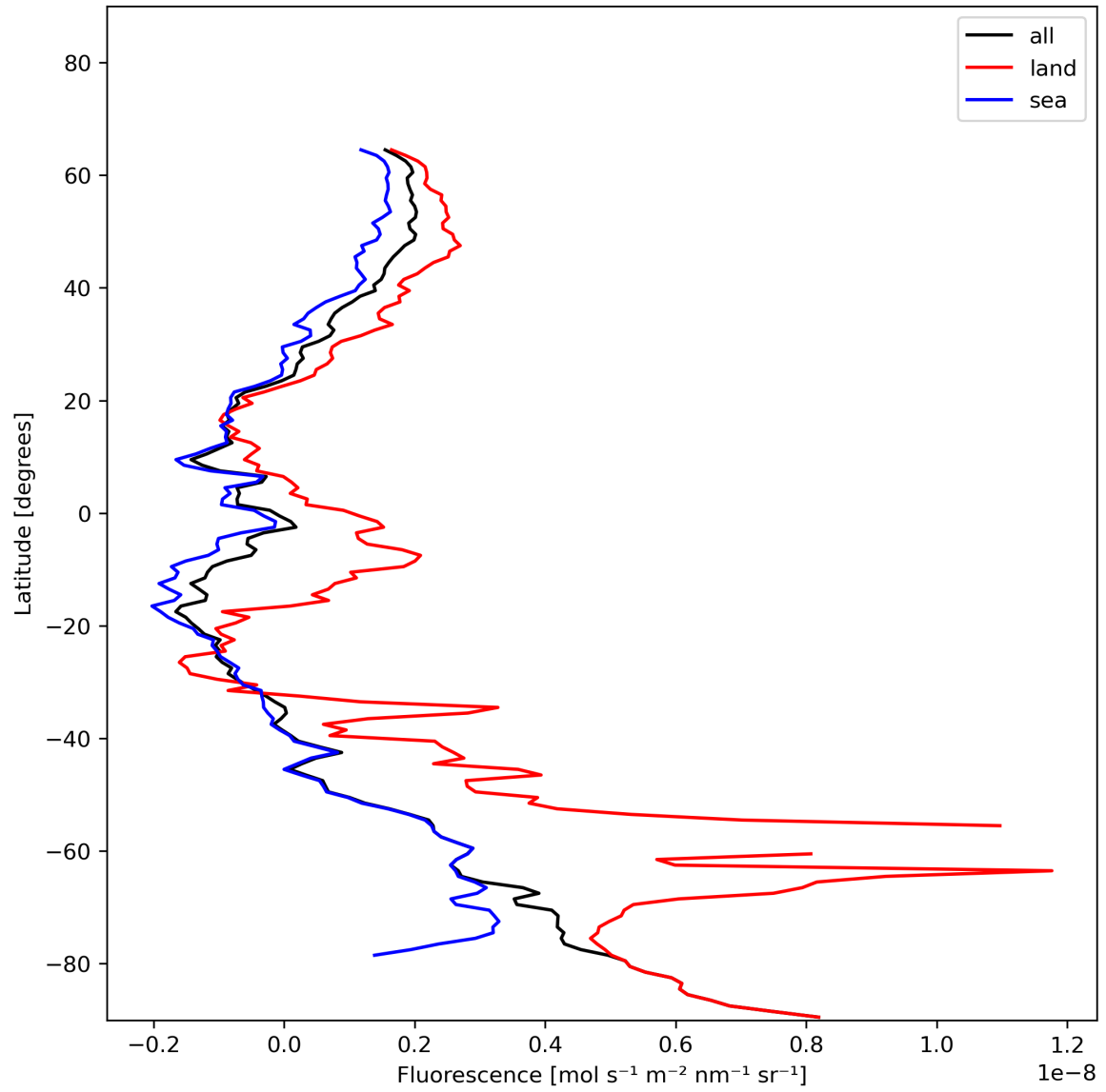
Figure 23: Zonal average of “Fluorescence” for 2023-12-27 to 2023-12-29.
