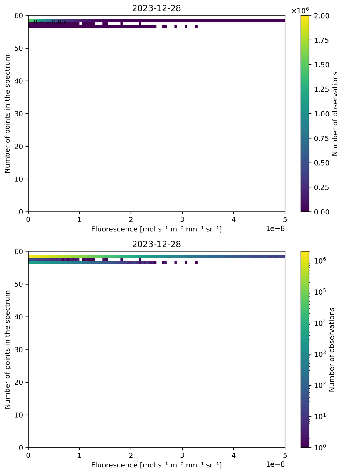
Figure 86: Scatter density plot of “Fluorescence” against “Number of points in the spectrum” for 2023-12-27 to 2023-12-29.
