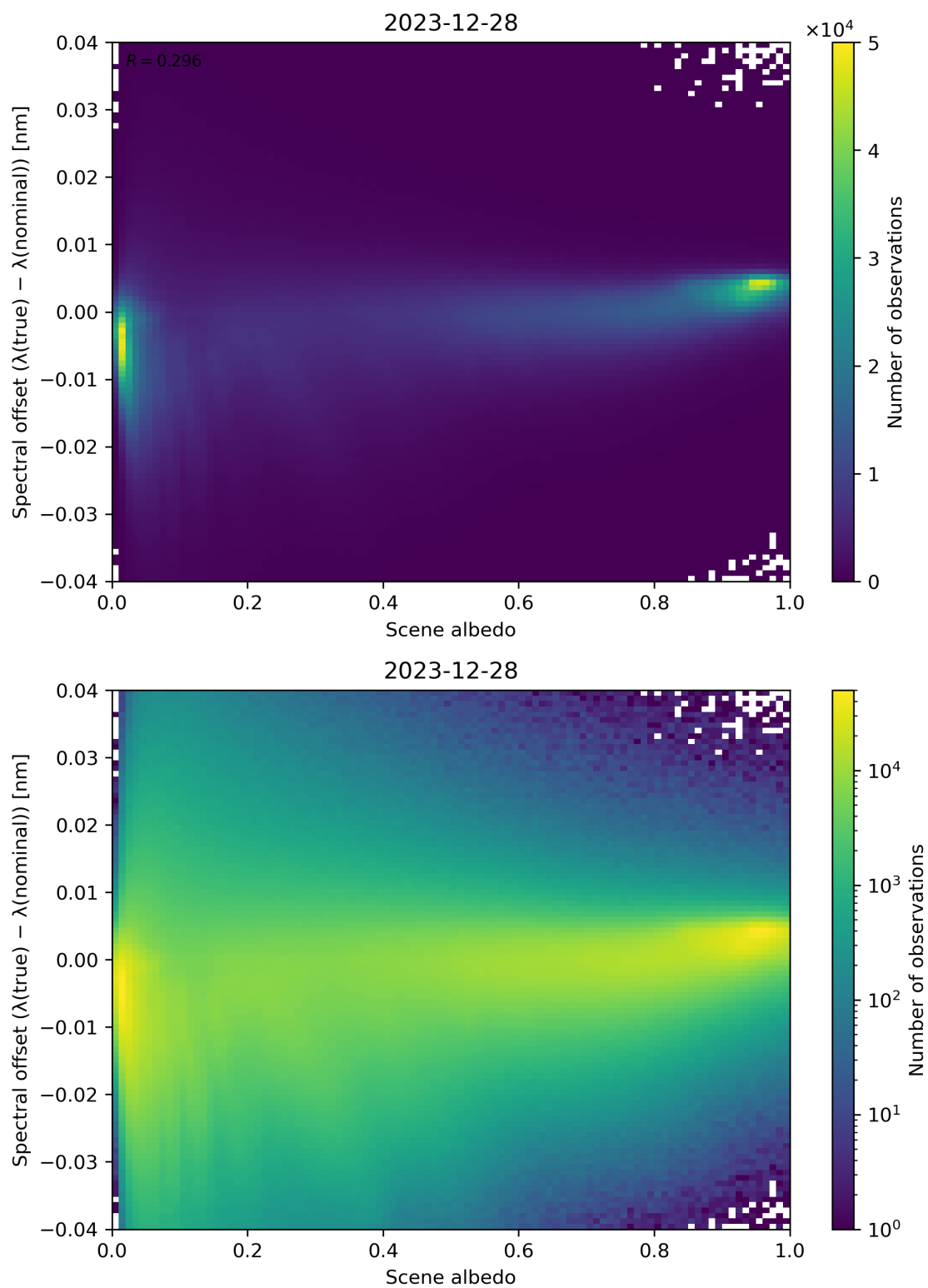
Figure 107: Scatter density plot of “Scene albedo” against “Spectral offset ( \lambda(\text{true}) - \lambda(\text{nominal}) )” for 2023-12-27 to 2023-12-29.
