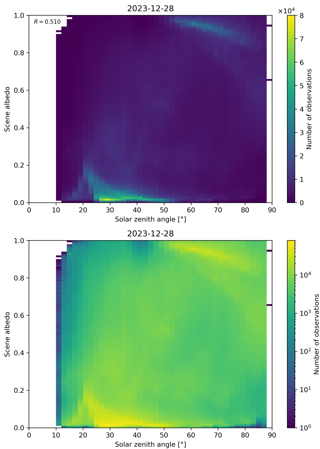
Figure 116: Scatter density plot of “Solar zenith angle” against “Scene albedo” for 2023-12-27 to 2023-12-29.
