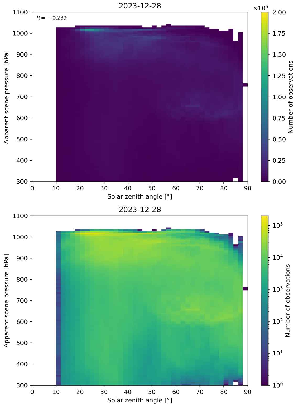
Figure 108: Scatter density plot of “Solar zenith angle” against “Apparent scene pressure” for 2023-12-27 to 2023-12-29.
