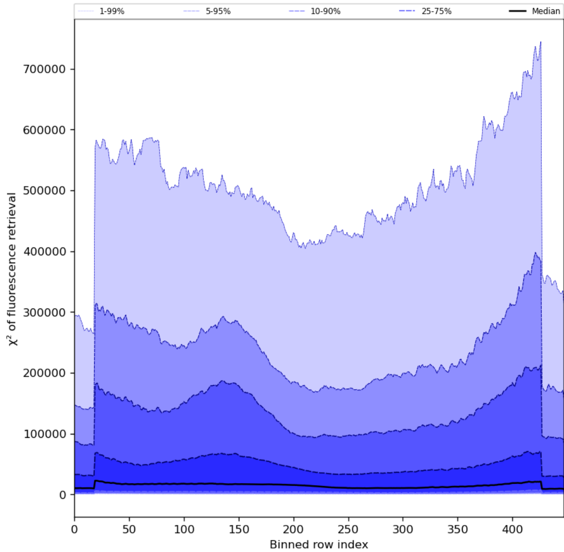
Figure 59: Along track statistics of “ \chi^2 of fluorescence retrieval” for 2023-12-27 to 2023-12-29
