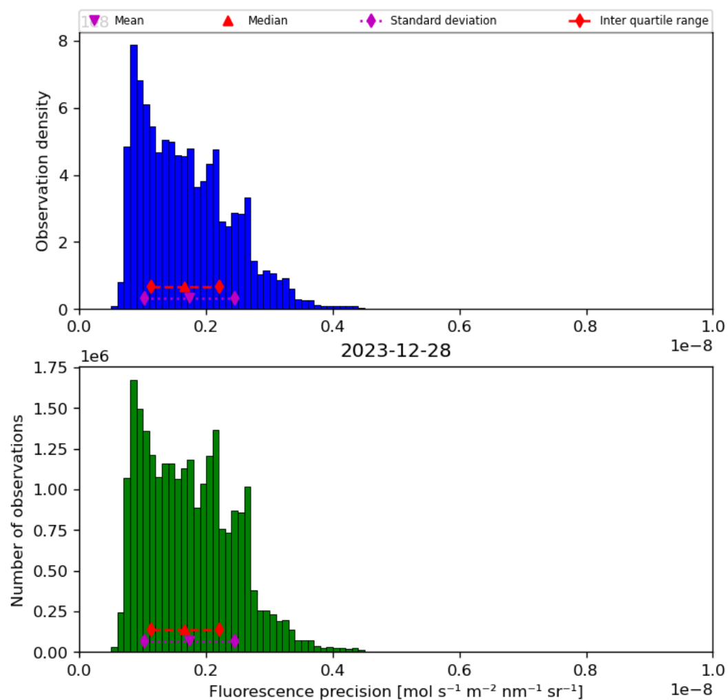
Figure 41: Histogram of “Fluorescence precision” for 2023-12-27 to 2023-12-29
