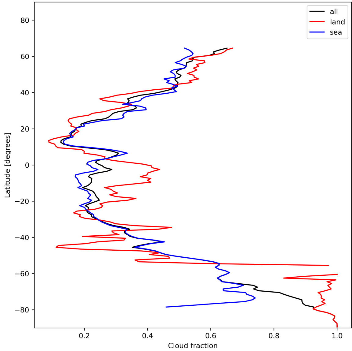
Figure 15: Zonal average of “Cloud fraction” for 2023-12-27 to 2023-12-29.
