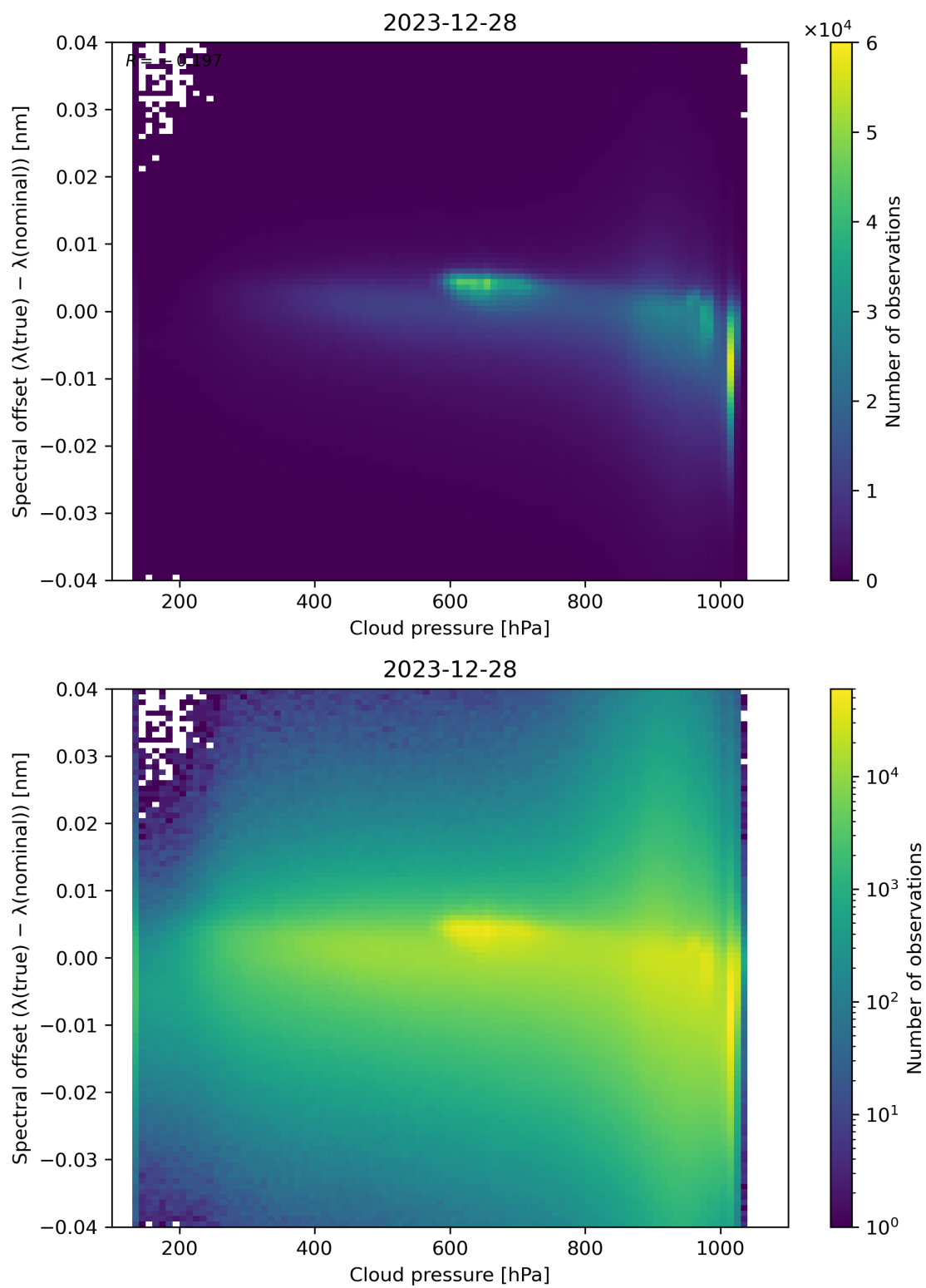
Figure 84: Scatter density plot of “Cloud pressure” against “Spectral offset ( \lambda(\text{true}) - \lambda(\text{nominal}) )” for 2023-12-27 to 2023-12-29.
