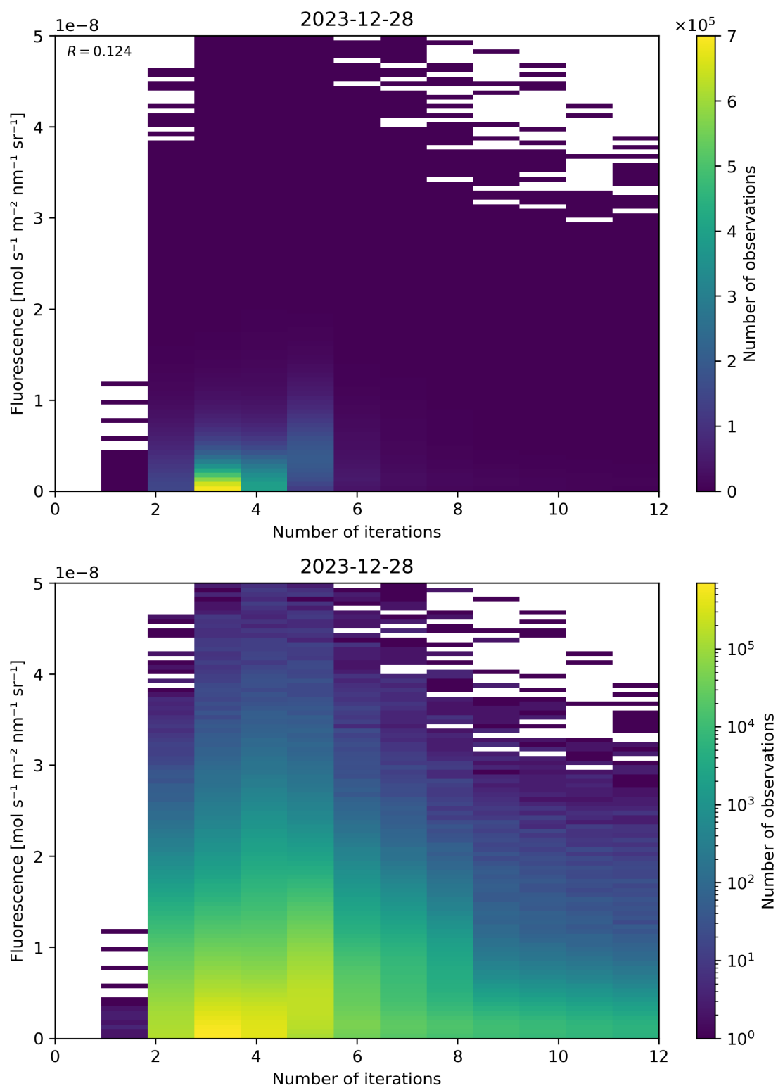
Figure 98: Scatter density plot of “Number of iterations” against “Fluorescence” for 2023-12-27 to 2023-12-29.
