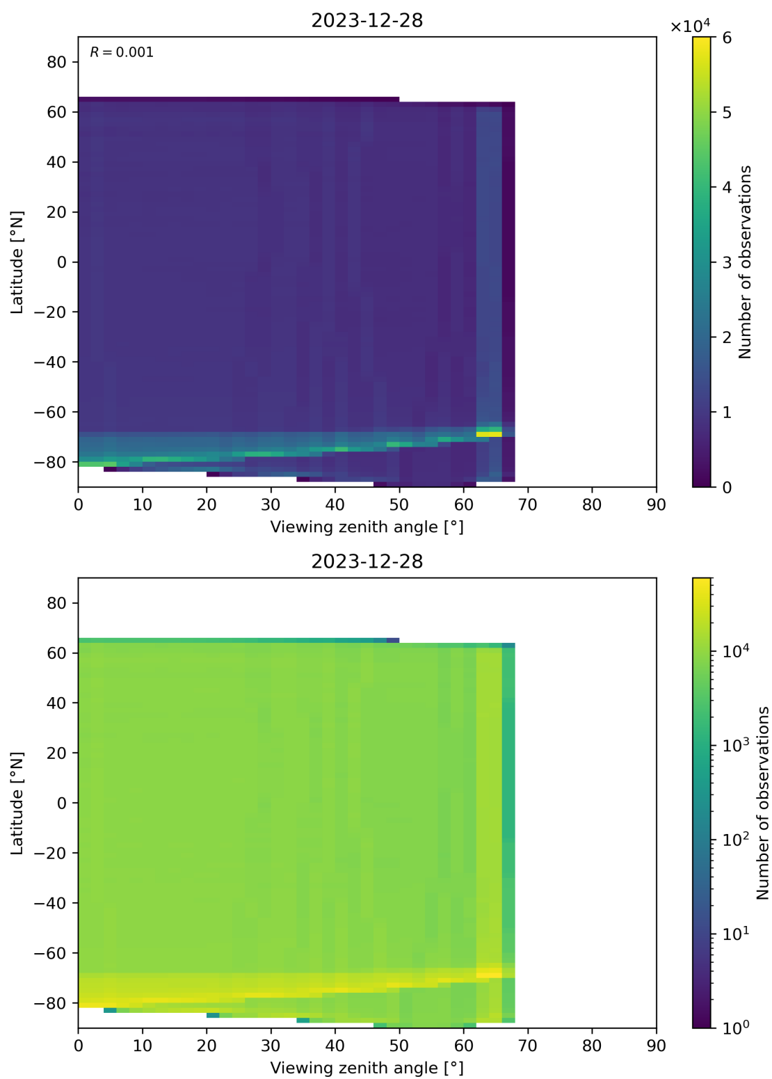
Figure 123: Scatter density plot of “Viewing zenith angle” against “Latitude” for 2023-12-27 to 2023-12-29.
