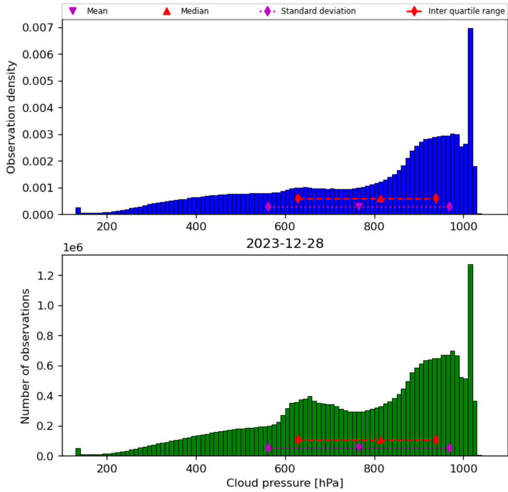
Figure 30: Histogram of “Cloud pressure” for 2023-12-27 to 2023-12-29
