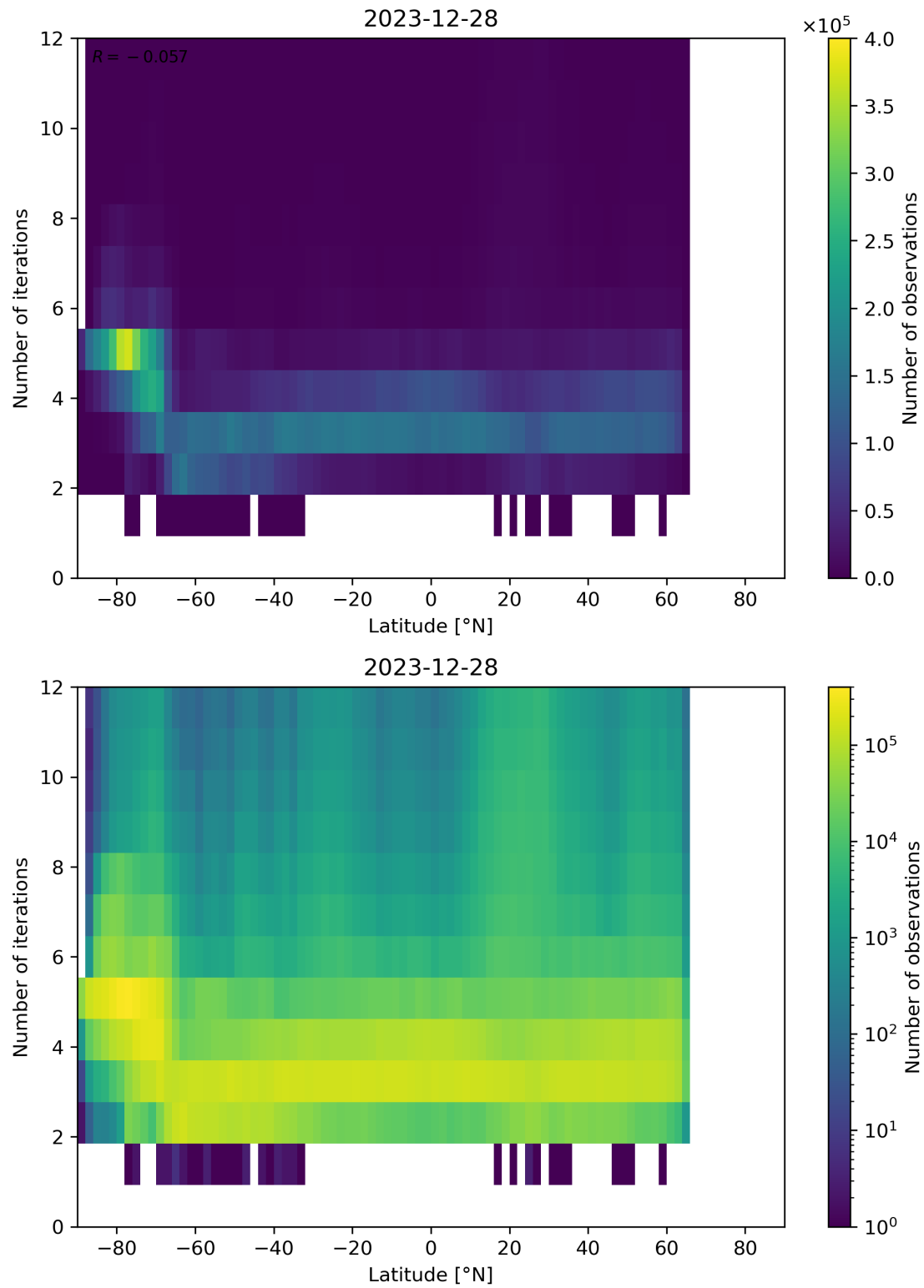
Figure 93: Scatter density plot of “Latitude” against “Number of iterations” for 2023-12-27 to 2023-12-29.
