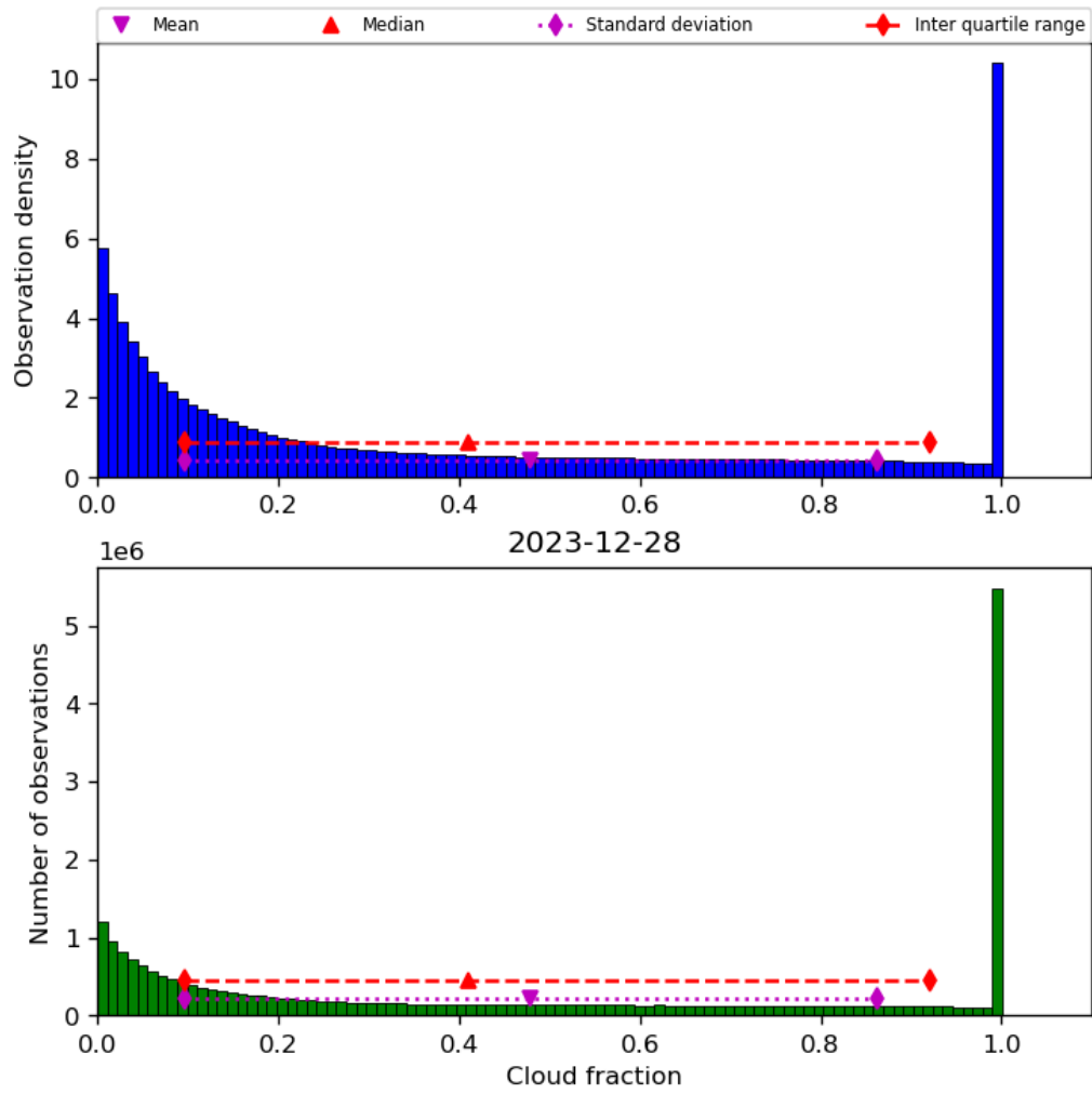
Figure 32: Histogram of “Cloud fraction” for 2023-12-27 to 2023-12-29
