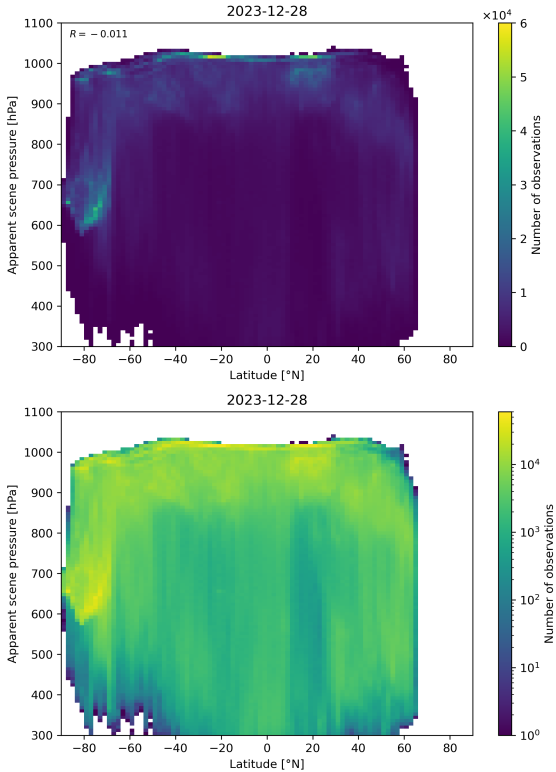
Figure 88: Scatter density plot of “Latitude” against “Apparent scene pressure” for 2023-12-27 to 2023-12-29.
