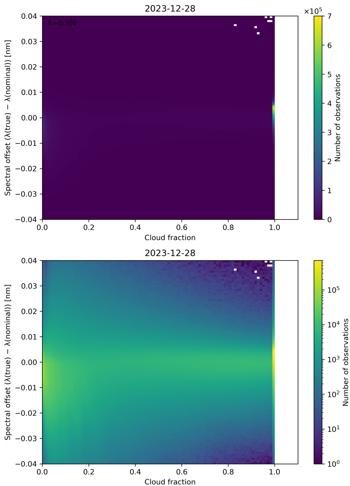
Figure 76: Scatter density plot of “Cloud fraction” against “Spectral offset ( \lambda(\text{true}) - \lambda(\text{nominal}) )” for 2023-12-27 to 2023-12-29.
