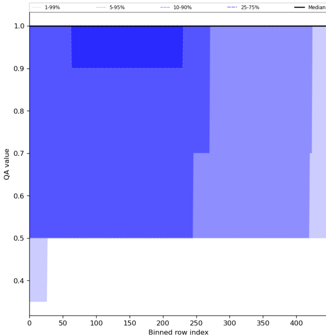
Figure 46: Along track statistics of “QA value” for 2023-12-27 to 2023-12-29
