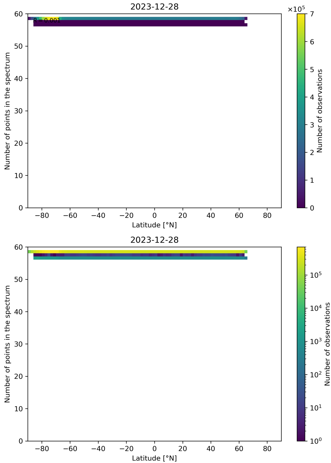
Figure 94: Scatter density plot of “Latitude” against “Number of points in the spectrum” for 2023-12-27 to 2023-12-29.
