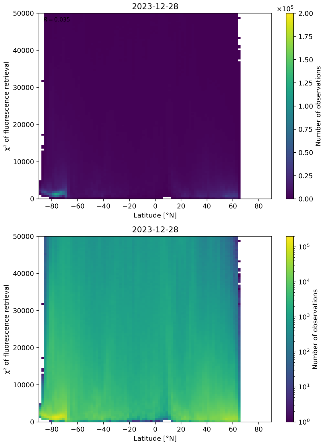
Figure 89: Scatter density plot of “Latitude” against “ \chi^2 of fluorescence retrieval” for 2023-12-27 to 2023-12-29.
