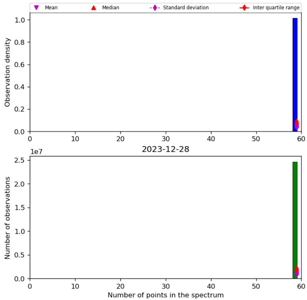
Figure 44: Histogram of “Number of points in the spectrum” for 2023-12-27 to 2023-12-29
