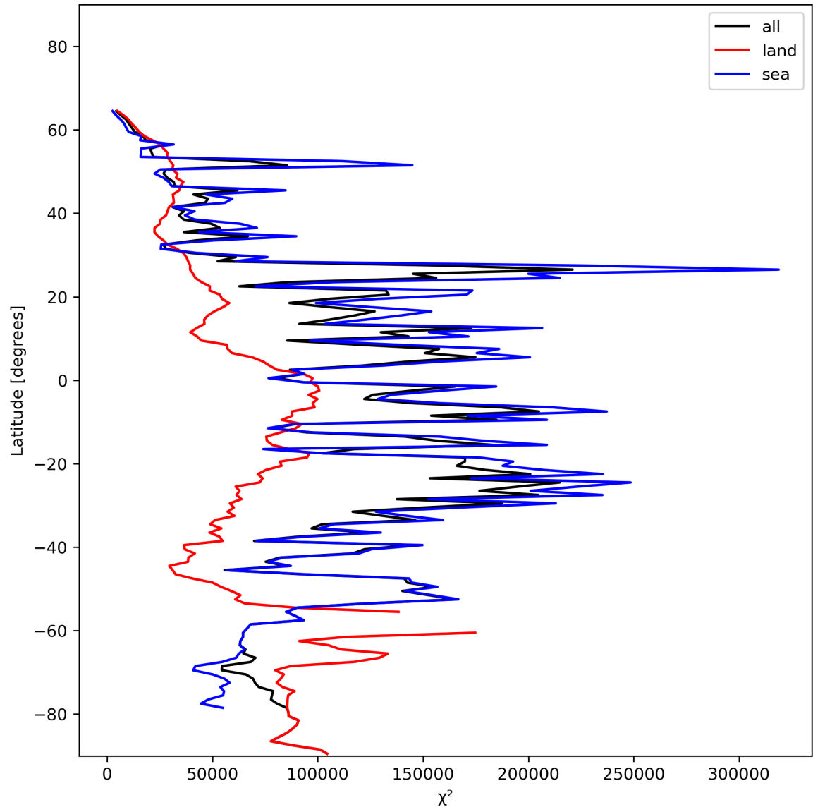
Figure 21: Zonal average of “ \chi^2 ” for 2023-12-27 to 2023-12-29.
