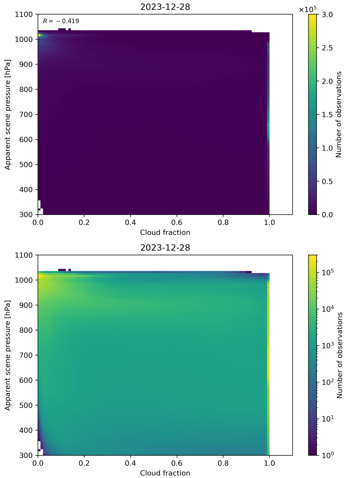
Figure 70: Scatter density plot of “Cloud fraction” against “Apparent scene pressure” for 2023-12-27 to 2023-12-29.
