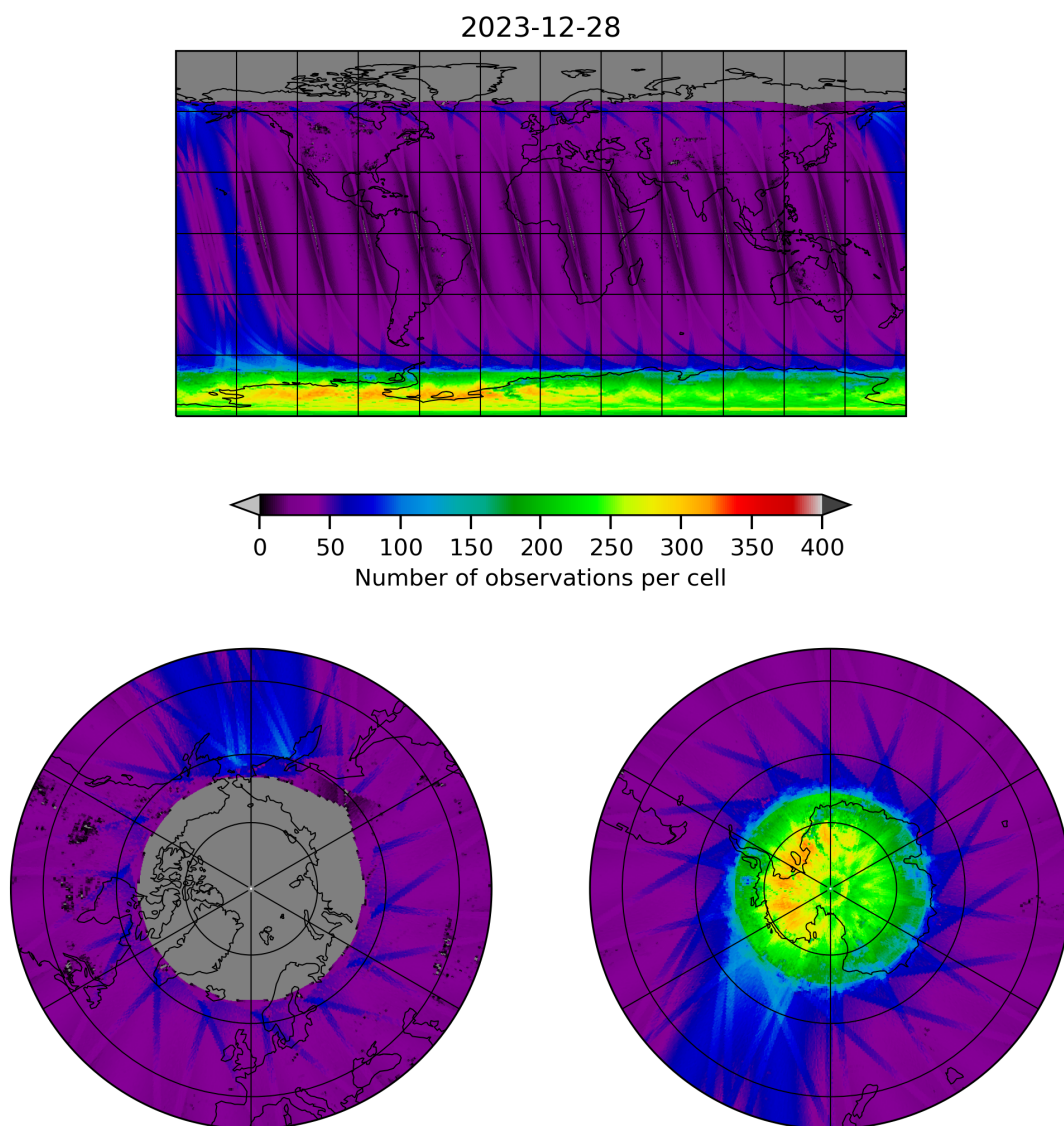
Figure 11: Map of the number of observations for 2023-12-27 to 2023-12-29
