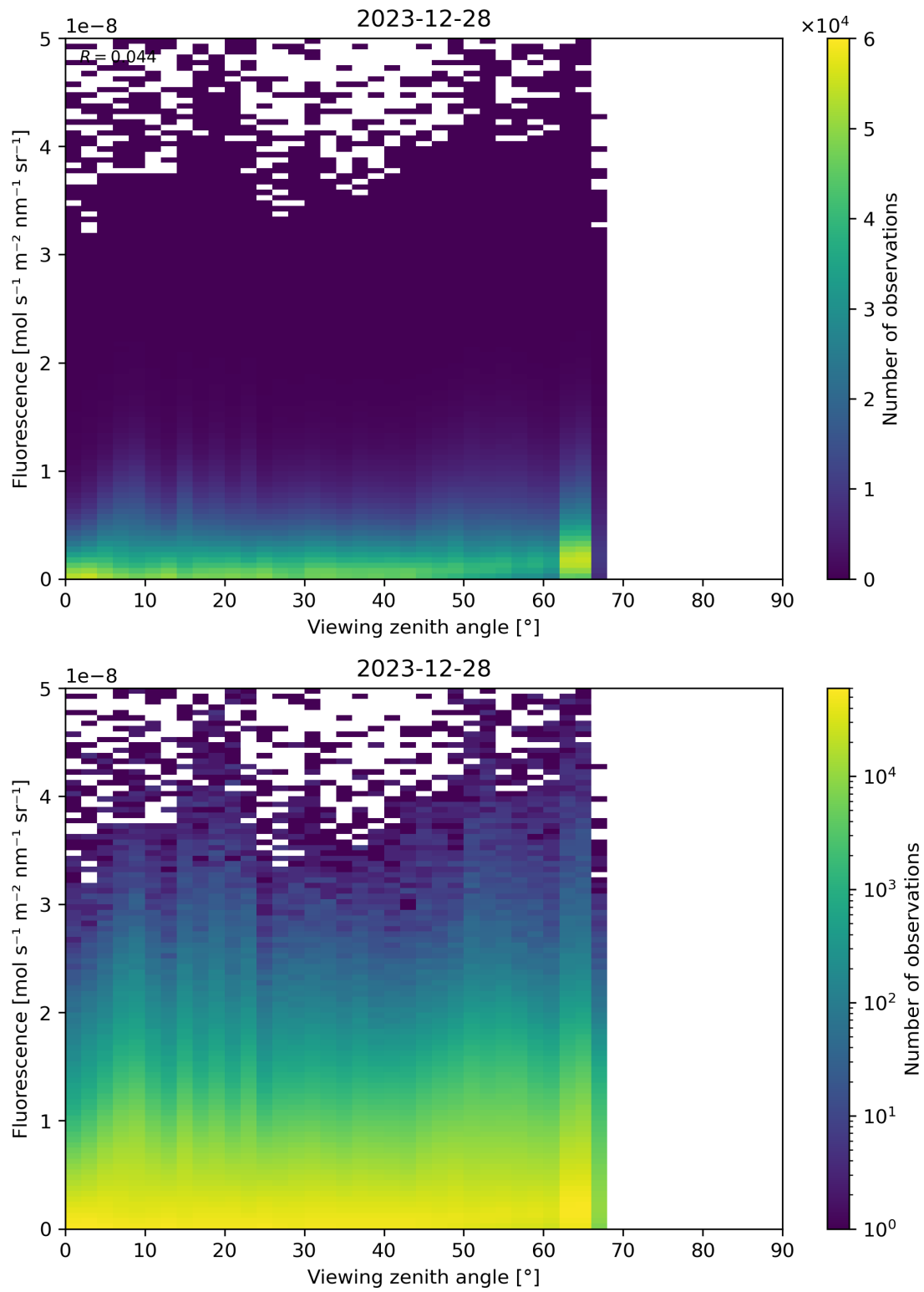
Figure 122: Scatter density plot of “Viewing zenith angle” against “Fluorescence” for 2023-12-27 to 2023-12-29.
