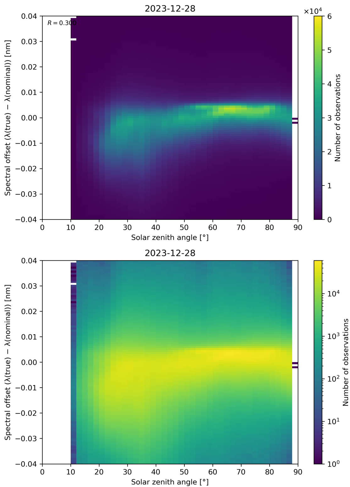
Figure 117: Scatter density plot of “Solar zenith angle” against “Spectral offset ( \lambda(\text{true}) - \lambda(\text{nominal}) )” for 2023-12-27 to 2023-12-29.
