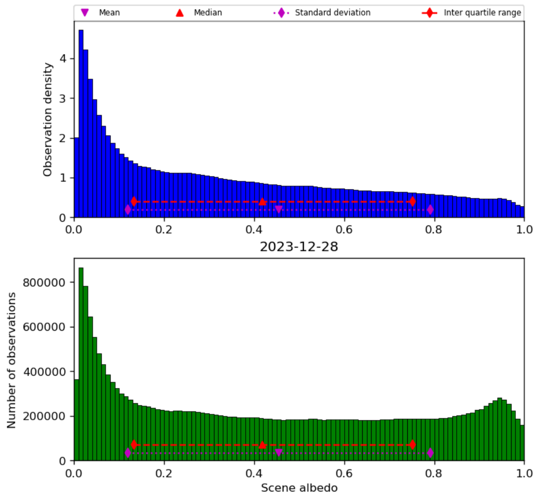
Figure 34: Histogram of “Scene albedo” for 2023-12-27 to 2023-12-29
