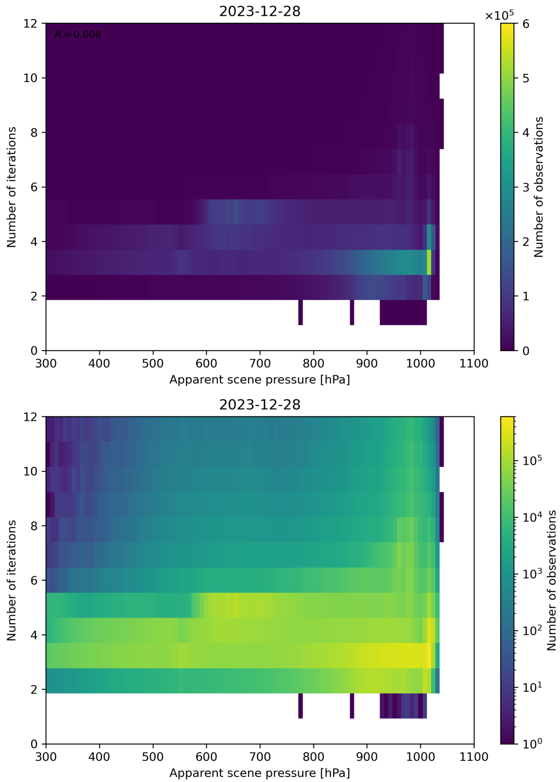
Figure 65: Scatter density plot of “Apparent scene pressure” against “Number of iterations” for 2023-12-27 to 2023-12-29.
