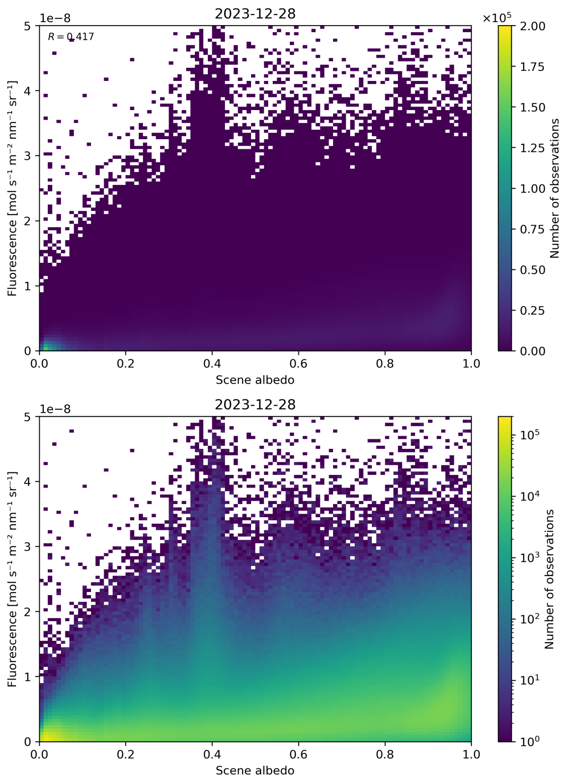
Figure 104: Scatter density plot of “Scene albedo” against “Fluorescence” for 2023-12-27 to 2023-12-29.
