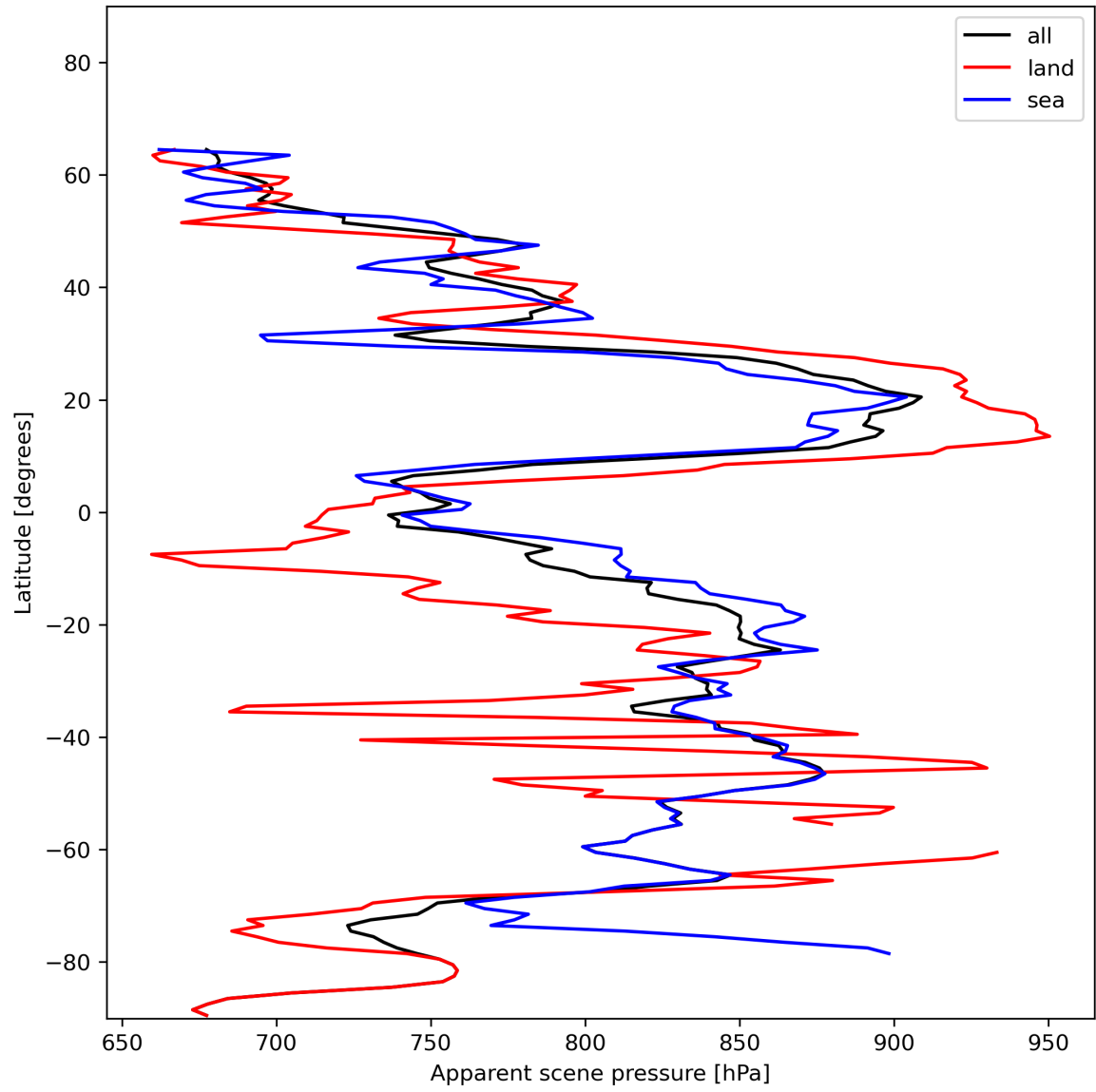
Figure 19: Zonal average of “Apparent scene pressure” for 2023-12-27 to 2023-12-29.
