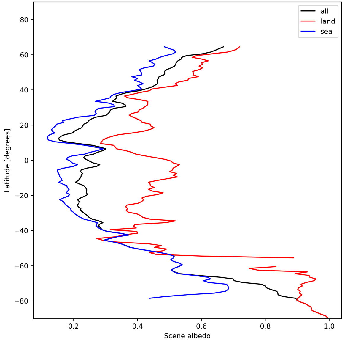
Figure 17: Zonal average of “Scene albedo” for 2023-12-27 to 2023-12-29.
