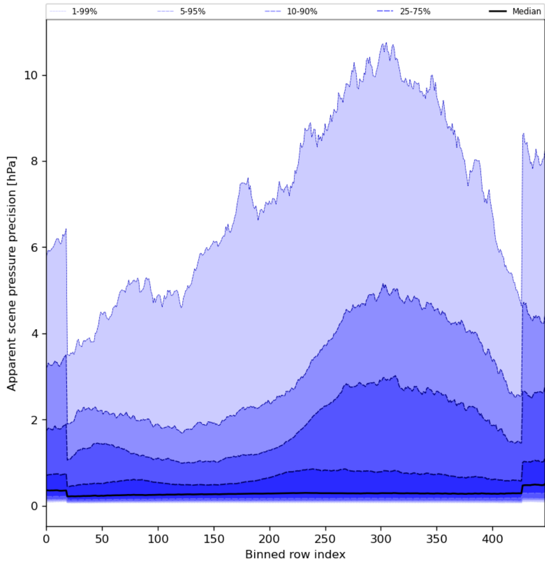
Figure 54: Along track statistics of “Apparent scene pressure precision” for 2023-12-27 to 2023-12-29
