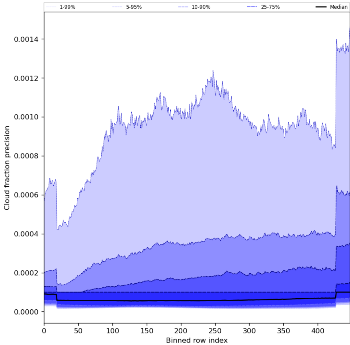
Figure 50: Along track statistics of “Cloud fraction precision” for 2023-12-27 to 2023-12-29
