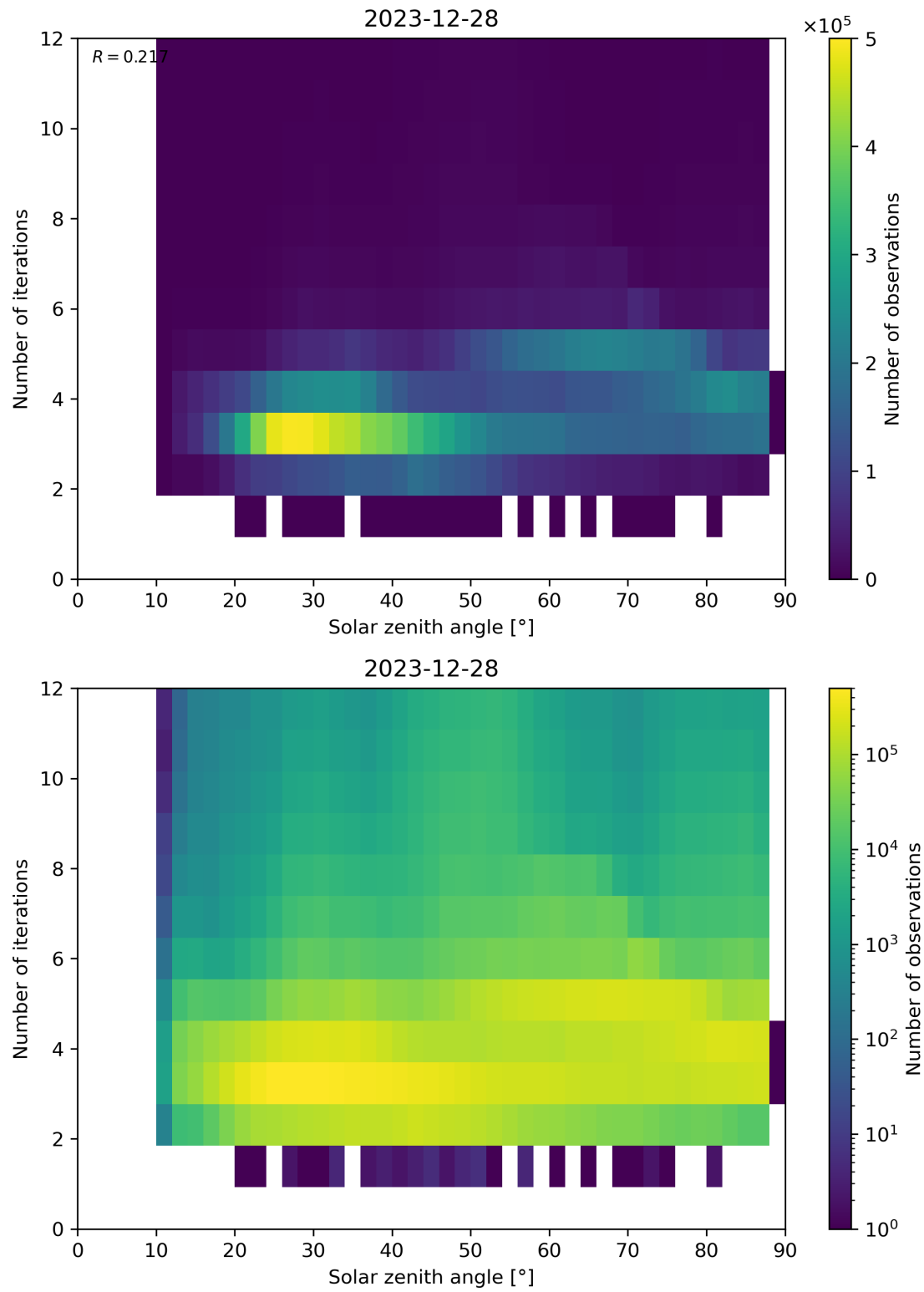
Figure 114: Scatter density plot of “Solar zenith angle” against “Number of iterations” for 2023-12-27 to 2023-12-29.
