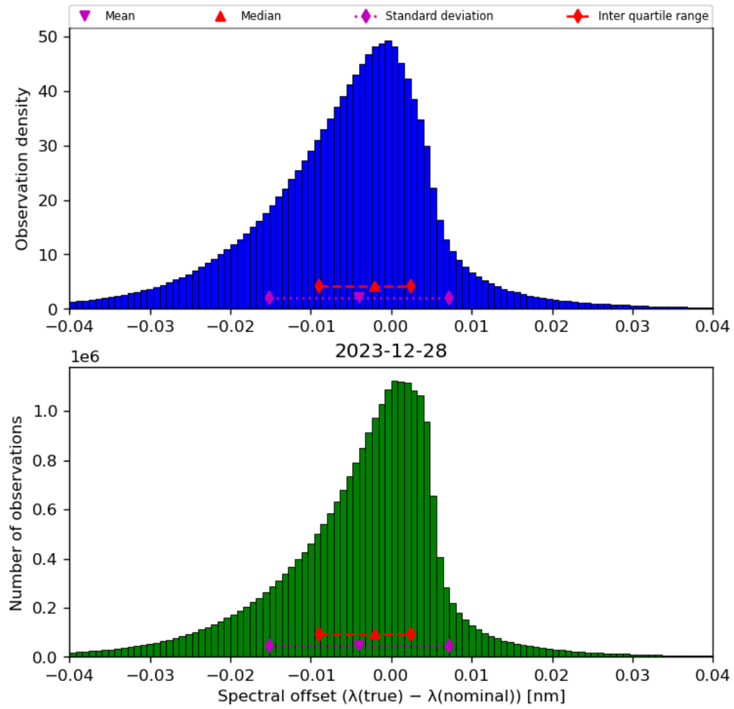
Figure 45: Histogram of “Spectral offset ( \lambda(\text{true}) - \lambda(\text{nominal}) )” for 2023-12-27 to 2023-12-29
