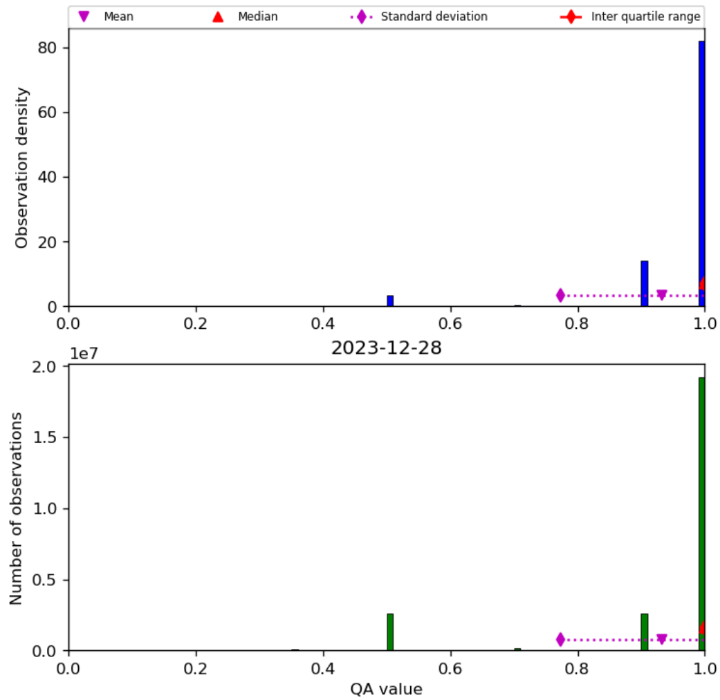
Figure 29: Histogram of “QA value” for 2023-12-27 to 2023-12-29
