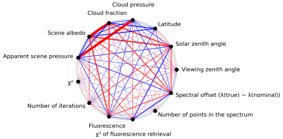
Figure 1: Map of correlation graph for 2023-12-27 to 2023-12-29.
