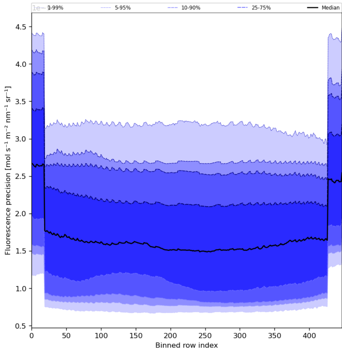
Figure 58: Along track statistics of “Fluorescence precision” for 2023-12-27 to 2023-12-29
