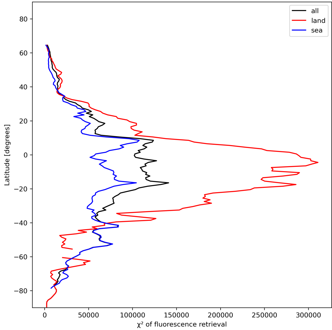
Figure 25: Zonal average of “ \chi^2 of fluorescence retrieval” for 2023-12-27 to 2023-12-29.
