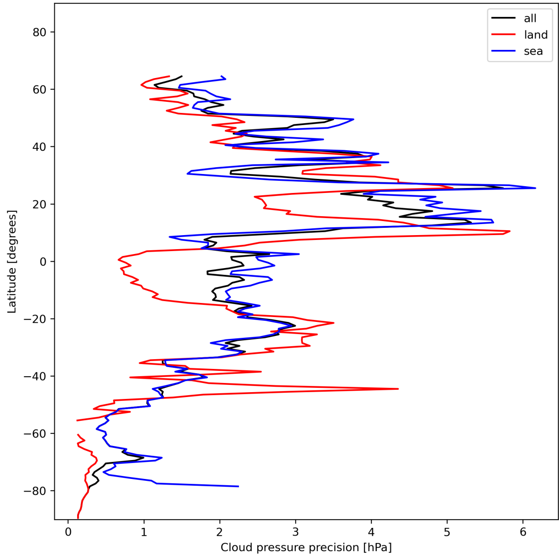
Figure 14: Zonal average of “Cloud pressure precision” for 2023-12-27 to 2023-12-29.
