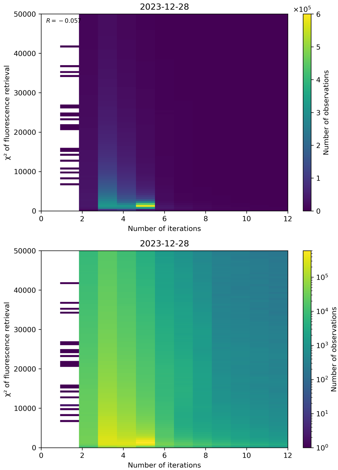
Figure 97: Scatter density plot of “Number of iterations” against “ \chi^2 of fluorescence retrieval” for 2023-12-27 to 2023-12-29.
