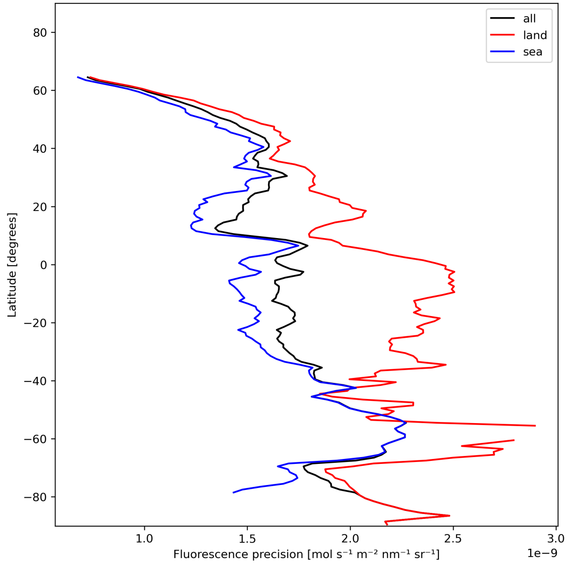
Figure 24: Zonal average of “Fluorescence precision” for 2023-12-27 to 2023-12-29.
