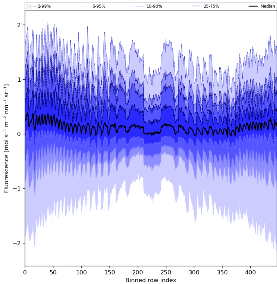
Figure 57: Along track statistics of "Fluorescence" for 2023-12-27 to 2023-12-29
