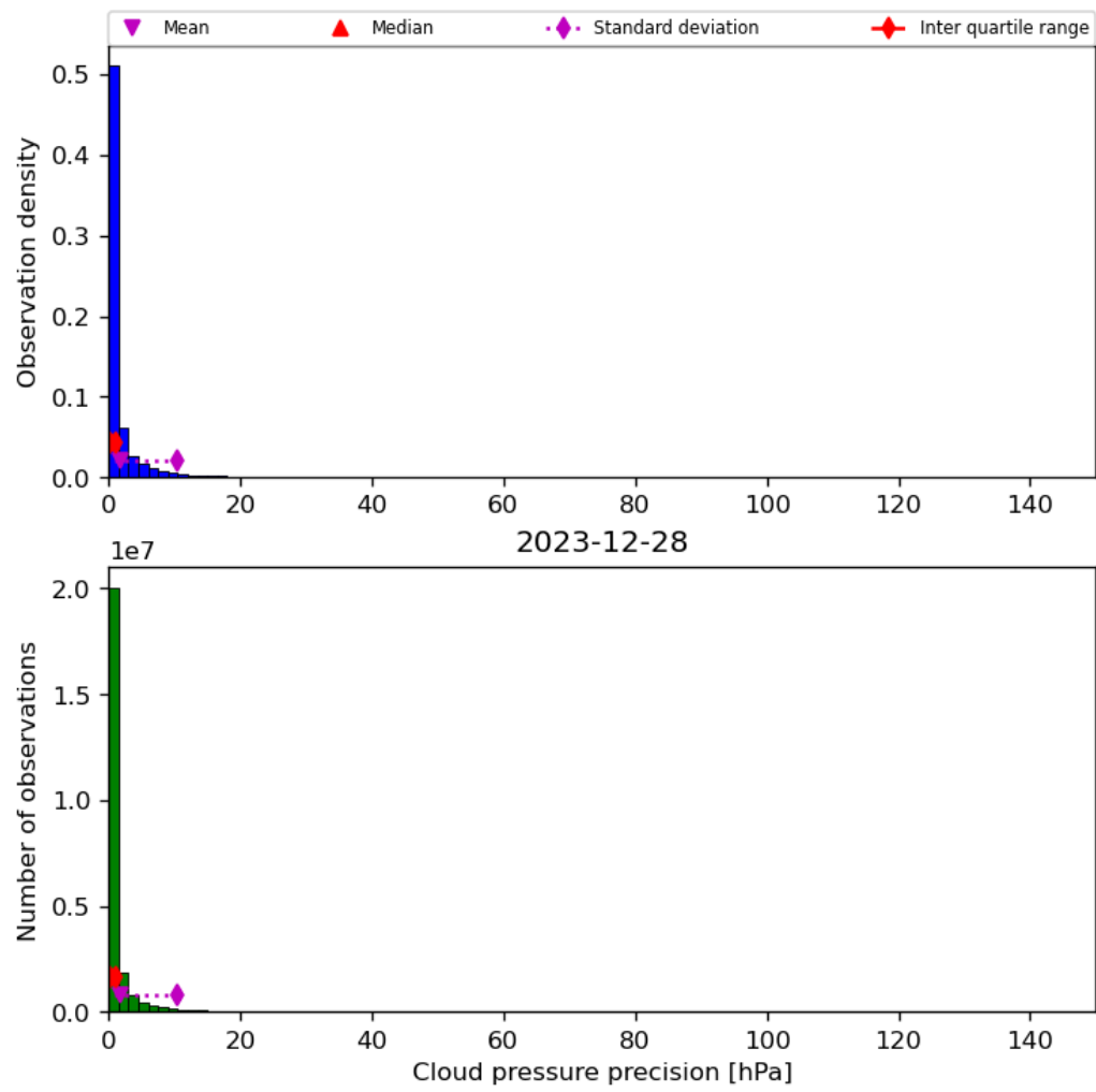
Figure 31: Histogram of “Cloud pressure precision” for 2023-12-27 to 2023-12-29
