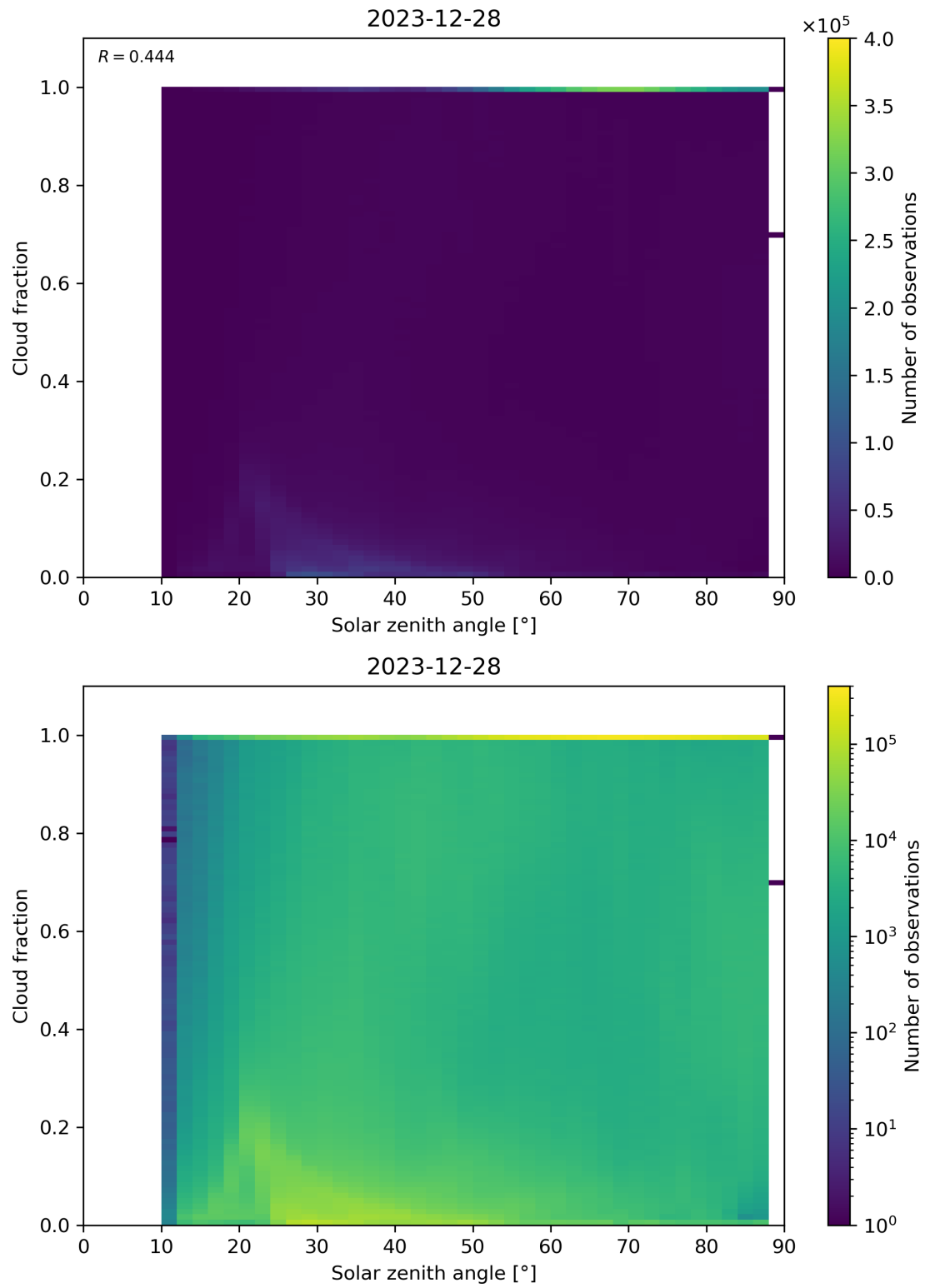
Figure 110: Scatter density plot of “Solar zenith angle” against “Cloud fraction” for 2023-12-27 to 2023-12-29.
