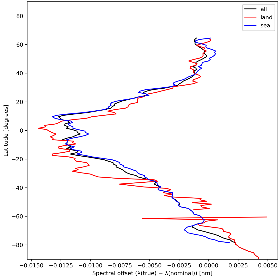
Figure 28: Zonal average of “Spectral offset ( \lambda(\text{true}) - \lambda(\text{nominal}) )” for 2023-12-27 to 2023-12-29.
