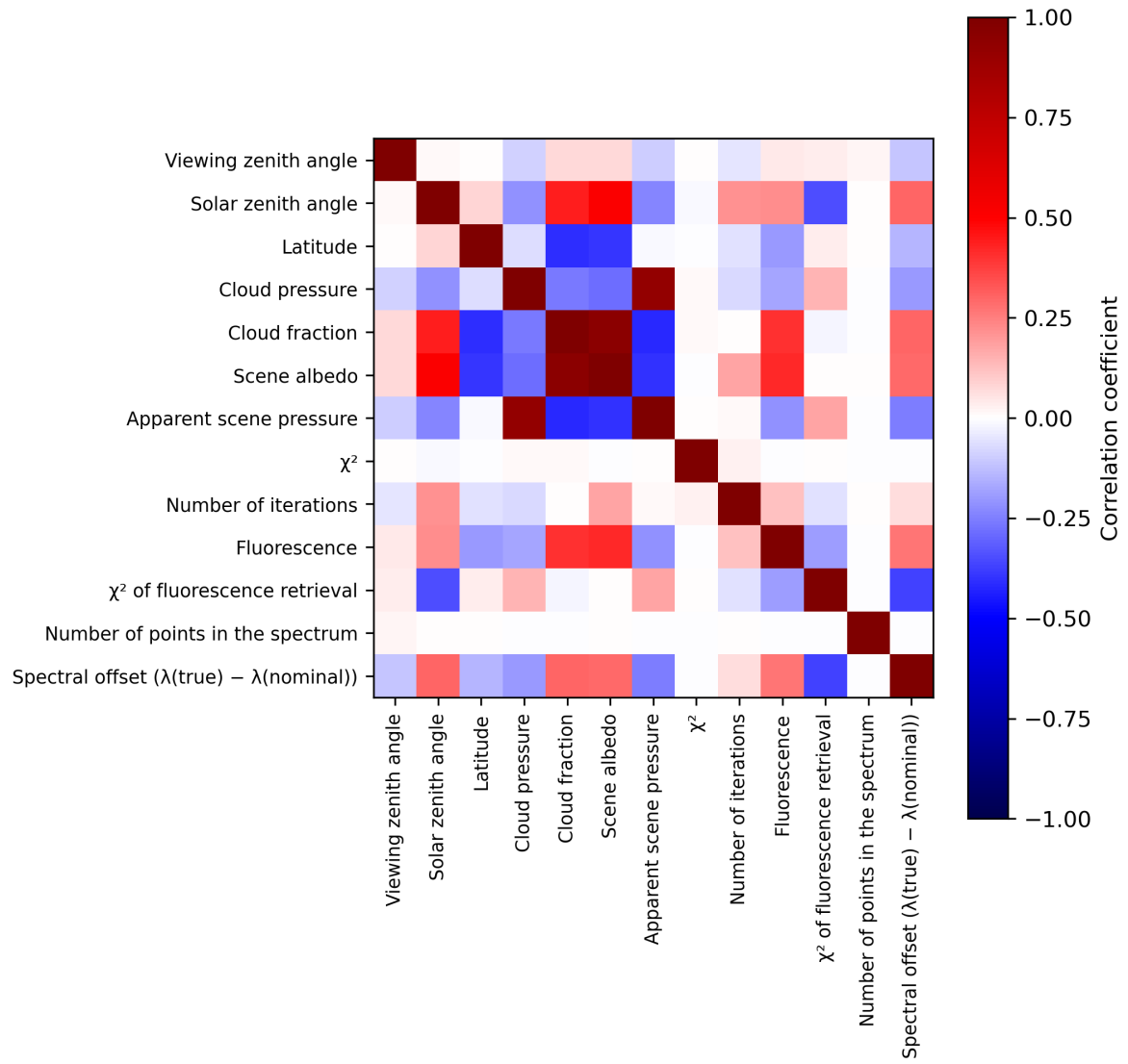
Figure 2: Map of correlation matrix for 2023-12-27 to 2023-12-29.
