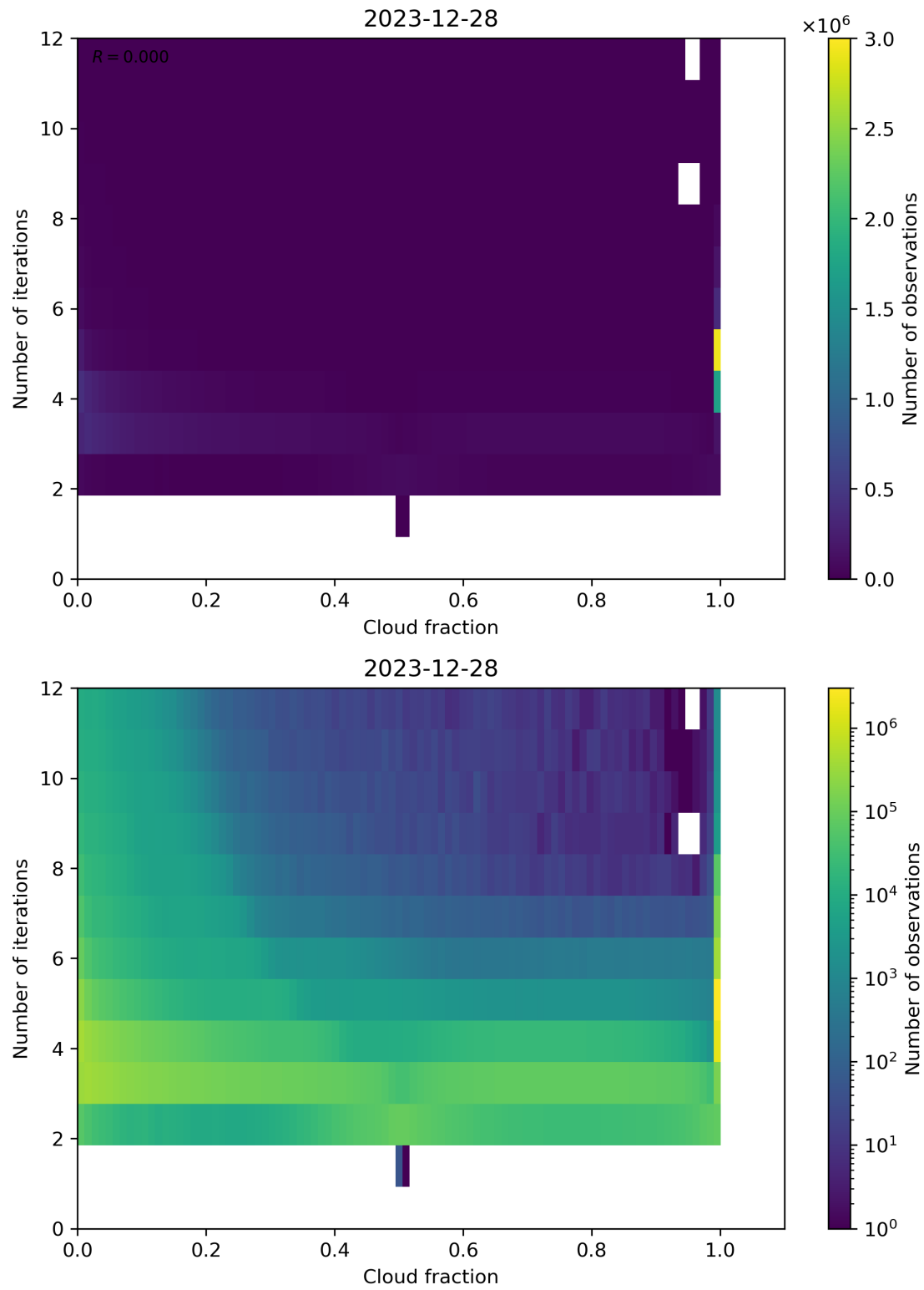
Figure 73: Scatter density plot of “Cloud fraction” against “Number of iterations” for 2023-12-27 to 2023-12-29.
