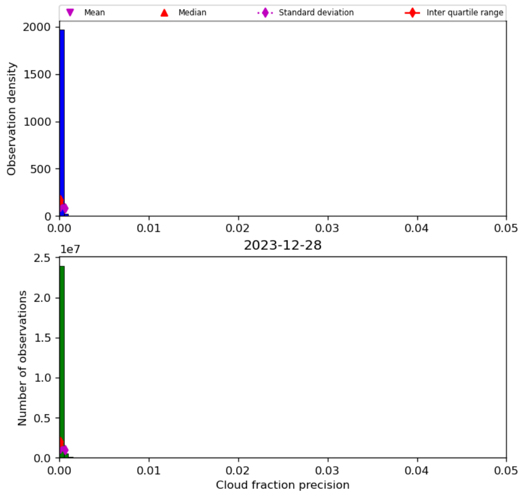
Figure 33: Histogram of “Cloud fraction precision” for 2023-12-27 to 2023-12-29
