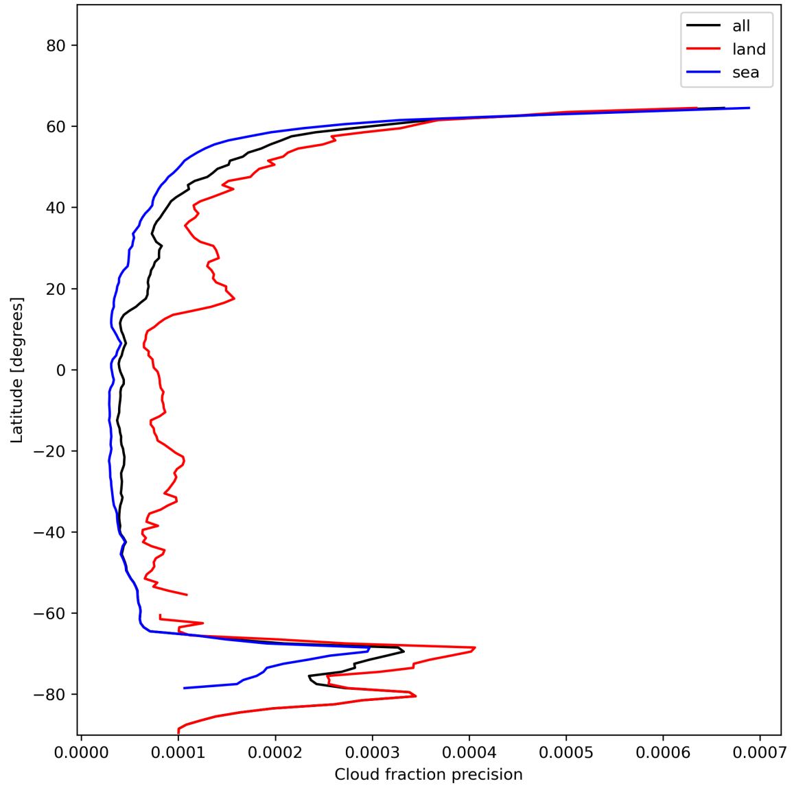
Figure 16: Zonal average of “Cloud fraction precision” for 2023-12-27 to 2023-12-29.
