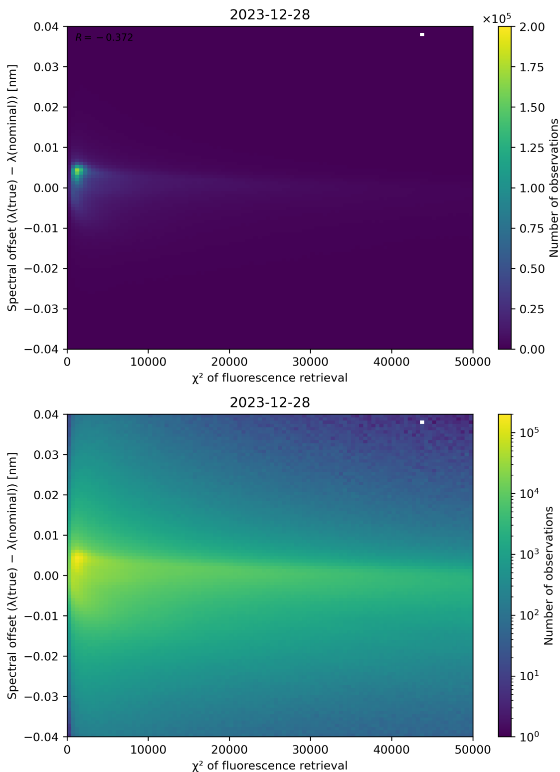
Figure 69: Scatter density plot of “ \chi^2 of fluorescence retrieval” against “Spectral offset ( \lambda(\text{true}) - \lambda(\text{nominal}) )” for 2023-12-27 to 2023-12-29.
