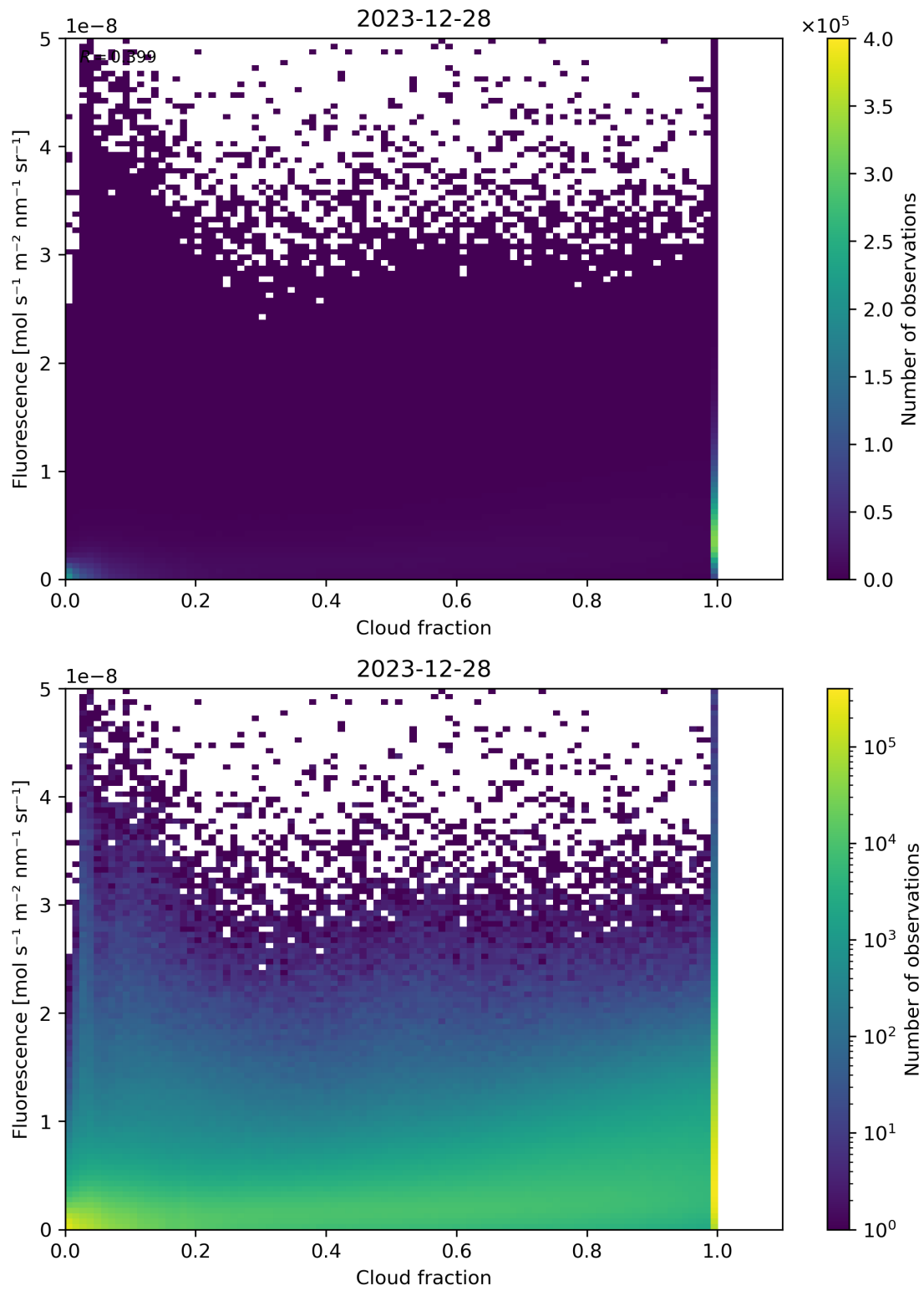
Figure 72: Scatter density plot of “Cloud fraction” against “Fluorescence” for 2023-12-27 to 2023-12-29.
