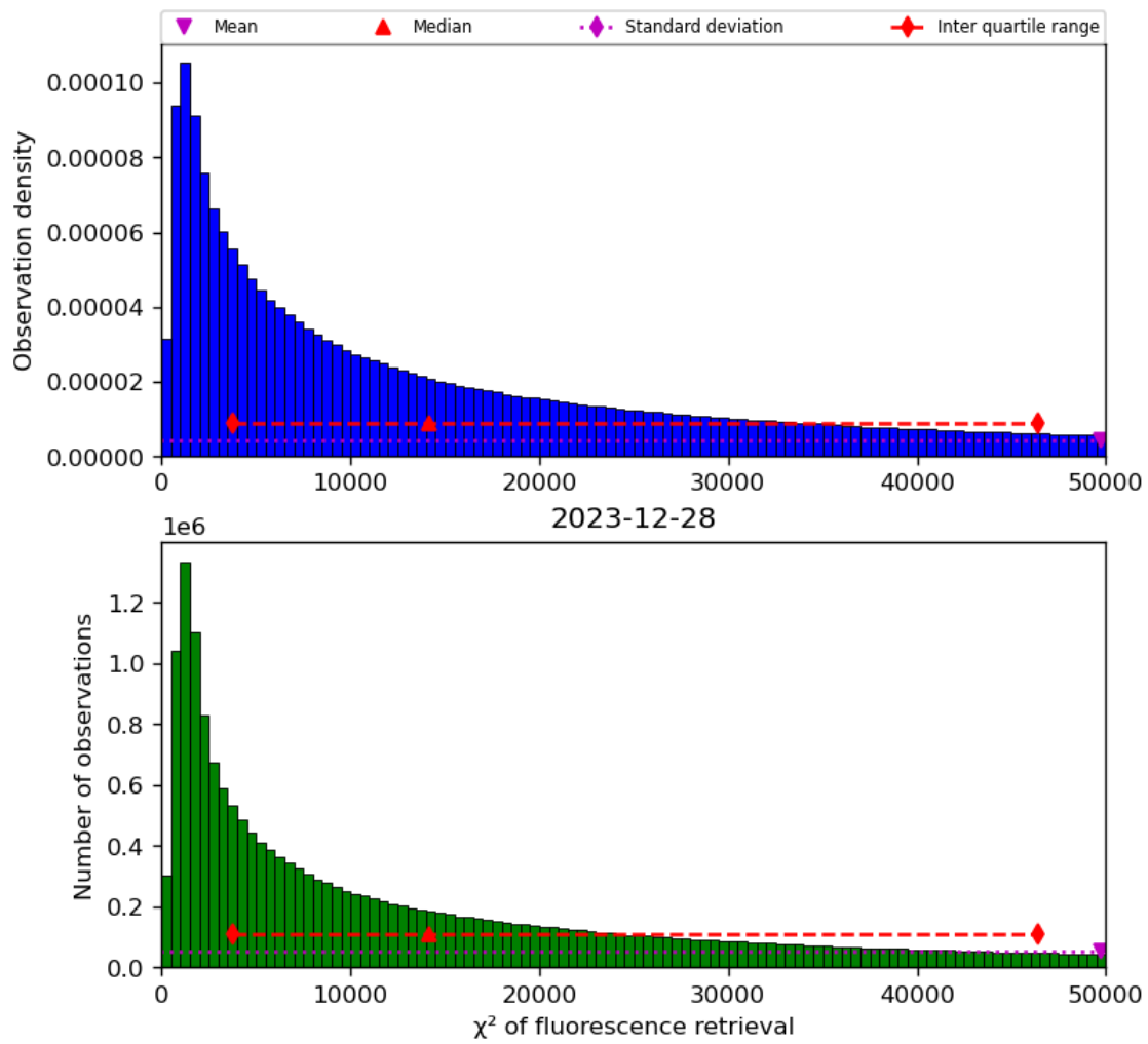
Figure 42: Histogram of “ \chi^2 of fluorescence retrieval” for 2023-12-27 to 2023-12-29
