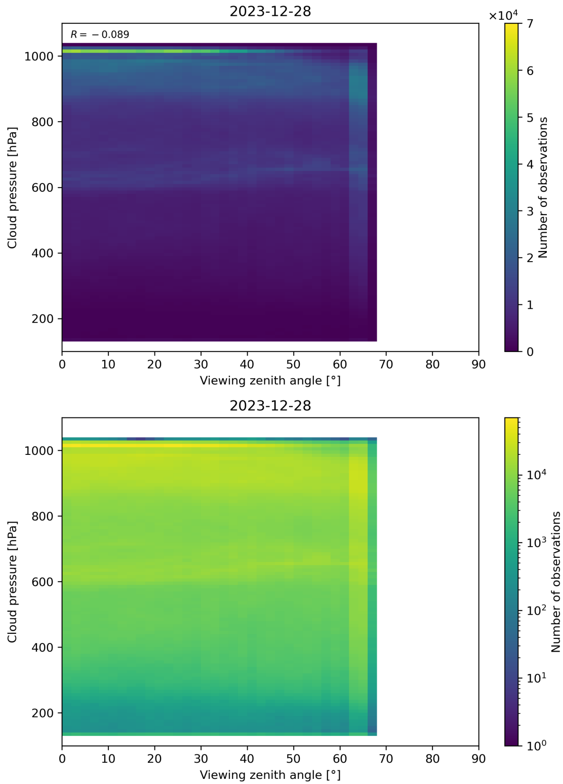
Figure 121: Scatter density plot of “Viewing zenith angle” against “Cloud pressure” for 2023-12-27 to 2023-12-29.
