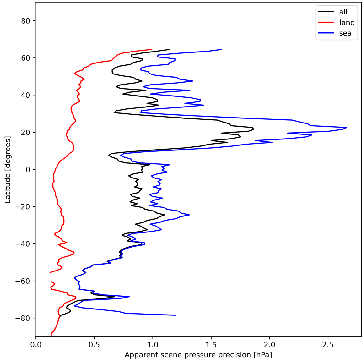
Figure 20: Zonal average of “Apparent scene pressure precision” for 2023-12-27 to 2023-12-29.
