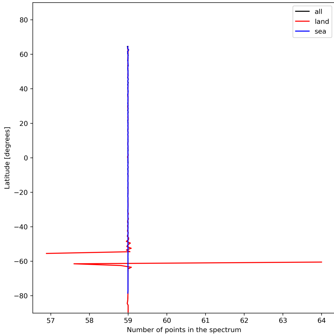
Figure 27: Zonal average of “Number of points in the spectrum” for 2023-12-27 to 2023-12-29.
