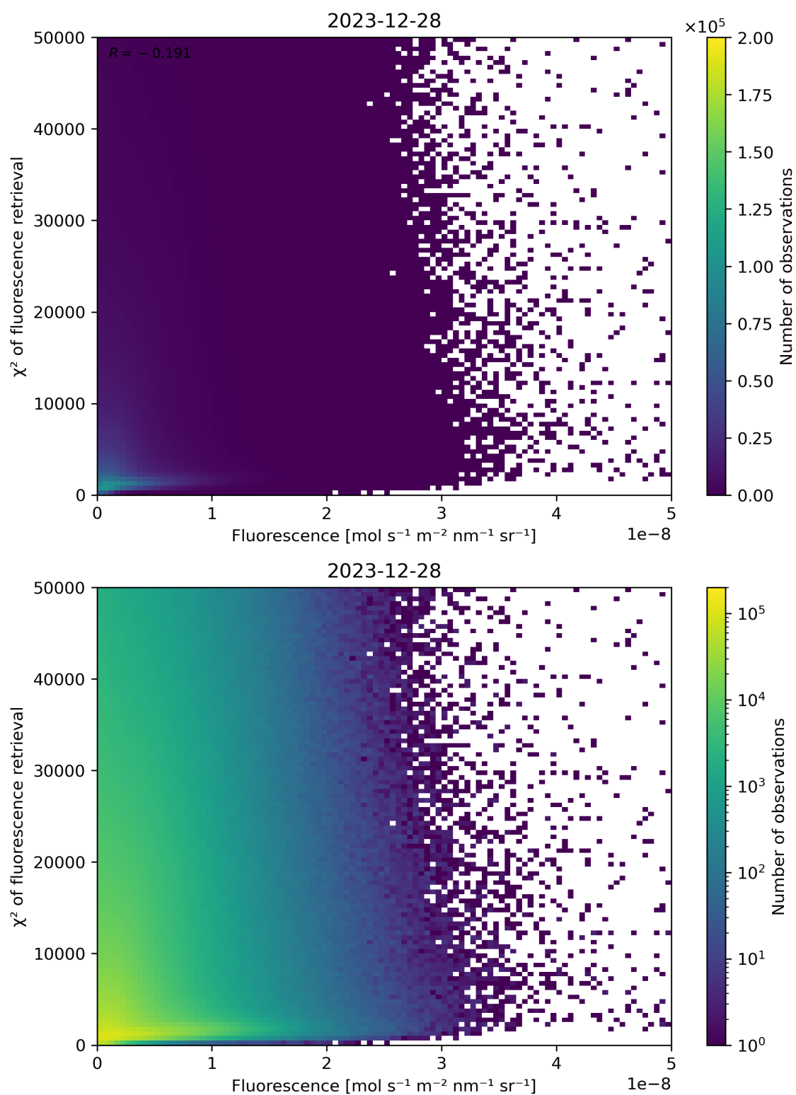
Figure 85: Scatter density plot of “Fluorescence” against “ \chi^2 of fluorescence retrieval” for 2023-12-27 to 2023-12-29.
