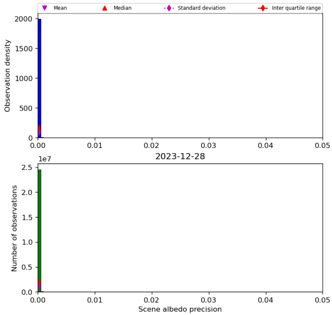
Figure 35: Histogram of “Scene albedo precision” for 2023-12-27 to 2023-12-29
