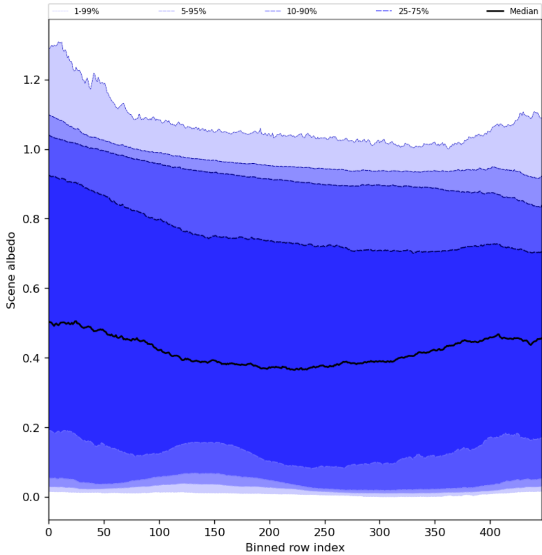
Figure 51: Along track statistics of “Scene albedo” for 2023-12-27 to 2023-12-29
