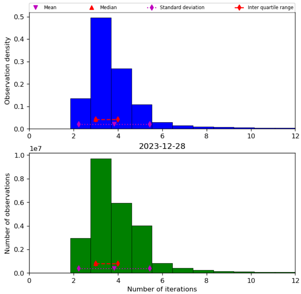
Figure 39: Histogram of “Number of iterations” for 2023-12-27 to 2023-12-29
