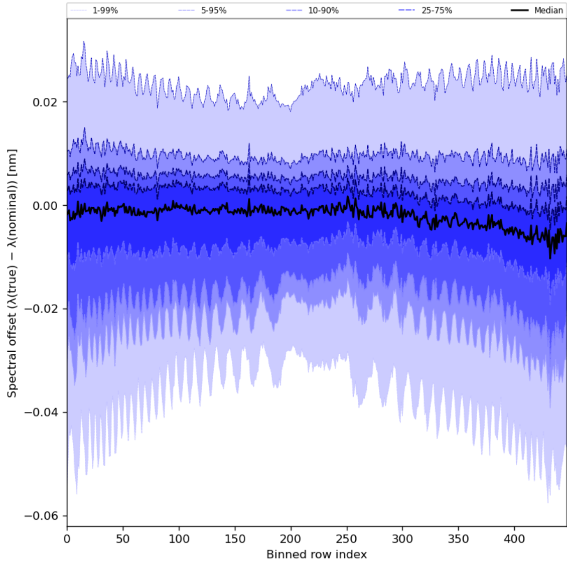
Figure 62: Along track statistics of “Spectral offset ( \lambda(\text{true}) - \lambda(\text{nominal}) )” for 2023-12-27 to 2023-12-29
