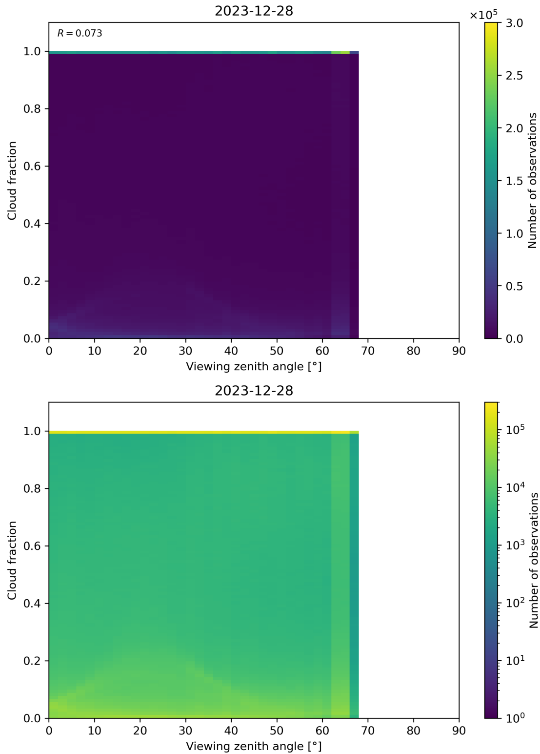
Figure 120: Scatter density plot of “Viewing zenith angle” against “Cloud fraction” for 2023-12-27 to 2023-12-29.
