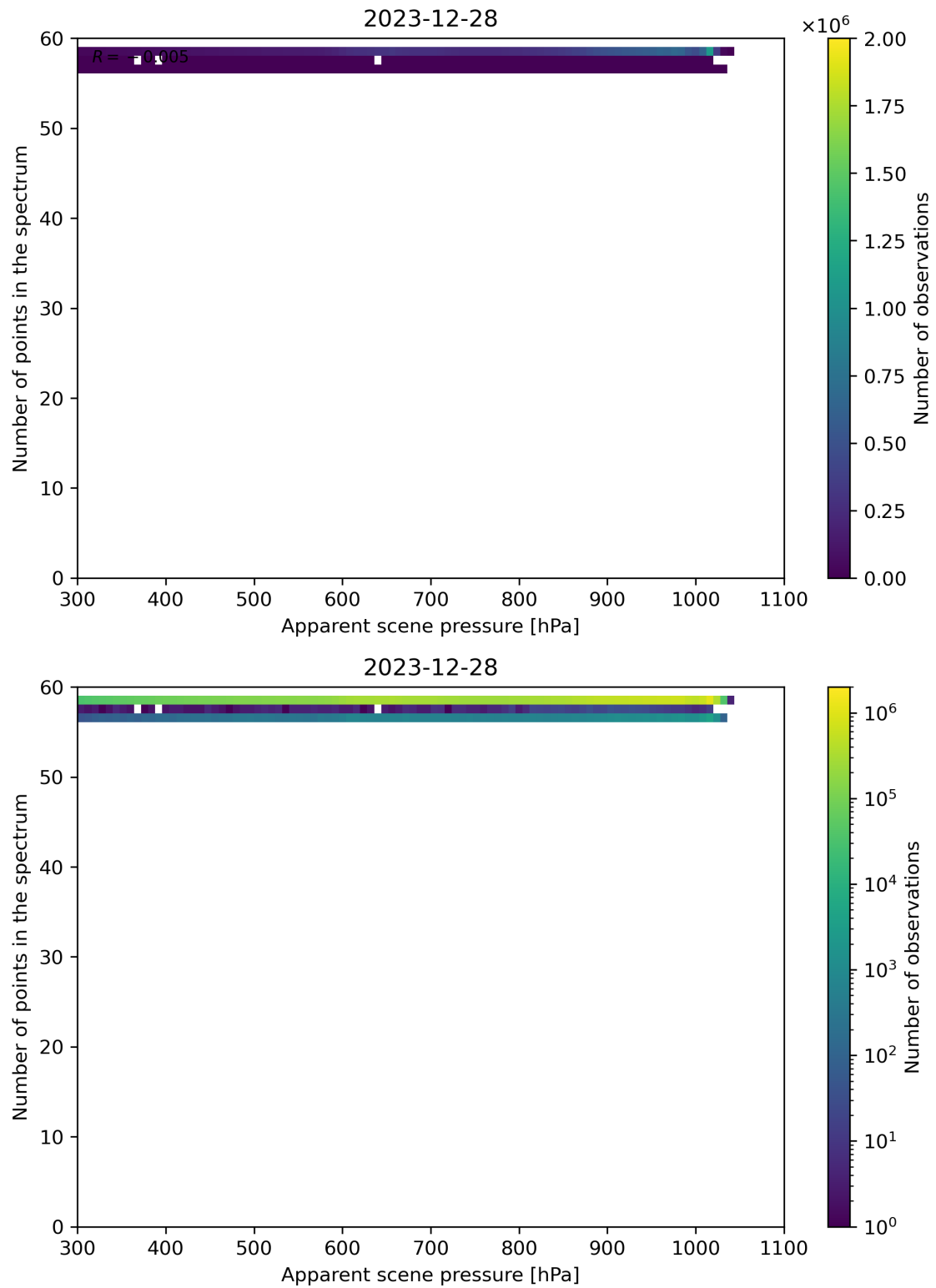
Figure 66: Scatter density plot of “Apparent scene pressure” against “Number of points in the spectrum” for 2023-12-27 to 2023-12-29.
