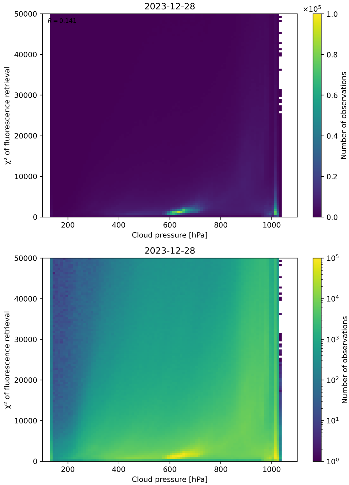
Figure 78: Scatter density plot of “Cloud pressure” against “ \chi^2 of fluorescence retrieval” for 2023-12-27 to 2023-12-29.
