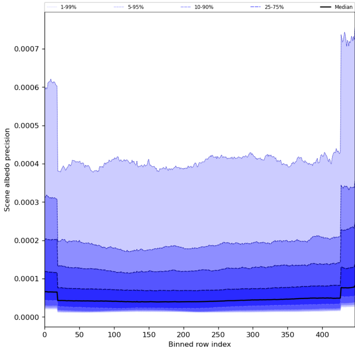
Figure 52: Along track statistics of “Scene albedo precision” for 2023-12-27 to 2023-12-29
