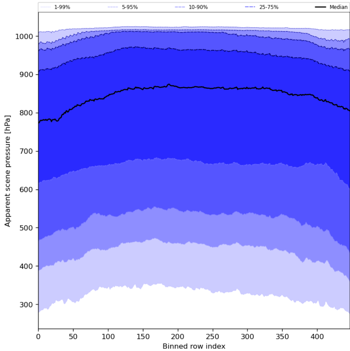
Figure 53: Along track statistics of “Apparent scene pressure” for 2023-12-27 to 2023-12-29
