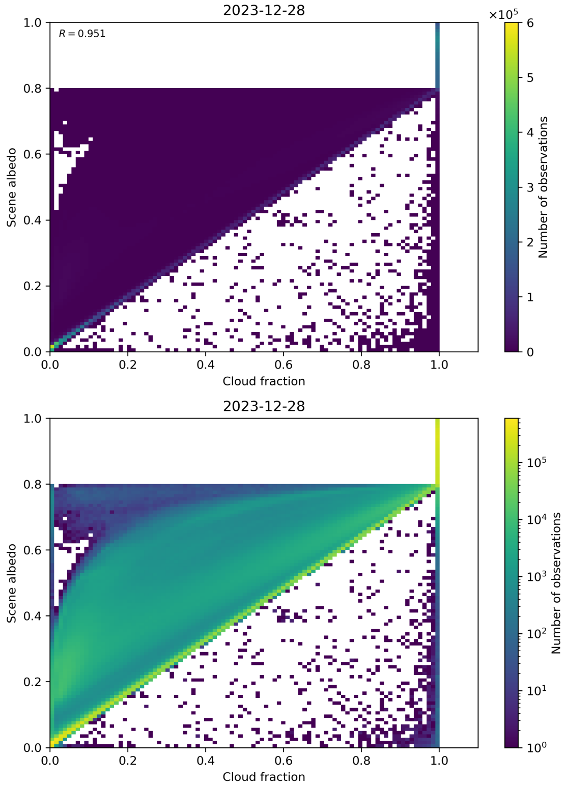
Figure 75: Scatter density plot of “Cloud fraction” against “Scene albedo” for 2023-12-27 to 2023-12-29.
