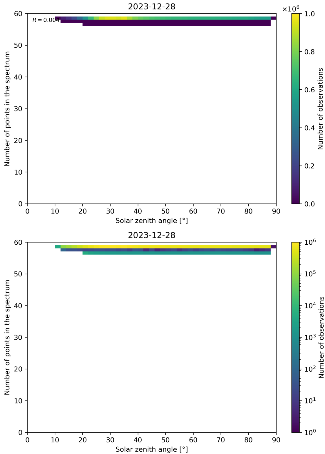
Figure 115: Scatter density plot of “Solar zenith angle” against “Number of points in the spectrum” for 2023-12-27 to 2023-12-29.
