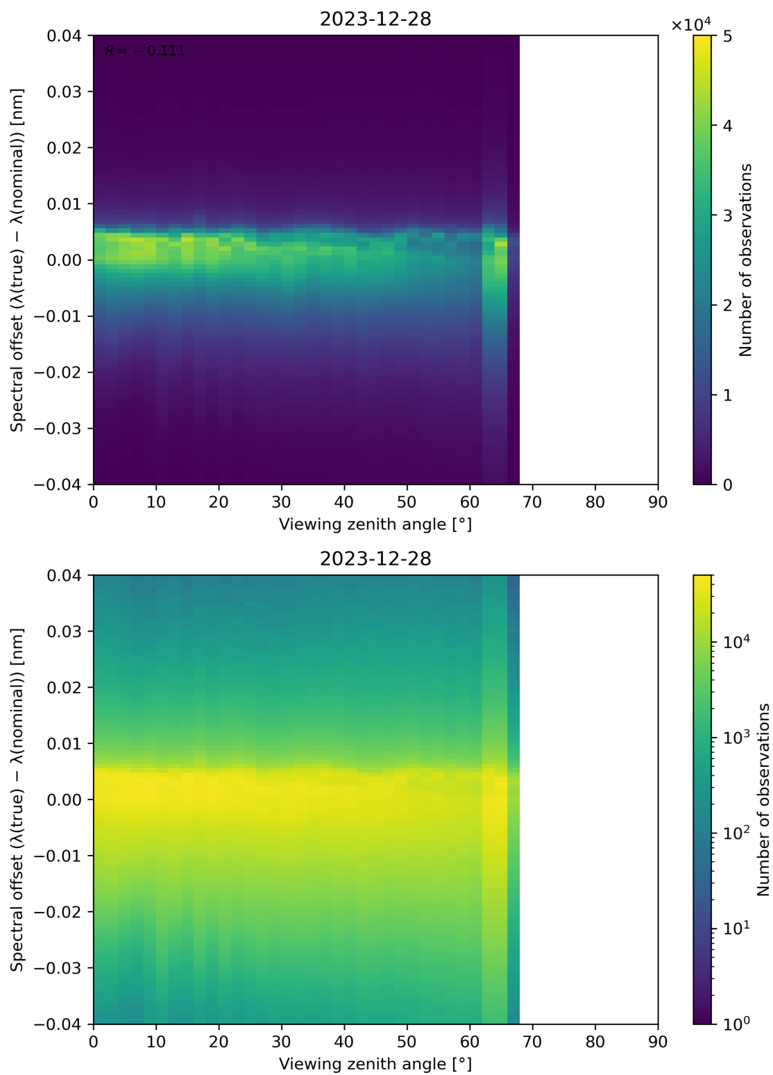
Figure 128: Scatter density plot of “Viewing zenith angle” against “Spectral offset ( \lambda(\text{true}) - \lambda(\text{nominal}) )” for 2023-12-27 to 2023-12-29.
