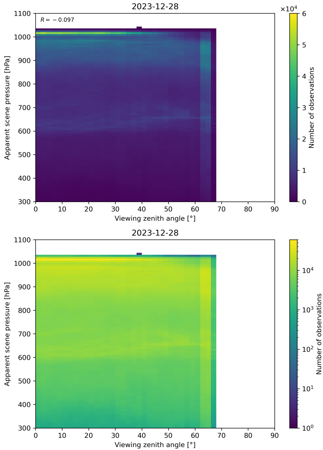
Figure 118: Scatter density plot of “Viewing zenith angle” against “Apparent scene pressure” for 2023-12-27 to 2023-12-29.
