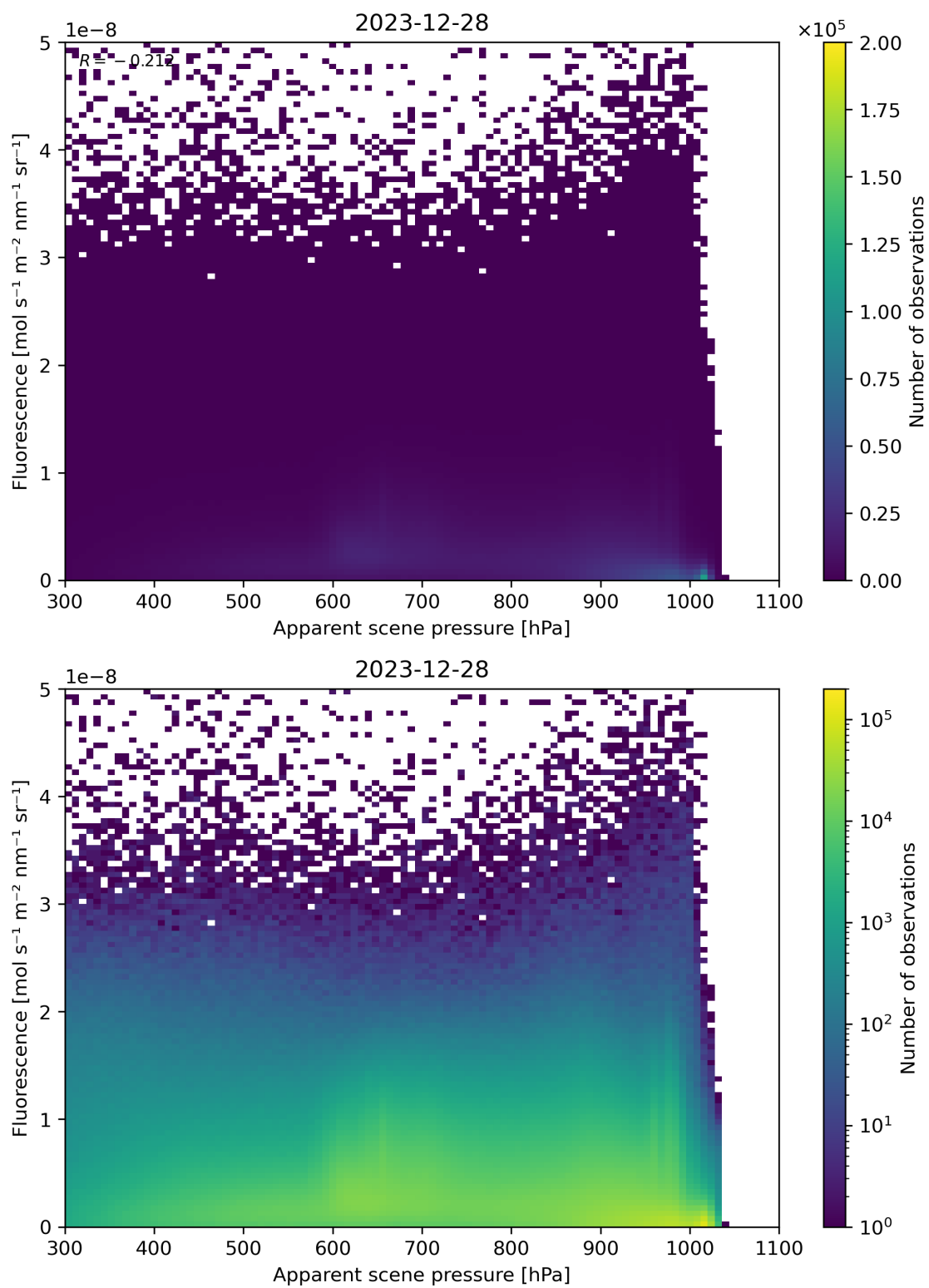
Figure 64: Scatter density plot of “Apparent scene pressure” against “Fluorescence” for 2023-12-27 to 2023-12-29.
