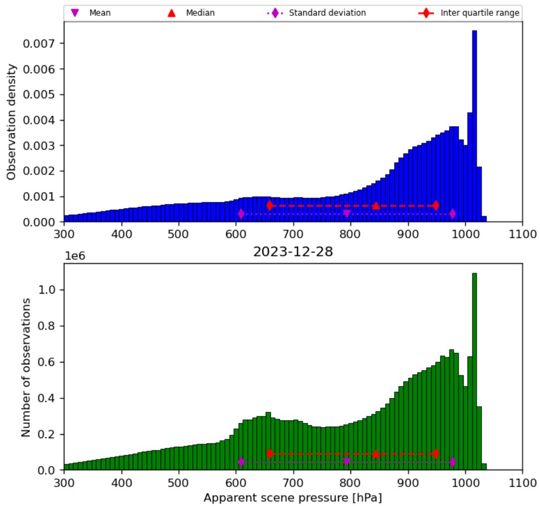
Figure 36: Histogram of “Apparent scene pressure” for 2023-12-27 to 2023-12-29
