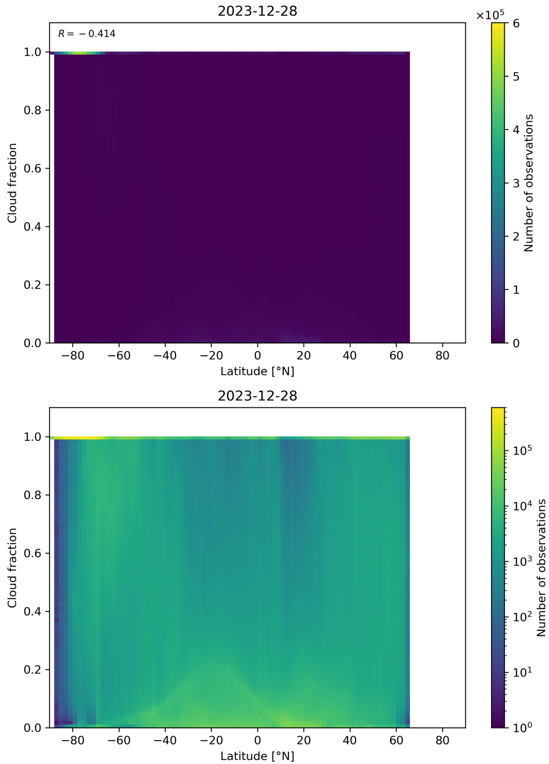
Figure 90: Scatter density plot of “Latitude” against “Cloud fraction” for 2023-12-27 to 2023-12-29.
