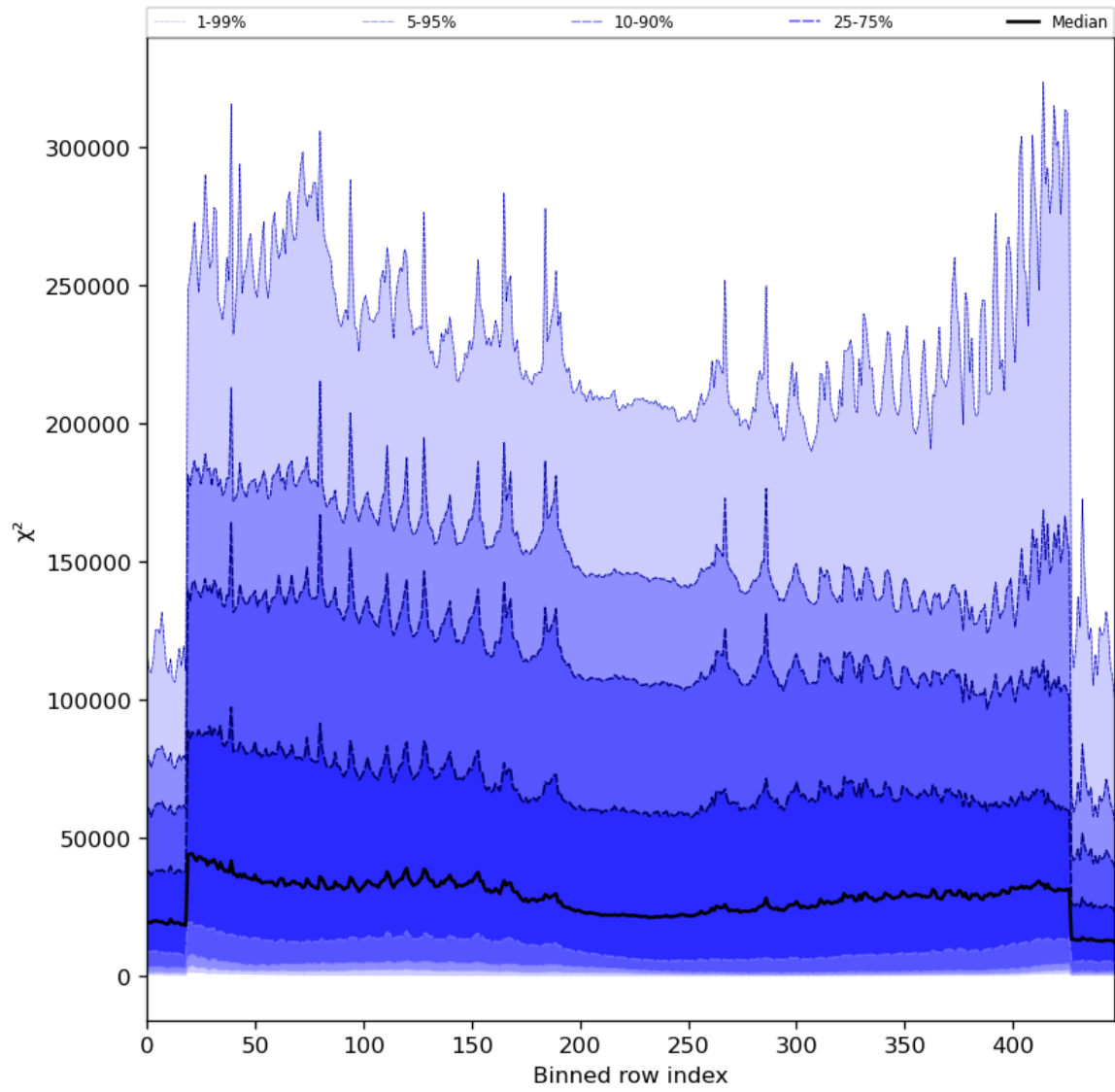
Figure 55: Along track statistics of “ \chi^2 ” for 2023-12-27 to 2023-12-29
