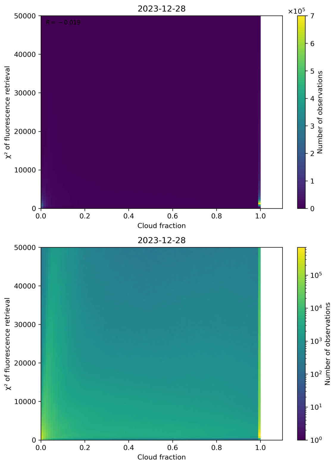
Figure 71: Scatter density plot of “Cloud fraction” against “ \chi^2 of fluorescence retrieval” for 2023-12-27 to 2023-12-29.
