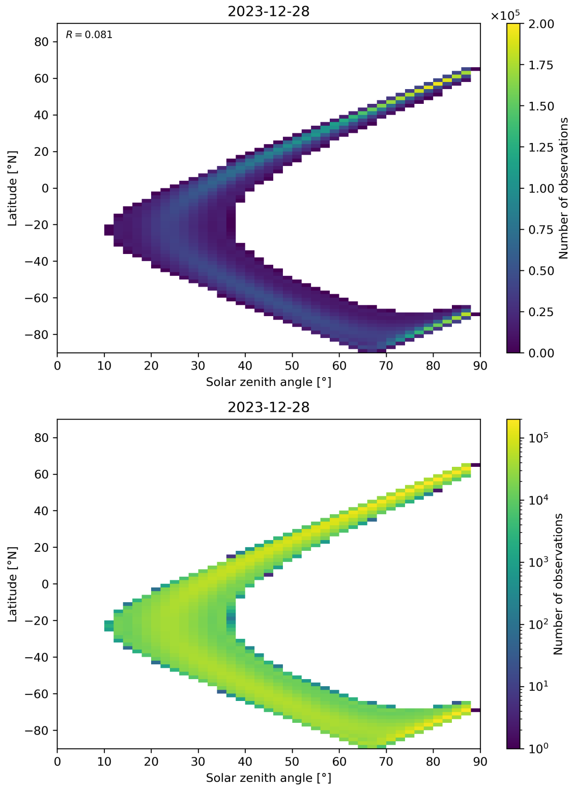
Figure 113: Scatter density plot of “Solar zenith angle” against “Latitude” for 2023-12-27 to 2023-12-29.
