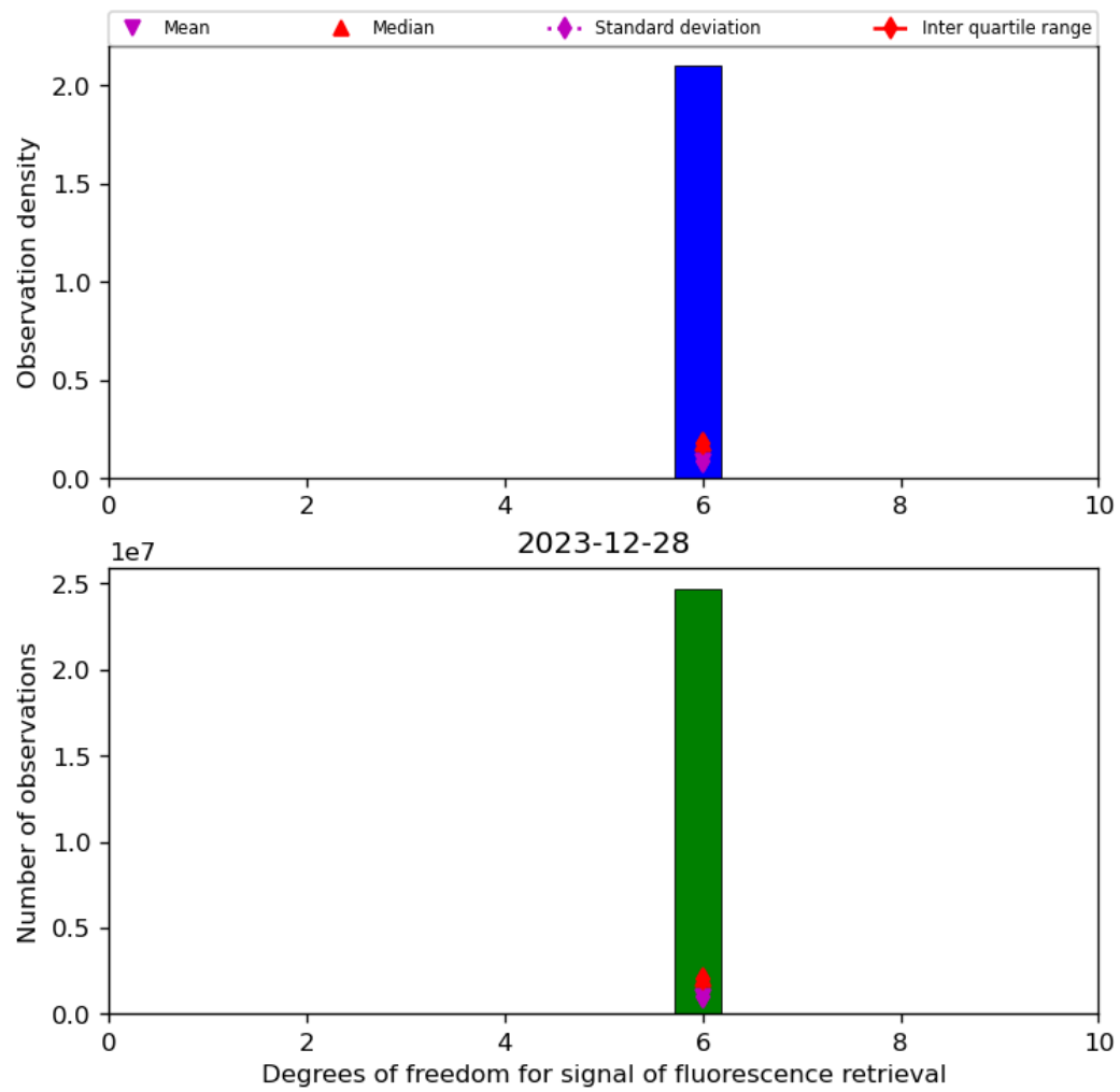
Figure 43: Histogram of “Degrees of freedom for signal of fluorescence retrieval” for 2023-12-27 to 2023-12-29
