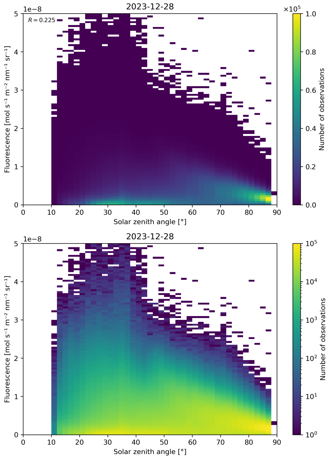
Figure 112: Scatter density plot of “Solar zenith angle” against “Fluorescence” for 2023-12-27 to 2023-12-29.
