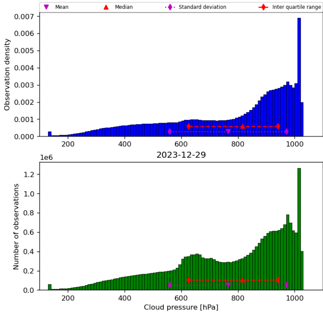
Figure 30: Histogram of “Cloud pressure” for 2023-12-28 to 2023-12-30
