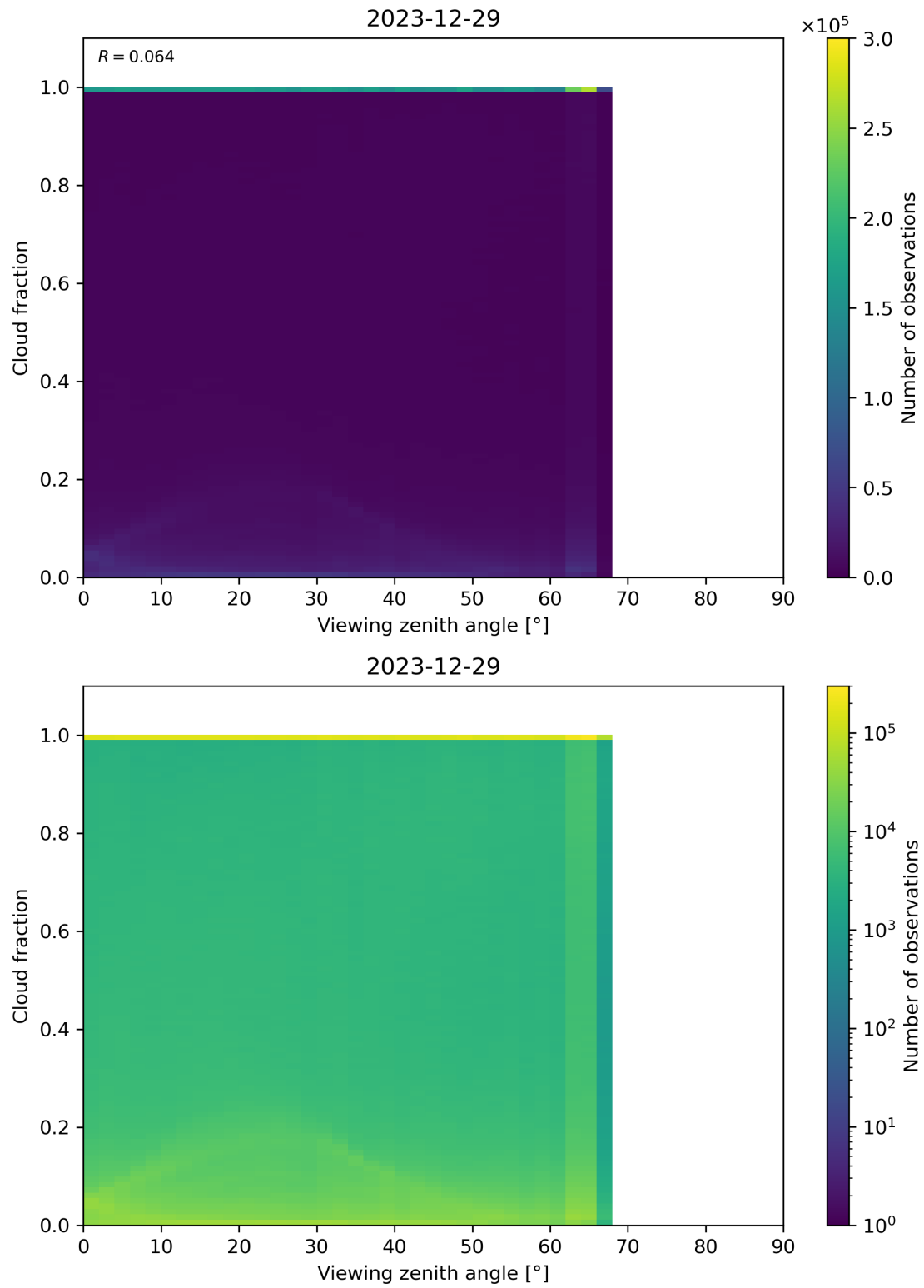
Figure 120: Scatter density plot of “Viewing zenith angle” against “Cloud fraction” for 2023-12-28 to 2023-12-30.
