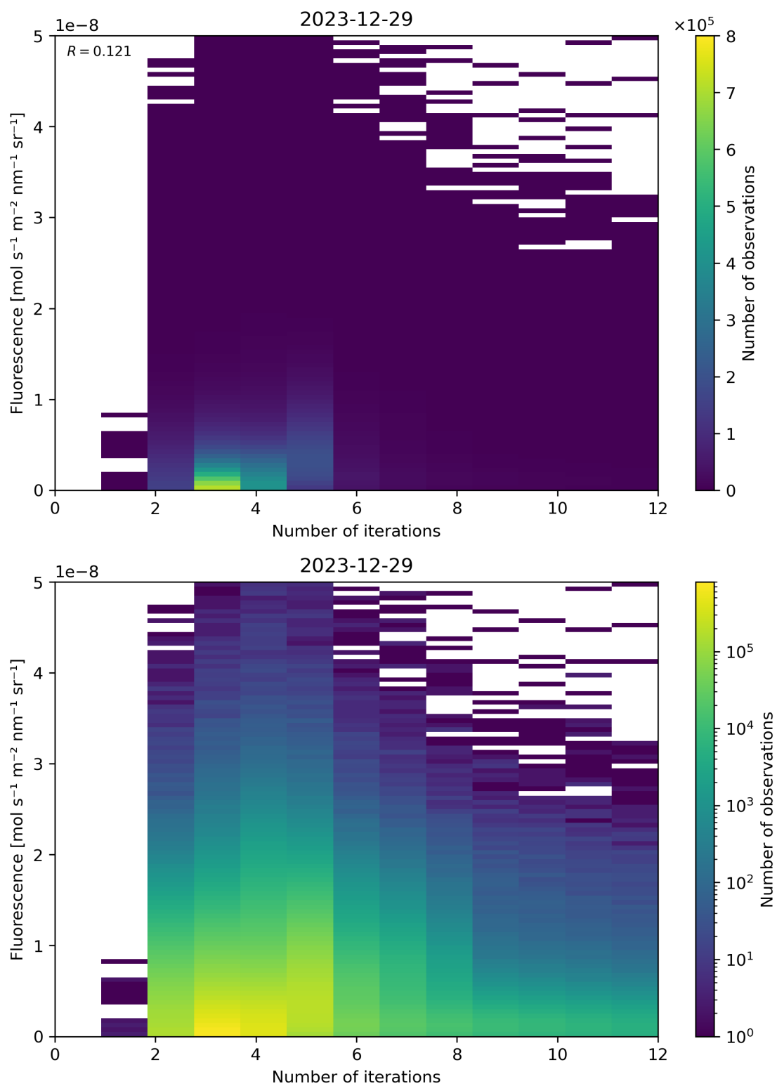
Figure 98: Scatter density plot of “Number of iterations” against “Fluorescence” for 2023-12-28 to 2023-12-30.
