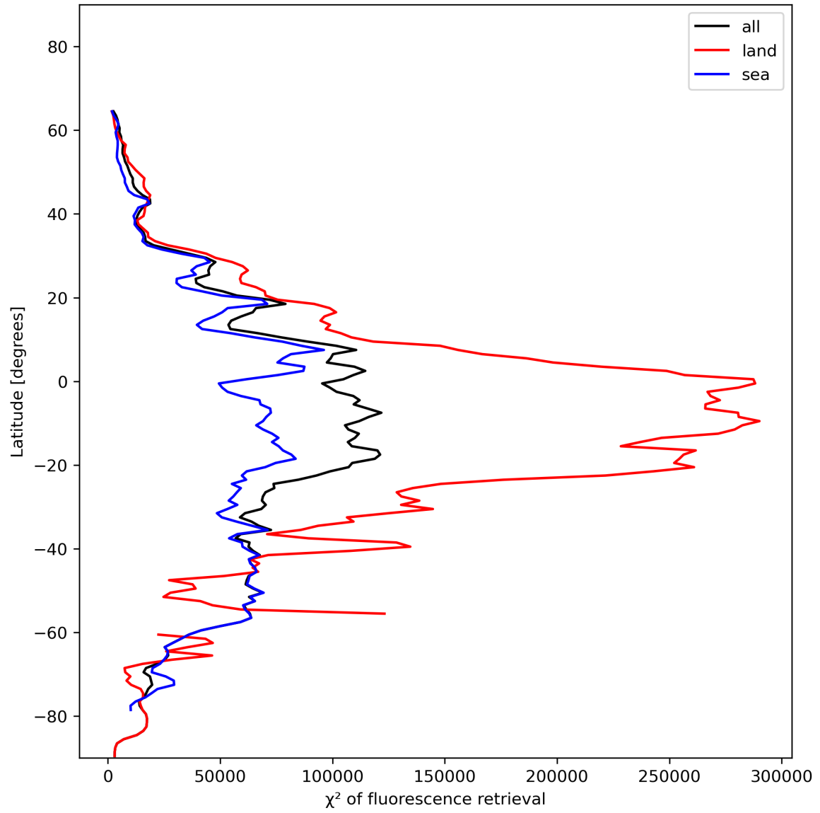
Figure 25: Zonal average of “ \chi^2 of fluorescence retrieval” for 2023-12-28 to 2023-12-30.
