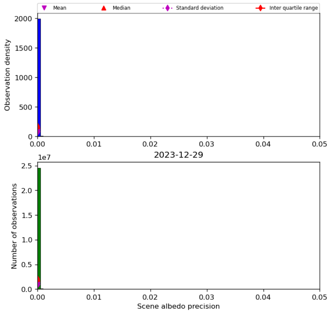
Figure 35: Histogram of “Scene albedo precision” for 2023-12-28 to 2023-12-30
