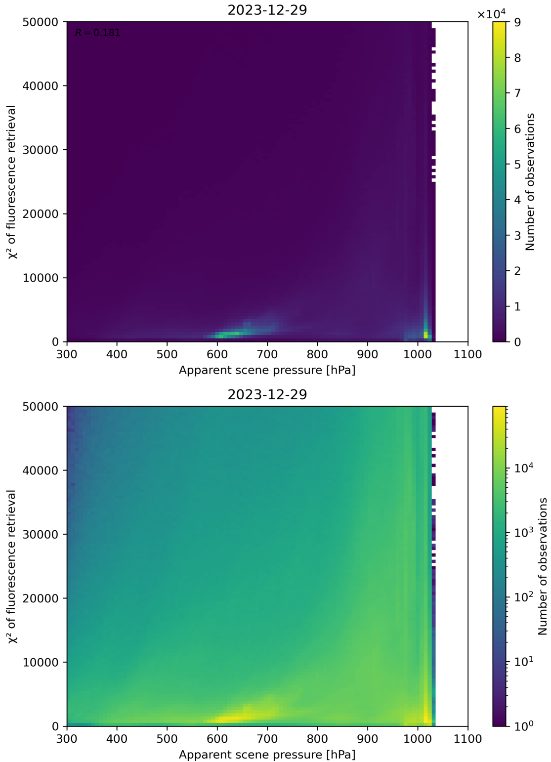
Figure 63: Scatter density plot of “Apparent scene pressure” against “ \chi^2 of fluorescence retrieval” for 2023-12-28 to 2023-12-30.
