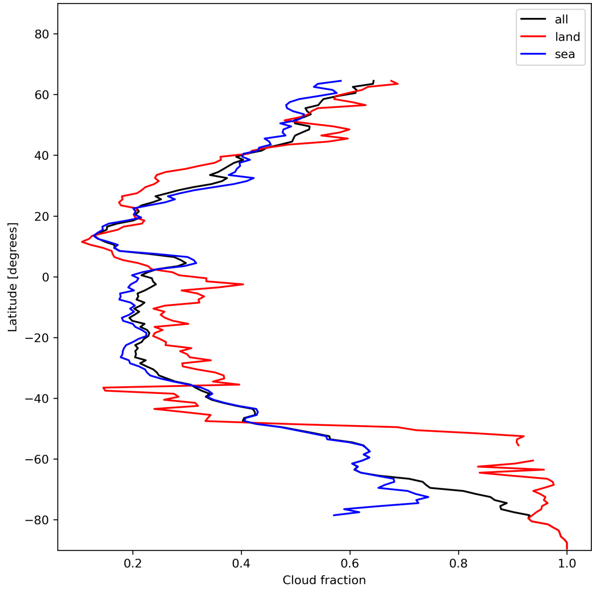
Figure 15: Zonal average of “Cloud fraction” for 2023-12-28 to 2023-12-30.
