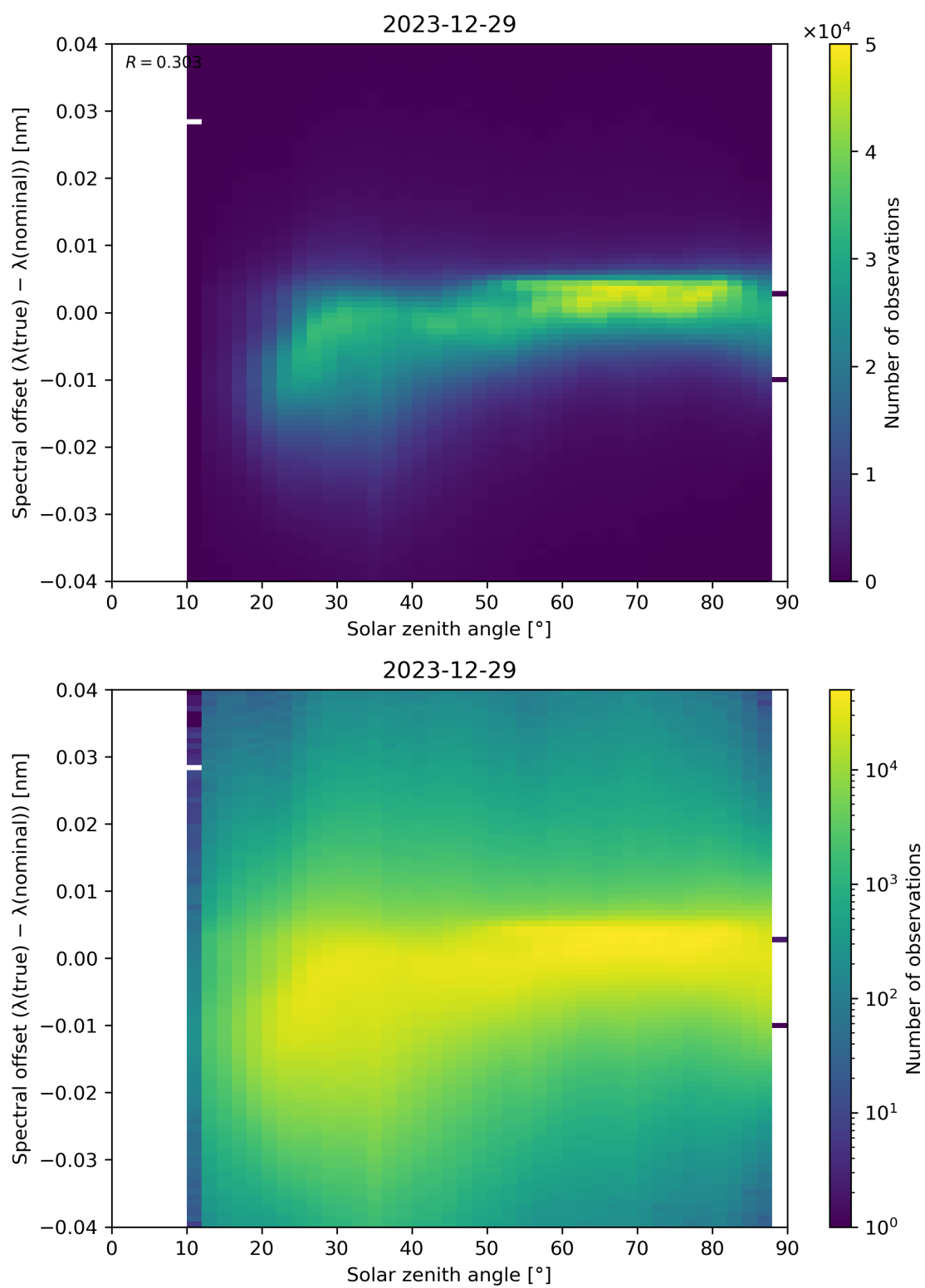
Figure 117: Scatter density plot of “Solar zenith angle” against “Spectral offset ( \lambda(\text{true}) - \lambda(\text{nominal}) )” for 2023-12-28 to 2023-12-30.
