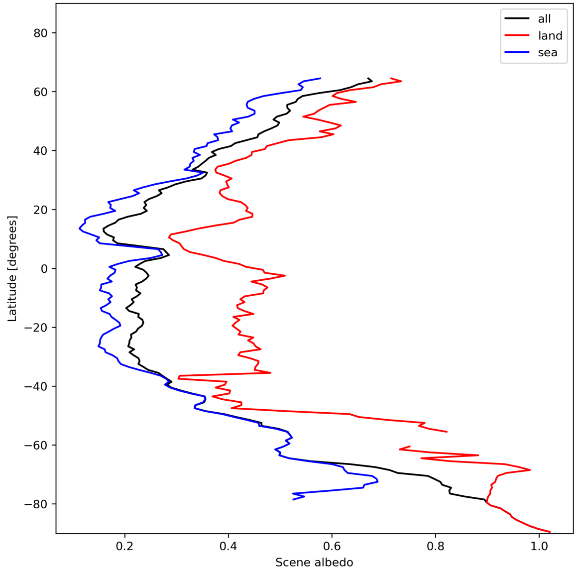
Figure 17: Zonal average of “Scene albedo” for 2023-12-28 to 2023-12-30.
