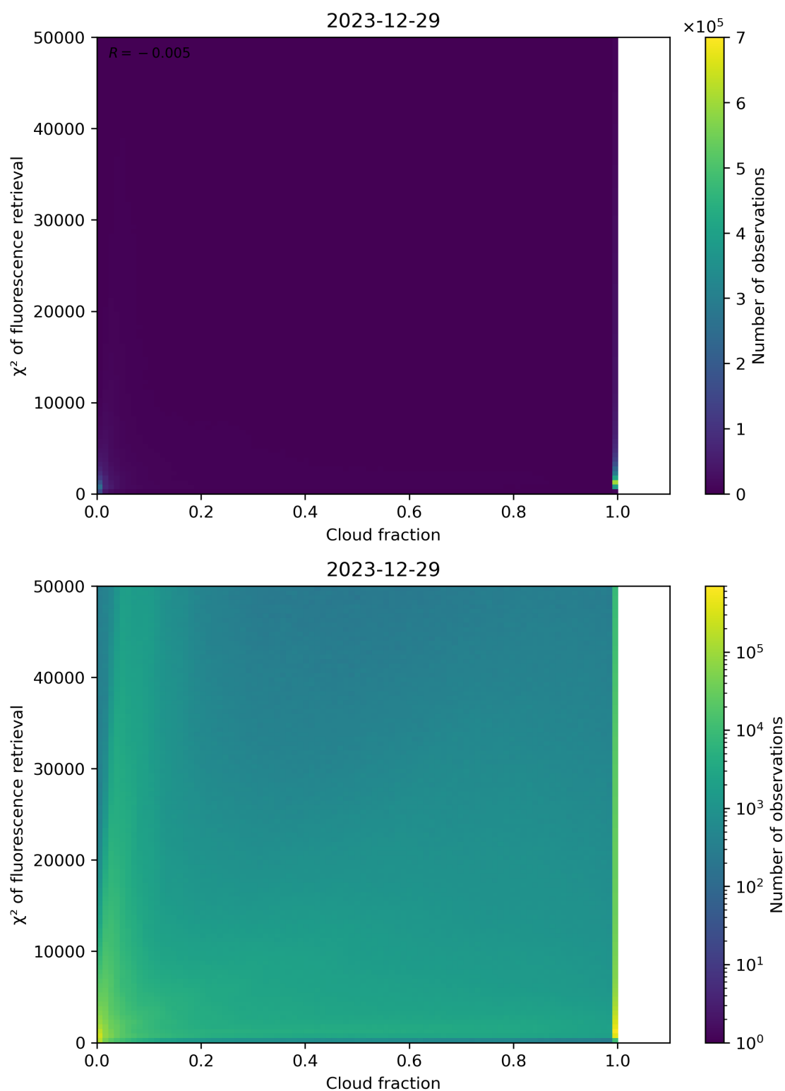
Figure 71: Scatter density plot of “Cloud fraction” against “ \chi^2 of fluorescence retrieval” for 2023-12-28 to 2023-12-30.
