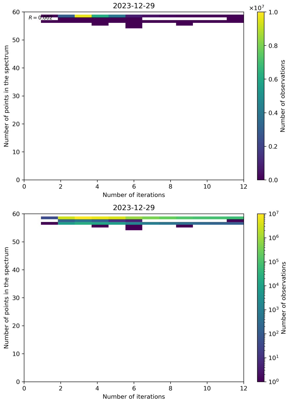
Figure 99: Scatter density plot of “Number of iterations” against “Number of points in the spectrum” for 2023-12-28 to 2023-12-30.
