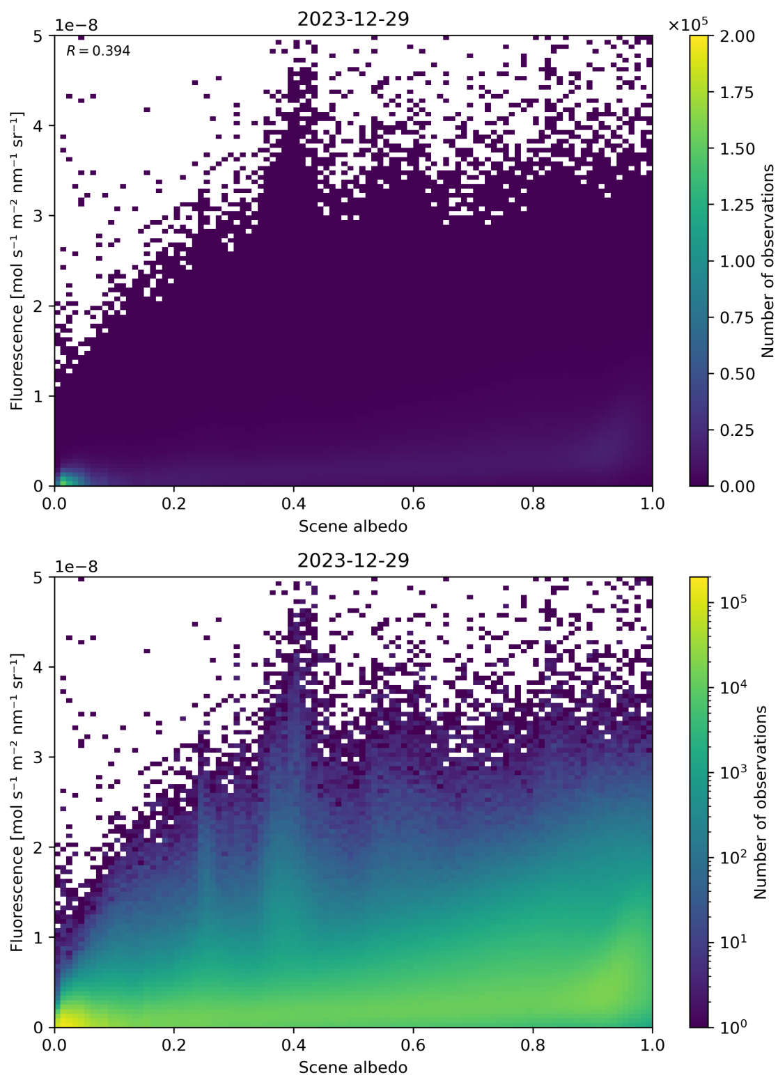
Figure 104: Scatter density plot of “Scene albedo” against “Fluorescence” for 2023-12-28 to 2023-12-30.
