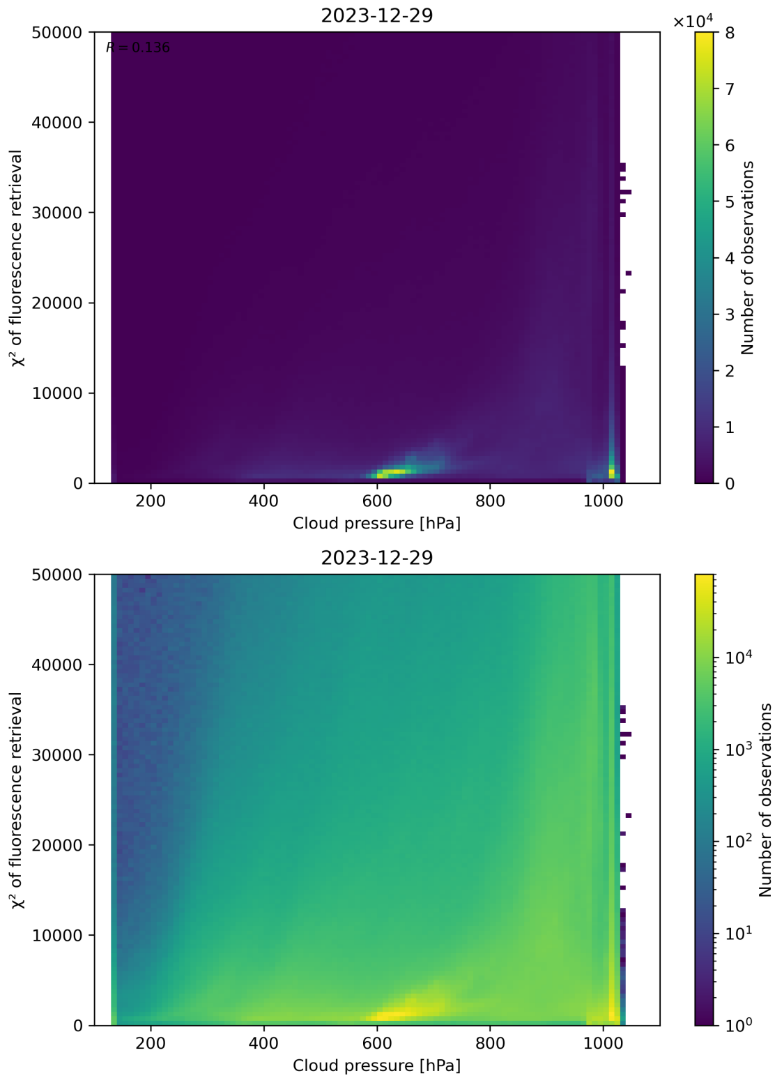
Figure 78: Scatter density plot of “Cloud pressure” against “ \chi^2 of fluorescence retrieval” for 2023-12-28 to 2023-12-30.
