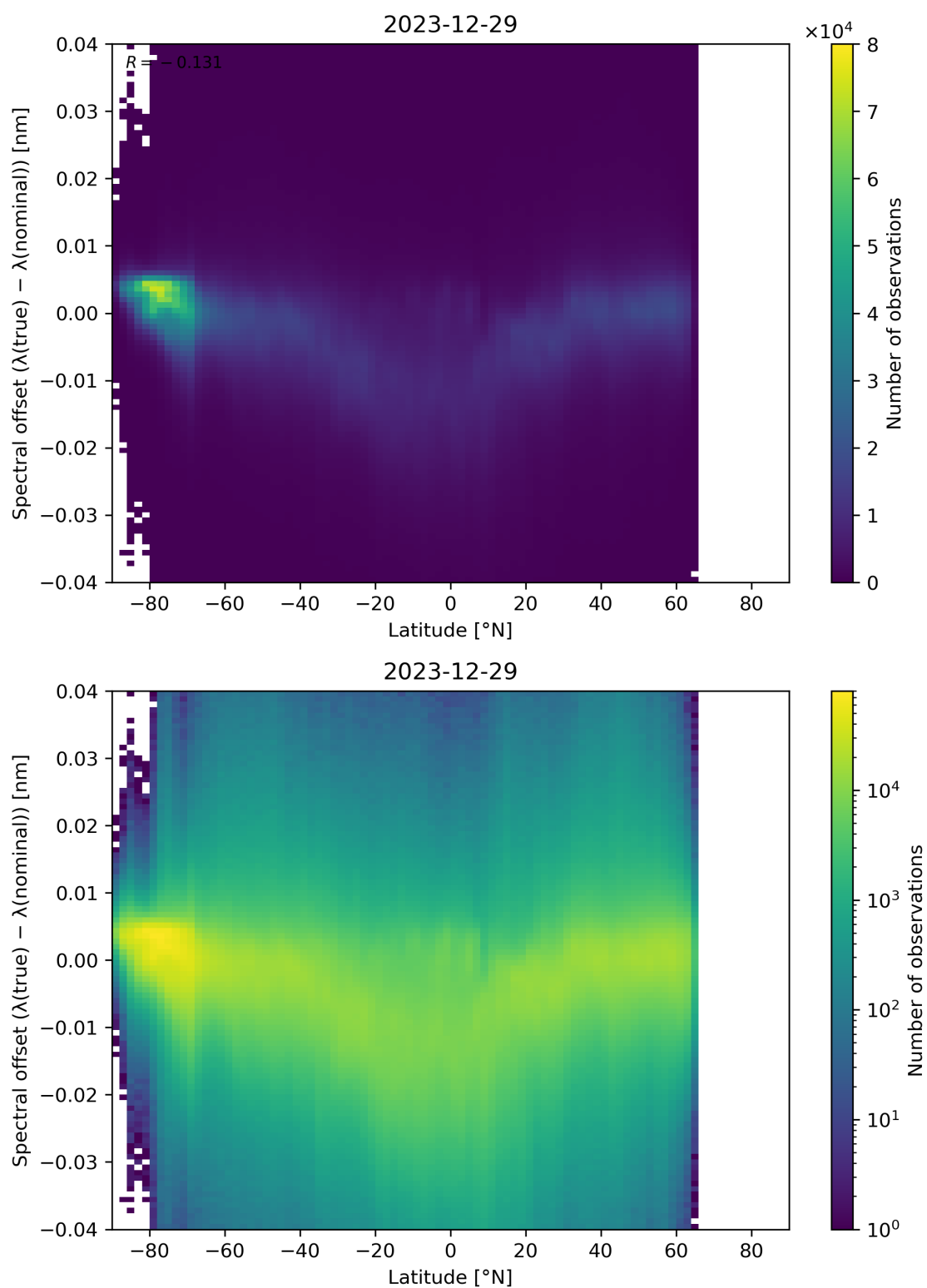
Figure 96: Scatter density plot of “Latitude” against “Spectral offset ( \lambda(\text{true}) - \lambda(\text{nominal}) )” for 2023-12-28 to 2023-12-30.
