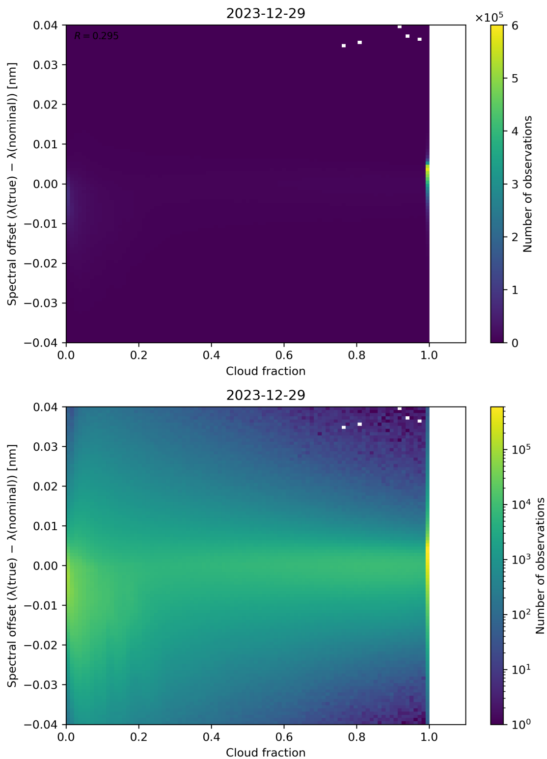
Figure 76: Scatter density plot of “Cloud fraction” against “Spectral offset ( \lambda(\text{true}) - \lambda(\text{nominal}) )” for 2023-12-28 to 2023-12-30.
