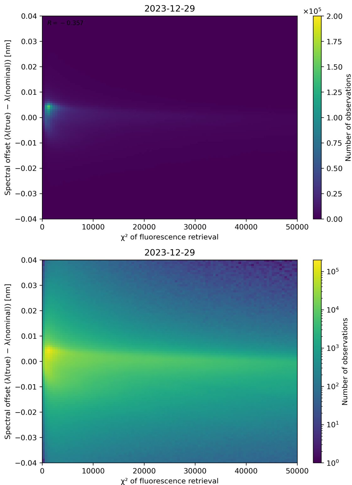
Figure 69: Scatter density plot of " \chi^2 of fluorescence retrieval" against "Spectral offset ( \lambda(\text{true}) - \lambda(\text{nominal}) )" for 2023-12-28 to 2023-12-30.
