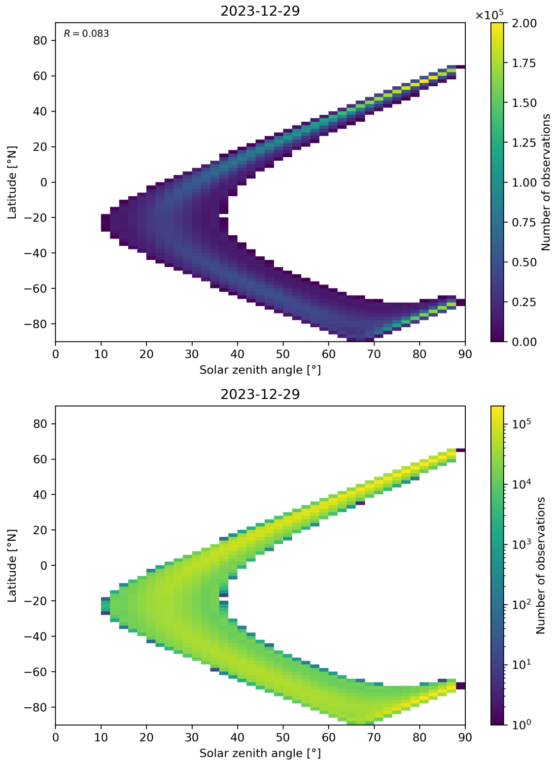
Figure 113: Scatter density plot of “Solar zenith angle” against “Latitude” for 2023-12-28 to 2023-12-30.
