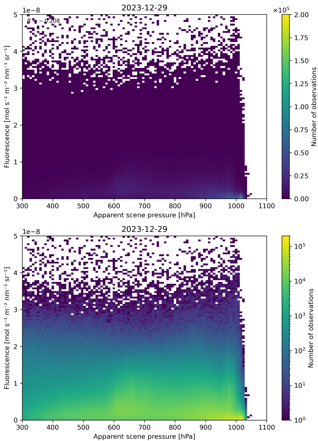
Figure 64: Scatter density plot of “Apparent scene pressure” against “Fluorescence” for 2023-12-28 to 2023-12-30.
