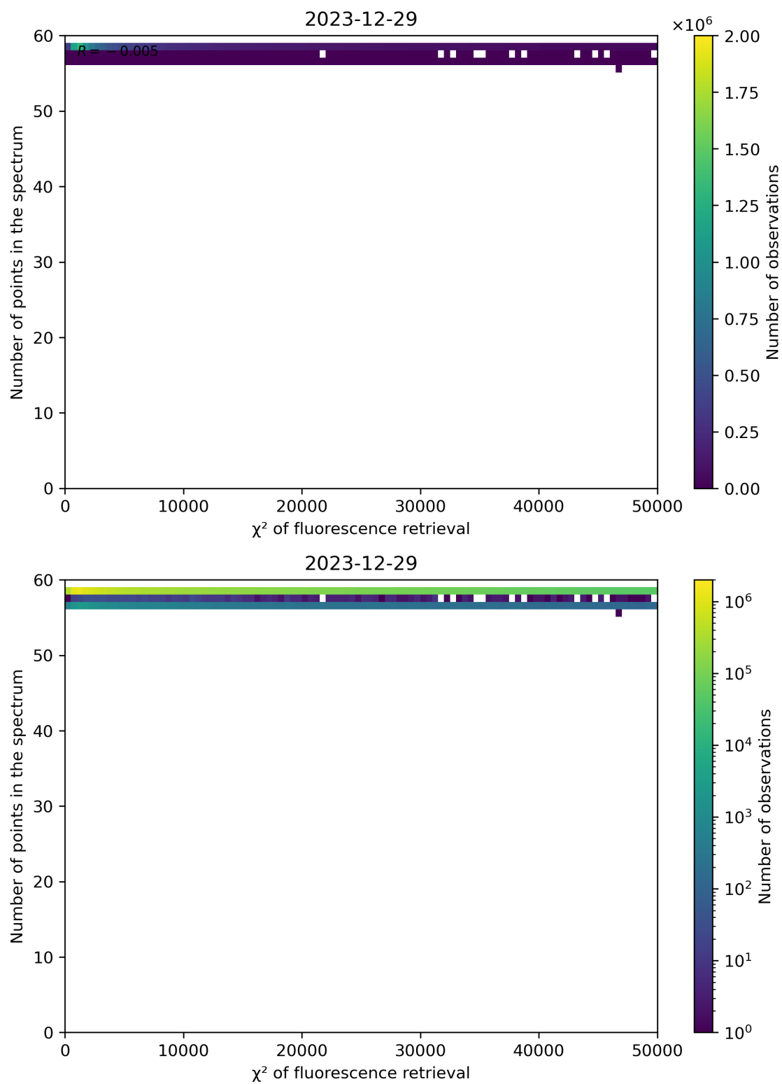
Figure 68: Scatter density plot of " \chi^2 of fluorescence retrieval" against "Number of points in the spectrum" for 2023-12-28 to 2023-12-30.
