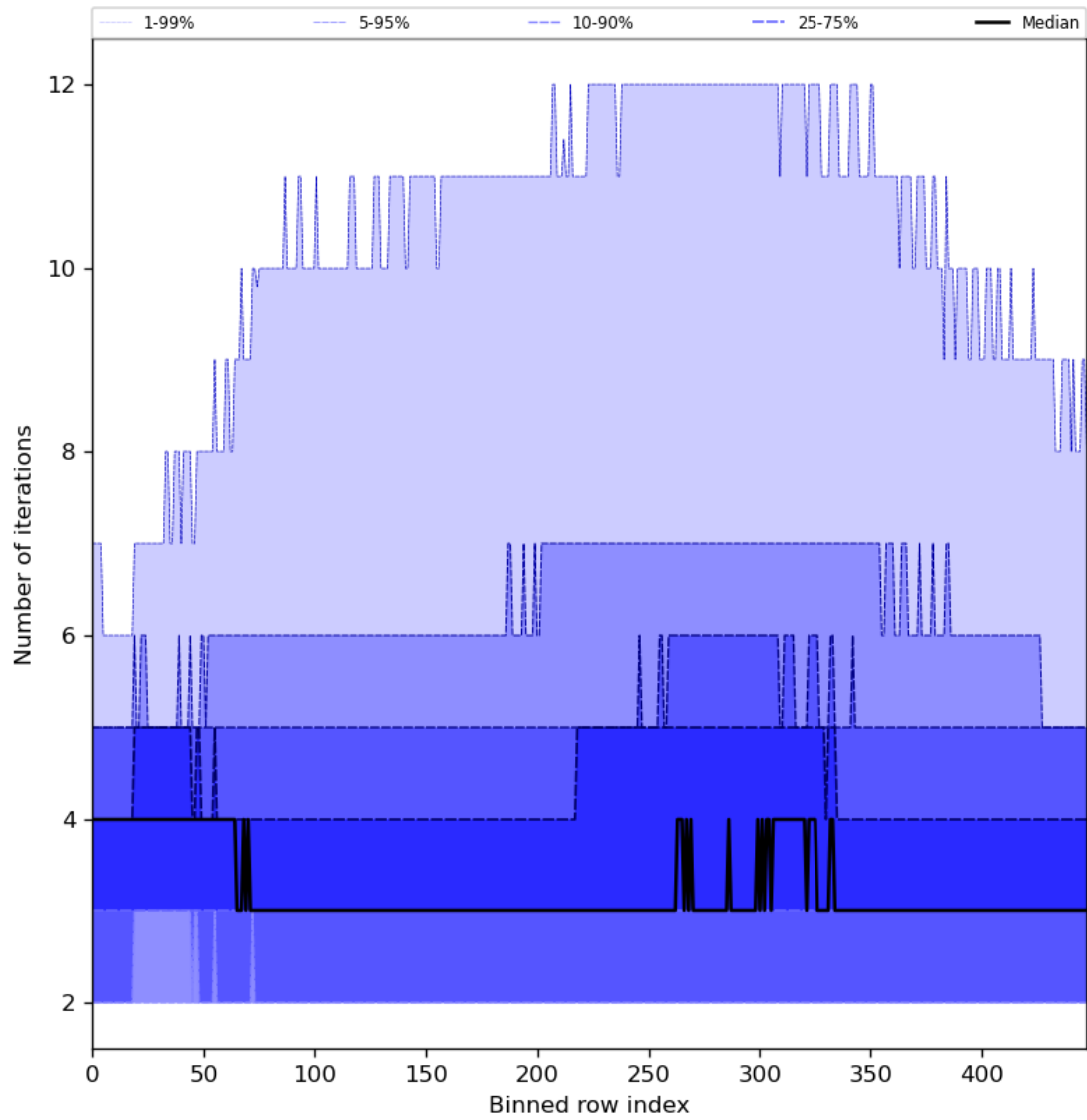
Figure 56: Along track statistics of “Number of iterations” for 2023-12-28 to 2023-12-30
