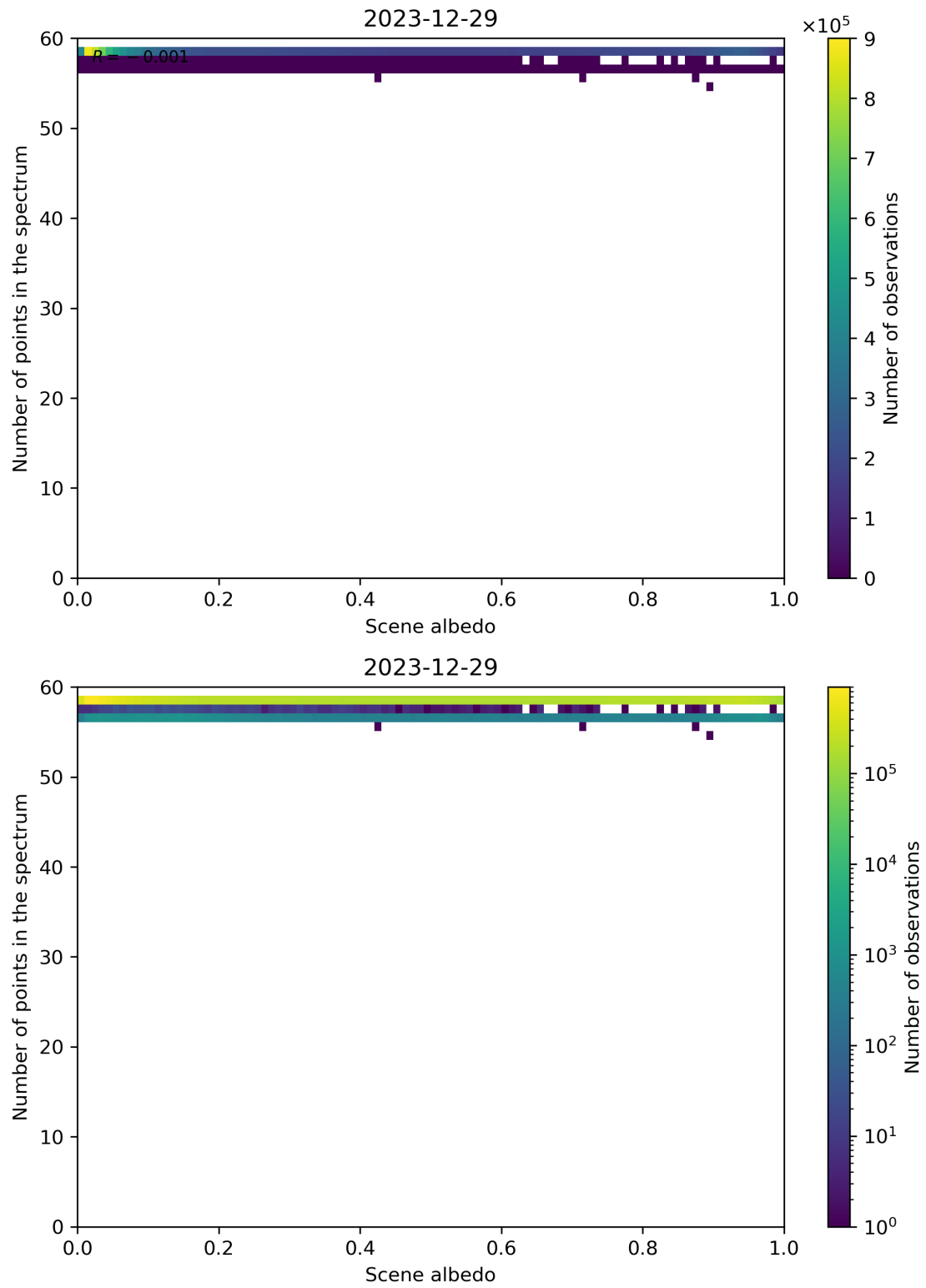
Figure 106: Scatter density plot of “Scene albedo” against “Number of points in the spectrum” for 2023-12-28 to 2023-12-30.
