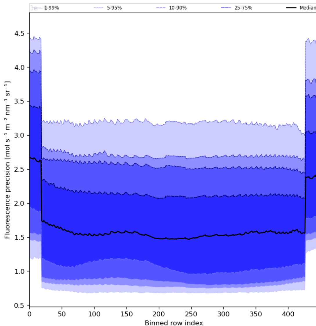
Figure 58: Along track statistics of “Fluorescence precision” for 2023-12-28 to 2023-12-30
