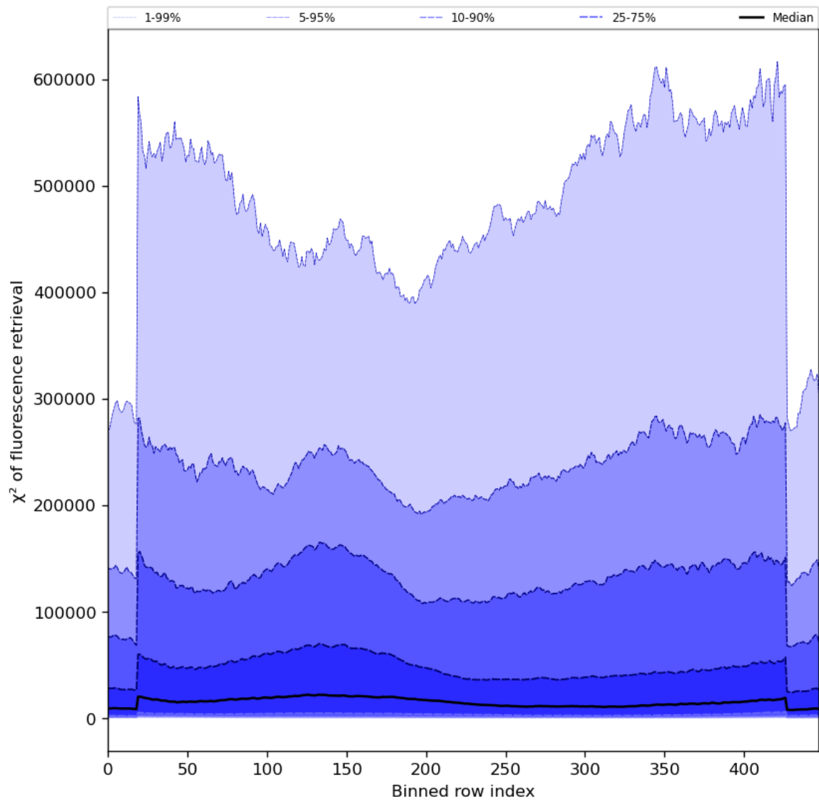
Figure 59: Along track statistics of “ \chi^2 of fluorescence retrieval” for 2023-12-28 to 2023-12-30
