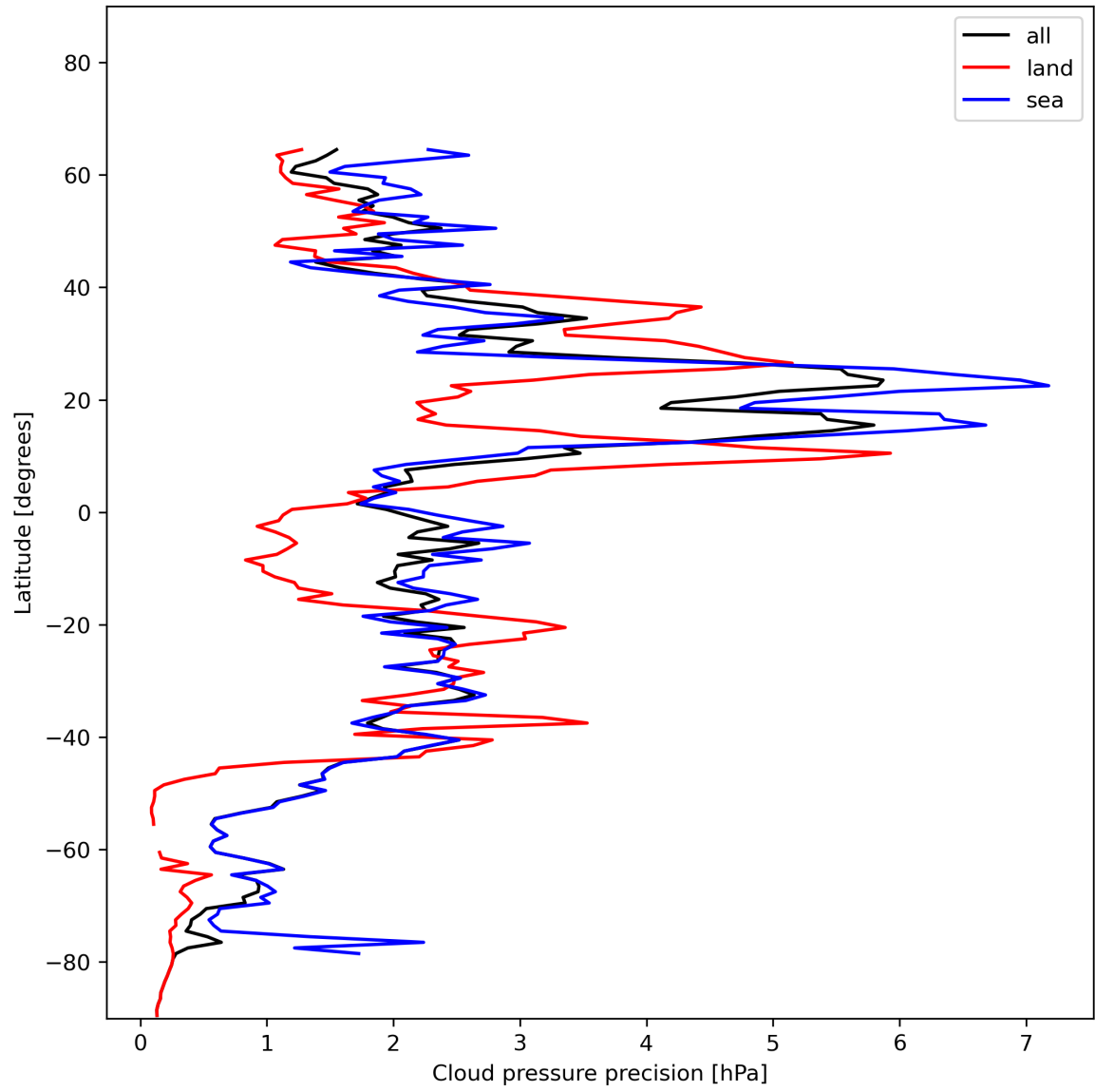
Figure 14: Zonal average of “Cloud pressure precision” for 2023-12-28 to 2023-12-30.
