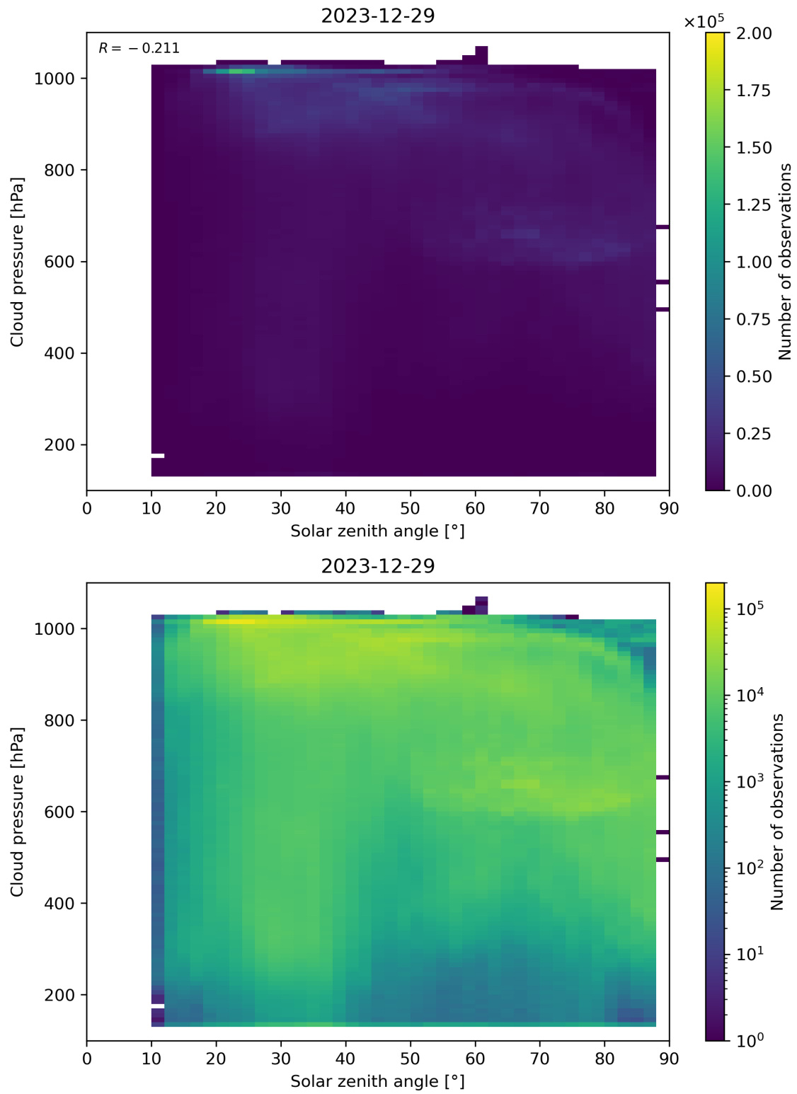
Figure 111: Scatter density plot of “Solar zenith angle” against “Cloud pressure” for 2023-12-28 to 2023-12-30.
