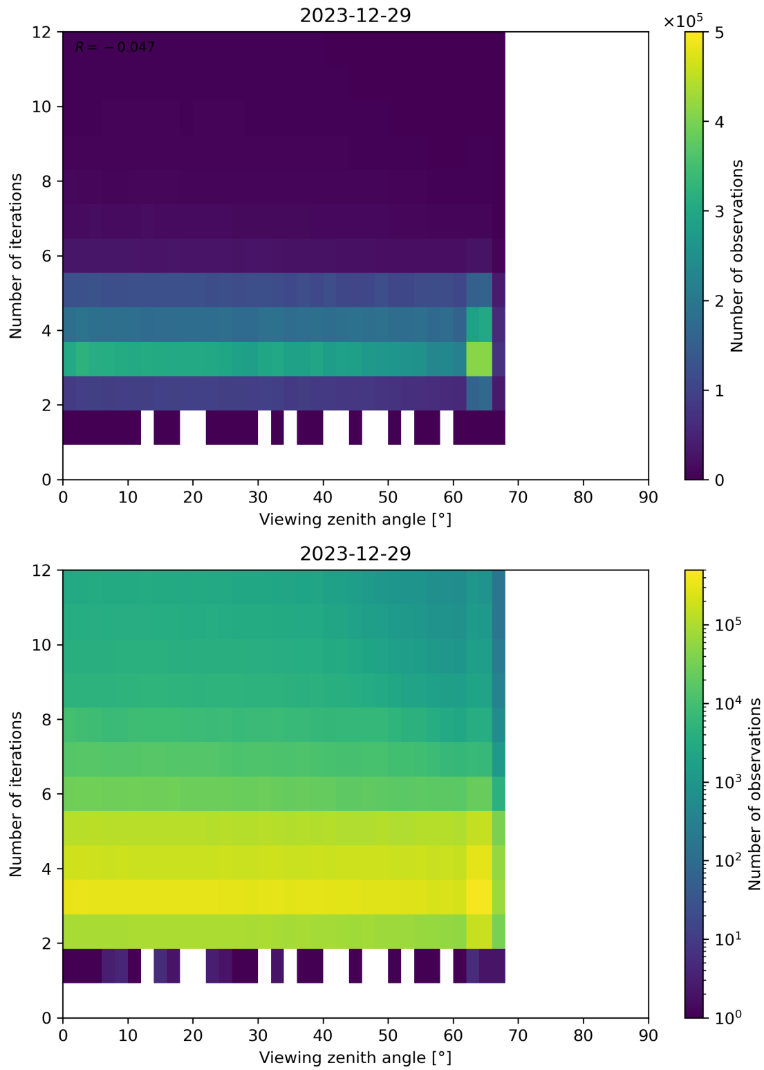
Figure 124: Scatter density plot of “Viewing zenith angle” against “Number of iterations” for 2023-12-28 to 2023-12-30.
