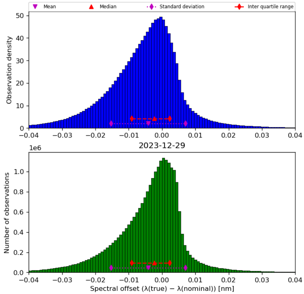
Figure 45: Histogram of “Spectral offset ( \lambda(\text{true}) - \lambda(\text{nominal}) )” for 2023-12-28 to 2023-12-30
