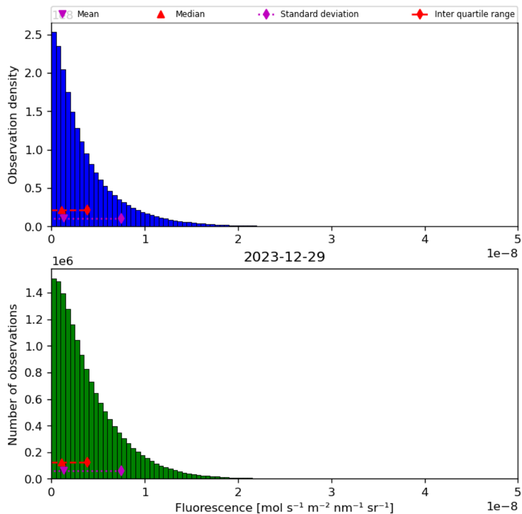
Figure 40: Histogram of “Fluorescence” for 2023-12-28 to 2023-12-30
