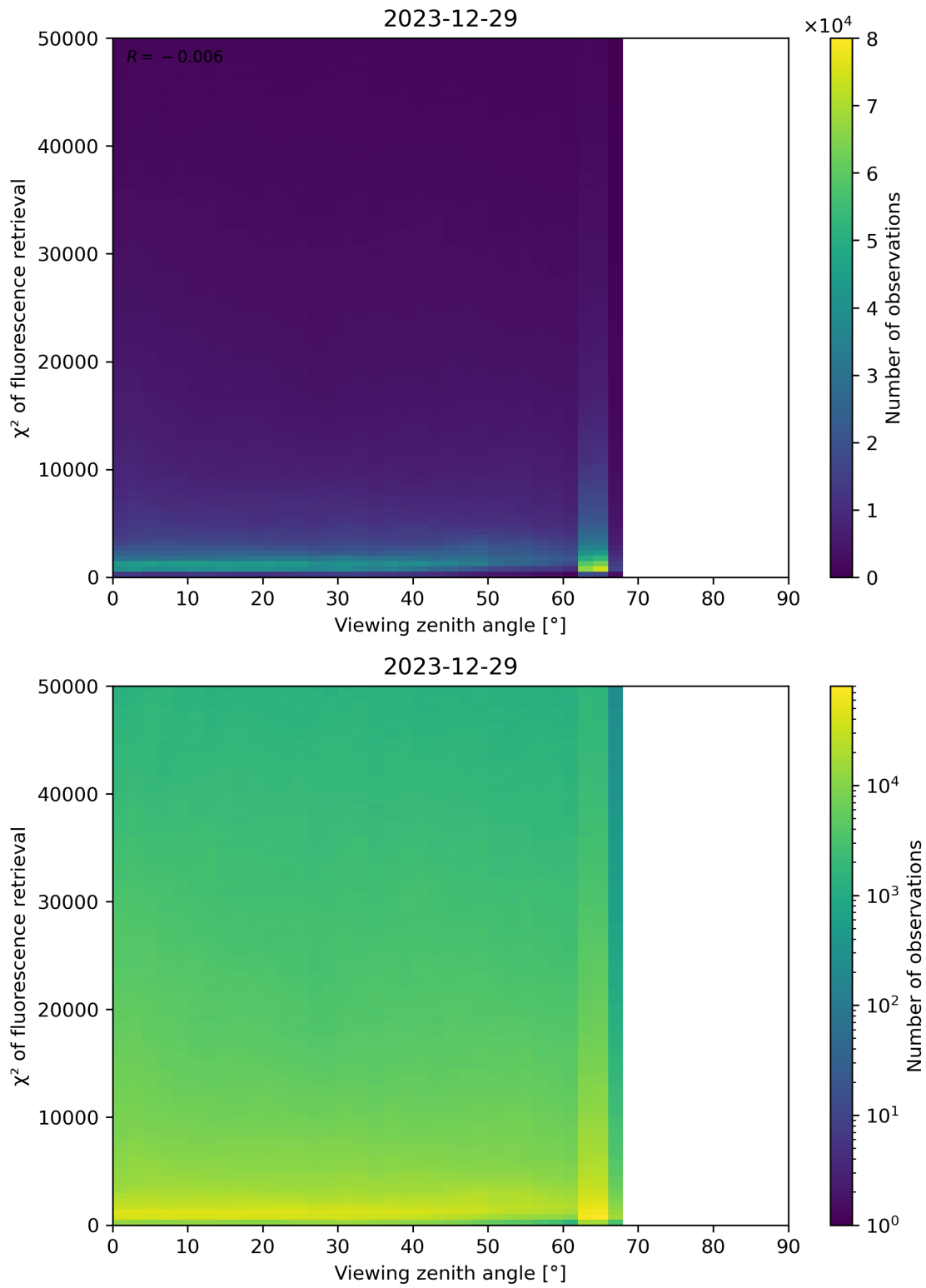
Figure 119: Scatter density plot of “Viewing zenith angle” against “ \chi^2 of fluorescence retrieval” for 2023-12-28 to 2023-12-30.
