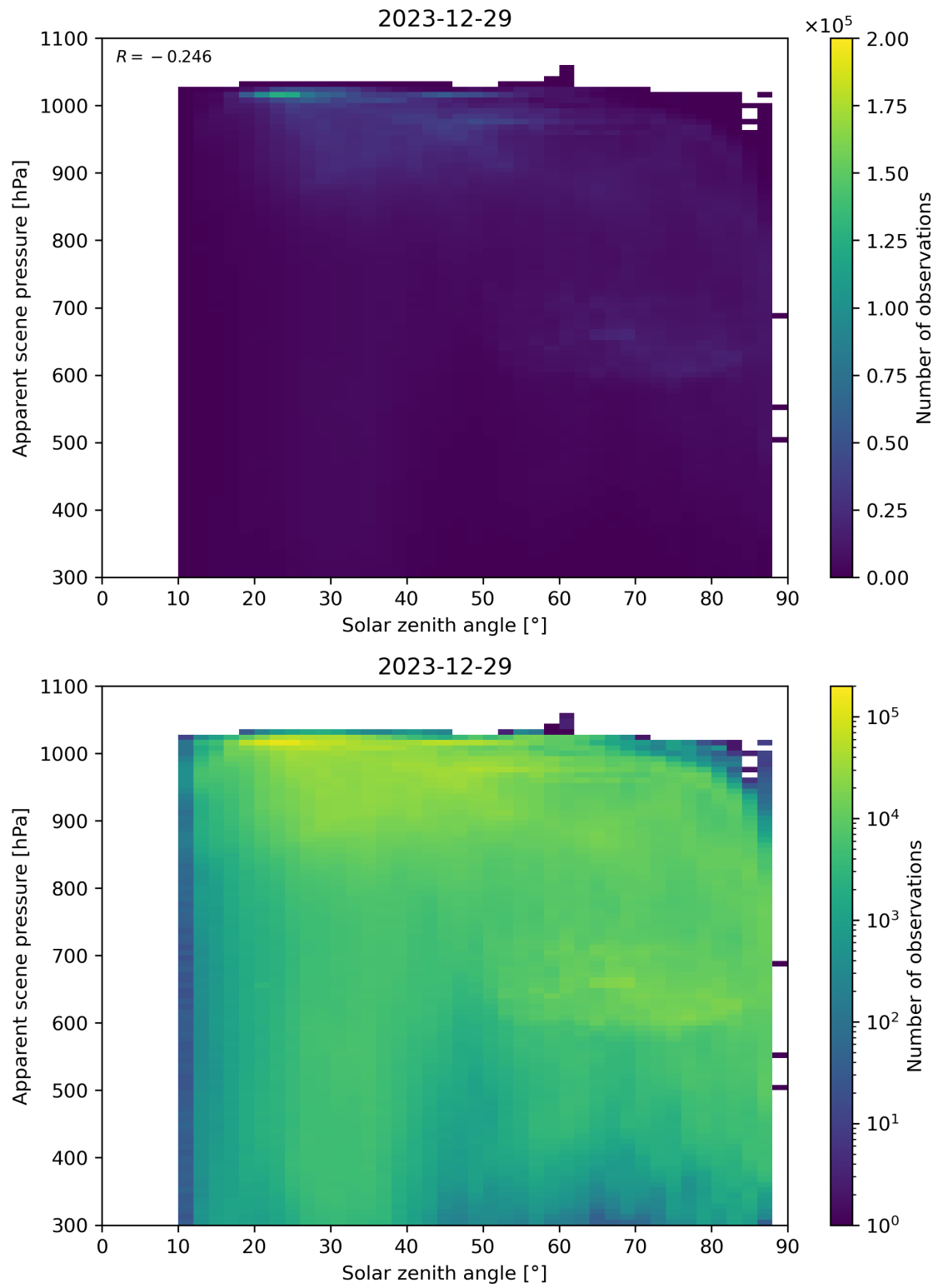
Figure 108: Scatter density plot of “Solar zenith angle” against “Apparent scene pressure” for 2023-12-28 to 2023-12-30.
