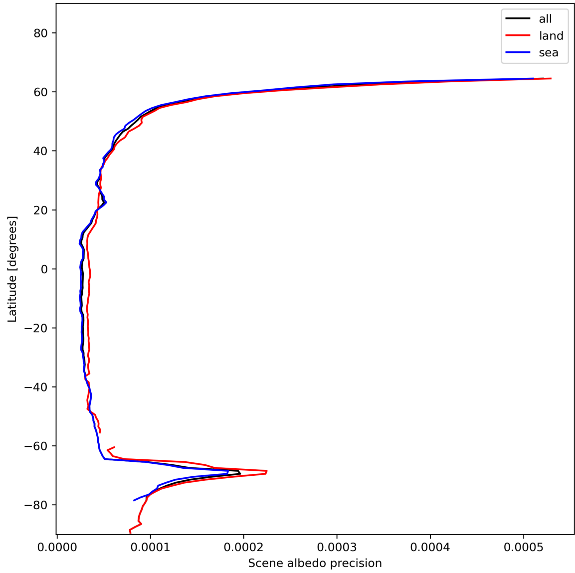
Figure 18: Zonal average of “Scene albedo precision” for 2023-12-28 to 2023-12-30.
