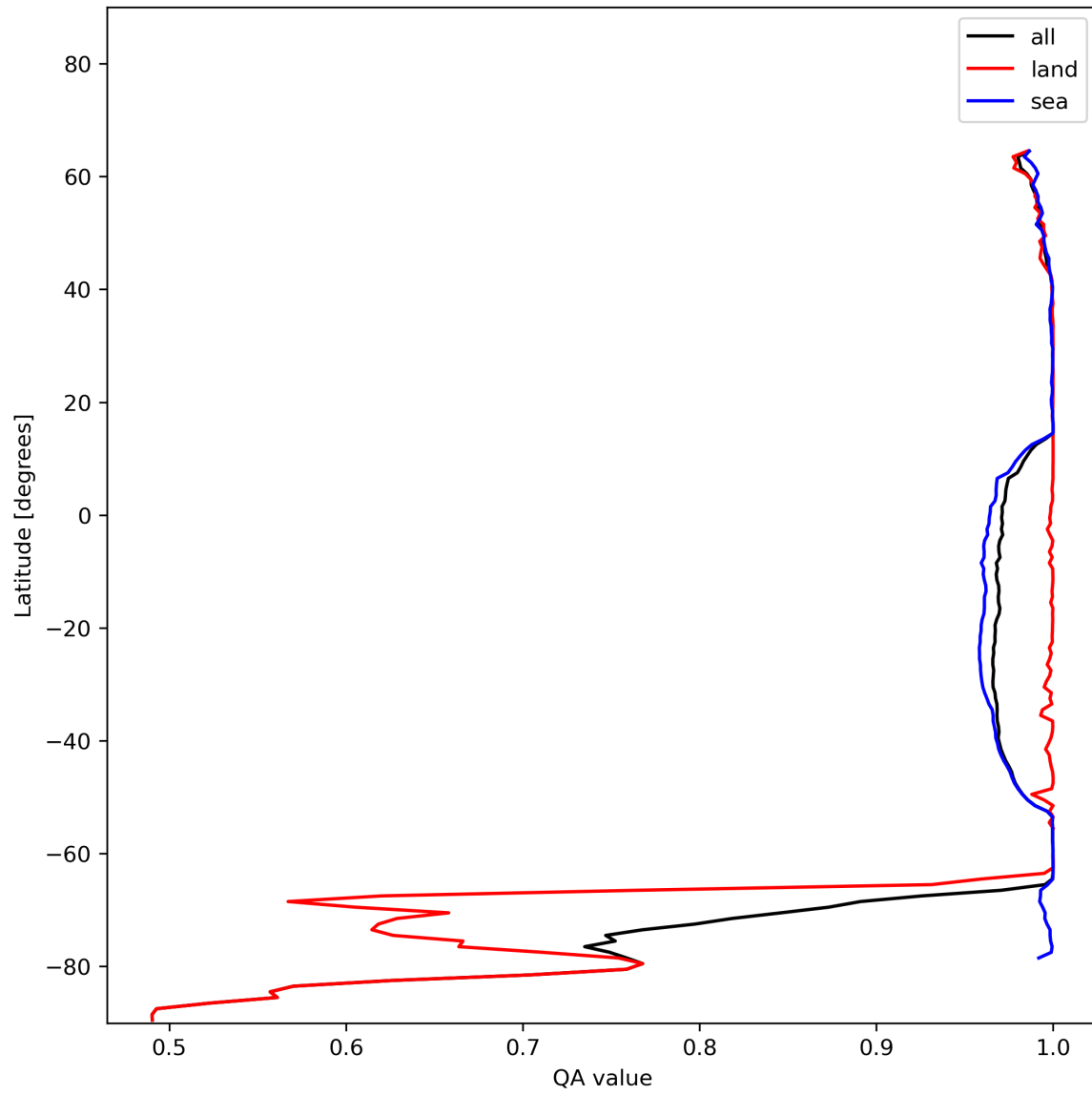
Figure 12: Zonal average of “QA value” for 2023-12-28 to 2023-12-30.
