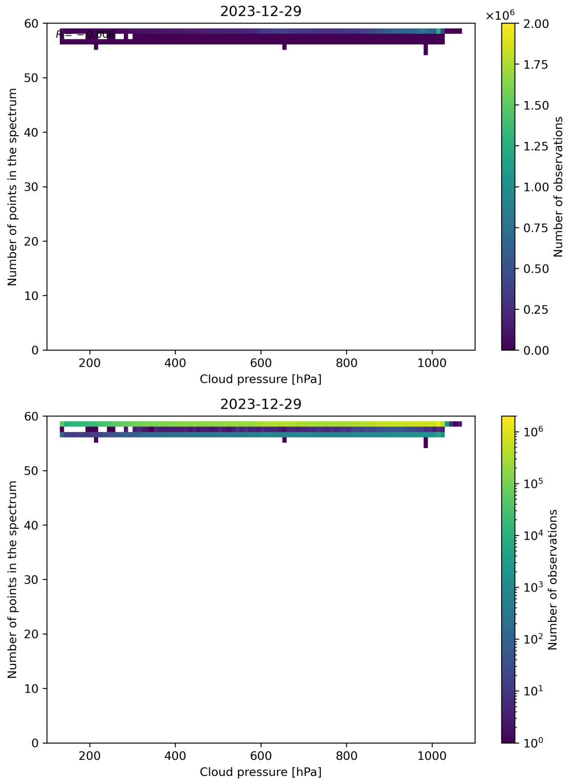
Figure 82: Scatter density plot of “Cloud pressure” against “Number of points in the spectrum” for 2023-12-28 to 2023-12-30.
