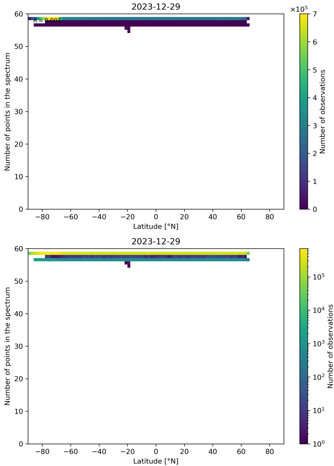
Figure 94: Scatter density plot of “Latitude” against “Number of points in the spectrum” for 2023-12-28 to 2023-12-30.
