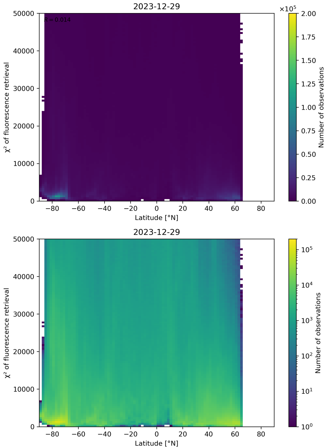
Figure 89: Scatter density plot of “Latitude” against “ \chi^2 of fluorescence retrieval” for 2023-12-28 to 2023-12-30.
