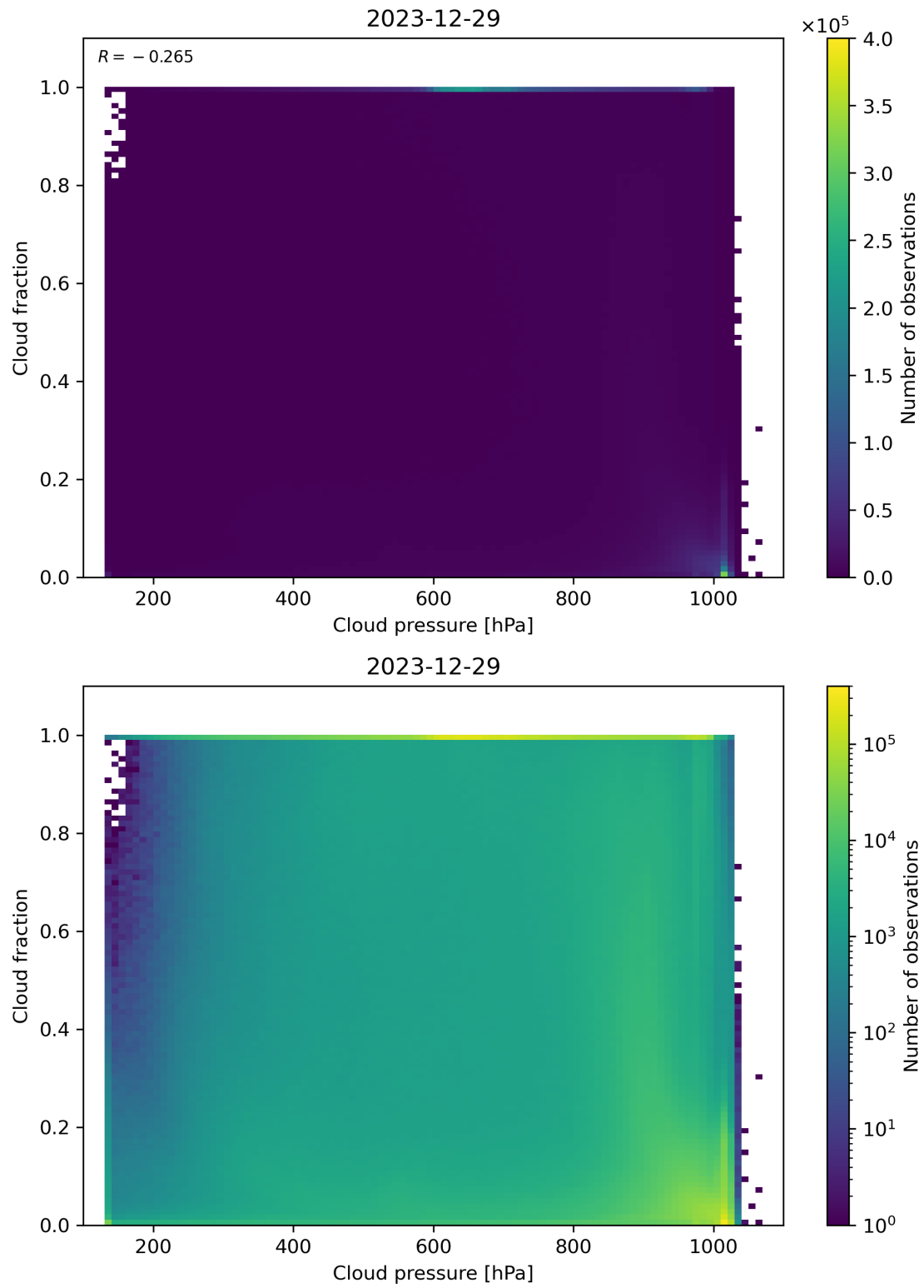
Figure 79: Scatter density plot of “Cloud pressure” against “Cloud fraction” for 2023-12-28 to 2023-12-30.
