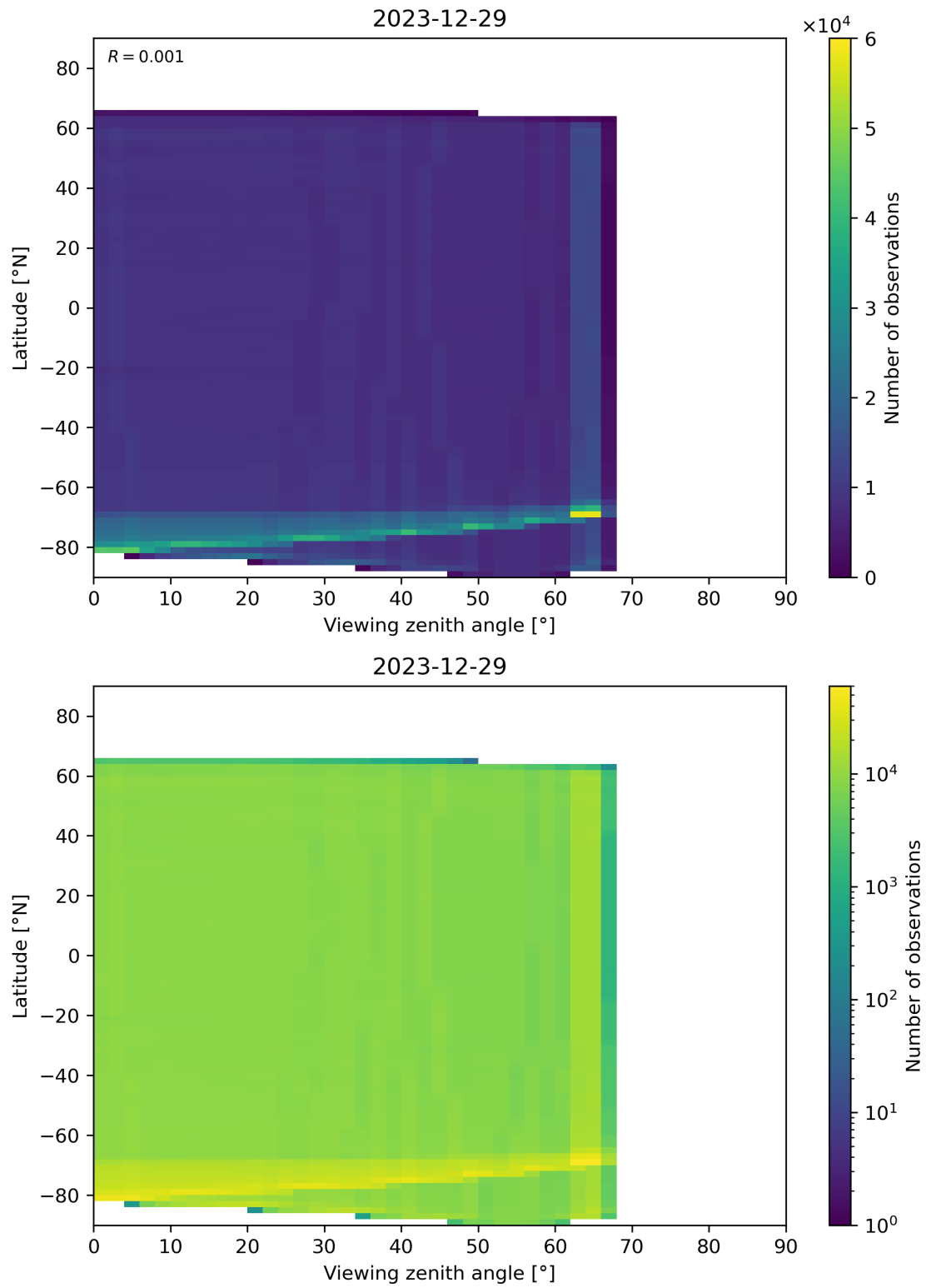
Figure 123: Scatter density plot of “Viewing zenith angle” against “Latitude” for 2023-12-28 to 2023-12-30.
