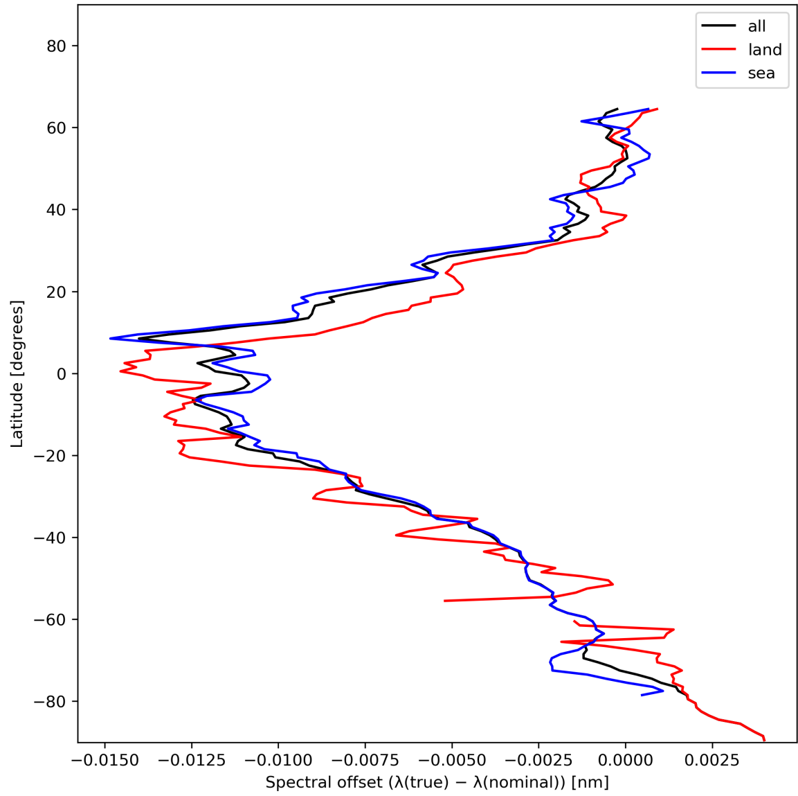
Figure 28: Zonal average of “Spectral offset ( \lambda(\text{true}) - \lambda(\text{nominal}) )” for 2023-12-28 to 2023-12-30.
