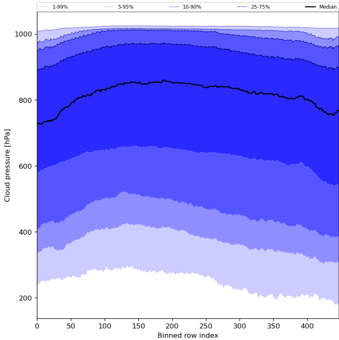
Figure 47: Along track statistics of “Cloud pressure” for 2023-12-28 to 2023-12-30
