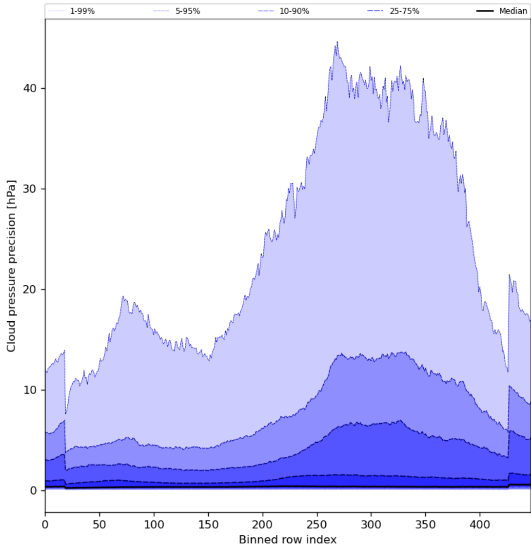
Figure 48: Along track statistics of “Cloud pressure precision” for 2023-12-28 to 2023-12-30
