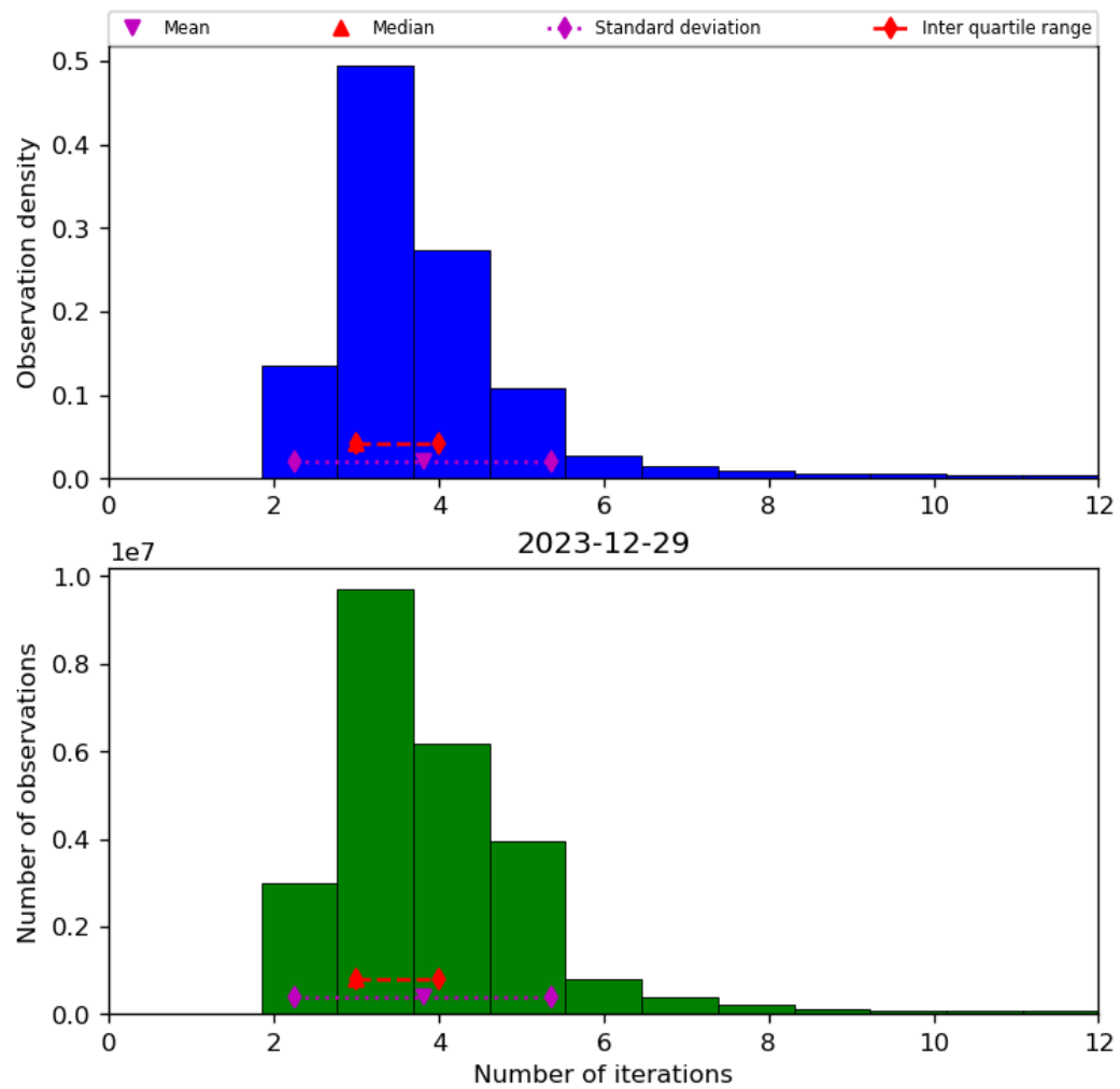
Figure 39: Histogram of “Number of iterations” for 2023-12-28 to 2023-12-30
