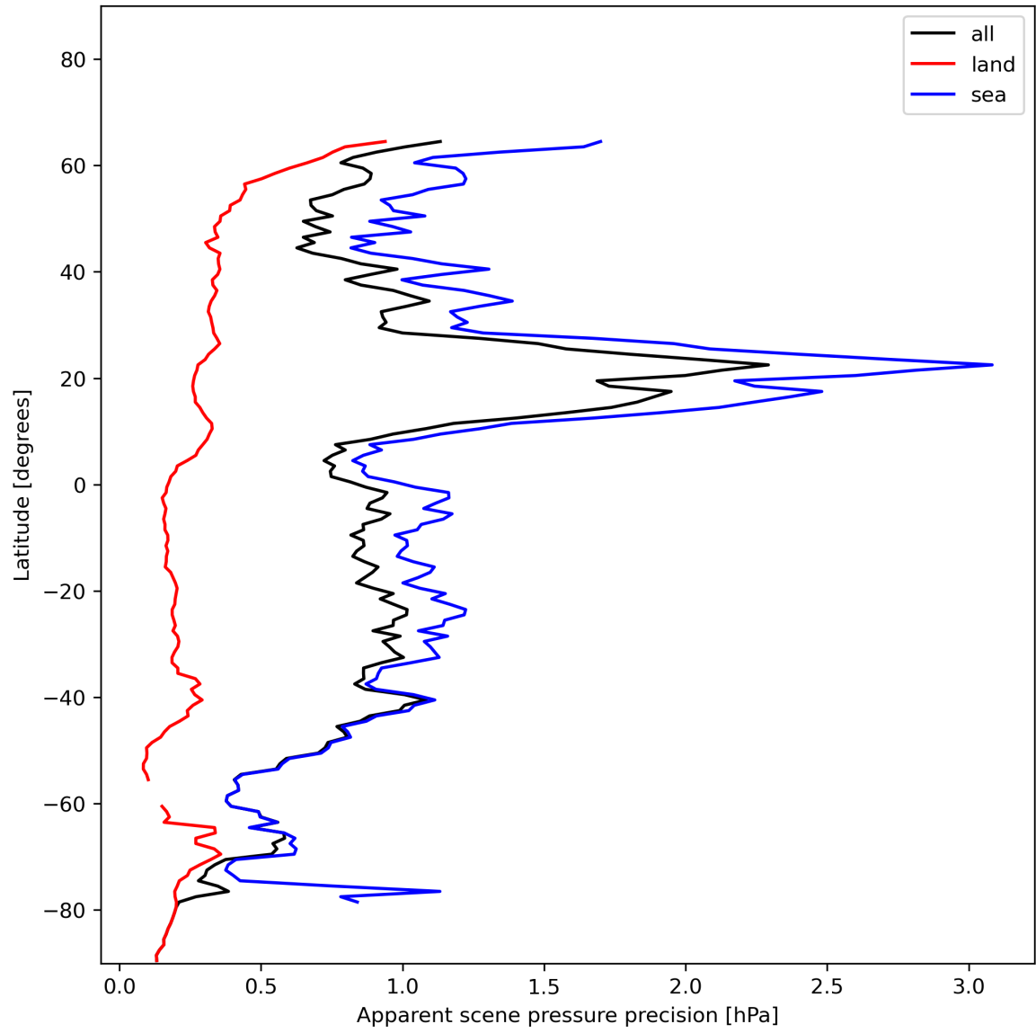
Figure 20: Zonal average of “Apparent scene pressure precision” for 2023-12-28 to 2023-12-30.
