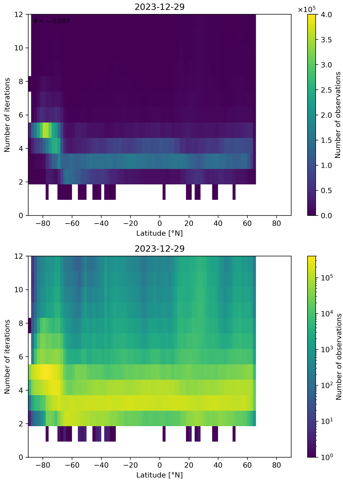
Figure 93: Scatter density plot of “Latitude” against “Number of iterations” for 2023-12-28 to 2023-12-30.
