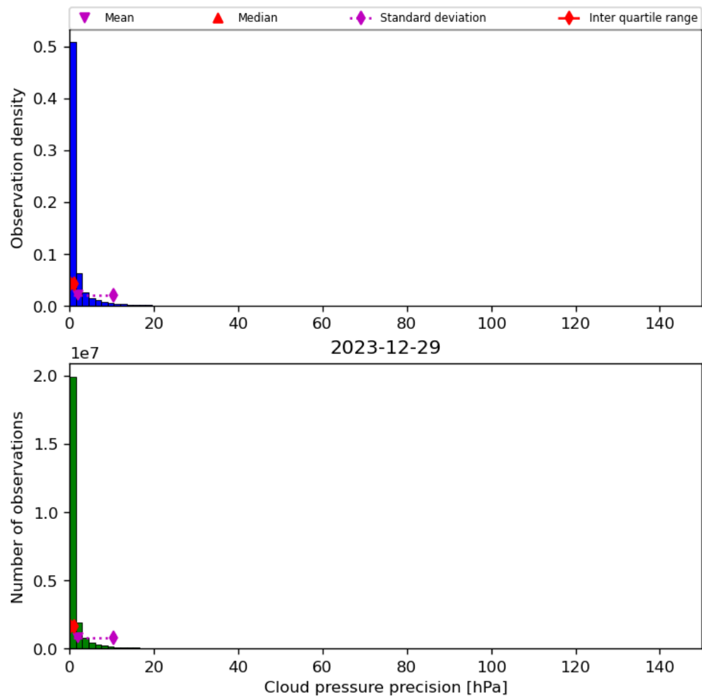
Figure 31: Histogram of “Cloud pressure precision” for 2023-12-28 to 2023-12-30
