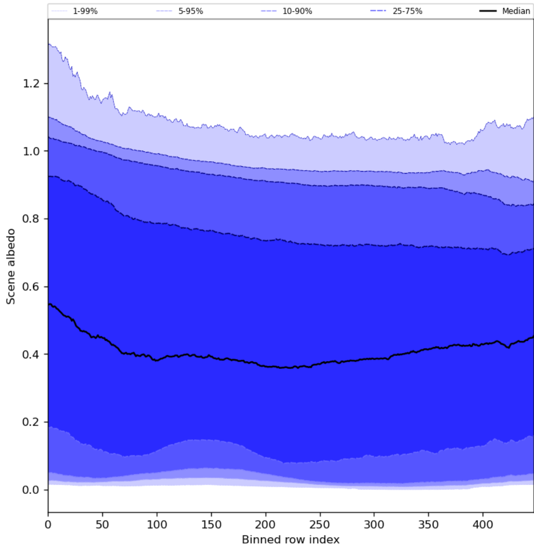
Figure 51: Along track statistics of "Scene albedo" for 2023-12-28 to 2023-12-30
