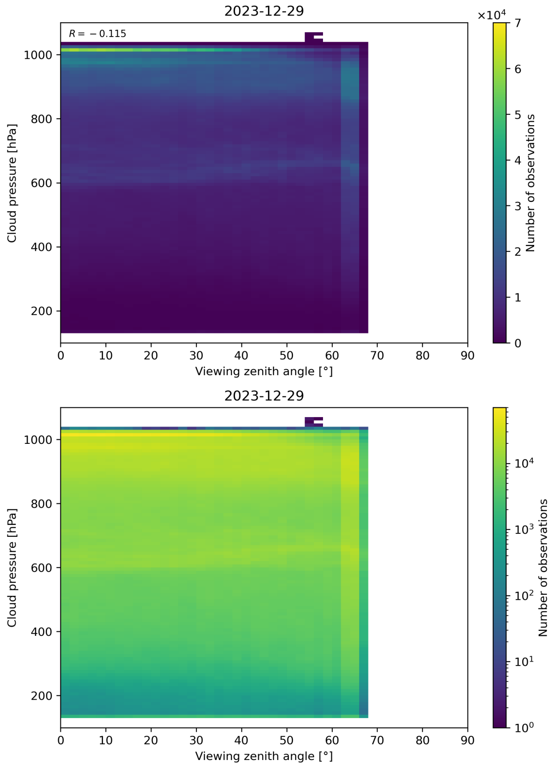
Figure 121: Scatter density plot of “Viewing zenith angle” against “Cloud pressure” for 2023-12-28 to 2023-12-30.
