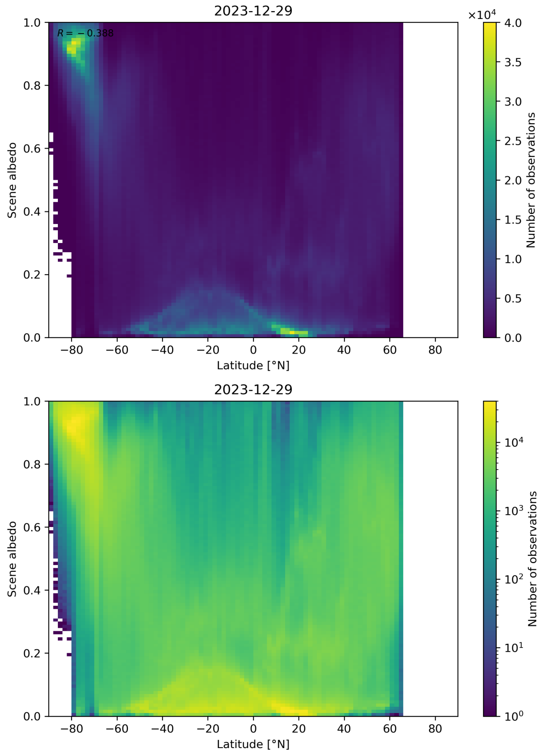
Figure 95: Scatter density plot of “Latitude” against “Scene albedo” for 2023-12-28 to 2023-12-30.
