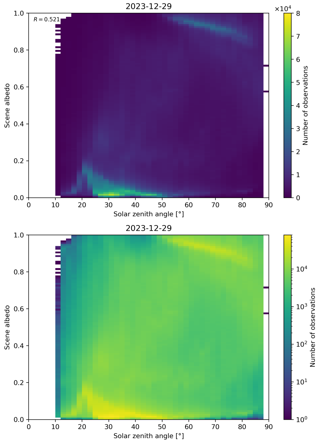
Figure 116: Scatter density plot of “Solar zenith angle” against “Scene albedo” for 2023-12-28 to 2023-12-30.
