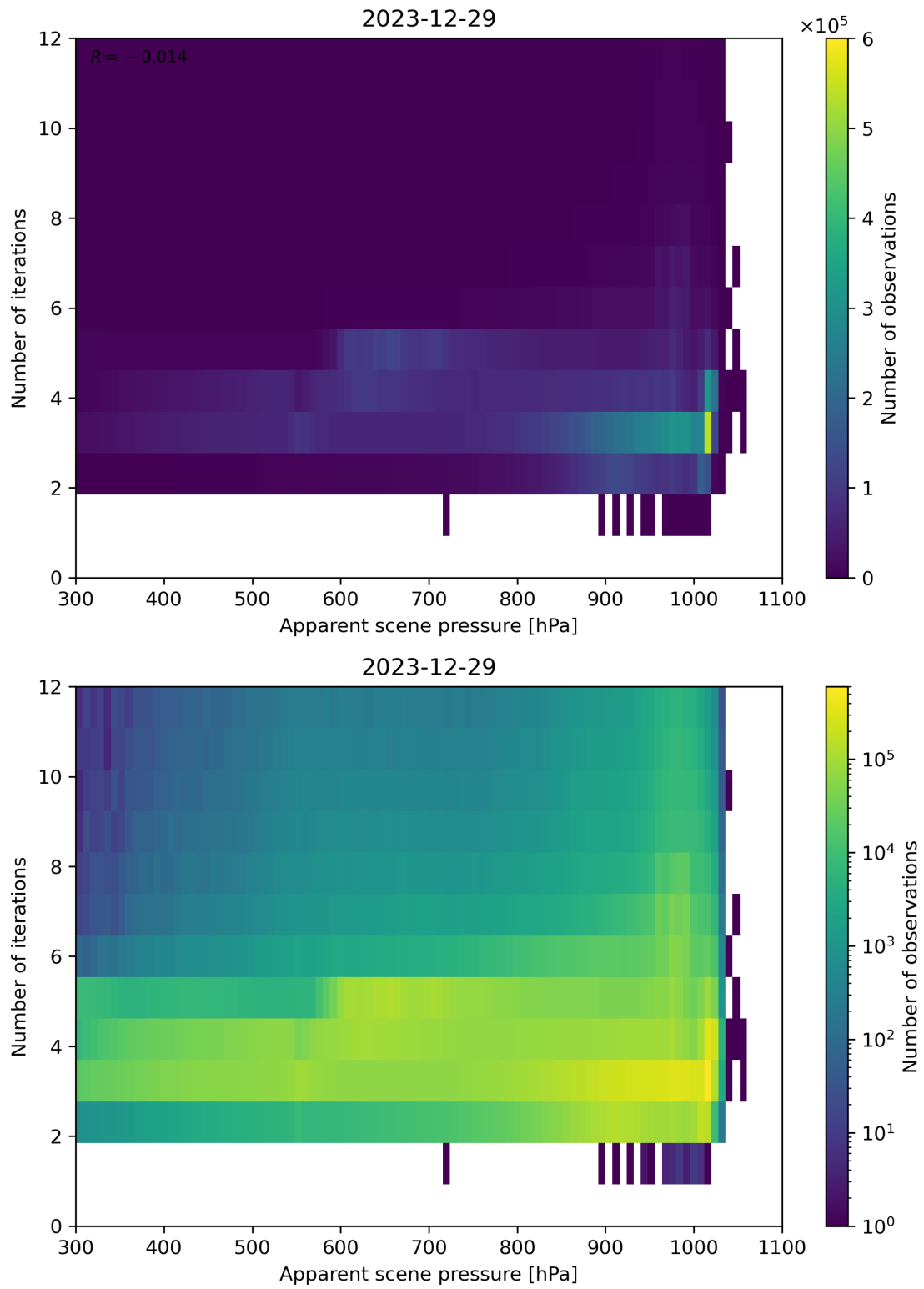
Figure 65: Scatter density plot of “Apparent scene pressure” against “Number of iterations” for 2023-12-28 to 2023-12-30.
