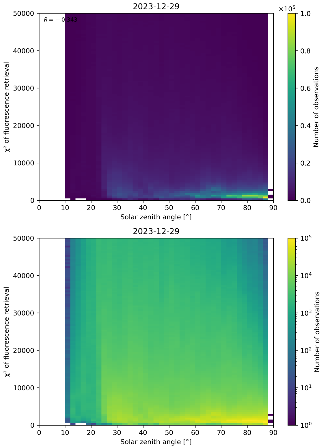
Figure 109: Scatter density plot of “Solar zenith angle” against “ \chi^2 of fluorescence retrieval” for 2023-12-28 to 2023-12-30.
