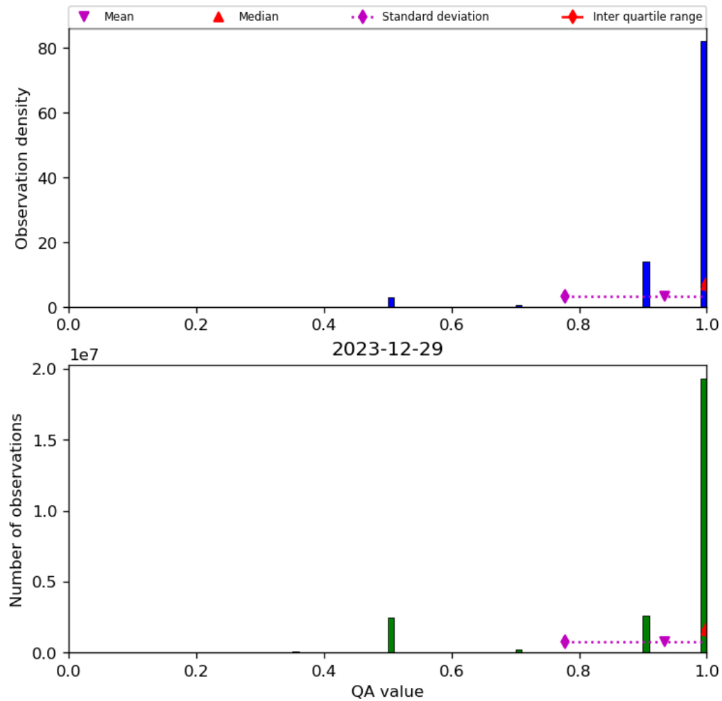
Figure 29: Histogram of “QA value” for 2023-12-28 to 2023-12-30
