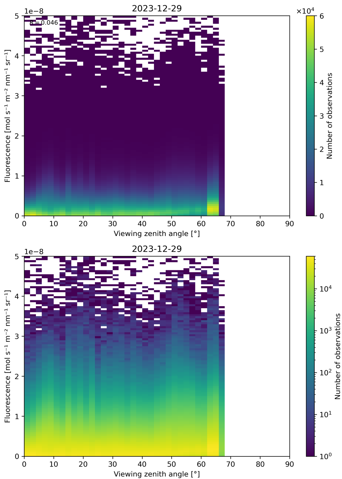
Figure 122: Scatter density plot of “Viewing zenith angle” against “Fluorescence” for 2023-12-28 to 2023-12-30.
