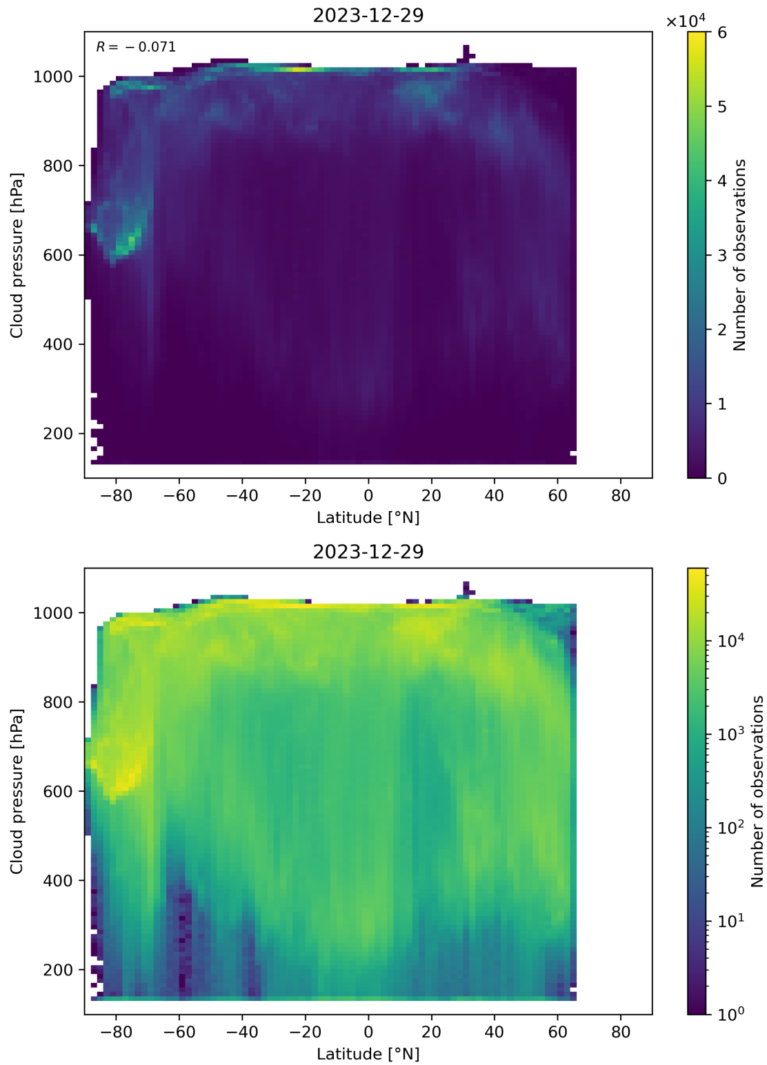
Figure 91: Scatter density plot of “Latitude” against “Cloud pressure” for 2023-12-28 to 2023-12-30.
