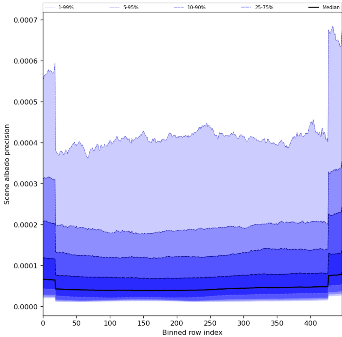
Figure 52: Along track statistics of “Scene albedo precision” for 2023-12-28 to 2023-12-30
