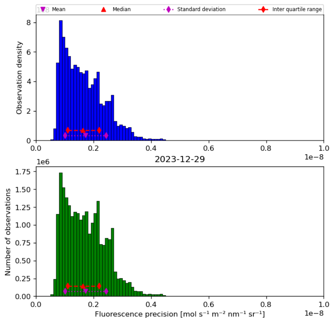
Figure 41: Histogram of “Fluorescence precision” for 2023-12-28 to 2023-12-30
