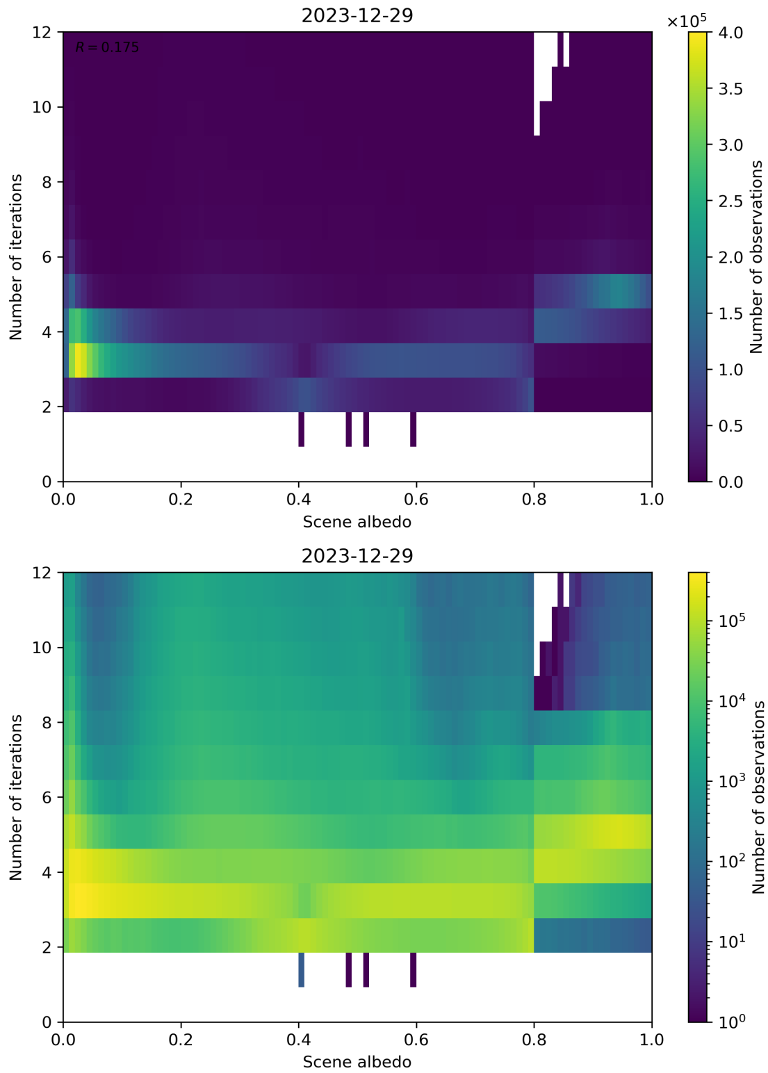
Figure 105: Scatter density plot of “Scene albedo” against “Number of iterations” for 2023-12-28 to 2023-12-30.
