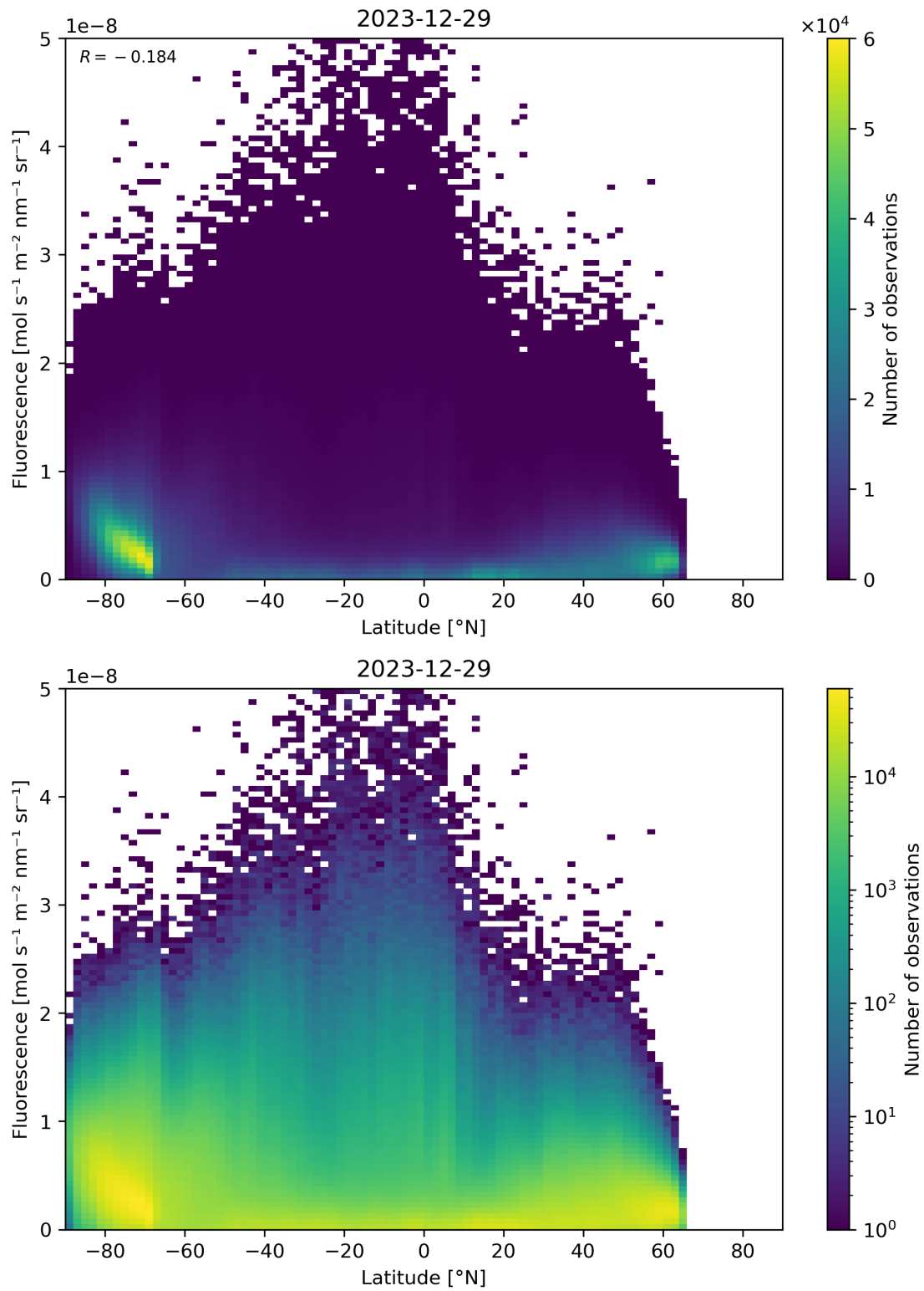
Figure 92: Scatter density plot of “Latitude” against “Fluorescence” for 2023-12-28 to 2023-12-30.
