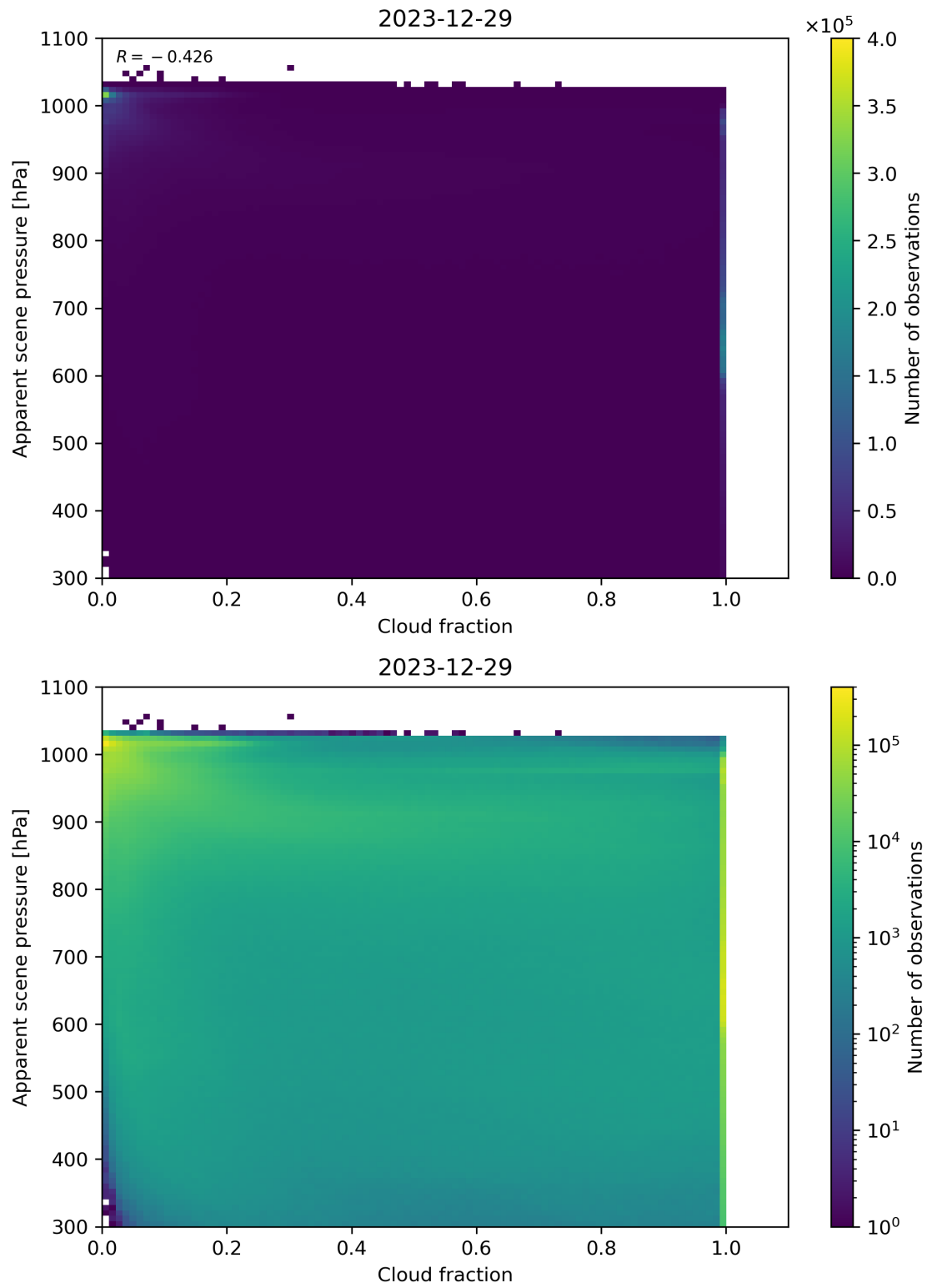
Figure 70: Scatter density plot of “Cloud fraction” against “Apparent scene pressure” for 2023-12-28 to 2023-12-30.
