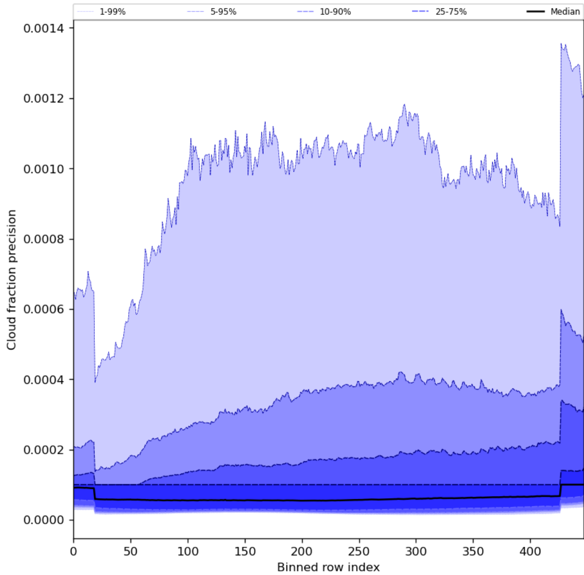
Figure 50: Along track statistics of “Cloud fraction precision” for 2023-12-28 to 2023-12-30
