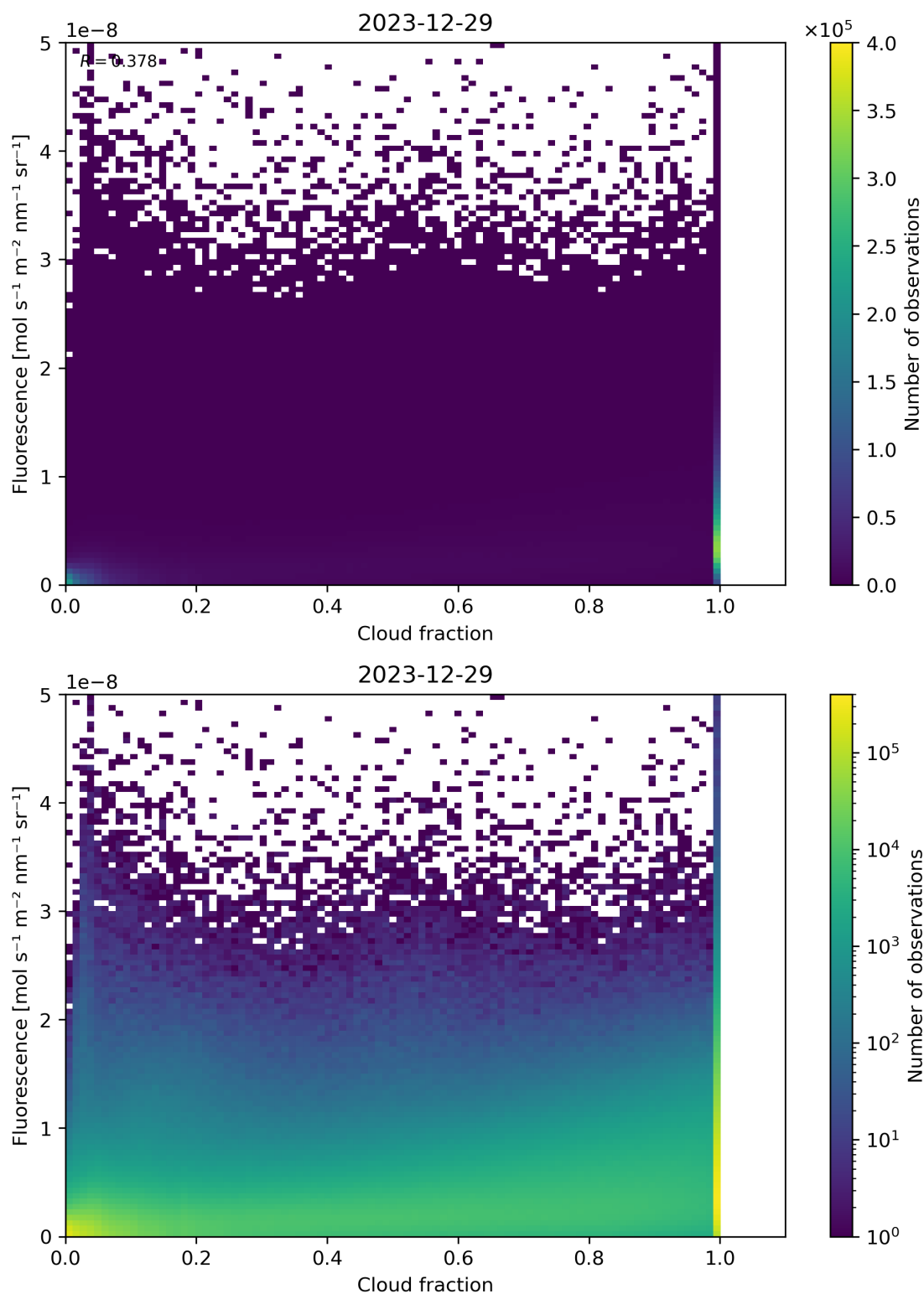
Figure 72: Scatter density plot of “Cloud fraction” against “Fluorescence” for 2023-12-28 to 2023-12-30.
