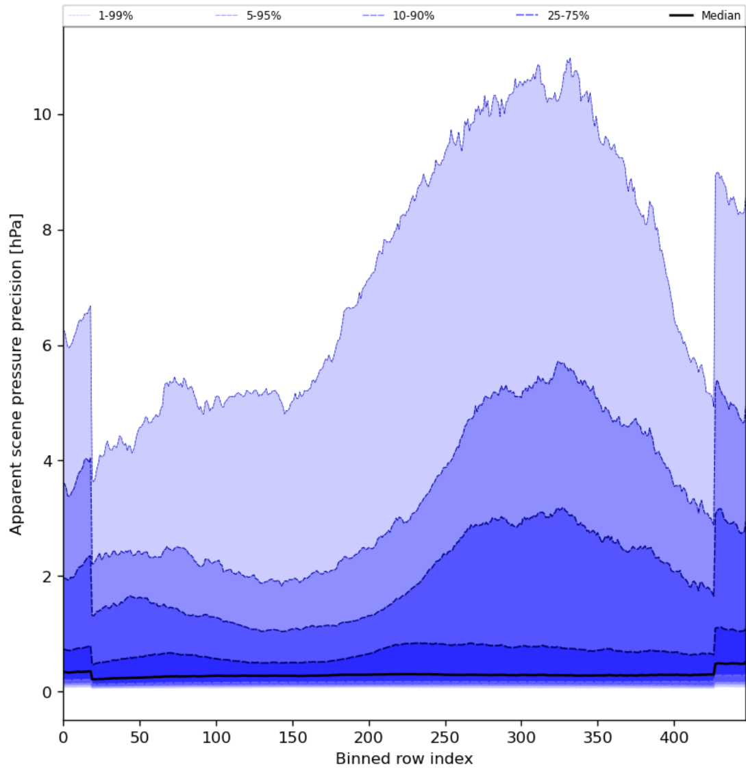
Figure 54: Along track statistics of “Apparent scene pressure precision” for 2023-12-28 to 2023-12-30
