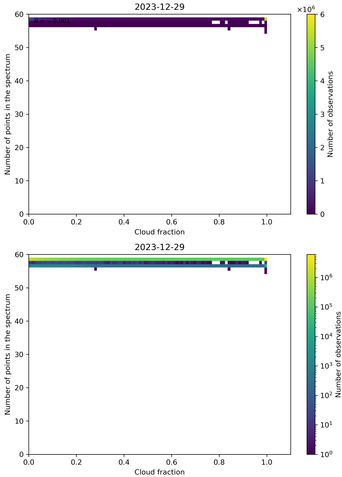
Figure 74: Scatter density plot of “Cloud fraction” against “Number of points in the spectrum” for 2023-12-28 to 2023-12-30.
