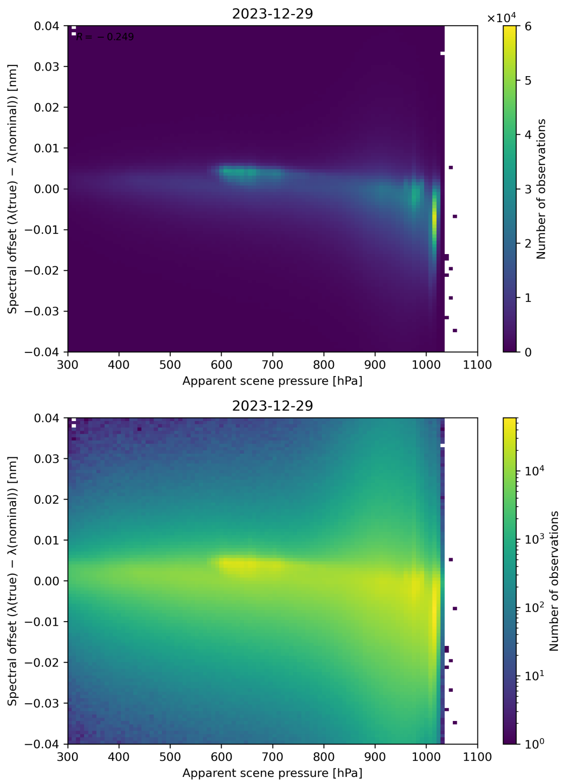
Figure 67: Scatter density plot of “Apparent scene pressure” against “Spectral offset ( \lambda(\text{true}) - \lambda(\text{nominal}) )” for 2023-12-28 to 2023-12-30.
