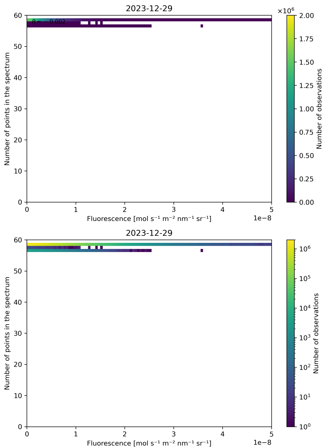
Figure 86: Scatter density plot of “Fluorescence” against “Number of points in the spectrum” for 2023-12-28 to 2023-12-30.
