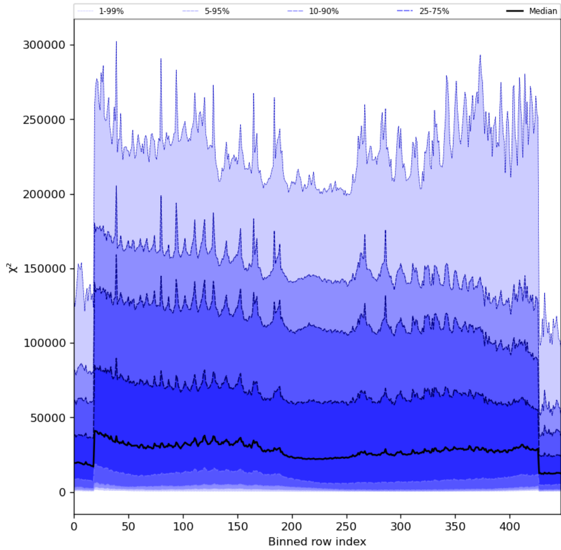
Figure 55: Along track statistics of “ \chi^2 ” for 2023-12-28 to 2023-12-30
