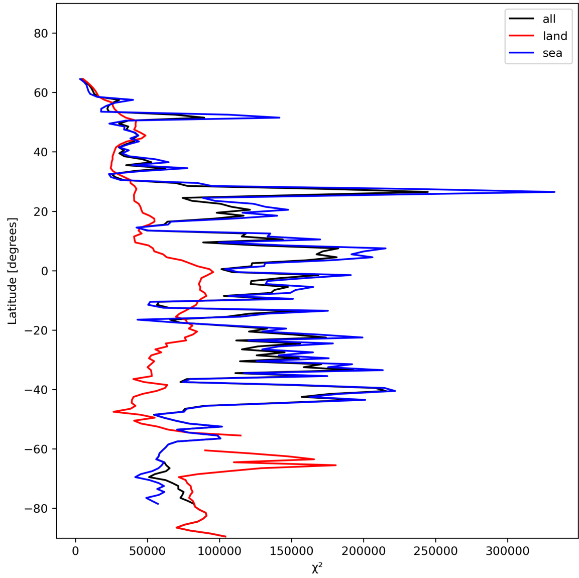
Figure 21: Zonal average of “ \chi^2 ” for 2023-12-28 to 2023-12-30.
