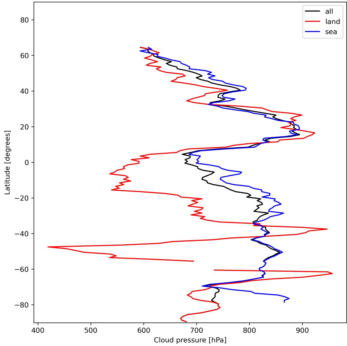
Figure 13: Zonal average of “Cloud pressure” for 2023-12-28 to 2023-12-30.
