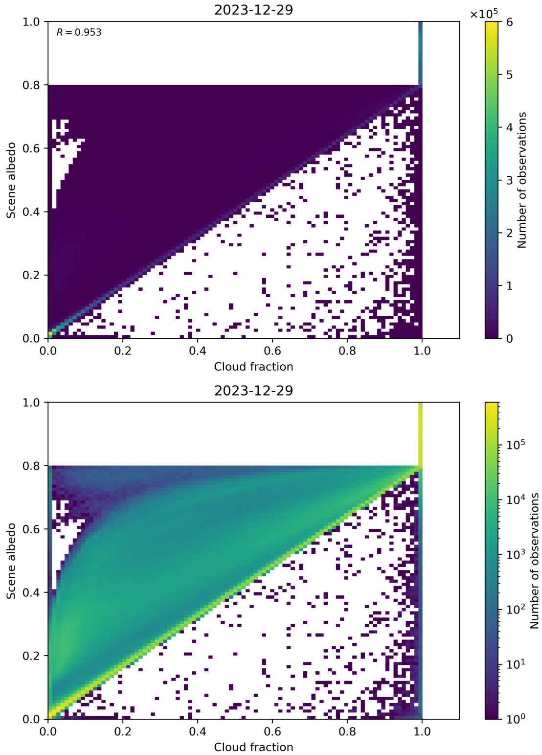
Figure 75: Scatter density plot of “Cloud fraction” against “Scene albedo” for 2023-12-28 to 2023-12-30.
