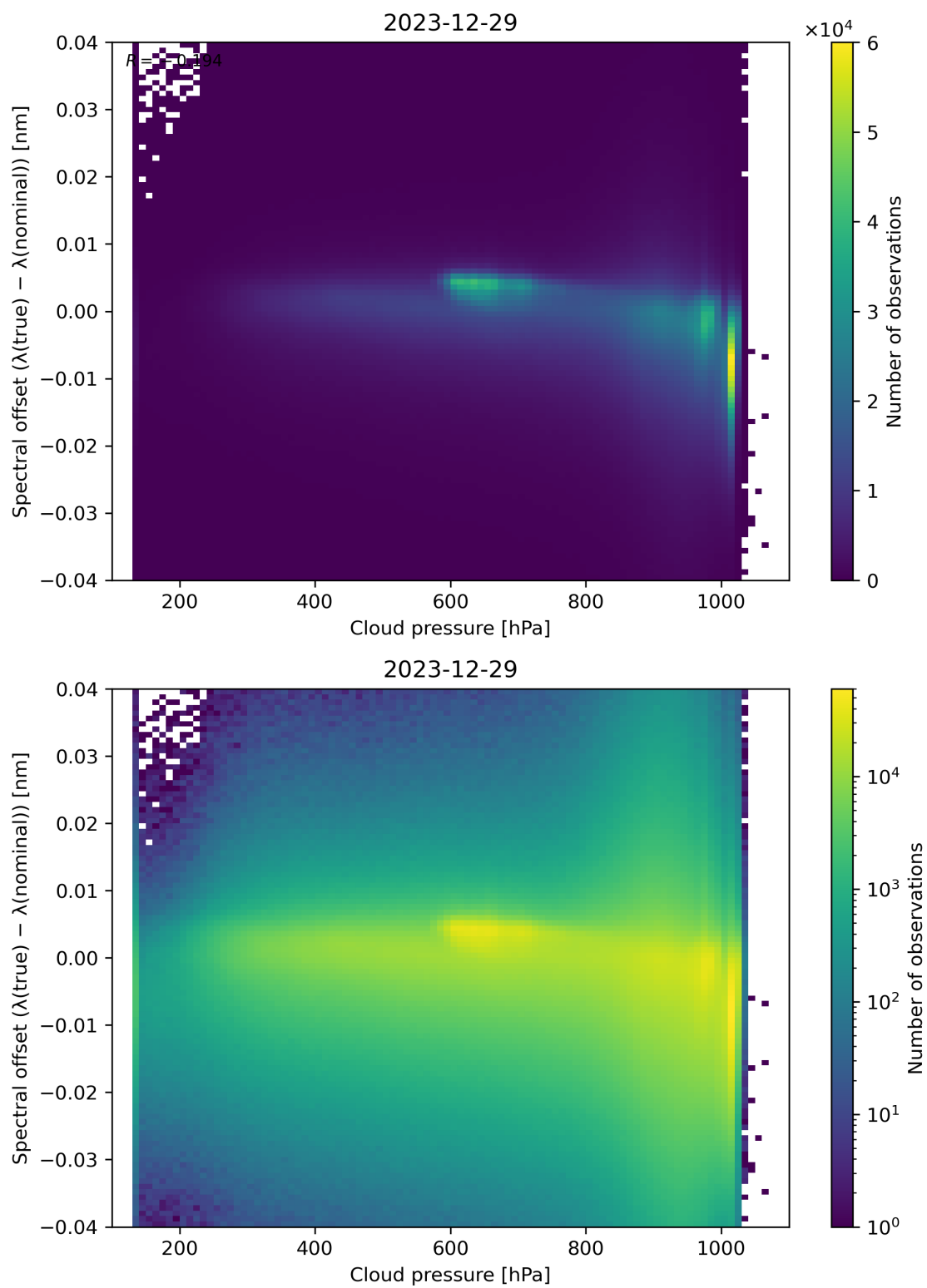
Figure 84: Scatter density plot of “Cloud pressure” against “Spectral offset ( \lambda(\text{true}) - \lambda(\text{nominal}) )” for 2023-12-28 to 2023-12-30.
