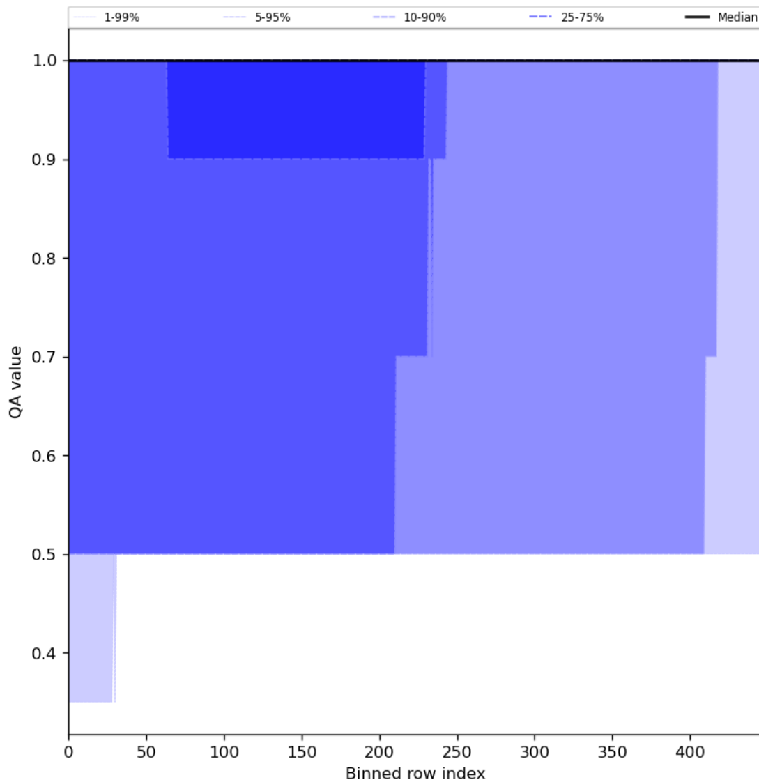
Figure 46: Along track statistics of “QA value” for 2023-12-28 to 2023-12-30
