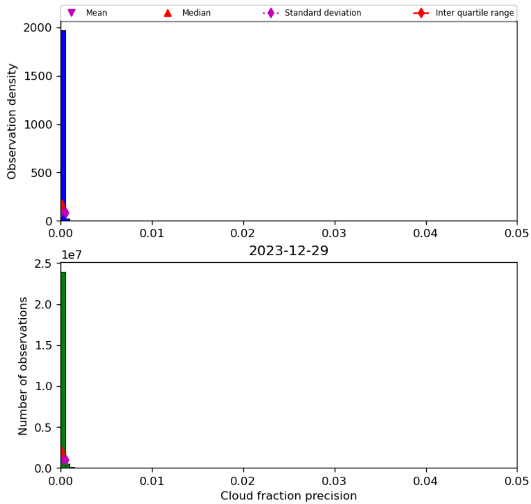
Figure 33: Histogram of “Cloud fraction precision” for 2023-12-28 to 2023-12-30
