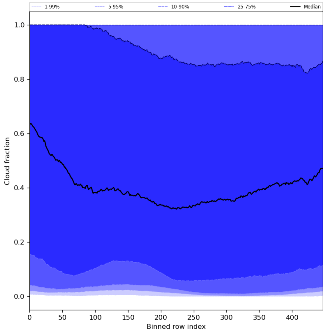
Figure 49: Along track statistics of “Cloud fraction” for 2023-12-28 to 2023-12-30
