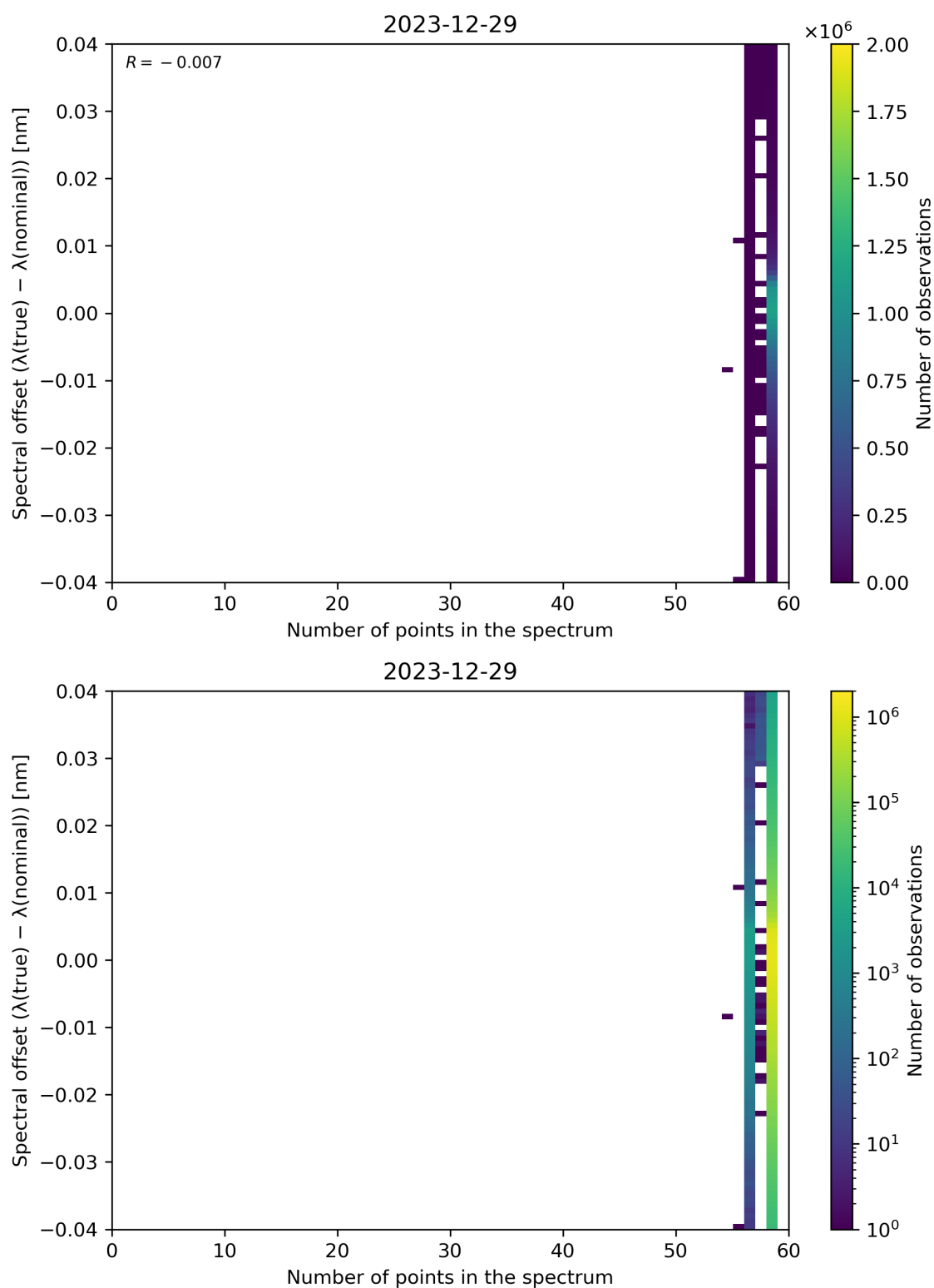
Figure 101: Scatter density plot of “Number of points in the spectrum” against “Spectral offset ( \lambda(\text{true}) - \lambda(\text{nominal}) )” for 2023-12-28 to 2023-12-30.
