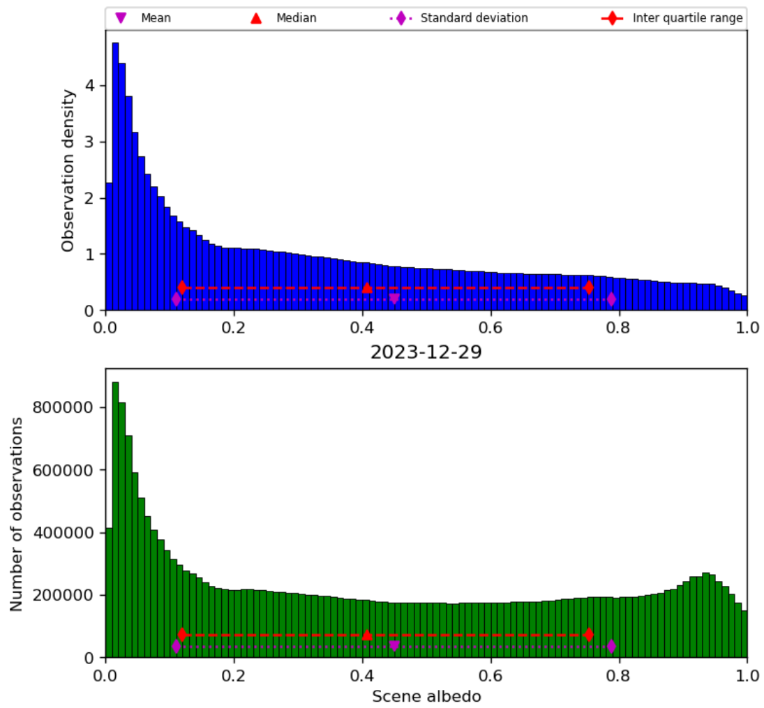
Figure 34: Histogram of “Scene albedo” for 2023-12-28 to 2023-12-30
