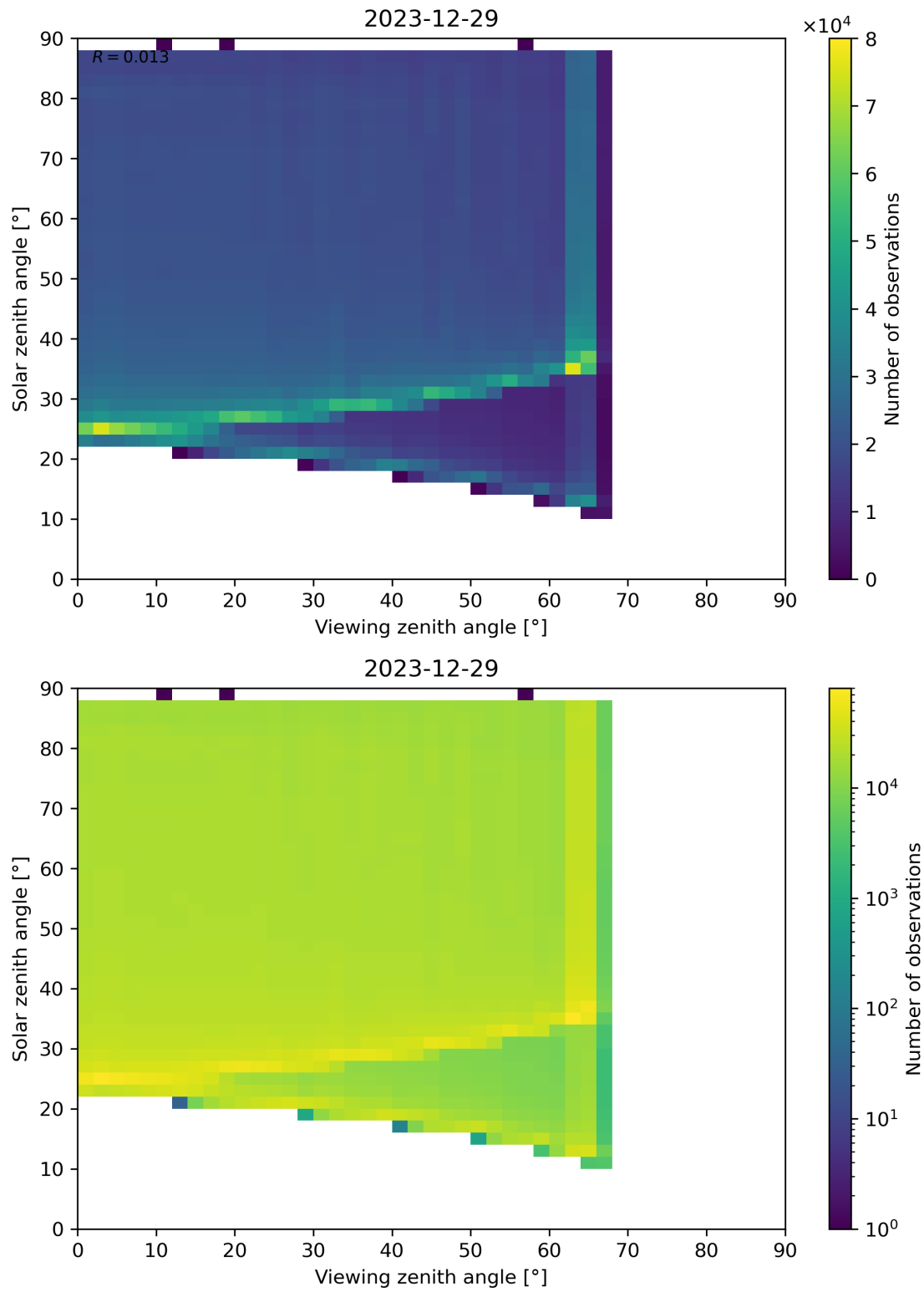
Figure 127: Scatter density plot of “Viewing zenith angle” against “Solar zenith angle” for 2023-12-28 to 2023-12-30.
