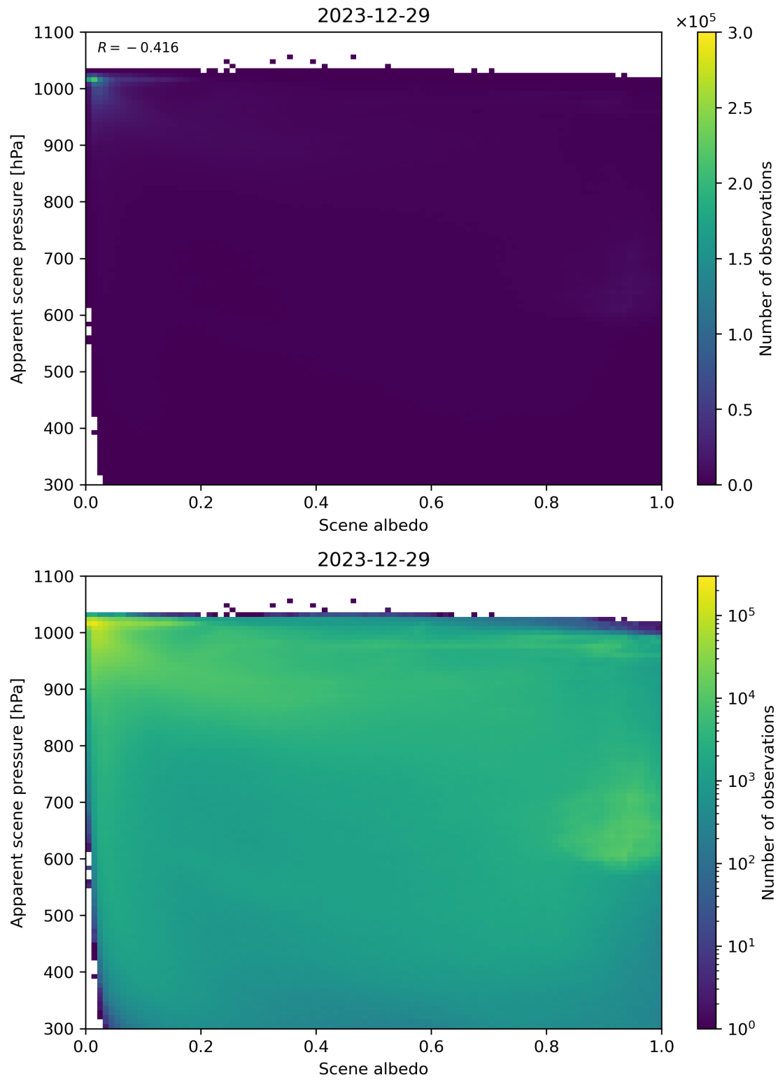
Figure 102: Scatter density plot of “Scene albedo” against “Apparent scene pressure” for 2023-12-28 to 2023-12-30.
