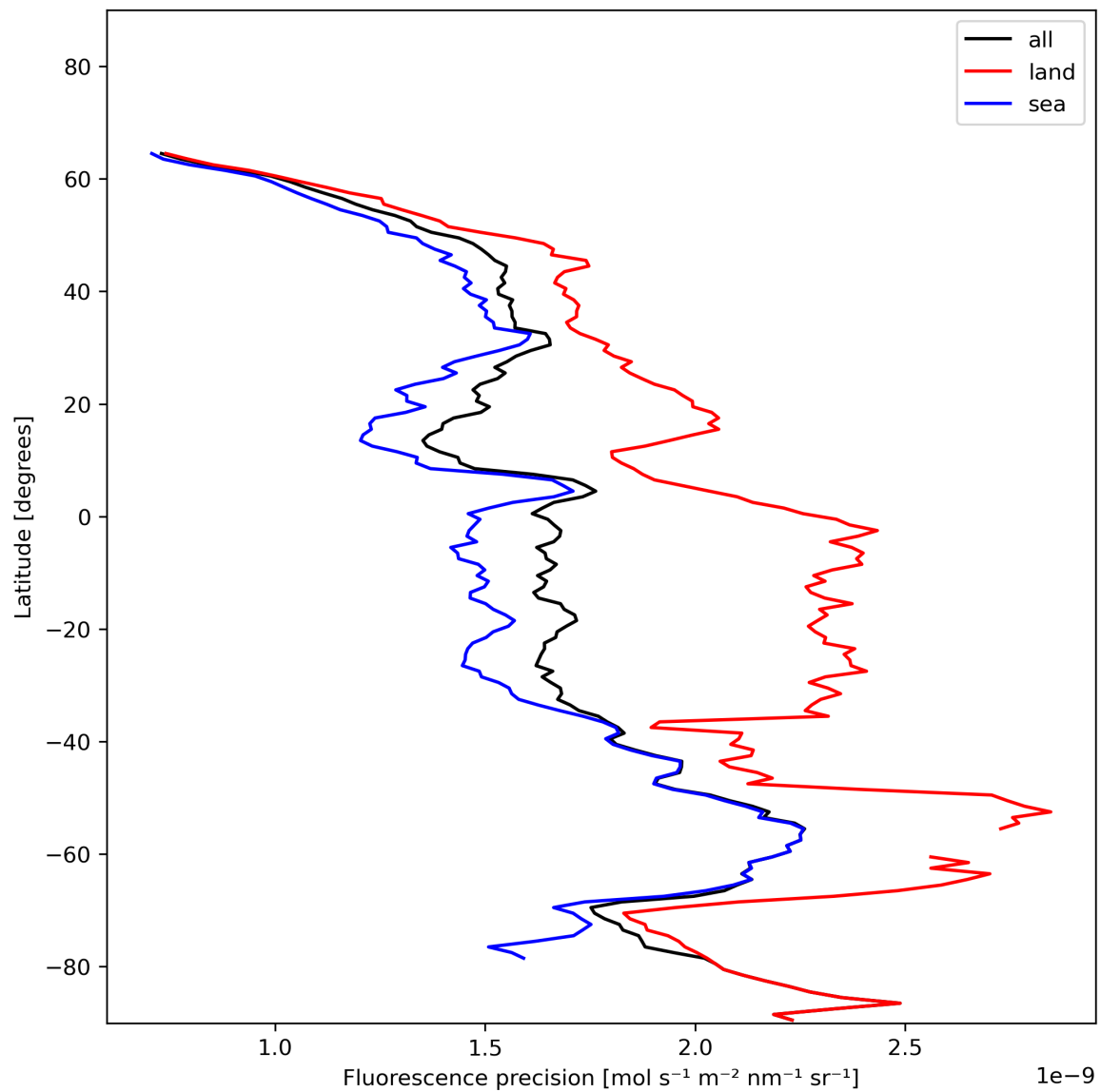
Figure 24: Zonal average of “Fluorescence precision” for 2023-12-28 to 2023-12-30.
