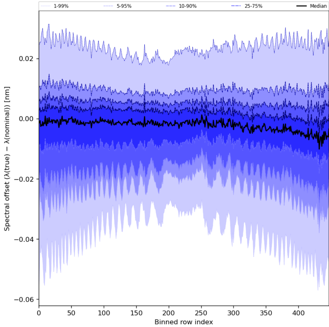
Figure 62: Along track statistics of “Spectral offset ( \lambda(\text{true}) - \lambda(\text{nominal}) )” for 2023-12-28 to 2023-12-30
