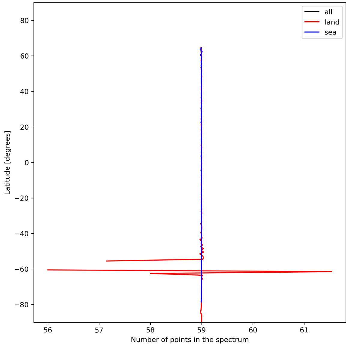
Figure 27: Zonal average of “Number of points in the spectrum” for 2023-12-28 to 2023-12-30.
