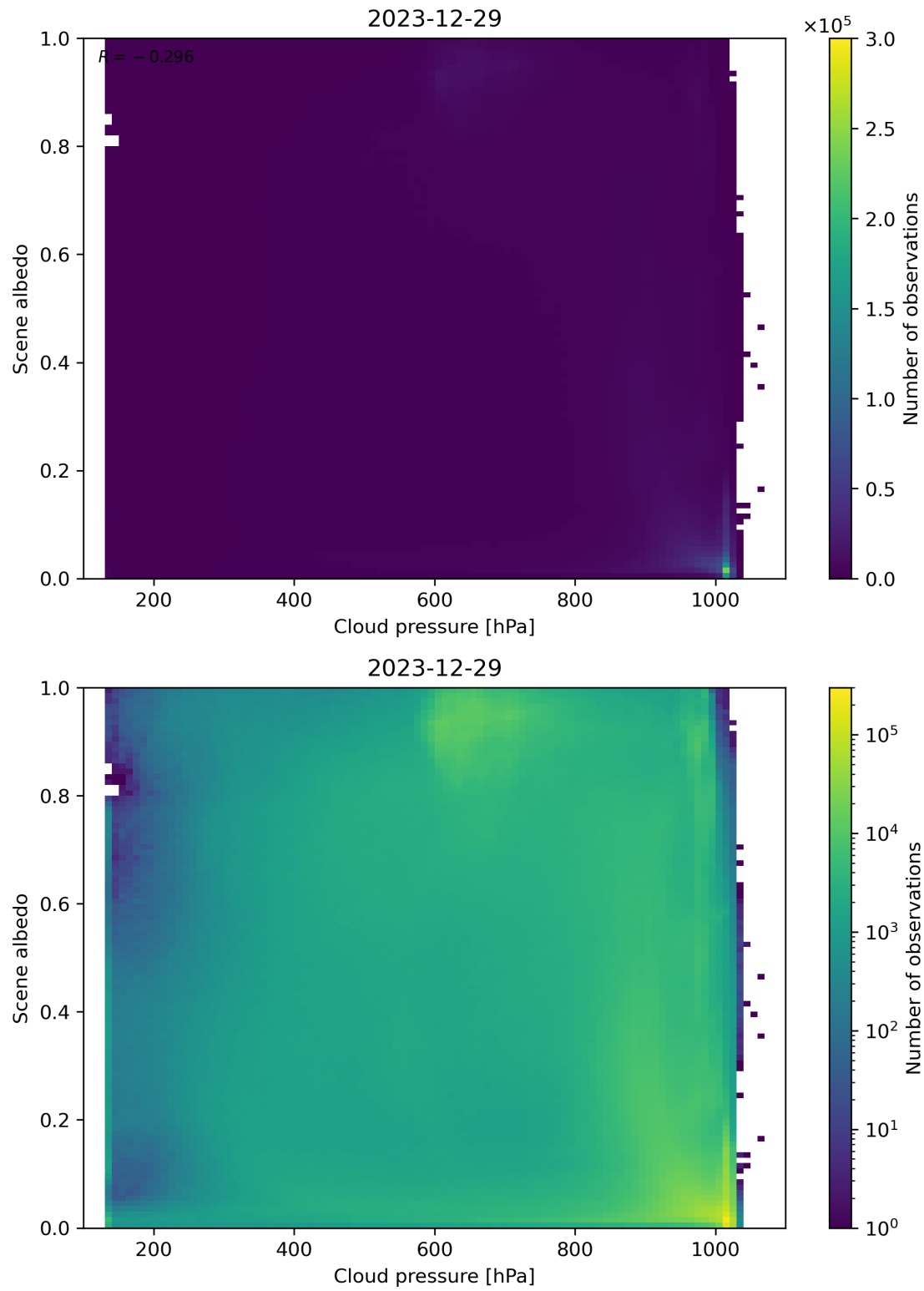
Figure 83: Scatter density plot of “Cloud pressure” against “Scene albedo” for 2023-12-28 to 2023-12-30.
