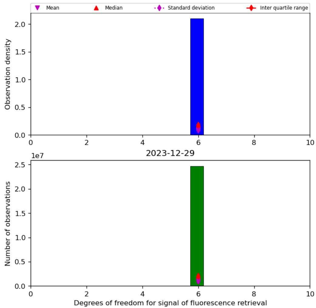
Figure 43: Histogram of “Degrees of freedom for signal of fluorescence retrieval” for 2023-12-28 to 2023-12-30
