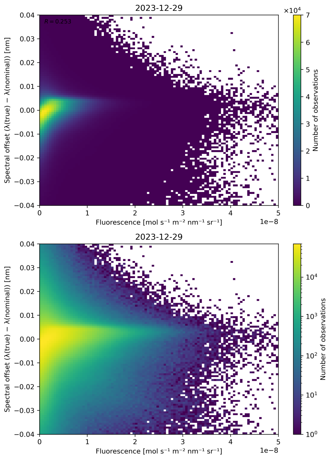
Figure 87: Scatter density plot of “Fluorescence” against “Spectral offset ( \lambda(\text{true}) - \lambda(\text{nominal}) )” for 2023-12-28 to 2023-12-30.
