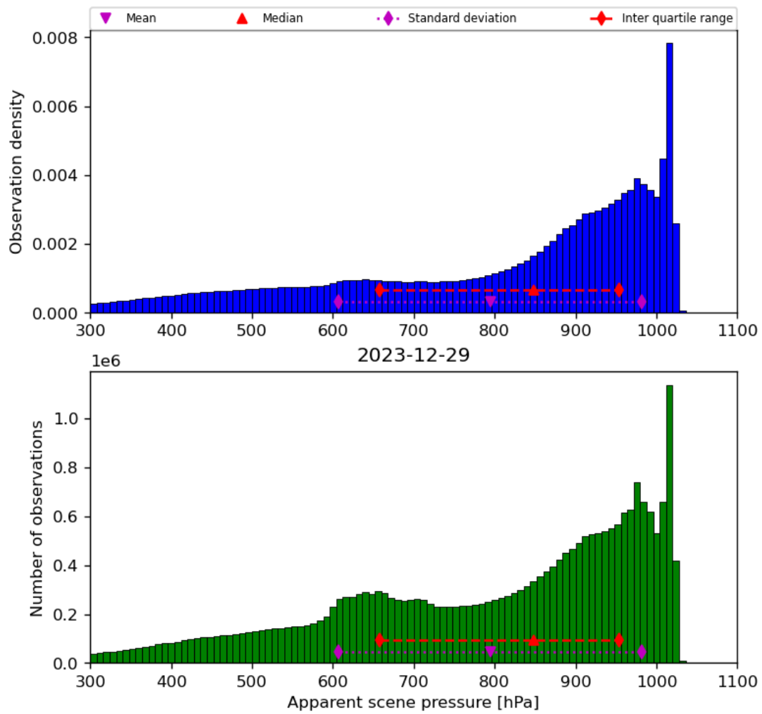
Figure 36: Histogram of “Apparent scene pressure” for 2023-12-28 to 2023-12-30
