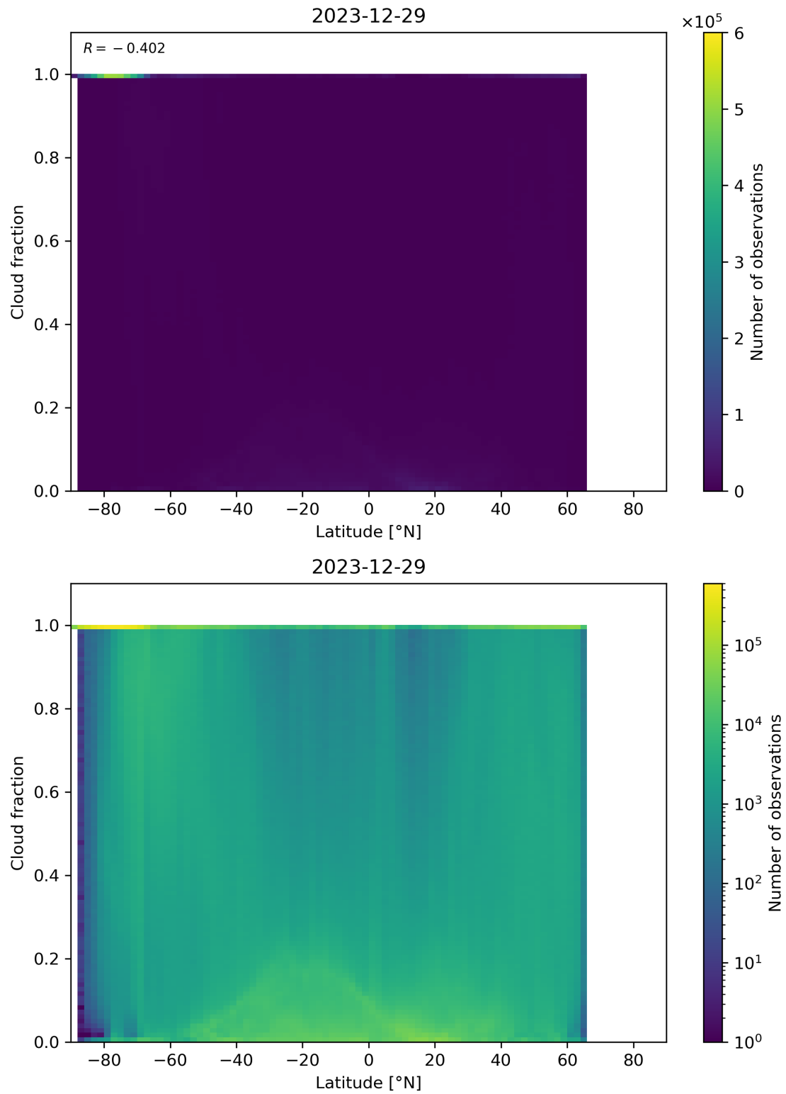
Figure 90: Scatter density plot of “Latitude” against “Cloud fraction” for 2023-12-28 to 2023-12-30.
