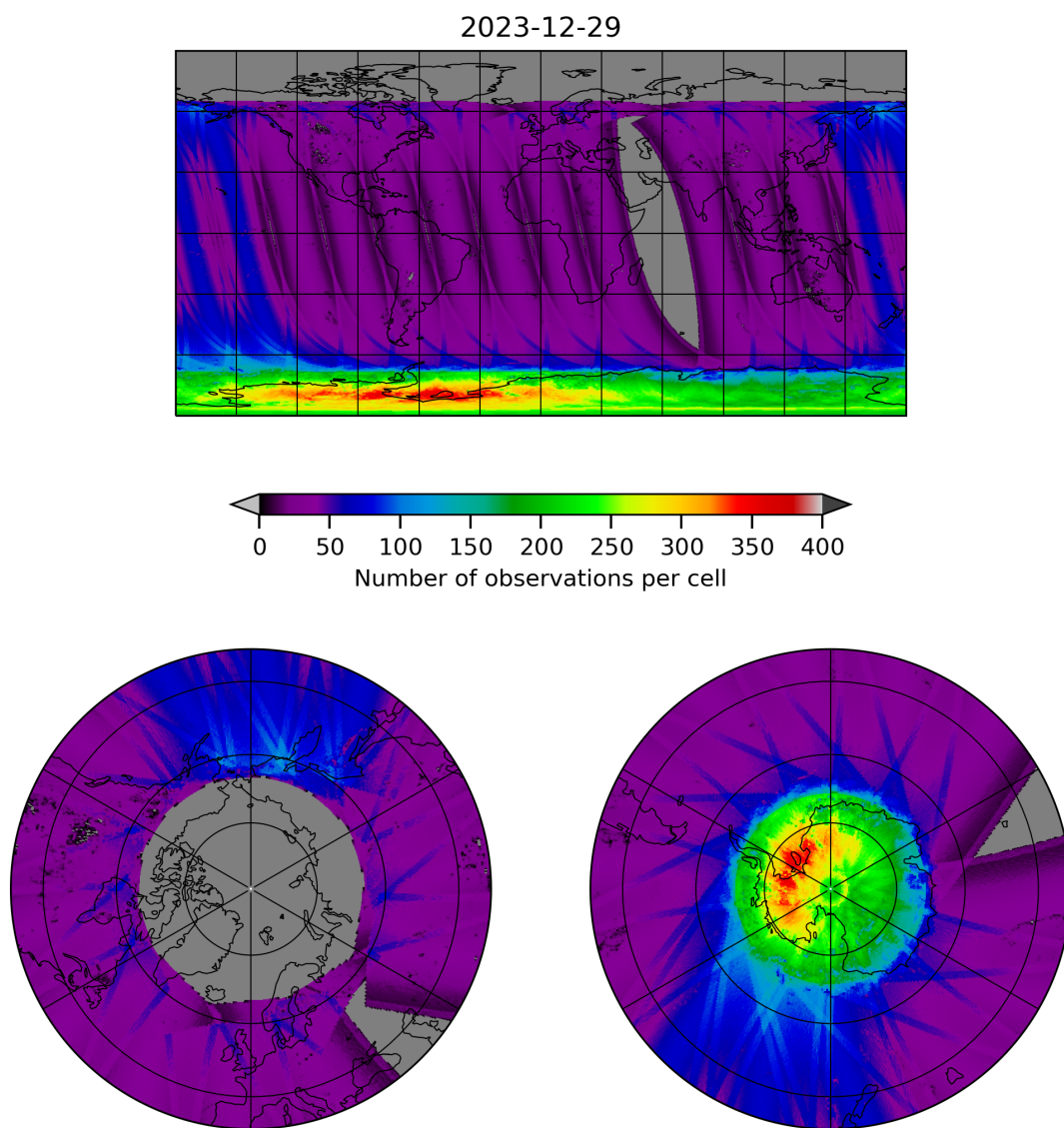
Figure 11: Map of the number of observations for 2023-12-28 to 2023-12-30
