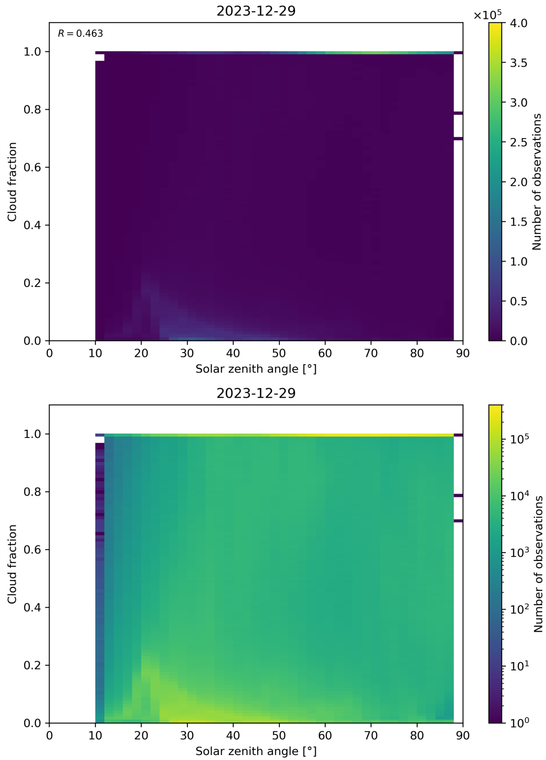
Figure 110: Scatter density plot of “Solar zenith angle” against “Cloud fraction” for 2023-12-28 to 2023-12-30.
