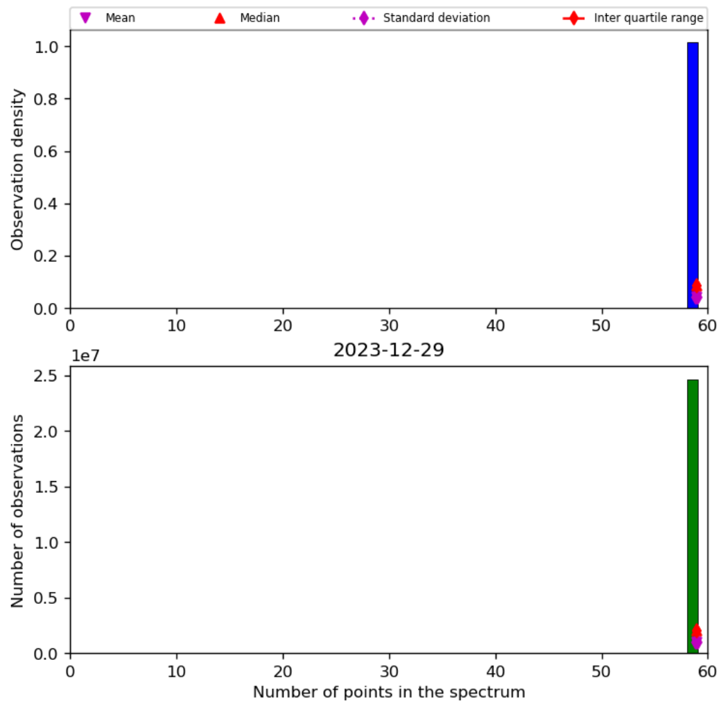
Figure 44: Histogram of "Number of points in the spectrum" for 2023-12-28 to 2023-12-30
