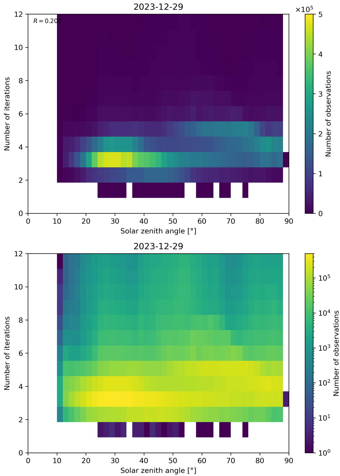
Figure 114: Scatter density plot of “Solar zenith angle” against “Number of iterations” for 2023-12-28 to 2023-12-30.
