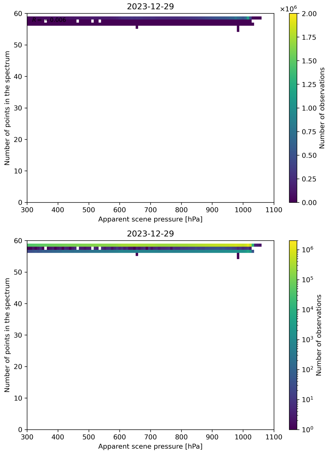
Figure 66: Scatter density plot of “Apparent scene pressure” against “Number of points in the spectrum” for 2023-12-28 to 2023-12-30.
