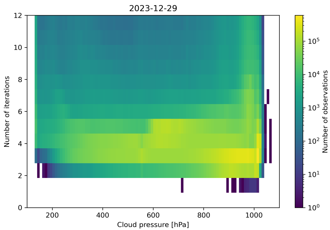
Figure 81: Scatter density plot of “Cloud pressure” against “Number of iterations” for 2023-12-28 to 2023-12-30.
