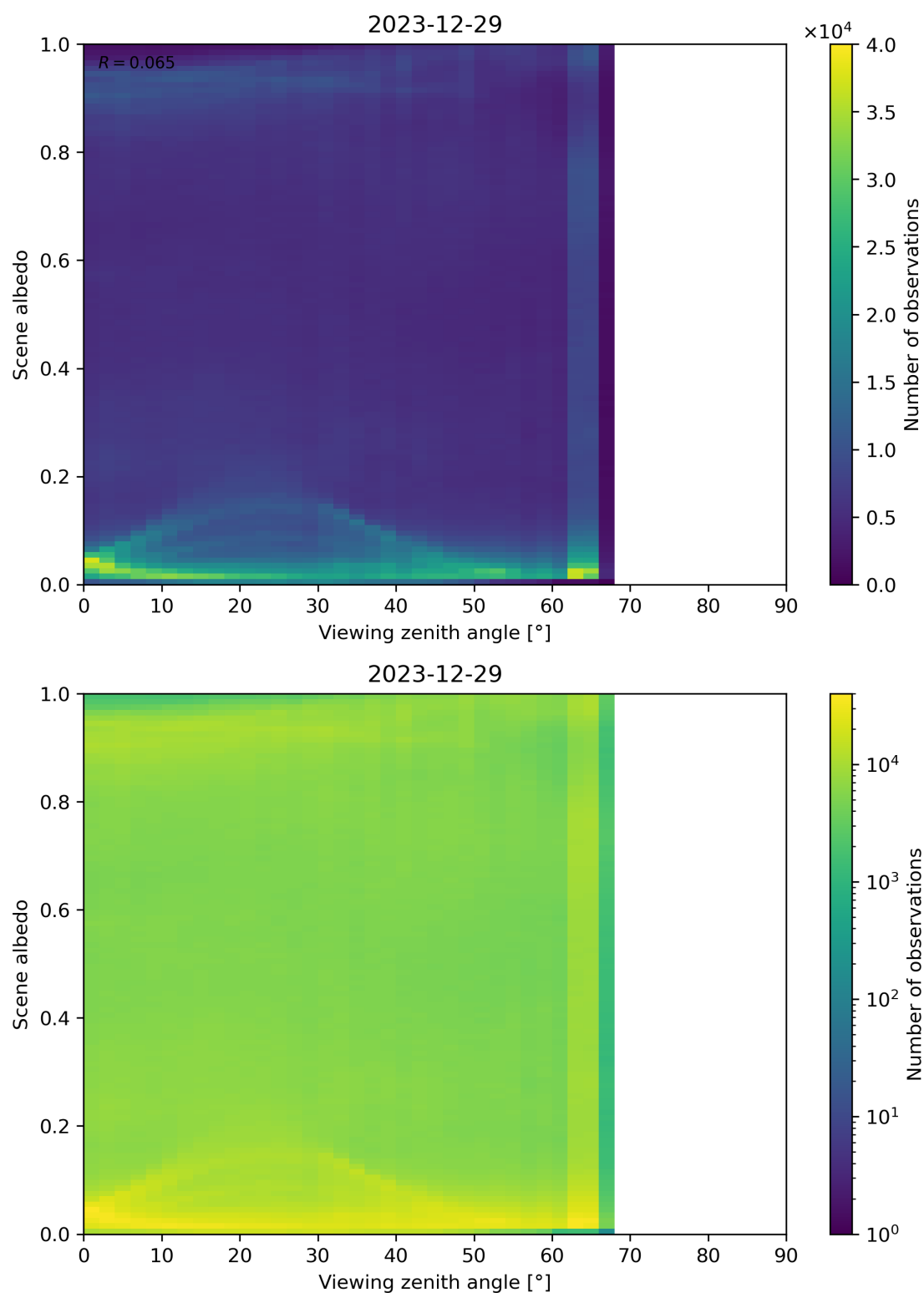
Figure 126: Scatter density plot of “Viewing zenith angle” against “Scene albedo” for 2023-12-28 to 2023-12-30.
