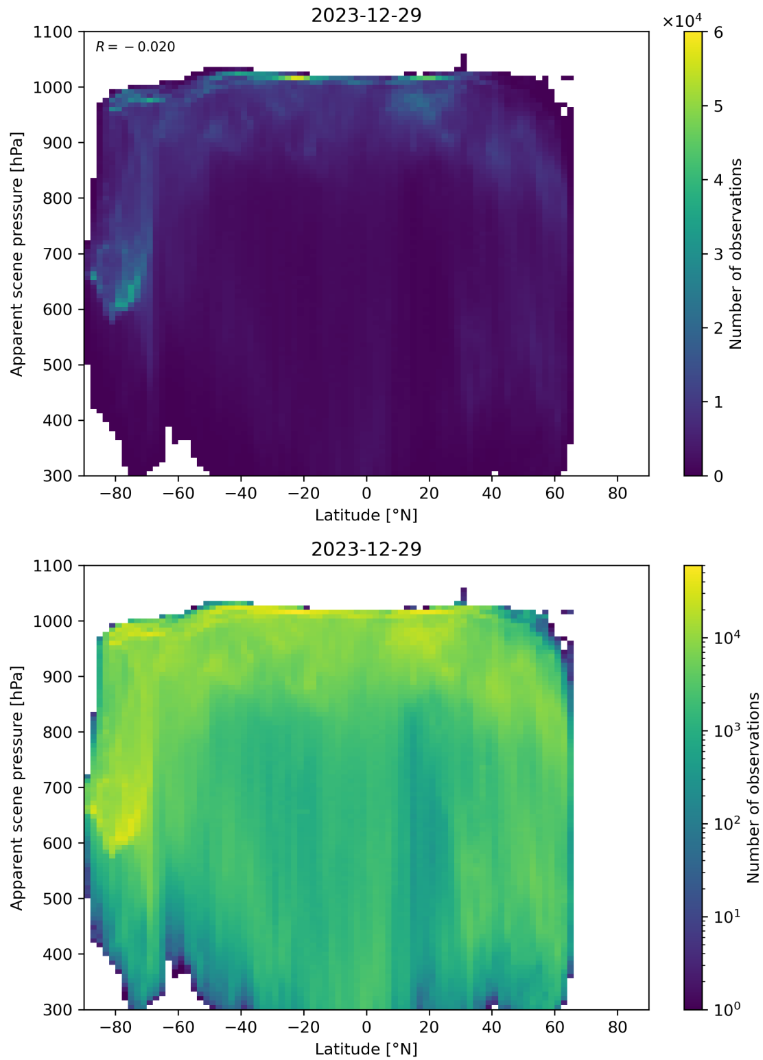
Figure 88: Scatter density plot of “Latitude” against “Apparent scene pressure” for 2023-12-28 to 2023-12-30.
