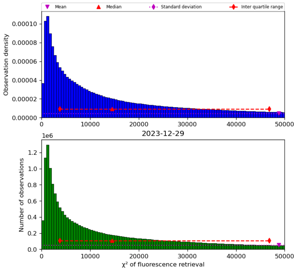
Figure 42: Histogram of “ \chi^2 of fluorescence retrieval” for 2023-12-28 to 2023-12-30
