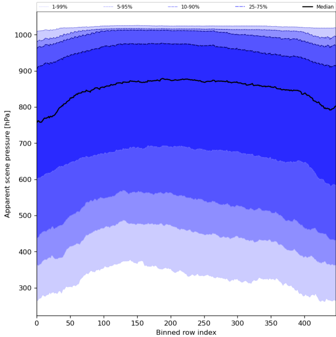
Figure 53: Along track statistics of “Apparent scene pressure” for 2023-12-28 to 2023-12-30
