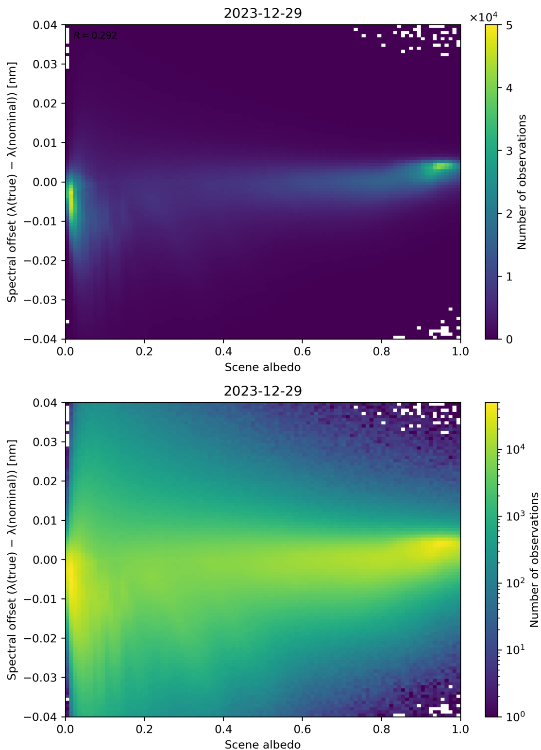
Figure 107: Scatter density plot of “Scene albedo” against “Spectral offset ( \lambda(\text{true}) - \lambda(\text{nominal}) )” for 2023-12-28 to 2023-12-30.
