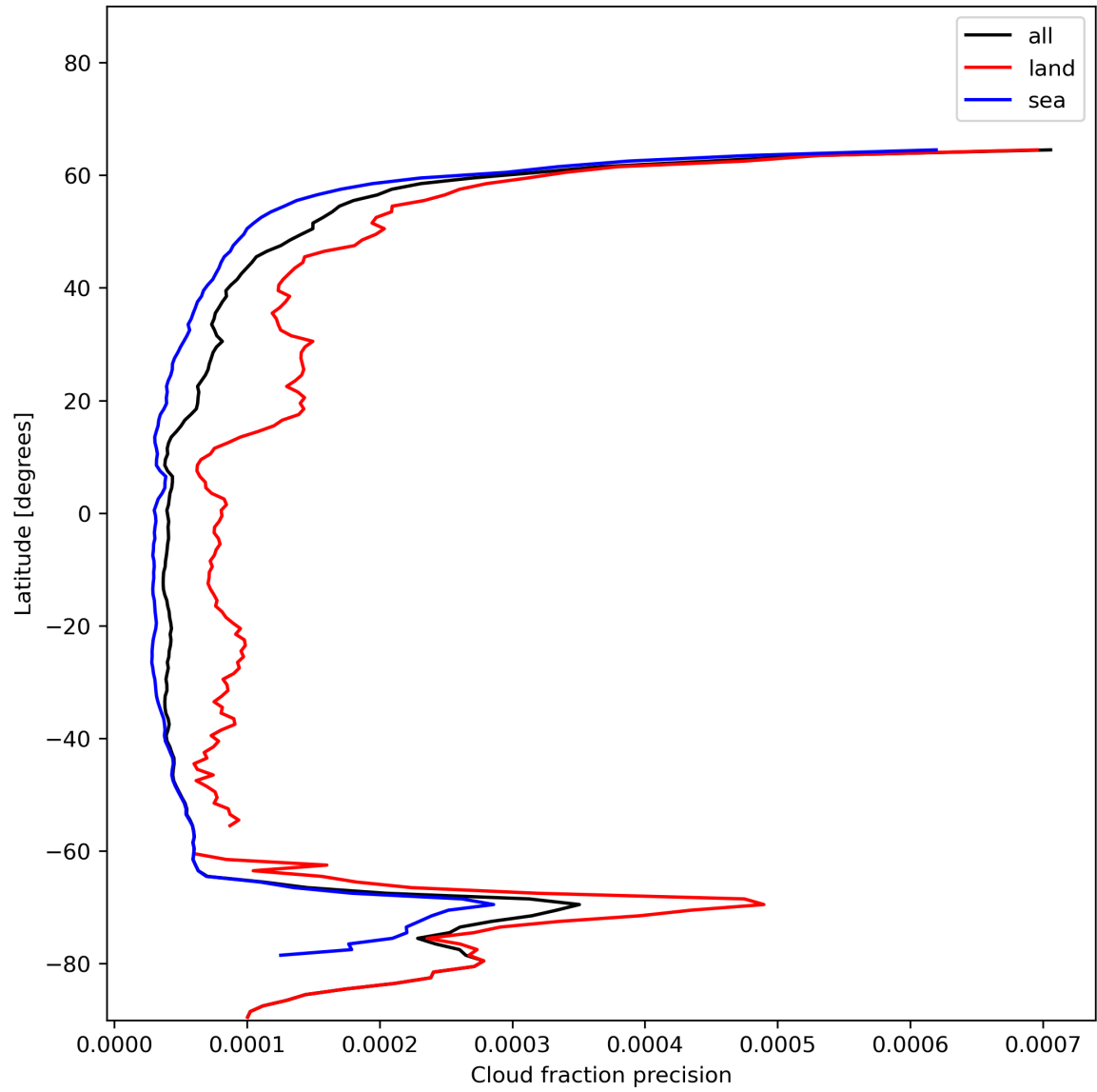
Figure 16: Zonal average of “Cloud fraction precision” for 2023-12-28 to 2023-12-30.
