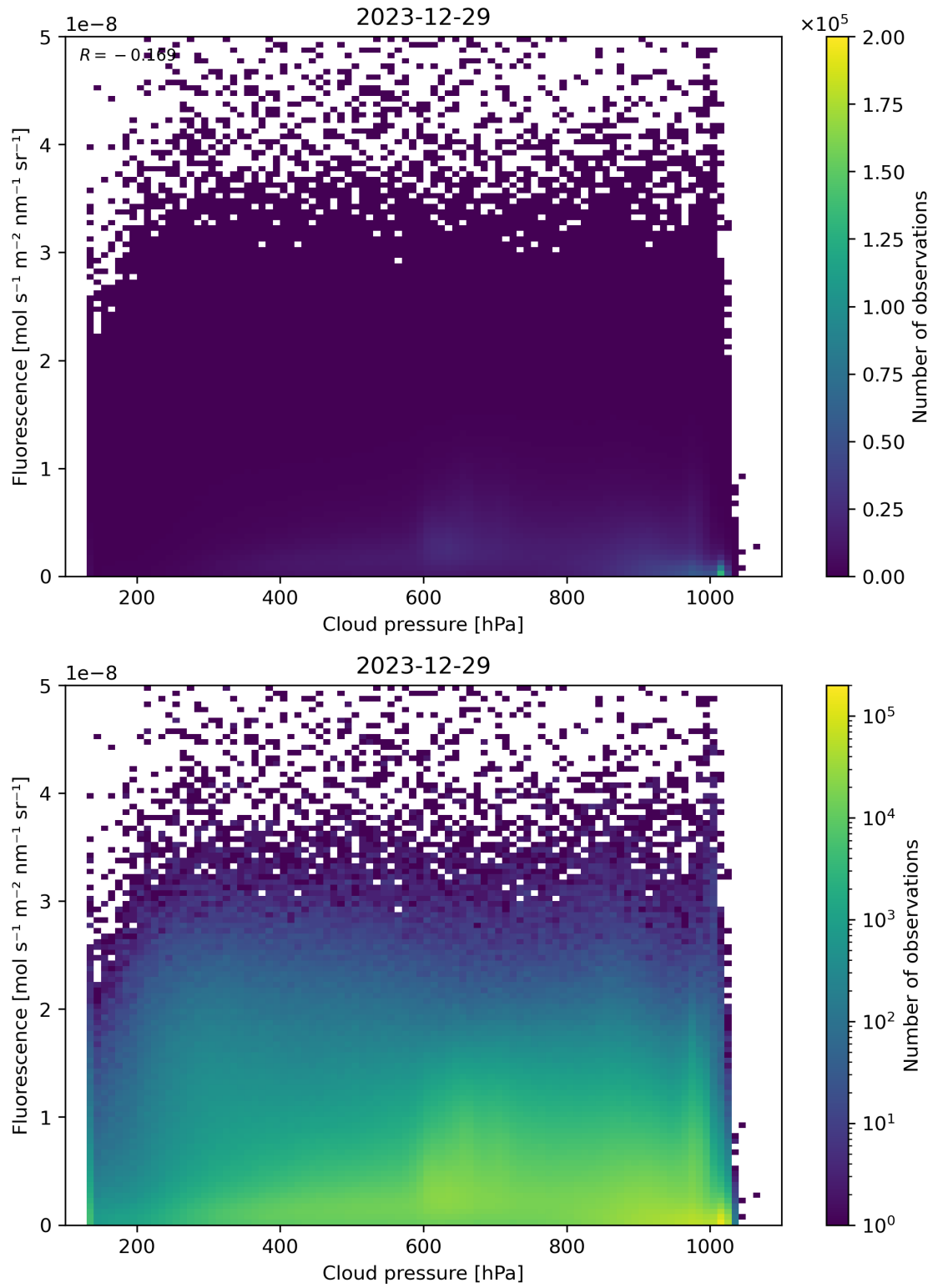
Figure 80: Scatter density plot of “Cloud pressure” against “Fluorescence” for 2023-12-28 to 2023-12-30.
