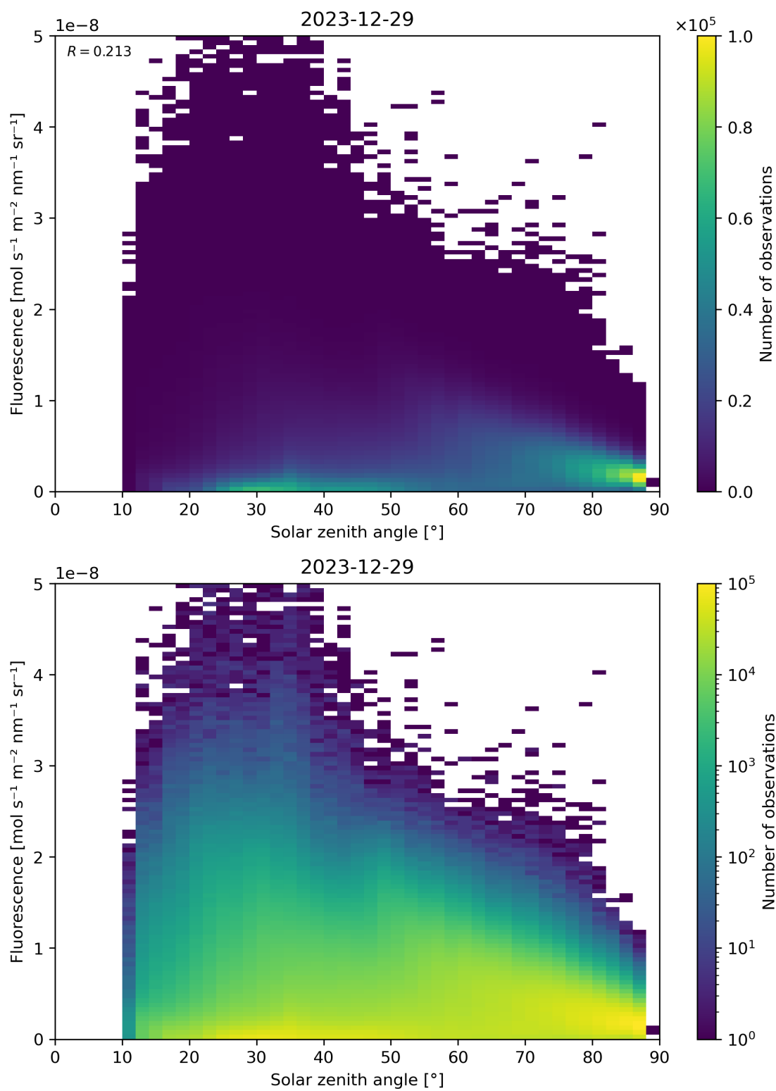
Figure 112: Scatter density plot of “Solar zenith angle” against “Fluorescence” for 2023-12-28 to 2023-12-30.
