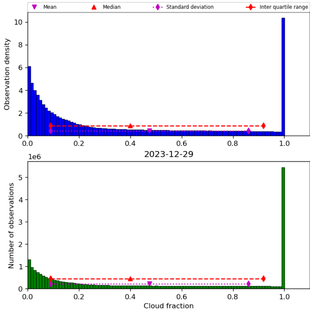
Figure 32: Histogram of “Cloud fraction” for 2023-12-28 to 2023-12-30
