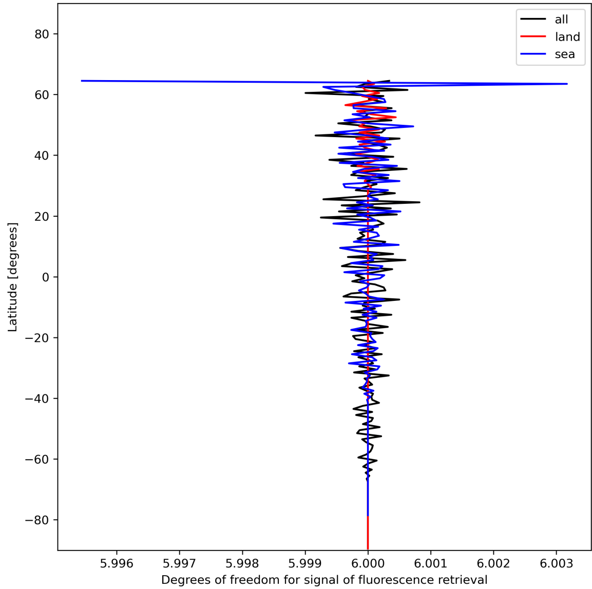
Figure 26: Zonal average of “Degrees of freedom for signal of fluorescence retrieval” for 2023-12-28 to 2023-12-30.
