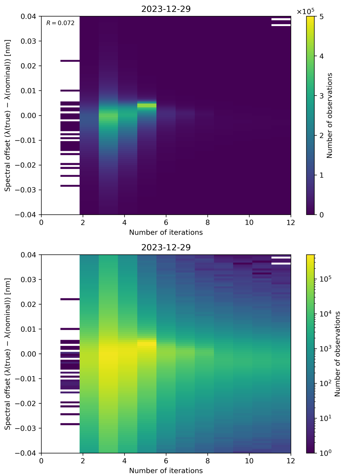
Figure 100: Scatter density plot of “Number of iterations” against “Spectral offset ( \lambda(\text{true}) - \lambda(\text{nominal}) )” for 2023-12-28 to 2023-12-30.
