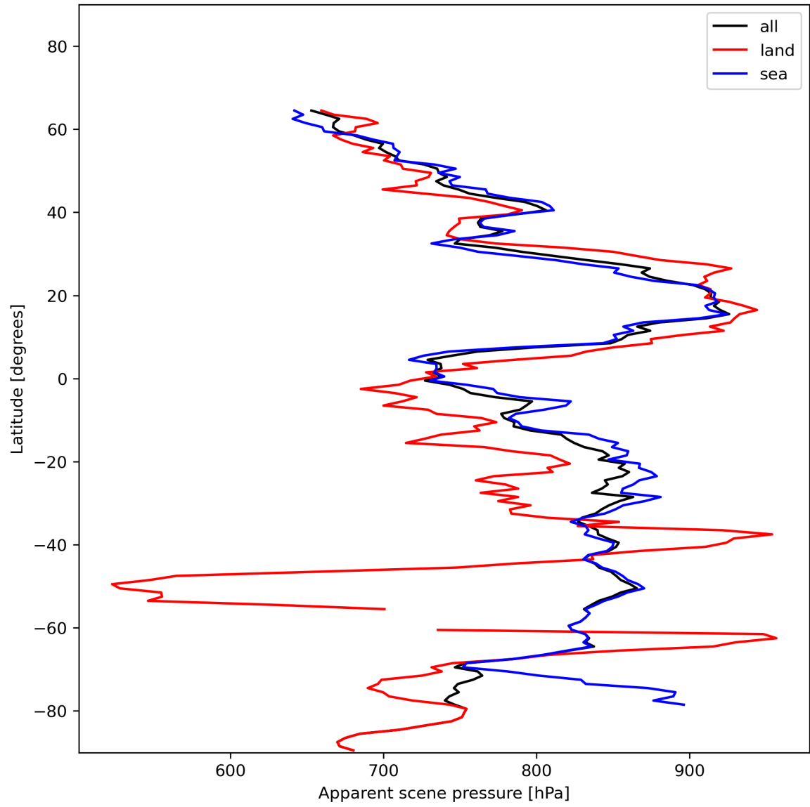
Figure 19: Zonal average of “Apparent scene pressure” for 2023-12-28 to 2023-12-30.
