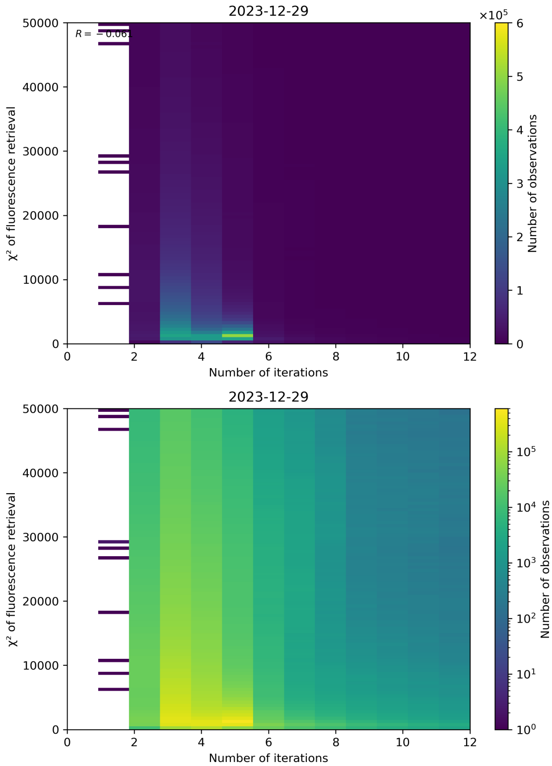
Figure 97: Scatter density plot of “Number of iterations” against “ \chi^2 of fluorescence retrieval” for 2023-12-28 to 2023-12-30.
