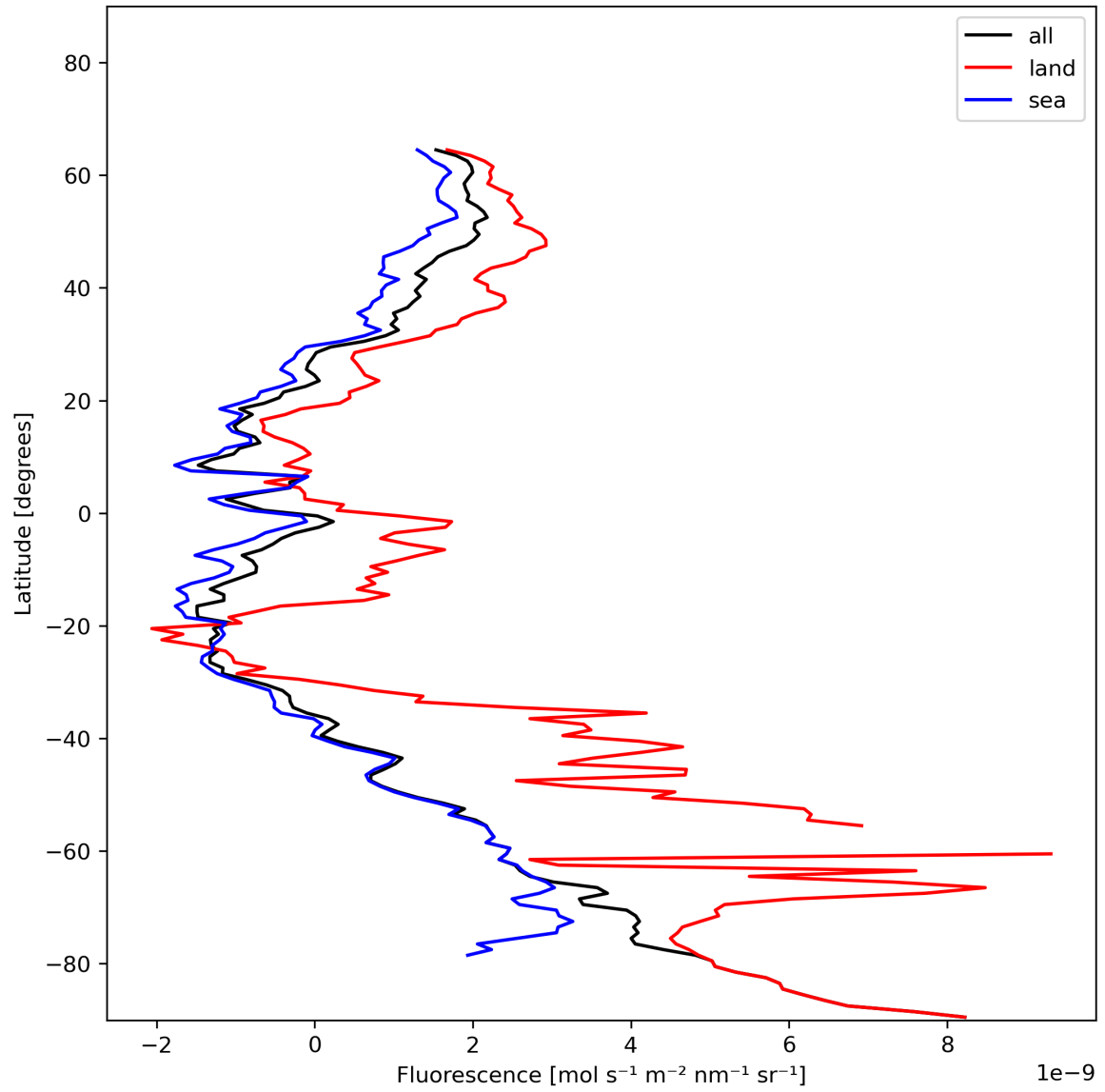
Figure 23: Zonal average of “Fluorescence” for 2023-12-28 to 2023-12-30.
