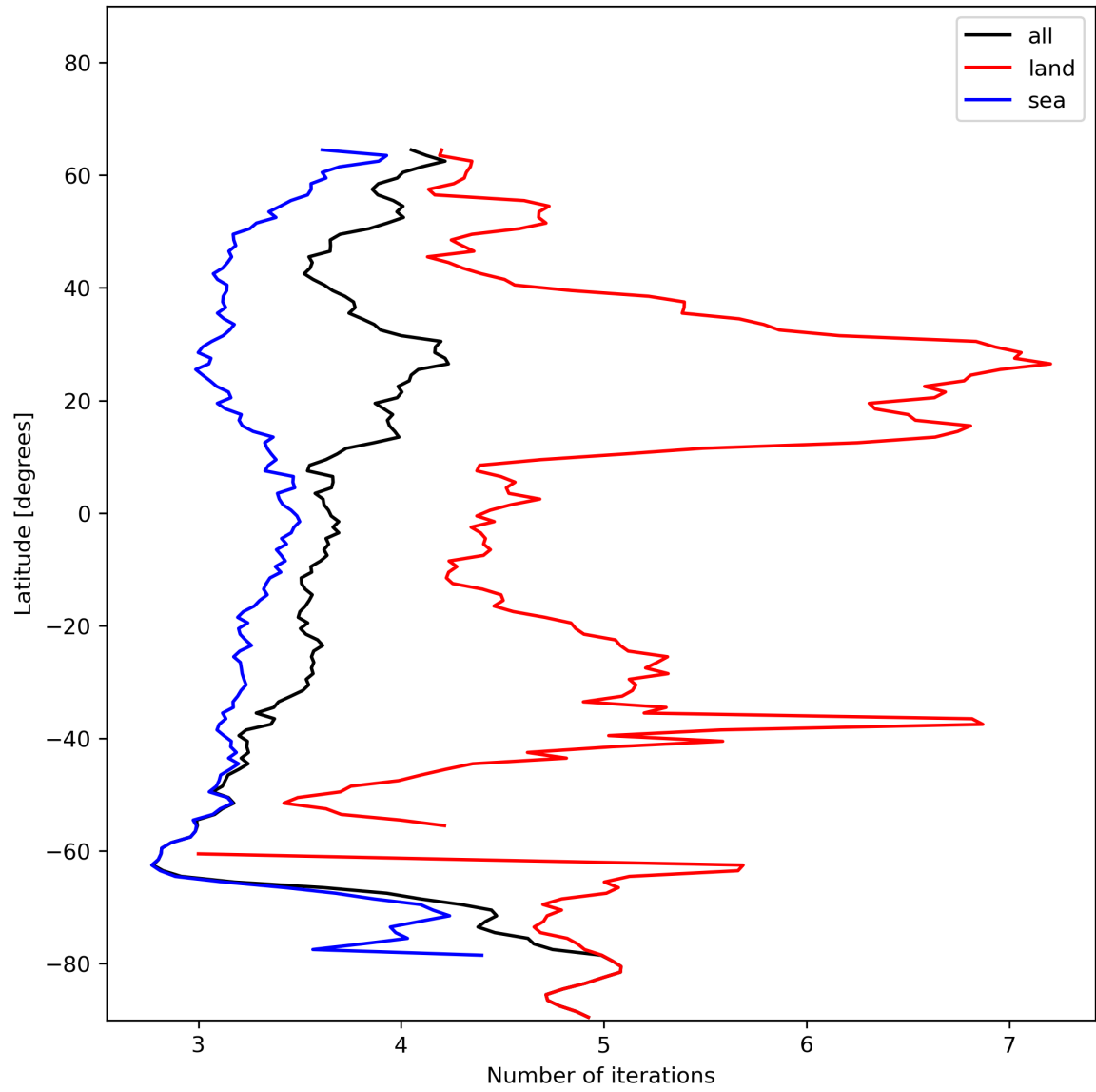
Figure 22: Zonal average of “Number of iterations” for 2023-12-28 to 2023-12-30.
