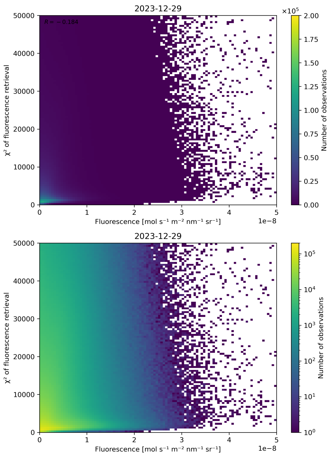
Figure 85: Scatter density plot of “Fluorescence” against “ \chi^2 of fluorescence retrieval” for 2023-12-28 to 2023-12-30.
