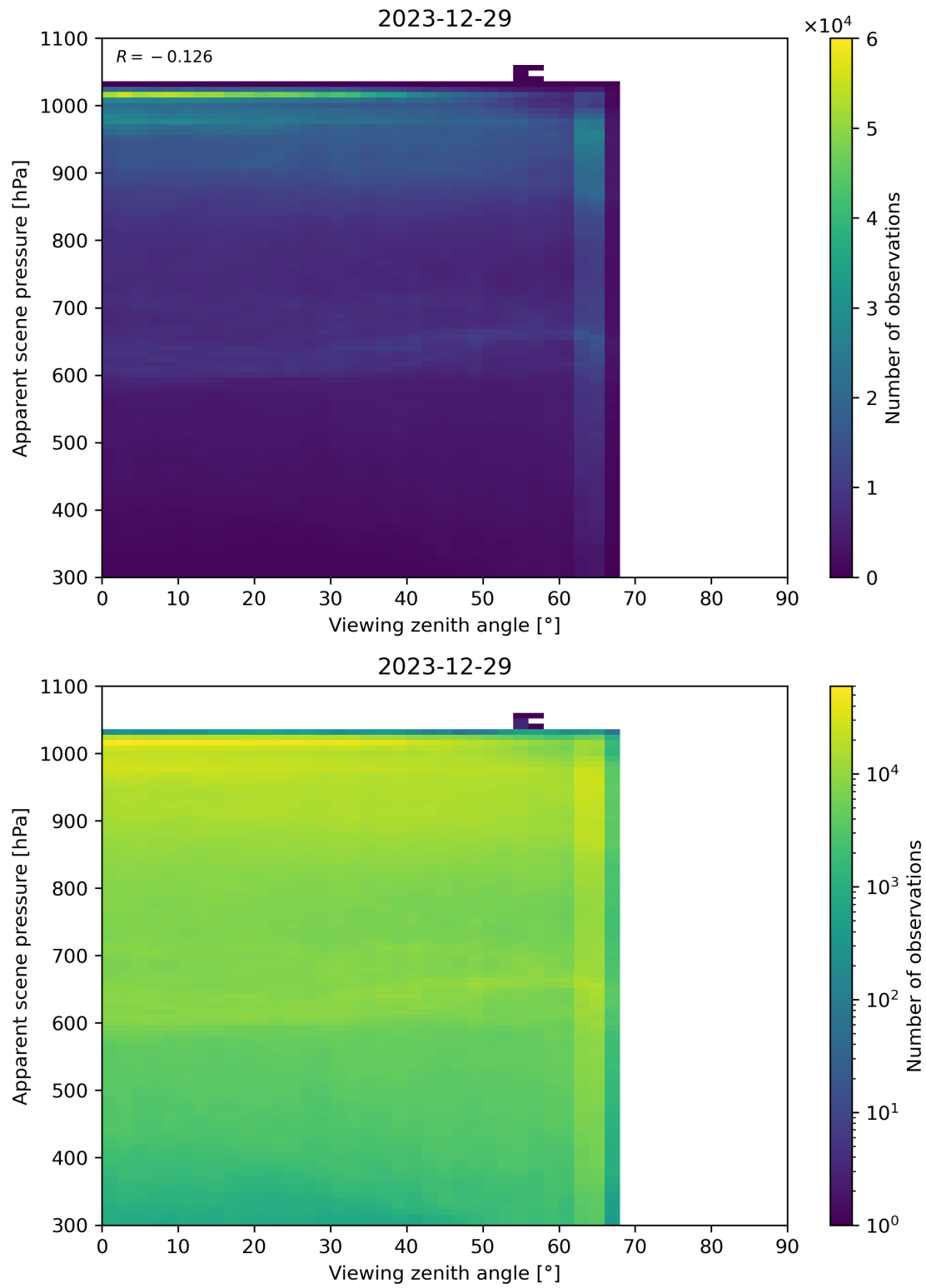
Figure 118: Scatter density plot of “Viewing zenith angle” against “Apparent scene pressure” for 2023-12-28 to 2023-12-30.
