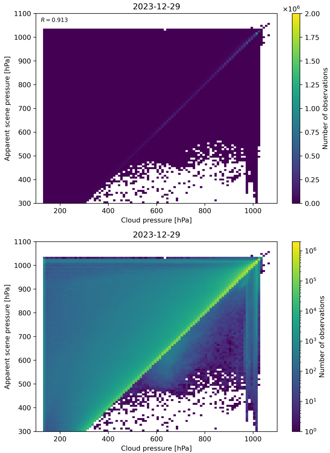
Figure 77: Scatter density plot of “Cloud pressure” against “Apparent scene pressure” for 2023-12-28 to 2023-12-30.
