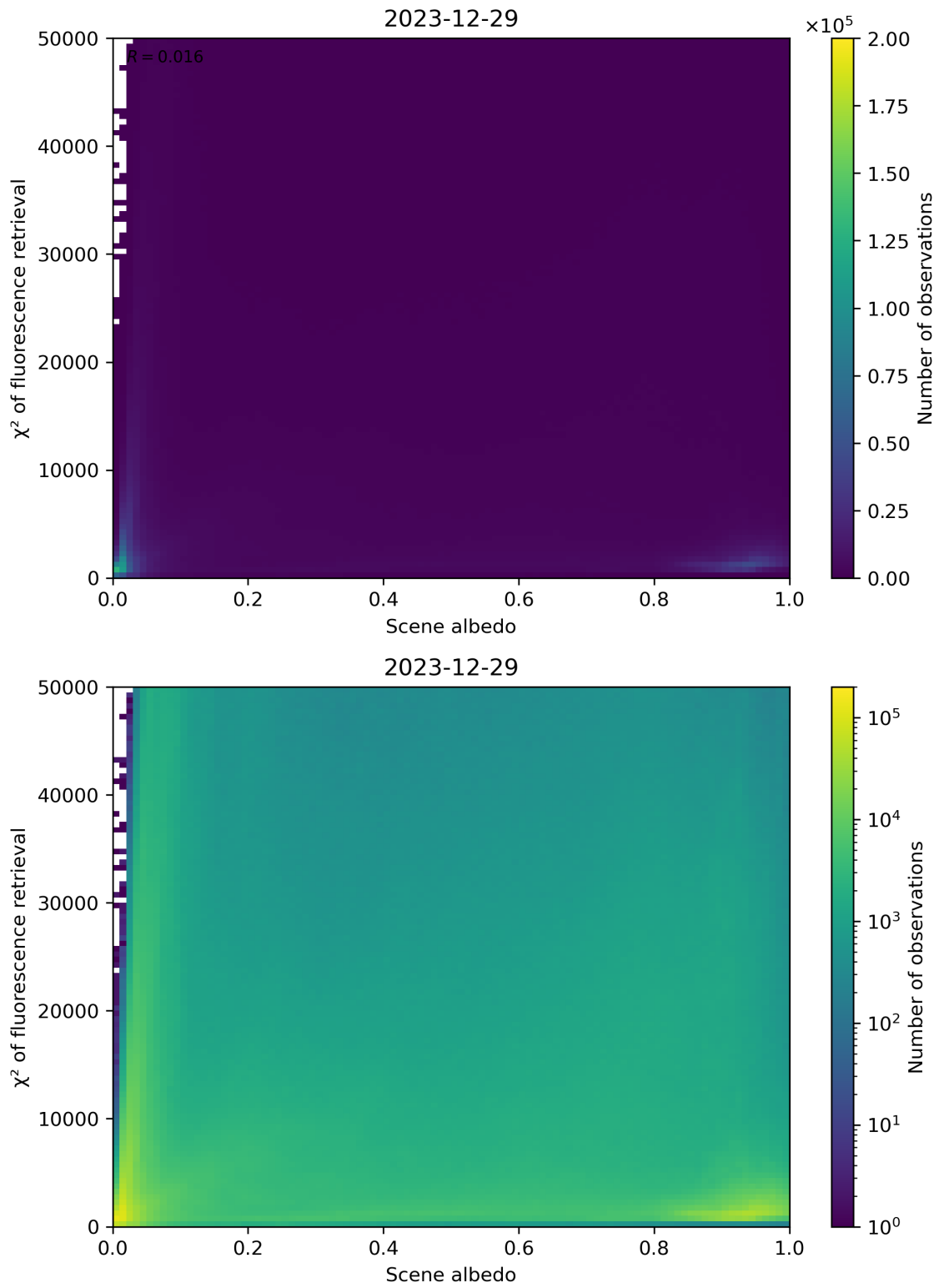
Figure 103: Scatter density plot of “Scene albedo” against “ \chi^2 of fluorescence retrieval” for 2023-12-28 to 2023-12-30.
