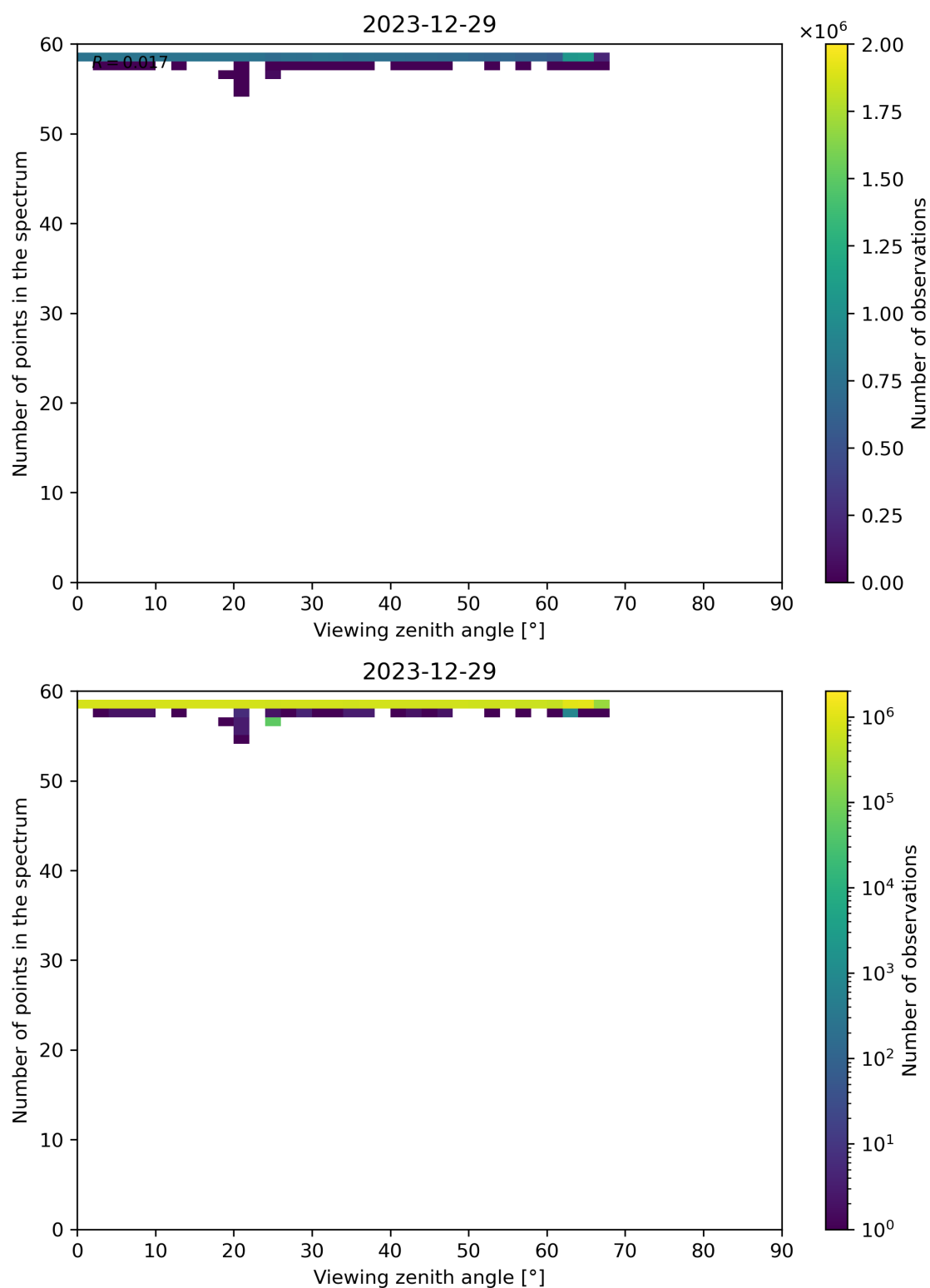
Figure 125: Scatter density plot of “Viewing zenith angle” against “Number of points in the spectrum” for 2023-12-28 to 2023-12-30.
