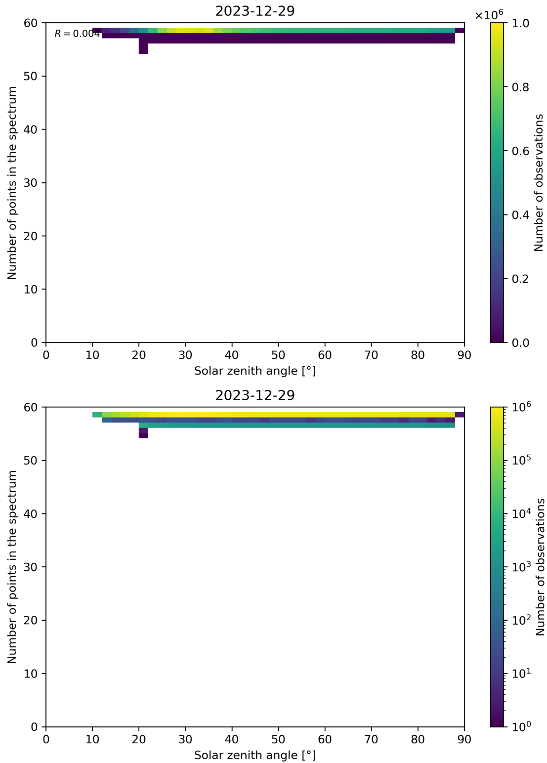
Figure 115: Scatter density plot of “Solar zenith angle” against “Number of points in the spectrum” for 2023-12-28 to 2023-12-30.
