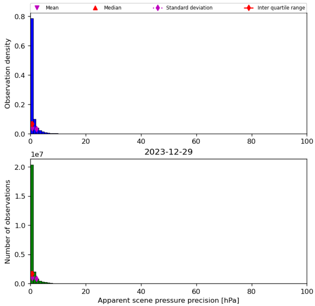
Figure 37: Histogram of “Apparent scene pressure precision” for 2023-12-28 to 2023-12-30
