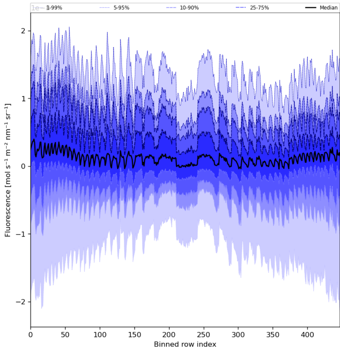
Figure 57: Along track statistics of “Fluorescence” for 2023-12-28 to 2023-12-30
