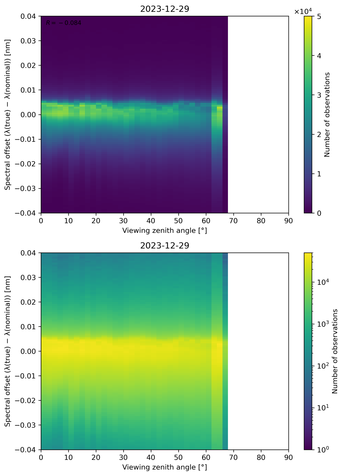
Figure 128: Scatter density plot of “Viewing zenith angle” against “Spectral offset ( \lambda(\text{true}) - \lambda(\text{nominal}) )” for 2023-12-28 to 2023-12-30.
