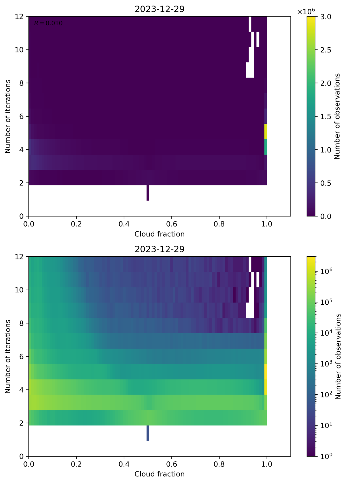
Figure 73: Scatter density plot of “Cloud fraction” against “Number of iterations” for 2023-12-28 to 2023-12-30.
