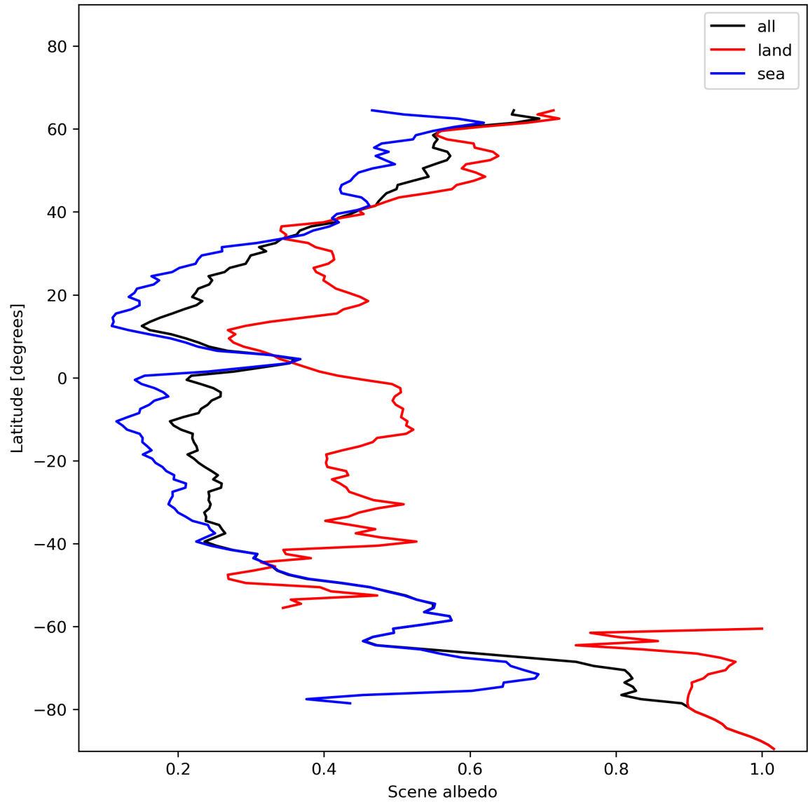
Figure 17: Zonal average of “Scene albedo” for 2023-12-30 to 2023-12-31.
