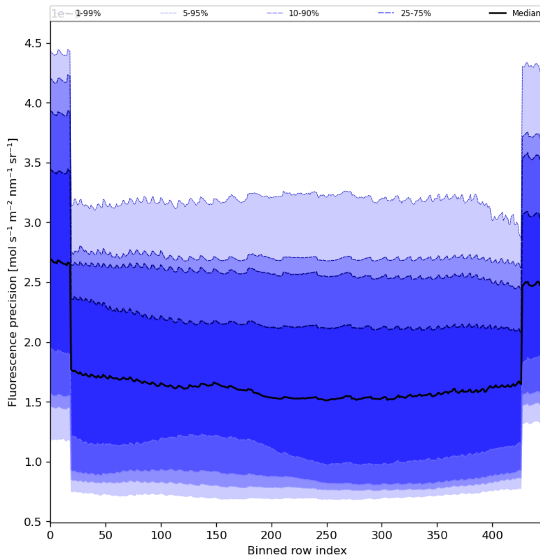
Figure 58: Along track statistics of “Fluorescence precision” for 2023-12-30 to 2023-12-31
