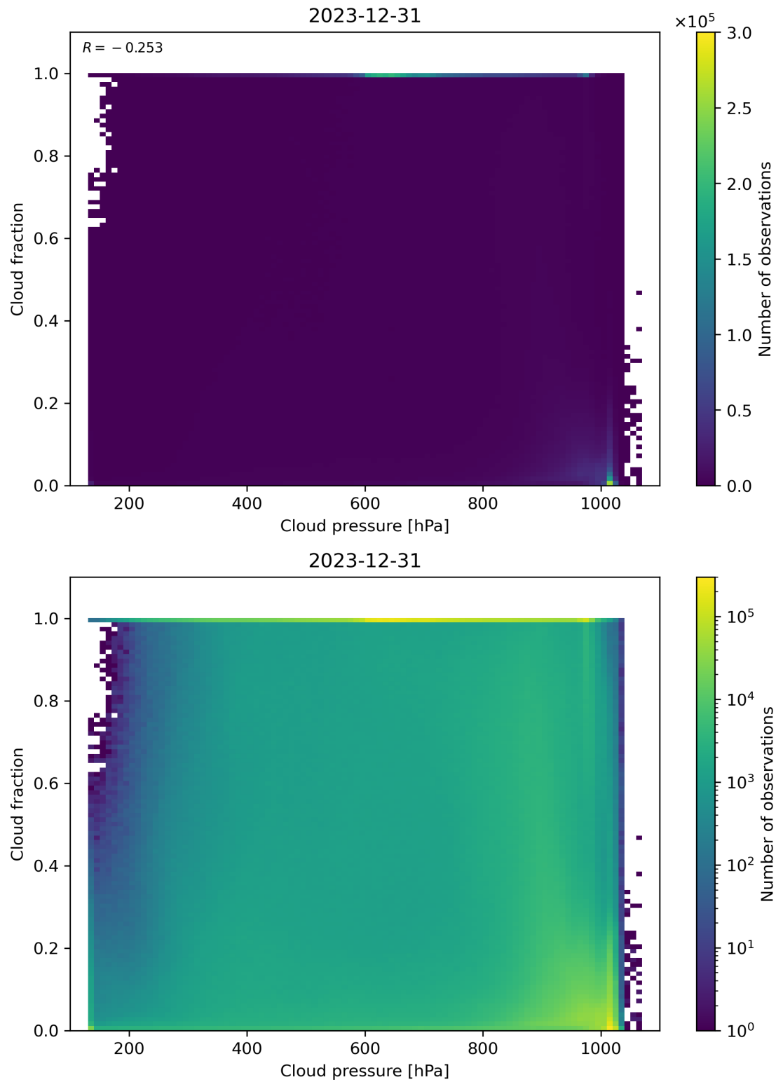
Figure 79: Scatter density plot of “Cloud pressure” against “Cloud fraction” for 2023-12-30 to 2023-12-31.
