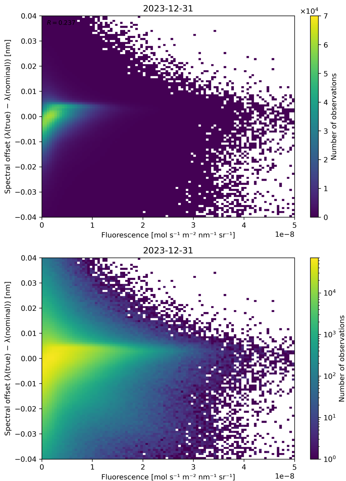
Figure 87: Scatter density plot of “Fluorescence” against “Spectral offset ( \lambda(\text{true}) - \lambda(\text{nominal}) )” for 2023-12-30 to 2023-12-31.
