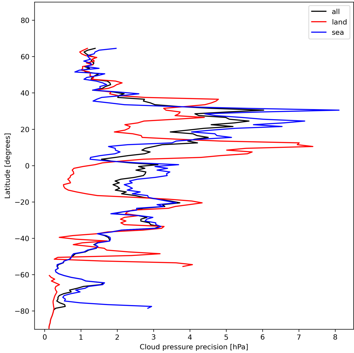
Figure 14: Zonal average of "Cloud pressure precision" for 2023-12-30 to 2023-12-31.
