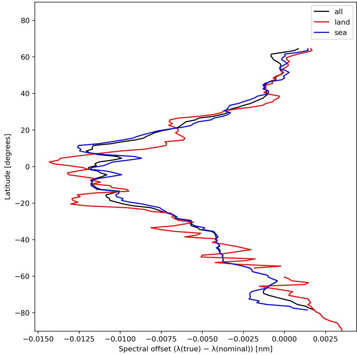
Figure 28: Zonal average of “Spectral offset ( \lambda(\text{true}) - \lambda(\text{nominal}) )” for 2023-12-30 to 2023-12-31.
