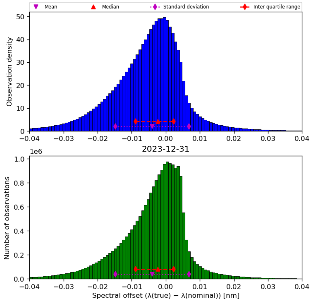
Figure 45: Histogram of “Spectral offset ( \lambda(\text{true}) - \lambda(\text{nominal}) )” for 2023-12-30 to 2023-12-31
