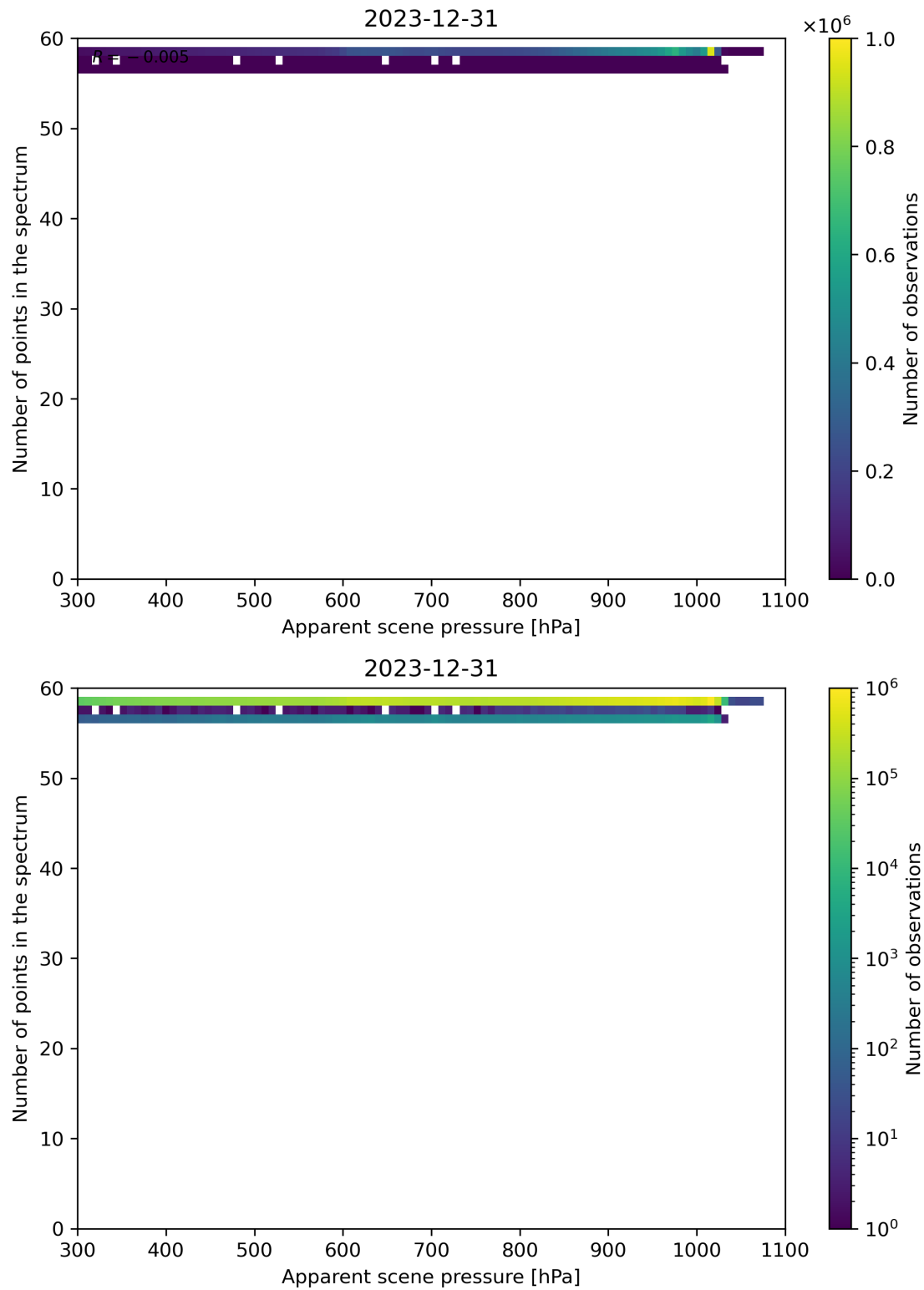
Figure 66: Scatter density plot of “Apparent scene pressure” against “Number of points in the spectrum” for 2023-12-30 to 2023-12-31.
