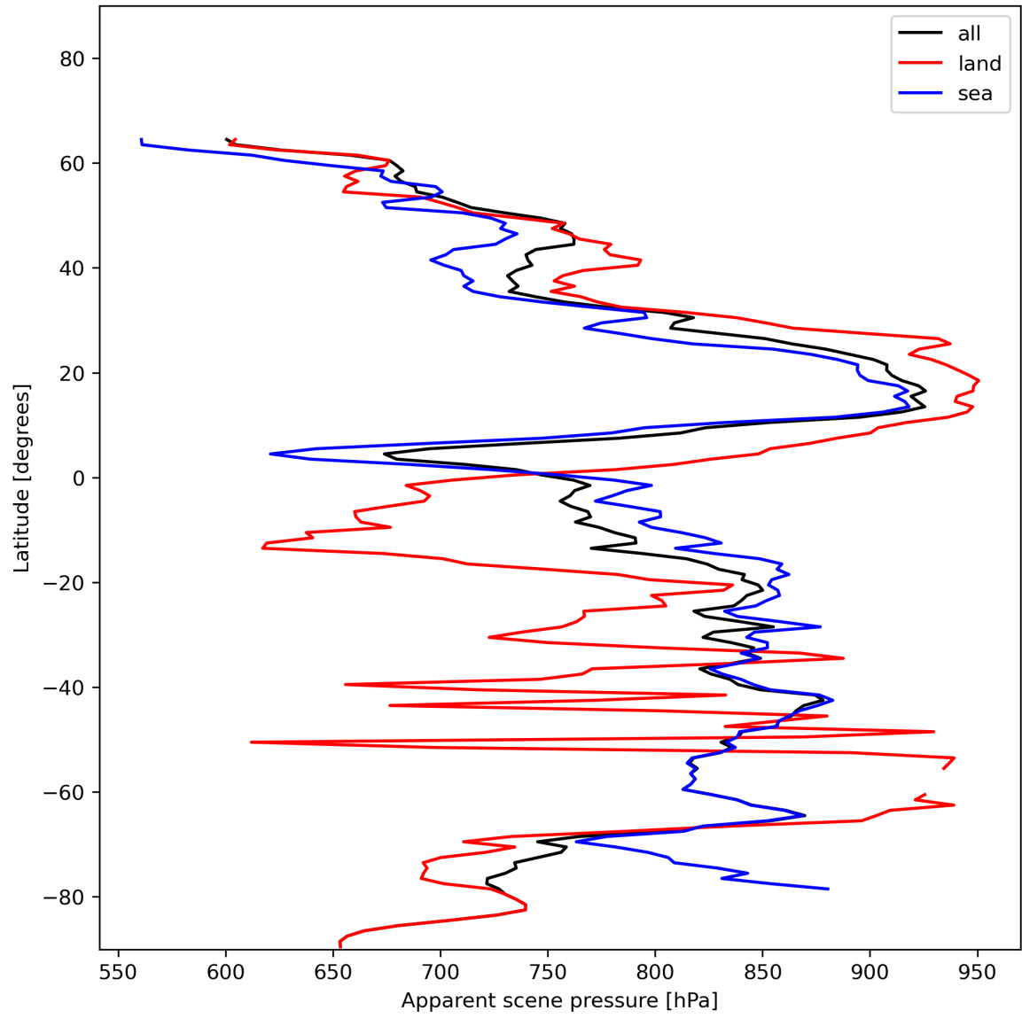
Figure 19: Zonal average of “Apparent scene pressure” for 2023-12-30 to 2023-12-31.
