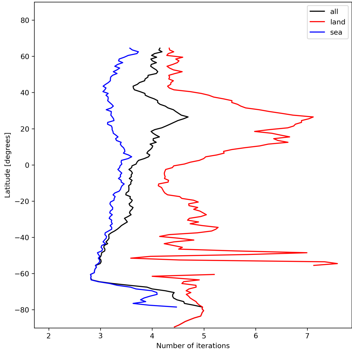
Figure 22: Zonal average of “Number of iterations” for 2023-12-30 to 2023-12-31.
