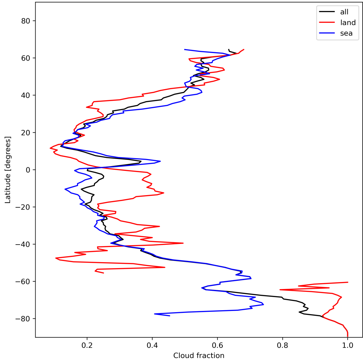
Figure 15: Zonal average of “Cloud fraction” for 2023-12-30 to 2023-12-31.
