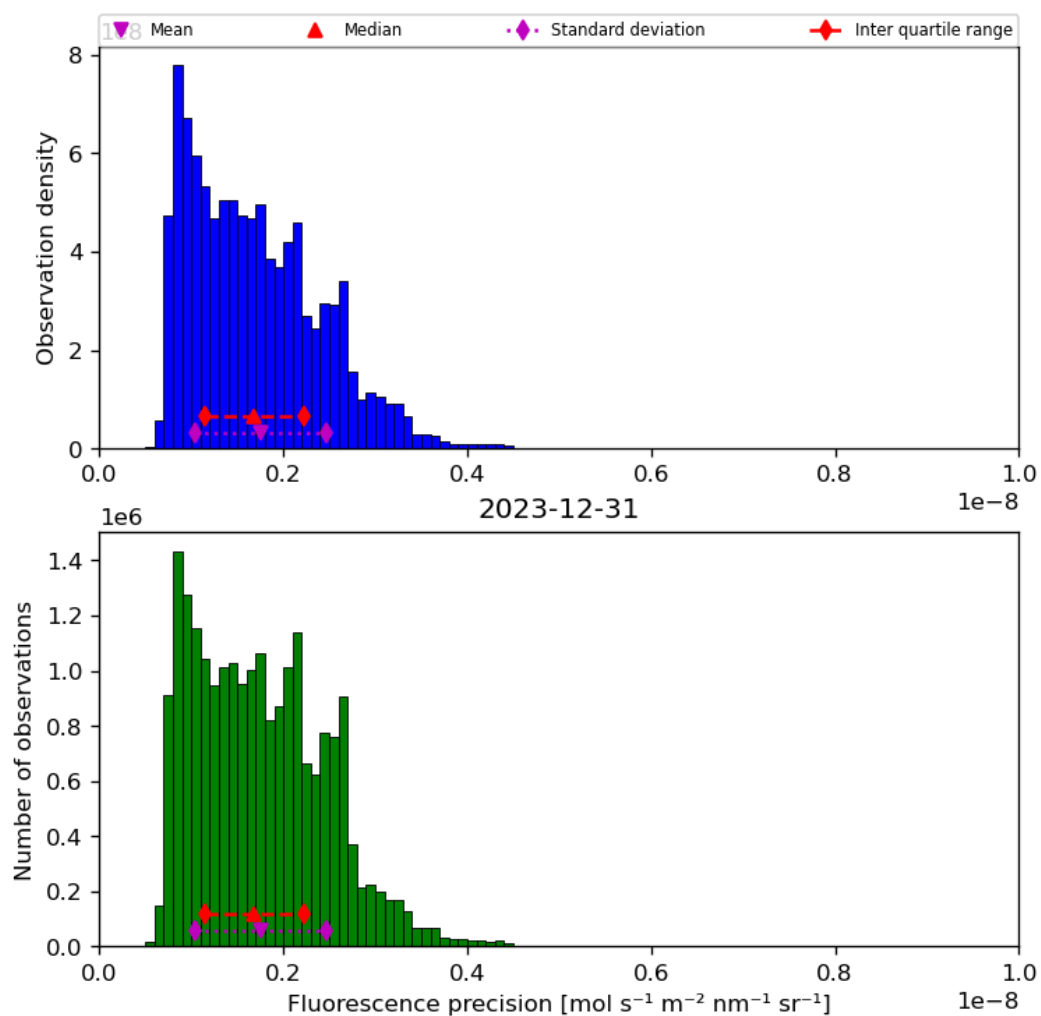
Figure 41: Histogram of “Fluorescence precision” for 2023-12-30 to 2023-12-31
