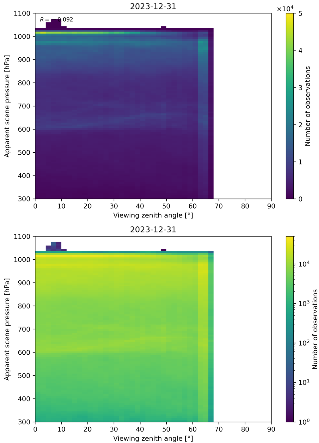
Figure 118: Scatter density plot of “Viewing zenith angle” against “Apparent scene pressure” for 2023-12-30 to 2023-12-31.
