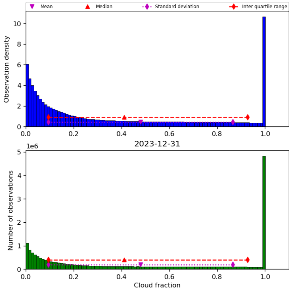
Figure 32: Histogram of “Cloud fraction” for 2023-12-30 to 2023-12-31
