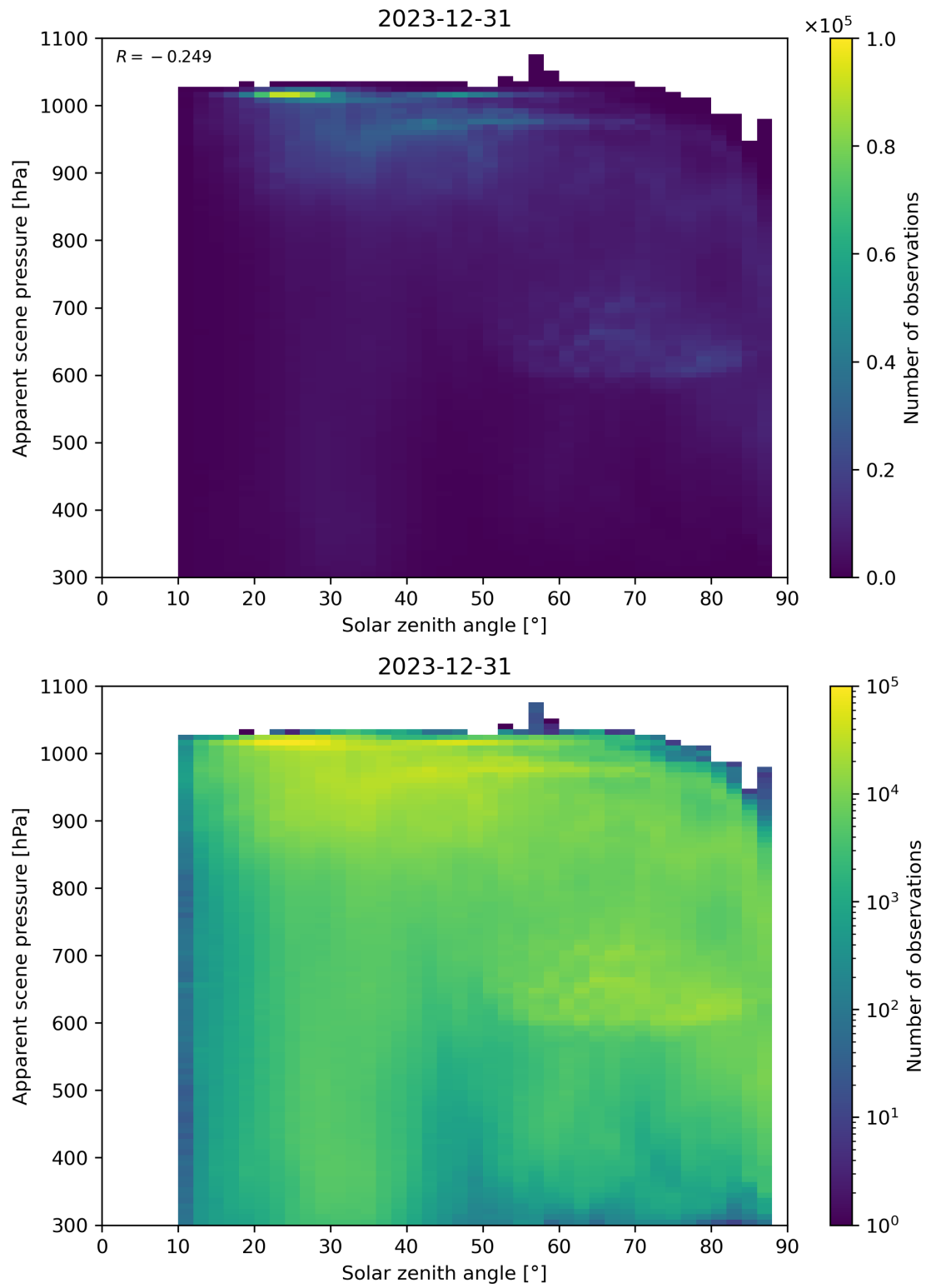
Figure 108: Scatter density plot of “Solar zenith angle” against “Apparent scene pressure” for 2023-12-30 to 2023-12-31.
