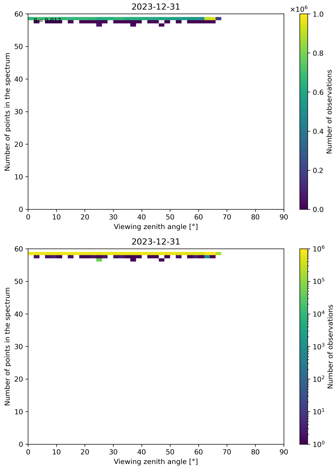
Figure 125: Scatter density plot of “Viewing zenith angle” against “Number of points in the spectrum” for 2023-12-30 to 2023-12-31.
