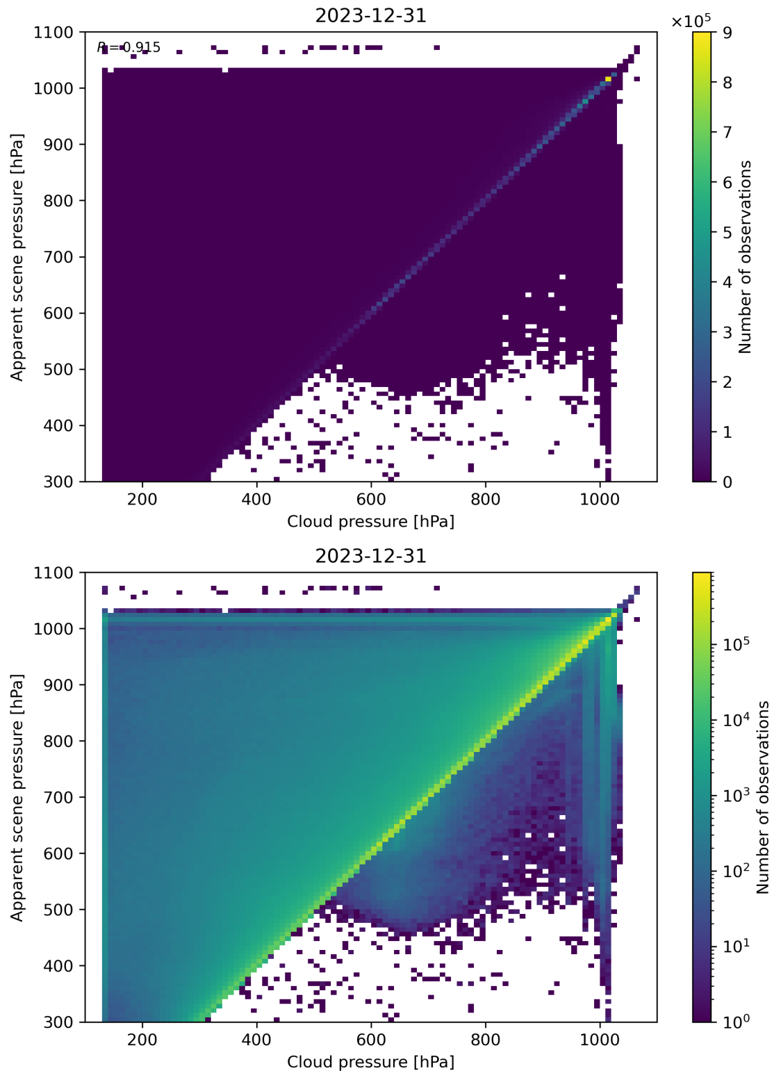
Figure 77: Scatter density plot of “Cloud pressure” against “Apparent scene pressure” for 2023-12-30 to 2023-12-31.
