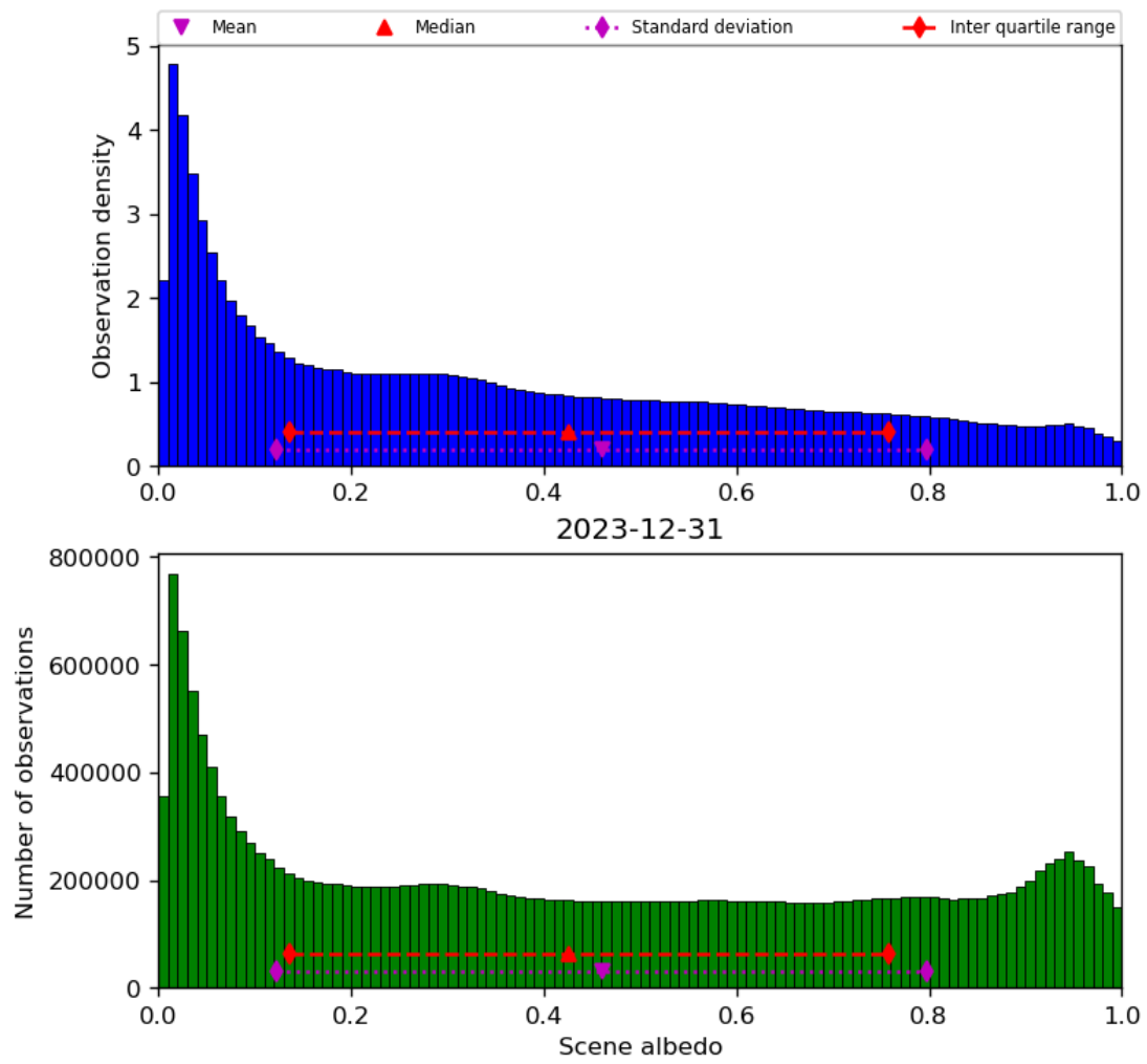
Figure 34: Histogram of “Scene albedo” for 2023-12-30 to 2023-12-31
