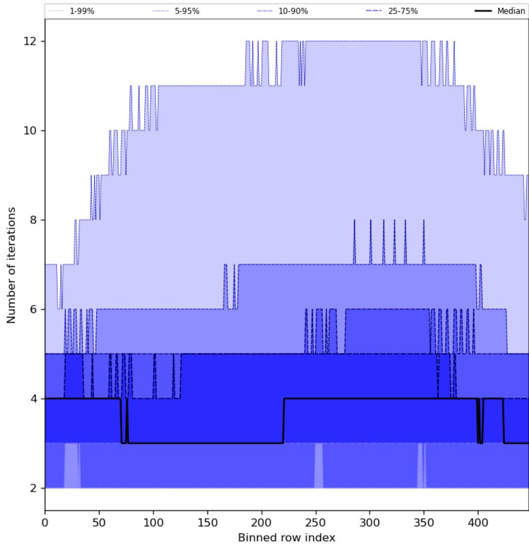
Figure 56: Along track statistics of “Number of iterations” for 2023-12-30 to 2023-12-31
