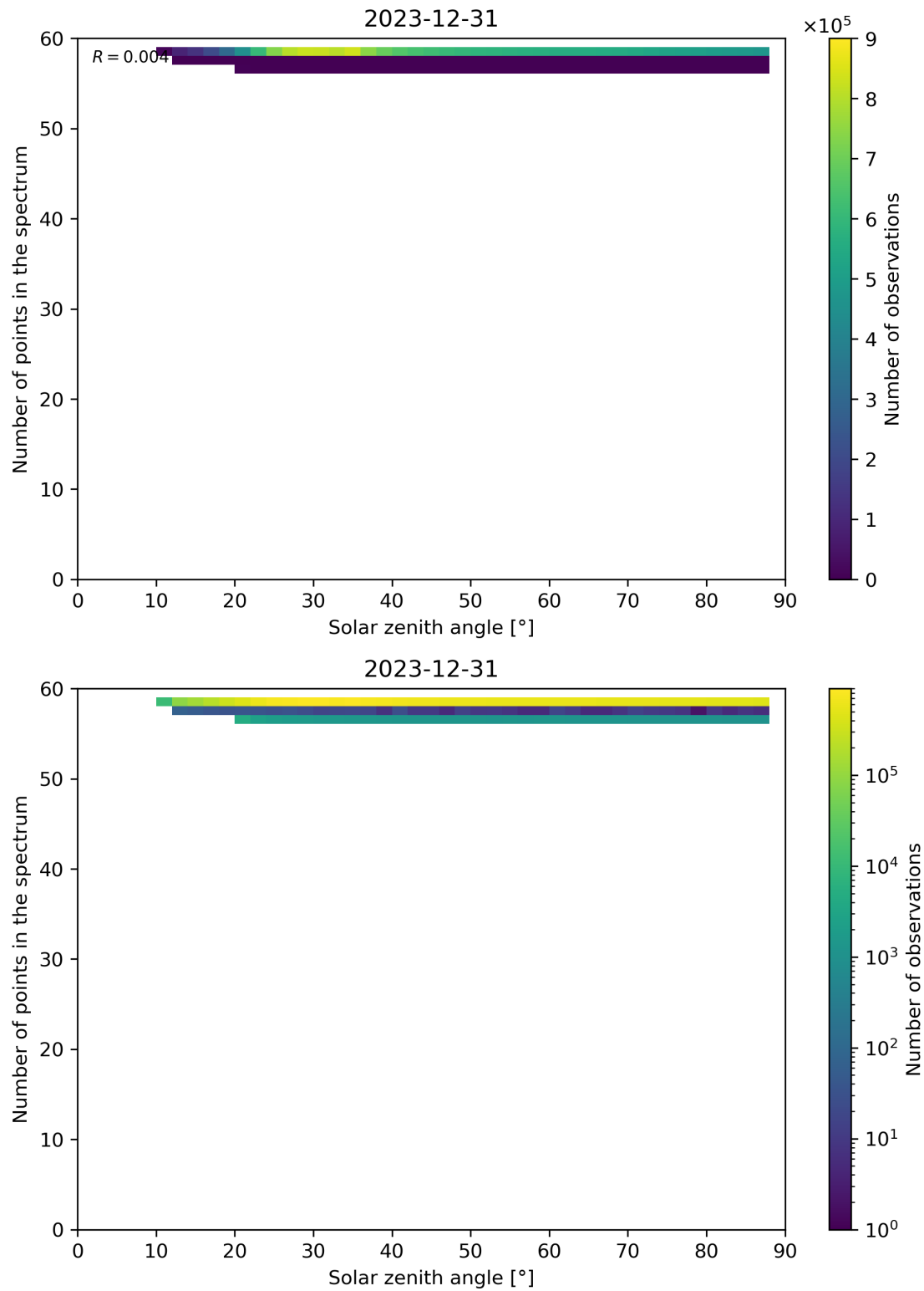
Figure 115: Scatter density plot of “Solar zenith angle” against “Number of points in the spectrum” for 2023-12-30 to 2023-12-31.
