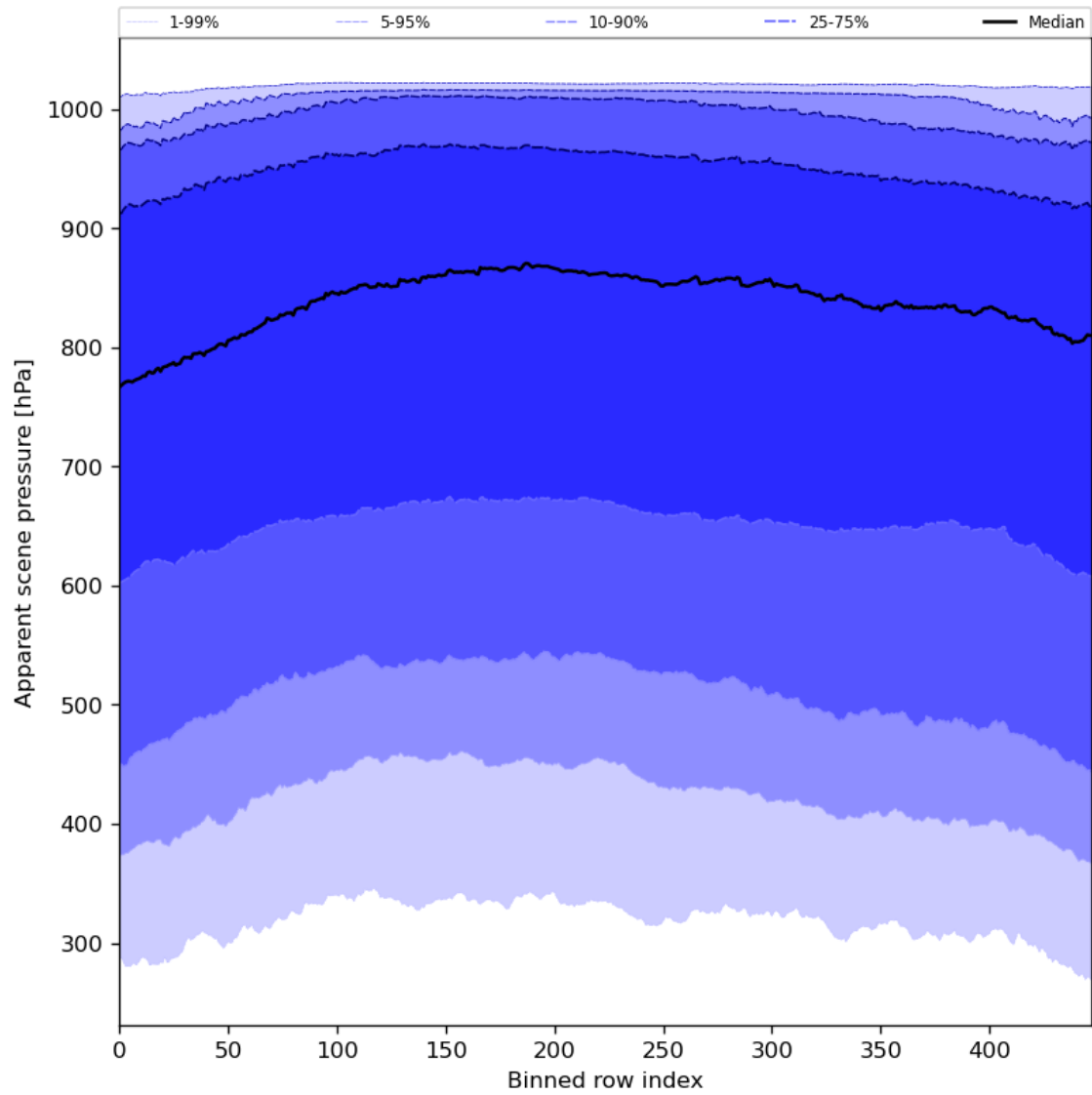
Figure 53: Along track statistics of “Apparent scene pressure” for 2023-12-30 to 2023-12-31
