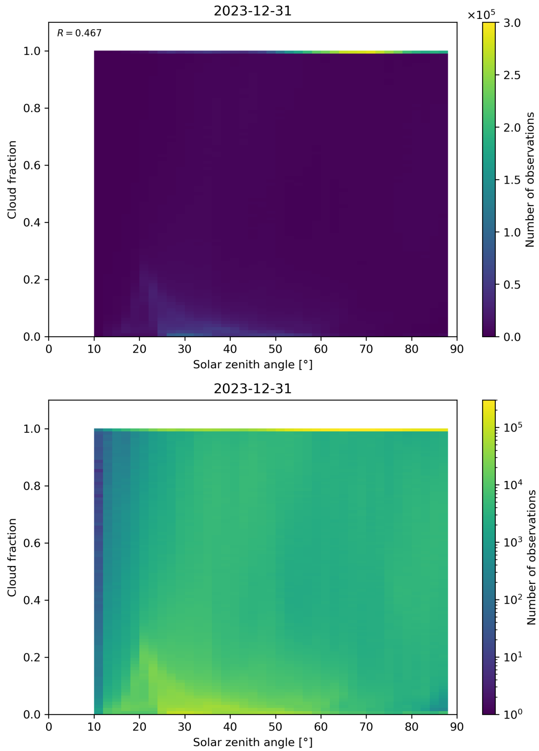
Figure 110: Scatter density plot of “Solar zenith angle” against “Cloud fraction” for 2023-12-30 to 2023-12-31.
