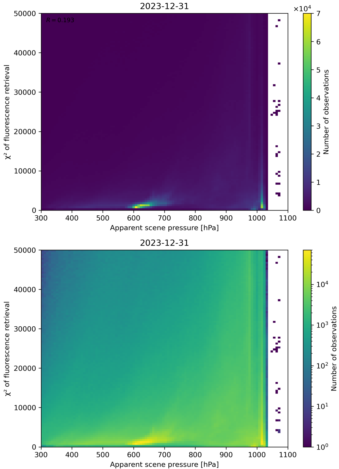
Figure 63: Scatter density plot of “Apparent scene pressure” against “ \chi^2 of fluorescence retrieval” for 2023-12-30 to 2023-12-31.
