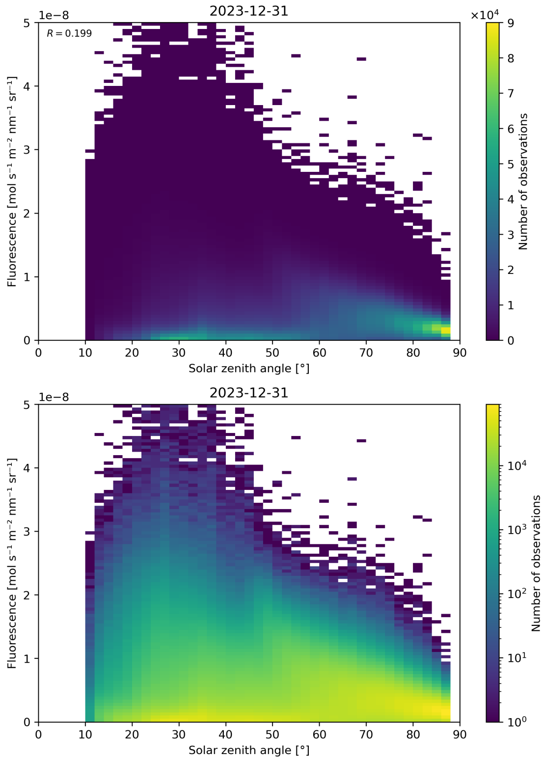
Figure 112: Scatter density plot of “Solar zenith angle” against “Fluorescence” for 2023-12-30 to 2023-12-31.
