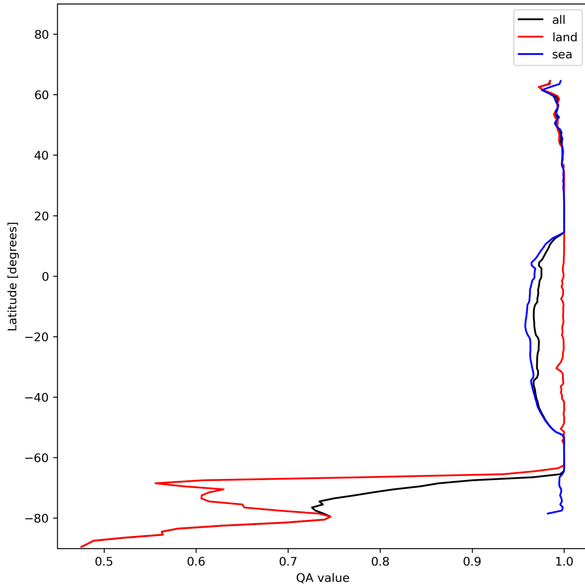
Figure 12: Zonal average of “QA value” for 2023-12-30 to 2023-12-31.
