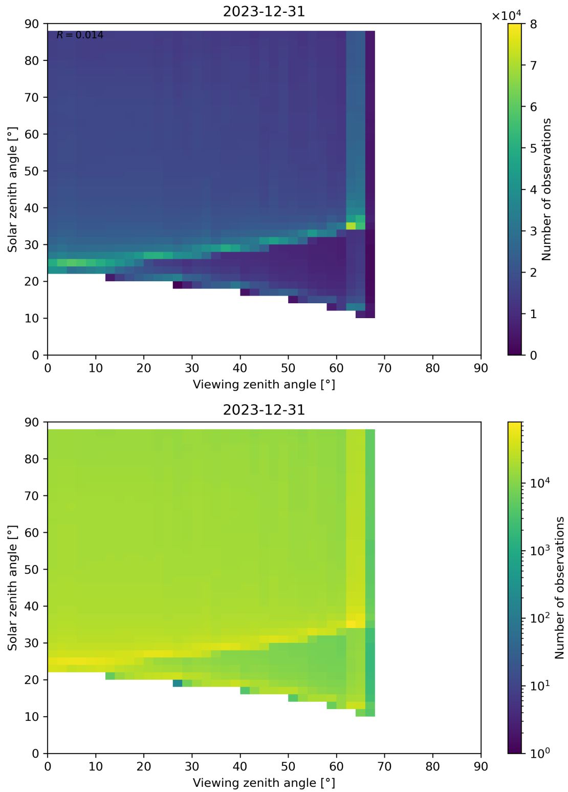
Figure 127: Scatter density plot of “Viewing zenith angle” against “Solar zenith angle” for 2023-12-30 to 2023-12-31.
