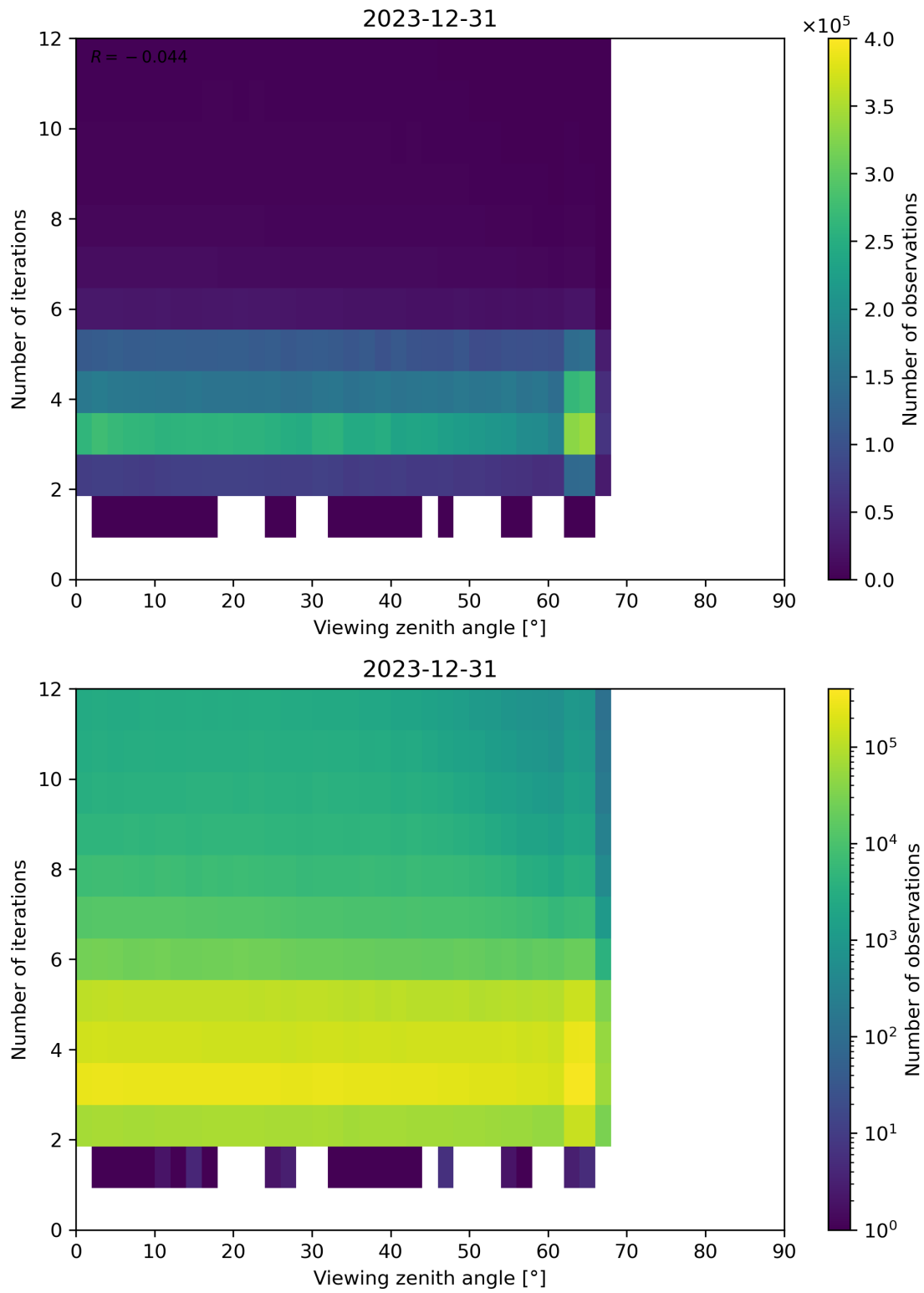
Figure 124: Scatter density plot of “Viewing zenith angle” against “Number of iterations” for 2023-12-30 to 2023-12-31.
