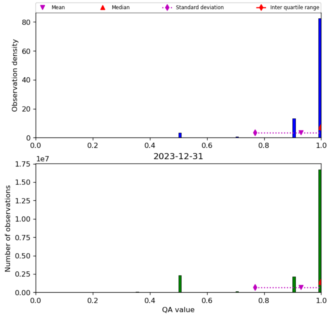
Figure 29: Histogram of “QA value” for 2023-12-30 to 2023-12-31
