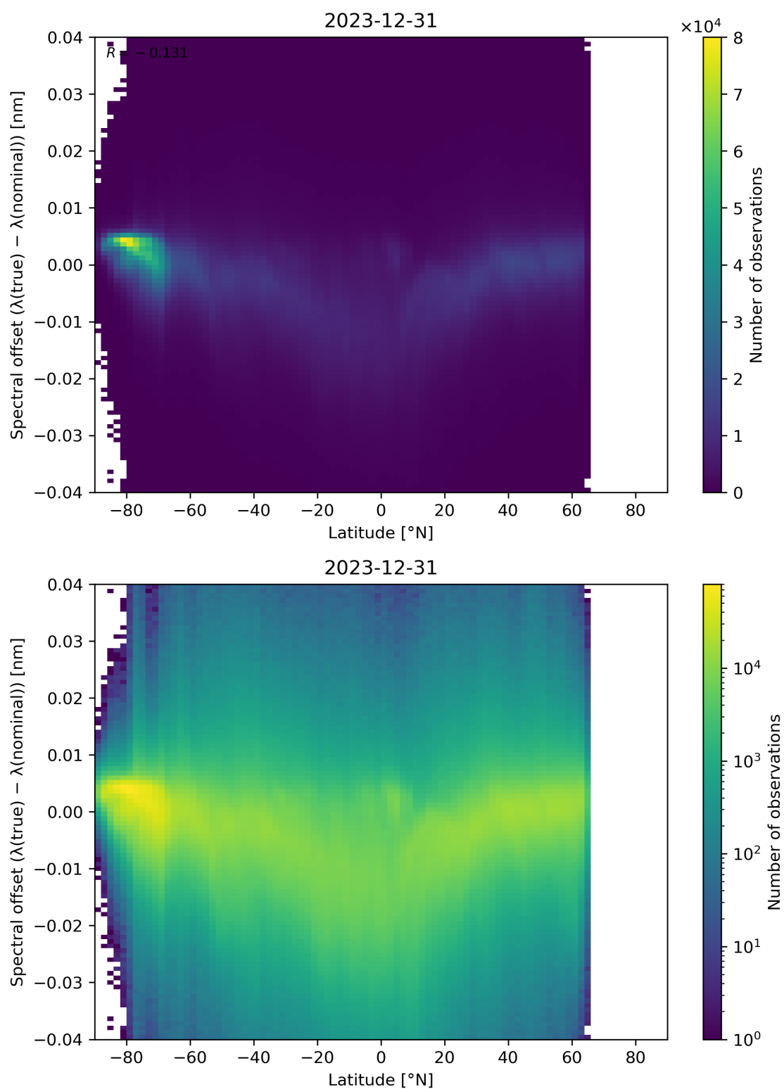
Figure 96: Scatter density plot of “Latitude” against “Spectral offset ( \lambda(\text{true}) - \lambda(\text{nominal}) )” for 2023-12-30 to 2023-12-31.
