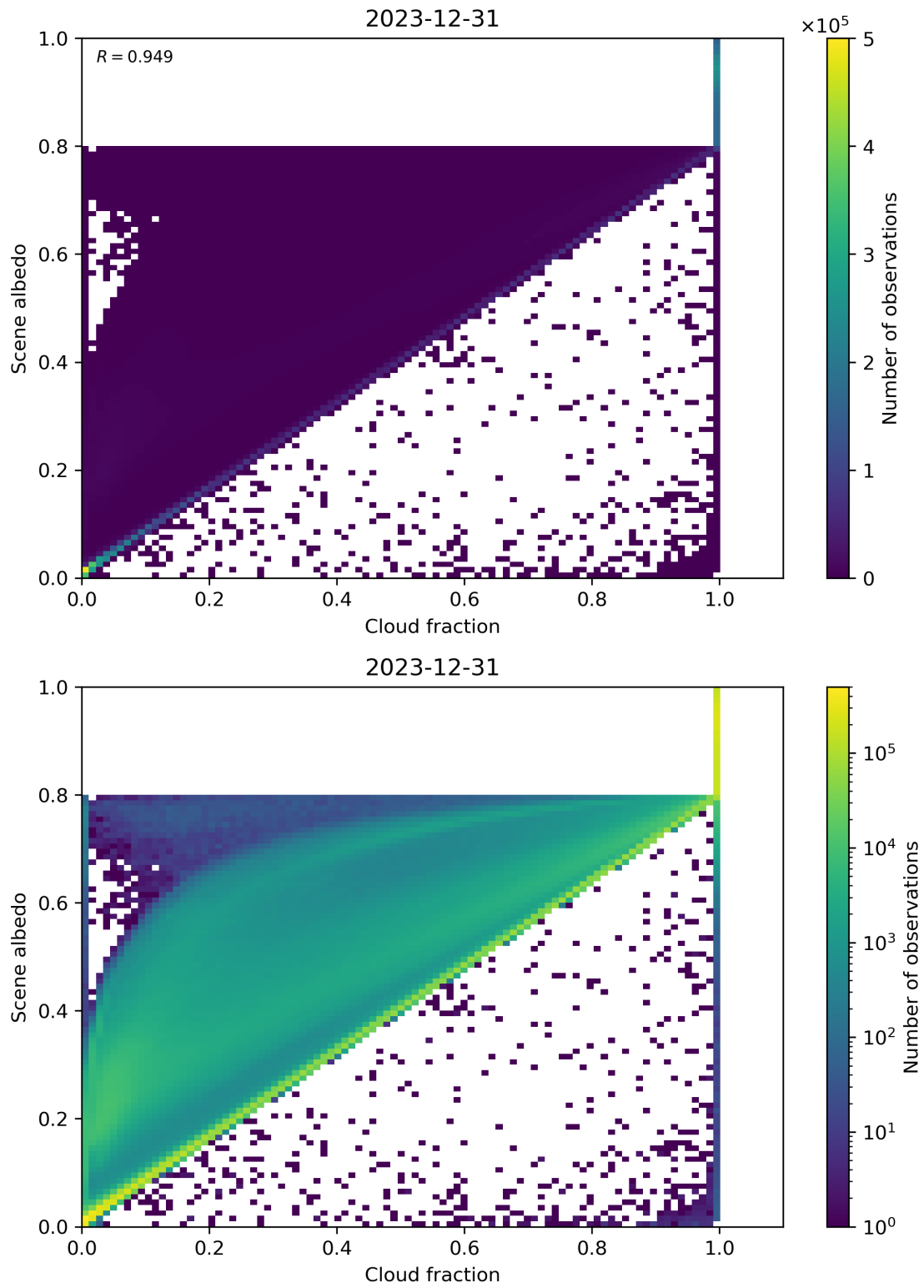
Figure 75: Scatter density plot of “Cloud fraction” against “Scene albedo” for 2023-12-30 to 2023-12-31.
