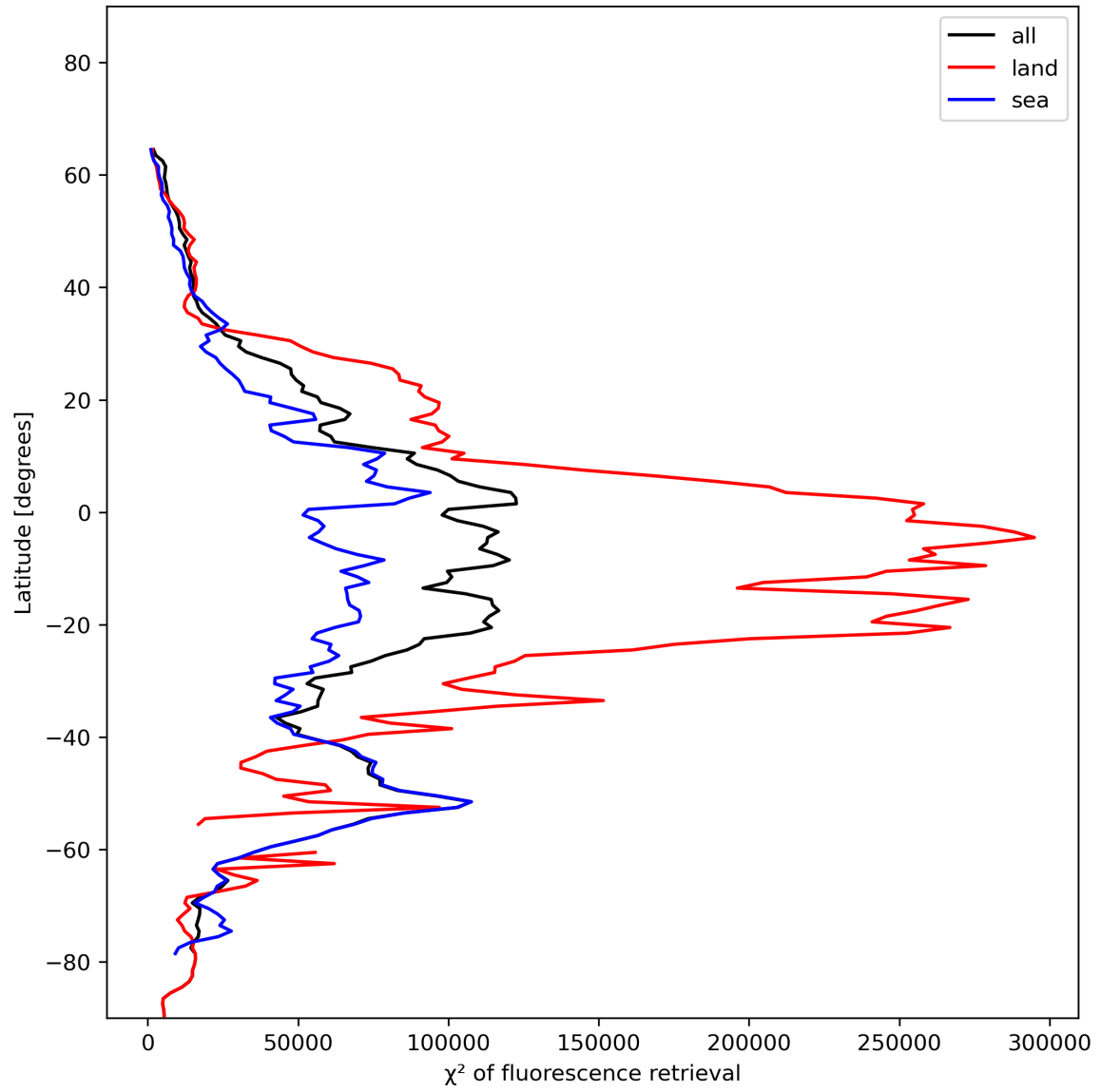
Figure 25: Zonal average of “ \chi^2 of fluorescence retrieval” for 2023-12-30 to 2023-12-31.
