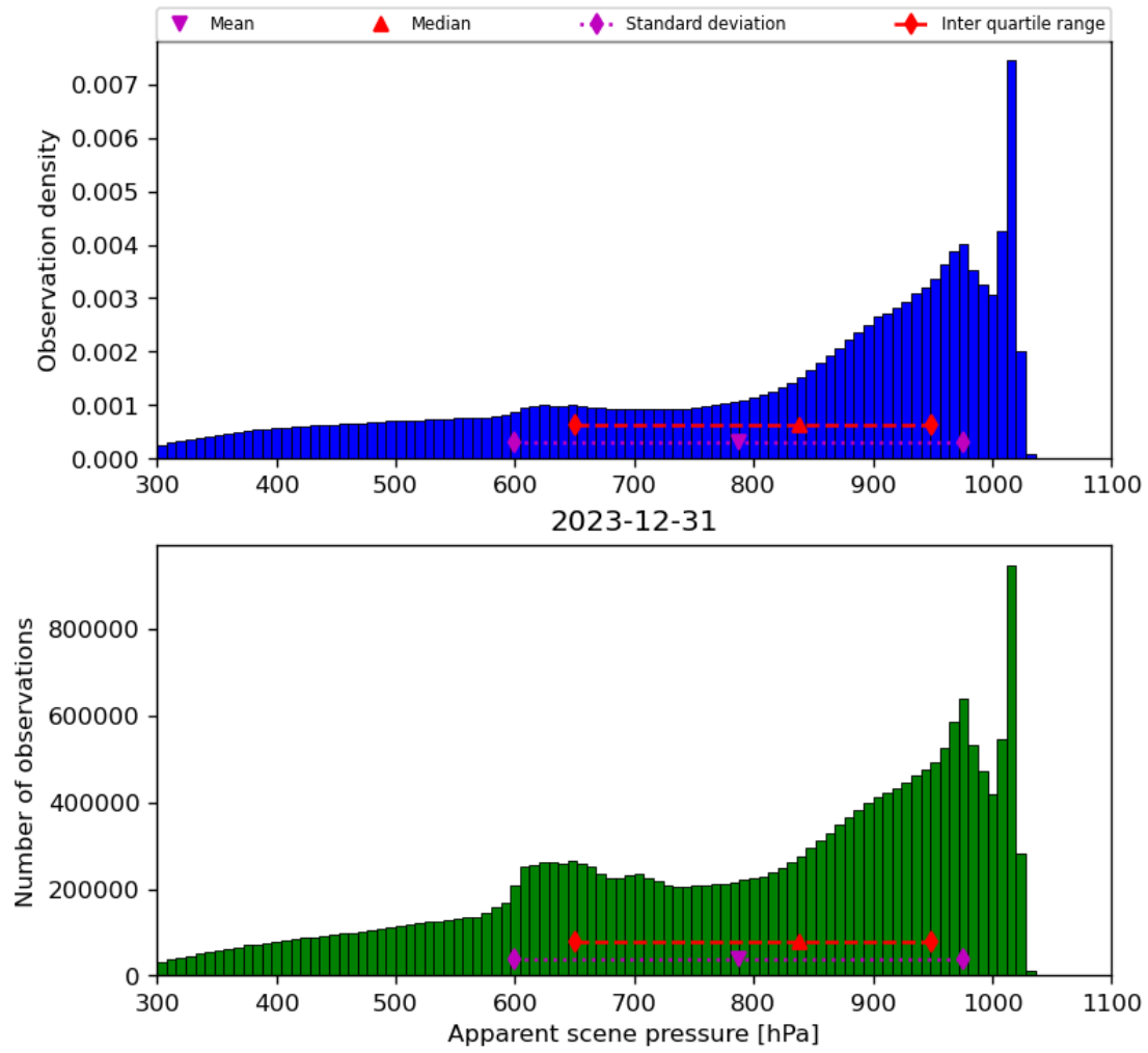
Figure 36: Histogram of “Apparent scene pressure” for 2023-12-30 to 2023-12-31
