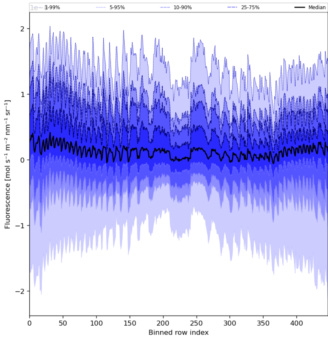
Figure 57: Along track statistics of “Fluorescence” for 2023-12-30 to 2023-12-31
