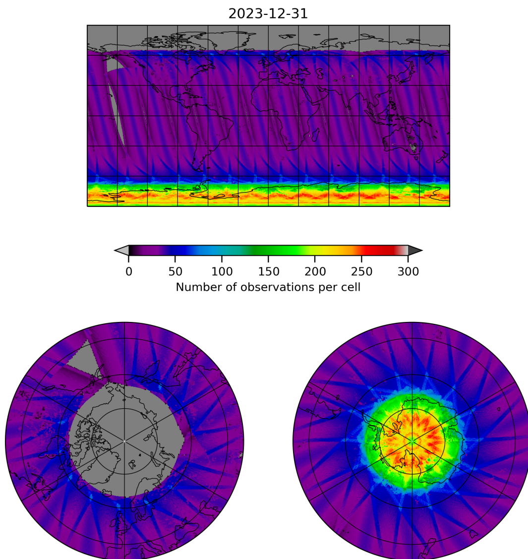
Figure 11: Map of the number of observations for 2023-12-30 to 2023-12-31
