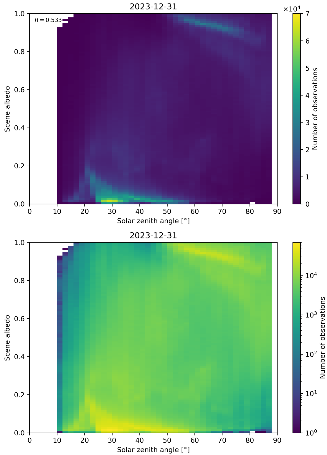
Figure 116: Scatter density plot of “Solar zenith angle” against “Scene albedo” for 2023-12-30 to 2023-12-31.
