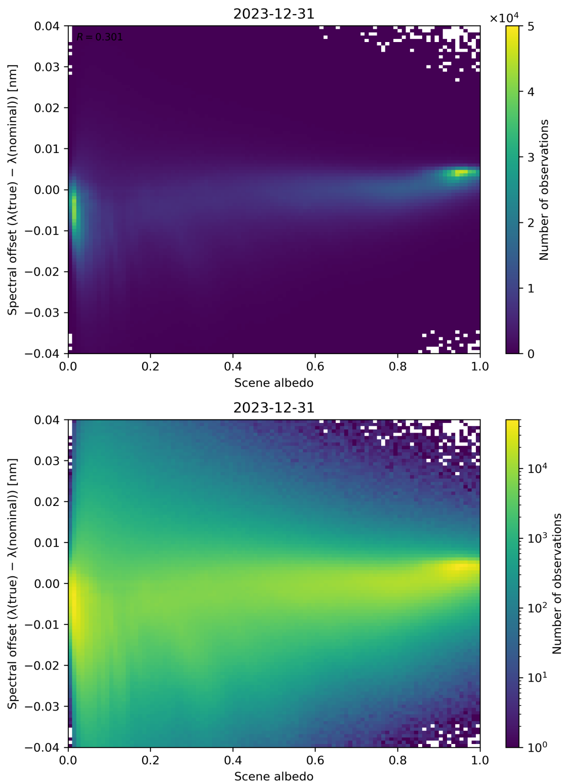
Figure 107: Scatter density plot of “Scene albedo” against “Spectral offset ( \lambda(\text{true}) - \lambda(\text{nominal}) )” for 2023-12-30 to 2023-12-31.
