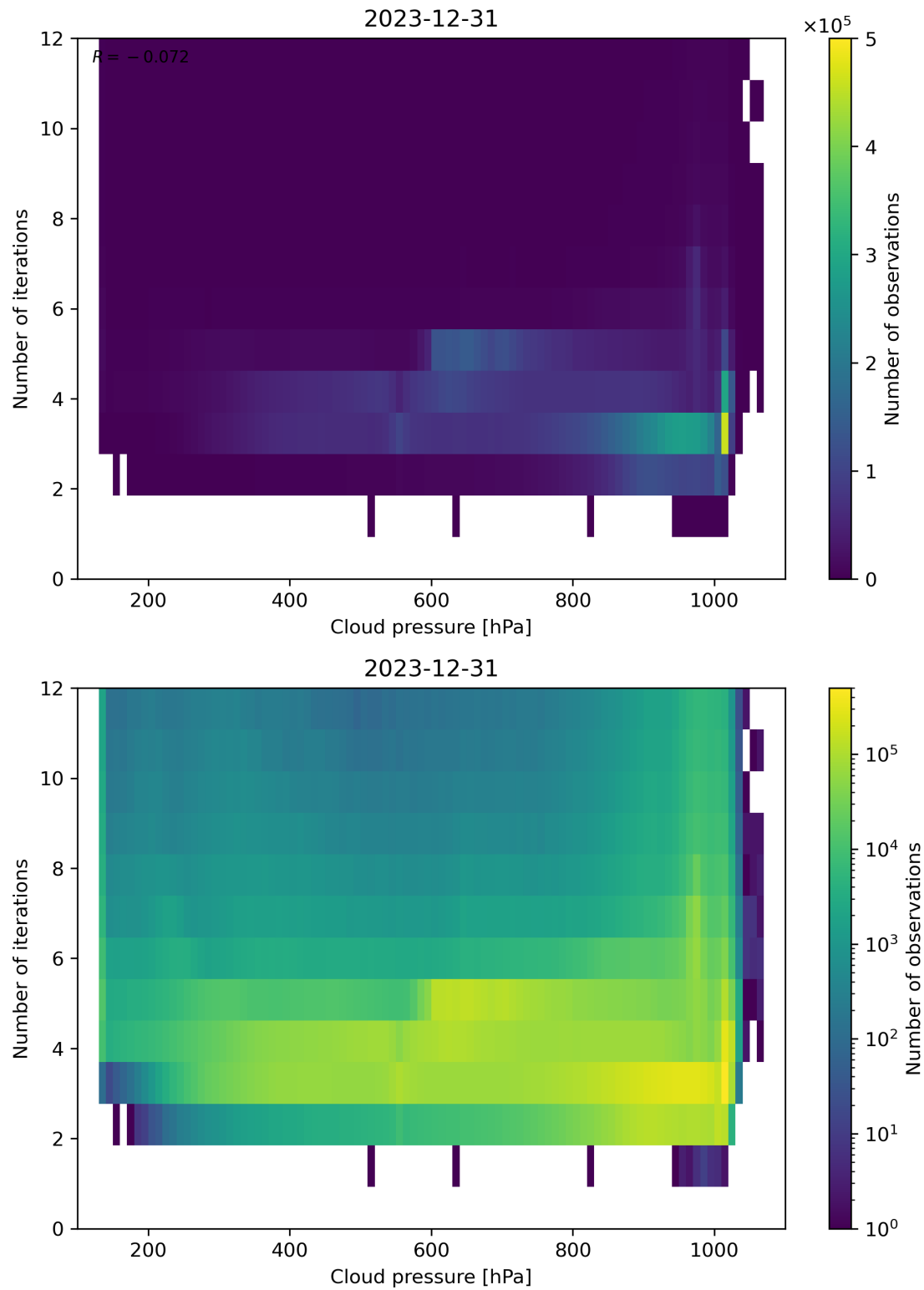
Figure 81: Scatter density plot of “Cloud pressure” against “Number of iterations” for 2023-12-30 to 2023-12-31.
