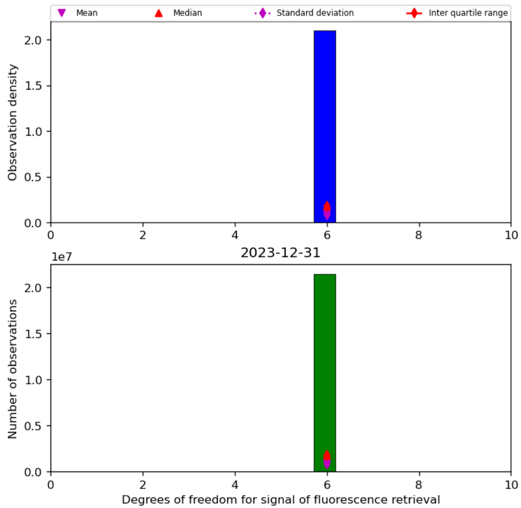
Figure 43: Histogram of “Degrees of freedom for signal of fluorescence retrieval” for 2023-12-30 to 2023-12-31
