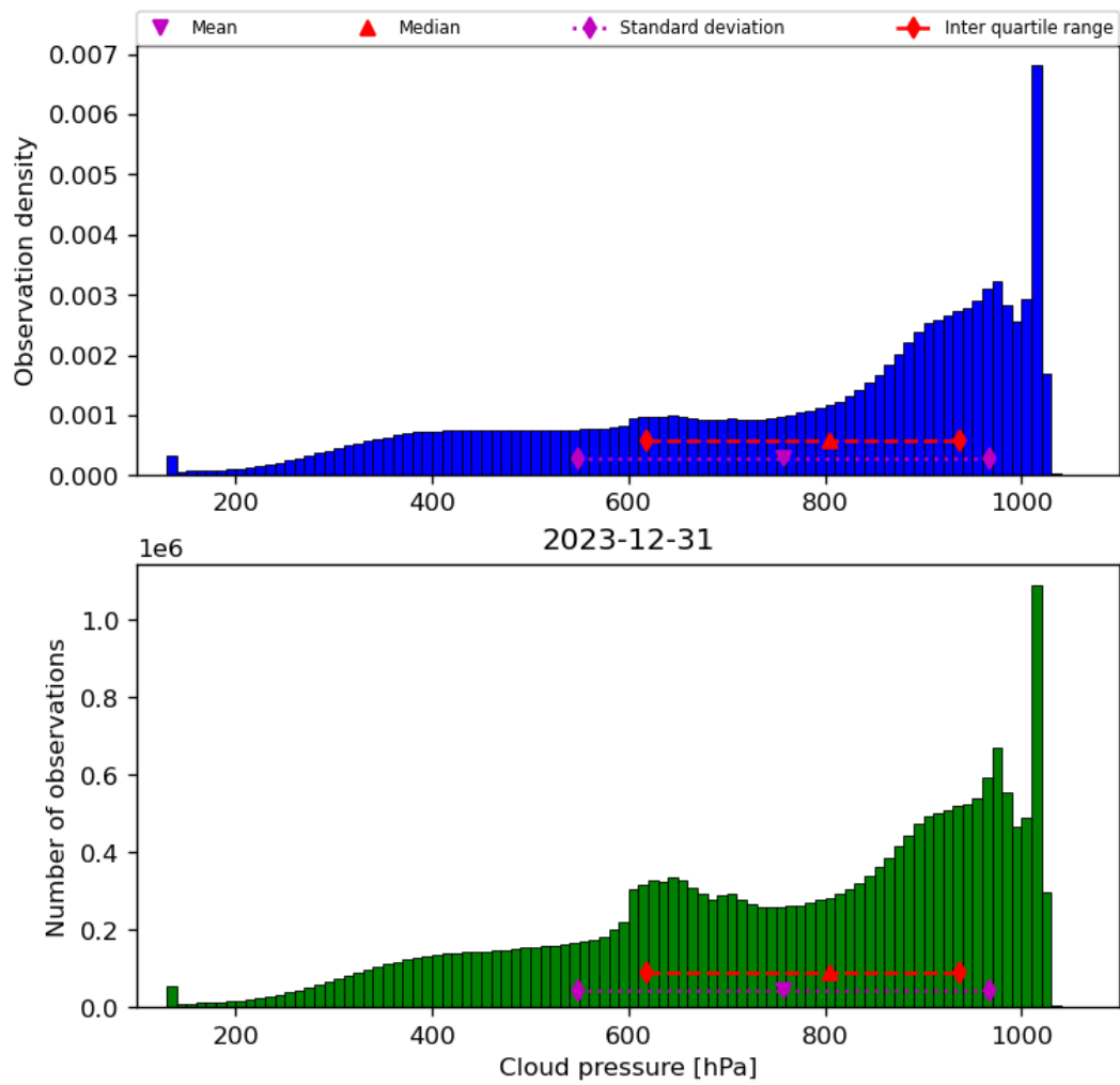
Figure 30: Histogram of “Cloud pressure” for 2023-12-30 to 2023-12-31
