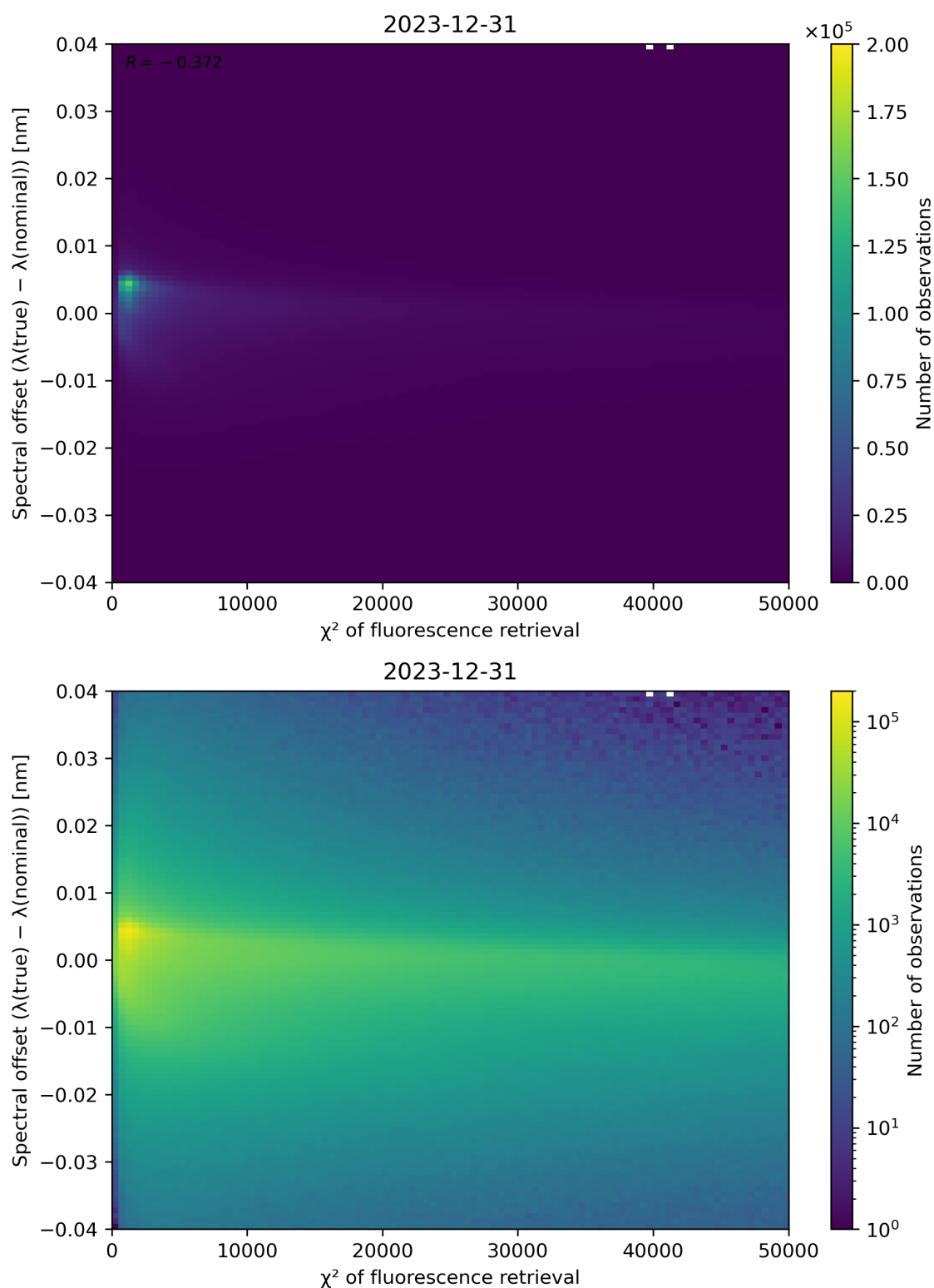
Figure 69: Scatter density plot of " \chi^2 of fluorescence retrieval" against "Spectral offset ( \lambda(\text{true}) - \lambda(\text{nominal}) )" for 2023-12-30 to 2023-12-31.
