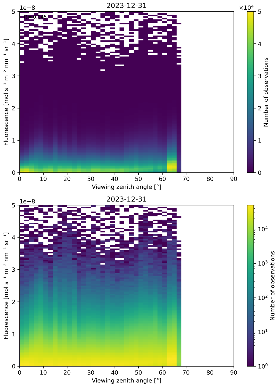
Figure 122: Scatter density plot of “Viewing zenith angle” against “Fluorescence” for 2023-12-30 to 2023-12-31.
