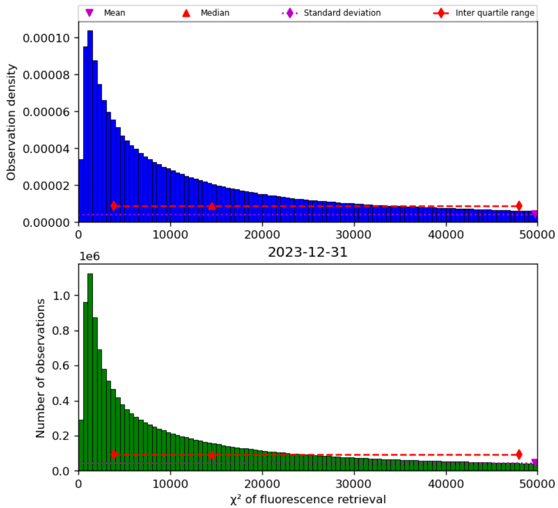
Figure 42: Histogram of “ \chi^2 of fluorescence retrieval” for 2023-12-30 to 2023-12-31
