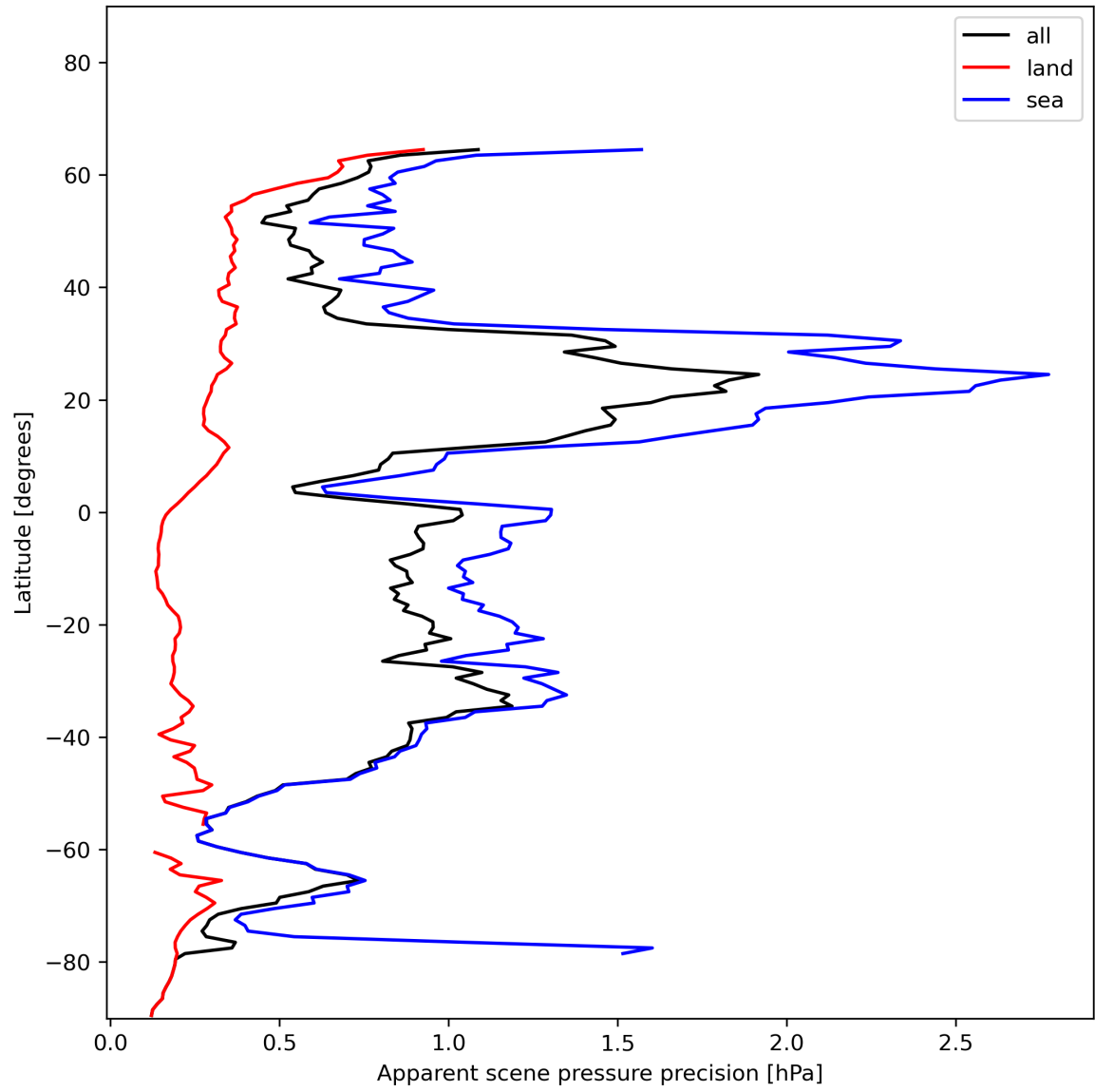
Figure 20: Zonal average of “Apparent scene pressure precision” for 2023-12-30 to 2023-12-31.
