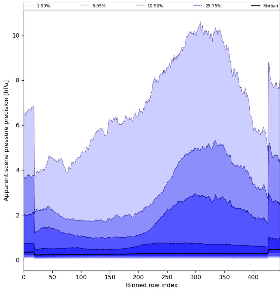
Figure 54: Along track statistics of “Apparent scene pressure precision” for 2023-12-30 to 2023-12-31
