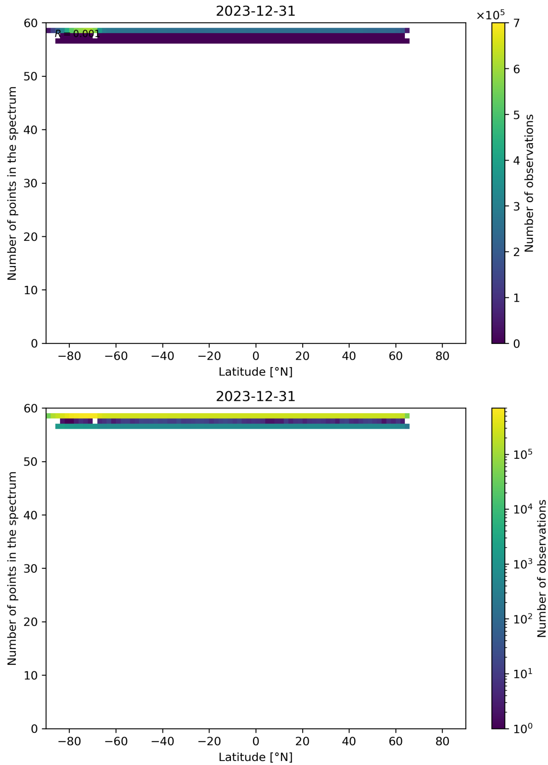
Figure 94: Scatter density plot of “Latitude” against “Number of points in the spectrum” for 2023-12-30 to 2023-12-31.
