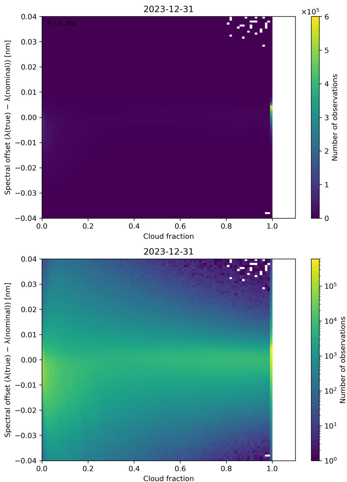
Figure 76: Scatter density plot of “Cloud fraction” against “Spectral offset ( \lambda(\text{true}) - \lambda(\text{nominal}) )” for 2023-12-30 to 2023-12-31.
