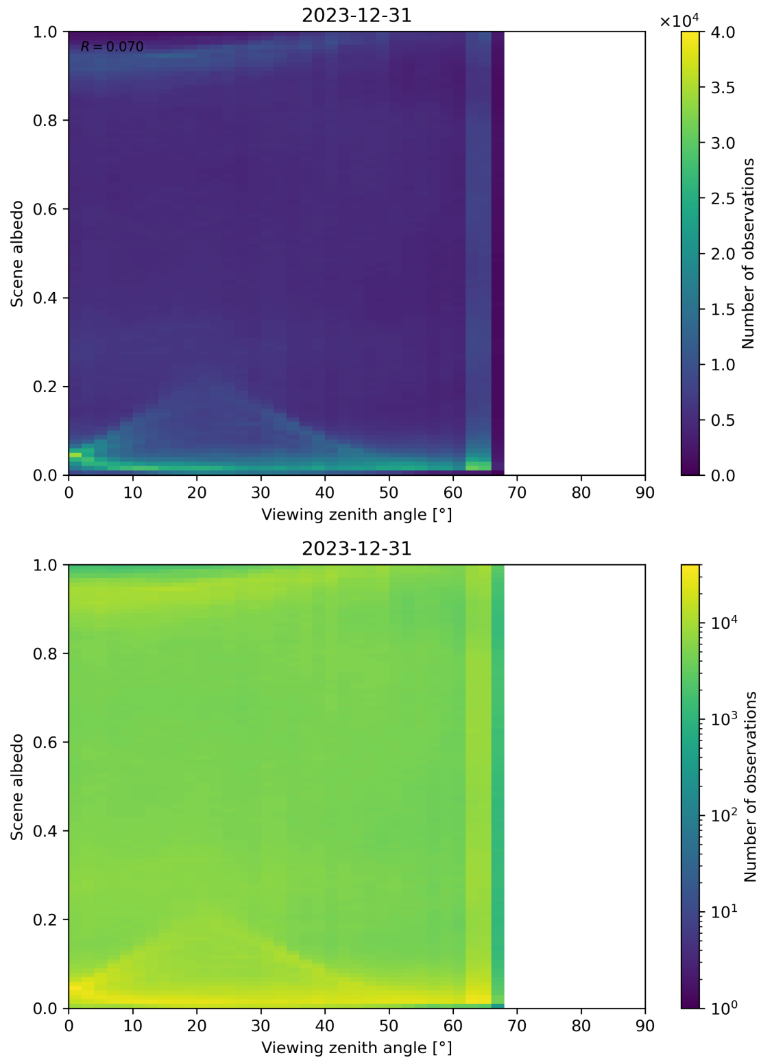
Figure 126: Scatter density plot of “Viewing zenith angle” against “Scene albedo” for 2023-12-30 to 2023-12-31.
