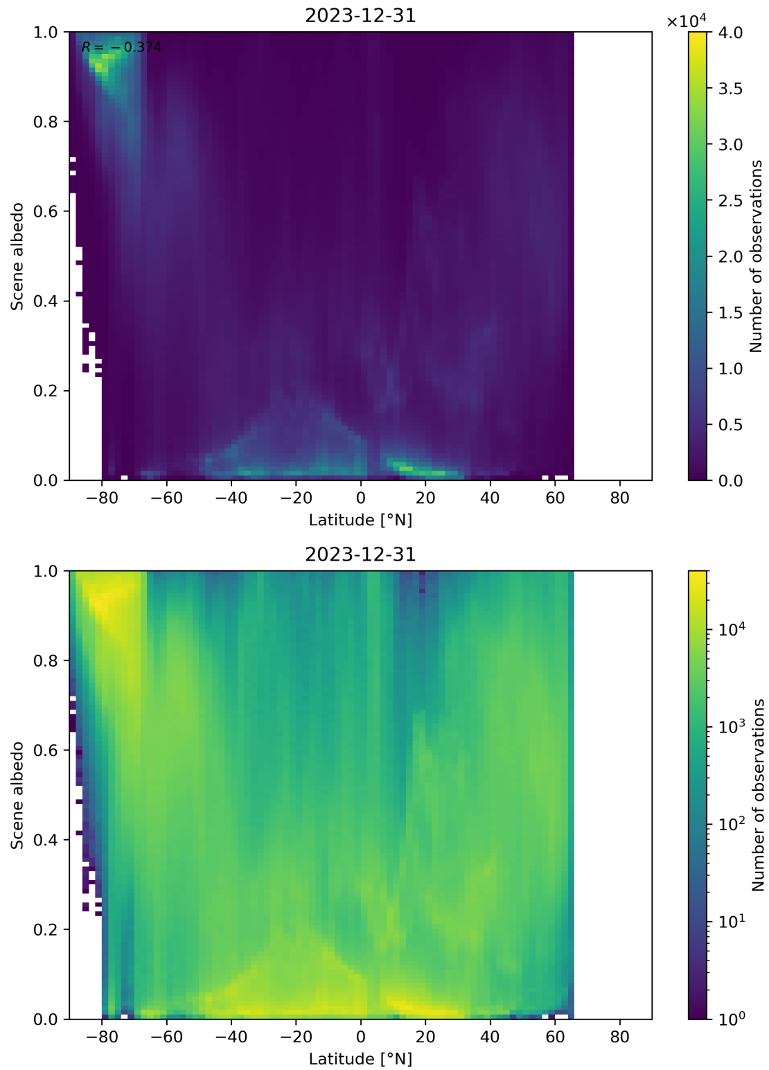
Figure 95: Scatter density plot of “Latitude” against “Scene albedo” for 2023-12-30 to 2023-12-31.
