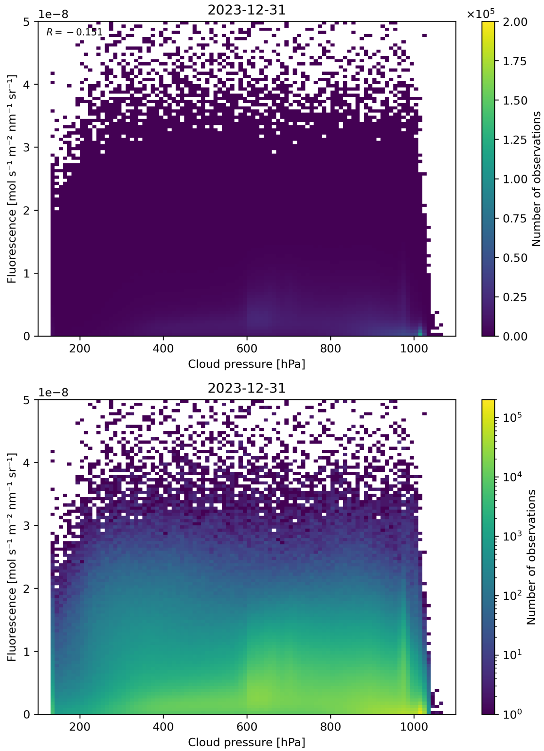
Figure 80: Scatter density plot of “Cloud pressure” against “Fluorescence” for 2023-12-30 to 2023-12-31.
