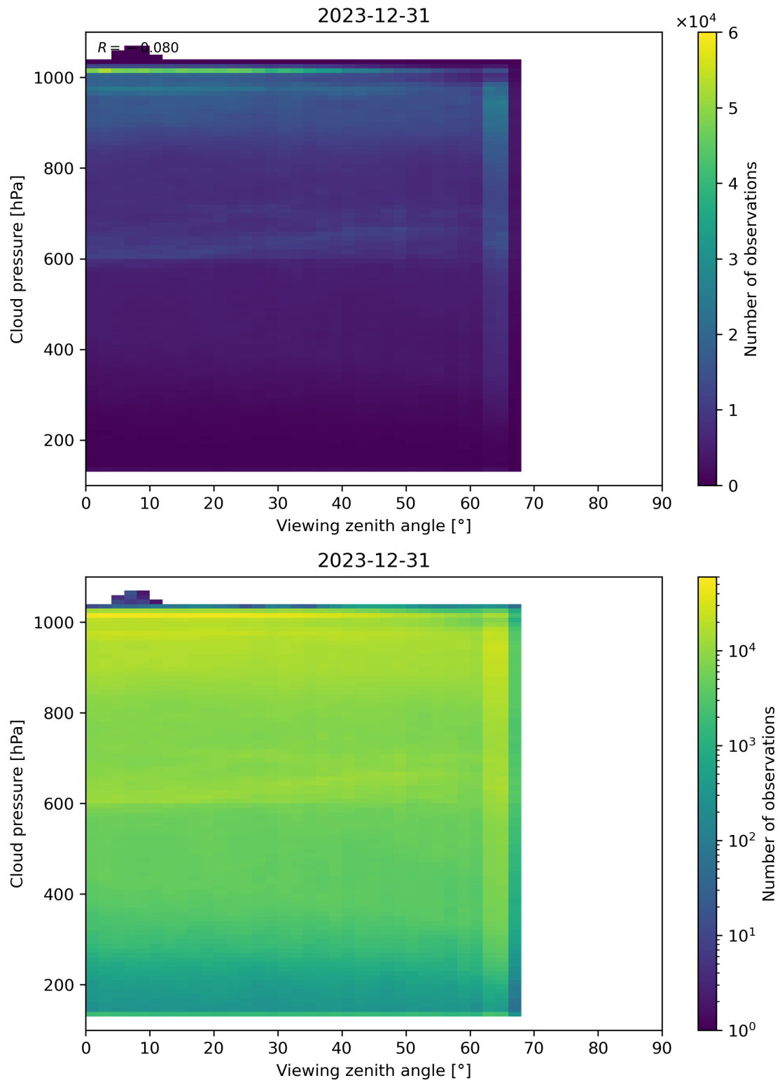
Figure 121: Scatter density plot of “Viewing zenith angle” against “Cloud pressure” for 2023-12-30 to 2023-12-31.
