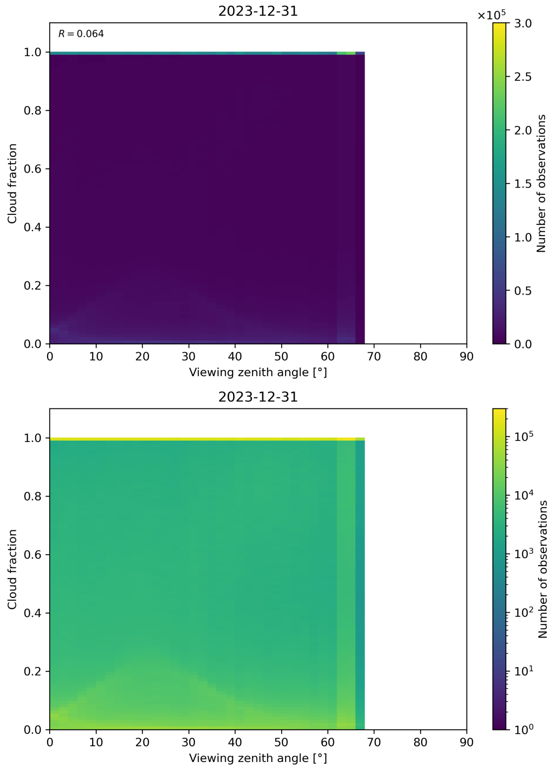
Figure 120: Scatter density plot of “Viewing zenith angle” against “Cloud fraction” for 2023-12-30 to 2023-12-31.
