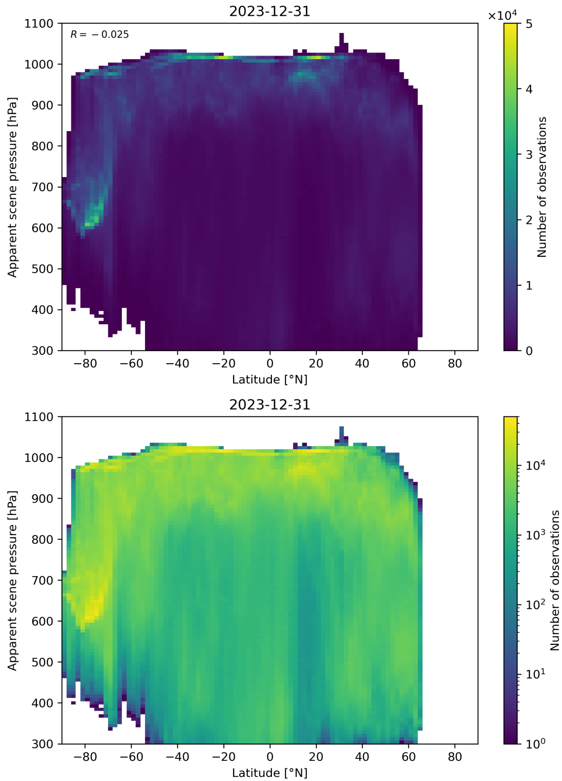
Figure 88: Scatter density plot of “Latitude” against “Apparent scene pressure” for 2023-12-30 to 2023-12-31.
