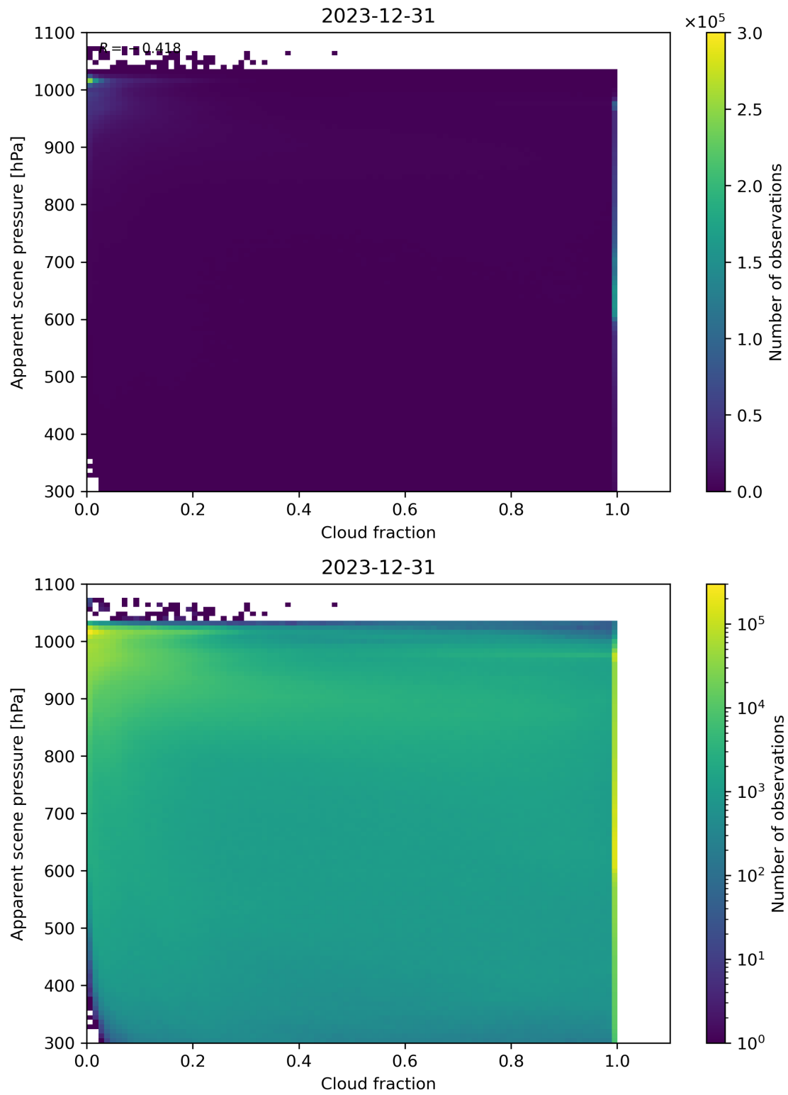
Figure 70: Scatter density plot of “Cloud fraction” against “Apparent scene pressure” for 2023-12-30 to 2023-12-31.
