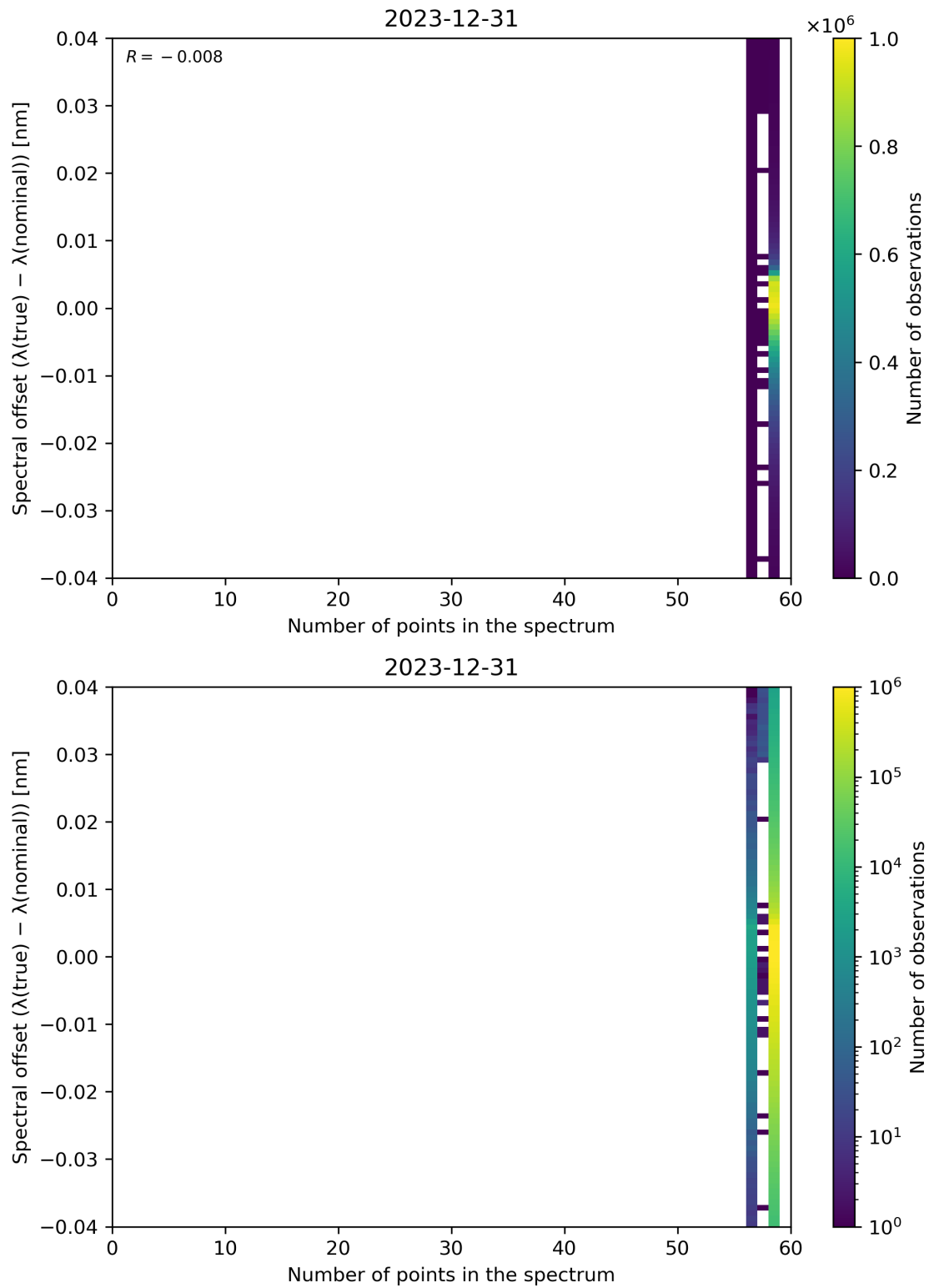
Figure 101: Scatter density plot of “Number of points in the spectrum” against “Spectral offset ( \lambda(\text{true}) - \lambda(\text{nominal}) )” for 2023-12-30 to 2023-12-31.
