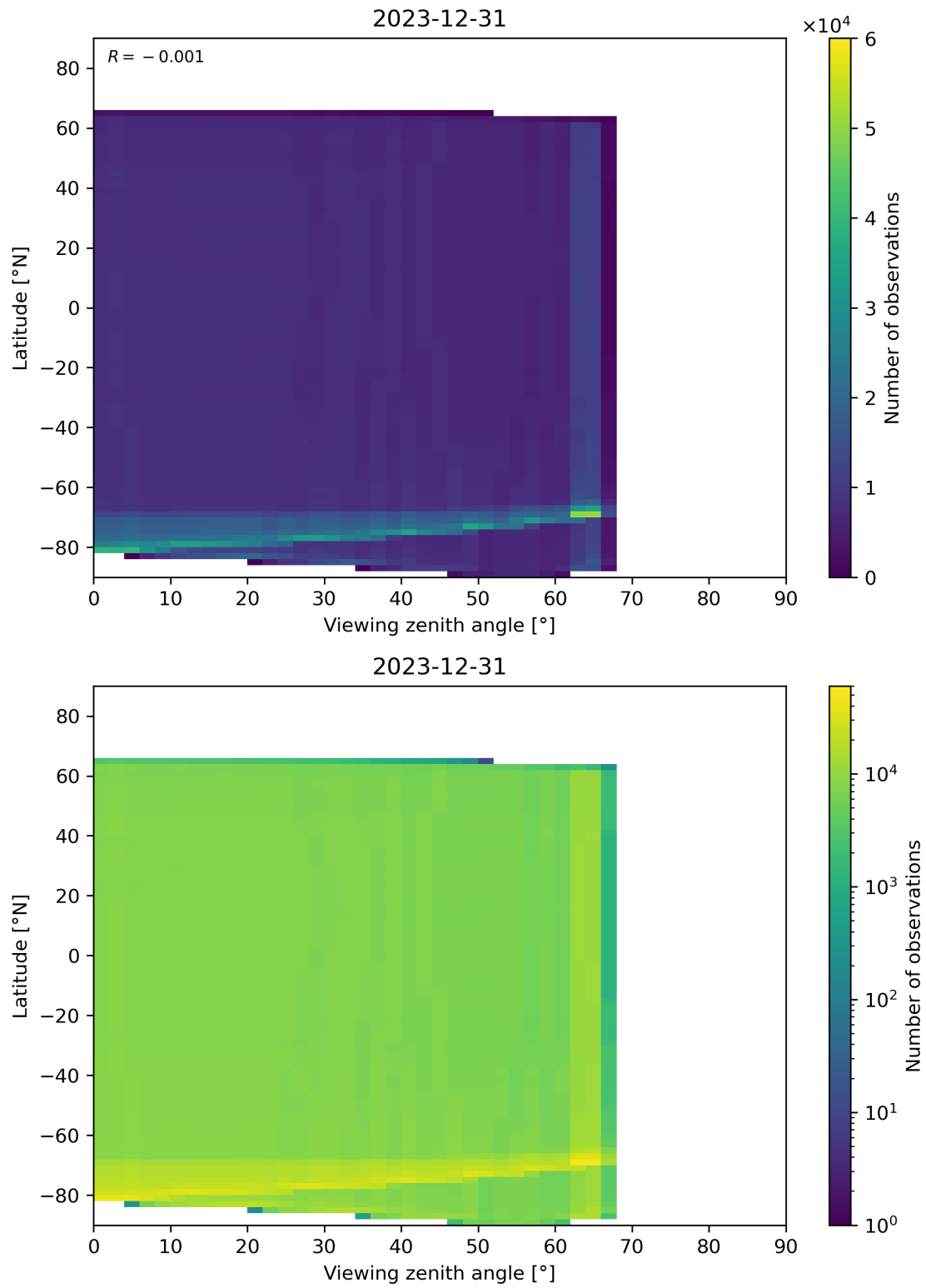
Figure 123: Scatter density plot of “Viewing zenith angle” against “Latitude” for 2023-12-30 to 2023-12-31.
