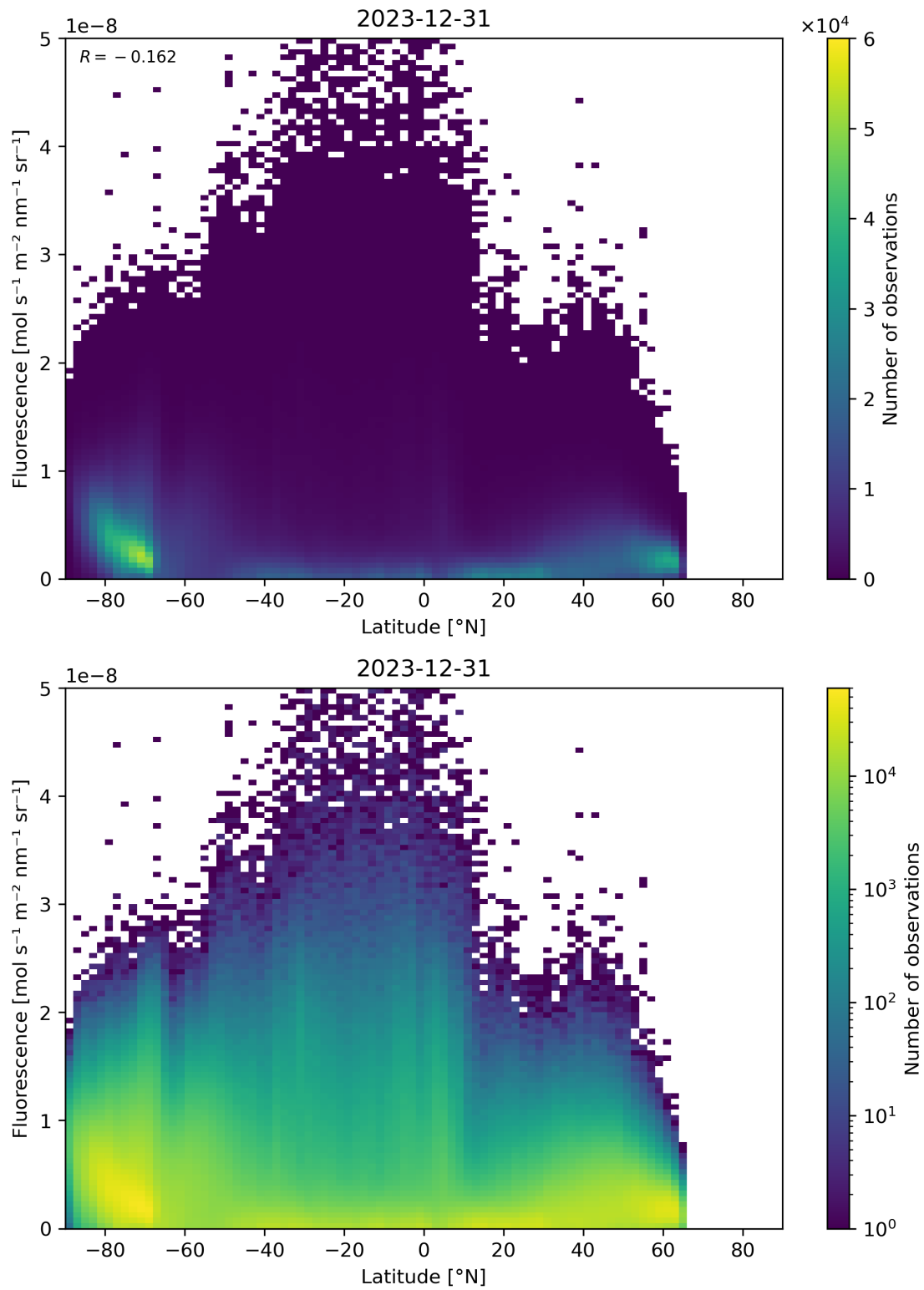
Figure 92: Scatter density plot of “Latitude” against “Fluorescence” for 2023-12-30 to 2023-12-31.
