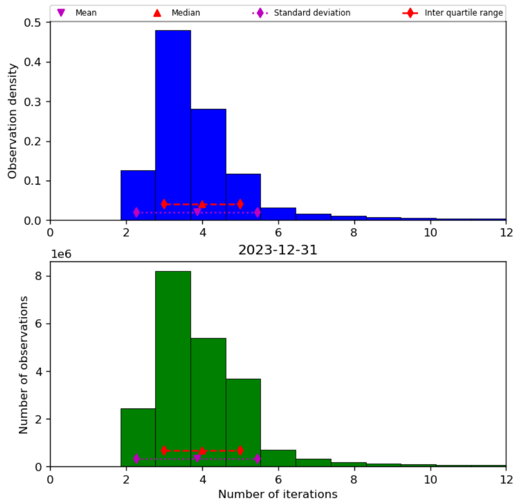
Figure 39: Histogram of “Number of iterations” for 2023-12-30 to 2023-12-31
