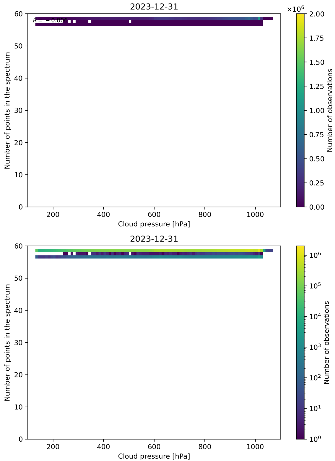
Figure 82: Scatter density plot of “Cloud pressure” against “Number of points in the spectrum” for 2023-12-30 to 2023-12-31.
