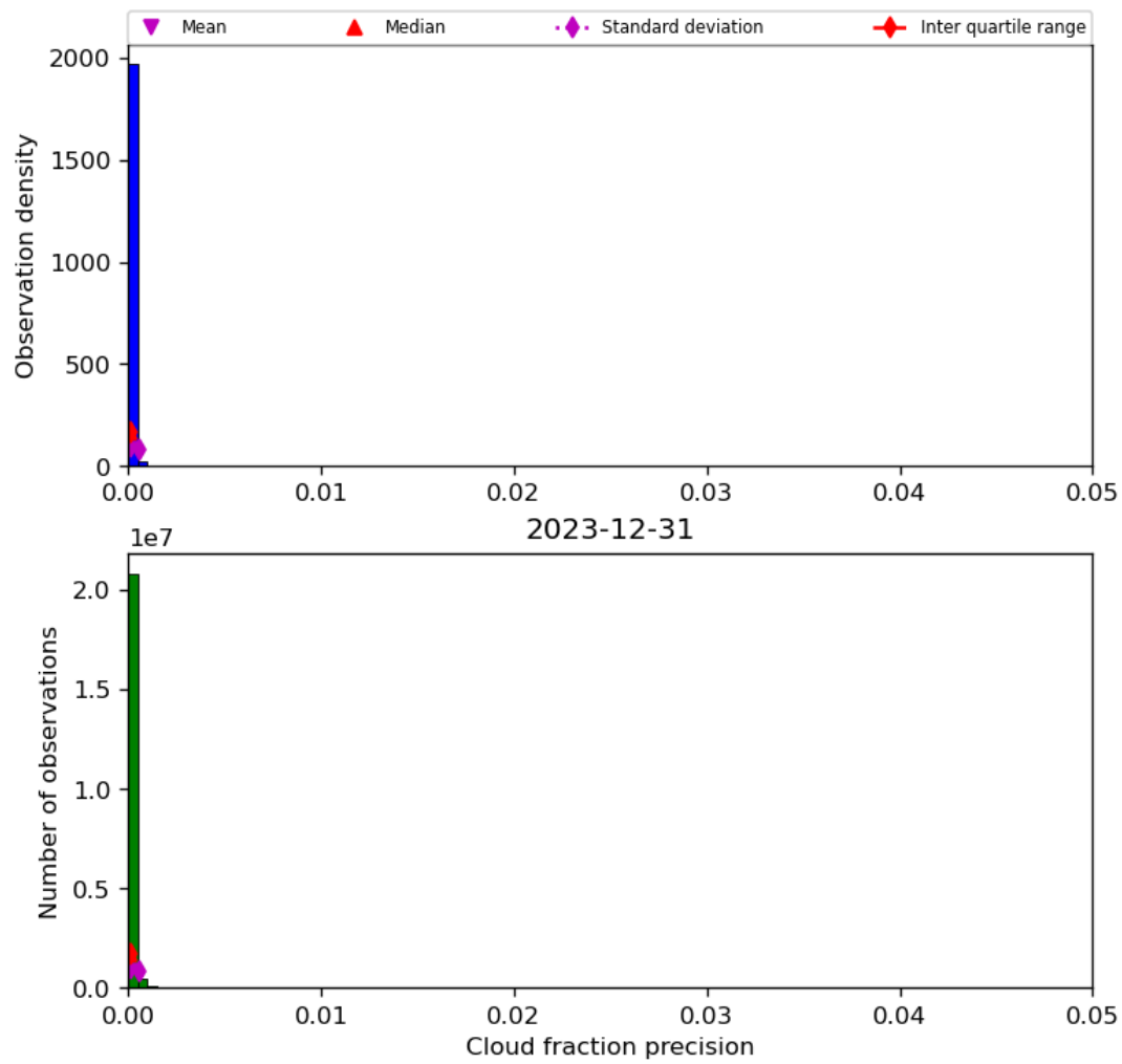
Figure 33: Histogram of “Cloud fraction precision” for 2023-12-30 to 2023-12-31
