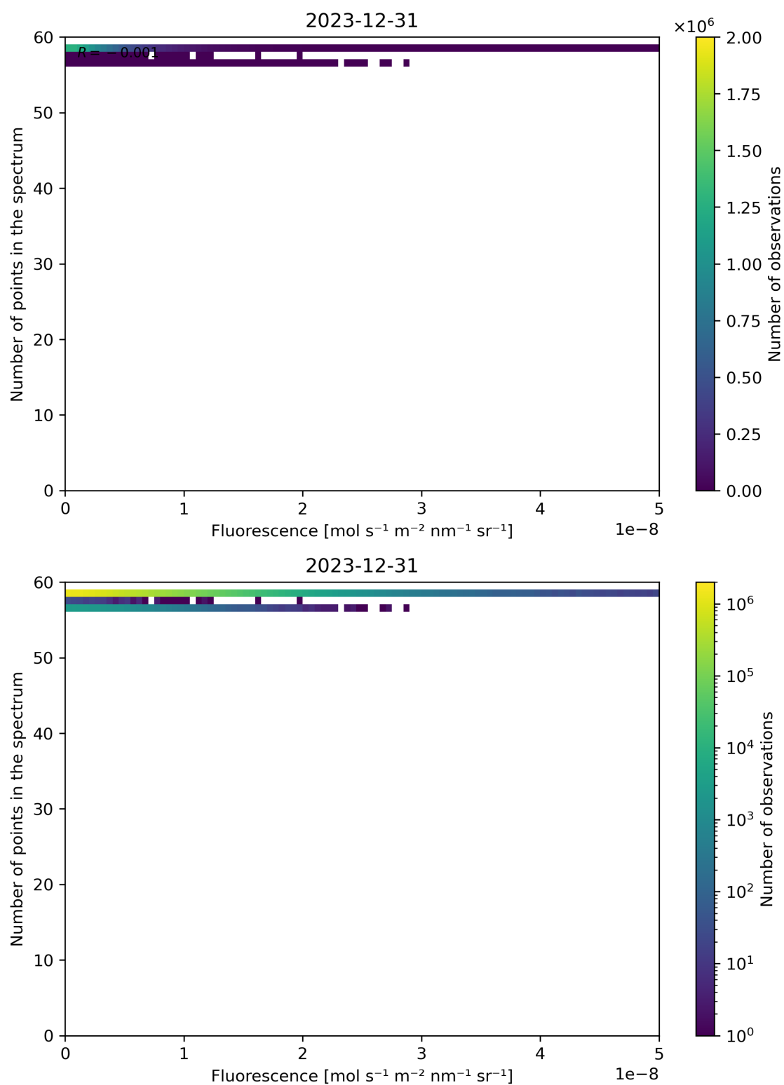
Figure 86: Scatter density plot of “Fluorescence” against “Number of points in the spectrum” for 2023-12-30 to 2023-12-31.
