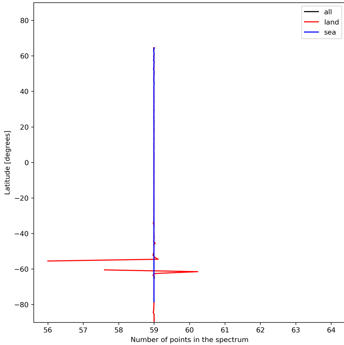
Figure 27: Zonal average of “Number of points in the spectrum” for 2023-12-30 to 2023-12-31.
