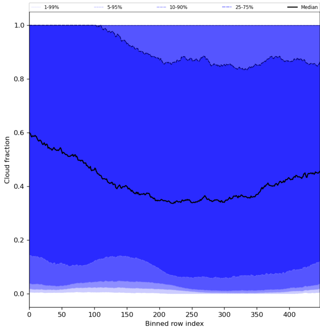
Figure 49: Along track statistics of “Cloud fraction” for 2023-12-30 to 2023-12-31
