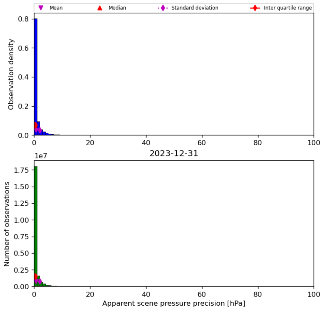
Figure 37: Histogram of “Apparent scene pressure precision” for 2023-12-30 to 2023-12-31
