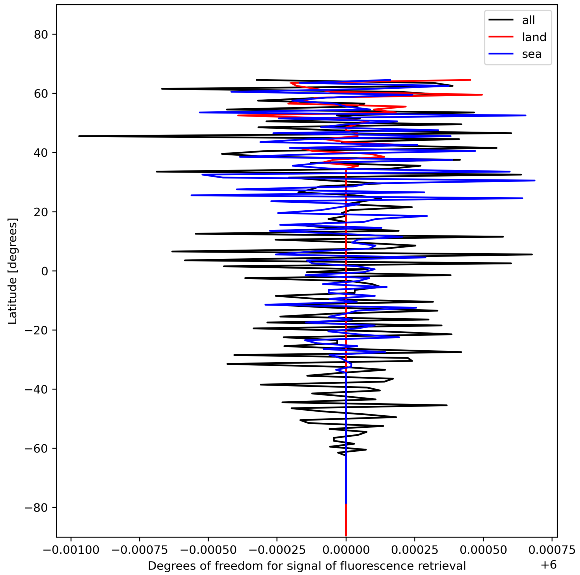
Figure 26: Zonal average of “Degrees of freedom for signal of fluorescence retrieval” for 2023-12-30 to 2023-12-31.
