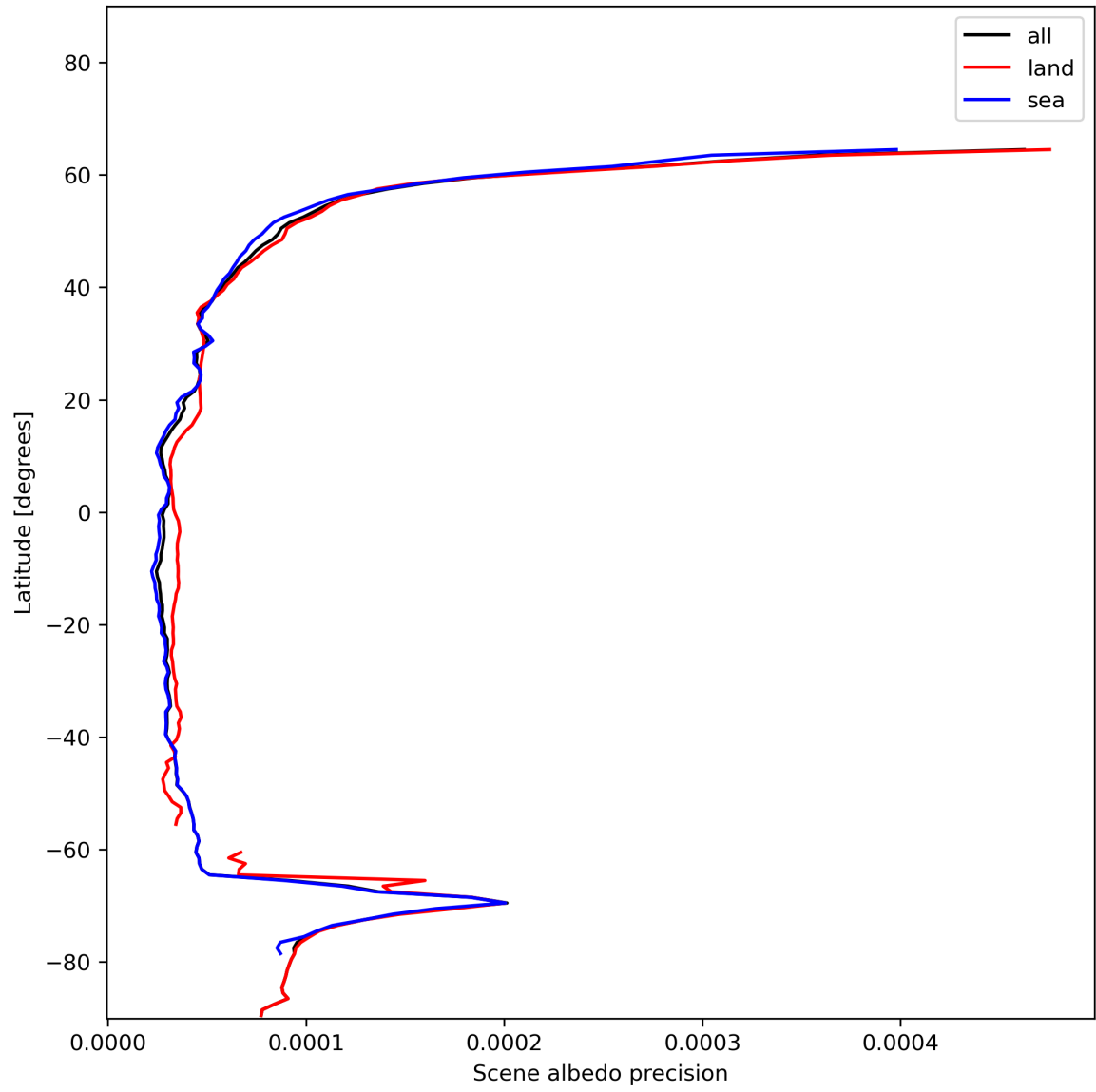
Figure 18: Zonal average of “Scene albedo precision” for 2023-12-30 to 2023-12-31.
