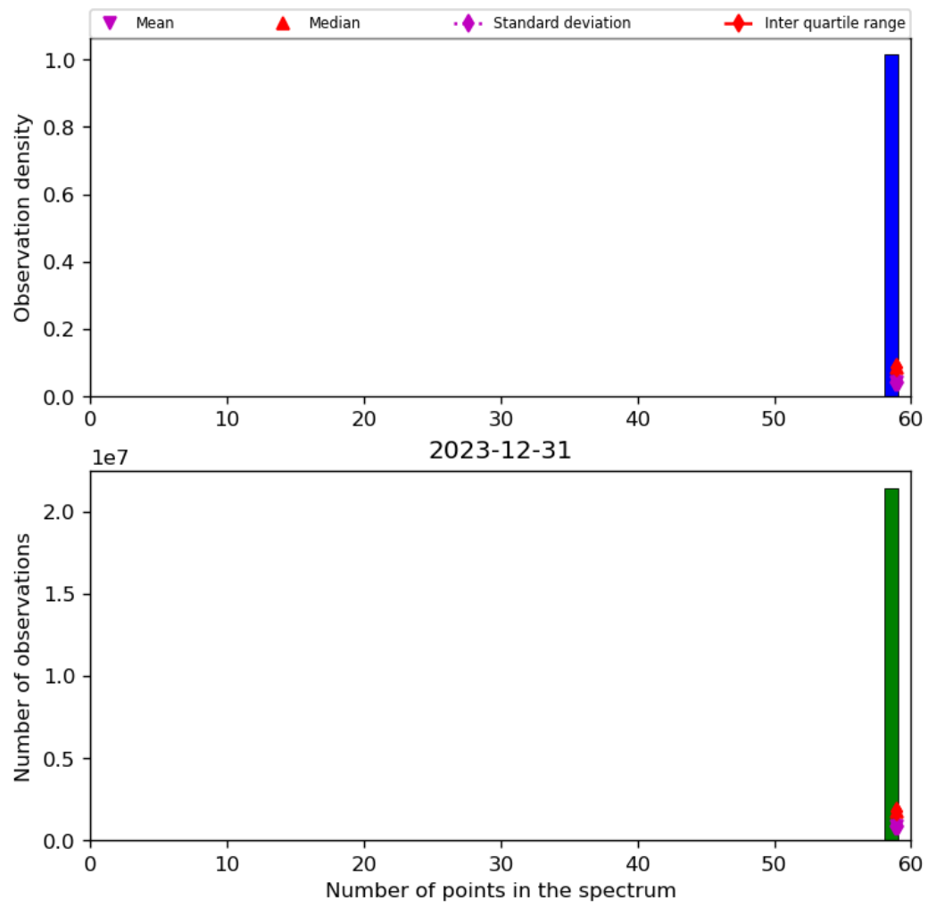
Figure 44: Histogram of “Number of points in the spectrum” for 2023-12-30 to 2023-12-31
