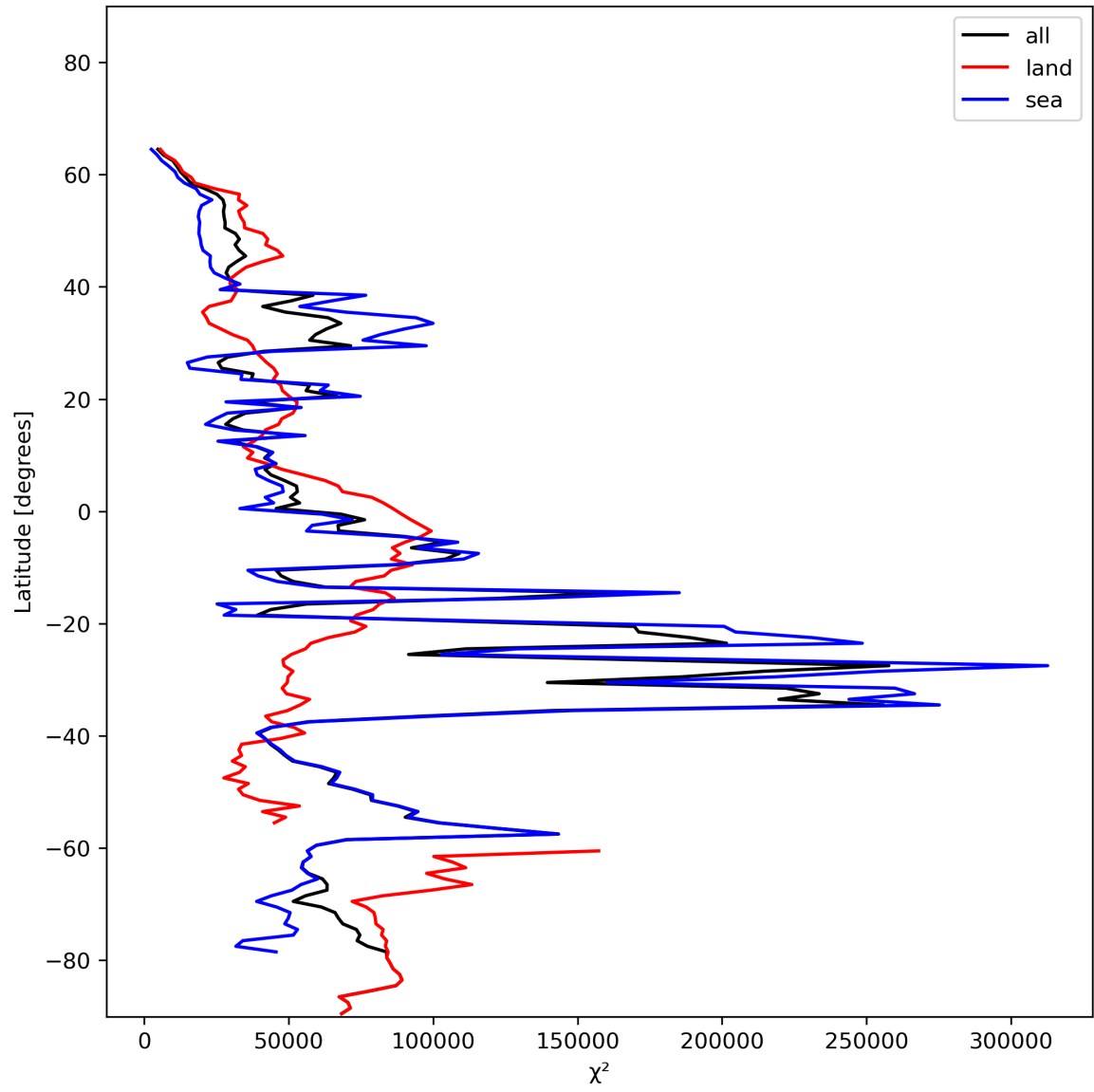
Figure 21: Zonal average of “ \chi^2 ” for 2023-12-30 to 2023-12-31.
