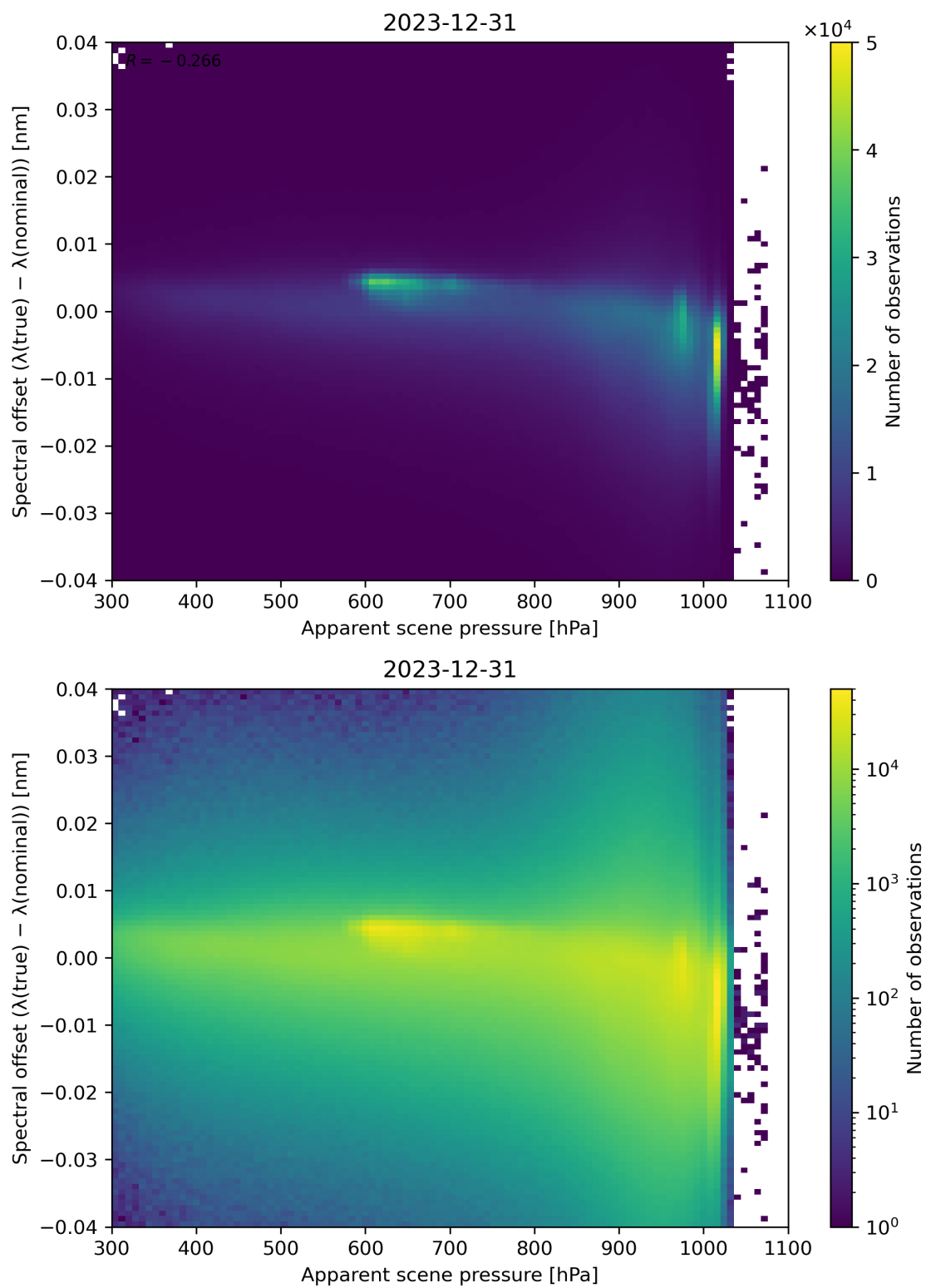
Figure 67: Scatter density plot of “Apparent scene pressure” against “Spectral offset ( \lambda(\text{true}) - \lambda(\text{nominal}) )” for 2023-12-30 to 2023-12-31.
