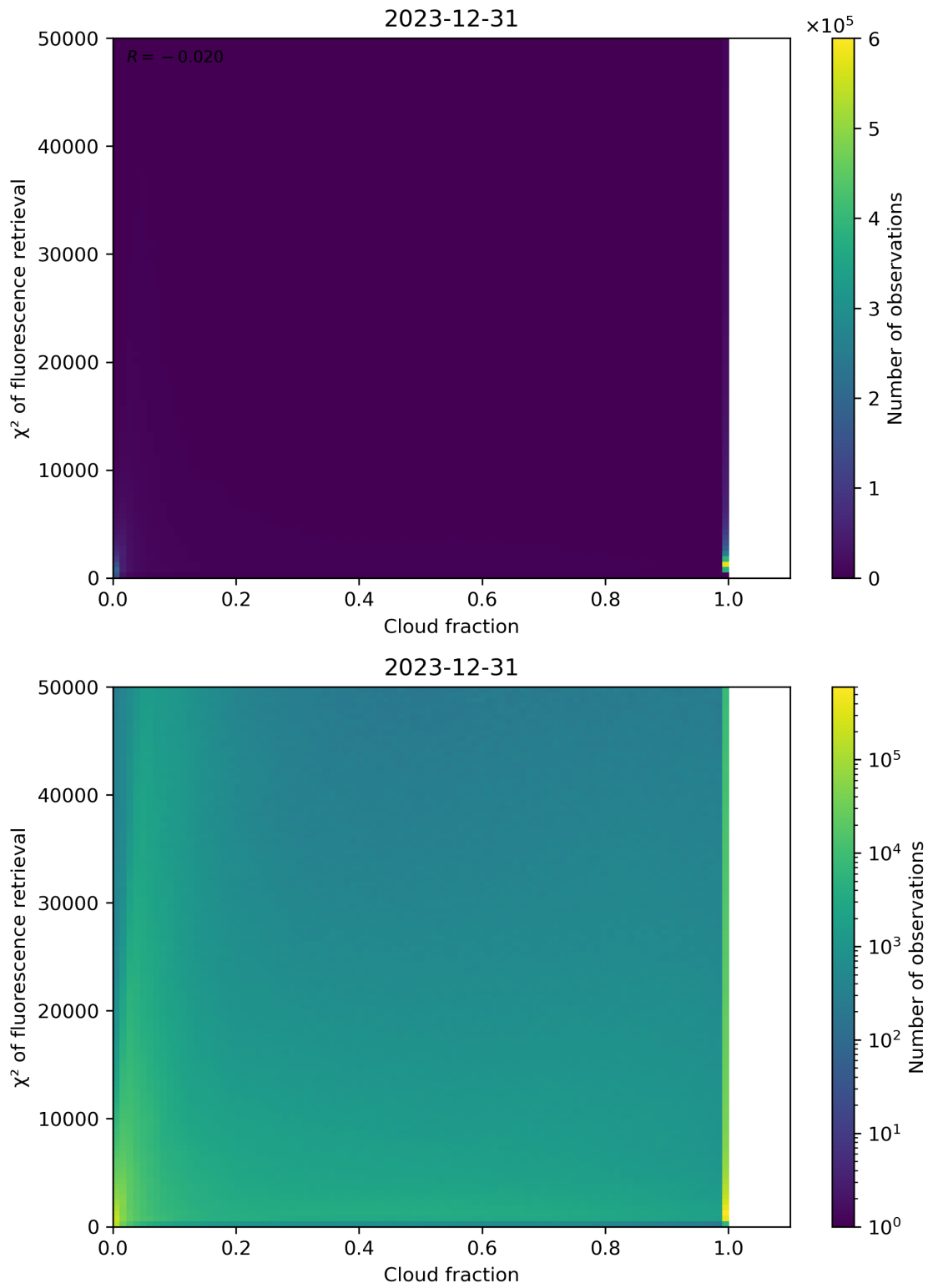
Figure 71: Scatter density plot of “Cloud fraction” against “ \chi^2 of fluorescence retrieval” for 2023-12-30 to 2023-12-31.
