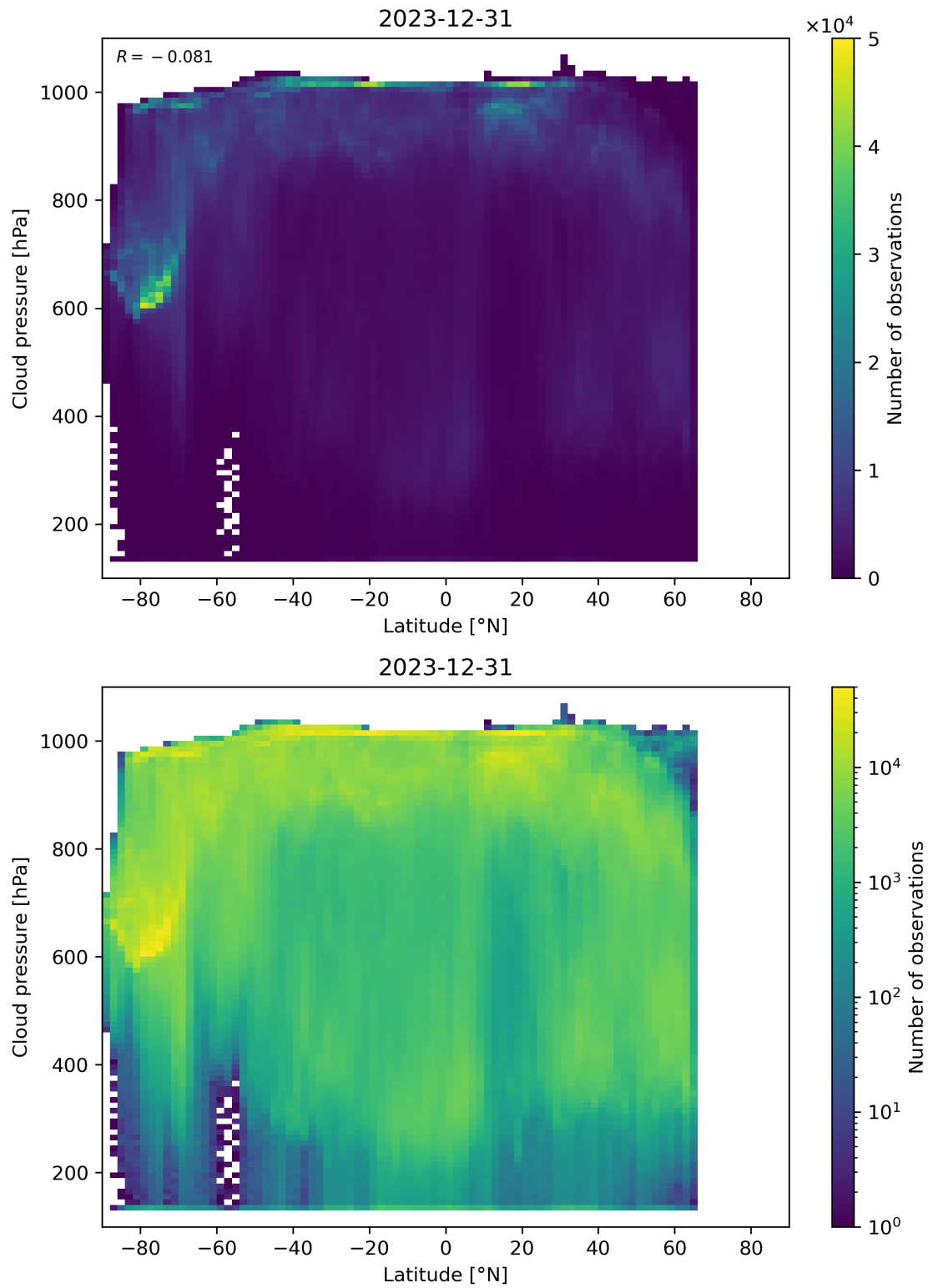
Figure 91: Scatter density plot of “Latitude” against “Cloud pressure” for 2023-12-30 to 2023-12-31.
