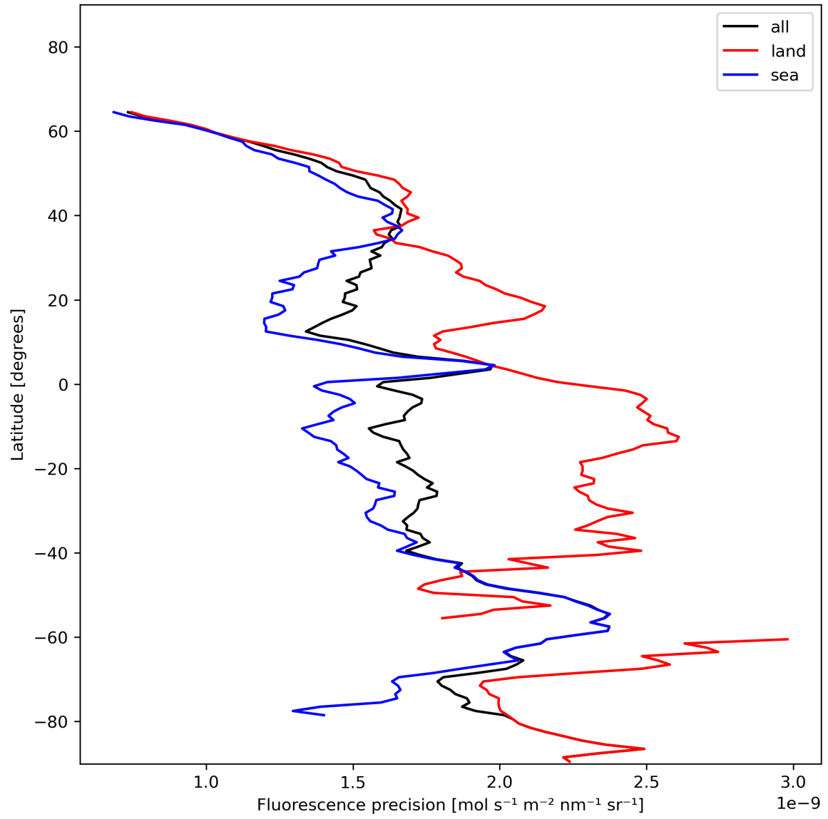
Figure 24: Zonal average of “Fluorescence precision” for 2023-12-30 to 2023-12-31.
