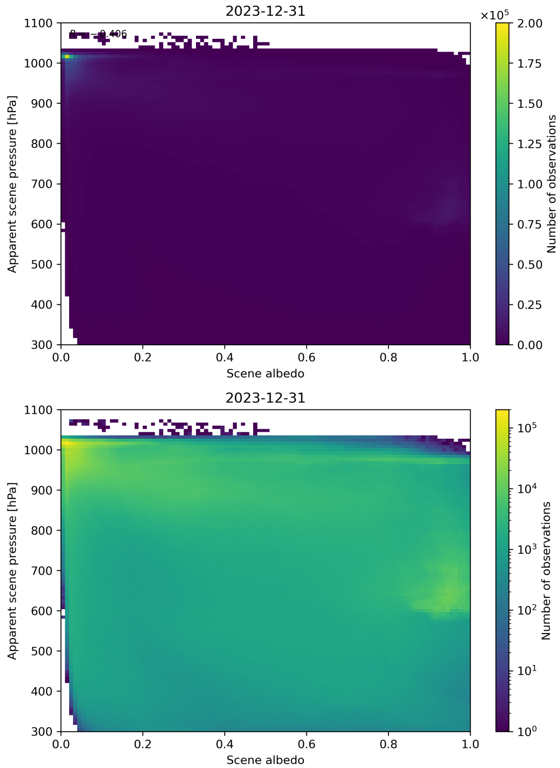
Figure 102: Scatter density plot of “Scene albedo” against “Apparent scene pressure” for 2023-12-30 to 2023-12-31.
