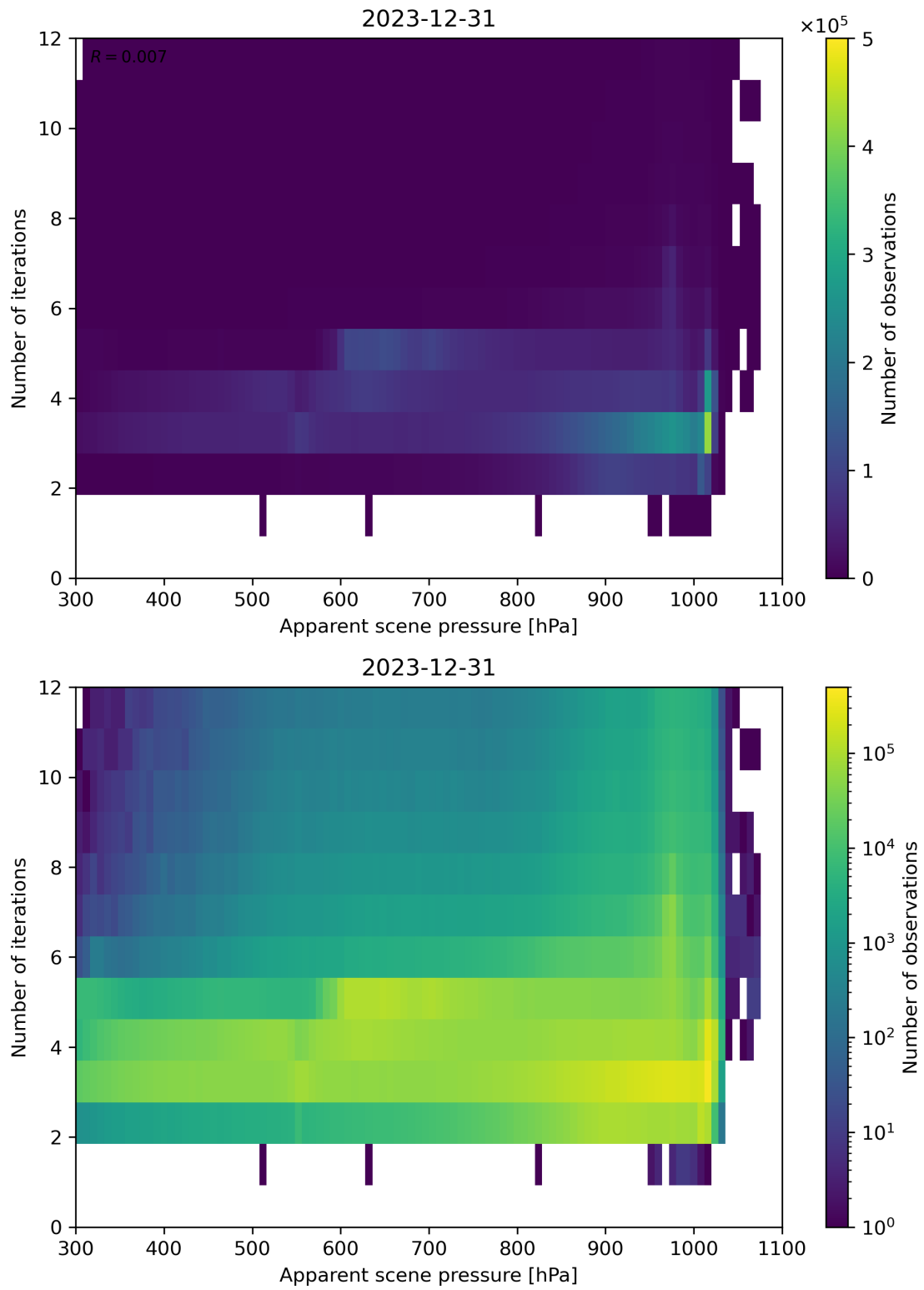
Figure 65: Scatter density plot of “Apparent scene pressure” against “Number of iterations” for 2023-12-30 to 2023-12-31.
