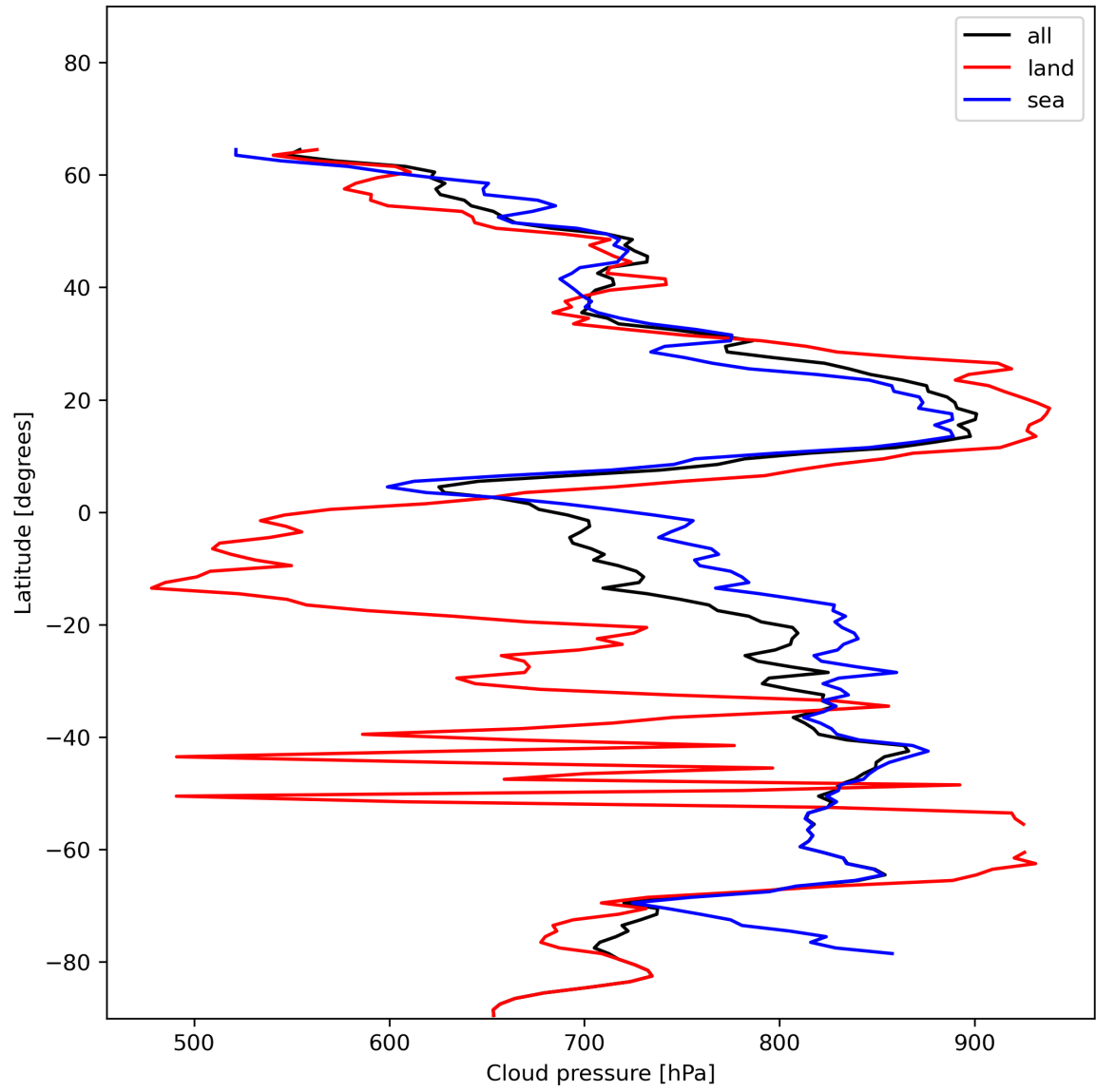
Figure 13: Zonal average of “Cloud pressure” for 2023-12-30 to 2023-12-31.
