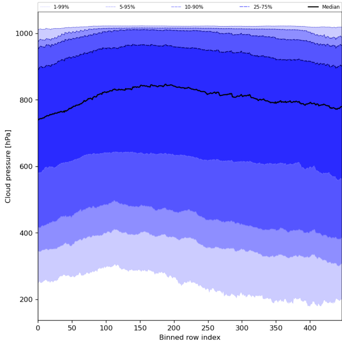
Figure 47: Along track statistics of “Cloud pressure” for 2023-12-30 to 2023-12-31
