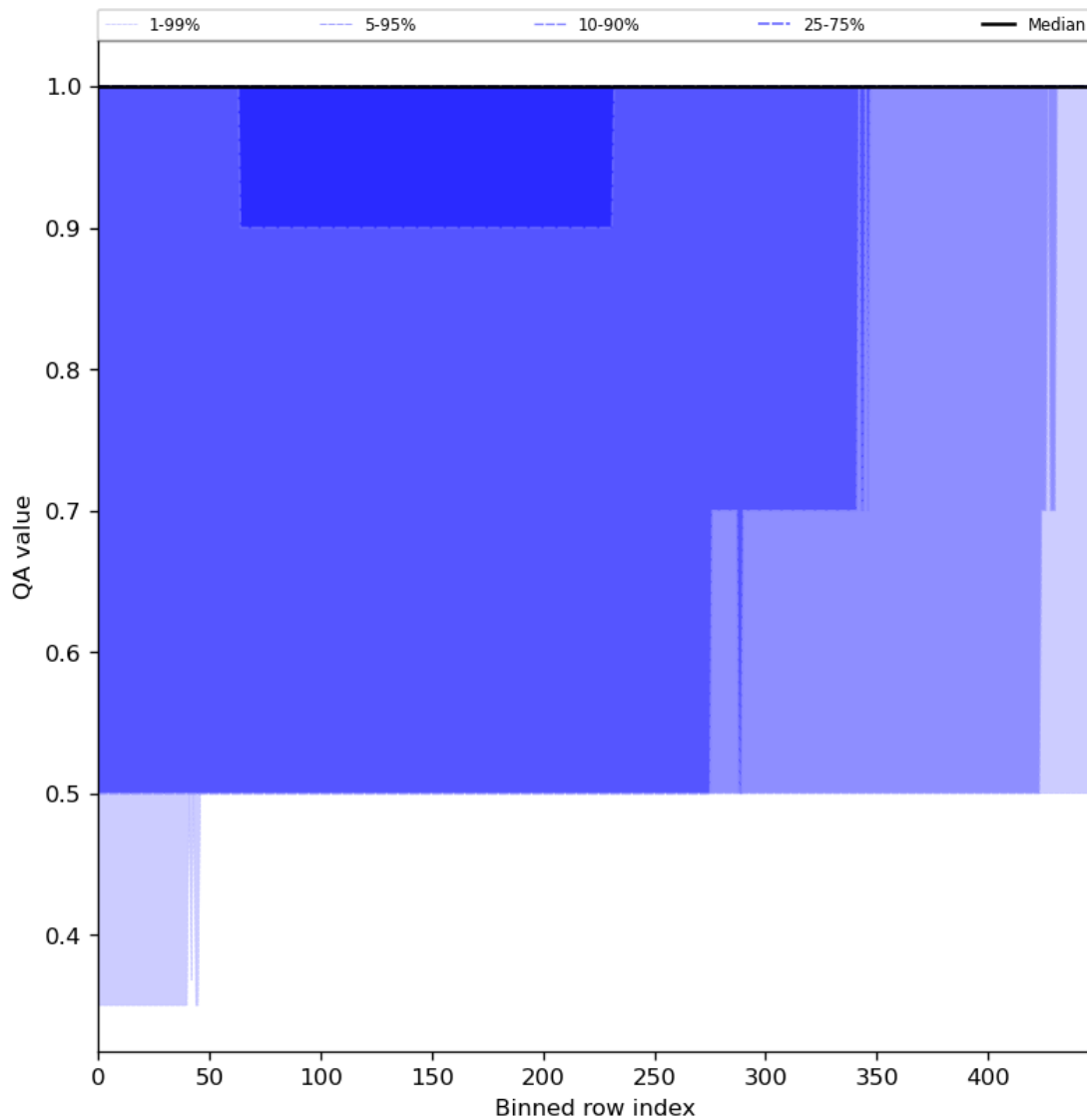
Figure 46: Along track statistics of “QA value” for 2023-12-30 to 2023-12-31
