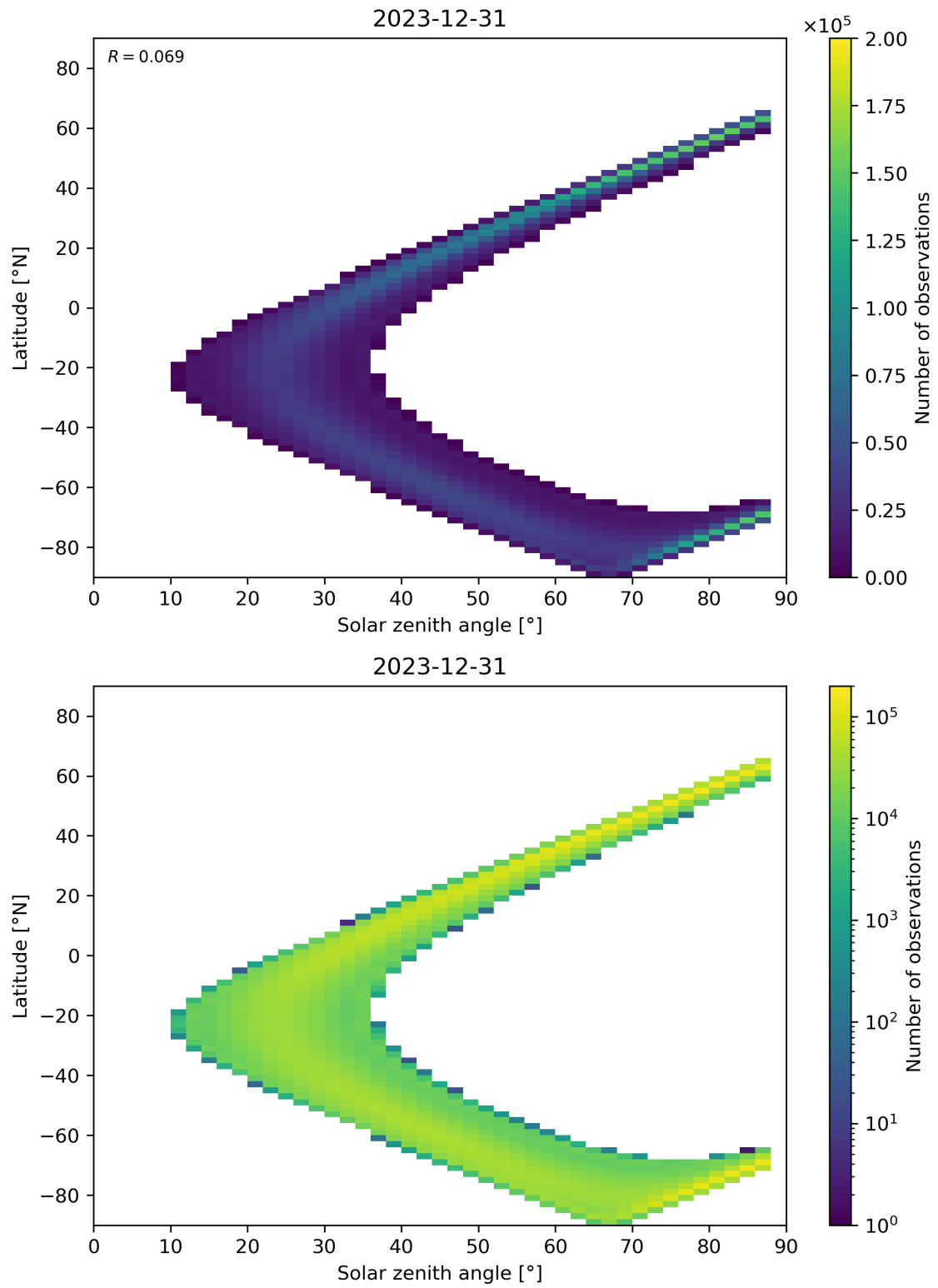
Figure 113: Scatter density plot of “Solar zenith angle” against “Latitude” for 2023-12-30 to 2023-12-31.
