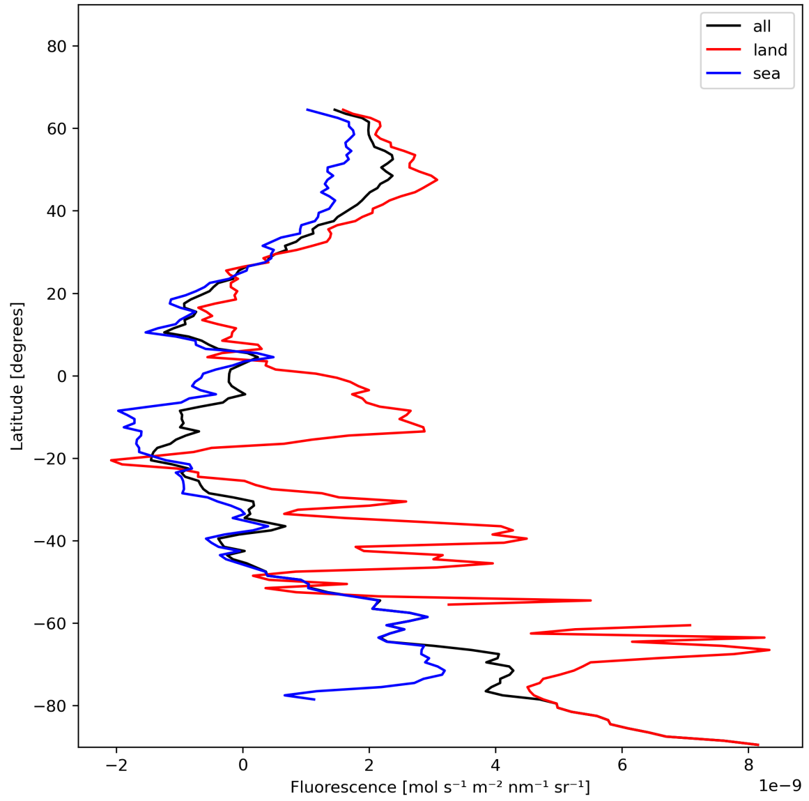
Figure 23: Zonal average of “Fluorescence” for 2023-12-30 to 2023-12-31.
