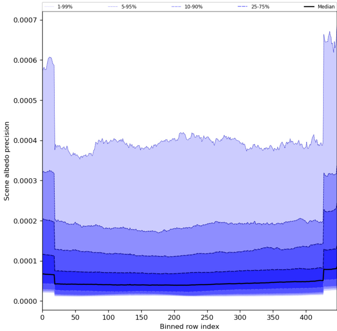
Figure 52: Along track statistics of “Scene albedo precision” for 2023-12-30 to 2023-12-31
