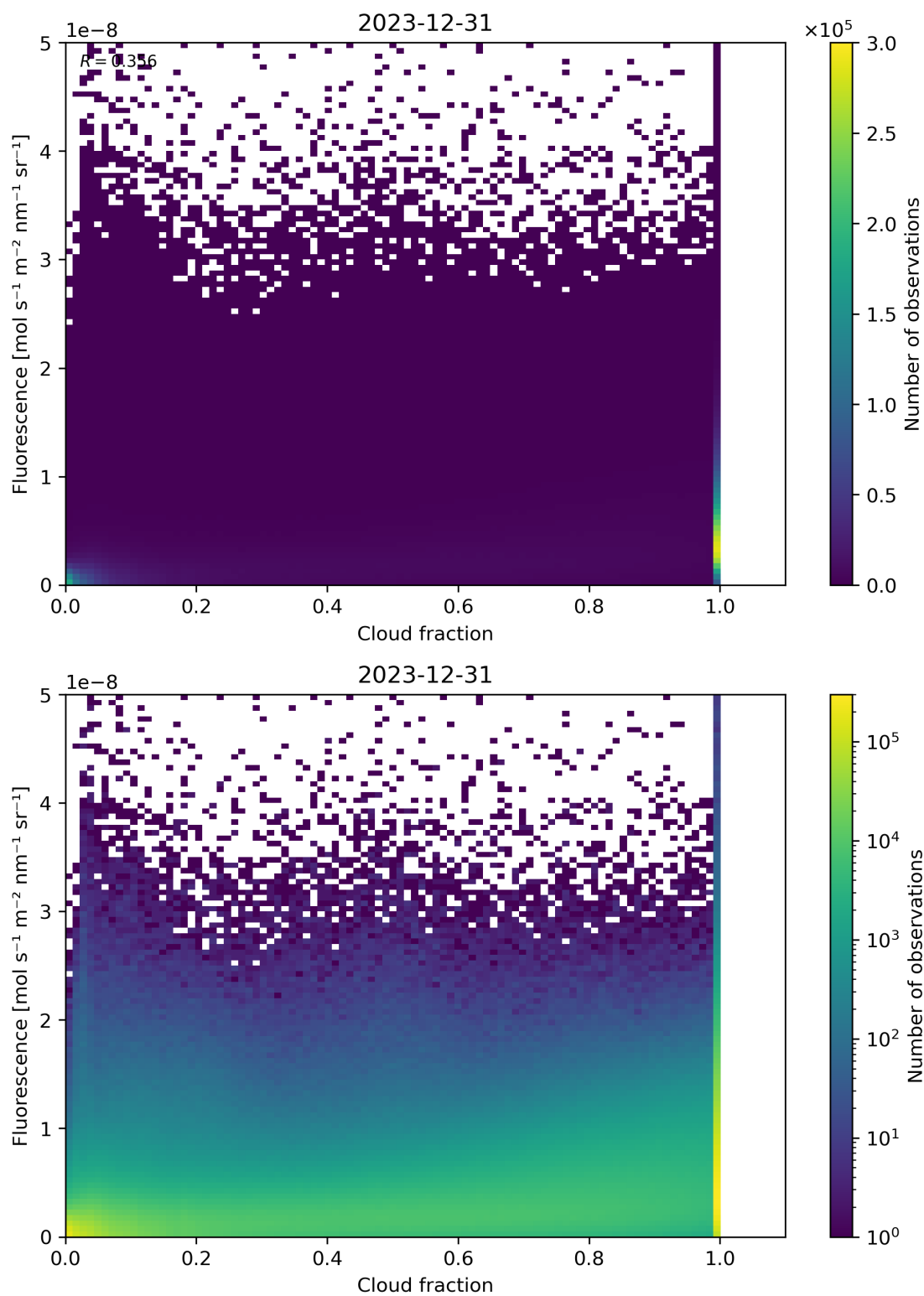
Figure 72: Scatter density plot of “Cloud fraction” against “Fluorescence” for 2023-12-30 to 2023-12-31.
