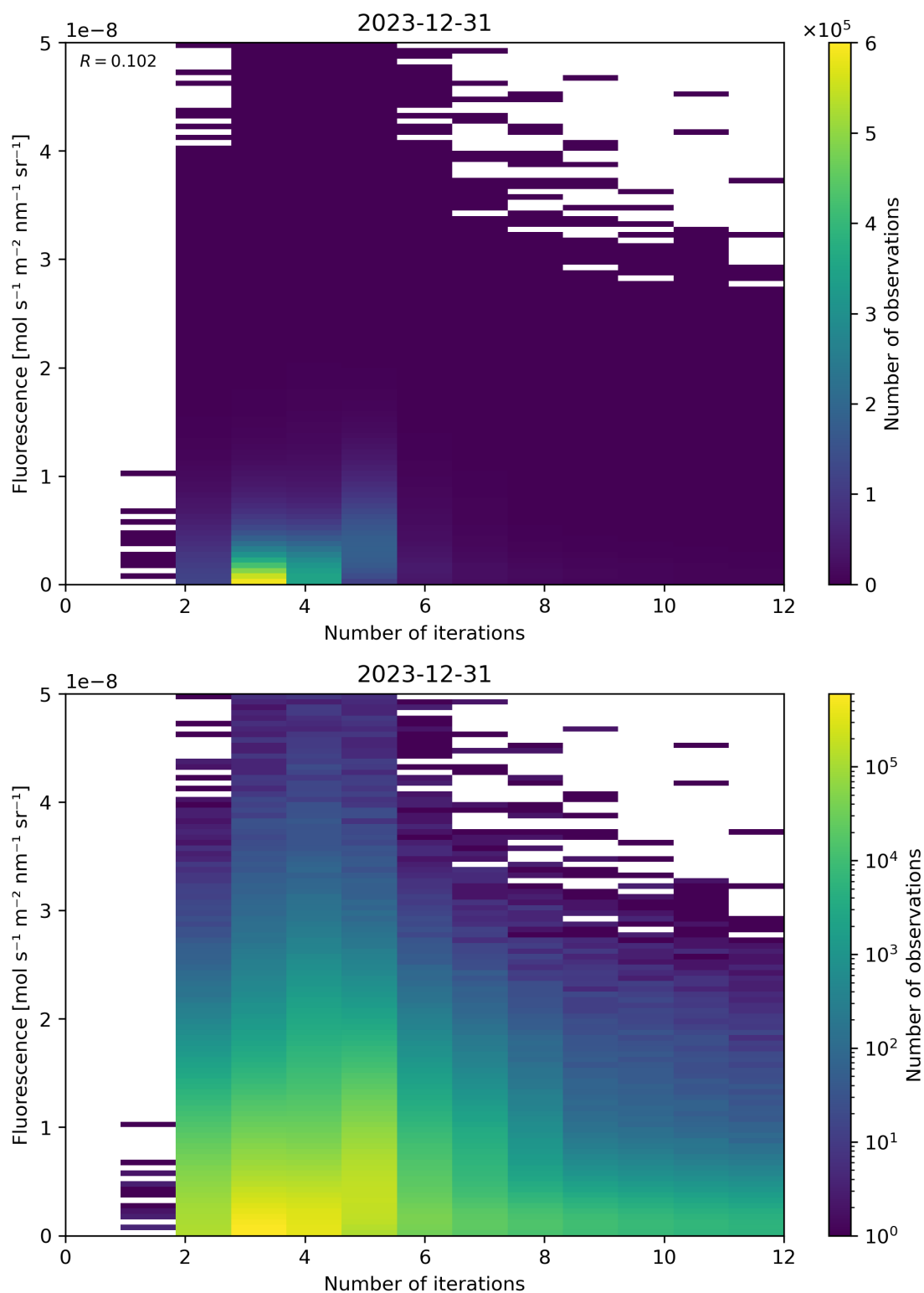
Figure 98: Scatter density plot of "Number of iterations" against "Fluorescence" for 2023-12-30 to 2023-12-31.
