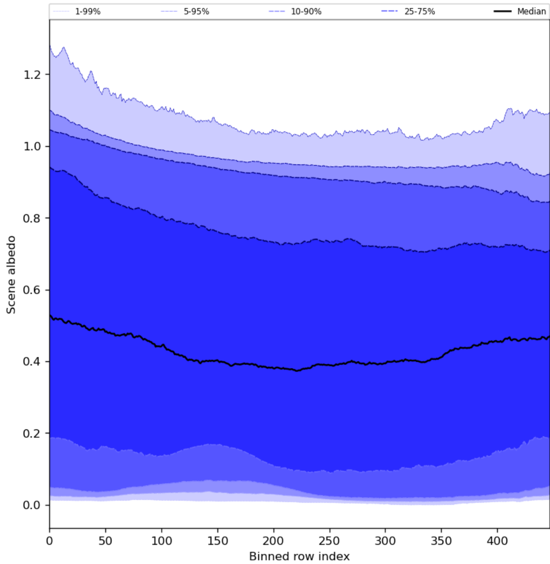
Figure 51: Along track statistics of “Scene albedo” for 2023-12-30 to 2023-12-31
