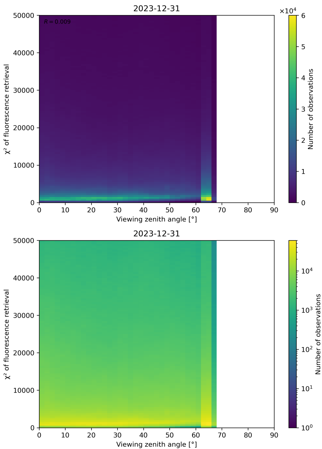
Figure 119: Scatter density plot of “Viewing zenith angle” against “ \chi^2 of fluorescence retrieval” for 2023-12-30 to 2023-12-31.
