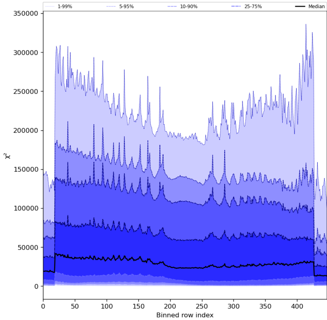
Figure 55: Along track statistics of “ \chi^2 ” for 2023-12-30 to 2023-12-31
