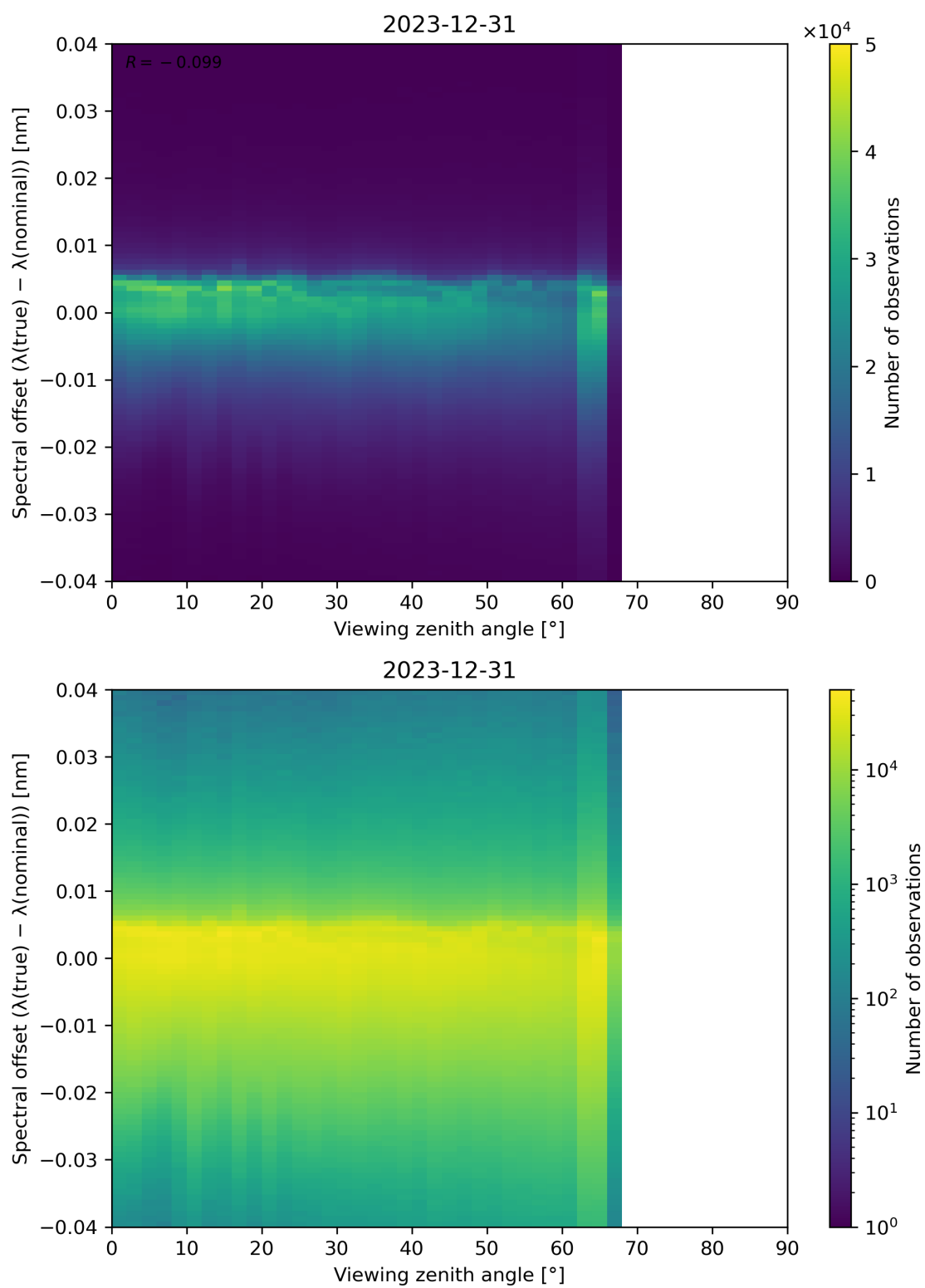
Figure 128: Scatter density plot of “Viewing zenith angle” against “Spectral offset ( \lambda(\text{true}) - \lambda(\text{nominal}) )” for 2023-12-30 to 2023-12-31.
