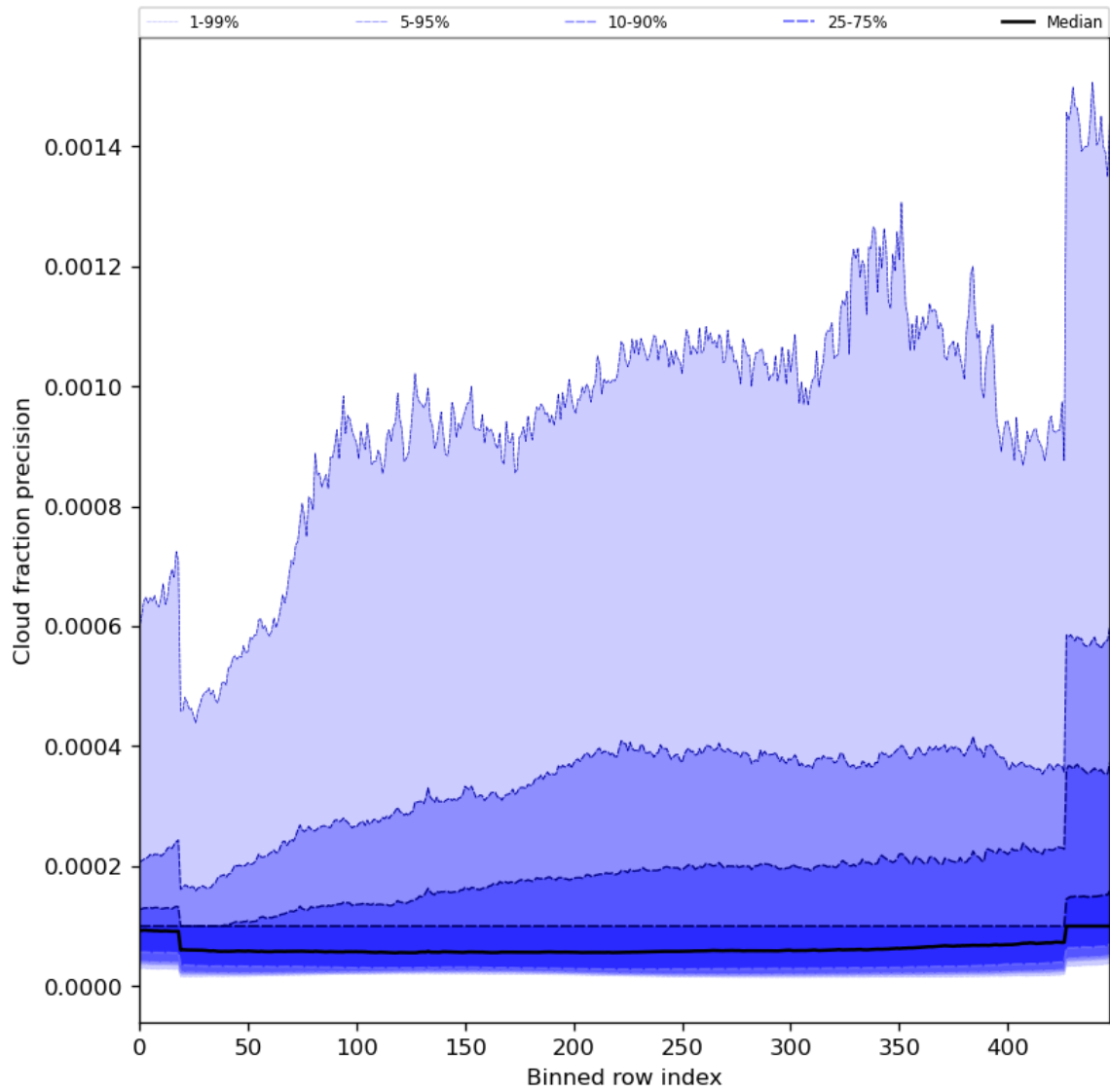
Figure 50: Along track statistics of “Cloud fraction precision” for 2023-12-30 to 2023-12-31
