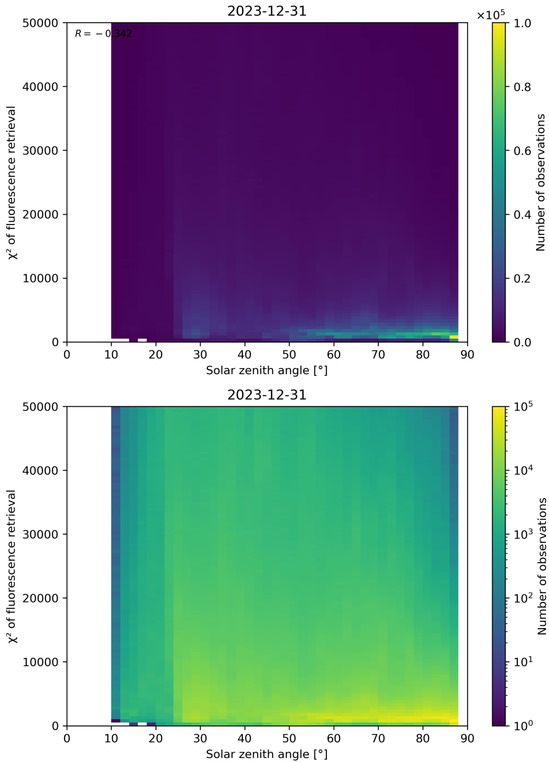
Figure 109: Scatter density plot of “Solar zenith angle” against “ \chi^2 of fluorescence retrieval” for 2023-12-30 to 2023-12-31.
