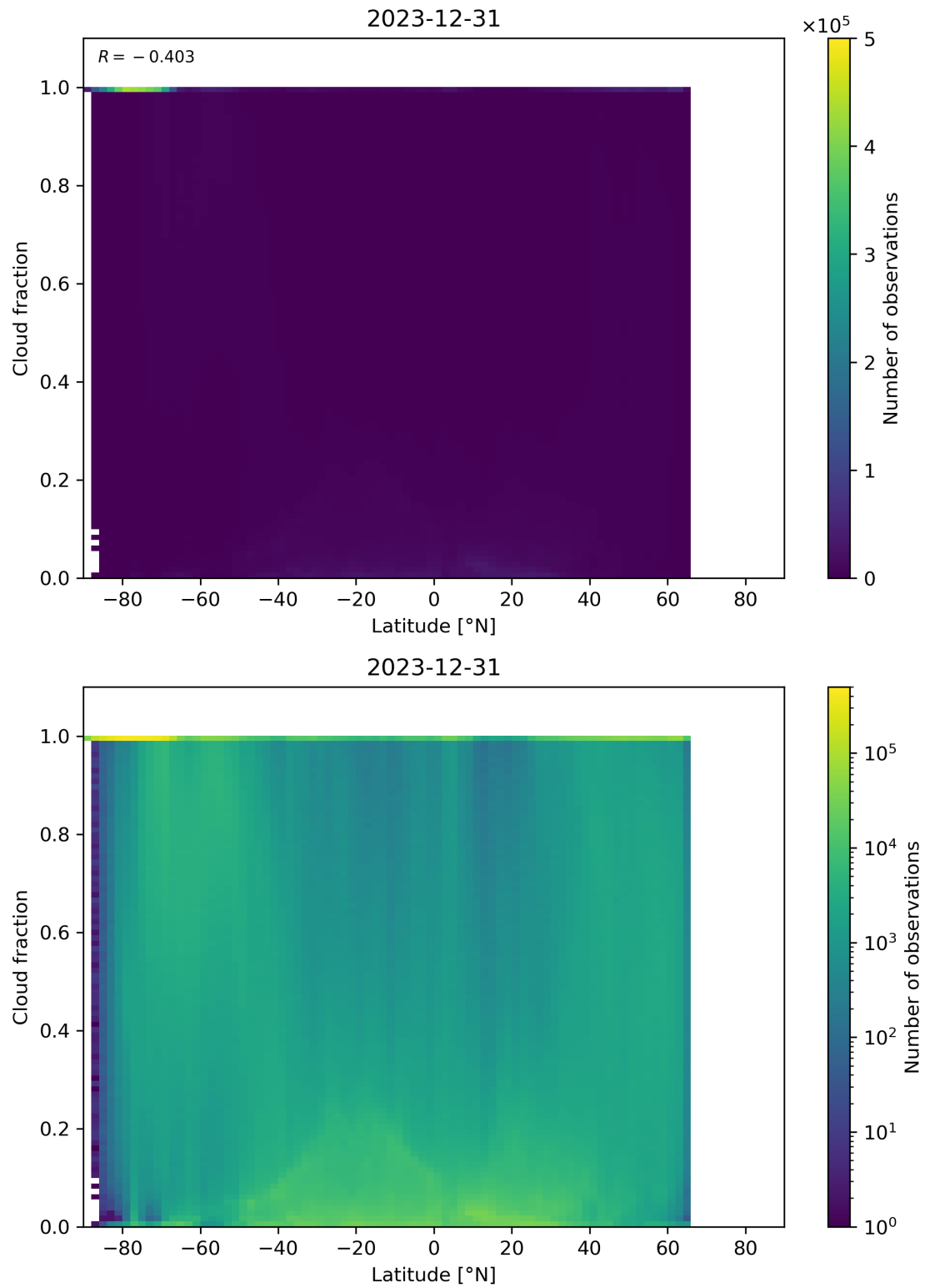
Figure 90: Scatter density plot of “Latitude” against “Cloud fraction” for 2023-12-30 to 2023-12-31.
