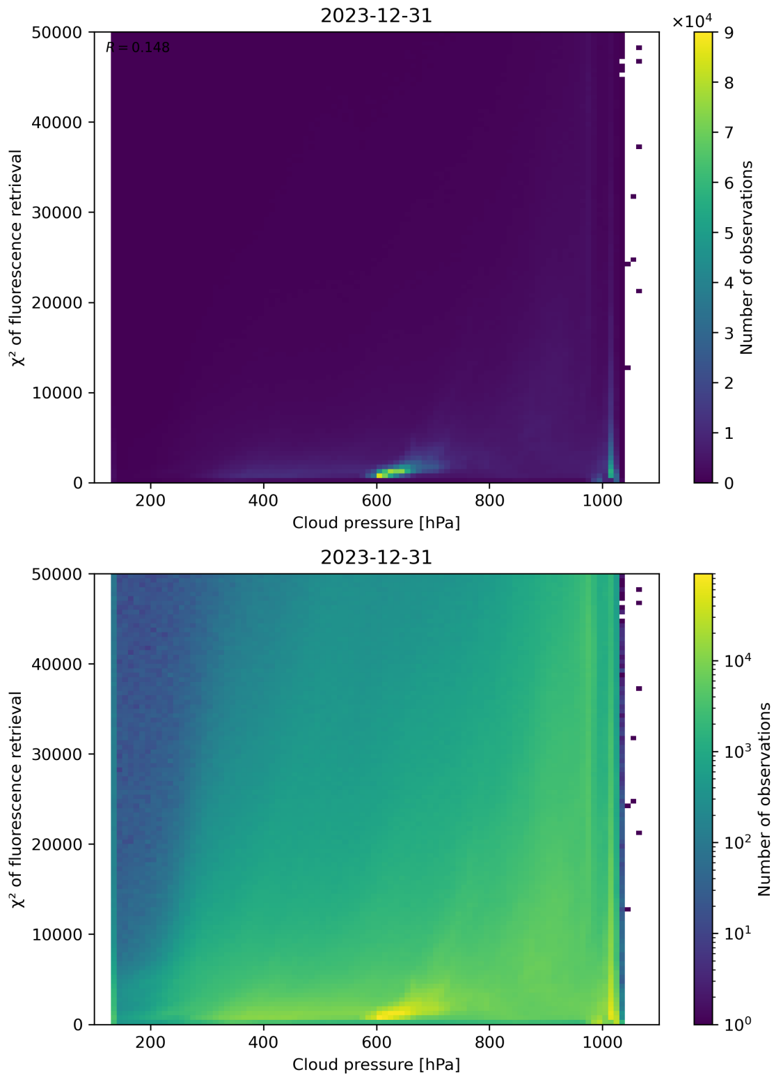
Figure 78: Scatter density plot of “Cloud pressure” against “ \chi^2 of fluorescence retrieval” for 2023-12-30 to 2023-12-31.
