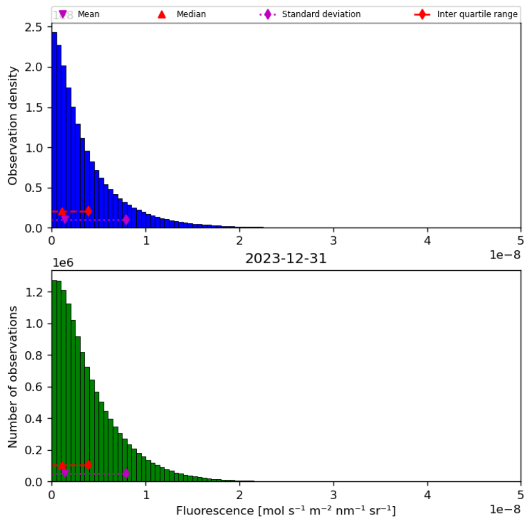
Figure 40: Histogram of “Fluorescence” for 2023-12-30 to 2023-12-31
