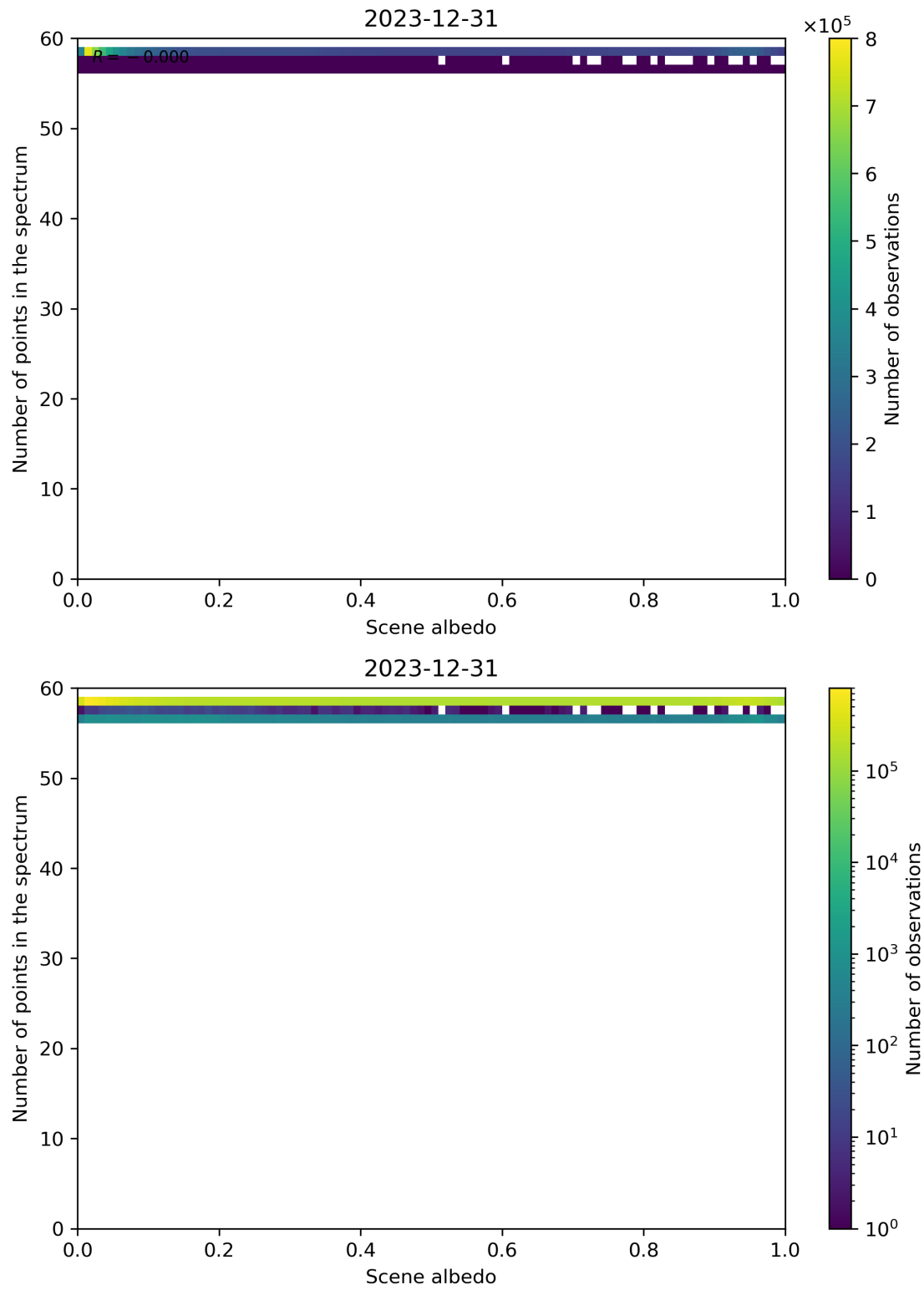
Figure 106: Scatter density plot of “Scene albedo” against “Number of points in the spectrum” for 2023-12-30 to 2023-12-31.
