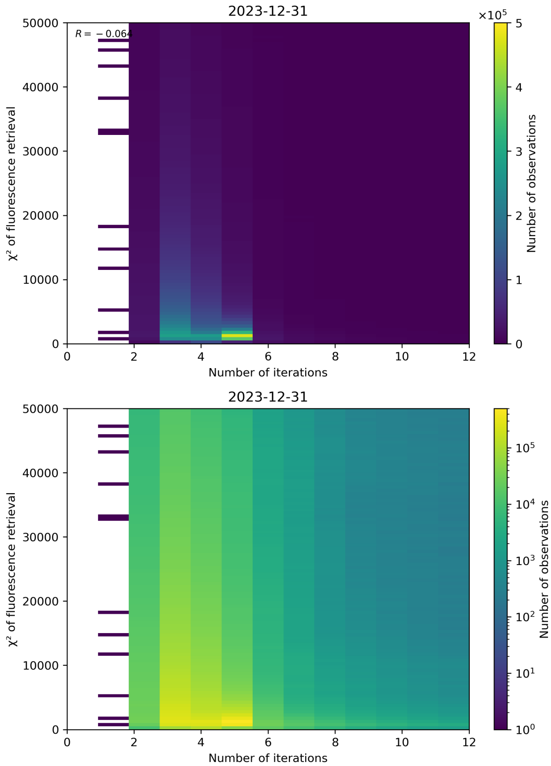
Figure 97: Scatter density plot of “Number of iterations” against “ \chi^2 of fluorescence retrieval” for 2023-12-30 to 2023-12-31.
