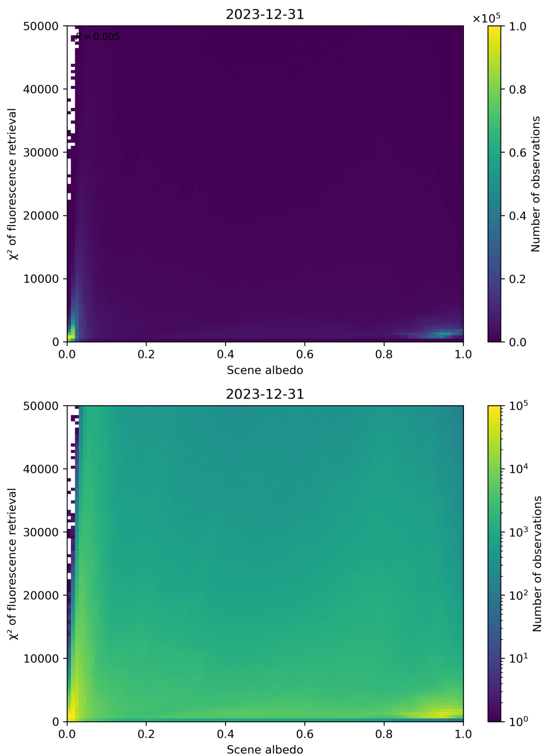
Figure 103: Scatter density plot of “Scene albedo” against “ \chi^2 of fluorescence retrieval” for 2023-12-30 to 2023-12-31.
