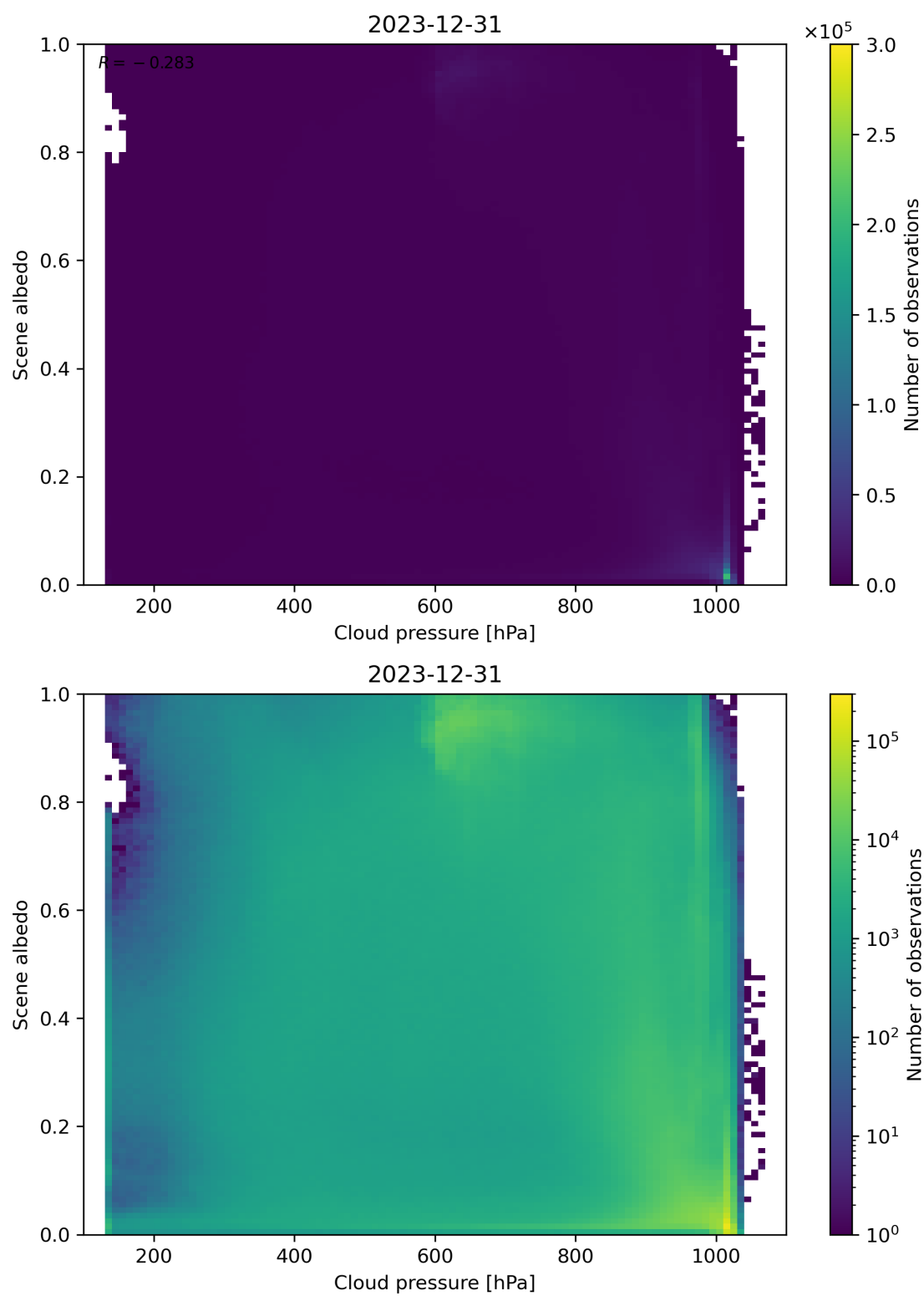
Figure 83: Scatter density plot of “Cloud pressure” against “Scene albedo” for 2023-12-30 to 2023-12-31.
