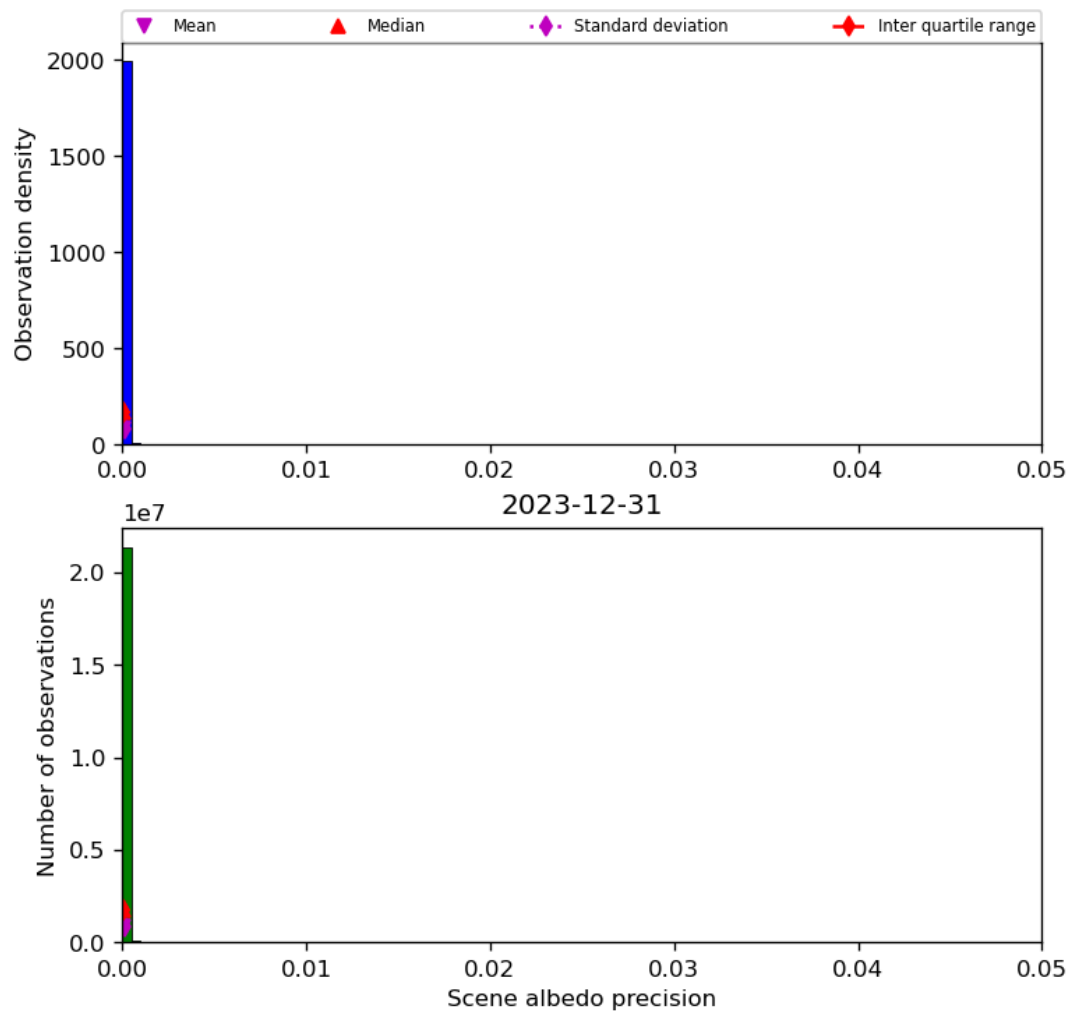
Figure 35: Histogram of “Scene albedo precision” for 2023-12-30 to 2023-12-31
