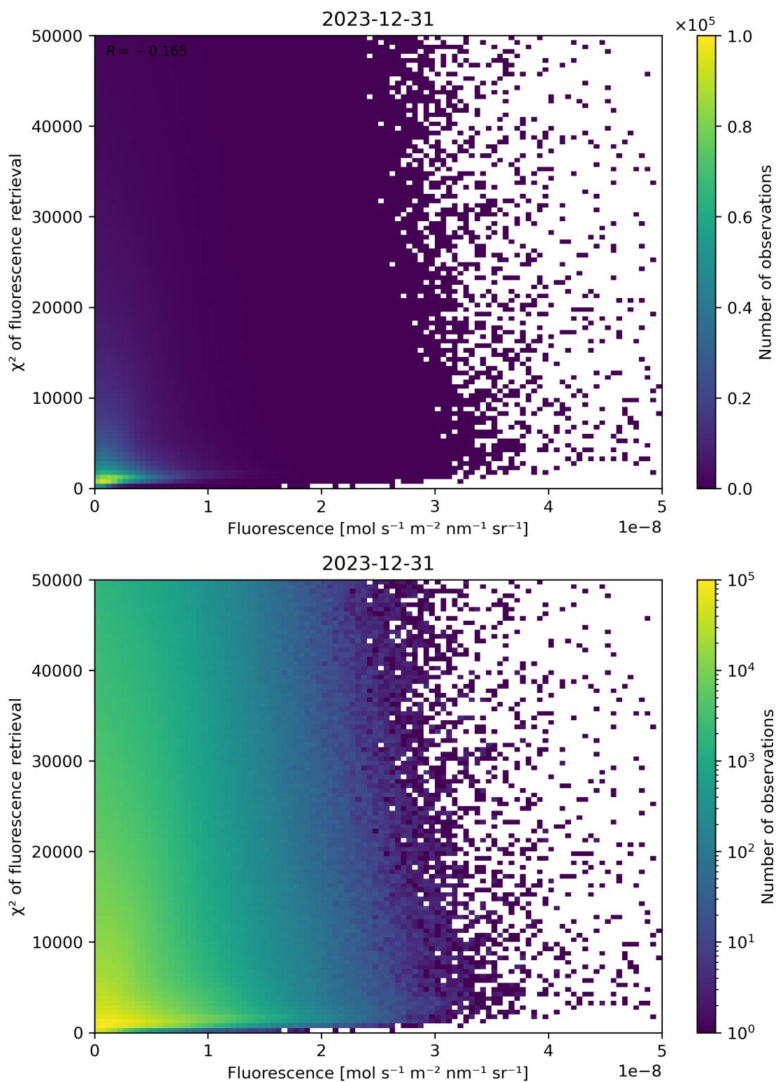
Figure 85: Scatter density plot of “Fluorescence” against “ \chi^2 of fluorescence retrieval” for 2023-12-30 to 2023-12-31.
