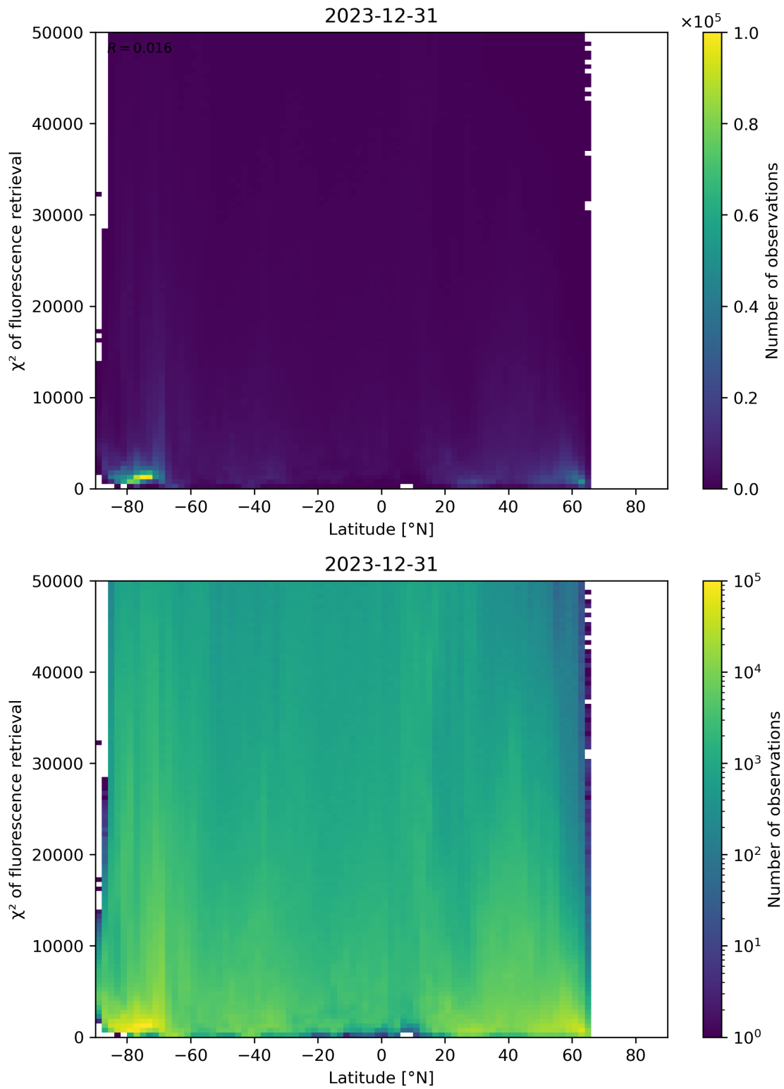
Figure 89: Scatter density plot of “Latitude” against “ \chi^2 of fluorescence retrieval” for 2023-12-30 to 2023-12-31.
