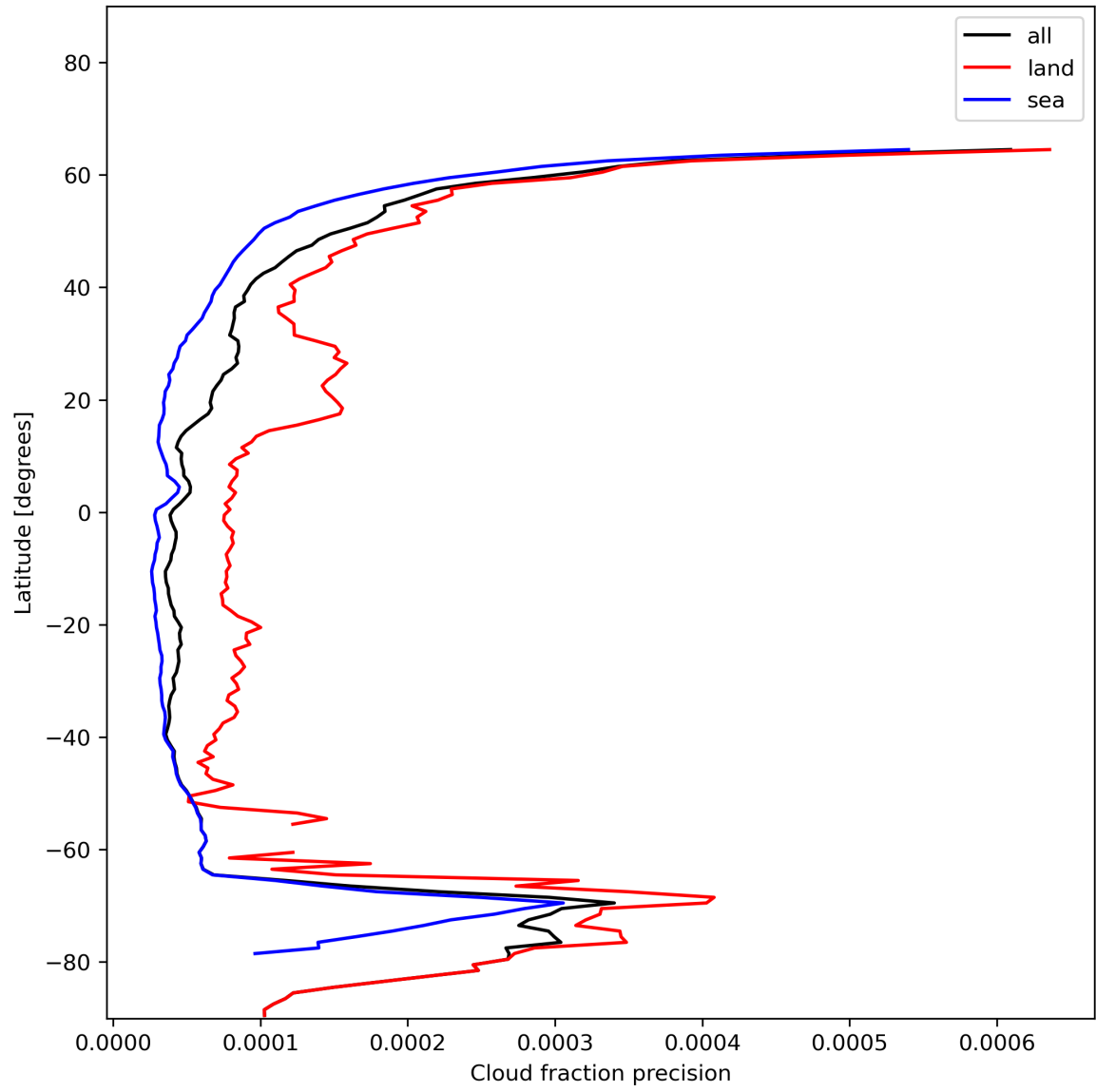
Figure 16: Zonal average of “Cloud fraction precision” for 2023-12-30 to 2023-12-31.
