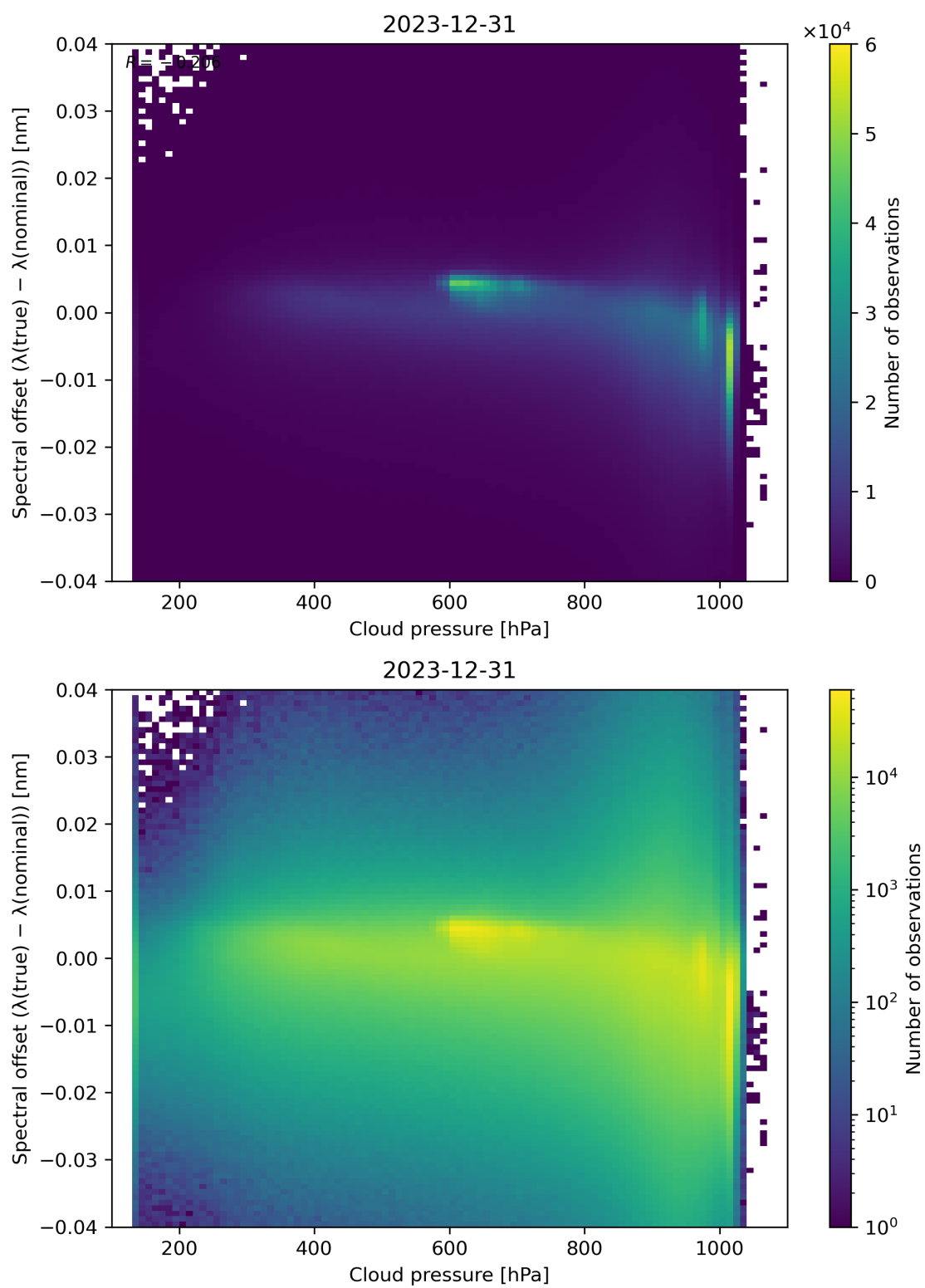
Figure 84: Scatter density plot of “Cloud pressure” against “Spectral offset ( \lambda(\text{true}) - \lambda(\text{nominal}) )” for 2023-12-30 to 2023-12-31.
