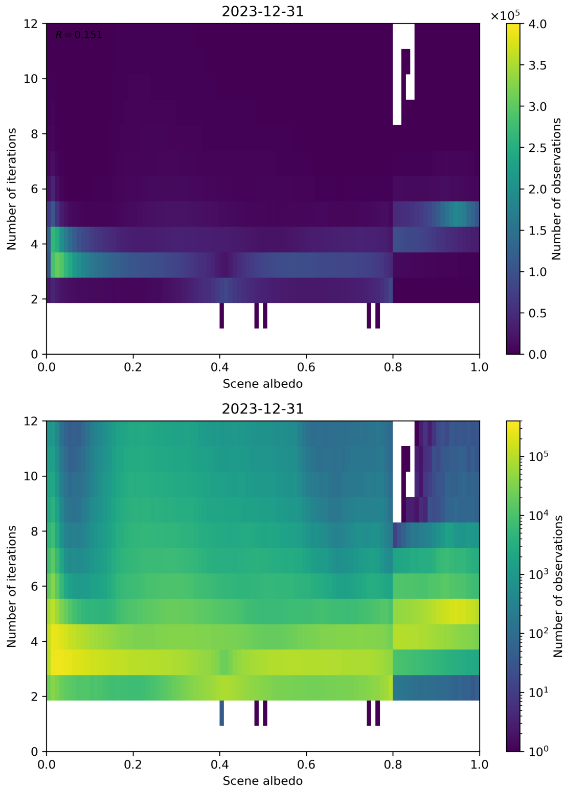
Figure 105: Scatter density plot of “Scene albedo” against “Number of iterations” for 2023-12-30 to 2023-12-31.
