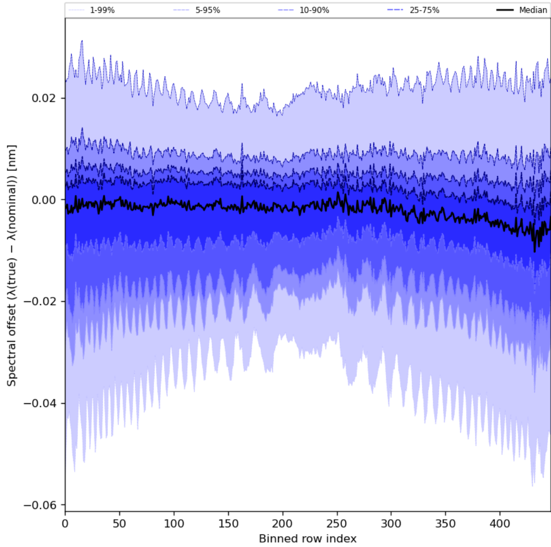
Figure 62: Along track statistics of “Spectral offset ( \lambda(\text{true}) - \lambda(\text{nominal}) )” for 2023-12-30 to 2023-12-31
