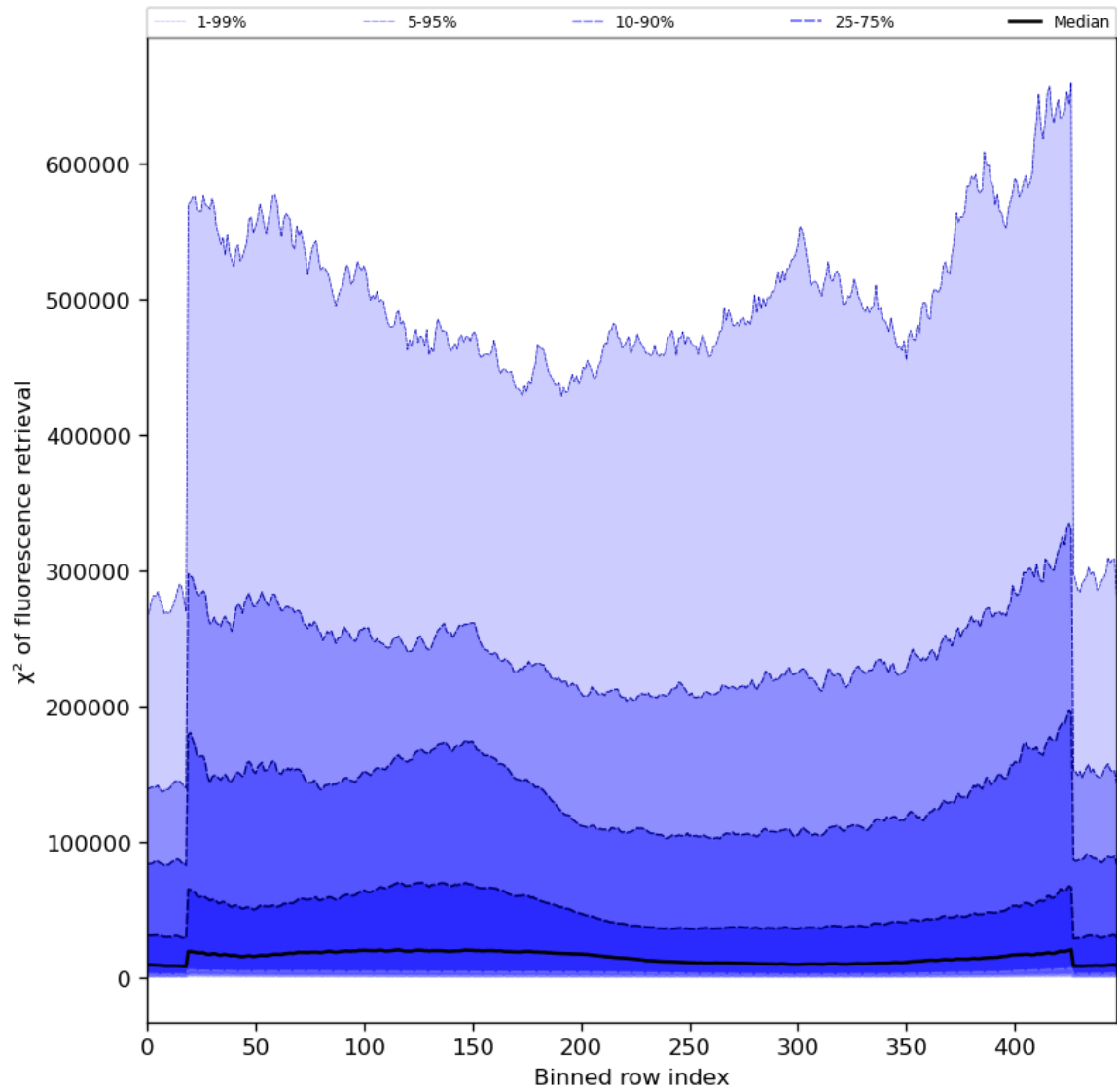
Figure 59: Along track statistics of “ \chi^2 of fluorescence retrieval” for 2023-12-30 to 2023-12-31
