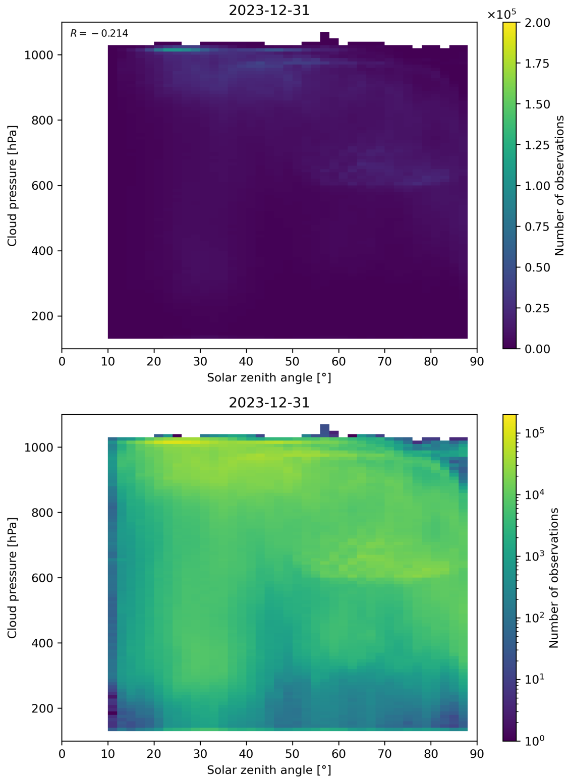
Figure 111: Scatter density plot of “Solar zenith angle” against “Cloud pressure” for 2023-12-30 to 2023-12-31.
