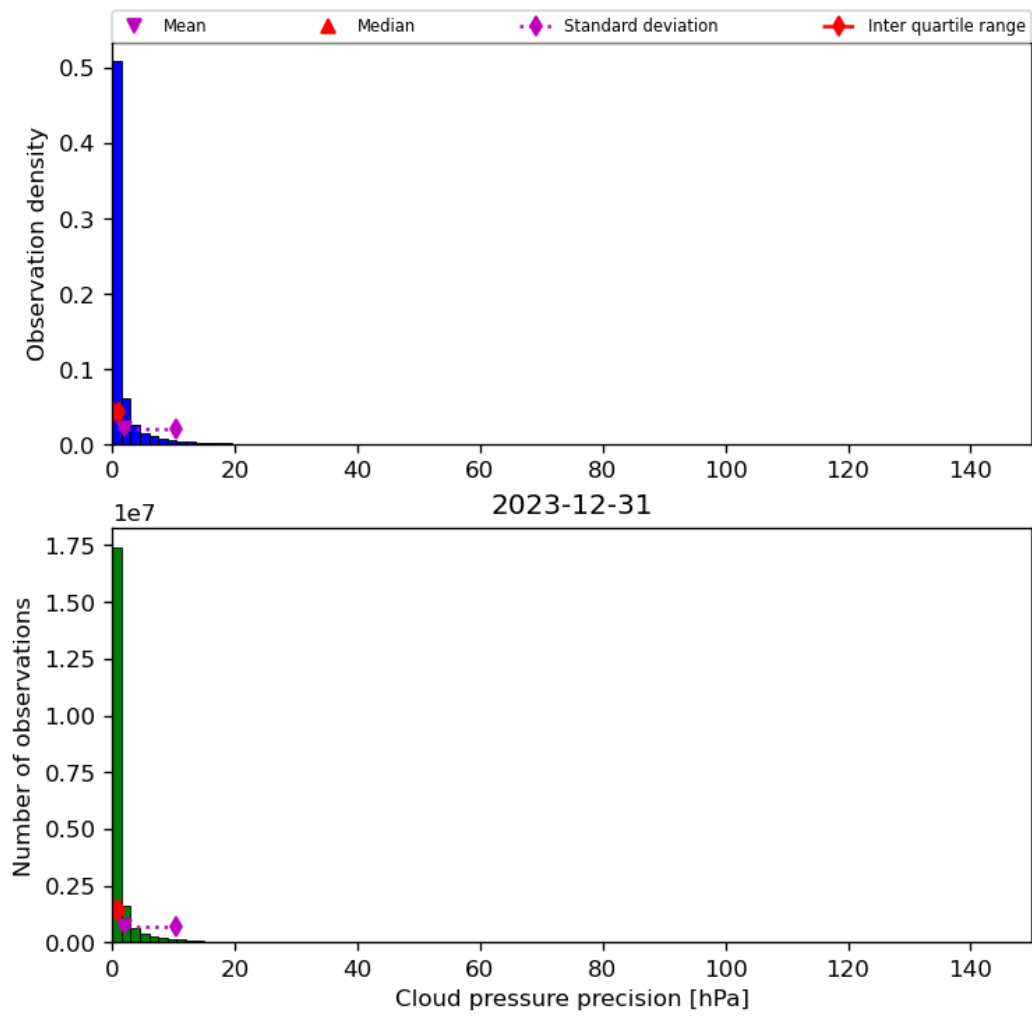
Figure 31: Histogram of “Cloud pressure precision” for 2023-12-30 to 2023-12-31
