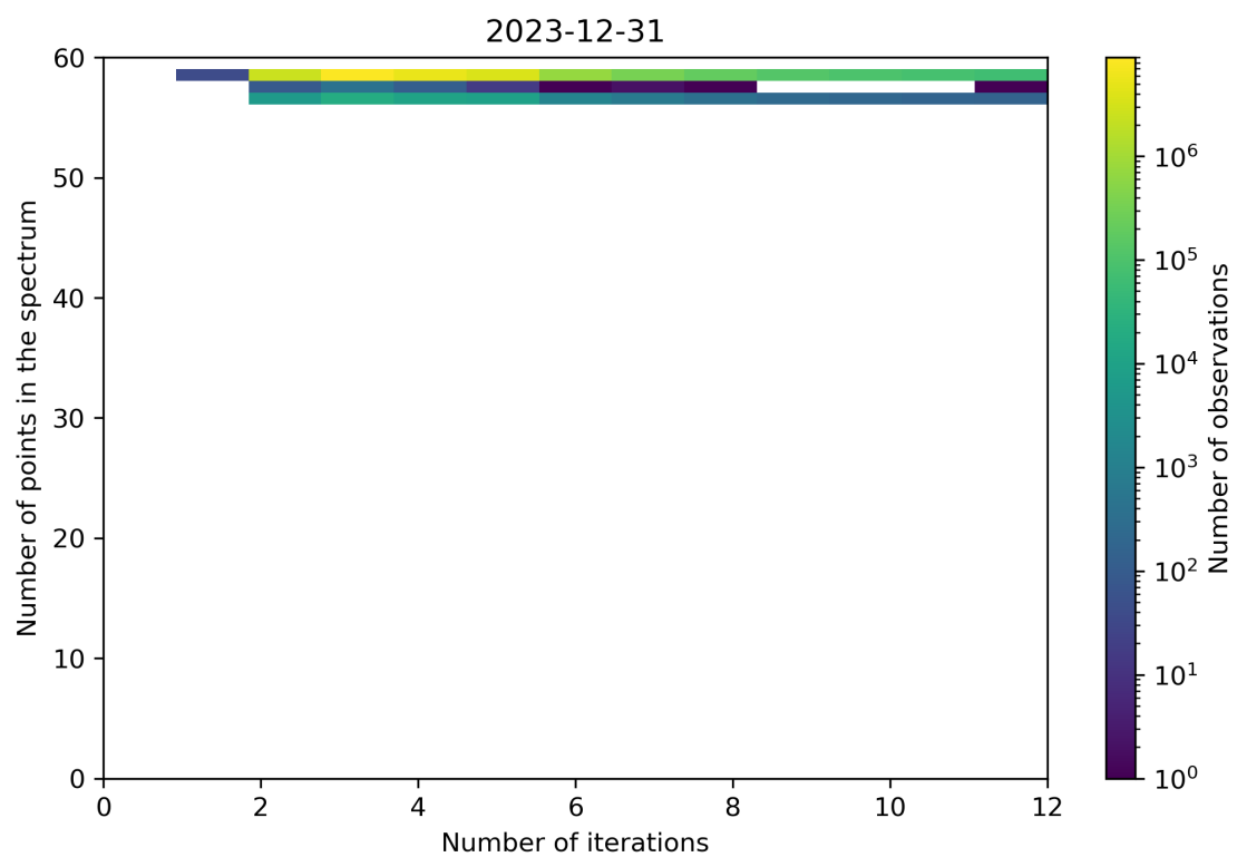
Figure 99: Scatter density plot of “Number of iterations” against “Number of points in the spectrum” for 2023-12-30 to 2023-12-31.
