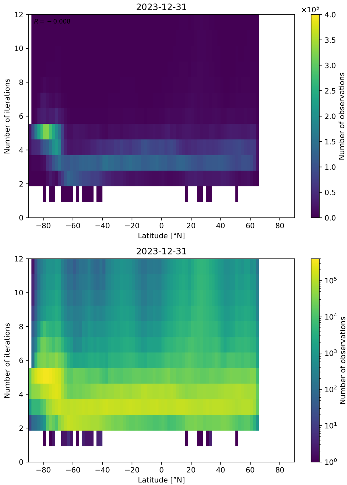
Figure 93: Scatter density plot of “Latitude” against “Number of iterations” for 2023-12-30 to 2023-12-31.
