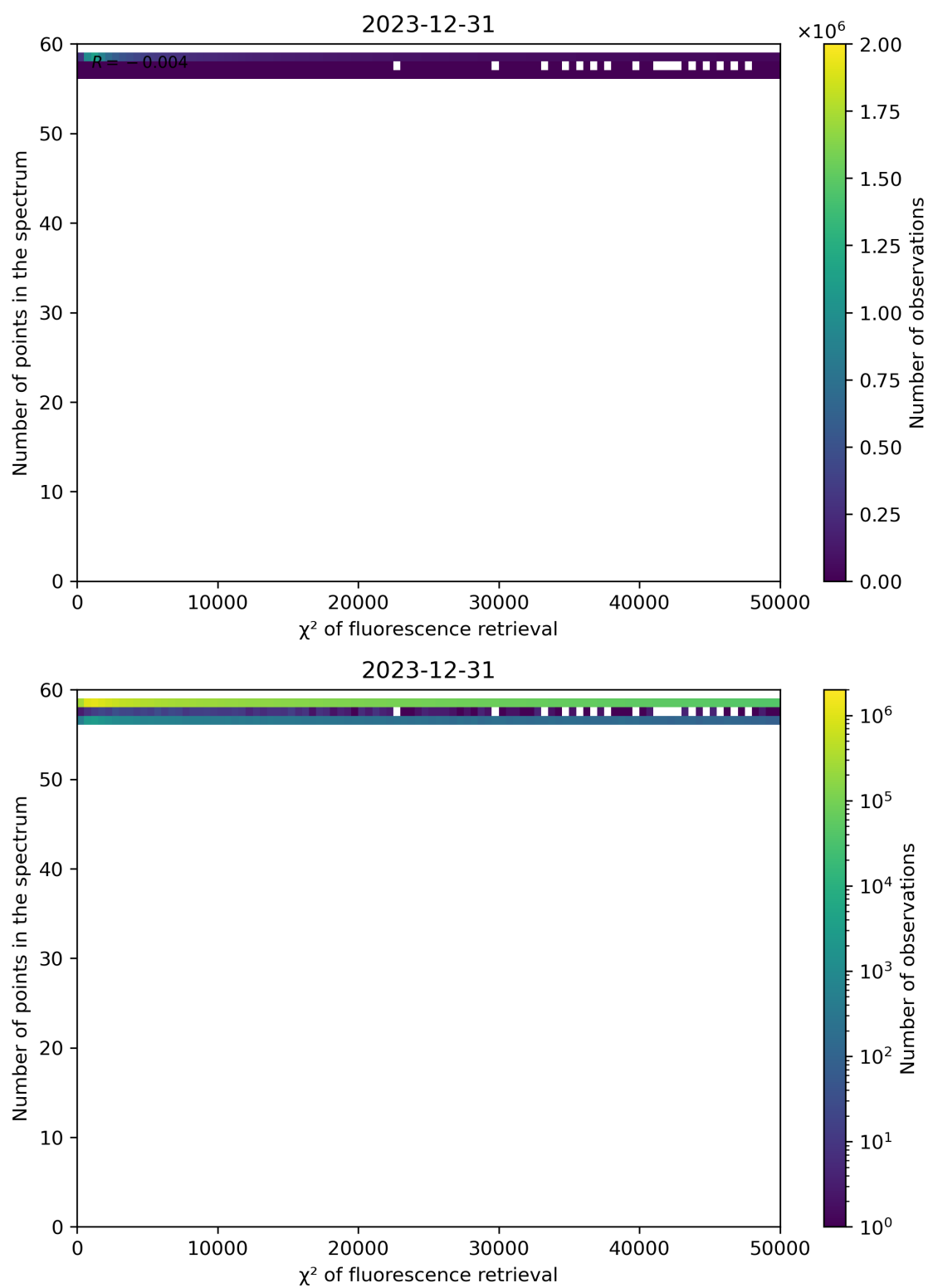
Figure 68: Scatter density plot of " \chi^2 of fluorescence retrieval" against "Number of points in the spectrum" for 2023-12-30 to 2023-12-31.
