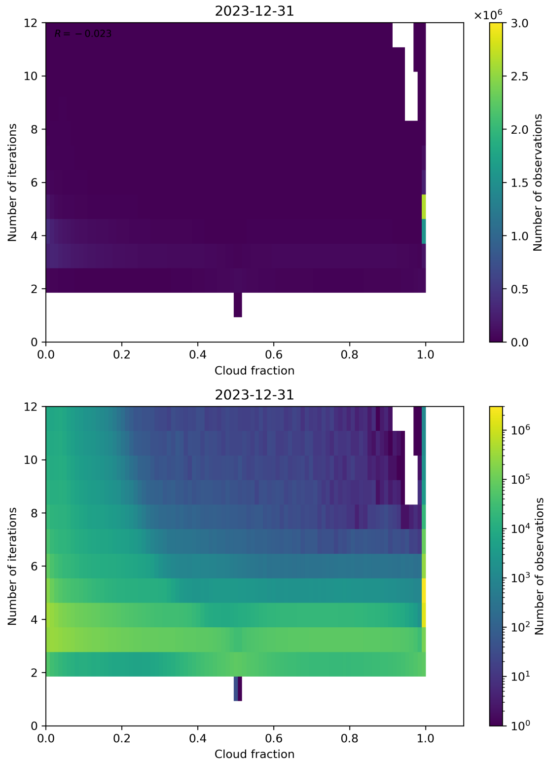
Figure 73: Scatter density plot of “Cloud fraction” against “Number of iterations” for 2023-12-30 to 2023-12-31.
