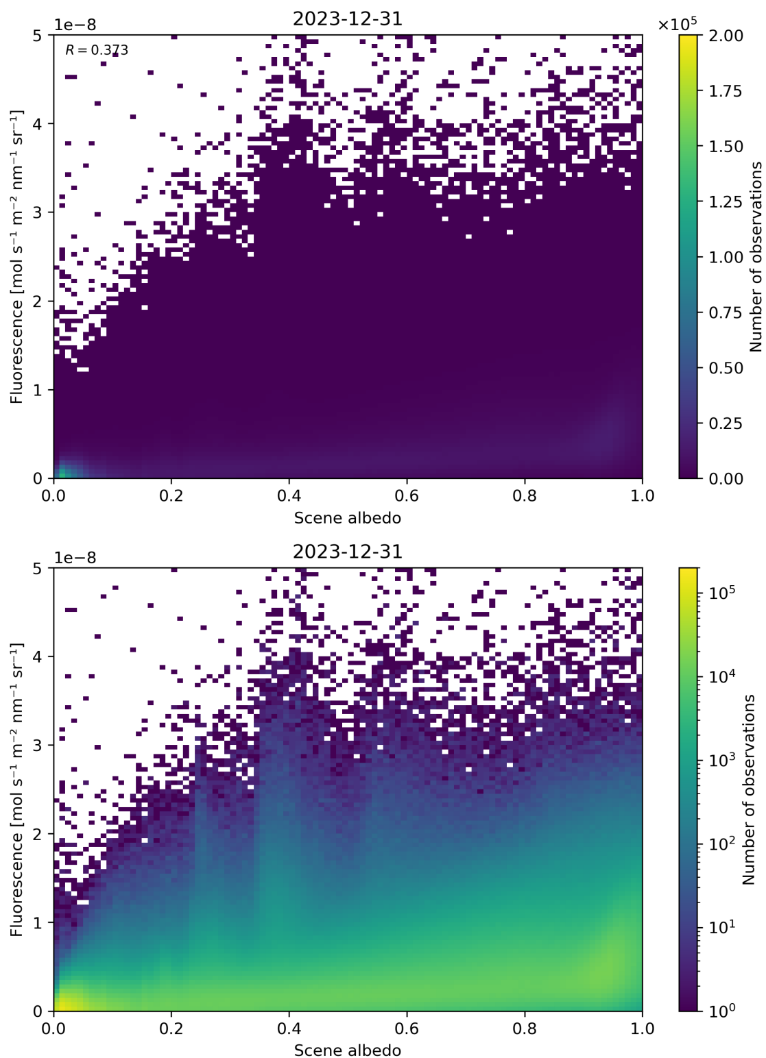
Figure 104: Scatter density plot of “Scene albedo” against “Fluorescence” for 2023-12-30 to 2023-12-31.
