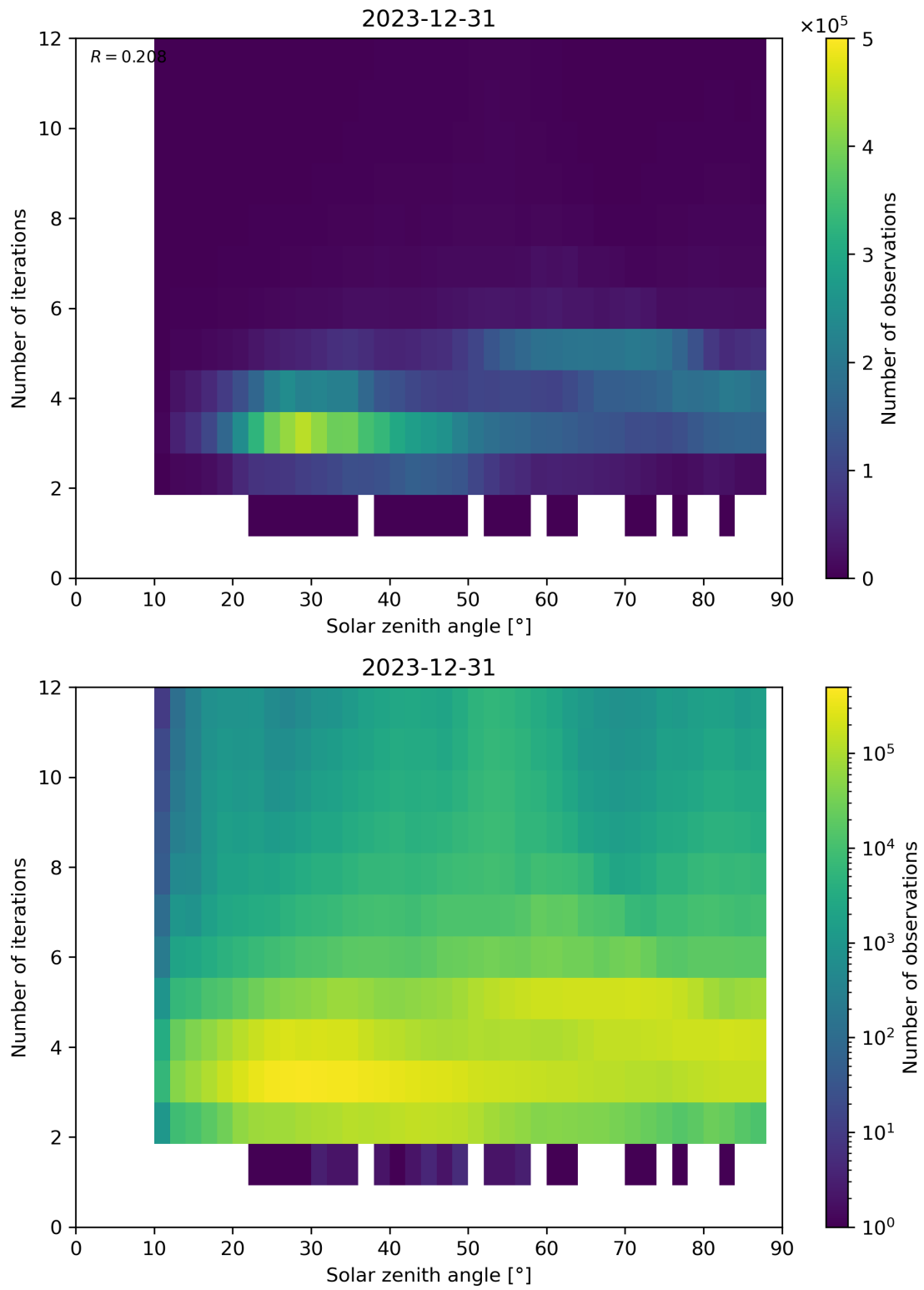
Figure 114: Scatter density plot of “Solar zenith angle” against “Number of iterations” for 2023-12-30 to 2023-12-31.
