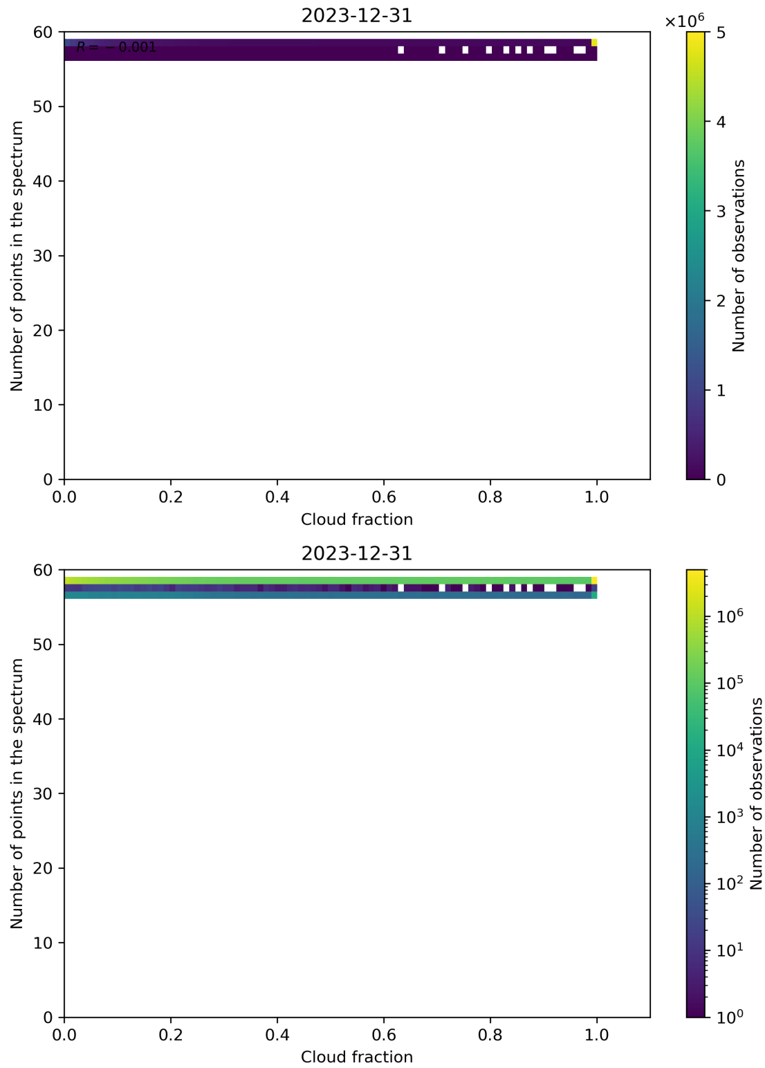
Figure 74: Scatter density plot of “Cloud fraction” against “Number of points in the spectrum” for 2023-12-30 to 2023-12-31.
