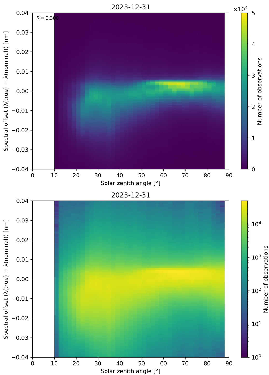
Figure 117: Scatter density plot of “Solar zenith angle” against “Spectral offset ( \lambda(\text{true}) - \lambda(\text{nominal}) )” for 2023-12-30 to 2023-12-31.
