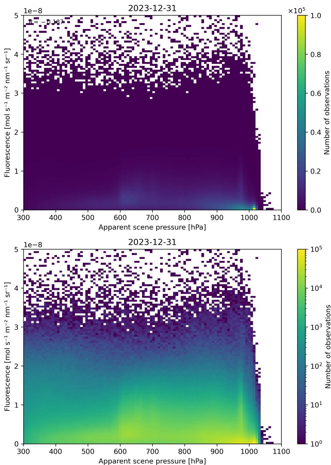
Figure 64: Scatter density plot of “Apparent scene pressure” against “Fluorescence” for 2023-12-30 to 2023-12-31.
