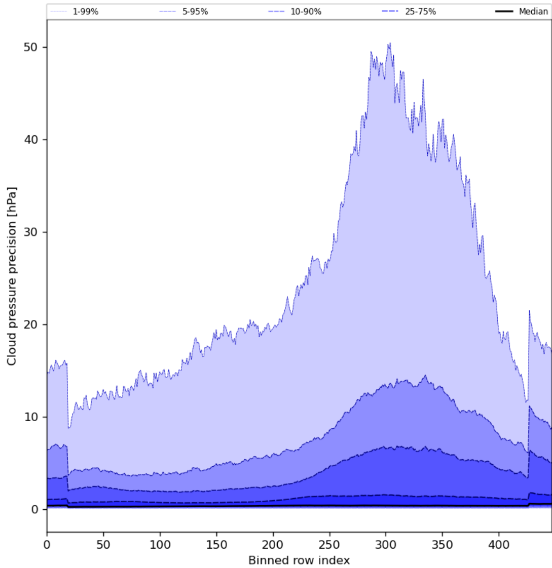
Figure 48: Along track statistics of “Cloud pressure precision” for 2023-12-30 to 2023-12-31
