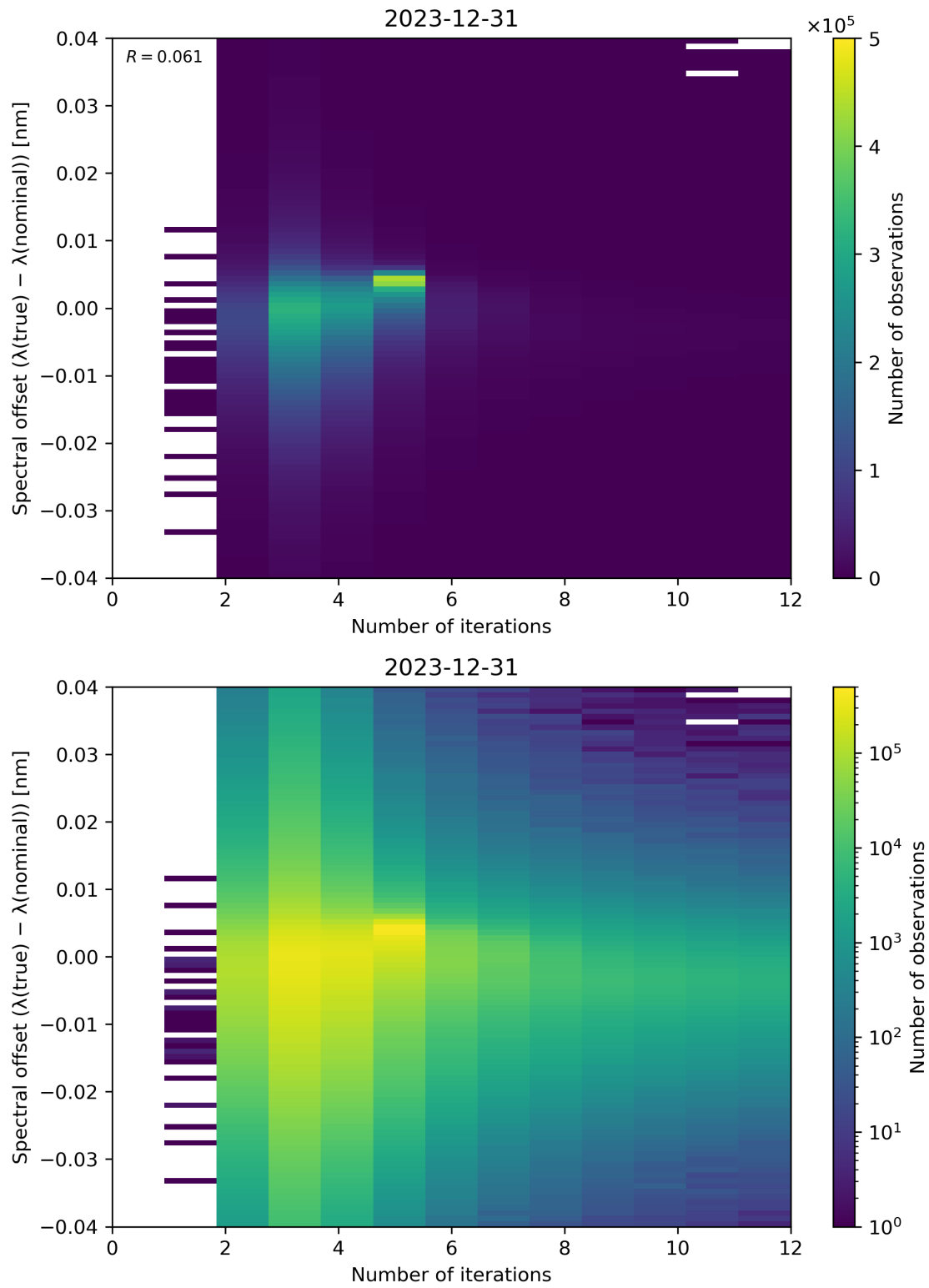
Figure 100: Scatter density plot of “Number of iterations” against “Spectral offset ( \lambda(\text{true}) - \lambda(\text{nominal}) )” for 2023-12-30 to 2023-12-31.
