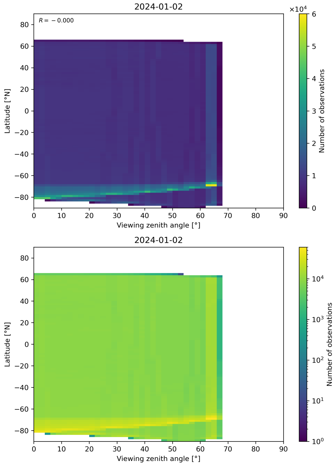
Figure 123: Scatter density plot of “Viewing zenith angle” against “Latitude” for 2024-01-01 to 2024-01-03.
