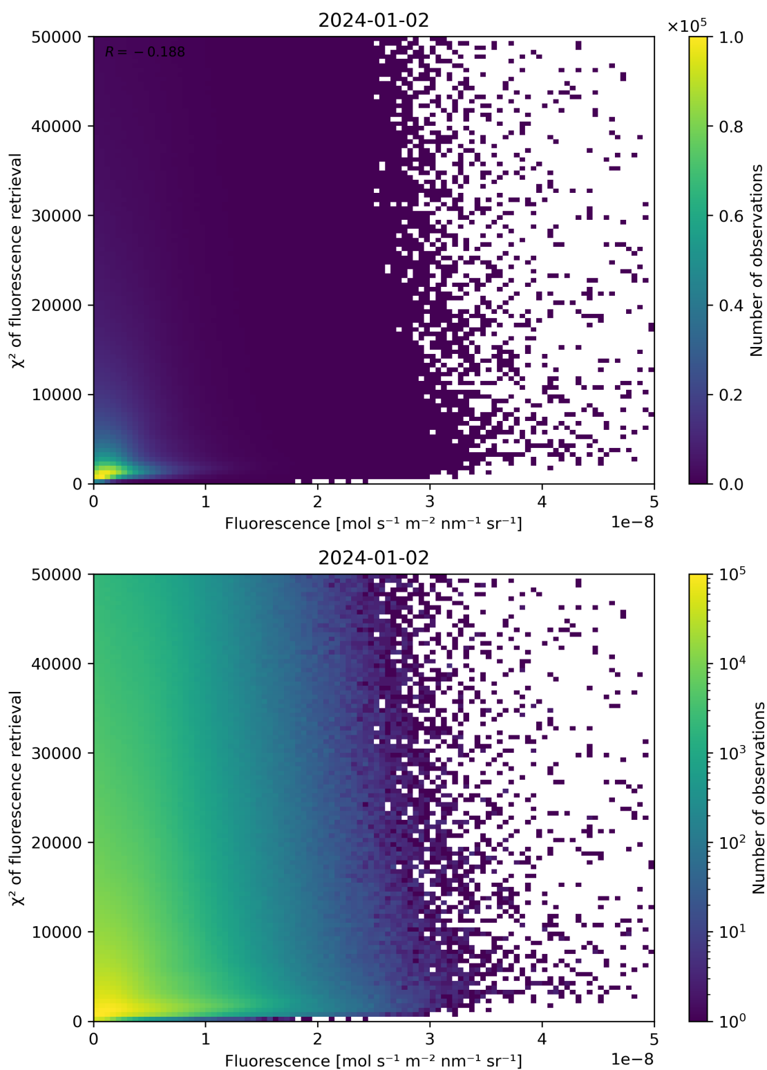
Figure 85: Scatter density plot of “Fluorescence” against “ \chi^2 of fluorescence retrieval” for 2024-01-01 to 2024-01-03.
