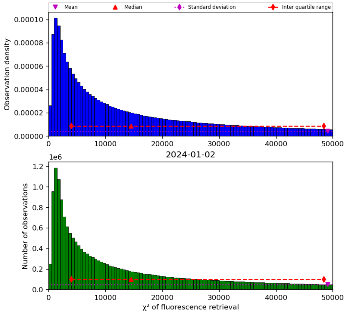
Figure 42: Histogram of “ \chi^2 of fluorescence retrieval” for 2024-01-01 to 2024-01-03
