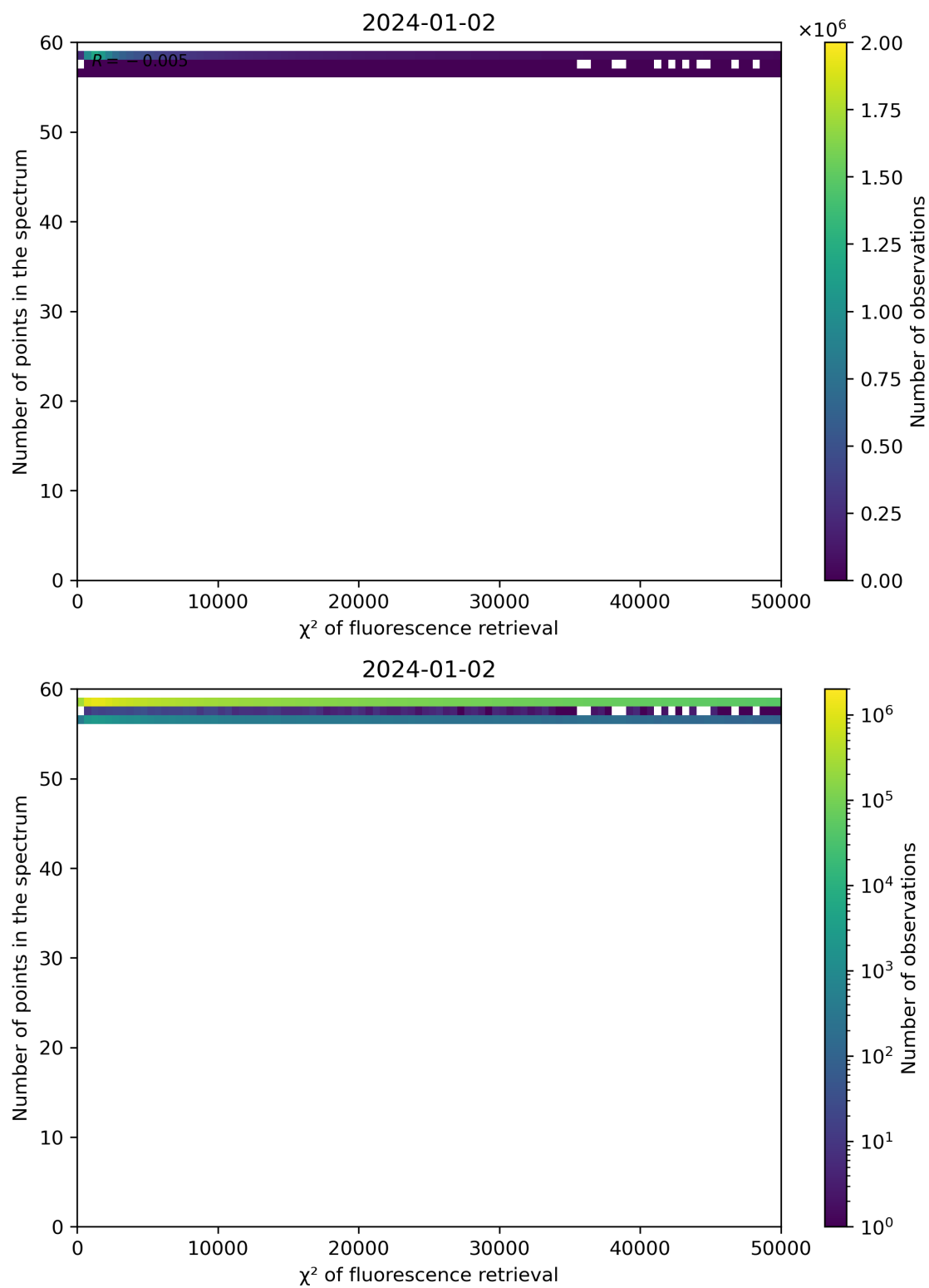
Figure 68: Scatter density plot of " \chi^2 of fluorescence retrieval" against "Number of points in the spectrum" for 2024-01-01 to 2024-01-03.
