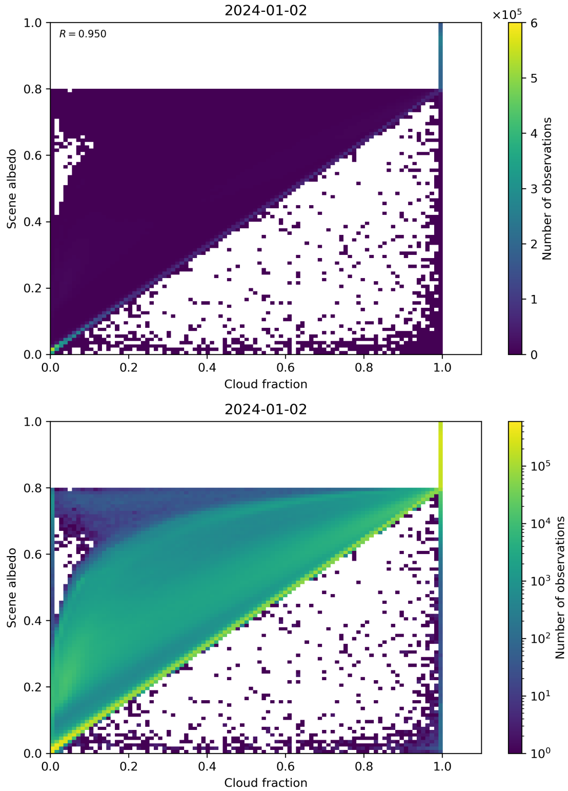
Figure 75: Scatter density plot of “Cloud fraction” against “Scene albedo” for 2024-01-01 to 2024-01-03.
