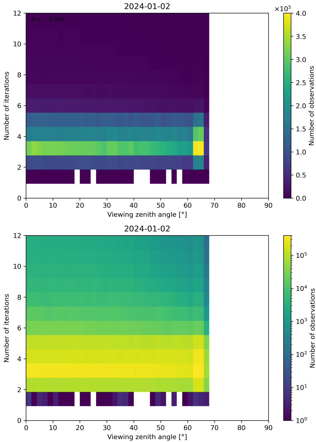
Figure 124: Scatter density plot of “Viewing zenith angle” against “Number of iterations” for 2024-01-01 to 2024-01-03.
