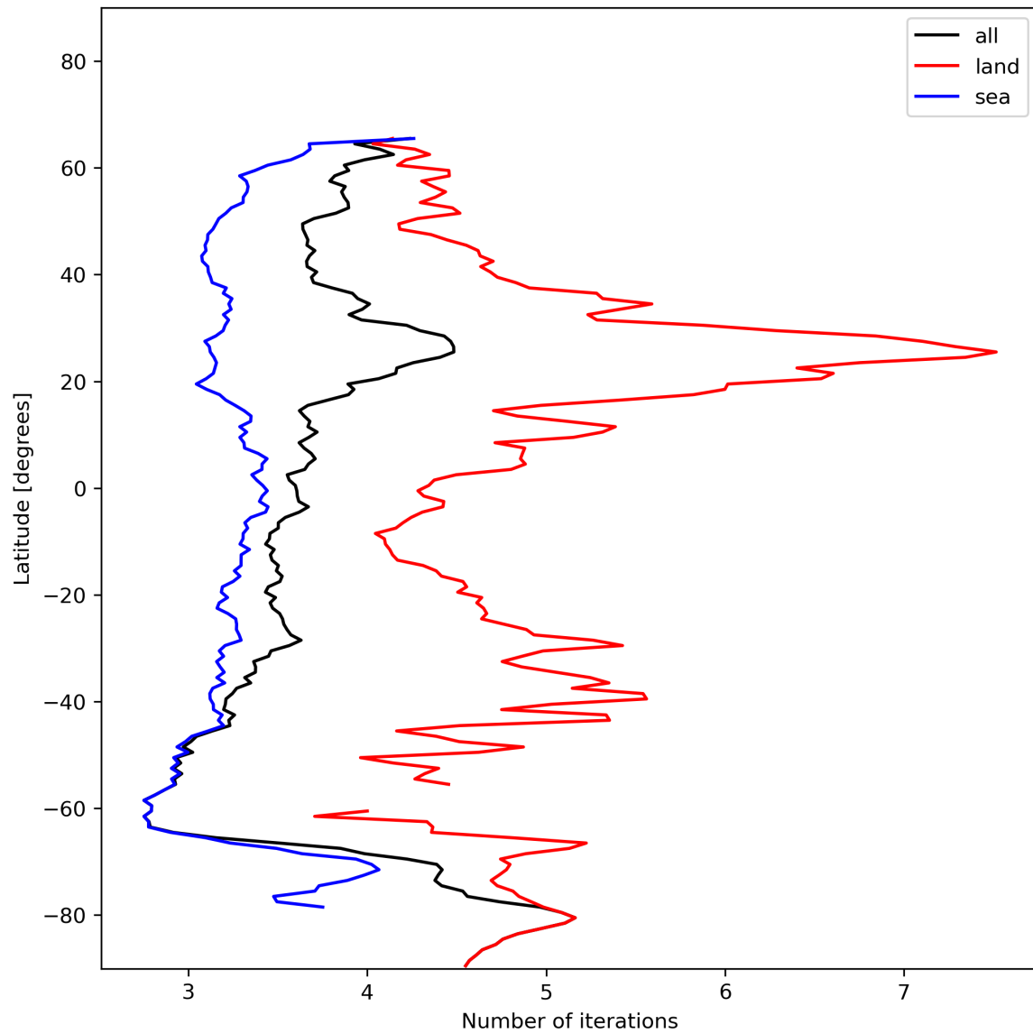
Figure 22: Zonal average of “Number of iterations” for 2024-01-01 to 2024-01-03.
