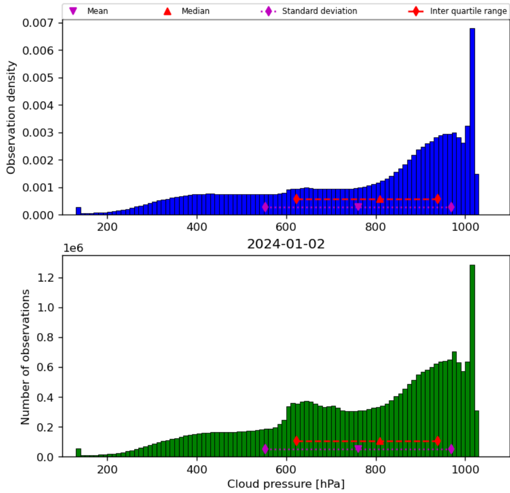
Figure 30: Histogram of “Cloud pressure” for 2024-01-01 to 2024-01-03
