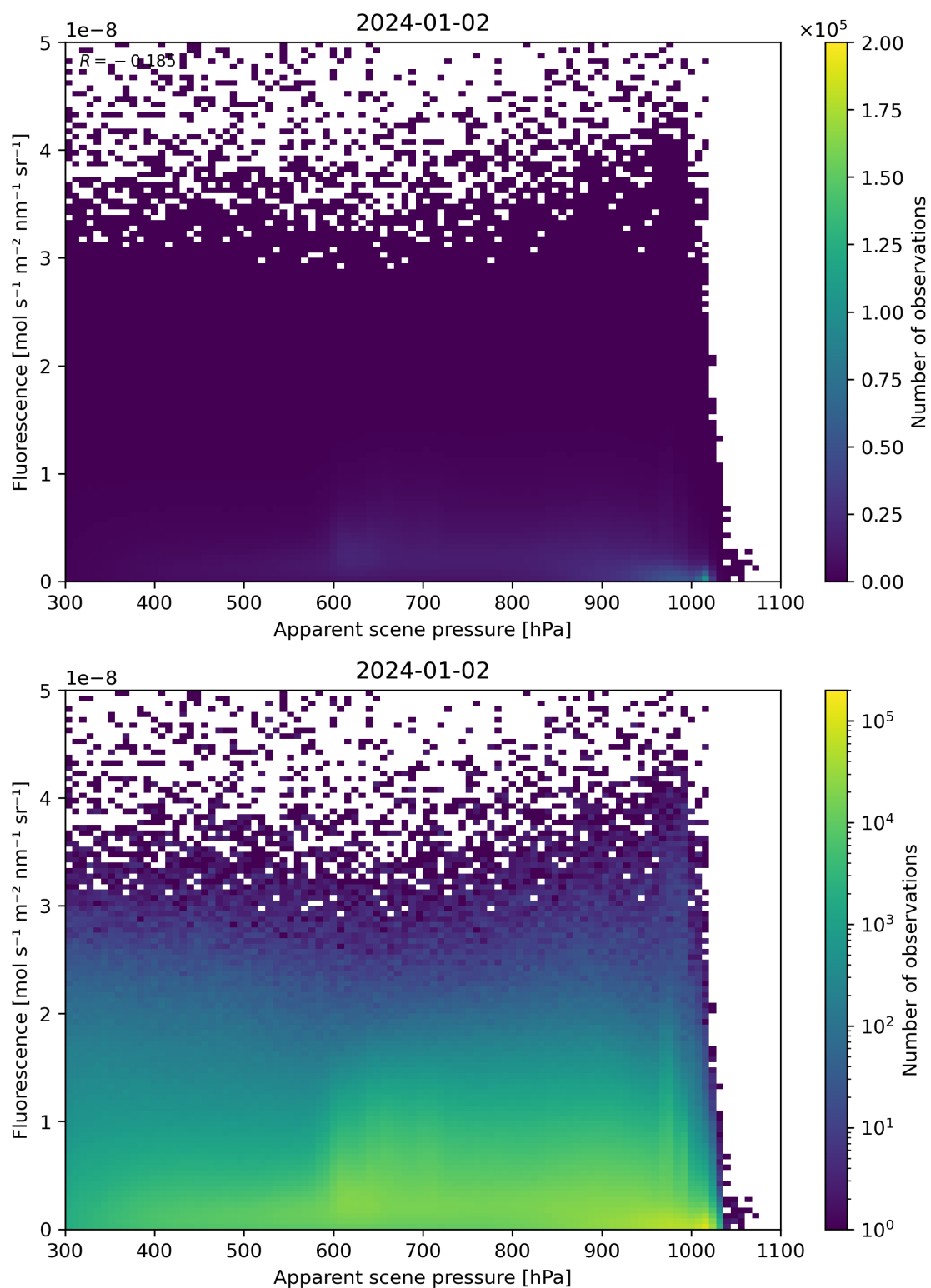
Figure 64: Scatter density plot of “Apparent scene pressure” against “Fluorescence” for 2024-01-01 to 2024-01-03.
