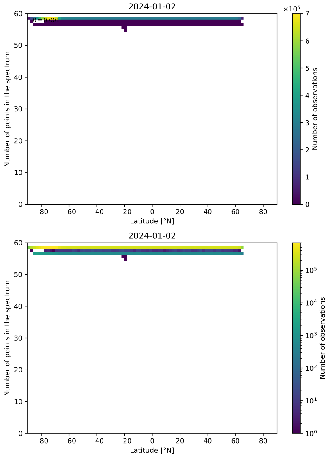
Figure 94: Scatter density plot of “Latitude” against “Number of points in the spectrum” for 2024-01-01 to 2024-01-03.
