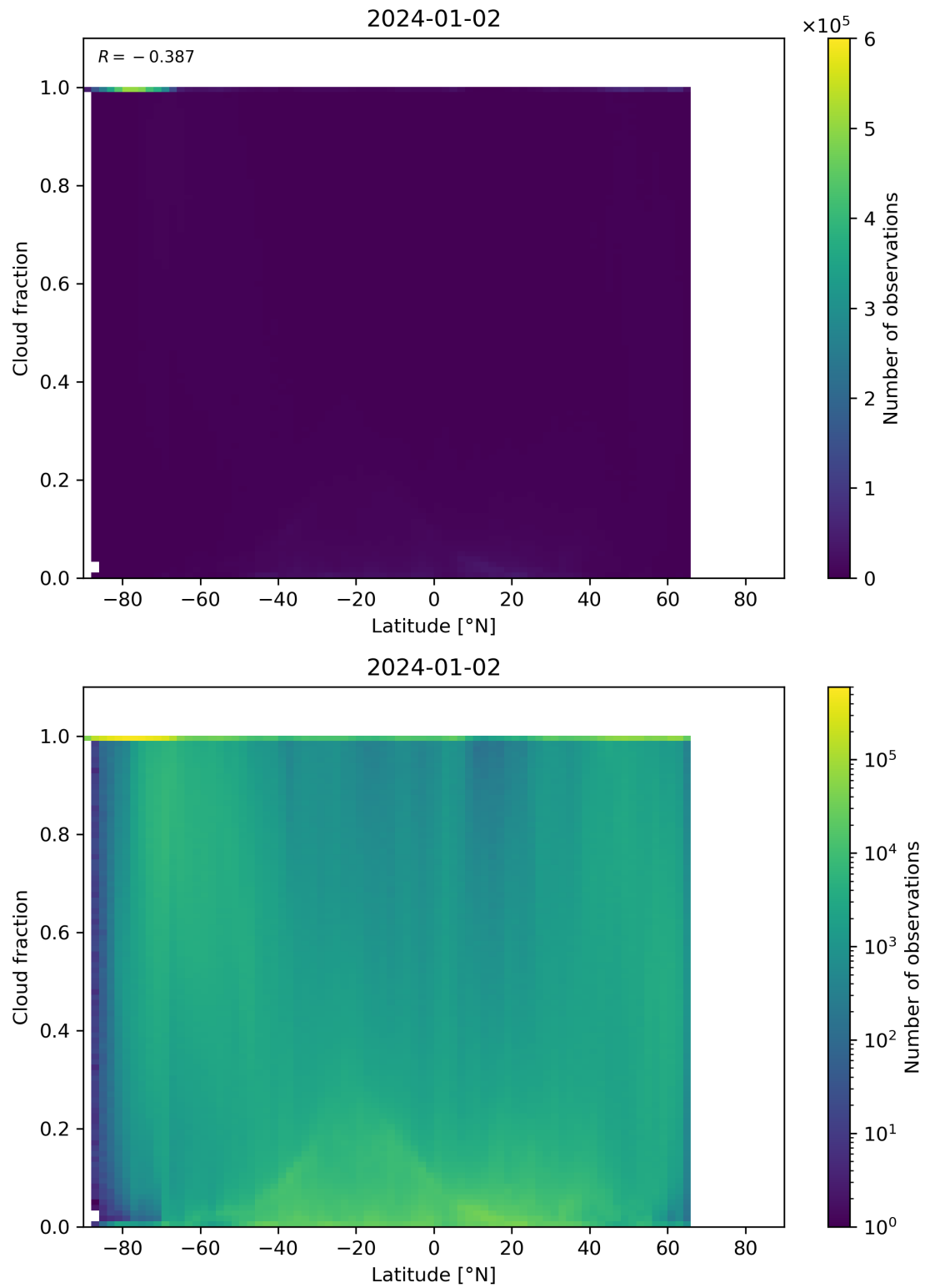
Figure 90: Scatter density plot of “Latitude” against “Cloud fraction” for 2024-01-01 to 2024-01-03.
