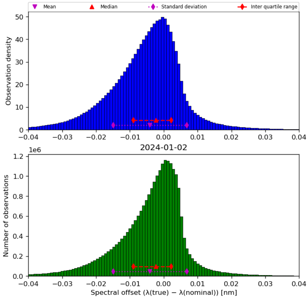
Figure 45: Histogram of “Spectral offset ( \lambda(\text{true}) - \lambda(\text{nominal}) )” for 2024-01-01 to 2024-01-03
