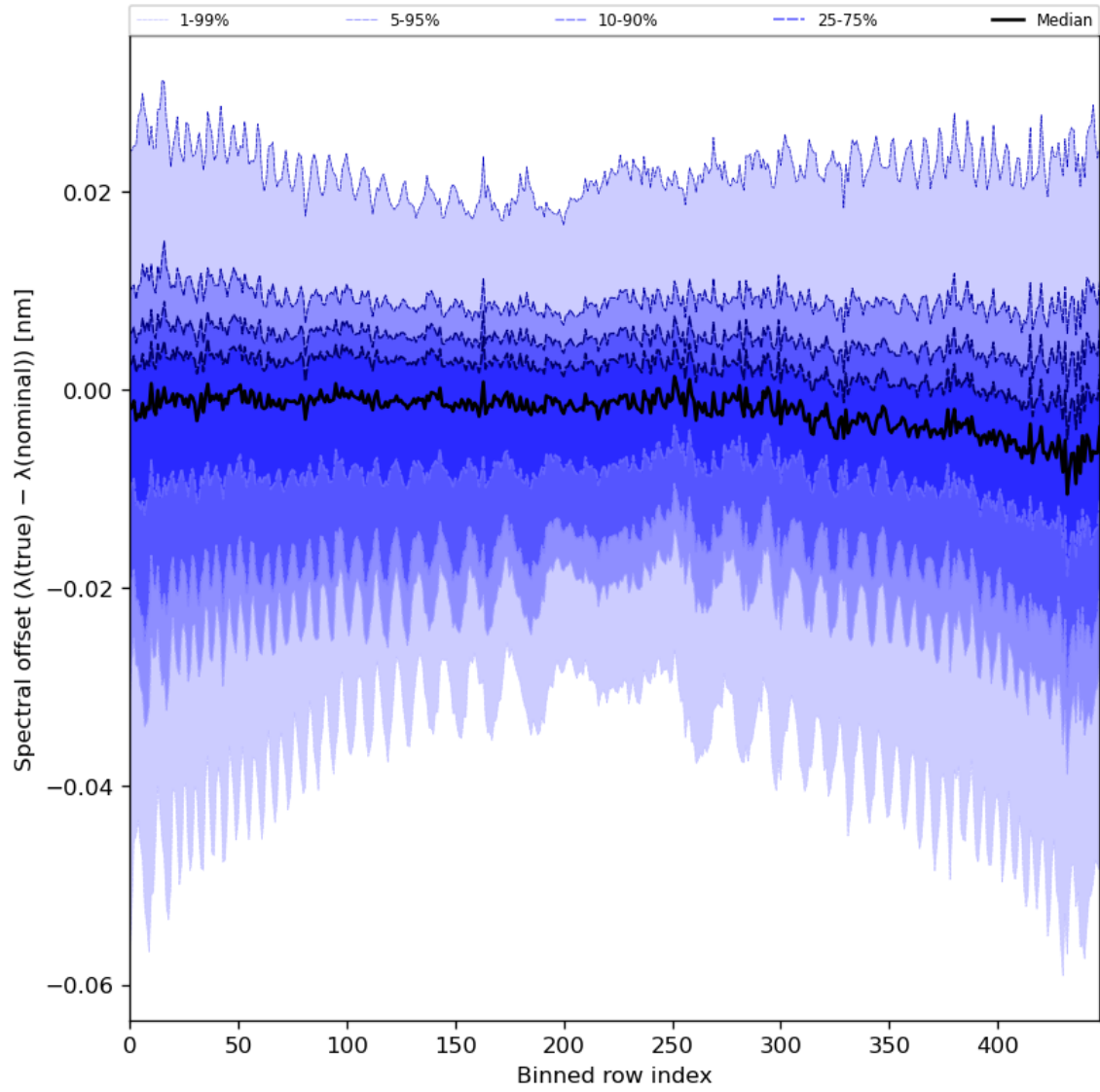
Figure 62: Along track statistics of “Spectral offset ( \lambda(\text{true}) - \lambda(\text{nominal}) )” for 2024-01-01 to 2024-01-03
