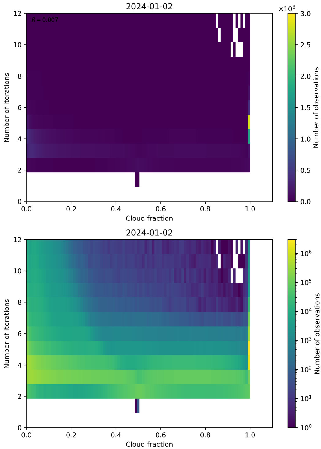
Figure 73: Scatter density plot of “Cloud fraction” against “Number of iterations” for 2024-01-01 to 2024-01-03.
