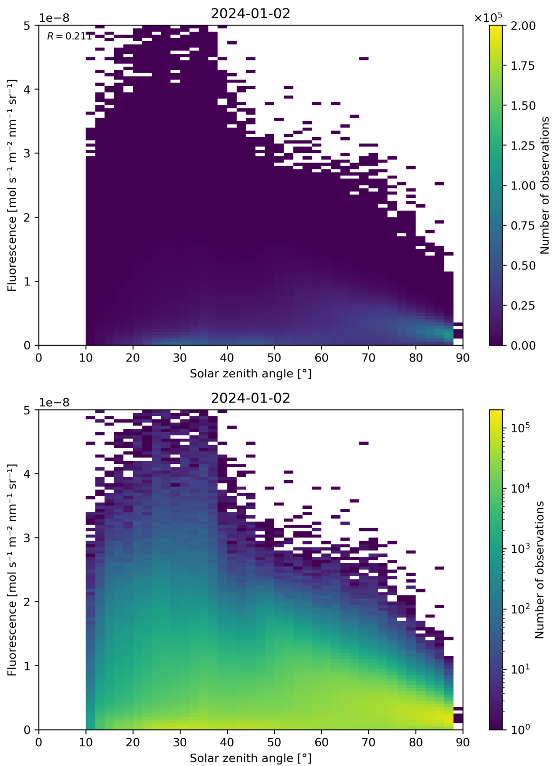
Figure 112: Scatter density plot of “Solar zenith angle” against “Fluorescence” for 2024-01-01 to 2024-01-03.
