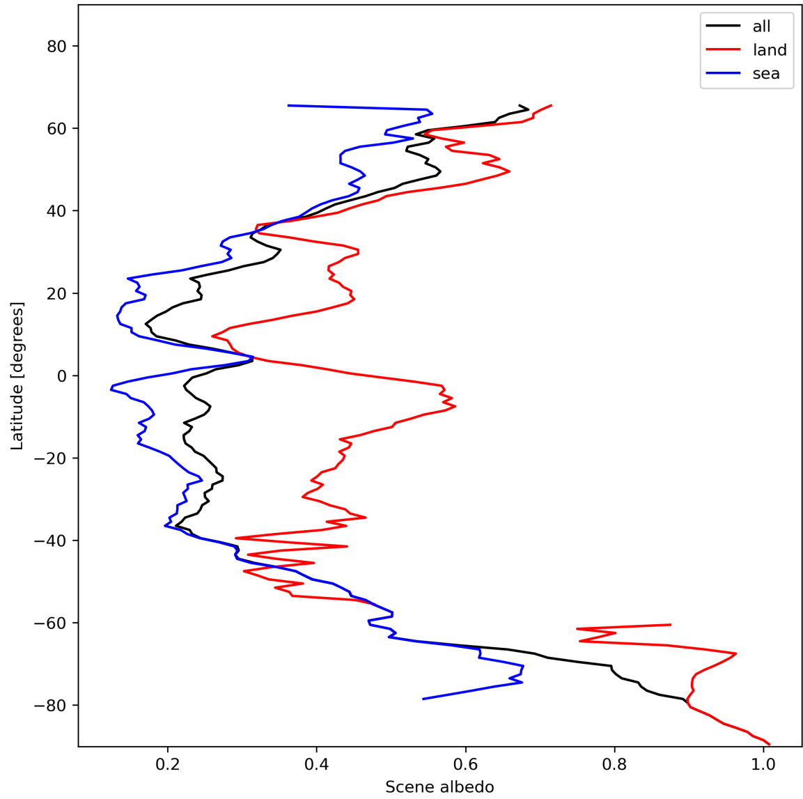
Figure 17: Zonal average of “Scene albedo” for 2024-01-01 to 2024-01-03.
