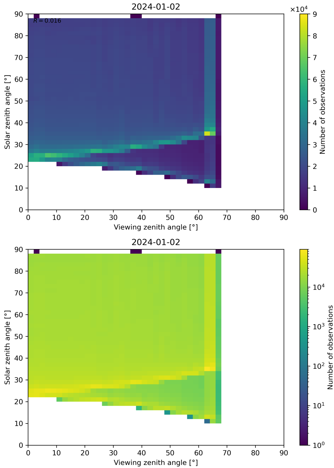
Figure 127: Scatter density plot of “Viewing zenith angle” against “Solar zenith angle” for 2024-01-01 to 2024-01-03.
