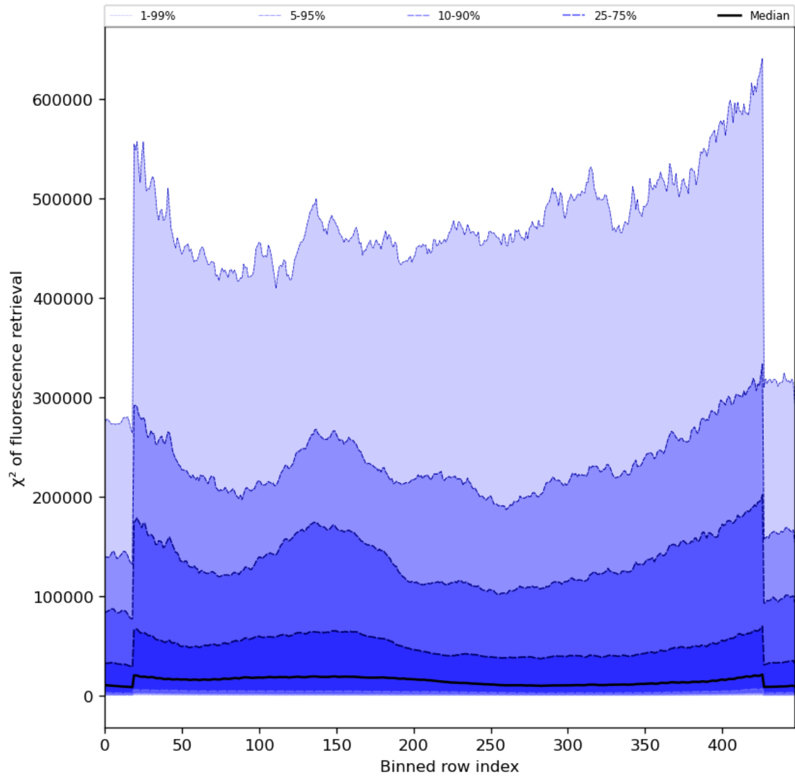
Figure 59: Along track statistics of “ \chi^2 of fluorescence retrieval” for 2024-01-01 to 2024-01-03
