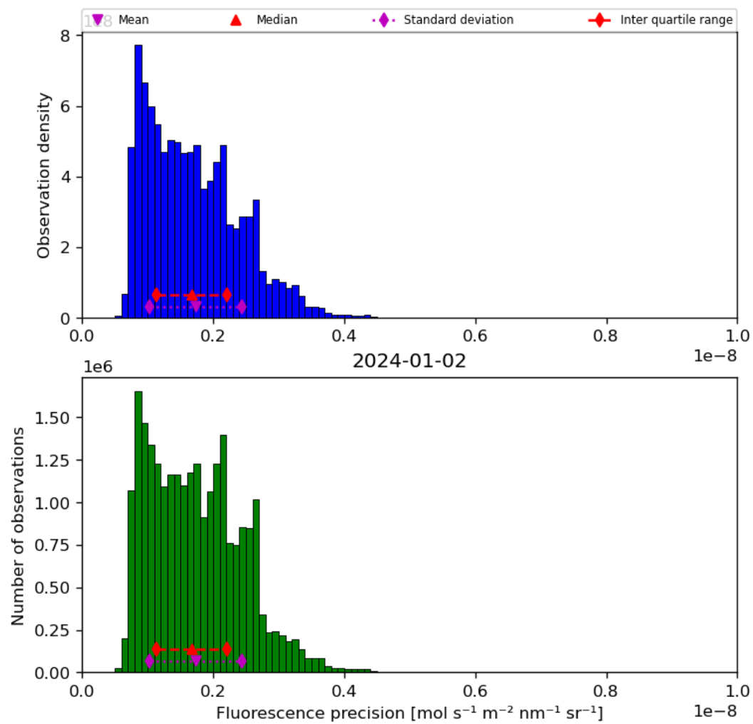
Figure 41: Histogram of “Fluorescence precision” for 2024-01-01 to 2024-01-03
