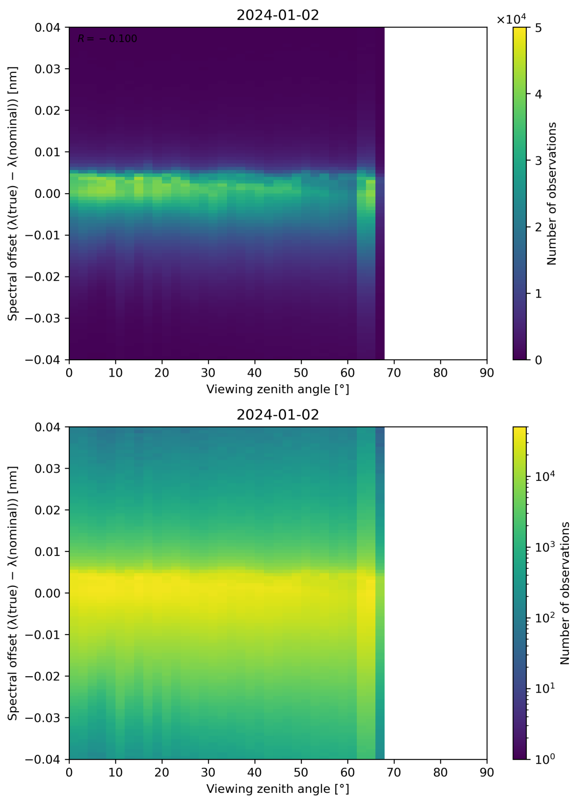
Figure 128: Scatter density plot of “Viewing zenith angle” against “Spectral offset ( \lambda(\text{true}) - \lambda(\text{nominal}) )” for 2024-01-01 to 2024-01-03.
