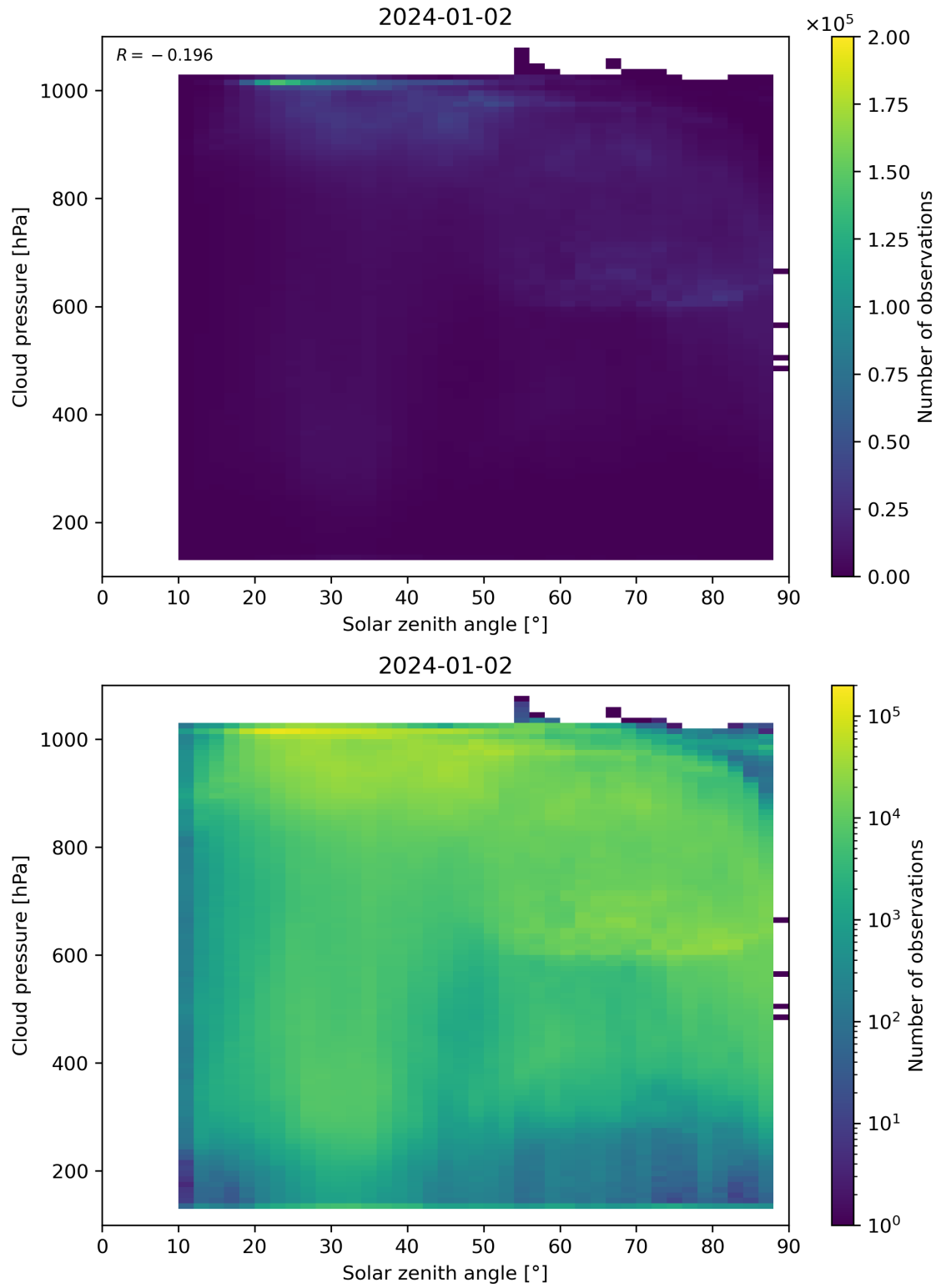
Figure 111: Scatter density plot of “Solar zenith angle” against “Cloud pressure” for 2024-01-01 to 2024-01-03.
