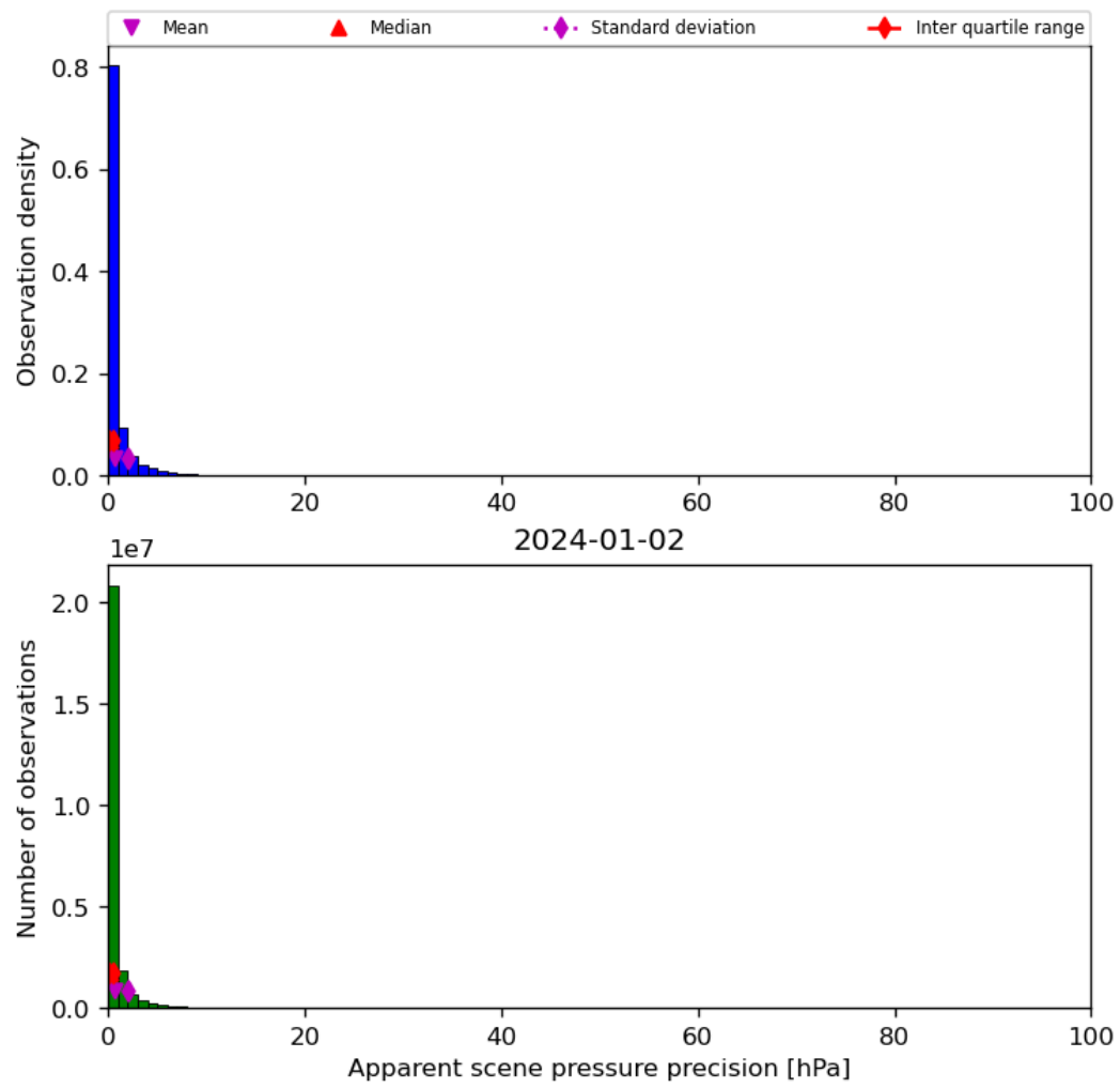
Figure 37: Histogram of “Apparent scene pressure precision” for 2024-01-01 to 2024-01-03
