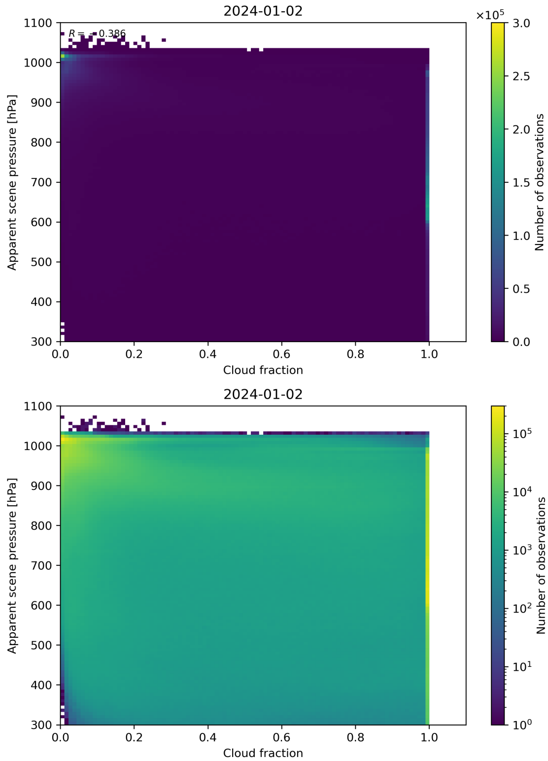
Figure 70: Scatter density plot of “Cloud fraction” against “Apparent scene pressure” for 2024-01-01 to 2024-01-03.
