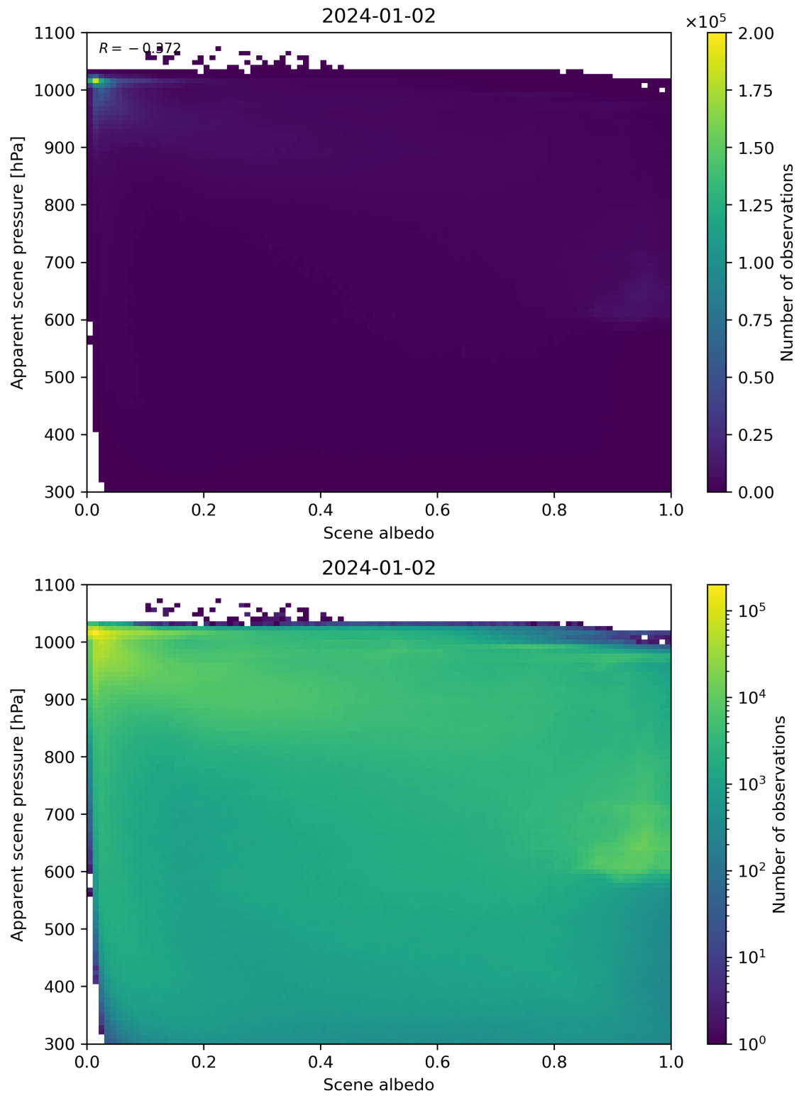
Figure 102: Scatter density plot of “Scene albedo” against “Apparent scene pressure” for 2024-01-01 to 2024-01-03.
