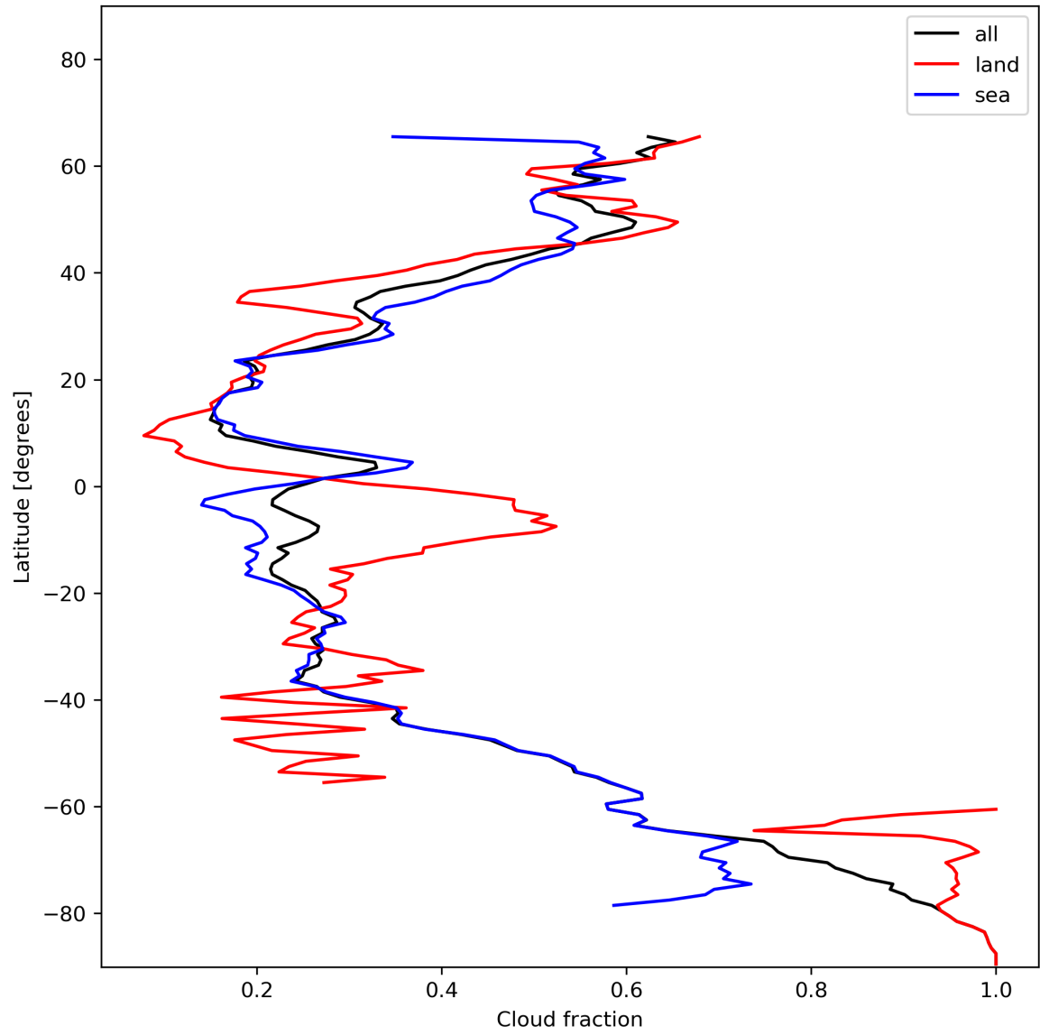
Figure 15: Zonal average of “Cloud fraction” for 2024-01-01 to 2024-01-03.
