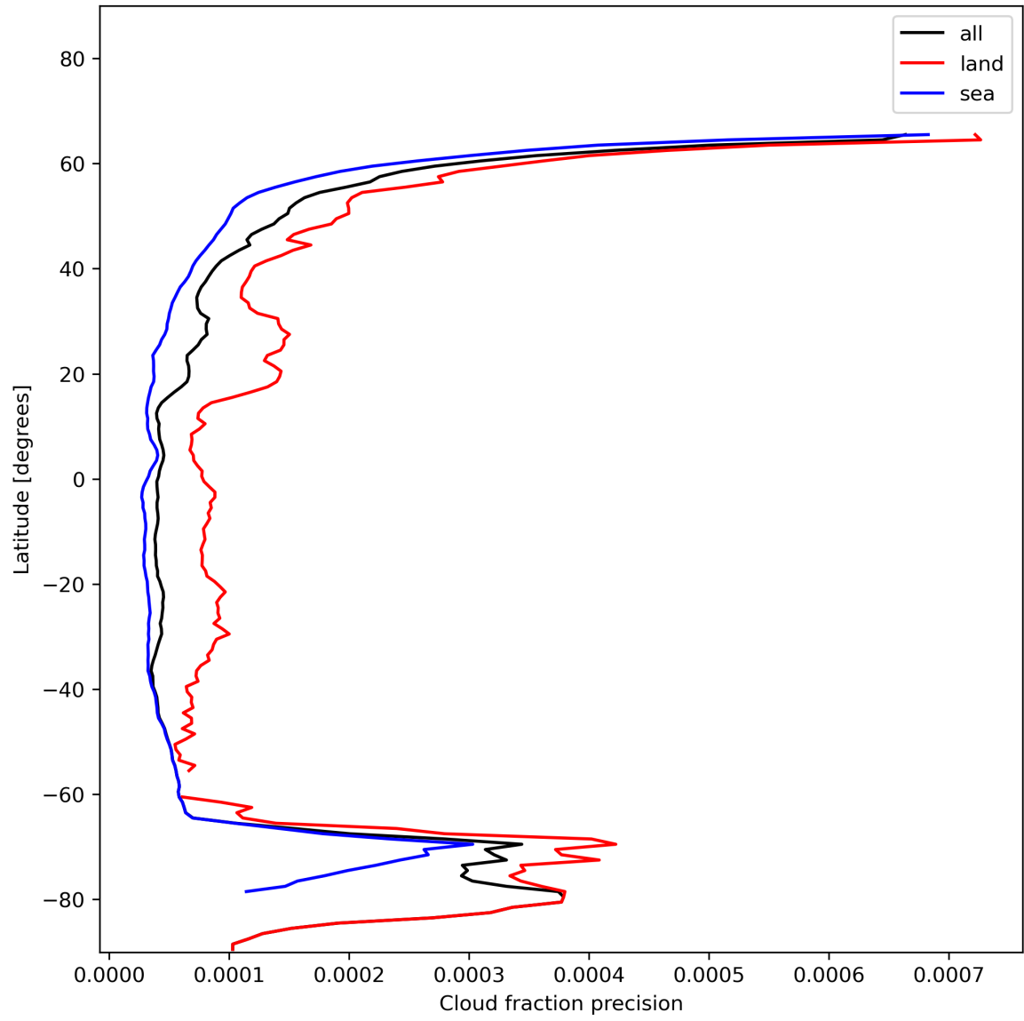
Figure 16: Zonal average of “Cloud fraction precision” for 2024-01-01 to 2024-01-03.
