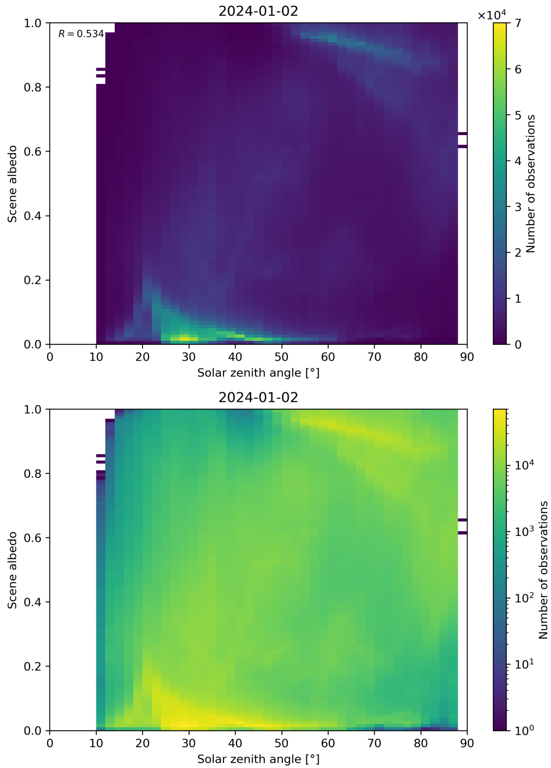
Figure 116: Scatter density plot of “Solar zenith angle” against “Scene albedo” for 2024-01-01 to 2024-01-03.
