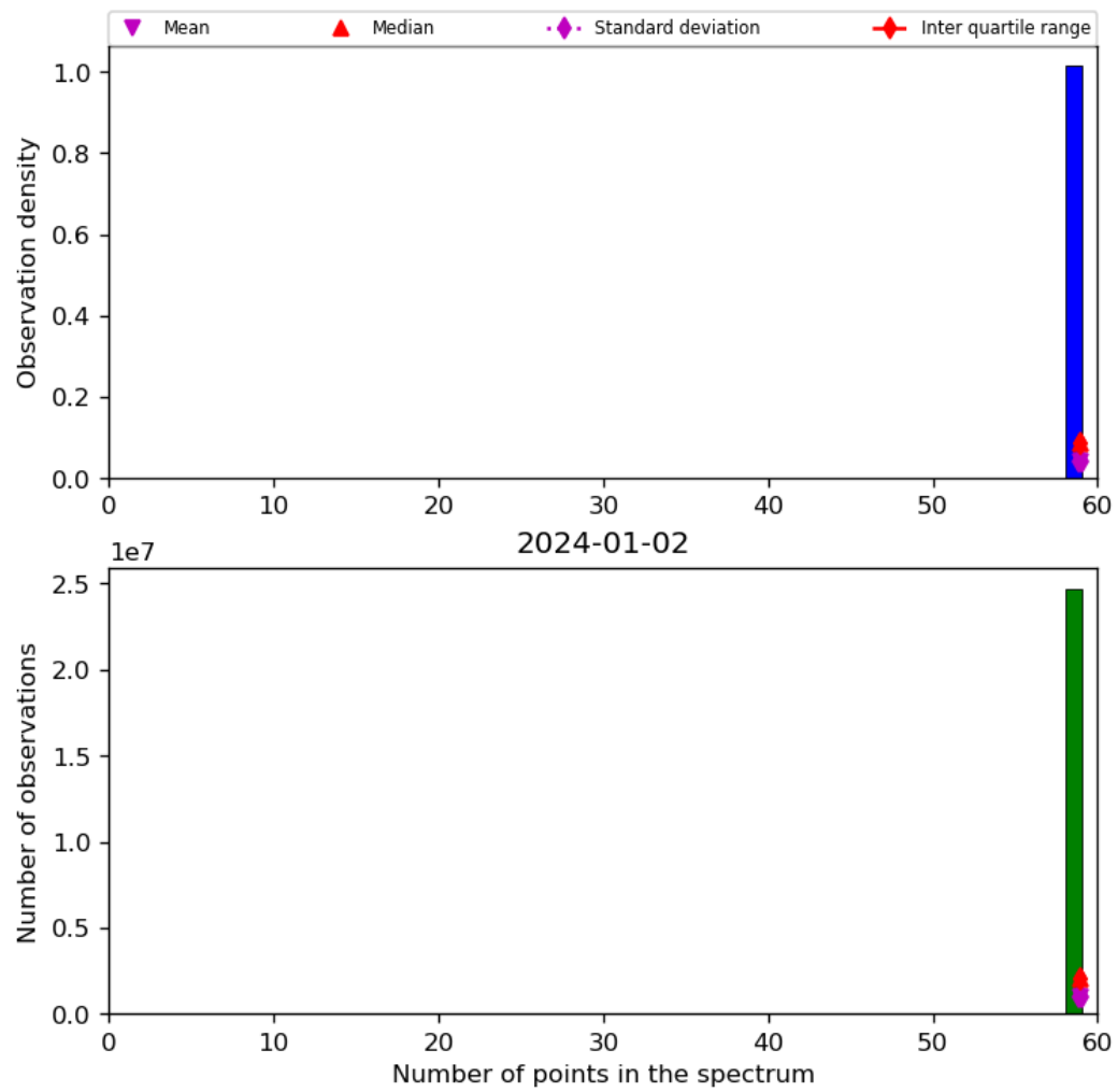
Figure 44: Histogram of “Number of points in the spectrum” for 2024-01-01 to 2024-01-03
