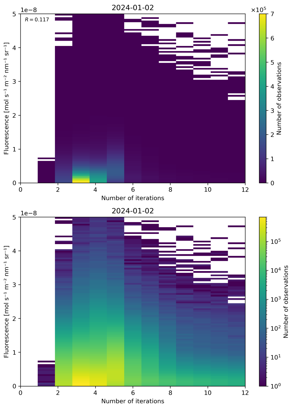
Figure 98: Scatter density plot of “Number of iterations” against “Fluorescence” for 2024-01-01 to 2024-01-03.
