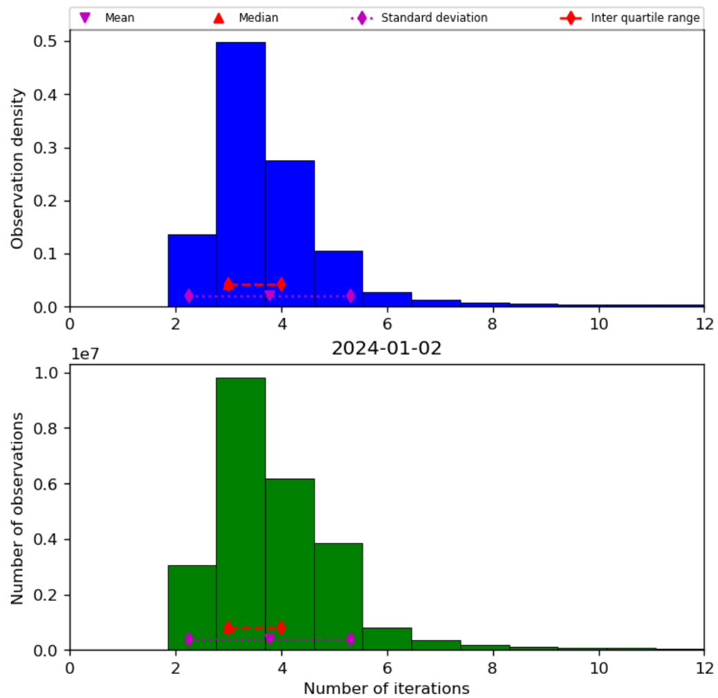
Figure 39: Histogram of “Number of iterations” for 2024-01-01 to 2024-01-03
