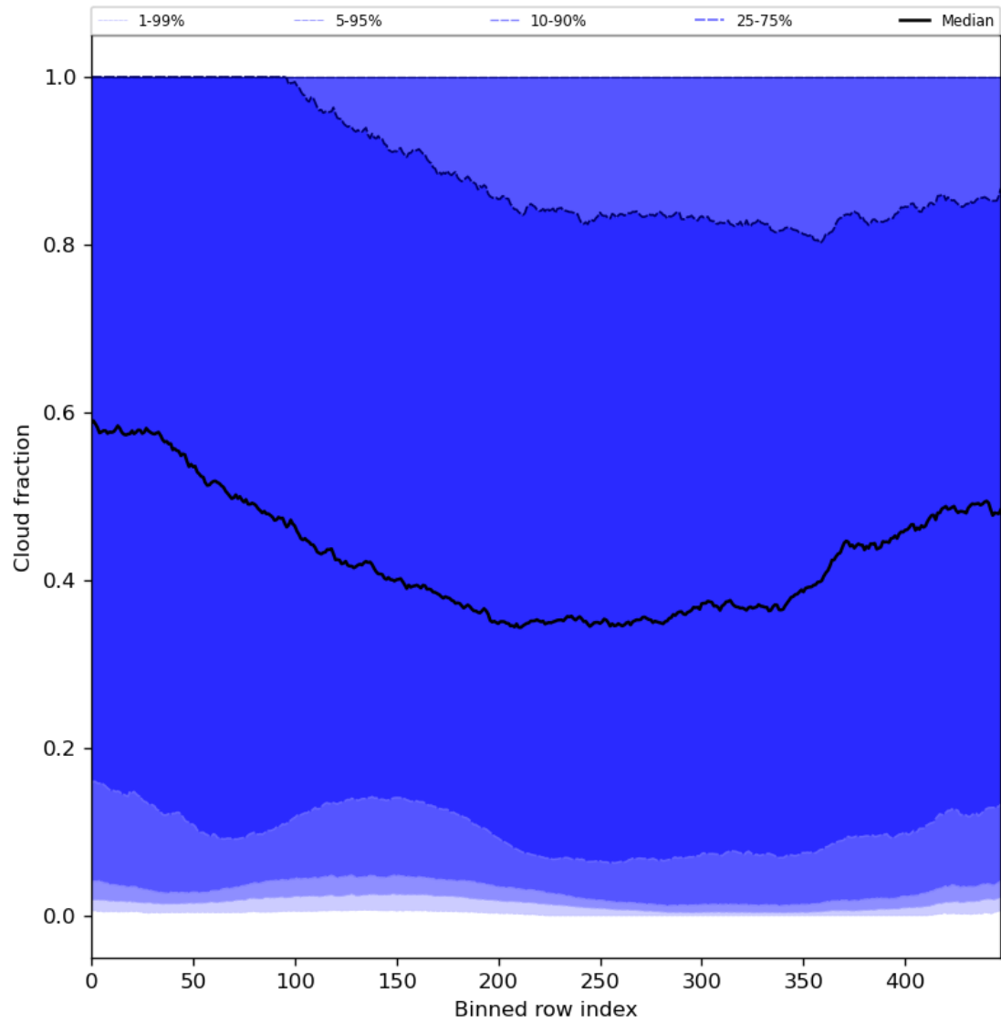
Figure 49: Along track statistics of “Cloud fraction” for 2024-01-01 to 2024-01-03
