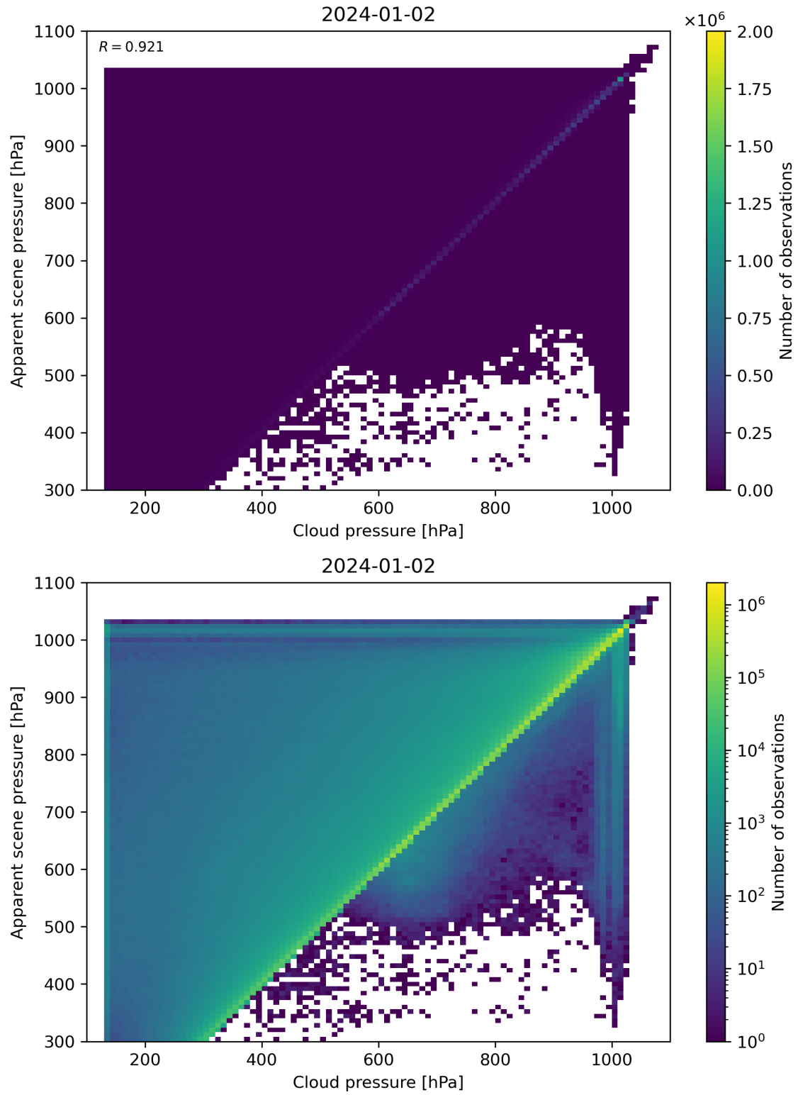
Figure 77: Scatter density plot of “Cloud pressure” against “Apparent scene pressure” for 2024-01-01 to 2024-01-03.
