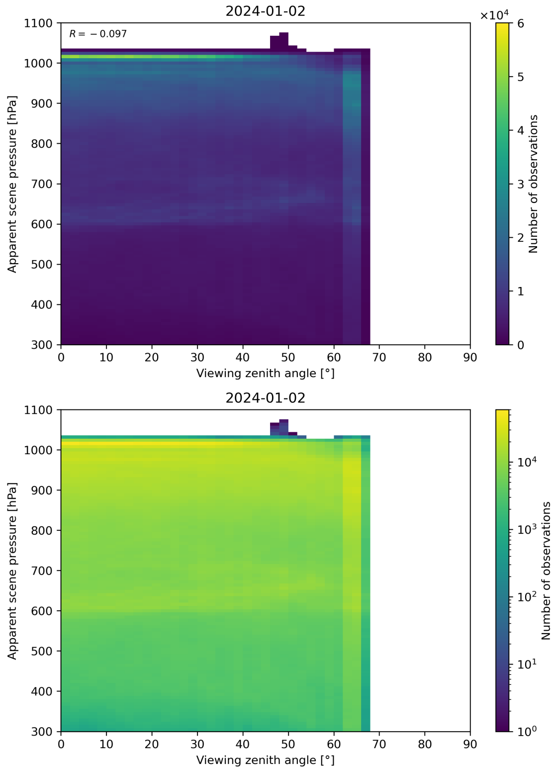
Figure 118: Scatter density plot of “Viewing zenith angle” against “Apparent scene pressure” for 2024-01-01 to 2024-01-03.
