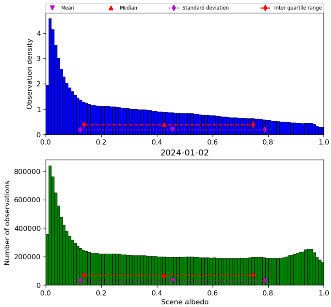
Figure 34: Histogram of “Scene albedo” for 2024-01-01 to 2024-01-03
