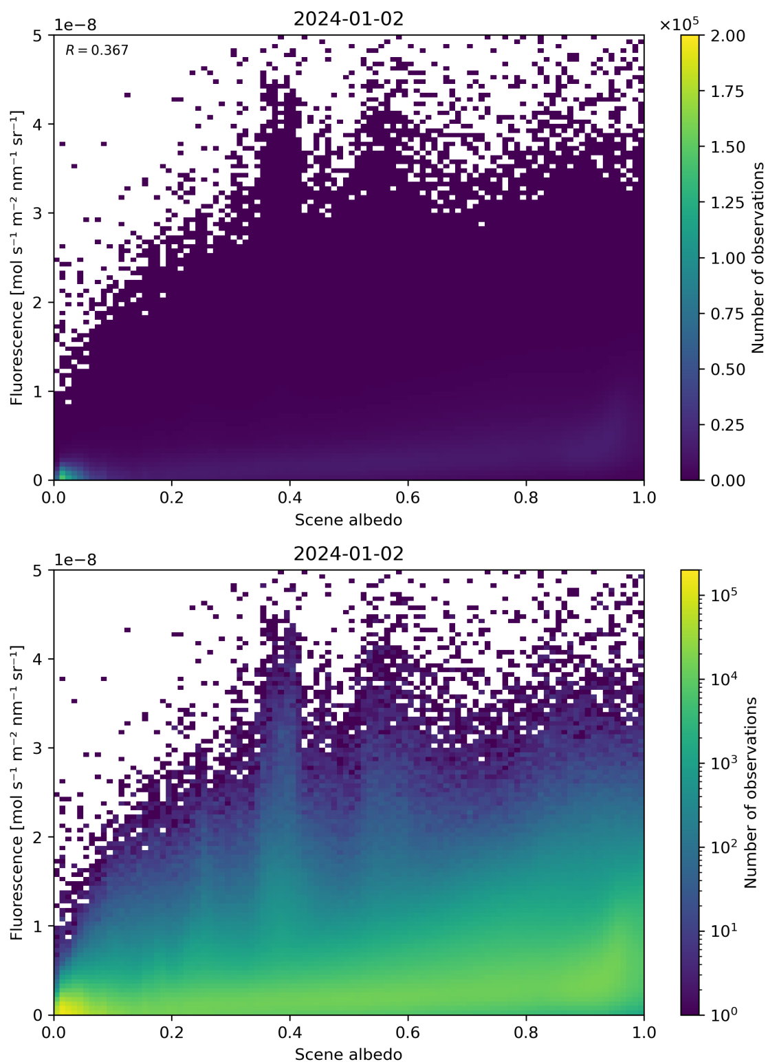
Figure 104: Scatter density plot of “Scene albedo” against “Fluorescence” for 2024-01-01 to 2024-01-03.
