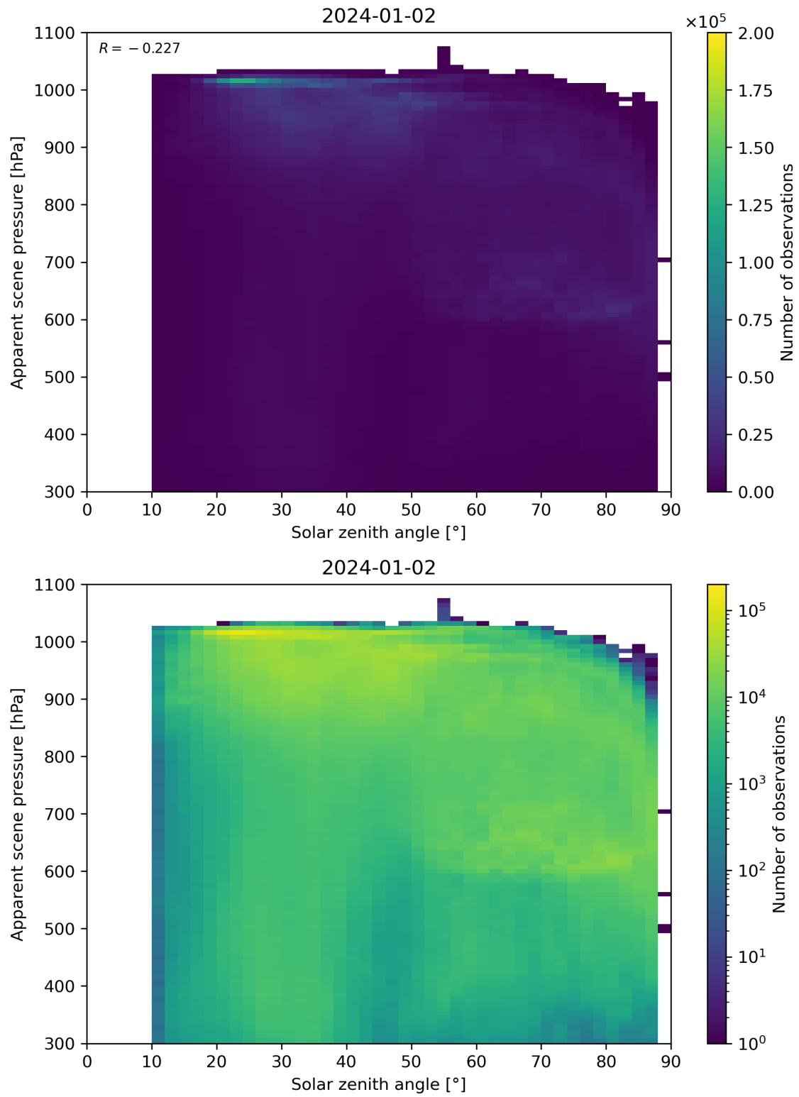
Figure 108: Scatter density plot of “Solar zenith angle” against “Apparent scene pressure” for 2024-01-01 to 2024-01-03.
