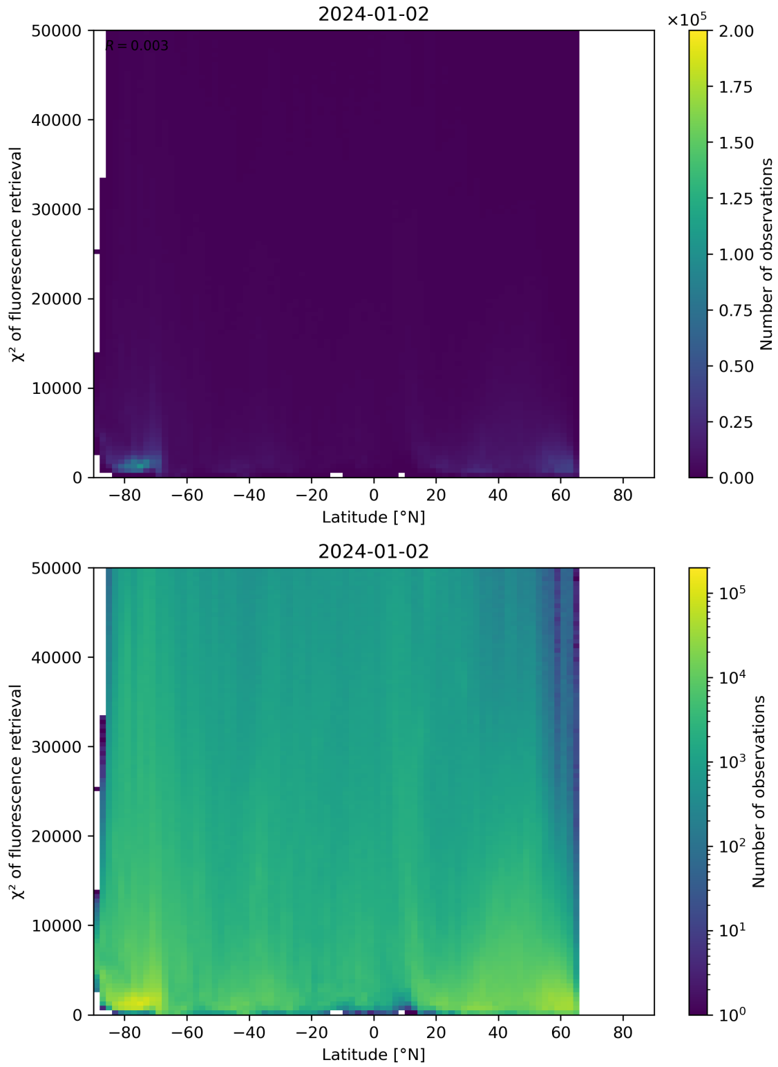
Figure 89: Scatter density plot of “Latitude” against “ \chi^2 of fluorescence retrieval” for 2024-01-01 to 2024-01-03.
