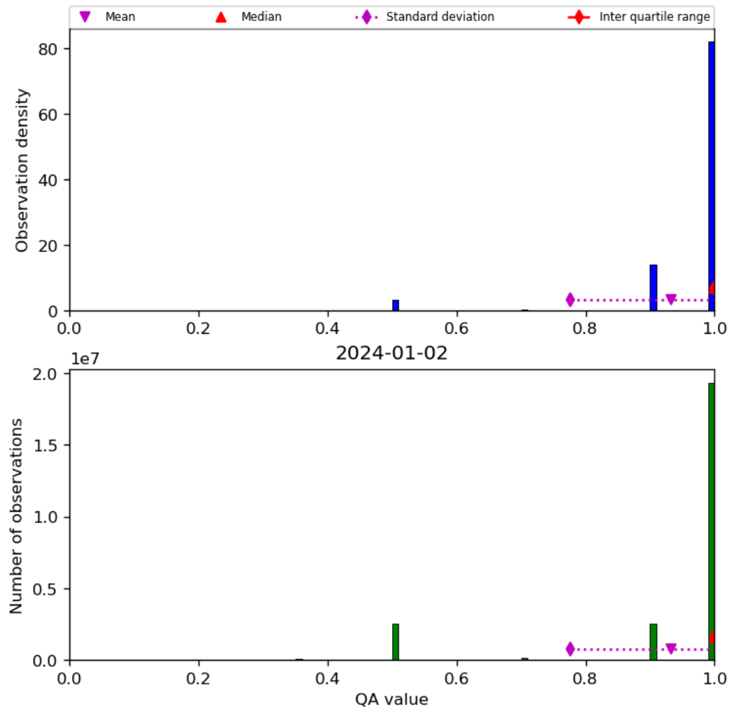
Figure 29: Histogram of “QA value” for 2024-01-01 to 2024-01-03
