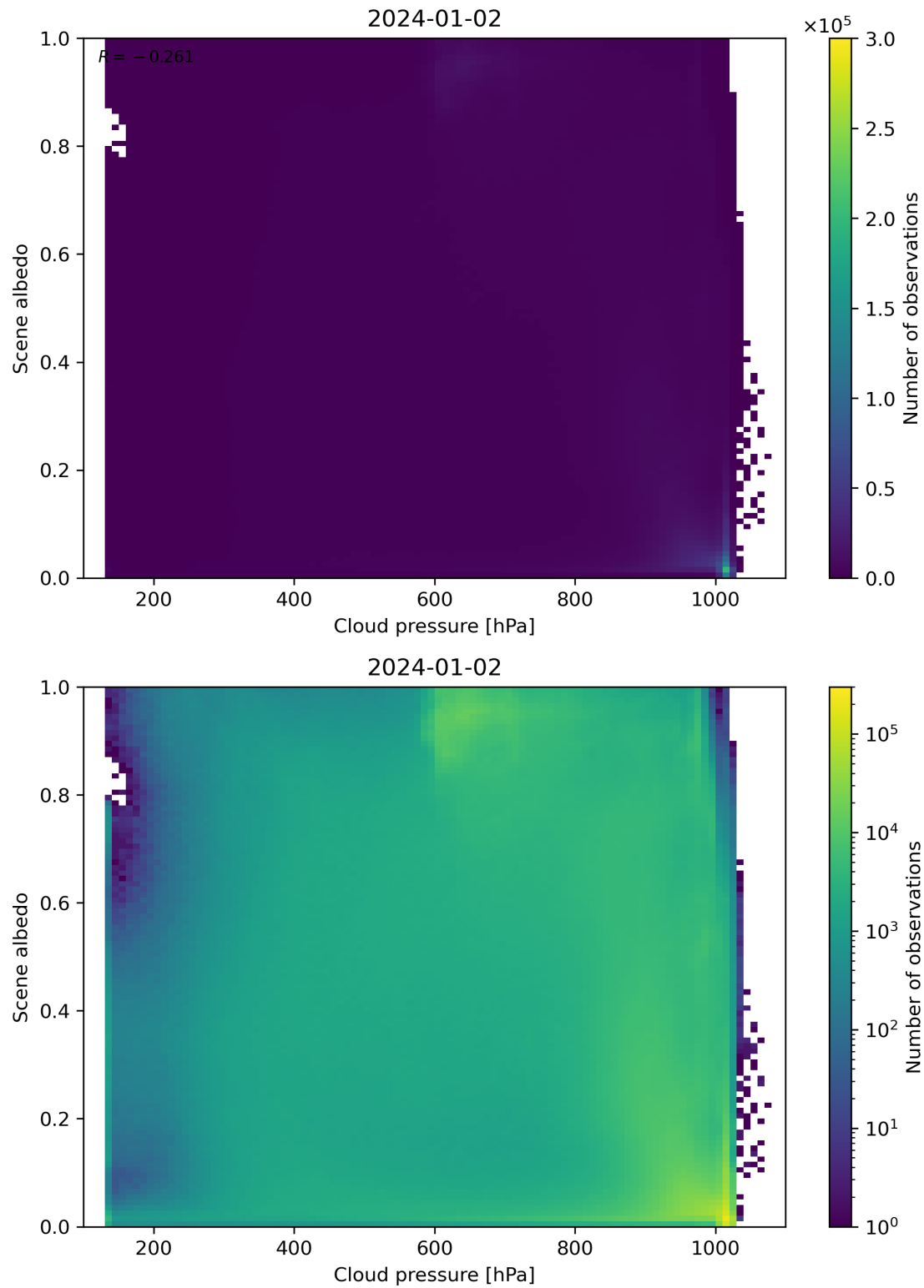
Figure 83: Scatter density plot of “Cloud pressure” against “Scene albedo” for 2024-01-01 to 2024-01-03.
