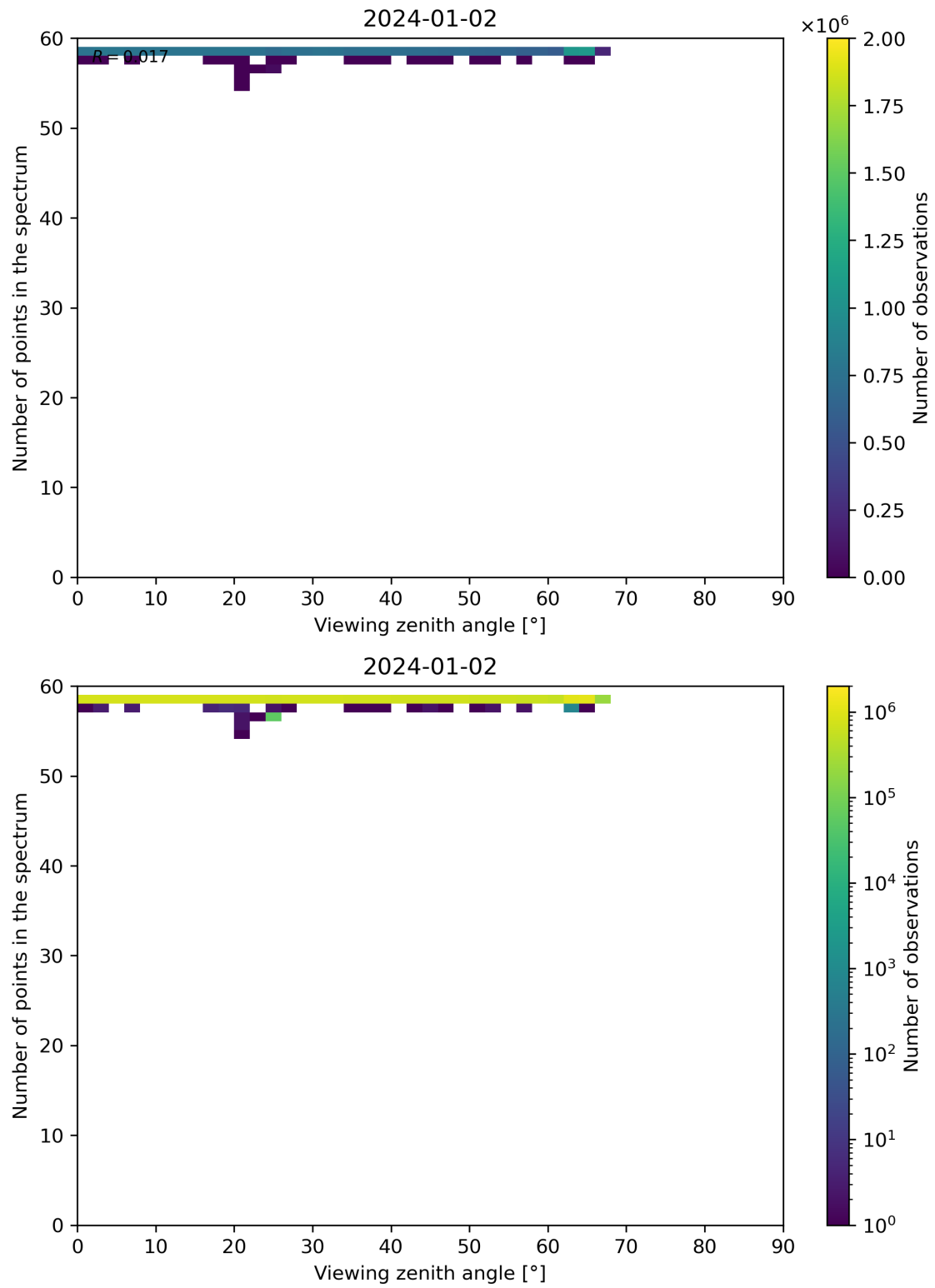
Figure 125: Scatter density plot of “Viewing zenith angle” against “Number of points in the spectrum” for 2024-01-01 to 2024-01-03.
