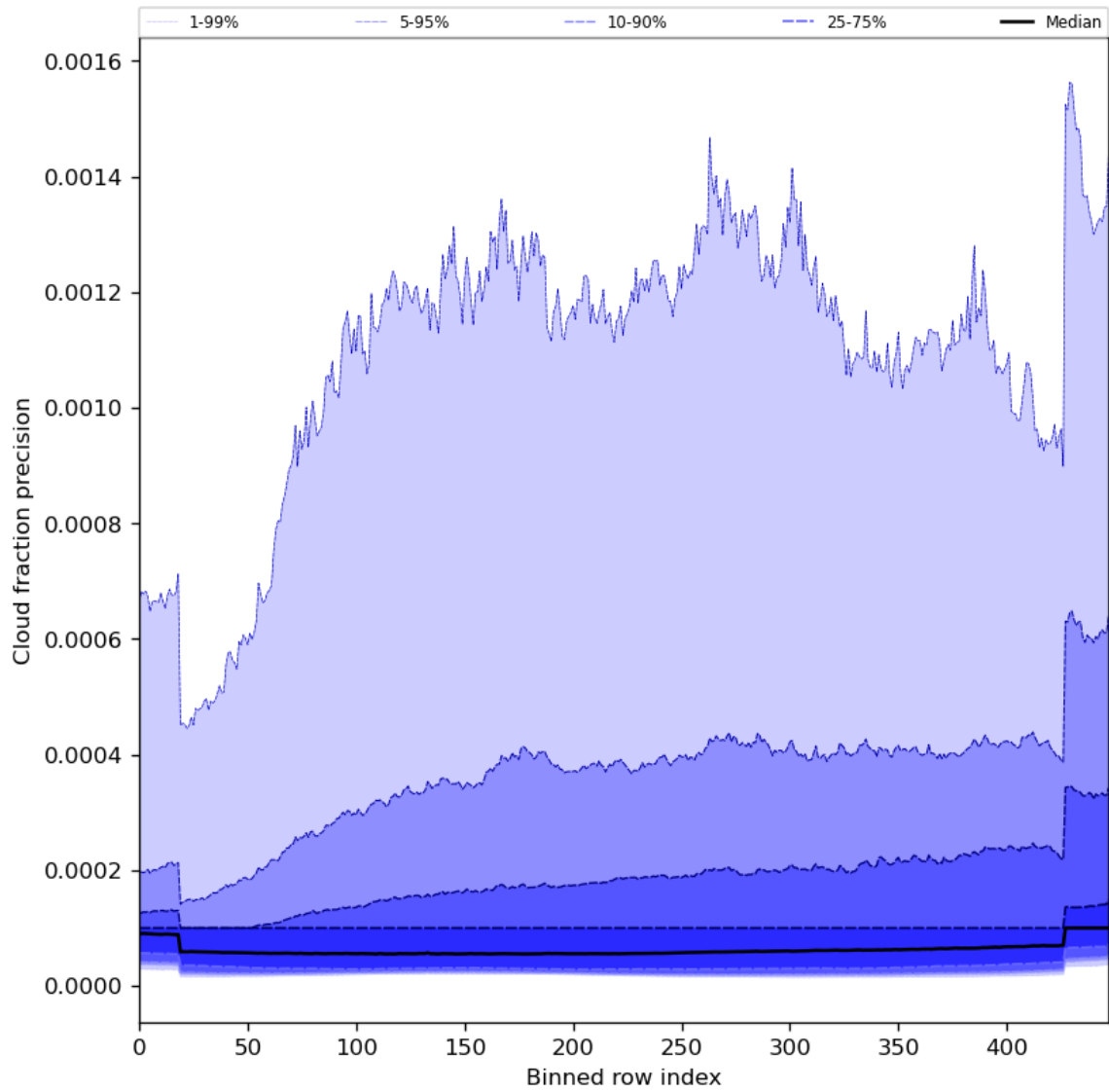
Figure 50: Along track statistics of “Cloud fraction precision” for 2024-01-01 to 2024-01-03
