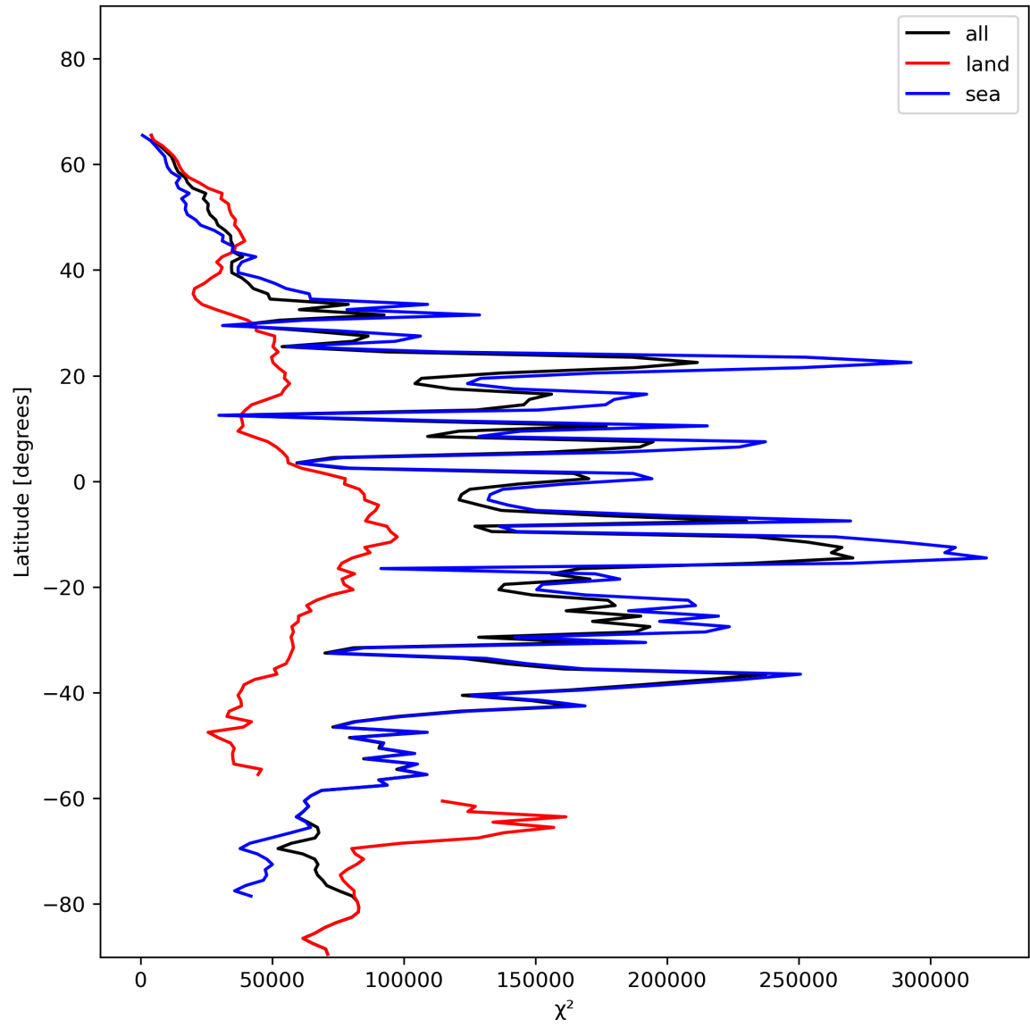
Figure 21: Zonal average of “ \chi^2 ” for 2024-01-01 to 2024-01-03.
