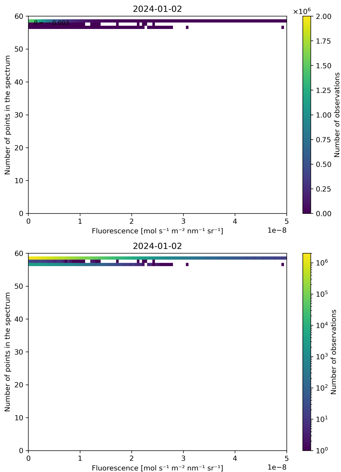
Figure 86: Scatter density plot of “Fluorescence” against “Number of points in the spectrum” for 2024-01-01 to 2024-01-03.
