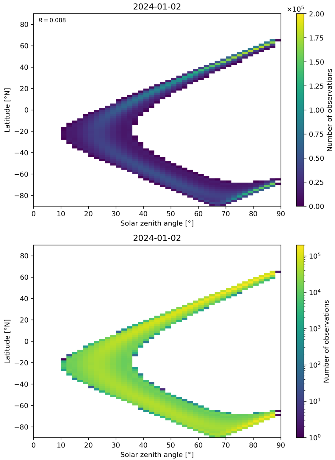
Figure 113: Scatter density plot of “Solar zenith angle” against “Latitude” for 2024-01-01 to 2024-01-03.
