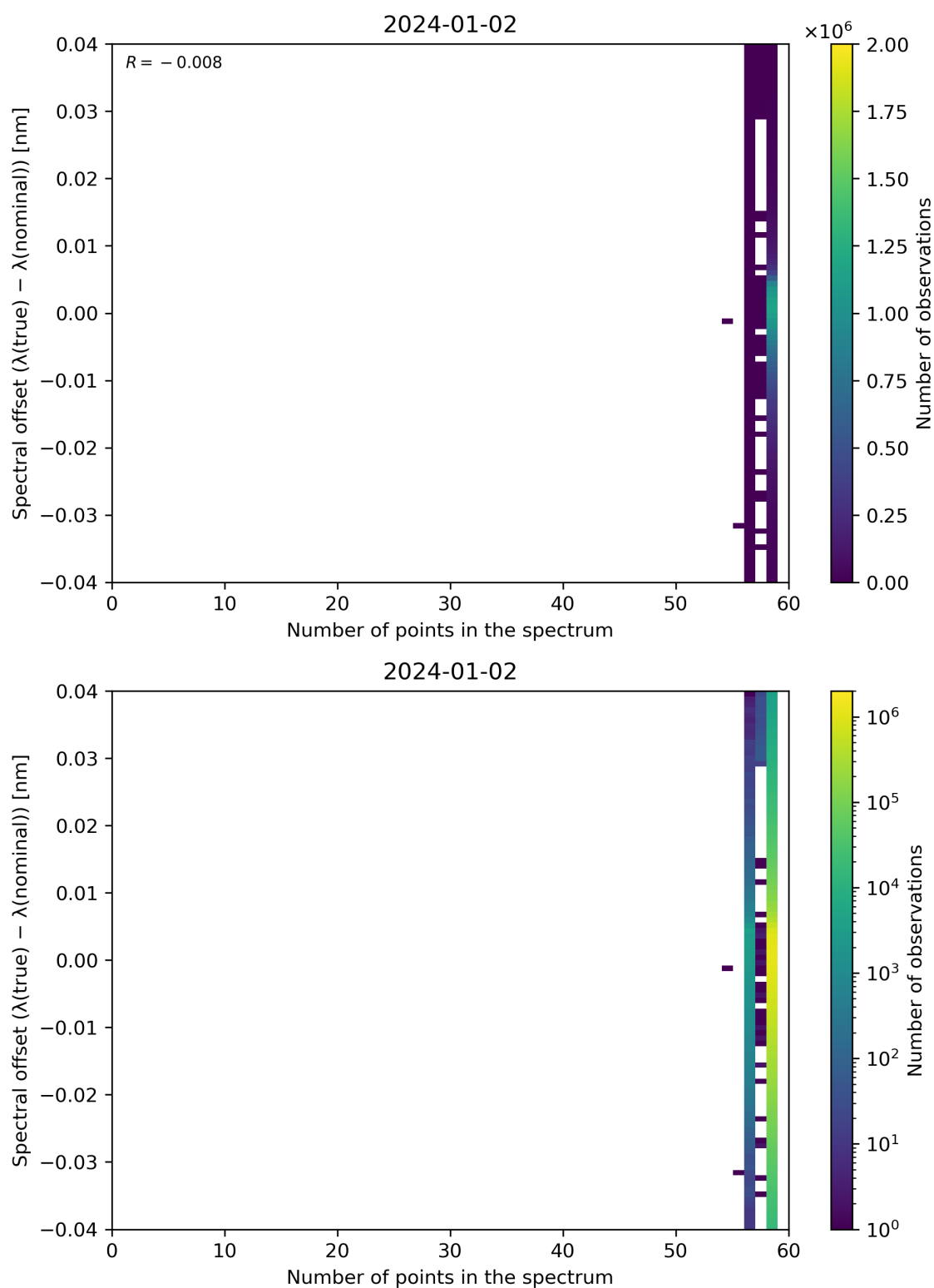
Figure 101: Scatter density plot of “Number of points in the spectrum” against “Spectral offset ( \lambda(\text{true}) - \lambda(\text{nominal}) )” for 2024-01-01 to 2024-01-03.
