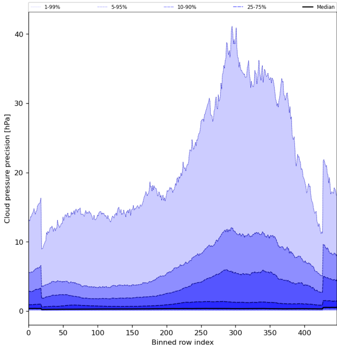
Figure 48: Along track statistics of “Cloud pressure precision” for 2024-01-01 to 2024-01-03
