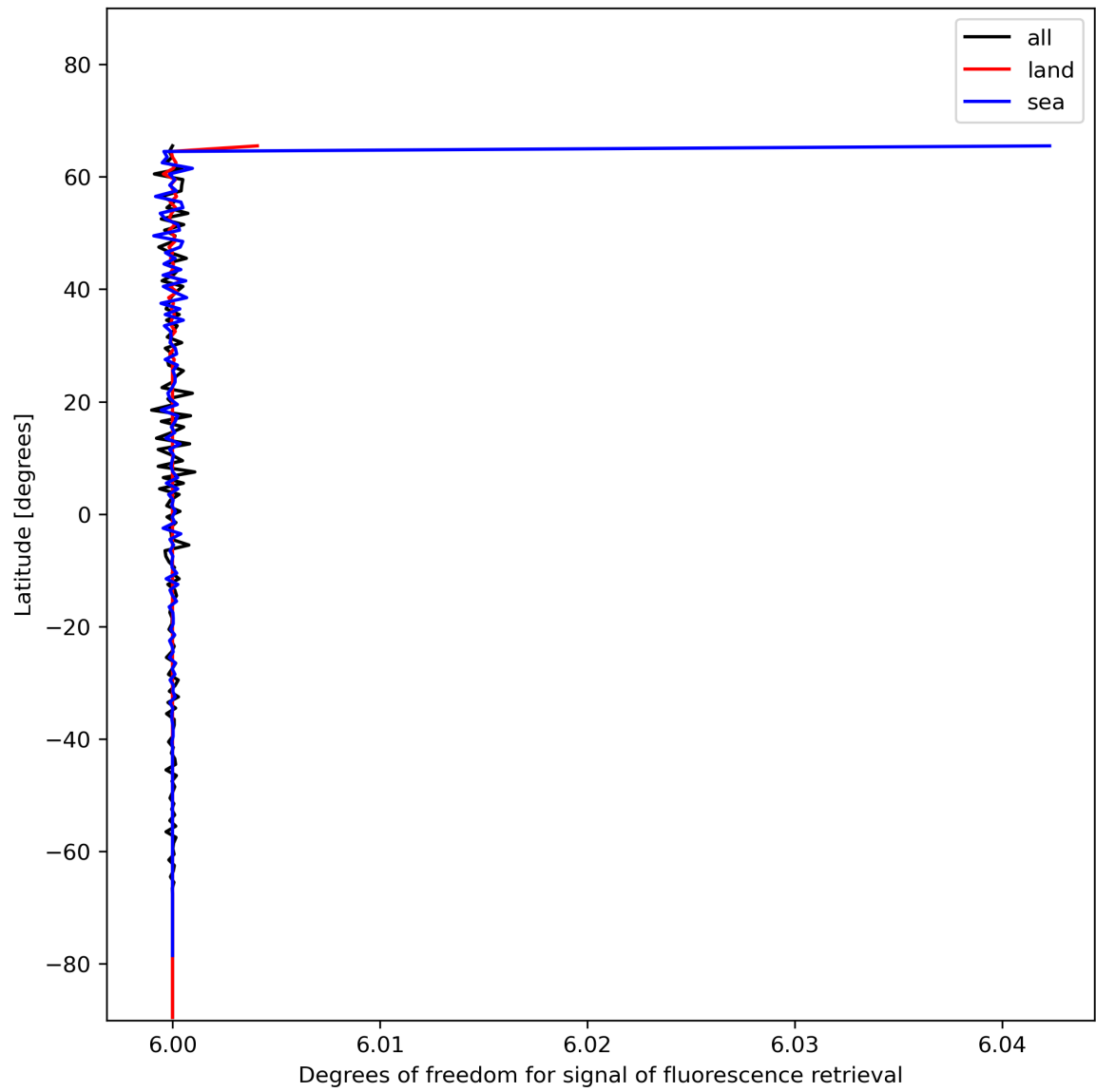
Figure 26: Zonal average of “Degrees of freedom for signal of fluorescence retrieval” for 2024-01-01 to 2024-01-03.
