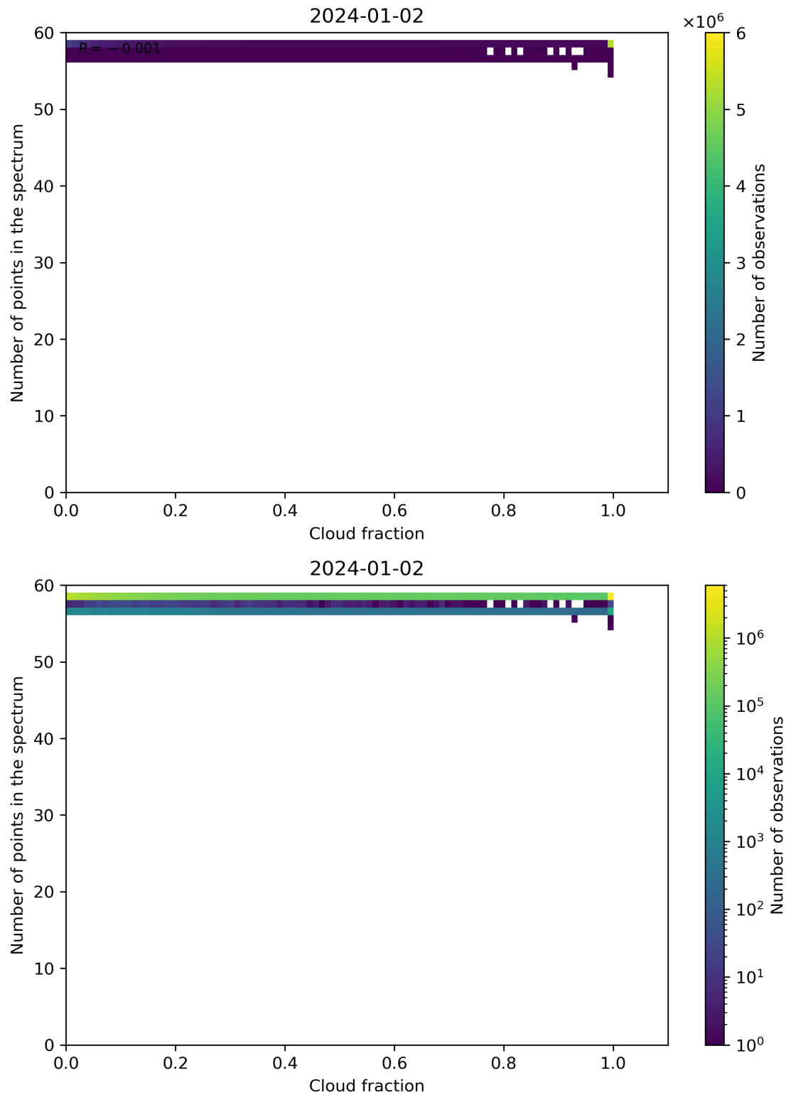
Figure 74: Scatter density plot of “Cloud fraction” against “Number of points in the spectrum” for 2024-01-01 to 2024-01-03.
