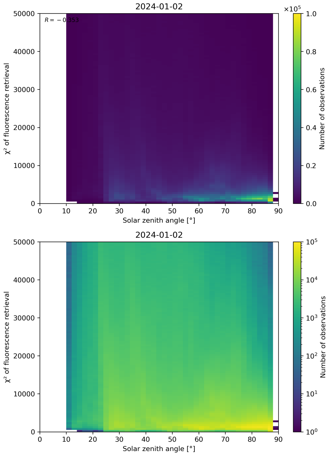
Figure 109: Scatter density plot of “Solar zenith angle” against “ \chi^2 of fluorescence retrieval” for 2024-01-01 to 2024-01-03.
