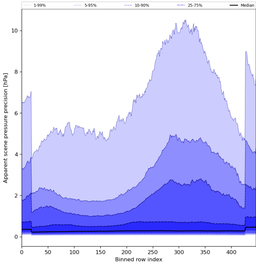
Figure 54: Along track statistics of “Apparent scene pressure precision” for 2024-01-01 to 2024-01-03
