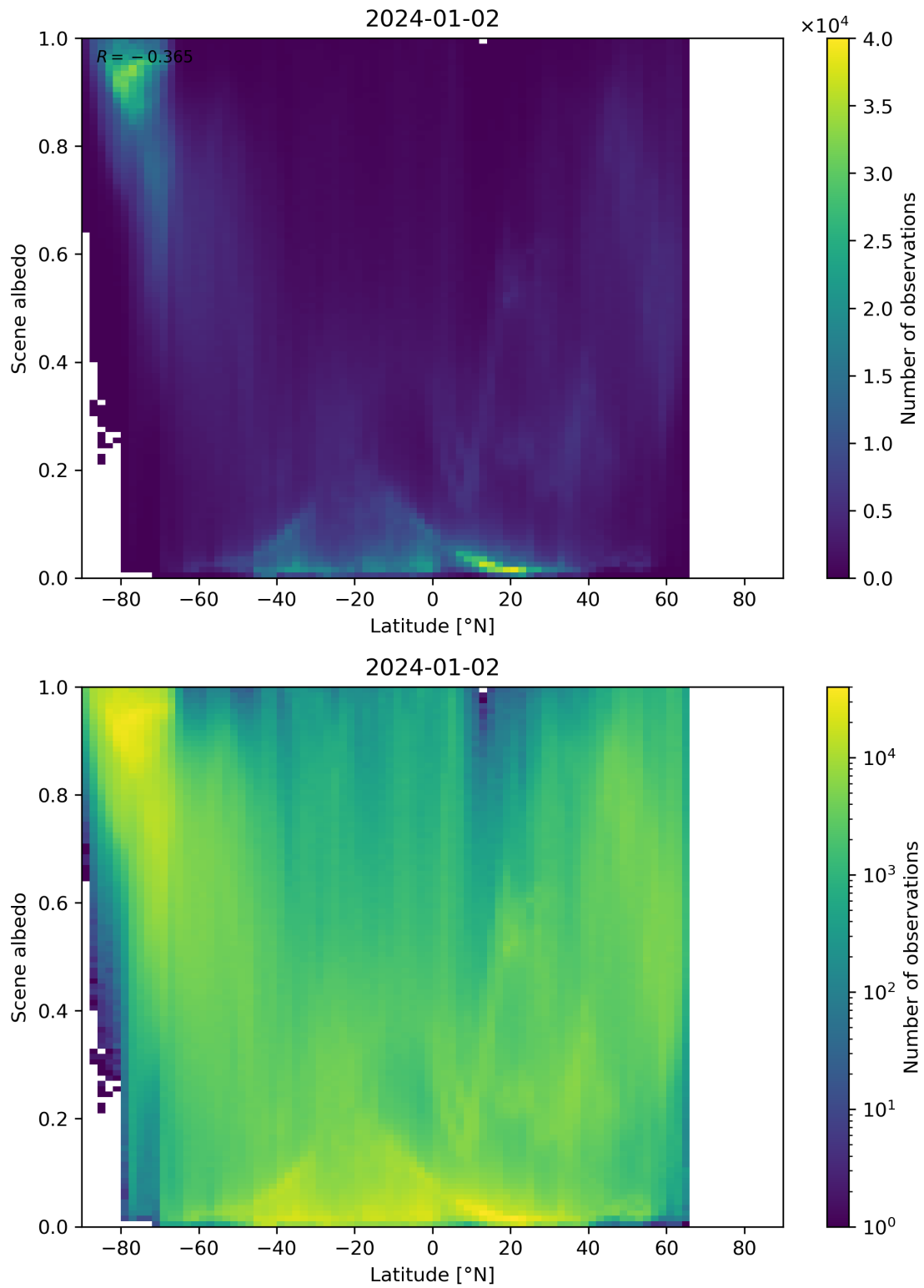
Figure 95: Scatter density plot of “Latitude” against “Scene albedo” for 2024-01-01 to 2024-01-03.
