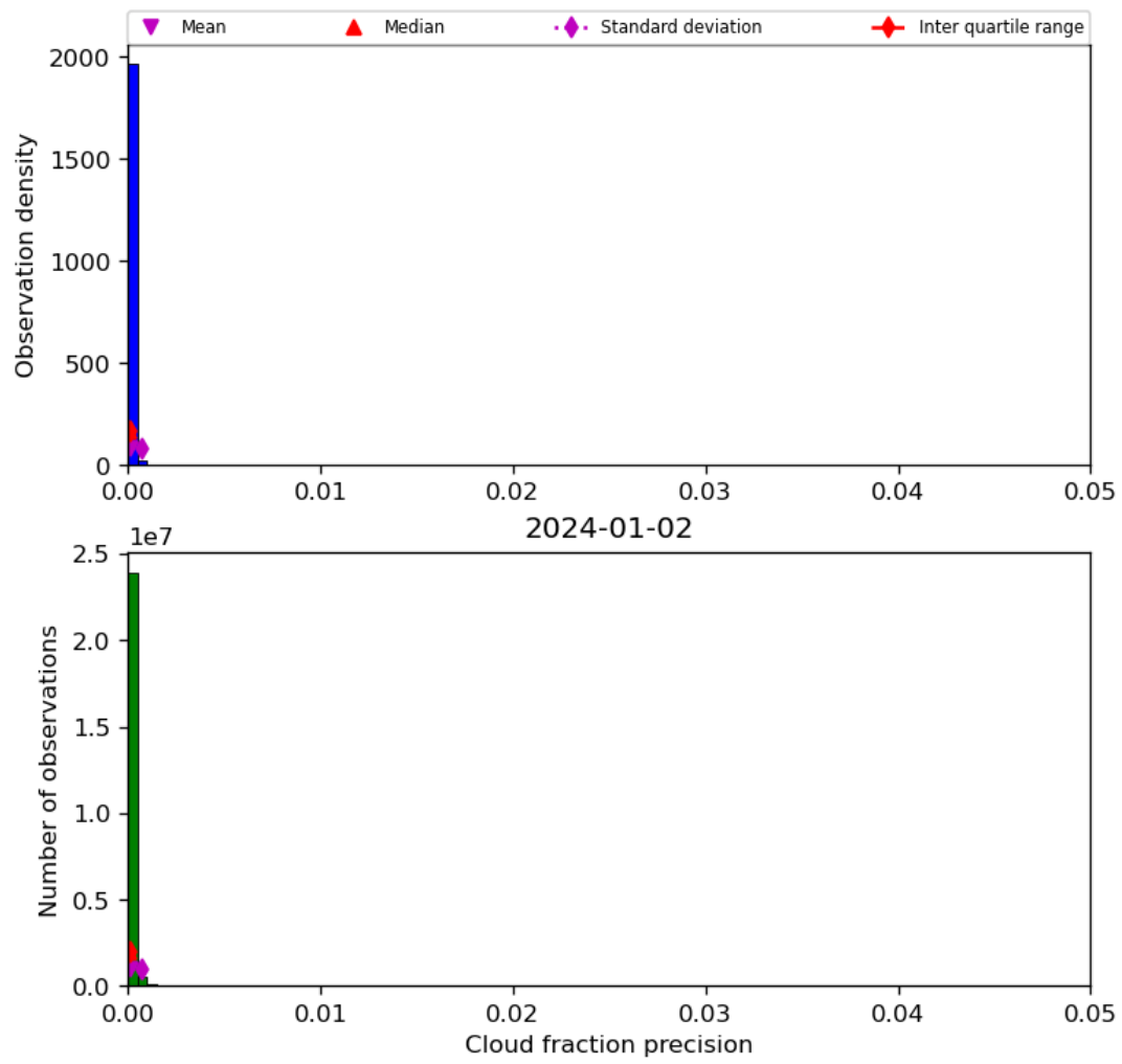
Figure 33: Histogram of “Cloud fraction precision” for 2024-01-01 to 2024-01-03
