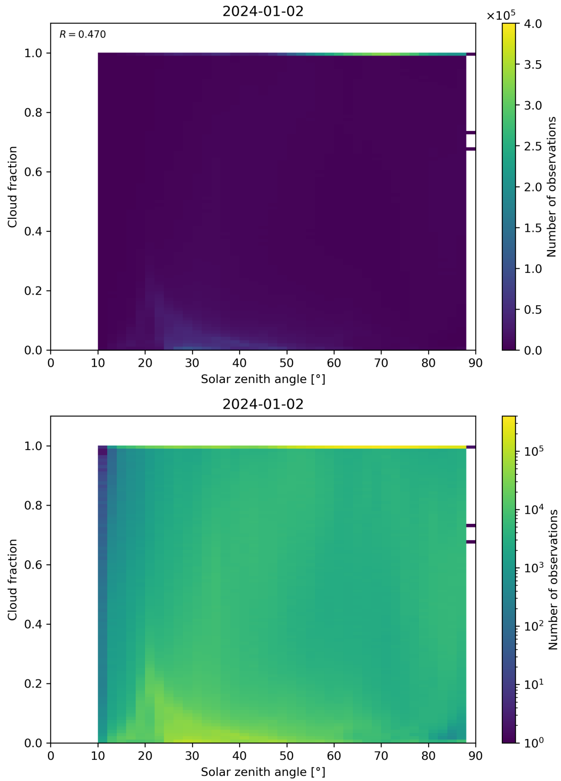
Figure 110: Scatter density plot of “Solar zenith angle” against “Cloud fraction” for 2024-01-01 to 2024-01-03.
