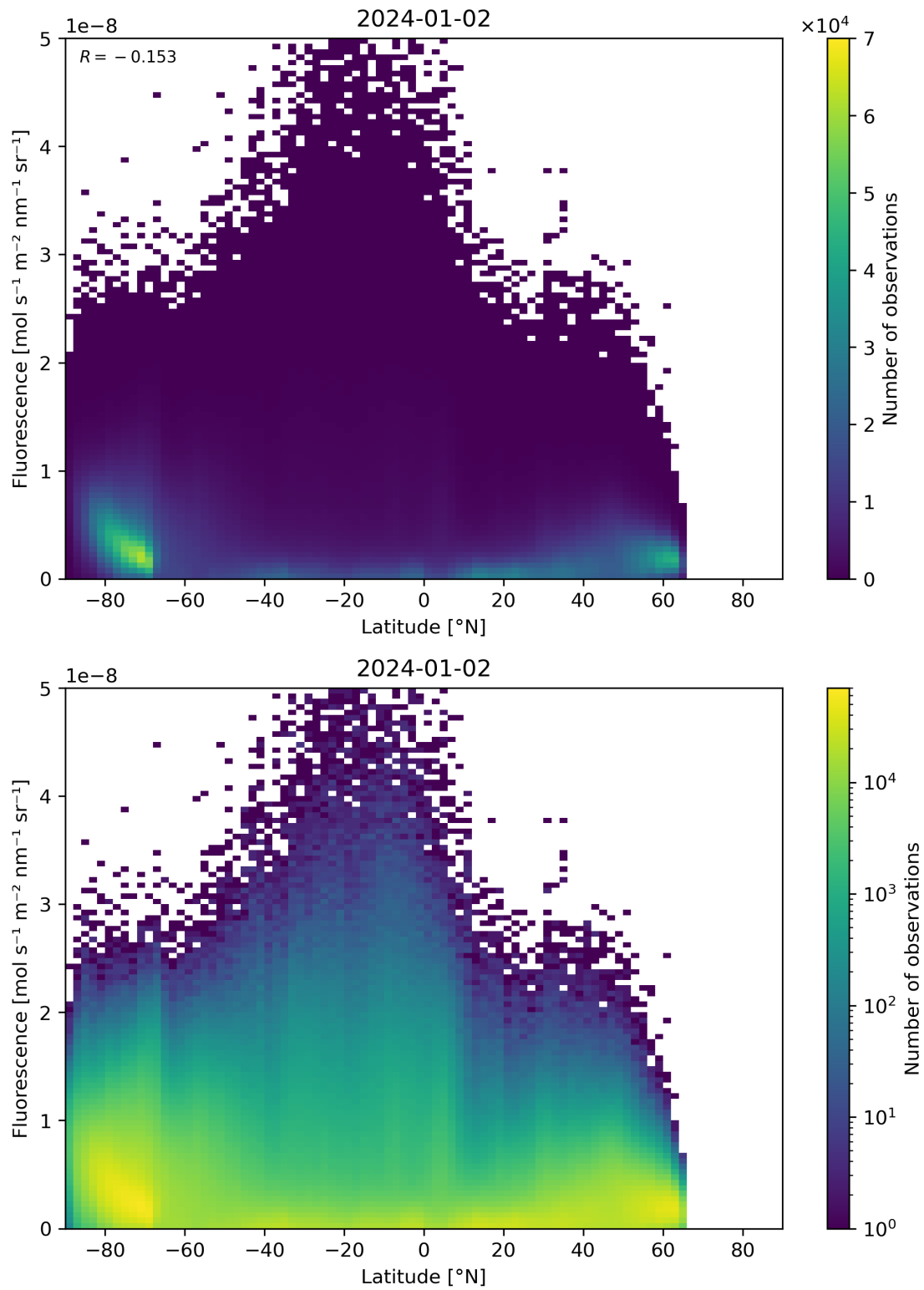
Figure 92: Scatter density plot of “Latitude” against “Fluorescence” for 2024-01-01 to 2024-01-03.
