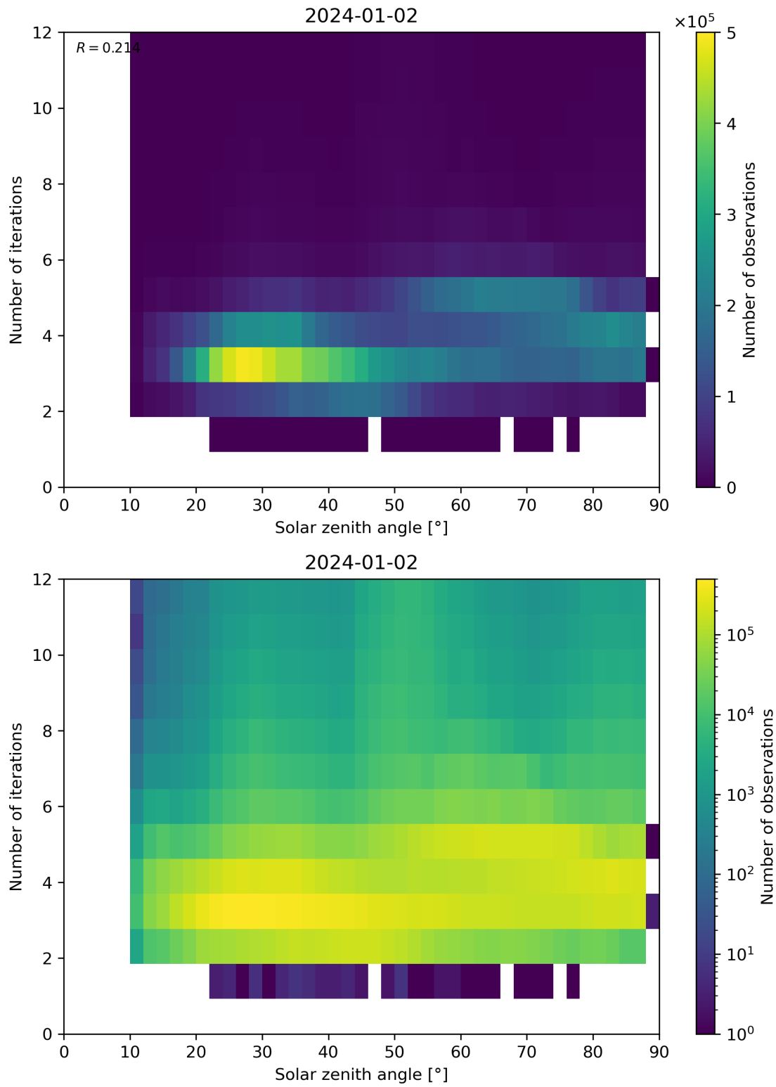
Figure 114: Scatter density plot of “Solar zenith angle” against “Number of iterations” for 2024-01-01 to 2024-01-03.
