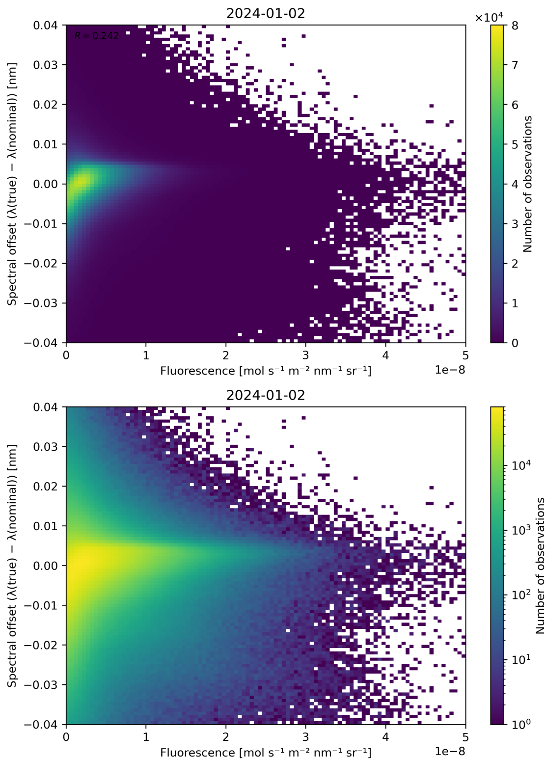
Figure 87: Scatter density plot of “Fluorescence” against “Spectral offset ( \lambda(\text{true}) - \lambda(\text{nominal}) )” for 2024-01-01 to 2024-01-03.
