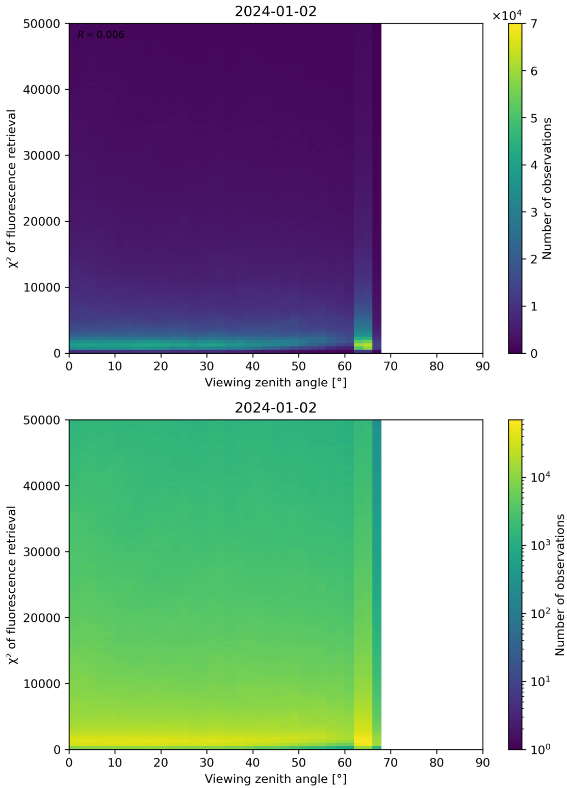
Figure 119: Scatter density plot of “Viewing zenith angle” against “ \chi^2 of fluorescence retrieval” for 2024-01-01 to 2024-01-03.
