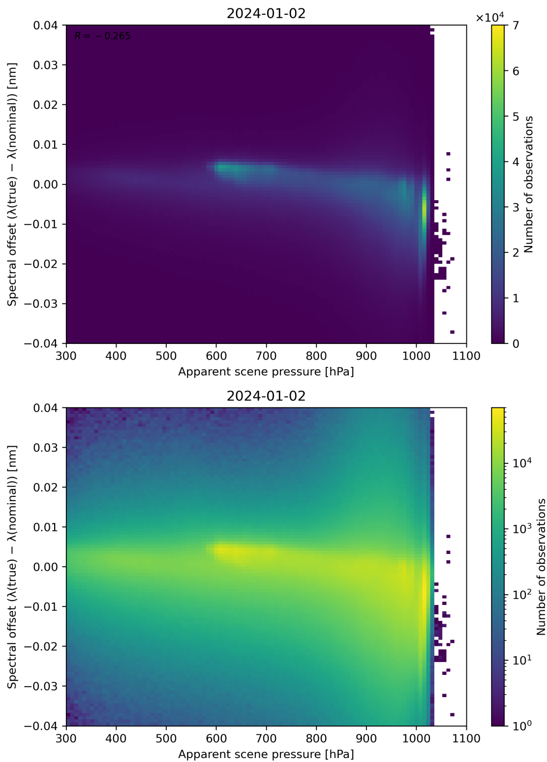
Figure 67: Scatter density plot of “Apparent scene pressure” against “Spectral offset ( \lambda(\text{true}) - \lambda(\text{nominal}) )” for 2024-01-01 to 2024-01-03.
