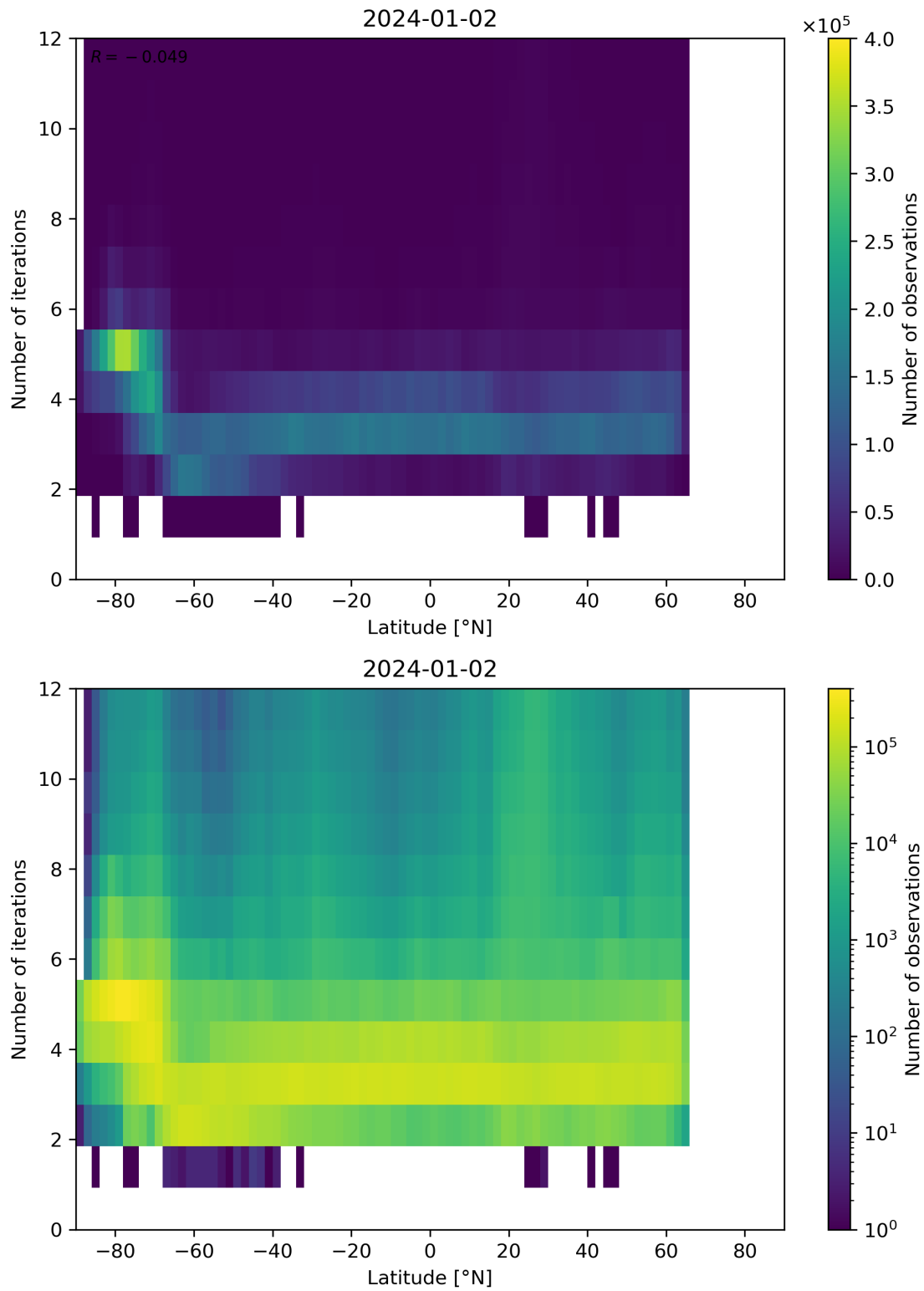
Figure 93: Scatter density plot of “Latitude” against “Number of iterations” for 2024-01-01 to 2024-01-03.
