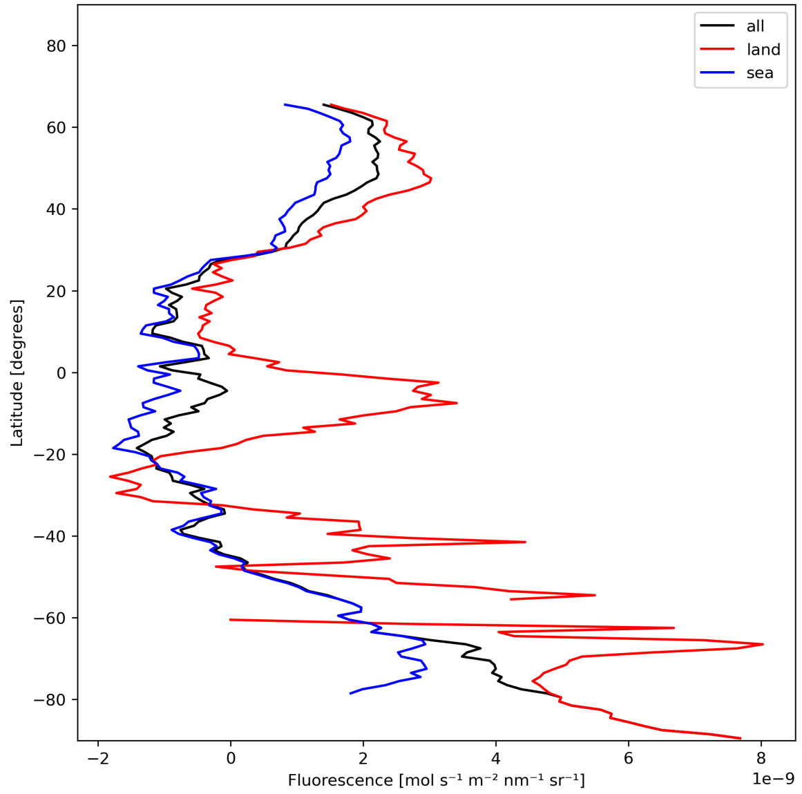
Figure 23: Zonal average of “Fluorescence” for 2024-01-01 to 2024-01-03.
