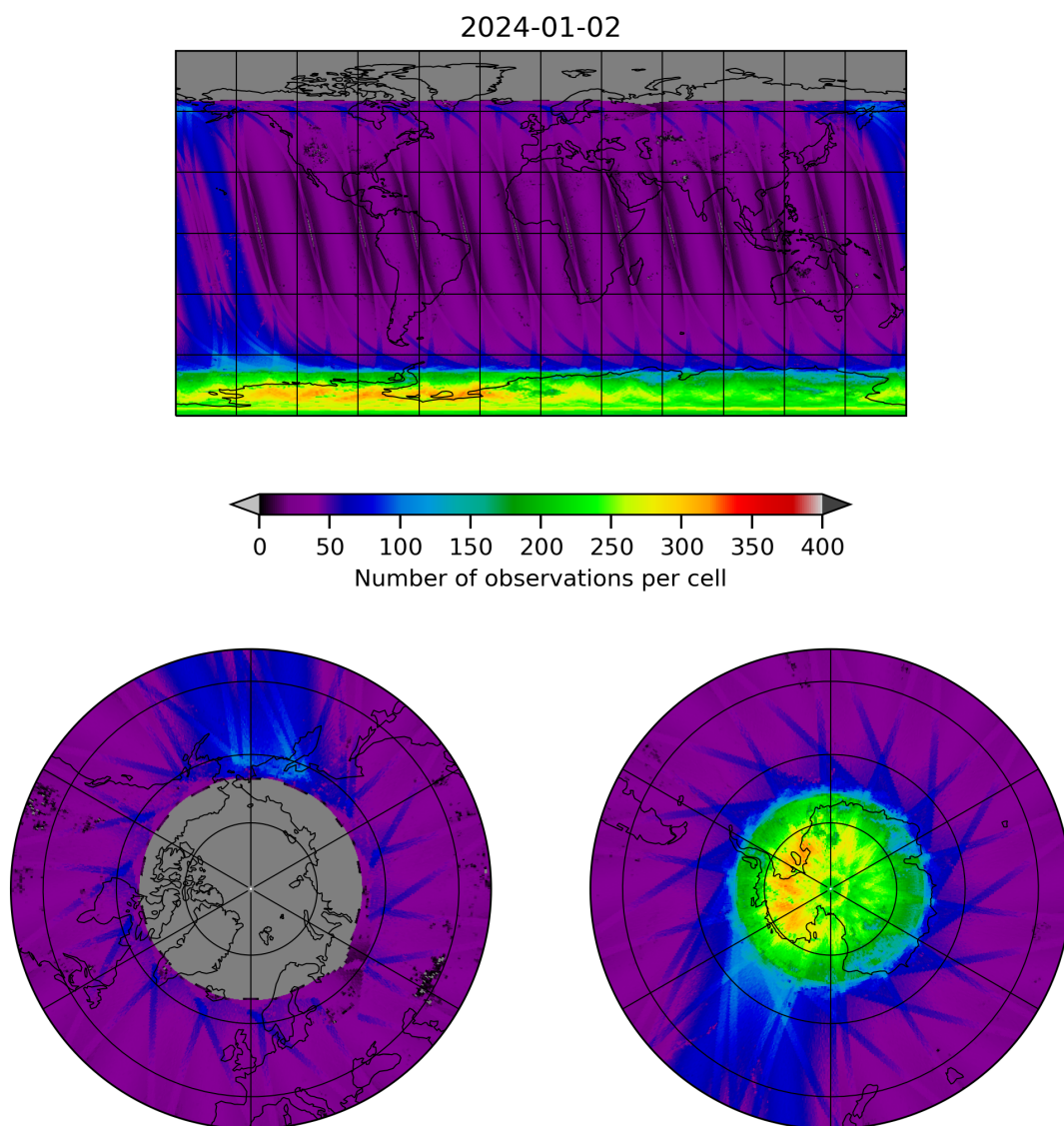
Figure 11: Map of the number of observations for 2024-01-01 to 2024-01-03
