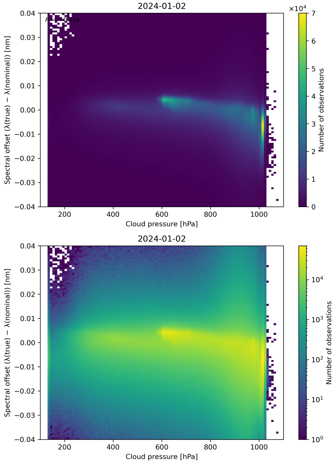
Figure 84: Scatter density plot of “Cloud pressure” against “Spectral offset ( \lambda(\text{true}) - \lambda(\text{nominal}) )” for 2024-01-01 to 2024-01-03.
