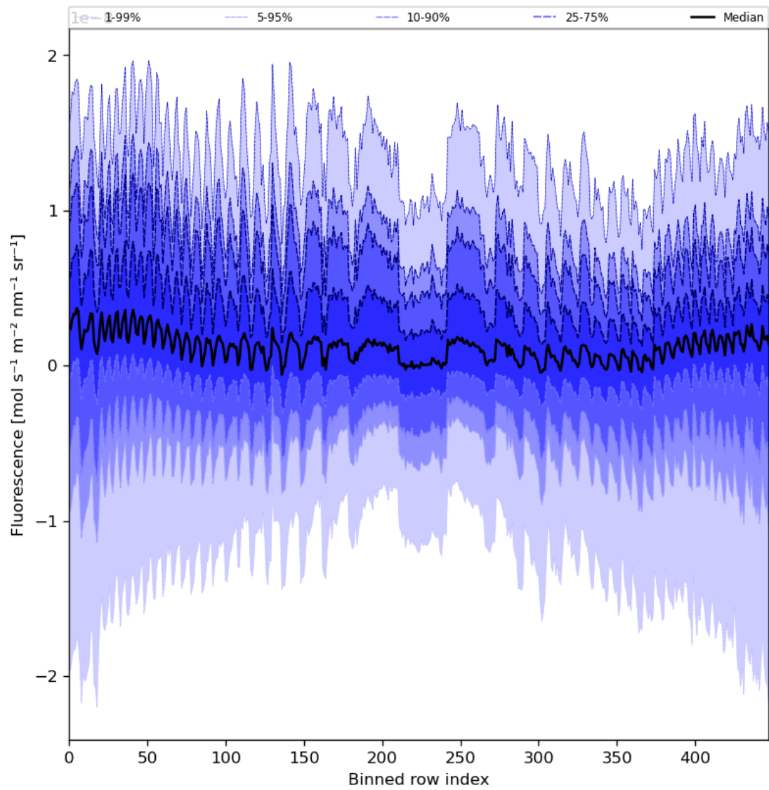
Figure 57: Along track statistics of “Fluorescence” for 2024-01-01 to 2024-01-03
