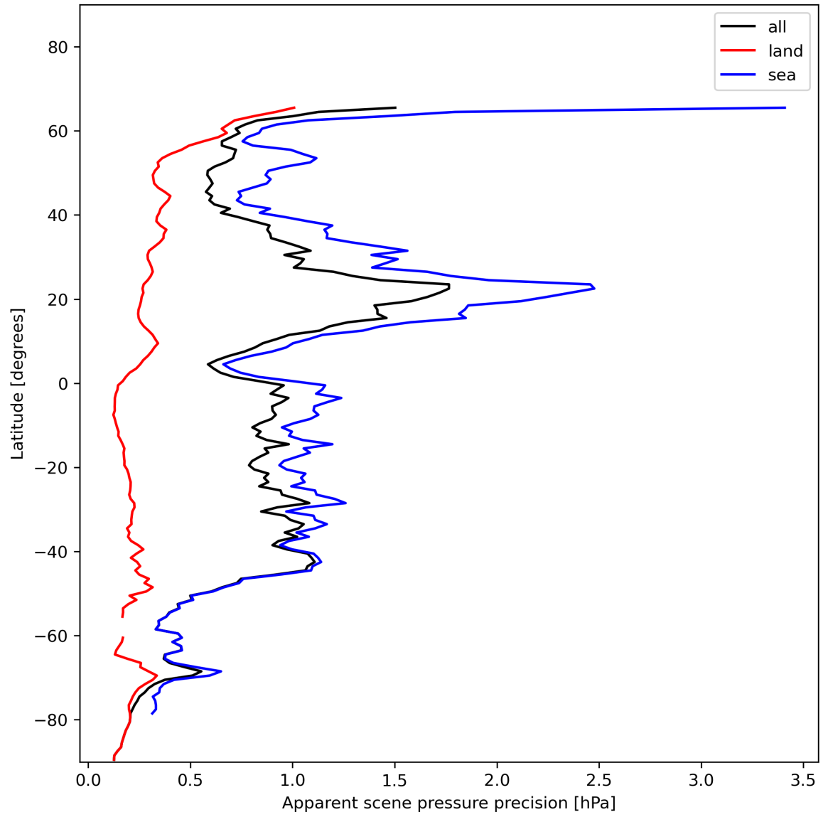
Figure 20: Zonal average of “Apparent scene pressure precision” for 2024-01-01 to 2024-01-03.
