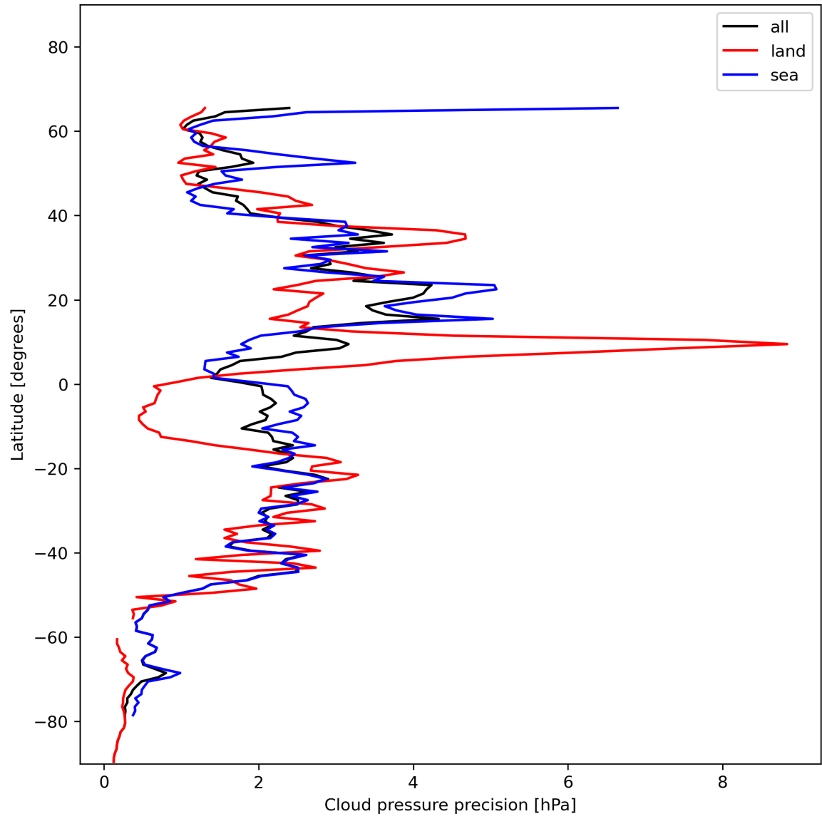
Figure 14: Zonal average of “Cloud pressure precision” for 2024-01-01 to 2024-01-03.
