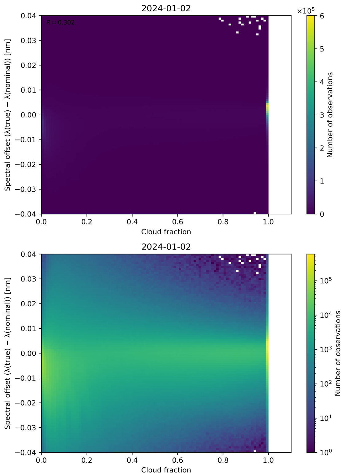
Figure 76: Scatter density plot of “Cloud fraction” against “Spectral offset ( \lambda(\text{true}) - \lambda(\text{nominal}) )” for 2024-01-01 to 2024-01-03.
