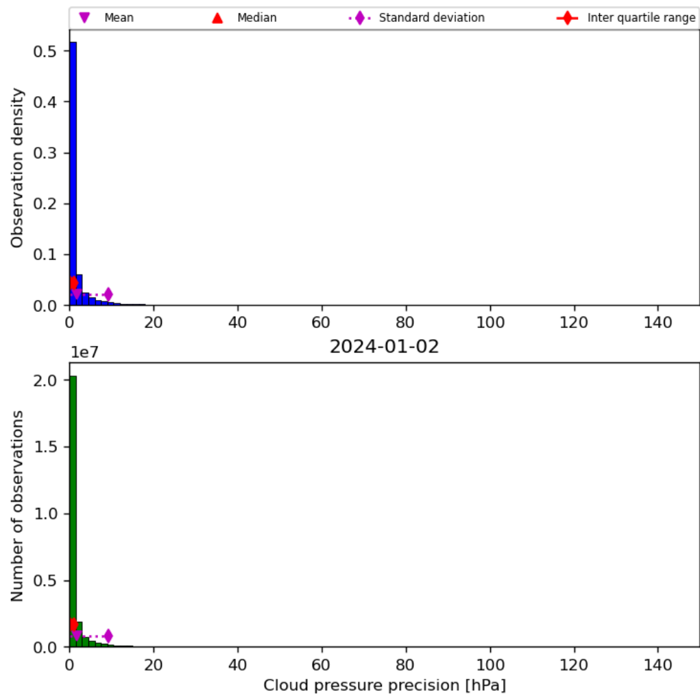
Figure 31: Histogram of “Cloud pressure precision” for 2024-01-01 to 2024-01-03
