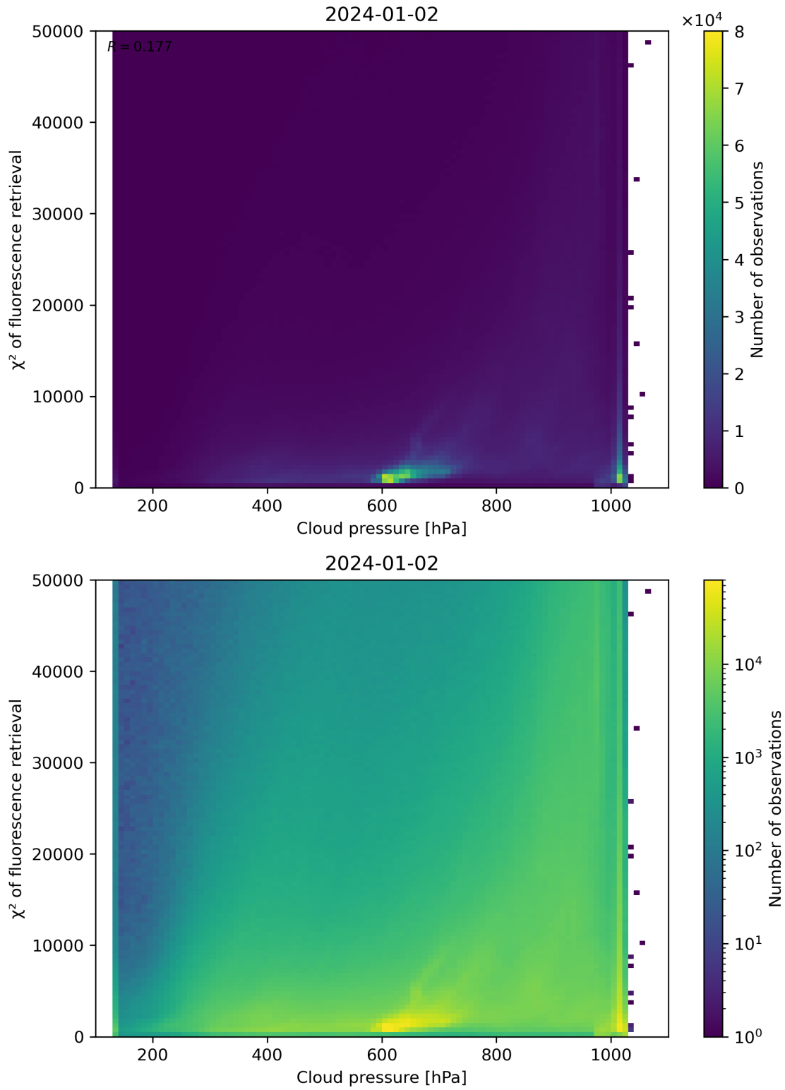
Figure 78: Scatter density plot of “Cloud pressure” against “ \chi^2 of fluorescence retrieval” for 2024-01-01 to 2024-01-03.
