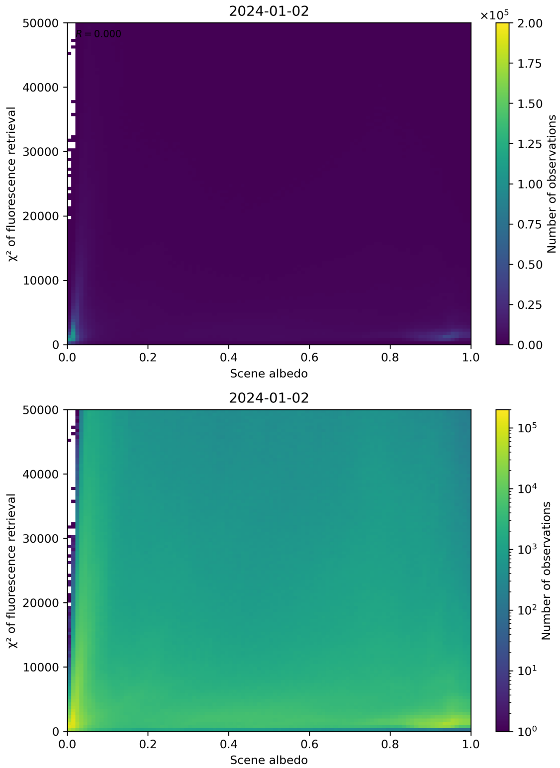
Figure 103: Scatter density plot of “Scene albedo” against “ \chi^2 of fluorescence retrieval” for 2024-01-01 to 2024-01-03.
