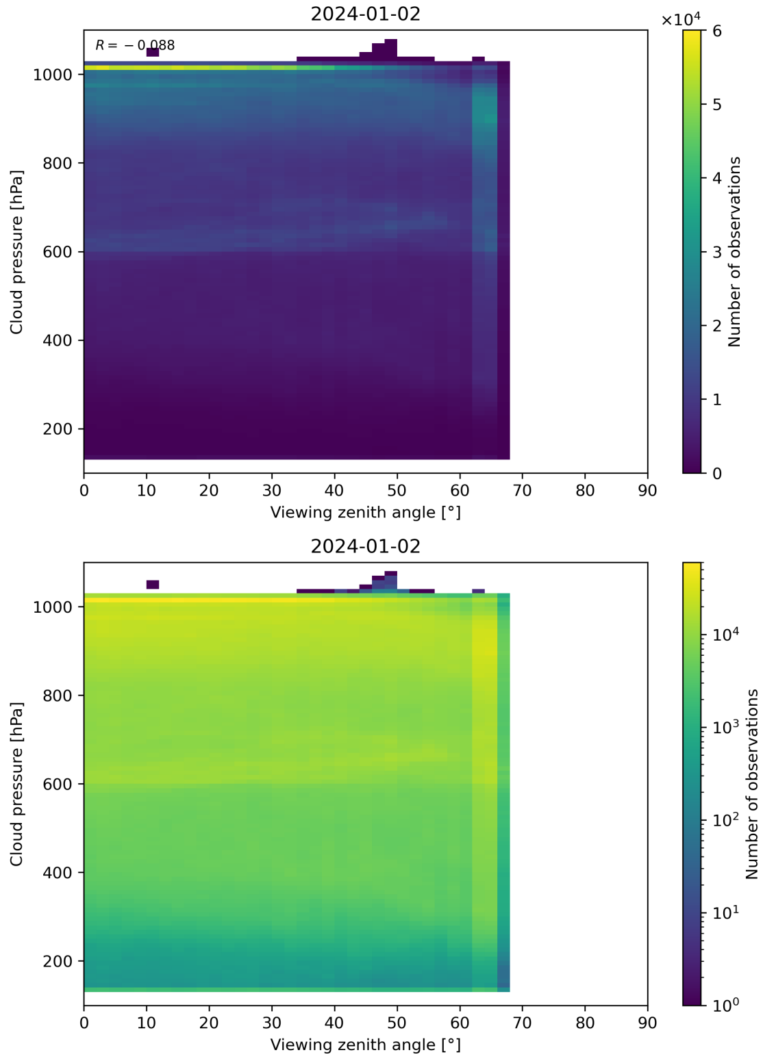
Figure 121: Scatter density plot of “Viewing zenith angle” against “Cloud pressure” for 2024-01-01 to 2024-01-03.
