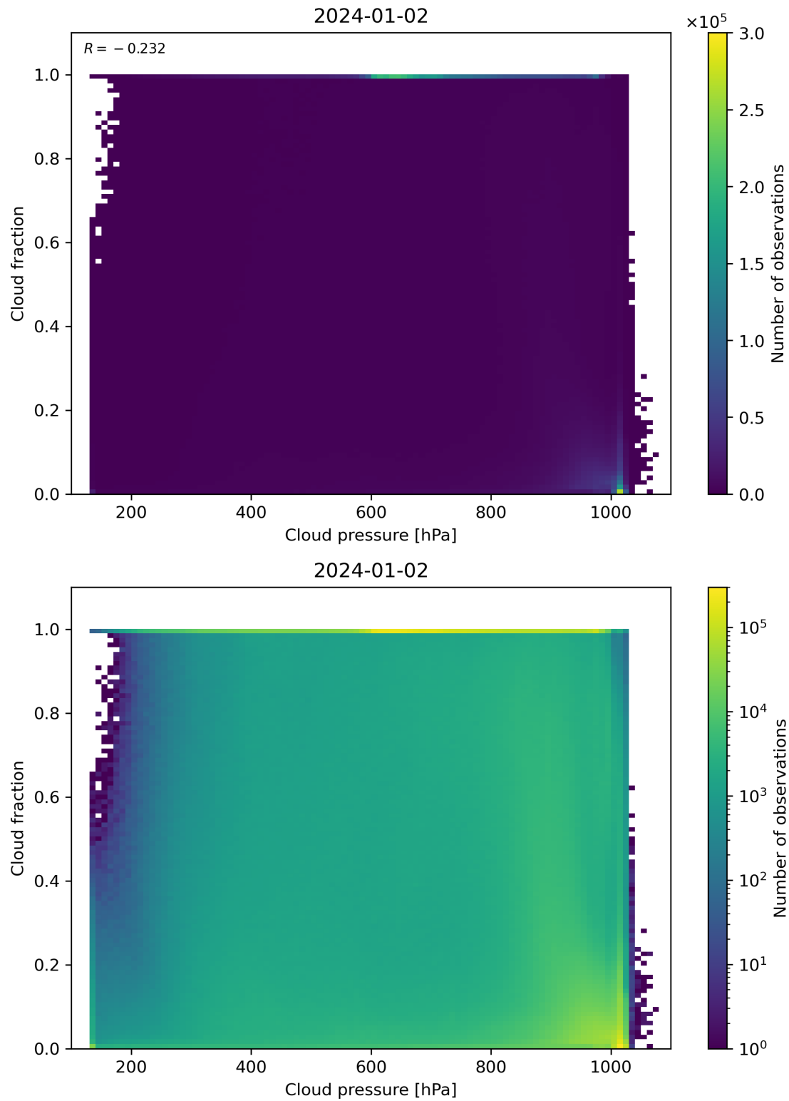
Figure 79: Scatter density plot of “Cloud pressure” against “Cloud fraction” for 2024-01-01 to 2024-01-03.
