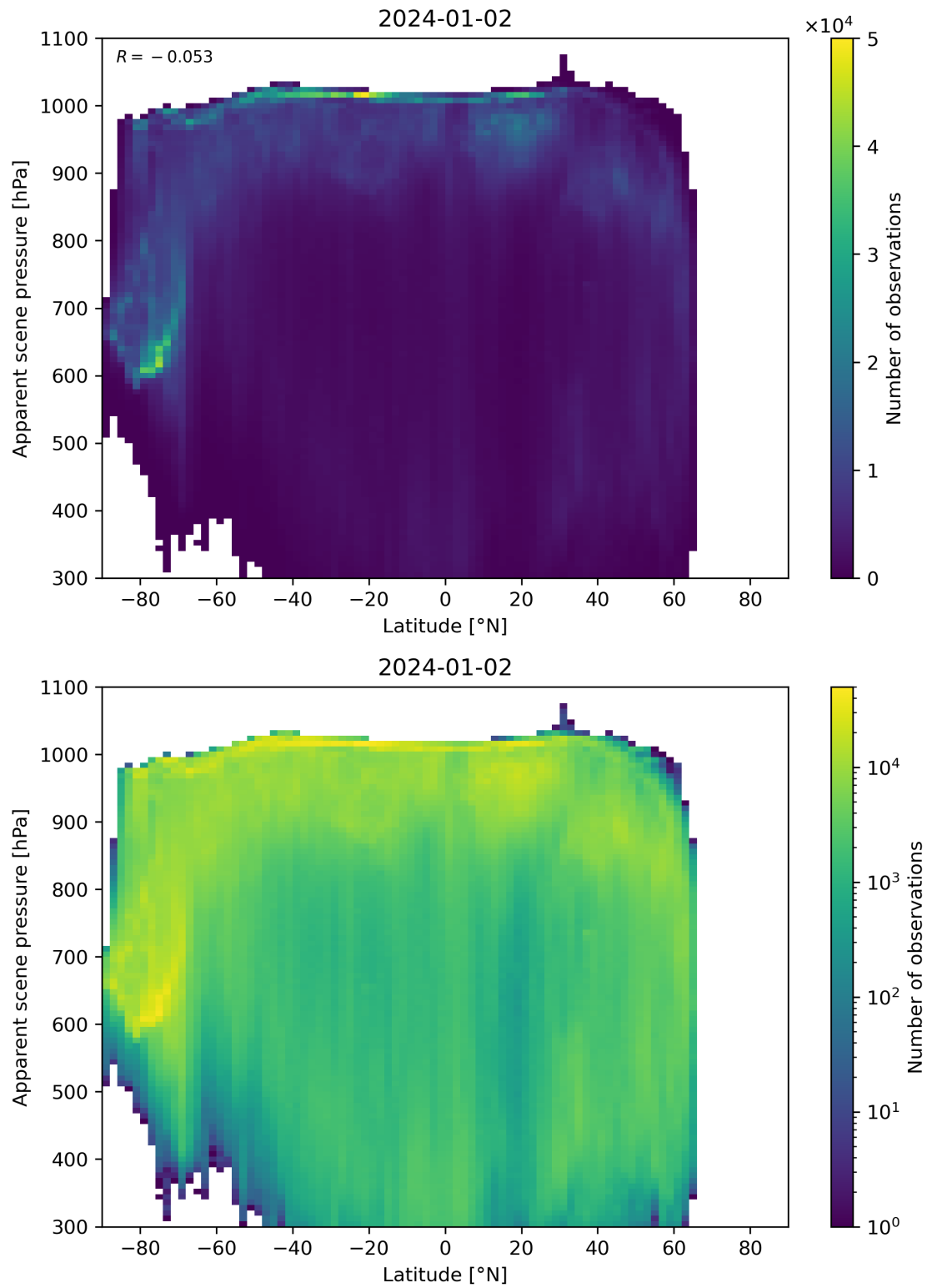
Figure 88: Scatter density plot of “Latitude” against “Apparent scene pressure” for 2024-01-01 to 2024-01-03.
