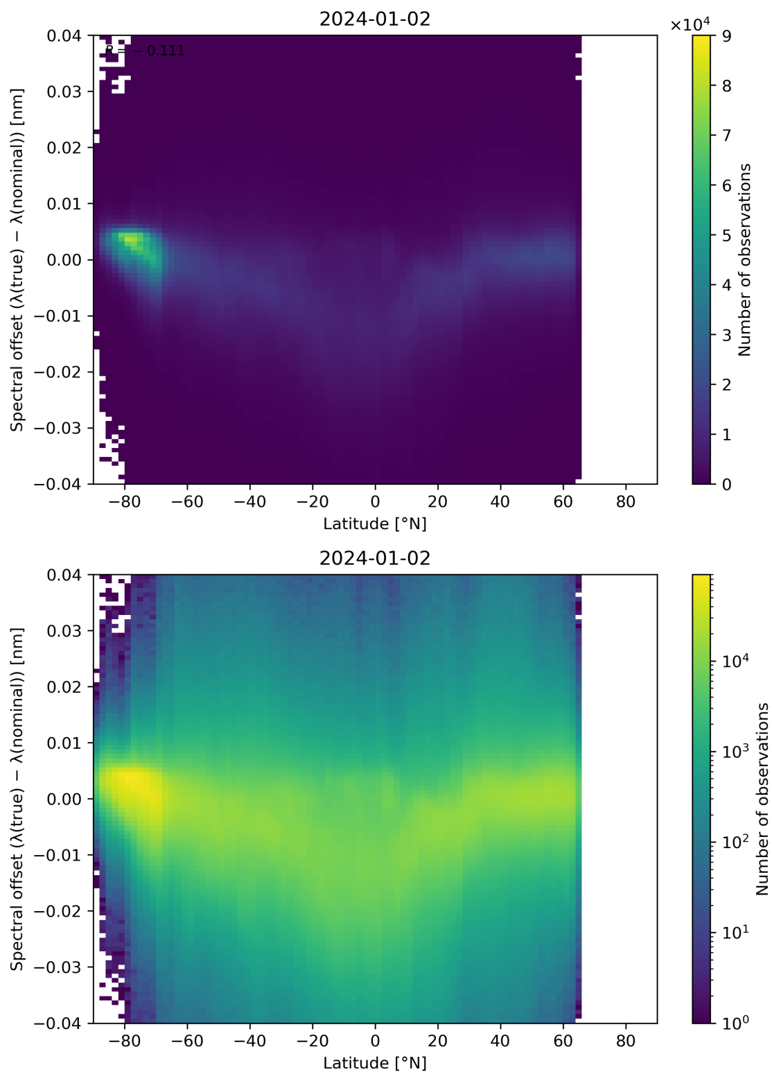
Figure 96: Scatter density plot of “Latitude” against “Spectral offset ( \lambda(\text{true}) - \lambda(\text{nominal}) )” for 2024-01-01 to 2024-01-03.
