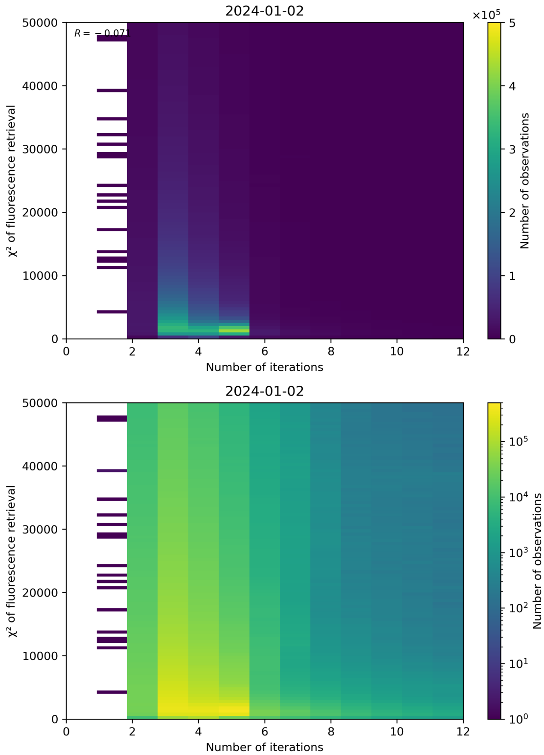
Figure 97: Scatter density plot of “Number of iterations” against “ \chi^2 of fluorescence retrieval” for 2024-01-01 to 2024-01-03.
