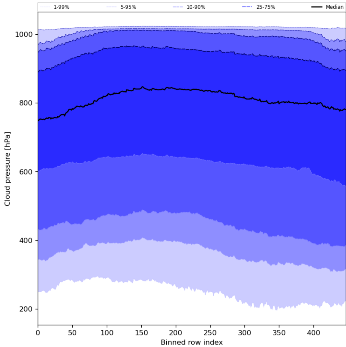
Figure 47: Along track statistics of “Cloud pressure” for 2024-01-01 to 2024-01-03
