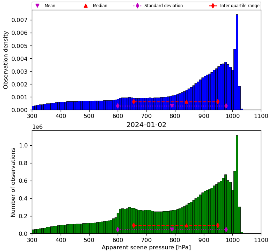
Figure 36: Histogram of “Apparent scene pressure” for 2024-01-01 to 2024-01-03
