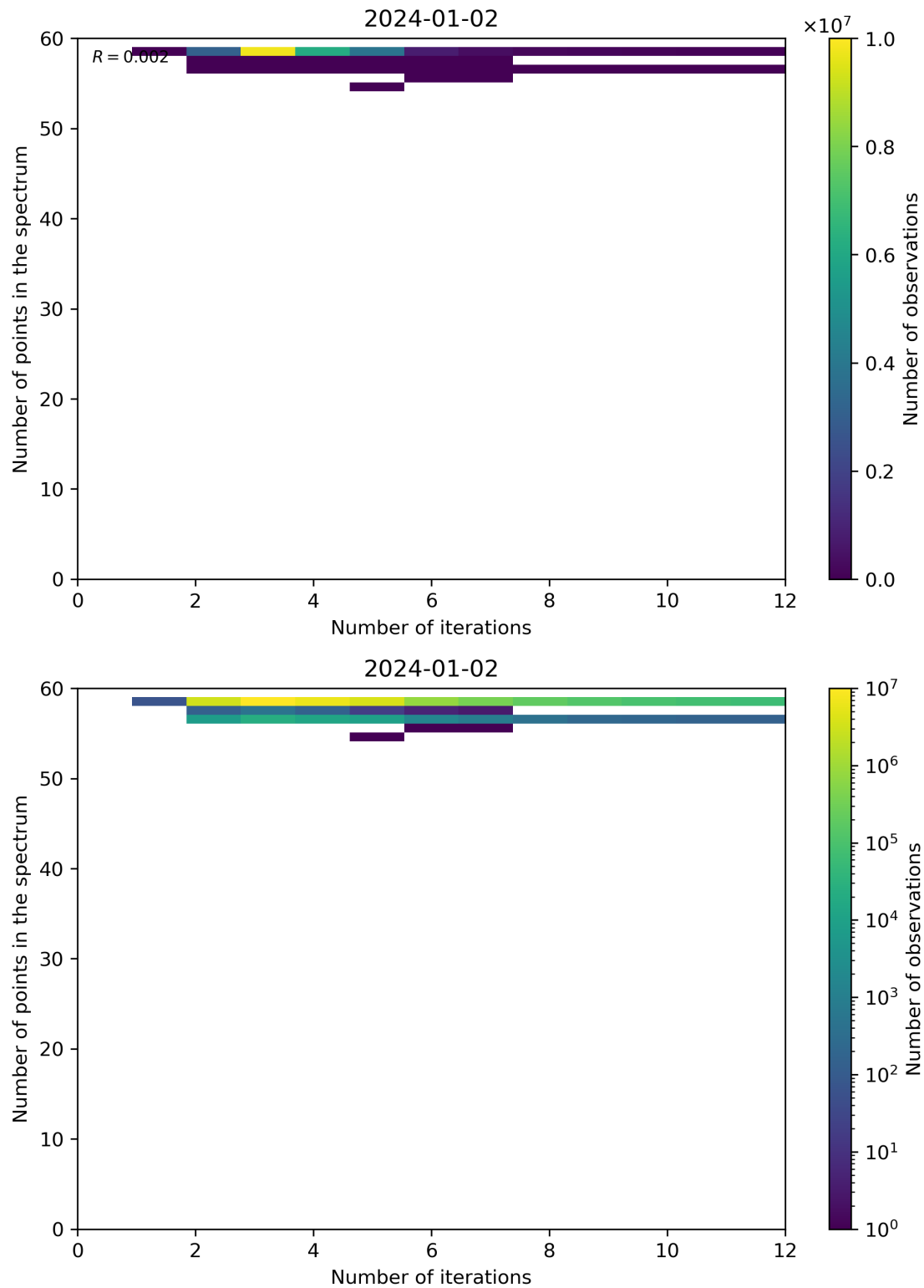
Figure 99: Scatter density plot of “Number of iterations” against “Number of points in the spectrum” for 2024-01-01 to 2024-01-03.
