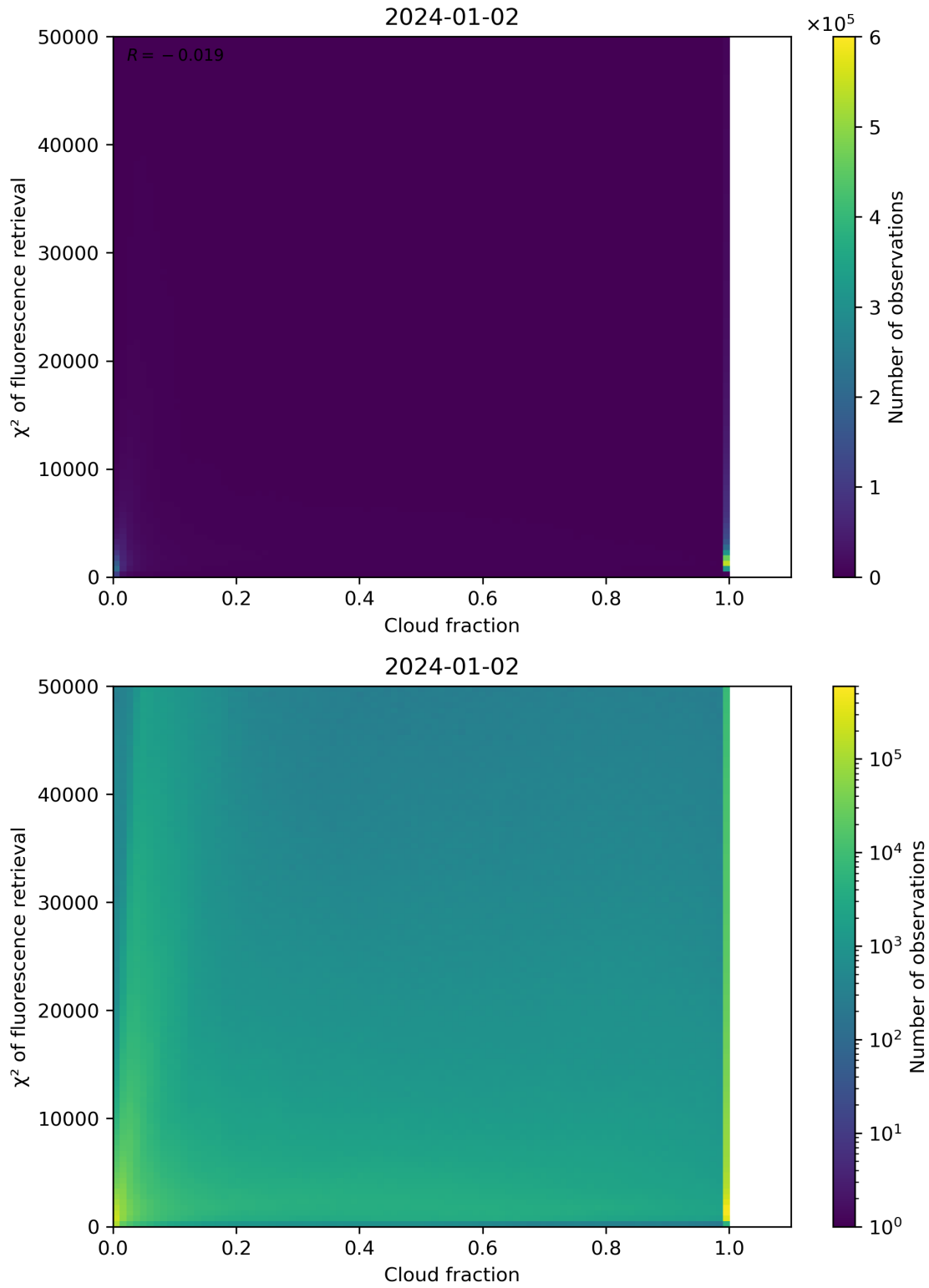
Figure 71: Scatter density plot of “Cloud fraction” against “ \chi^2 of fluorescence retrieval” for 2024-01-01 to 2024-01-03.
