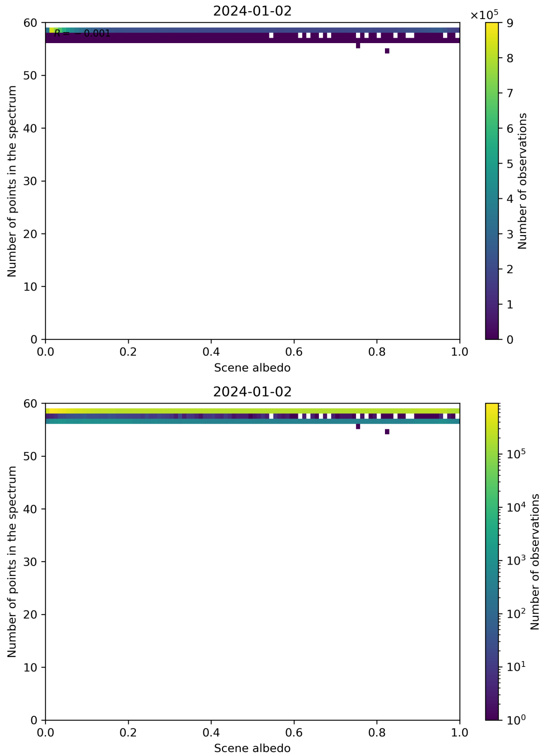
Figure 106: Scatter density plot of “Scene albedo” against “Number of points in the spectrum” for 2024-01-01 to 2024-01-03.
