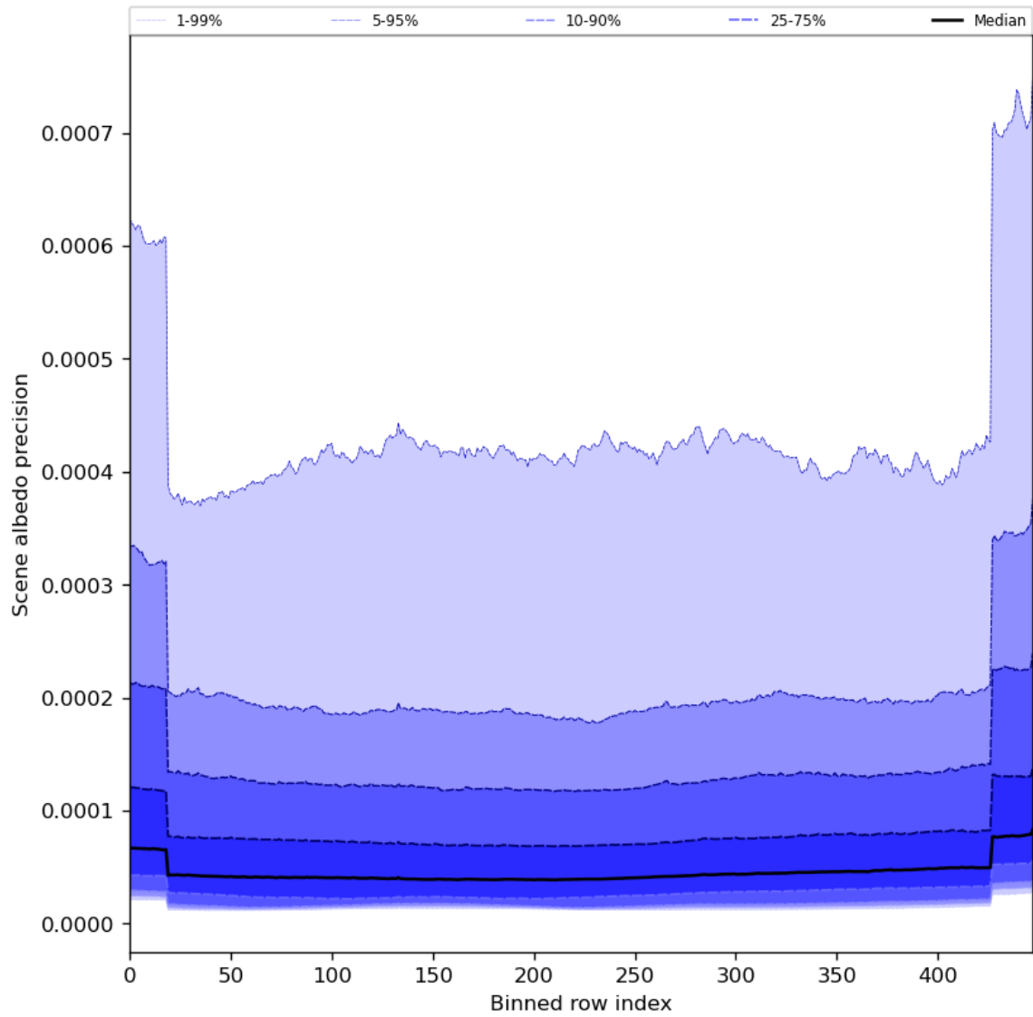
Figure 52: Along track statistics of “Scene albedo precision” for 2024-01-01 to 2024-01-03
