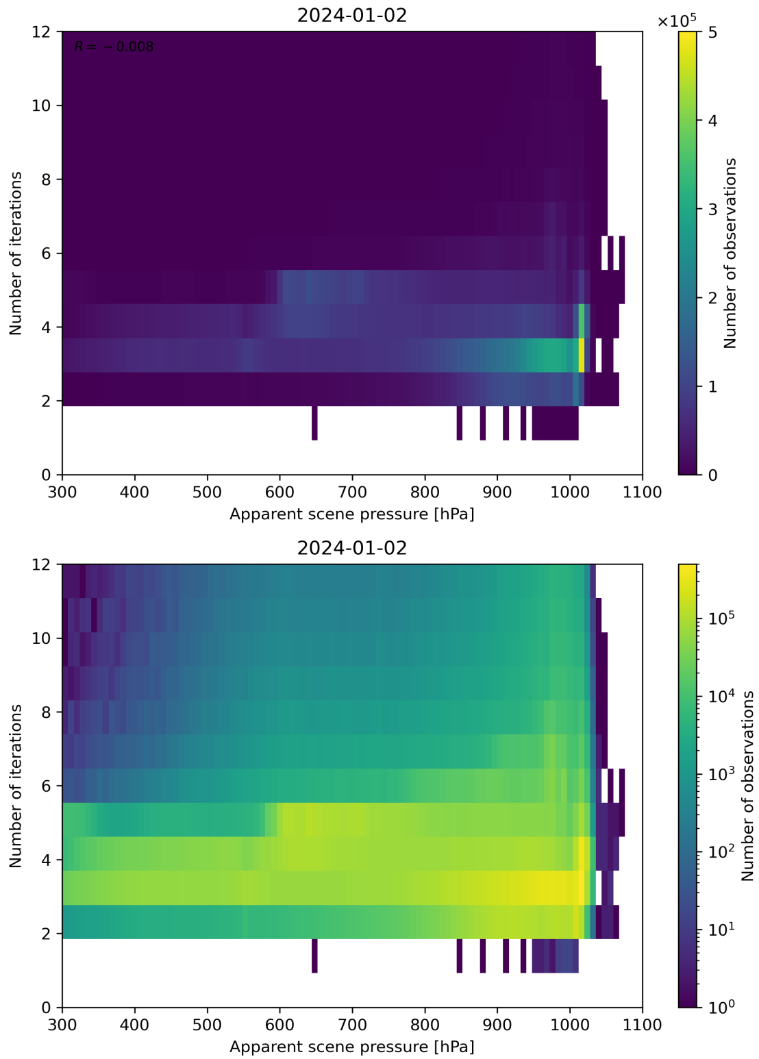
Figure 65: Scatter density plot of “Apparent scene pressure” against “Number of iterations” for 2024-01-01 to 2024-01-03.
