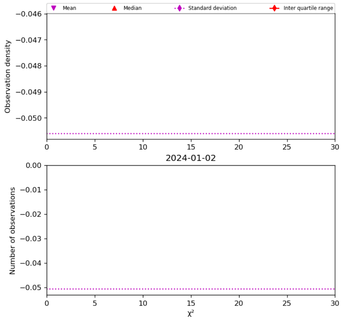
Figure 38: Histogram of “ \chi^2 ” for 2024-01-01 to 2024-01-03
