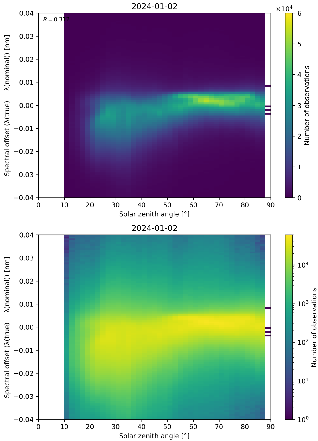
Figure 117: Scatter density plot of “Solar zenith angle” against “Spectral offset ( \lambda(\text{true}) - \lambda(\text{nominal}) )” for 2024-01-01 to 2024-01-03.
