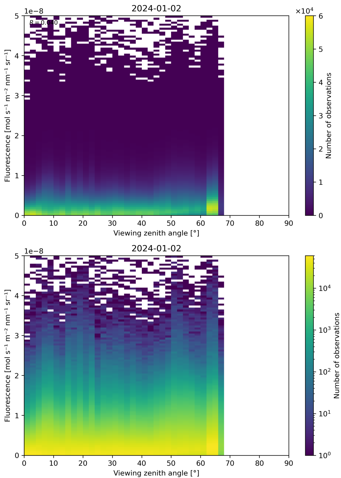
Figure 122: Scatter density plot of “Viewing zenith angle” against “Fluorescence” for 2024-01-01 to 2024-01-03.
