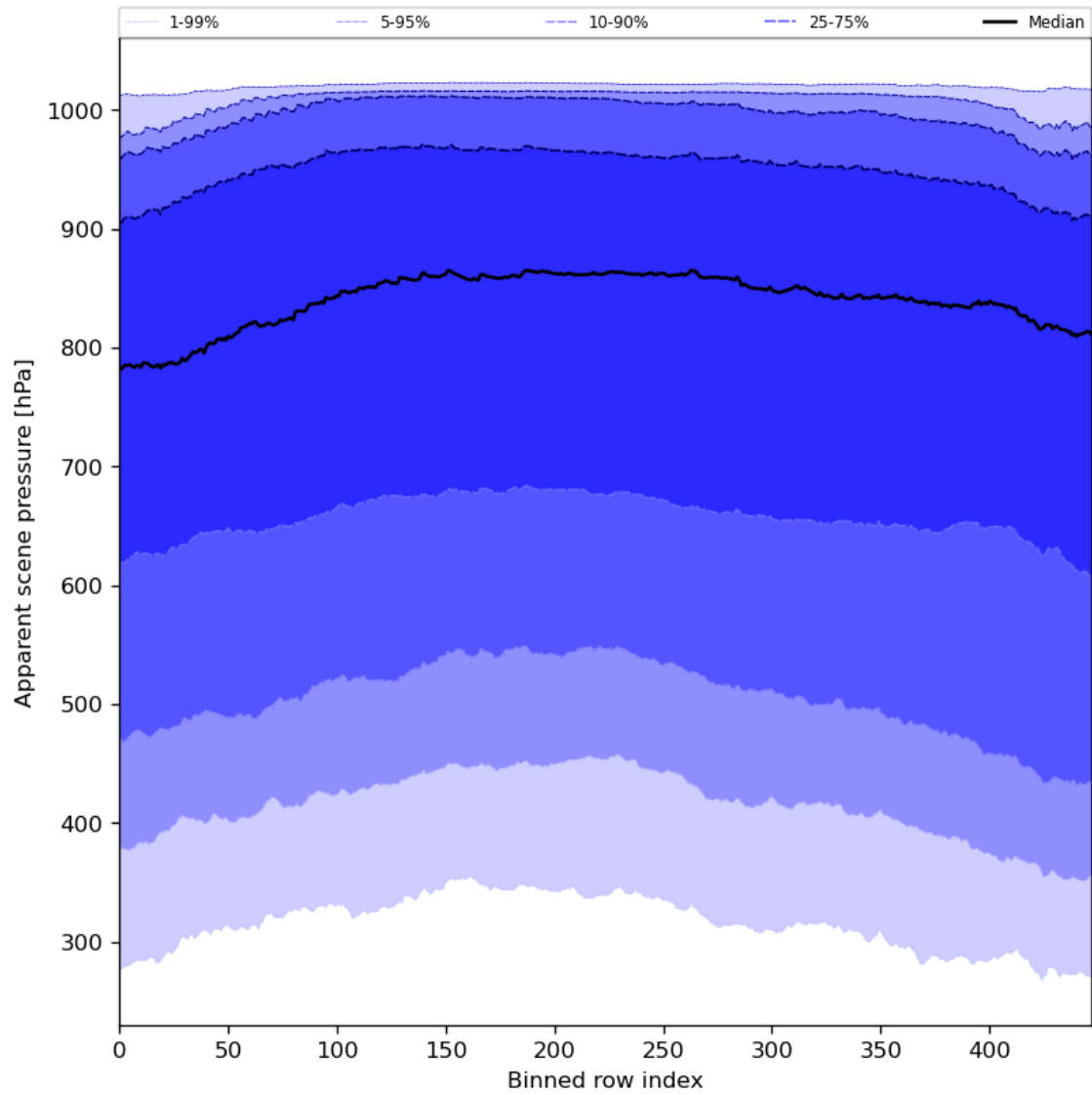
Figure 53: Along track statistics of “Apparent scene pressure” for 2024-01-01 to 2024-01-03
