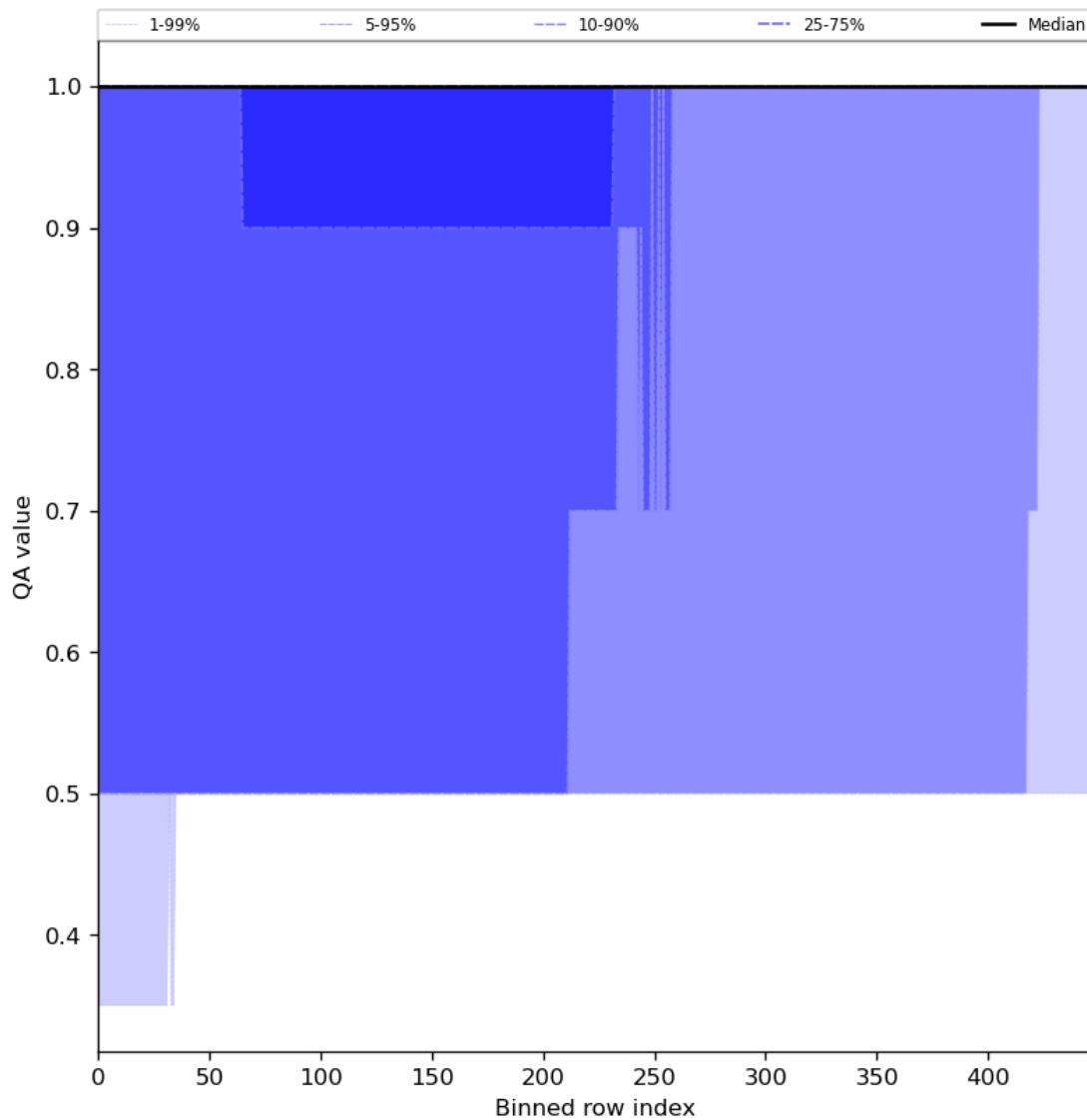
Figure 46: Along track statistics of “QA value” for 2024-01-01 to 2024-01-03
