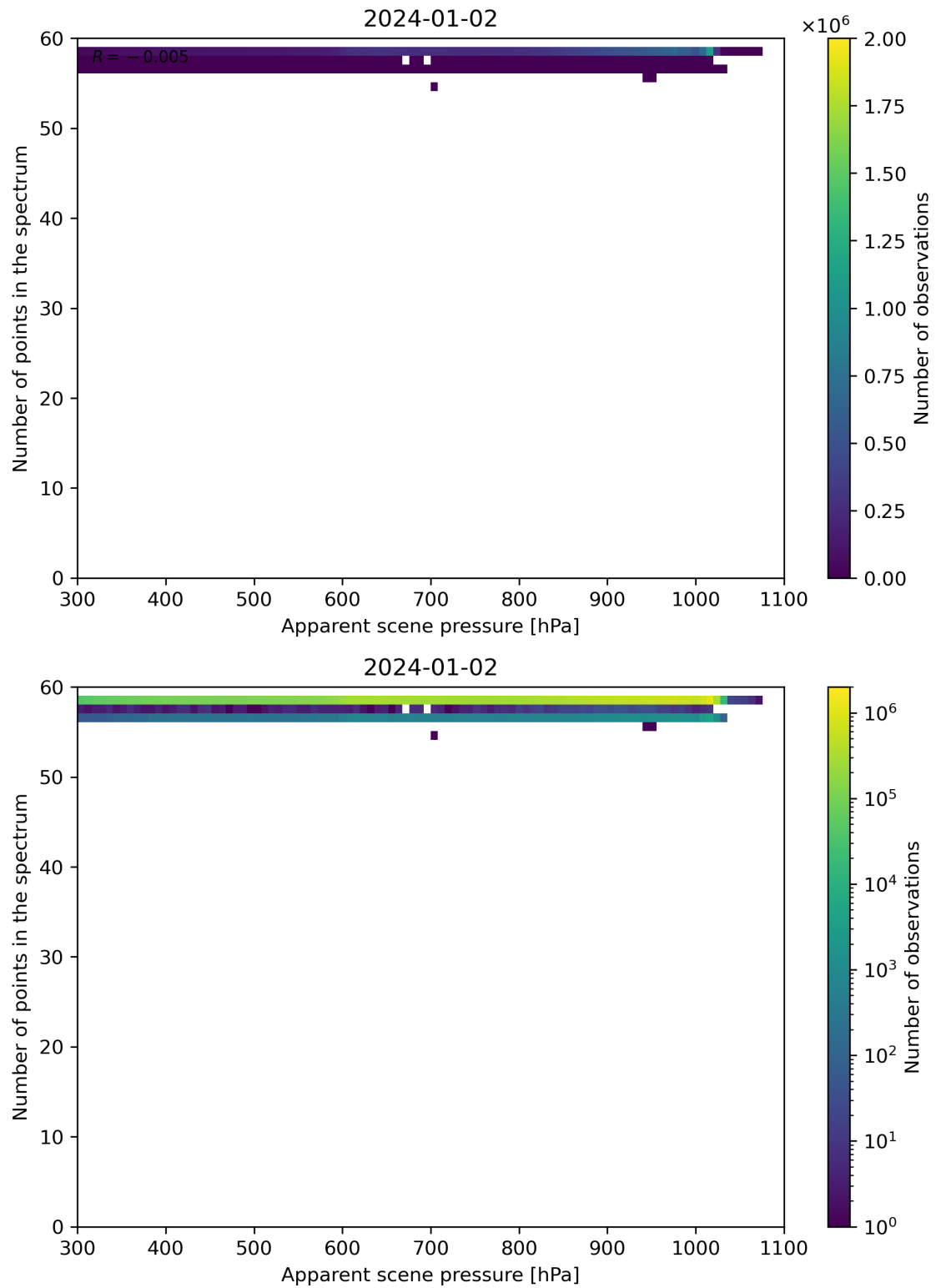
Figure 66: Scatter density plot of “Apparent scene pressure” against “Number of points in the spectrum” for 2024-01-01 to 2024-01-03.
