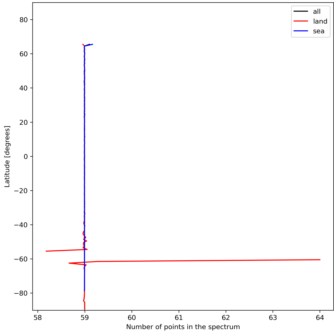
Figure 27: Zonal average of “Number of points in the spectrum” for 2024-01-01 to 2024-01-03.
