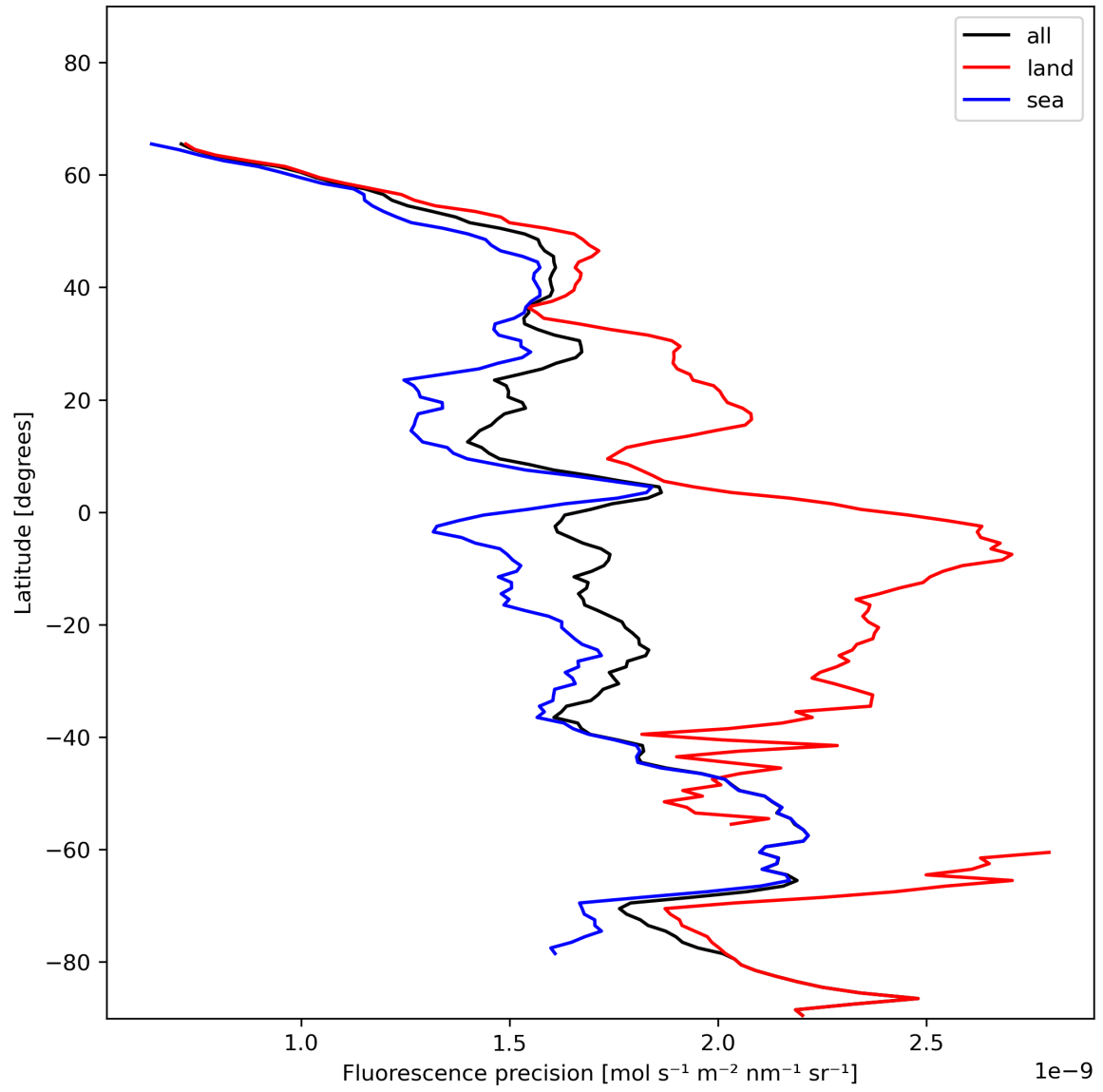
Figure 24: Zonal average of “Fluorescence precision” for 2024-01-01 to 2024-01-03.
