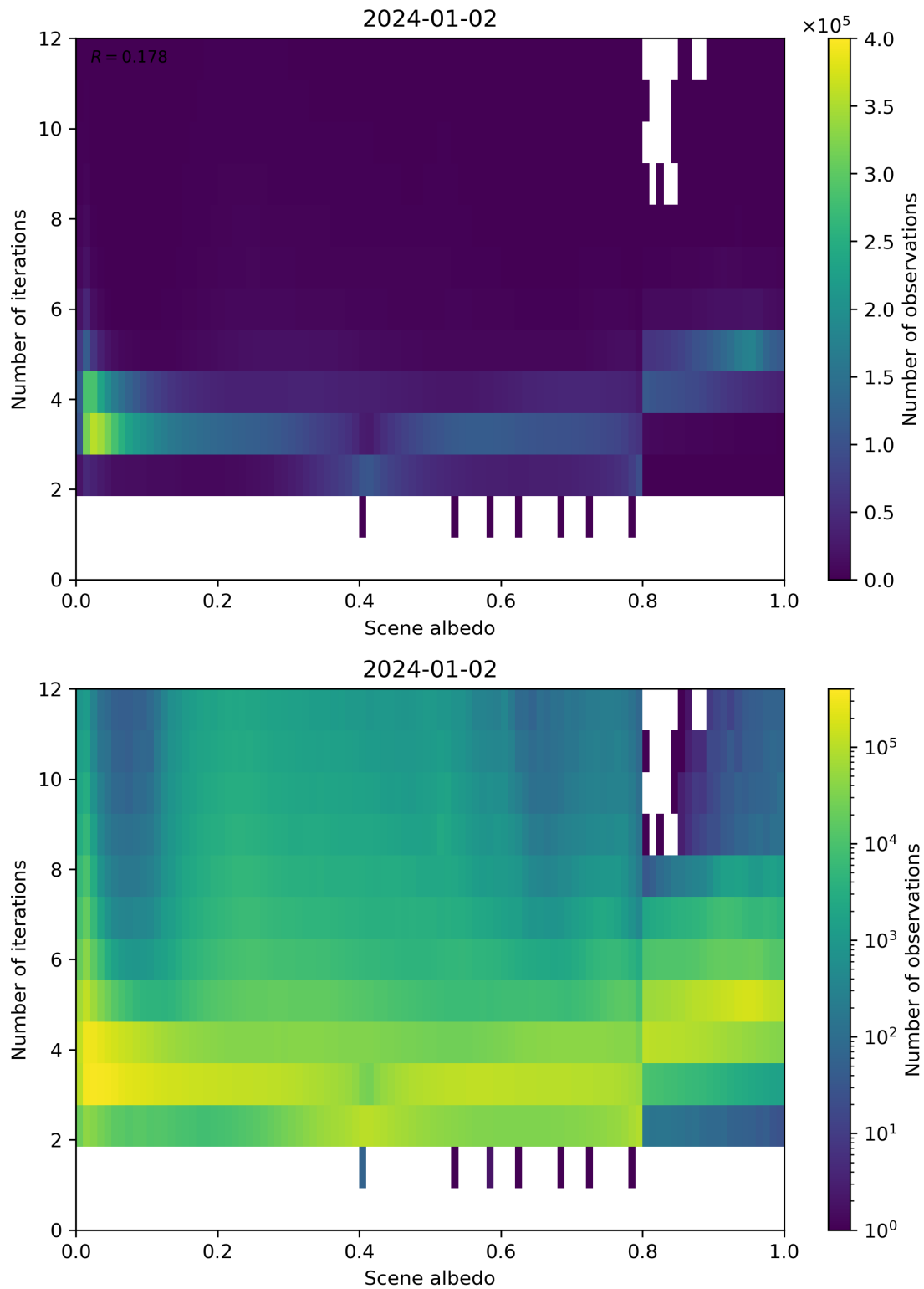
Figure 105: Scatter density plot of “Scene albedo” against “Number of iterations” for 2024-01-01 to 2024-01-03.
