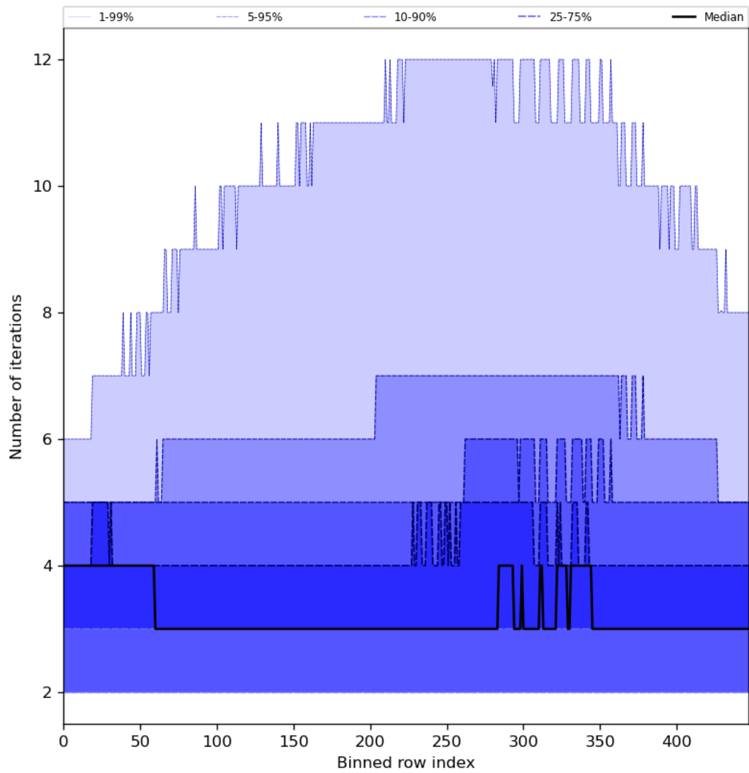
Figure 56: Along track statistics of “Number of iterations” for 2024-01-01 to 2024-01-03
