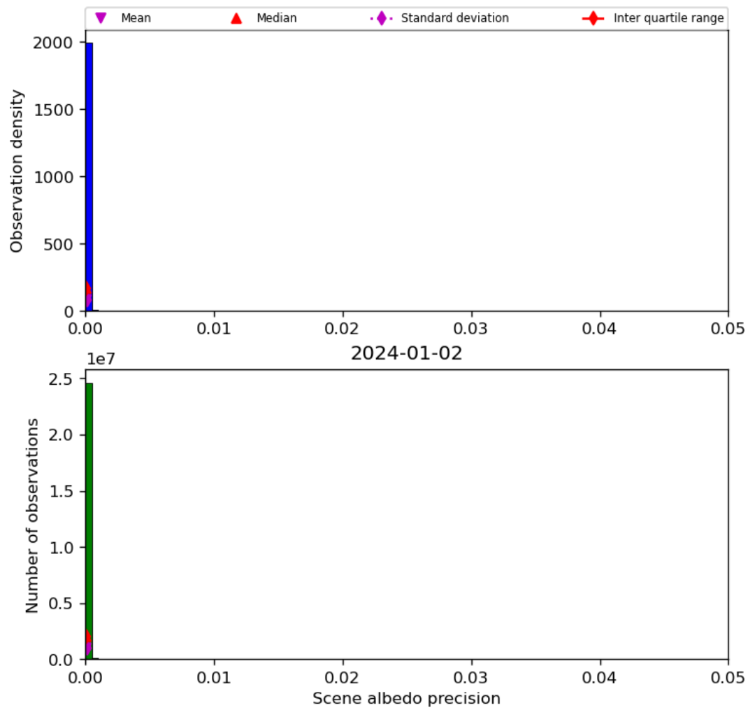
Figure 35: Histogram of “Scene albedo precision” for 2024-01-01 to 2024-01-03
