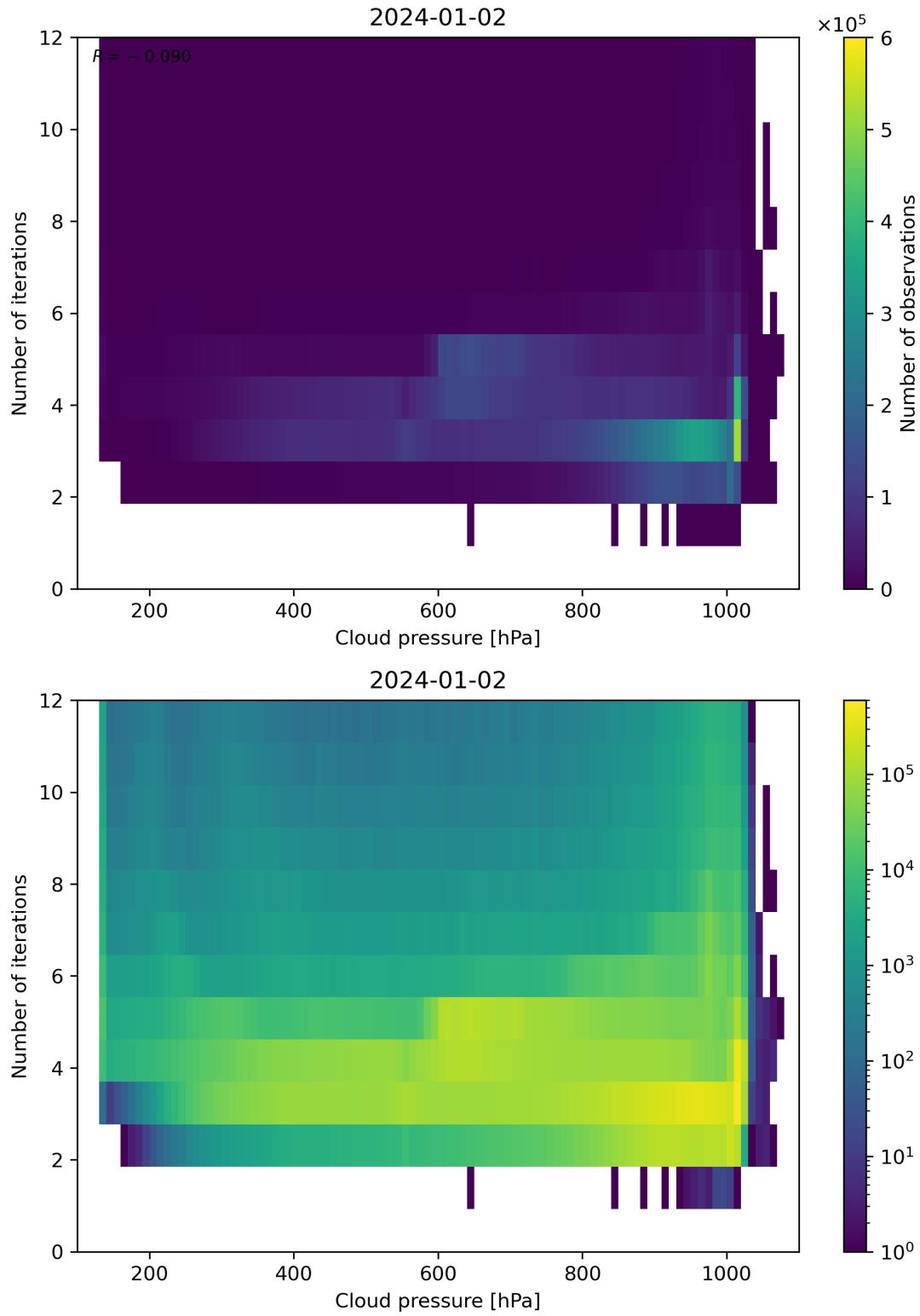
Figure 81: Scatter density plot of “Cloud pressure” against “Number of iterations” for 2024-01-01 to 2024-01-03.
