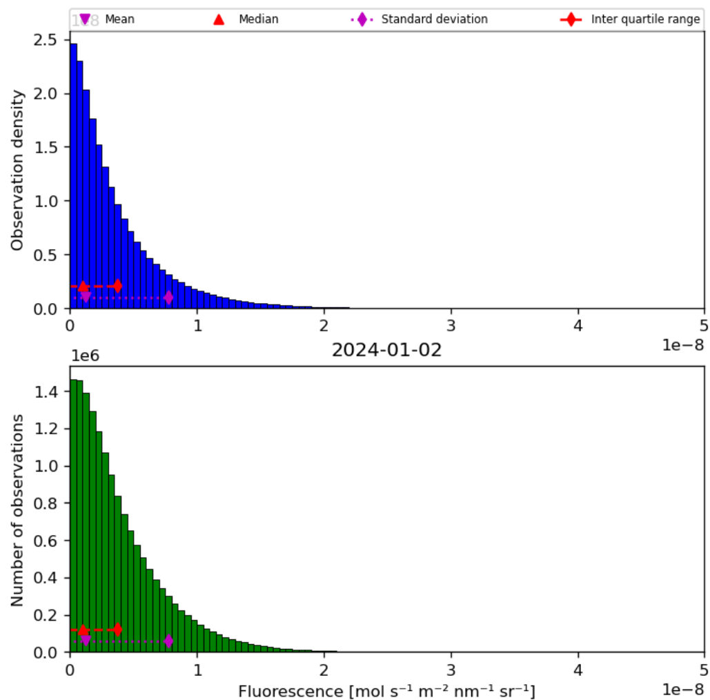
Figure 40: Histogram of “Fluorescence” for 2024-01-01 to 2024-01-03
