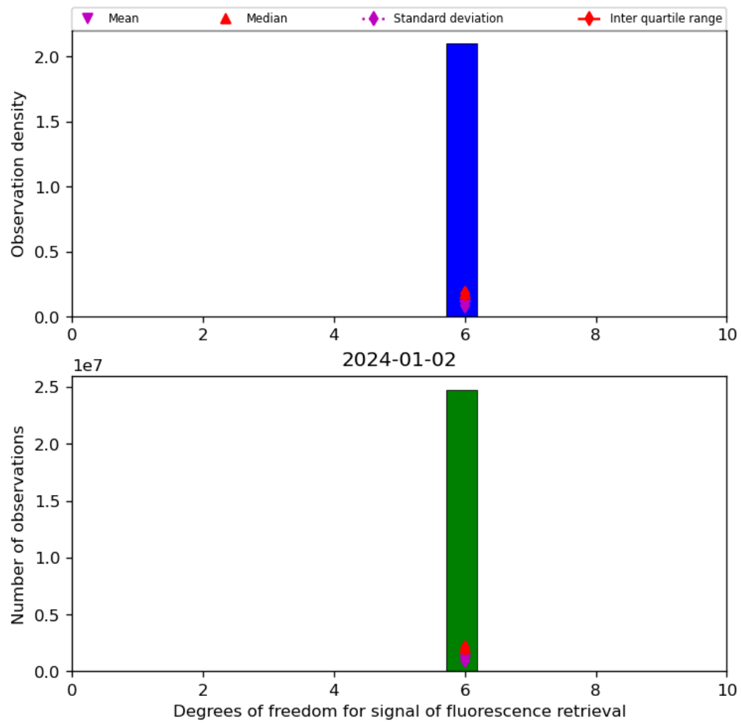
Figure 43: Histogram of “Degrees of freedom for signal of fluorescence retrieval” for 2024-01-01 to 2024-01-03
