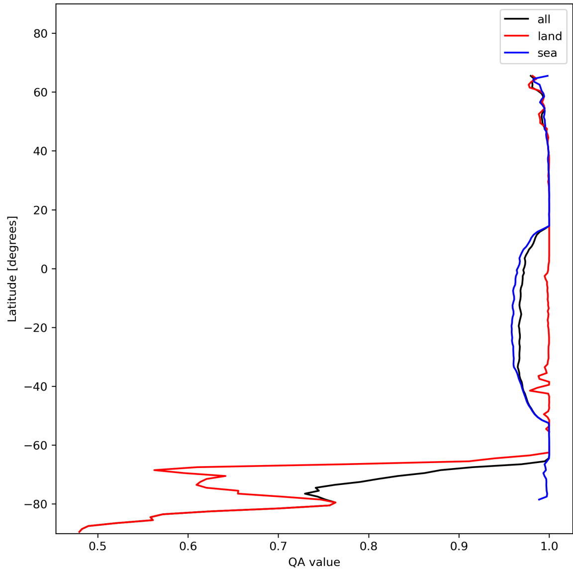
Figure 12: Zonal average of “QA value” for 2024-01-01 to 2024-01-03.
