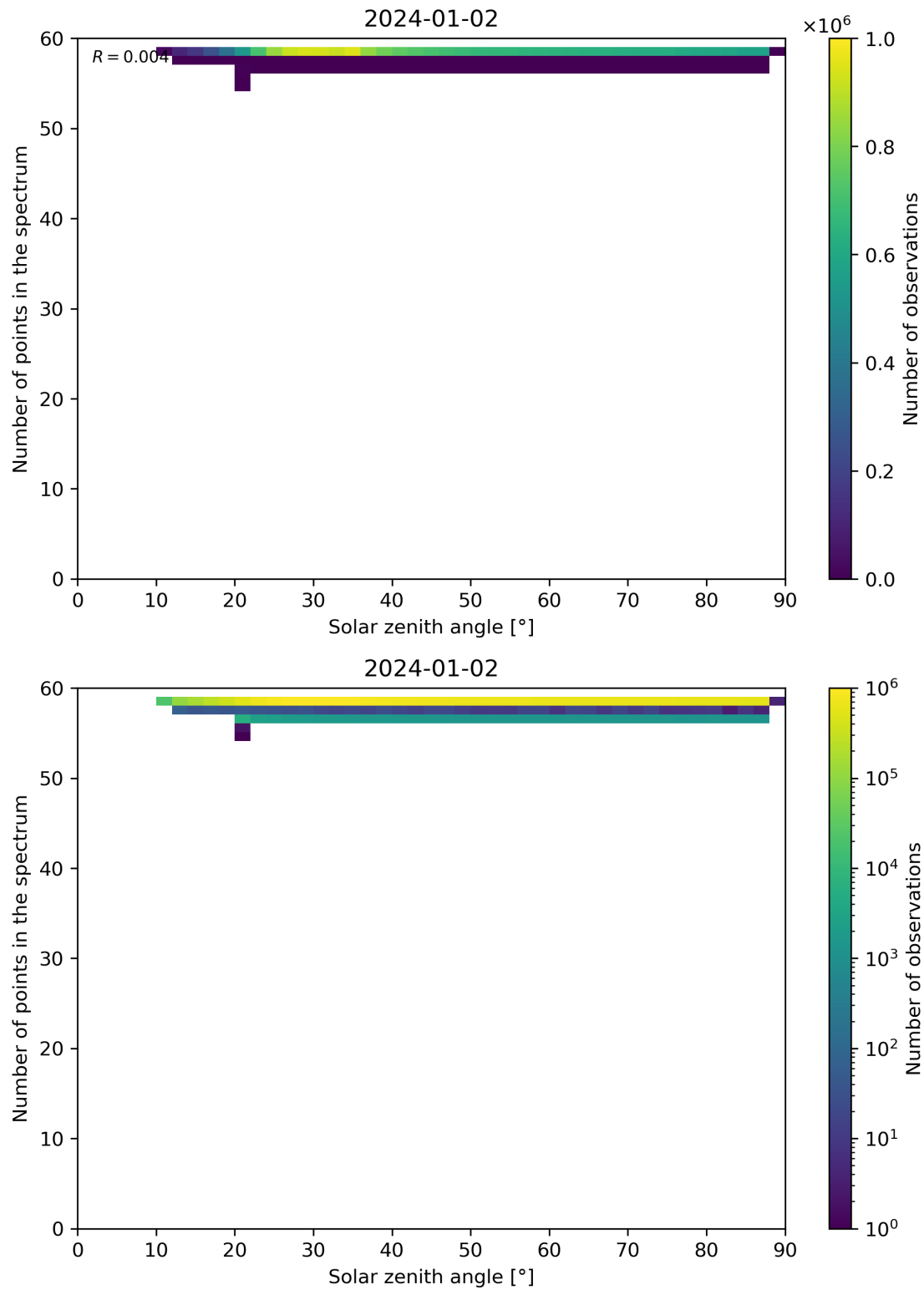
Figure 115: Scatter density plot of “Solar zenith angle” against “Number of points in the spectrum” for 2024-01-01 to 2024-01-03.
