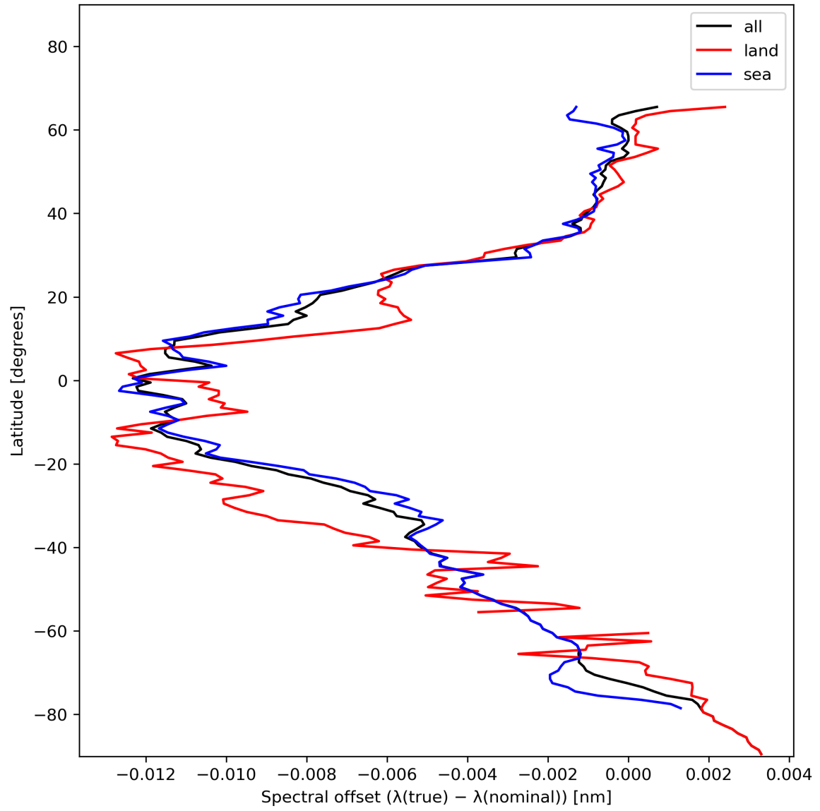
Figure 28: Zonal average of “Spectral offset ( \lambda(\text{true}) - \lambda(\text{nominal}) )” for 2024-01-01 to 2024-01-03.
