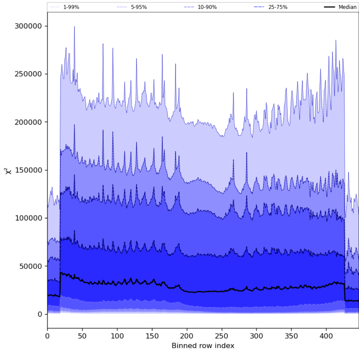
Figure 55: Along track statistics of “ \chi^2 ” for 2024-01-01 to 2024-01-03
