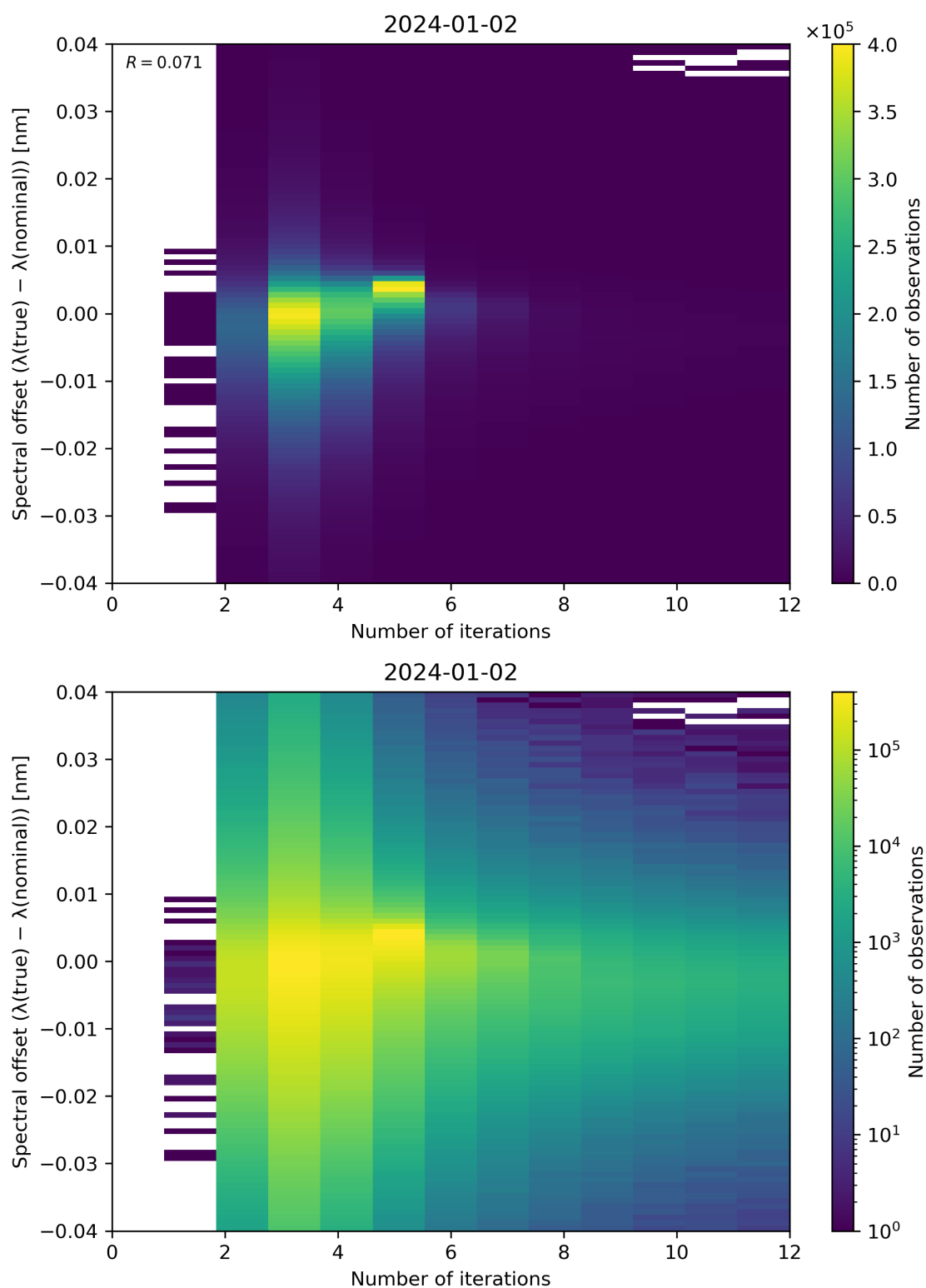
Figure 100: Scatter density plot of “Number of iterations” against “Spectral offset ( \lambda(\text{true}) - \lambda(\text{nominal}) )” for 2024-01-01 to 2024-01-03.
