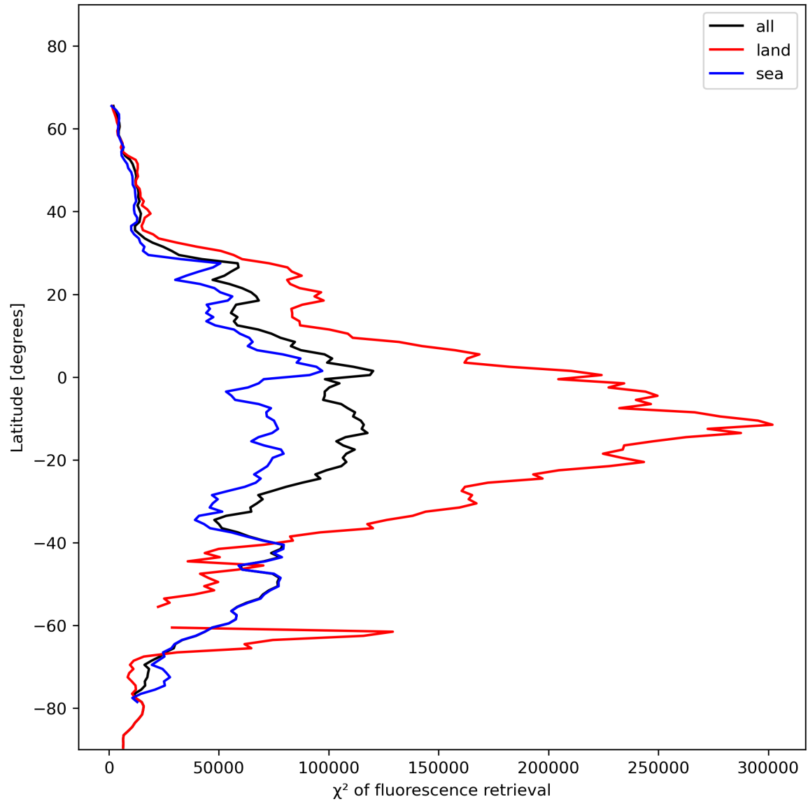
Figure 25: Zonal average of “ \chi^2 of fluorescence retrieval” for 2024-01-01 to 2024-01-03.
