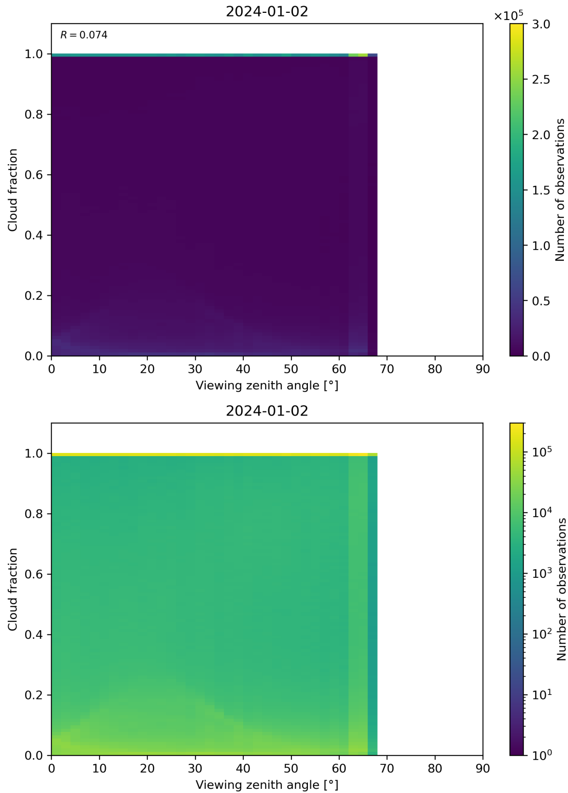
Figure 120: Scatter density plot of “Viewing zenith angle” against “Cloud fraction” for 2024-01-01 to 2024-01-03.
