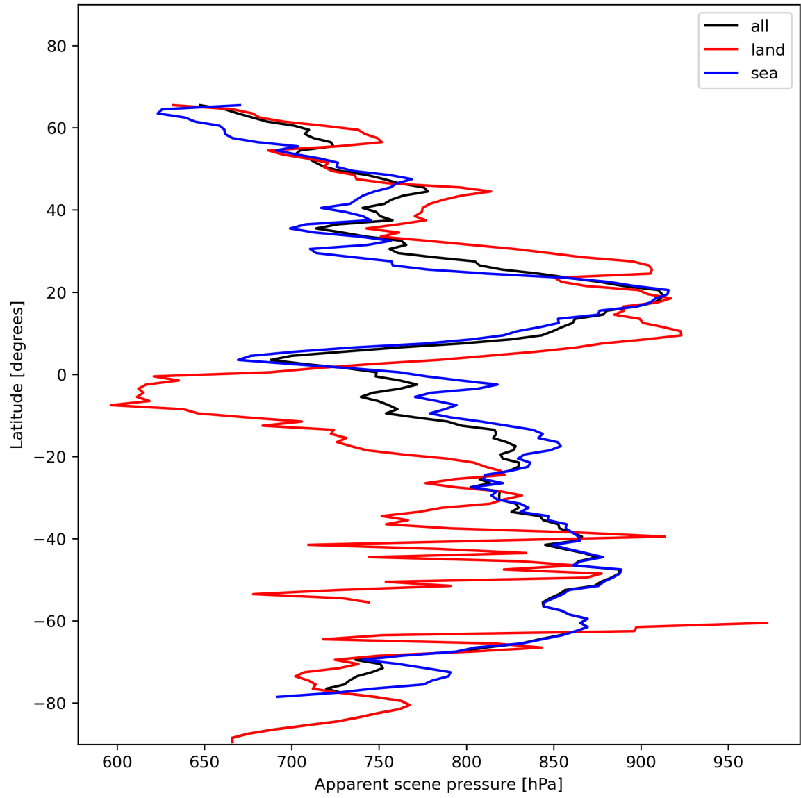
Figure 19: Zonal average of “Apparent scene pressure” for 2024-01-01 to 2024-01-03.
