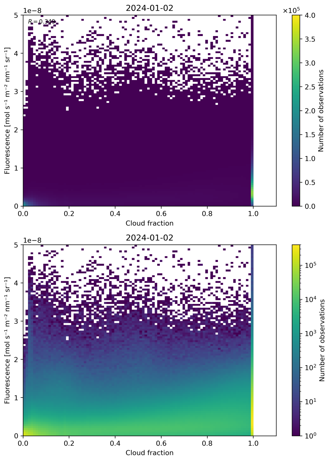
Figure 72: Scatter density plot of “Cloud fraction” against “Fluorescence” for 2024-01-01 to 2024-01-03.
