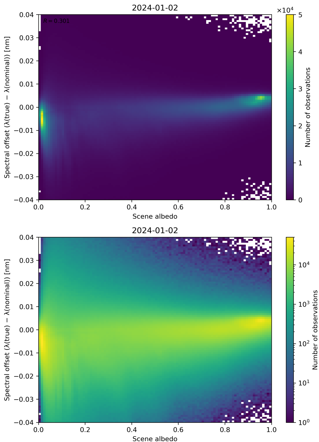
Figure 107: Scatter density plot of “Scene albedo” against “Spectral offset ( \lambda(\text{true}) - \lambda(\text{nominal}) )” for 2024-01-01 to 2024-01-03.
