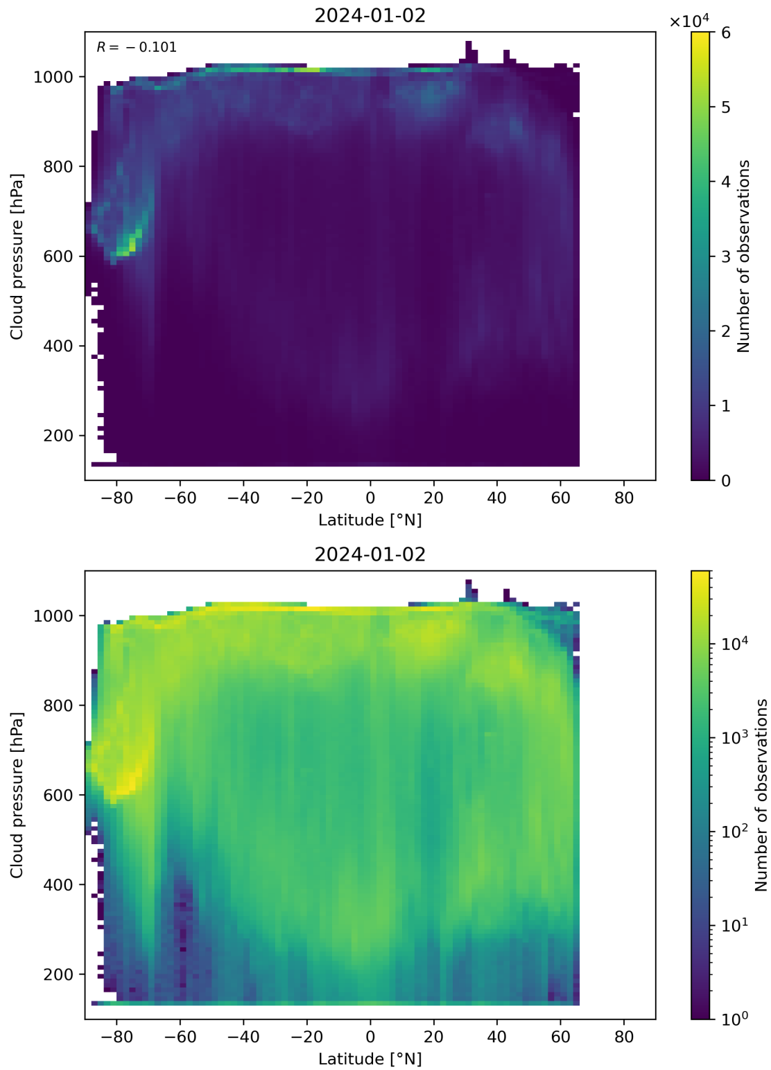
Figure 91: Scatter density plot of “Latitude” against “Cloud pressure” for 2024-01-01 to 2024-01-03.
