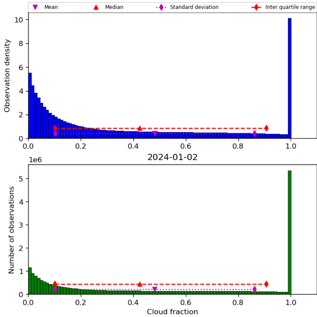
Figure 32: Histogram of “Cloud fraction” for 2024-01-01 to 2024-01-03
