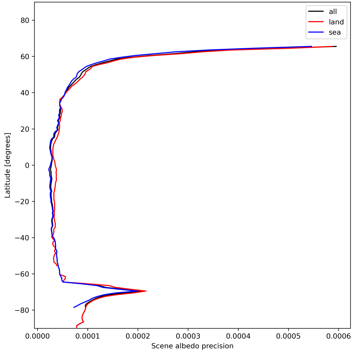
Figure 18: Zonal average of “Scene albedo precision” for 2024-01-01 to 2024-01-03.
