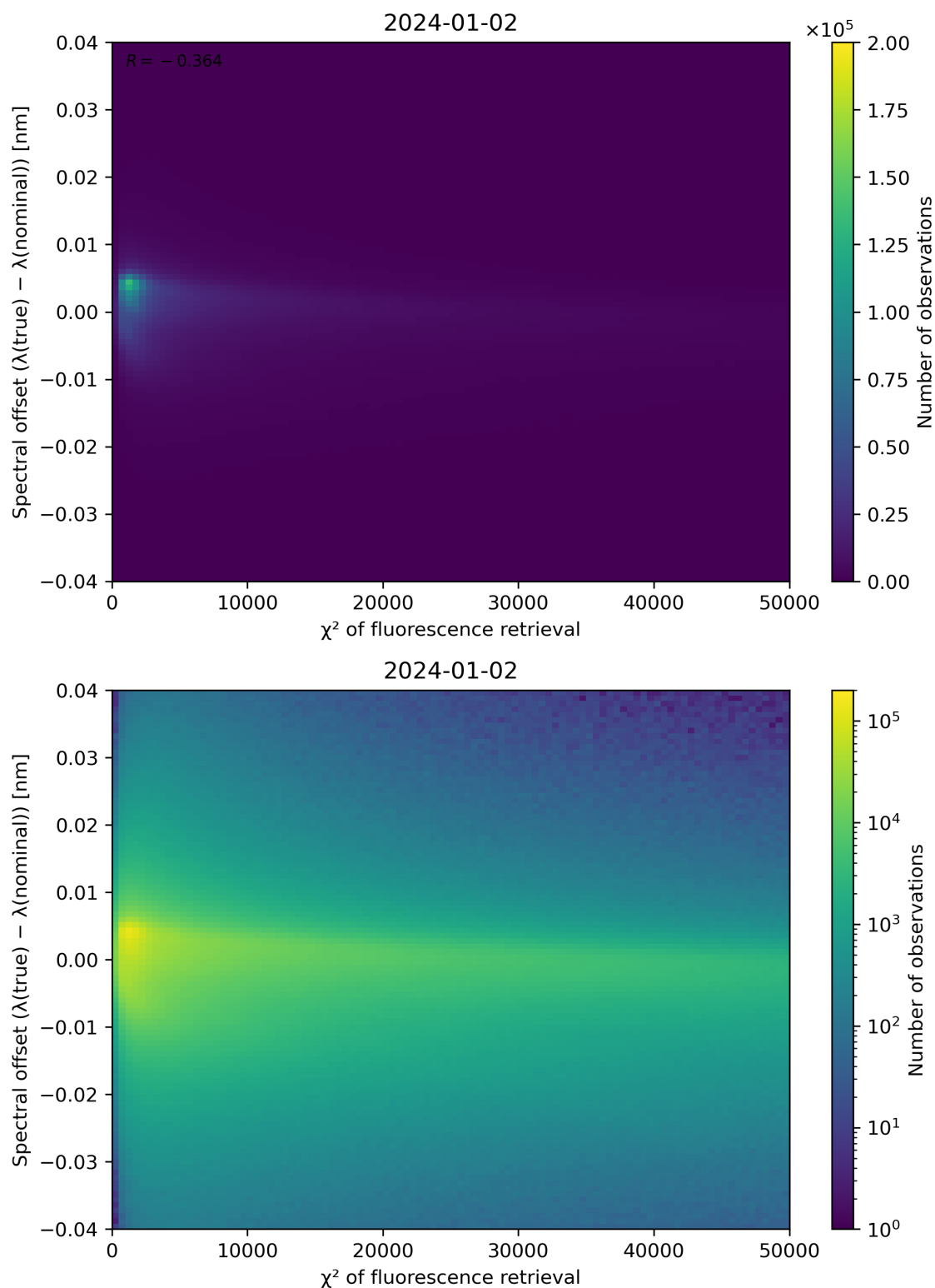
Figure 69: Scatter density plot of " \chi^2 of fluorescence retrieval" against "Spectral offset ( \lambda(\text{true}) - \lambda(\text{nominal}) )" for 2024-01-01 to 2024-01-03.
