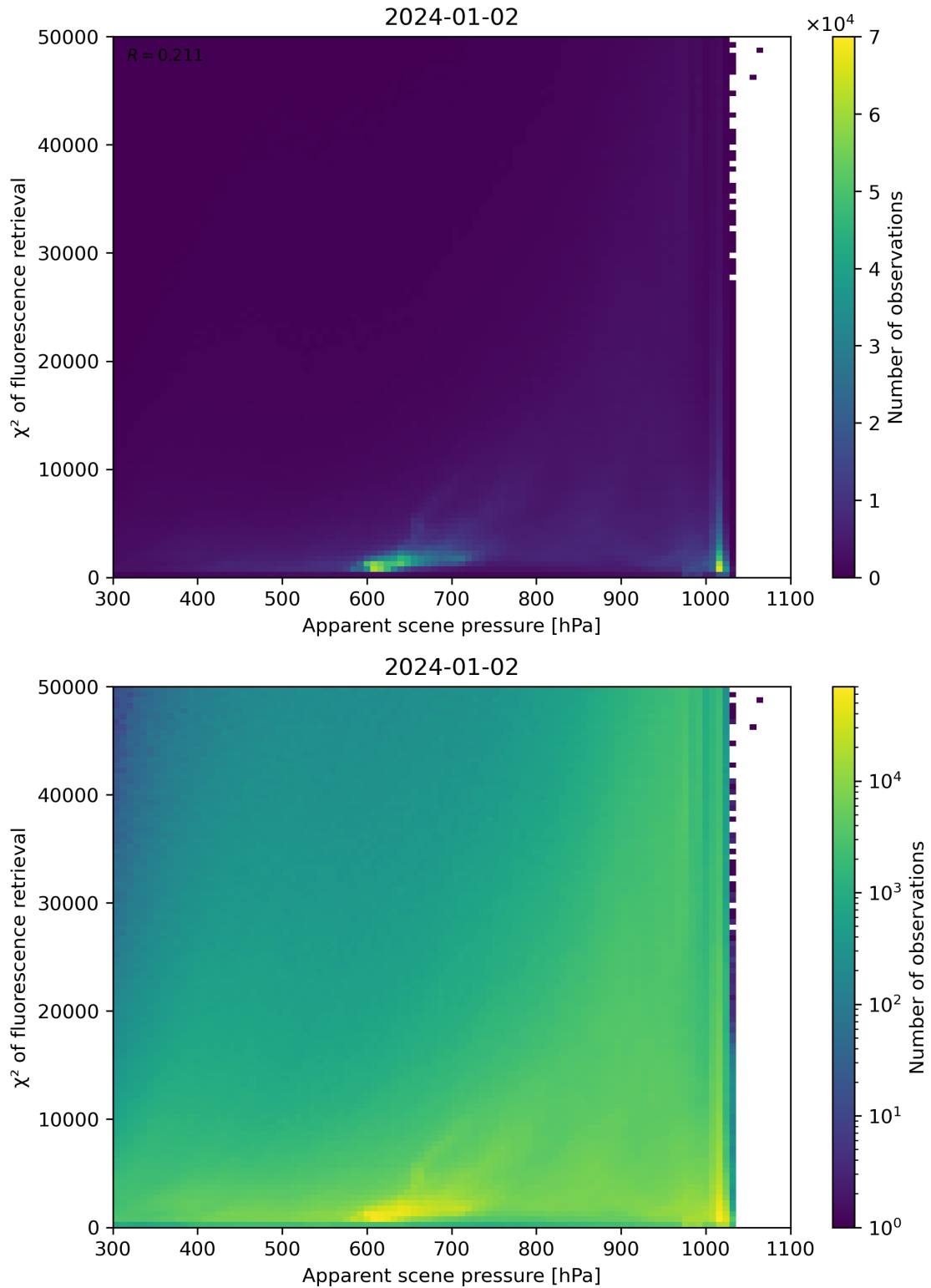
Figure 63: Scatter density plot of “Apparent scene pressure” against “ \chi^2 of fluorescence retrieval” for 2024-01-01 to 2024-01-03.
