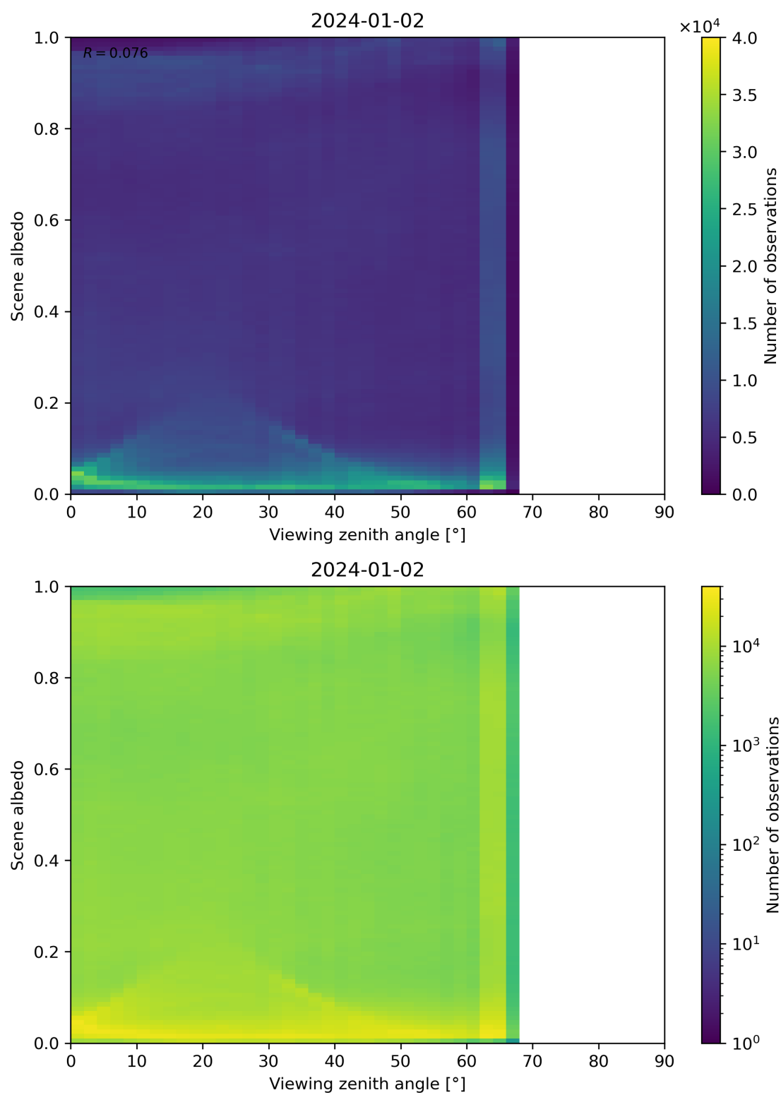
Figure 126: Scatter density plot of “Viewing zenith angle” against “Scene albedo” for 2024-01-01 to 2024-01-03.
