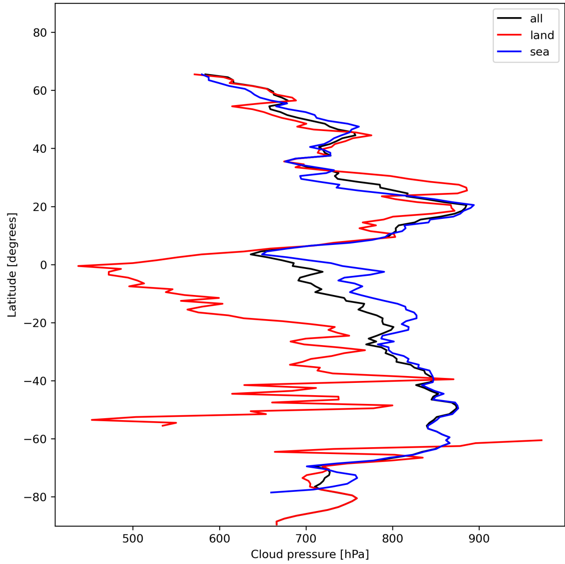
Figure 13: Zonal average of “Cloud pressure” for 2024-01-01 to 2024-01-03.
