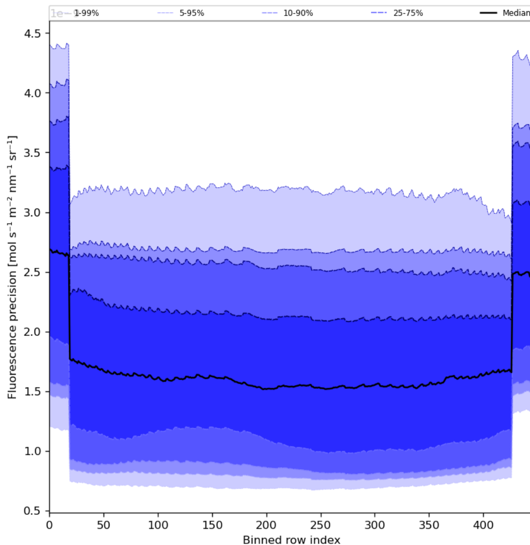
Figure 58: Along track statistics of “Fluorescence precision” for 2024-01-01 to 2024-01-03
