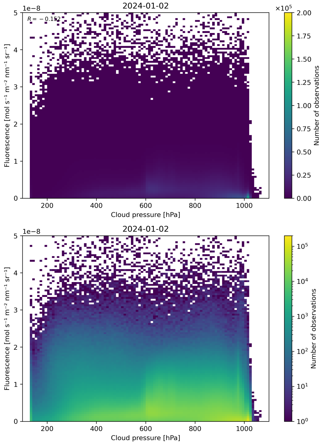
Figure 80: Scatter density plot of “Cloud pressure” against “Fluorescence” for 2024-01-01 to 2024-01-03.
