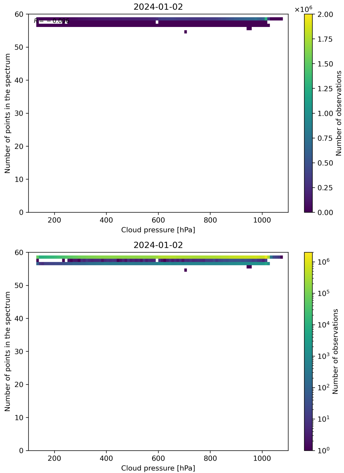
Figure 82: Scatter density plot of “Cloud pressure” against “Number of points in the spectrum” for 2024-01-01 to 2024-01-03.
