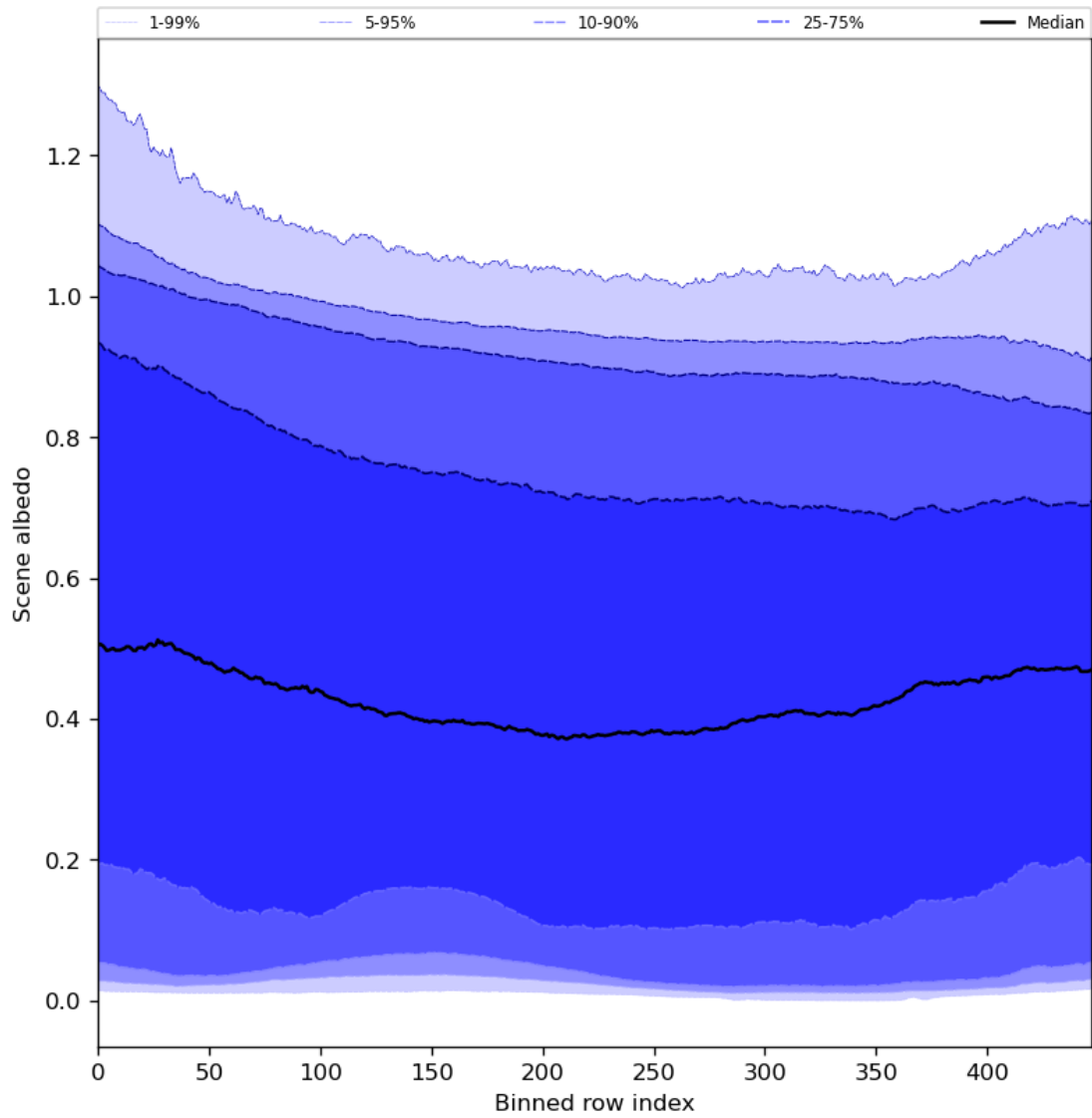
Figure 51: Along track statistics of “Scene albedo” for 2024-01-01 to 2024-01-03
