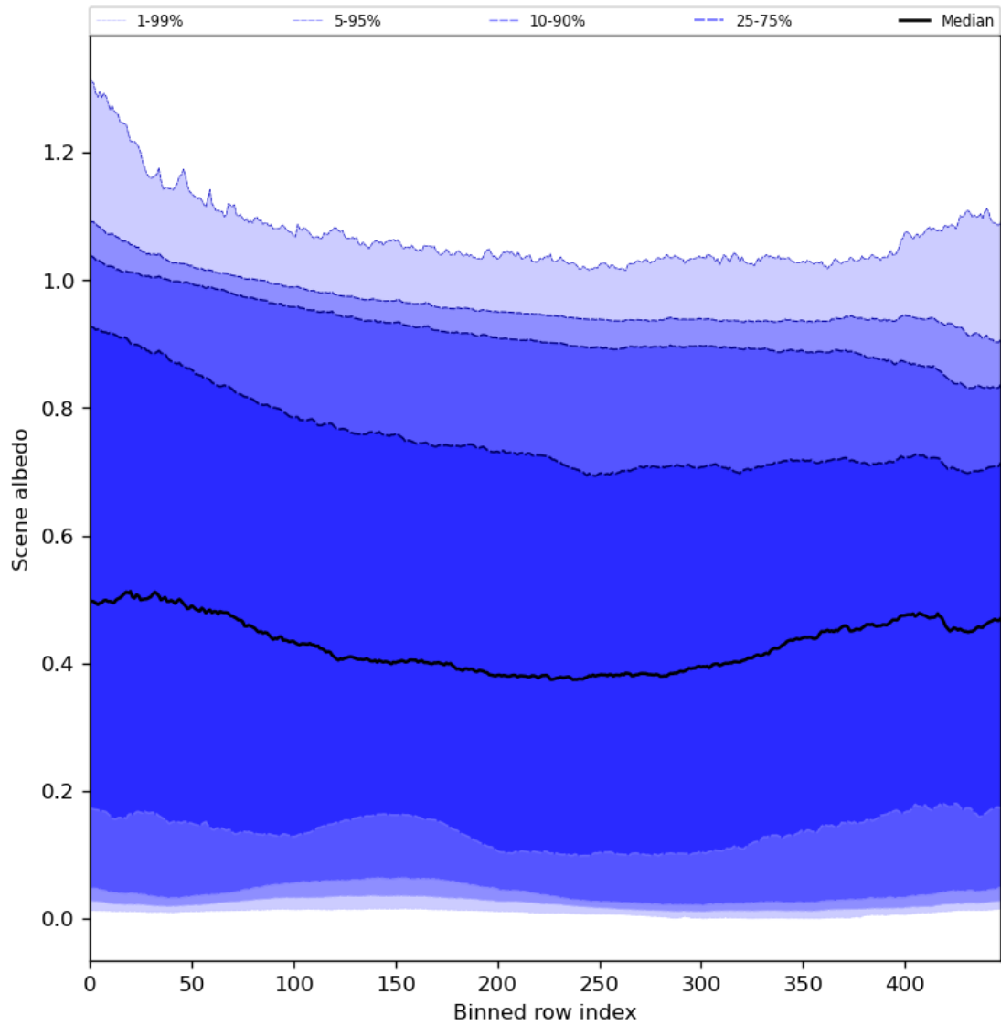
Figure 51: Along track statistics of “Scene albedo” for 2024-01-02 to 2024-01-04
