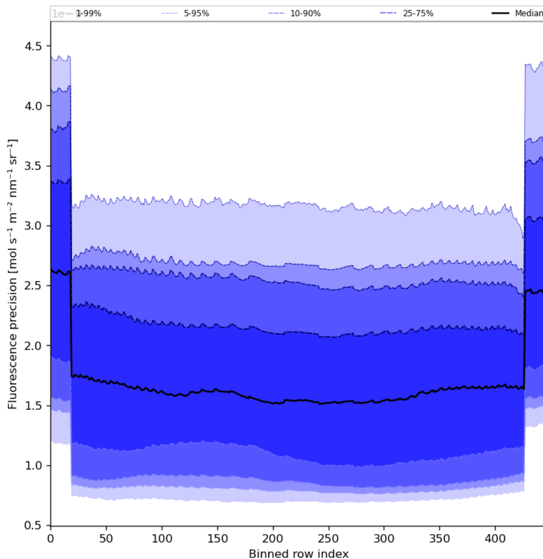
Figure 58: Along track statistics of “Fluorescence precision” for 2024-01-02 to 2024-01-04
