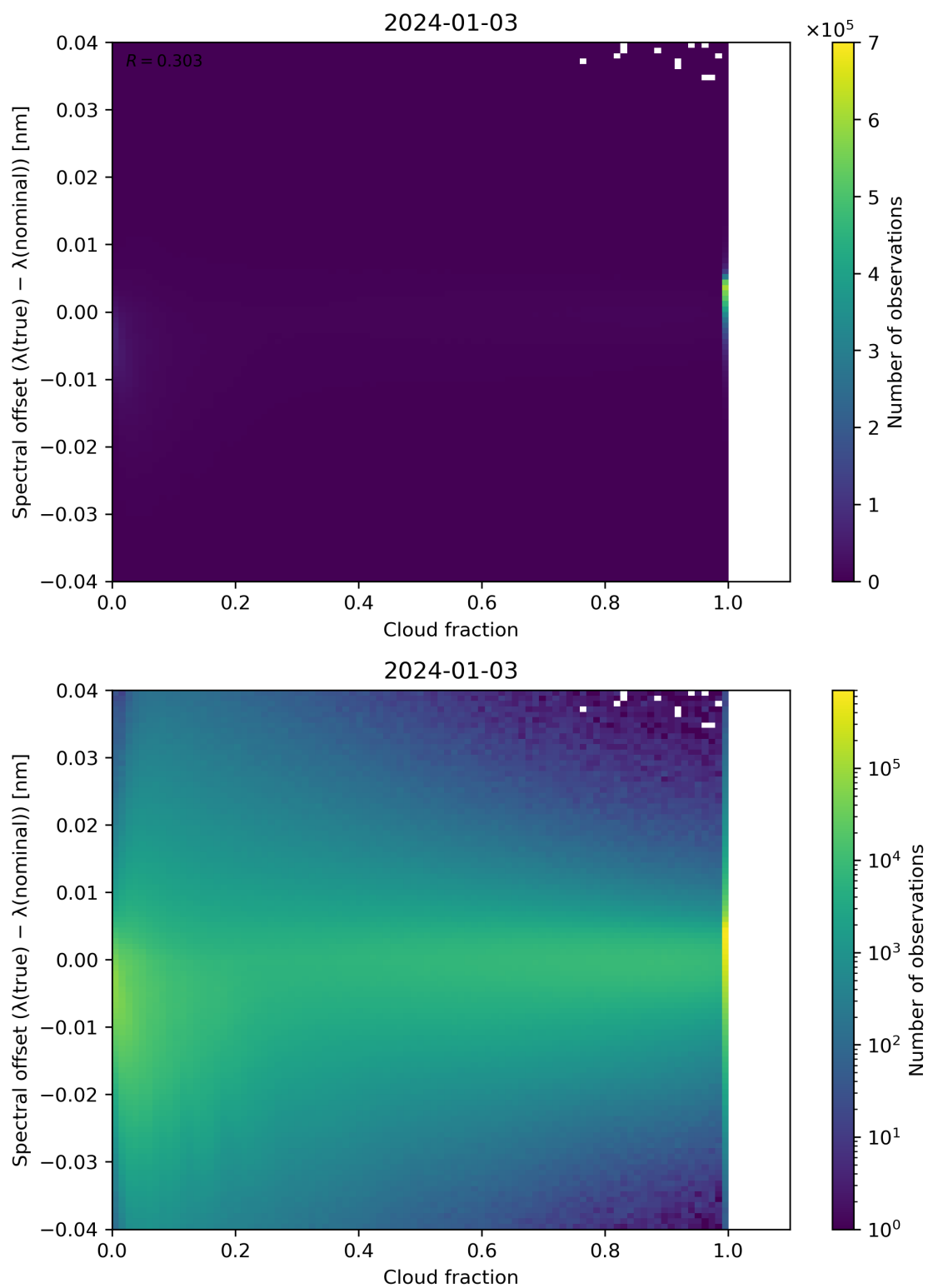
Figure 76: Scatter density plot of “Cloud fraction” against “Spectral offset ( \lambda(\text{true}) - \lambda(\text{nominal}) )” for 2024-01-02 to 2024-01-04.
