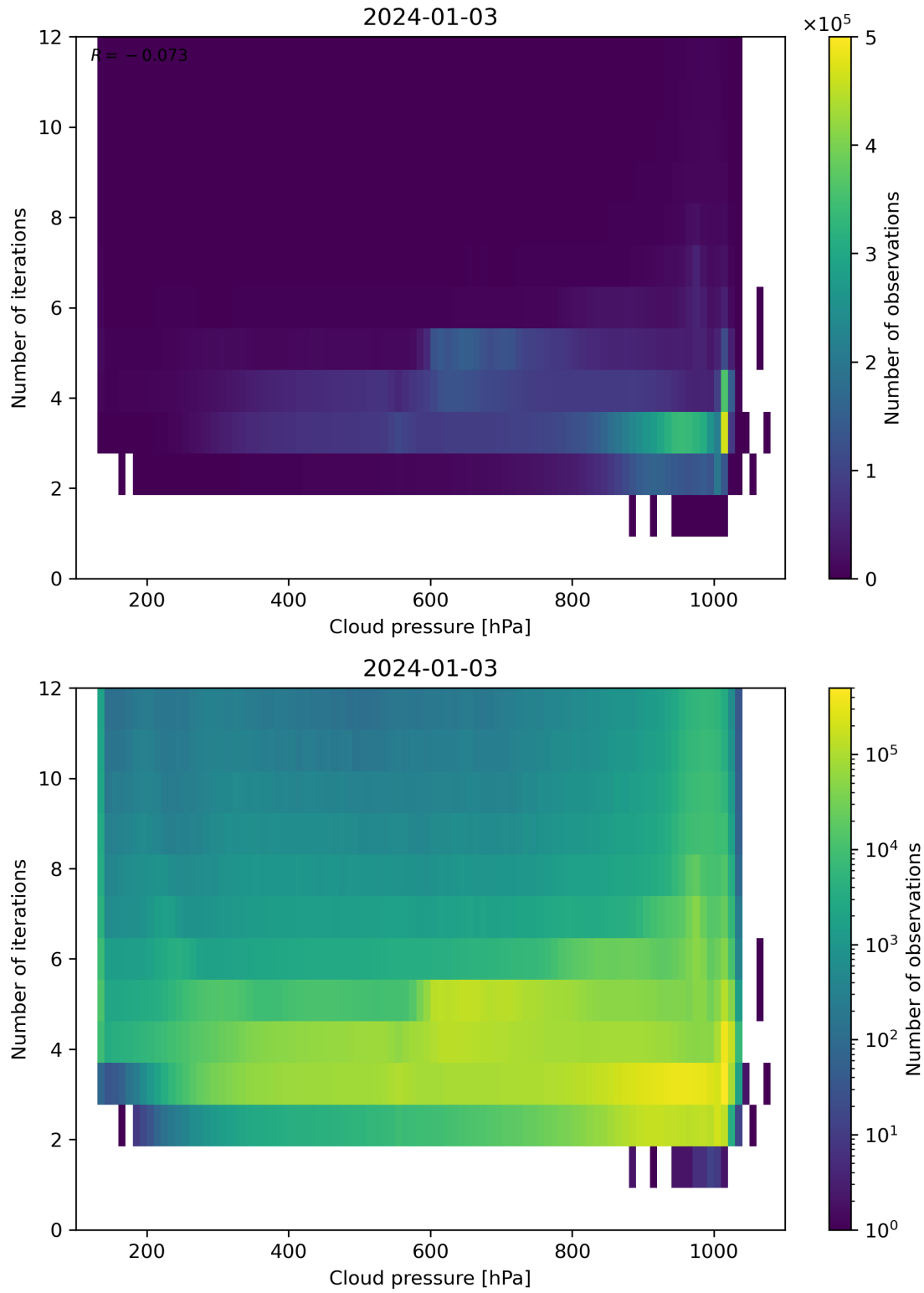
Figure 81: Scatter density plot of “Cloud pressure” against “Number of iterations” for 2024-01-02 to 2024-01-04.
