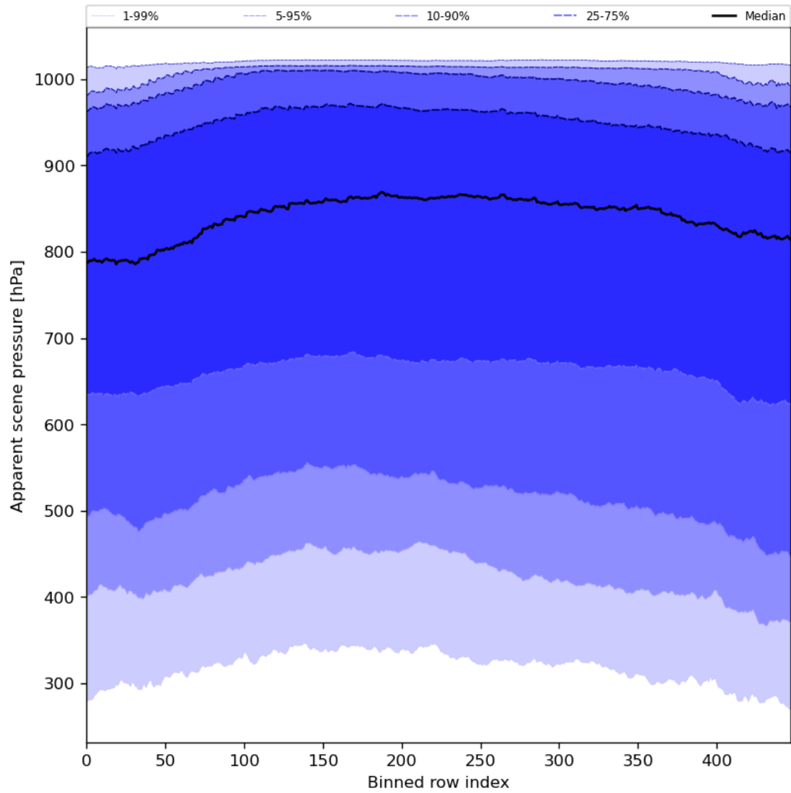
Figure 53: Along track statistics of “Apparent scene pressure” for 2024-01-02 to 2024-01-04
