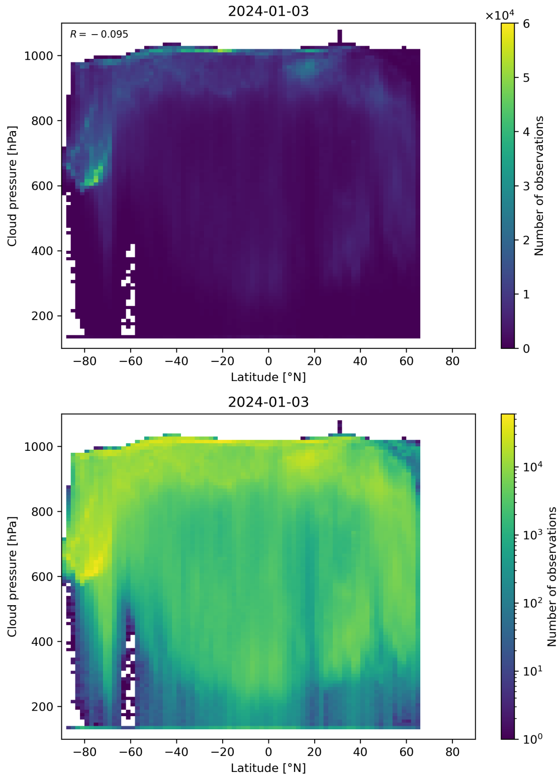
Figure 91: Scatter density plot of “Latitude” against “Cloud pressure” for 2024-01-02 to 2024-01-04.
