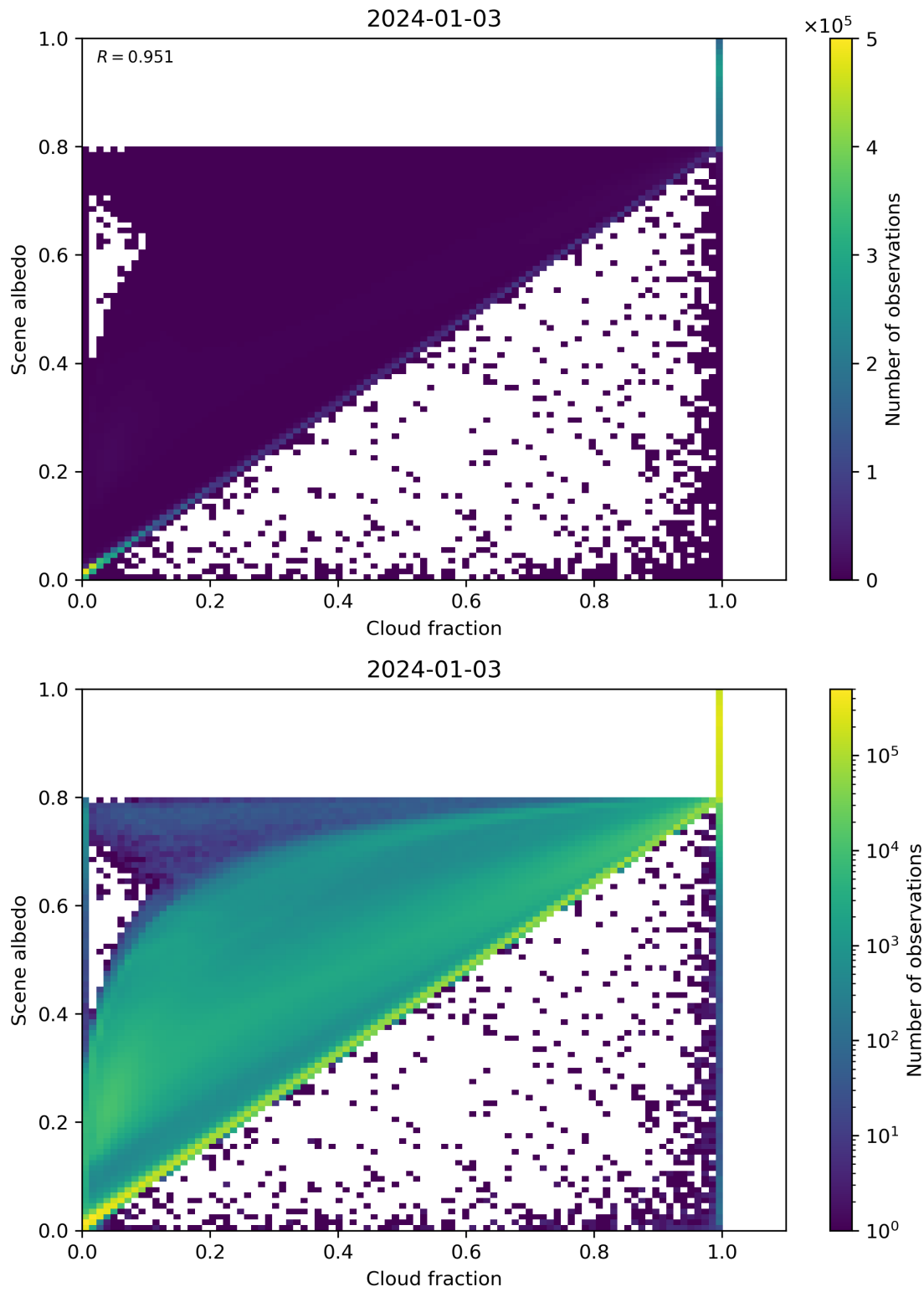
Figure 75: Scatter density plot of “Cloud fraction” against “Scene albedo” for 2024-01-02 to 2024-01-04.
