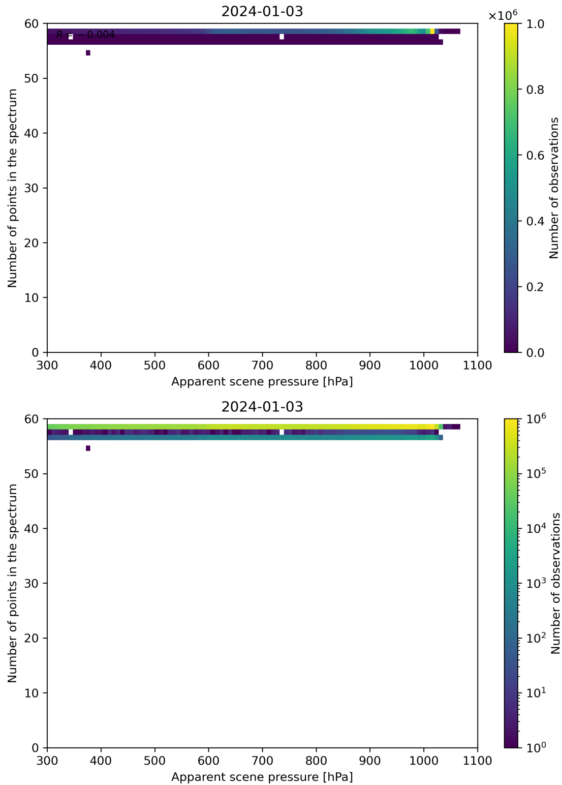
Figure 66: Scatter density plot of “Apparent scene pressure” against “Number of points in the spectrum” for 2024-01-02 to 2024-01-04.
