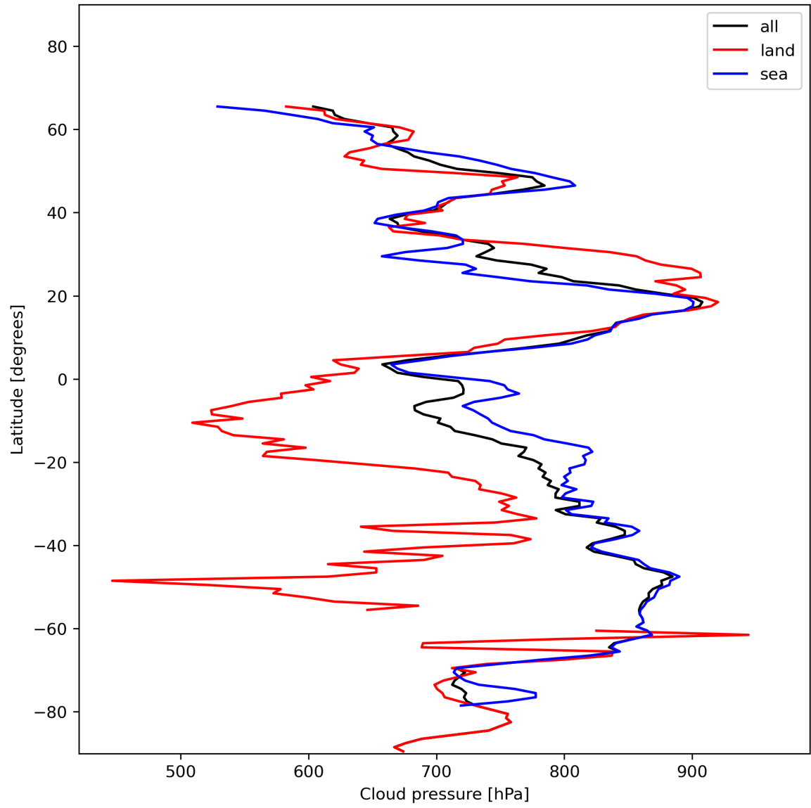
Figure 13: Zonal average of “Cloud pressure” for 2024-01-02 to 2024-01-04.
