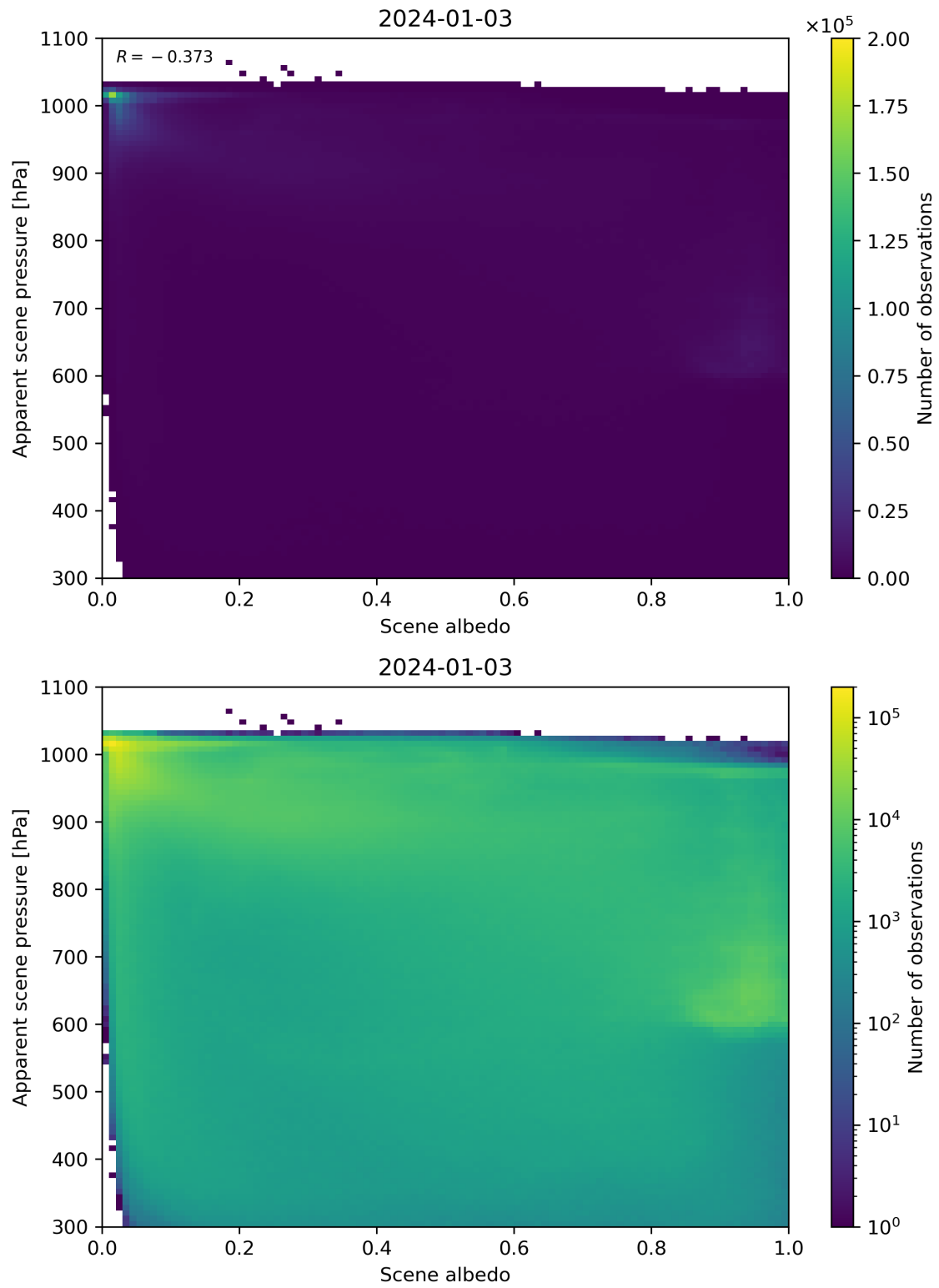
Figure 102: Scatter density plot of “Scene albedo” against “Apparent scene pressure” for 2024-01-02 to 2024-01-04.
