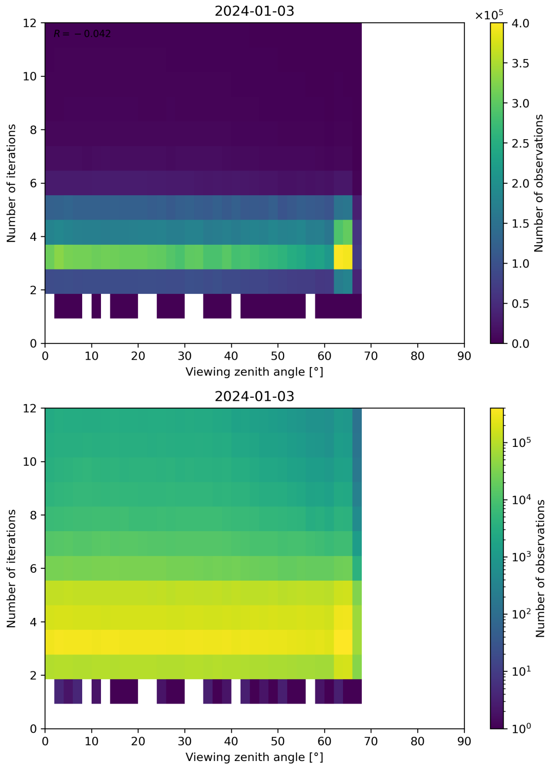
Figure 124: Scatter density plot of “Viewing zenith angle” against “Number of iterations” for 2024-01-02 to 2024-01-04.
