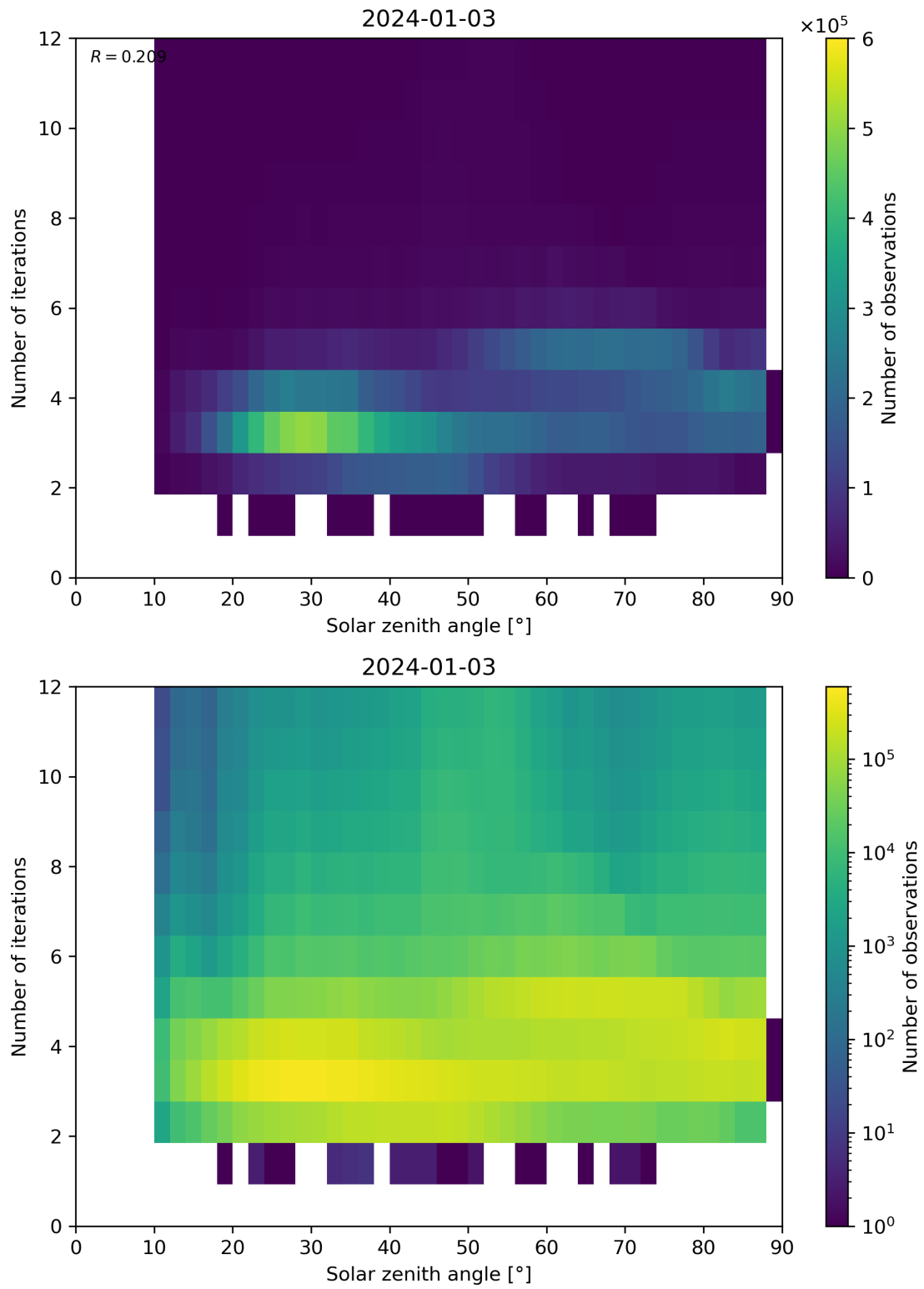
Figure 114: Scatter density plot of “Solar zenith angle” against “Number of iterations” for 2024-01-02 to 2024-01-04.
