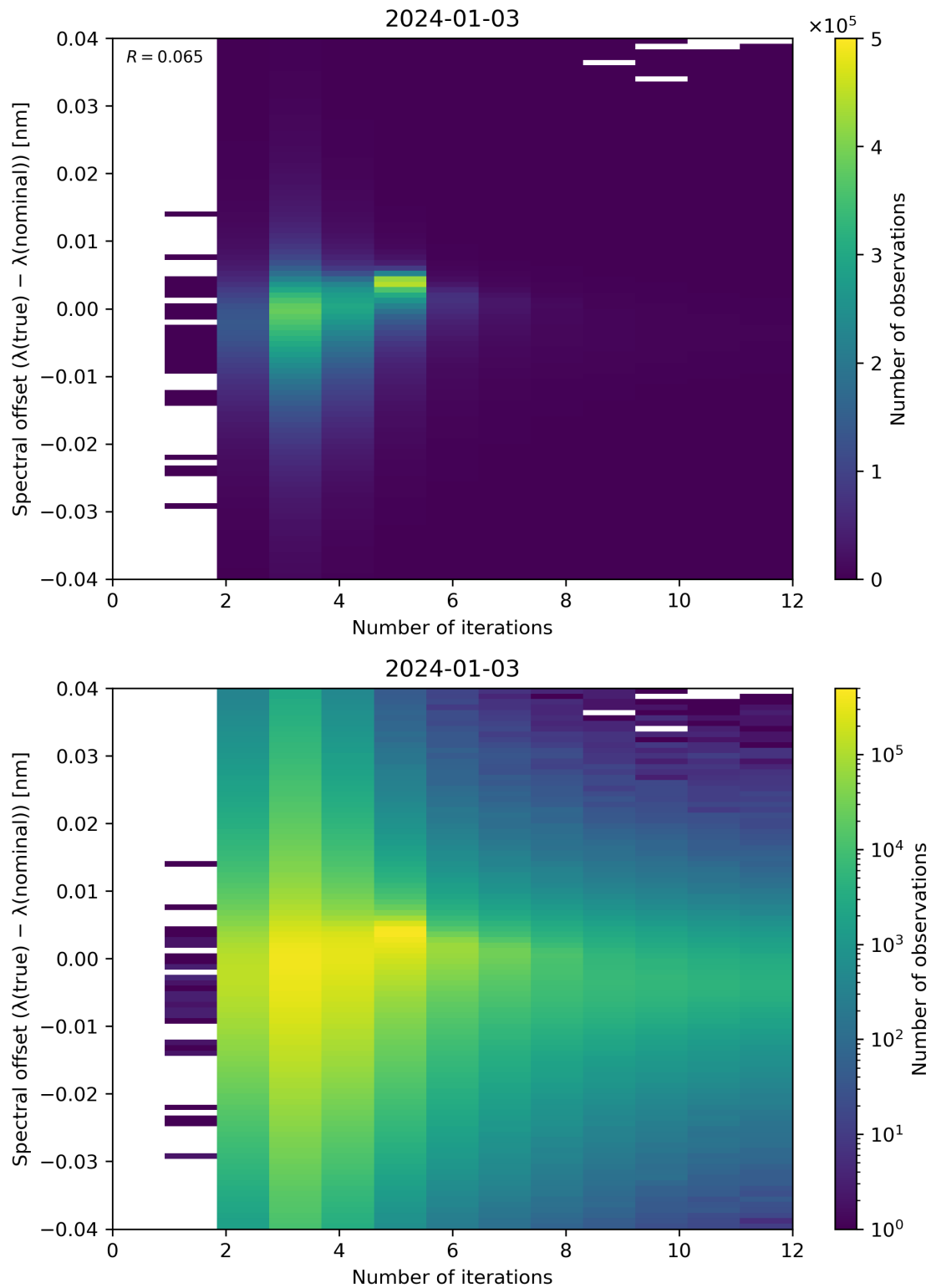
Figure 100: Scatter density plot of “Number of iterations” against “Spectral offset ( \lambda(\text{true}) - \lambda(\text{nominal}) )” for 2024-01-02 to 2024-01-04.
