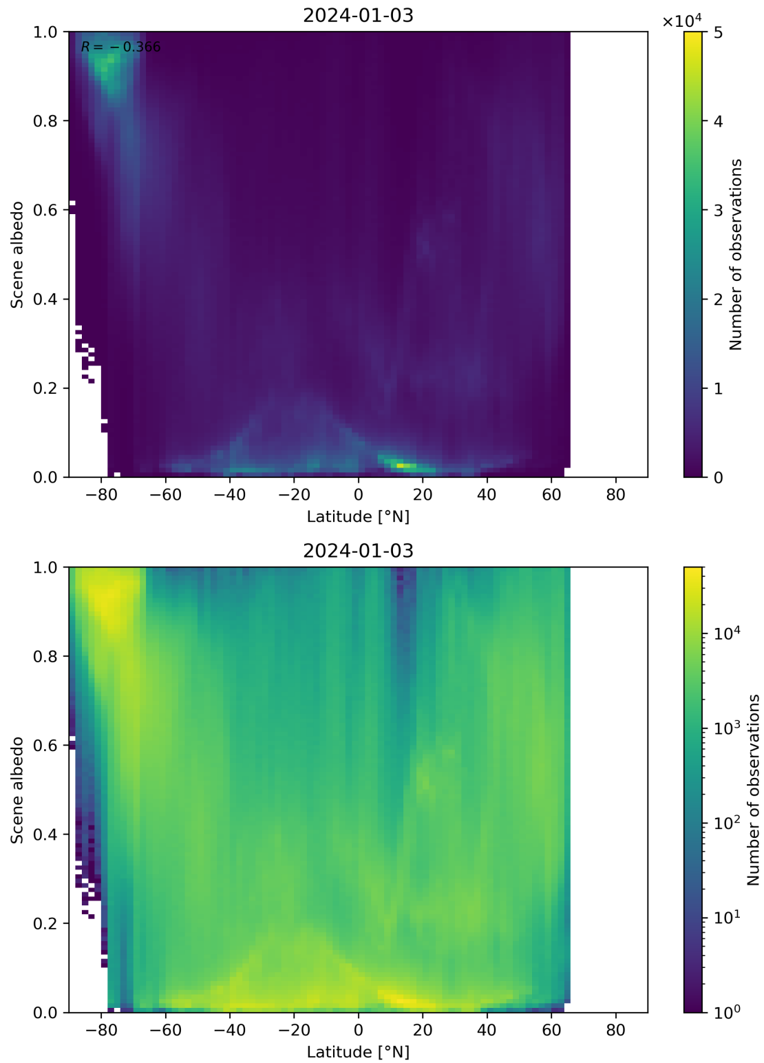
Figure 95: Scatter density plot of “Latitude” against “Scene albedo” for 2024-01-02 to 2024-01-04.
