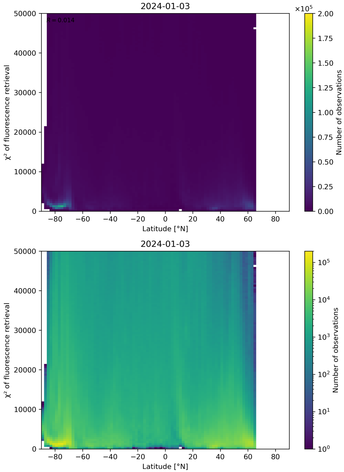
Figure 89: Scatter density plot of “Latitude” against “ \chi^2 of fluorescence retrieval” for 2024-01-02 to 2024-01-04.
