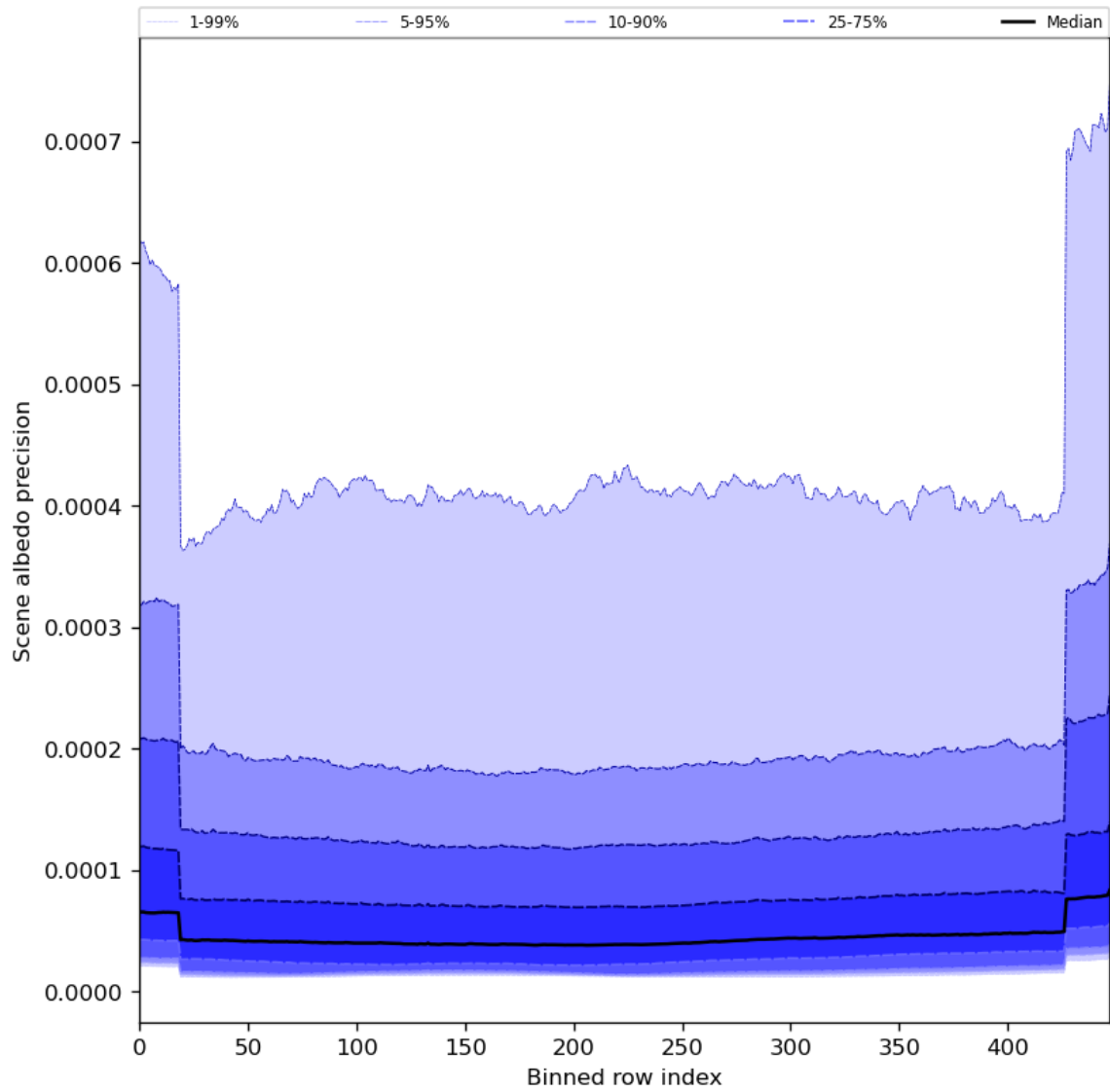
Figure 52: Along track statistics of “Scene albedo precision” for 2024-01-02 to 2024-01-04
