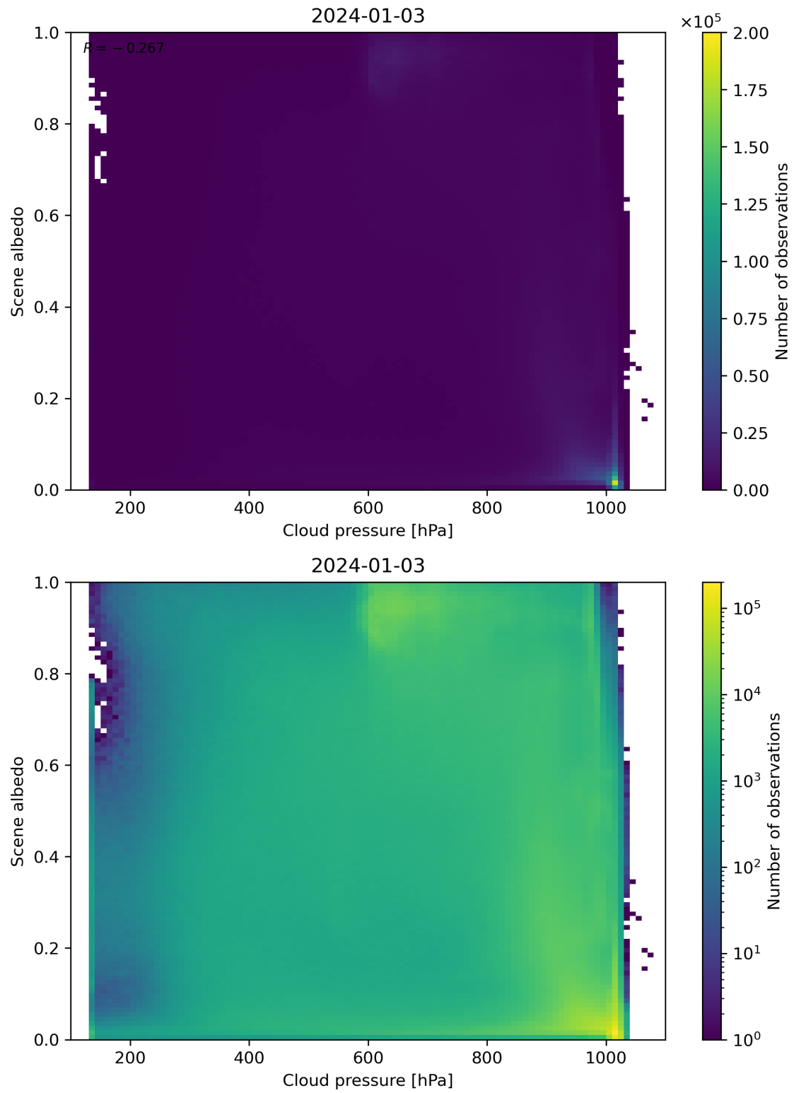
Figure 83: Scatter density plot of “Cloud pressure” against “Scene albedo” for 2024-01-02 to 2024-01-04.
