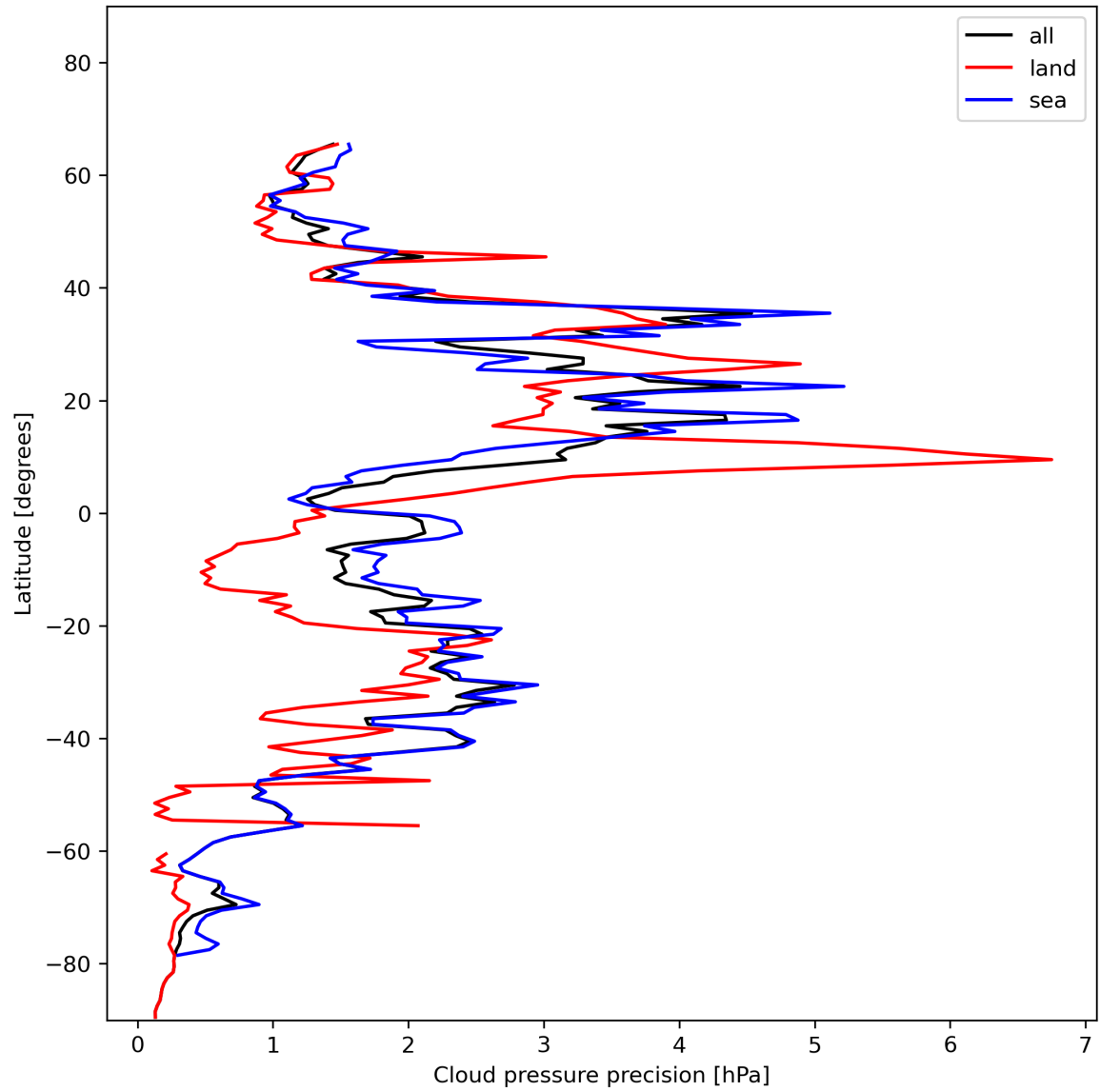
Figure 14: Zonal average of “Cloud pressure precision” for 2024-01-02 to 2024-01-04.
