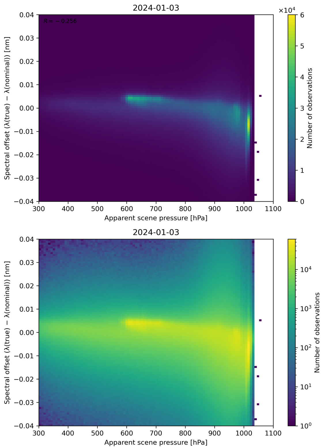
Figure 67: Scatter density plot of “Apparent scene pressure” against “Spectral offset ( \lambda(\text{true}) - \lambda(\text{nominal}) )” for 2024-01-02 to 2024-01-04.
