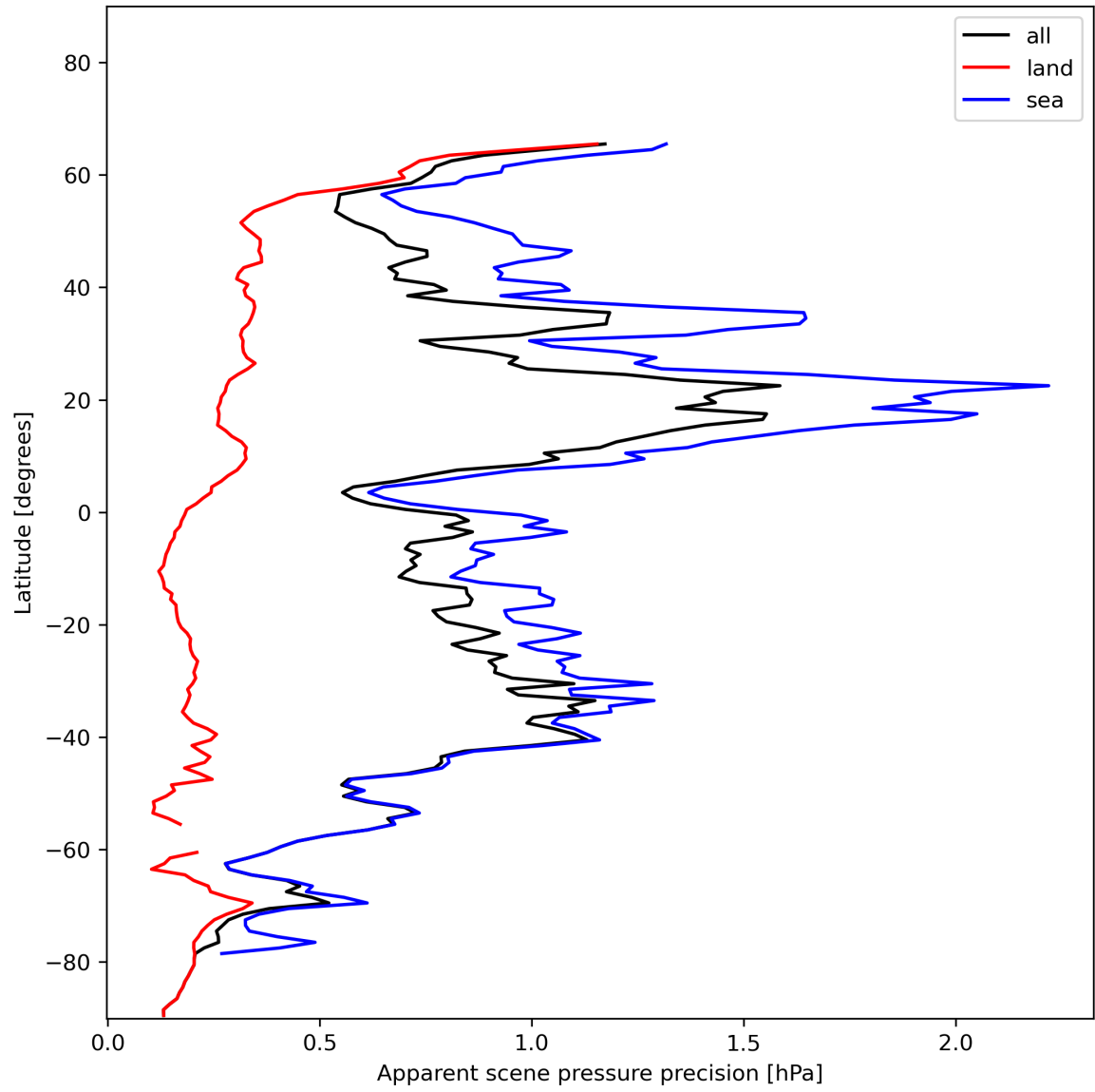
Figure 20: Zonal average of “Apparent scene pressure precision” for 2024-01-02 to 2024-01-04.
