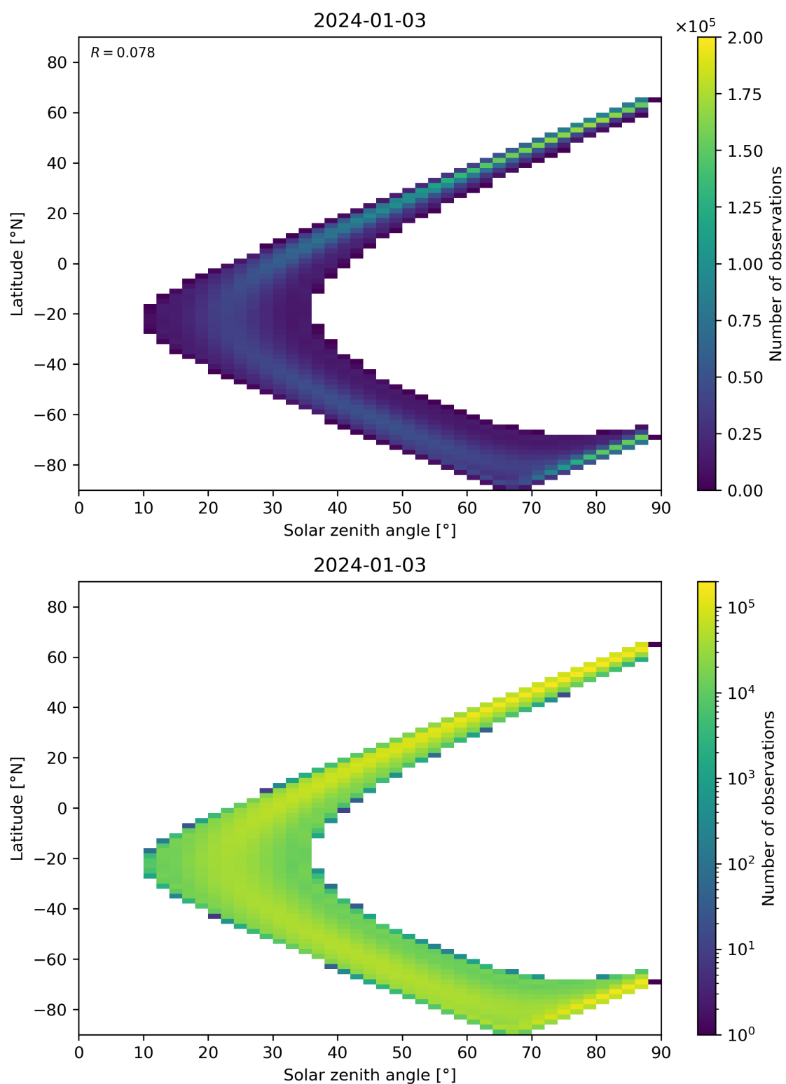
Figure 113: Scatter density plot of “Solar zenith angle” against “Latitude” for 2024-01-02 to 2024-01-04.
