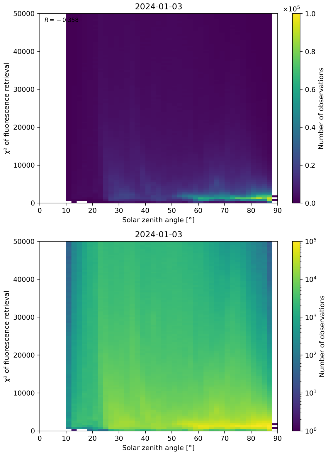
Figure 109: Scatter density plot of “Solar zenith angle” against “ \chi^2 of fluorescence retrieval” for 2024-01-02 to 2024-01-04.
