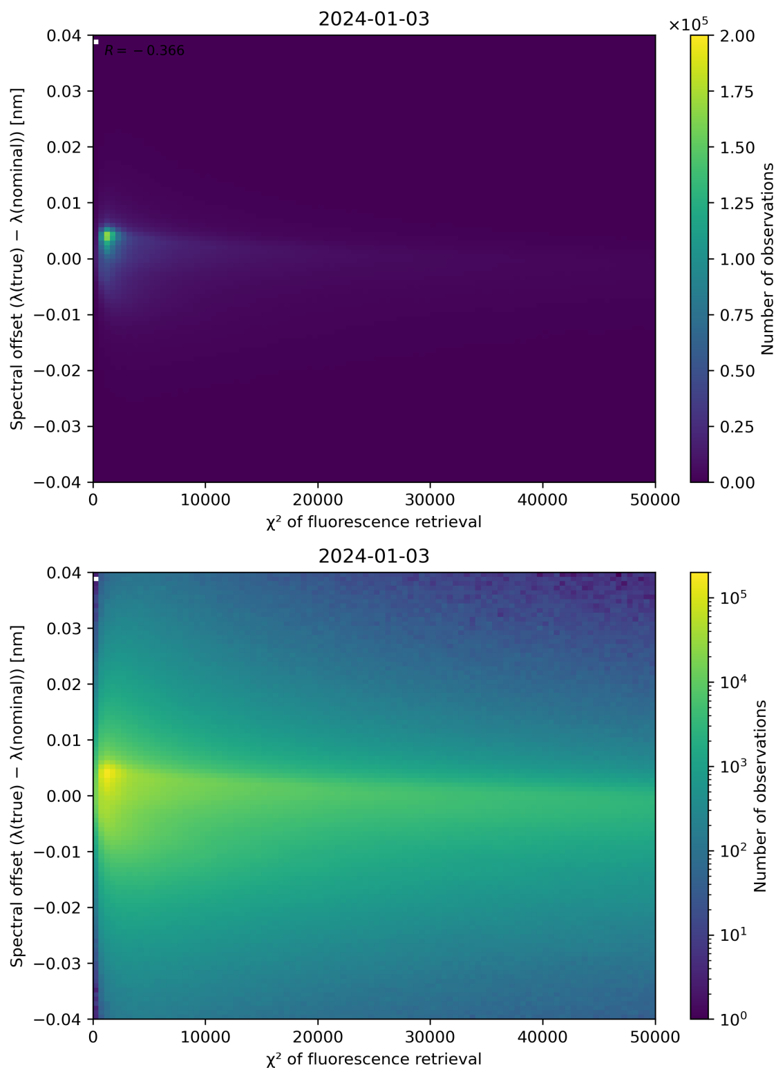
Figure 69: Scatter density plot of " \chi^2 of fluorescence retrieval" against "Spectral offset ( \lambda(\text{true}) - \lambda(\text{nominal})) " for 2024-01-02 to 2024-01-04.
