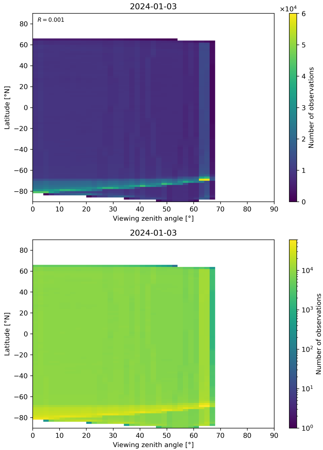
Figure 123: Scatter density plot of “Viewing zenith angle” against “Latitude” for 2024-01-02 to 2024-01-04.
