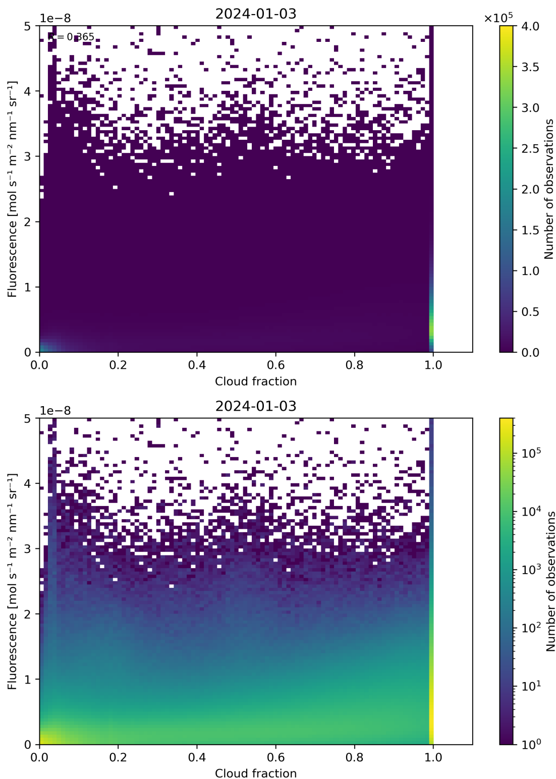
Figure 72: Scatter density plot of “Cloud fraction” against “Fluorescence” for 2024-01-02 to 2024-01-04.
