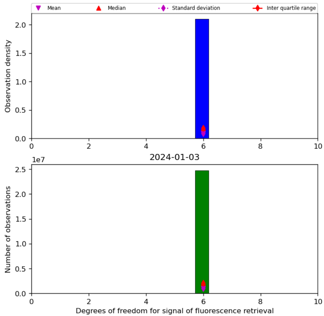
Figure 43: Histogram of “Degrees of freedom for signal of fluorescence retrieval” for 2024-01-02 to 2024-01-04
