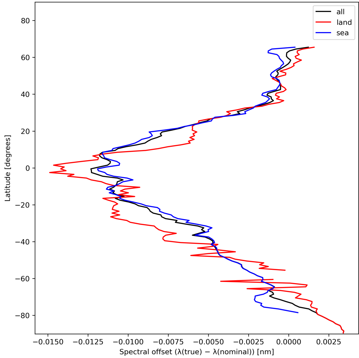
Figure 28: Zonal average of “Spectral offset ( \lambda(\text{true}) - \lambda(\text{nominal}) )” for 2024-01-02 to 2024-01-04.
