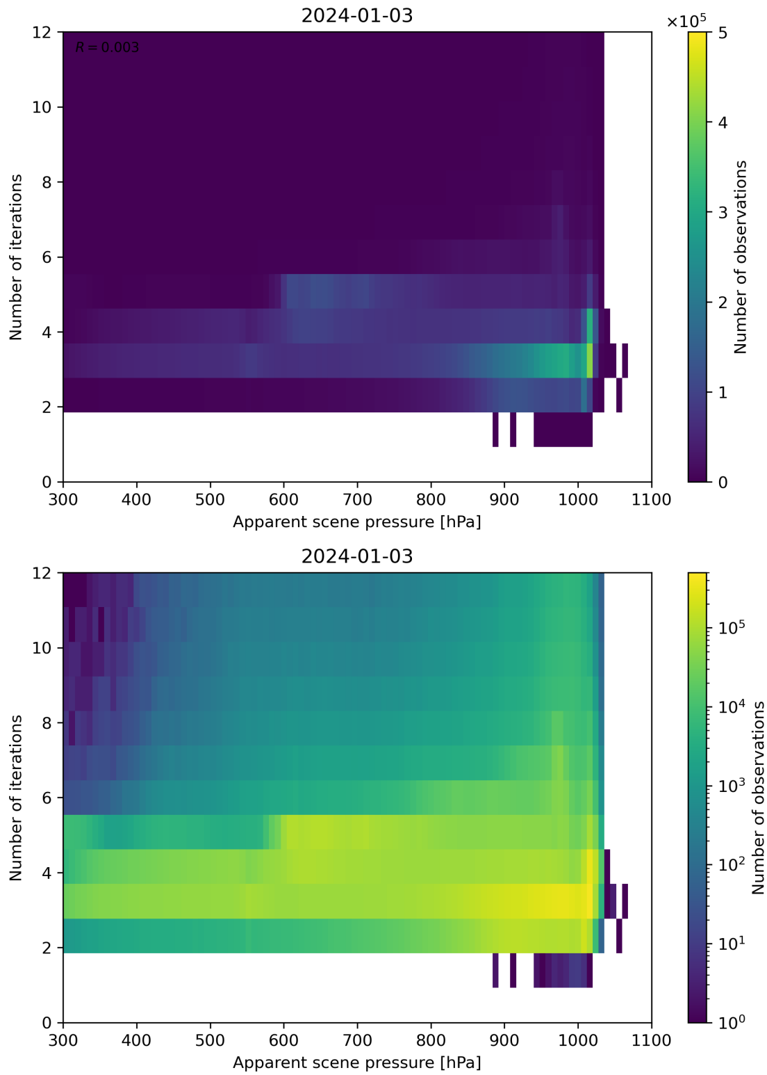
Figure 65: Scatter density plot of “Apparent scene pressure” against “Number of iterations” for 2024-01-02 to 2024-01-04.
