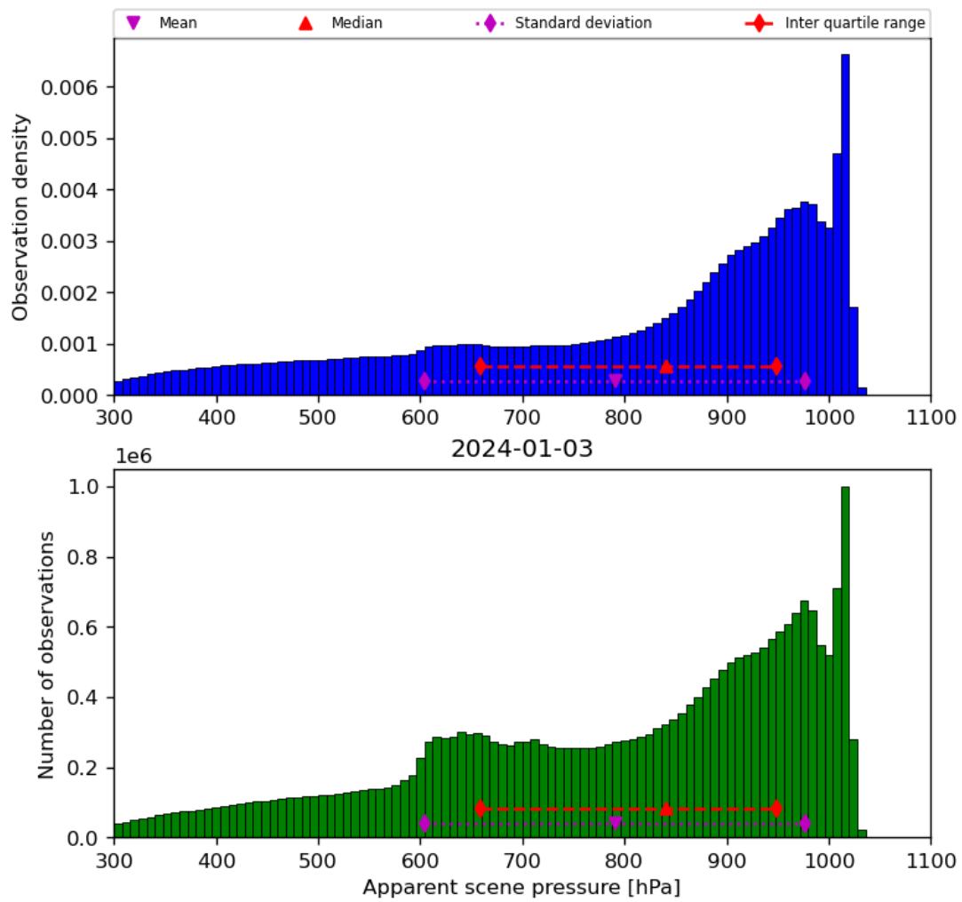
Figure 36: Histogram of “Apparent scene pressure” for 2024-01-02 to 2024-01-04
