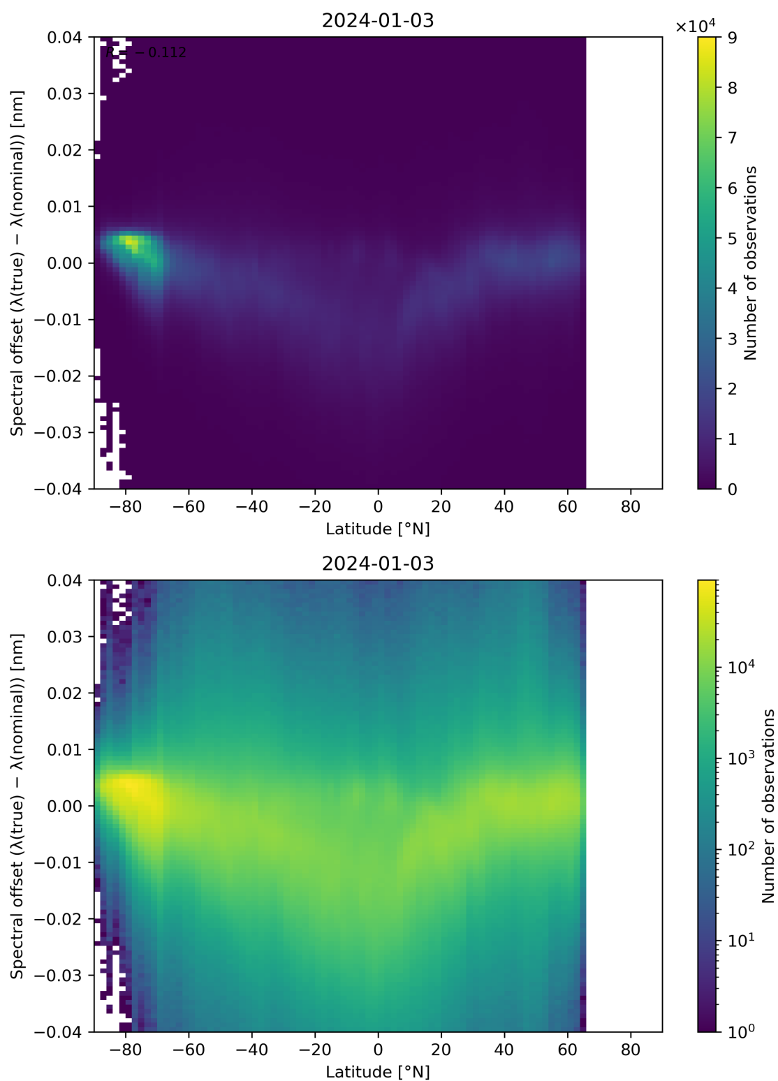
Figure 96: Scatter density plot of “Latitude” against “Spectral offset ( \lambda(\text{true}) - \lambda(\text{nominal}) )” for 2024-01-02 to 2024-01-04.
