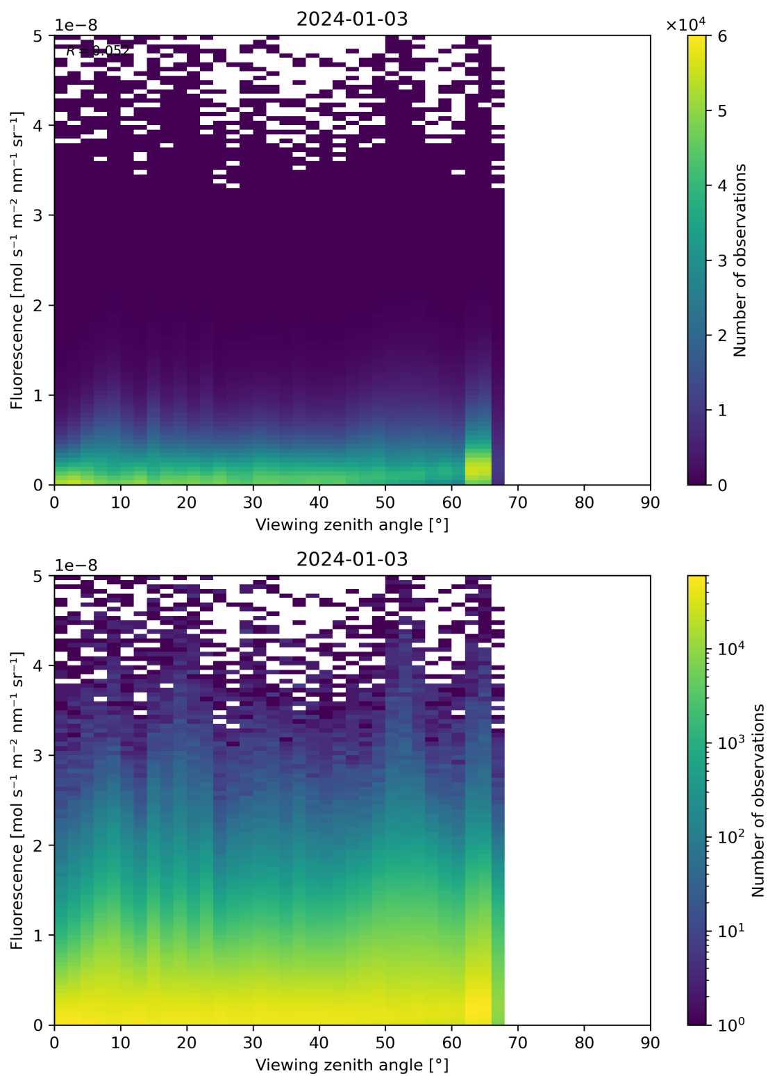
Figure 122: Scatter density plot of “Viewing zenith angle” against “Fluorescence” for 2024-01-02 to 2024-01-04.
