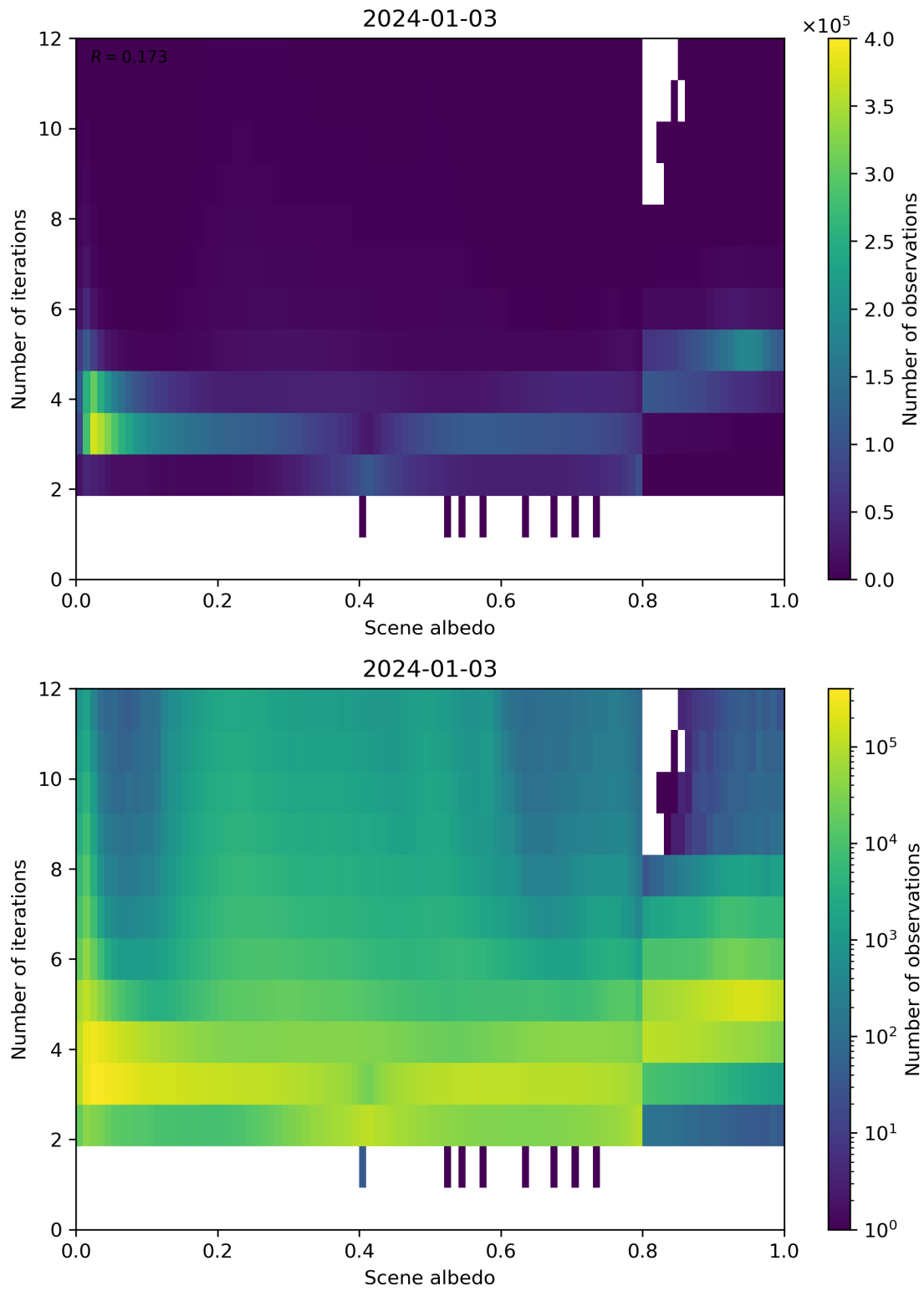
Figure 105: Scatter density plot of “Scene albedo” against “Number of iterations” for 2024-01-02 to 2024-01-04.
