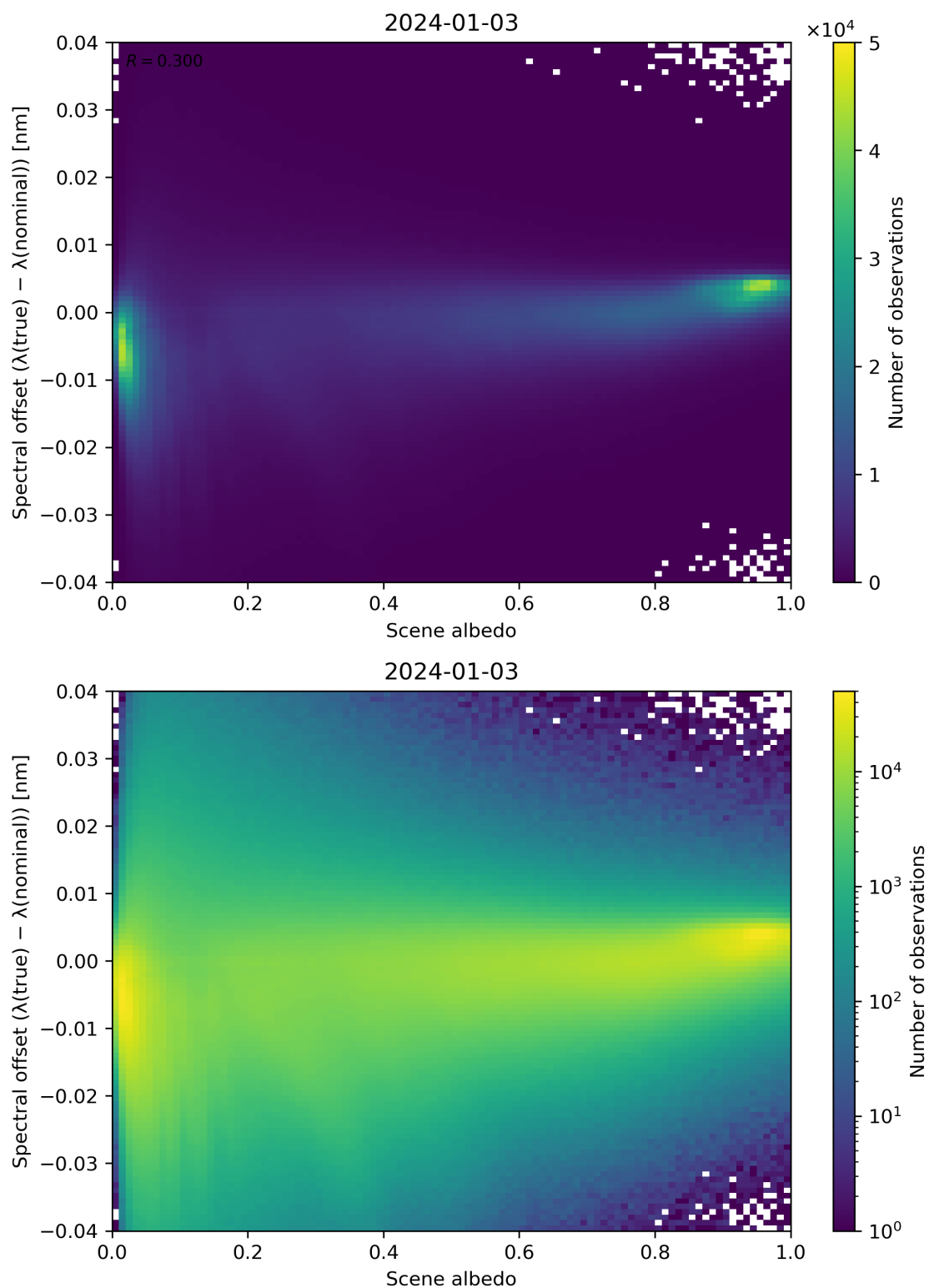
Figure 107: Scatter density plot of “Scene albedo” against “Spectral offset ( \lambda(\text{true}) - \lambda(\text{nominal}) )” for 2024-01-02 to 2024-01-04.
