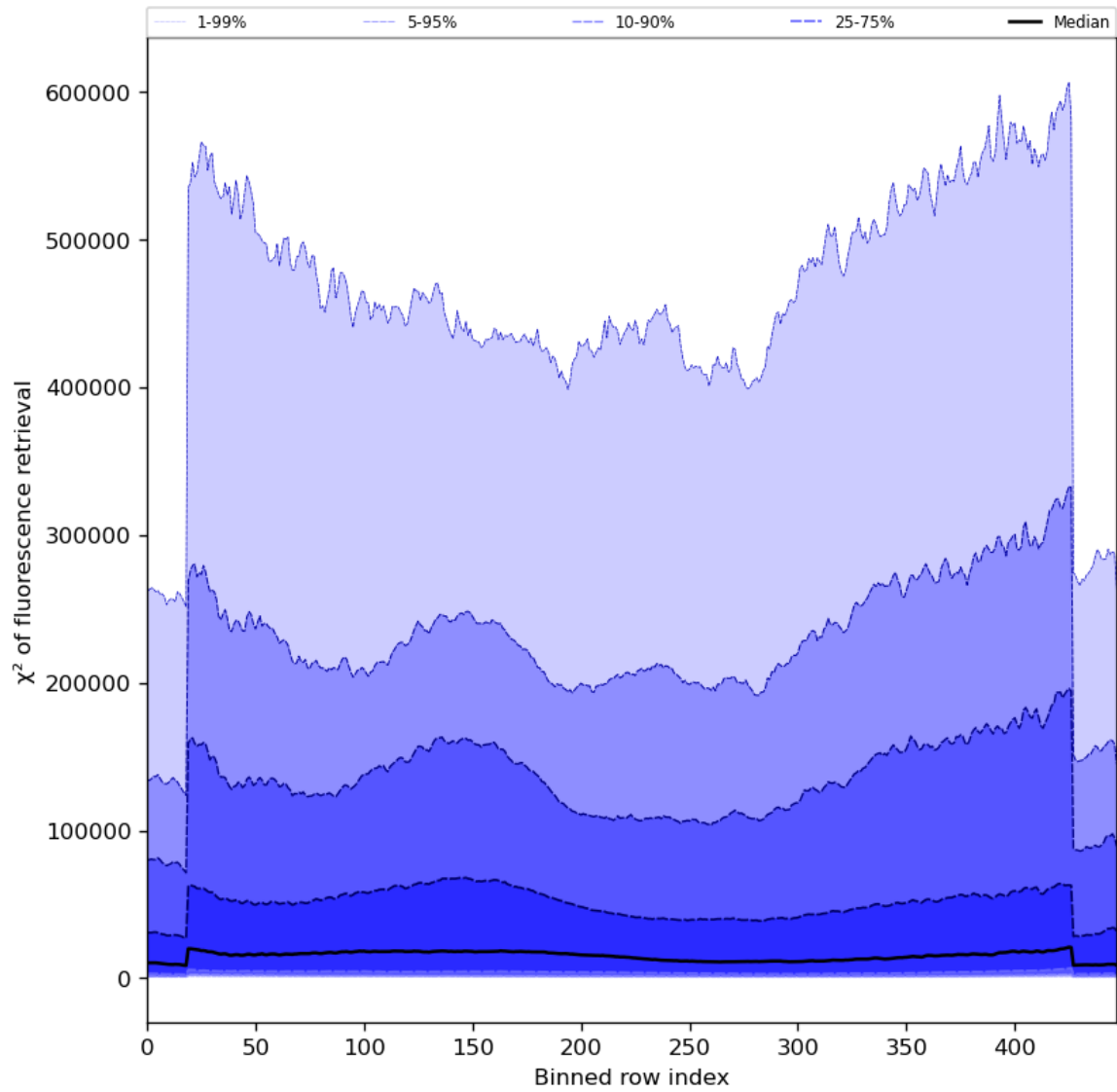
Figure 59: Along track statistics of “ \chi^2 of fluorescence retrieval” for 2024-01-02 to 2024-01-04
