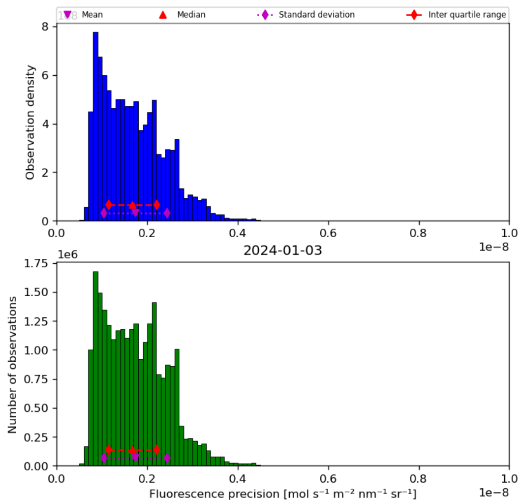
Figure 41: Histogram of “Fluorescence precision” for 2024-01-02 to 2024-01-04
