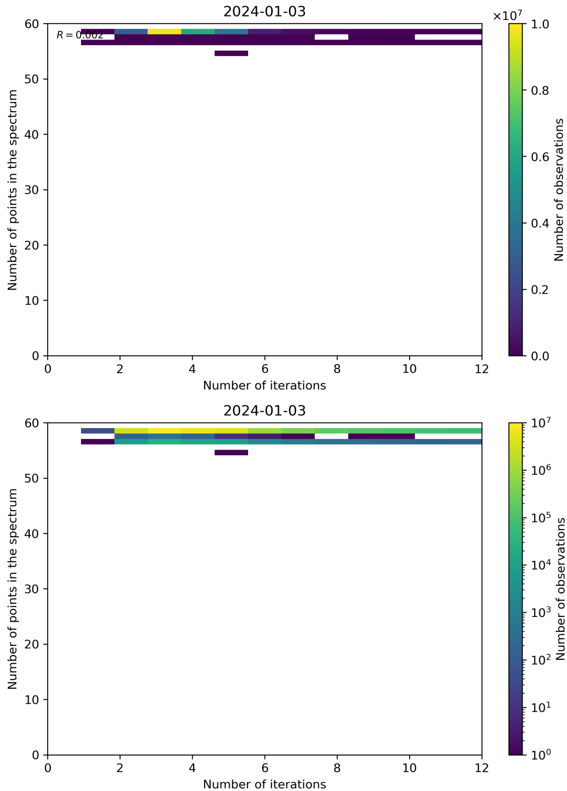
Figure 99: Scatter density plot of “Number of iterations” against “Number of points in the spectrum” for 2024-01-02 to 2024-01-04.
