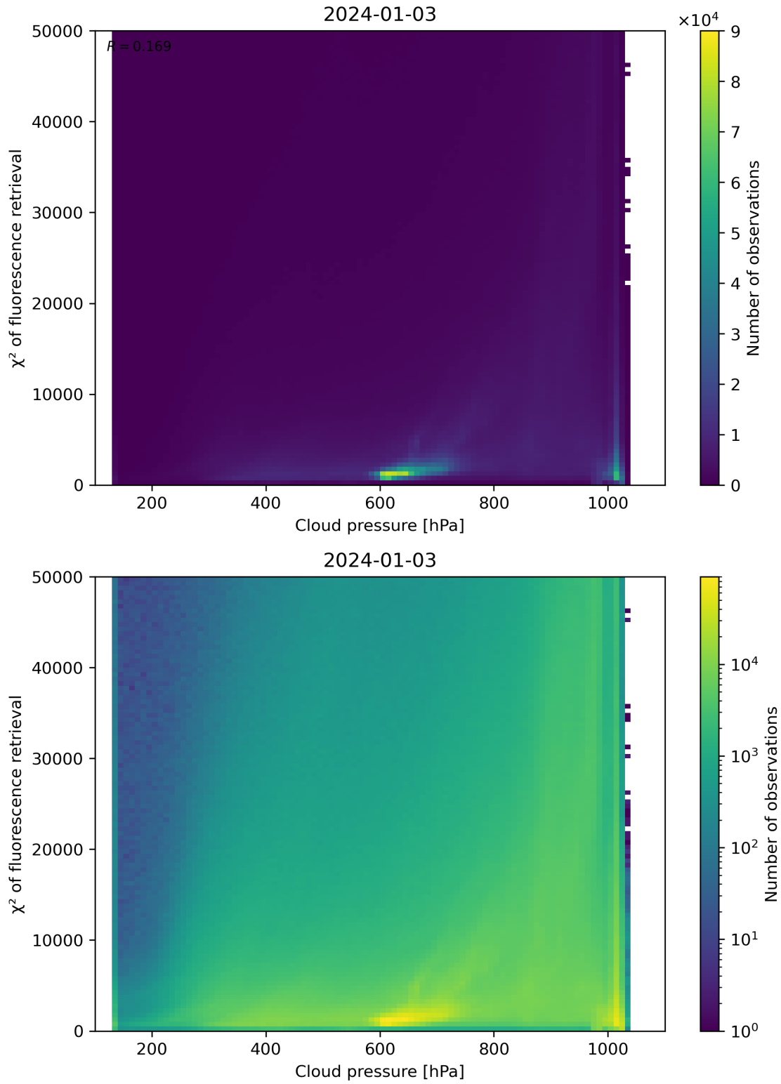
Figure 78: Scatter density plot of “Cloud pressure” against “ \chi^2 of fluorescence retrieval” for 2024-01-02 to 2024-01-04.
