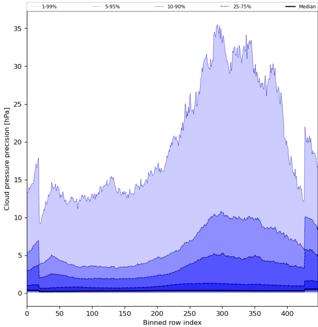
Figure 48: Along track statistics of “Cloud pressure precision” for 2024-01-02 to 2024-01-04
