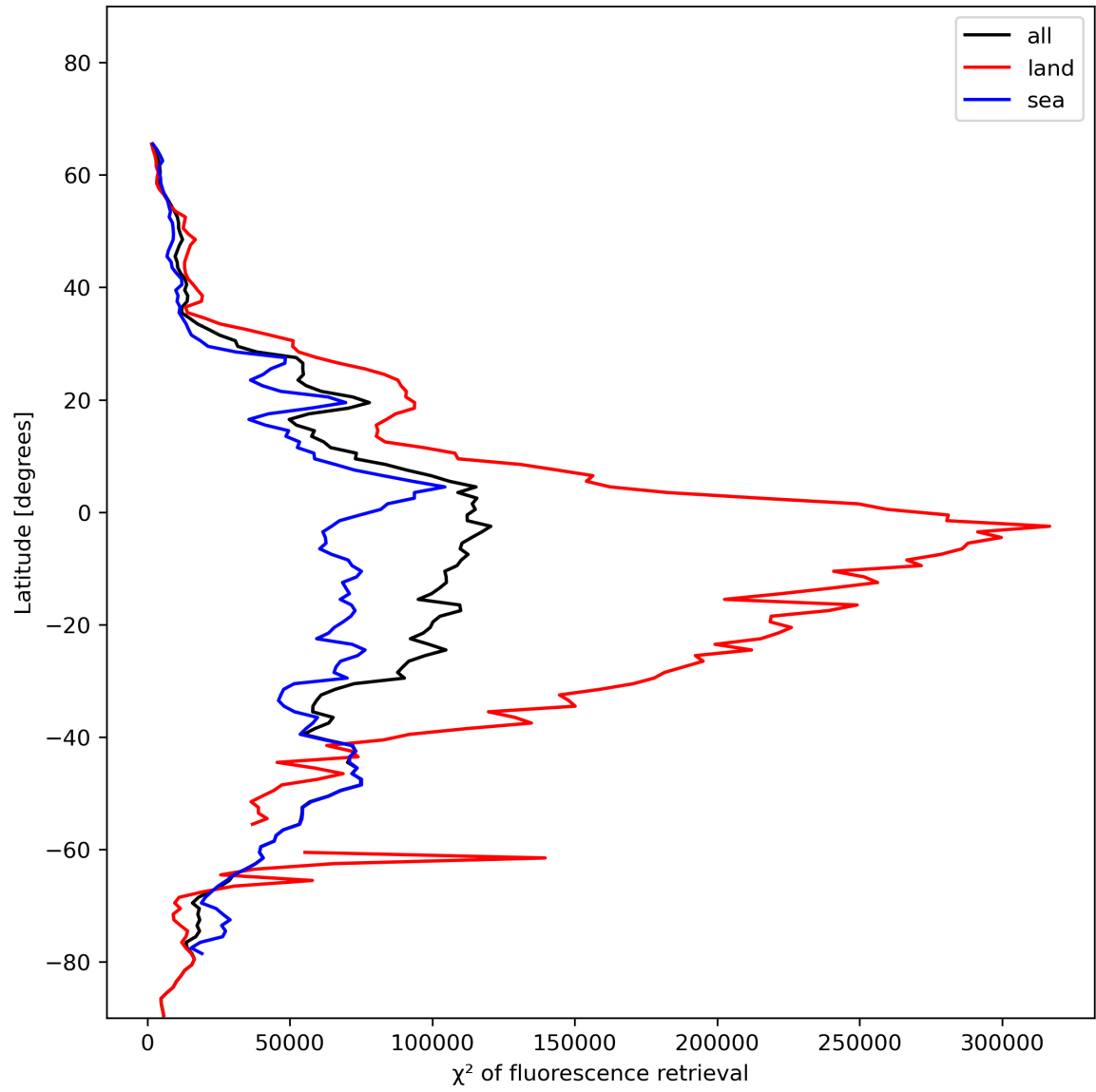
Figure 25: Zonal average of “ \chi^2 of fluorescence retrieval” for 2024-01-02 to 2024-01-04.
