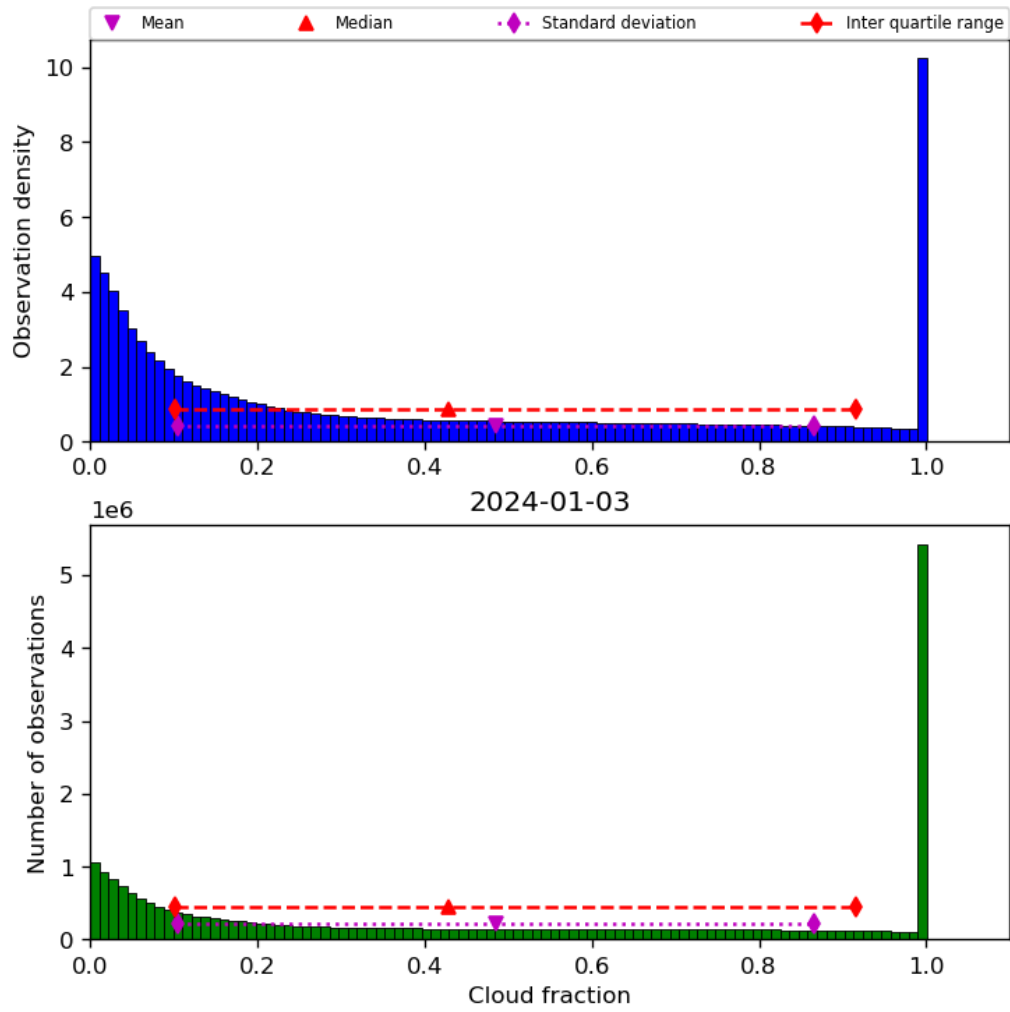
Figure 32: Histogram of “Cloud fraction” for 2024-01-02 to 2024-01-04
