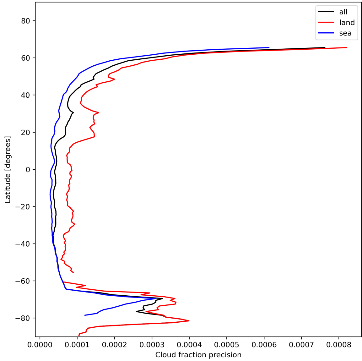
Figure 16: Zonal average of “Cloud fraction precision” for 2024-01-02 to 2024-01-04.
