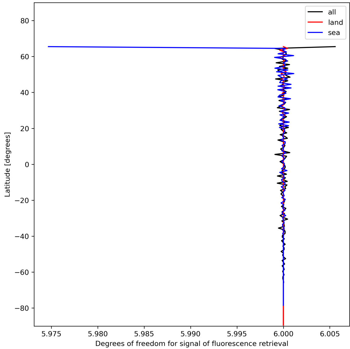
Figure 26: Zonal average of “Degrees of freedom for signal of fluorescence retrieval” for 2024-01-02 to 2024-01-04.
