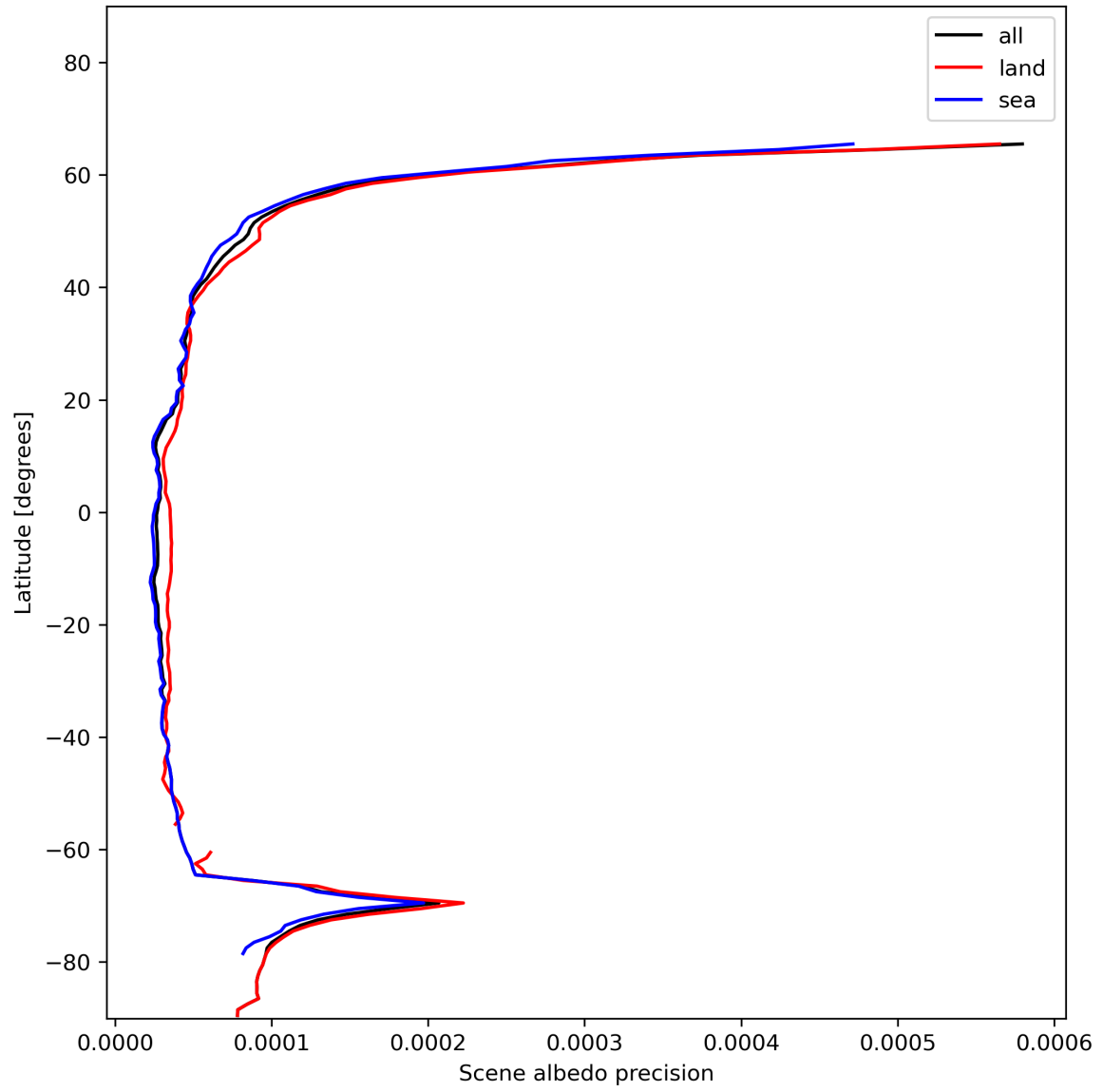
Figure 18: Zonal average of “Scene albedo precision” for 2024-01-02 to 2024-01-04.
