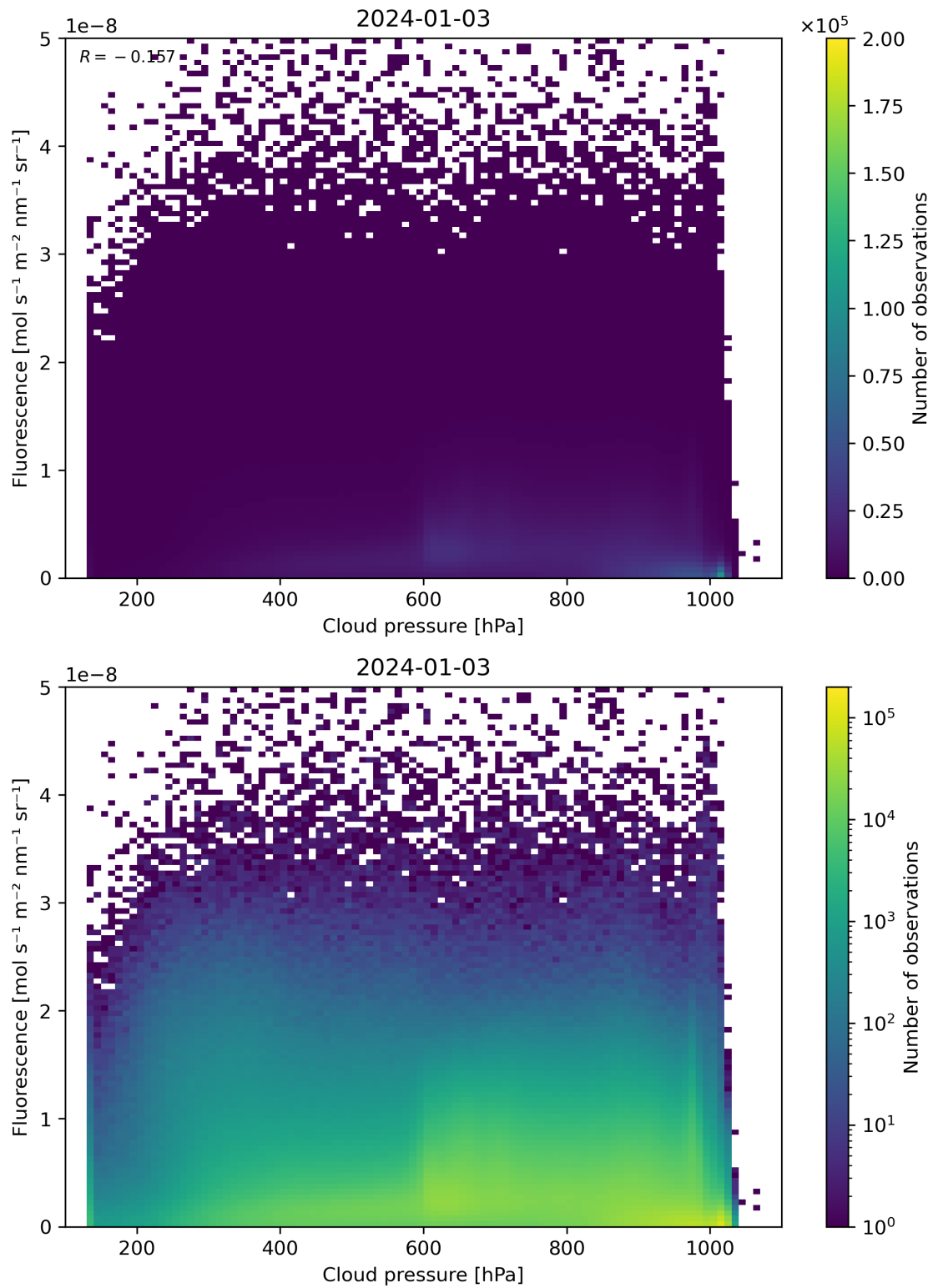
Figure 80: Scatter density plot of “Cloud pressure” against “Fluorescence” for 2024-01-02 to 2024-01-04.
