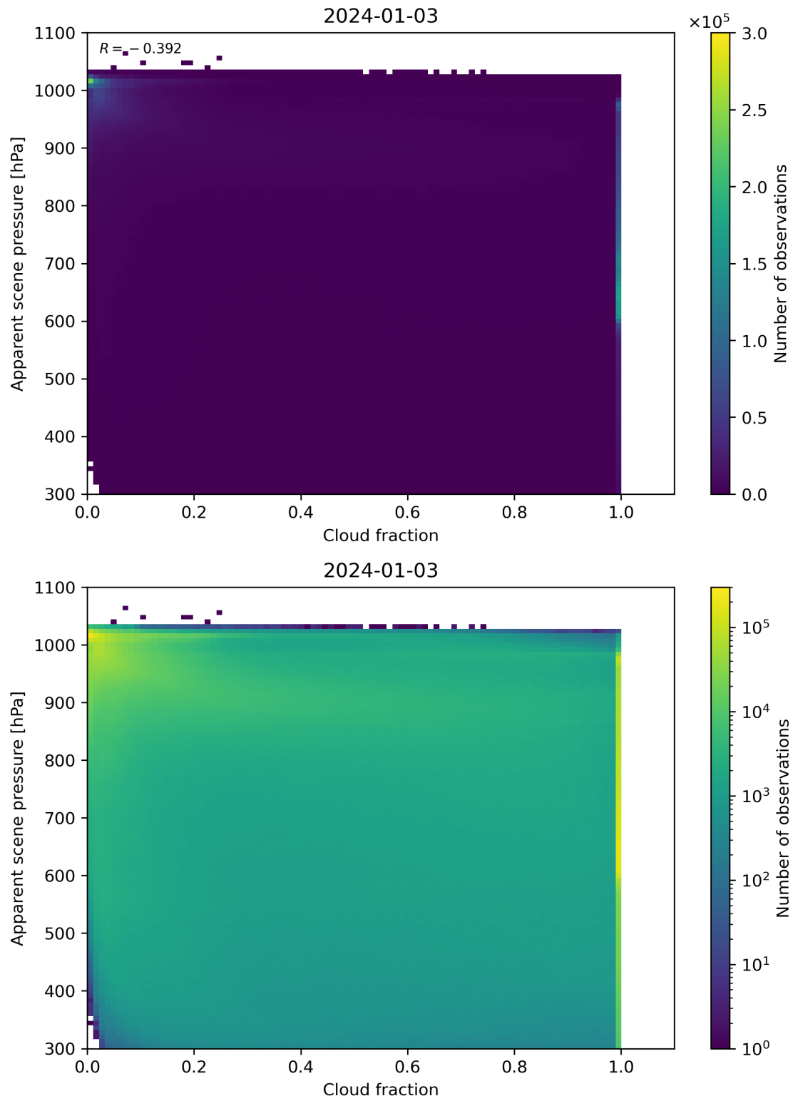
Figure 70: Scatter density plot of “Cloud fraction” against “Apparent scene pressure” for 2024-01-02 to 2024-01-04.
