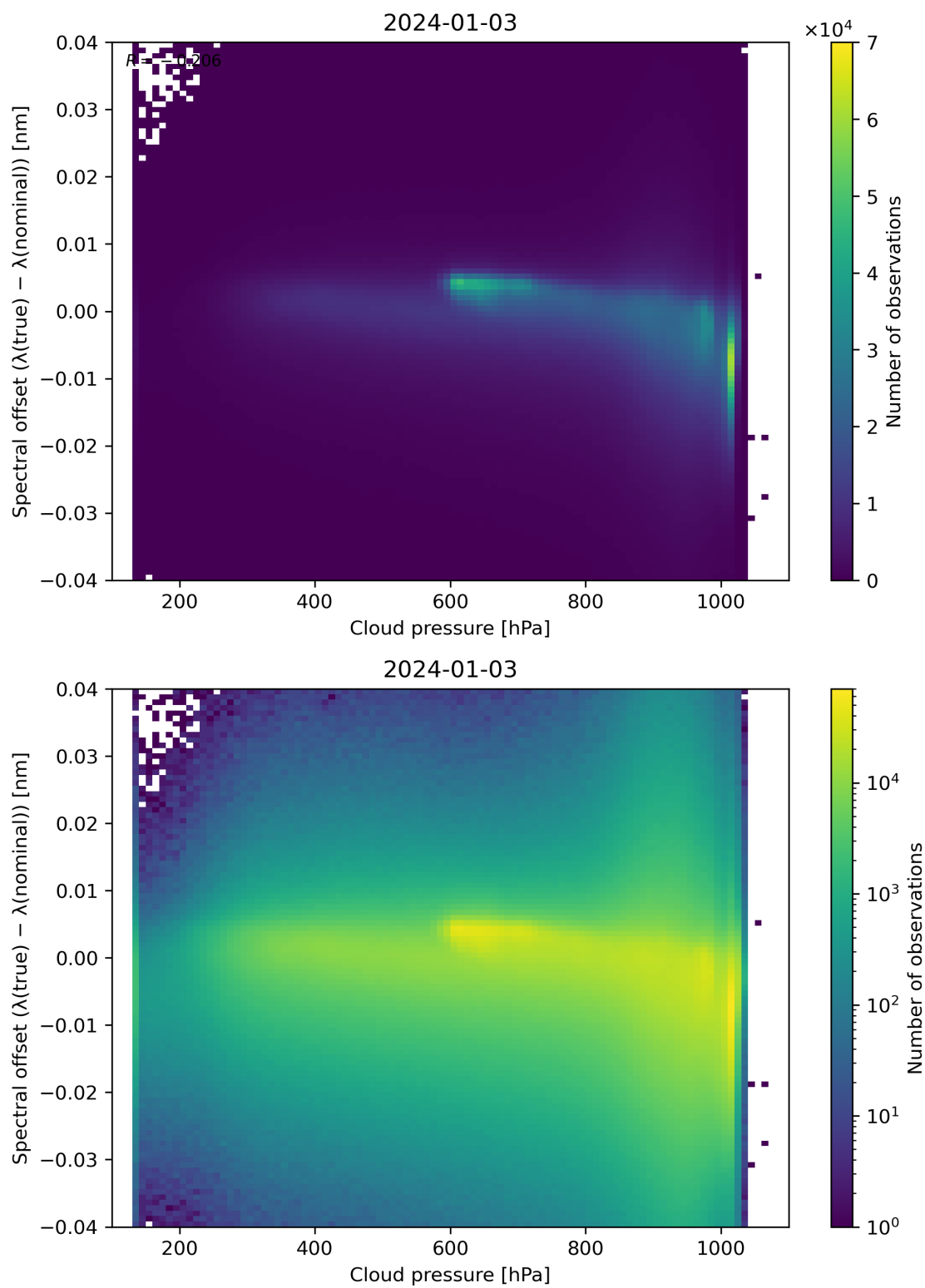
Figure 84: Scatter density plot of “Cloud pressure” against “Spectral offset ( \lambda(\text{true}) - \lambda(\text{nominal}) )” for 2024-01-02 to 2024-01-04.
