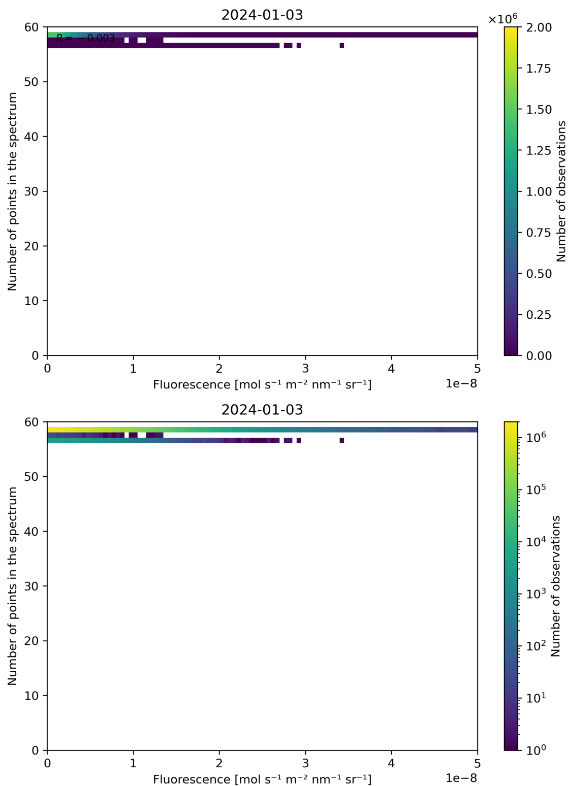
Figure 86: Scatter density plot of “Fluorescence” against “Number of points in the spectrum” for 2024-01-02 to 2024-01-04.
