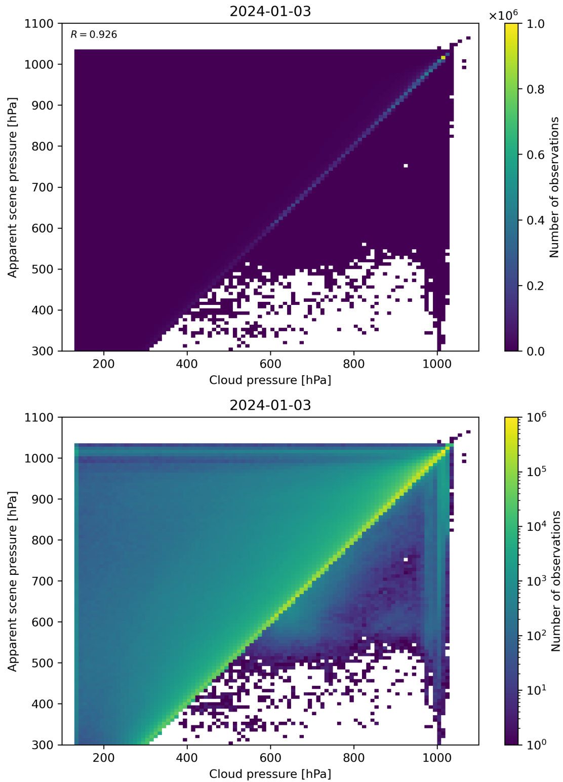
Figure 77: Scatter density plot of “Cloud pressure” against “Apparent scene pressure” for 2024-01-02 to 2024-01-04.
