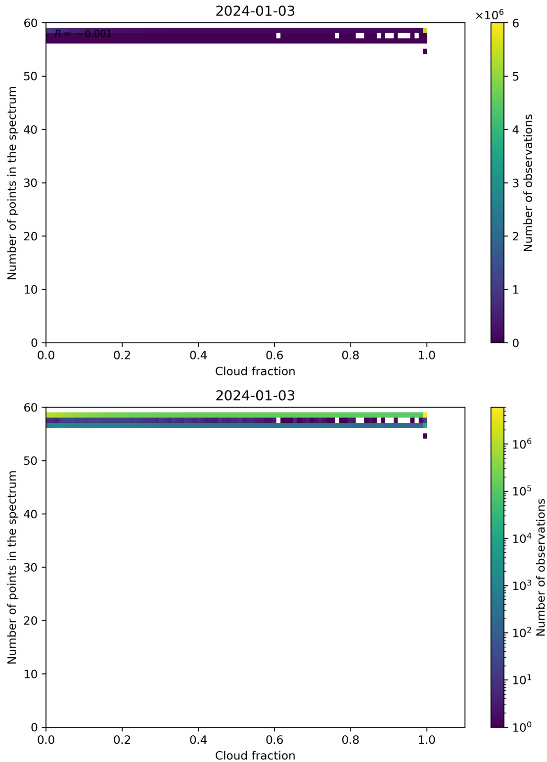
Figure 74: Scatter density plot of “Cloud fraction” against “Number of points in the spectrum” for 2024-01-02 to 2024-01-04.
