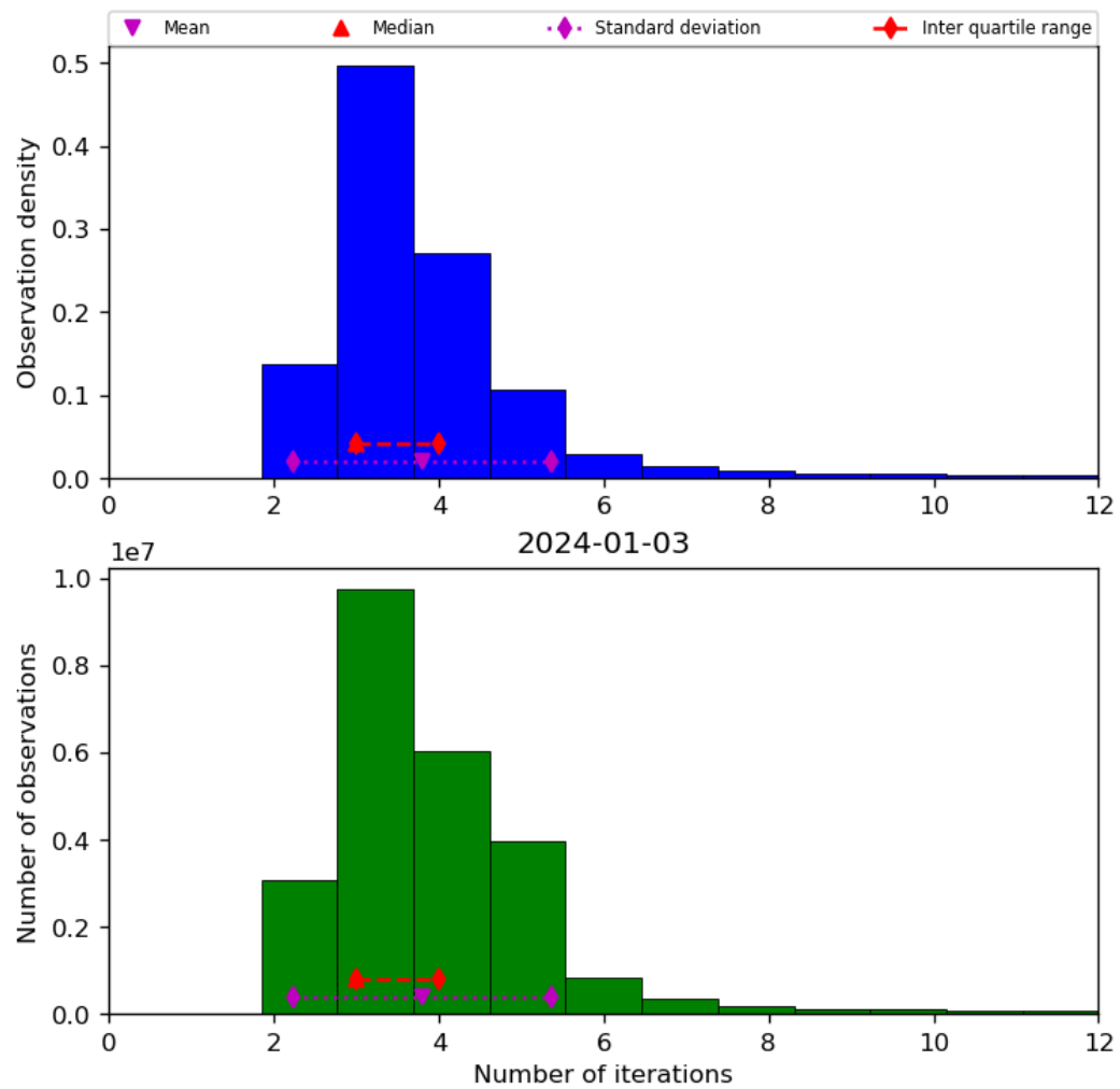
Figure 39: Histogram of “Number of iterations” for 2024-01-02 to 2024-01-04
