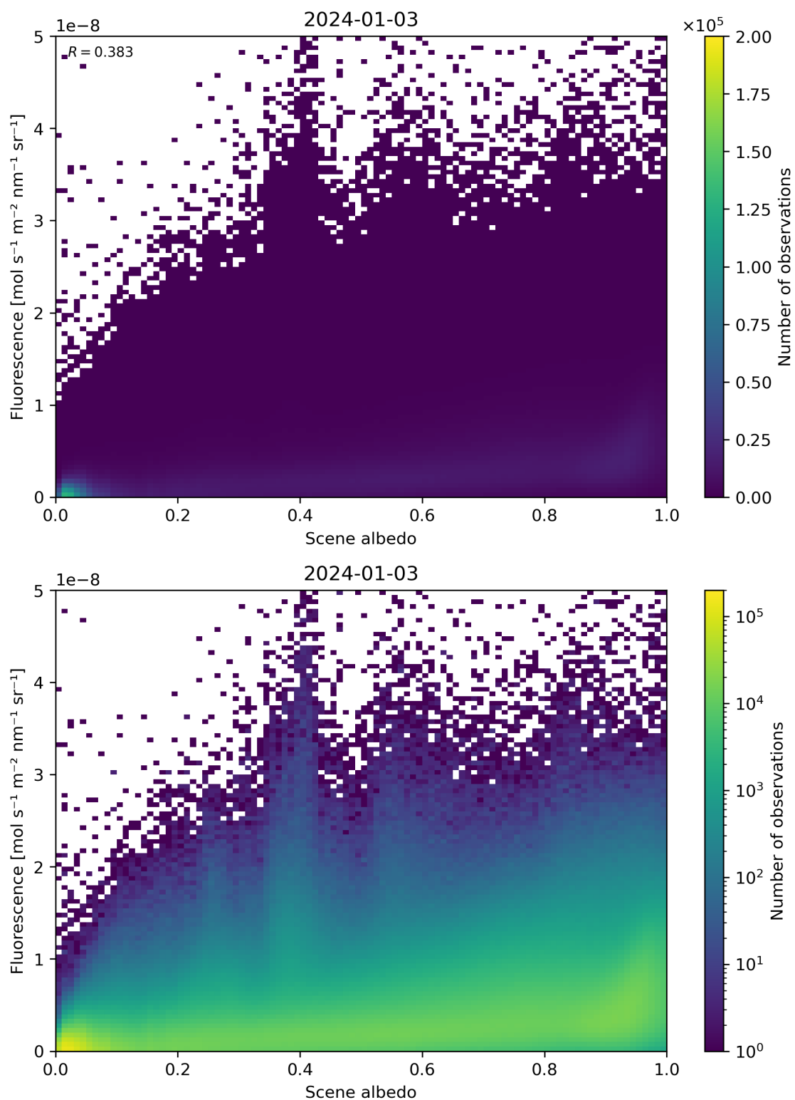
Figure 104: Scatter density plot of “Scene albedo” against “Fluorescence” for 2024-01-02 to 2024-01-04.
