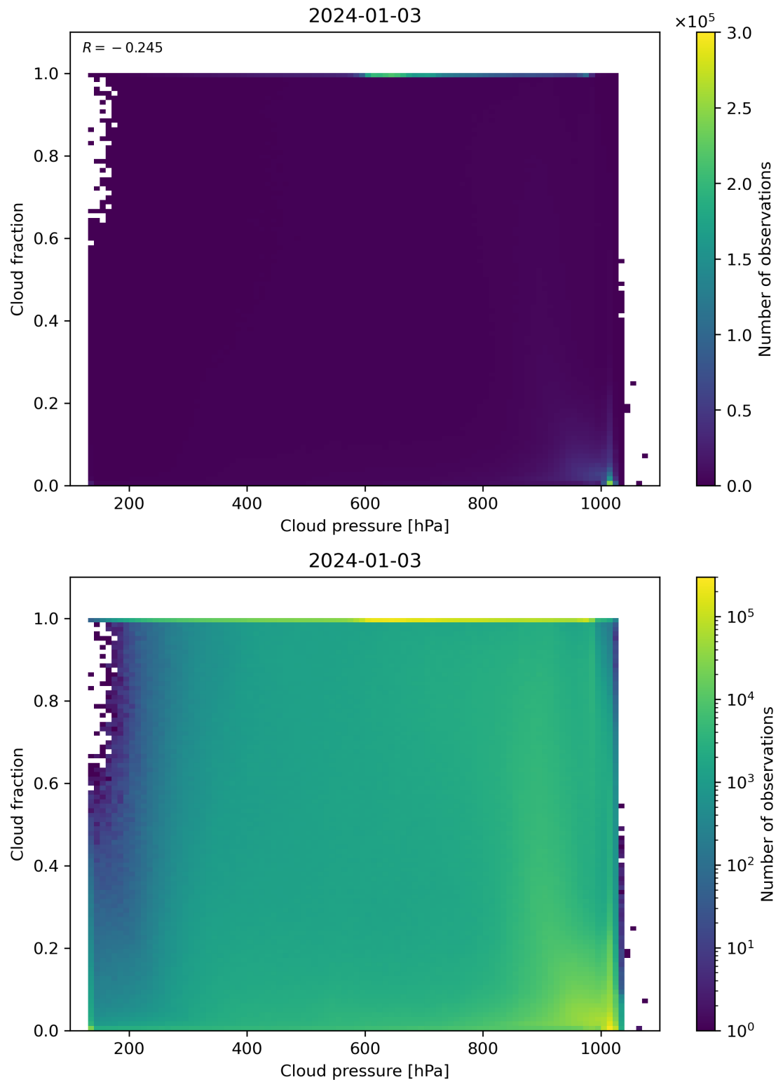
Figure 79: Scatter density plot of “Cloud pressure” against “Cloud fraction” for 2024-01-02 to 2024-01-04.
