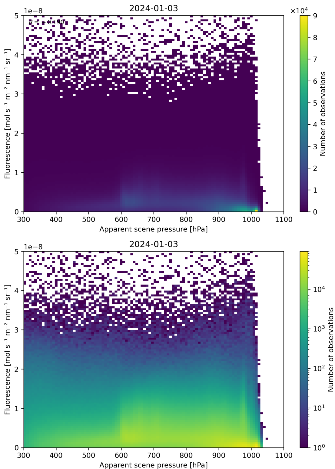
Figure 64: Scatter density plot of “Apparent scene pressure” against “Fluorescence” for 2024-01-02 to 2024-01-04.
