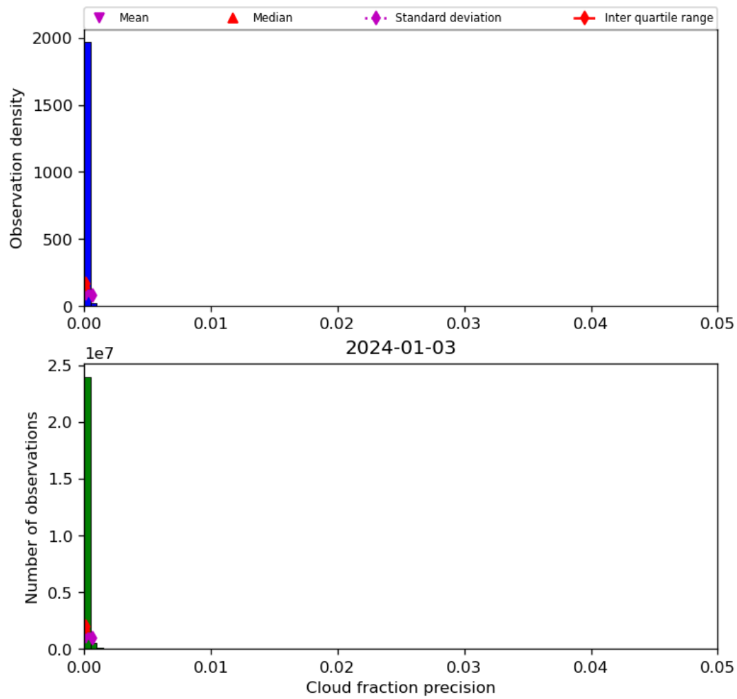
Figure 33: Histogram of “Cloud fraction precision” for 2024-01-02 to 2024-01-04
