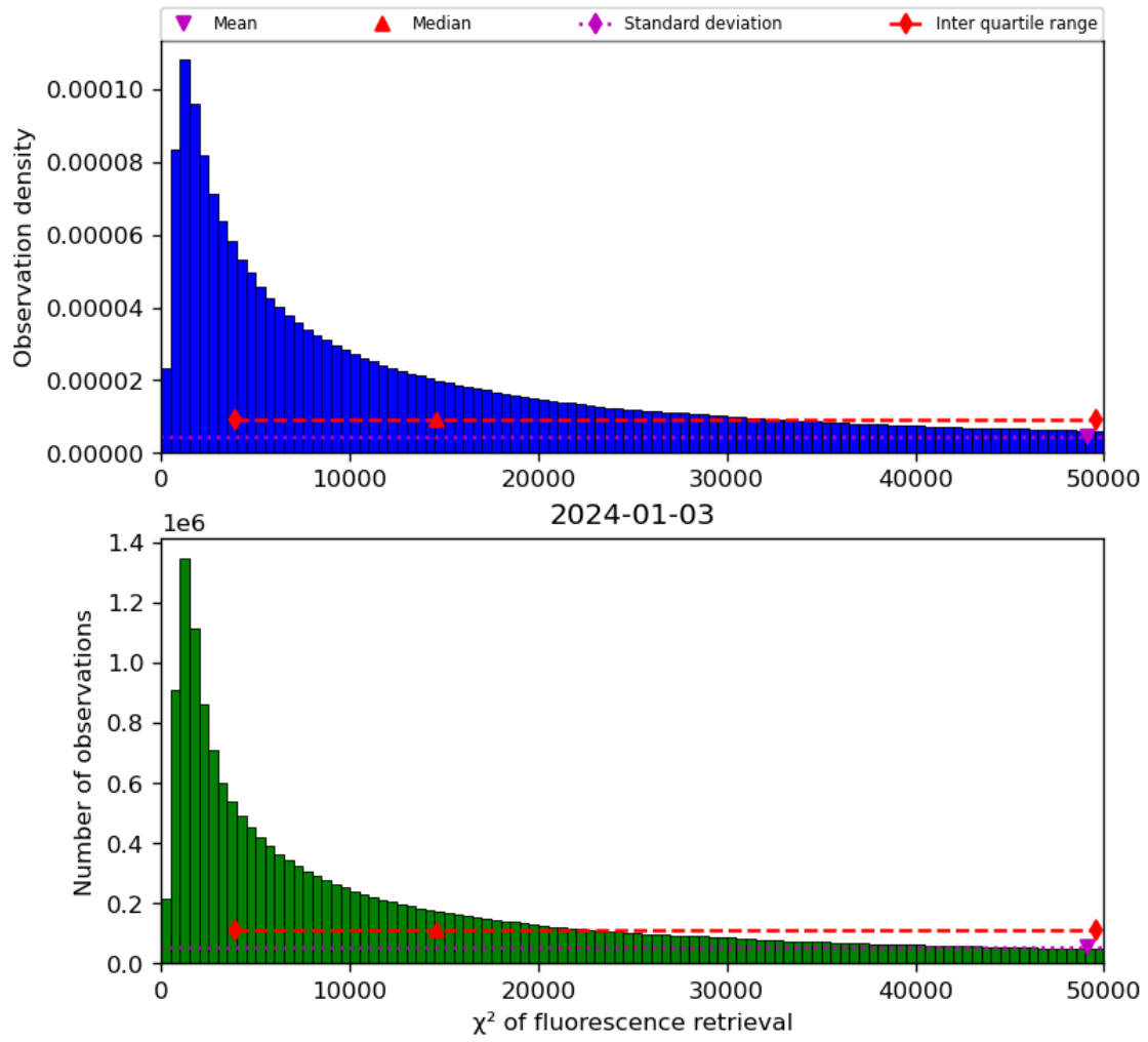
Figure 42: Histogram of “ \chi^2 of fluorescence retrieval” for 2024-01-02 to 2024-01-04
