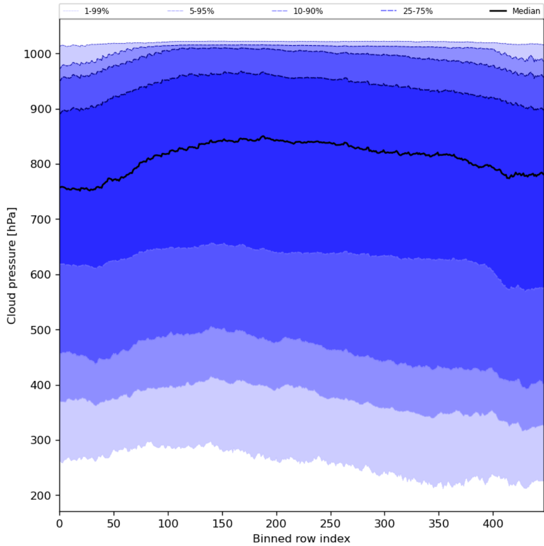
Figure 47: Along track statistics of “Cloud pressure” for 2024-01-02 to 2024-01-04
