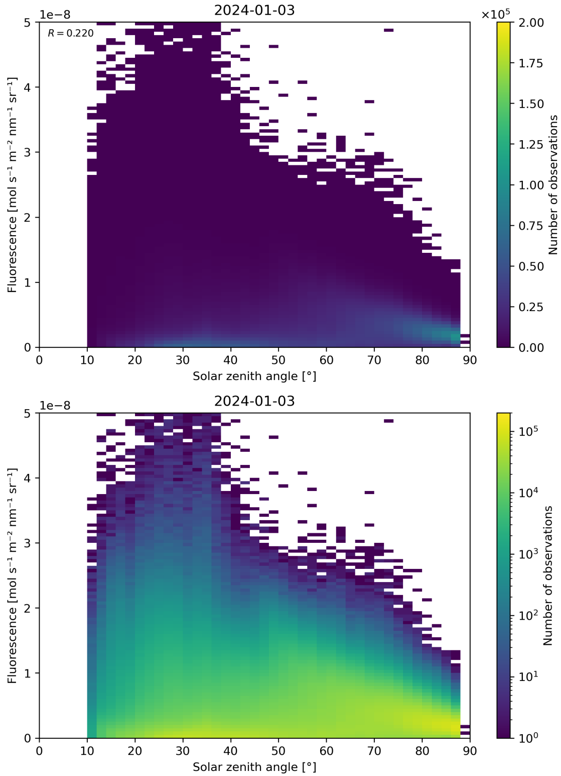
Figure 112: Scatter density plot of “Solar zenith angle” against “Fluorescence” for 2024-01-02 to 2024-01-04.
