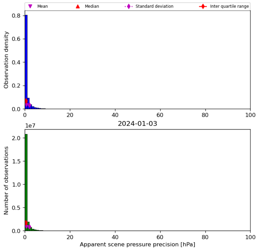
Figure 37: Histogram of “Apparent scene pressure precision” for 2024-01-02 to 2024-01-04
