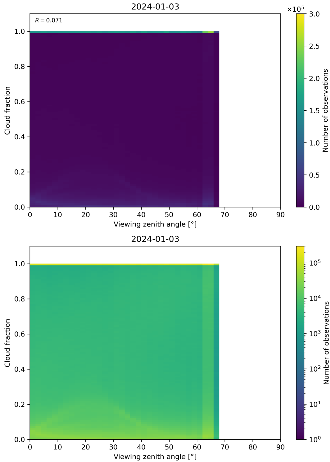
Figure 120: Scatter density plot of “Viewing zenith angle” against “Cloud fraction” for 2024-01-02 to 2024-01-04.
