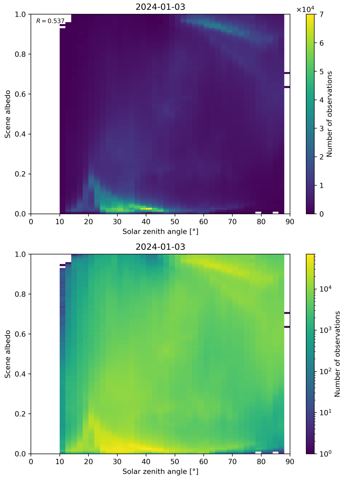
Figure 116: Scatter density plot of “Solar zenith angle” against “Scene albedo” for 2024-01-02 to 2024-01-04.
