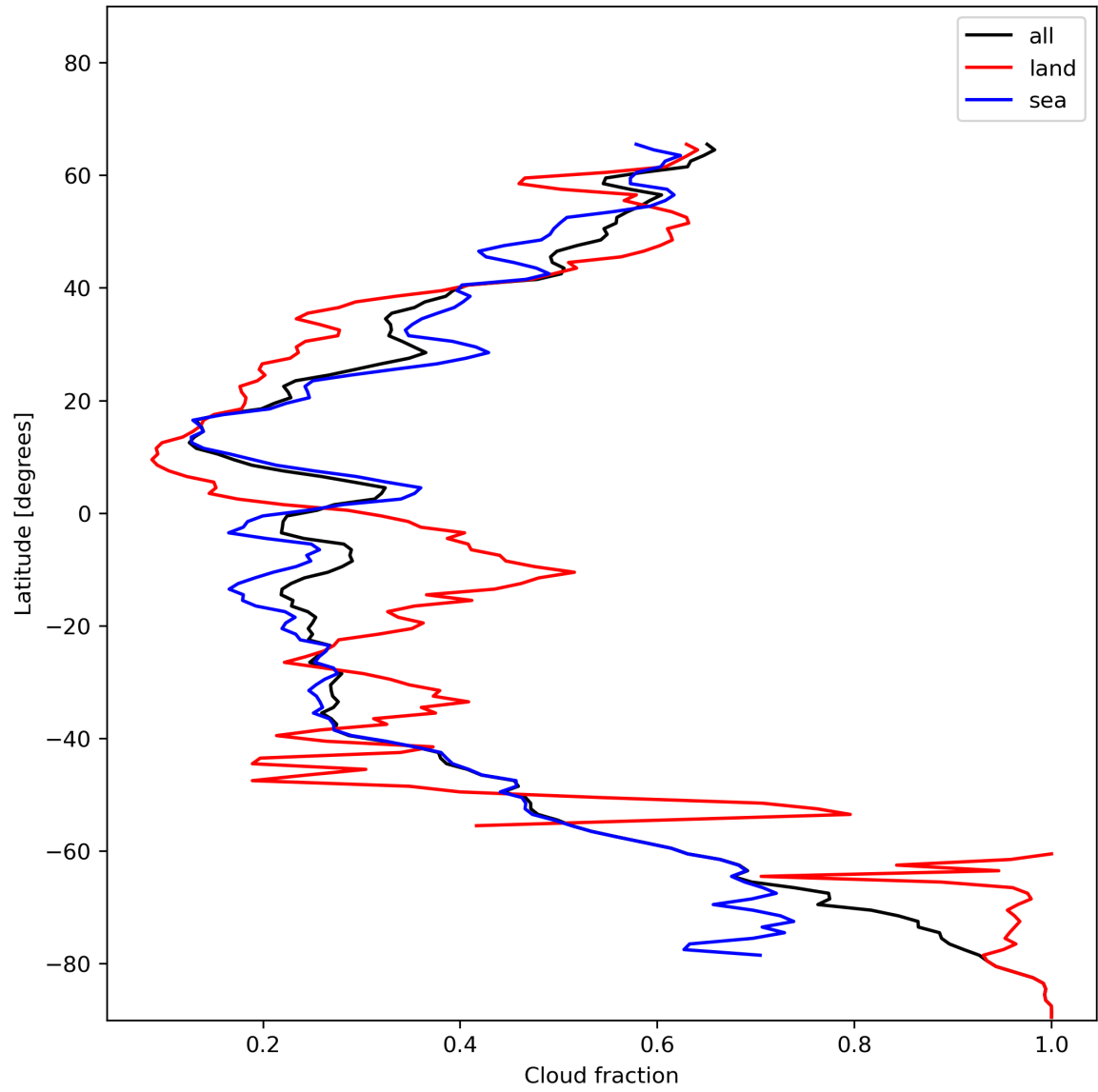
Figure 15: Zonal average of “Cloud fraction” for 2024-01-02 to 2024-01-04.
