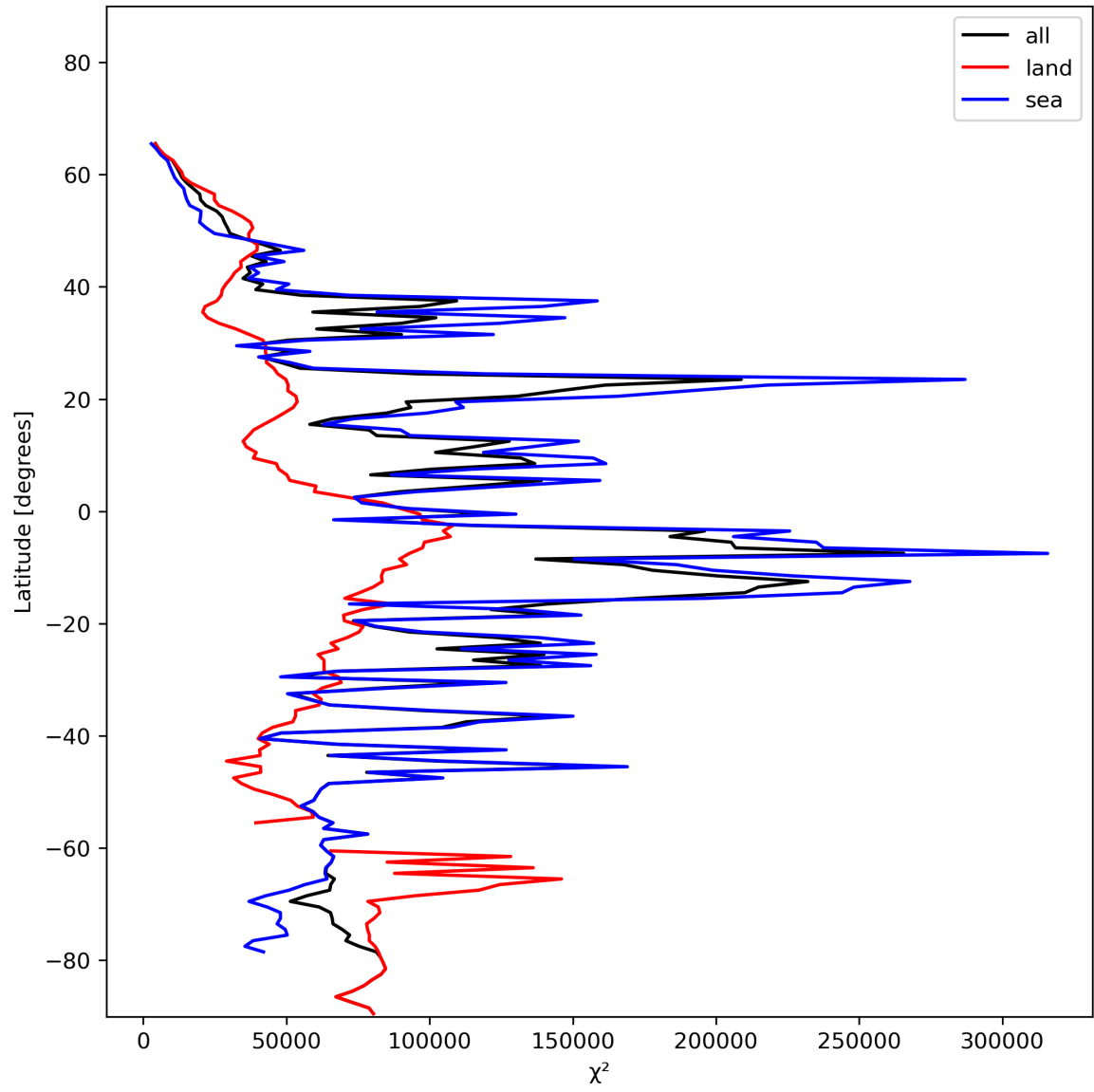
Figure 21: Zonal average of “ \chi^2 ” for 2024-01-02 to 2024-01-04.
