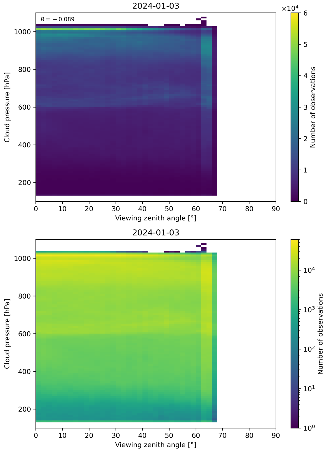
Figure 121: Scatter density plot of “Viewing zenith angle” against “Cloud pressure” for 2024-01-02 to 2024-01-04.
