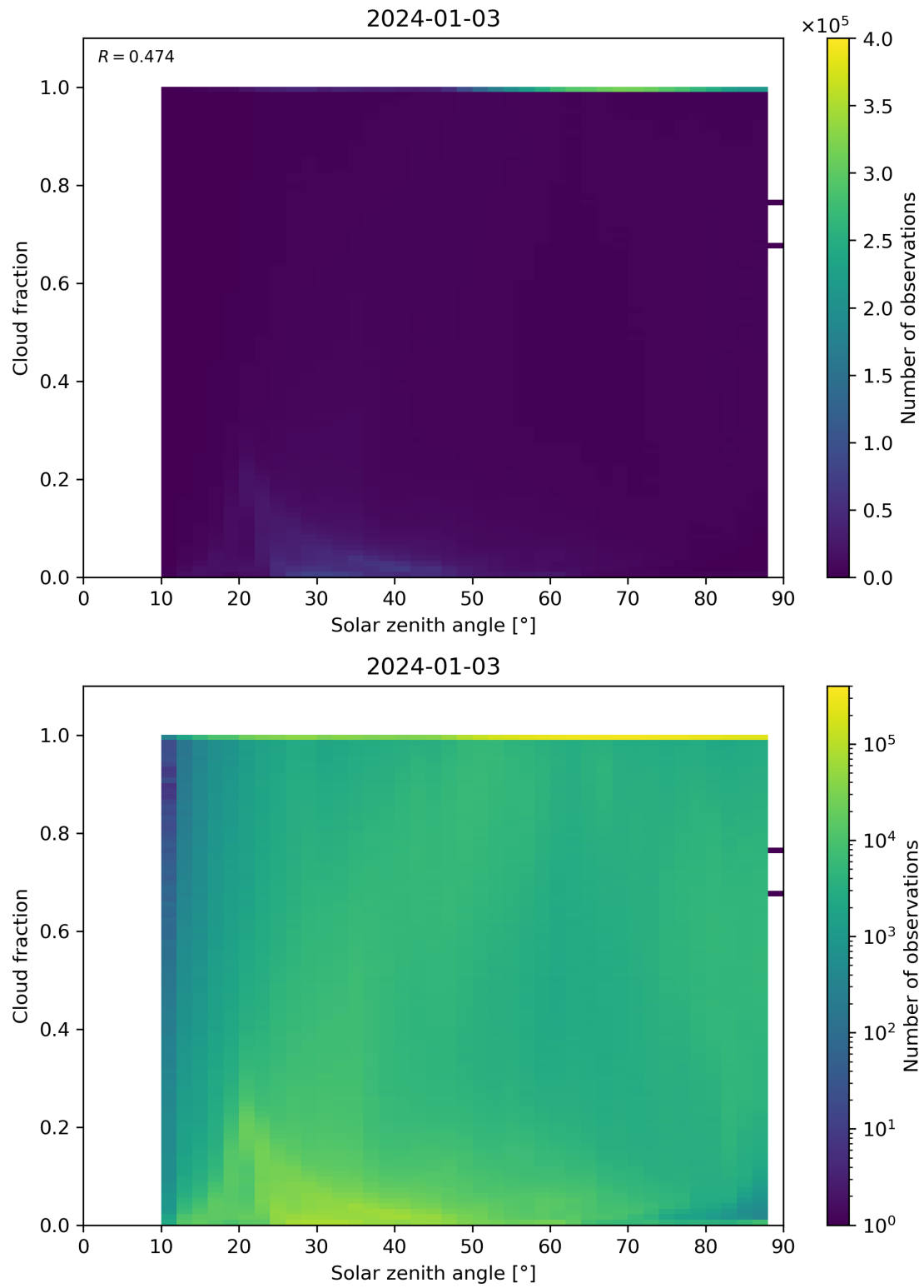
Figure 110: Scatter density plot of “Solar zenith angle” against “Cloud fraction” for 2024-01-02 to 2024-01-04.
