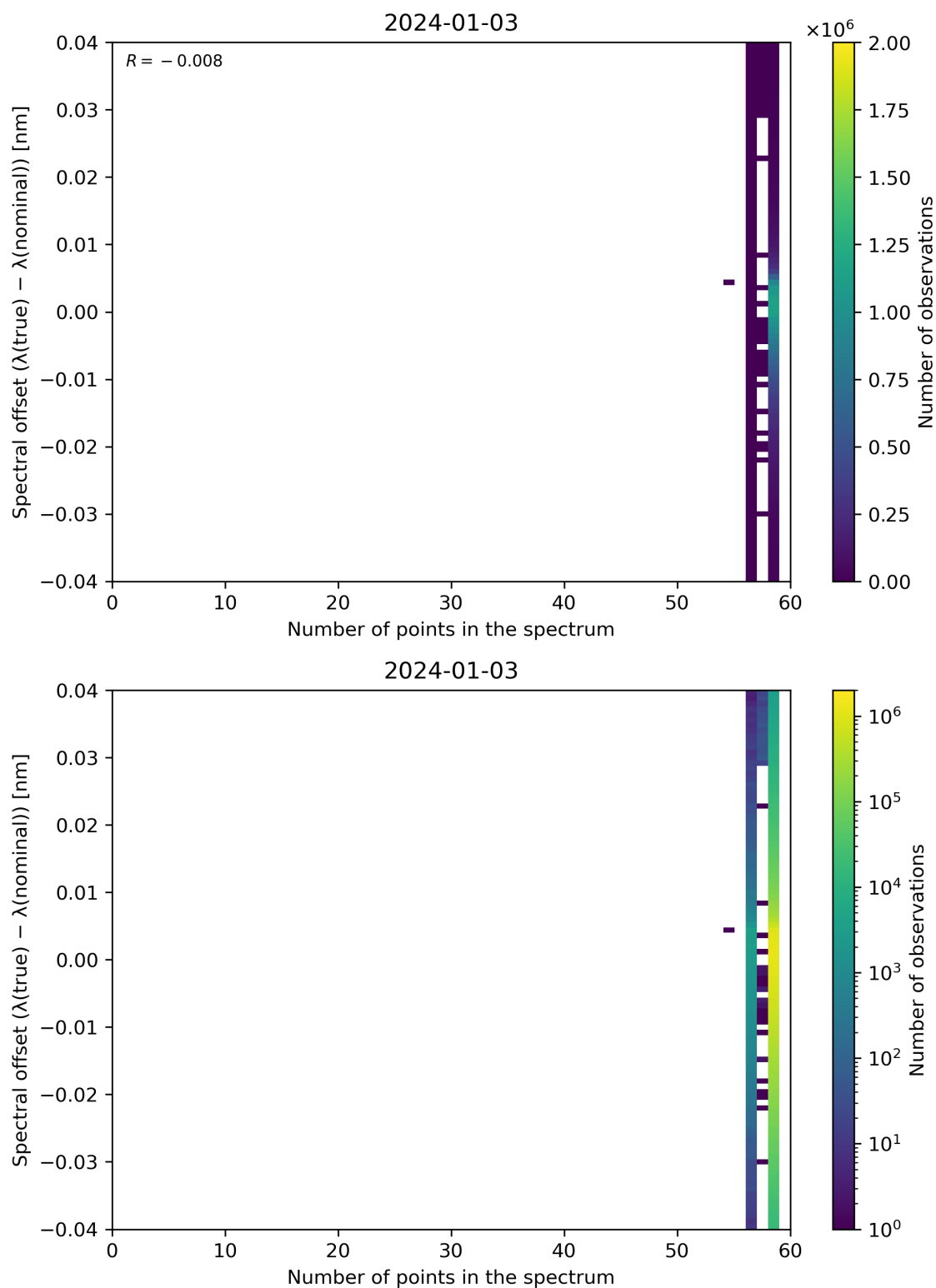
Figure 101: Scatter density plot of “Number of points in the spectrum” against “Spectral offset ( \lambda(\text{true}) - \lambda(\text{nominal}) )” for 2024-01-02 to 2024-01-04.
