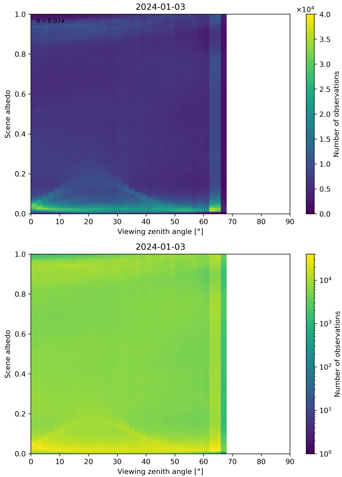
Figure 126: Scatter density plot of “Viewing zenith angle” against “Scene albedo” for 2024-01-02 to 2024-01-04.
