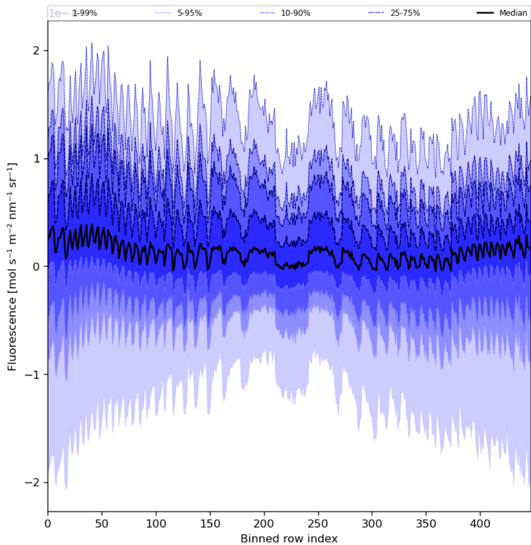
Figure 57: Along track statistics of “Fluorescence” for 2024-01-02 to 2024-01-04
