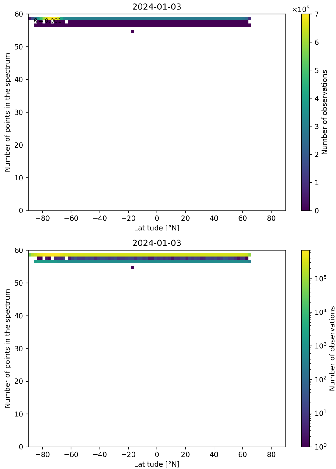
Figure 94: Scatter density plot of “Latitude” against “Number of points in the spectrum” for 2024-01-02 to 2024-01-04.
