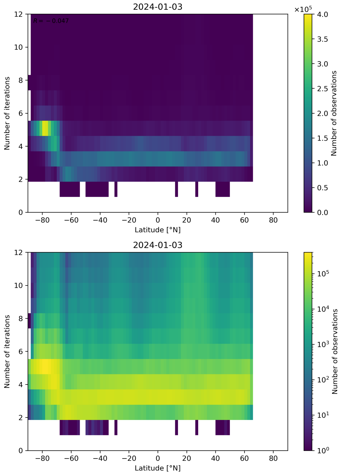
Figure 93: Scatter density plot of “Latitude” against “Number of iterations” for 2024-01-02 to 2024-01-04.
