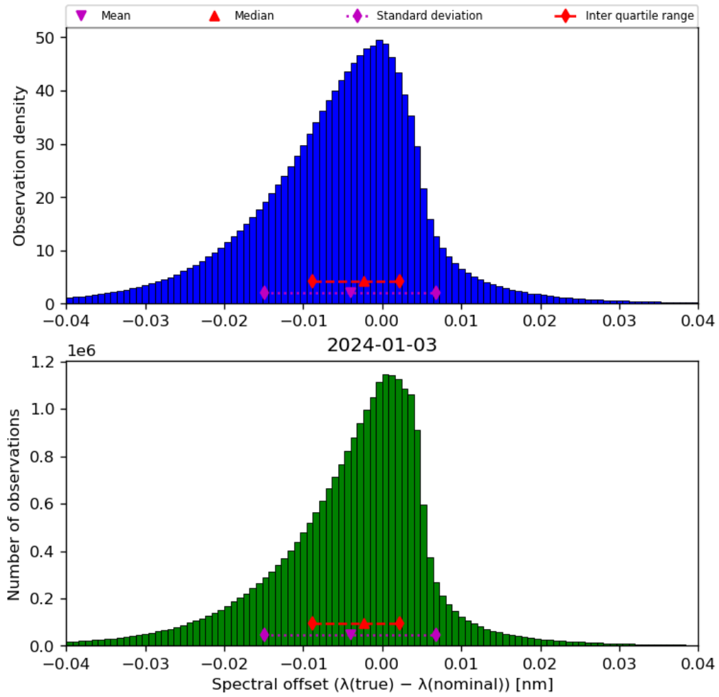
Figure 45: Histogram of “Spectral offset ( \lambda(\text{true}) - \lambda(\text{nominal}) )” for 2024-01-02 to 2024-01-04
