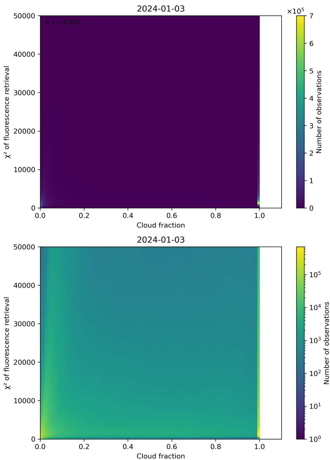
Figure 71: Scatter density plot of “Cloud fraction” against “ \chi^2 of fluorescence retrieval” for 2024-01-02 to 2024-01-04.
