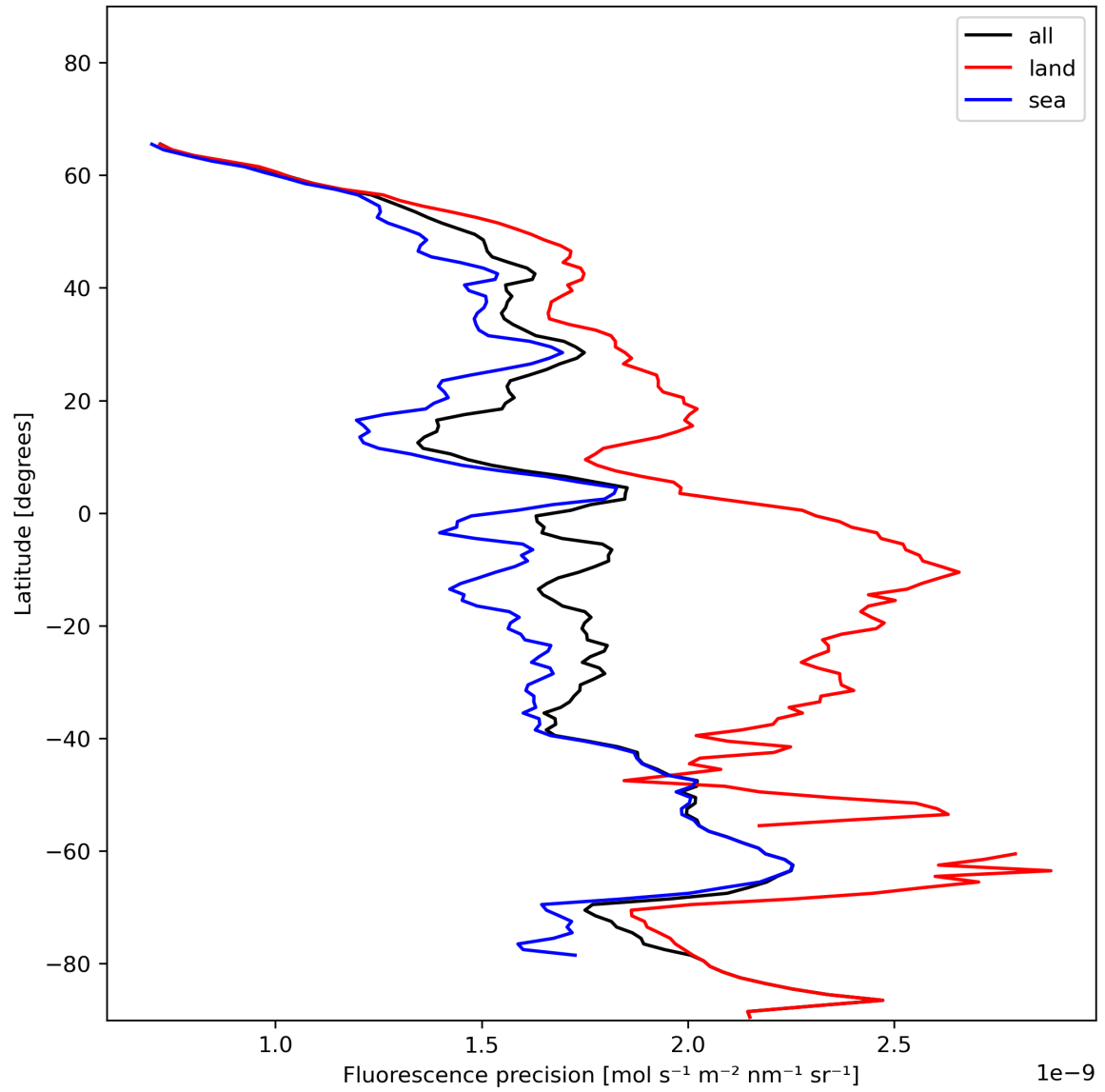
Figure 24: Zonal average of “Fluorescence precision” for 2024-01-02 to 2024-01-04.
