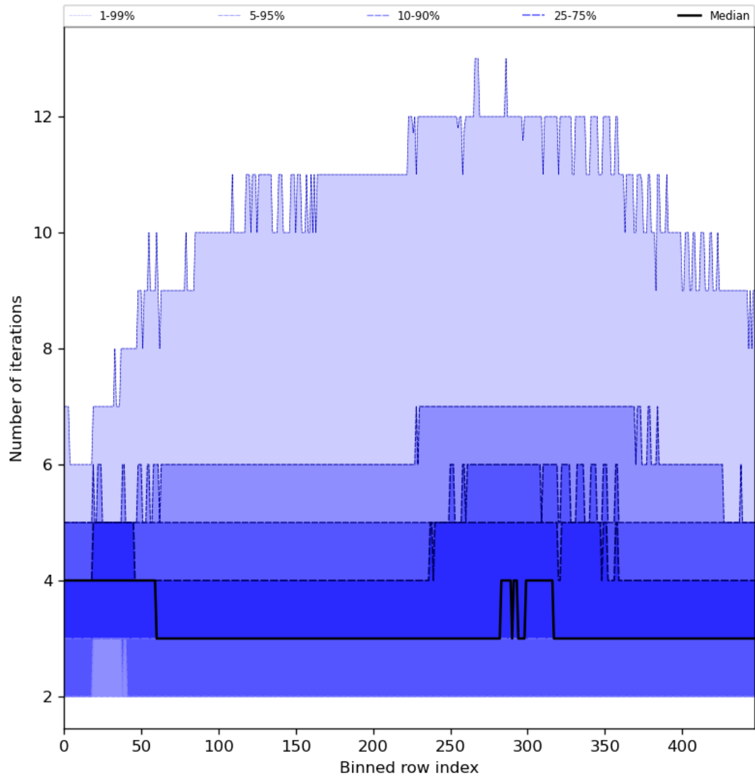
Figure 56: Along track statistics of “Number of iterations” for 2024-01-02 to 2024-01-04
