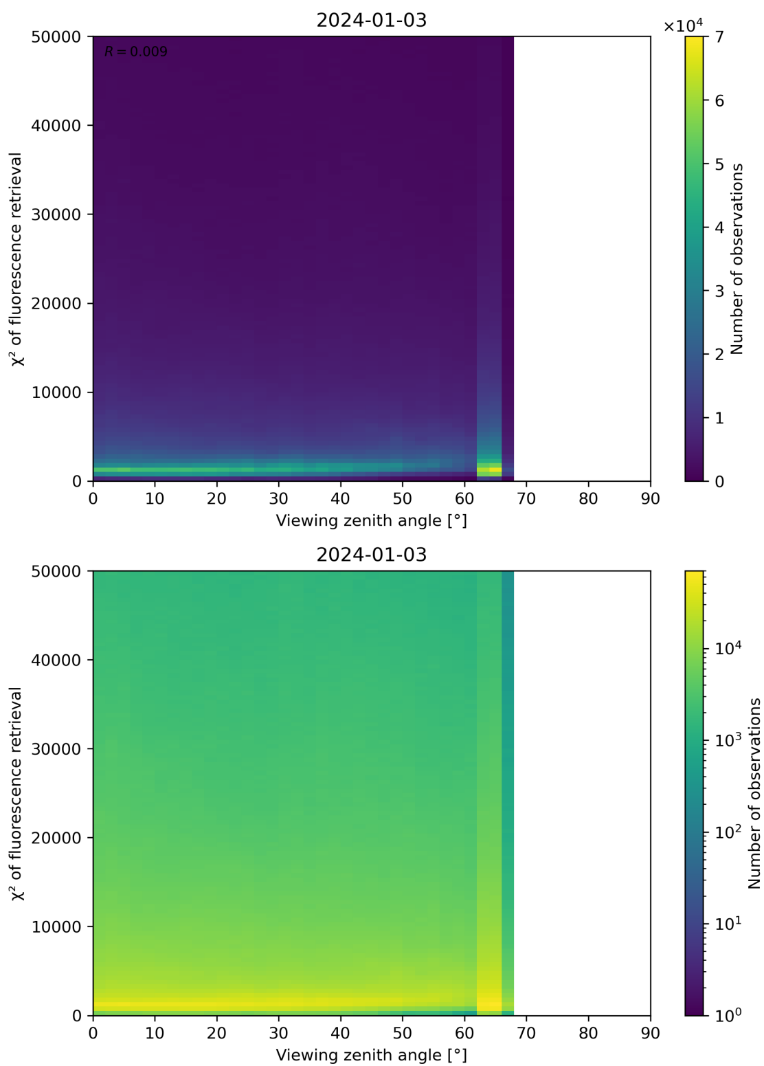
Figure 119: Scatter density plot of “Viewing zenith angle” against “ \chi^2 of fluorescence retrieval” for 2024-01-02 to 2024-01-04.
