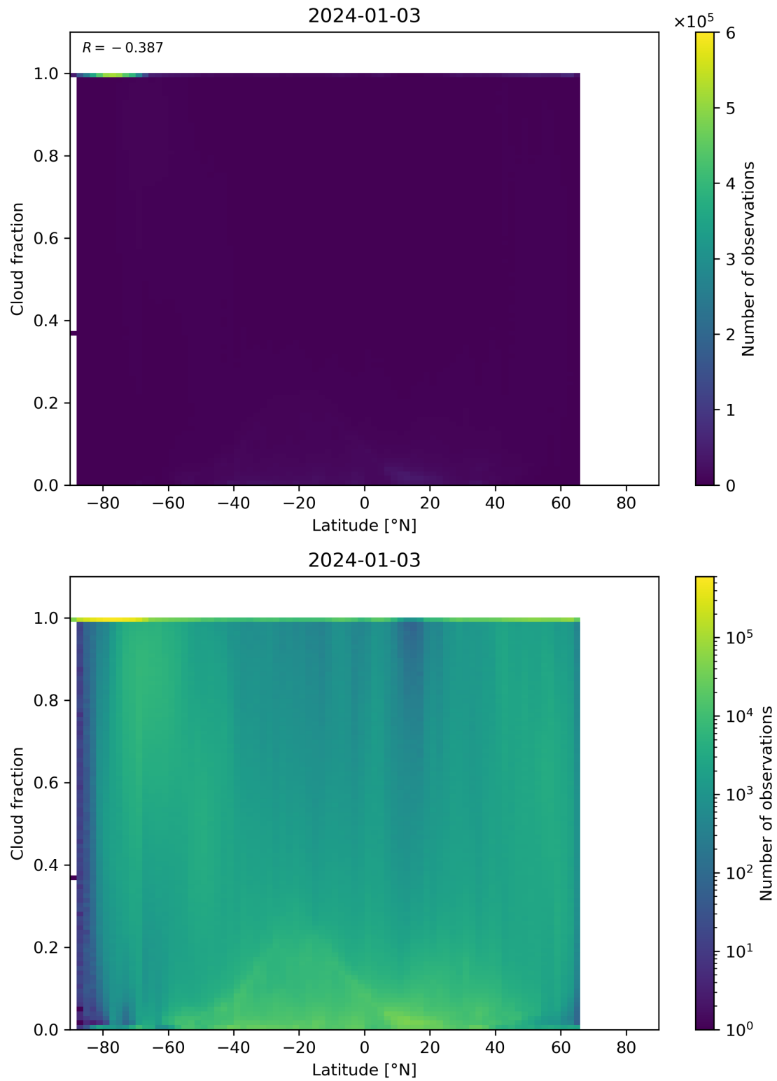
Figure 90: Scatter density plot of “Latitude” against “Cloud fraction” for 2024-01-02 to 2024-01-04.
