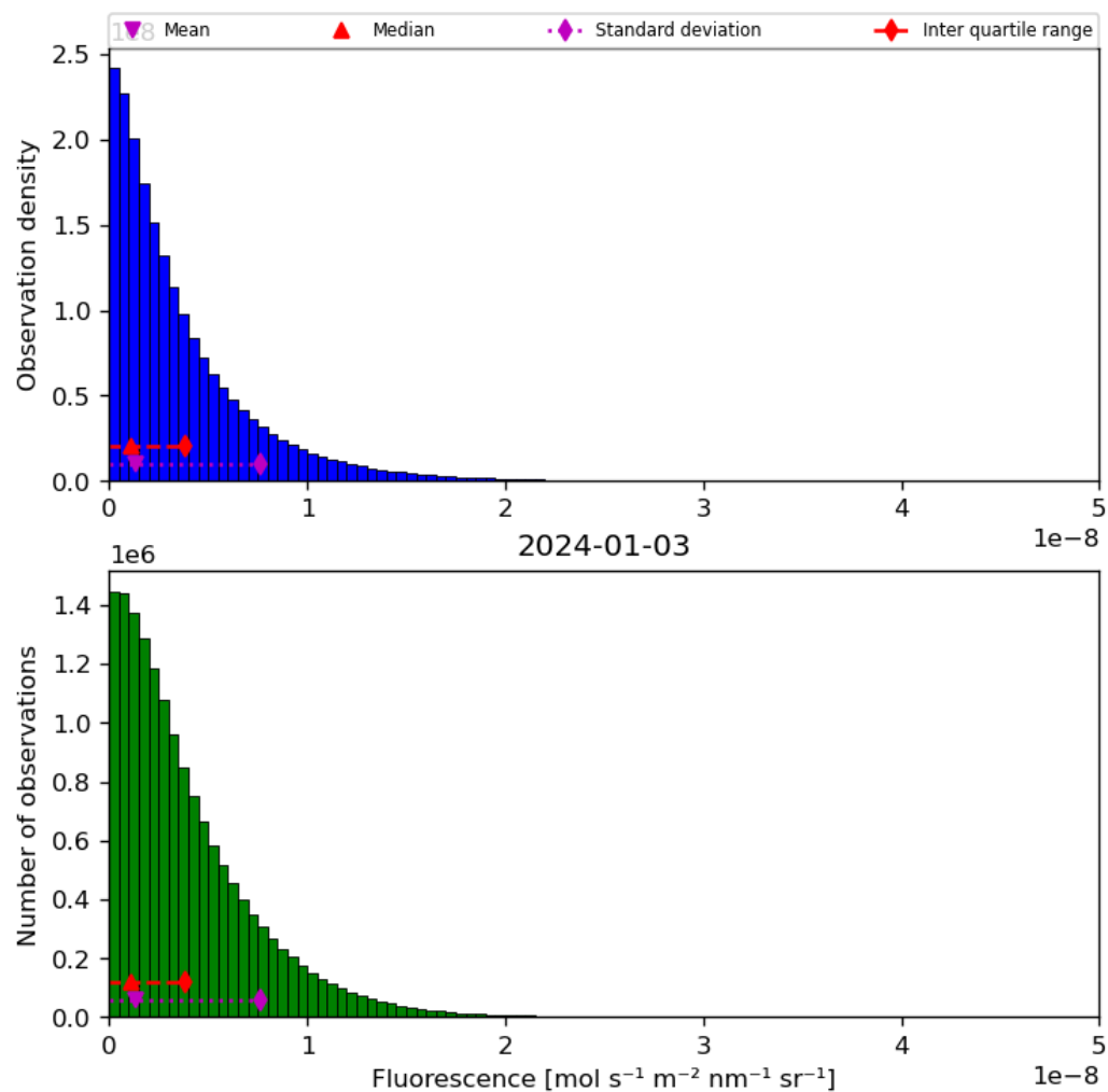
Figure 40: Histogram of “Fluorescence” for 2024-01-02 to 2024-01-04
