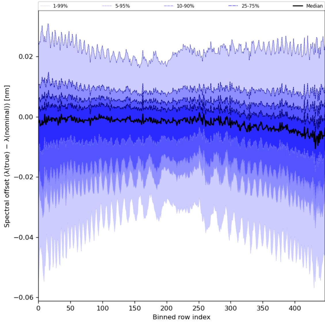
Figure 62: Along track statistics of “Spectral offset ( \lambda(\text{true}) - \lambda(\text{nominal}) )” for 2024-01-02 to 2024-01-04
