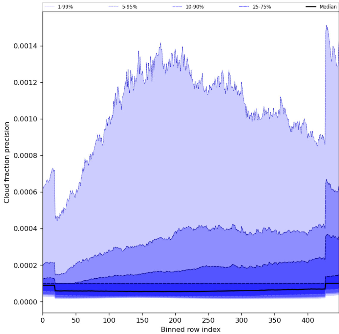
Figure 50: Along track statistics of “Cloud fraction precision” for 2024-01-02 to 2024-01-04
