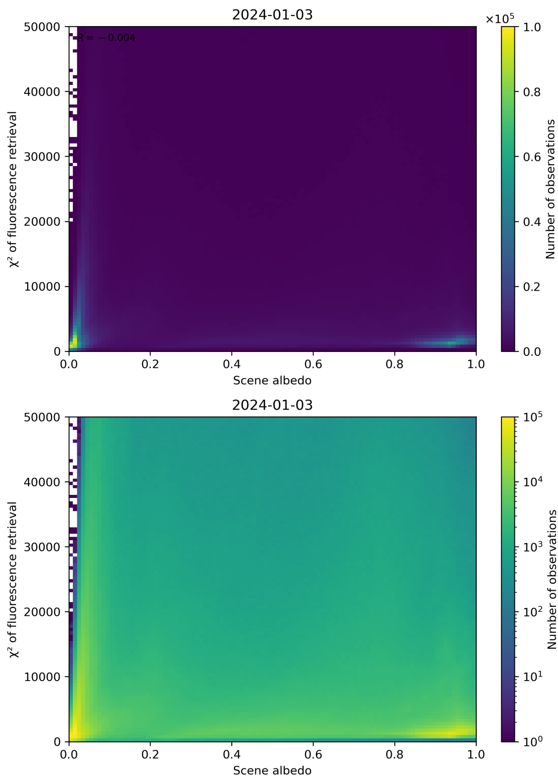
Figure 103: Scatter density plot of “Scene albedo” against “ \chi^2 of fluorescence retrieval” for 2024-01-02 to 2024-01-04.
