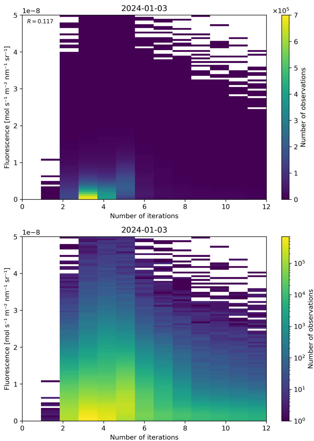
Figure 98: Scatter density plot of “Number of iterations” against “Fluorescence” for 2024-01-02 to 2024-01-04.
