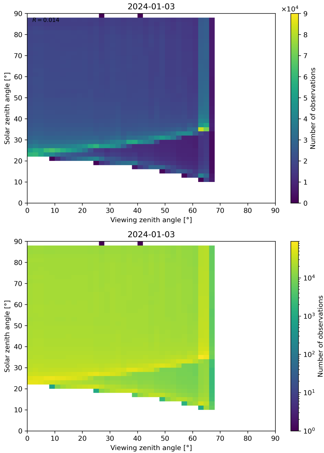
Figure 127: Scatter density plot of “Viewing zenith angle” against “Solar zenith angle” for 2024-01-02 to 2024-01-04.
