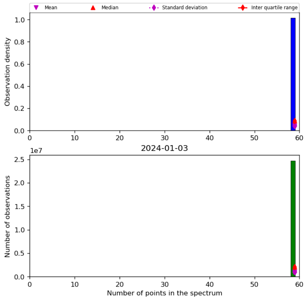
Figure 44: Histogram of “Number of points in the spectrum” for 2024-01-02 to 2024-01-04
