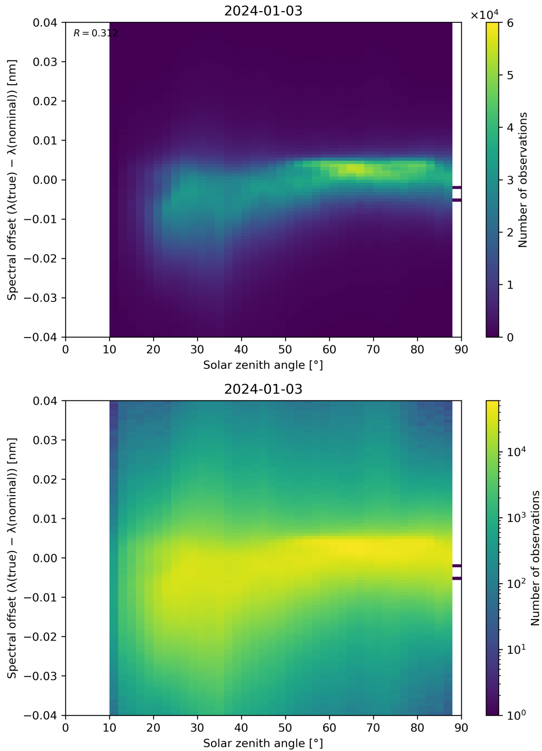
Figure 117: Scatter density plot of “Solar zenith angle” against “Spectral offset ( \lambda(\text{true}) - \lambda(\text{nominal}) )” for 2024-01-02 to 2024-01-04.
