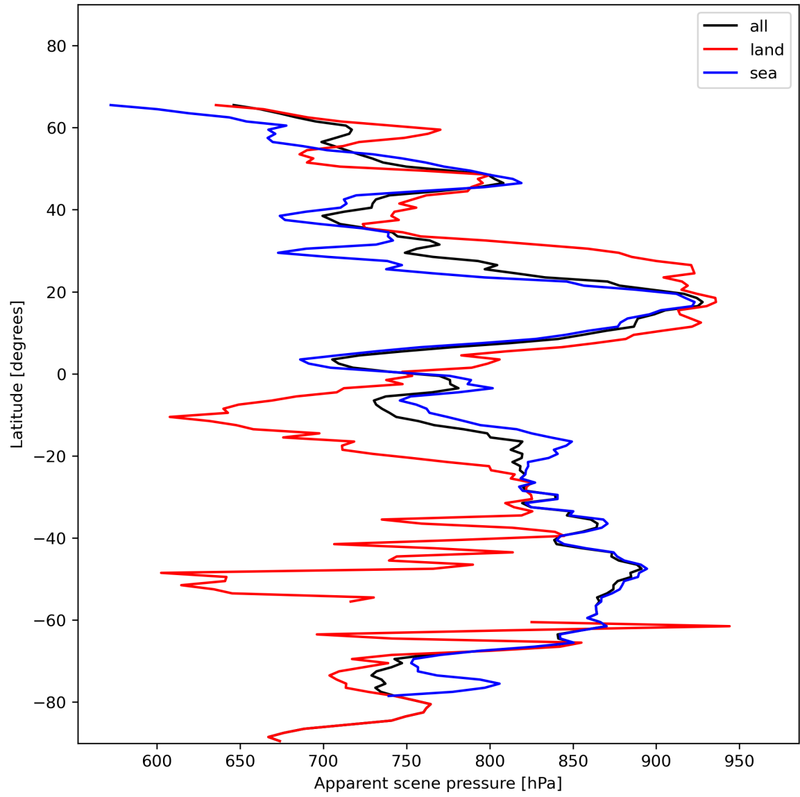
Figure 19: Zonal average of “Apparent scene pressure” for 2024-01-02 to 2024-01-04.
