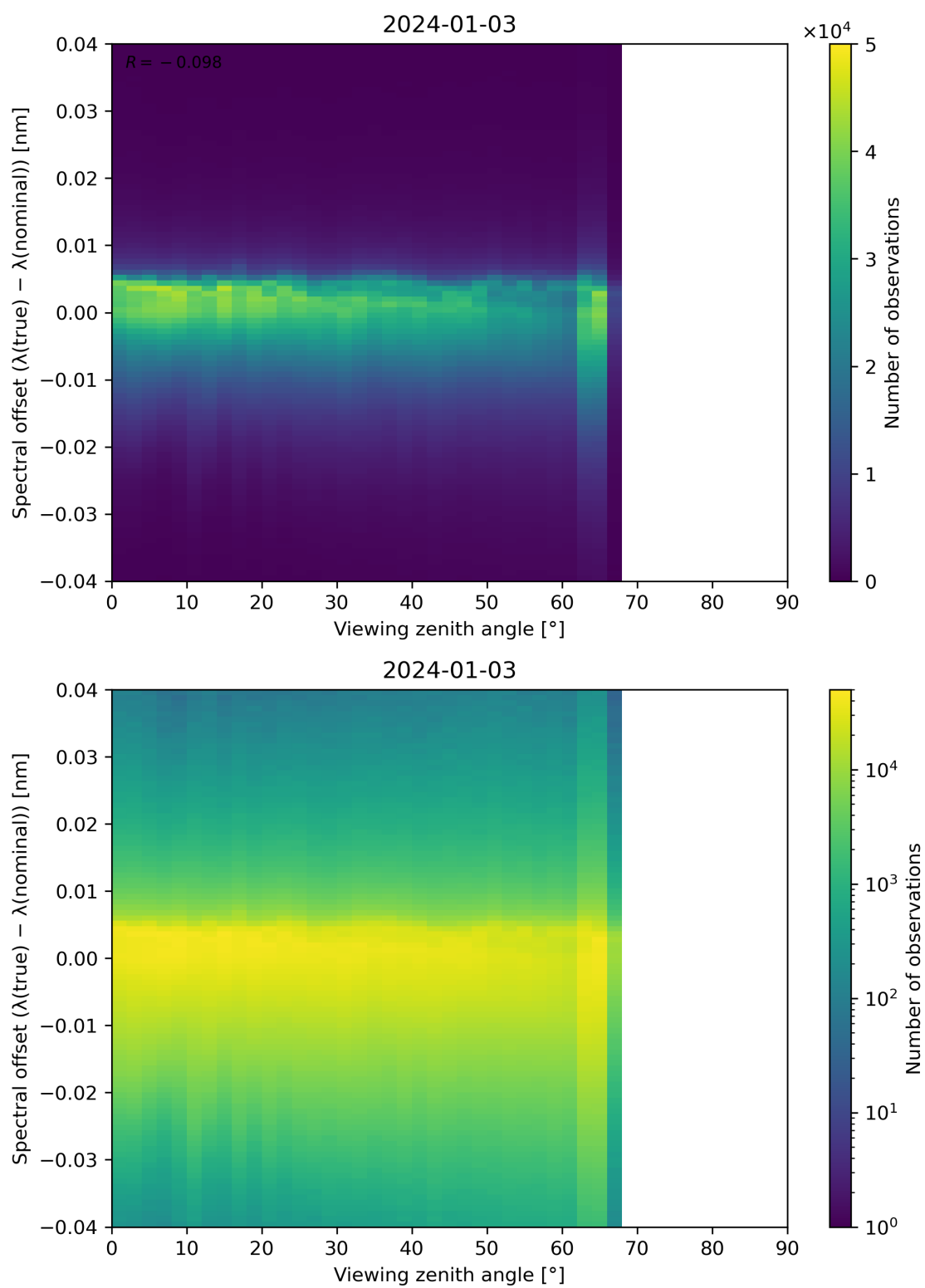
Figure 128: Scatter density plot of “Viewing zenith angle” against “Spectral offset ( \lambda(\text{true}) - \lambda(\text{nominal}) )” for 2024-01-02 to 2024-01-04.
