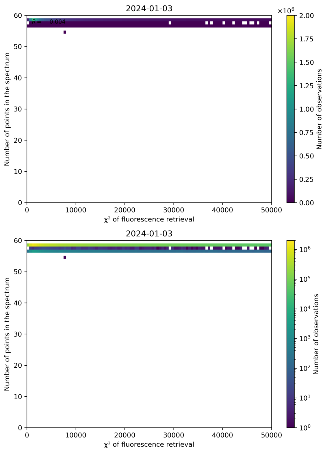
Figure 68: Scatter density plot of " \chi^2 of fluorescence retrieval" against "Number of points in the spectrum" for 2024-01-02 to 2024-01-04.
