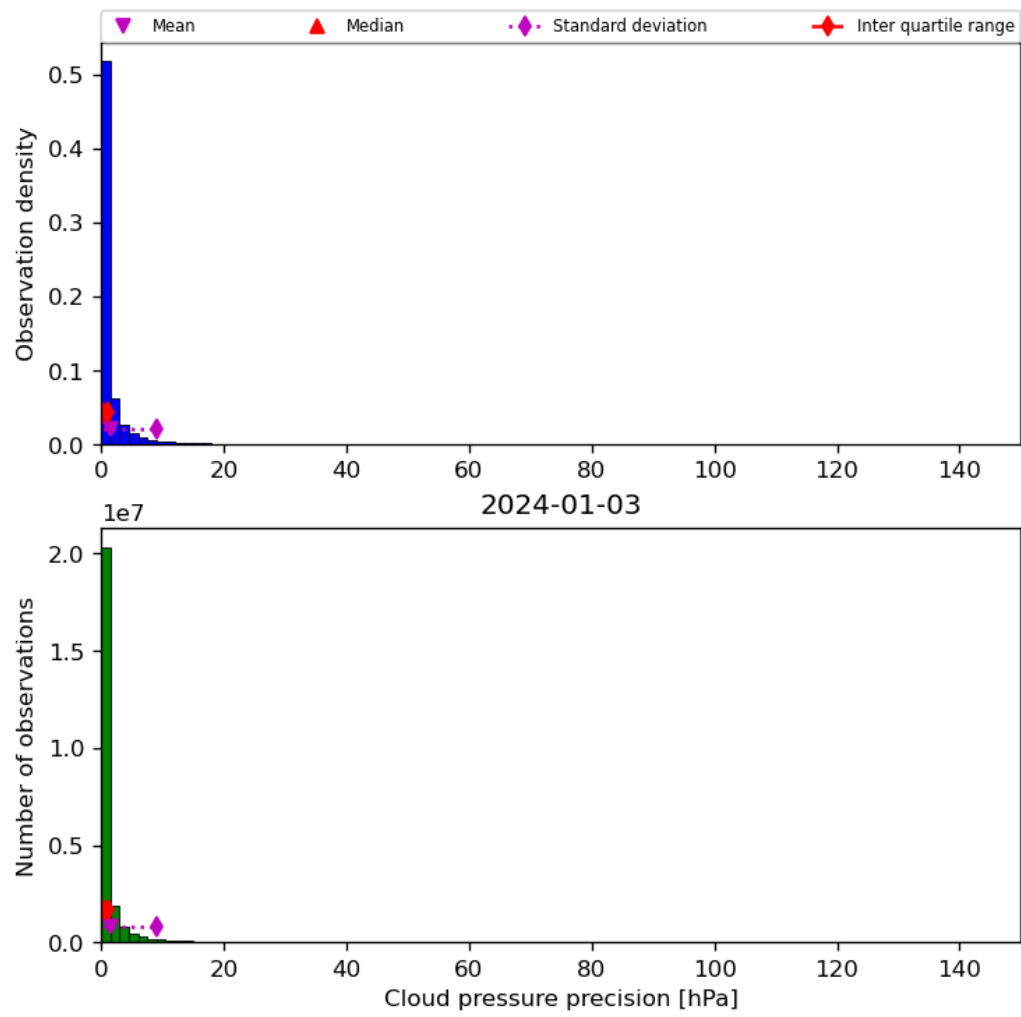
Figure 31: Histogram of “Cloud pressure precision” for 2024-01-02 to 2024-01-04
