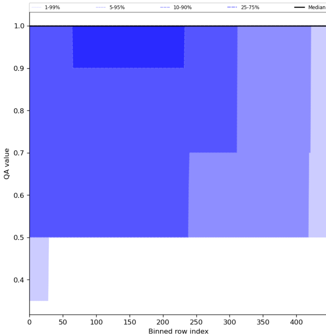
Figure 46: Along track statistics of “QA value” for 2024-01-02 to 2024-01-04
