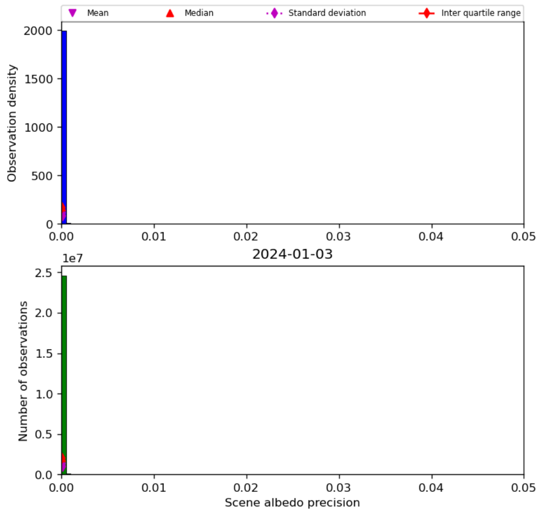
Figure 35: Histogram of “Scene albedo precision” for 2024-01-02 to 2024-01-04
