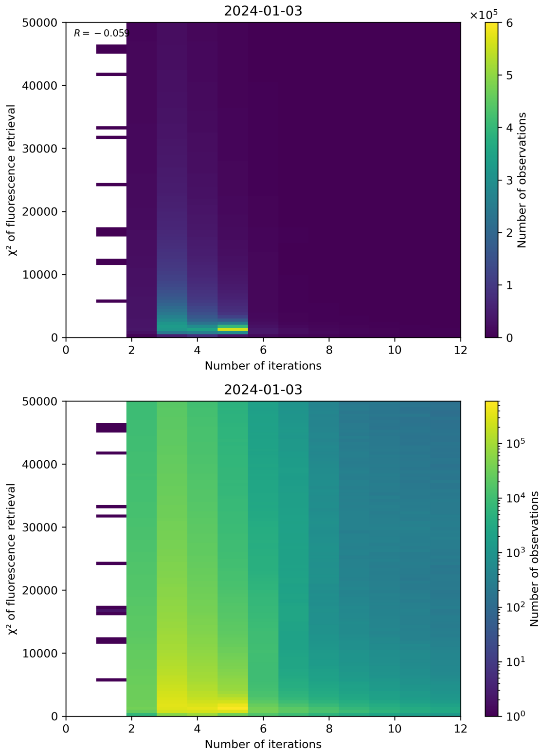
Figure 97: Scatter density plot of “Number of iterations” against “ \chi^2 of fluorescence retrieval” for 2024-01-02 to 2024-01-04.
