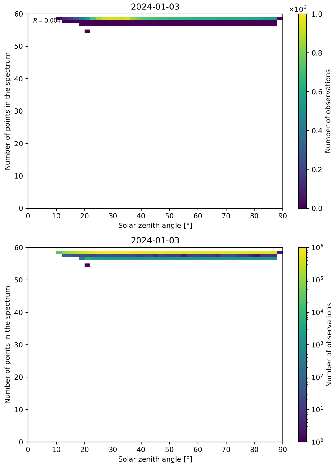
Figure 115: Scatter density plot of “Solar zenith angle” against “Number of points in the spectrum” for 2024-01-02 to 2024-01-04.
