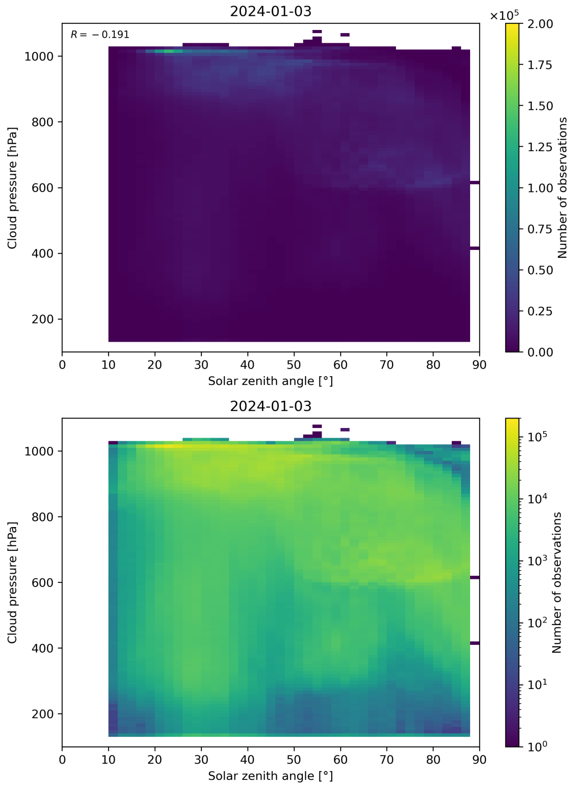
Figure 111: Scatter density plot of “Solar zenith angle” against “Cloud pressure” for 2024-01-02 to 2024-01-04.
