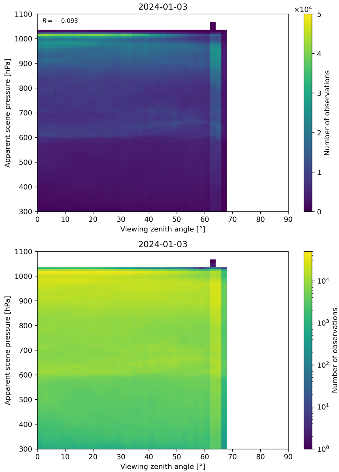
Figure 118: Scatter density plot of “Viewing zenith angle” against “Apparent scene pressure” for 2024-01-02 to 2024-01-04.
