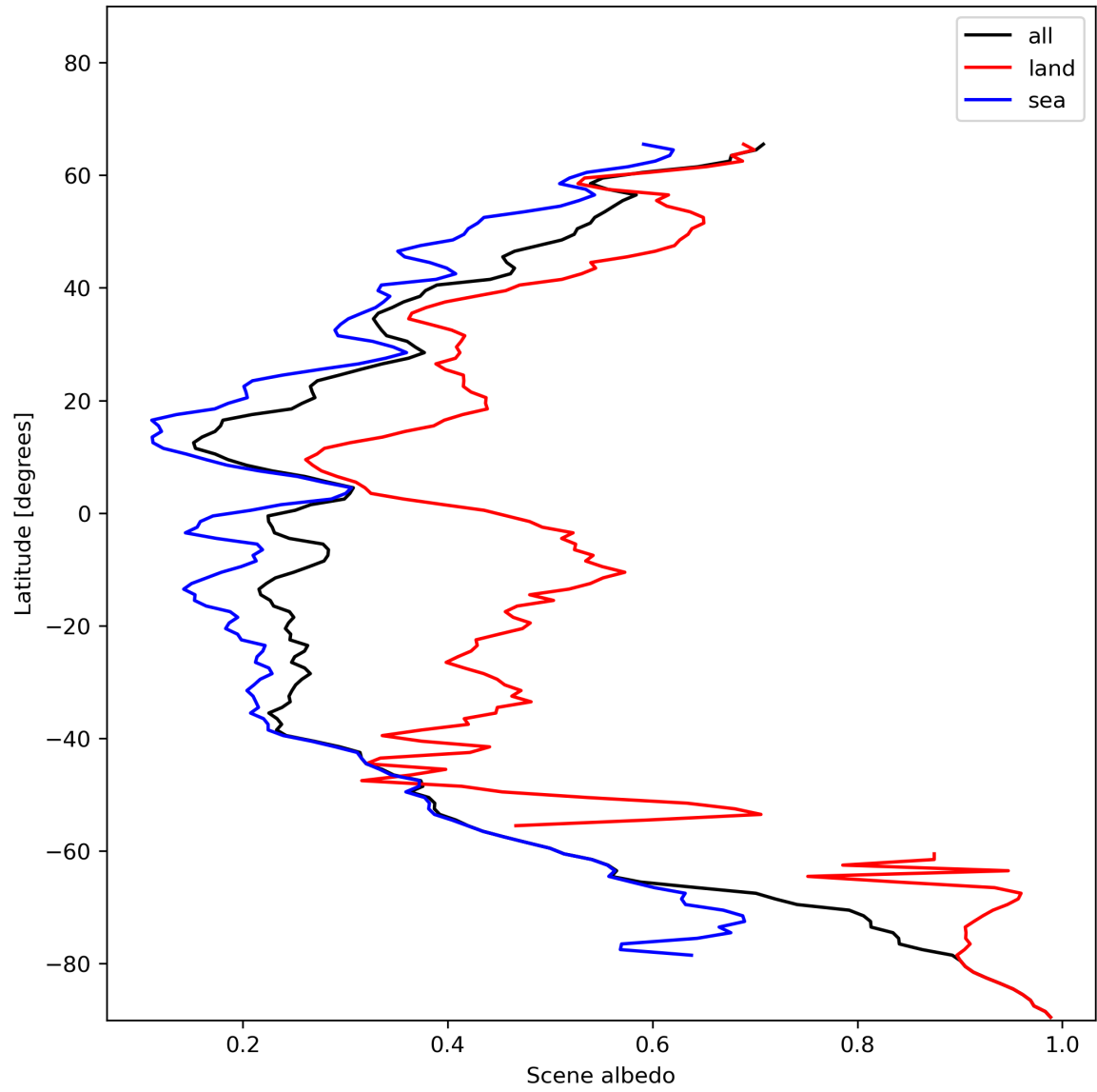
Figure 17: Zonal average of “Scene albedo” for 2024-01-02 to 2024-01-04.
