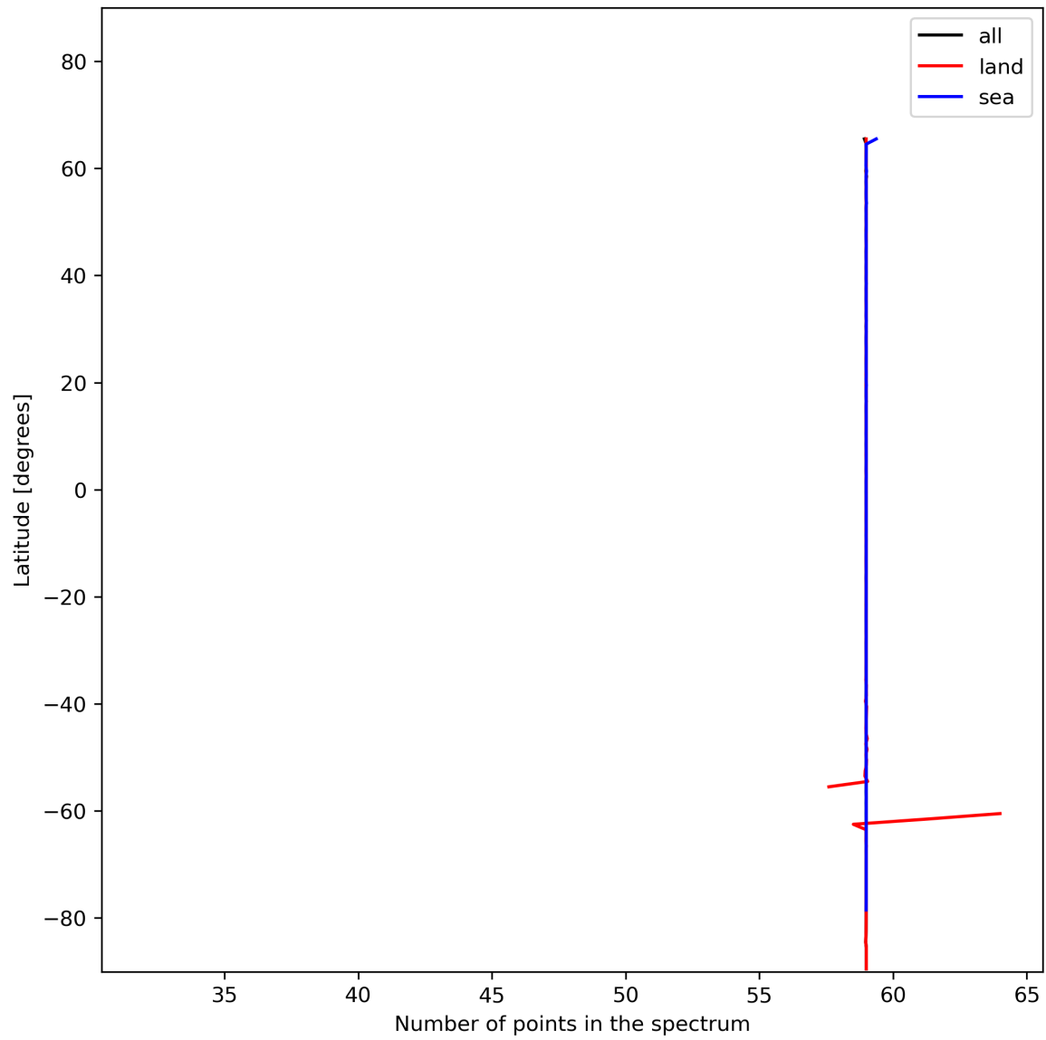
Figure 27: Zonal average of “Number of points in the spectrum” for 2024-01-02 to 2024-01-04.
