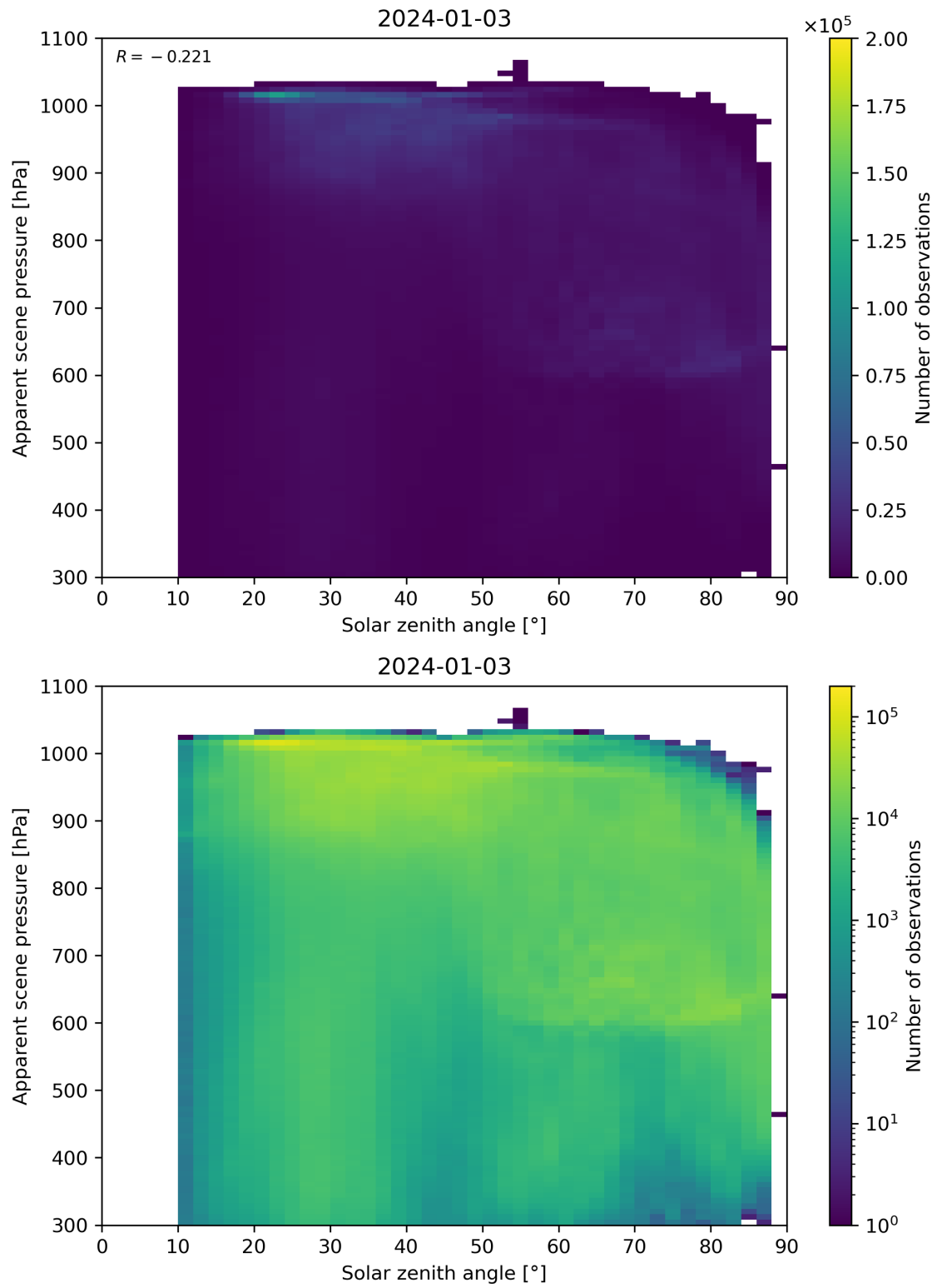
Figure 108: Scatter density plot of “Solar zenith angle” against “Apparent scene pressure” for 2024-01-02 to 2024-01-04.
