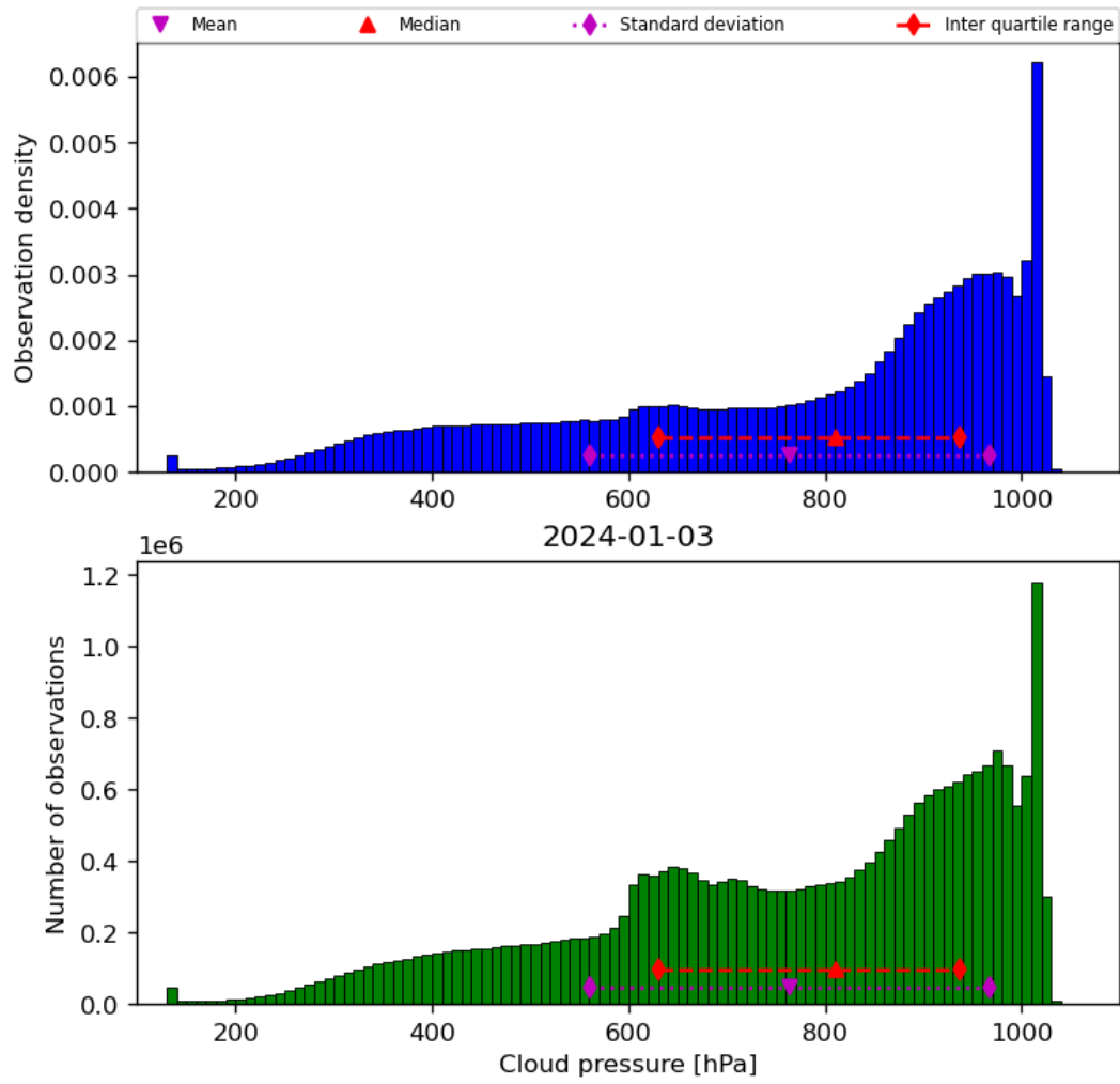
Figure 30: Histogram of “Cloud pressure” for 2024-01-02 to 2024-01-04
