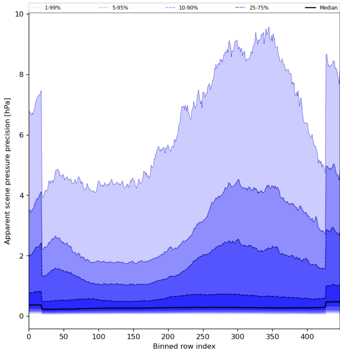
Figure 54: Along track statistics of “Apparent scene pressure precision” for 2024-01-02 to 2024-01-04
