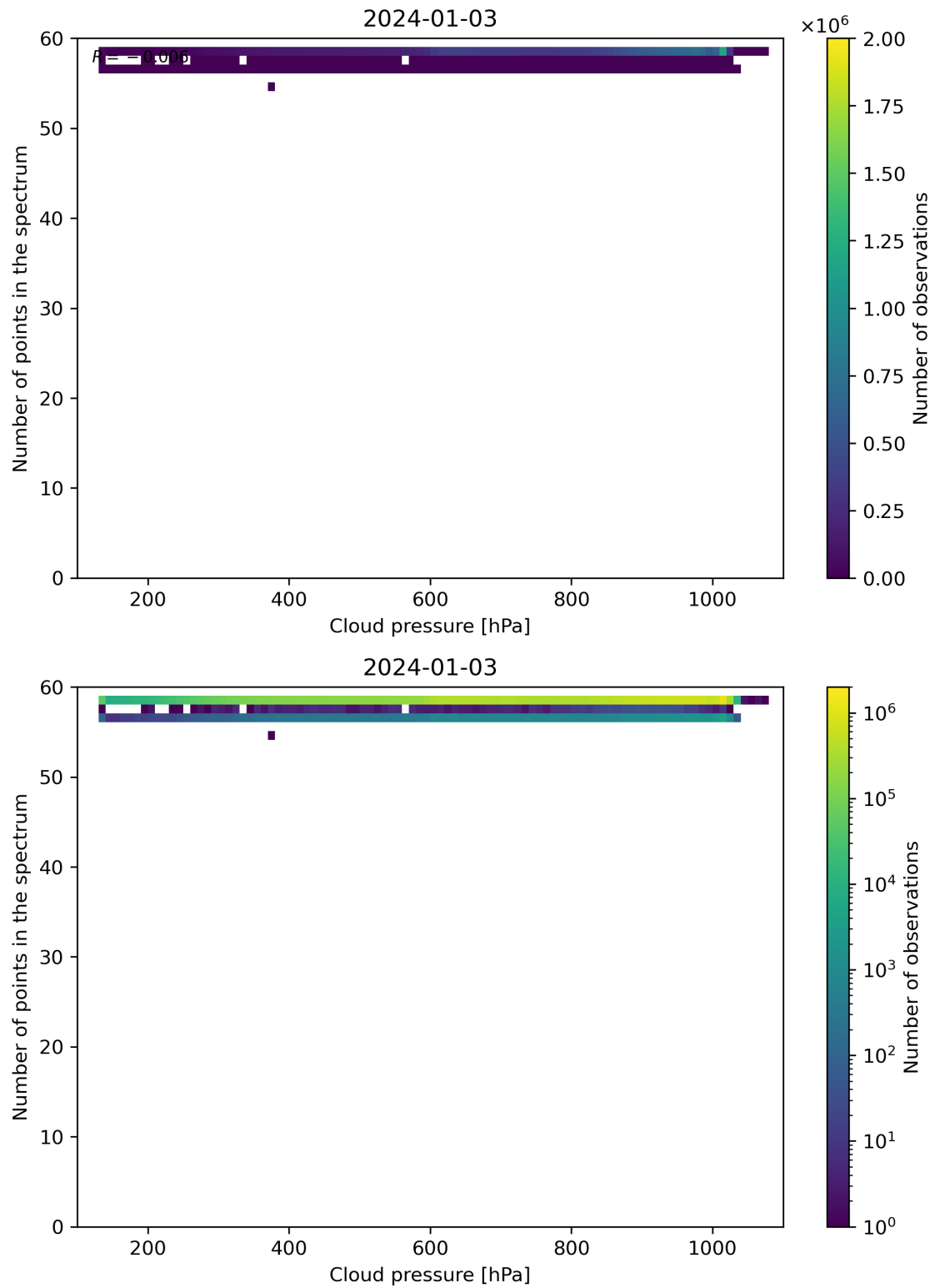
Figure 82: Scatter density plot of “Cloud pressure” against “Number of points in the spectrum” for 2024-01-02 to 2024-01-04.
