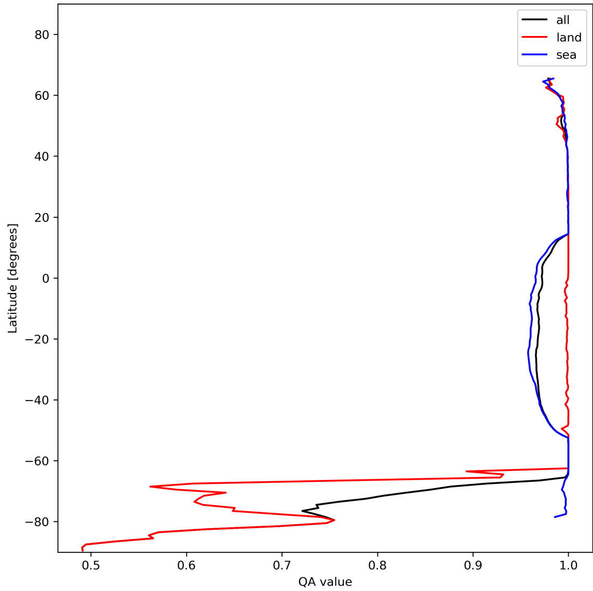
Figure 12: Zonal average of “QA value” for 2024-01-02 to 2024-01-04.
