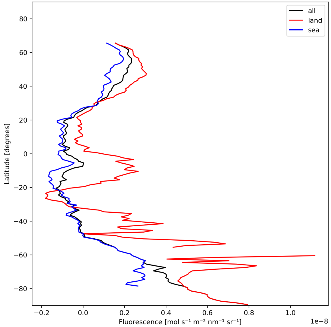
Figure 23: Zonal average of “Fluorescence” for 2024-01-02 to 2024-01-04.
