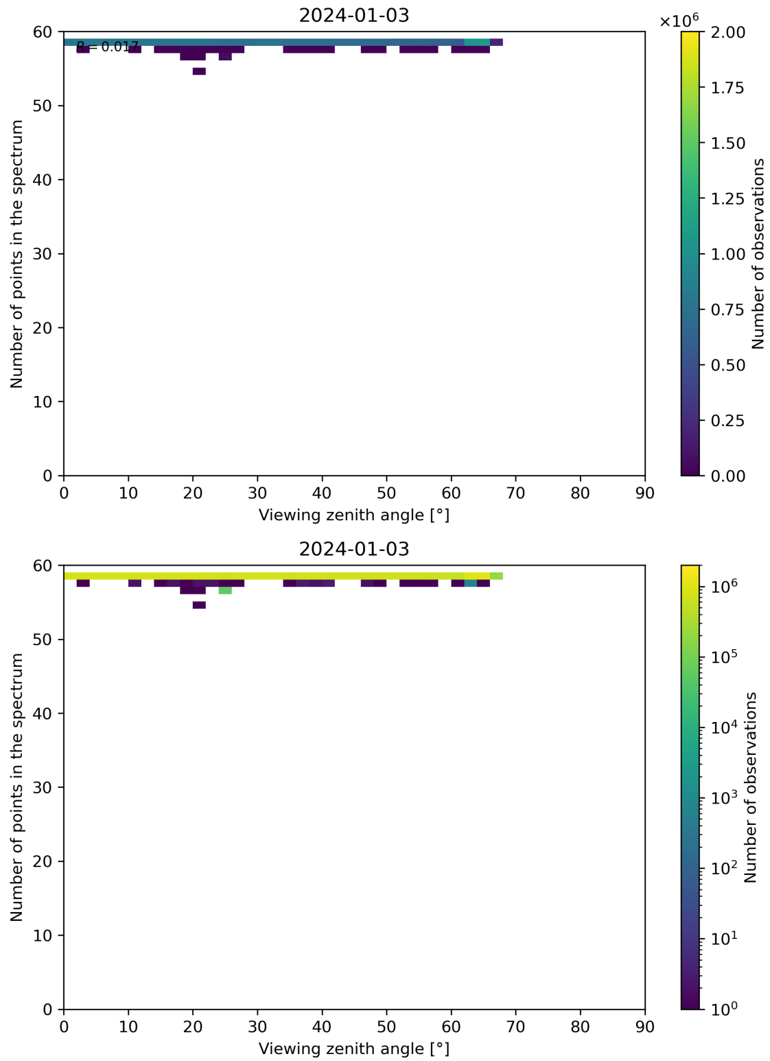
Figure 125: Scatter density plot of “Viewing zenith angle” against “Number of points in the spectrum” for 2024-01-02 to 2024-01-04.
