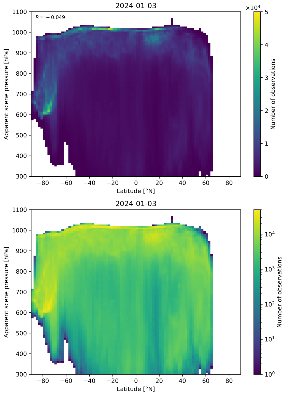
Figure 88: Scatter density plot of “Latitude” against “Apparent scene pressure” for 2024-01-02 to 2024-01-04.
