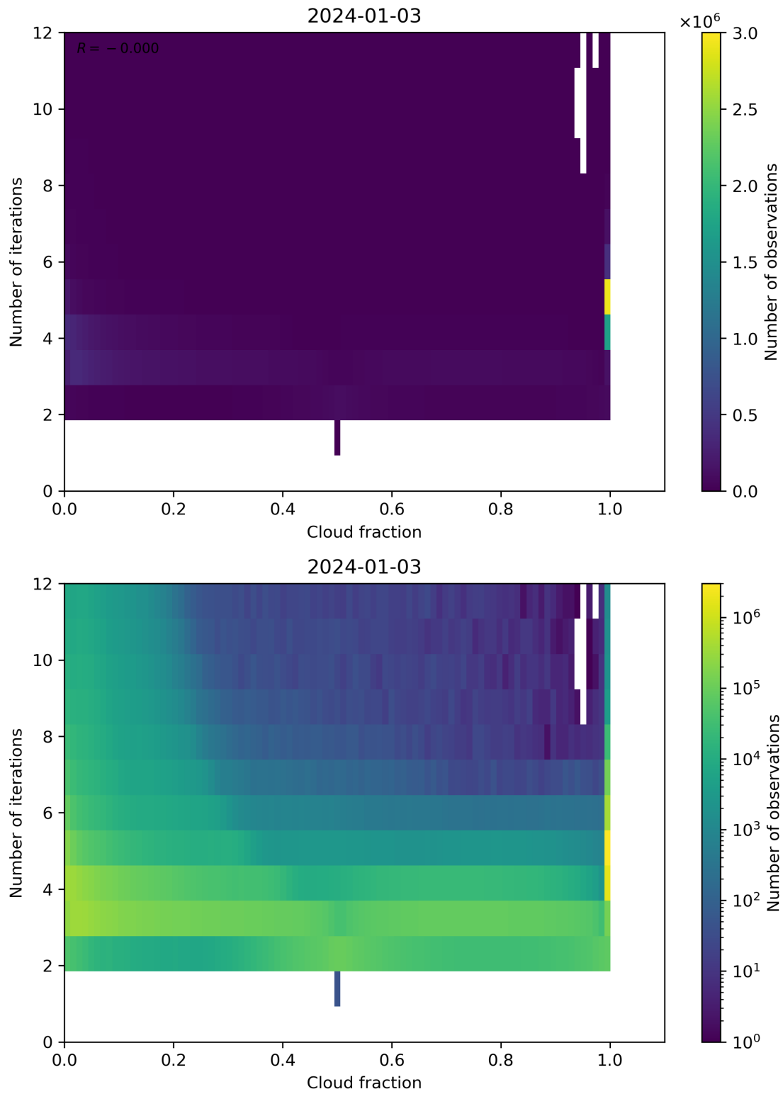
Figure 73: Scatter density plot of “Cloud fraction” against “Number of iterations” for 2024-01-02 to 2024-01-04.
