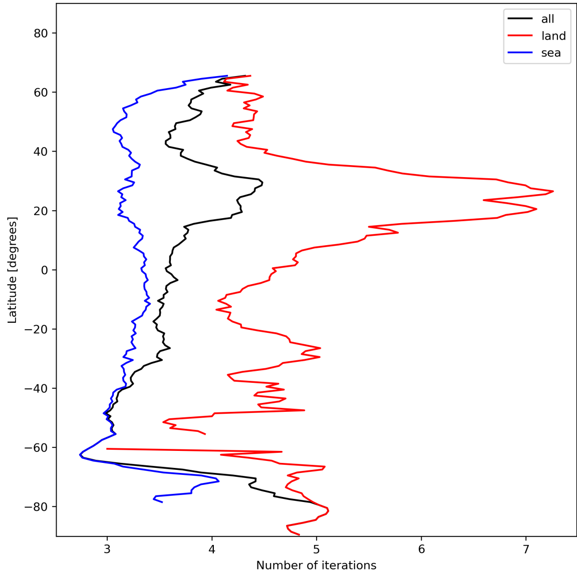
Figure 22: Zonal average of “Number of iterations” for 2024-01-02 to 2024-01-04.
