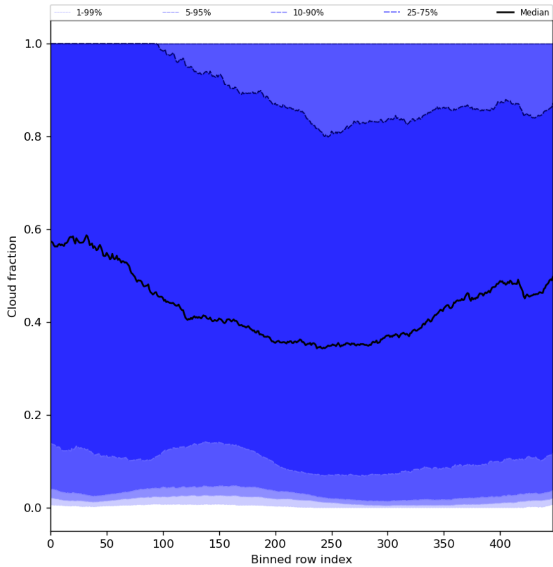
Figure 49: Along track statistics of “Cloud fraction” for 2024-01-02 to 2024-01-04
