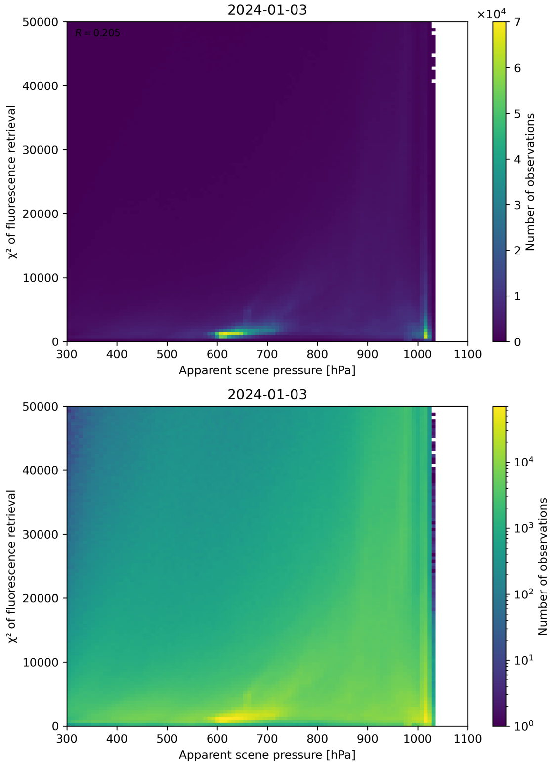
Figure 63: Scatter density plot of “Apparent scene pressure” against “ \chi^2 of fluorescence retrieval” for 2024-01-02 to 2024-01-04.
