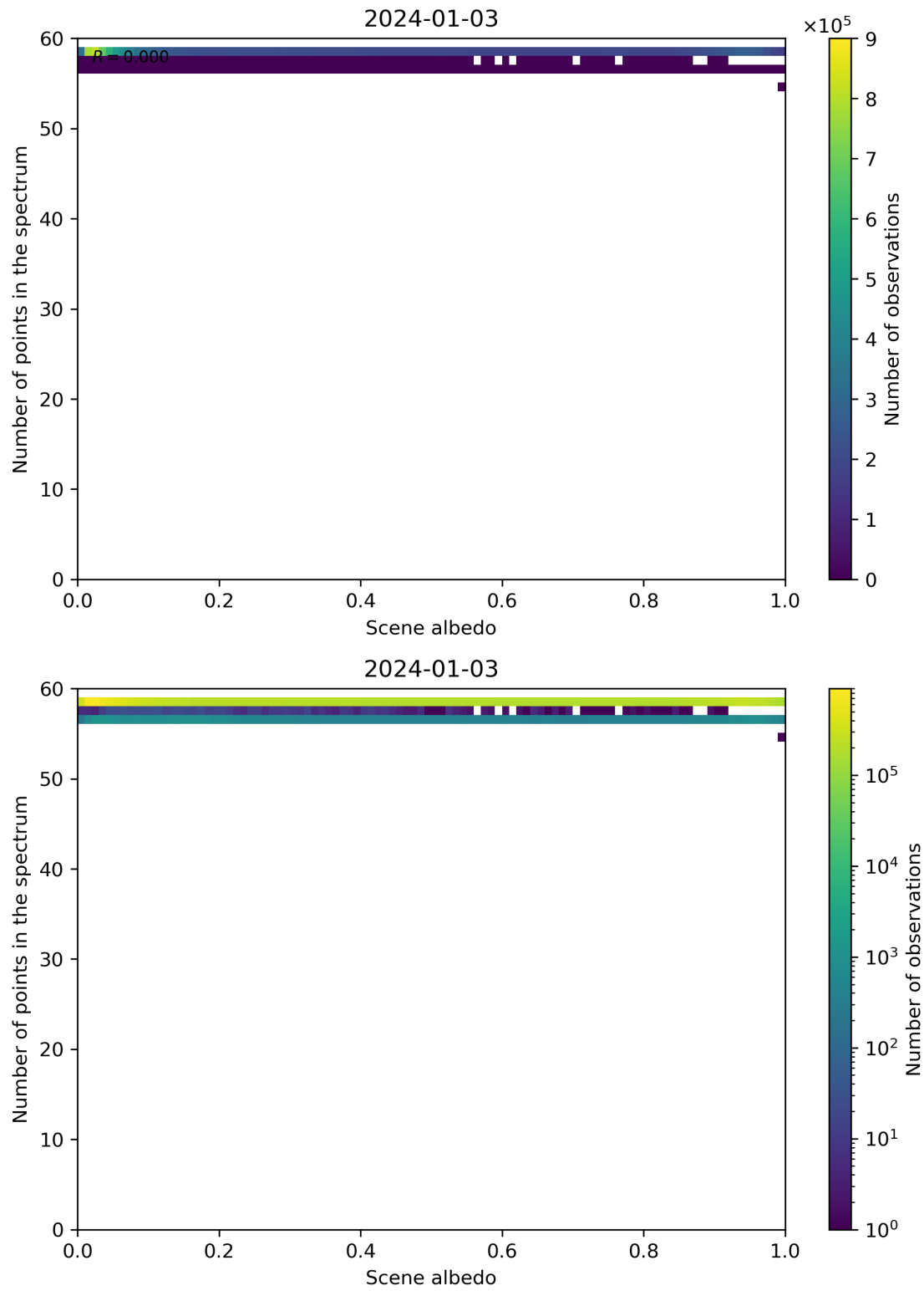
Figure 106: Scatter density plot of “Scene albedo” against “Number of points in the spectrum” for 2024-01-02 to 2024-01-04.
