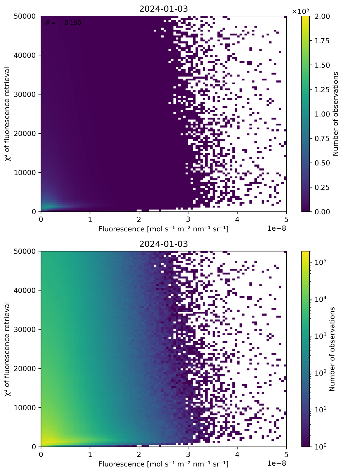
Figure 85: Scatter density plot of “Fluorescence” against “ \chi^2 of fluorescence retrieval” for 2024-01-02 to 2024-01-04.
