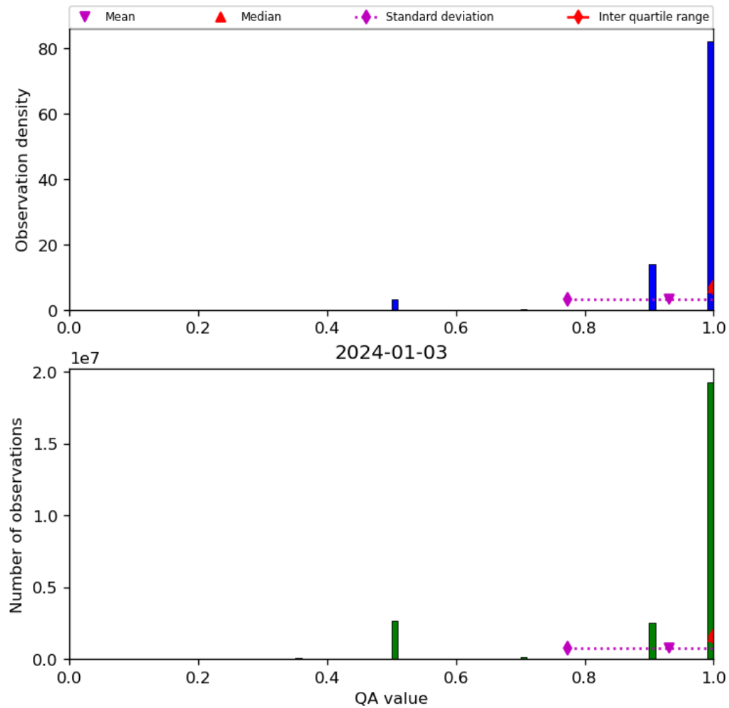
Figure 29: Histogram of “QA value” for 2024-01-02 to 2024-01-04
