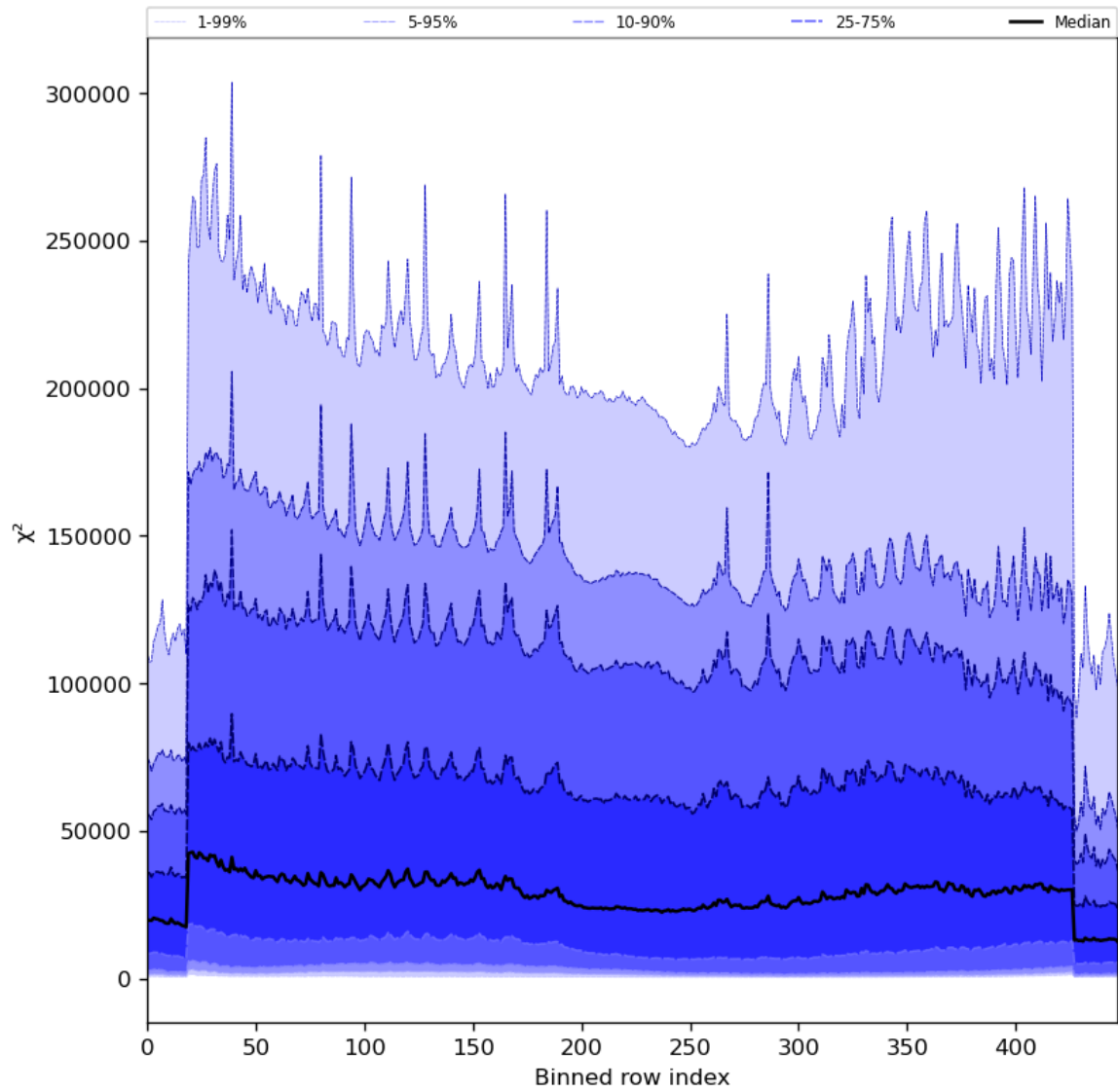
Figure 55: Along track statistics of “ \chi^2 ” for 2024-01-02 to 2024-01-04
