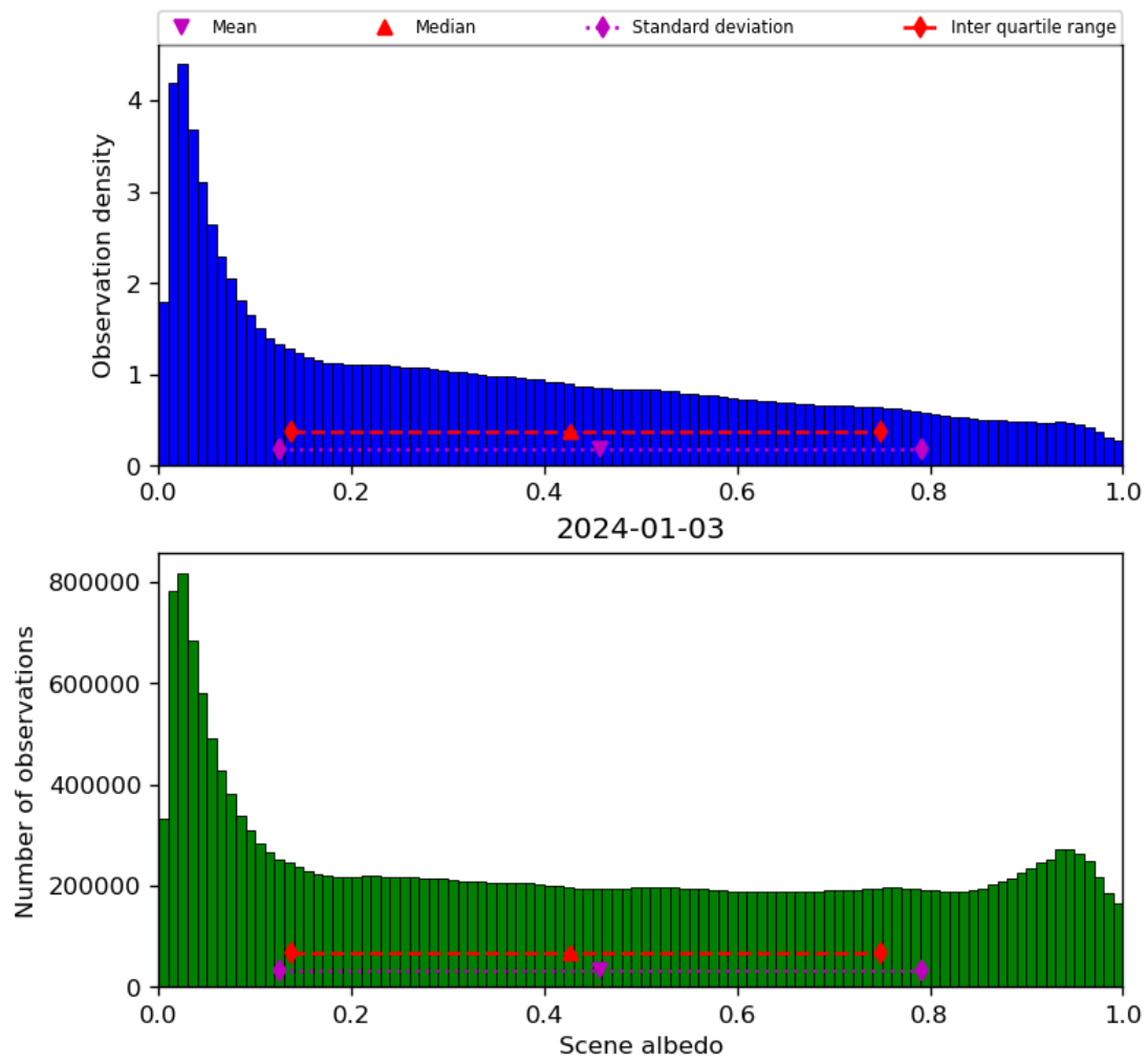
Figure 34: Histogram of “Scene albedo” for 2024-01-02 to 2024-01-04
