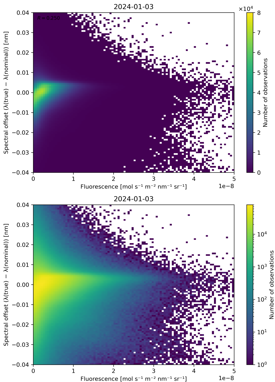
Figure 87: Scatter density plot of “Fluorescence” against “Spectral offset ( \lambda(\text{true}) - \lambda(\text{nominal}) )” for 2024-01-02 to 2024-01-04.
