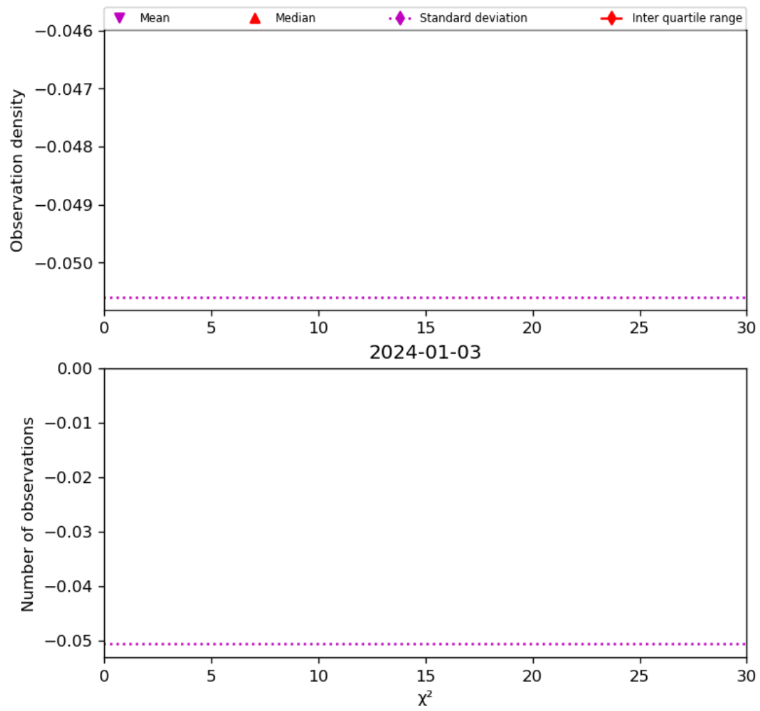
Figure 38: Histogram of “ \chi^2 ” for 2024-01-02 to 2024-01-04
