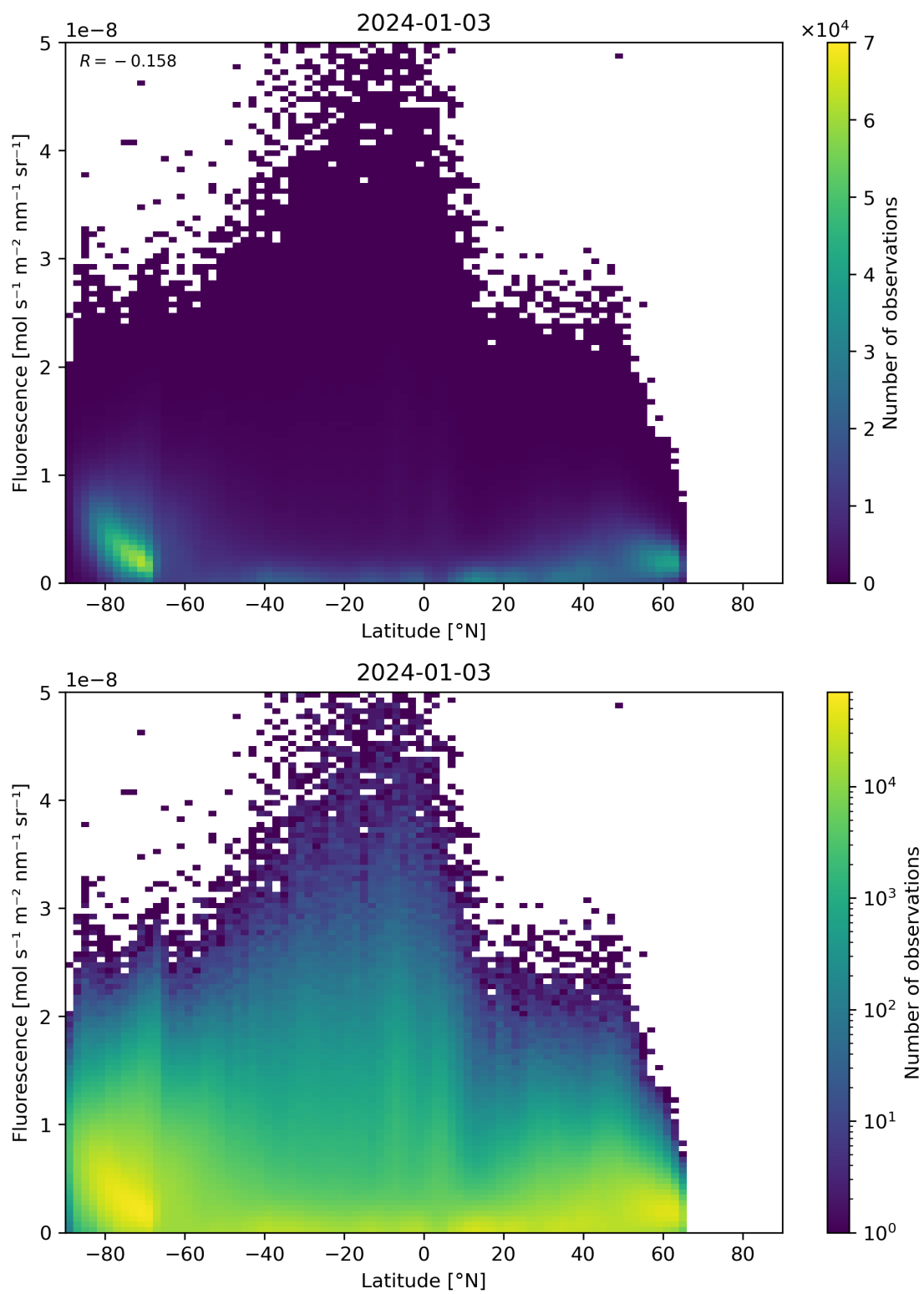
Figure 92: Scatter density plot of “Latitude” against “Fluorescence” for 2024-01-02 to 2024-01-04.
