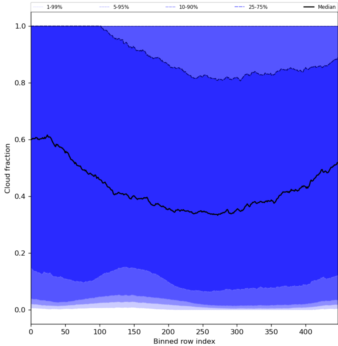
Figure 49: Along track statistics of “Cloud fraction” for 2024-01-03 to 2024-01-05
