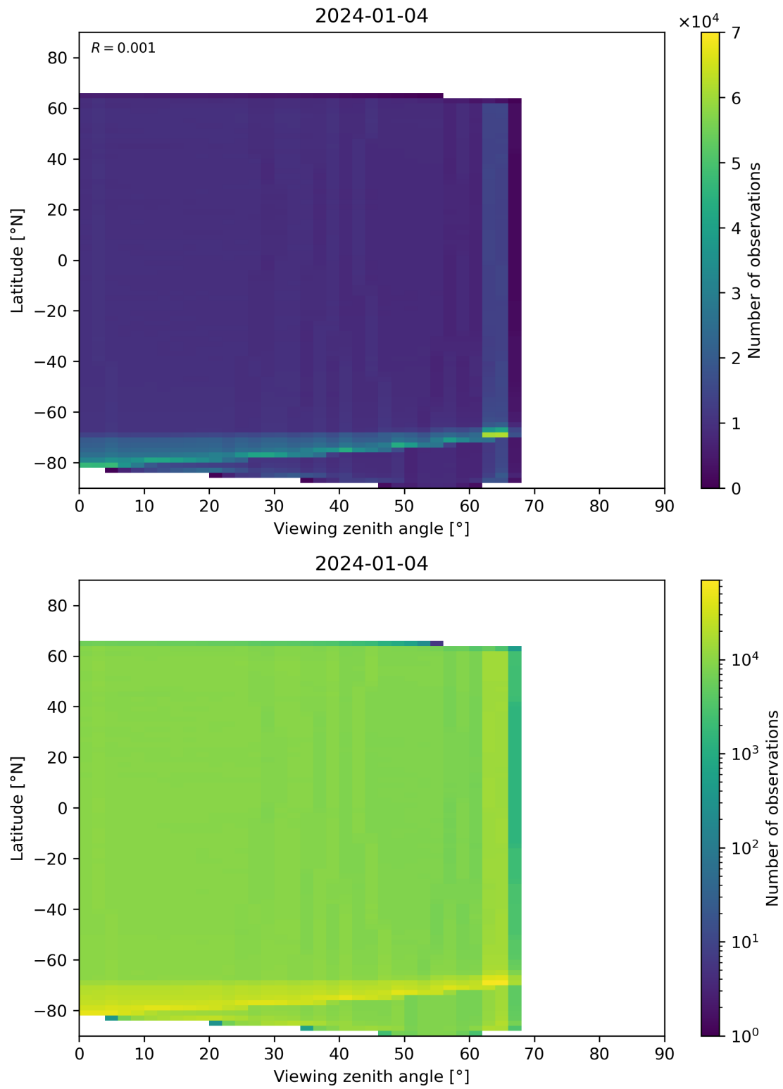
Figure 123: Scatter density plot of “Viewing zenith angle” against “Latitude” for 2024-01-03 to 2024-01-05.
