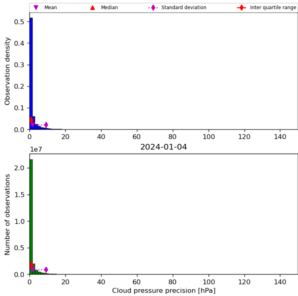
Figure 31: Histogram of “Cloud pressure precision” for 2024-01-03 to 2024-01-05
