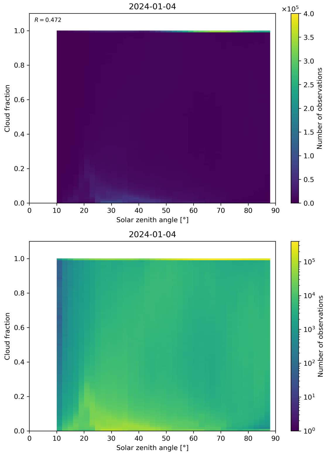
Figure 110: Scatter density plot of “Solar zenith angle” against “Cloud fraction” for 2024-01-03 to 2024-01-05.
