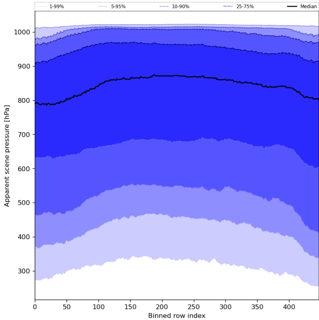
Figure 53: Along track statistics of “Apparent scene pressure” for 2024-01-03 to 2024-01-05
