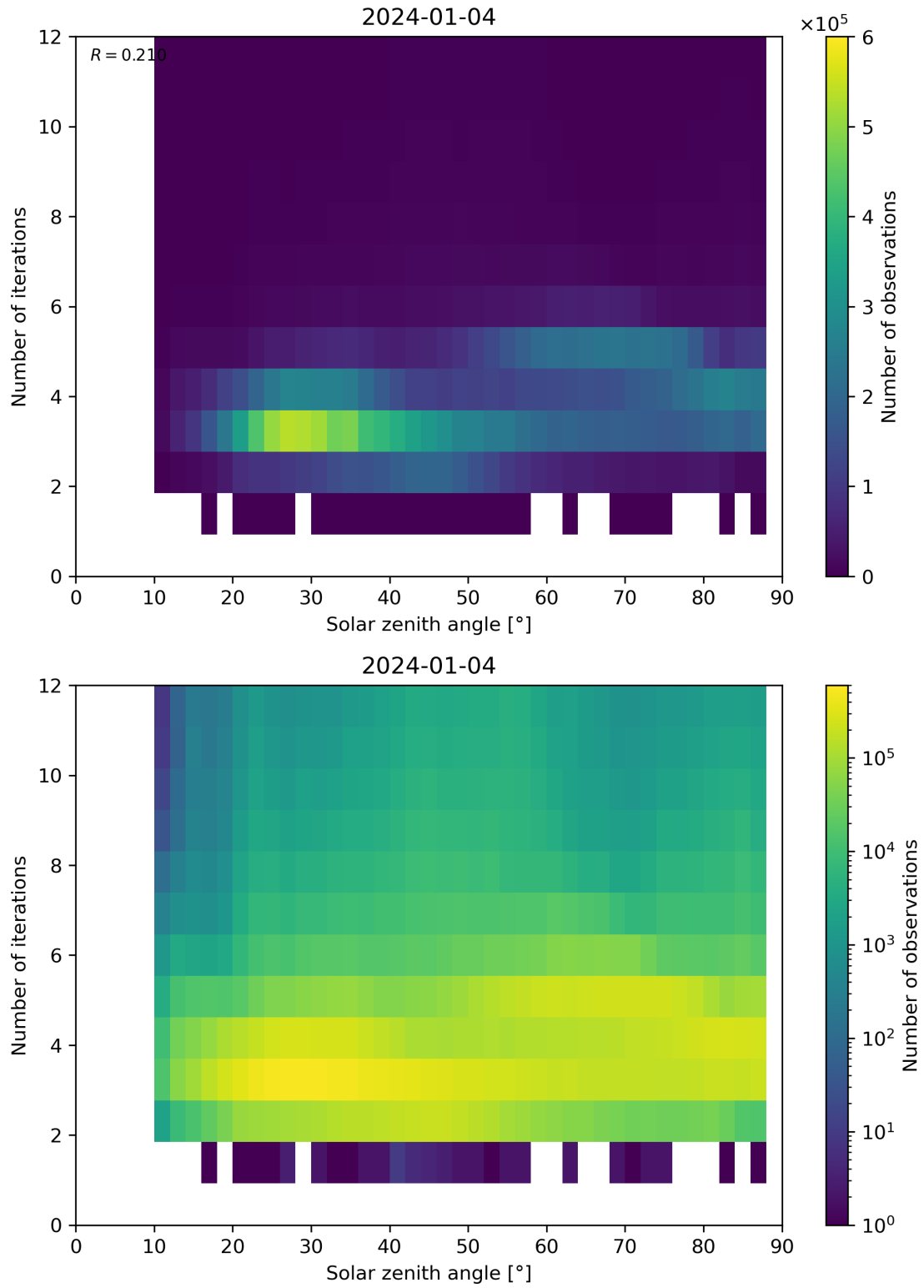
Figure 114: Scatter density plot of “Solar zenith angle” against “Number of iterations” for 2024-01-03 to 2024-01-05.
