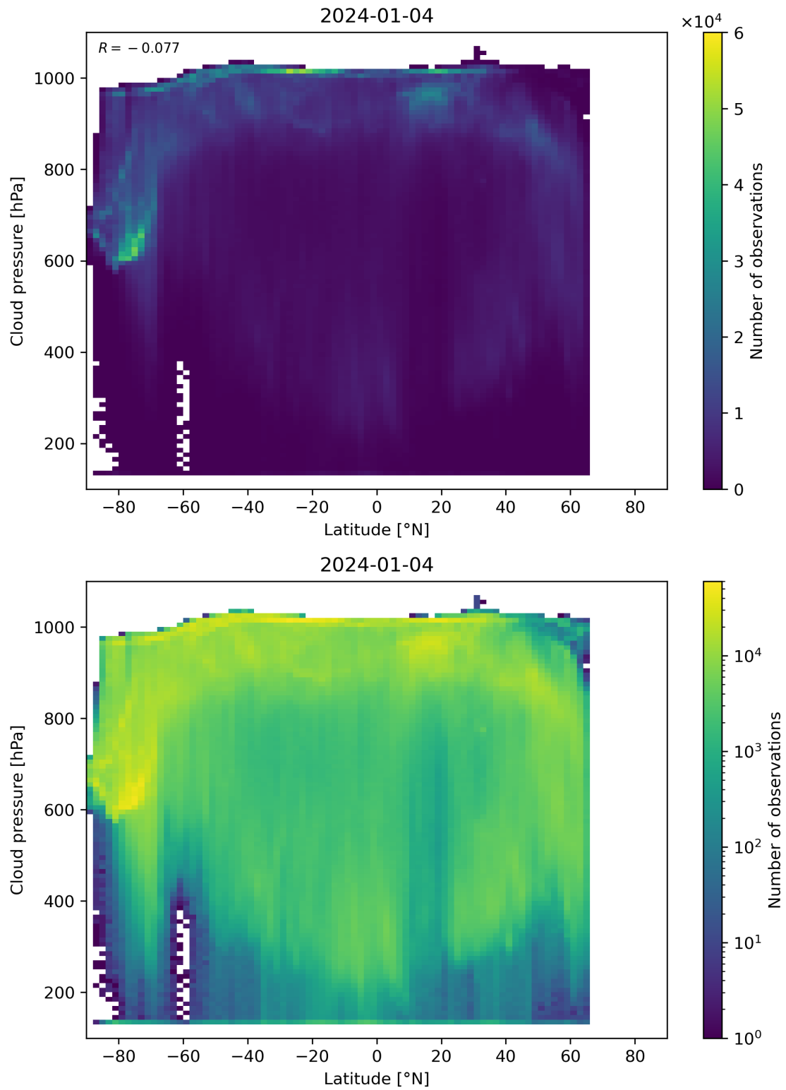
Figure 91: Scatter density plot of “Latitude” against “Cloud pressure” for 2024-01-03 to 2024-01-05.
