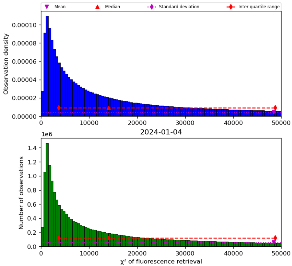
Figure 42: Histogram of “ \chi^2 of fluorescence retrieval” for 2024-01-03 to 2024-01-05
