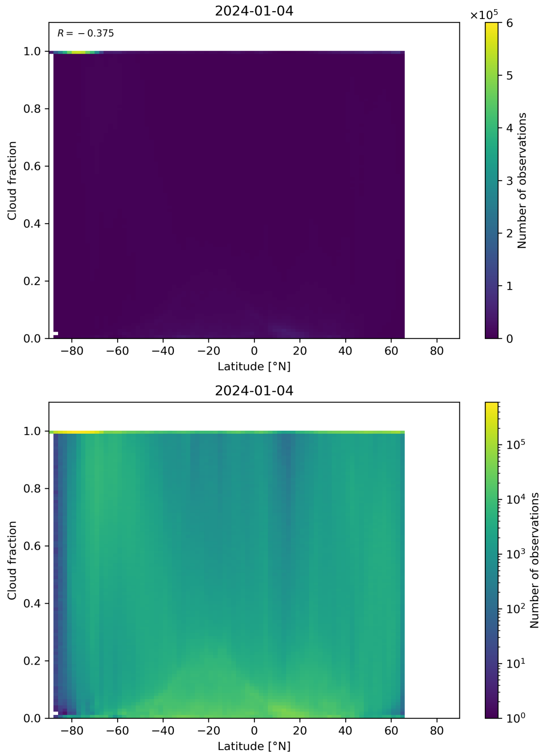
Figure 90: Scatter density plot of “Latitude” against “Cloud fraction” for 2024-01-03 to 2024-01-05.
