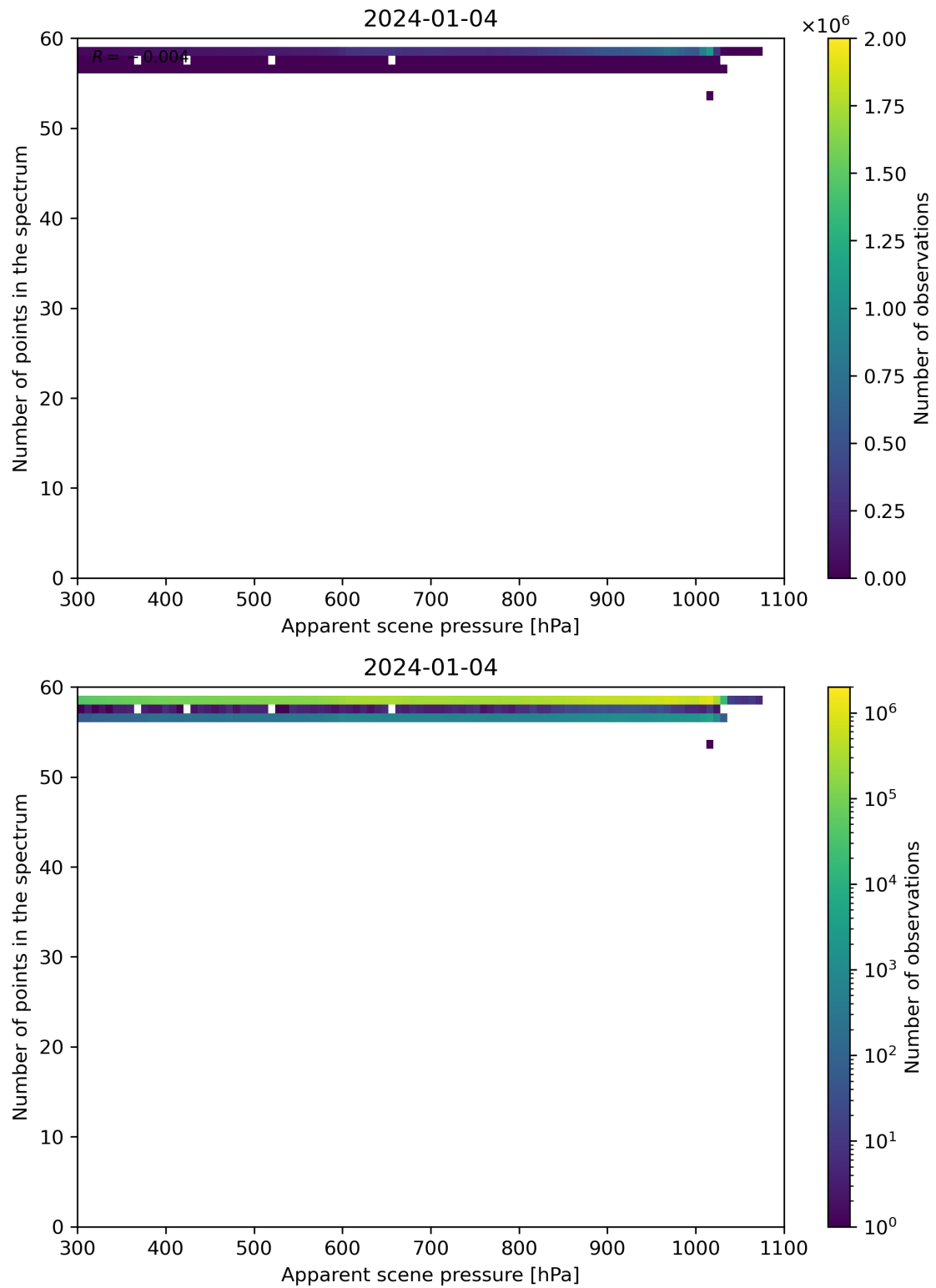
Figure 66: Scatter density plot of “Apparent scene pressure” against “Number of points in the spectrum” for 2024-01-03 to 2024-01-05.
