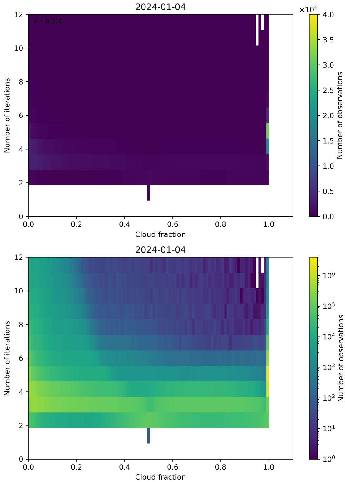
Figure 73: Scatter density plot of “Cloud fraction” against “Number of iterations” for 2024-01-03 to 2024-01-05.
