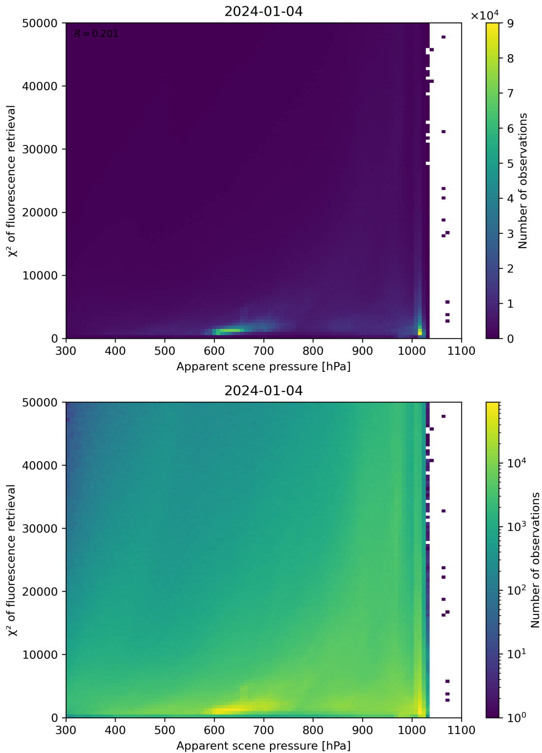
Figure 63: Scatter density plot of “Apparent scene pressure” against “ \chi^2 of fluorescence retrieval” for 2024-01-03 to 2024-01-05.
