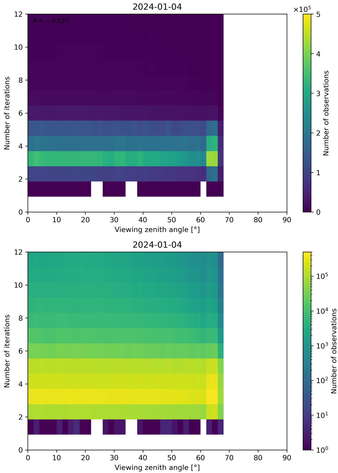
Figure 124: Scatter density plot of “Viewing zenith angle” against “Number of iterations” for 2024-01-03 to 2024-01-05.
