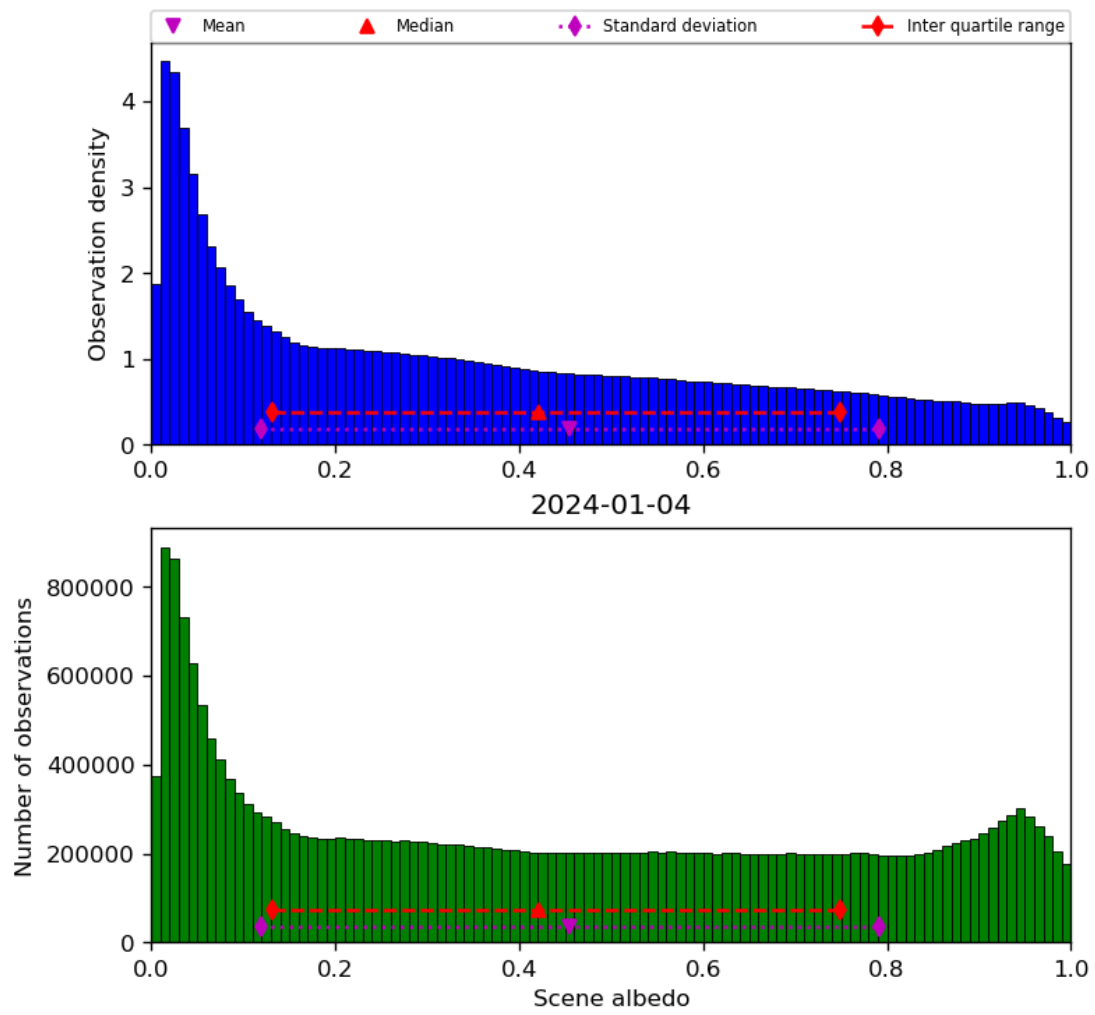
Figure 34: Histogram of “Scene albedo” for 2024-01-03 to 2024-01-05
