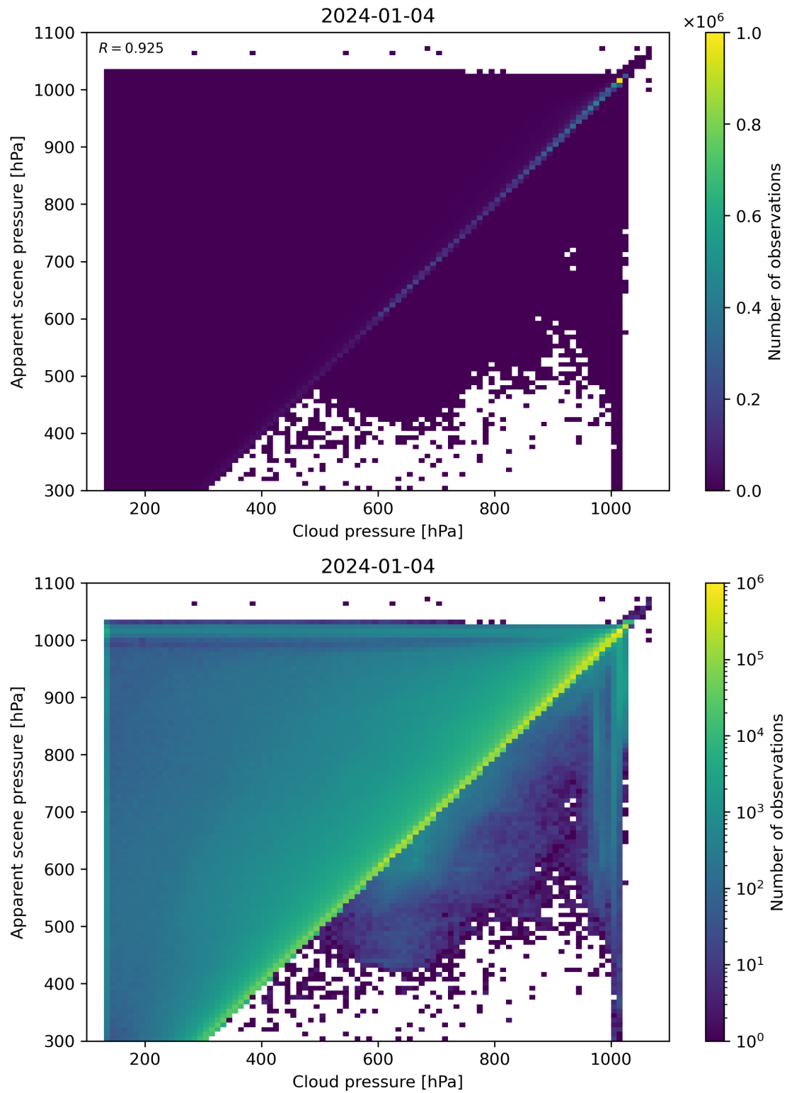
Figure 77: Scatter density plot of “Cloud pressure” against “Apparent scene pressure” for 2024-01-03 to 2024-01-05.
