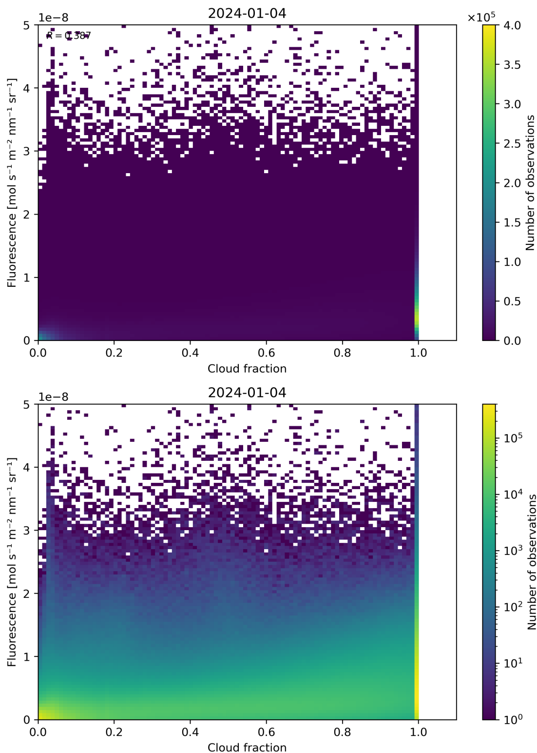
Figure 72: Scatter density plot of “Cloud fraction” against “Fluorescence” for 2024-01-03 to 2024-01-05.
