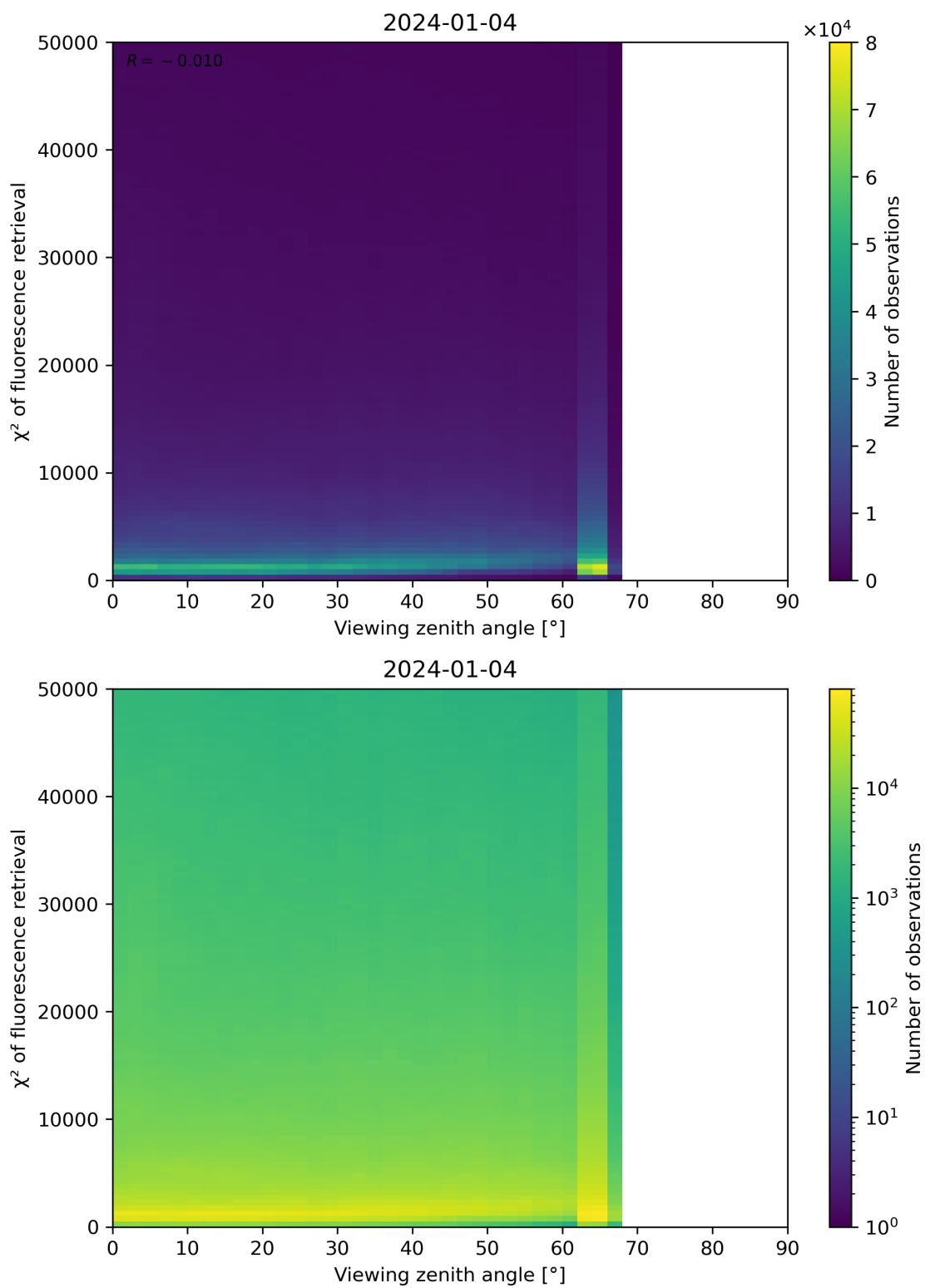
Figure 119: Scatter density plot of “Viewing zenith angle” against “ \chi^2 of fluorescence retrieval” for 2024-01-03 to 2024-01-05.
