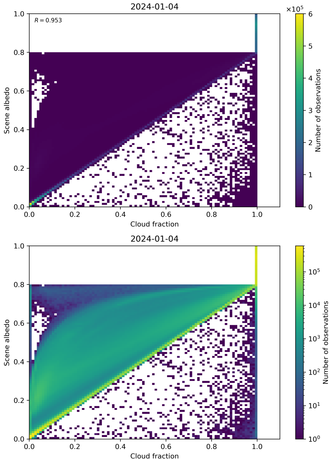
Figure 75: Scatter density plot of “Cloud fraction” against “Scene albedo” for 2024-01-03 to 2024-01-05.
