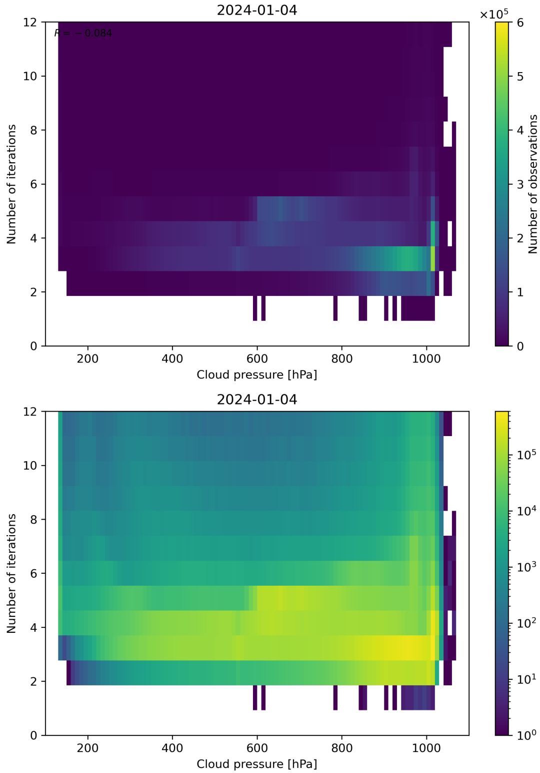
Figure 81: Scatter density plot of “Cloud pressure” against “Number of iterations” for 2024-01-03 to 2024-01-05.
