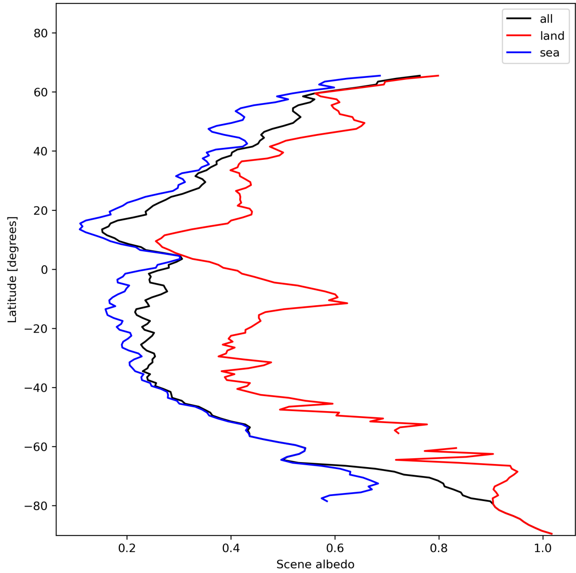
Figure 17: Zonal average of “Scene albedo” for 2024-01-03 to 2024-01-05.
