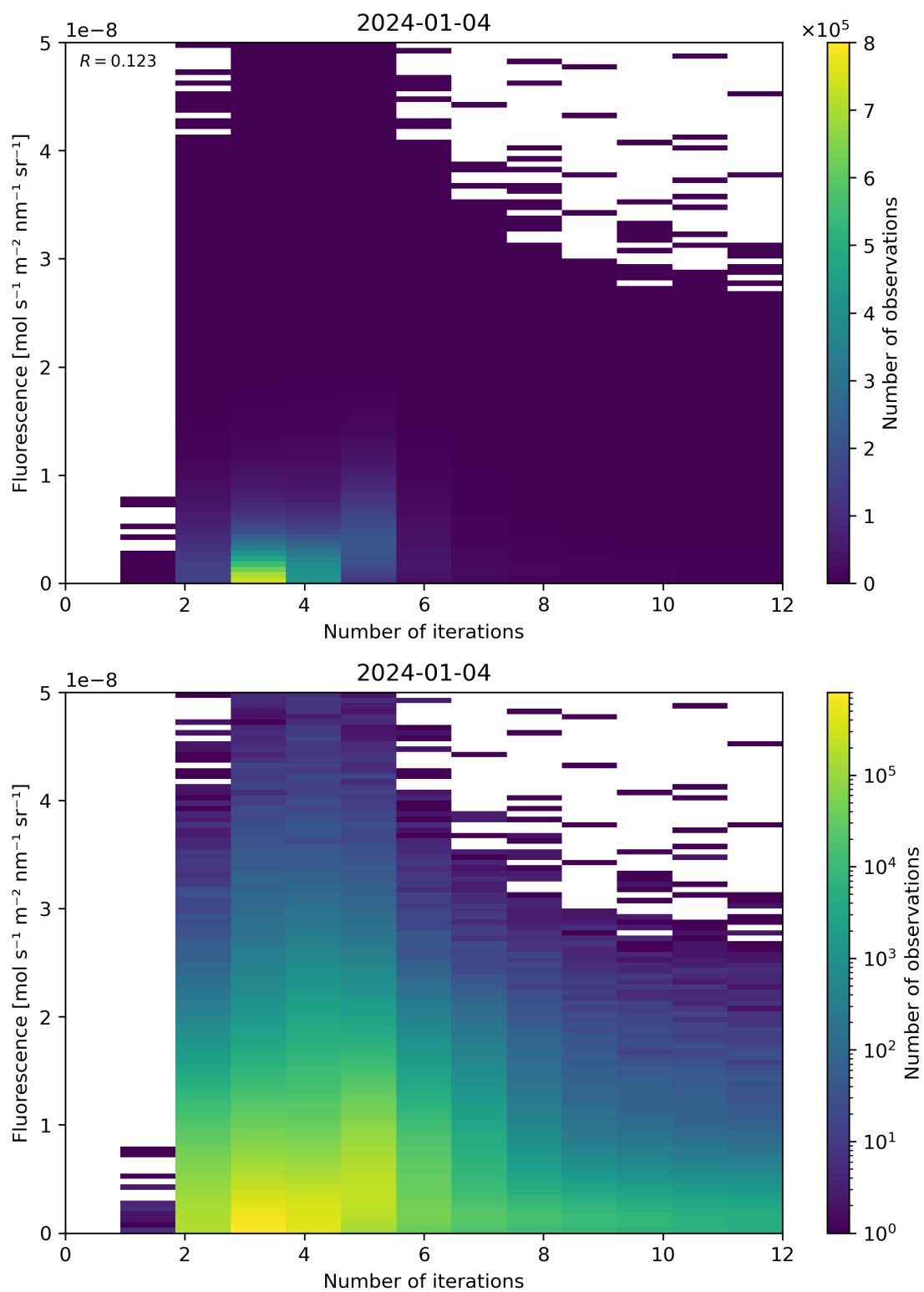
Figure 98: Scatter density plot of “Number of iterations” against “Fluorescence” for 2024-01-03 to 2024-01-05.
