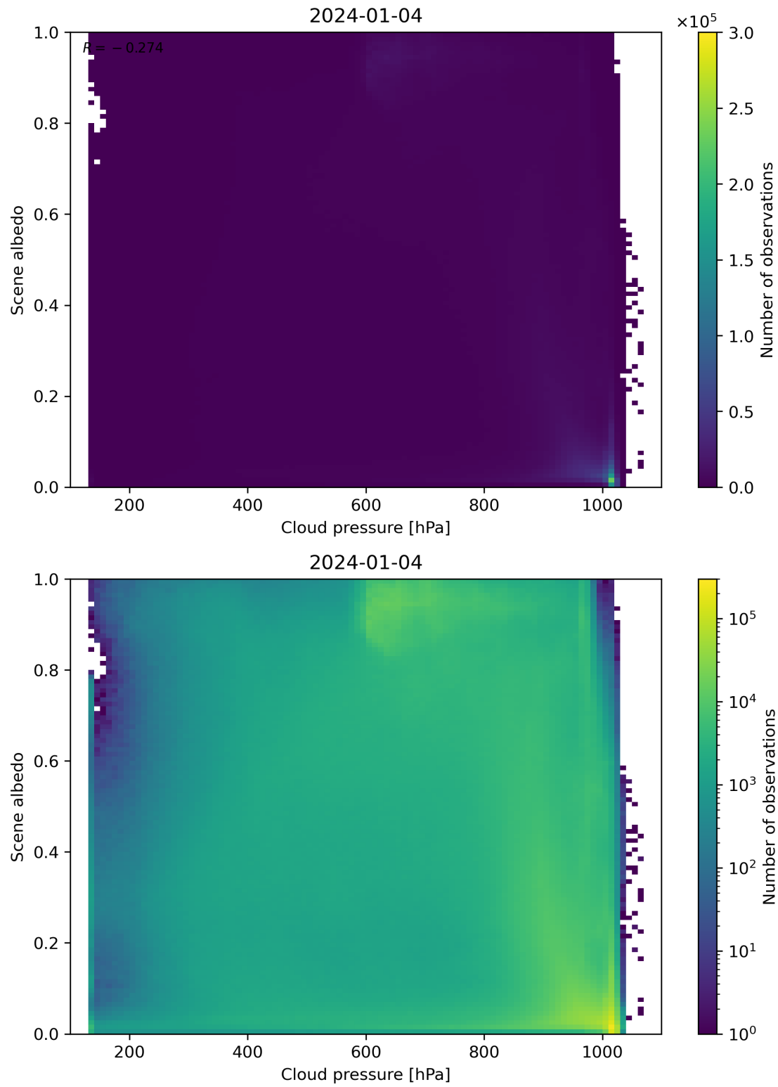
Figure 83: Scatter density plot of “Cloud pressure” against “Scene albedo” for 2024-01-03 to 2024-01-05.
