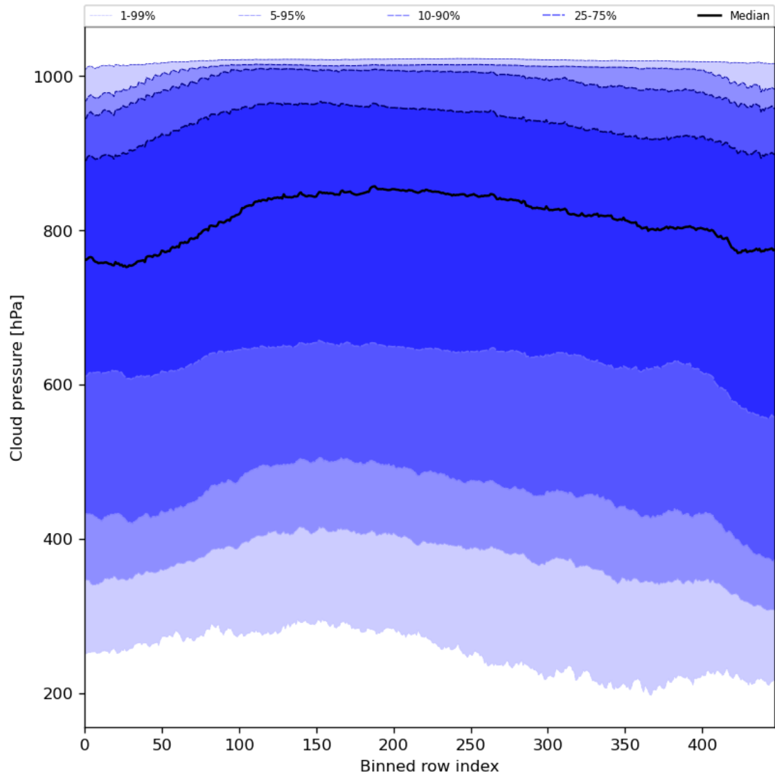
Figure 47: Along track statistics of “Cloud pressure” for 2024-01-03 to 2024-01-05
