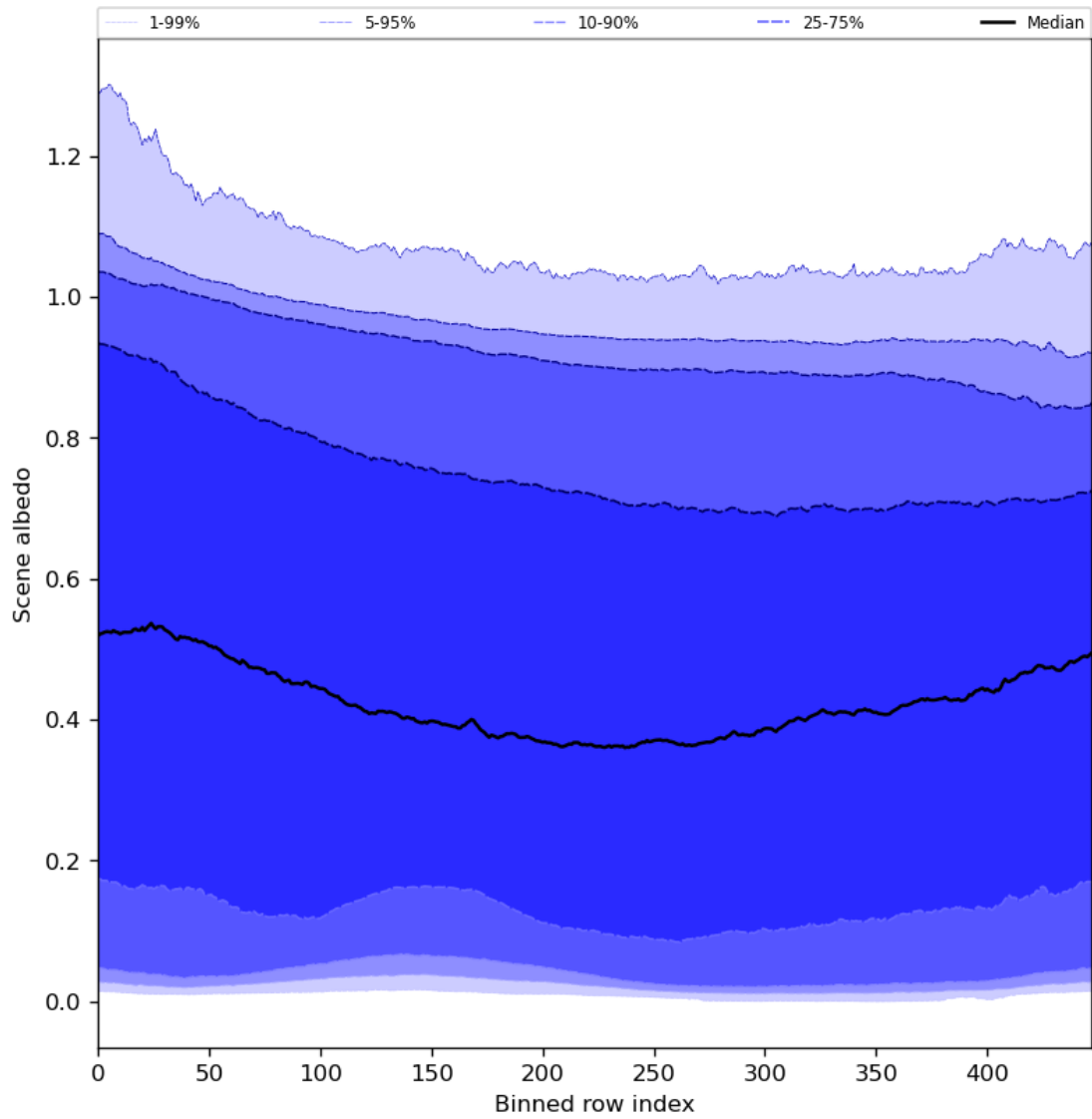
Figure 51: Along track statistics of “Scene albedo” for 2024-01-03 to 2024-01-05
