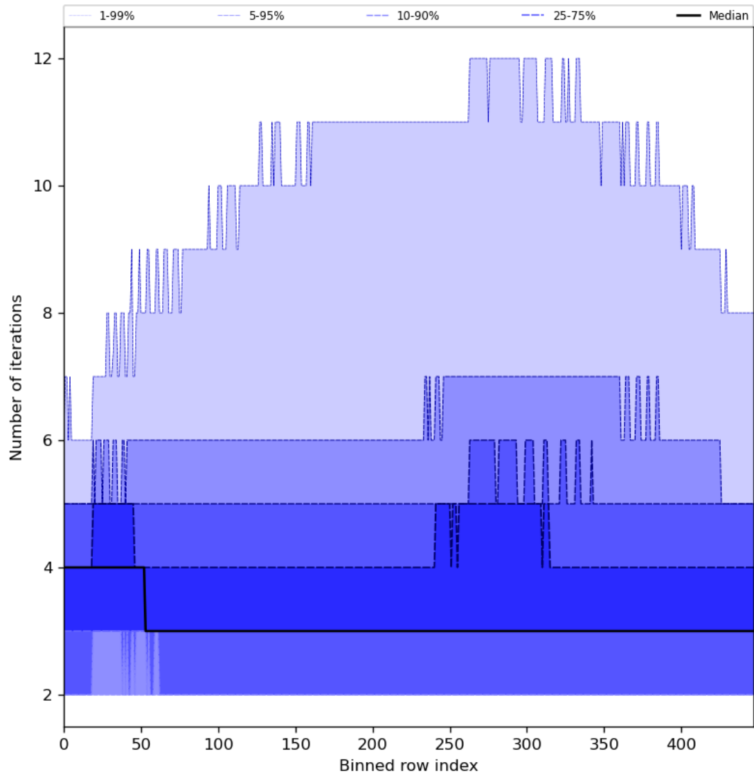
Figure 56: Along track statistics of “Number of iterations” for 2024-01-03 to 2024-01-05
