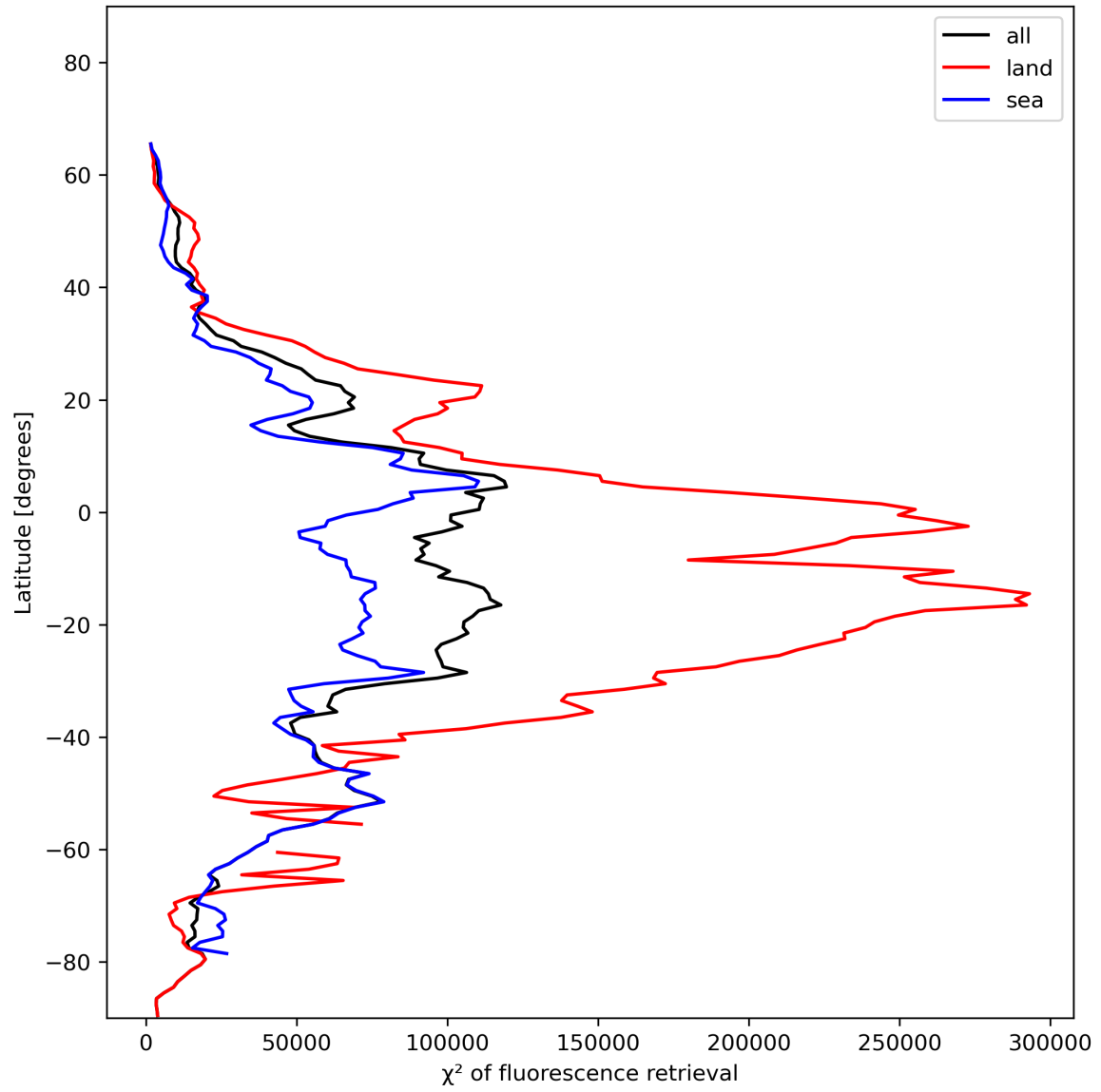
Figure 25: Zonal average of “ \chi^2 of fluorescence retrieval” for 2024-01-03 to 2024-01-05.
