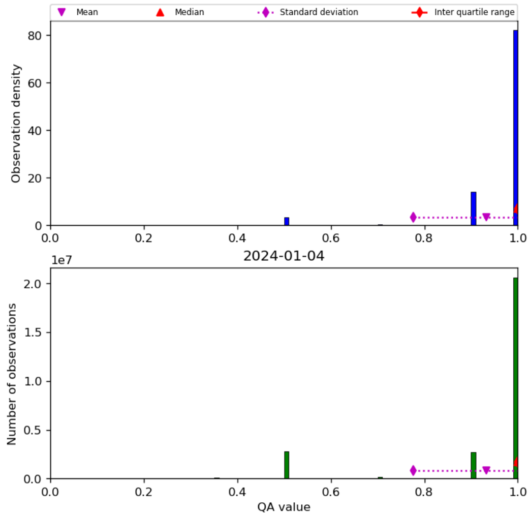
Figure 29: Histogram of “QA value” for 2024-01-03 to 2024-01-05
