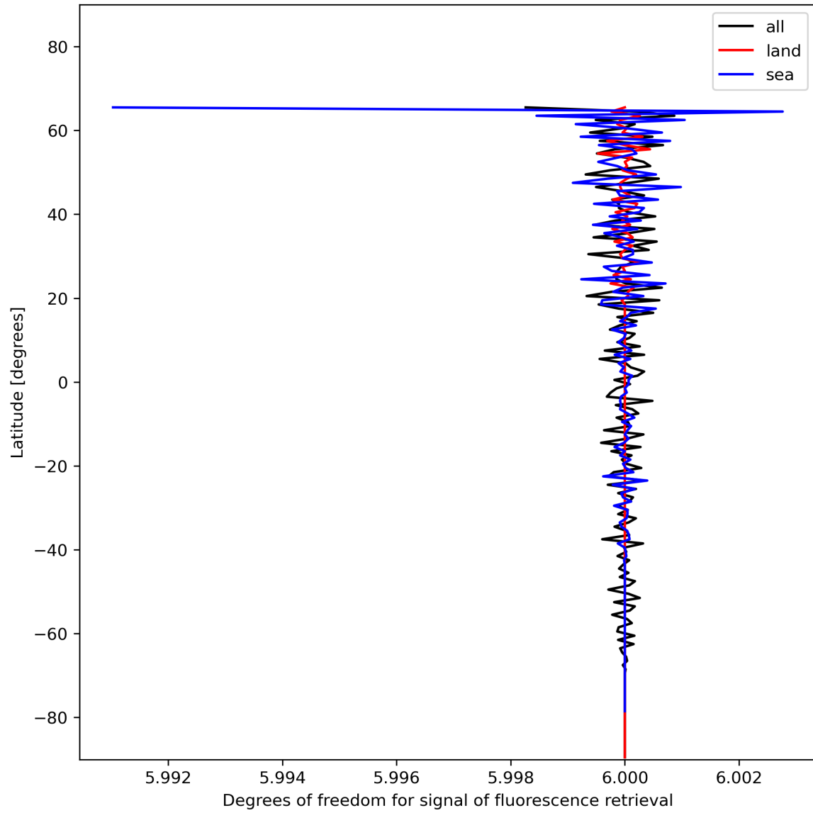
Figure 26: Zonal average of “Degrees of freedom for signal of fluorescence retrieval” for 2024-01-03 to 2024-01-05.
