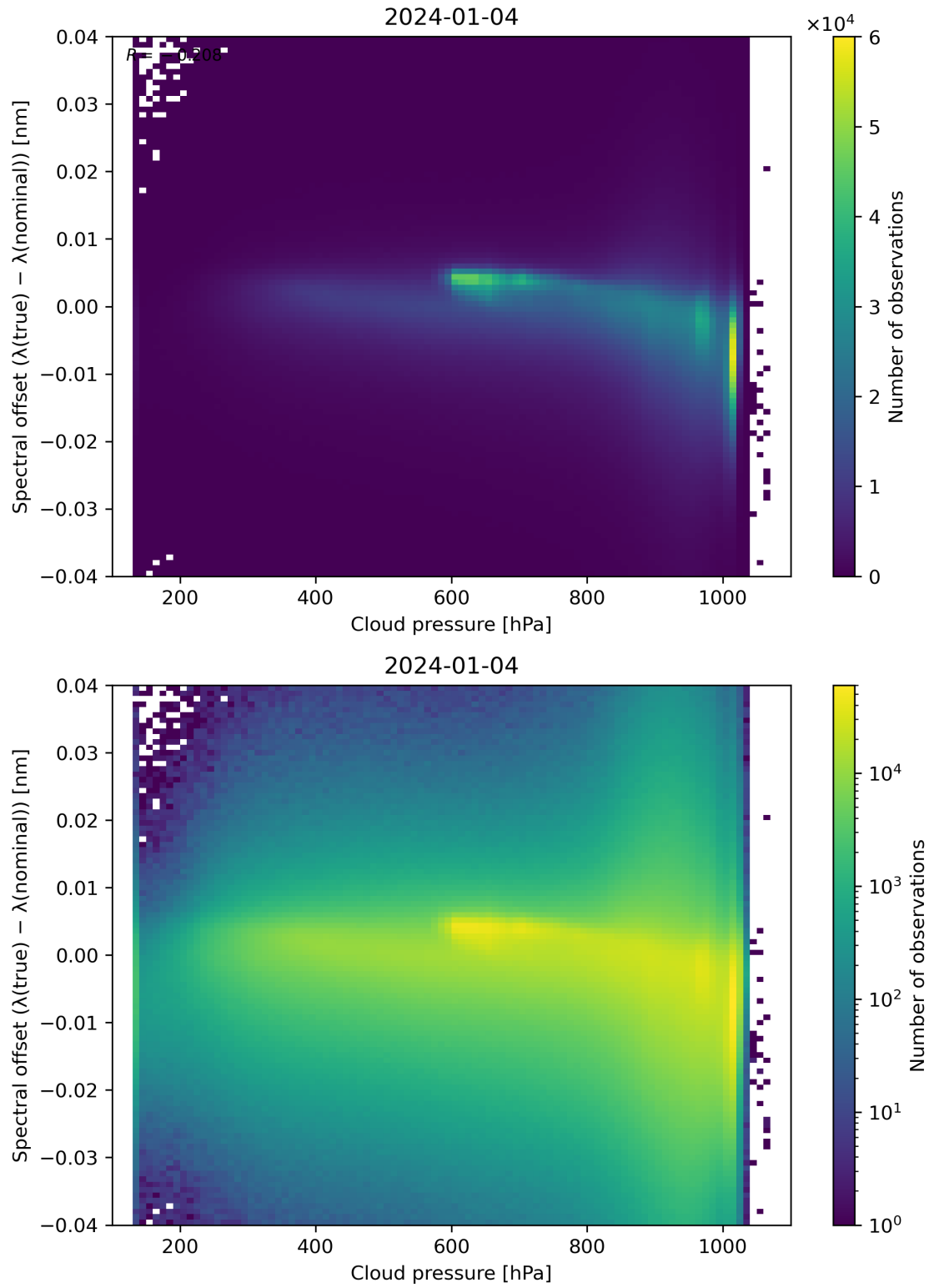
Figure 84: Scatter density plot of “Cloud pressure” against “Spectral offset ( \lambda(\text{true}) - \lambda(\text{nominal}) )” for 2024-01-03 to 2024-01-05.
