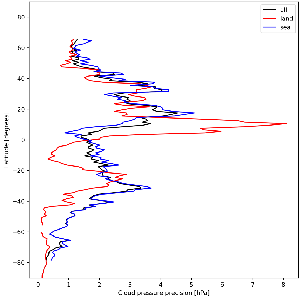
Figure 14: Zonal average of “Cloud pressure precision” for 2024-01-03 to 2024-01-05.
