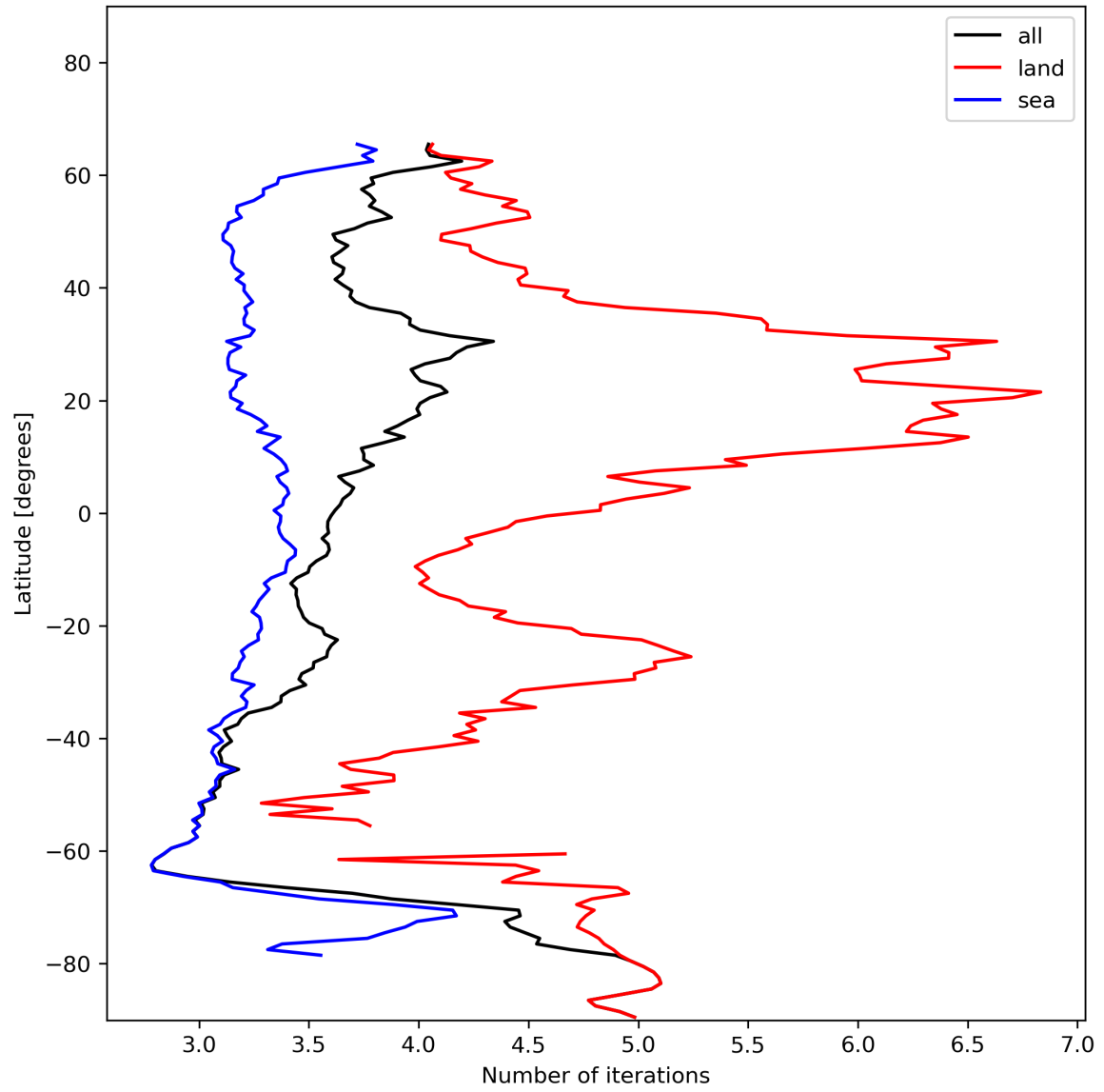
Figure 22: Zonal average of “Number of iterations” for 2024-01-03 to 2024-01-05.
