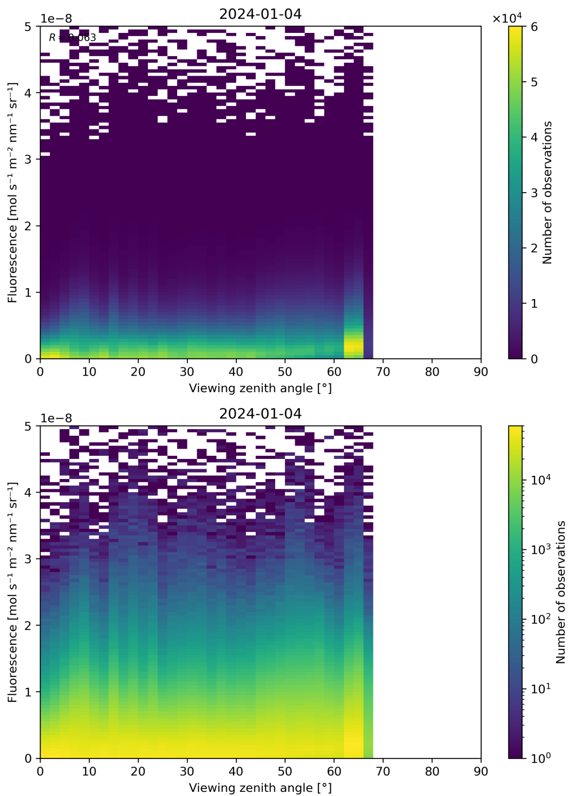
Figure 122: Scatter density plot of “Viewing zenith angle” against “Fluorescence” for 2024-01-03 to 2024-01-05.
