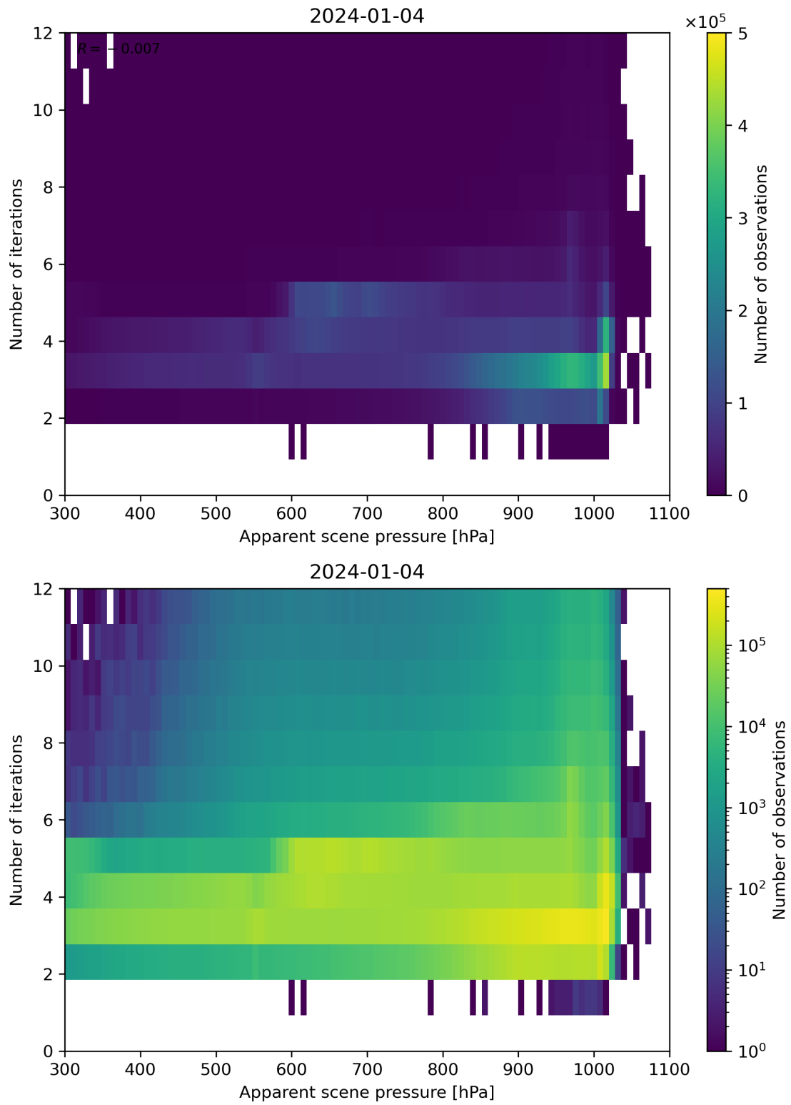
Figure 65: Scatter density plot of “Apparent scene pressure” against “Number of iterations” for 2024-01-03 to 2024-01-05.
