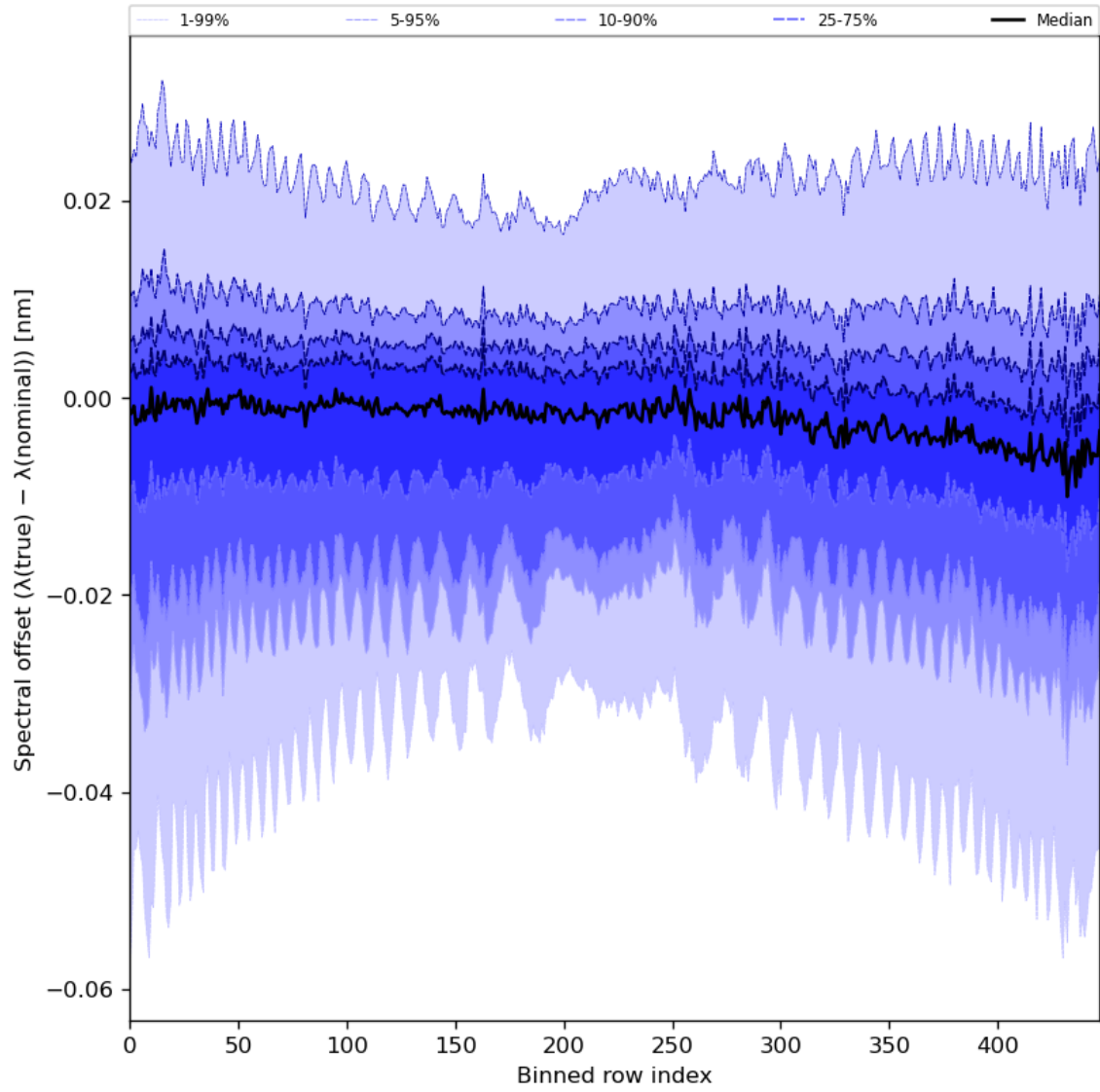
Figure 62: Along track statistics of “Spectral offset ( \lambda(\text{true}) - \lambda(\text{nominal}) )” for 2024-01-03 to 2024-01-05
