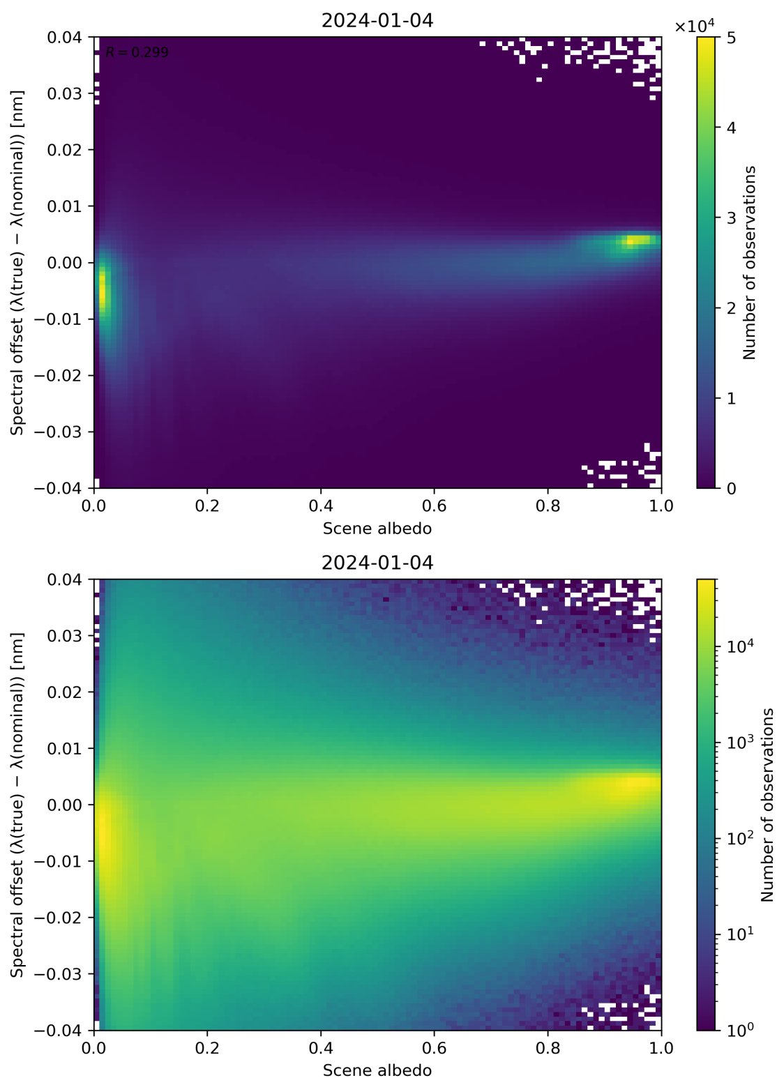
Figure 107: Scatter density plot of “Scene albedo” against “Spectral offset ( \lambda(\text{true}) - \lambda(\text{nominal}) )” for 2024-01-03 to 2024-01-05.
