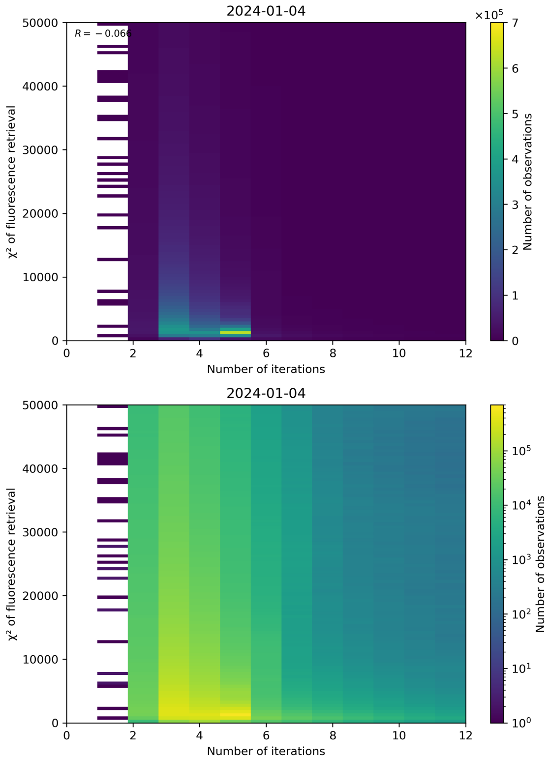
Figure 97: Scatter density plot of “Number of iterations” against “ \chi^2 of fluorescence retrieval” for 2024-01-03 to 2024-01-05.
