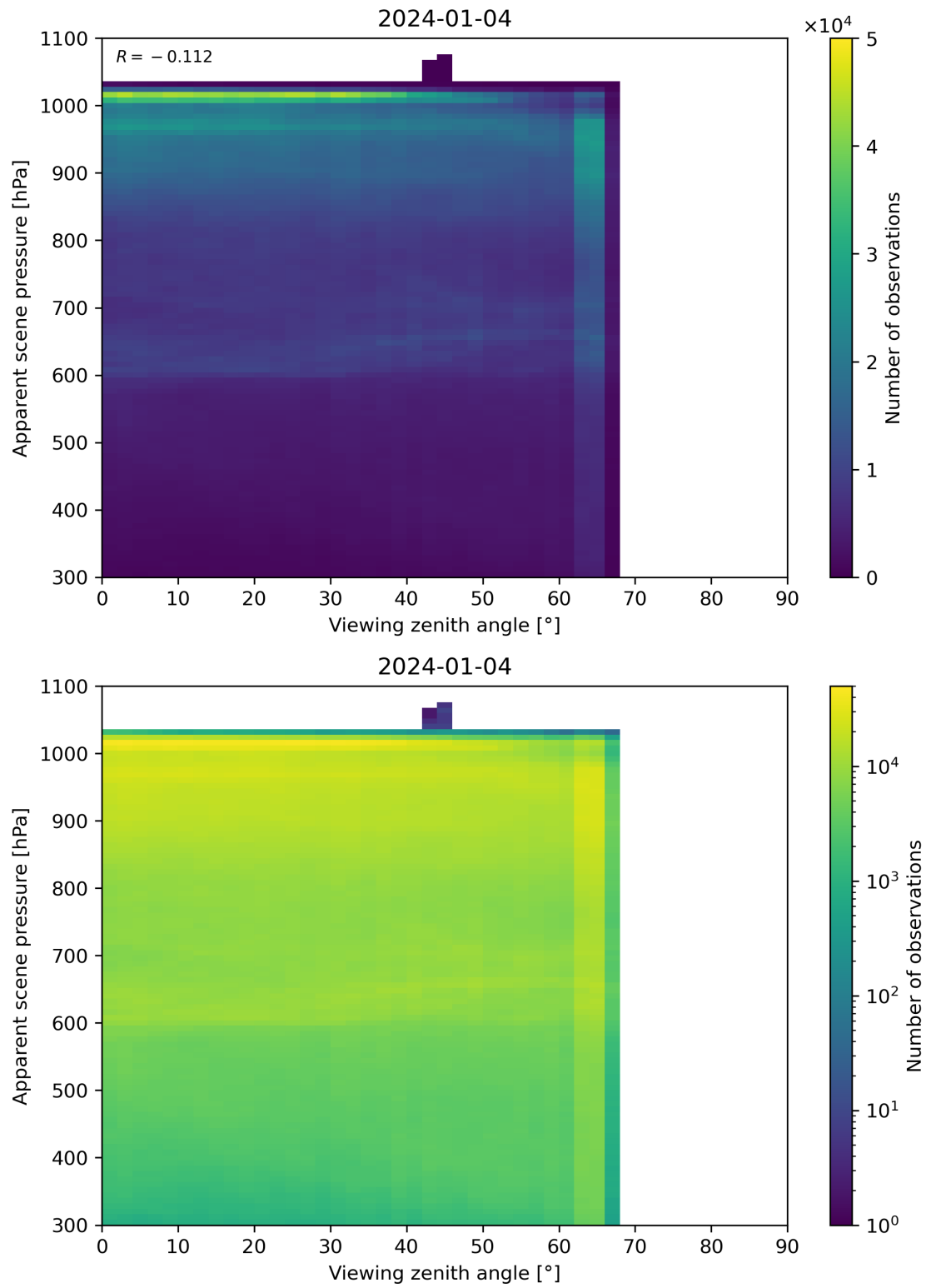
Figure 118: Scatter density plot of “Viewing zenith angle” against “Apparent scene pressure” for 2024-01-03 to 2024-01-05.
