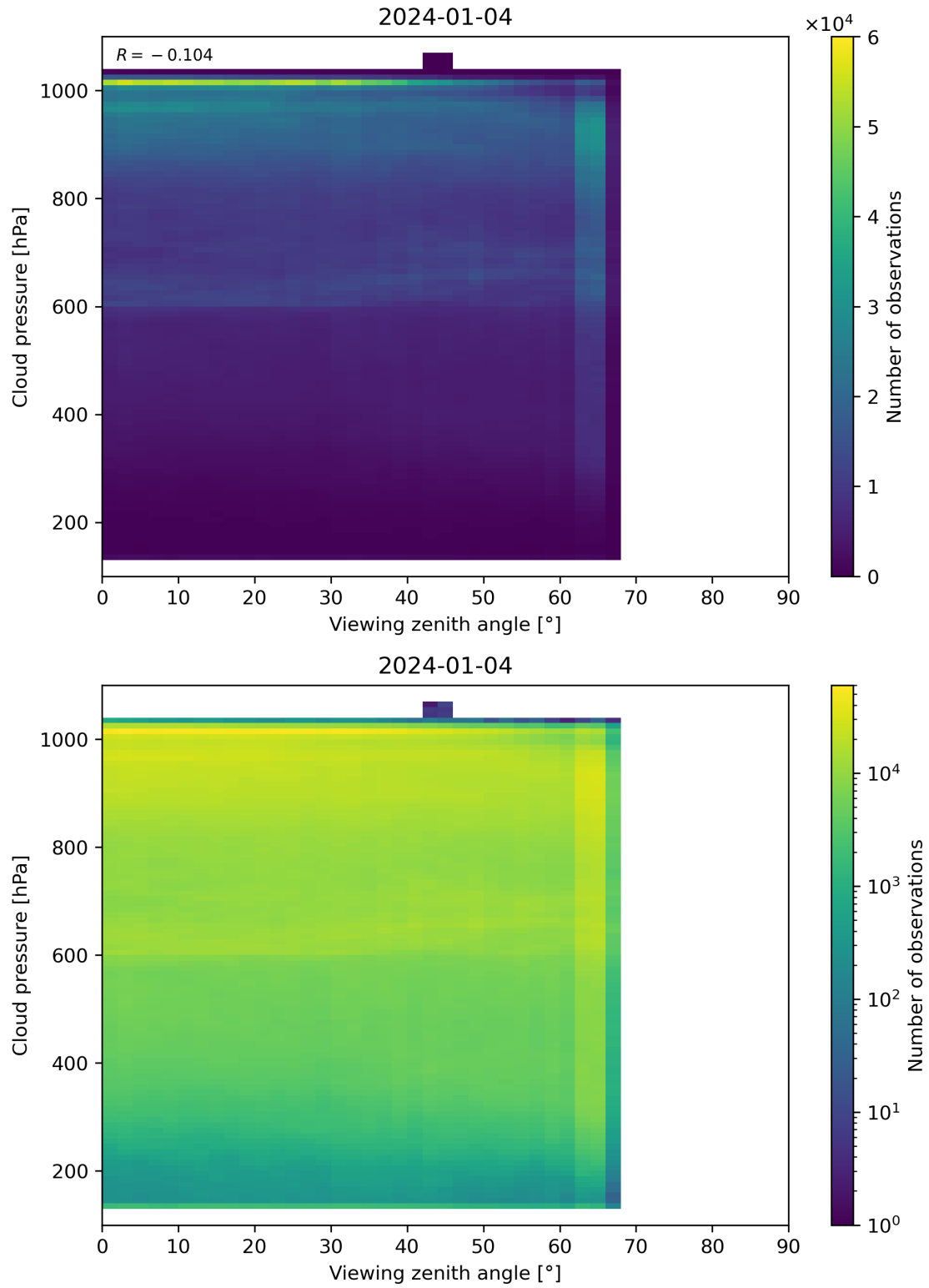
Figure 121: Scatter density plot of “Viewing zenith angle” against “Cloud pressure” for 2024-01-03 to 2024-01-05.
