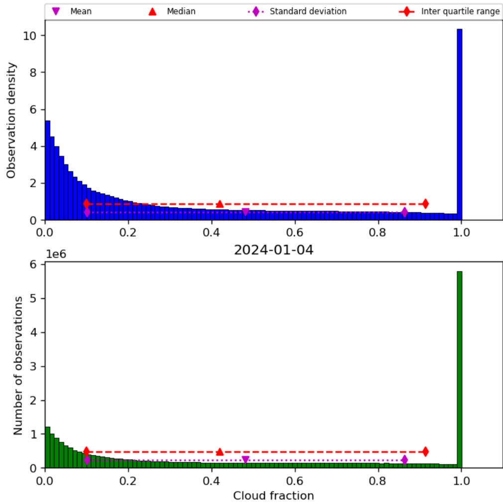
Figure 32: Histogram of “Cloud fraction” for 2024-01-03 to 2024-01-05
