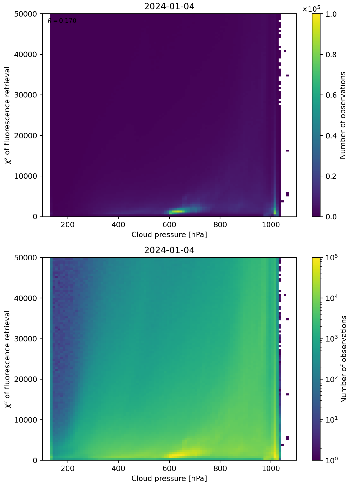
Figure 78: Scatter density plot of “Cloud pressure” against “ \chi^2 of fluorescence retrieval” for 2024-01-03 to 2024-01-05.
