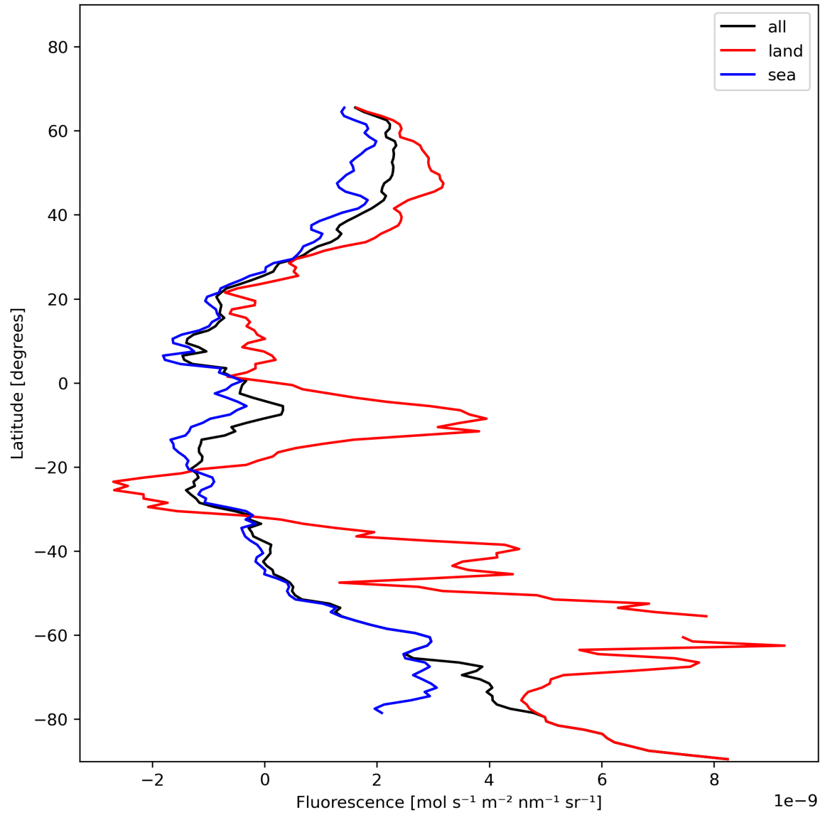
Figure 23: Zonal average of “Fluorescence” for 2024-01-03 to 2024-01-05.
