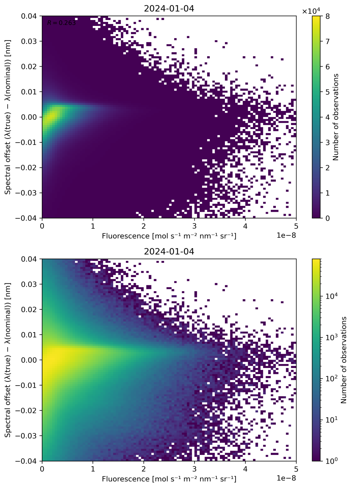
Figure 87: Scatter density plot of “Fluorescence” against “Spectral offset ( \lambda(\text{true}) - \lambda(\text{nominal}) )” for 2024-01-03 to 2024-01-05.
