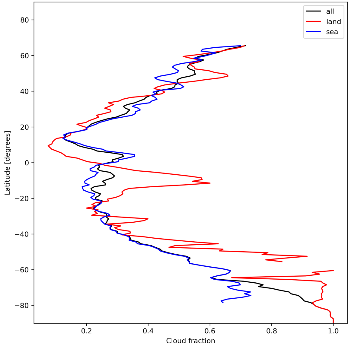
Figure 15: Zonal average of “Cloud fraction” for 2024-01-03 to 2024-01-05.
