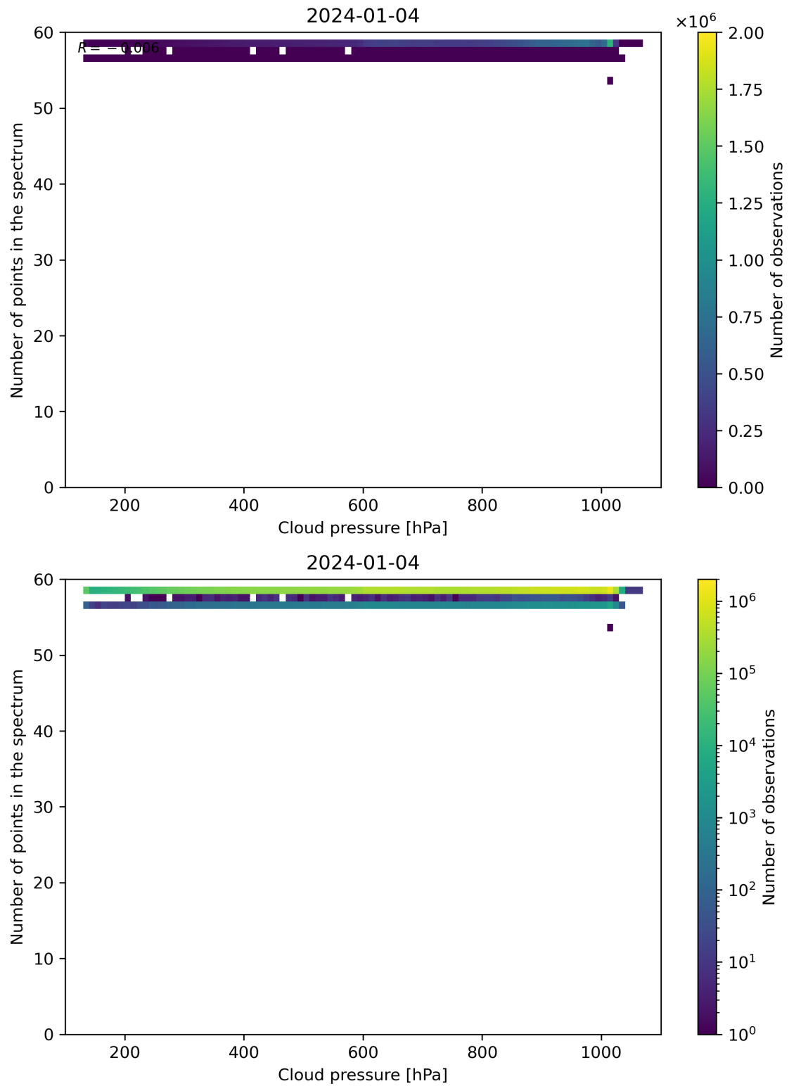
Figure 82: Scatter density plot of “Cloud pressure” against “Number of points in the spectrum” for 2024-01-03 to 2024-01-05.
