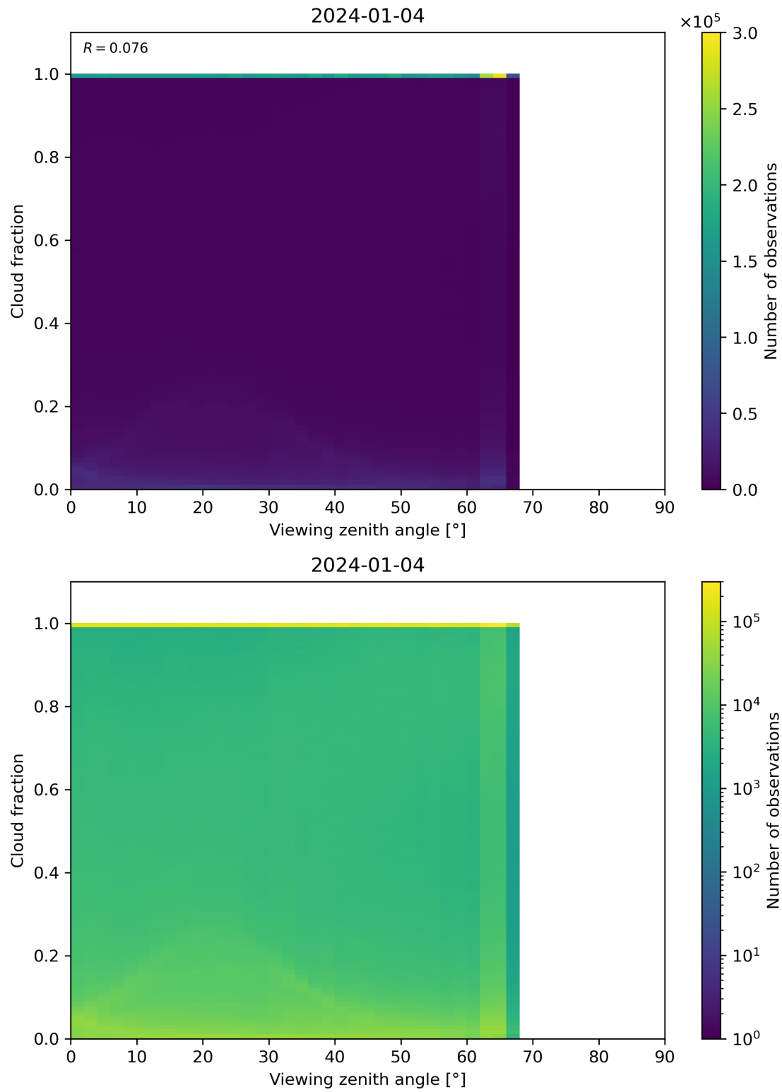
Figure 120: Scatter density plot of “Viewing zenith angle” against “Cloud fraction” for 2024-01-03 to 2024-01-05.
