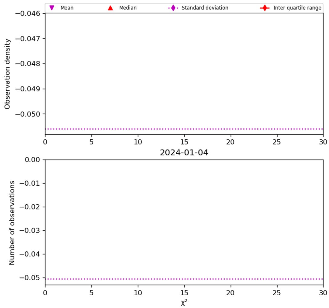
Figure 38: Histogram of “ \chi^2 ” for 2024-01-03 to 2024-01-05
