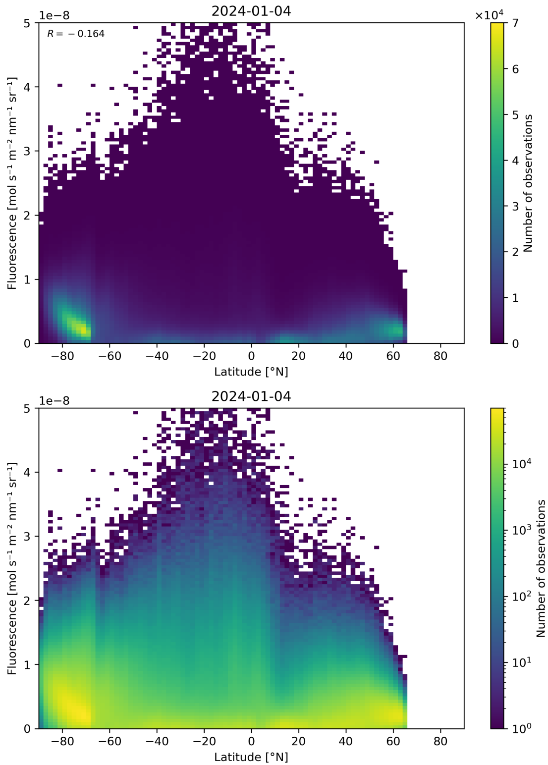
Figure 92: Scatter density plot of “Latitude” against “Fluorescence” for 2024-01-03 to 2024-01-05.
