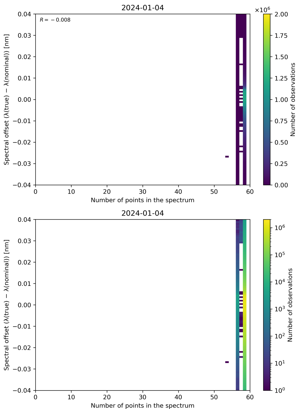
Figure 101: Scatter density plot of “Number of points in the spectrum” against “Spectral offset ( \lambda(\text{true}) - \lambda(\text{nominal}) )” for 2024-01-03 to 2024-01-05.
