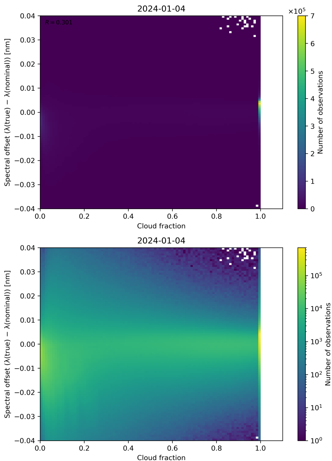
Figure 76: Scatter density plot of “Cloud fraction” against “Spectral offset ( \lambda(\text{true}) - \lambda(\text{nominal}) )” for 2024-01-03 to 2024-01-05.
