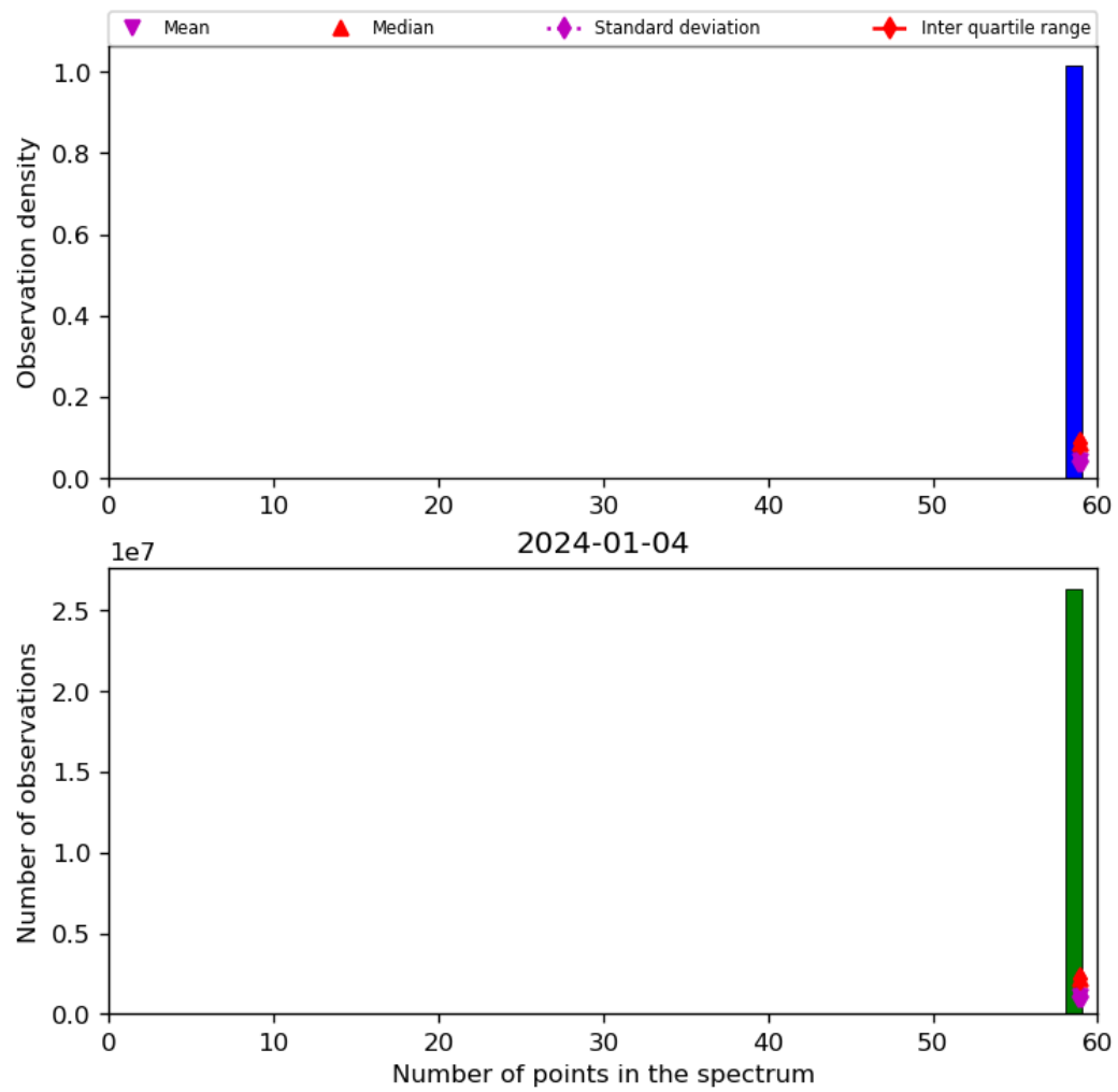
Figure 44: Histogram of “Number of points in the spectrum” for 2024-01-03 to 2024-01-05
