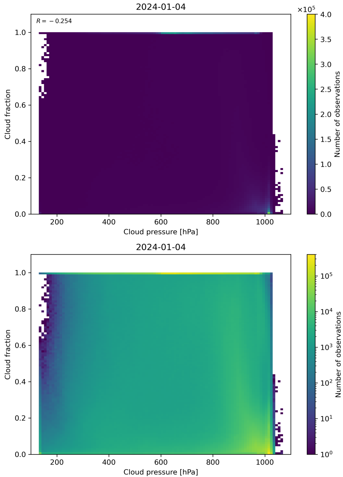
Figure 79: Scatter density plot of “Cloud pressure” against “Cloud fraction” for 2024-01-03 to 2024-01-05.
