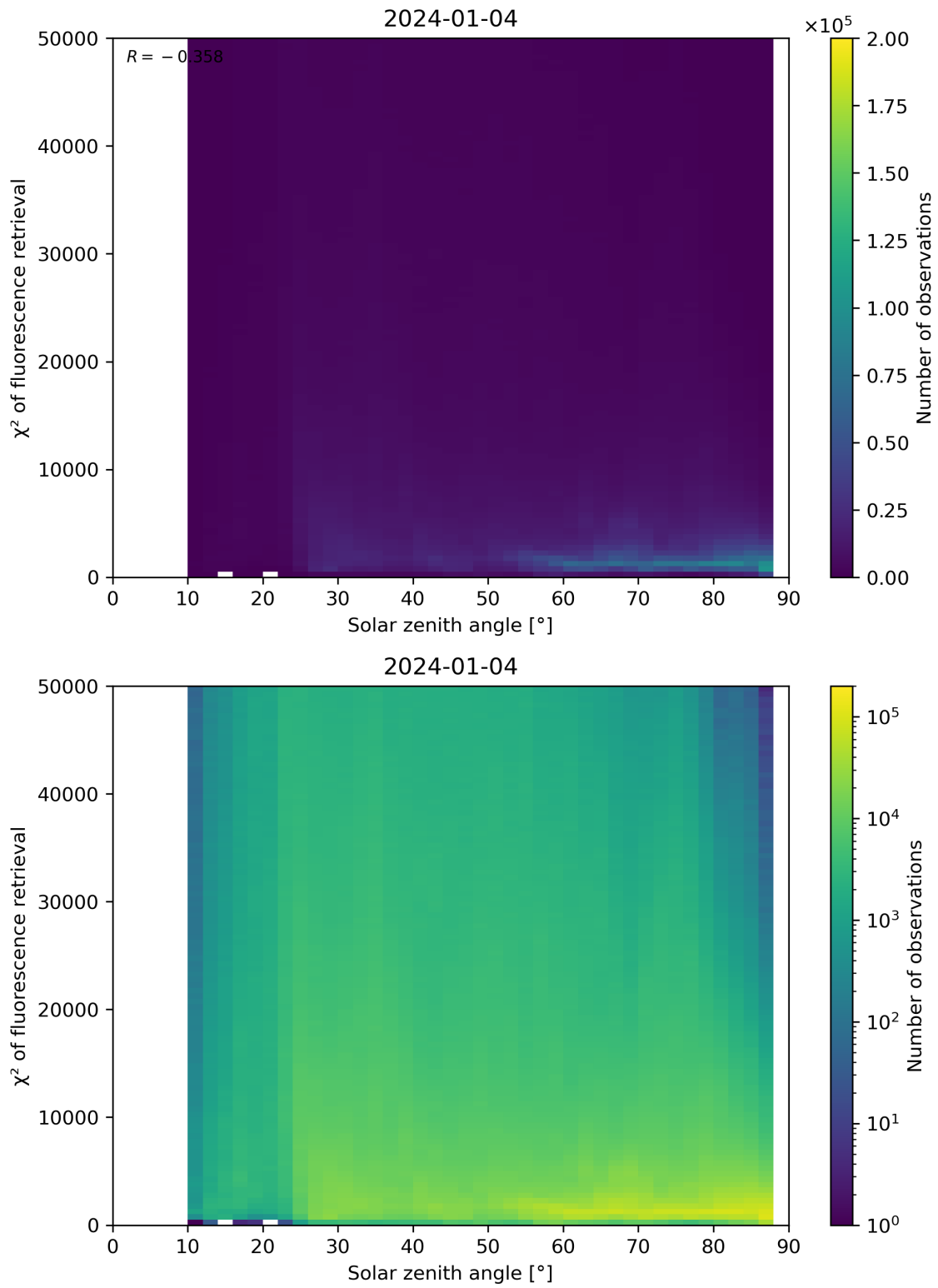
Figure 109: Scatter density plot of “Solar zenith angle” against “ \chi^2 of fluorescence retrieval” for 2024-01-03 to 2024-01-05.
