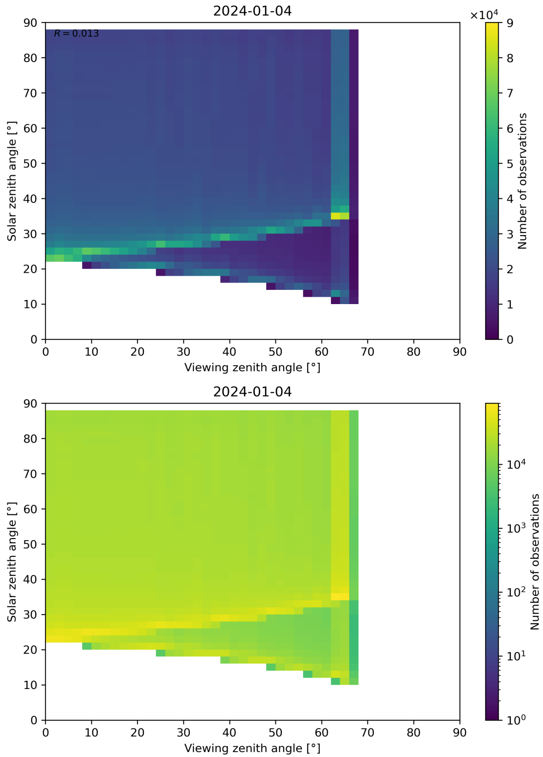
Figure 127: Scatter density plot of “Viewing zenith angle” against “Solar zenith angle” for 2024-01-03 to 2024-01-05.
