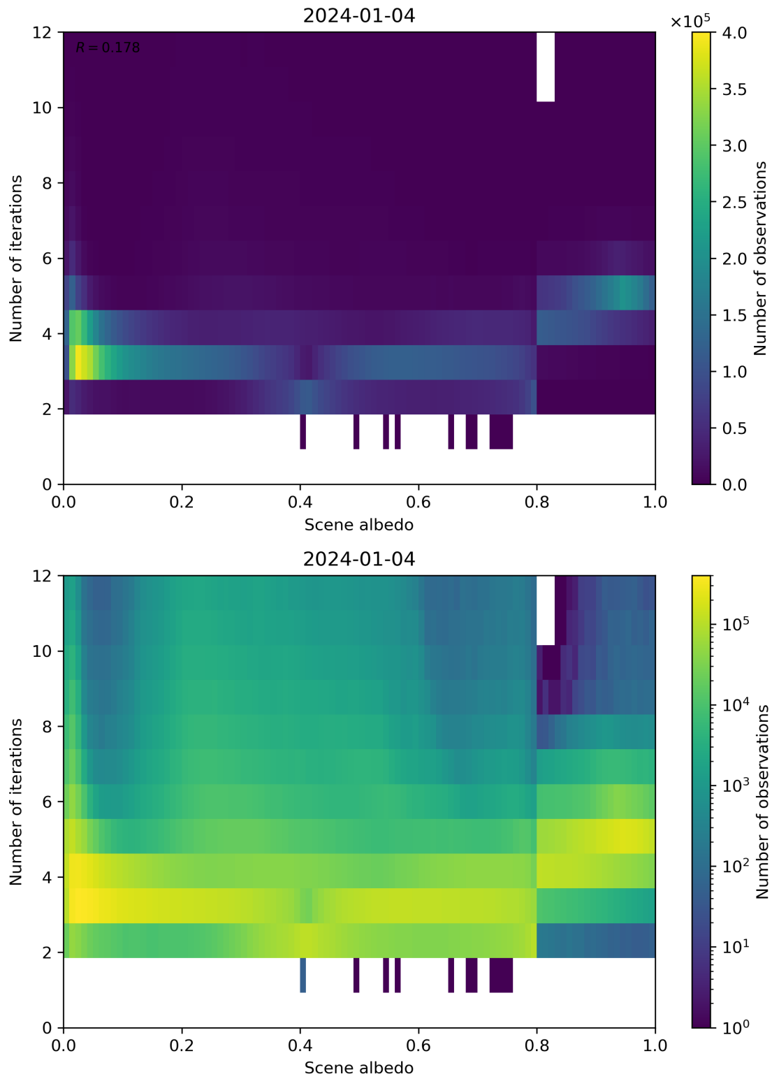
Figure 105: Scatter density plot of “Scene albedo” against “Number of iterations” for 2024-01-03 to 2024-01-05.
