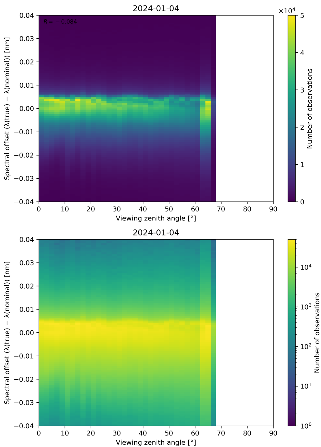
Figure 128: Scatter density plot of “Viewing zenith angle” against “Spectral offset ( \lambda(\text{true}) - \lambda(\text{nominal}) )” for 2024-01-03 to 2024-01-05.
