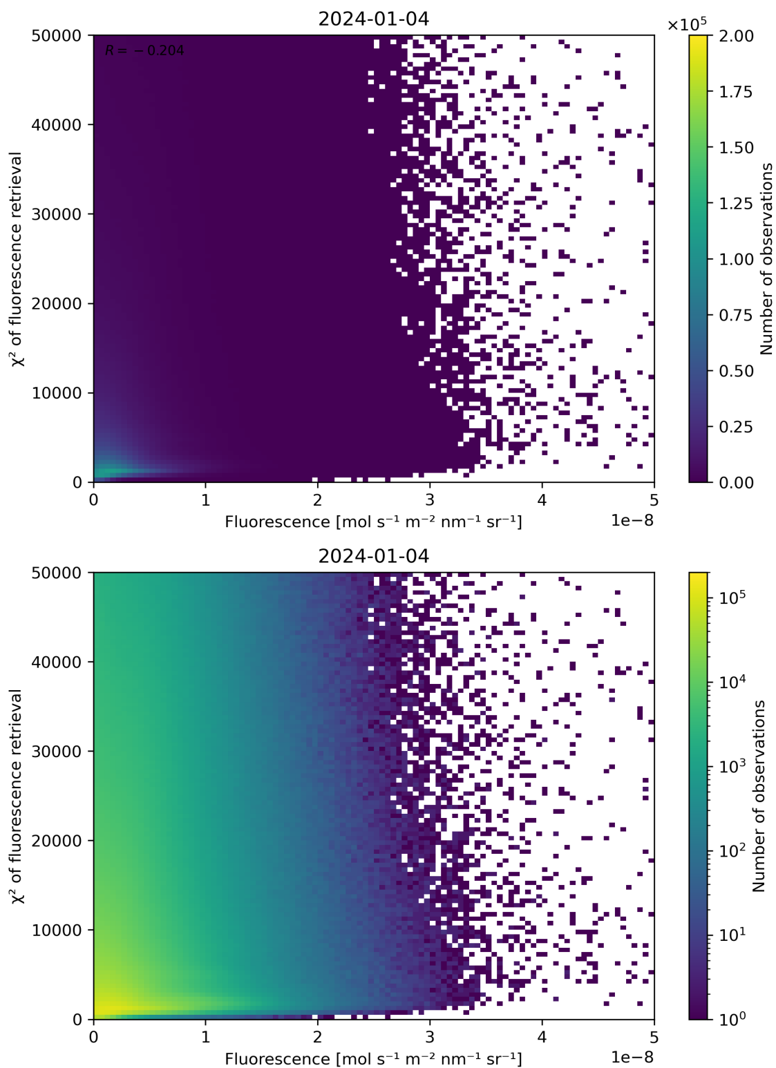
Figure 85: Scatter density plot of “Fluorescence” against “ \chi^2 of fluorescence retrieval” for 2024-01-03 to 2024-01-05.
