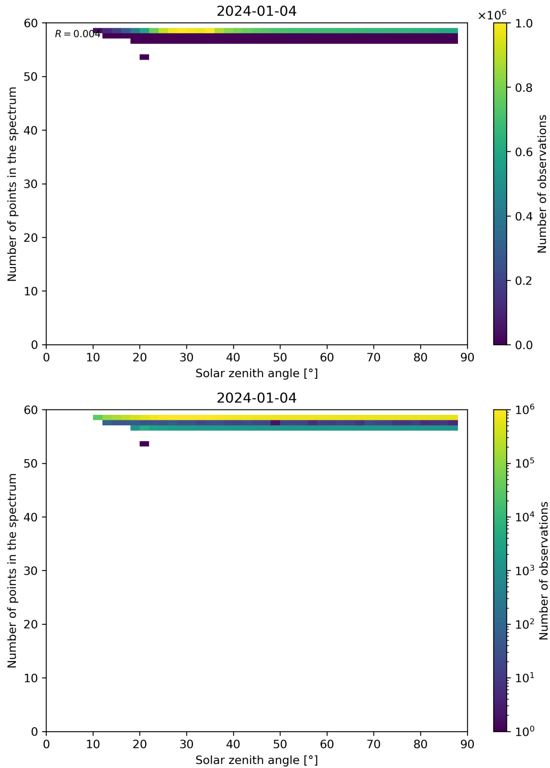
Figure 115: Scatter density plot of “Solar zenith angle” against “Number of points in the spectrum” for 2024-01-03 to 2024-01-05.
