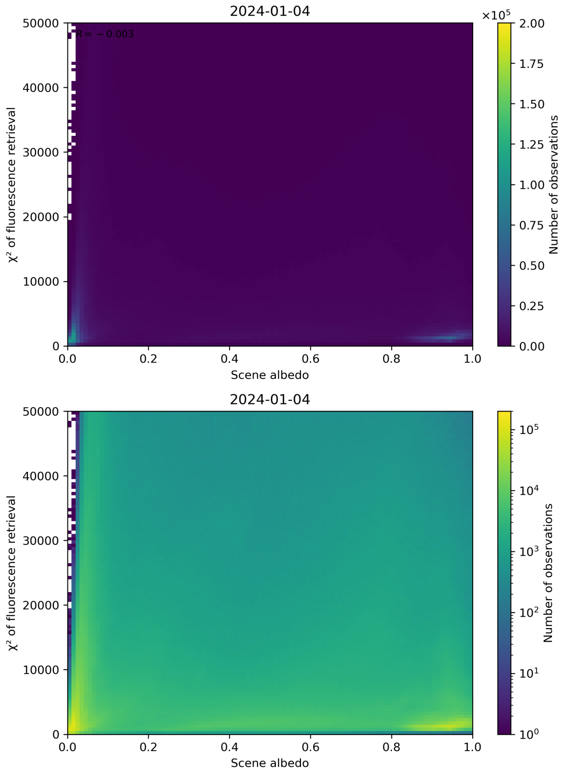
Figure 103: Scatter density plot of “Scene albedo” against “ \chi^2 of fluorescence retrieval” for 2024-01-03 to 2024-01-05.
