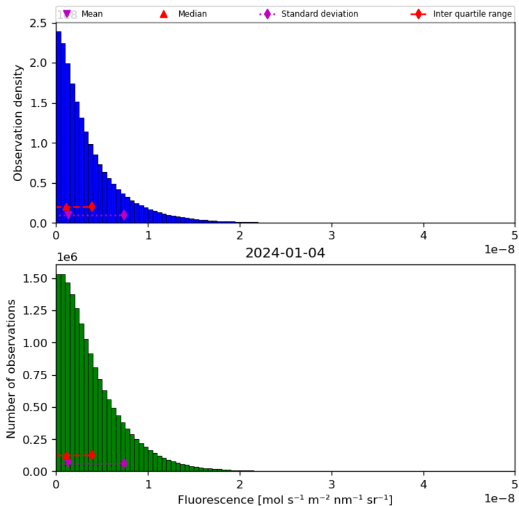
Figure 40: Histogram of “Fluorescence” for 2024-01-03 to 2024-01-05
