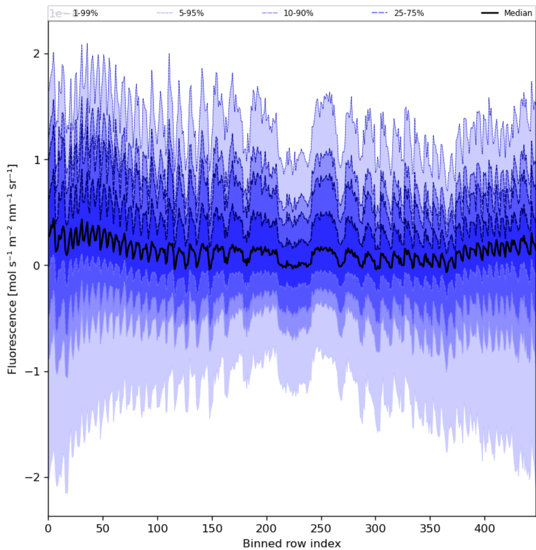
Figure 57: Along track statistics of “Fluorescence” for 2024-01-03 to 2024-01-05
