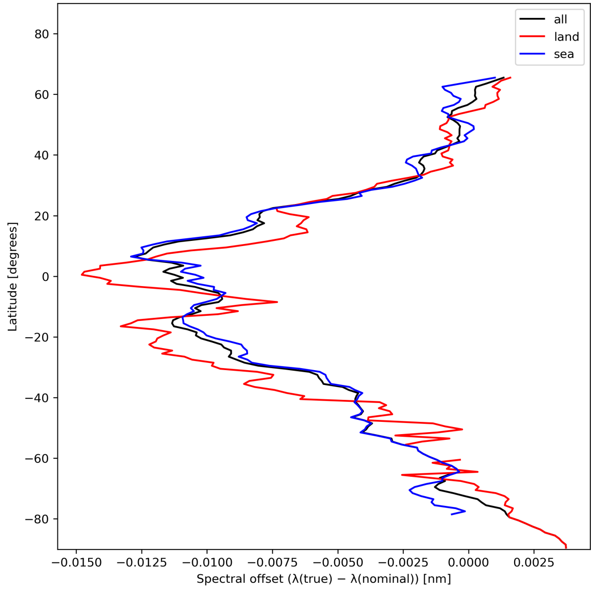
Figure 28: Zonal average of “Spectral offset ( \lambda(\text{true}) - \lambda(\text{nominal}) )” for 2024-01-03 to 2024-01-05.
