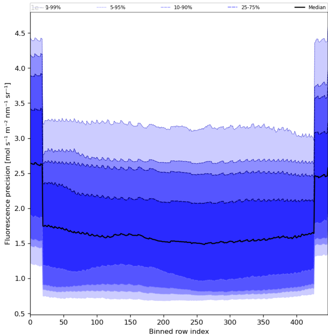
Figure 58: Along track statistics of “Fluorescence precision” for 2024-01-03 to 2024-01-05
