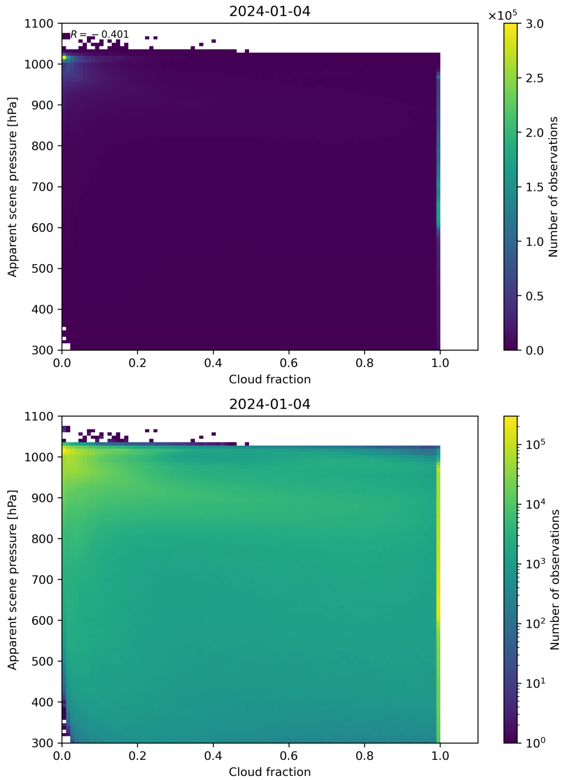
Figure 70: Scatter density plot of “Cloud fraction” against “Apparent scene pressure” for 2024-01-03 to 2024-01-05.
