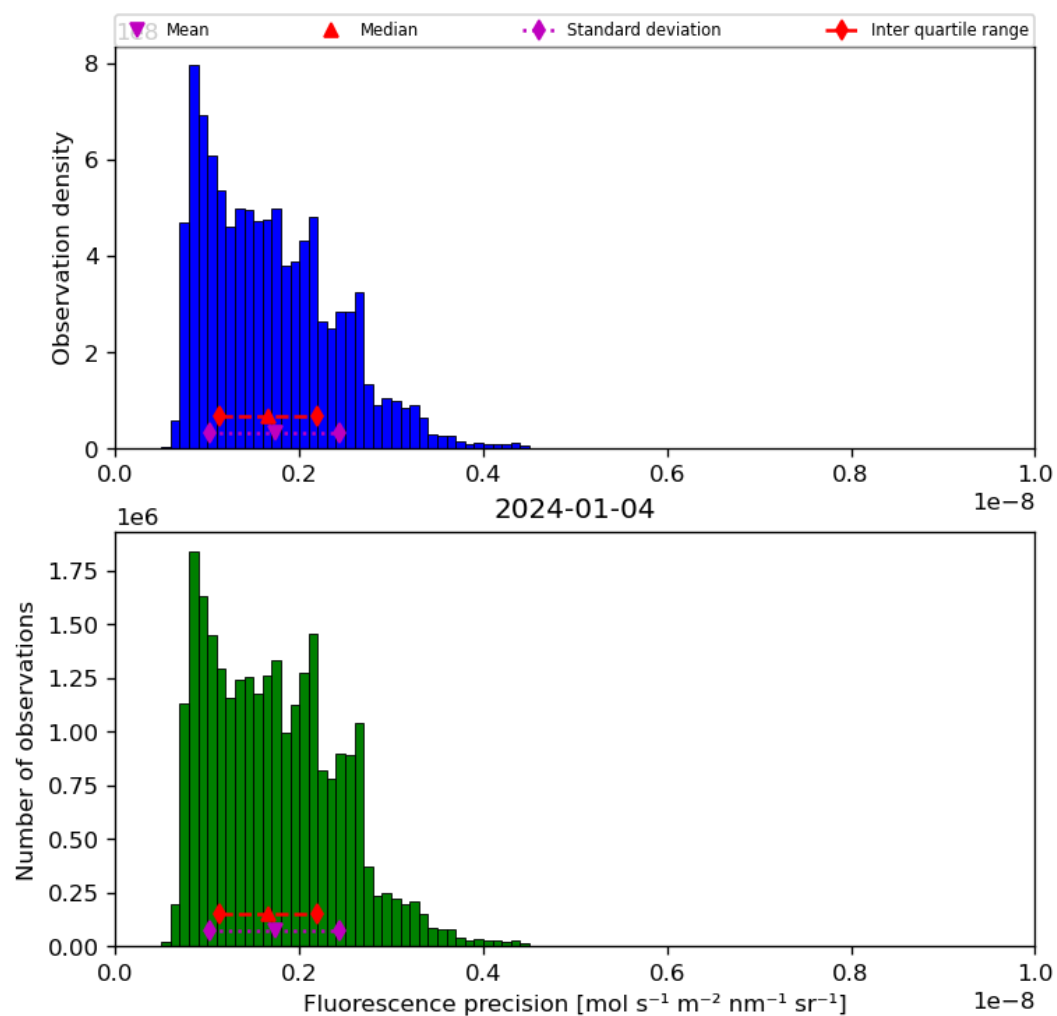
Figure 41: Histogram of “Fluorescence precision” for 2024-01-03 to 2024-01-05
