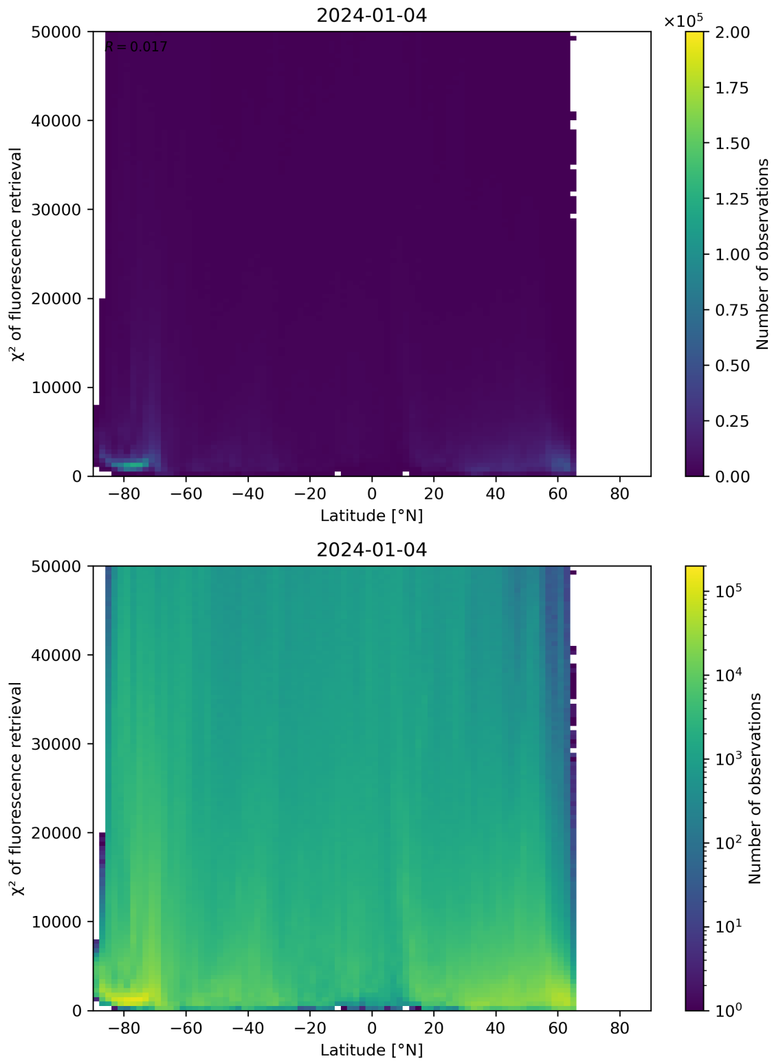
Figure 89: Scatter density plot of “Latitude” against “ \chi^2 of fluorescence retrieval” for 2024-01-03 to 2024-01-05.
