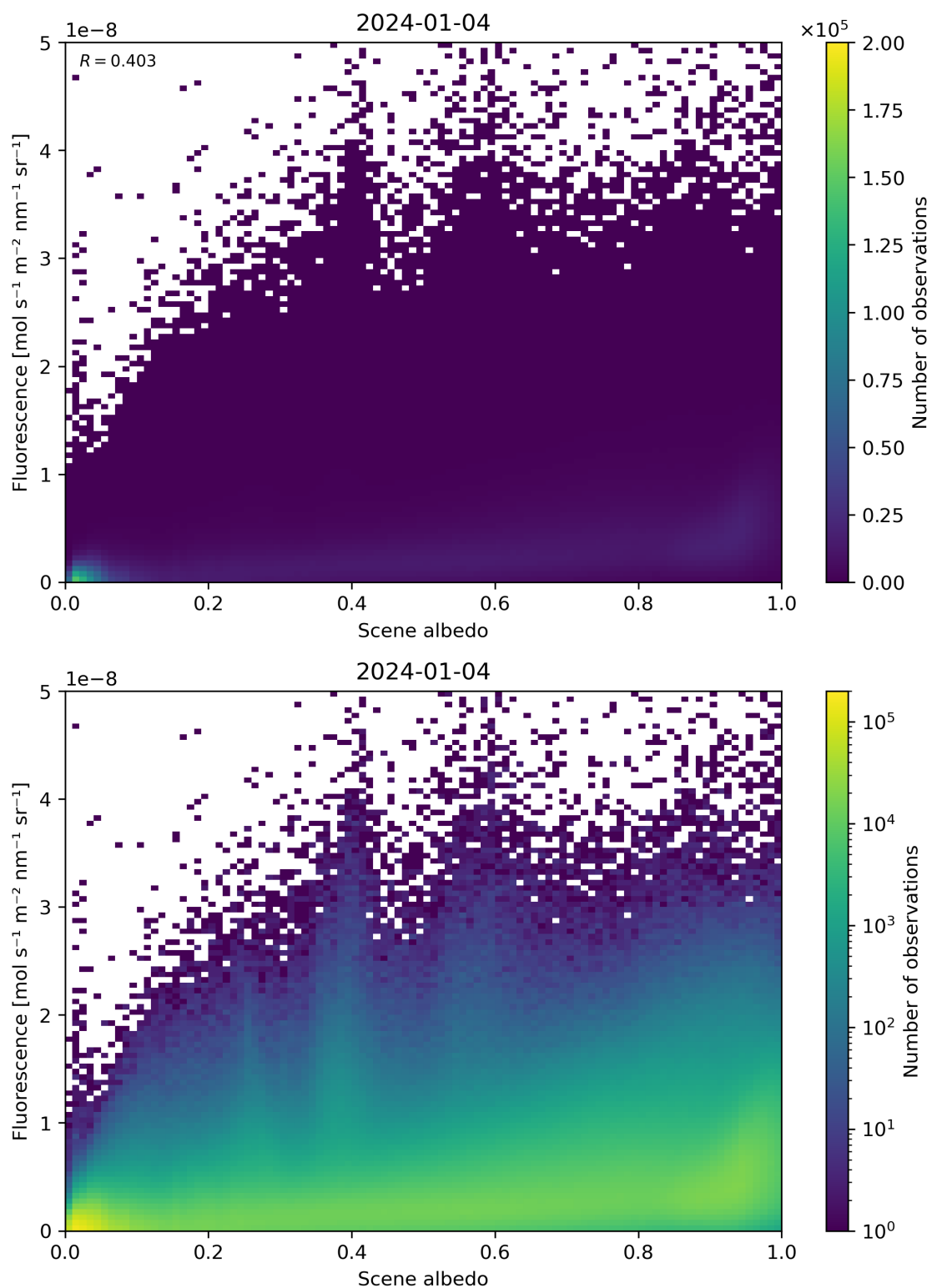
Figure 104: Scatter density plot of “Scene albedo” against “Fluorescence” for 2024-01-03 to 2024-01-05.
