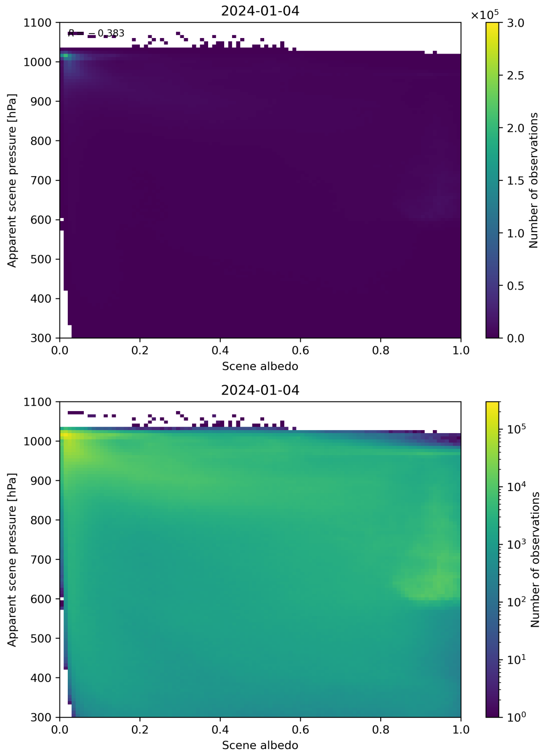
Figure 102: Scatter density plot of “Scene albedo” against “Apparent scene pressure” for 2024-01-03 to 2024-01-05.
