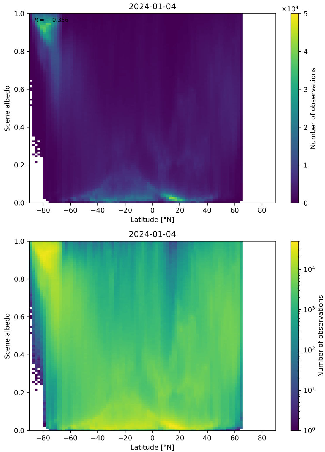
Figure 95: Scatter density plot of “Latitude” against “Scene albedo” for 2024-01-03 to 2024-01-05.
