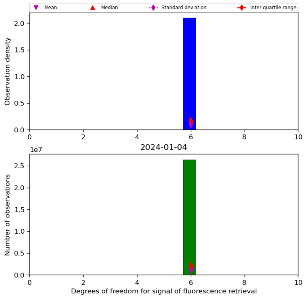
Figure 43: Histogram of “Degrees of freedom for signal of fluorescence retrieval” for 2024-01-03 to 2024-01-05
