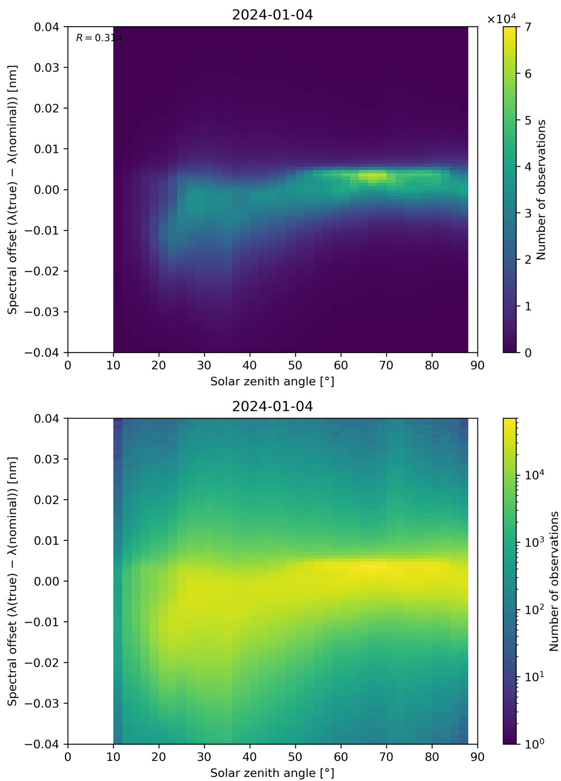
Figure 117: Scatter density plot of “Solar zenith angle” against “Spectral offset ( \lambda(\text{true}) - \lambda(\text{nominal}) )” for 2024-01-03 to 2024-01-05.
