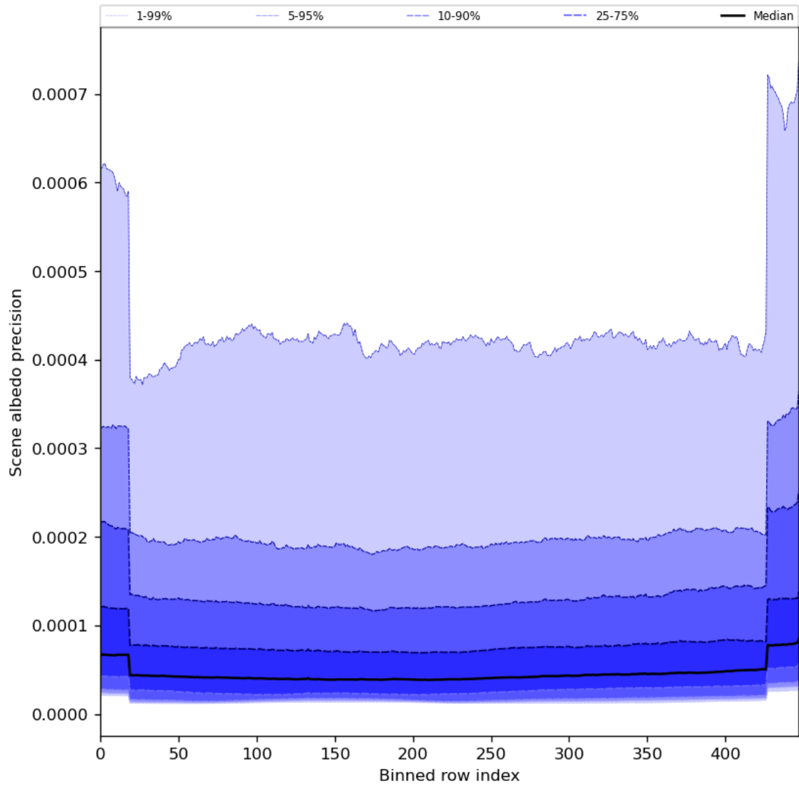
Figure 52: Along track statistics of “Scene albedo precision” for 2024-01-03 to 2024-01-05
