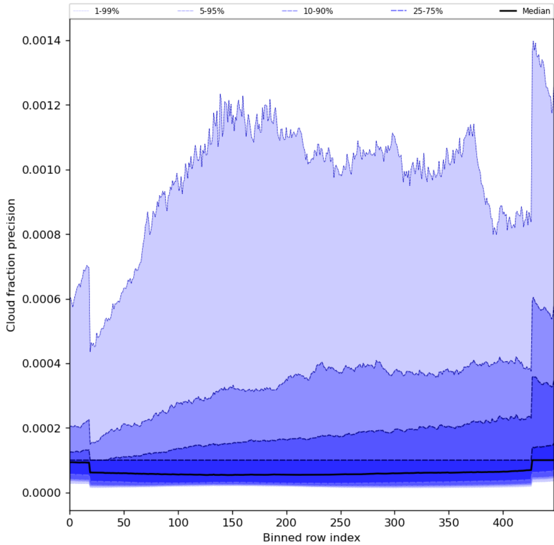
Figure 50: Along track statistics of “Cloud fraction precision” for 2024-01-03 to 2024-01-05
