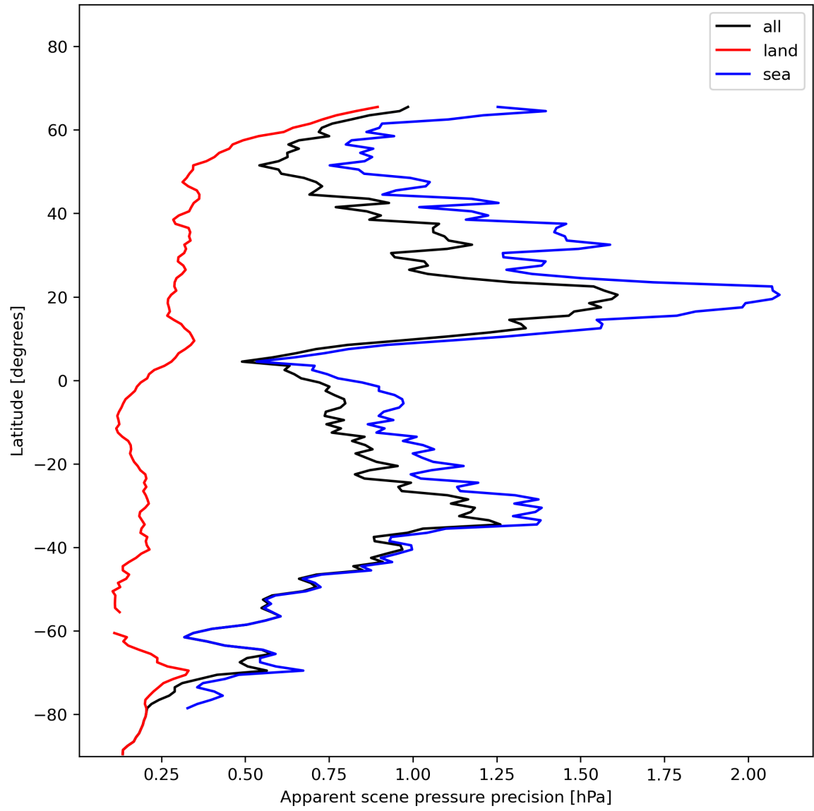
Figure 20: Zonal average of “Apparent scene pressure precision” for 2024-01-03 to 2024-01-05.
