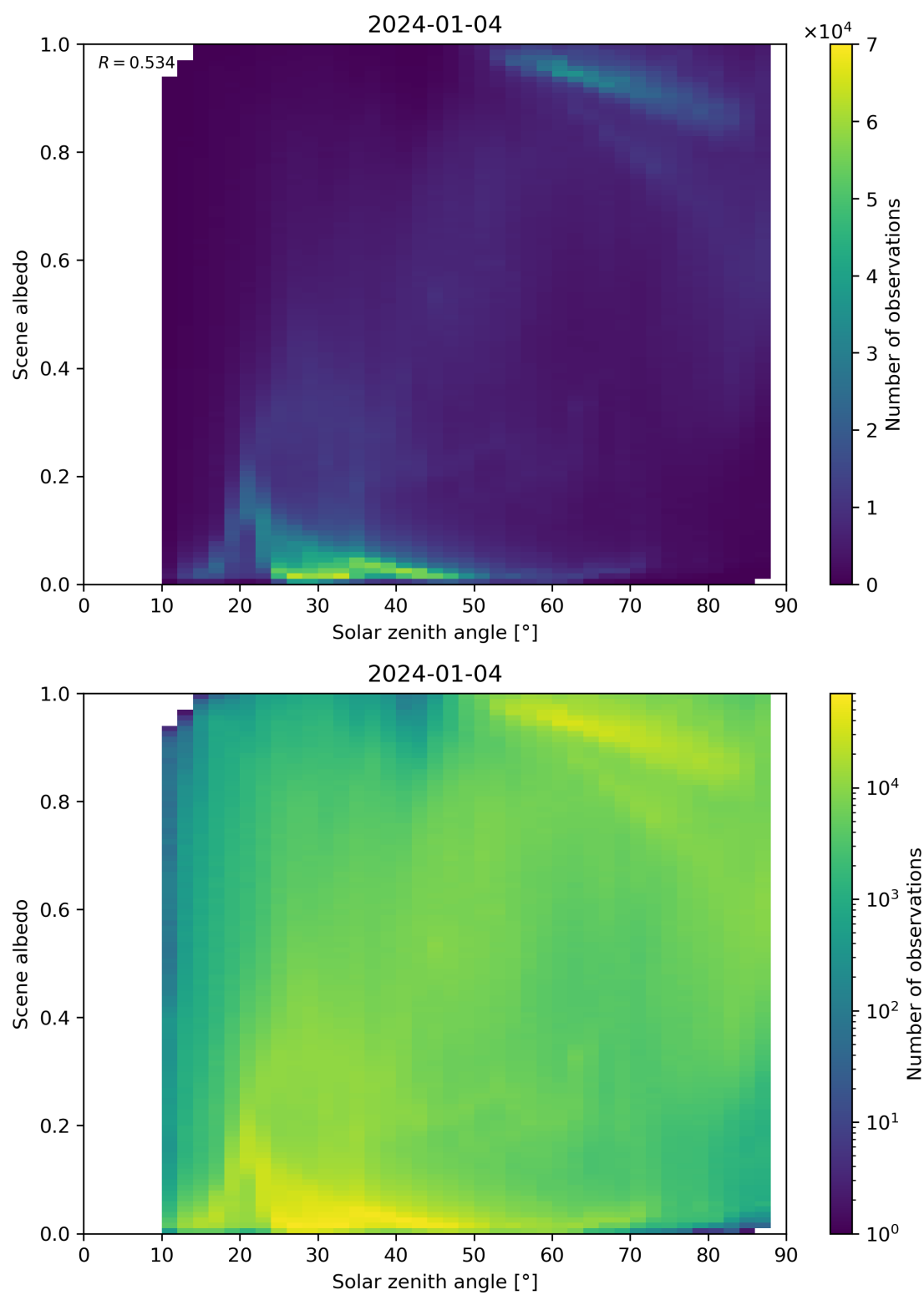
Figure 116: Scatter density plot of “Solar zenith angle” against “Scene albedo” for 2024-01-03 to 2024-01-05.
