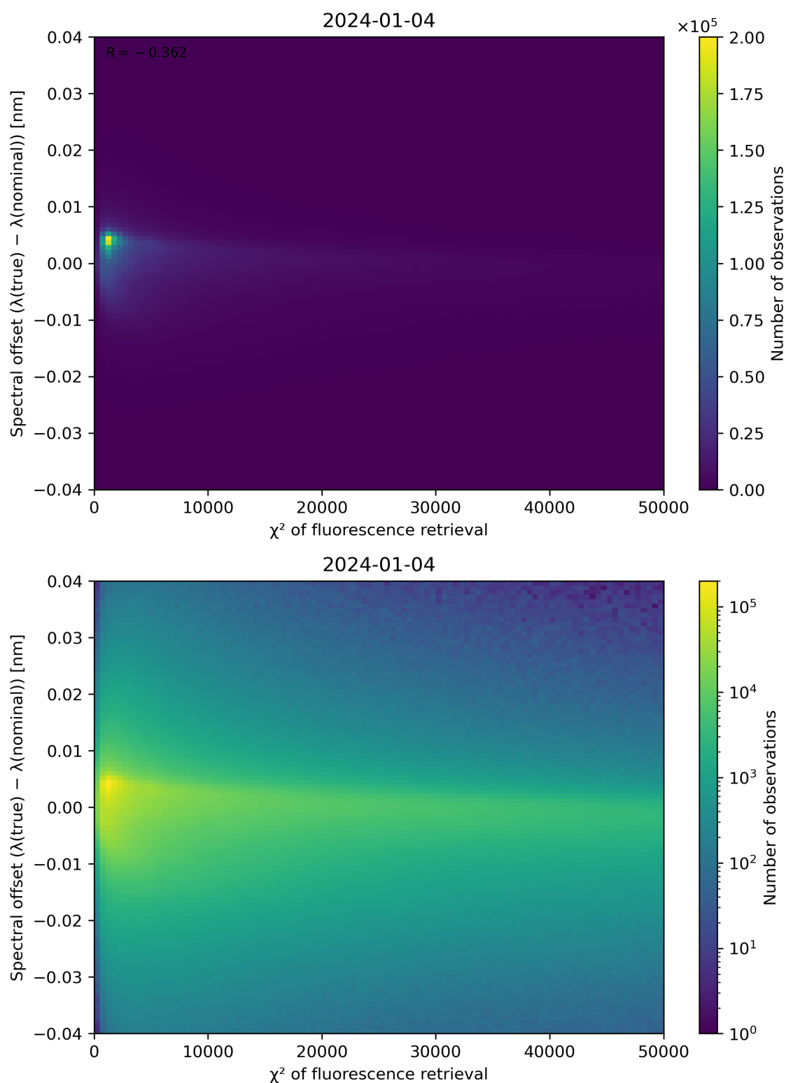
Figure 69: Scatter density plot of " \chi^2 of fluorescence retrieval" against "Spectral offset ( \lambda(\text{true}) - \lambda(\text{nominal}) )" for 2024-01-03 to 2024-01-05.
