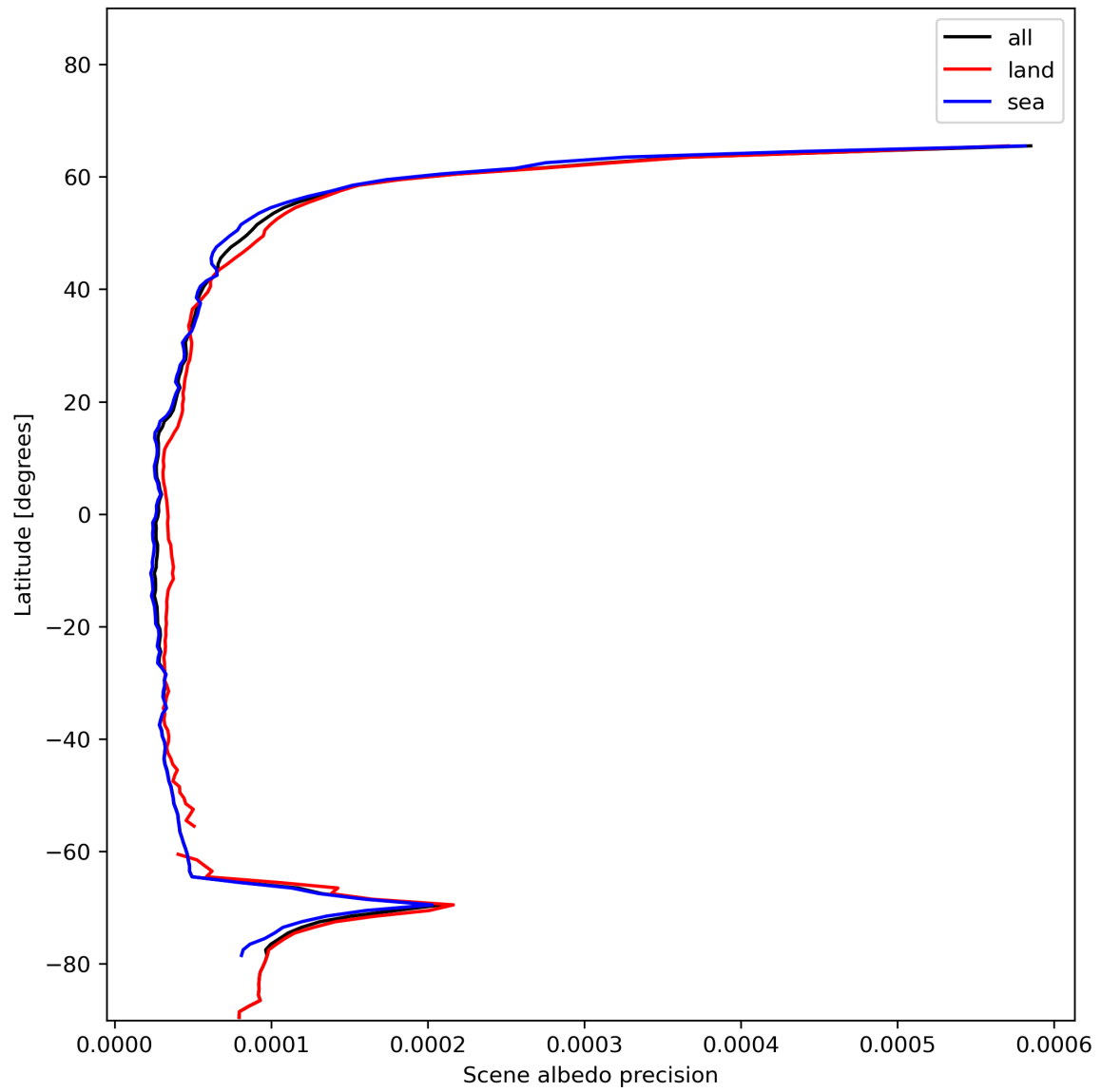
Figure 18: Zonal average of “Scene albedo precision” for 2024-01-03 to 2024-01-05.
