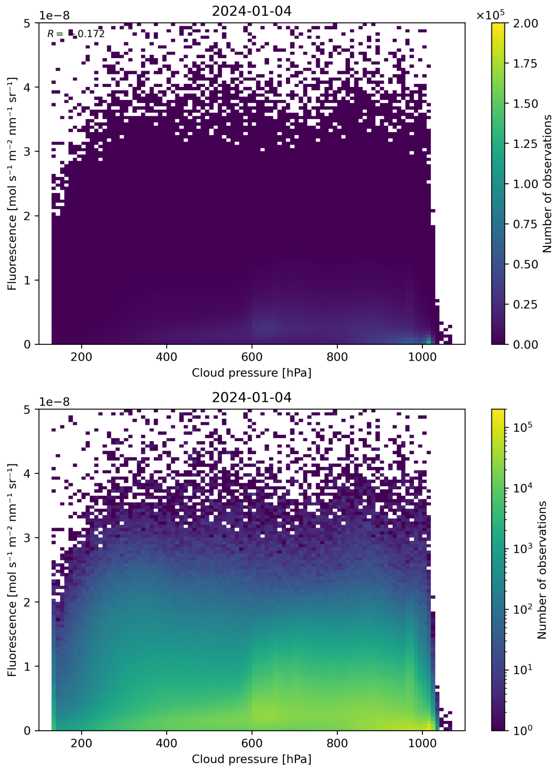
Figure 80: Scatter density plot of “Cloud pressure” against “Fluorescence” for 2024-01-03 to 2024-01-05.
