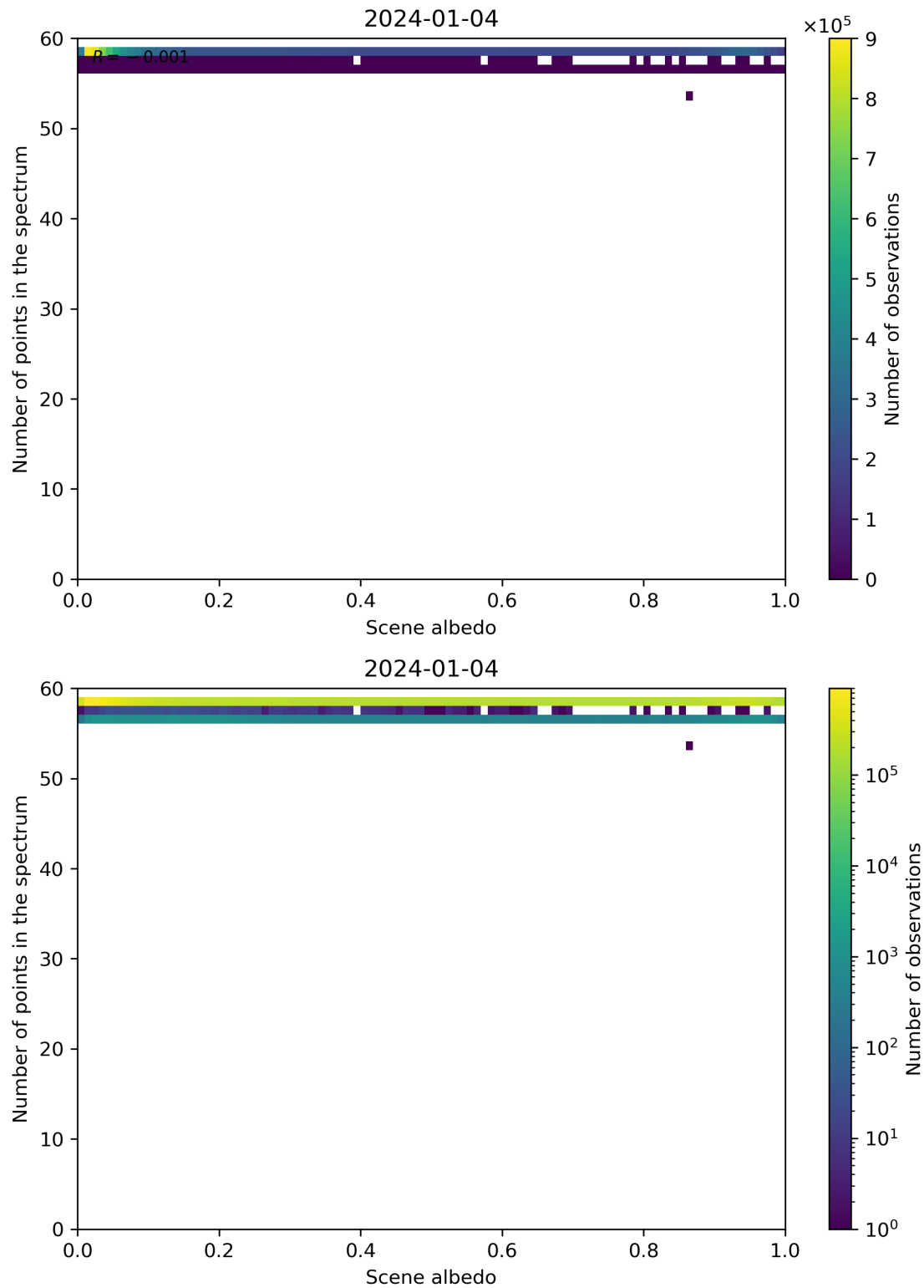
Figure 106: Scatter density plot of “Scene albedo” against “Number of points in the spectrum” for 2024-01-03 to 2024-01-05.
