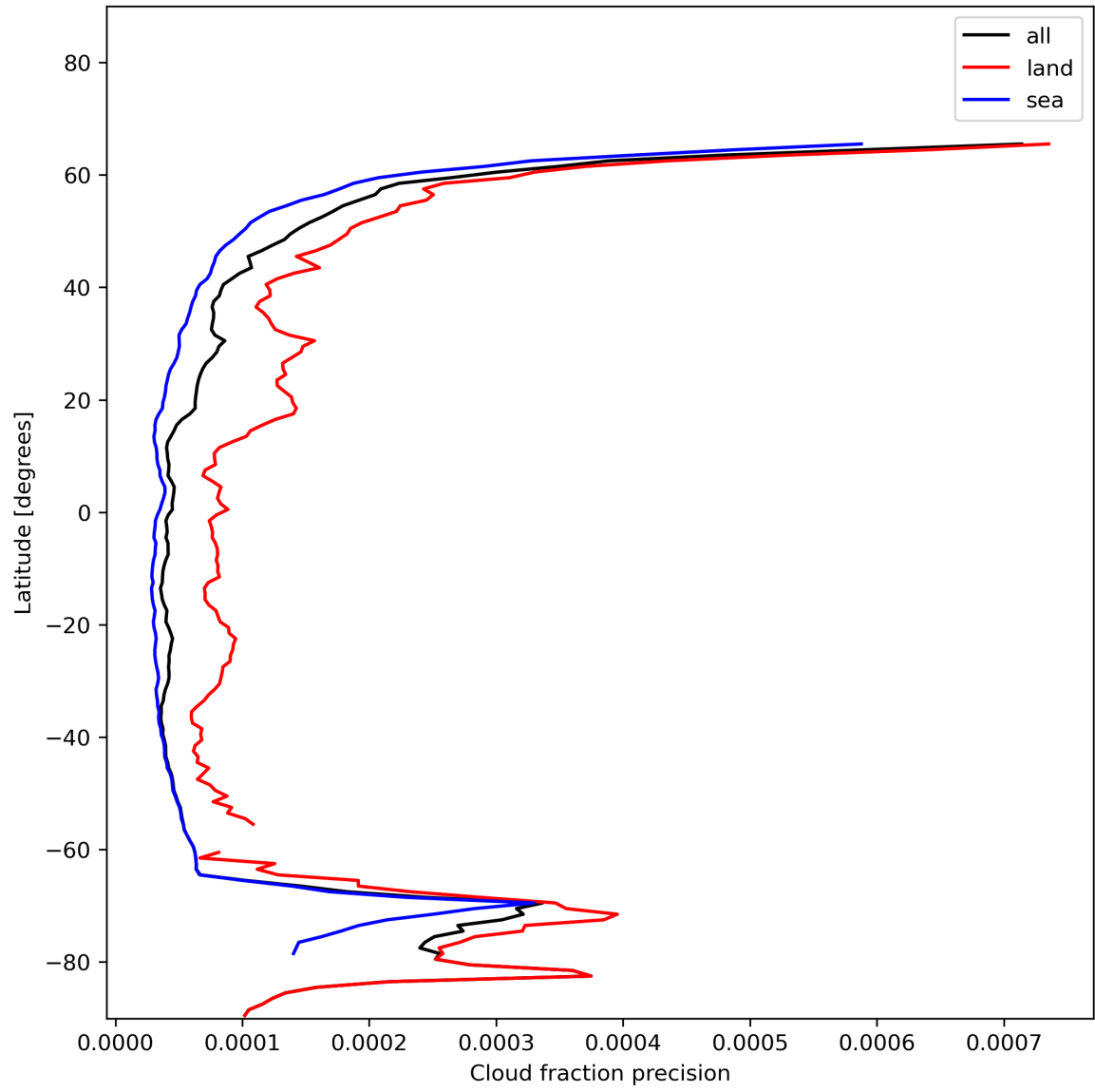
Figure 16: Zonal average of “Cloud fraction precision” for 2024-01-03 to 2024-01-05.
