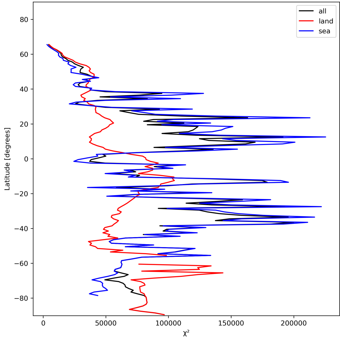
Figure 21: Zonal average of “ \chi^2 ” for 2024-01-03 to 2024-01-05.
