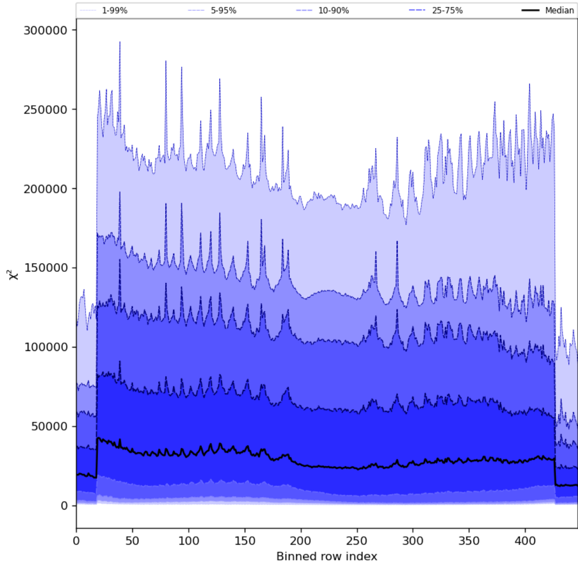
Figure 55: Along track statistics of “ \chi^2 ” for 2024-01-03 to 2024-01-05
