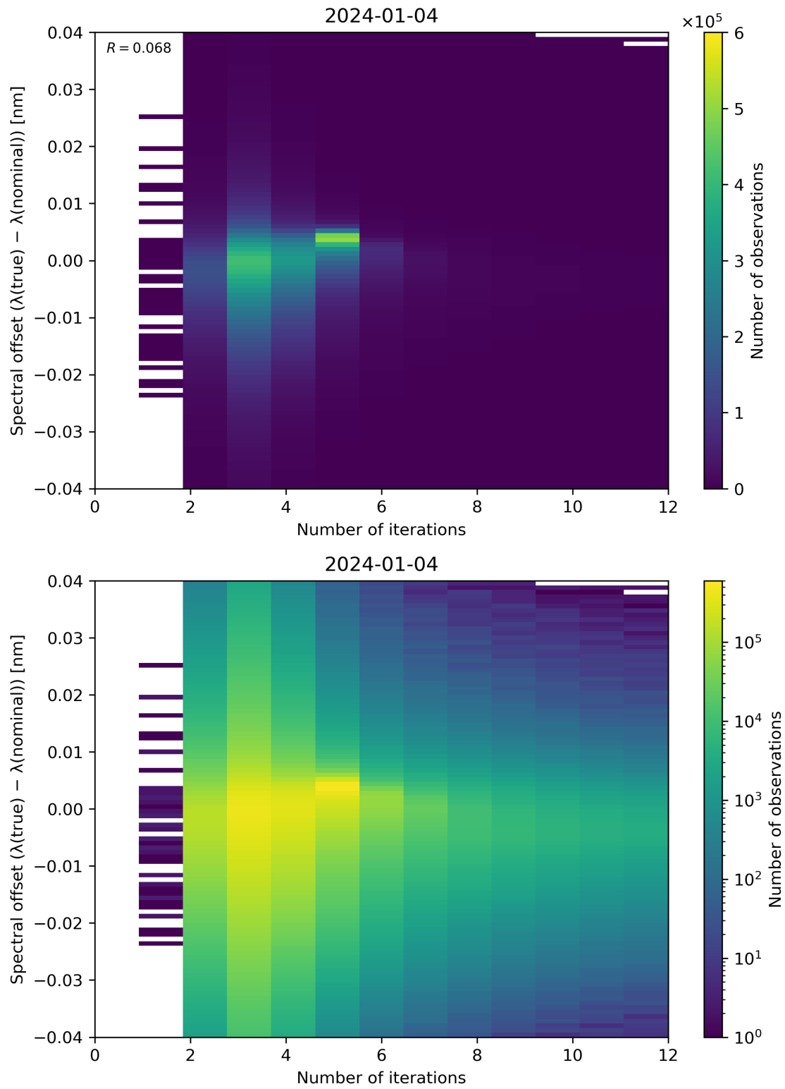
Figure 100: Scatter density plot of “Number of iterations” against “Spectral offset ( \lambda(\text{true}) - \lambda(\text{nominal}) )” for 2024-01-03 to 2024-01-05.
