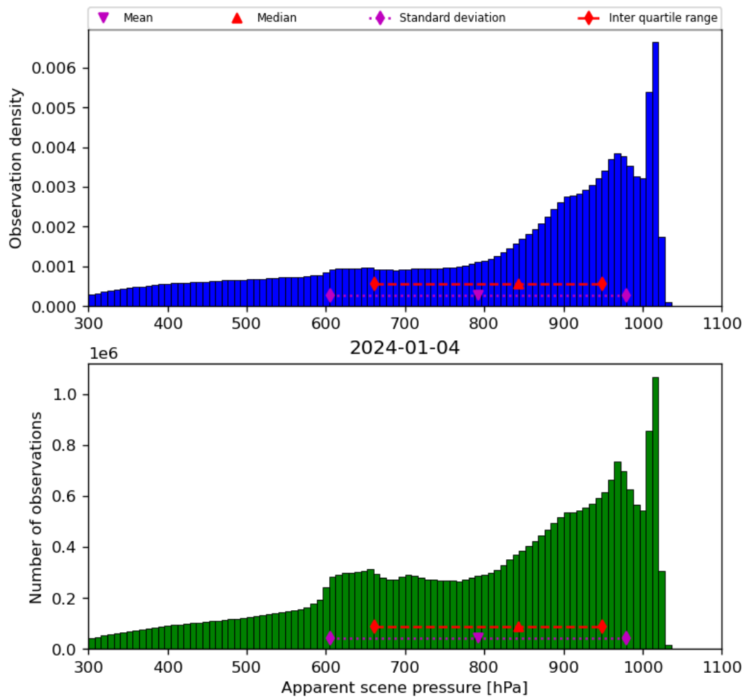
Figure 36: Histogram of “Apparent scene pressure” for 2024-01-03 to 2024-01-05
