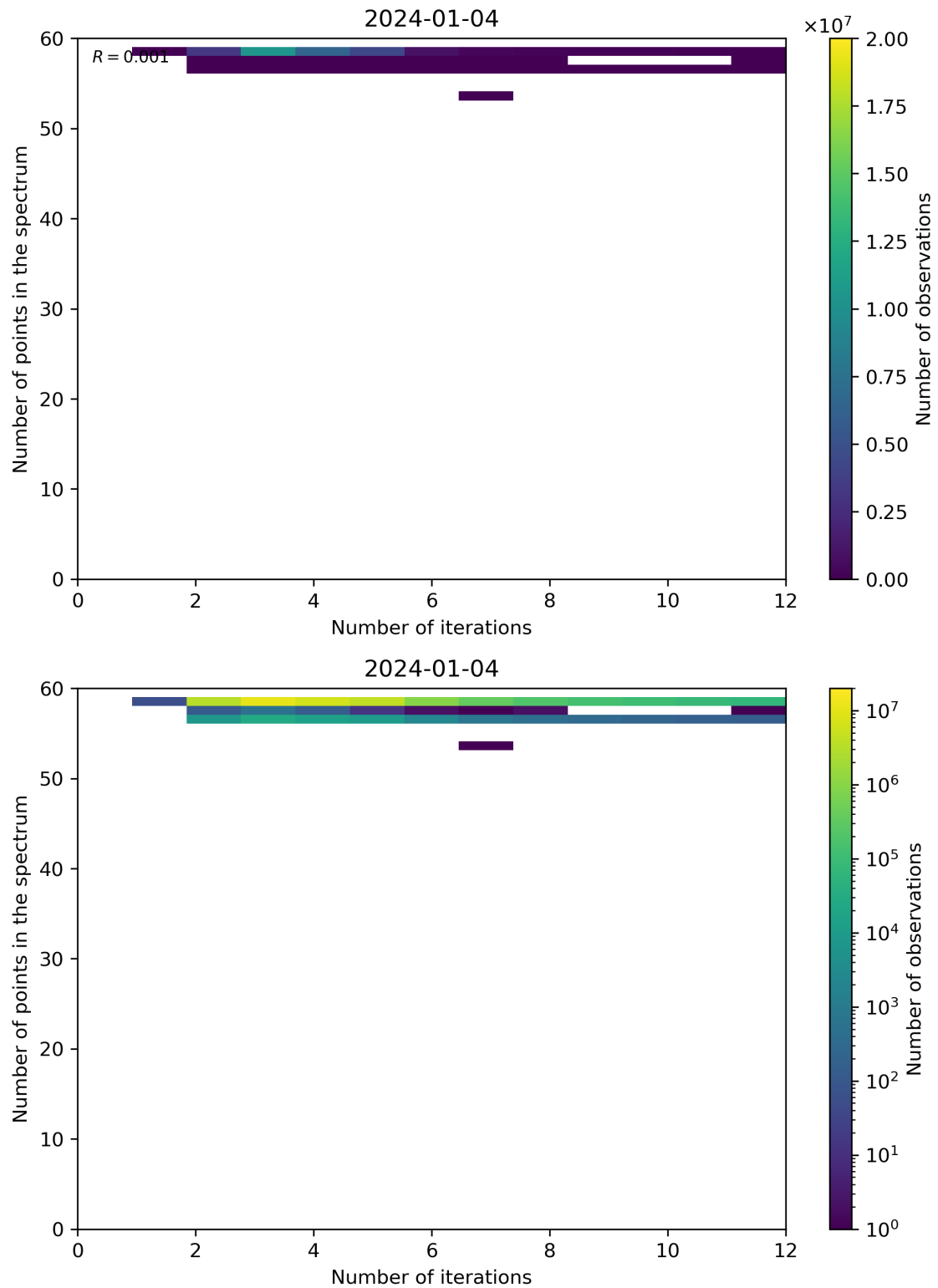
Figure 99: Scatter density plot of “Number of iterations” against “Number of points in the spectrum” for 2024-01-03 to 2024-01-05.
