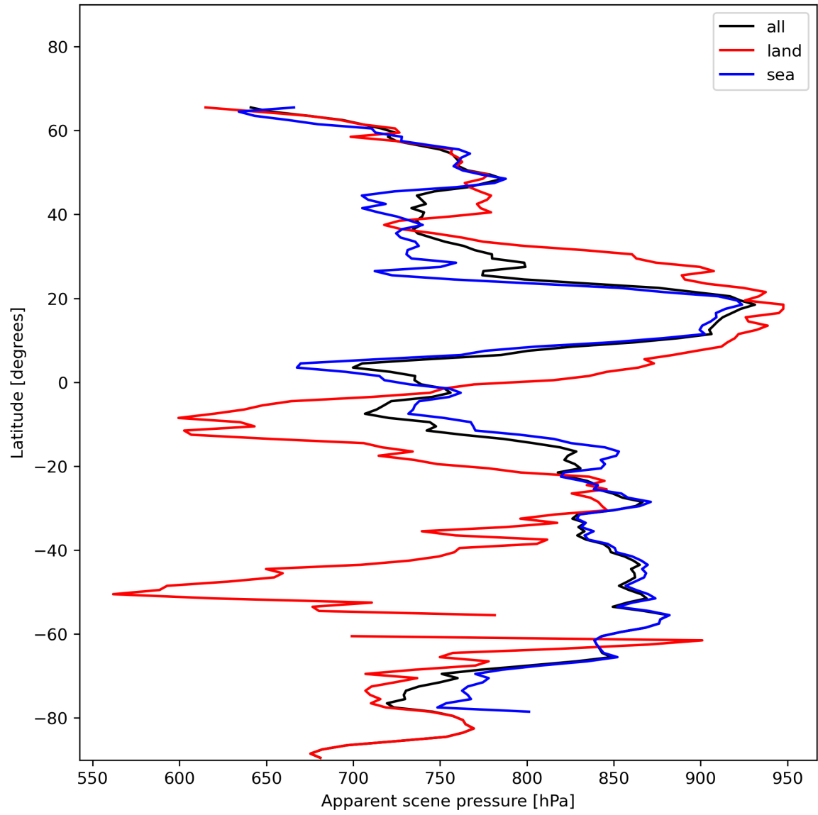
Figure 19: Zonal average of “Apparent scene pressure” for 2024-01-03 to 2024-01-05.
