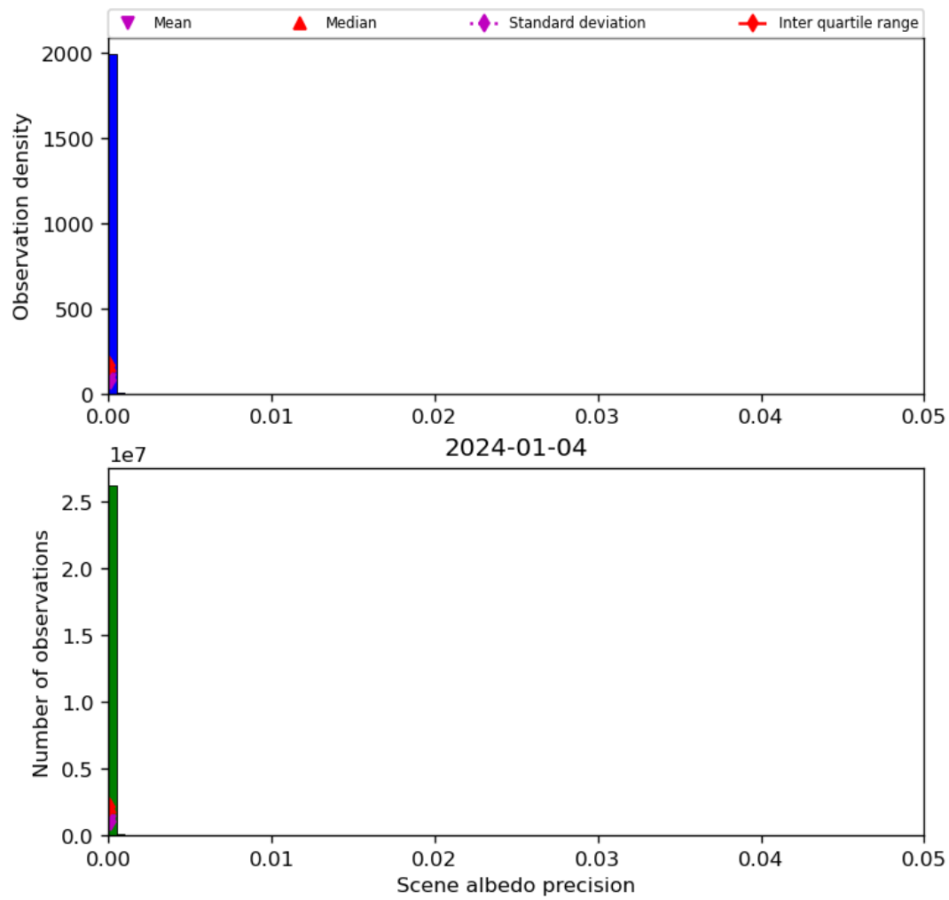
Figure 35: Histogram of “Scene albedo precision” for 2024-01-03 to 2024-01-05
