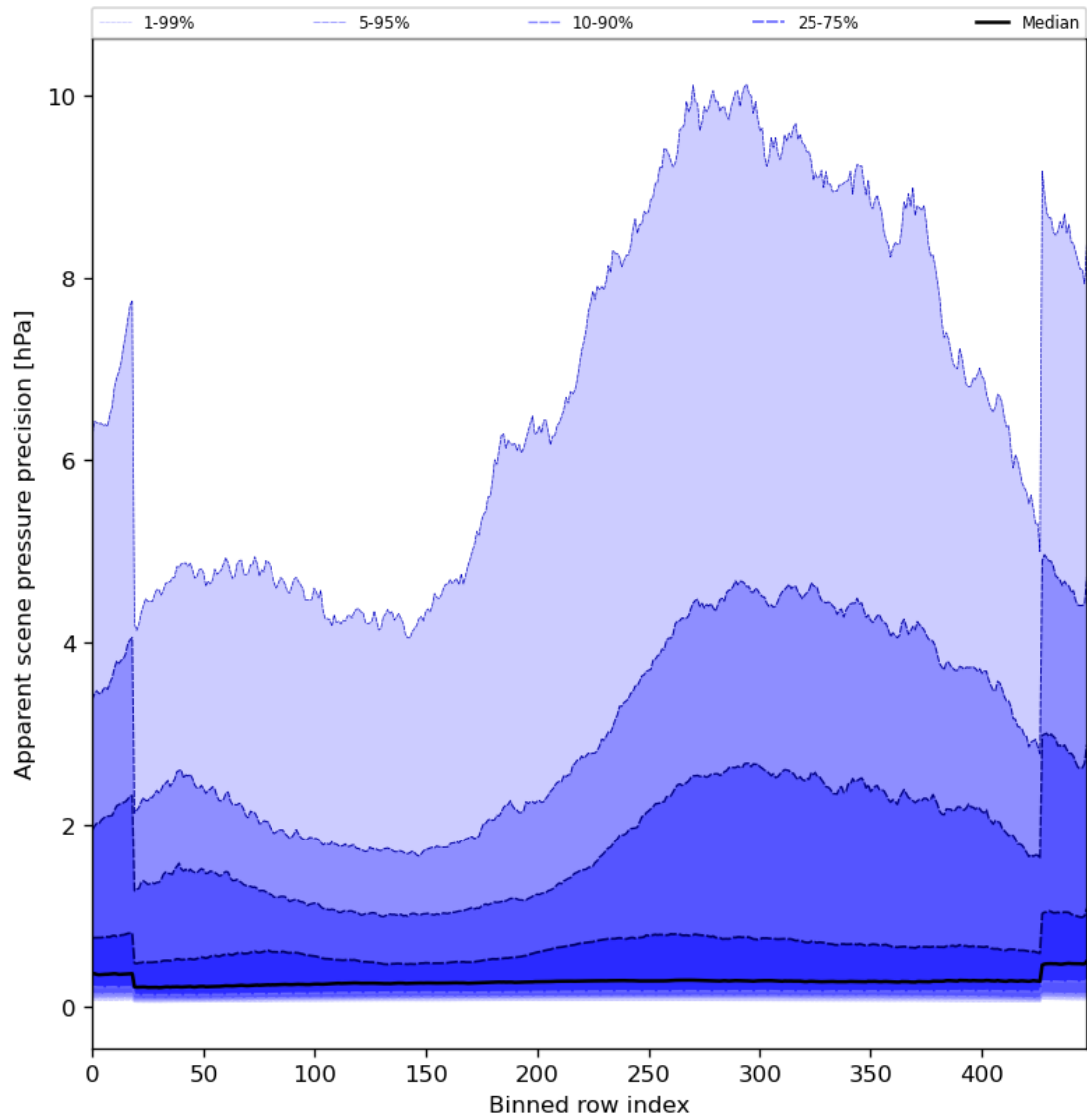
Figure 54: Along track statistics of “Apparent scene pressure precision” for 2024-01-03 to 2024-01-05
