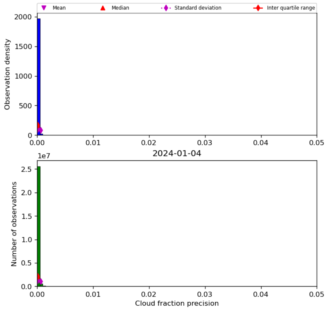
Figure 33: Histogram of “Cloud fraction precision” for 2024-01-03 to 2024-01-05
