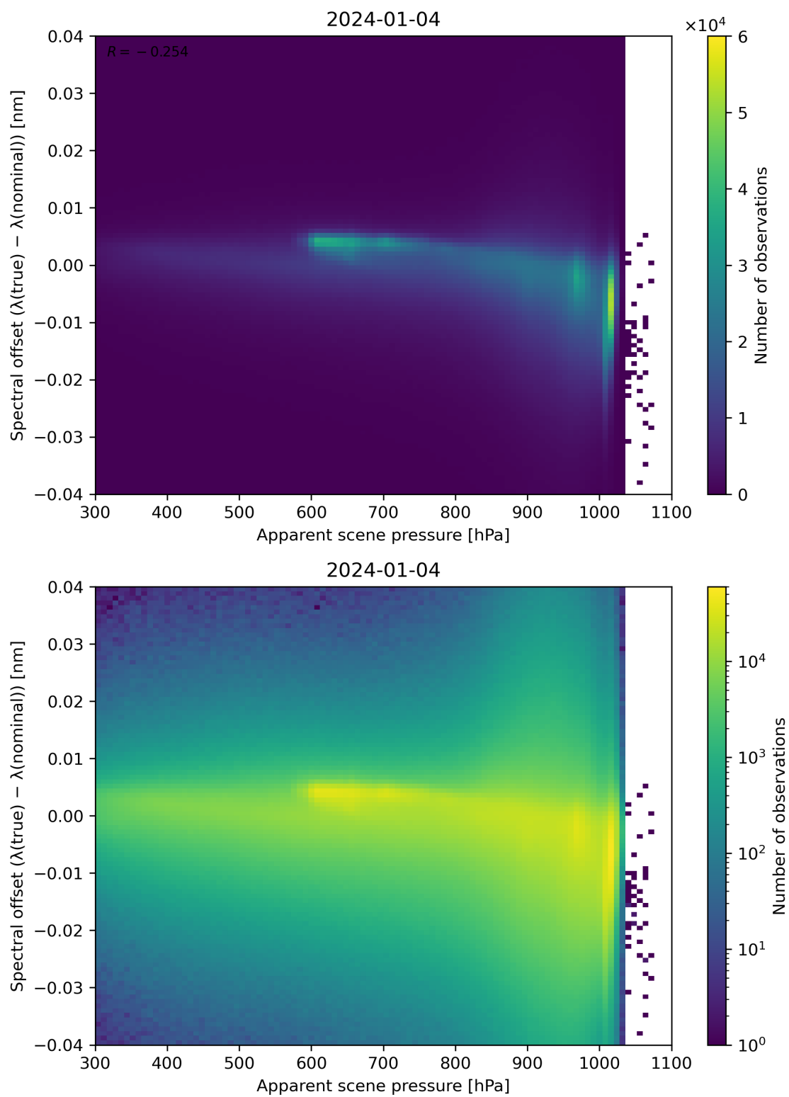
Figure 67: Scatter density plot of “Apparent scene pressure” against “Spectral offset ( \lambda(\text{true}) - \lambda(\text{nominal}) )” for 2024-01-03 to 2024-01-05.
