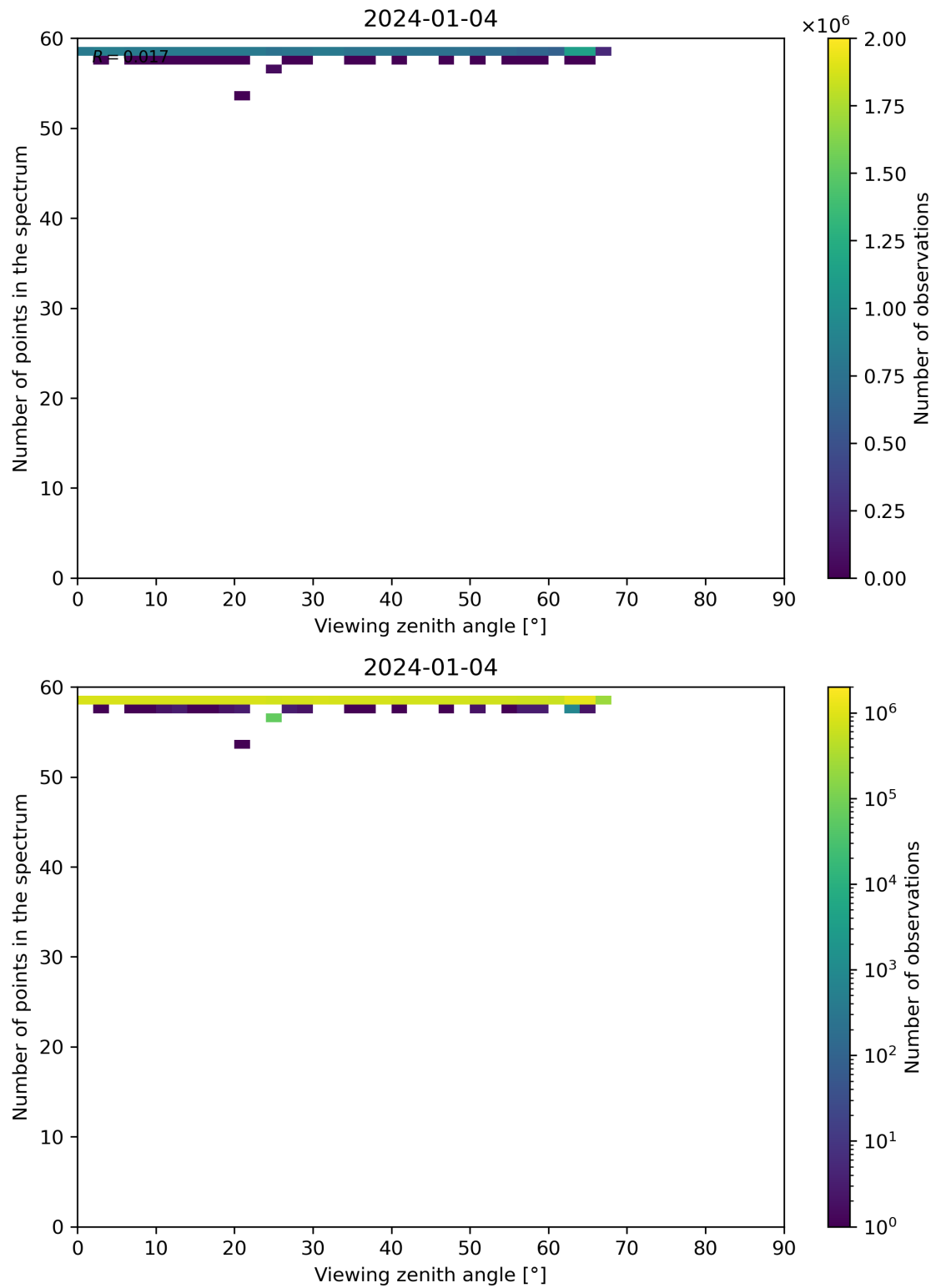
Figure 125: Scatter density plot of “Viewing zenith angle” against “Number of points in the spectrum” for 2024-01-03 to 2024-01-05.
