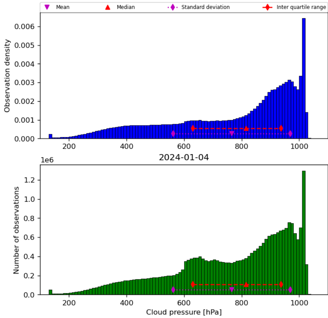
Figure 30: Histogram of “Cloud pressure” for 2024-01-03 to 2024-01-05
