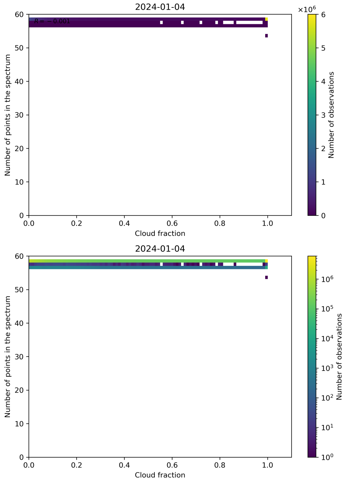
Figure 74: Scatter density plot of “Cloud fraction” against “Number of points in the spectrum” for 2024-01-03 to 2024-01-05.
