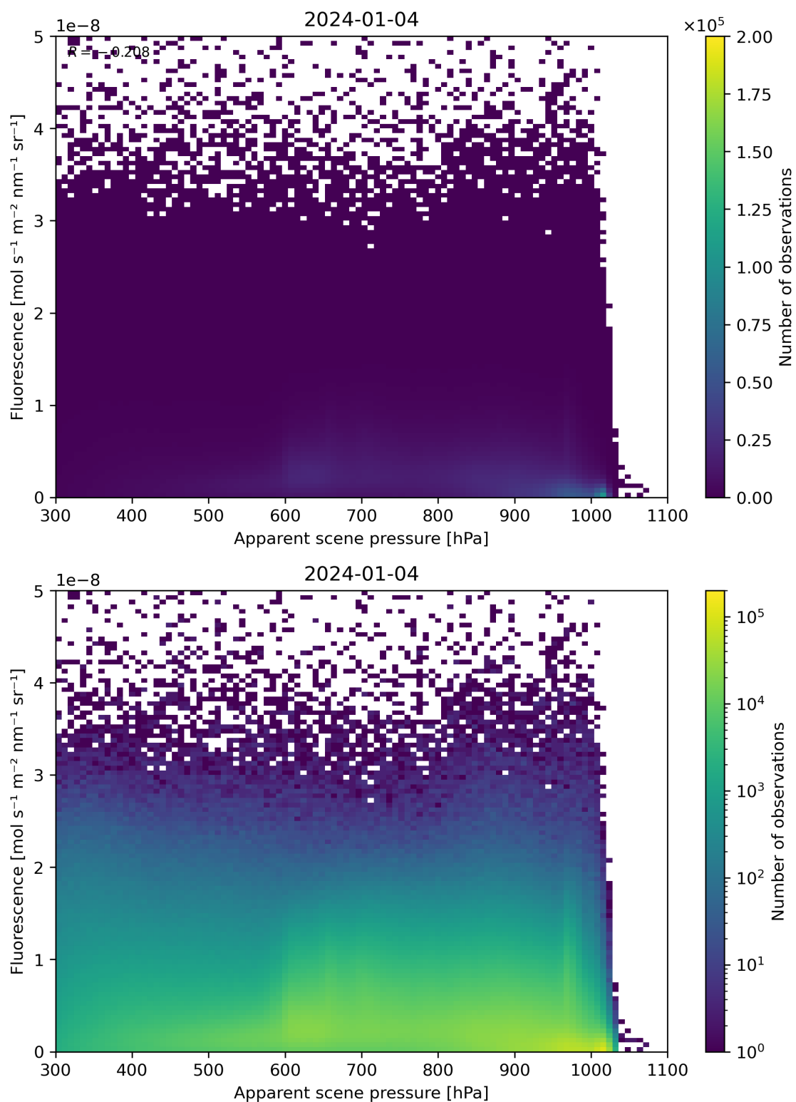
Figure 64: Scatter density plot of “Apparent scene pressure” against “Fluorescence” for 2024-01-03 to 2024-01-05.
