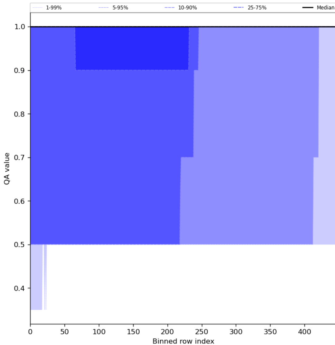
Figure 46: Along track statistics of “QA value” for 2024-01-03 to 2024-01-05
