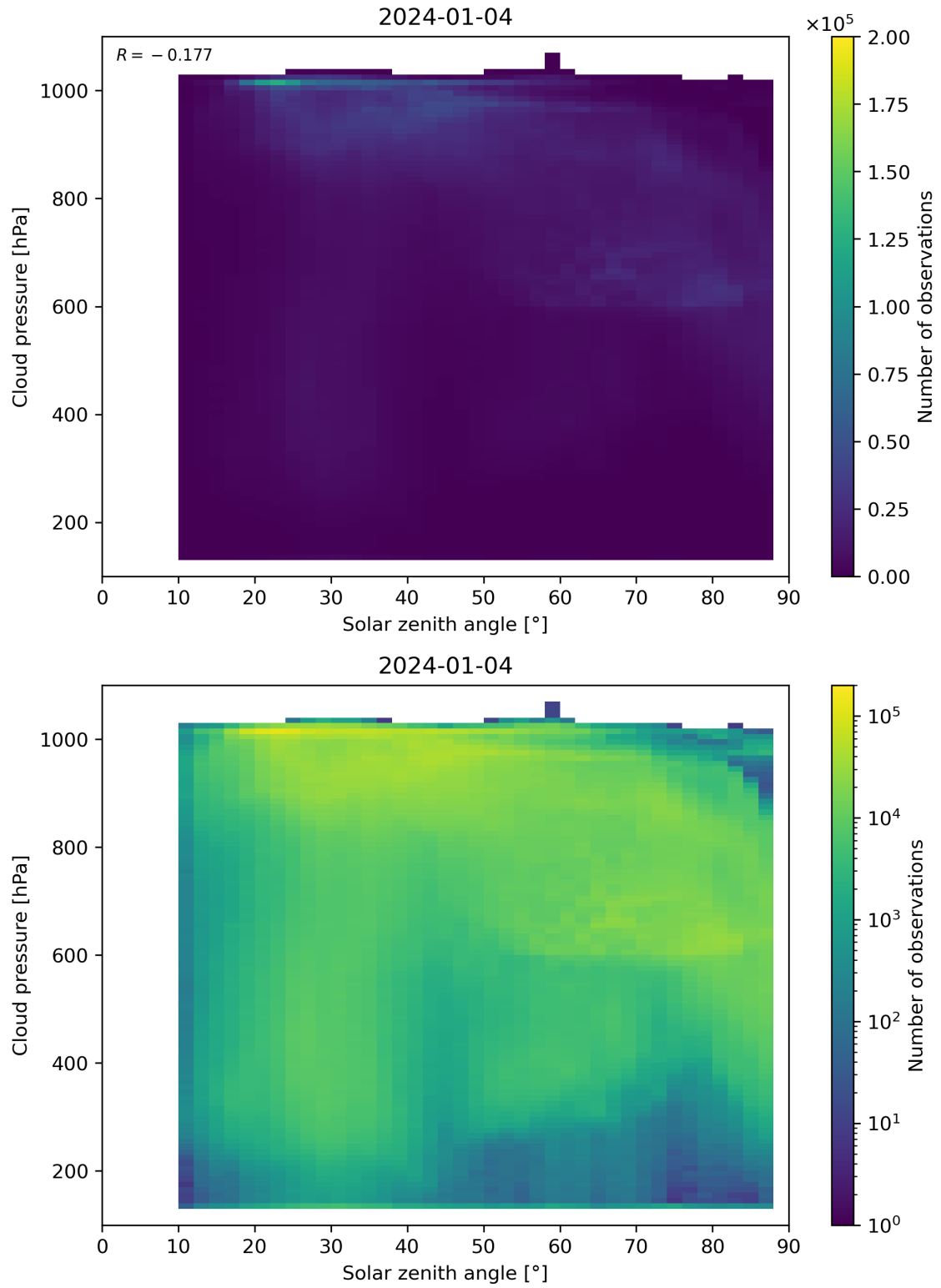
Figure 111: Scatter density plot of “Solar zenith angle” against “Cloud pressure” for 2024-01-03 to 2024-01-05.
