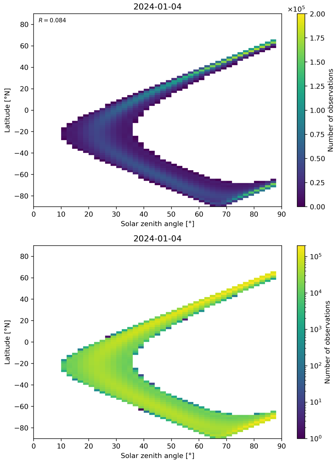
Figure 113: Scatter density plot of “Solar zenith angle” against “Latitude” for 2024-01-03 to 2024-01-05.
