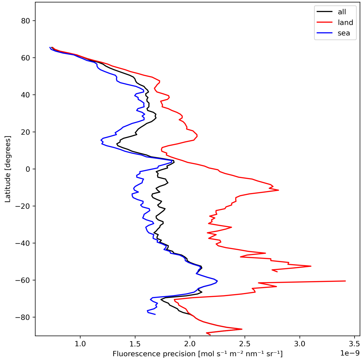
Figure 24: Zonal average of "Fluorescence precision" for 2024-01-03 to 2024-01-05.
