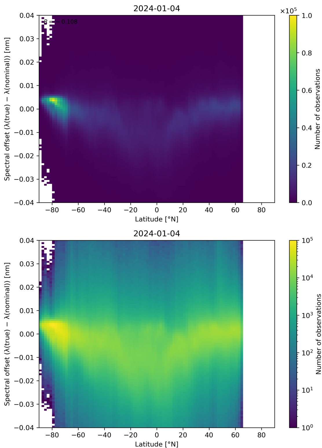
Figure 96: Scatter density plot of “Latitude” against “Spectral offset ( \lambda(\text{true}) - \lambda(\text{nominal}) )” for 2024-01-03 to 2024-01-05.
