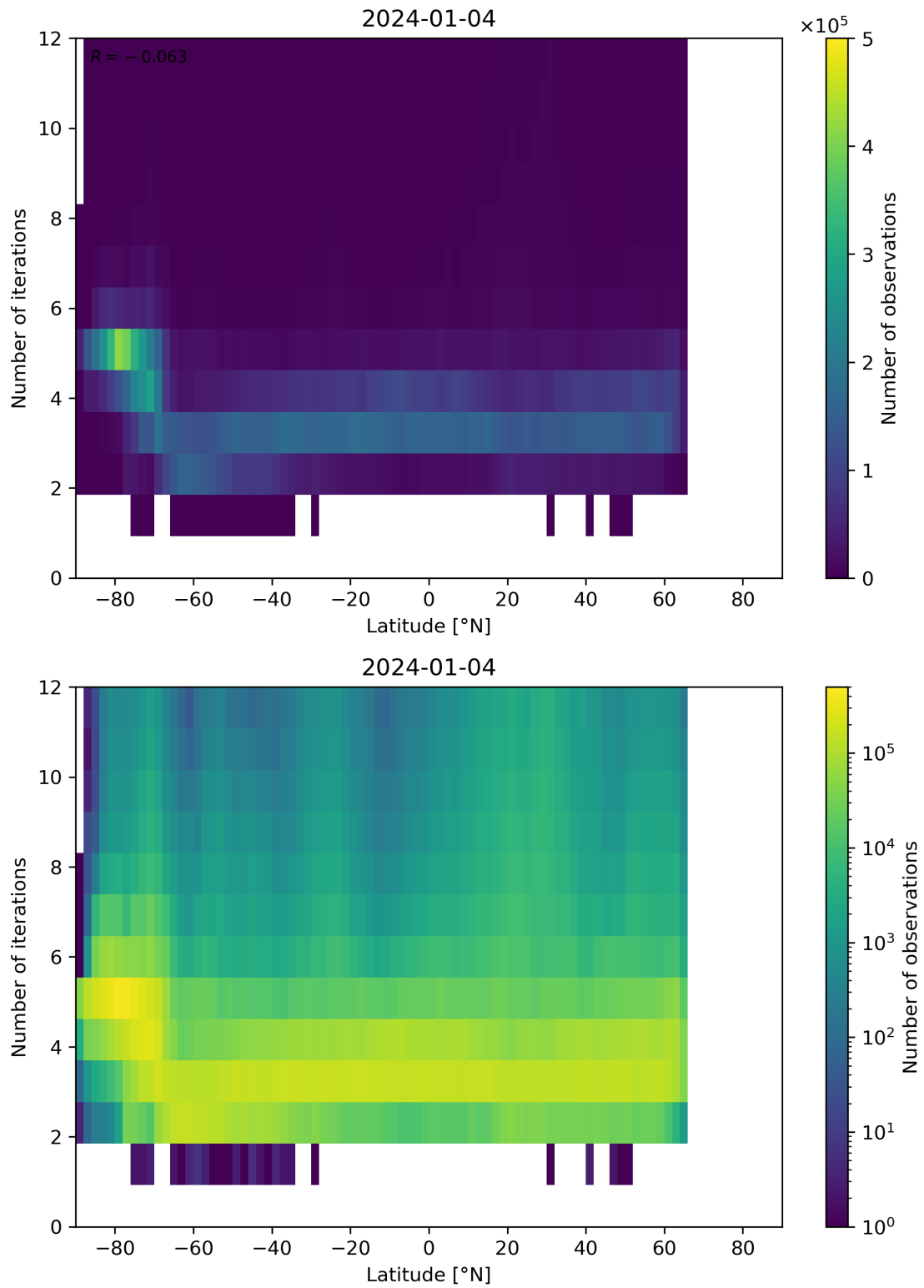
Figure 93: Scatter density plot of “Latitude” against “Number of iterations” for 2024-01-03 to 2024-01-05.
