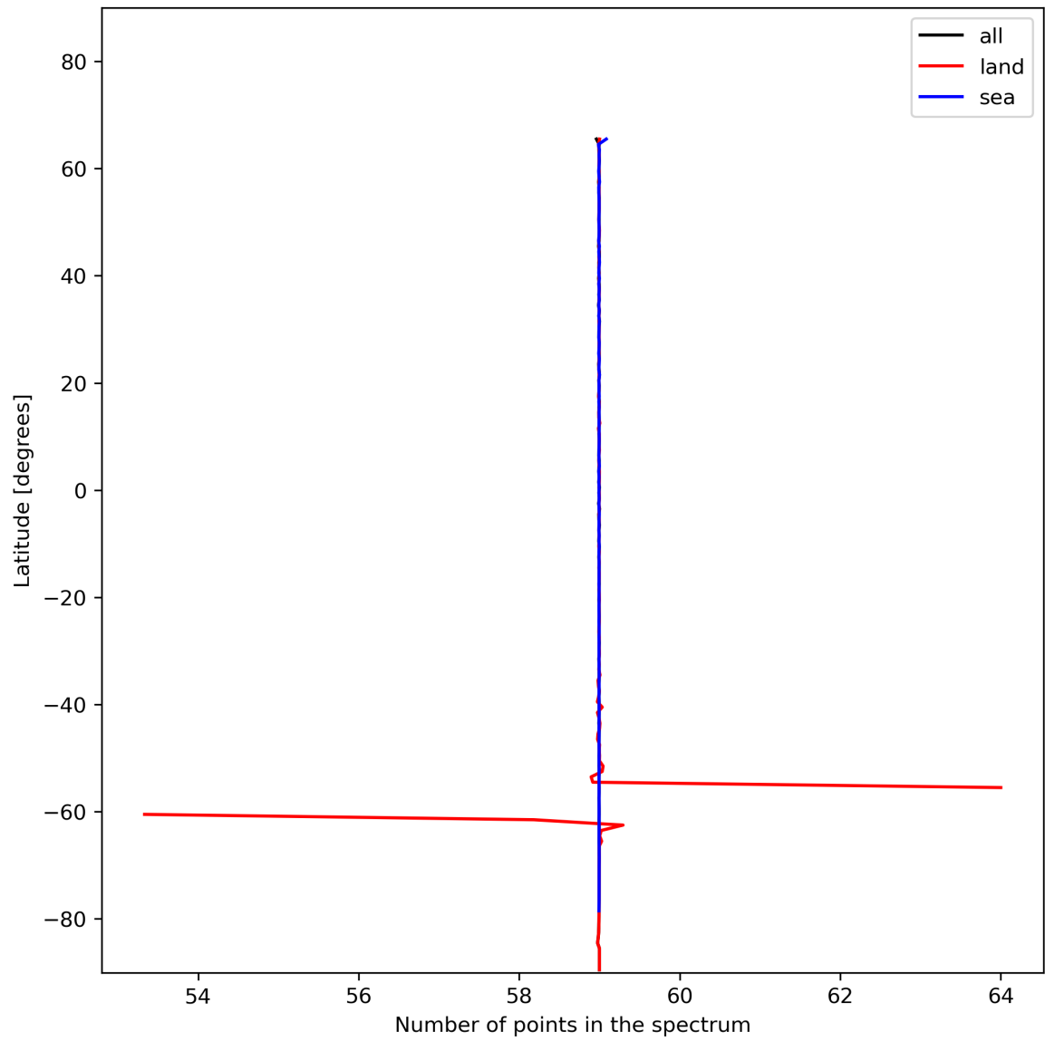
Figure 27: Zonal average of “Number of points in the spectrum” for 2024-01-03 to 2024-01-05.
