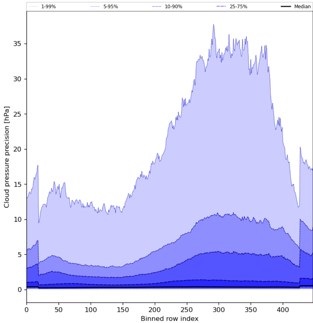
Figure 48: Along track statistics of “Cloud pressure precision” for 2024-01-03 to 2024-01-05
