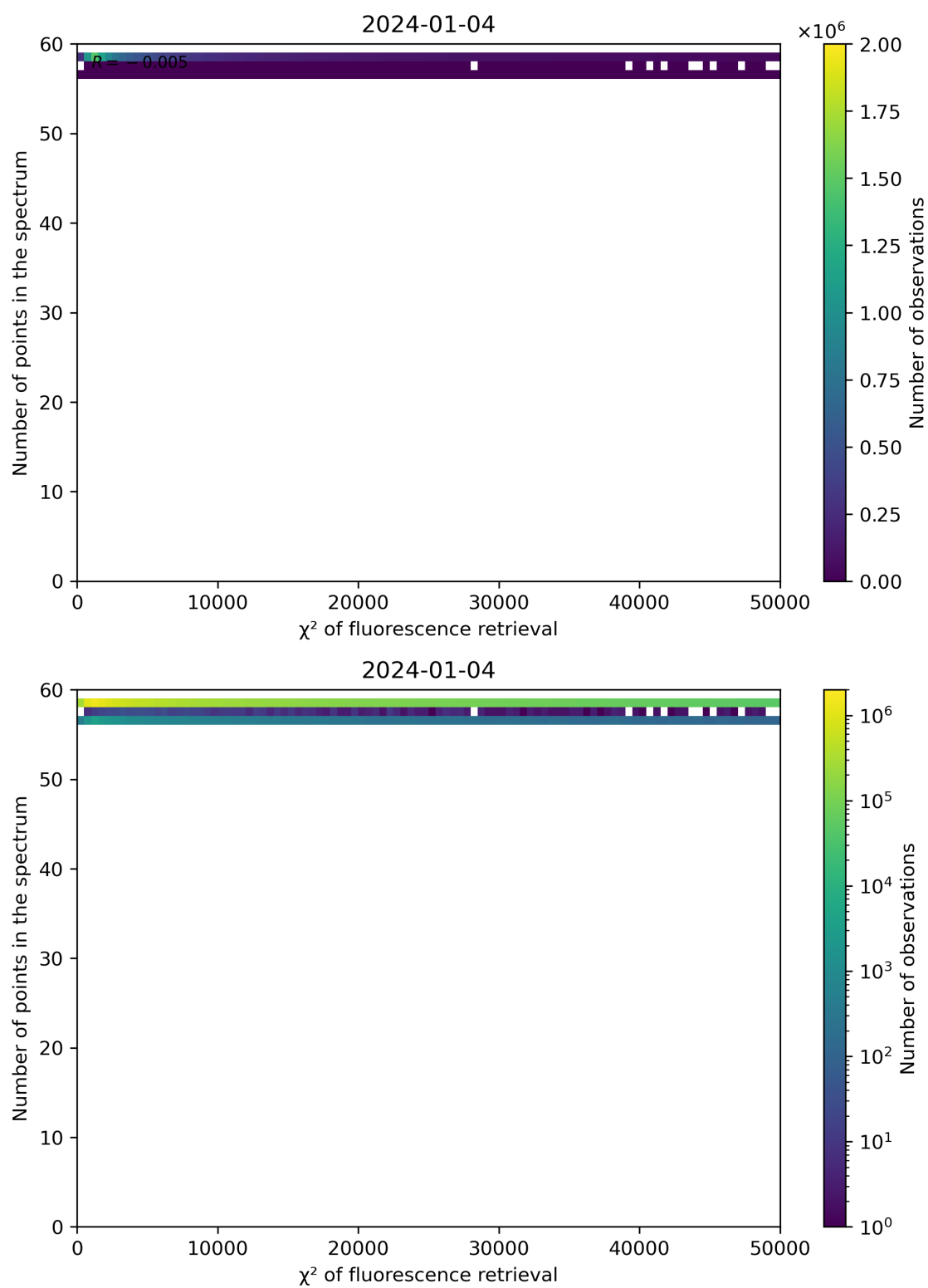
Figure 68: Scatter density plot of " \chi^2 of fluorescence retrieval" against "Number of points in the spectrum" for 2024-01-03 to 2024-01-05.
