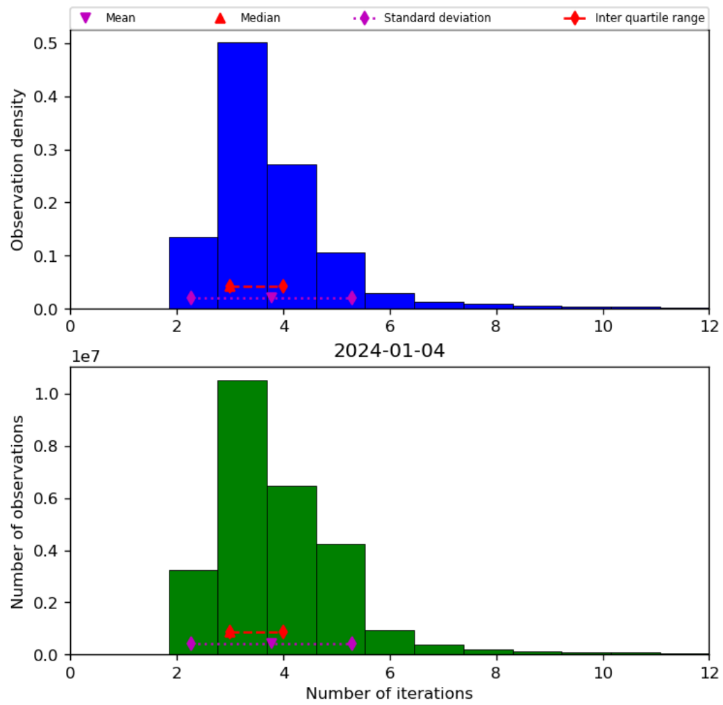
Figure 39: Histogram of “Number of iterations” for 2024-01-03 to 2024-01-05
