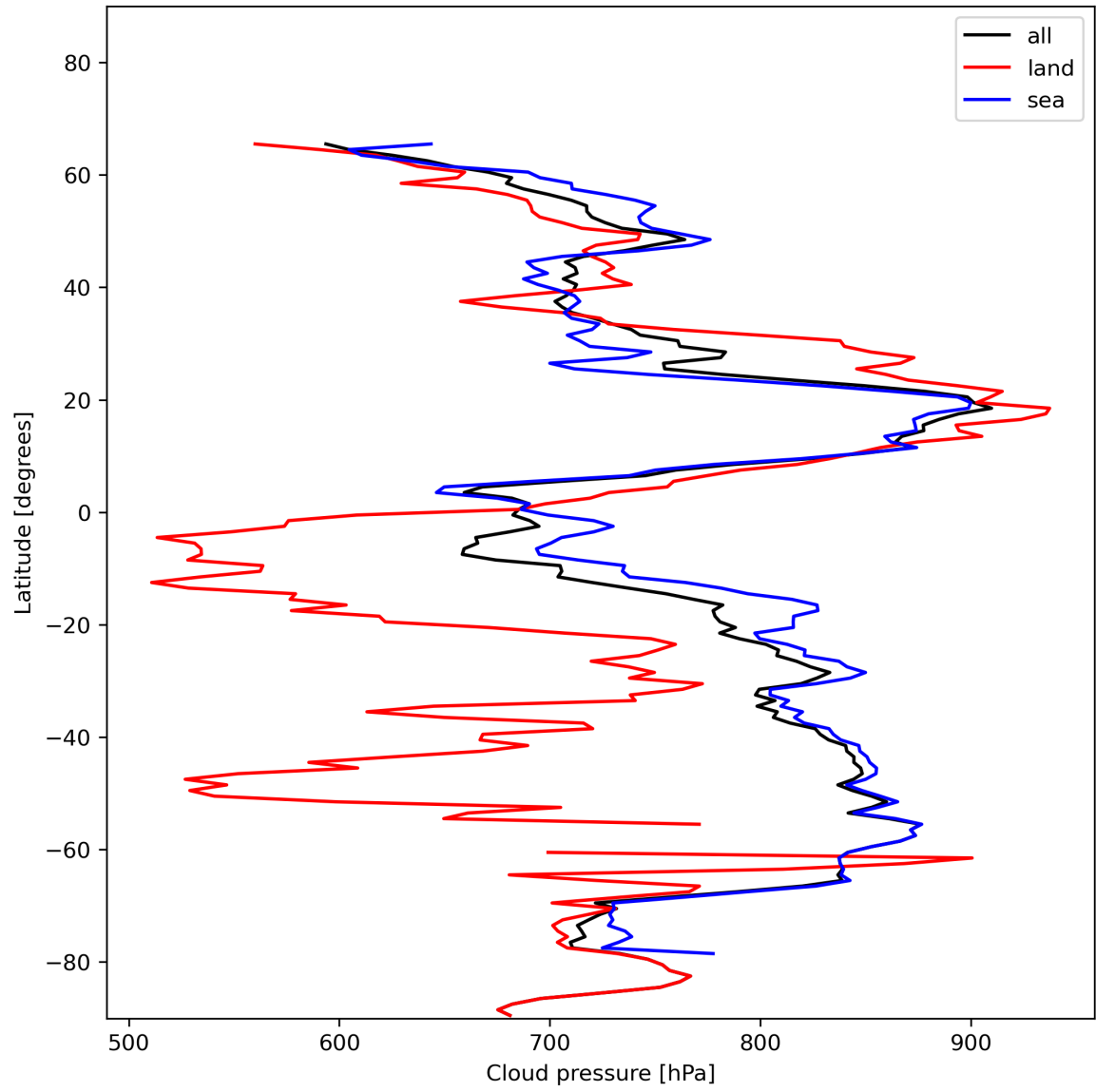
Figure 13: Zonal average of “Cloud pressure” for 2024-01-03 to 2024-01-05.
