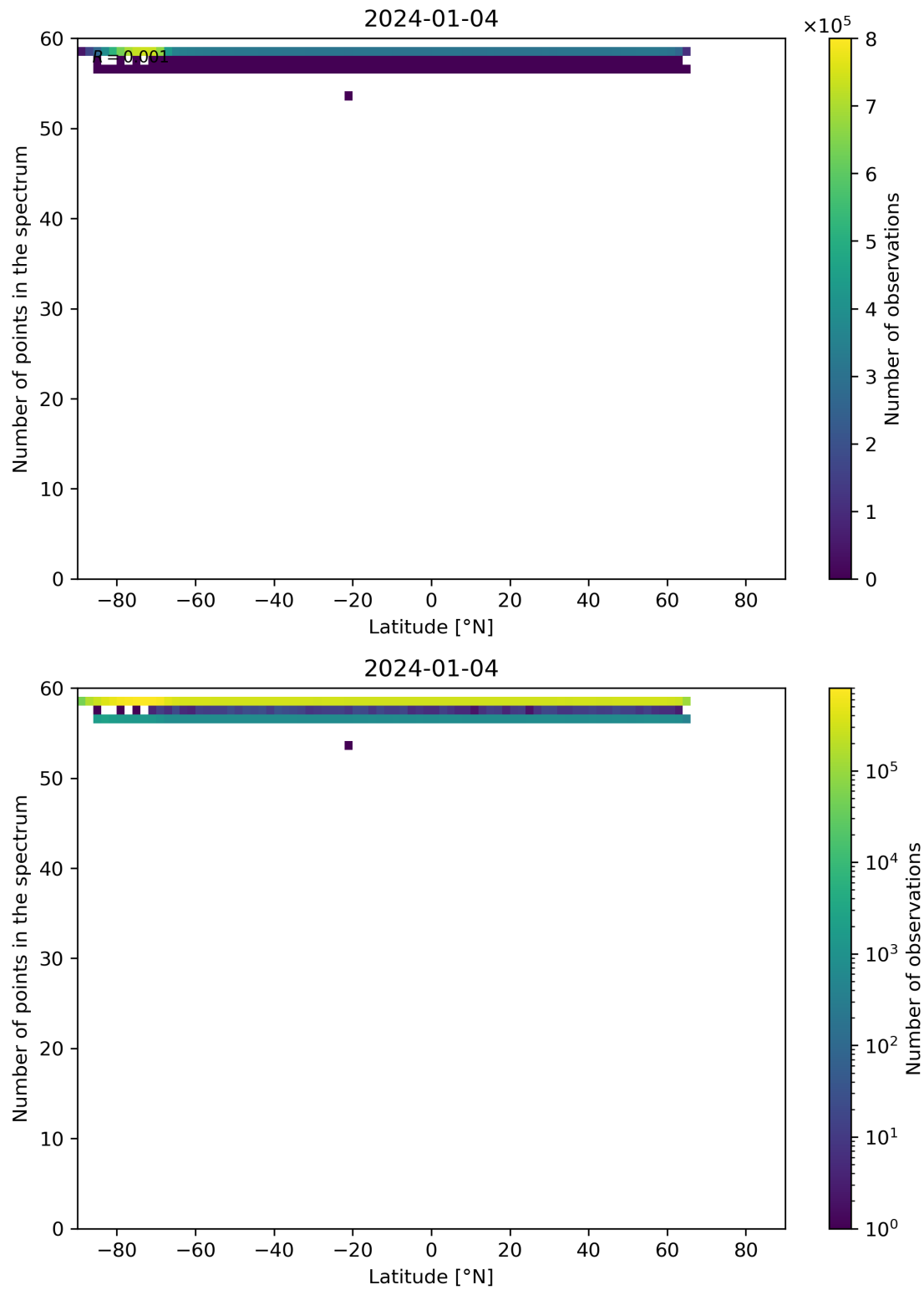
Figure 94: Scatter density plot of “Latitude” against “Number of points in the spectrum” for 2024-01-03 to 2024-01-05.
