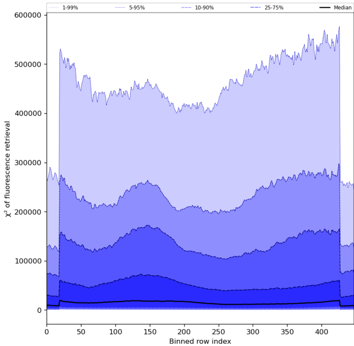
Figure 59: Along track statistics of “ \chi^2 of fluorescence retrieval” for 2024-01-03 to 2024-01-05
