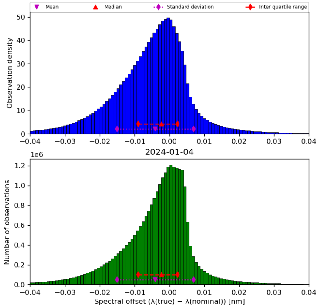
Figure 45: Histogram of “Spectral offset ( \lambda(\text{true}) - \lambda(\text{nominal}) )” for 2024-01-03 to 2024-01-05
