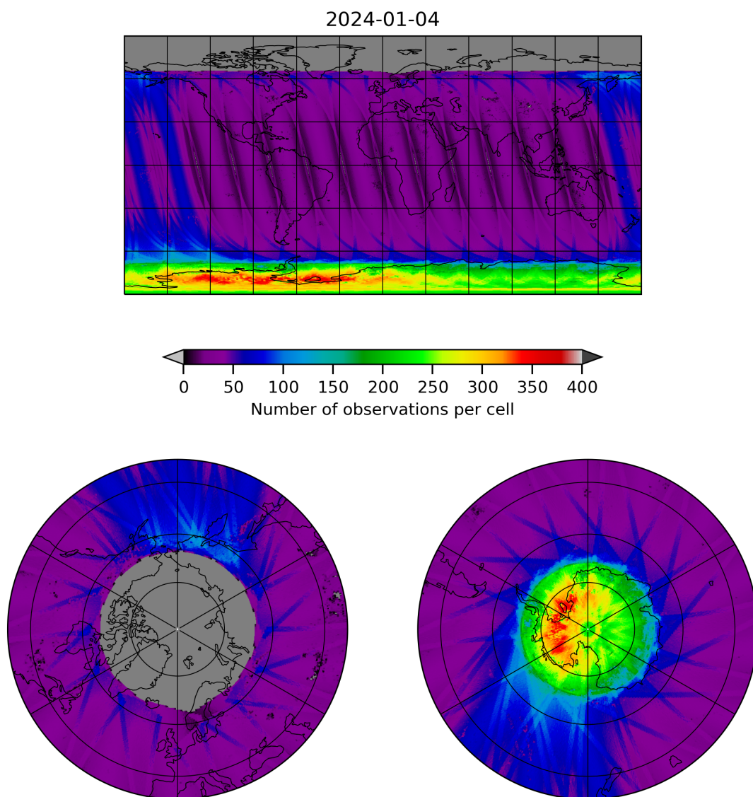
Figure 11: Map of the number of observations for 2024-01-03 to 2024-01-05
