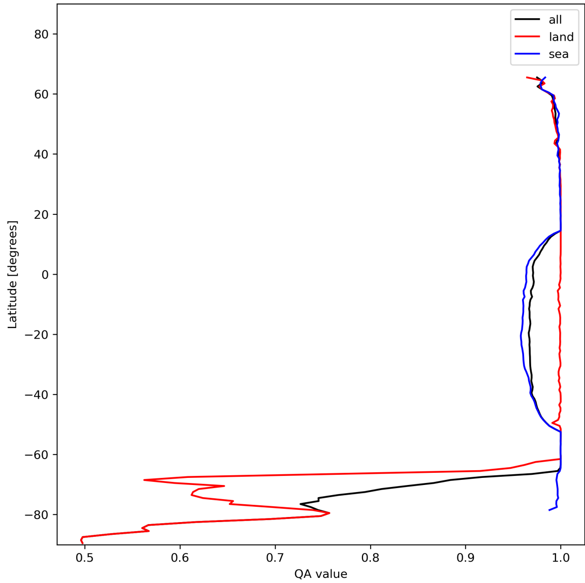
Figure 12: Zonal average of “QA value” for 2024-01-03 to 2024-01-05.
