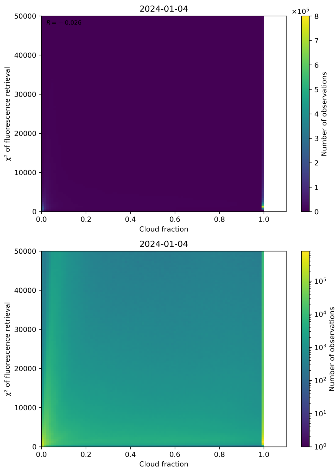
Figure 71: Scatter density plot of “Cloud fraction” against “ \chi^2 of fluorescence retrieval” for 2024-01-03 to 2024-01-05.
