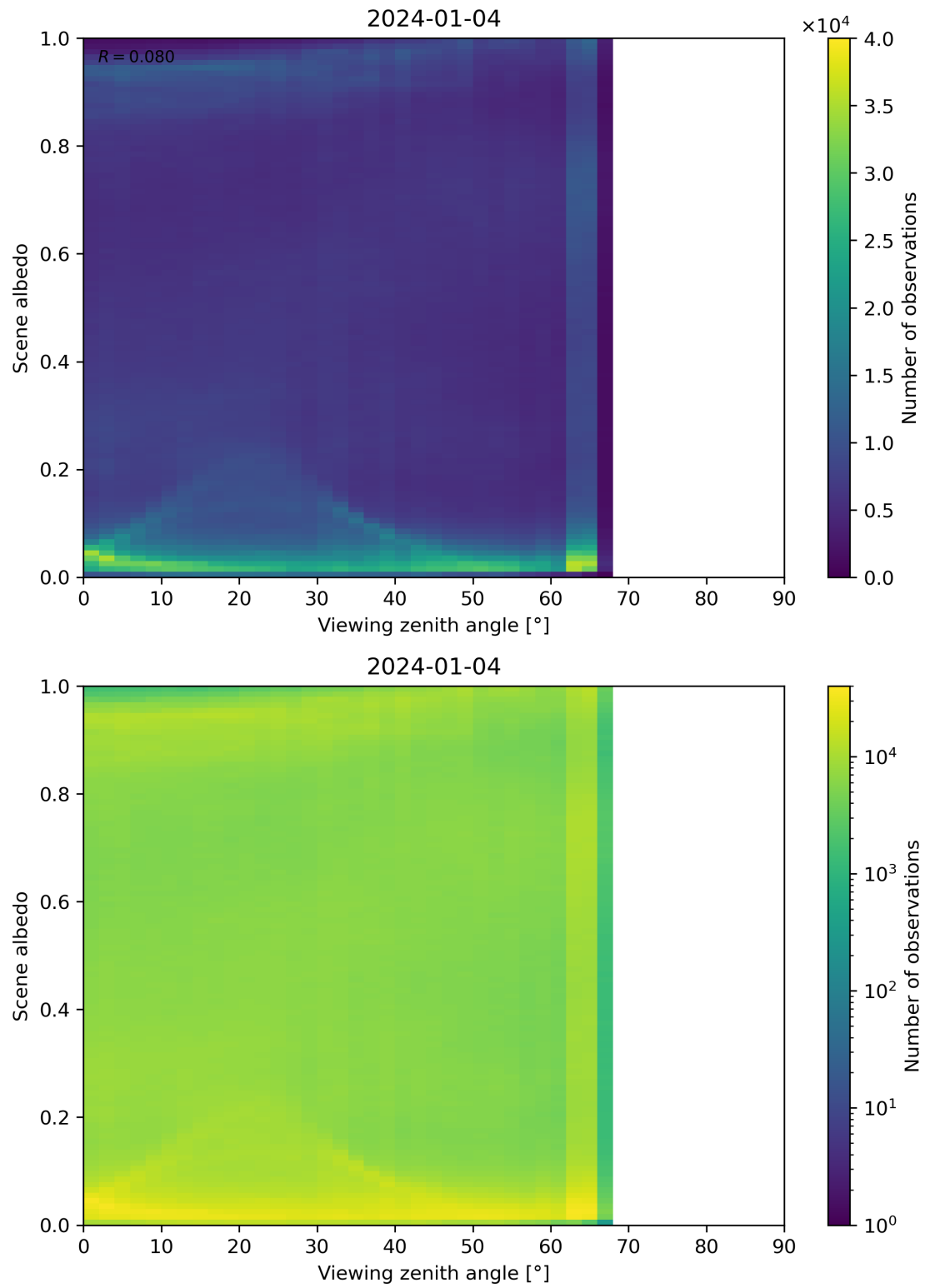
Figure 126: Scatter density plot of “Viewing zenith angle” against “Scene albedo” for 2024-01-03 to 2024-01-05.
