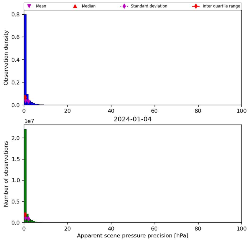
Figure 37: Histogram of “Apparent scene pressure precision” for 2024-01-03 to 2024-01-05
