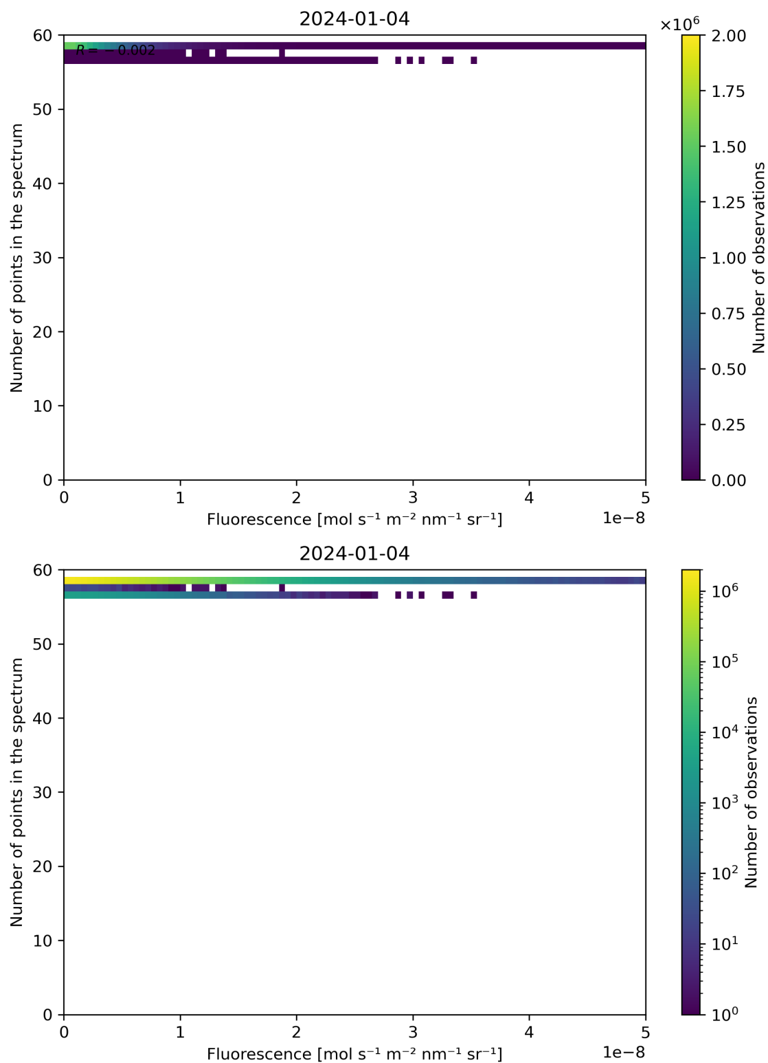
Figure 86: Scatter density plot of “Fluorescence” against “Number of points in the spectrum” for 2024-01-03 to 2024-01-05.
