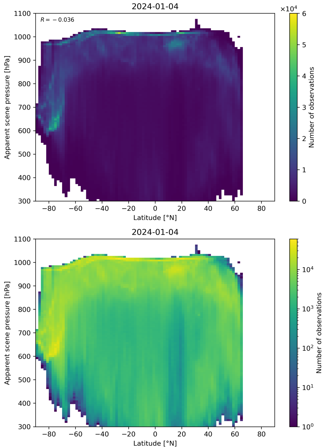
Figure 88: Scatter density plot of “Latitude” against “Apparent scene pressure” for 2024-01-03 to 2024-01-05.
