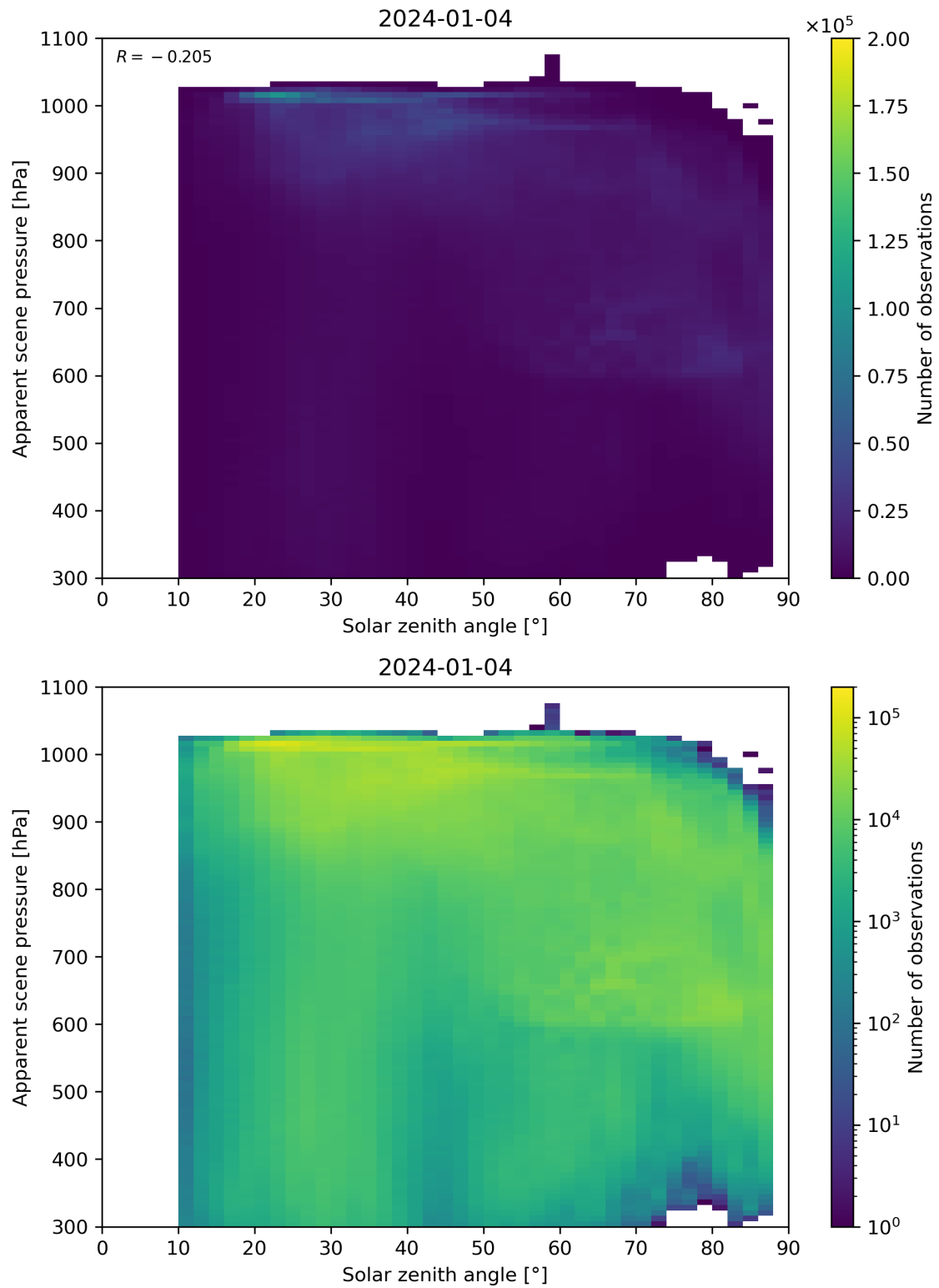
Figure 108: Scatter density plot of “Solar zenith angle” against “Apparent scene pressure” for 2024-01-03 to 2024-01-05.
