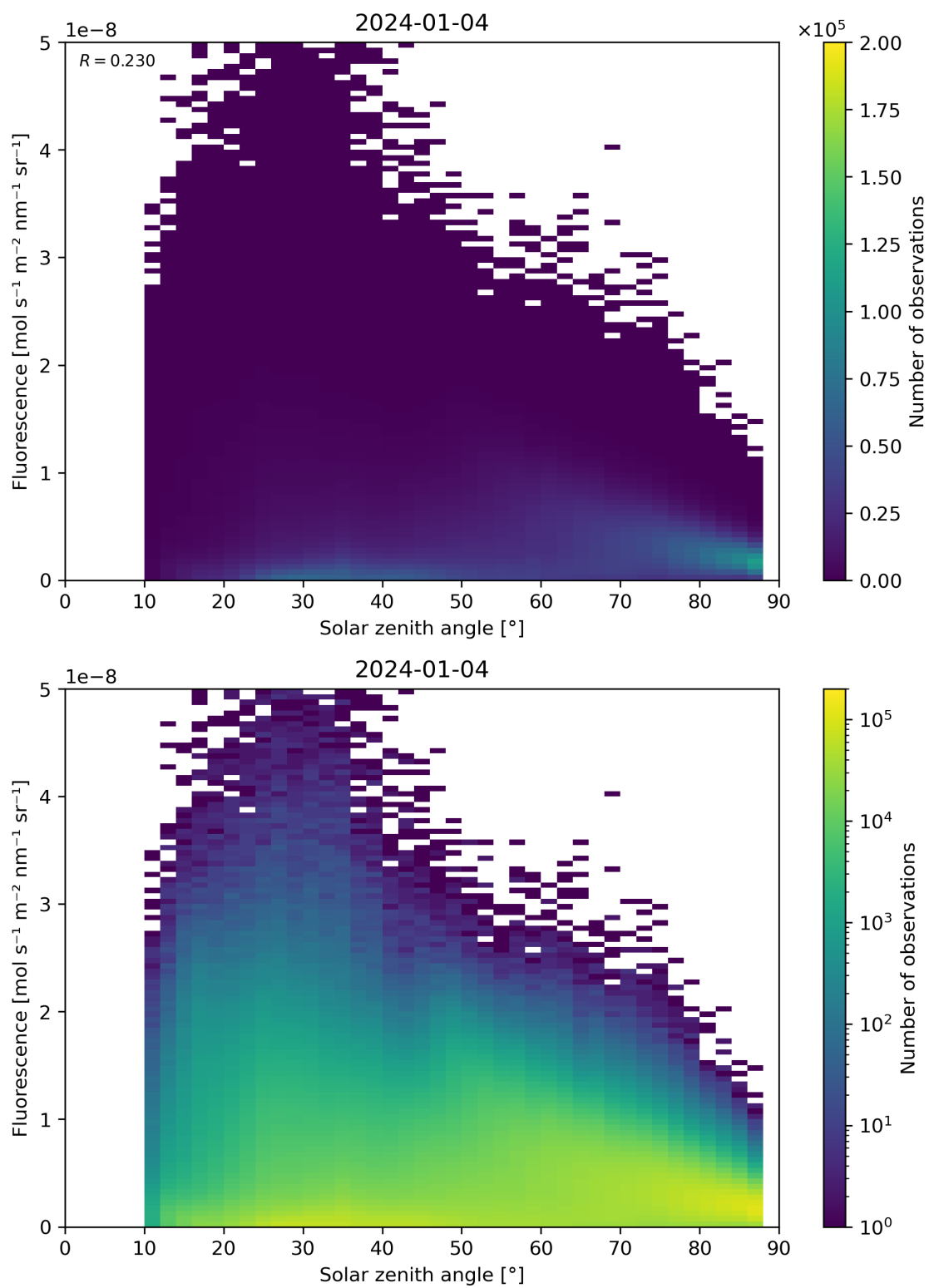
Figure 112: Scatter density plot of “Solar zenith angle” against “Fluorescence” for 2024-01-03 to 2024-01-05.
