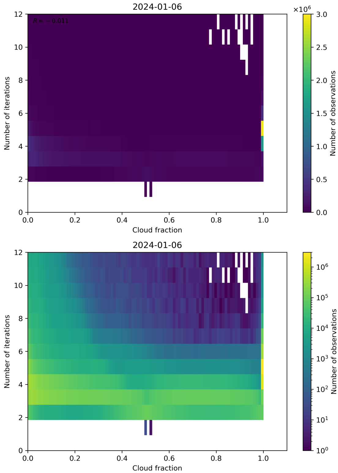
Figure 73: Scatter density plot of “Cloud fraction” against “Number of iterations” for 2024-01-05 to 2024-01-07.
