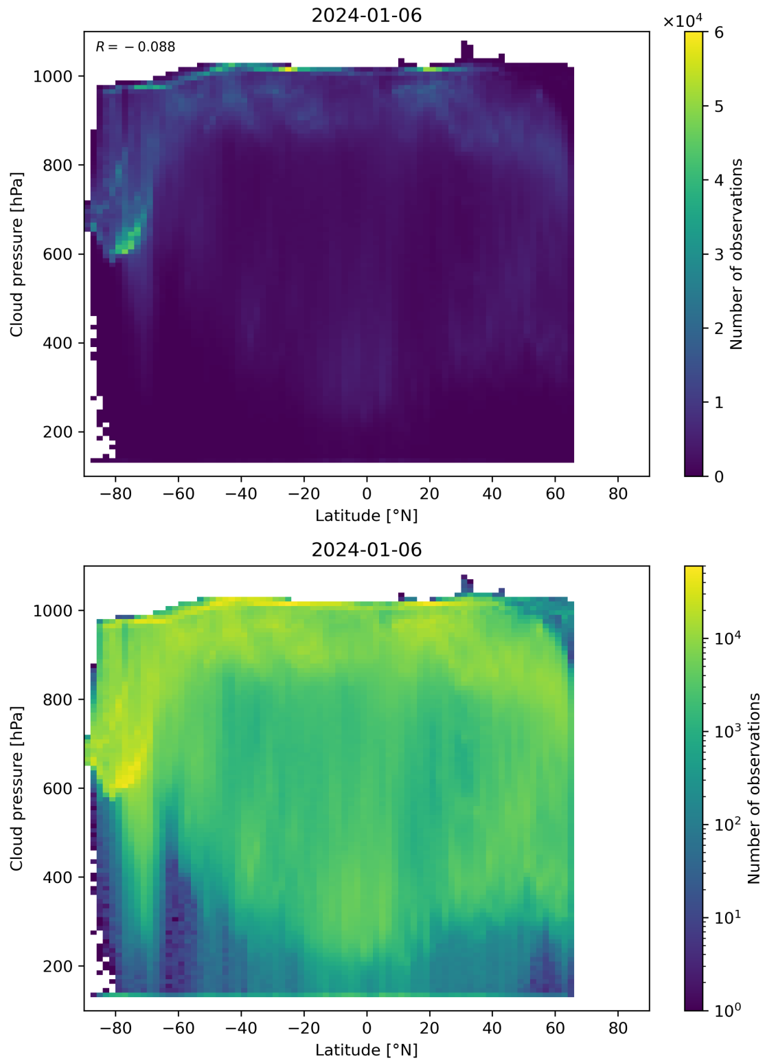
Figure 91: Scatter density plot of “Latitude” against “Cloud pressure” for 2024-01-05 to 2024-01-07.
