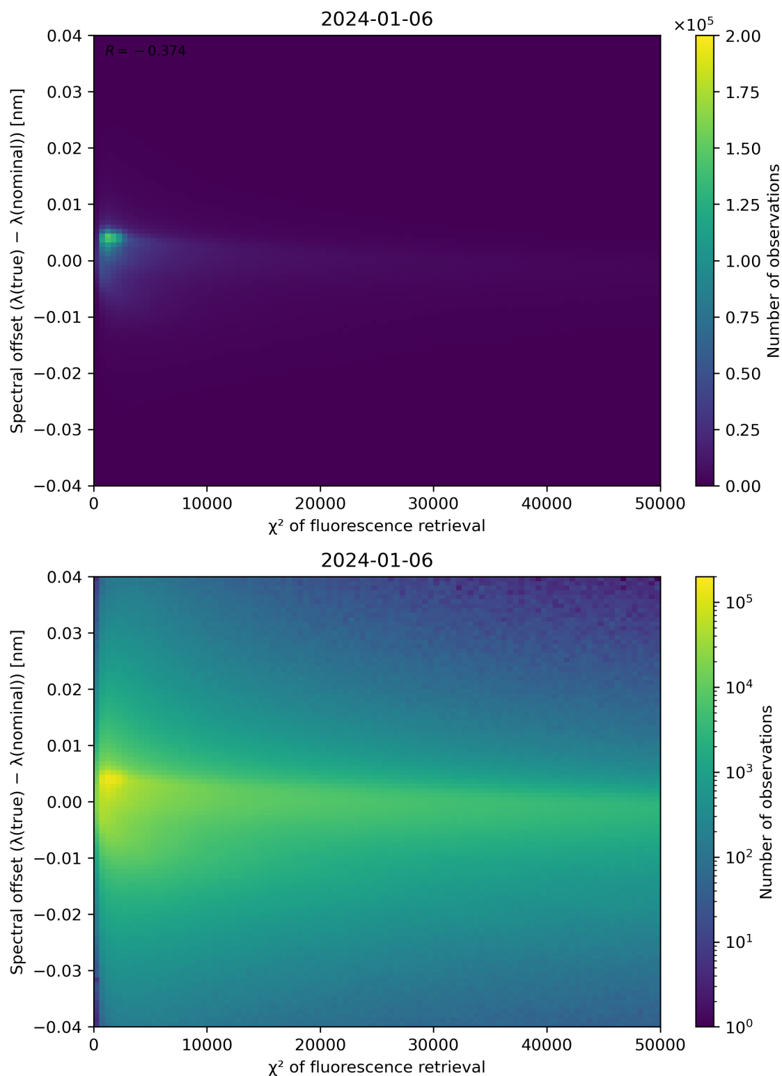
Figure 69: Scatter density plot of " \chi^2 of fluorescence retrieval" against "Spectral offset ( \lambda(\text{true}) - \lambda(\text{nominal}) )" for 2024-01-05 to 2024-01-07.
