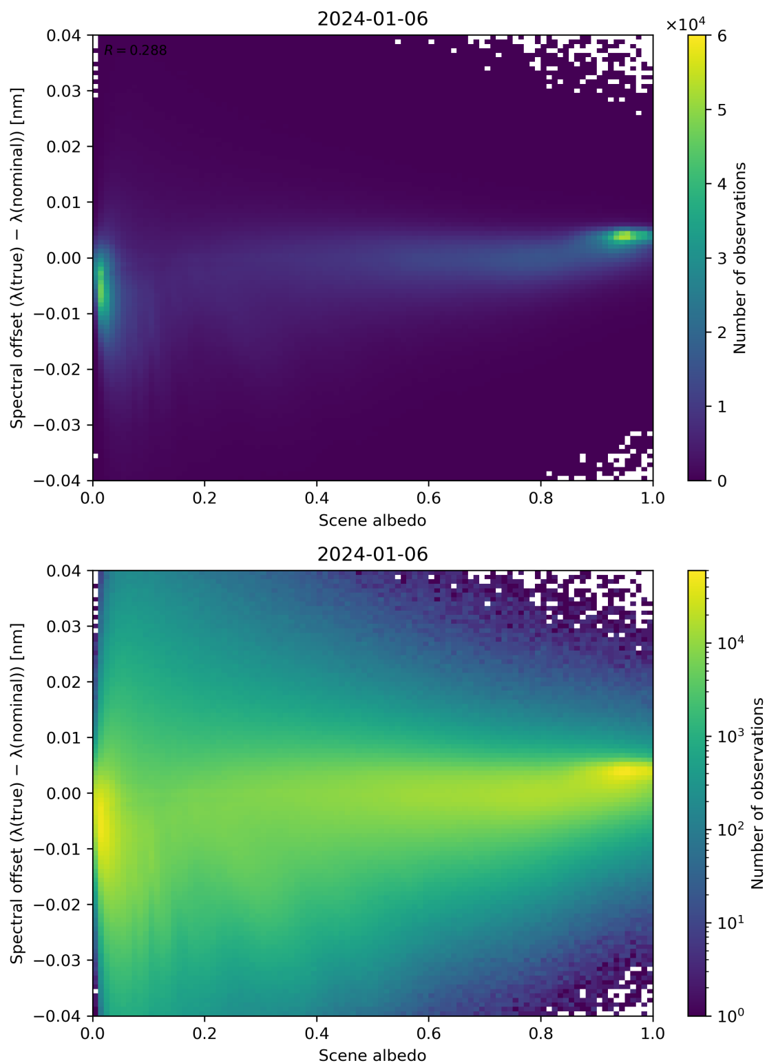
Figure 107: Scatter density plot of “Scene albedo” against “Spectral offset ( \lambda(\text{true}) - \lambda(\text{nominal}) )” for 2024-01-05 to 2024-01-07.
