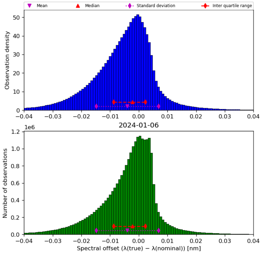
Figure 45: Histogram of “Spectral offset ( \lambda(\text{true}) - \lambda(\text{nominal}) )” for 2024-01-05 to 2024-01-07
