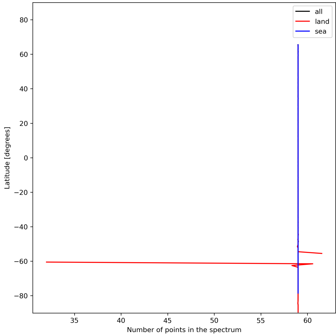
Figure 27: Zonal average of “Number of points in the spectrum” for 2024-01-05 to 2024-01-07.
