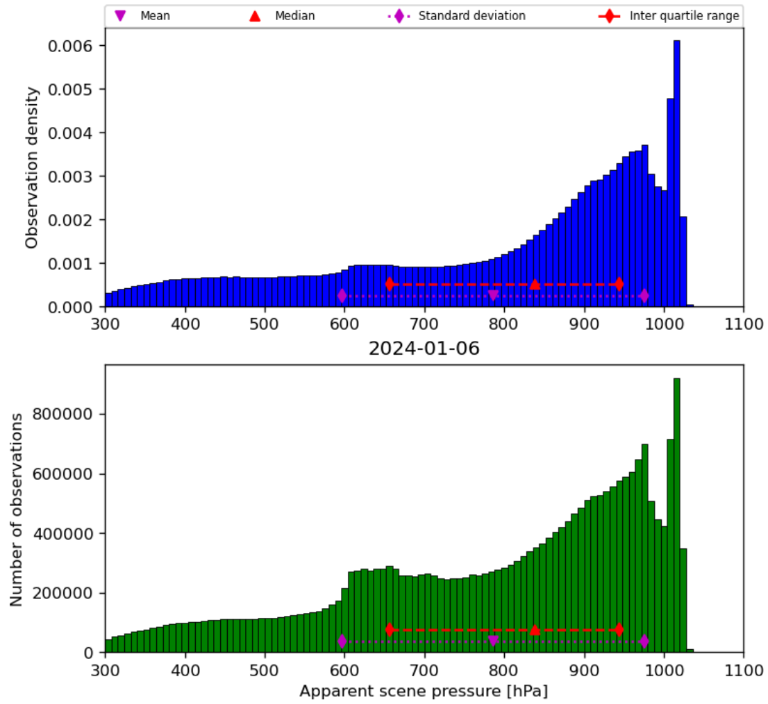
Figure 36: Histogram of “Apparent scene pressure” for 2024-01-05 to 2024-01-07
