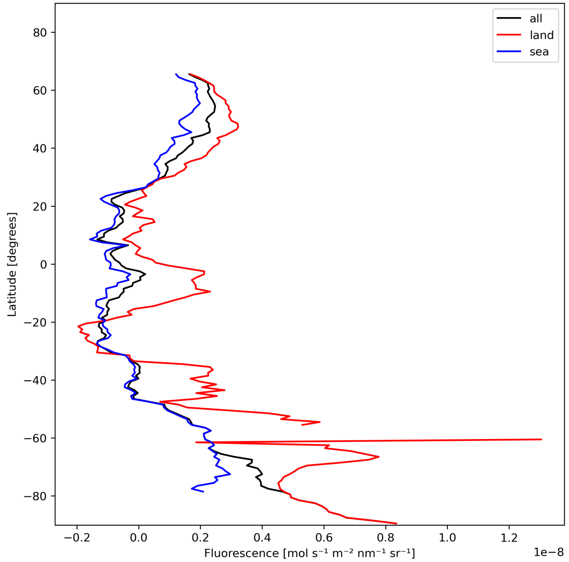
Figure 23: Zonal average of “Fluorescence” for 2024-01-05 to 2024-01-07.
