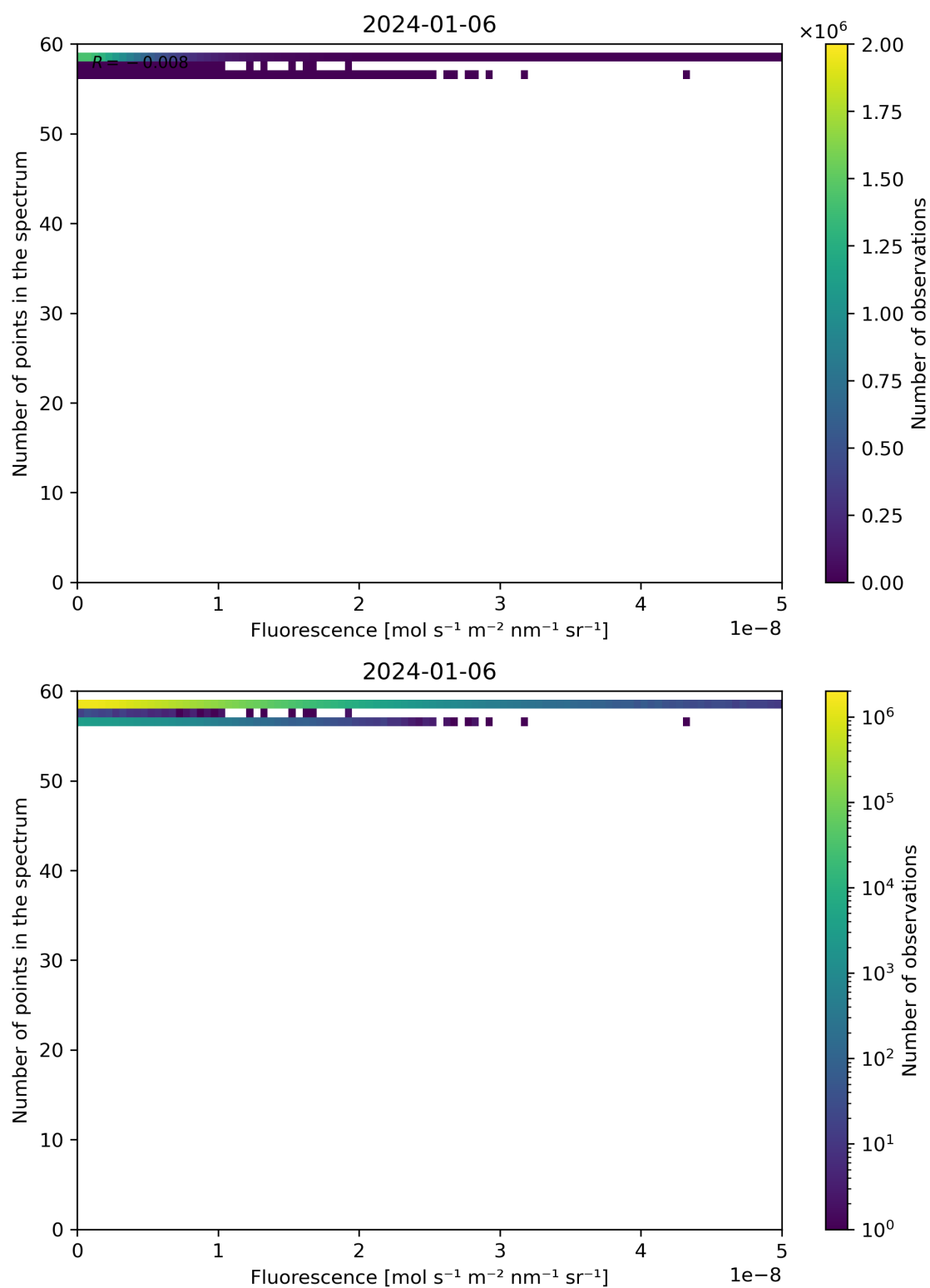
Figure 86: Scatter density plot of “Fluorescence” against “Number of points in the spectrum” for 2024-01-05 to 2024-01-07.
