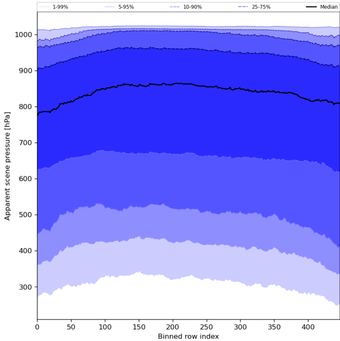
Figure 53: Along track statistics of “Apparent scene pressure” for 2024-01-05 to 2024-01-07
