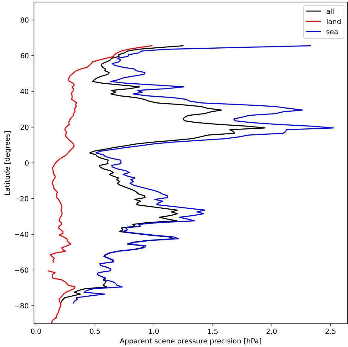
Figure 20: Zonal average of “Apparent scene pressure precision” for 2024-01-05 to 2024-01-07.
