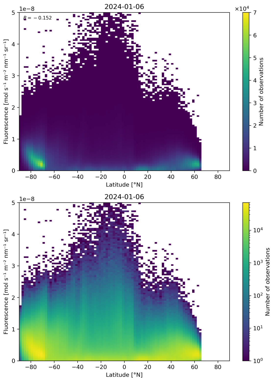
Figure 92: Scatter density plot of “Latitude” against “Fluorescence” for 2024-01-05 to 2024-01-07.
