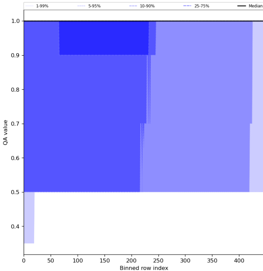
Figure 46: Along track statistics of “QA value” for 2024-01-05 to 2024-01-07
