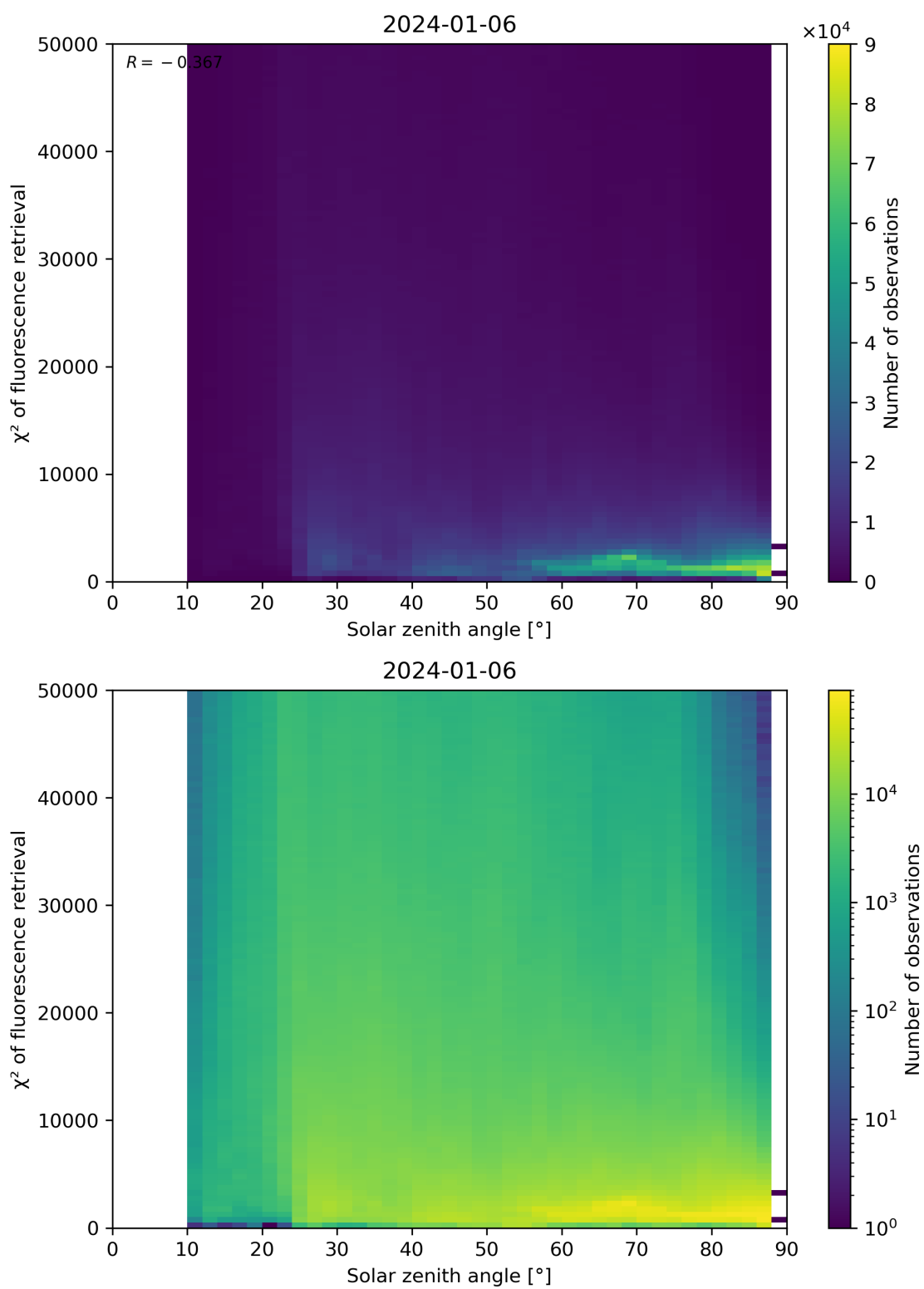
Figure 109: Scatter density plot of “Solar zenith angle” against “ \chi^2 of fluorescence retrieval” for 2024-01-05 to 2024-01-07.
