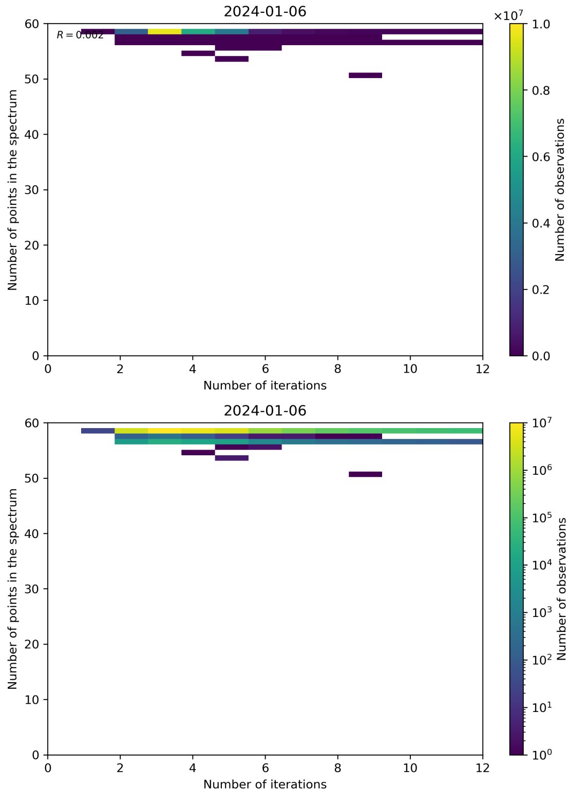
Figure 99: Scatter density plot of “Number of iterations” against “Number of points in the spectrum” for 2024-01-05 to 2024-01-07.
