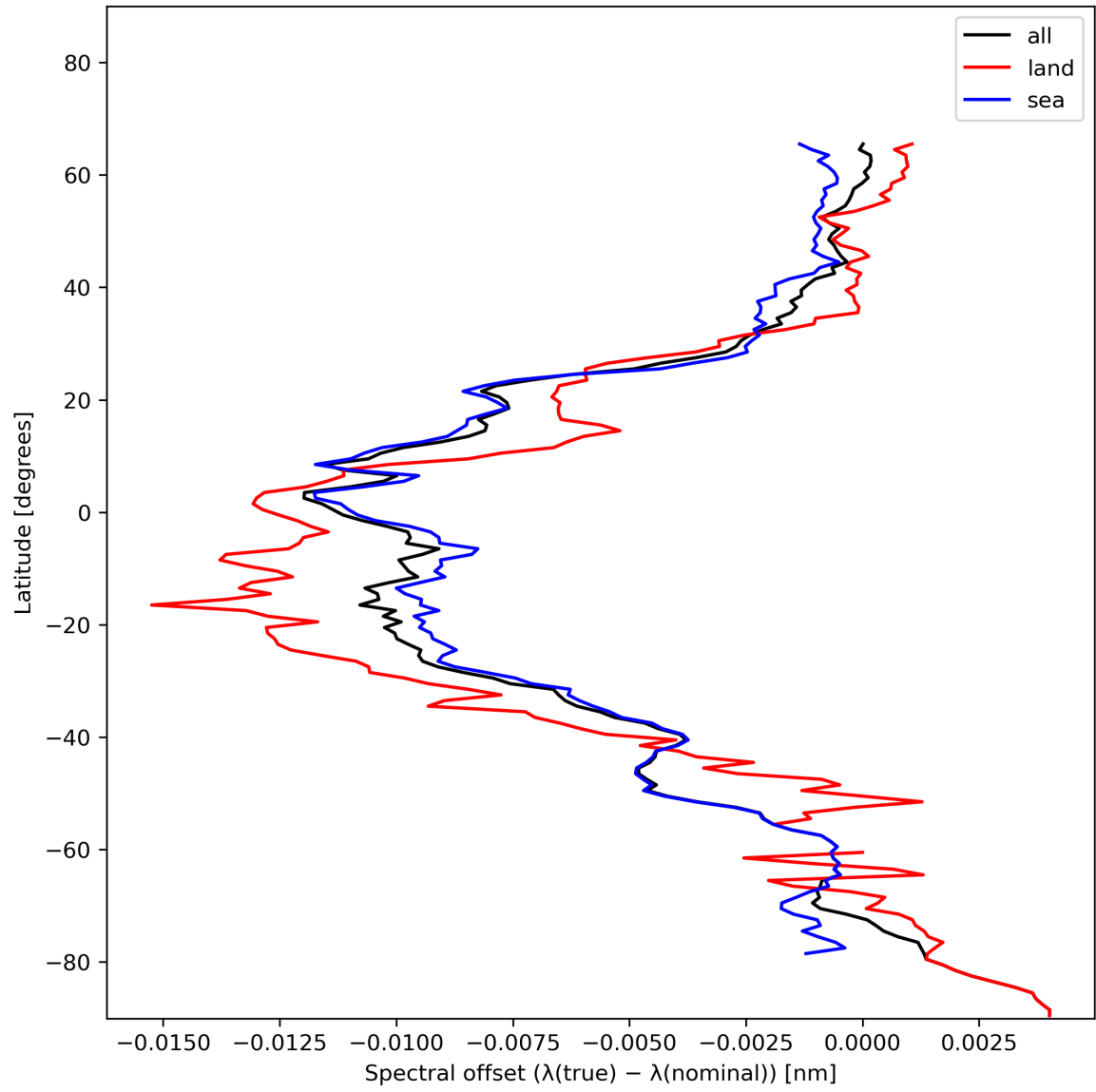
Figure 28: Zonal average of “Spectral offset ( \lambda(\text{true}) - \lambda(\text{nominal}) )” for 2024-01-05 to 2024-01-07.
