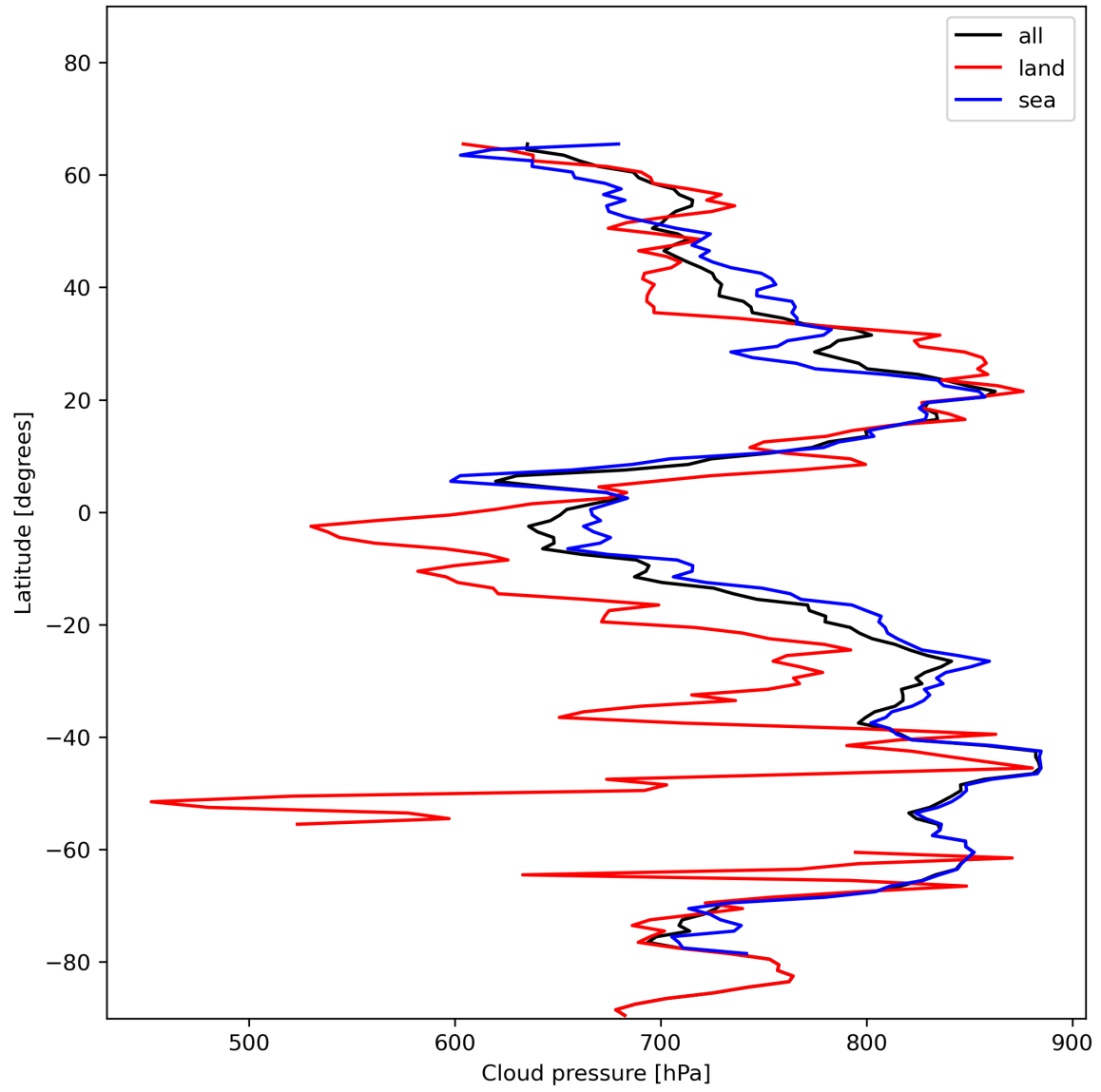
Figure 13: Zonal average of “Cloud pressure” for 2024-01-05 to 2024-01-07.
