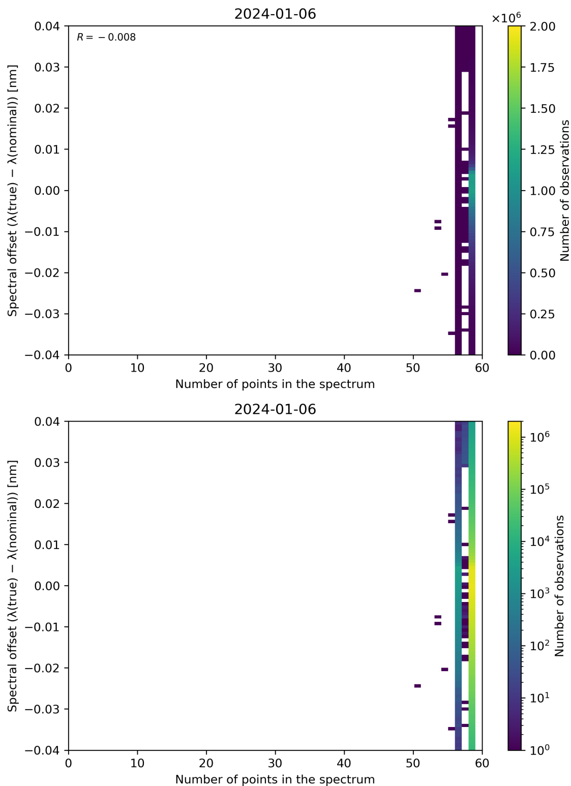
Figure 101: Scatter density plot of “Number of points in the spectrum” against “Spectral offset ( \lambda(\text{true}) - \lambda(\text{nominal}) )” for 2024-01-05 to 2024-01-07.
