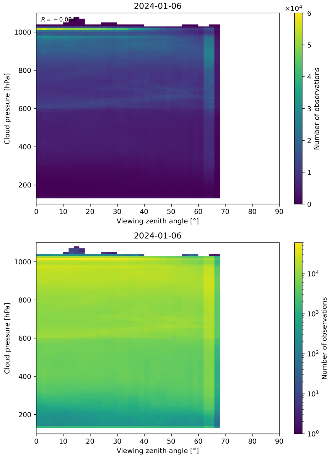
Figure 121: Scatter density plot of “Viewing zenith angle” against “Cloud pressure” for 2024-01-05 to 2024-01-07.
