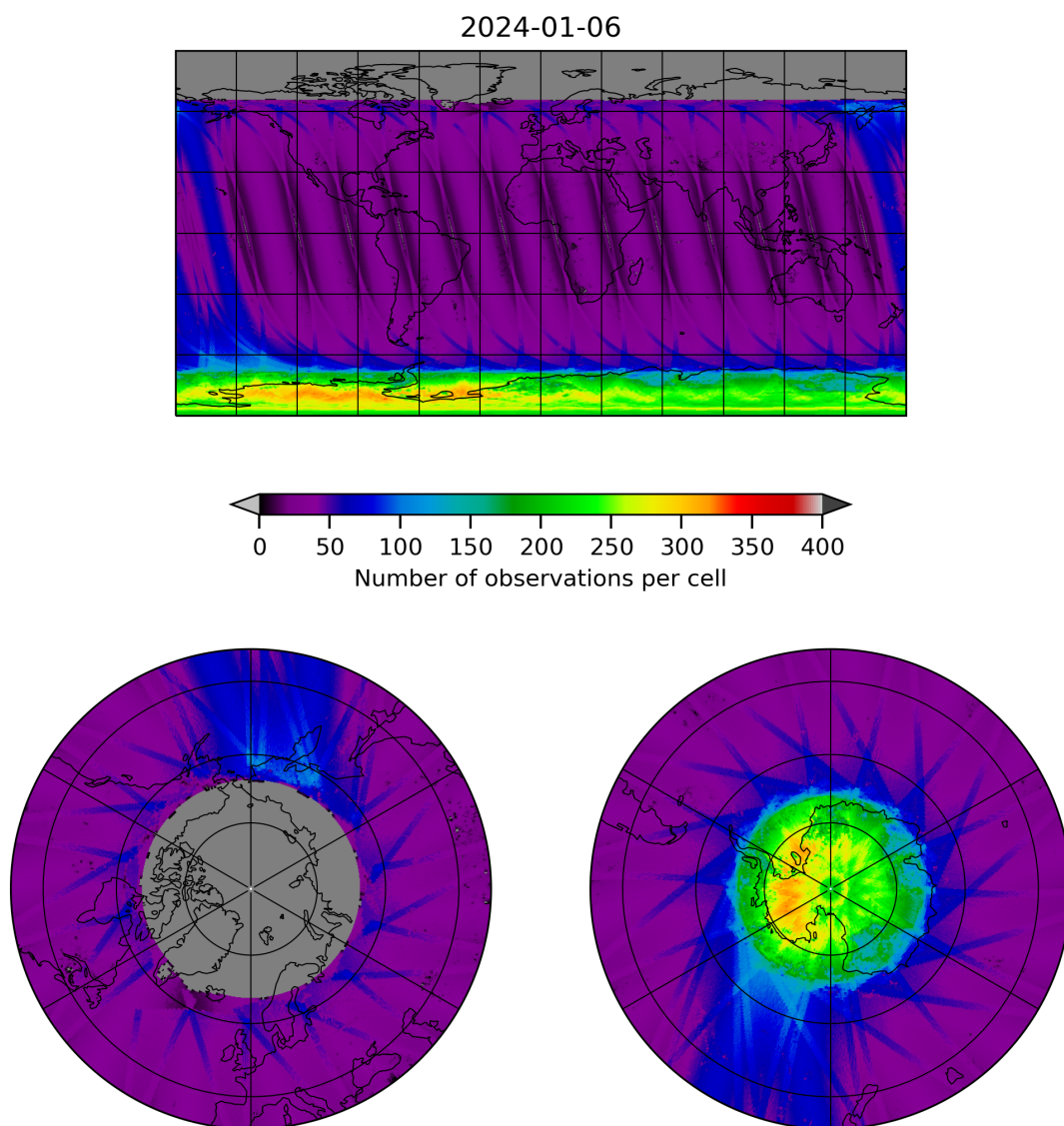
Figure 11: Map of the number of observations for 2024-01-05 to 2024-01-07
