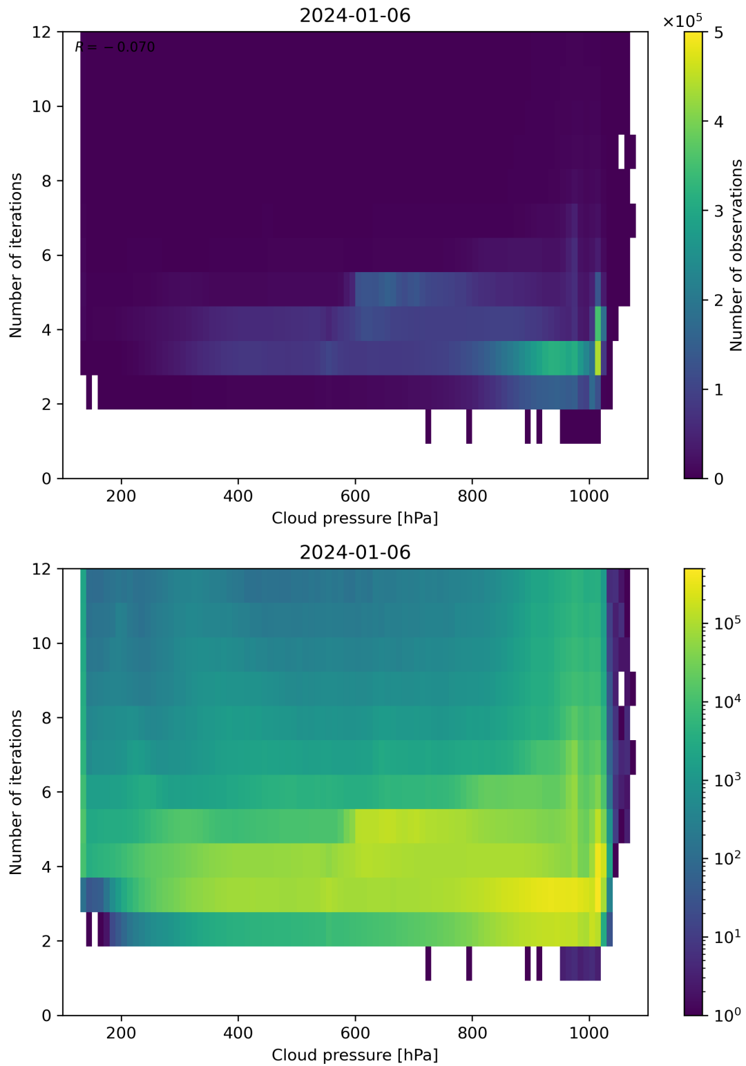
Figure 81: Scatter density plot of “Cloud pressure” against “Number of iterations” for 2024-01-05 to 2024-01-07.
