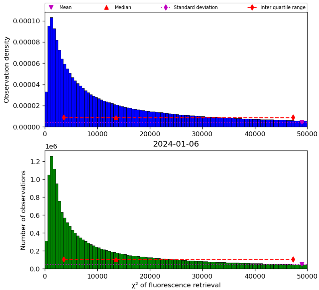
Figure 42: Histogram of “ \chi^2 of fluorescence retrieval” for 2024-01-05 to 2024-01-07
