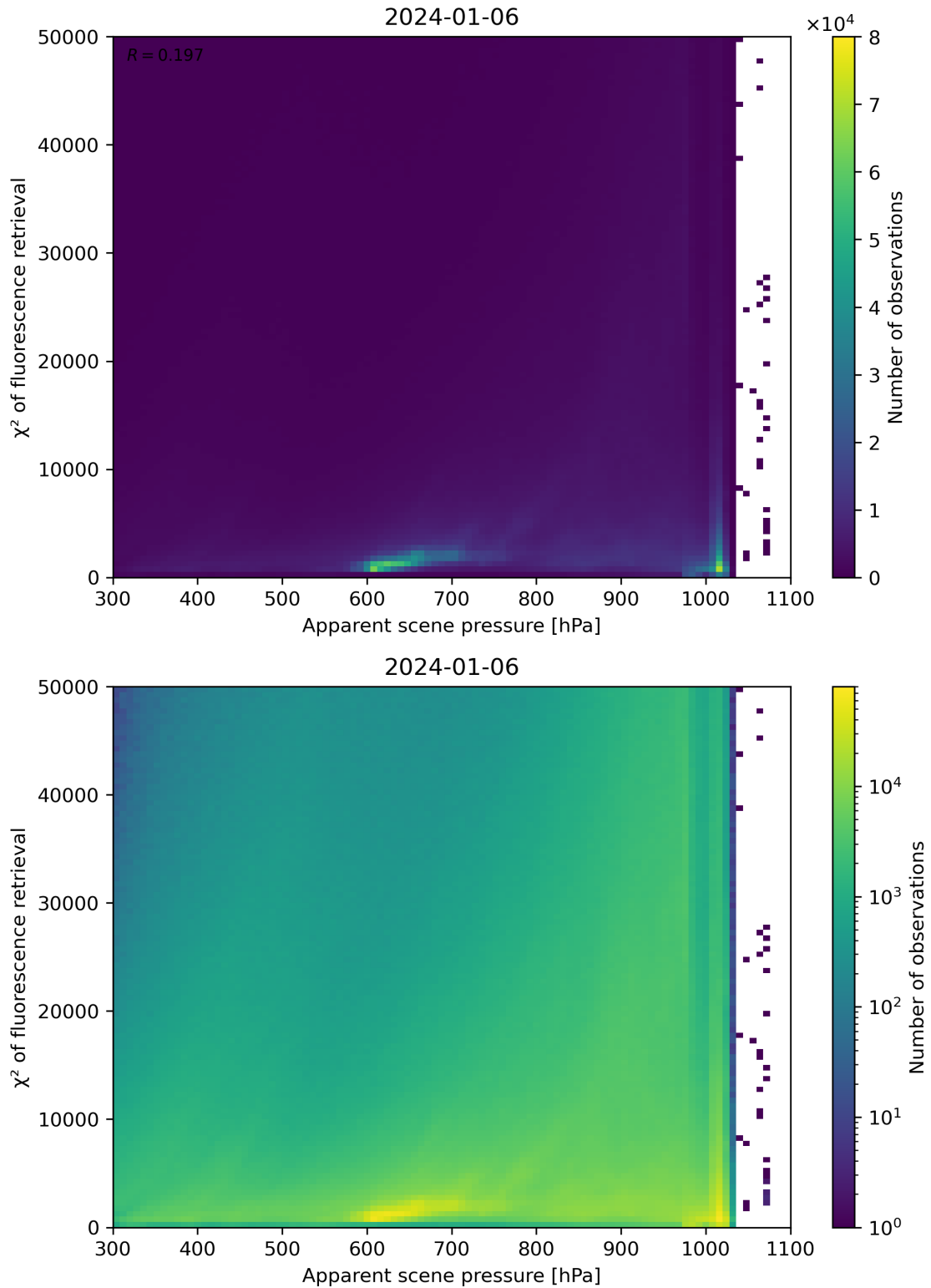
Figure 63: Scatter density plot of “Apparent scene pressure” against “ \chi^2 of fluorescence retrieval” for 2024-01-05 to 2024-01-07.
