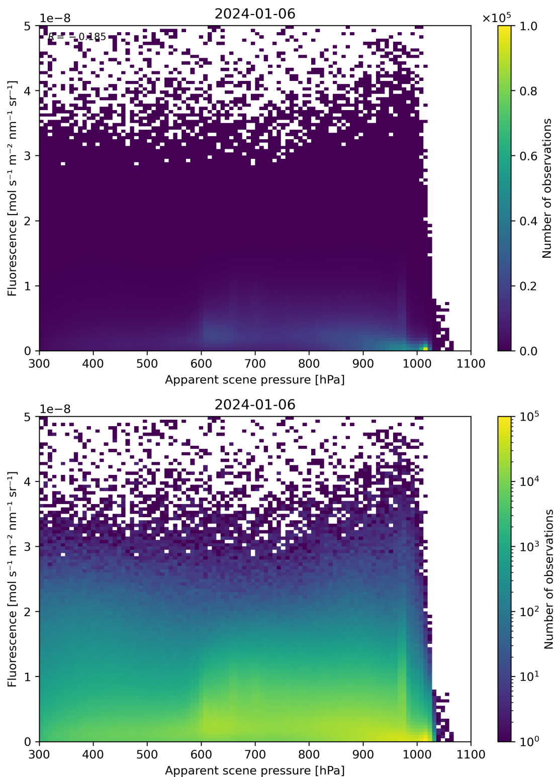
Figure 64: Scatter density plot of “Apparent scene pressure” against “Fluorescence” for 2024-01-05 to 2024-01-07.
