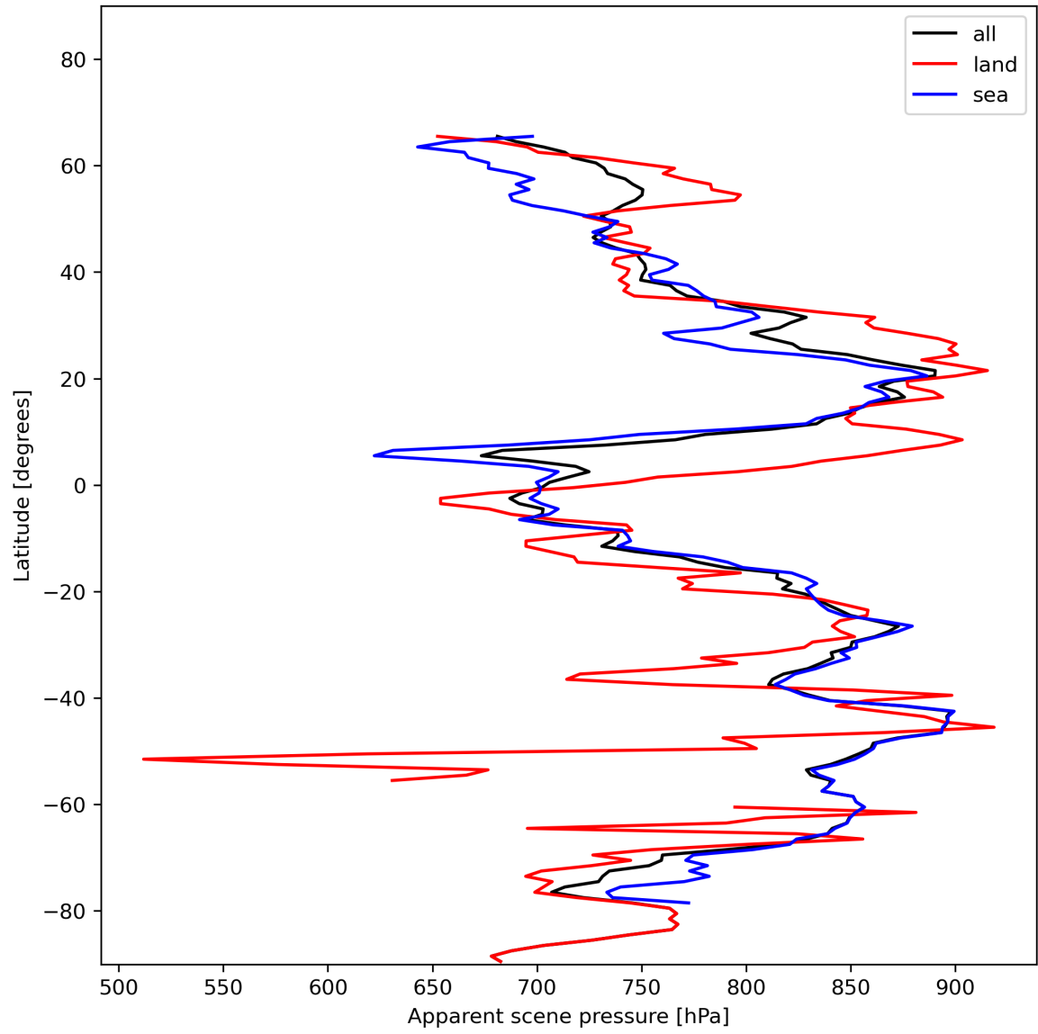
Figure 19: Zonal average of “Apparent scene pressure” for 2024-01-05 to 2024-01-07.
