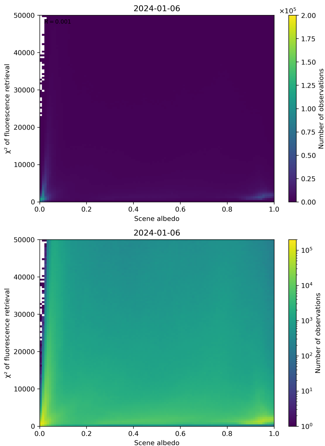
Figure 103: Scatter density plot of “Scene albedo” against “ \chi^2 of fluorescence retrieval” for 2024-01-05 to 2024-01-07.
