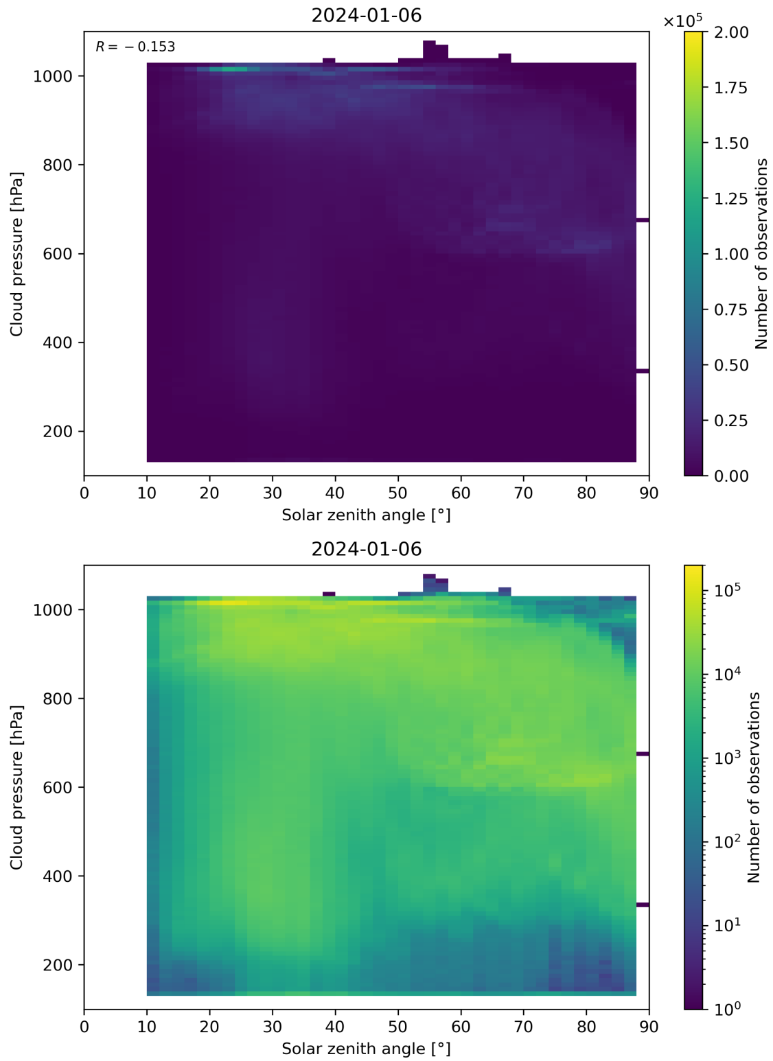
Figure 111: Scatter density plot of “Solar zenith angle” against “Cloud pressure” for 2024-01-05 to 2024-01-07.
