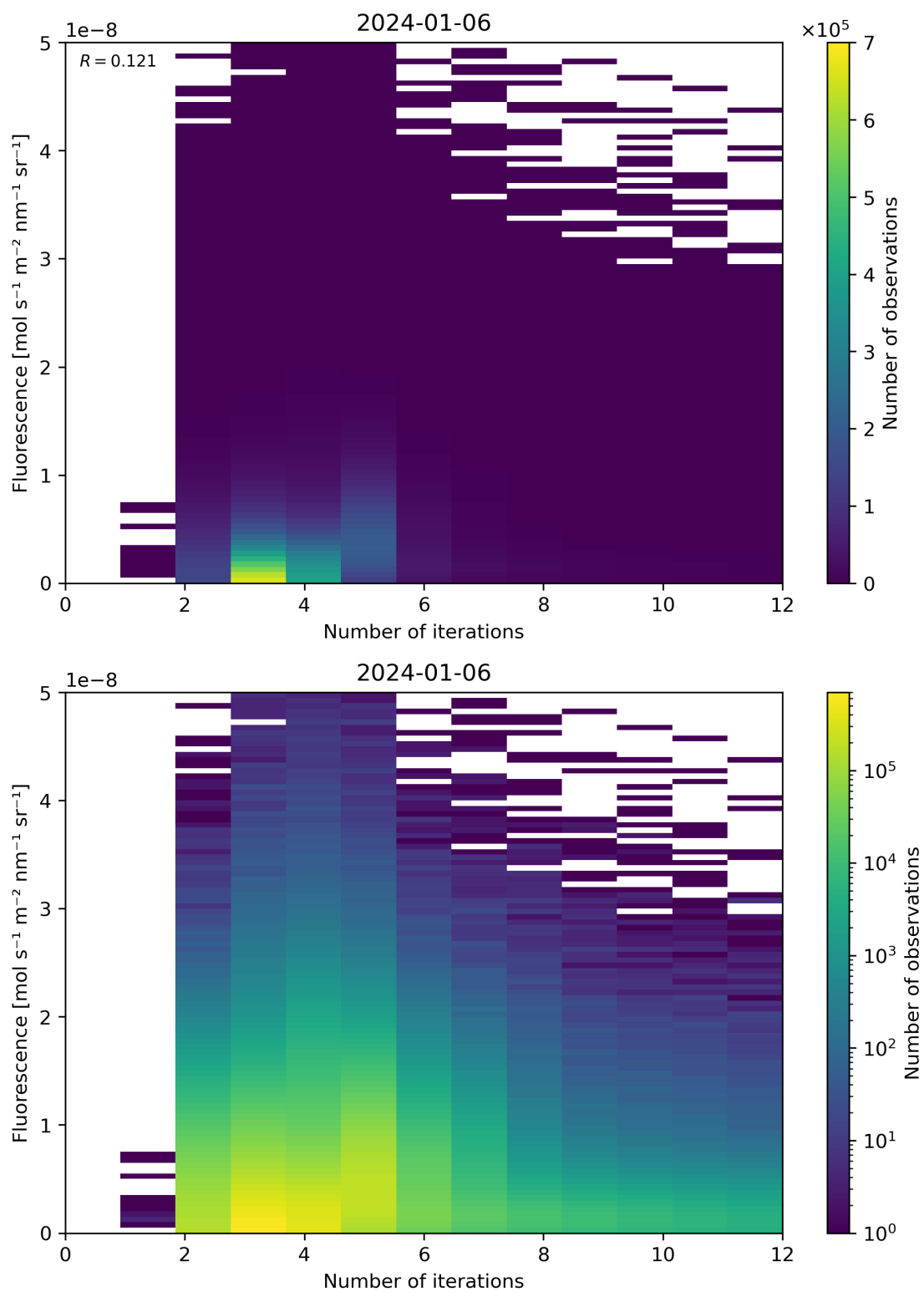
Figure 98: Scatter density plot of “Number of iterations” against “Fluorescence” for 2024-01-05 to 2024-01-07.
