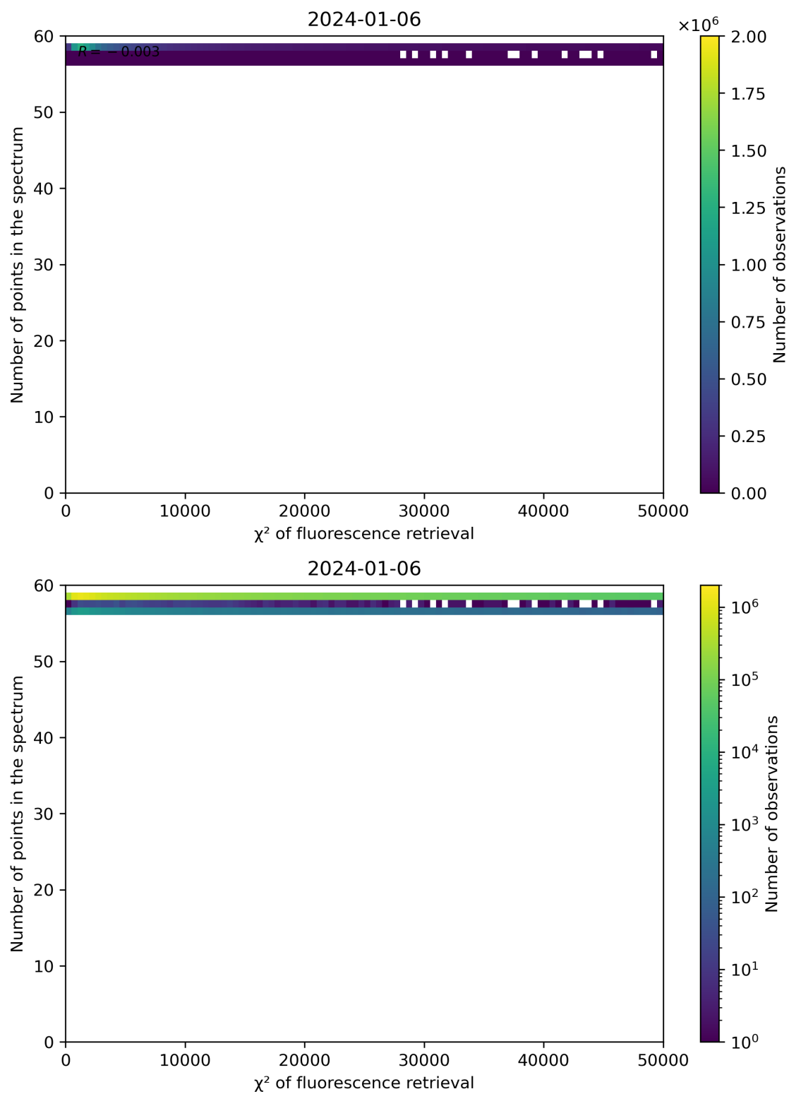
Figure 68: Scatter density plot of " \chi^2 of fluorescence retrieval" against "Number of points in the spectrum" for 2024-01-05 to 2024-01-07.
