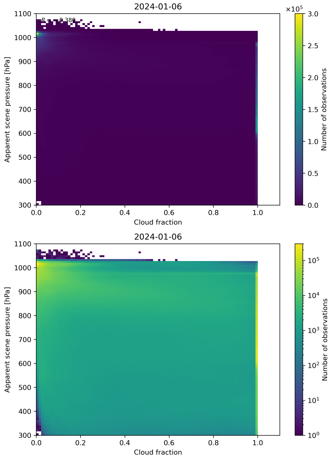
Figure 70: Scatter density plot of “Cloud fraction” against “Apparent scene pressure” for 2024-01-05 to 2024-01-07.
