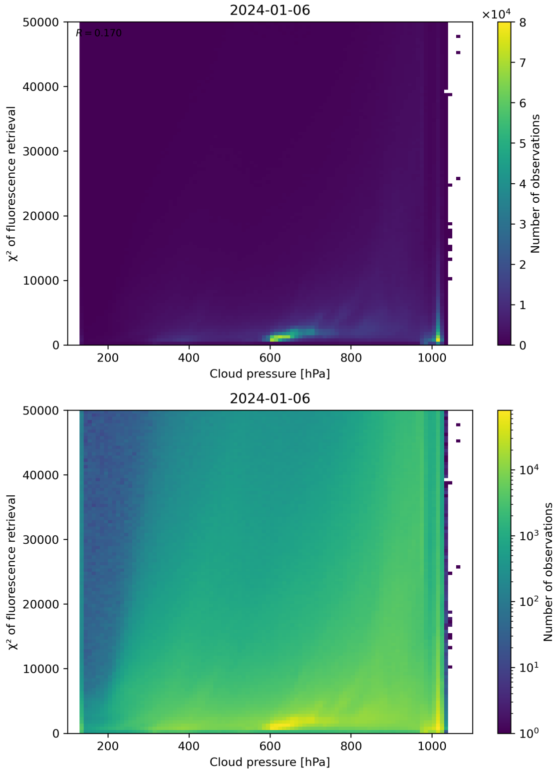
Figure 78: Scatter density plot of “Cloud pressure” against “ \chi^2 of fluorescence retrieval” for 2024-01-05 to 2024-01-07.
