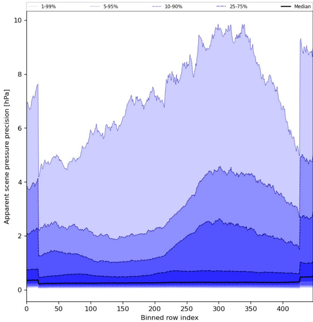
Figure 54: Along track statistics of “Apparent scene pressure precision” for 2024-01-05 to 2024-01-07
