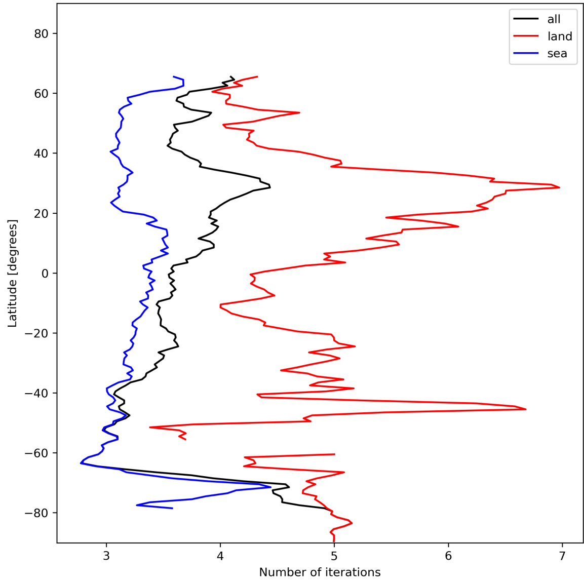
Figure 22: Zonal average of “Number of iterations” for 2024-01-05 to 2024-01-07.
