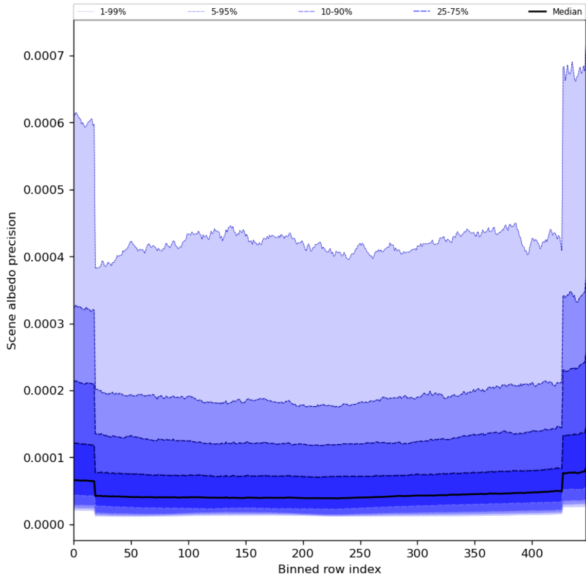
Figure 52: Along track statistics of “Scene albedo precision” for 2024-01-05 to 2024-01-07
