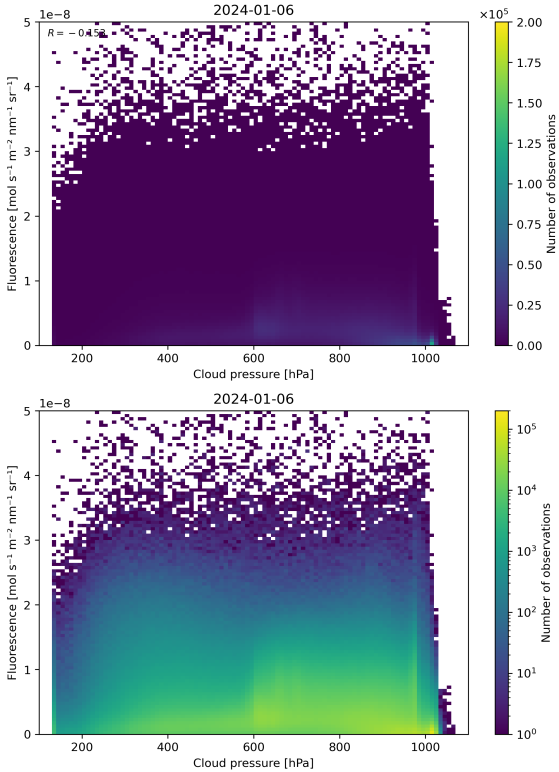
Figure 80: Scatter density plot of “Cloud pressure” against “Fluorescence” for 2024-01-05 to 2024-01-07.
