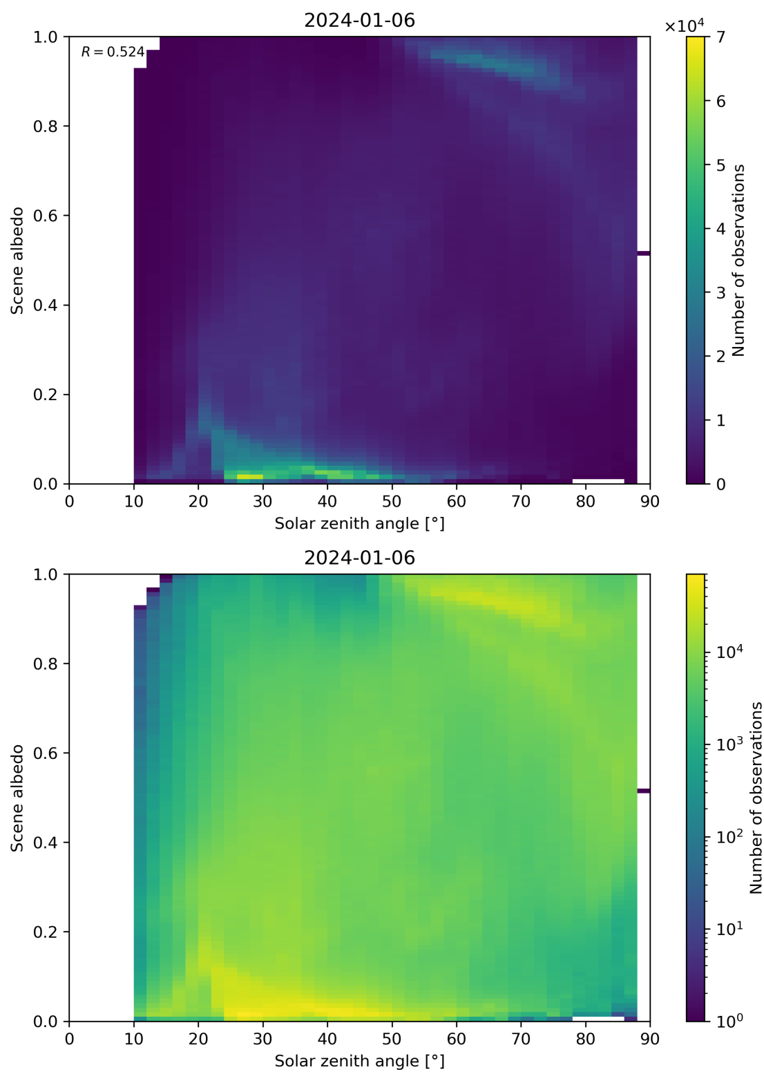
Figure 116: Scatter density plot of “Solar zenith angle” against “Scene albedo” for 2024-01-05 to 2024-01-07.
