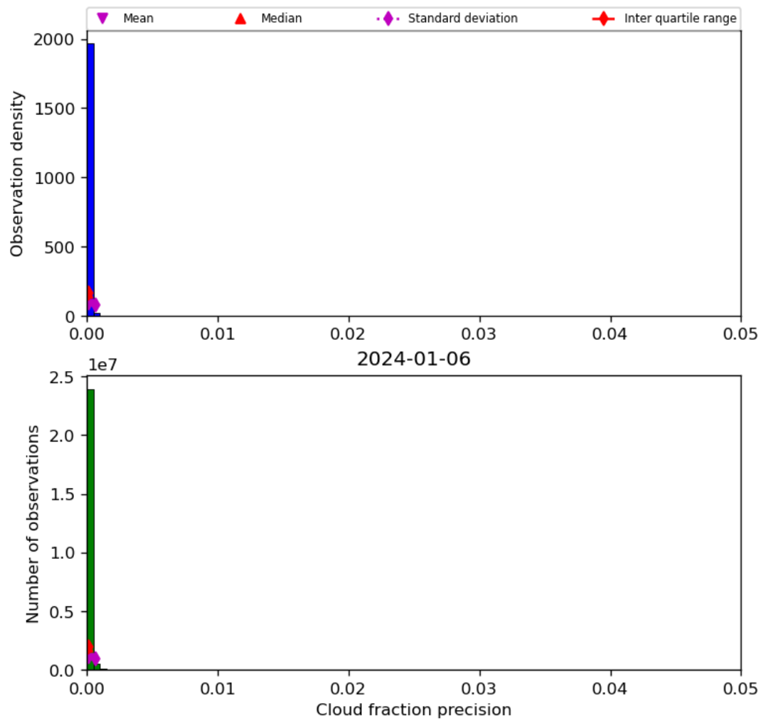
Figure 33: Histogram of “Cloud fraction precision” for 2024-01-05 to 2024-01-07
