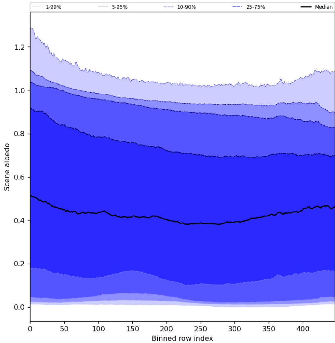
Figure 51: Along track statistics of “Scene albedo” for 2024-01-05 to 2024-01-07
