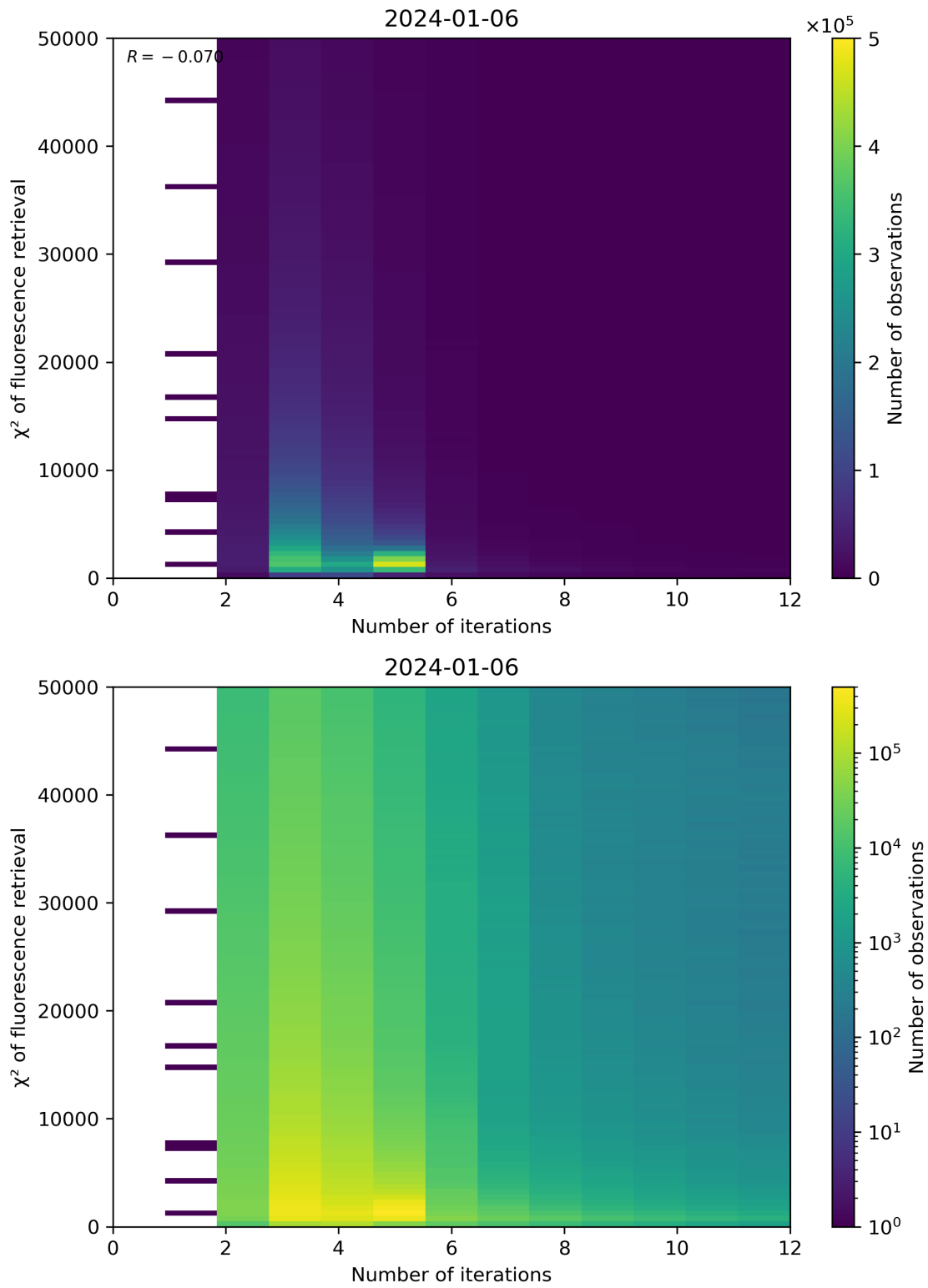
Figure 97: Scatter density plot of “Number of iterations” against “ \chi^2 of fluorescence retrieval” for 2024-01-05 to 2024-01-07.
