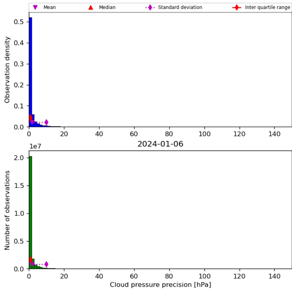
Figure 31: Histogram of “Cloud pressure precision” for 2024-01-05 to 2024-01-07
