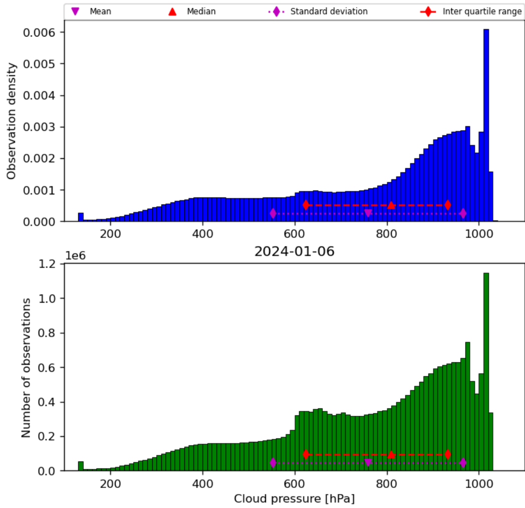
Figure 30: Histogram of “Cloud pressure” for 2024-01-05 to 2024-01-07
