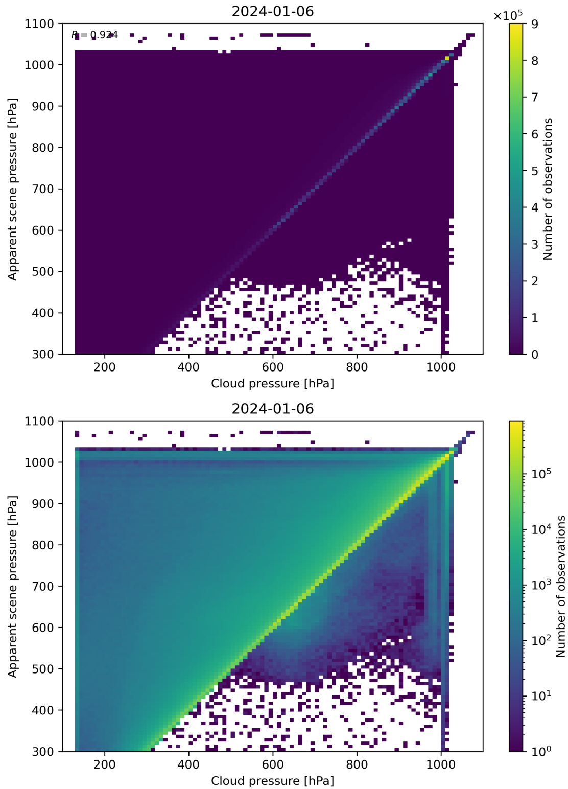
Figure 77: Scatter density plot of “Cloud pressure” against “Apparent scene pressure” for 2024-01-05 to 2024-01-07.
