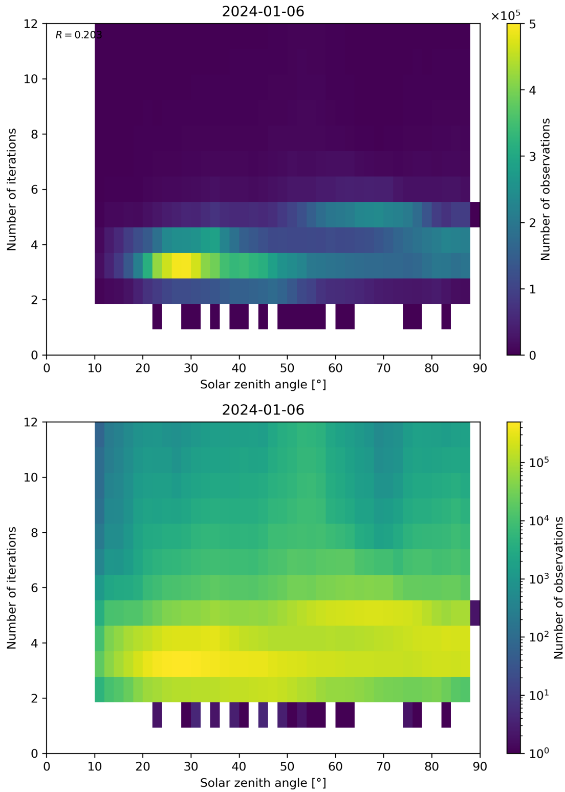
Figure 114: Scatter density plot of “Solar zenith angle” against “Number of iterations” for 2024-01-05 to 2024-01-07.
