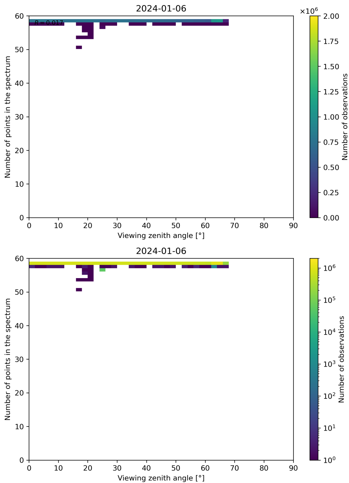
Figure 125: Scatter density plot of “Viewing zenith angle” against “Number of points in the spectrum” for 2024-01-05 to 2024-01-07.
