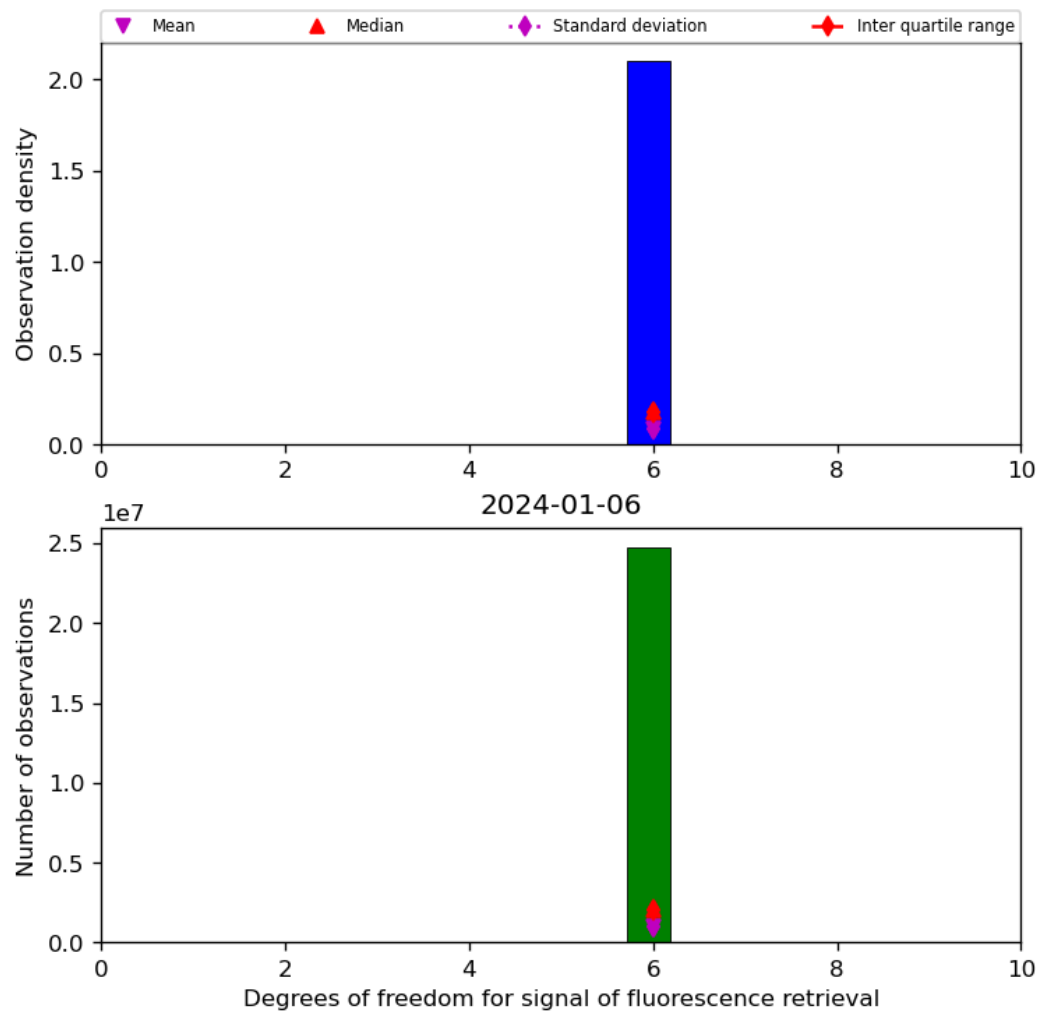
Figure 43: Histogram of “Degrees of freedom for signal of fluorescence retrieval” for 2024-01-05 to 2024-01-07
