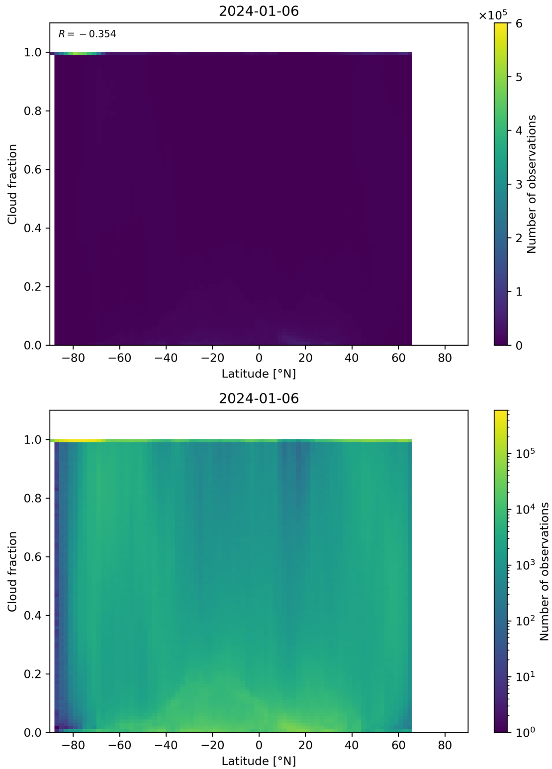
Figure 90: Scatter density plot of “Latitude” against “Cloud fraction” for 2024-01-05 to 2024-01-07.
