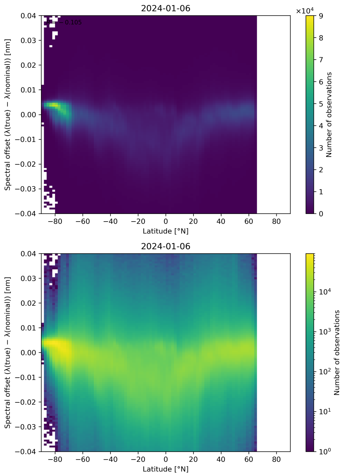
Figure 96: Scatter density plot of “Latitude” against “Spectral offset ( \lambda(\text{true}) - \lambda(\text{nominal}) )” for 2024-01-05 to 2024-01-07.
