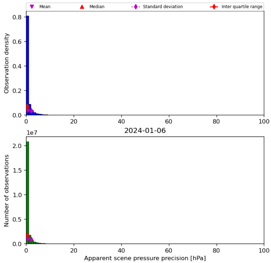
Figure 37: Histogram of “Apparent scene pressure precision” for 2024-01-05 to 2024-01-07
