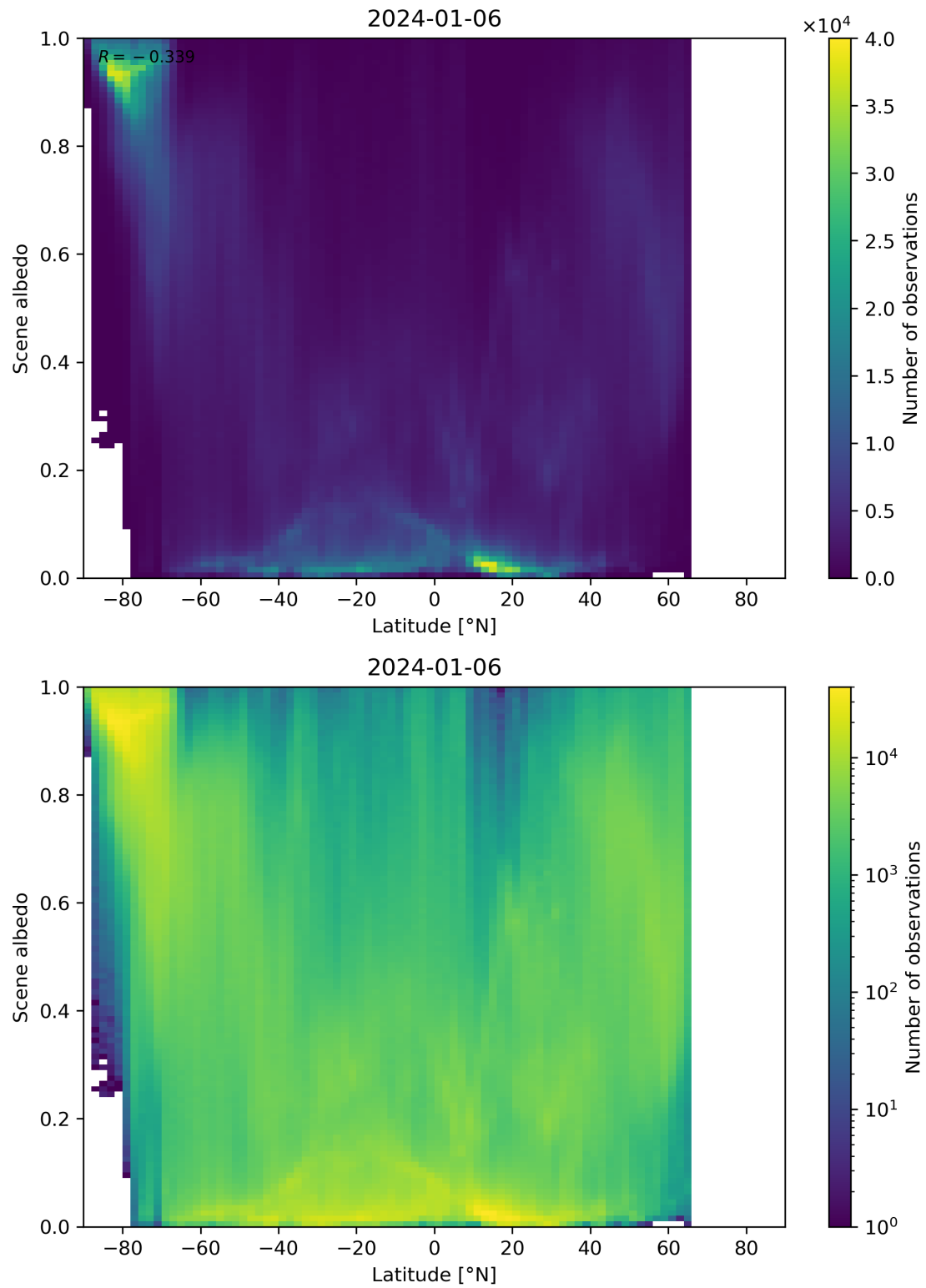
Figure 95: Scatter density plot of “Latitude” against “Scene albedo” for 2024-01-05 to 2024-01-07.
