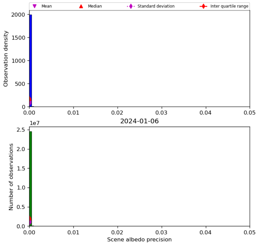
Figure 35: Histogram of “Scene albedo precision” for 2024-01-05 to 2024-01-07
