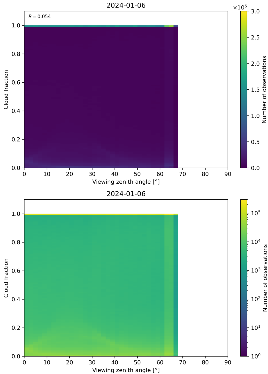
Figure 120: Scatter density plot of “Viewing zenith angle” against “Cloud fraction” for 2024-01-05 to 2024-01-07.
