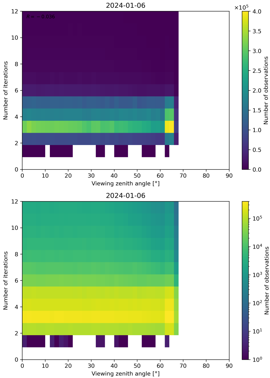
Figure 124: Scatter density plot of “Viewing zenith angle” against “Number of iterations” for 2024-01-05 to 2024-01-07.
