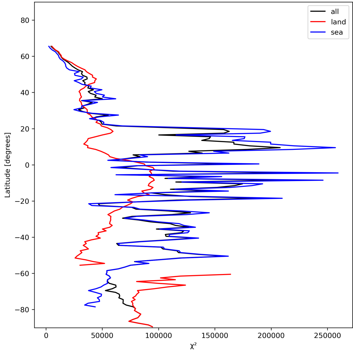
Figure 21: Zonal average of “ \chi^2 ” for 2024-01-05 to 2024-01-07.
