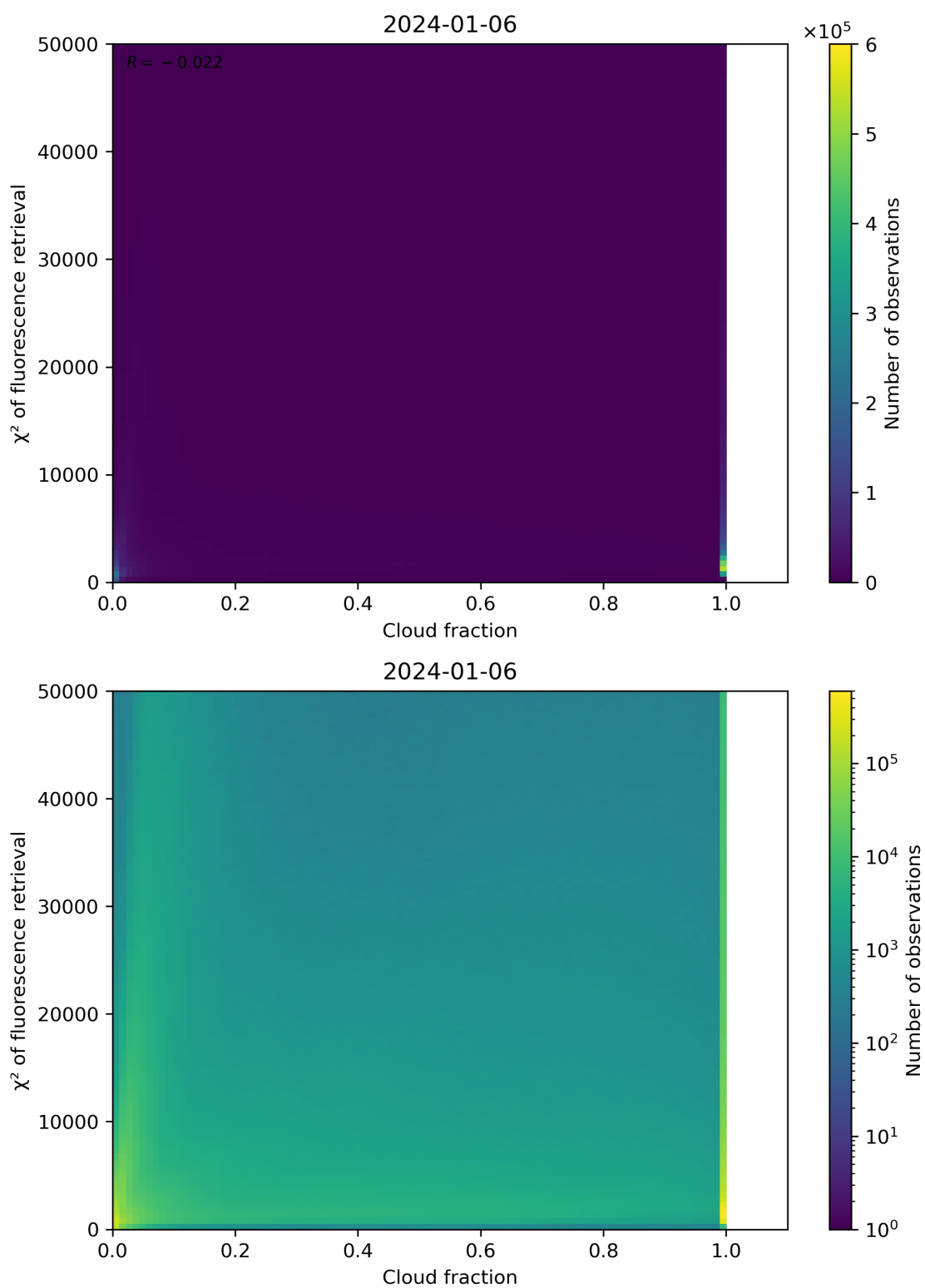
Figure 71: Scatter density plot of “Cloud fraction” against “ \chi^2 of fluorescence retrieval” for 2024-01-05 to 2024-01-07.
