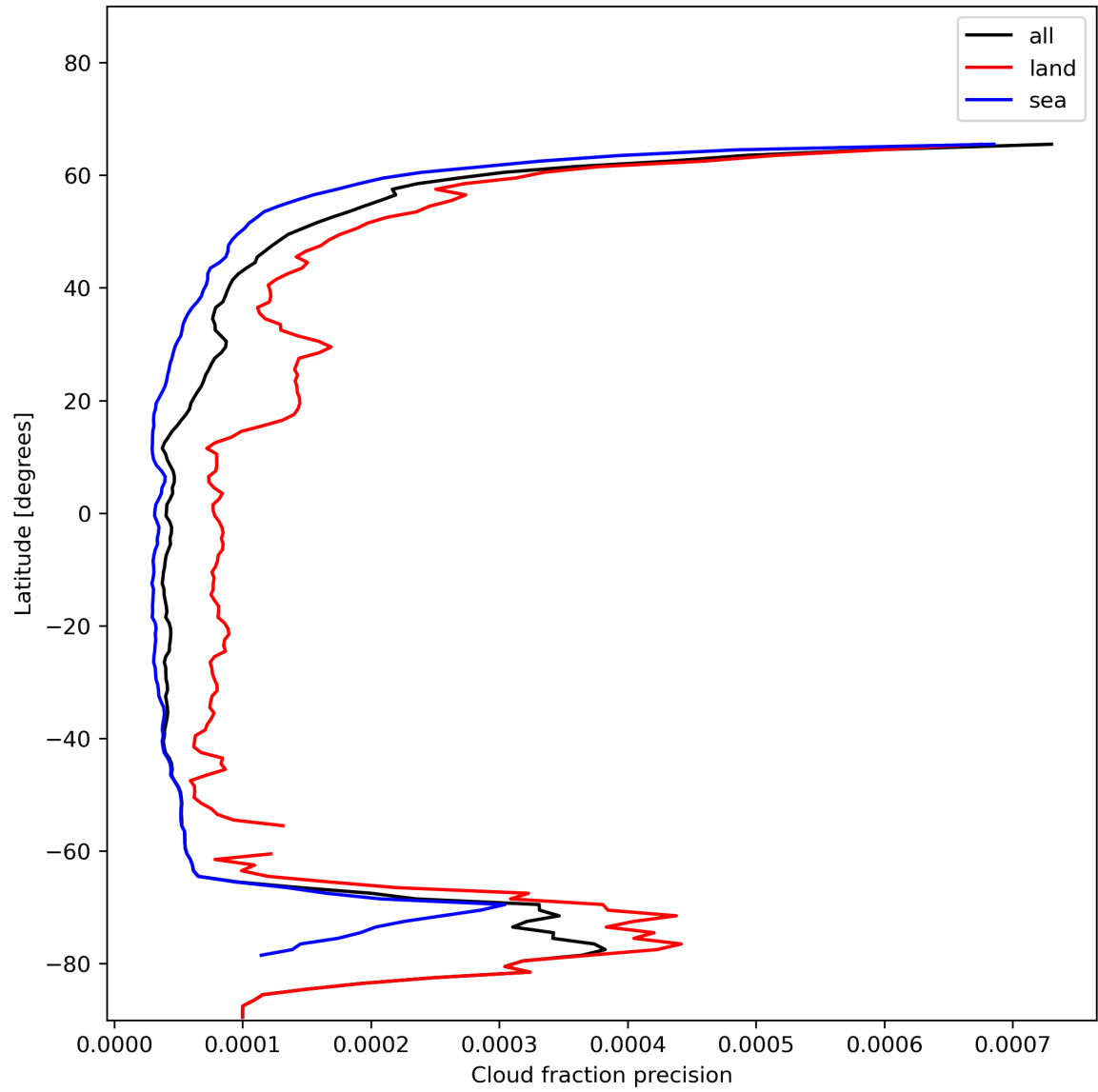
Figure 16: Zonal average of “Cloud fraction precision” for 2024-01-05 to 2024-01-07.
