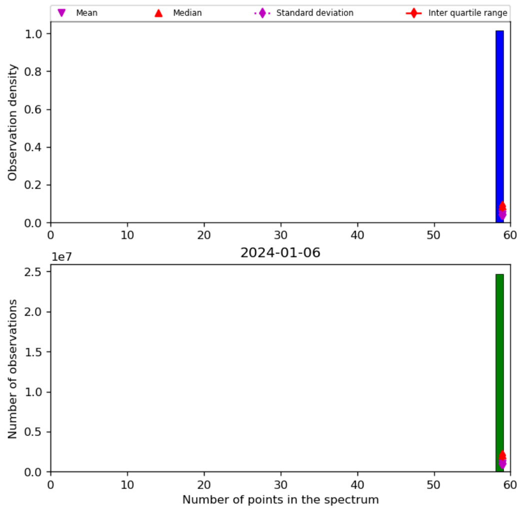
Figure 44: Histogram of “Number of points in the spectrum” for 2024-01-05 to 2024-01-07
