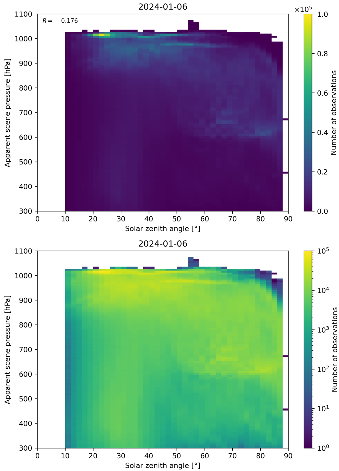
Figure 108: Scatter density plot of “Solar zenith angle” against “Apparent scene pressure” for 2024-01-05 to 2024-01-07.
