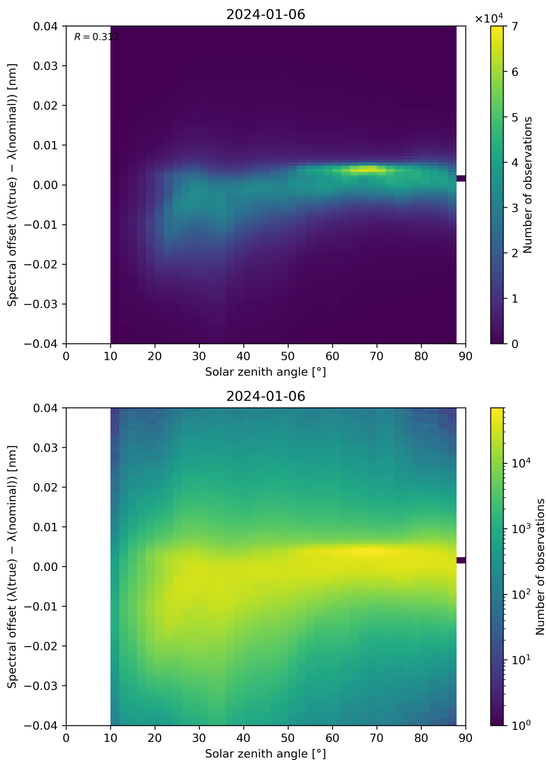
Figure 117: Scatter density plot of “Solar zenith angle” against “Spectral offset ( \lambda(\text{true}) - \lambda(\text{nominal}) )” for 2024-01-05 to 2024-01-07.
