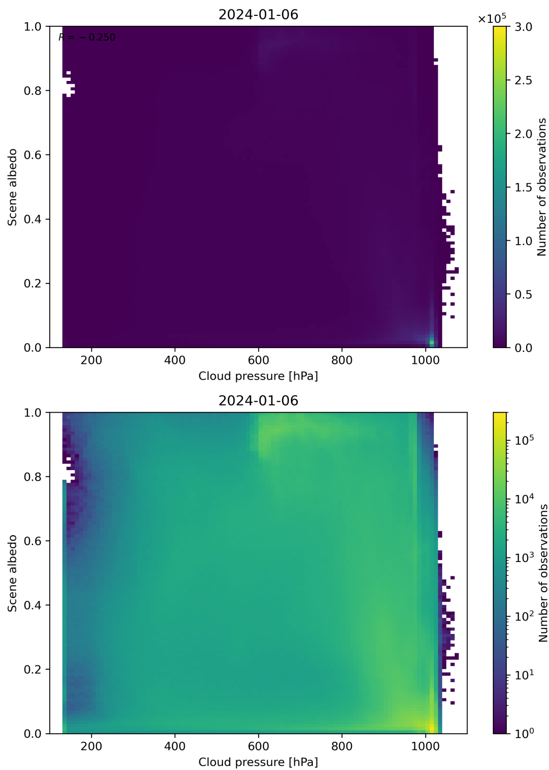
Figure 83: Scatter density plot of “Cloud pressure” against “Scene albedo” for 2024-01-05 to 2024-01-07.
