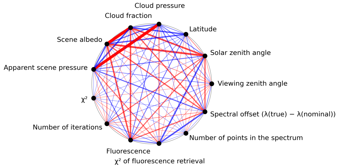
Figure 1: Map of correlation graph for 2024-01-05 to 2024-01-07.
