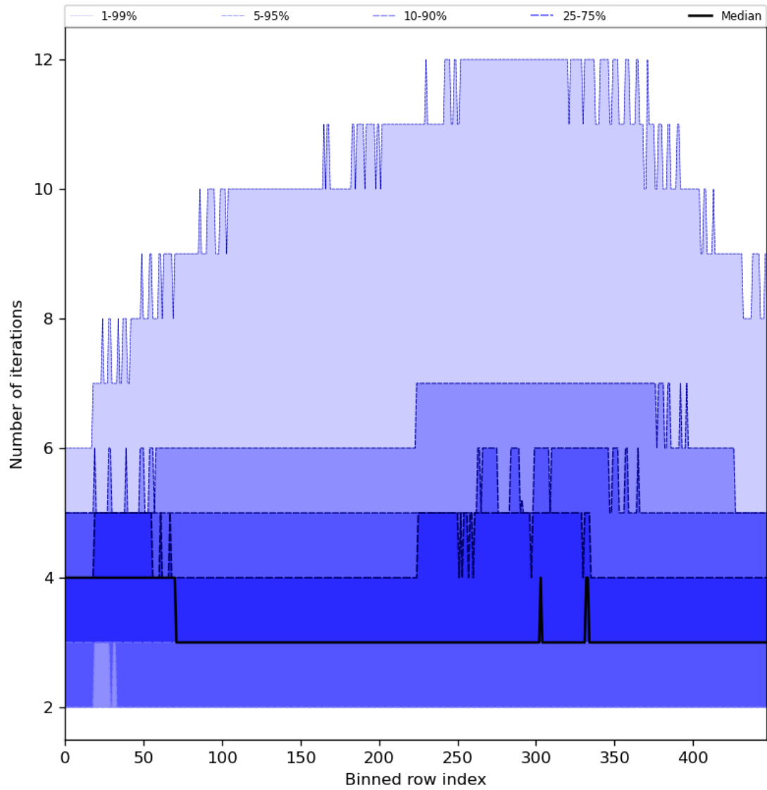
Figure 56: Along track statistics of “Number of iterations” for 2024-01-05 to 2024-01-07
