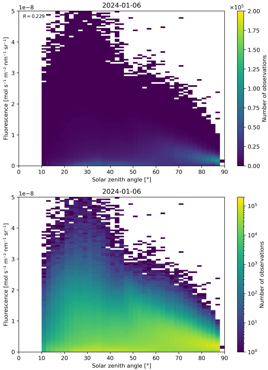
Figure 112: Scatter density plot of “Solar zenith angle” against “Fluorescence” for 2024-01-05 to 2024-01-07.
