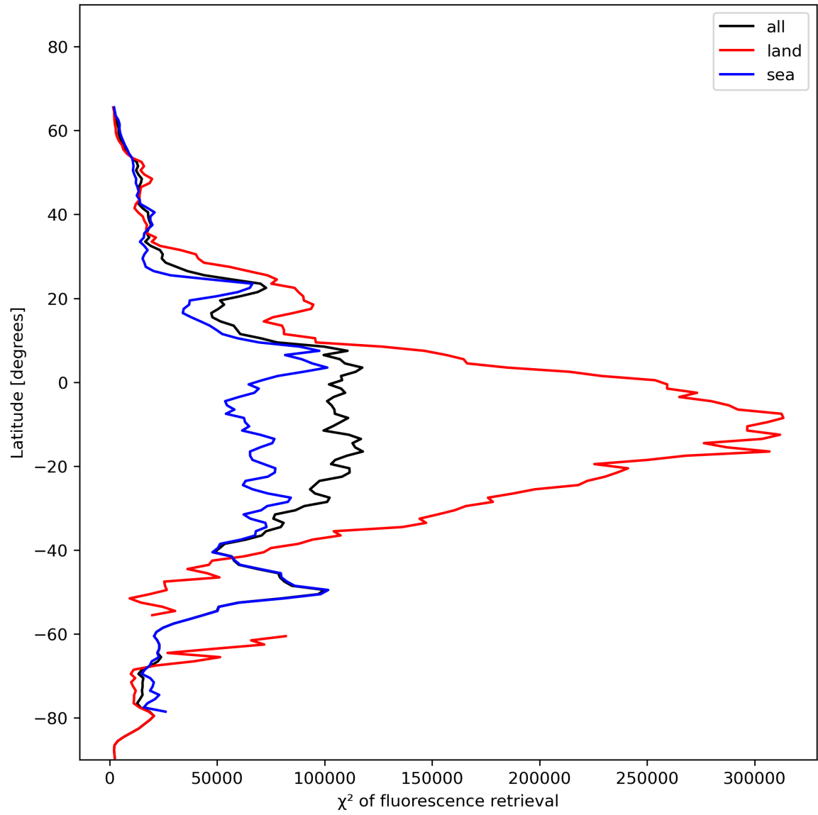
Figure 25: Zonal average of “ \chi^2 of fluorescence retrieval” for 2024-01-05 to 2024-01-07.
