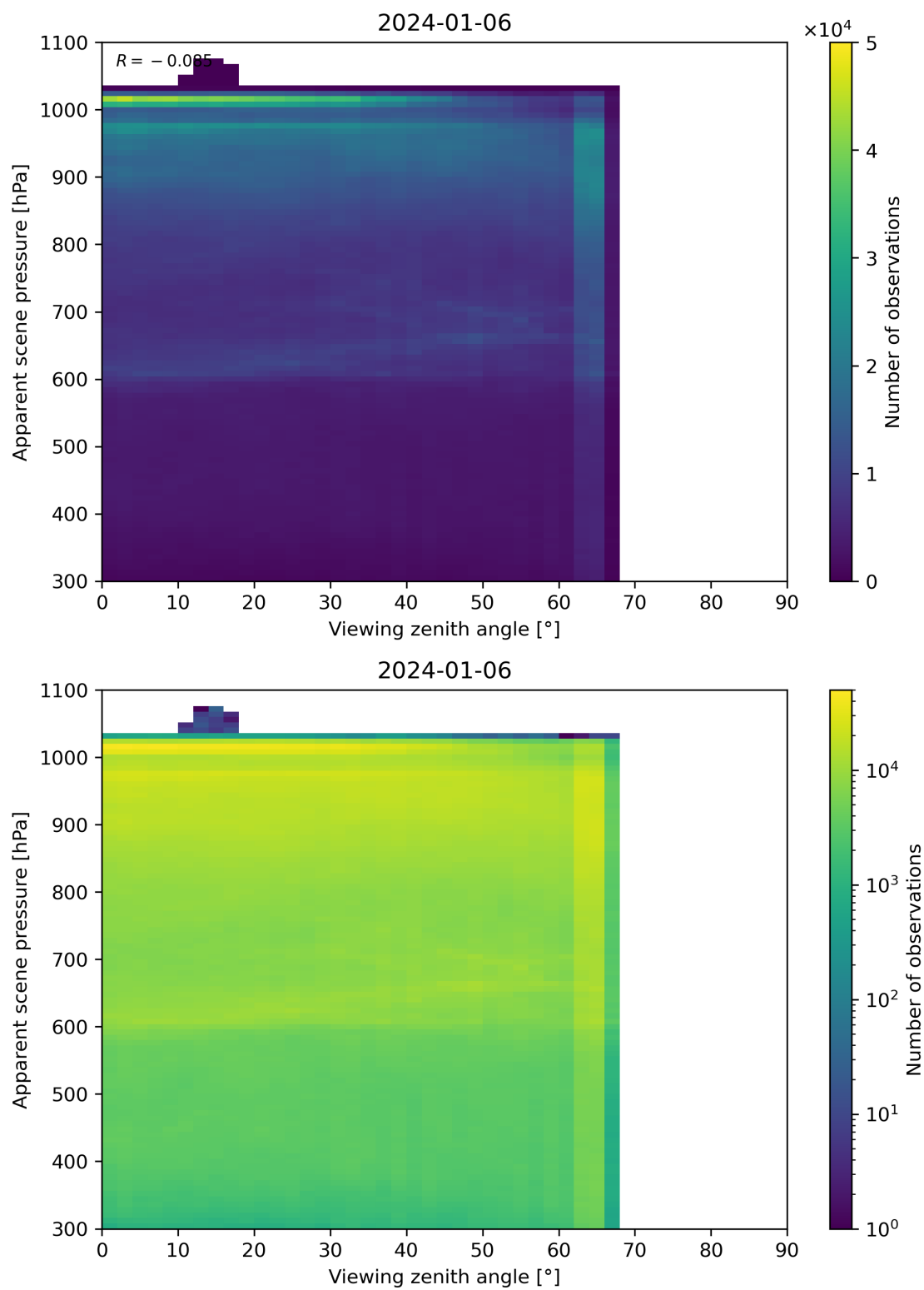
Figure 118: Scatter density plot of “Viewing zenith angle” against “Apparent scene pressure” for 2024-01-05 to 2024-01-07.
