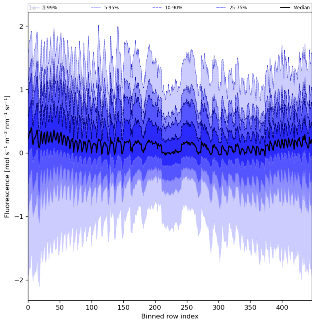
Figure 57: Along track statistics of “Fluorescence” for 2024-01-05 to 2024-01-07
