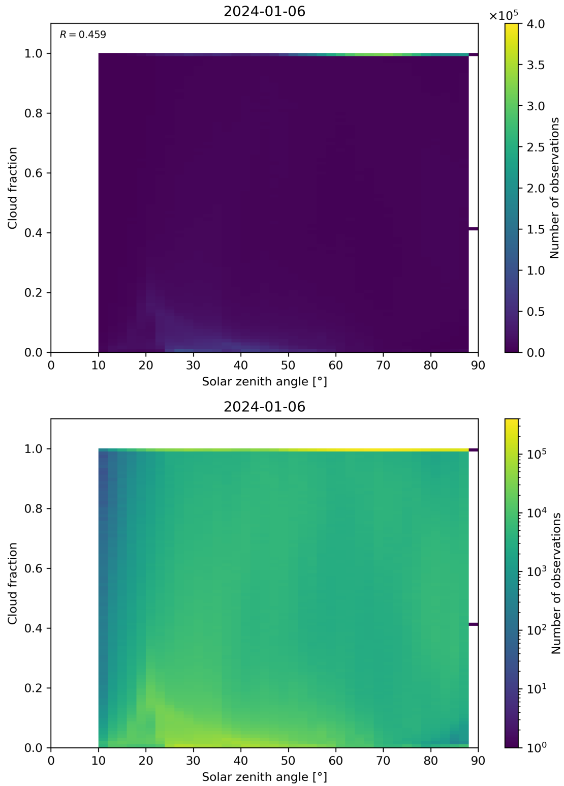
Figure 110: Scatter density plot of “Solar zenith angle” against “Cloud fraction” for 2024-01-05 to 2024-01-07.
