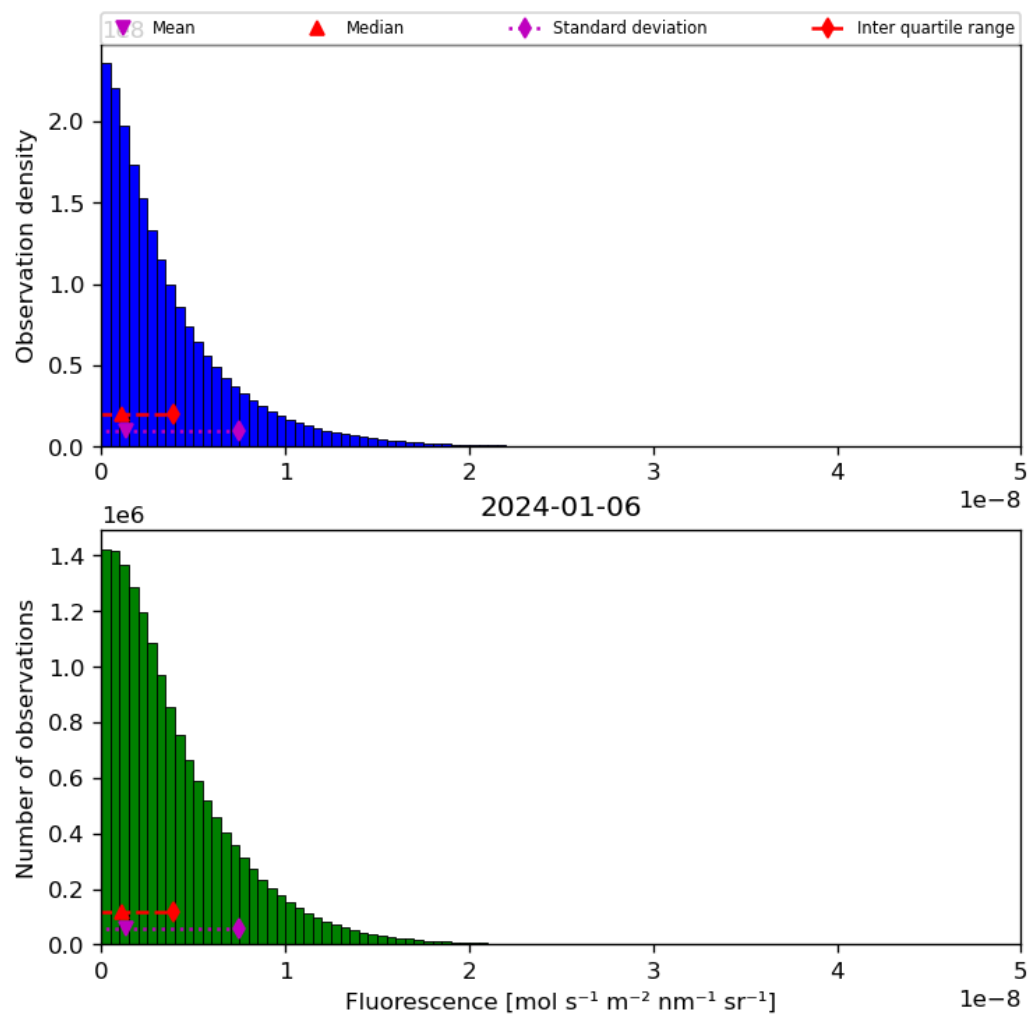
Figure 40: Histogram of “Fluorescence” for 2024-01-05 to 2024-01-07
