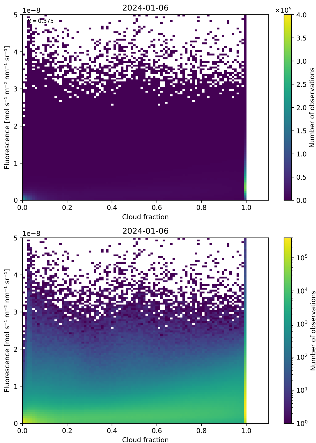
Figure 72: Scatter density plot of “Cloud fraction” against “Fluorescence” for 2024-01-05 to 2024-01-07.
