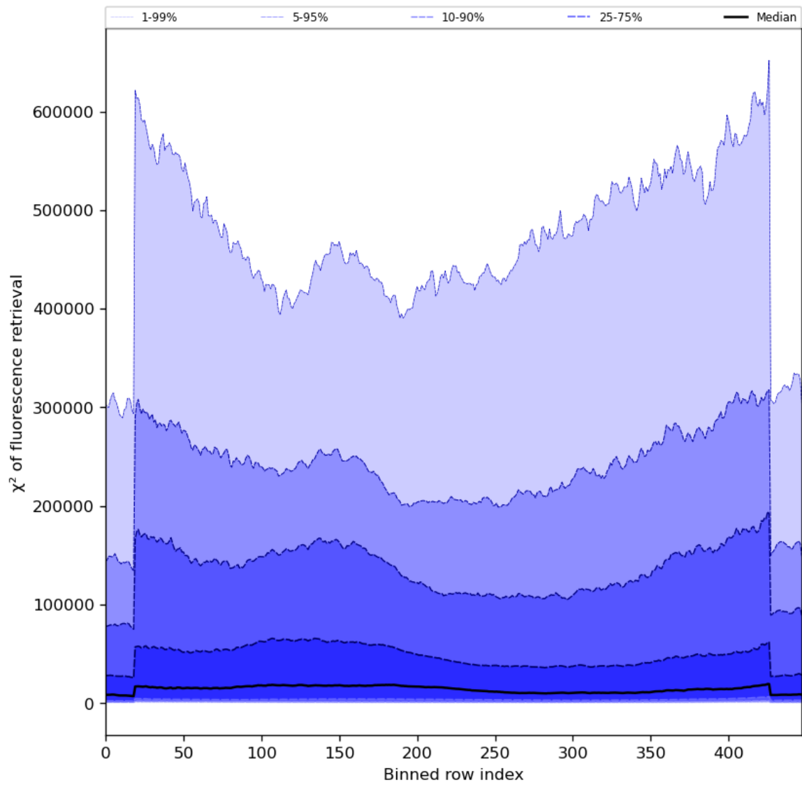
Figure 59: Along track statistics of “ \chi^2 of fluorescence retrieval” for 2024-01-05 to 2024-01-07
