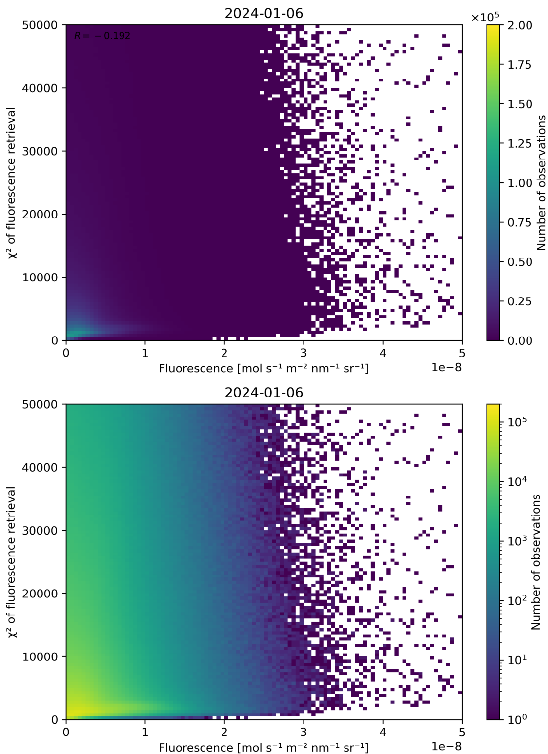
Figure 85: Scatter density plot of “Fluorescence” against “ \chi^2 of fluorescence retrieval” for 2024-01-05 to 2024-01-07.
