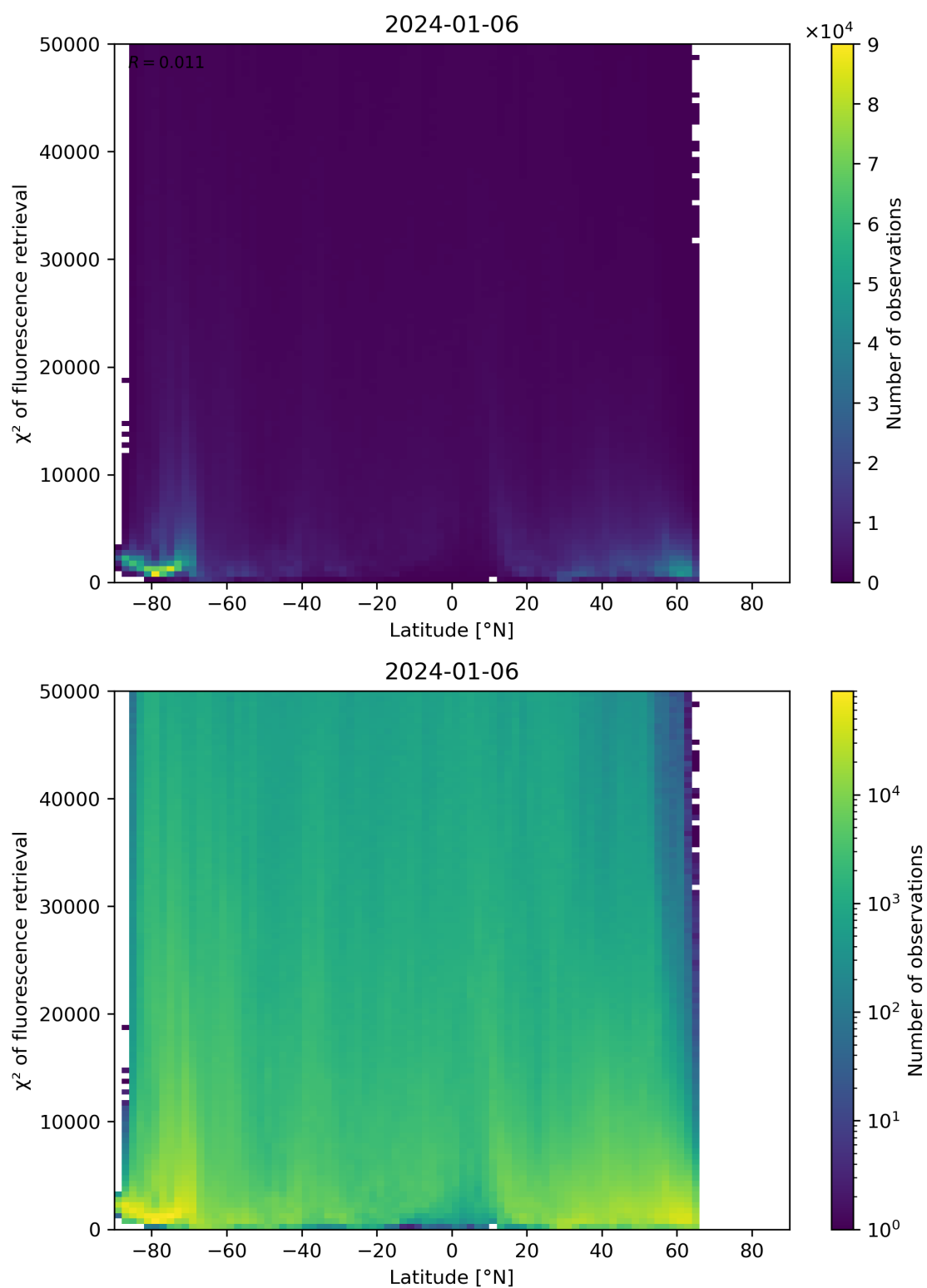
Figure 89: Scatter density plot of “Latitude” against “ \chi^2 of fluorescence retrieval” for 2024-01-05 to 2024-01-07.
