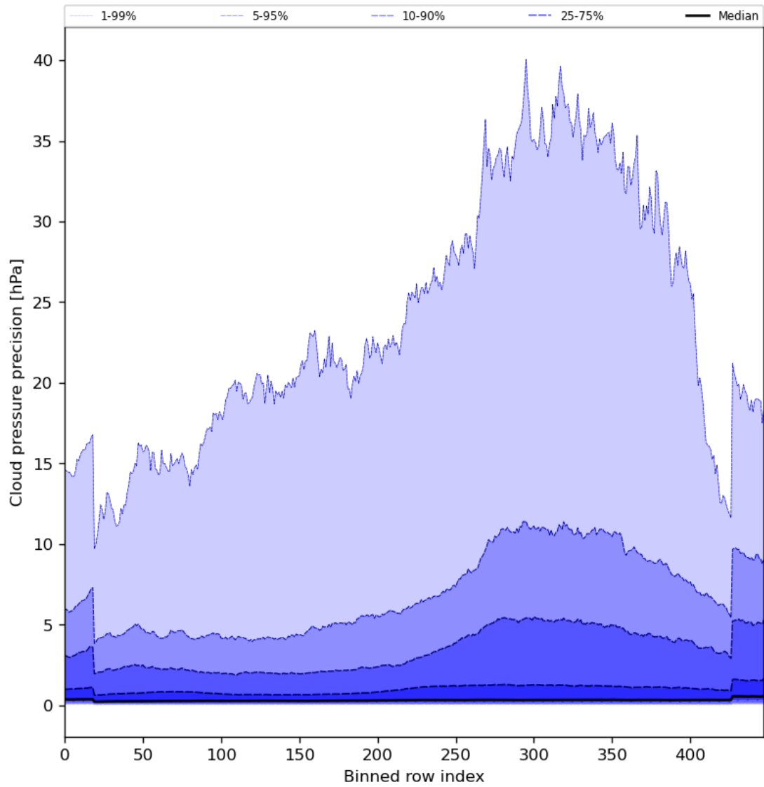
Figure 48: Along track statistics of “Cloud pressure precision” for 2024-01-05 to 2024-01-07
