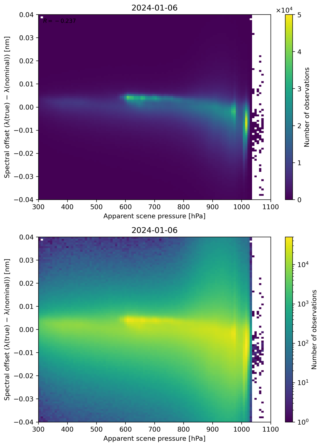
Figure 67: Scatter density plot of “Apparent scene pressure” against “Spectral offset ( \lambda(\text{true}) - \lambda(\text{nominal}) )” for 2024-01-05 to 2024-01-07.
