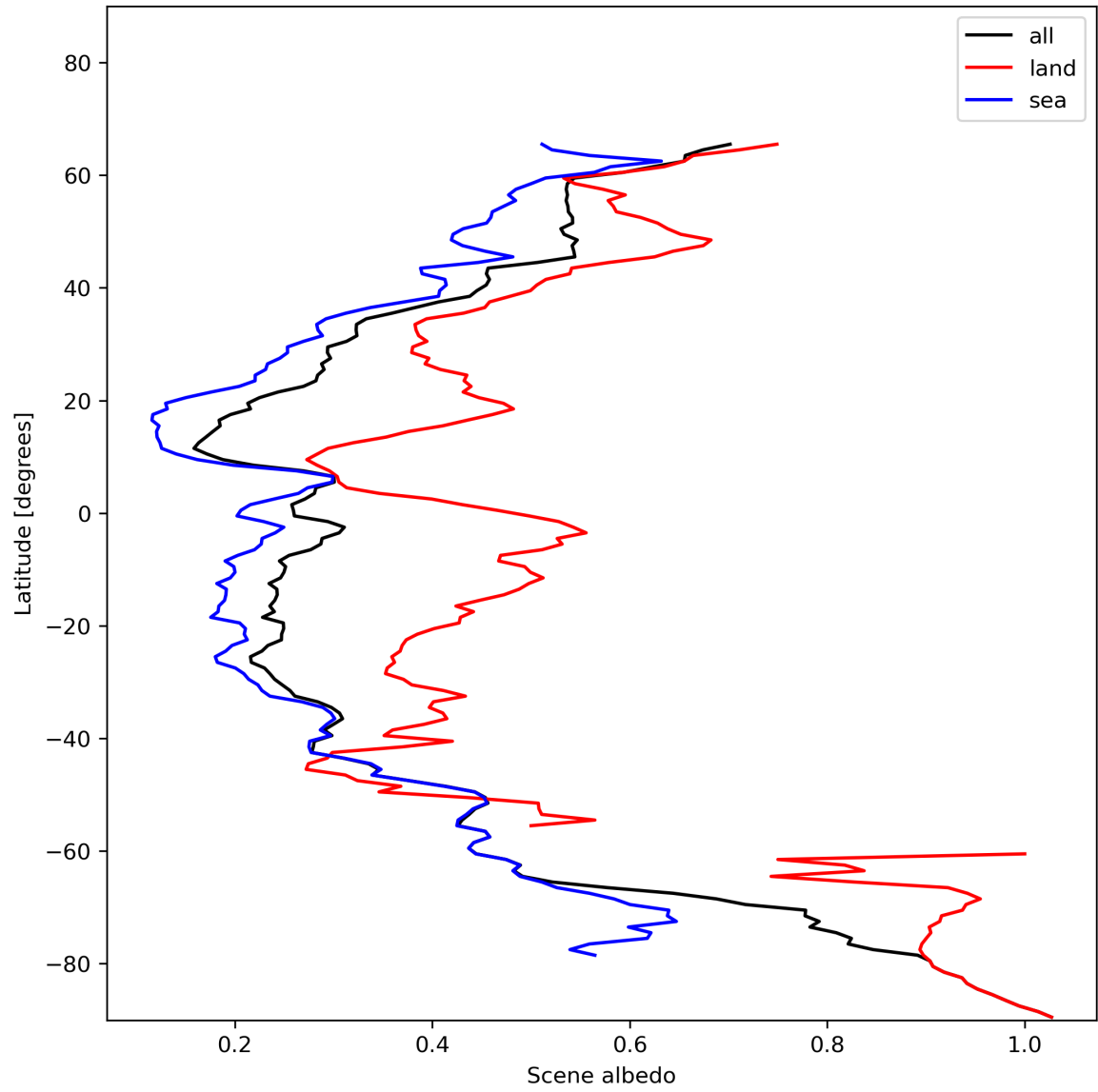
Figure 17: Zonal average of “Scene albedo” for 2024-01-05 to 2024-01-07.
