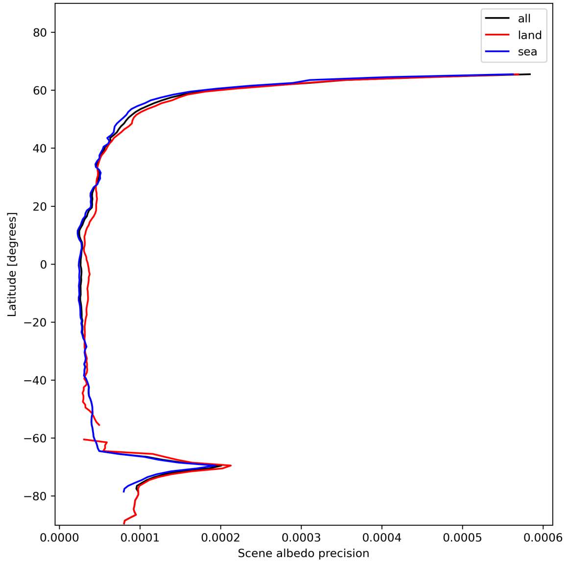
Figure 18: Zonal average of “Scene albedo precision” for 2024-01-05 to 2024-01-07.
