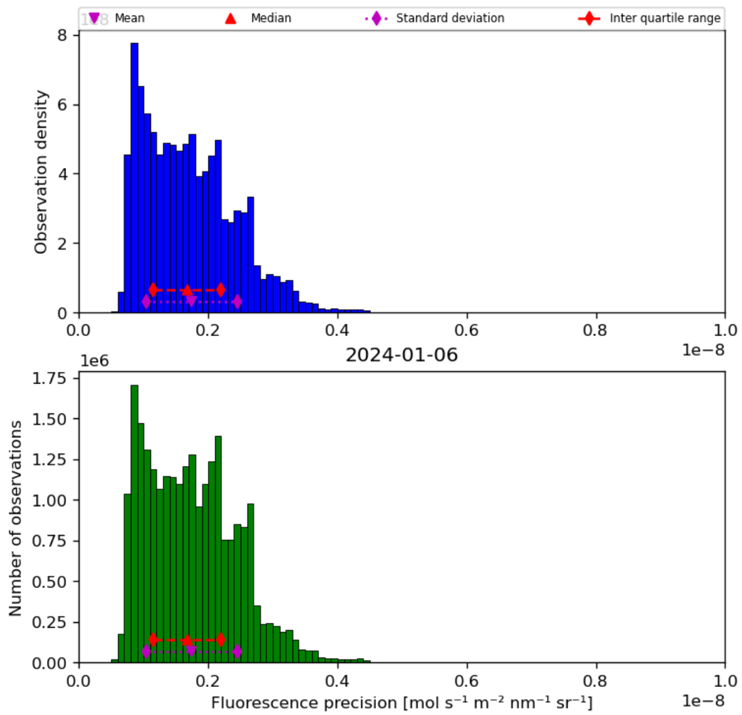
Figure 41: Histogram of “Fluorescence precision” for 2024-01-05 to 2024-01-07
