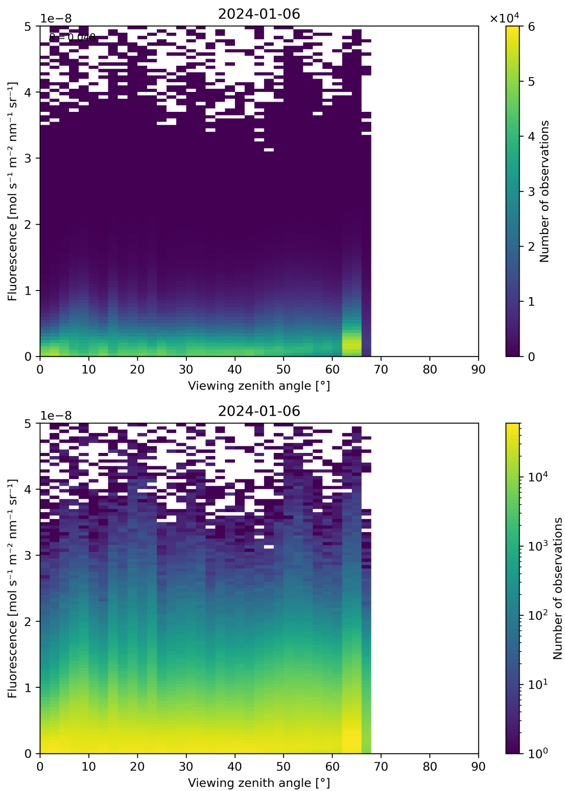
Figure 122: Scatter density plot of “Viewing zenith angle” against “Fluorescence” for 2024-01-05 to 2024-01-07.
