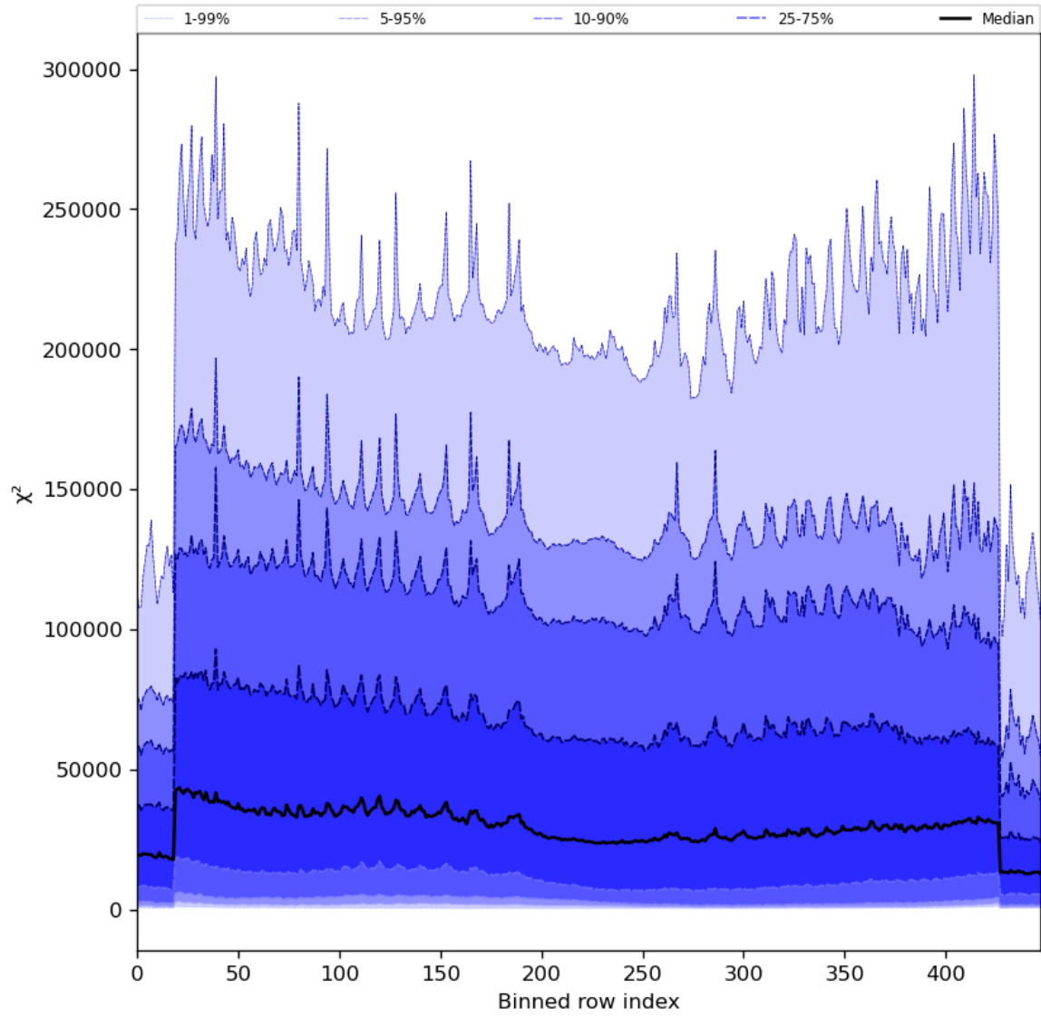
Figure 55: Along track statistics of “ \chi^2 ” for 2024-01-05 to 2024-01-07
