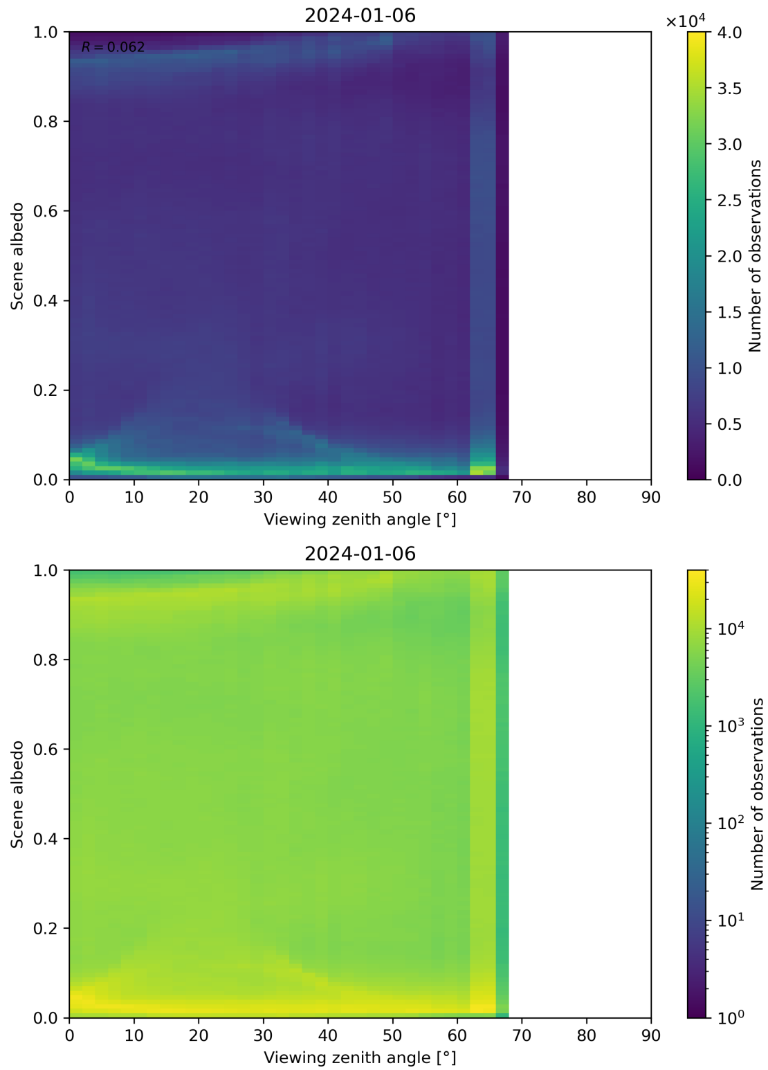
Figure 126: Scatter density plot of “Viewing zenith angle” against “Scene albedo” for 2024-01-05 to 2024-01-07.
