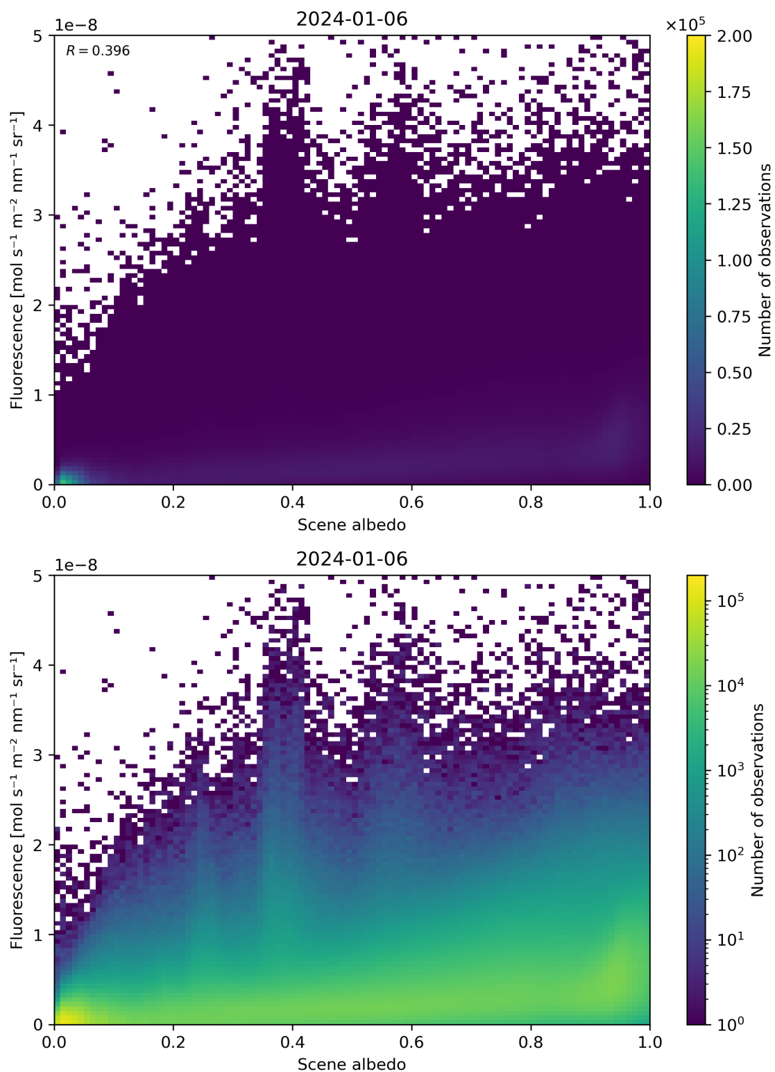
Figure 104: Scatter density plot of “Scene albedo” against “Fluorescence” for 2024-01-05 to 2024-01-07.
