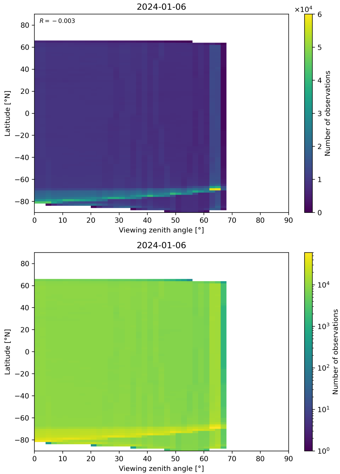
Figure 123: Scatter density plot of “Viewing zenith angle” against “Latitude” for 2024-01-05 to 2024-01-07.
