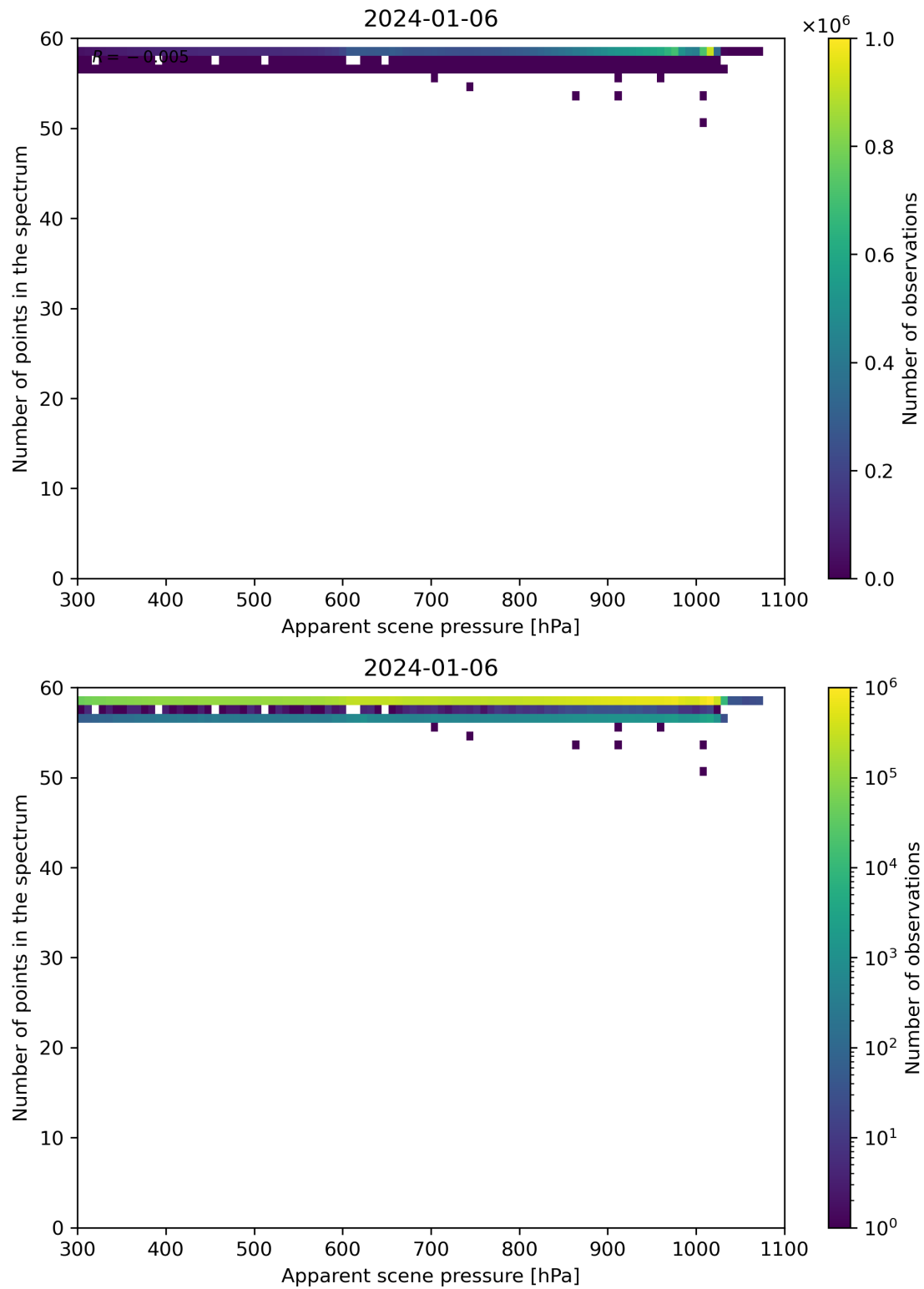
Figure 66: Scatter density plot of “Apparent scene pressure” against “Number of points in the spectrum” for 2024-01-05 to 2024-01-07.
