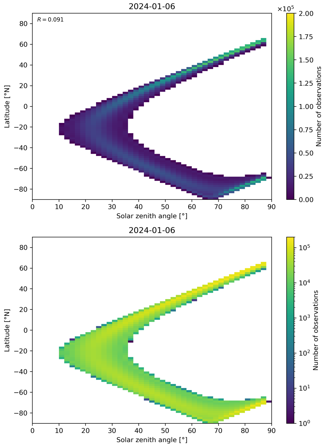
Figure 113: Scatter density plot of “Solar zenith angle” against “Latitude” for 2024-01-05 to 2024-01-07.
