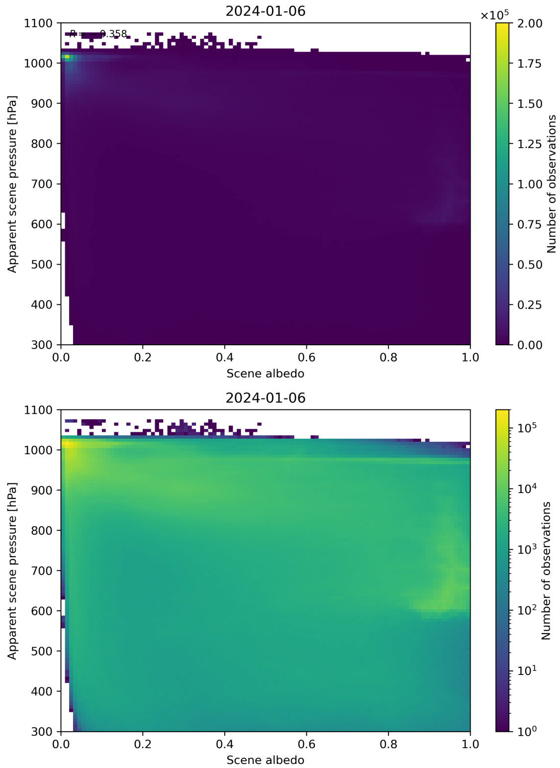
Figure 102: Scatter density plot of “Scene albedo” against “Apparent scene pressure” for 2024-01-05 to 2024-01-07.
