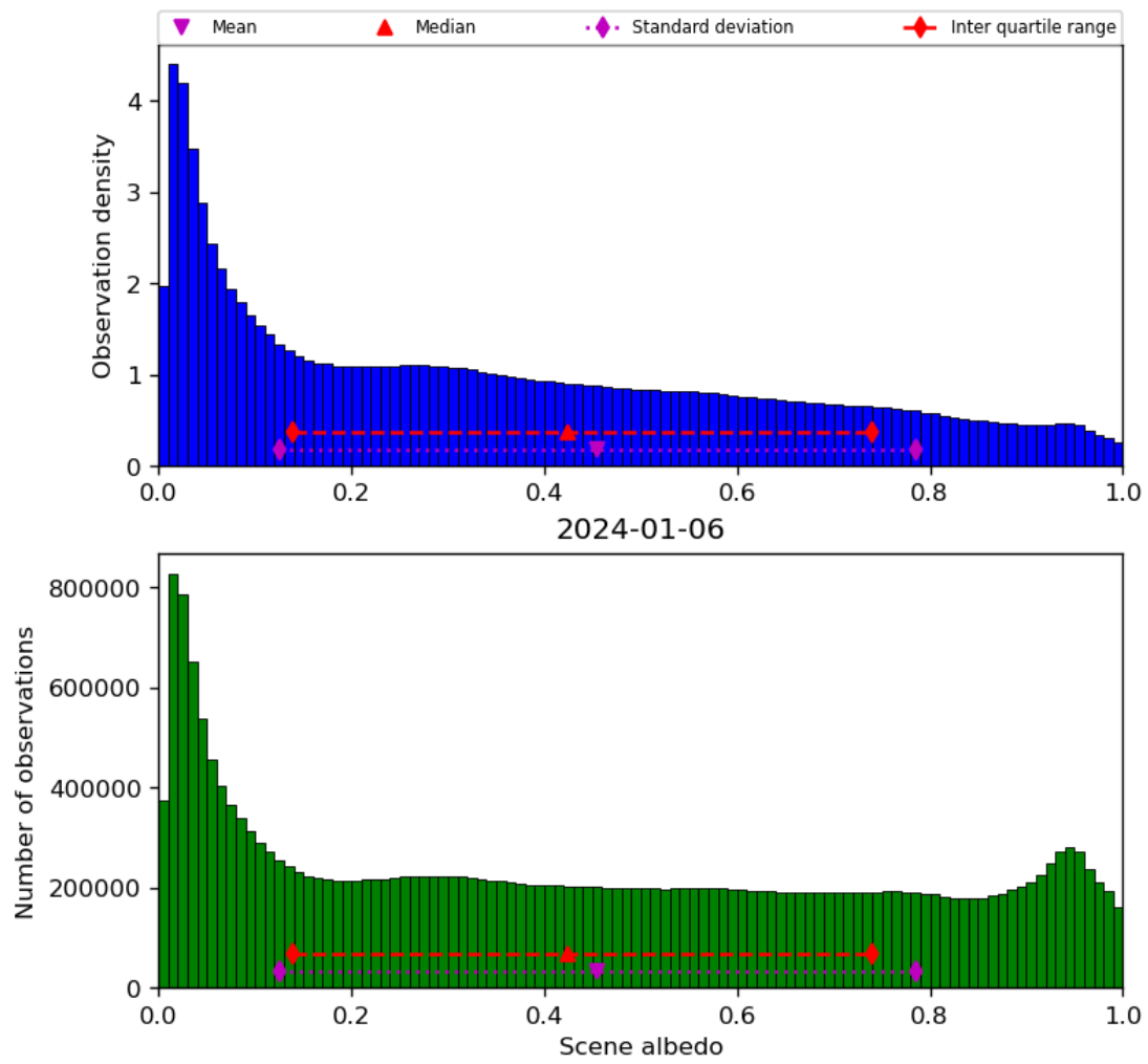
Figure 34: Histogram of “Scene albedo” for 2024-01-05 to 2024-01-07
