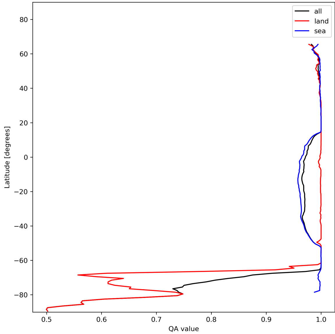
Figure 12: Zonal average of “QA value” for 2024-01-05 to 2024-01-07.
