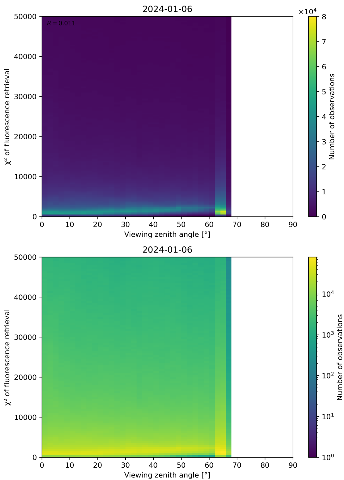
Figure 119: Scatter density plot of “Viewing zenith angle” against “ \chi^2 of fluorescence retrieval” for 2024-01-05 to 2024-01-07.
