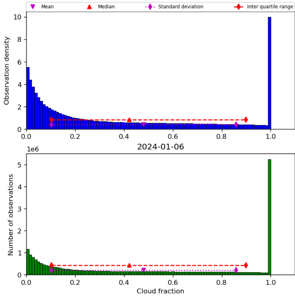
Figure 32: Histogram of “Cloud fraction” for 2024-01-05 to 2024-01-07
