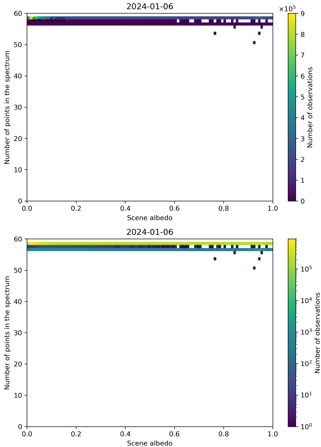
Figure 106: Scatter density plot of “Scene albedo” against “Number of points in the spectrum” for 2024-01-05 to 2024-01-07.
