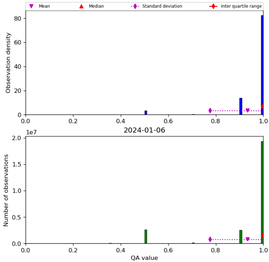
Figure 29: Histogram of “QA value” for 2024-01-05 to 2024-01-07
