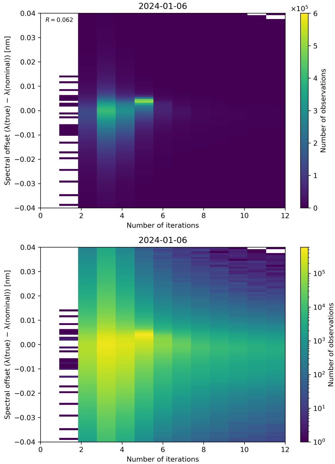
Figure 100: Scatter density plot of “Number of iterations” against “Spectral offset ( \lambda(\text{true}) - \lambda(\text{nominal}) )” for 2024-01-05 to 2024-01-07.
