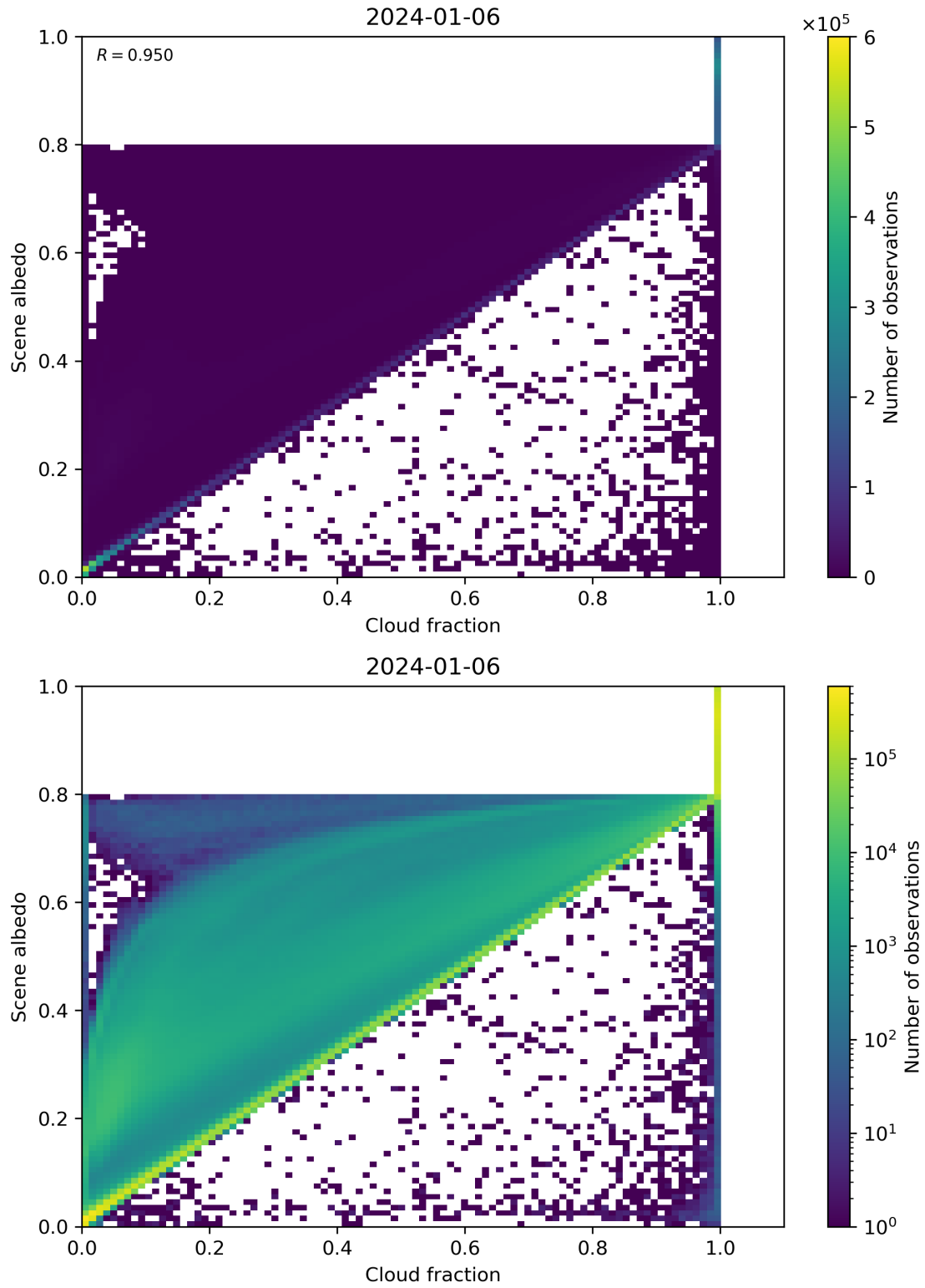
Figure 75: Scatter density plot of “Cloud fraction” against “Scene albedo” for 2024-01-05 to 2024-01-07.
