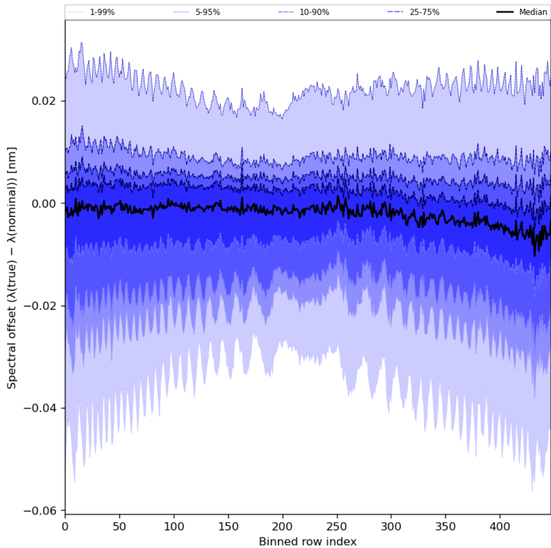
Figure 62: Along track statistics of “Spectral offset ( \lambda(\text{true}) - \lambda(\text{nominal}) )” for 2024-01-05 to 2024-01-07
