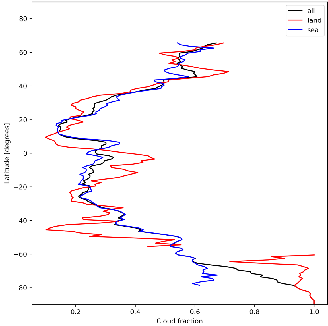
Figure 15: Zonal average of “Cloud fraction” for 2024-01-05 to 2024-01-07.
