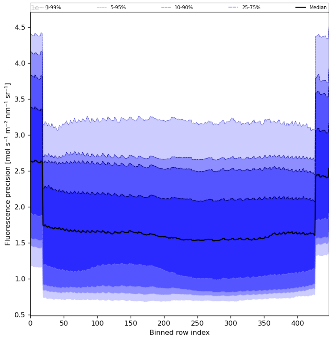
Figure 58: Along track statistics of “Fluorescence precision” for 2024-01-05 to 2024-01-07
