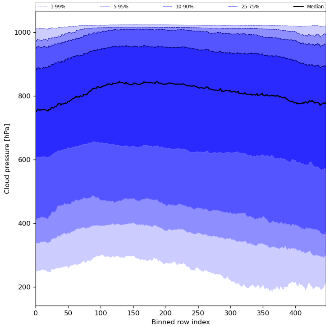
Figure 47: Along track statistics of “Cloud pressure” for 2024-01-05 to 2024-01-07
