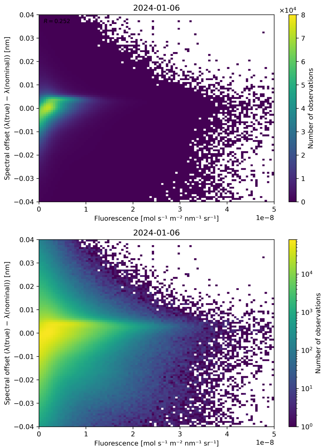
Figure 87: Scatter density plot of “Fluorescence” against “Spectral offset ( \lambda(\text{true}) - \lambda(\text{nominal}) )” for 2024-01-05 to 2024-01-07.
