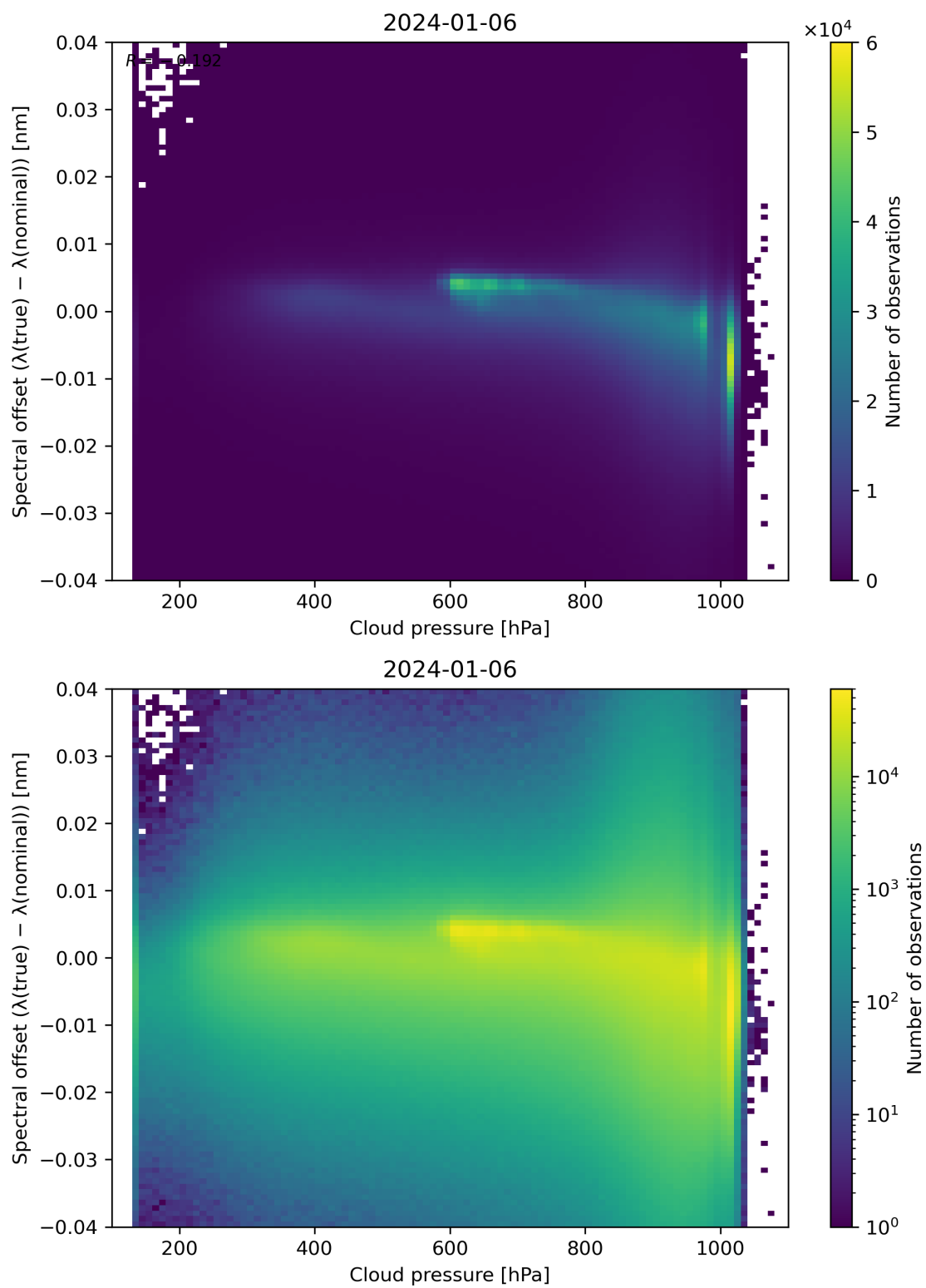
Figure 84: Scatter density plot of “Cloud pressure” against “Spectral offset ( \lambda(\text{true}) - \lambda(\text{nominal}) )” for 2024-01-05 to 2024-01-07.
