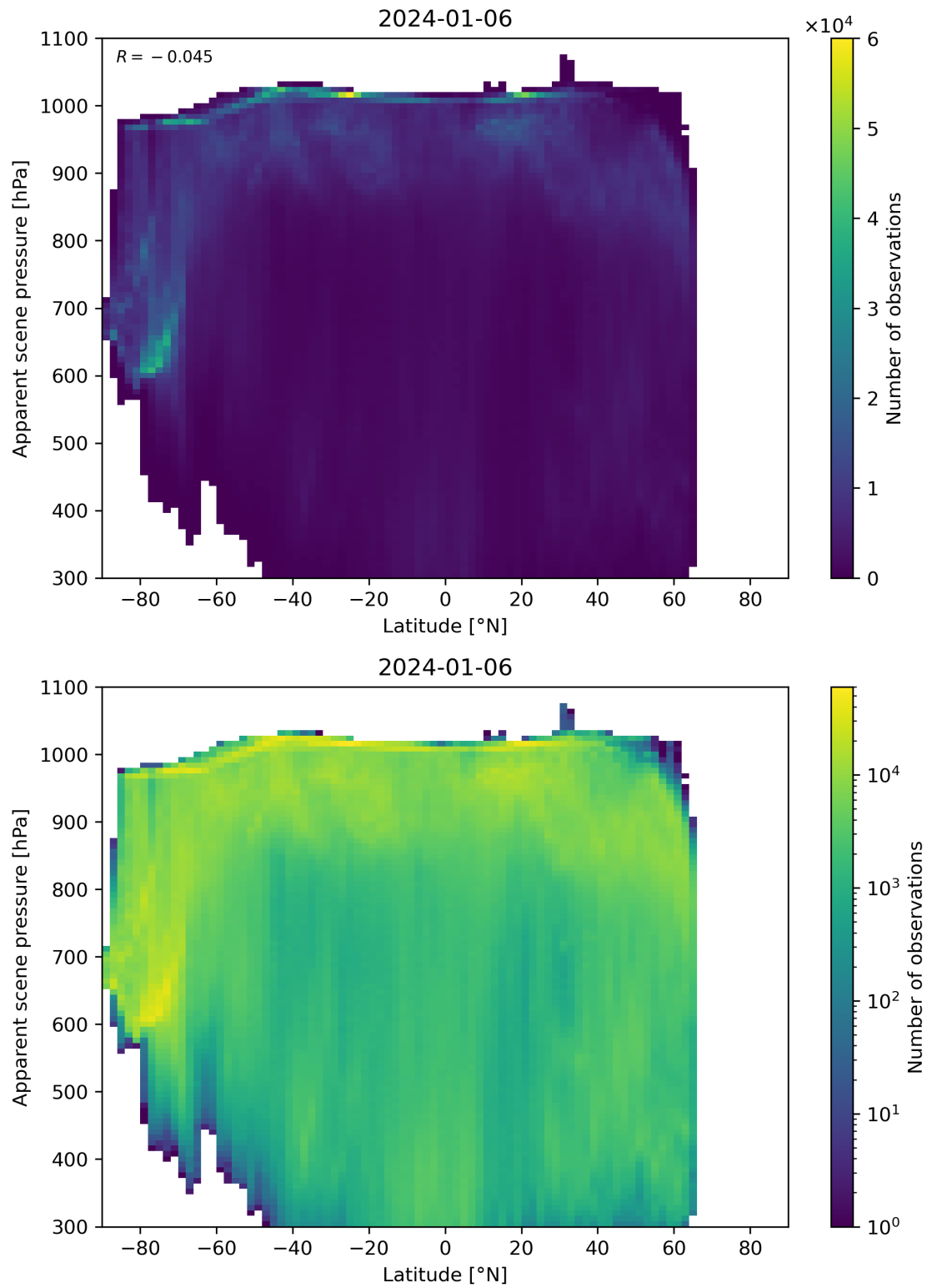
Figure 88: Scatter density plot of “Latitude” against “Apparent scene pressure” for 2024-01-05 to 2024-01-07.
