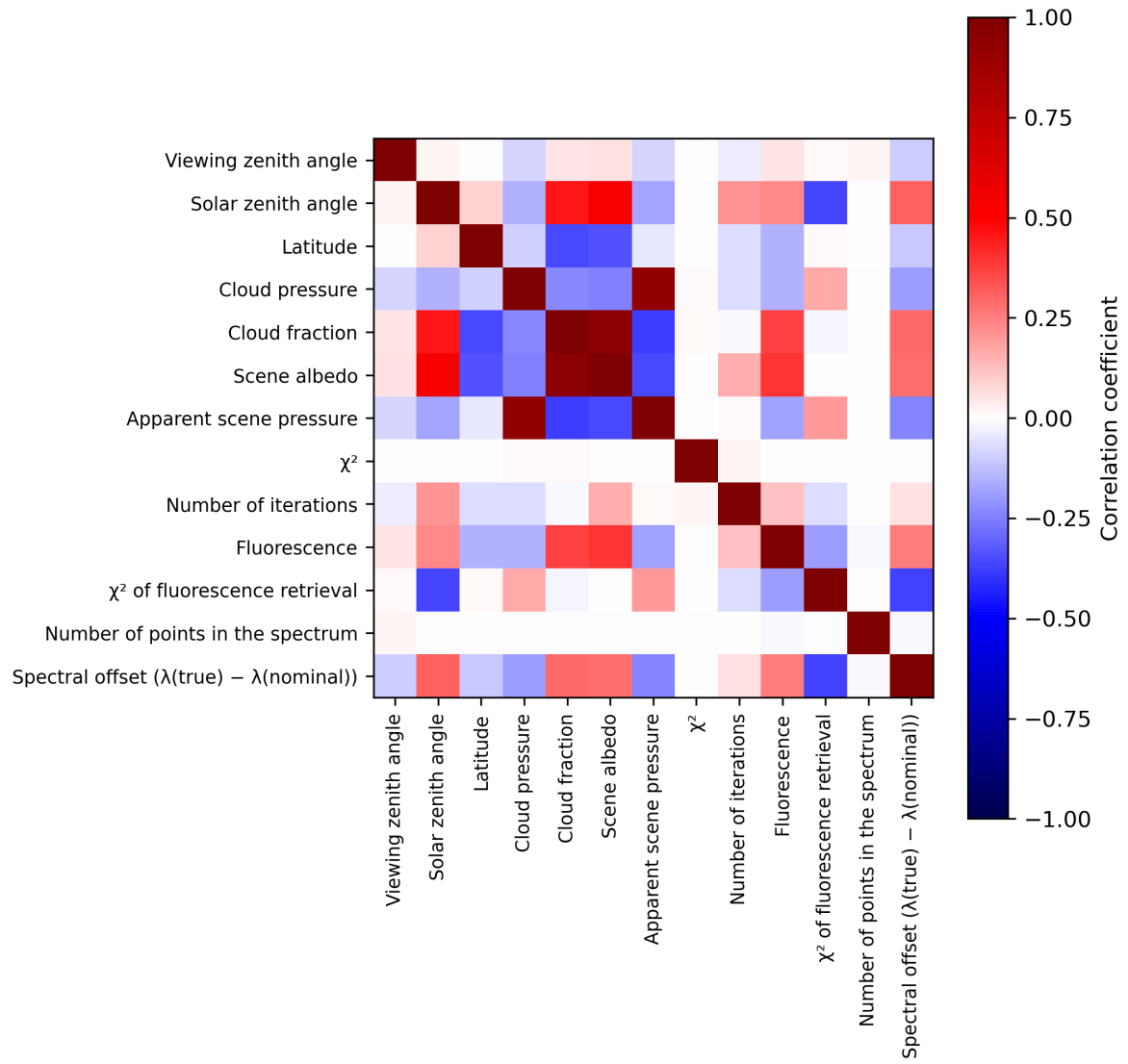
Figure 2: Map of correlation matrix for 2024-01-05 to 2024-01-07.
