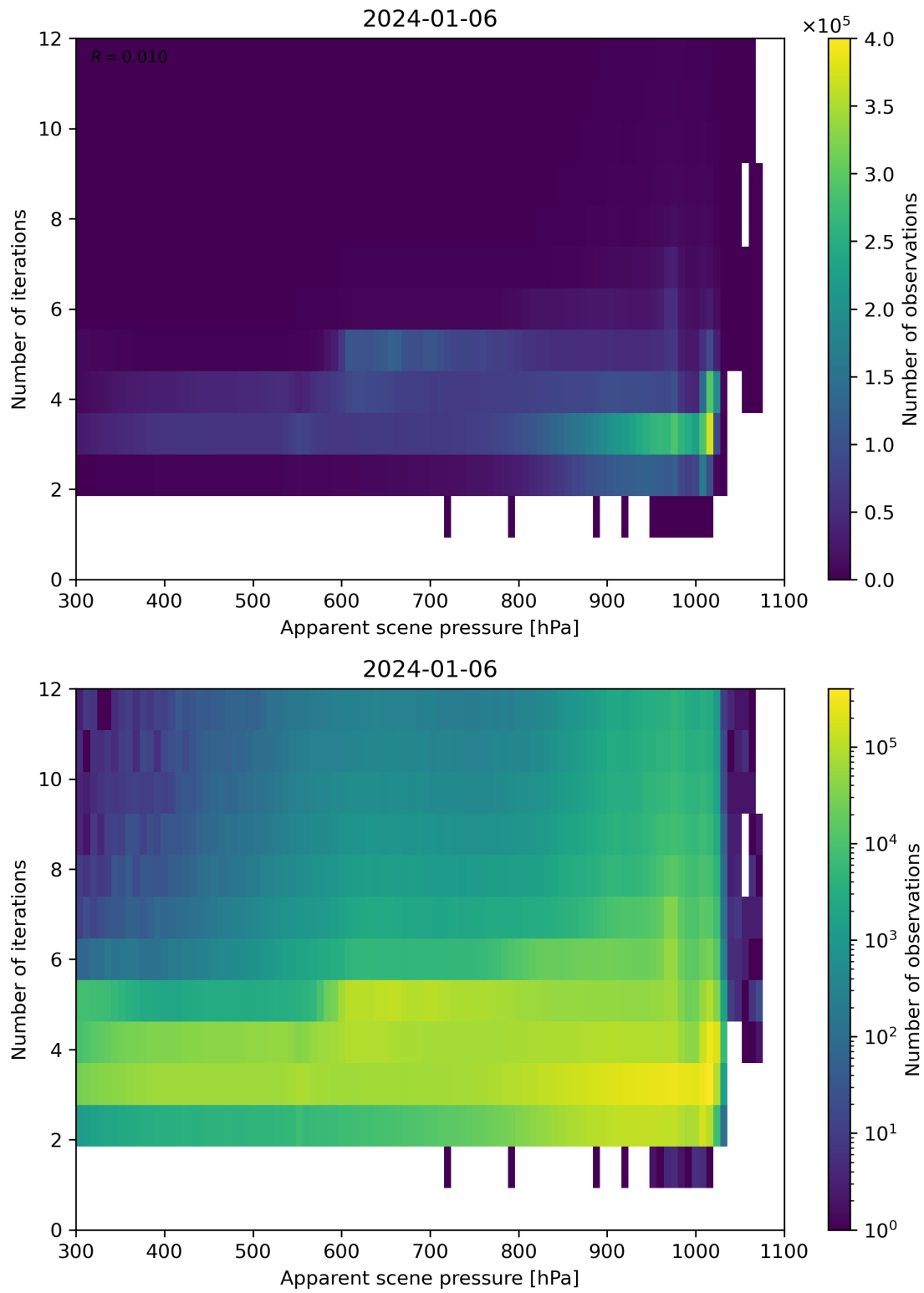
Figure 65: Scatter density plot of “Apparent scene pressure” against “Number of iterations” for 2024-01-05 to 2024-01-07.
