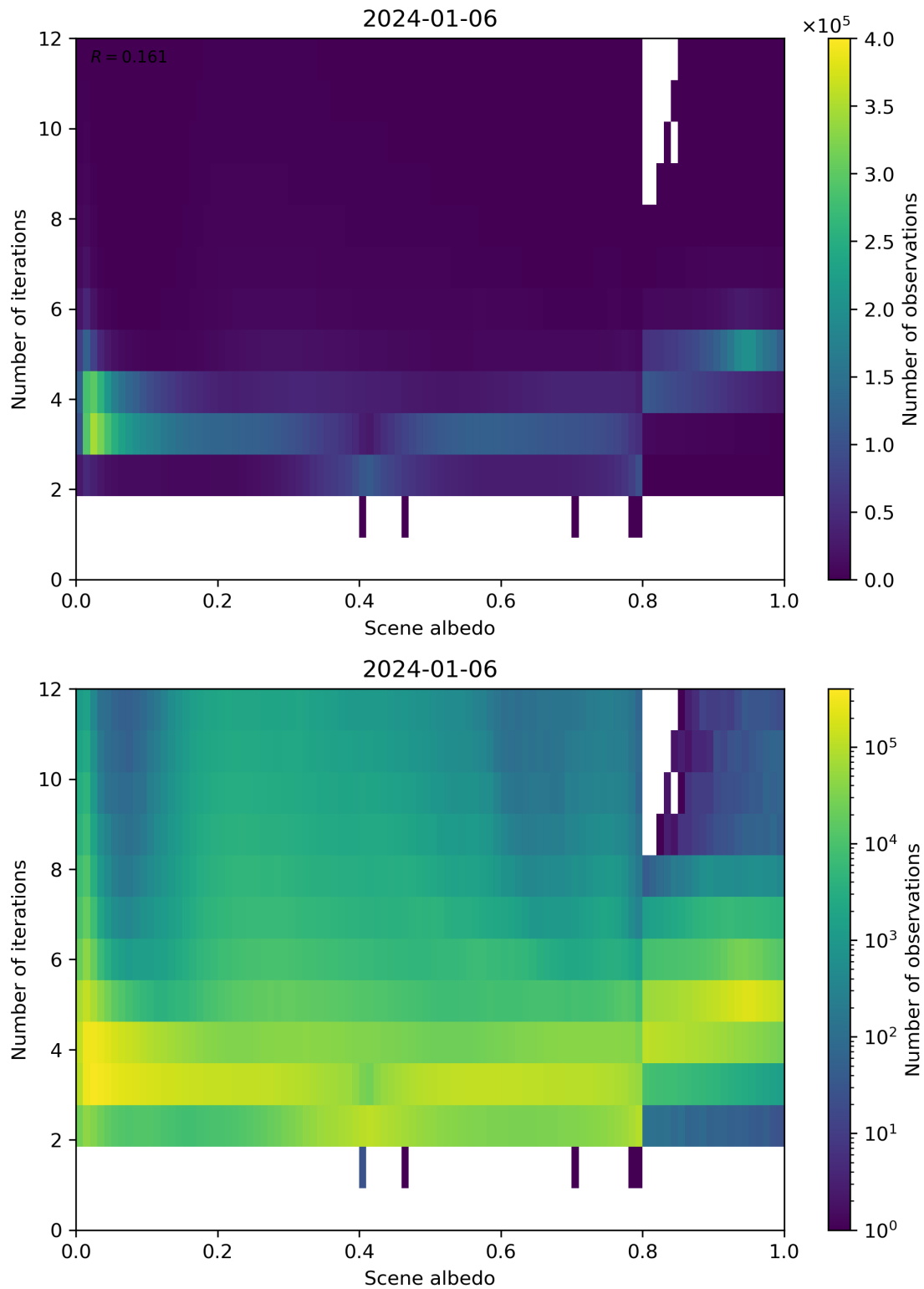
Figure 105: Scatter density plot of “Scene albedo” against “Number of iterations” for 2024-01-05 to 2024-01-07.
