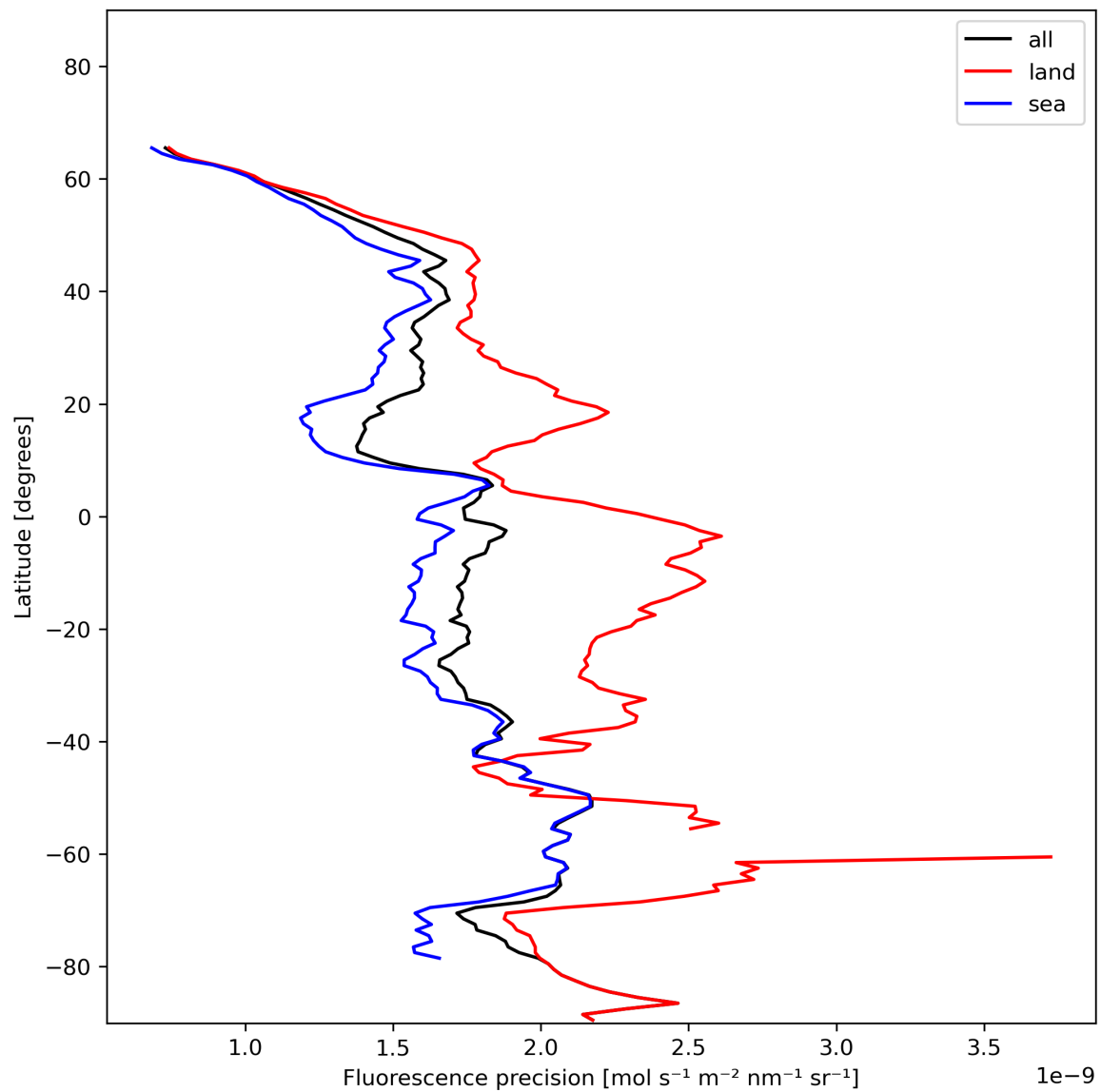
Figure 24: Zonal average of “Fluorescence precision” for 2024-01-05 to 2024-01-07.
