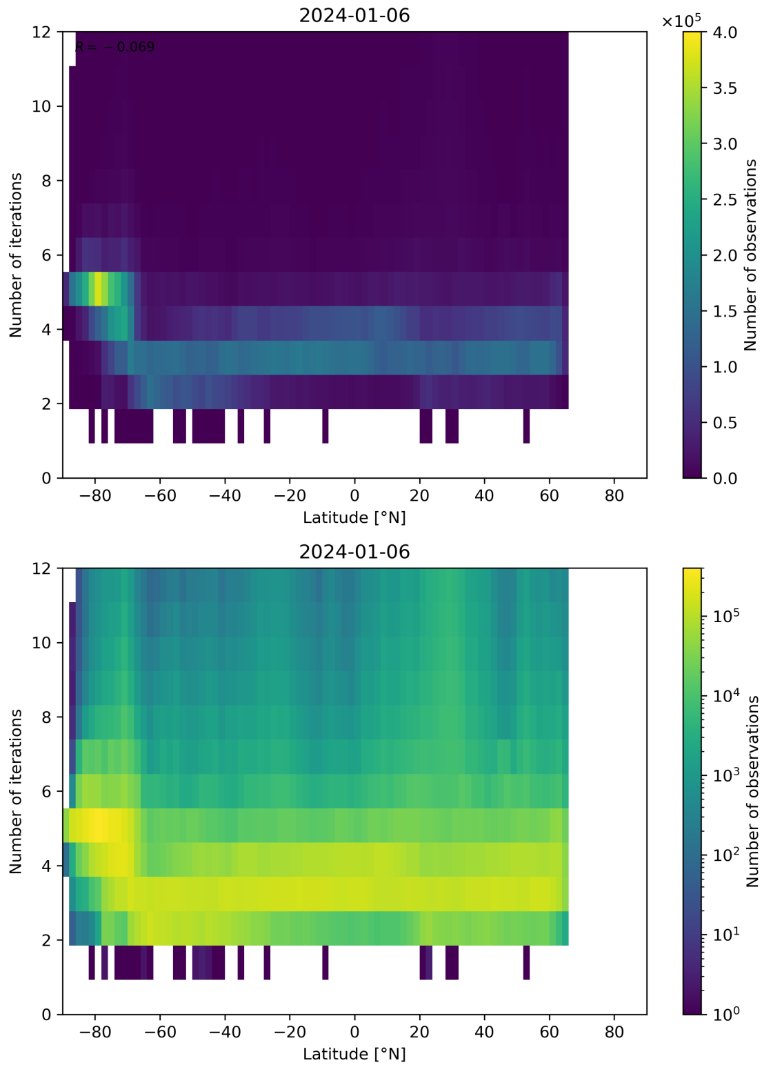
Figure 93: Scatter density plot of “Latitude” against “Number of iterations” for 2024-01-05 to 2024-01-07.
