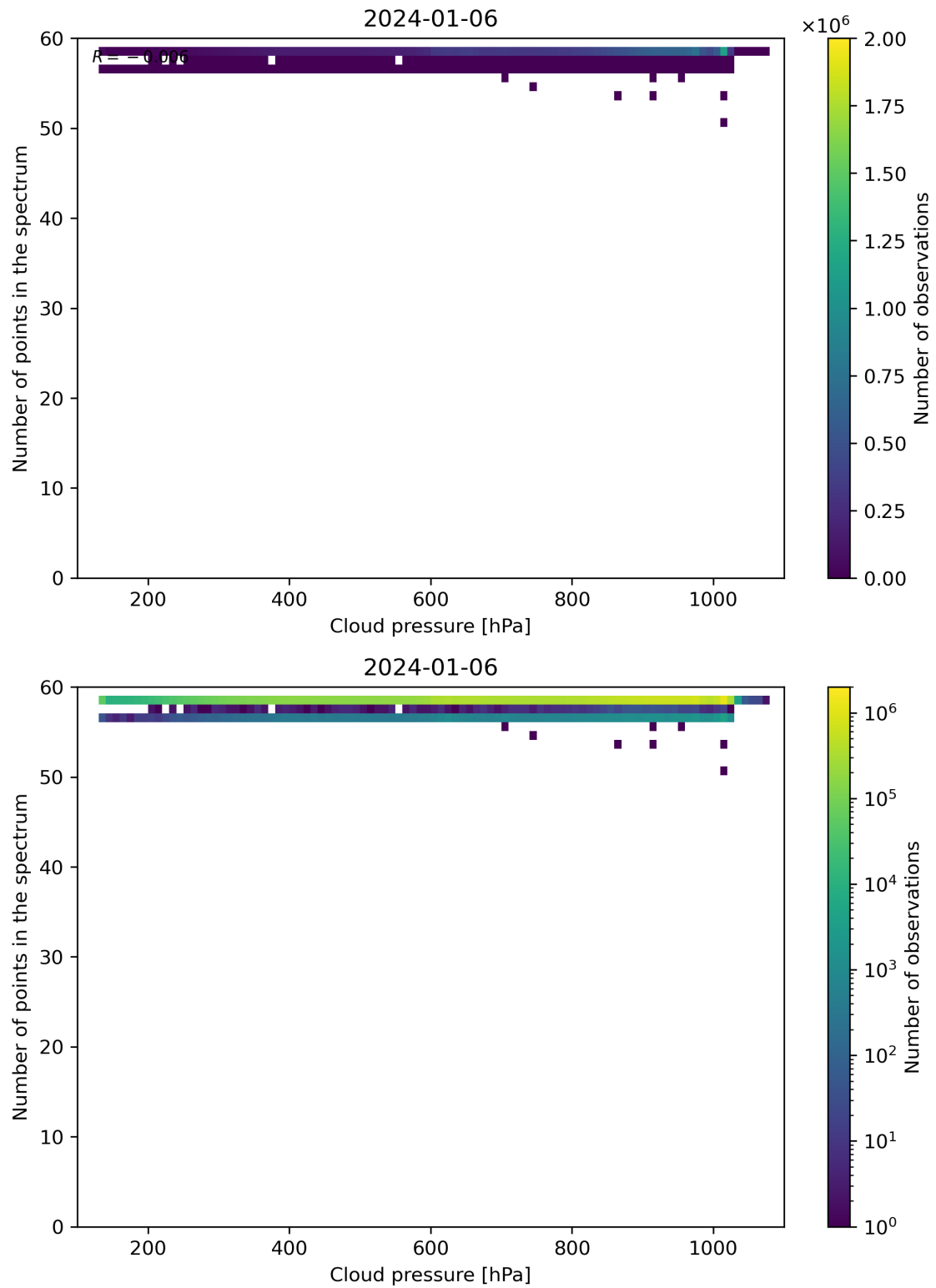
Figure 82: Scatter density plot of “Cloud pressure” against “Number of points in the spectrum” for 2024-01-05 to 2024-01-07.
