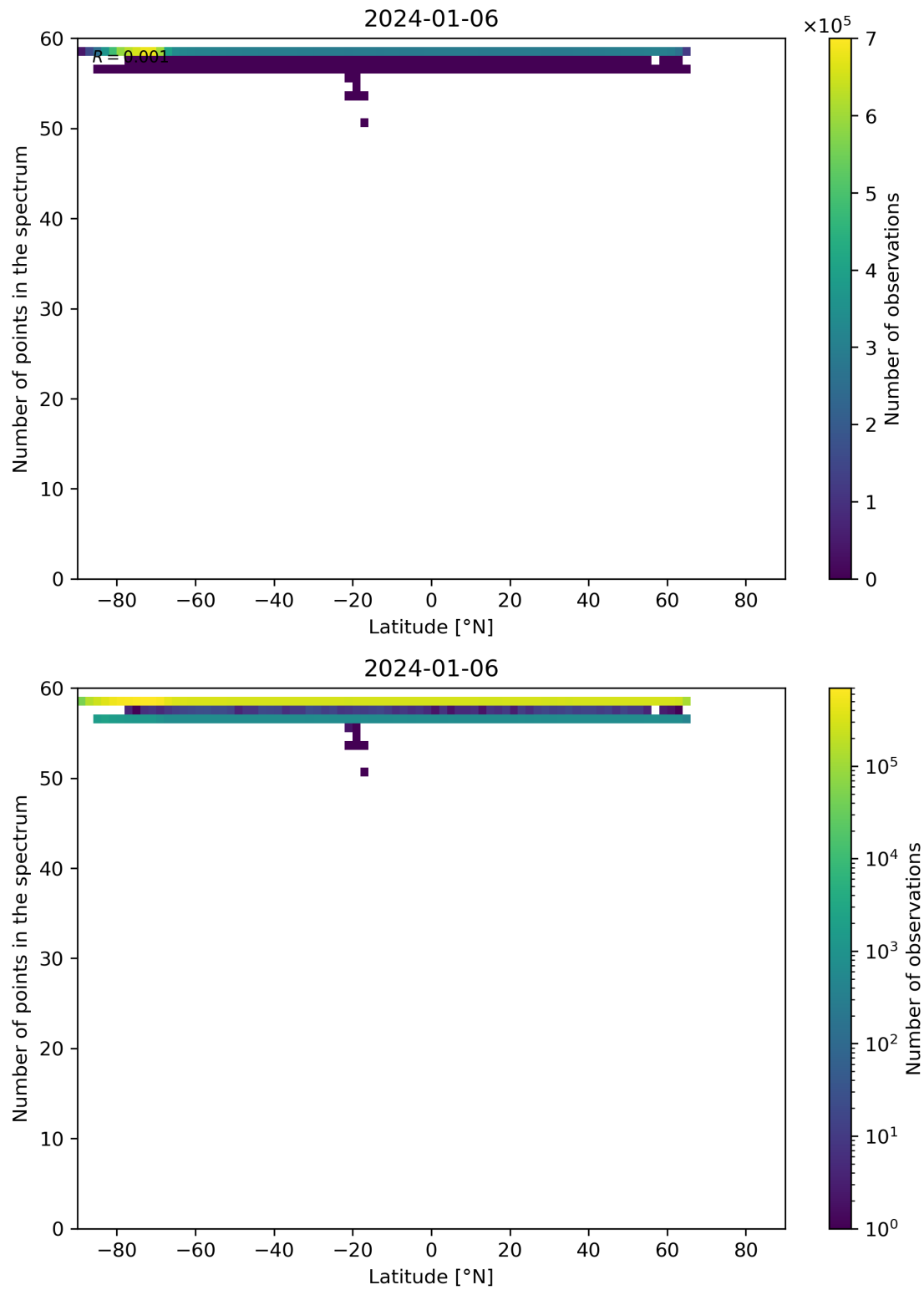
Figure 94: Scatter density plot of “Latitude” against “Number of points in the spectrum” for 2024-01-05 to 2024-01-07.
