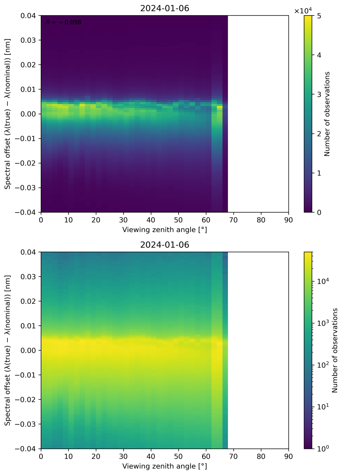
Figure 128: Scatter density plot of “Viewing zenith angle” against “Spectral offset ( \lambda(\text{true}) - \lambda(\text{nominal}) )” for 2024-01-05 to 2024-01-07.
