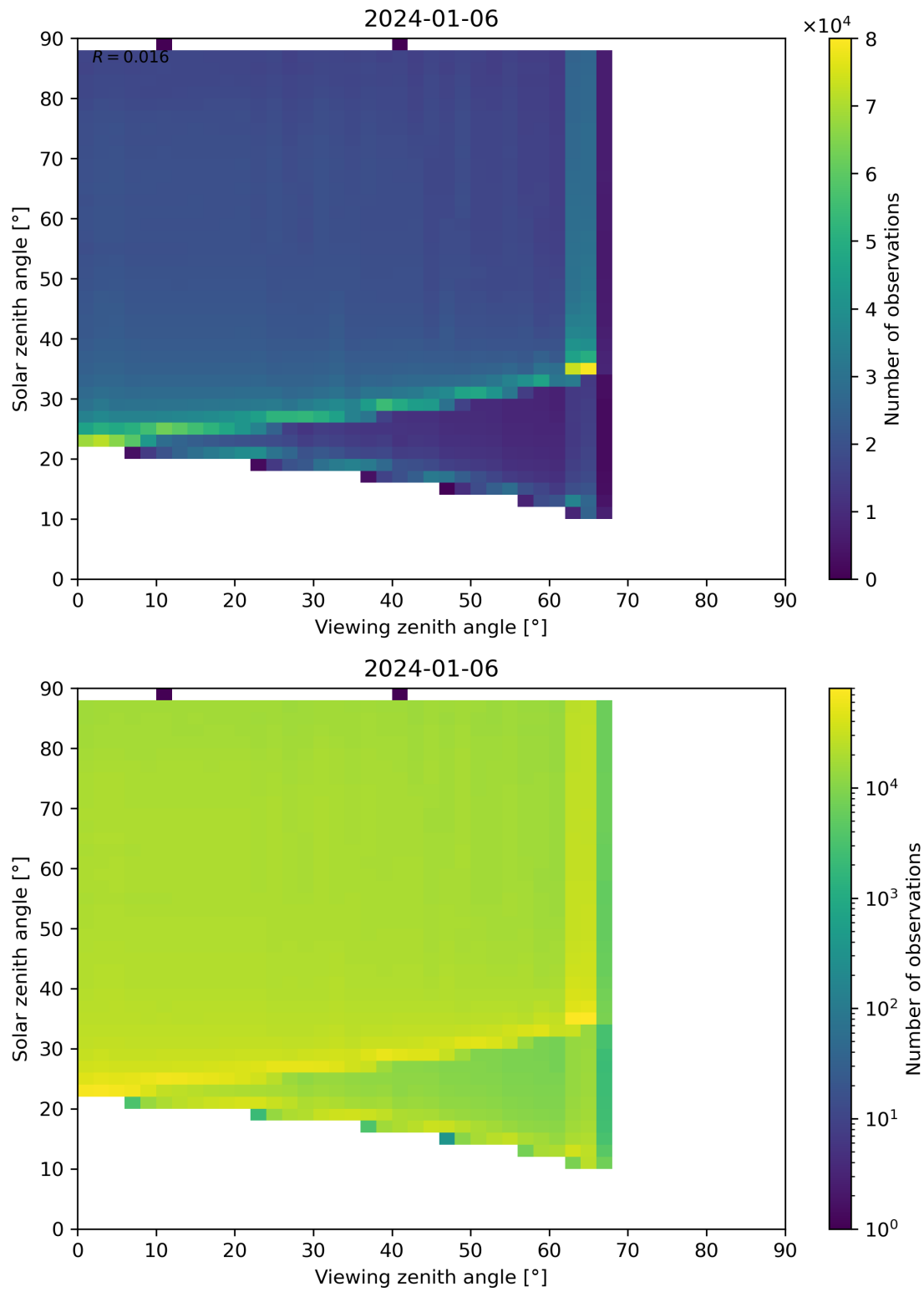
Figure 127: Scatter density plot of “Viewing zenith angle” against “Solar zenith angle” for 2024-01-05 to 2024-01-07.
