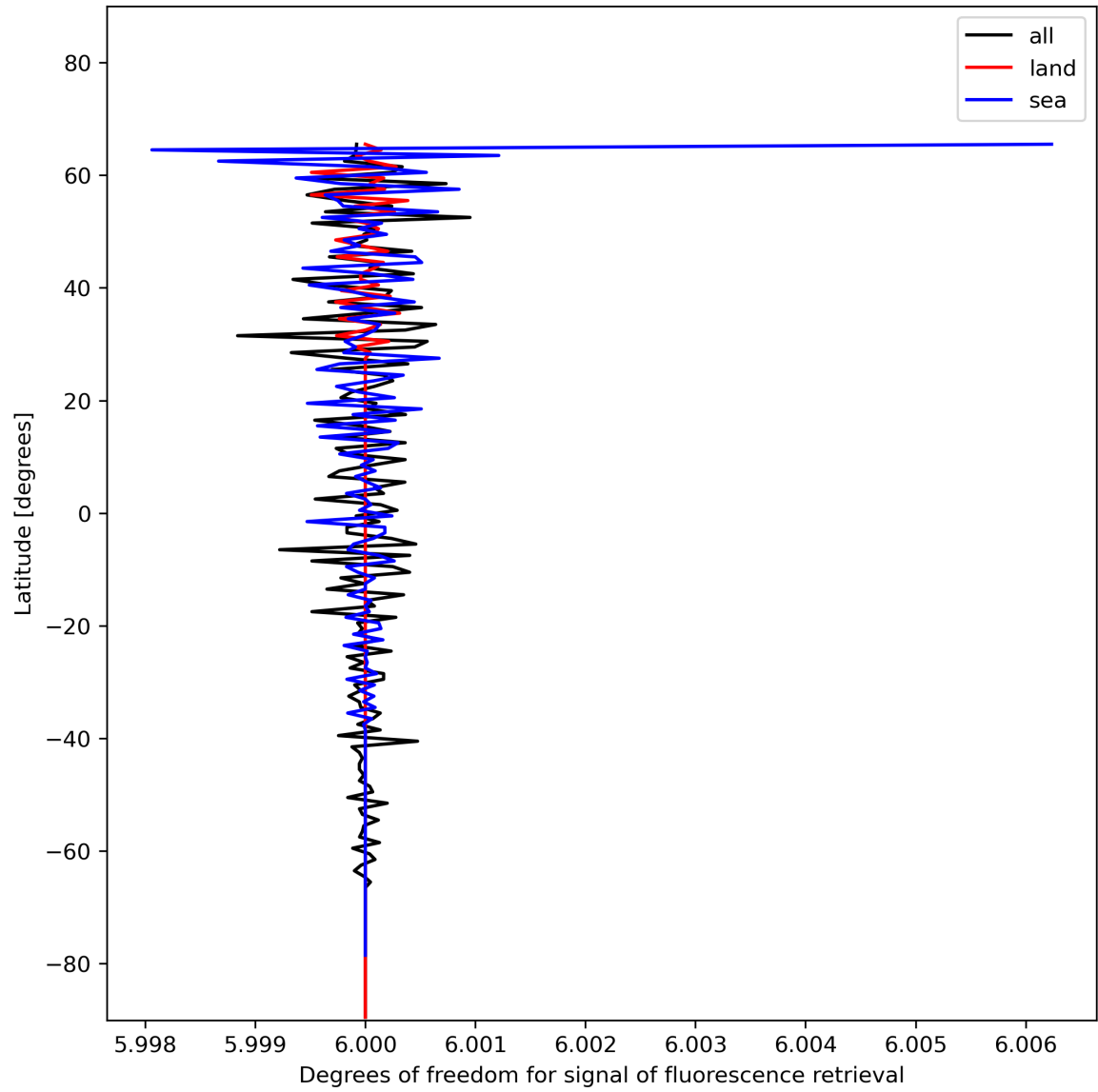
Figure 26: Zonal average of “Degrees of freedom for signal of fluorescence retrieval” for 2024-01-05 to 2024-01-07.
