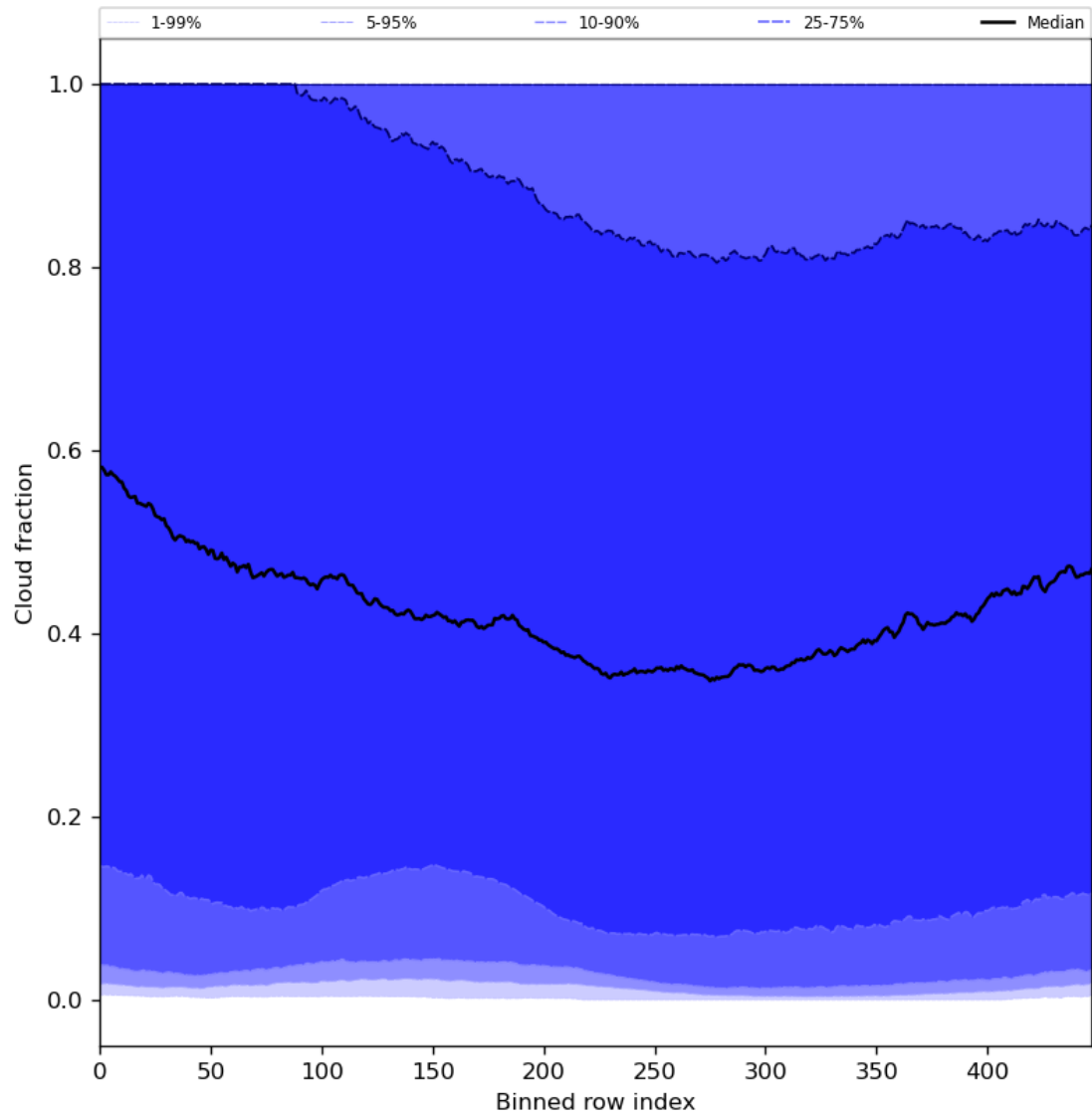
Figure 49: Along track statistics of “Cloud fraction” for 2024-01-05 to 2024-01-07
