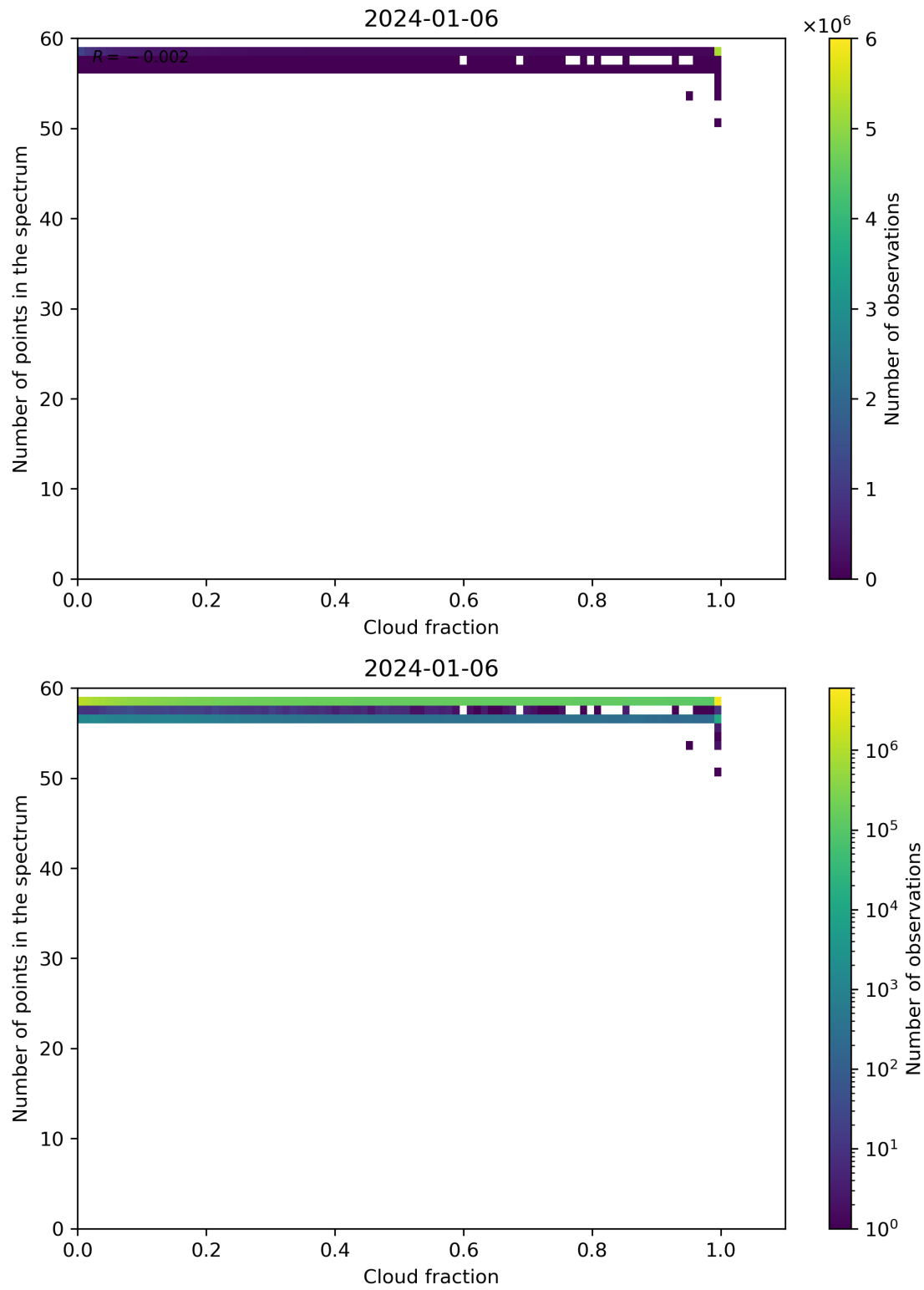
Figure 74: Scatter density plot of “Cloud fraction” against “Number of points in the spectrum” for 2024-01-05 to 2024-01-07.
