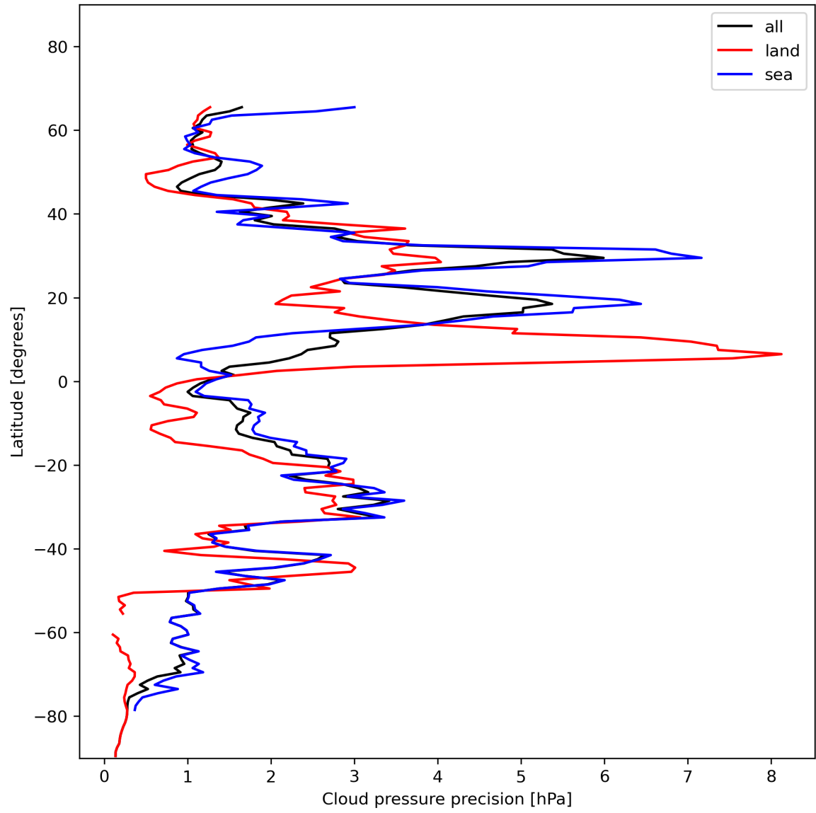
Figure 14: Zonal average of “Cloud pressure precision” for 2024-01-05 to 2024-01-07.
