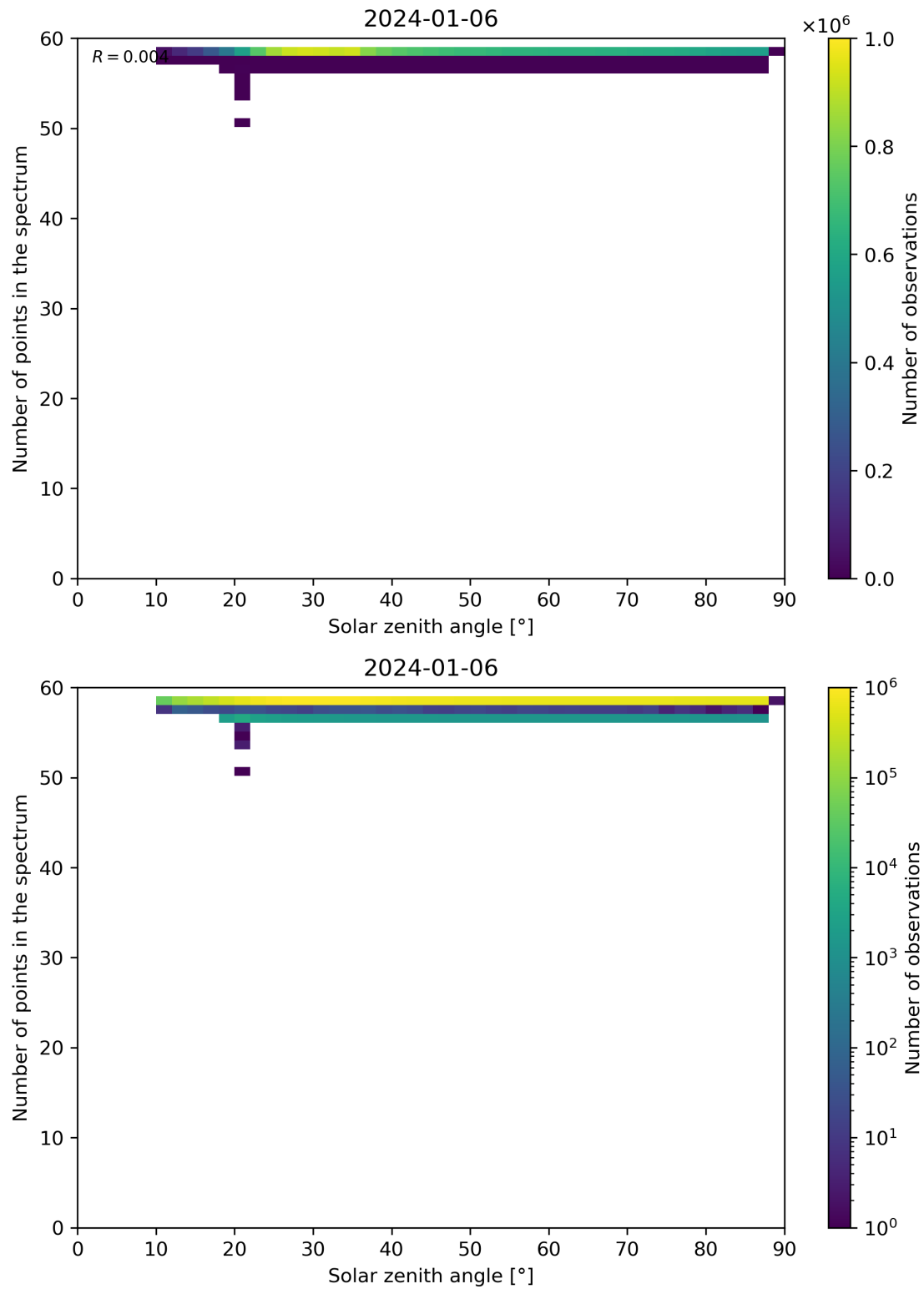
Figure 115: Scatter density plot of “Solar zenith angle” against “Number of points in the spectrum” for 2024-01-05 to 2024-01-07.
