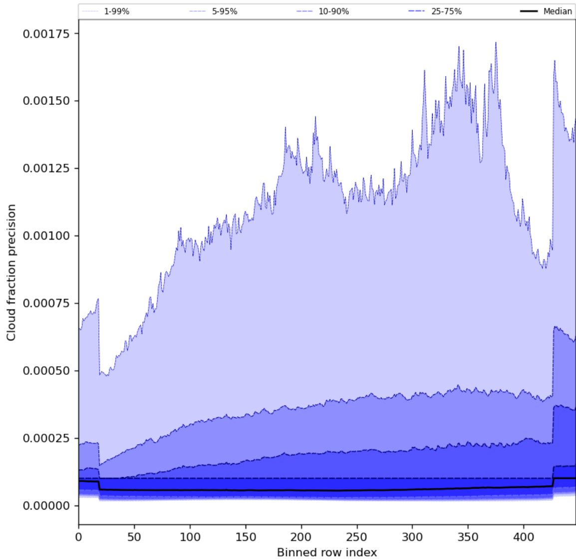
Figure 50: Along track statistics of “Cloud fraction precision” for 2024-01-05 to 2024-01-07
