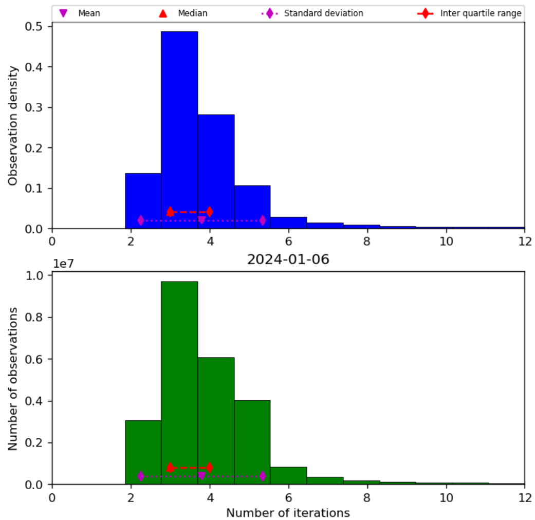
Figure 39: Histogram of “Number of iterations” for 2024-01-05 to 2024-01-07
