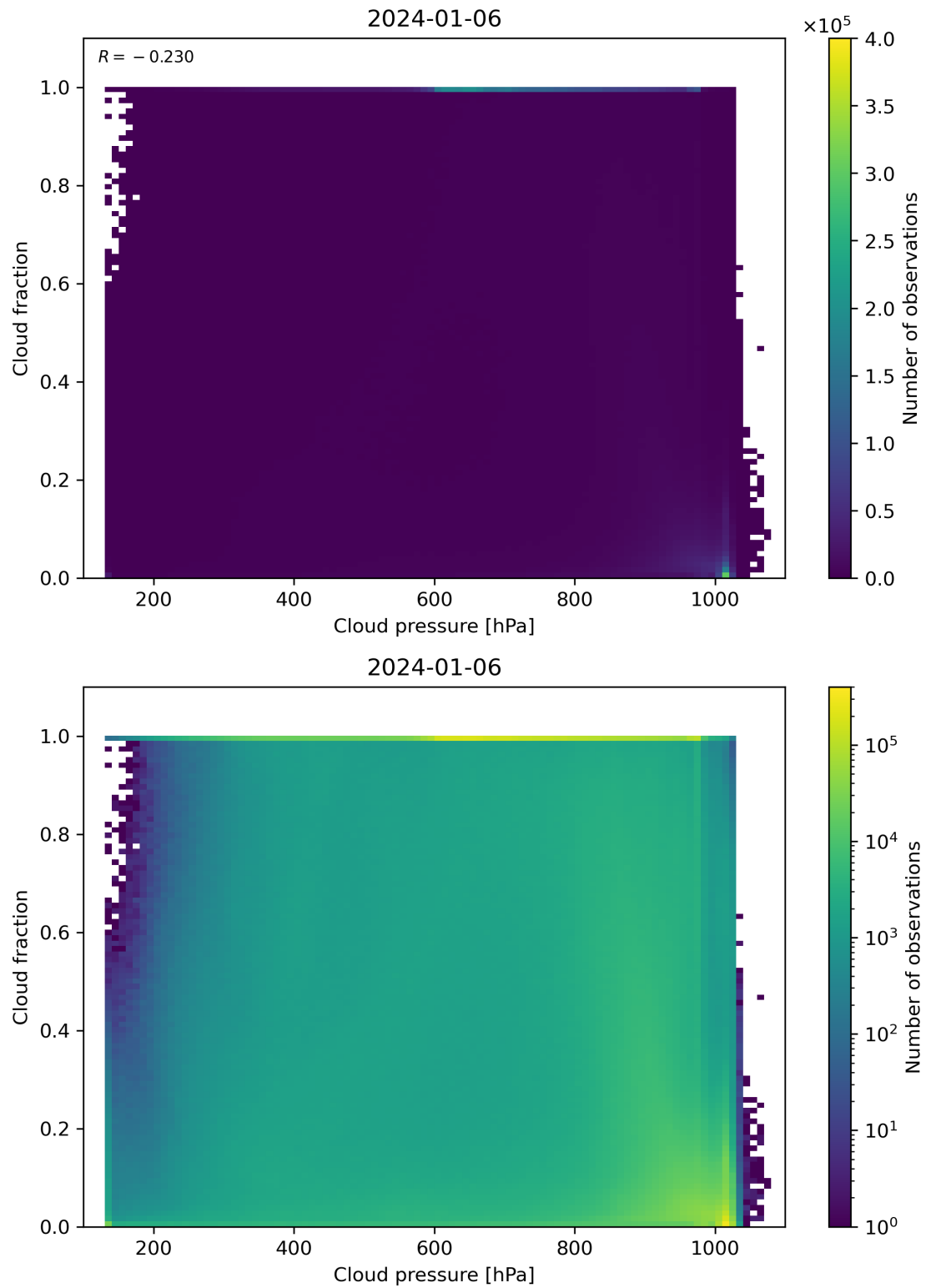
Figure 79: Scatter density plot of “Cloud pressure” against “Cloud fraction” for 2024-01-05 to 2024-01-07.
