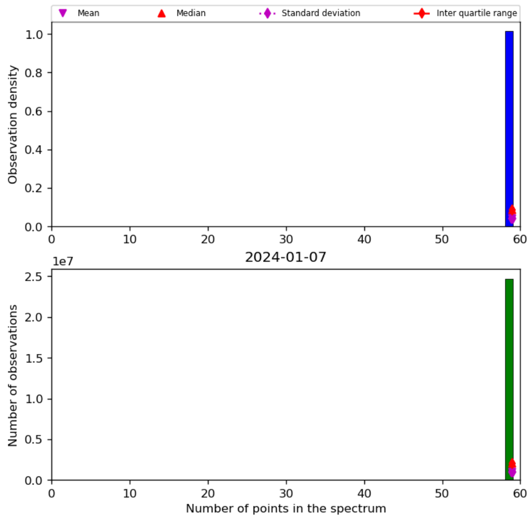
Figure 44: Histogram of “Number of points in the spectrum” for 2024-01-06 to 2024-01-08
