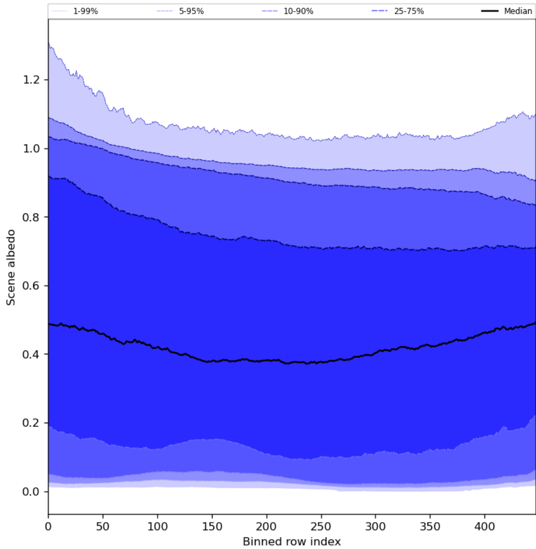
Figure 51: Along track statistics of “Scene albedo” for 2024-01-06 to 2024-01-08
