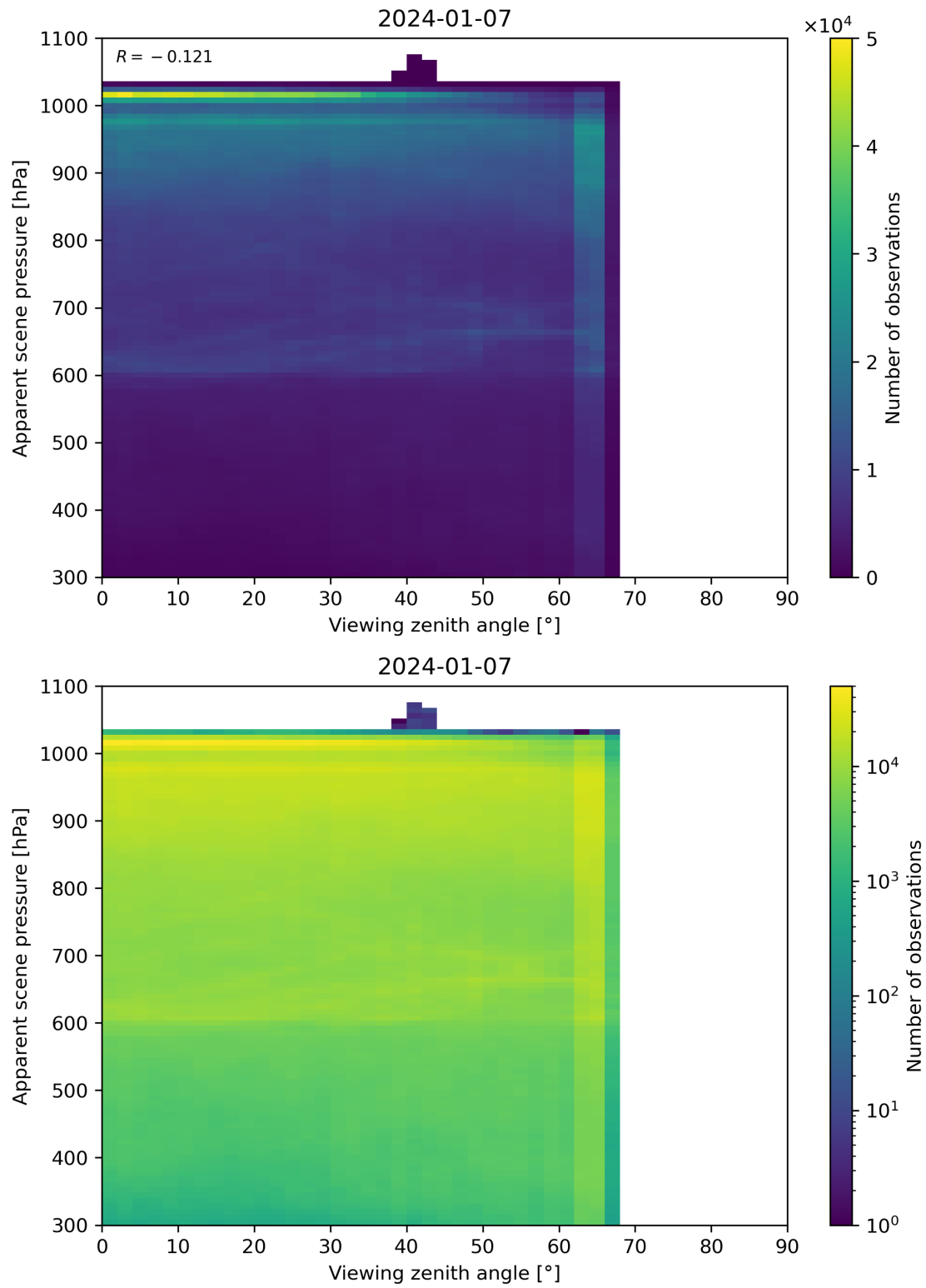
Figure 118: Scatter density plot of “Viewing zenith angle” against “Apparent scene pressure” for 2024-01-06 to 2024-01-08.
