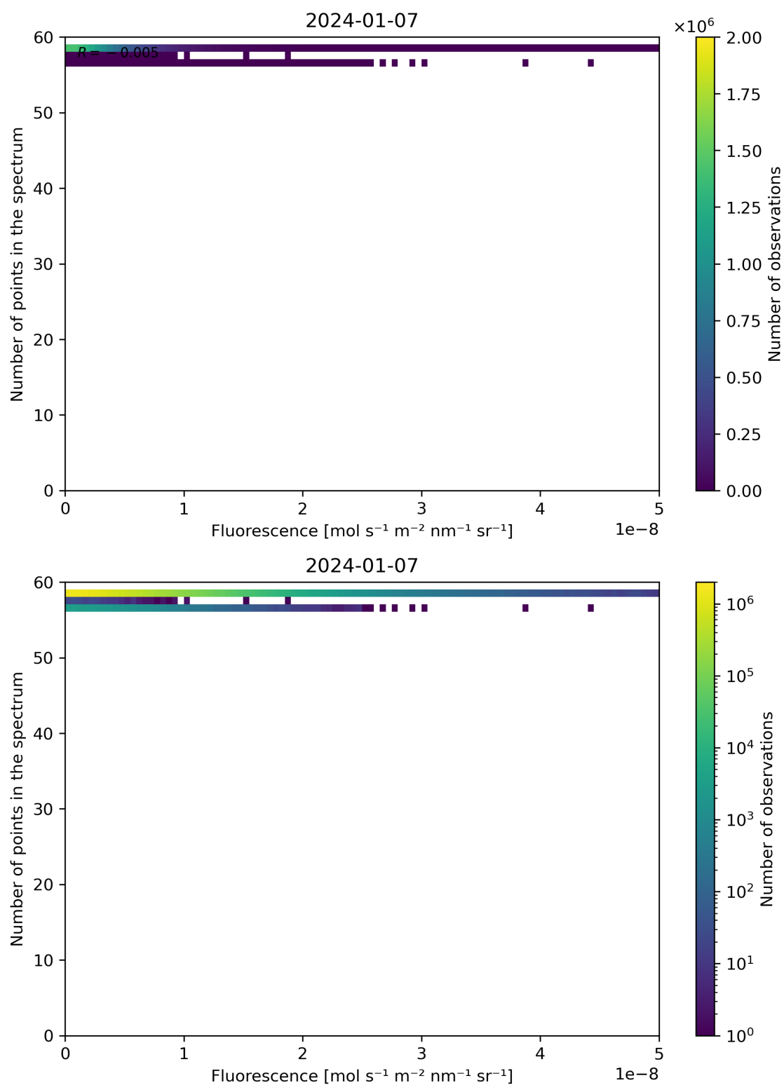
Figure 86: Scatter density plot of “Fluorescence” against “Number of points in the spectrum” for 2024-01-06 to 2024-01-08.
