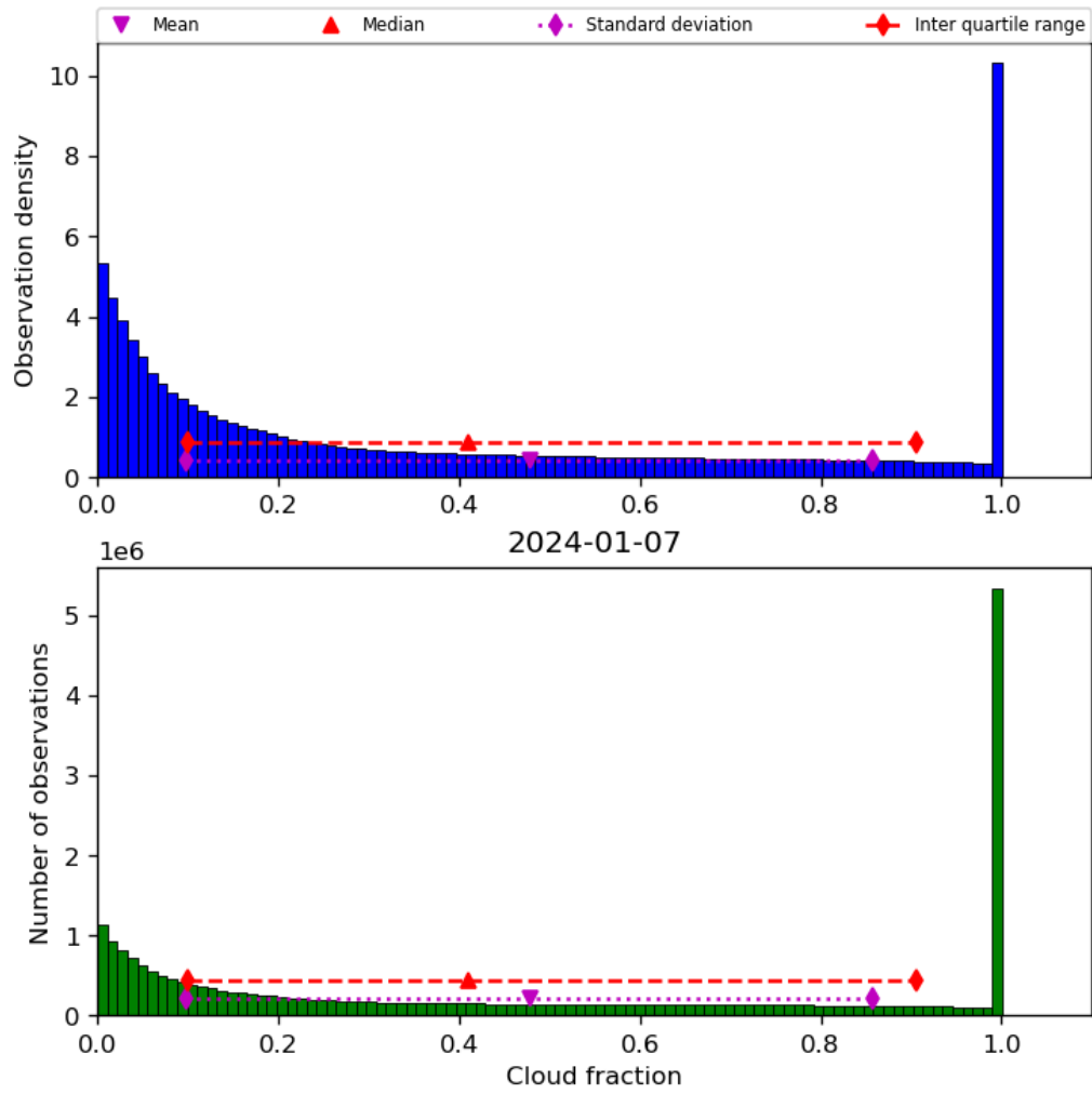
Figure 32: Histogram of “Cloud fraction” for 2024-01-06 to 2024-01-08
