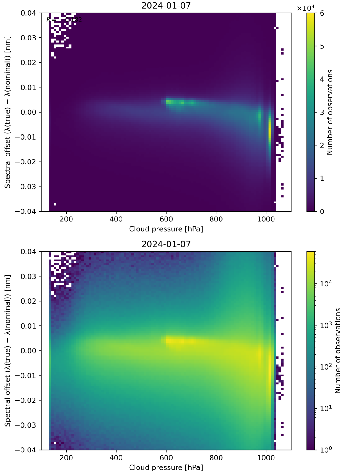
Figure 84: Scatter density plot of “Cloud pressure” against “Spectral offset ( \lambda(\text{true}) - \lambda(\text{nominal}) )” for 2024-01-06 to 2024-01-08.
