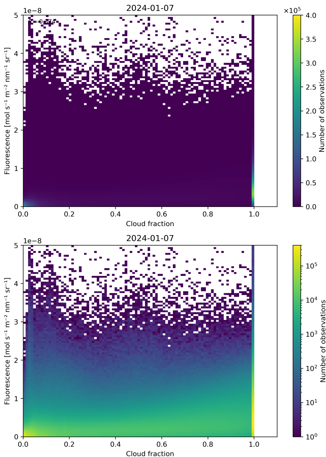
Figure 72: Scatter density plot of “Cloud fraction” against “Fluorescence” for 2024-01-06 to 2024-01-08.
