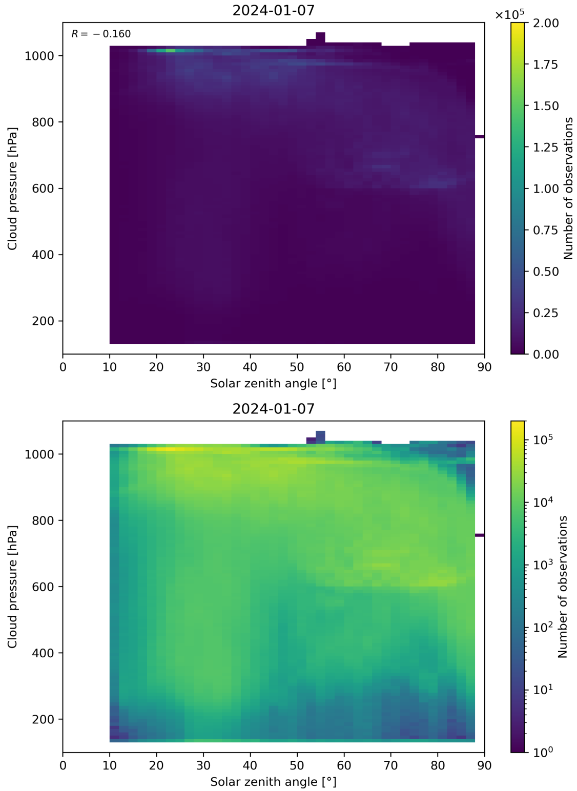
Figure 111: Scatter density plot of “Solar zenith angle” against “Cloud pressure” for 2024-01-06 to 2024-01-08.
