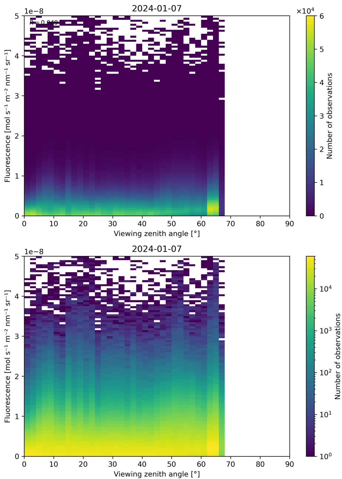
Figure 122: Scatter density plot of “Viewing zenith angle” against “Fluorescence” for 2024-01-06 to 2024-01-08.
