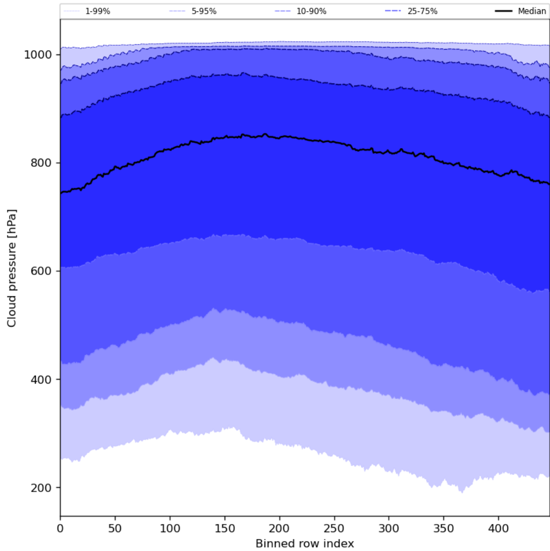
Figure 47: Along track statistics of “Cloud pressure” for 2024-01-06 to 2024-01-08
