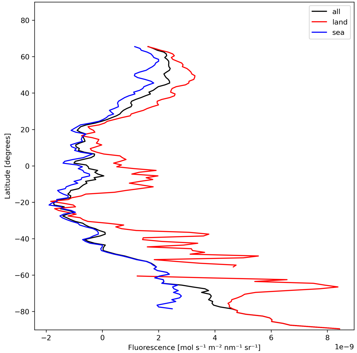
Figure 23: Zonal average of “Fluorescence” for 2024-01-06 to 2024-01-08.
