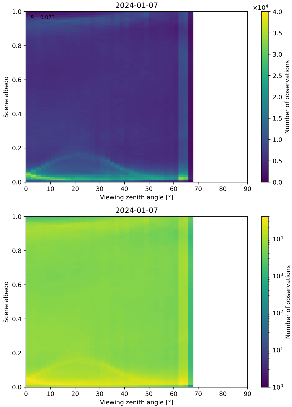
Figure 126: Scatter density plot of “Viewing zenith angle” against “Scene albedo” for 2024-01-06 to 2024-01-08.
