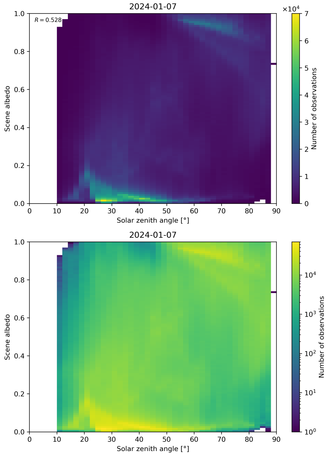
Figure 116: Scatter density plot of “Solar zenith angle” against “Scene albedo” for 2024-01-06 to 2024-01-08.
