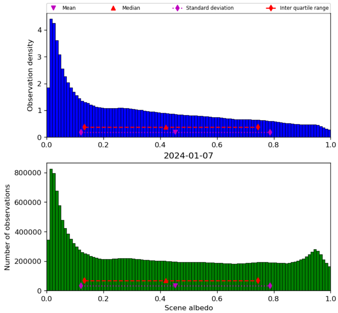
Figure 34: Histogram of “Scene albedo” for 2024-01-06 to 2024-01-08
