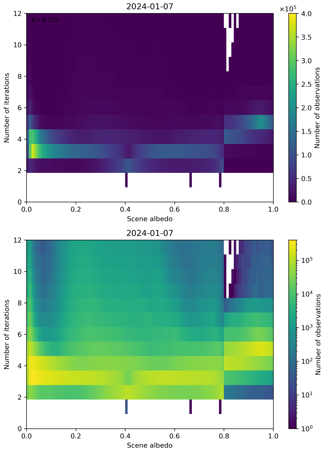
Figure 105: Scatter density plot of “Scene albedo” against “Number of iterations” for 2024-01-06 to 2024-01-08.
