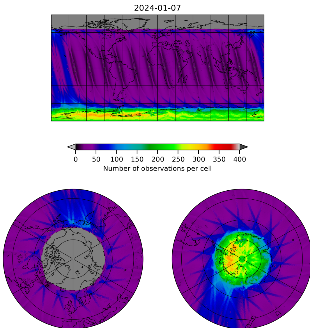
Figure 11: Map of the number of observations for 2024-01-06 to 2024-01-08
