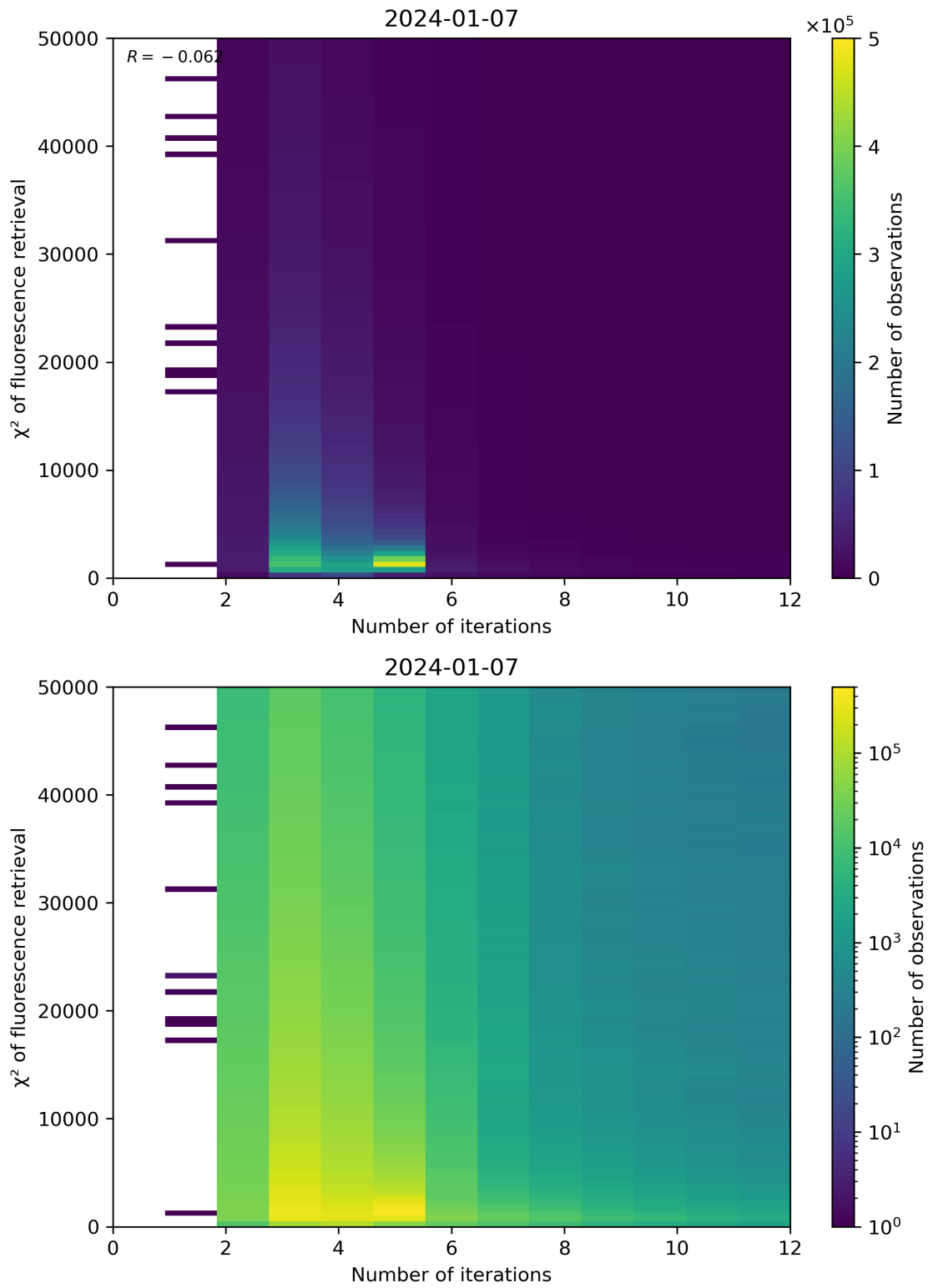
Figure 97: Scatter density plot of “Number of iterations” against “ \chi^2 of fluorescence retrieval” for 2024-01-06 to 2024-01-08.
