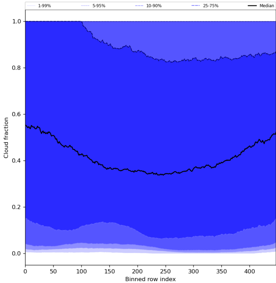
Figure 49: Along track statistics of “Cloud fraction” for 2024-01-06 to 2024-01-08
