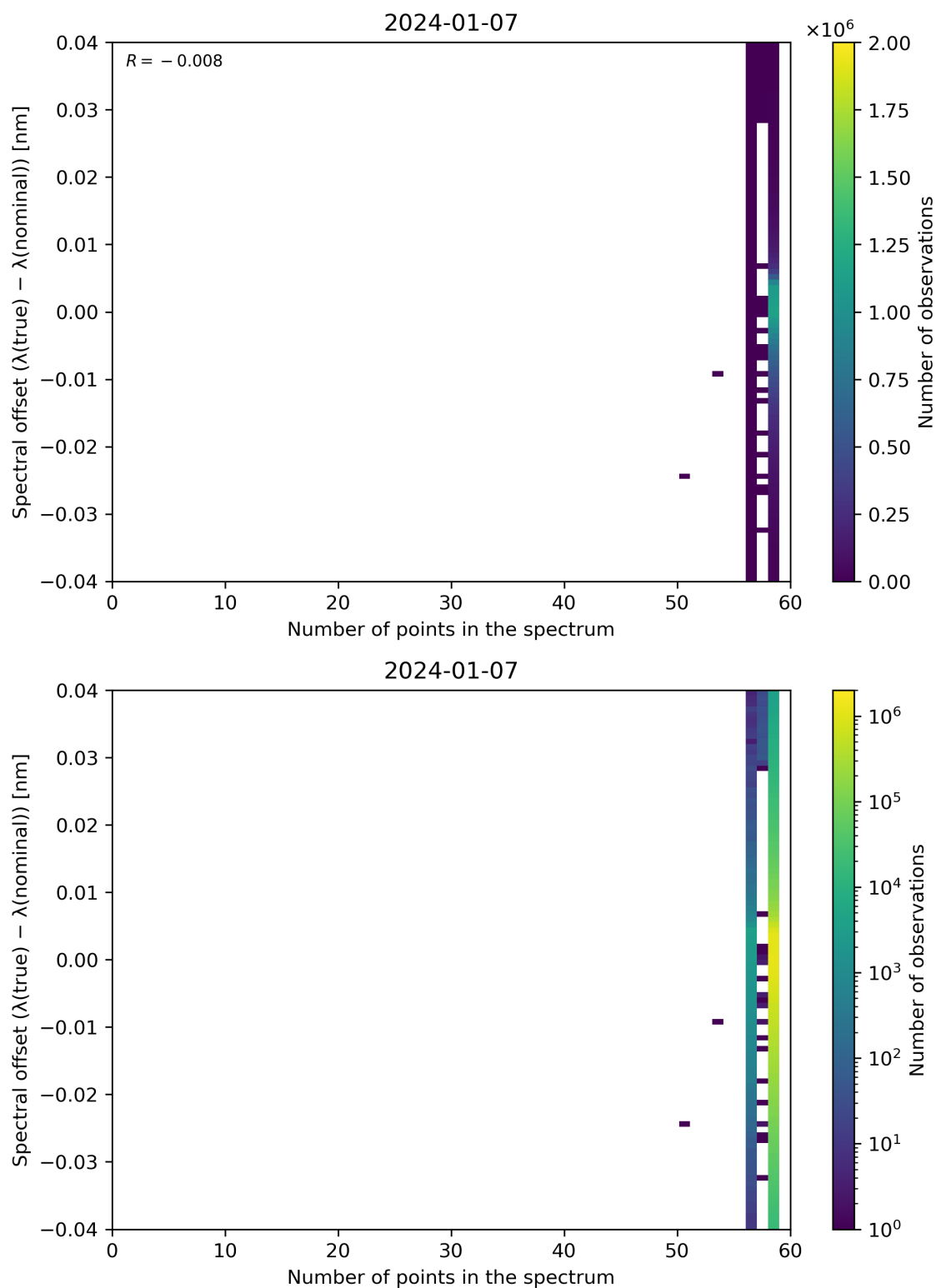
Figure 101: Scatter density plot of “Number of points in the spectrum” against “Spectral offset ( \lambda(\text{true}) - \lambda(\text{nominal}) )” for 2024-01-06 to 2024-01-08.
