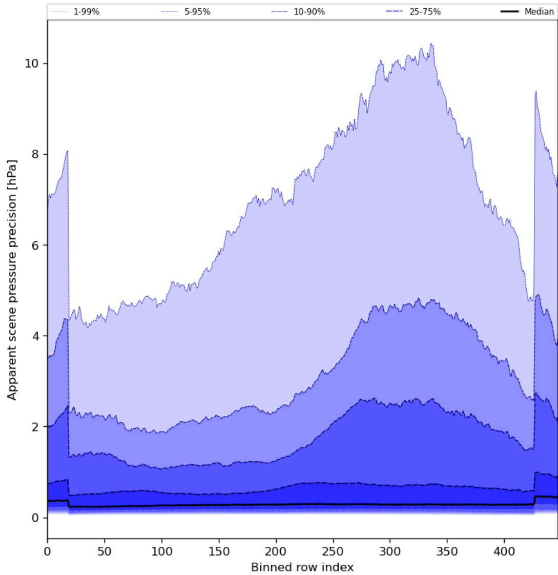
Figure 54: Along track statistics of “Apparent scene pressure precision” for 2024-01-06 to 2024-01-08
