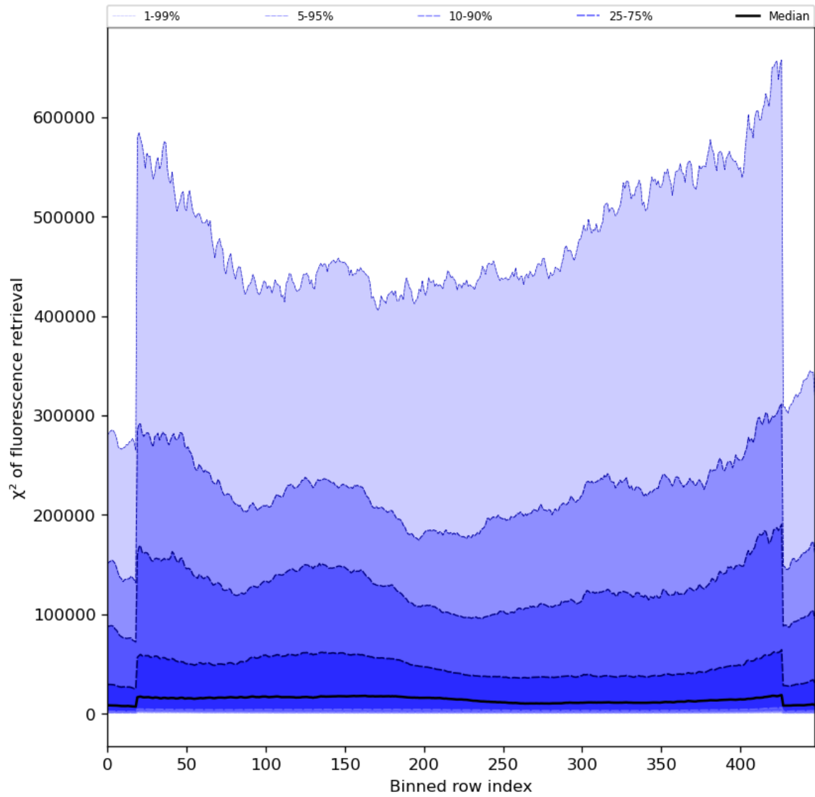
Figure 59: Along track statistics of “ \chi^2 of fluorescence retrieval” for 2024-01-06 to 2024-01-08
