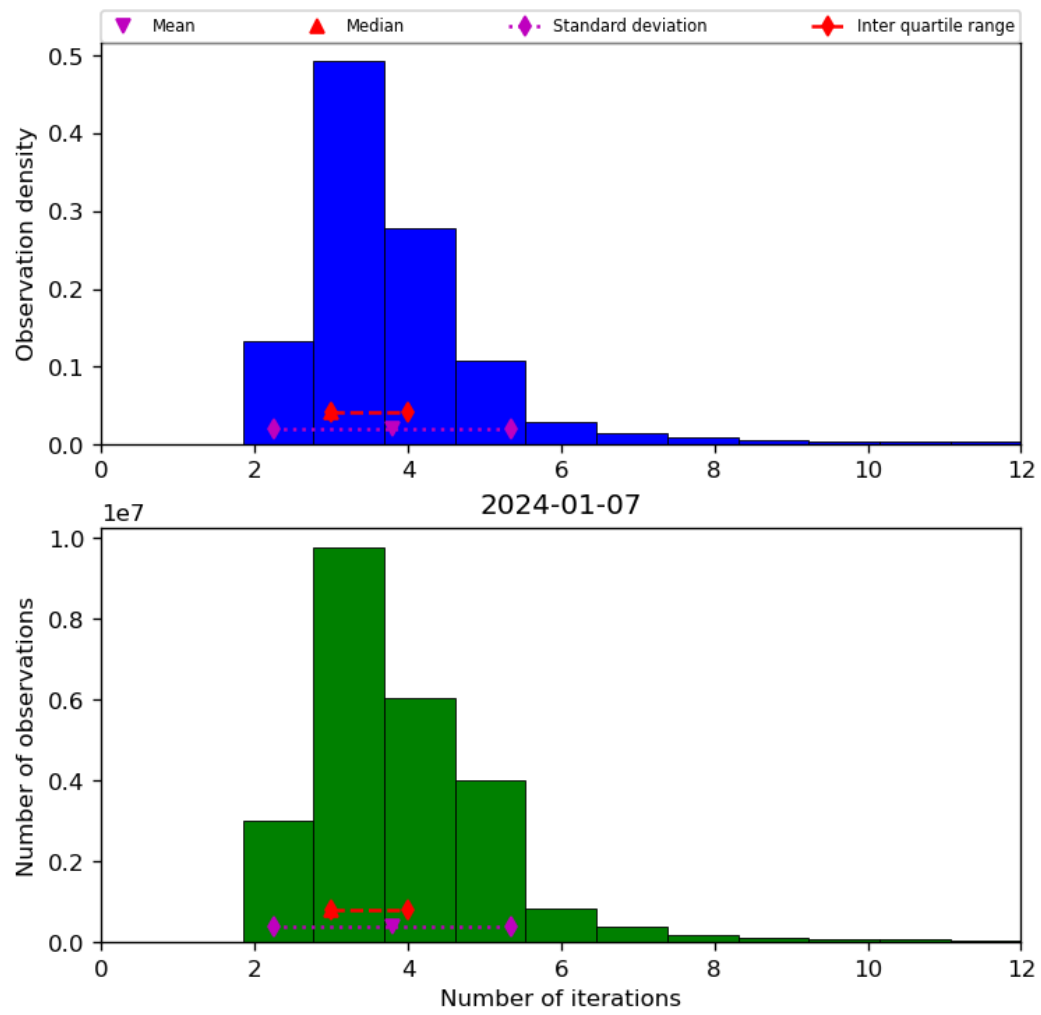
Figure 39: Histogram of “Number of iterations” for 2024-01-06 to 2024-01-08
