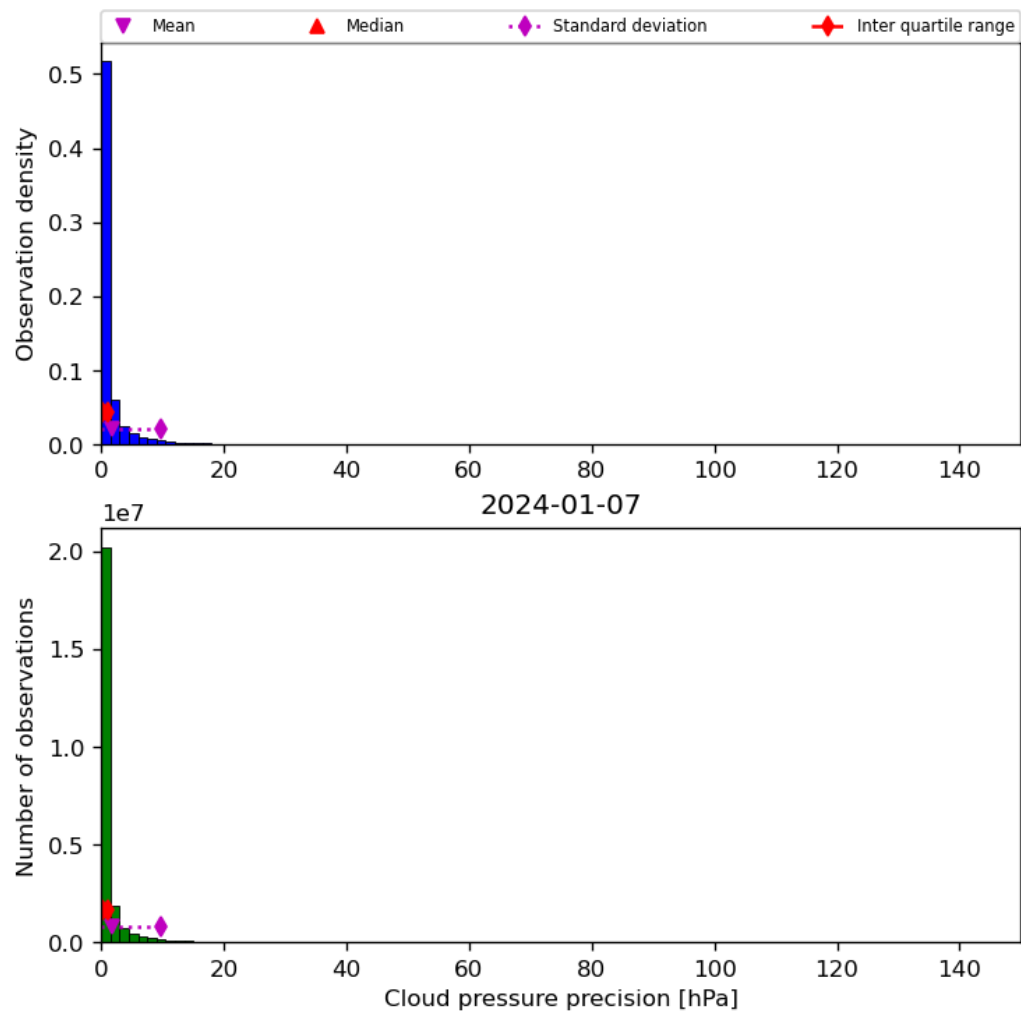
Figure 31: Histogram of “Cloud pressure precision” for 2024-01-06 to 2024-01-08
