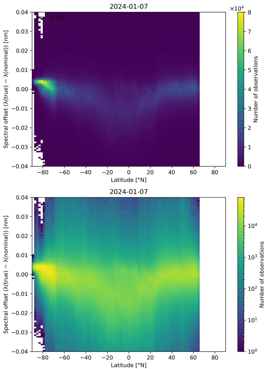
Figure 96: Scatter density plot of “Latitude” against “Spectral offset ( \lambda(\text{true}) - \lambda(\text{nominal}) )” for 2024-01-06 to 2024-01-08.
