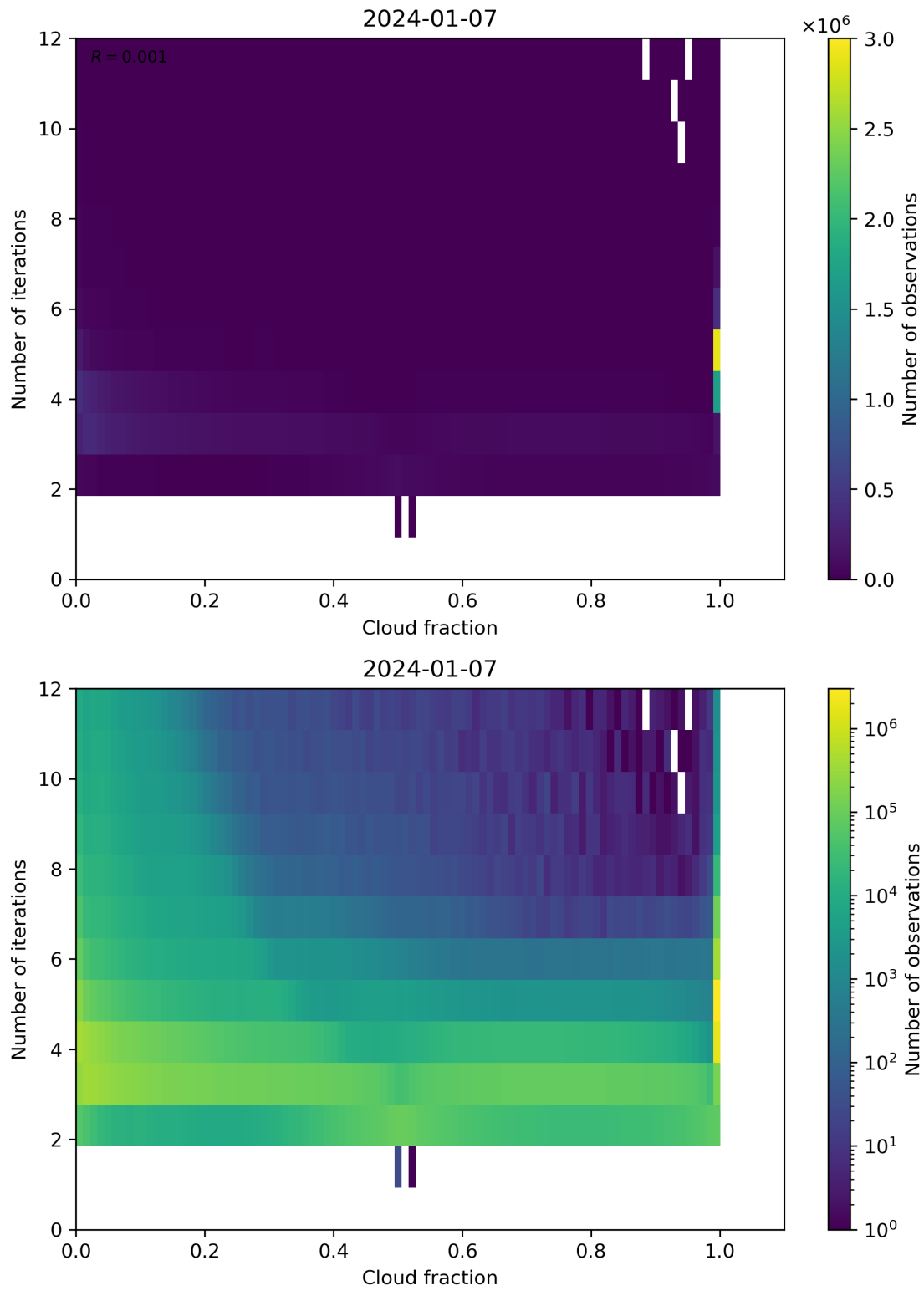
Figure 73: Scatter density plot of “Cloud fraction” against “Number of iterations” for 2024-01-06 to 2024-01-08.
