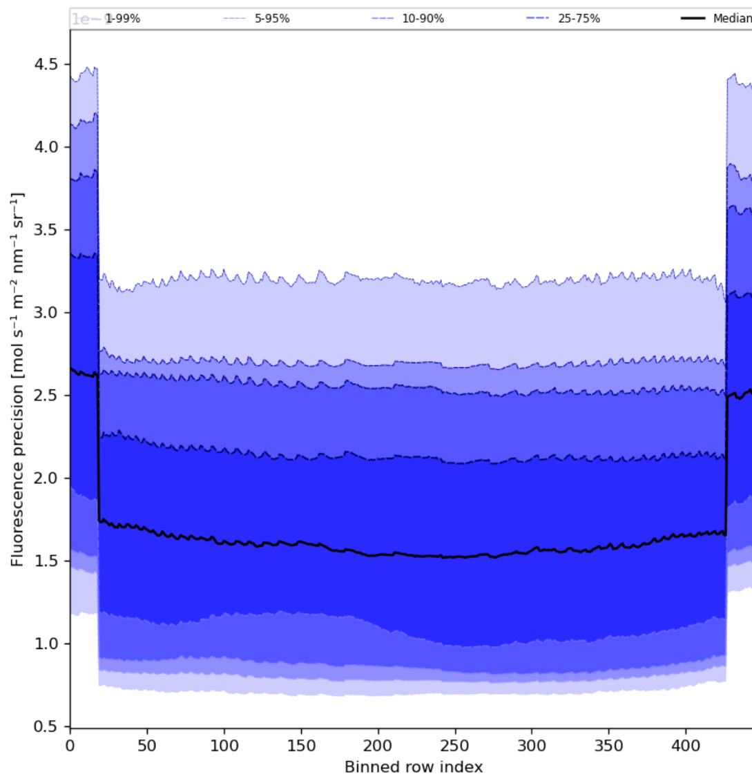
Figure 58: Along track statistics of “Fluorescence precision” for 2024-01-06 to 2024-01-08
