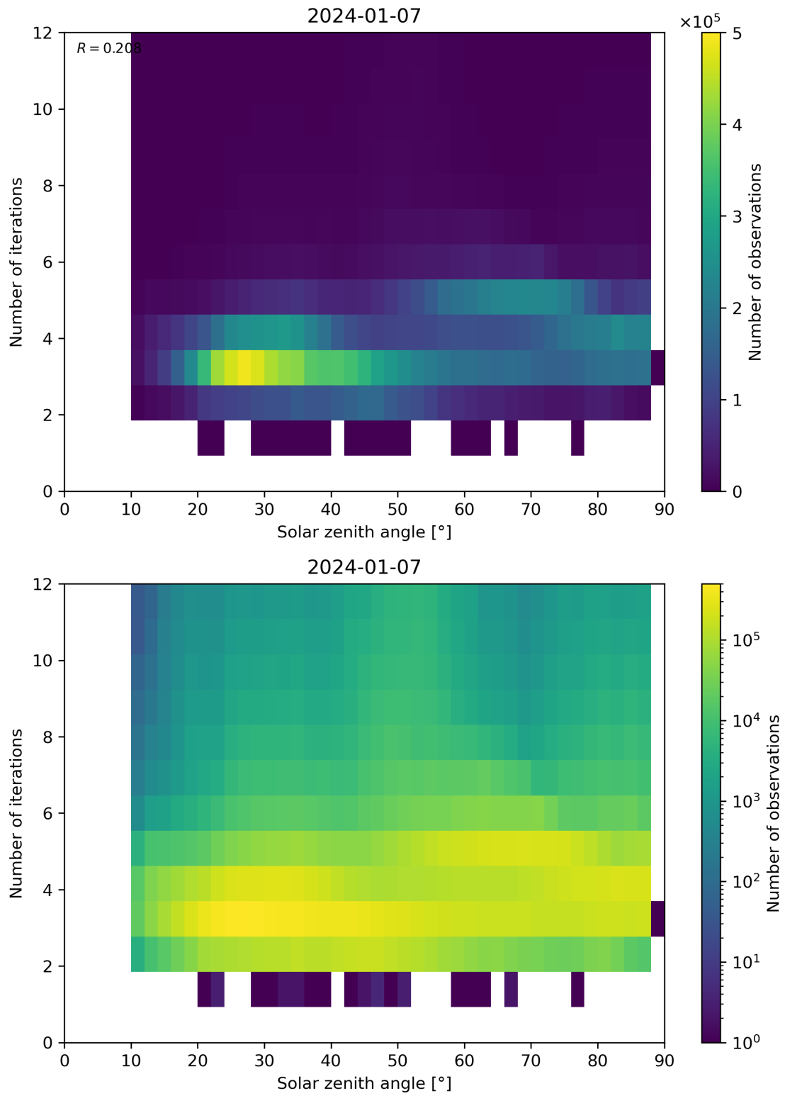
Figure 114: Scatter density plot of “Solar zenith angle” against “Number of iterations” for 2024-01-06 to 2024-01-08.
