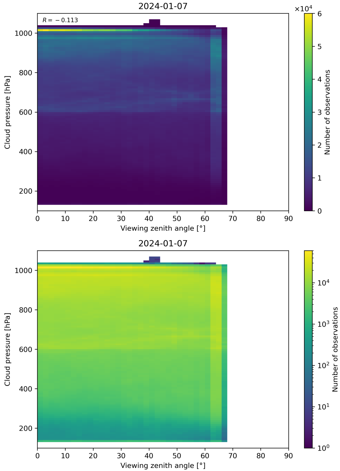
Figure 121: Scatter density plot of “Viewing zenith angle” against “Cloud pressure” for 2024-01-06 to 2024-01-08.
