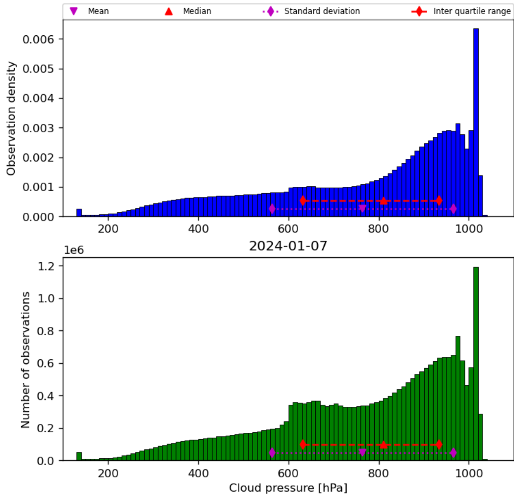
Figure 30: Histogram of “Cloud pressure” for 2024-01-06 to 2024-01-08
