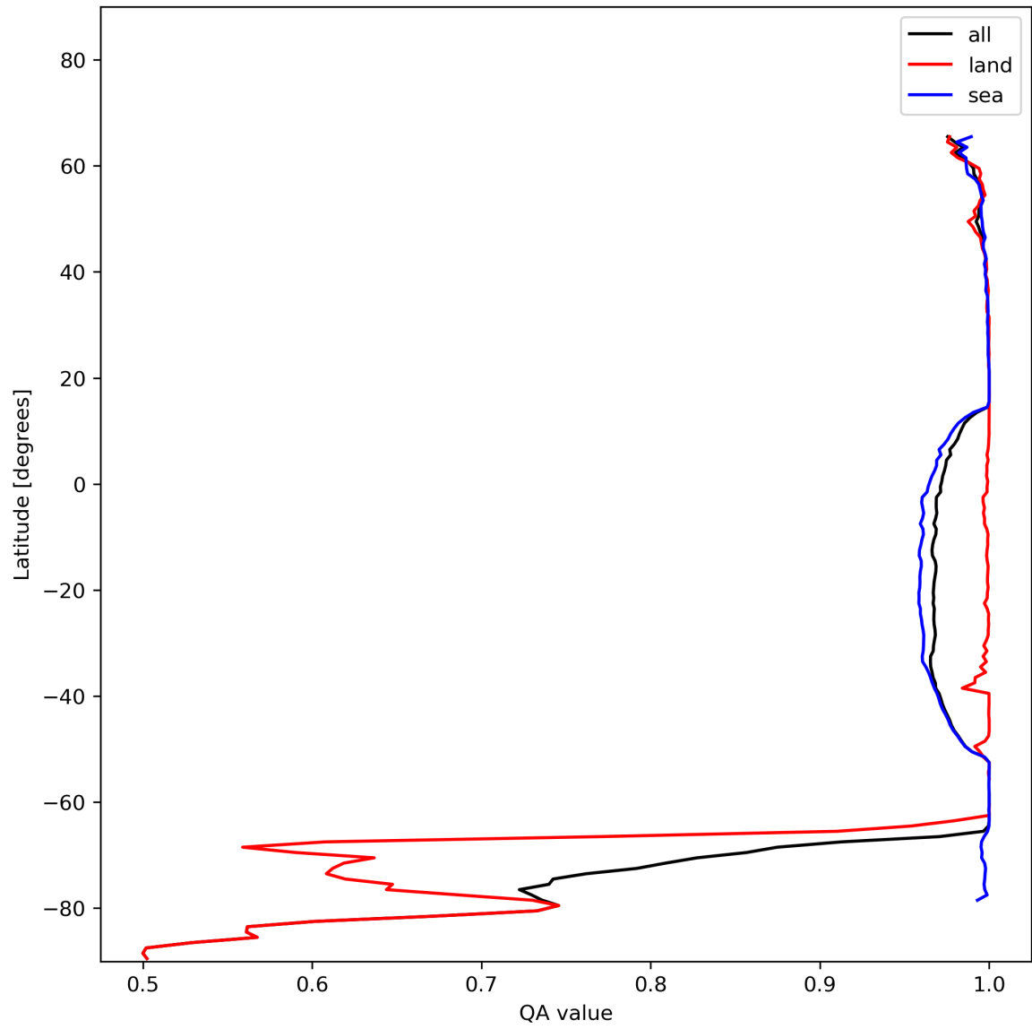
Figure 12: Zonal average of “QA value” for 2024-01-06 to 2024-01-08.
