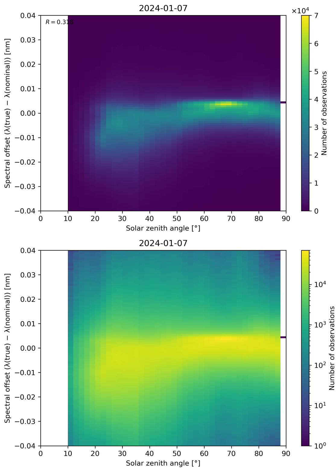
Figure 117: Scatter density plot of “Solar zenith angle” against “Spectral offset ( \lambda(\text{true}) - \lambda(\text{nominal}) )” for 2024-01-06 to 2024-01-08.
