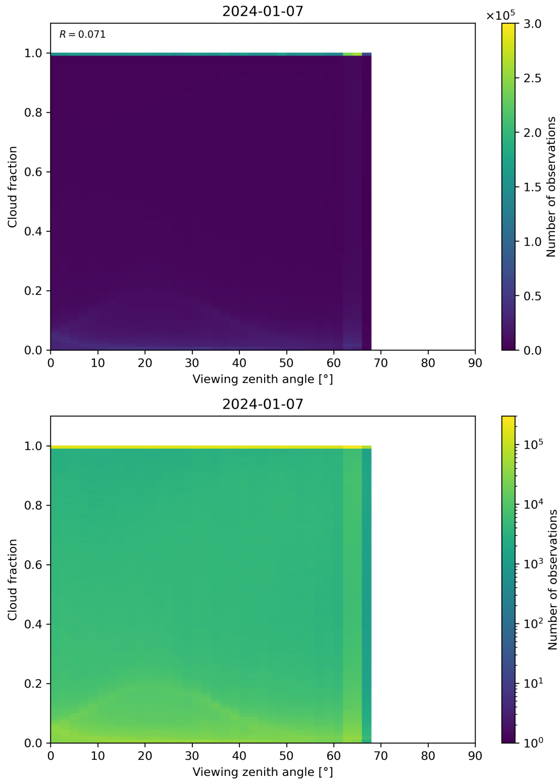
Figure 120: Scatter density plot of “Viewing zenith angle” against “Cloud fraction” for 2024-01-06 to 2024-01-08.
