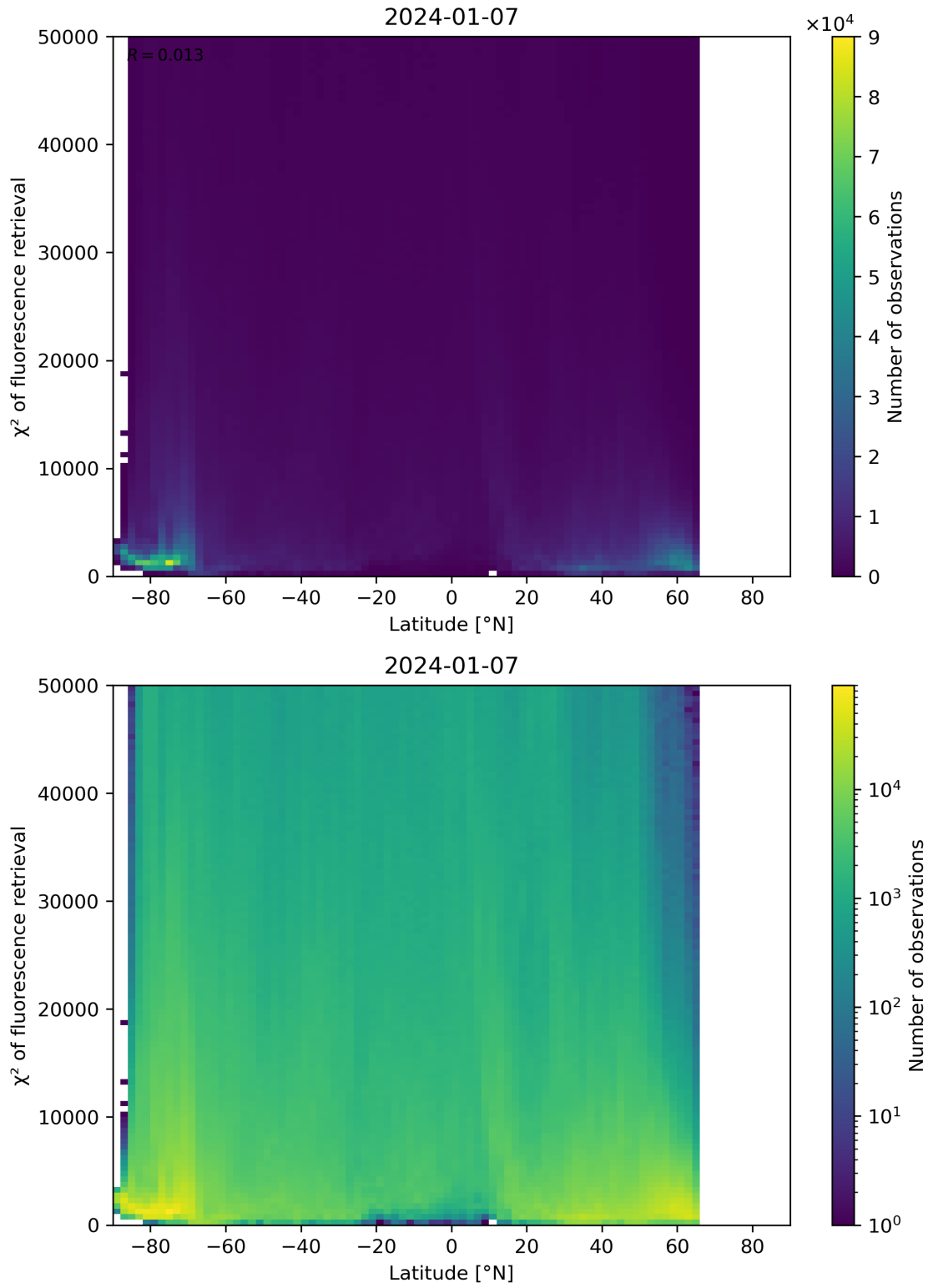
Figure 89: Scatter density plot of “Latitude” against “ \chi^2 of fluorescence retrieval” for 2024-01-06 to 2024-01-08.
