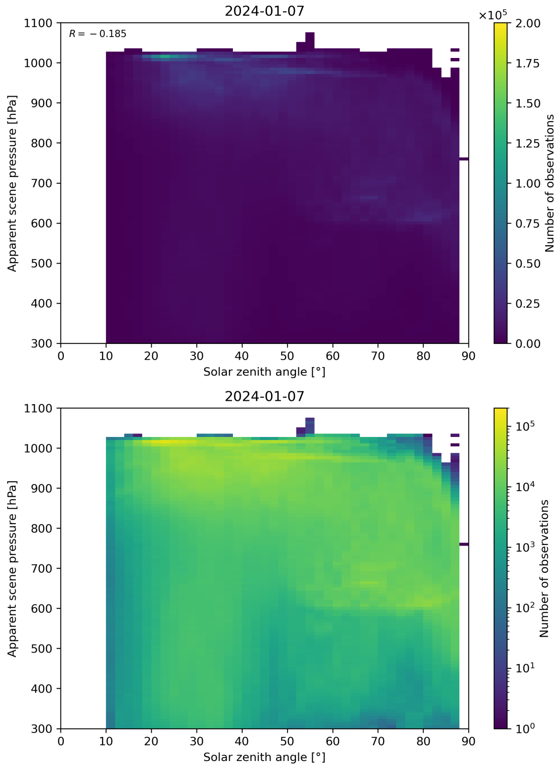
Figure 108: Scatter density plot of “Solar zenith angle” against “Apparent scene pressure” for 2024-01-06 to 2024-01-08.
