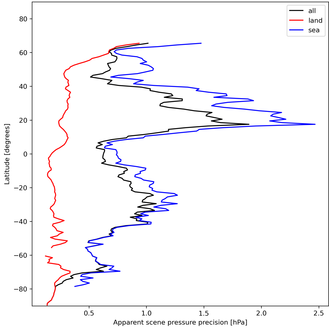
Figure 20: Zonal average of “Apparent scene pressure precision” for 2024-01-06 to 2024-01-08.
