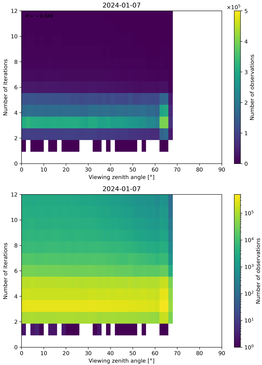
Figure 124: Scatter density plot of “Viewing zenith angle” against “Number of iterations” for 2024-01-06 to 2024-01-08.
