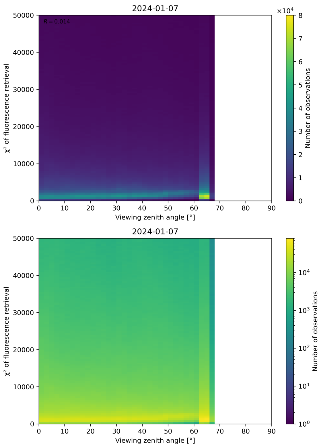
Figure 119: Scatter density plot of “Viewing zenith angle” against “ \chi^2 of fluorescence retrieval” for 2024-01-06 to 2024-01-08.
