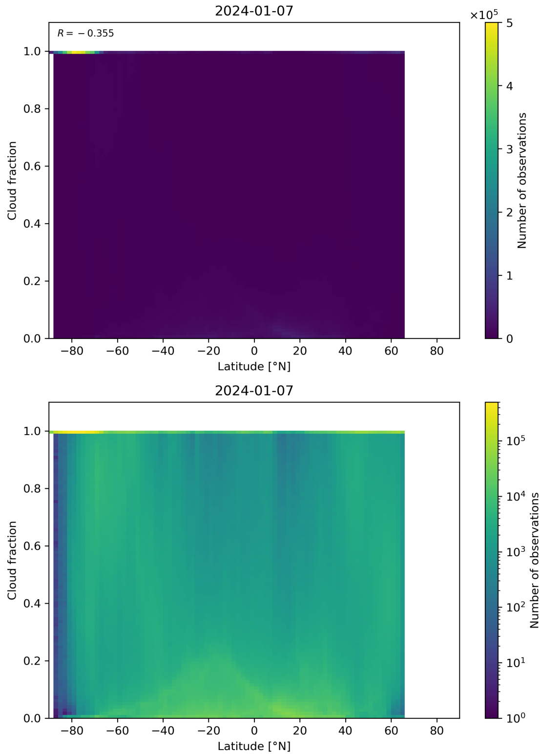
Figure 90: Scatter density plot of “Latitude” against “Cloud fraction” for 2024-01-06 to 2024-01-08.
