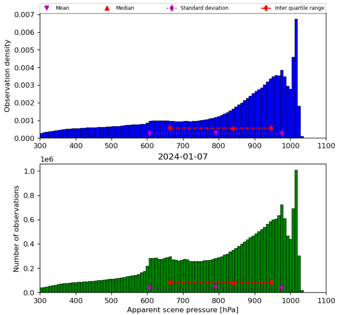
Figure 36: Histogram of “Apparent scene pressure” for 2024-01-06 to 2024-01-08
