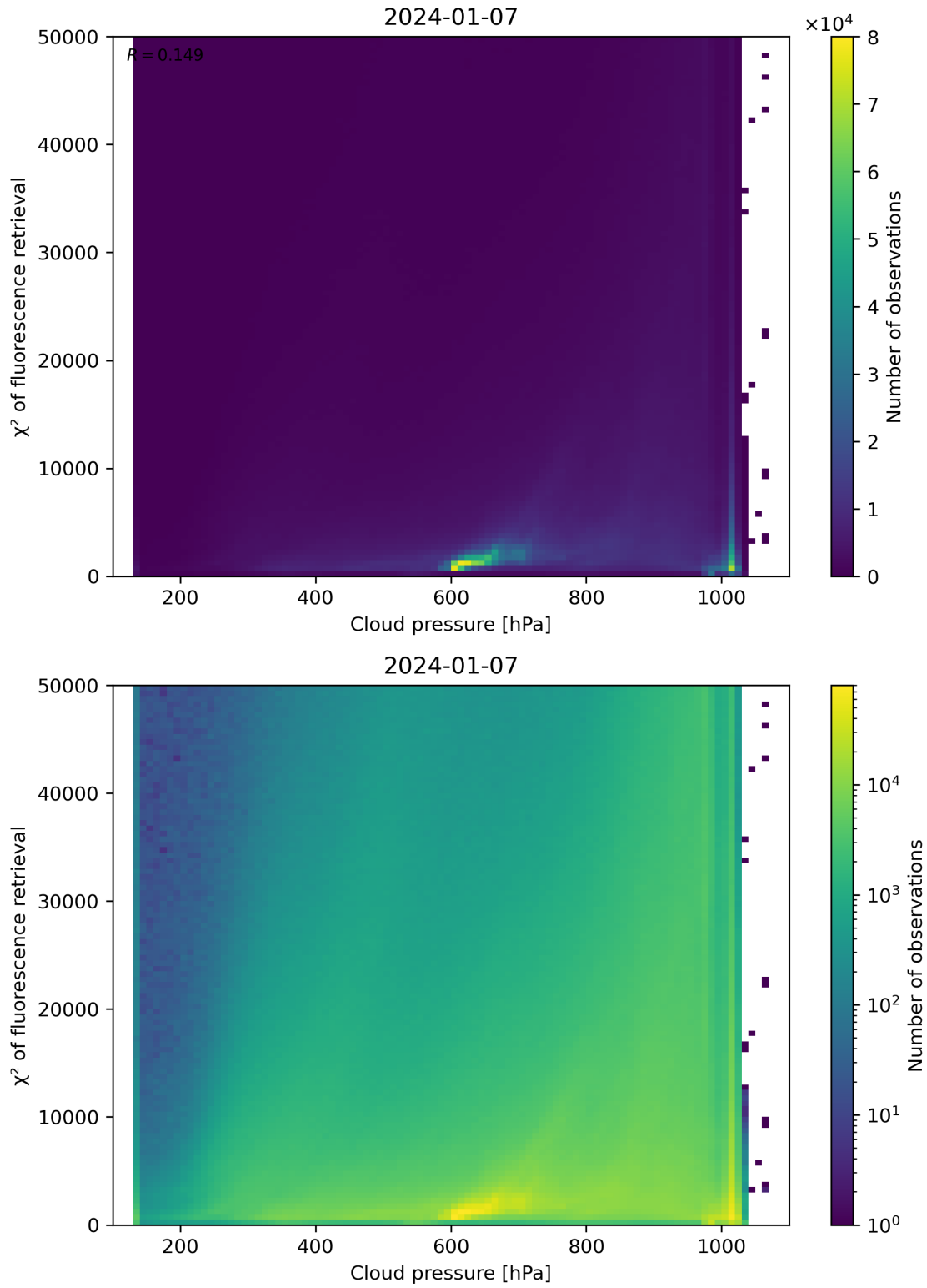
Figure 78: Scatter density plot of “Cloud pressure” against “ \chi^2 of fluorescence retrieval” for 2024-01-06 to 2024-01-08.
