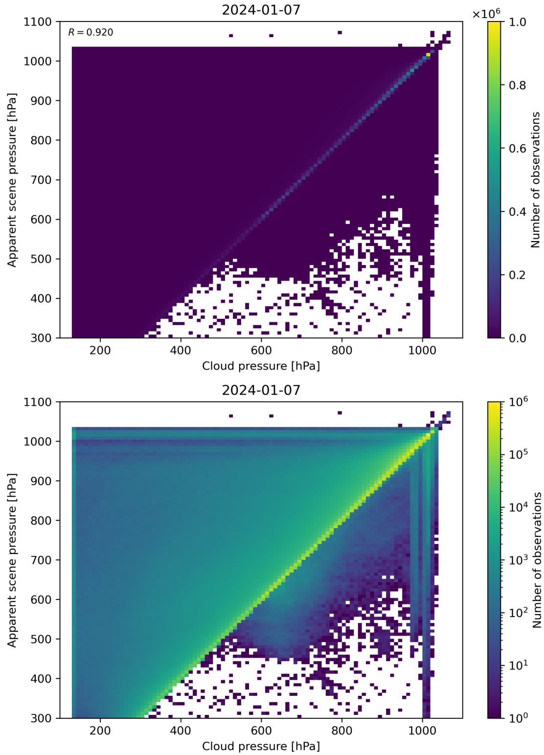
Figure 77: Scatter density plot of “Cloud pressure” against “Apparent scene pressure” for 2024-01-06 to 2024-01-08.
