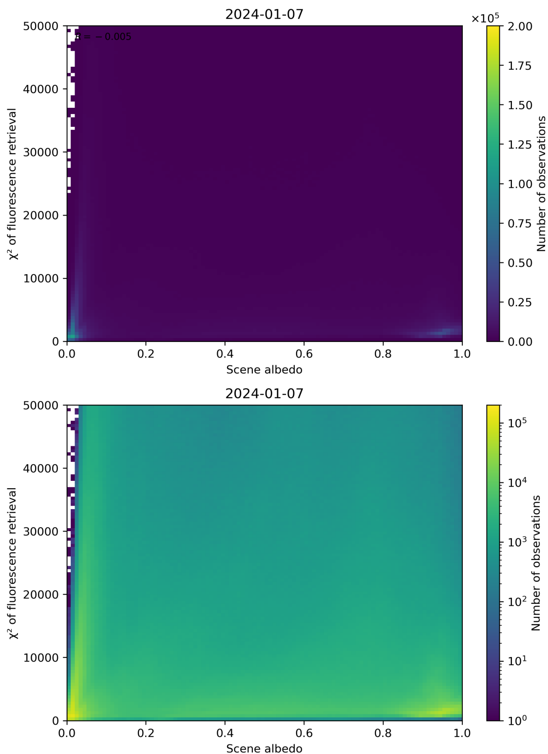
Figure 103: Scatter density plot of “Scene albedo” against “ \chi^2 of fluorescence retrieval” for 2024-01-06 to 2024-01-08.
