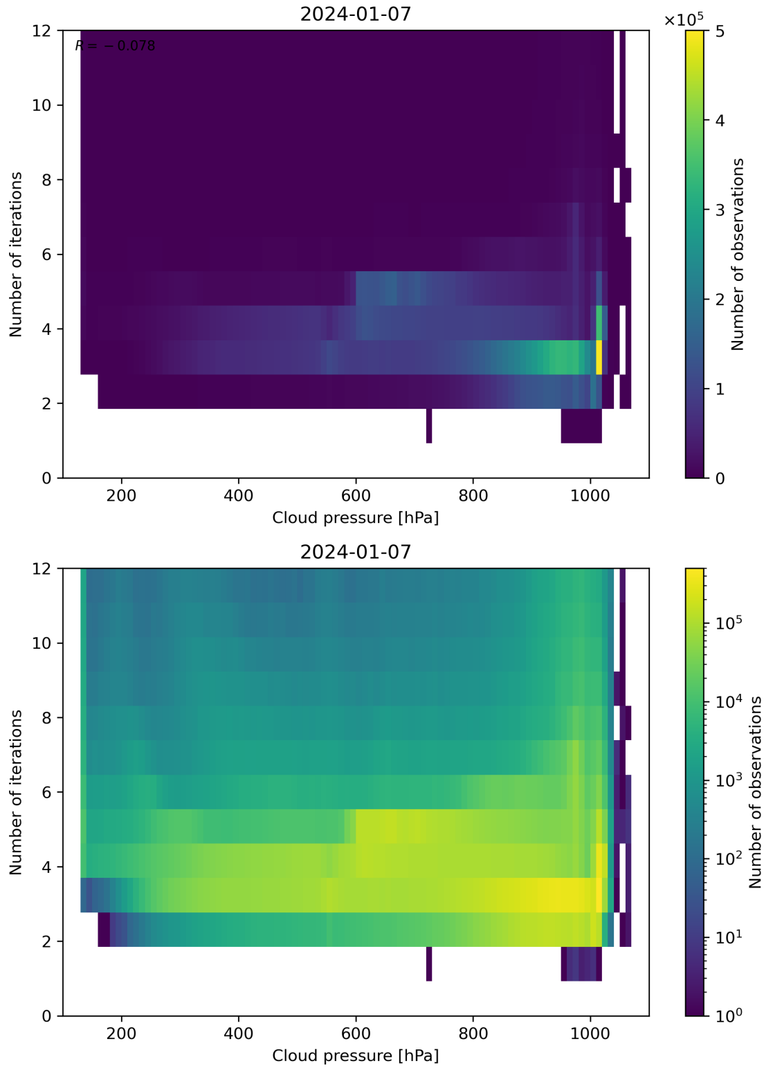
Figure 81: Scatter density plot of “Cloud pressure” against “Number of iterations” for 2024-01-06 to 2024-01-08.
