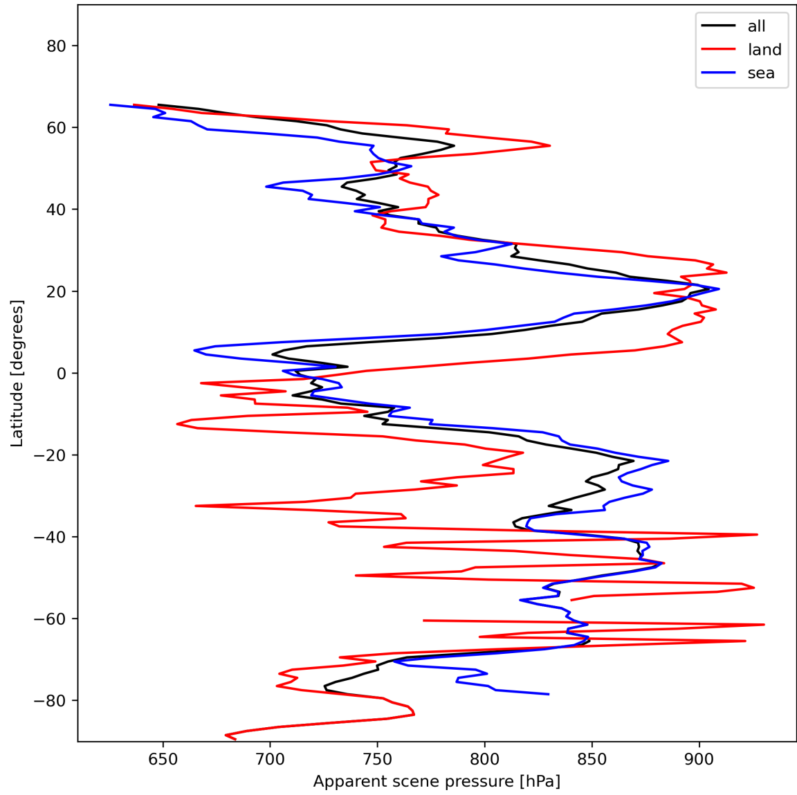
Figure 19: Zonal average of “Apparent scene pressure” for 2024-01-06 to 2024-01-08.
