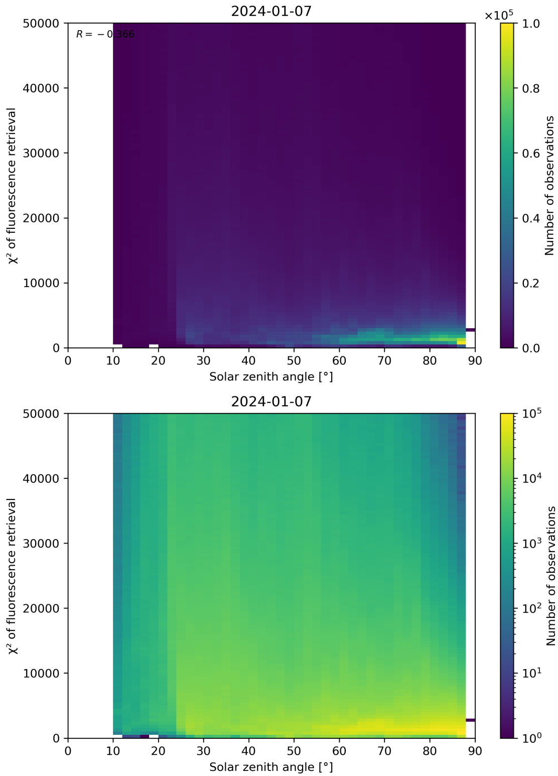
Figure 109: Scatter density plot of “Solar zenith angle” against “ \chi^2 of fluorescence retrieval” for 2024-01-06 to 2024-01-08.
