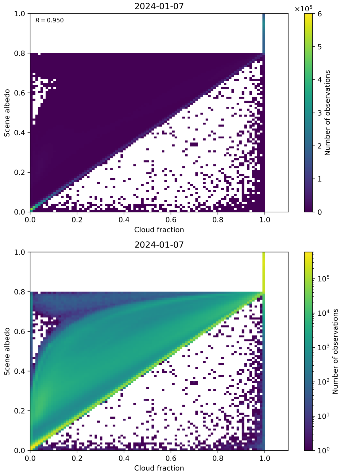
Figure 75: Scatter density plot of “Cloud fraction” against “Scene albedo” for 2024-01-06 to 2024-01-08.
