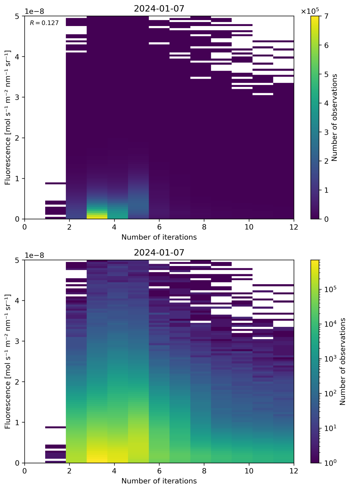
Figure 98: Scatter density plot of “Number of iterations” against “Fluorescence” for 2024-01-06 to 2024-01-08.
