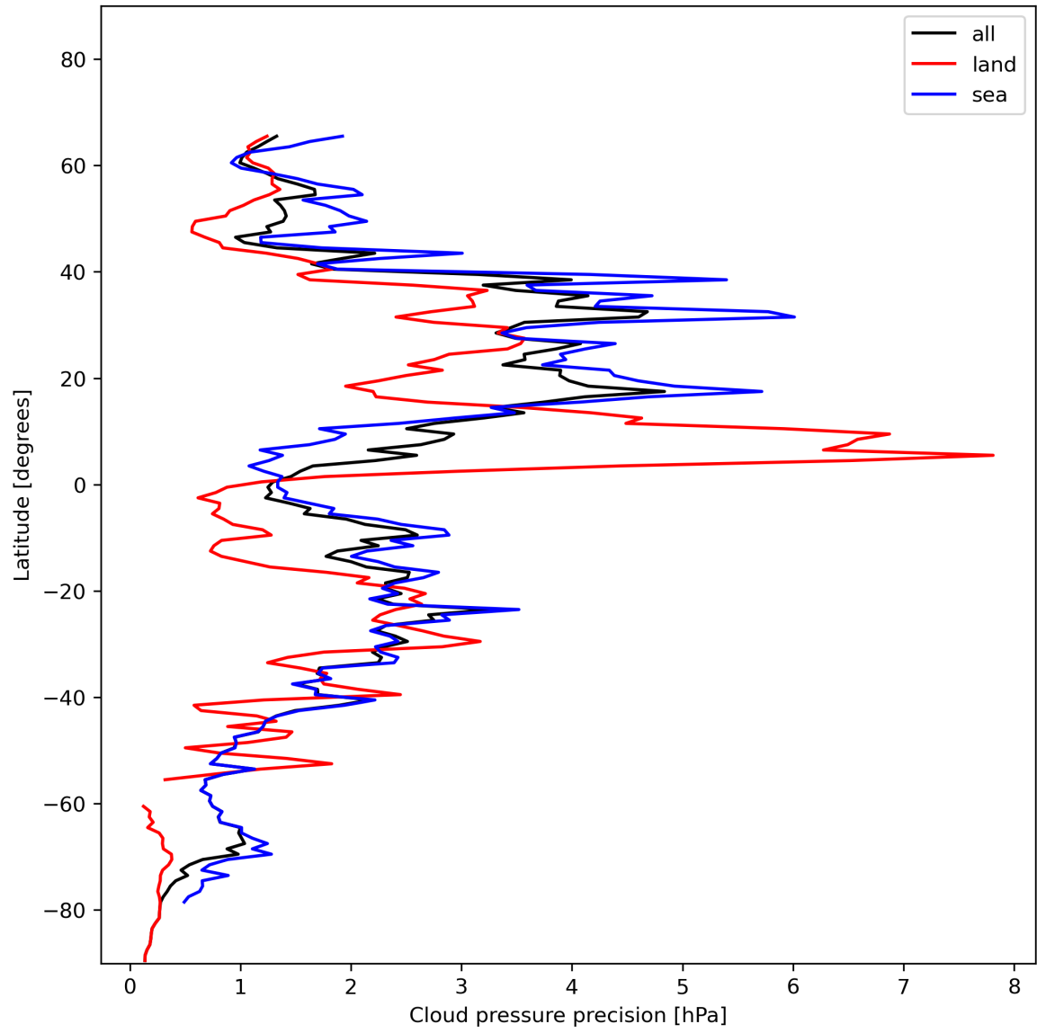
Figure 14: Zonal average of “Cloud pressure precision” for 2024-01-06 to 2024-01-08.
