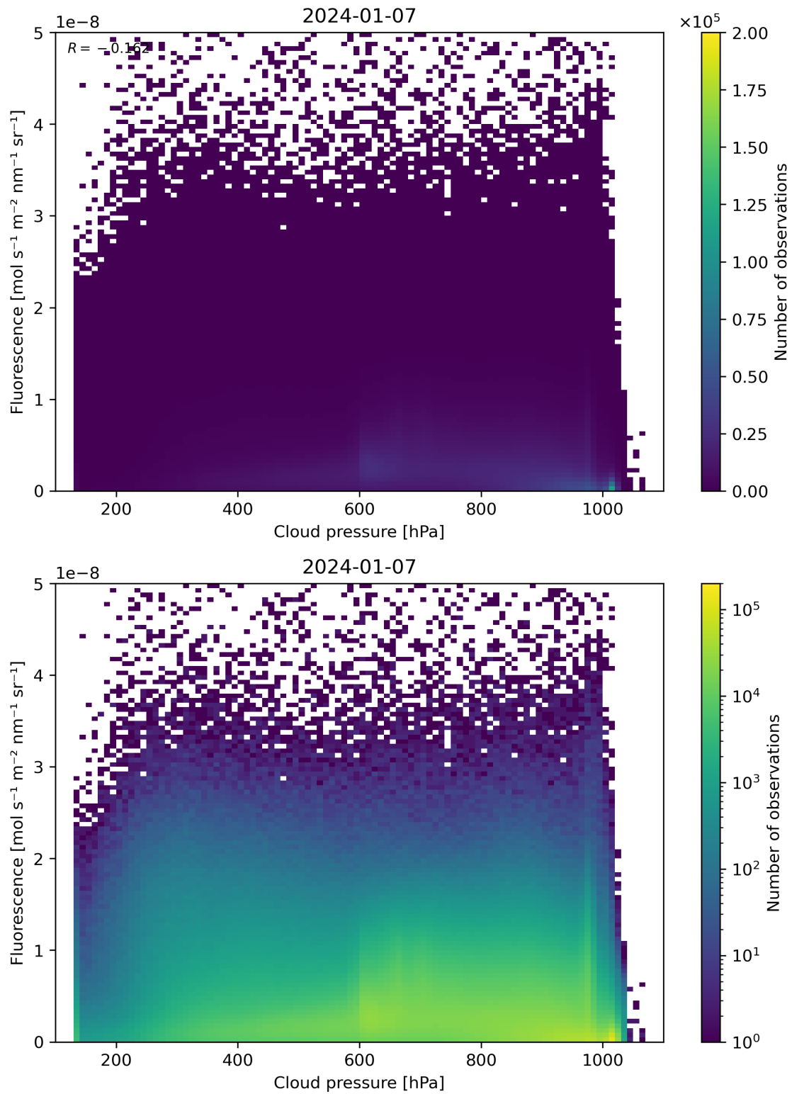
Figure 80: Scatter density plot of “Cloud pressure” against “Fluorescence” for 2024-01-06 to 2024-01-08.
