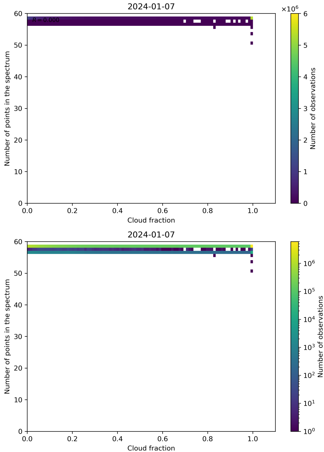
Figure 74: Scatter density plot of “Cloud fraction” against “Number of points in the spectrum” for 2024-01-06 to 2024-01-08.
