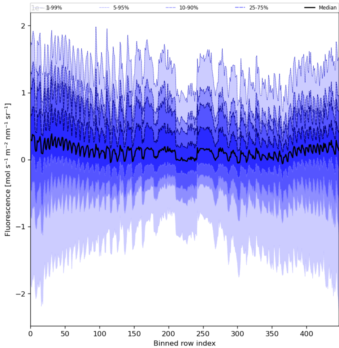
Figure 57: Along track statistics of “Fluorescence” for 2024-01-06 to 2024-01-08
