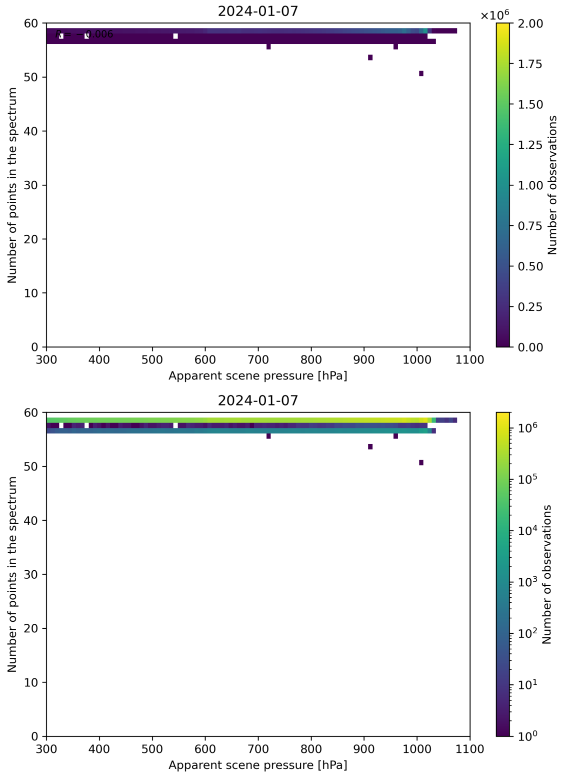
Figure 66: Scatter density plot of “Apparent scene pressure” against “Number of points in the spectrum” for 2024-01-06 to 2024-01-08.
