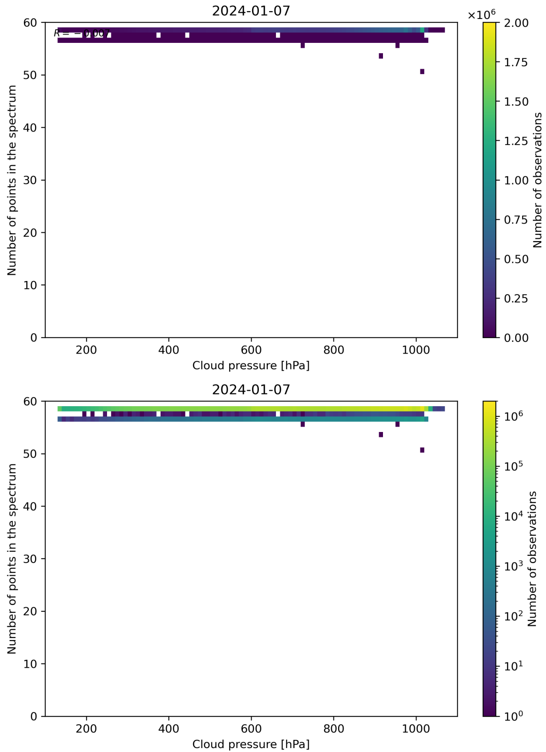
Figure 82: Scatter density plot of “Cloud pressure” against “Number of points in the spectrum” for 2024-01-06 to 2024-01-08.
