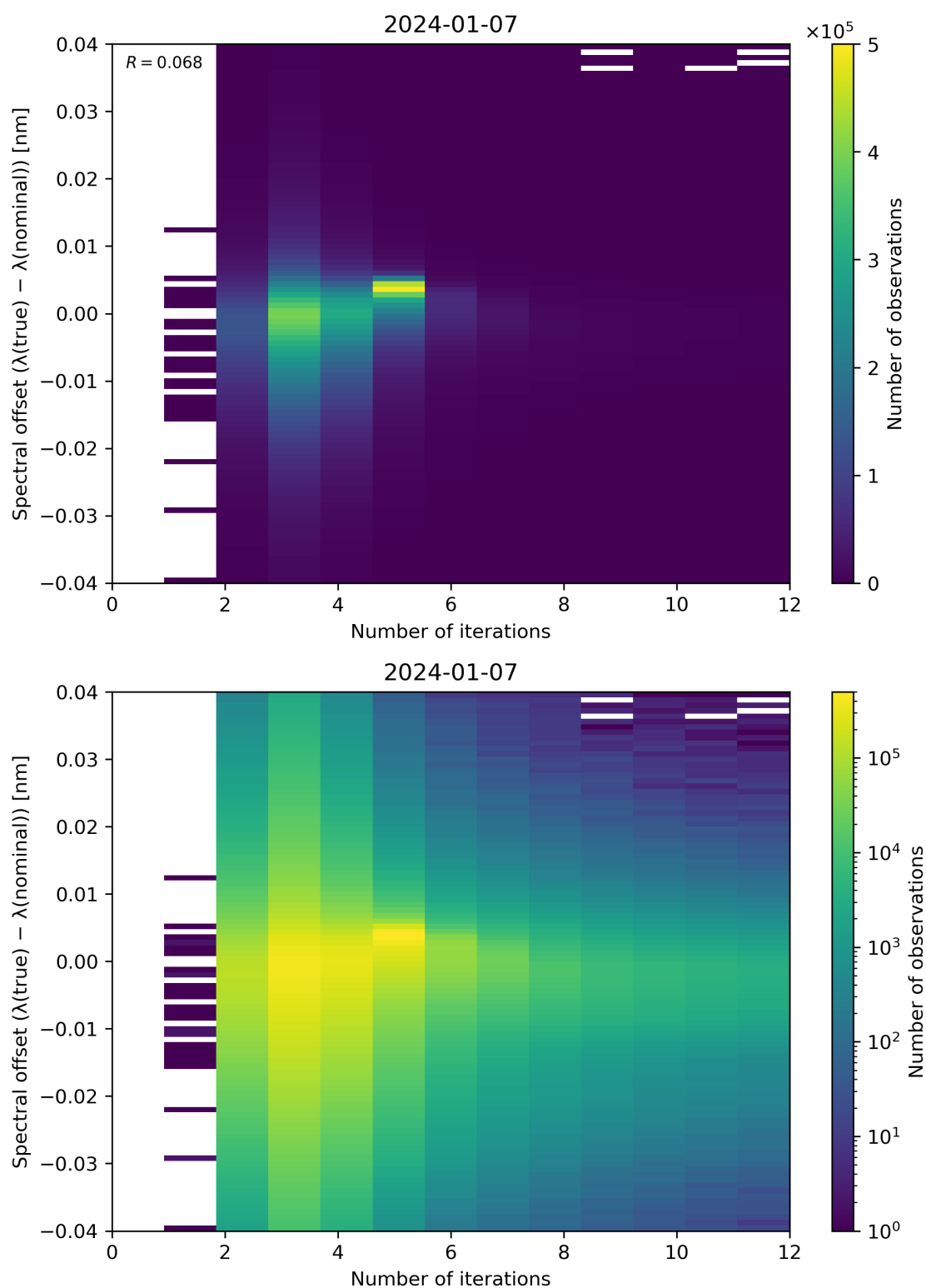
Figure 100: Scatter density plot of “Number of iterations” against “Spectral offset ( \lambda(\text{true}) - \lambda(\text{nominal}) )” for 2024-01-06 to 2024-01-08.
