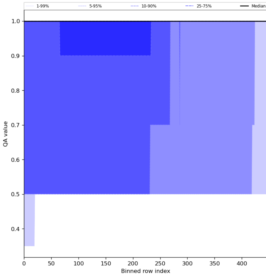
Figure 46: Along track statistics of “QA value” for 2024-01-06 to 2024-01-08
