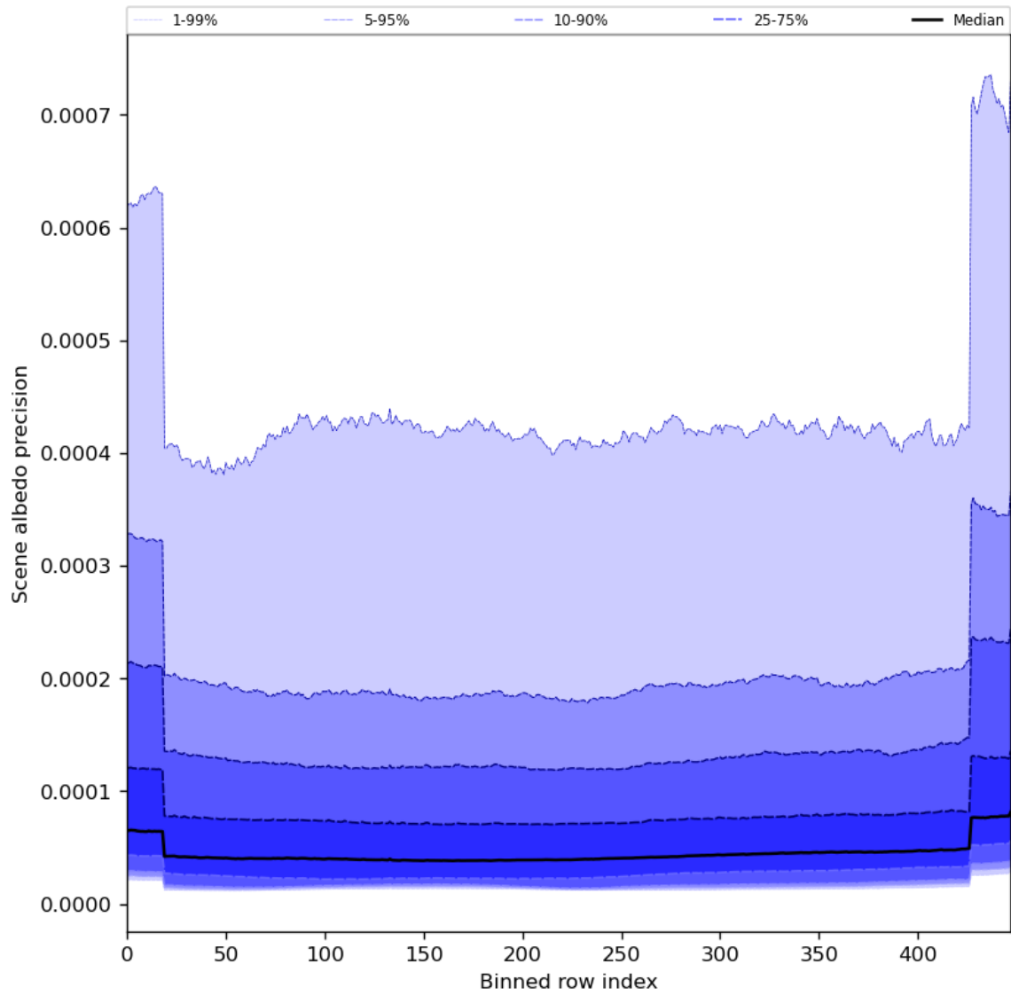
Figure 52: Along track statistics of “Scene albedo precision” for 2024-01-06 to 2024-01-08
