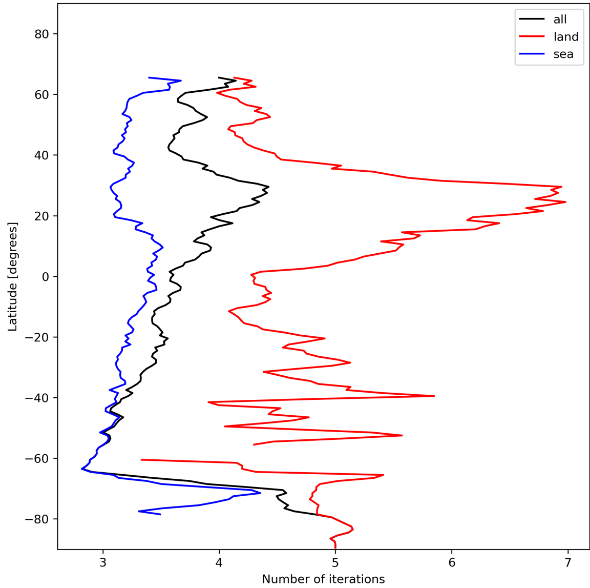
Figure 22: Zonal average of “Number of iterations” for 2024-01-06 to 2024-01-08.
