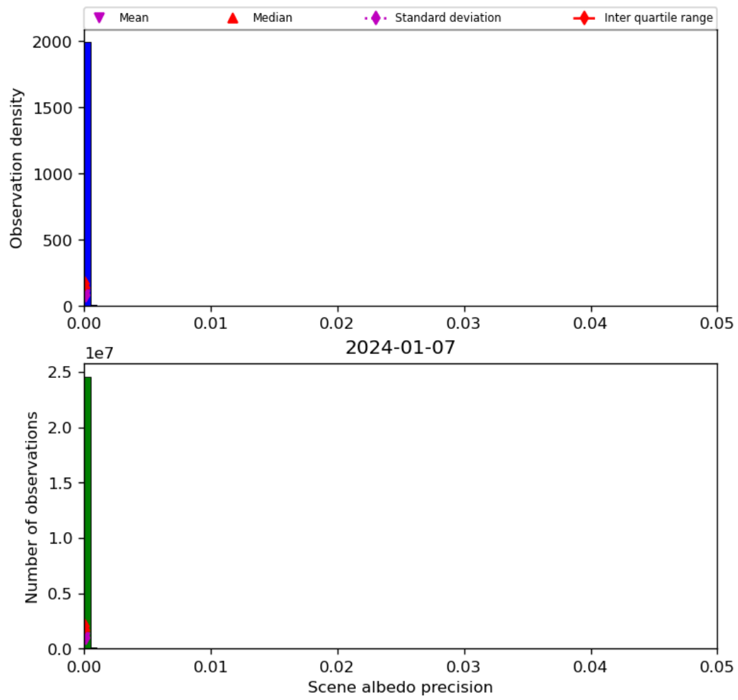
Figure 35: Histogram of “Scene albedo precision” for 2024-01-06 to 2024-01-08
