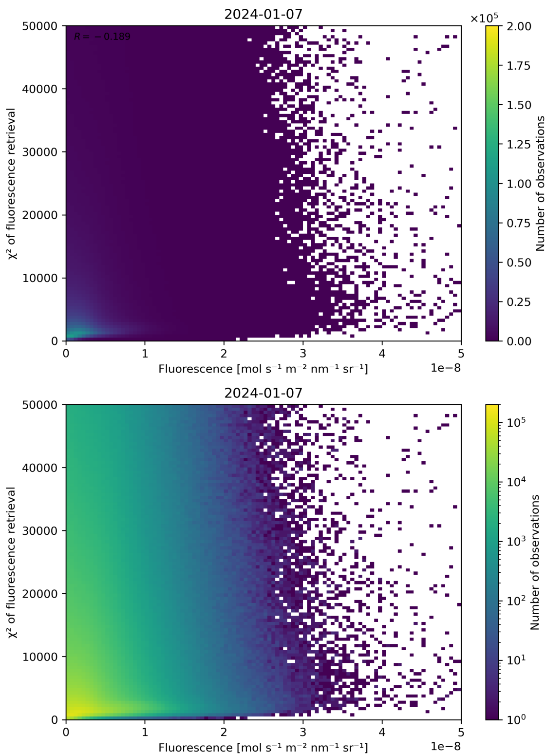
Figure 85: Scatter density plot of “Fluorescence” against “ \chi^2 of fluorescence retrieval” for 2024-01-06 to 2024-01-08.
