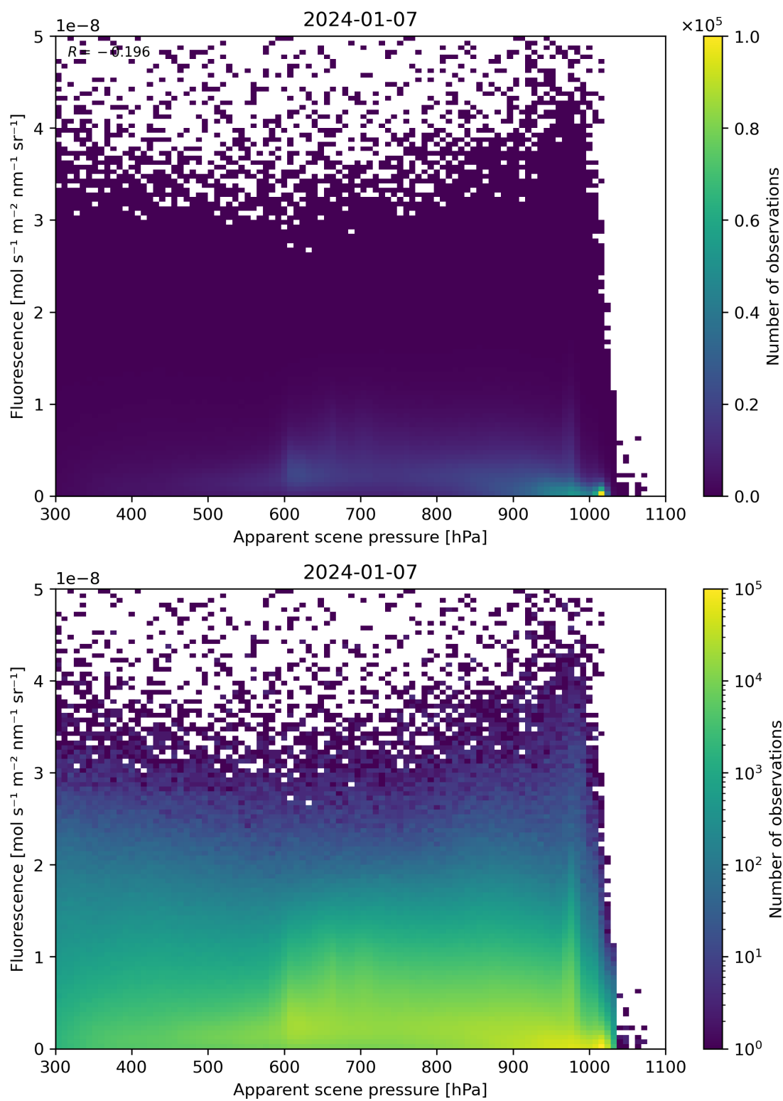
Figure 64: Scatter density plot of “Apparent scene pressure” against “Fluorescence” for 2024-01-06 to 2024-01-08.
