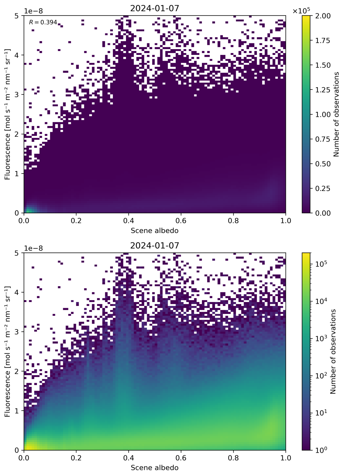
Figure 104: Scatter density plot of “Scene albedo” against “Fluorescence” for 2024-01-06 to 2024-01-08.
