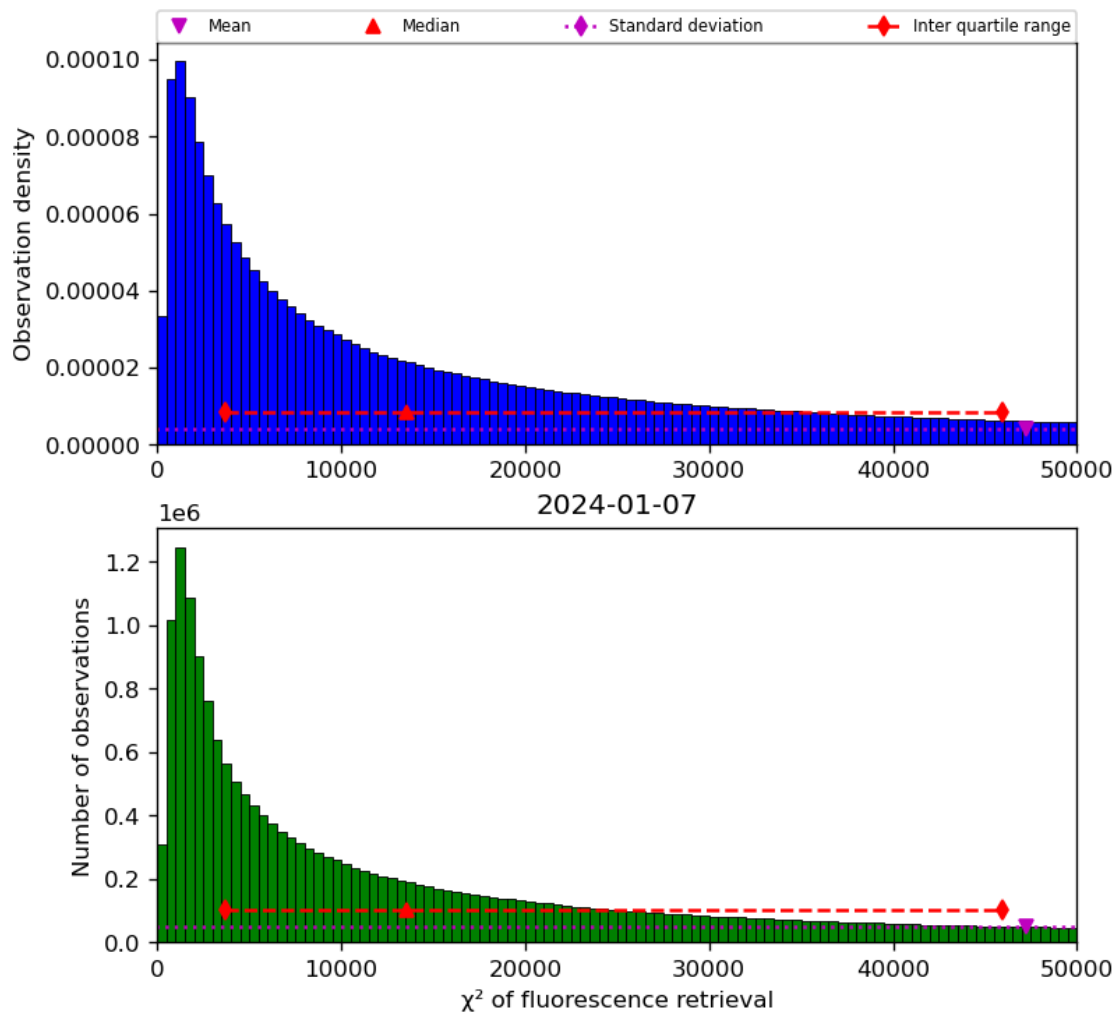
Figure 42: Histogram of “ \chi^2 of fluorescence retrieval” for 2024-01-06 to 2024-01-08
