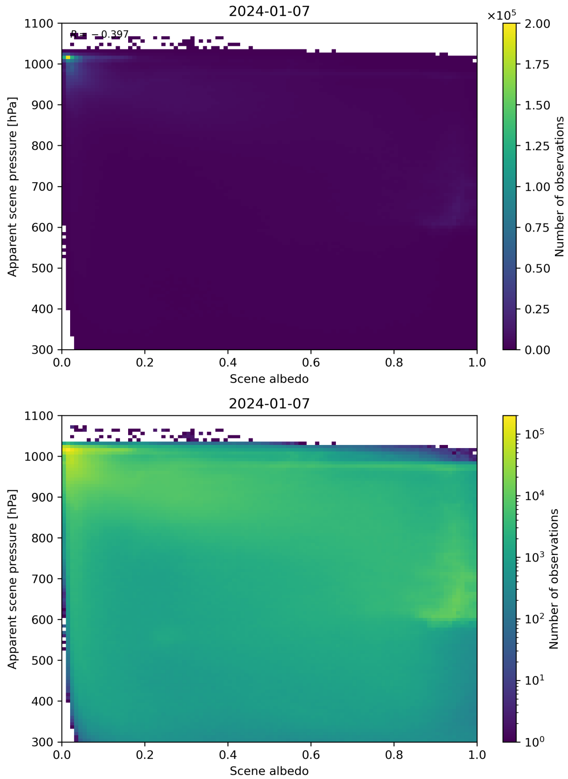
Figure 102: Scatter density plot of “Scene albedo” against “Apparent scene pressure” for 2024-01-06 to 2024-01-08.
