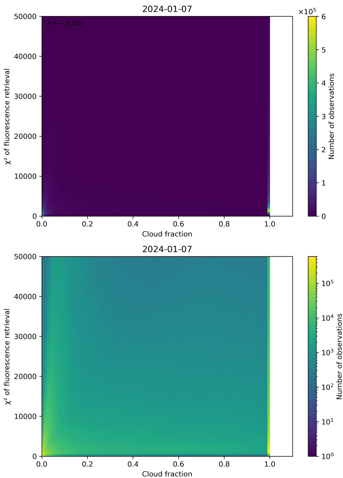
Figure 71: Scatter density plot of “Cloud fraction” against “ \chi^2 of fluorescence retrieval” for 2024-01-06 to 2024-01-08.
