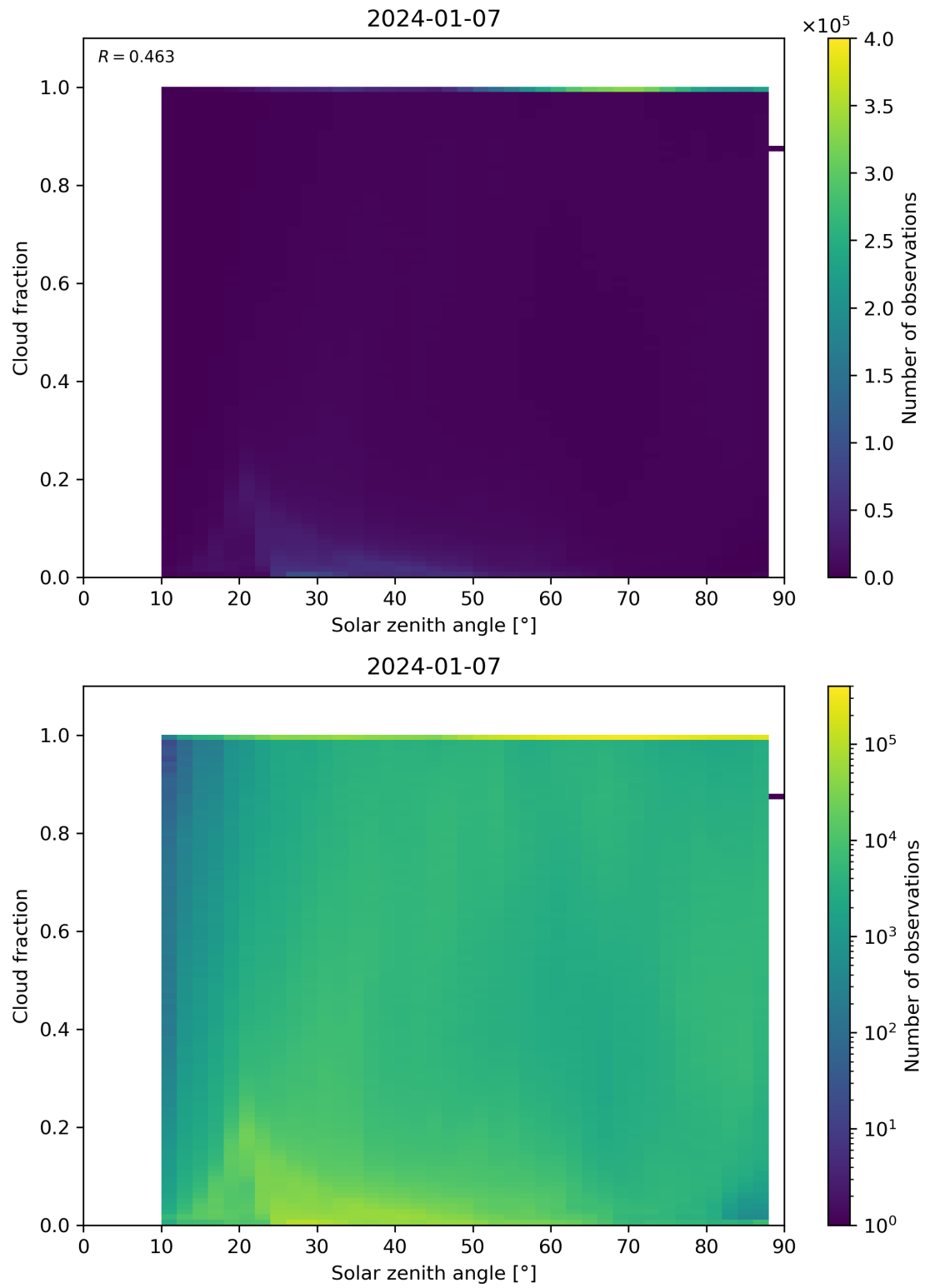
Figure 110: Scatter density plot of “Solar zenith angle” against “Cloud fraction” for 2024-01-06 to 2024-01-08.
