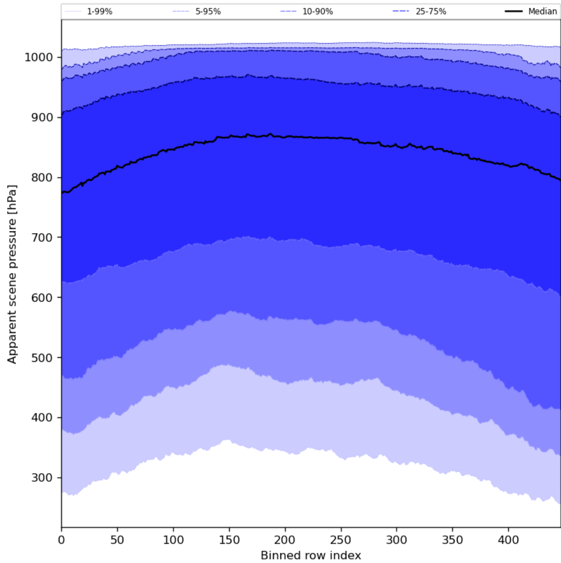
Figure 53: Along track statistics of “Apparent scene pressure” for 2024-01-06 to 2024-01-08
