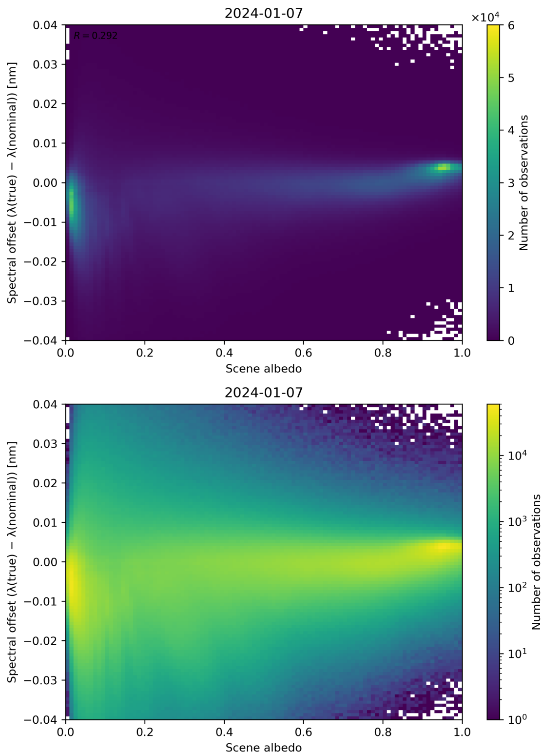
Figure 107: Scatter density plot of “Scene albedo” against “Spectral offset ( \lambda(\text{true}) - \lambda(\text{nominal}) )” for 2024-01-06 to 2024-01-08.
