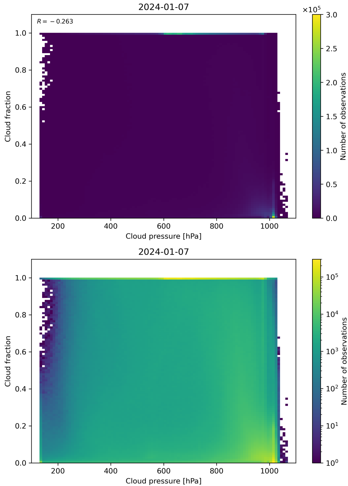
Figure 79: Scatter density plot of “Cloud pressure” against “Cloud fraction” for 2024-01-06 to 2024-01-08.
