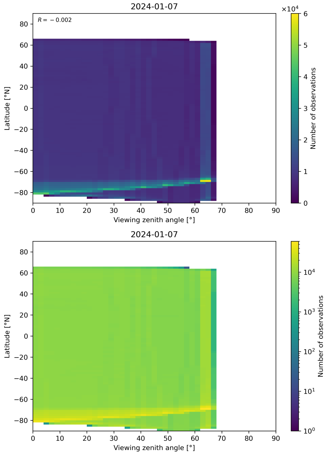
Figure 123: Scatter density plot of “Viewing zenith angle” against “Latitude” for 2024-01-06 to 2024-01-08.
