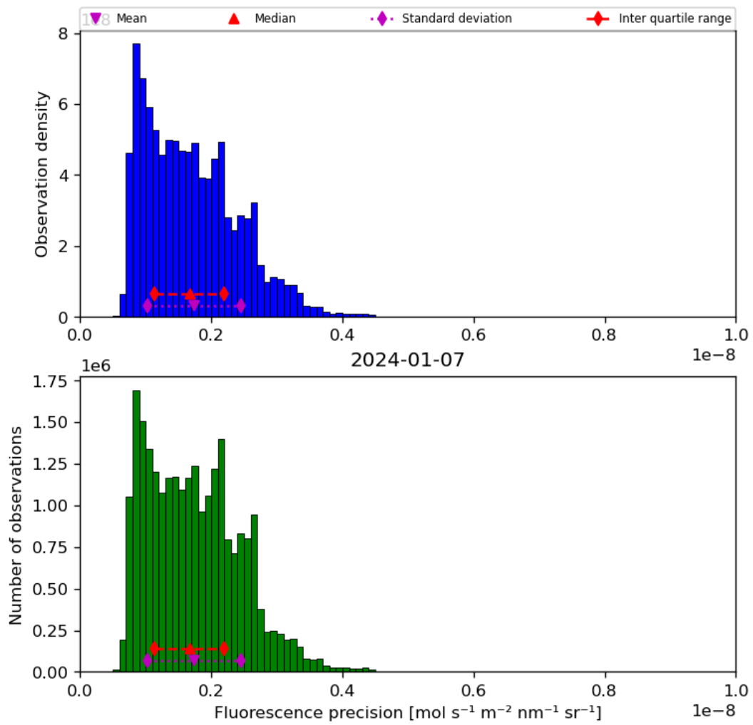
Figure 41: Histogram of “Fluorescence precision” for 2024-01-06 to 2024-01-08
