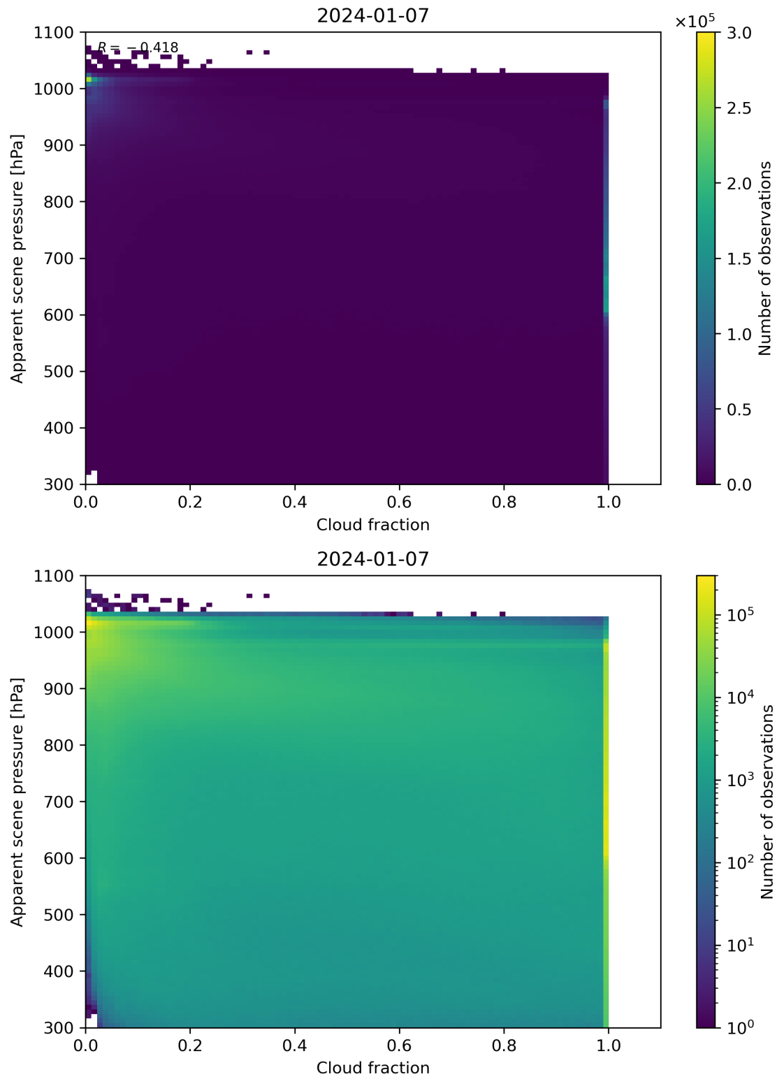
Figure 70: Scatter density plot of “Cloud fraction” against “Apparent scene pressure” for 2024-01-06 to 2024-01-08.
