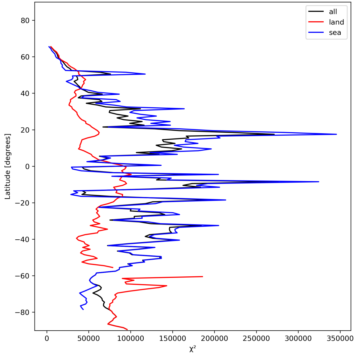
Figure 21: Zonal average of “ \chi^2 ” for 2024-01-06 to 2024-01-08.
