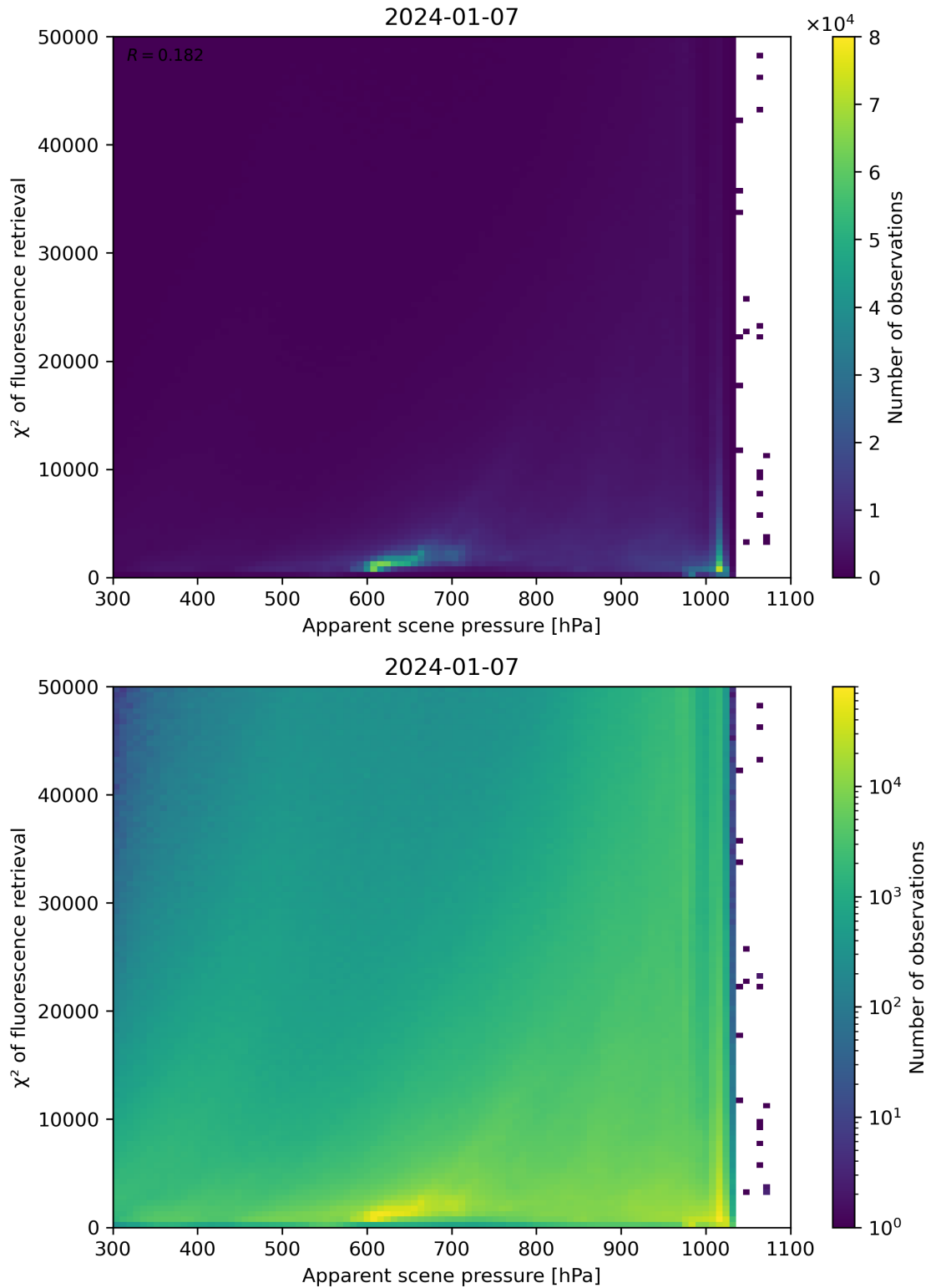
Figure 63: Scatter density plot of “Apparent scene pressure” against “ \chi^2 of fluorescence retrieval” for 2024-01-06 to 2024-01-08.
