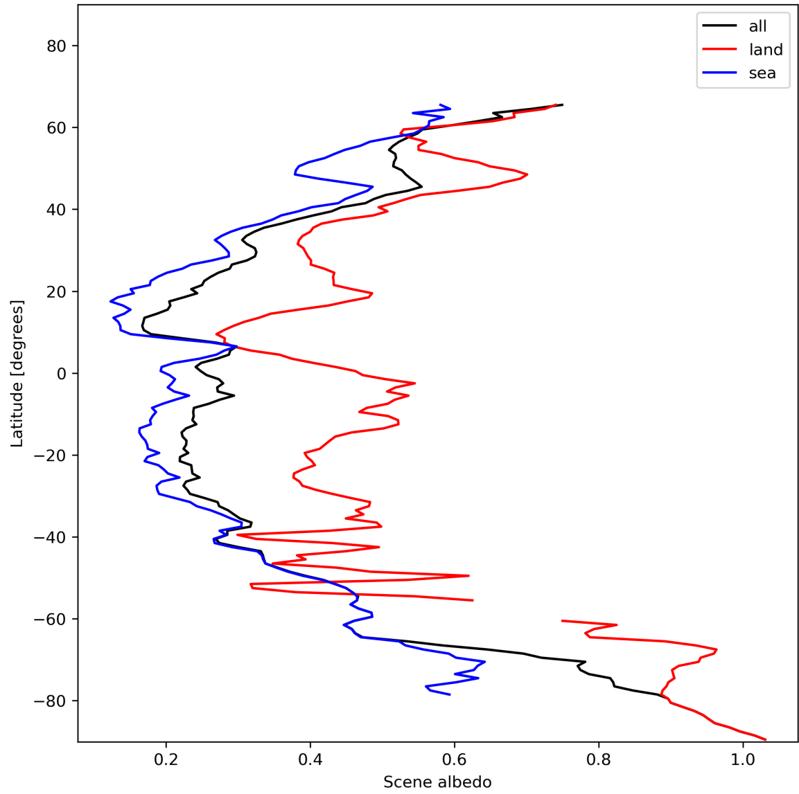
Figure 17: Zonal average of "Scene albedo" for 2024-01-06 to 2024-01-08.
