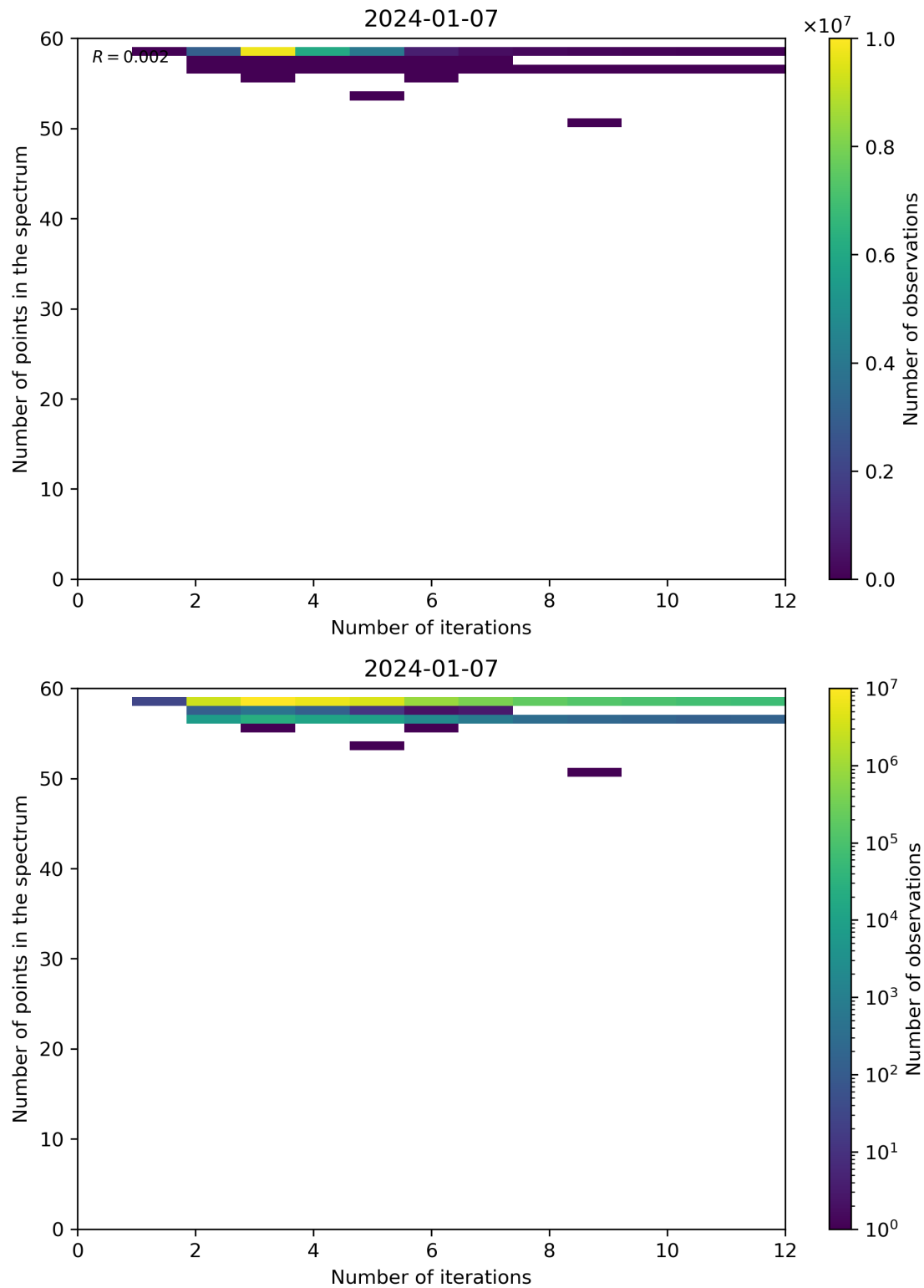
Figure 99: Scatter density plot of “Number of iterations” against “Number of points in the spectrum” for 2024-01-06 to 2024-01-08.
