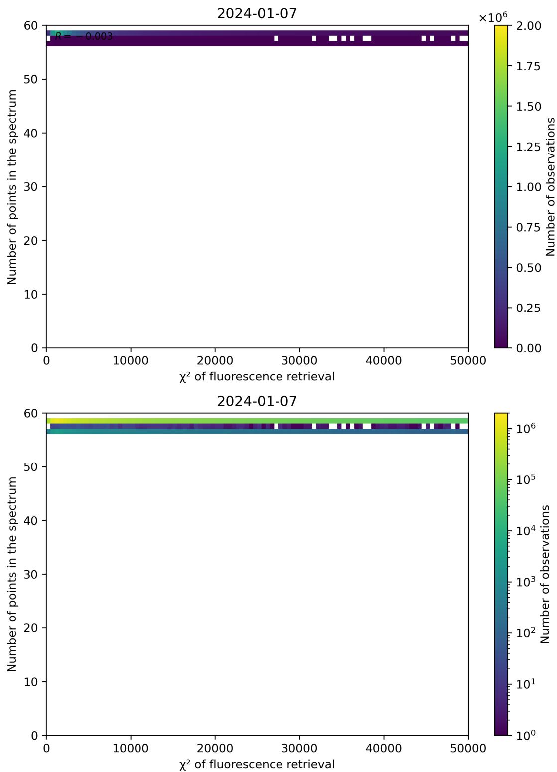
Figure 68: Scatter density plot of " \chi^2 of fluorescence retrieval" against "Number of points in the spectrum" for 2024-01-06 to 2024-01-08.
