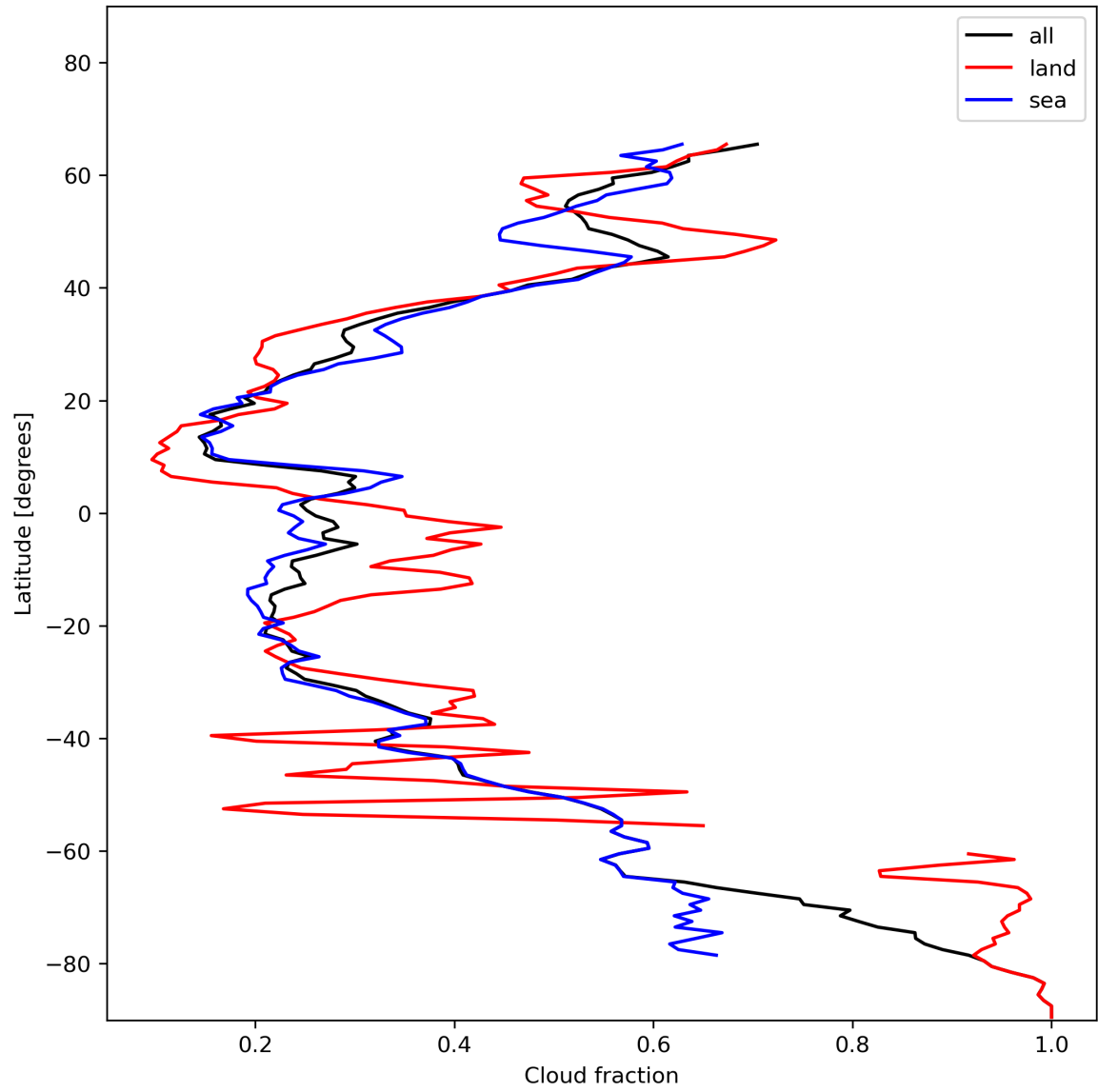
Figure 15: Zonal average of “Cloud fraction” for 2024-01-06 to 2024-01-08.
