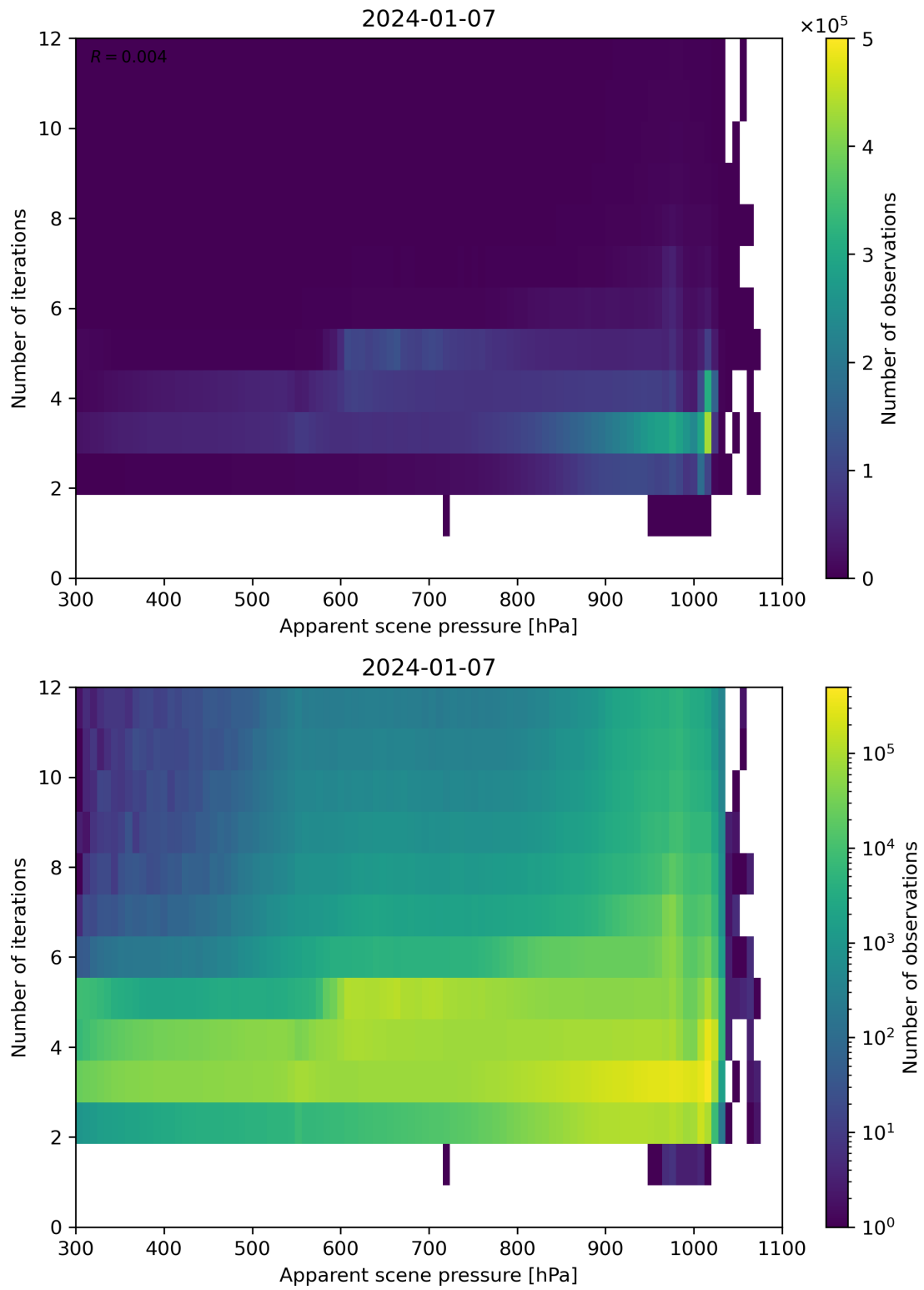
Figure 65: Scatter density plot of “Apparent scene pressure” against “Number of iterations” for 2024-01-06 to 2024-01-08.
