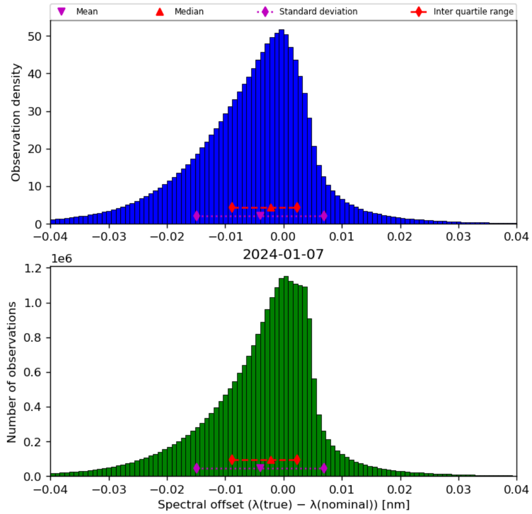
Figure 45: Histogram of “Spectral offset ( \lambda(\text{true}) - \lambda(\text{nominal}) )” for 2024-01-06 to 2024-01-08
