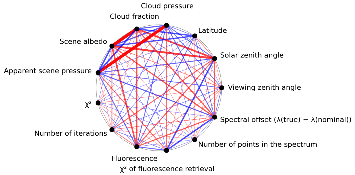
Figure 1: Map of correlation graph for 2024-01-06 to 2024-01-08.
