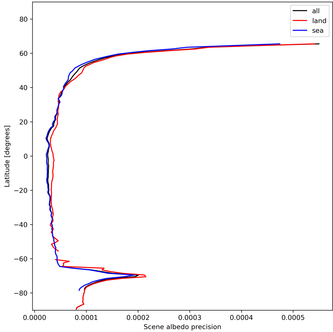
Figure 18: Zonal average of “Scene albedo precision” for 2024-01-06 to 2024-01-08.
