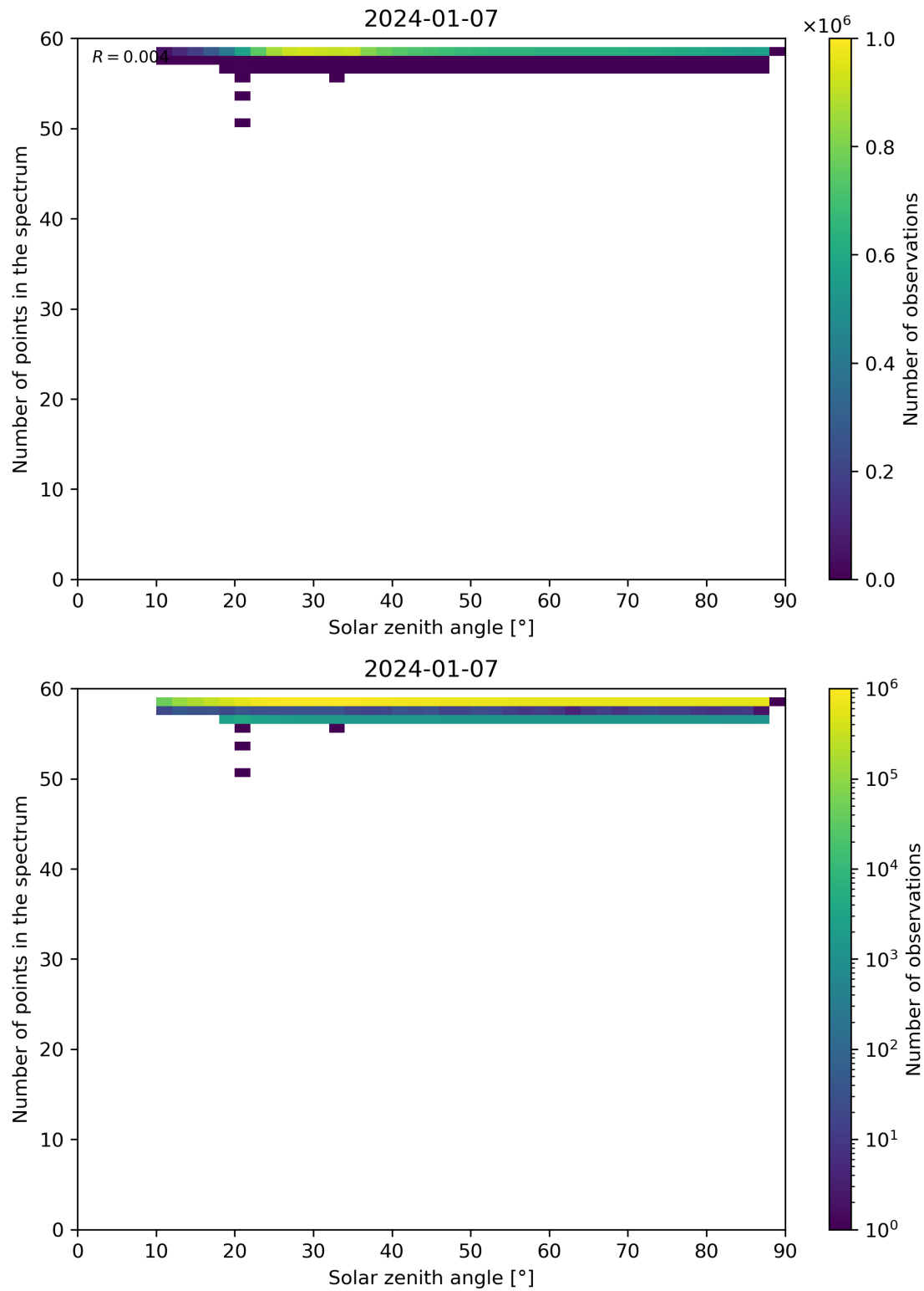
Figure 115: Scatter density plot of “Solar zenith angle” against “Number of points in the spectrum” for 2024-01-06 to 2024-01-08.
