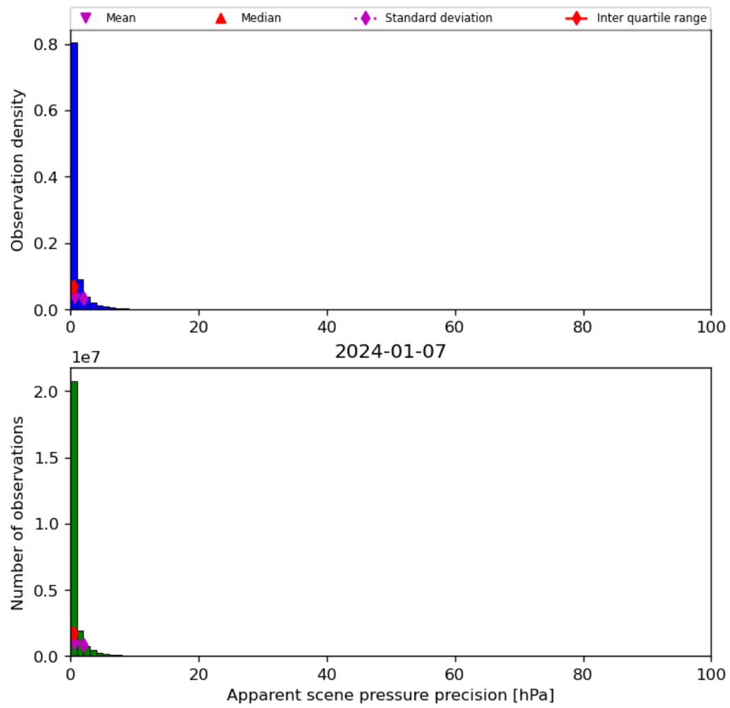
Figure 37: Histogram of “Apparent scene pressure precision” for 2024-01-06 to 2024-01-08
