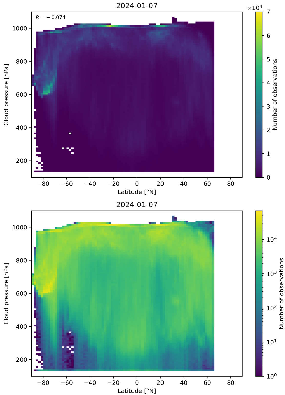
Figure 91: Scatter density plot of “Latitude” against “Cloud pressure” for 2024-01-06 to 2024-01-08.
