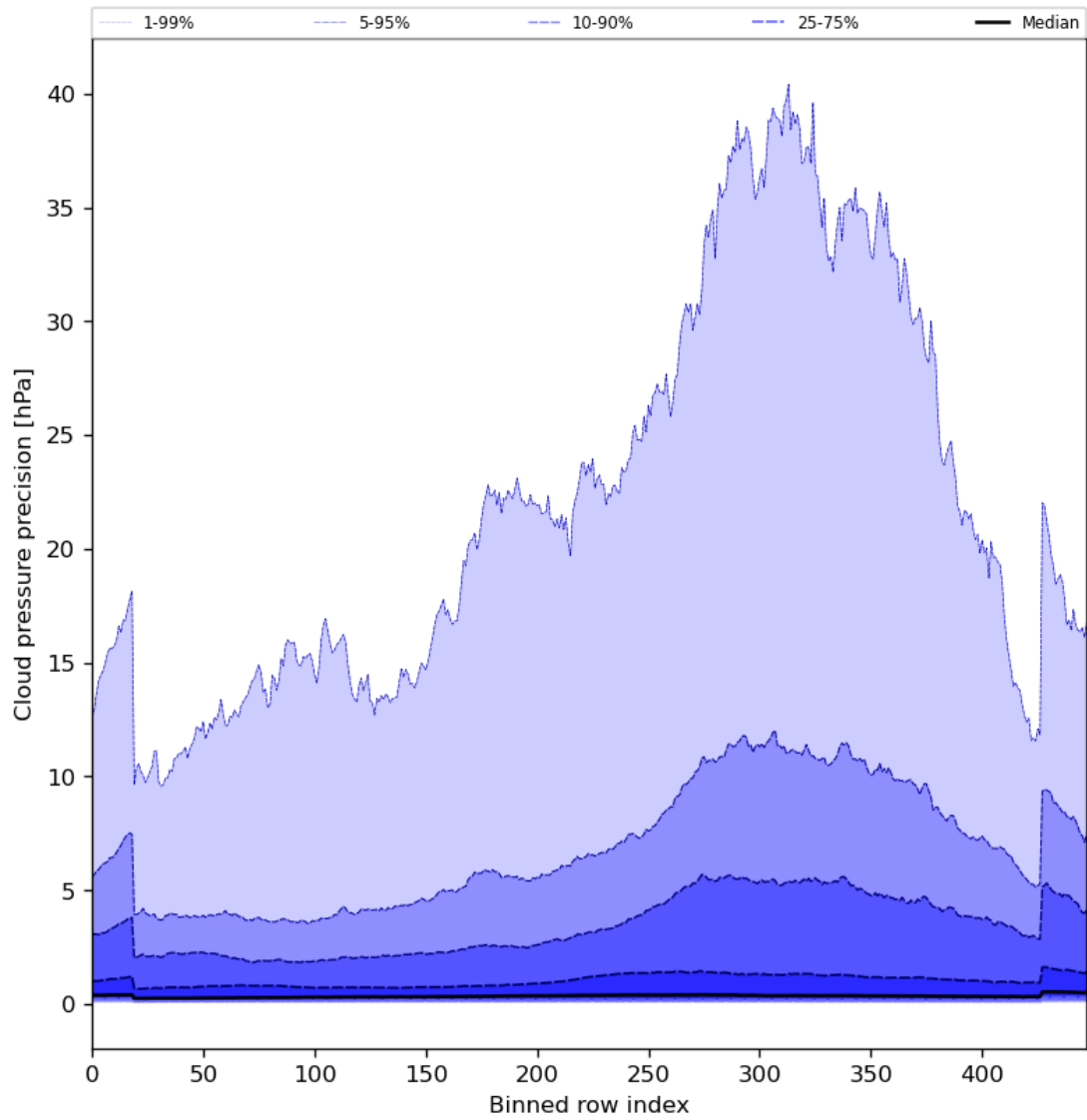
Figure 48: Along track statistics of “Cloud pressure precision” for 2024-01-06 to 2024-01-08
