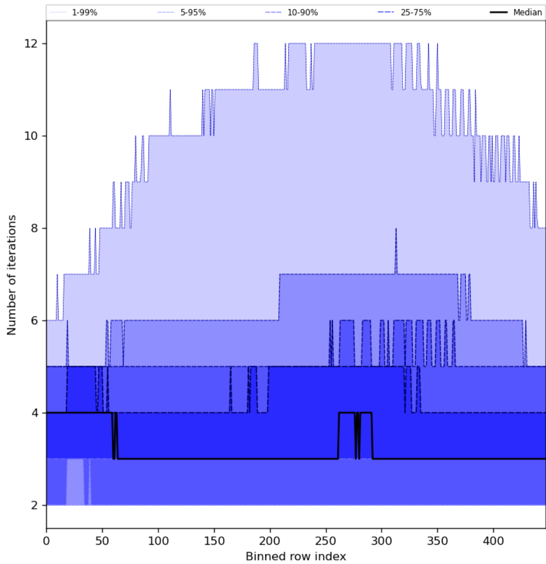
Figure 56: Along track statistics of “Number of iterations” for 2024-01-06 to 2024-01-08
