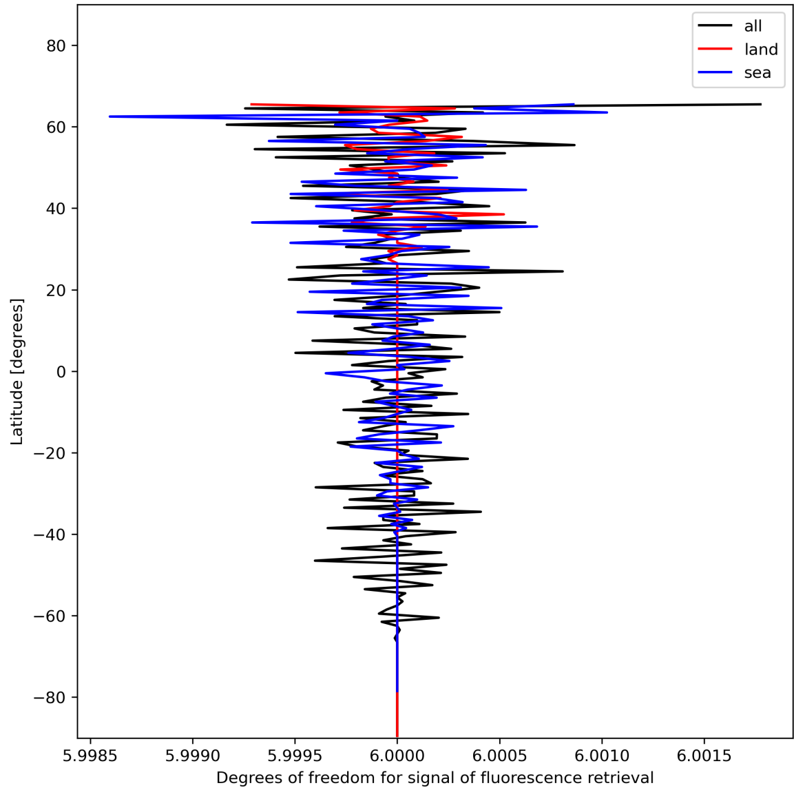
Figure 26: Zonal average of “Degrees of freedom for signal of fluorescence retrieval” for 2024-01-06 to 2024-01-08.
