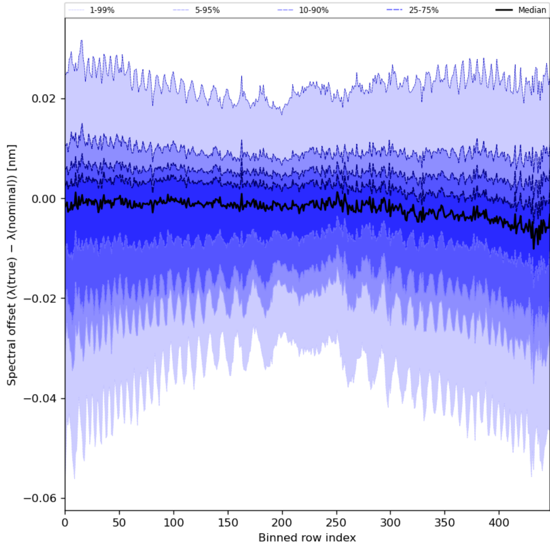
Figure 62: Along track statistics of “Spectral offset ( \lambda(\text{true}) - \lambda(\text{nominal}) )” for 2024-01-06 to 2024-01-08
