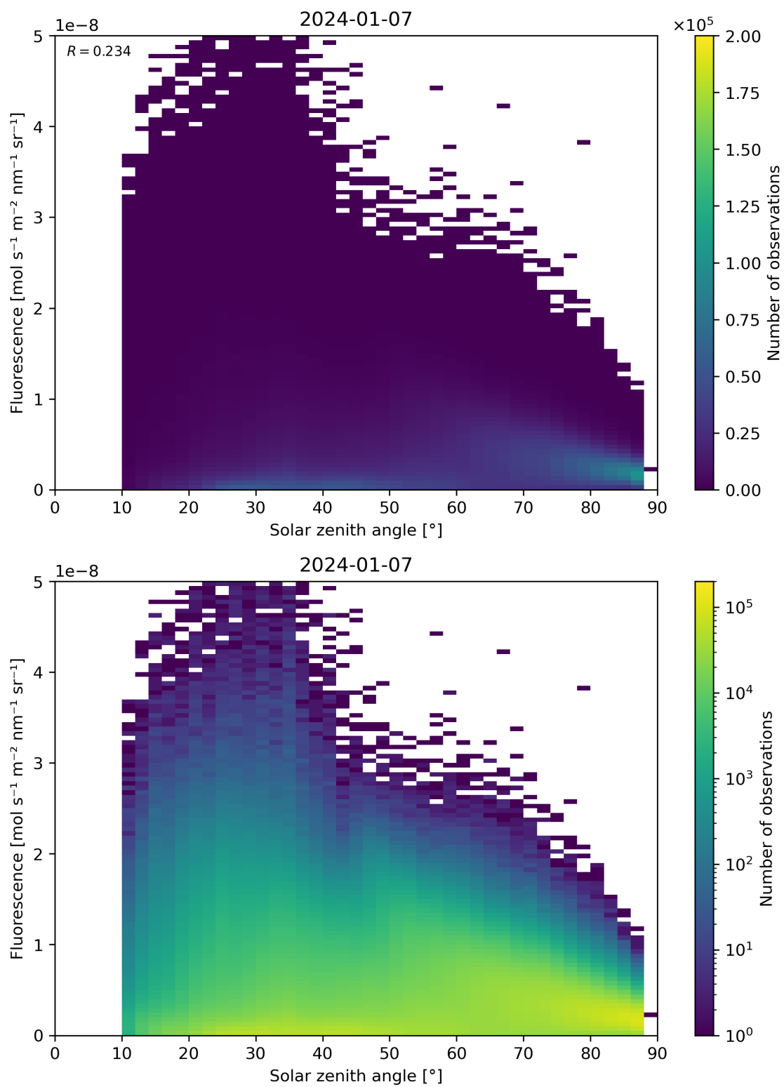
Figure 112: Scatter density plot of “Solar zenith angle” against “Fluorescence” for 2024-01-06 to 2024-01-08.
