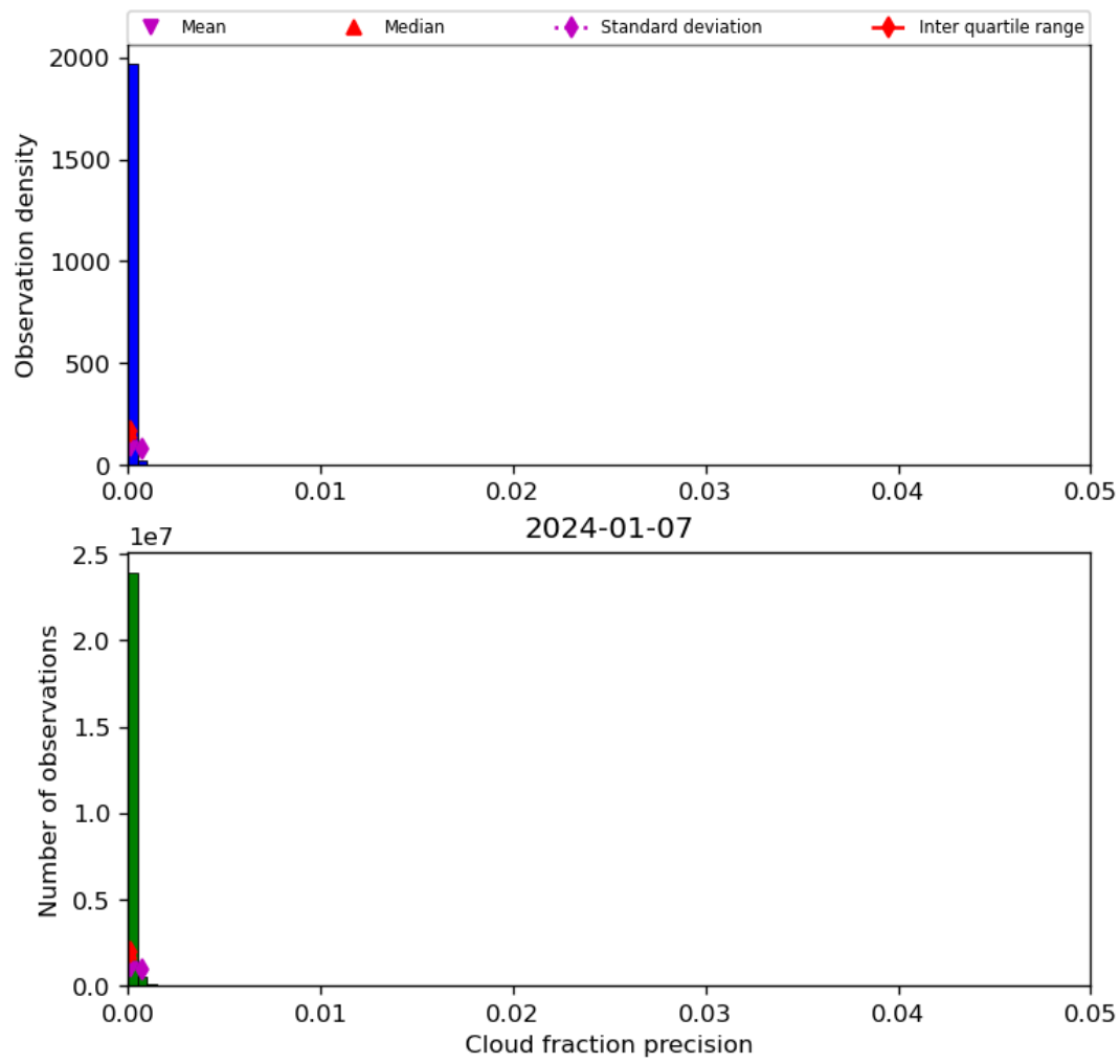
Figure 33: Histogram of “Cloud fraction precision” for 2024-01-06 to 2024-01-08
