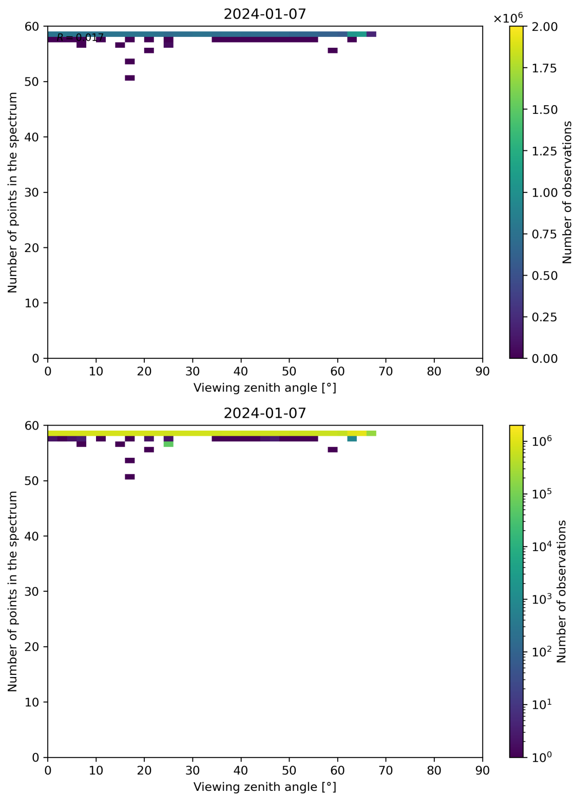
Figure 125: Scatter density plot of “Viewing zenith angle” against “Number of points in the spectrum” for 2024-01-06 to 2024-01-08.
