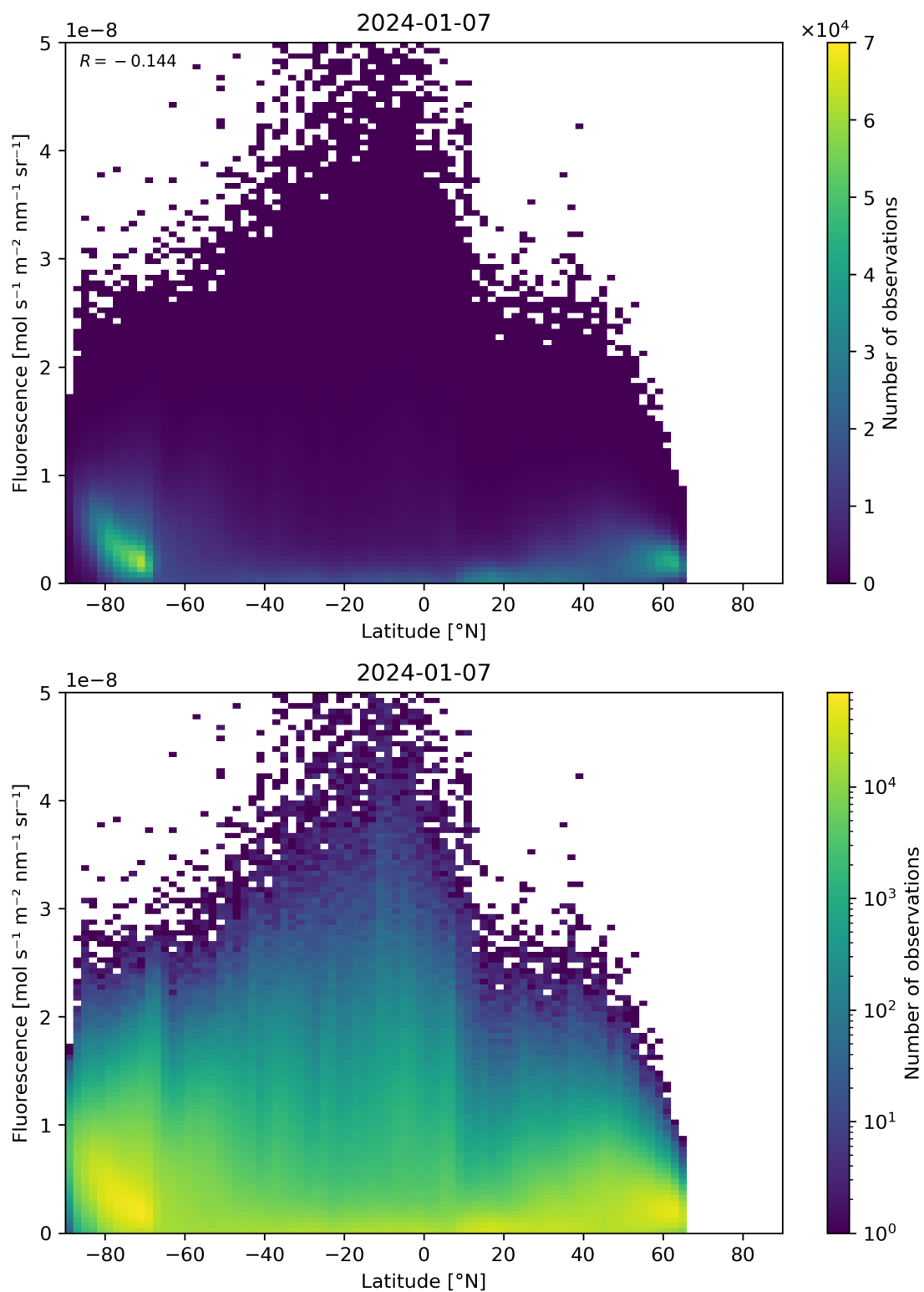
Figure 92: Scatter density plot of “Latitude” against “Fluorescence” for 2024-01-06 to 2024-01-08.
