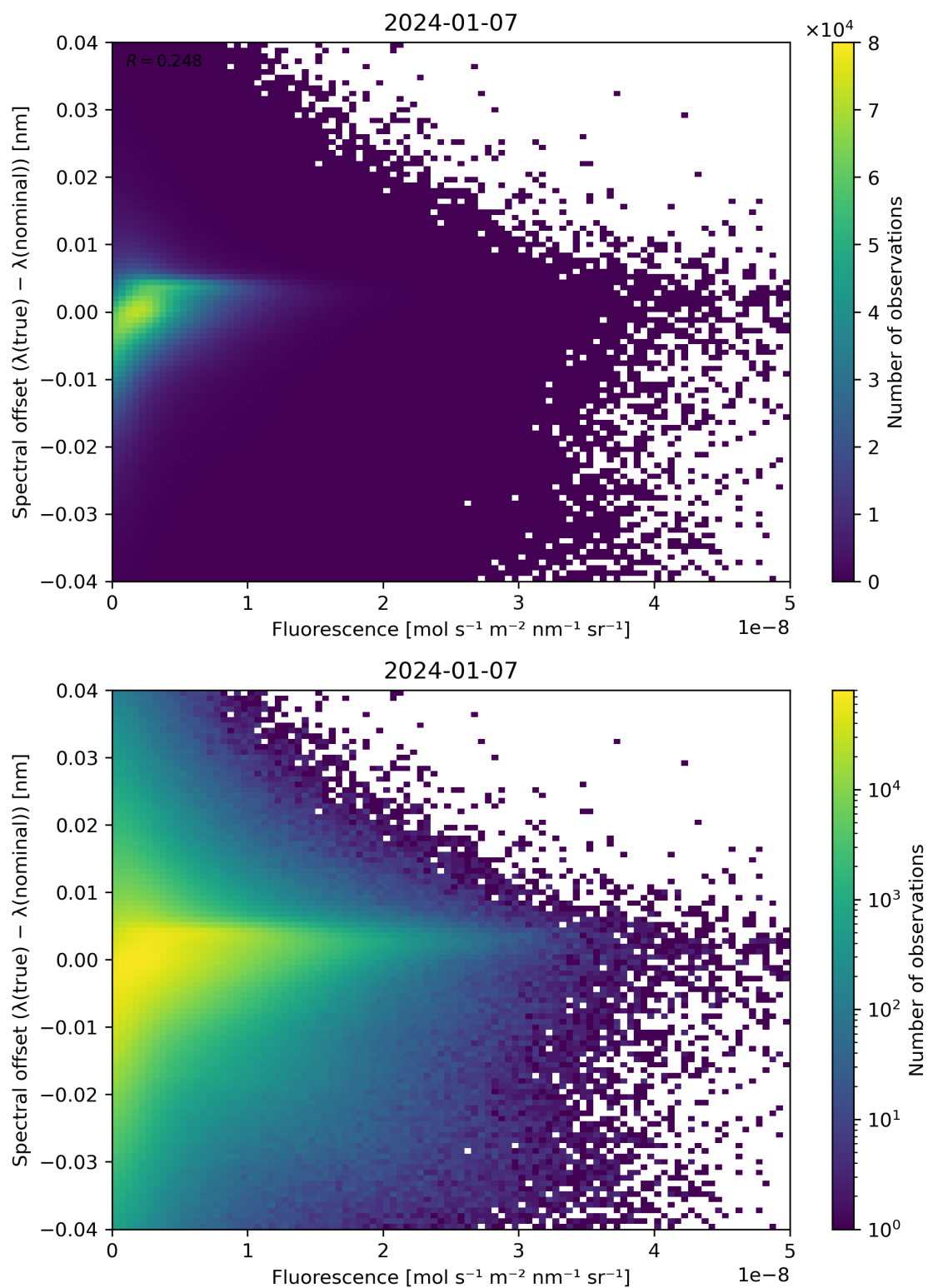
Figure 87: Scatter density plot of “Fluorescence” against “Spectral offset ( \lambda(\text{true}) - \lambda(\text{nominal}) )” for 2024-01-06 to 2024-01-08.
