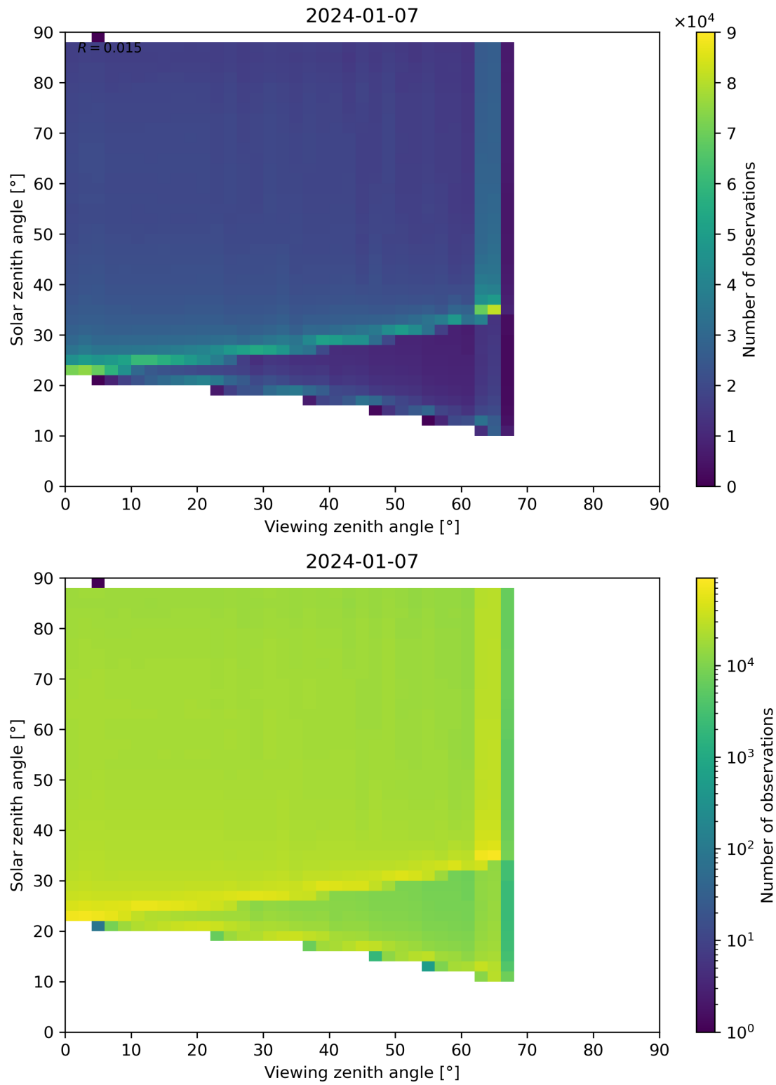
Figure 127: Scatter density plot of “Viewing zenith angle” against “Solar zenith angle” for 2024-01-06 to 2024-01-08.
