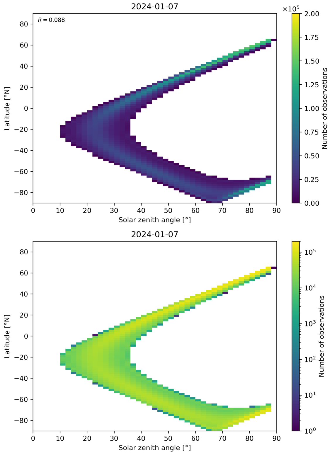
Figure 113: Scatter density plot of “Solar zenith angle” against “Latitude” for 2024-01-06 to 2024-01-08.
