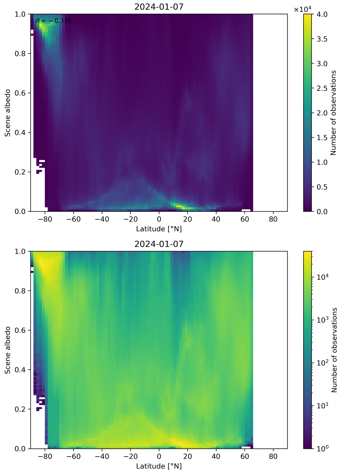
Figure 95: Scatter density plot of “Latitude” against “Scene albedo” for 2024-01-06 to 2024-01-08.
