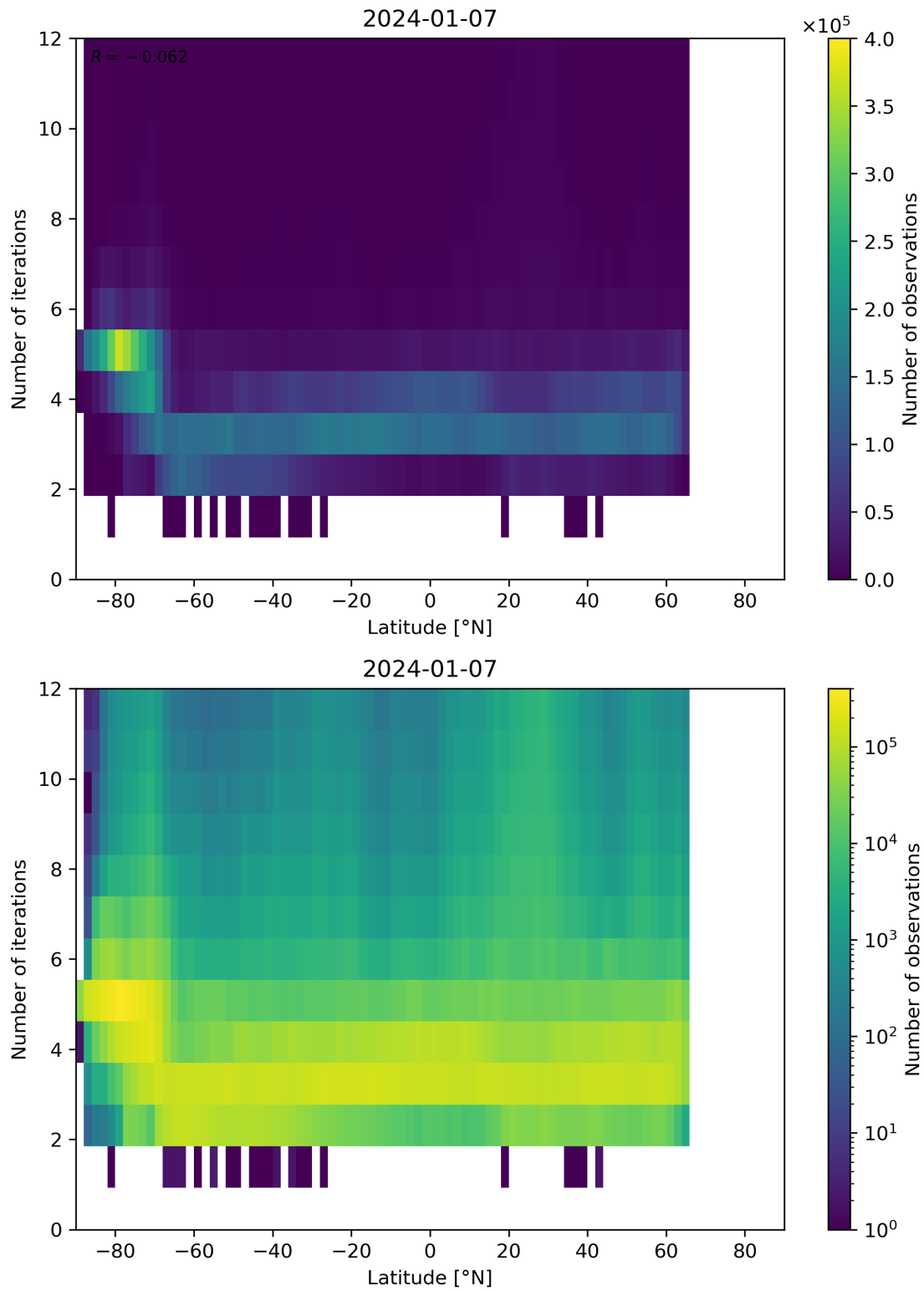
Figure 93: Scatter density plot of “Latitude” against “Number of iterations” for 2024-01-06 to 2024-01-08.
