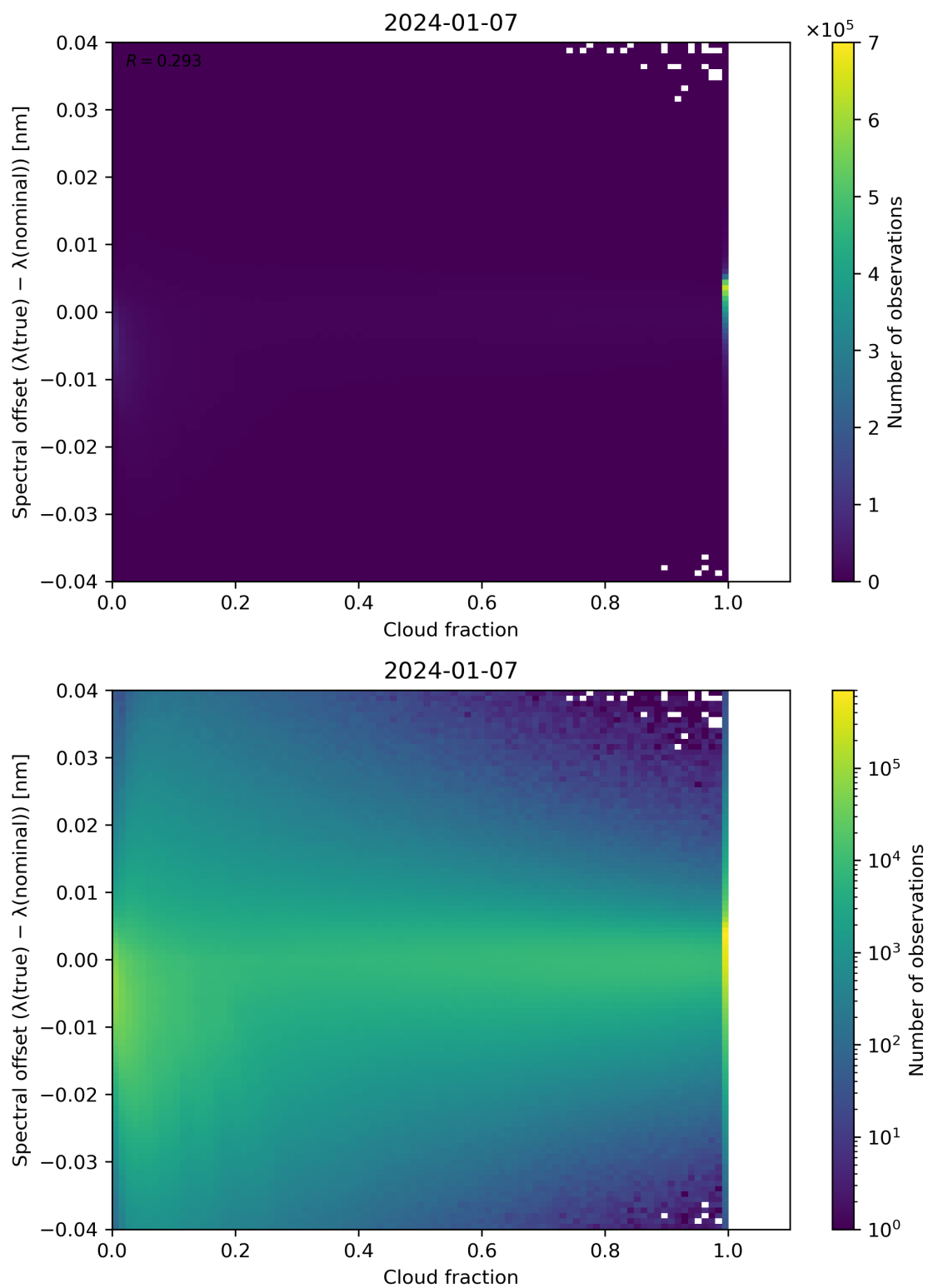
Figure 76: Scatter density plot of “Cloud fraction” against “Spectral offset ( \lambda(\text{true}) - \lambda(\text{nominal}) )” for 2024-01-06 to 2024-01-08.
