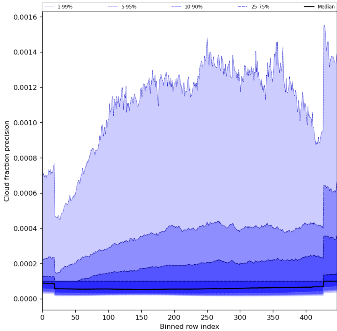
Figure 50: Along track statistics of “Cloud fraction precision” for 2024-01-06 to 2024-01-08
