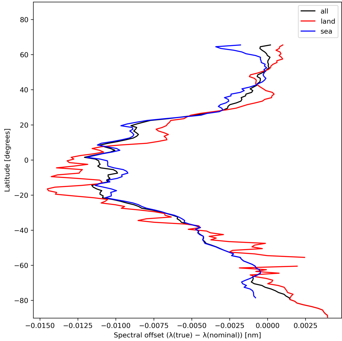
Figure 28: Zonal average of “Spectral offset ( \lambda(\text{true}) - \lambda(\text{nominal}) )” for 2024-01-06 to 2024-01-08.
