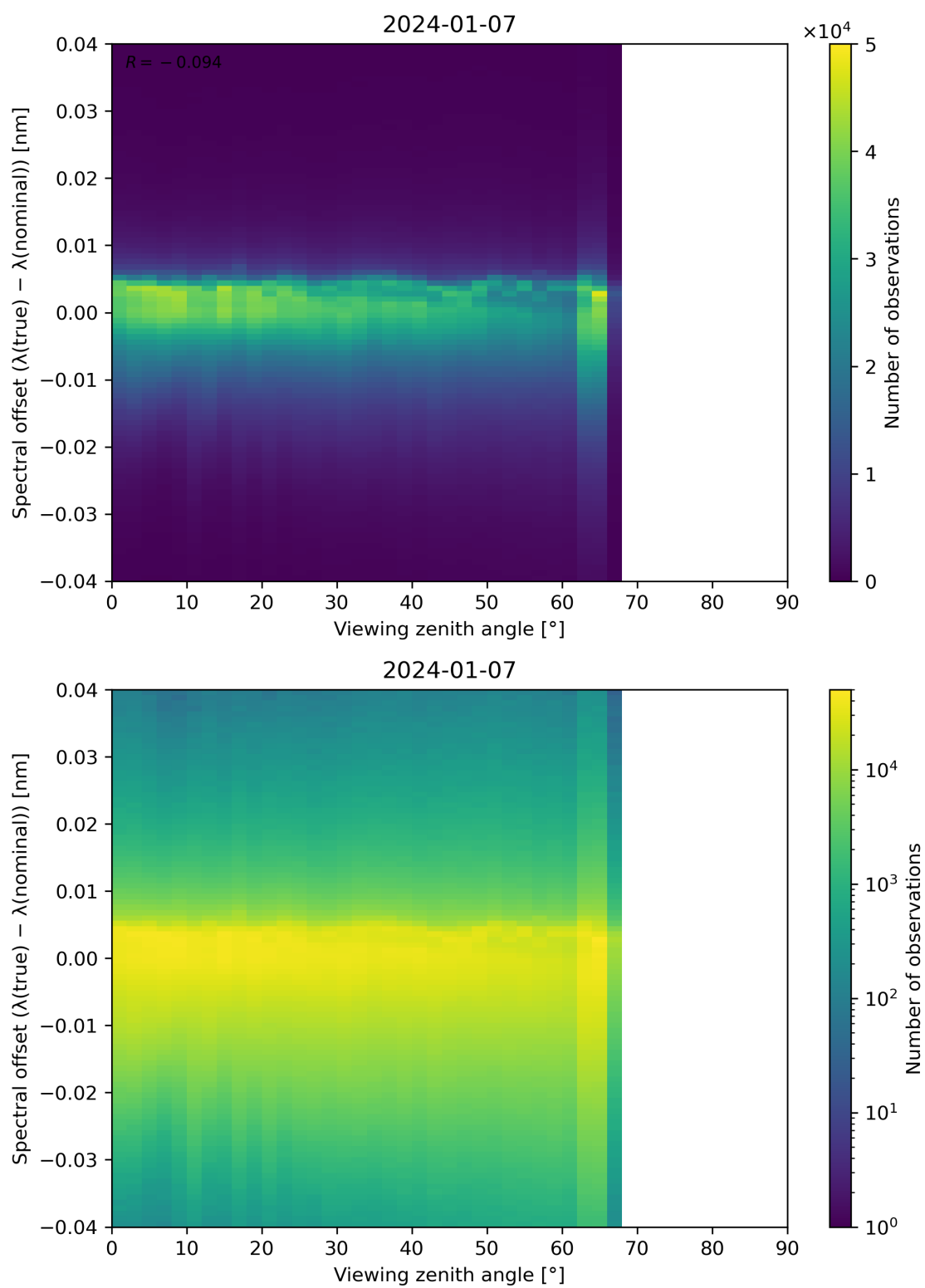
Figure 128: Scatter density plot of “Viewing zenith angle” against “Spectral offset ( \lambda(\text{true}) - \lambda(\text{nominal}) )” for 2024-01-06 to 2024-01-08.
