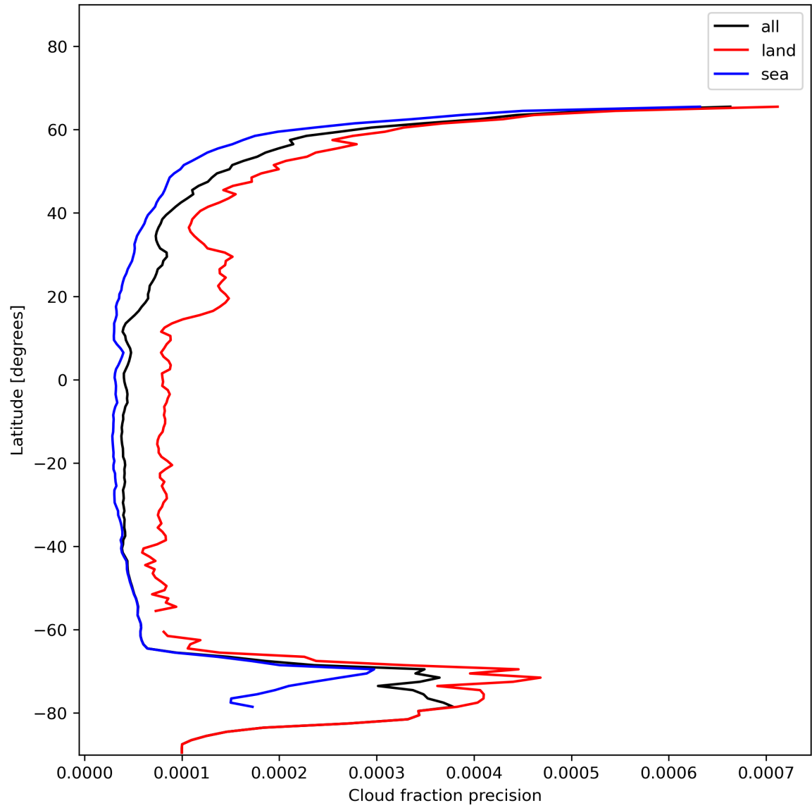
Figure 16: Zonal average of “Cloud fraction precision” for 2024-01-06 to 2024-01-08.
