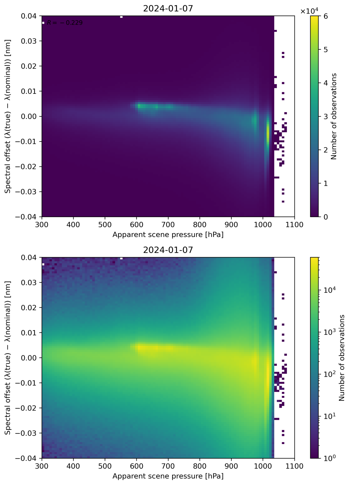
Figure 67: Scatter density plot of “Apparent scene pressure” against “Spectral offset ( \lambda(\text{true}) - \lambda(\text{nominal}) )” for 2024-01-06 to 2024-01-08.
