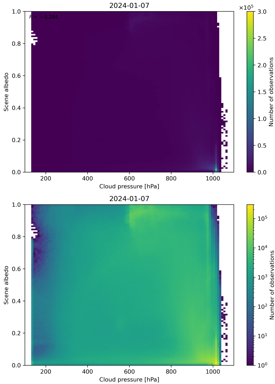
Figure 83: Scatter density plot of “Cloud pressure” against “Scene albedo” for 2024-01-06 to 2024-01-08.
