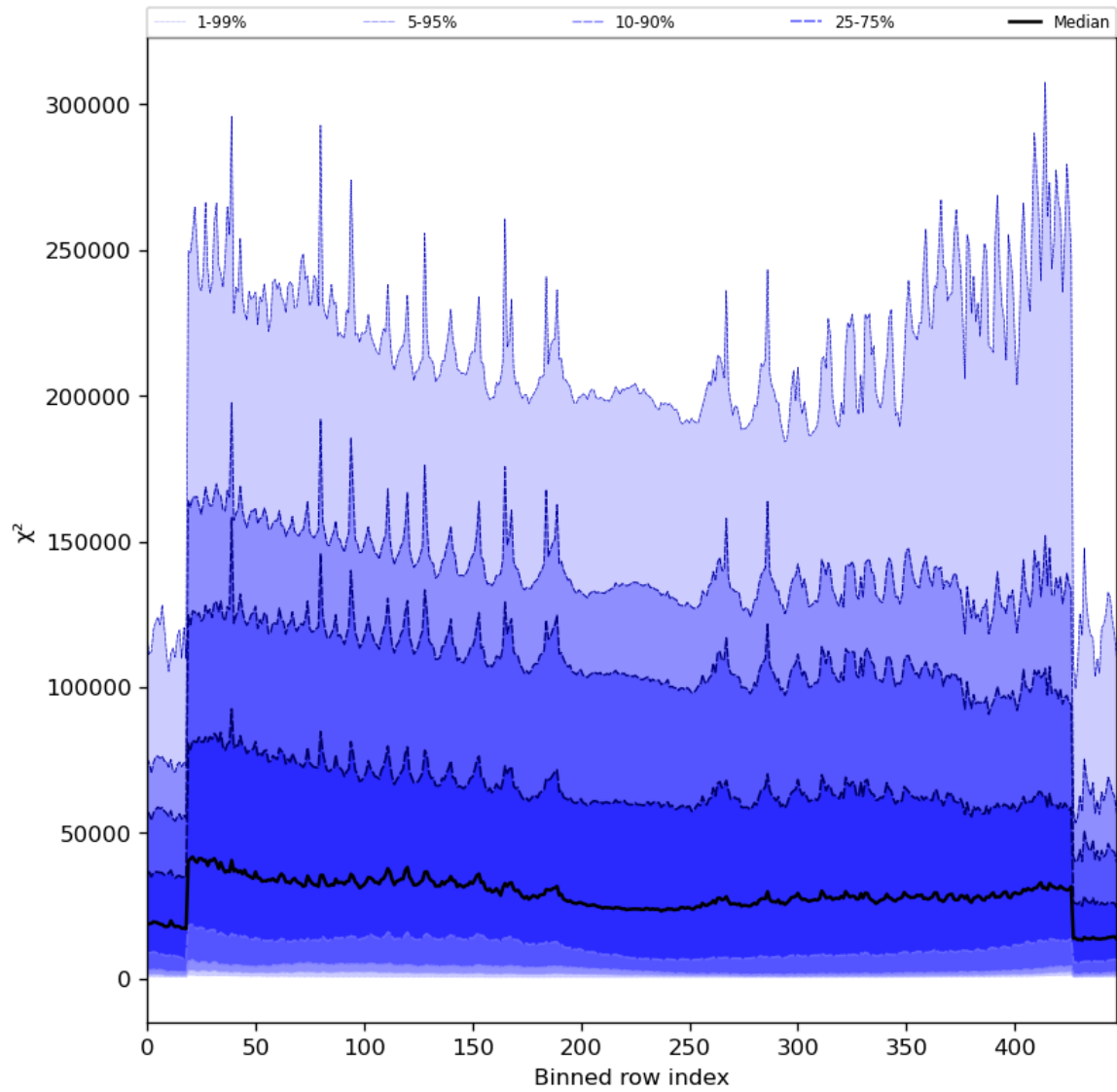
Figure 55: Along track statistics of “ \chi^2 ” for 2024-01-06 to 2024-01-08
