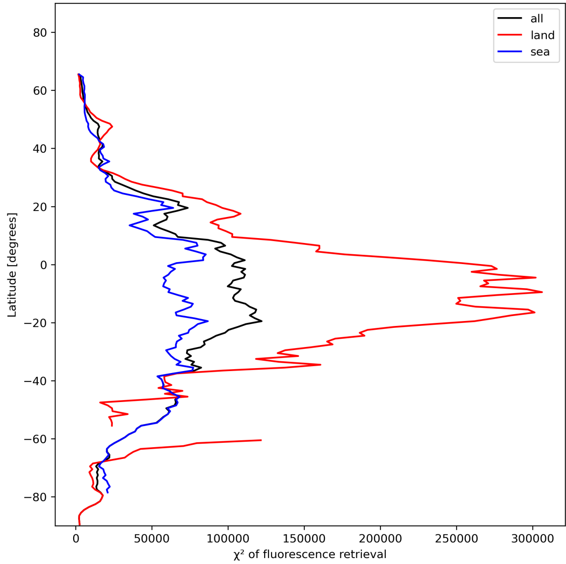
Figure 25: Zonal average of “ \chi^2 of fluorescence retrieval” for 2024-01-06 to 2024-01-08.
