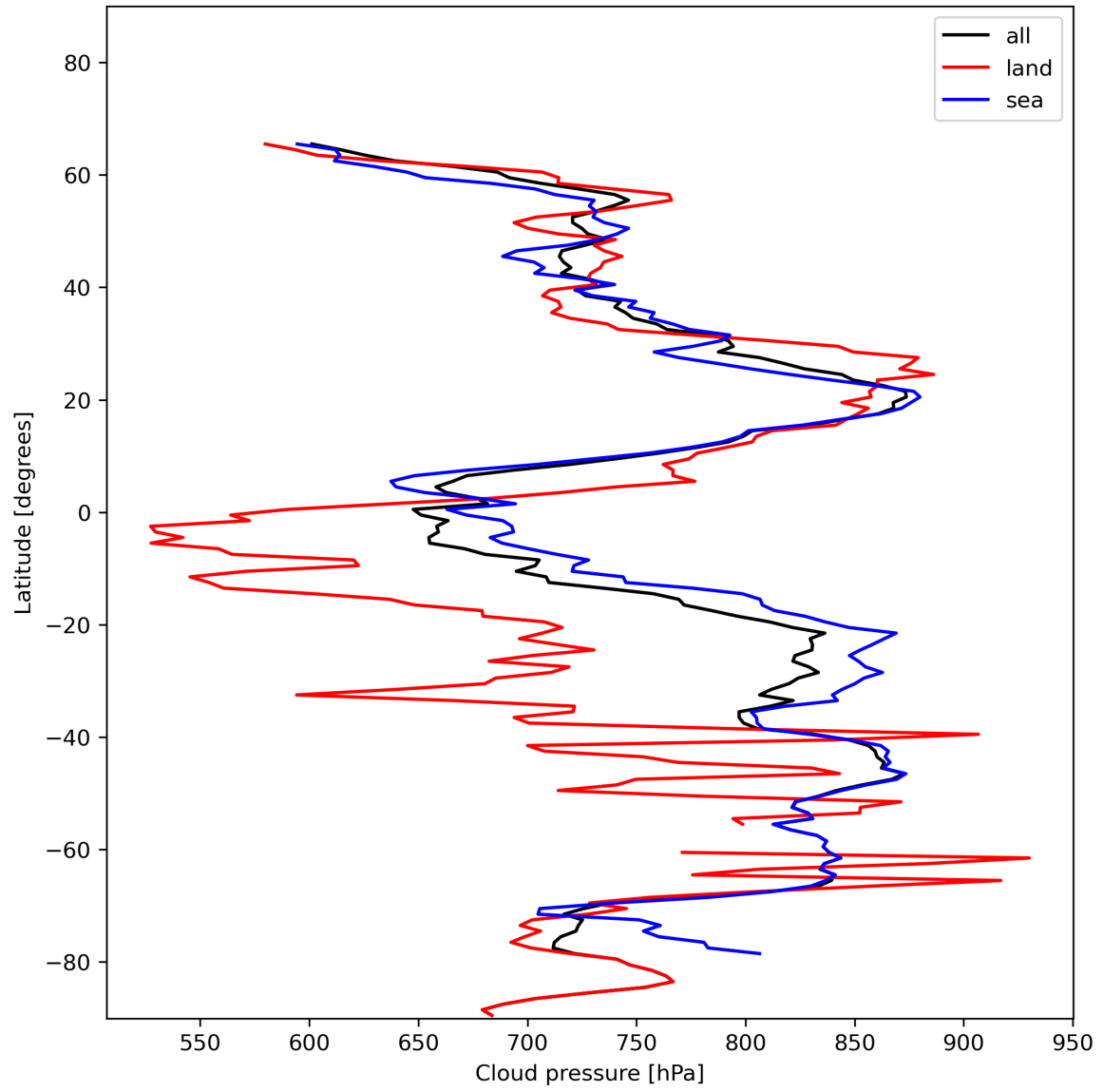
Figure 13: Zonal average of “Cloud pressure” for 2024-01-06 to 2024-01-08.
