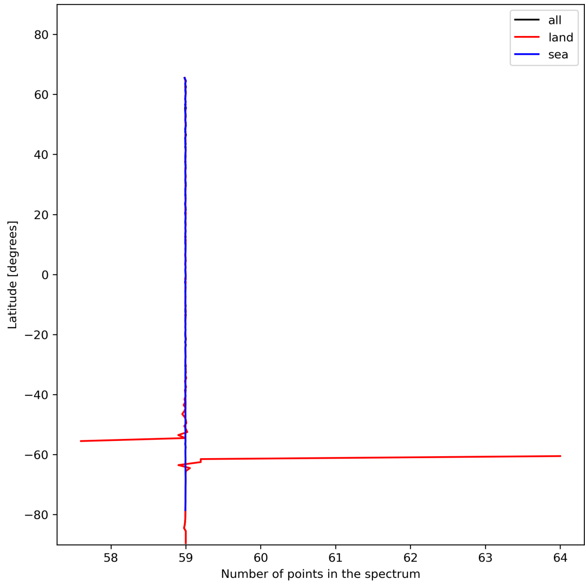
Figure 27: Zonal average of “Number of points in the spectrum” for 2024-01-06 to 2024-01-08.
