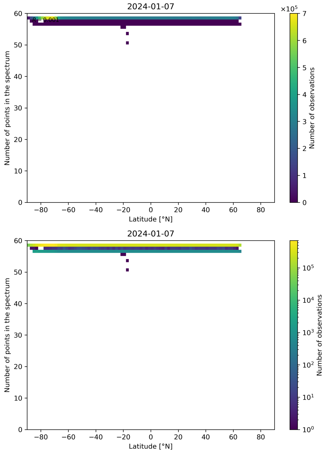
Figure 94: Scatter density plot of “Latitude” against “Number of points in the spectrum” for 2024-01-06 to 2024-01-08.
