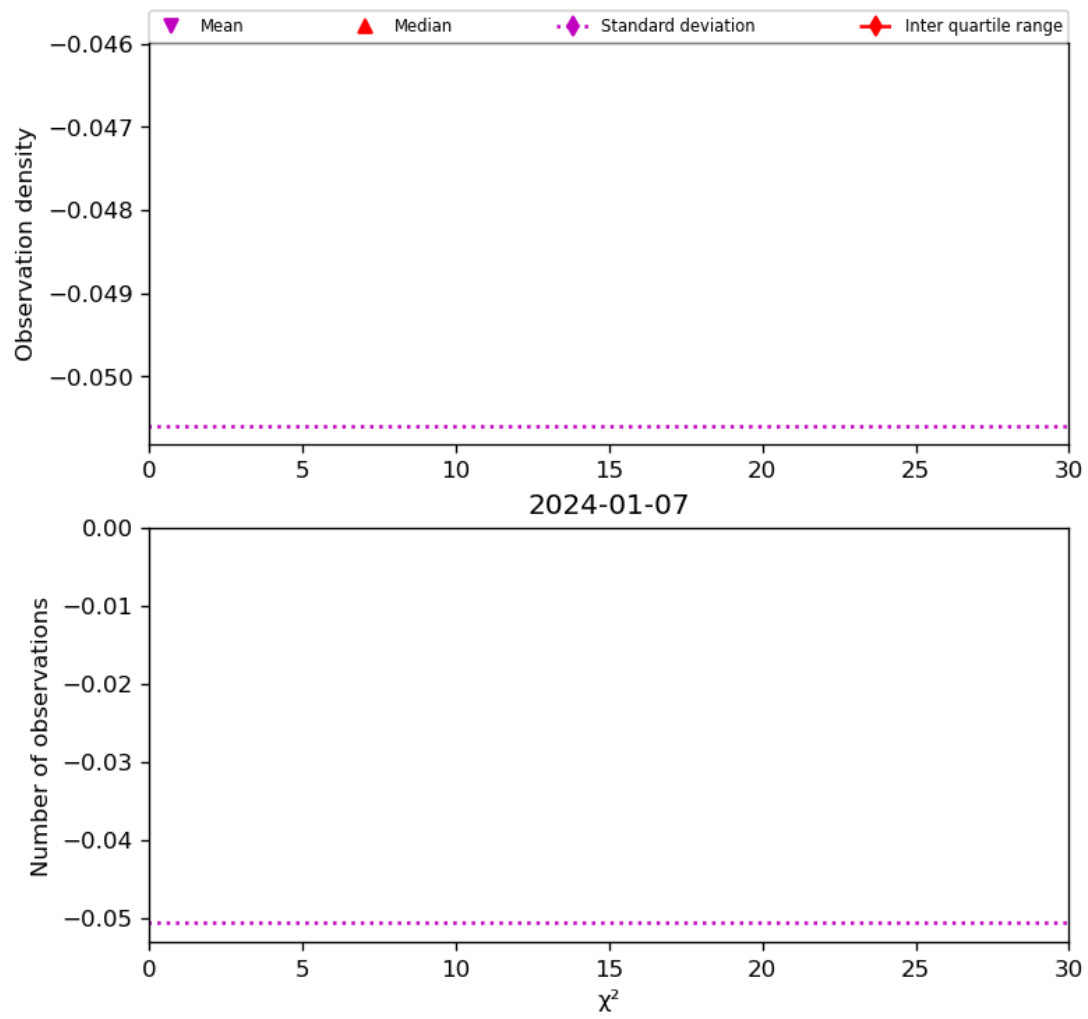
Figure 38: Histogram of “ \chi^2 ” for 2024-01-06 to 2024-01-08
