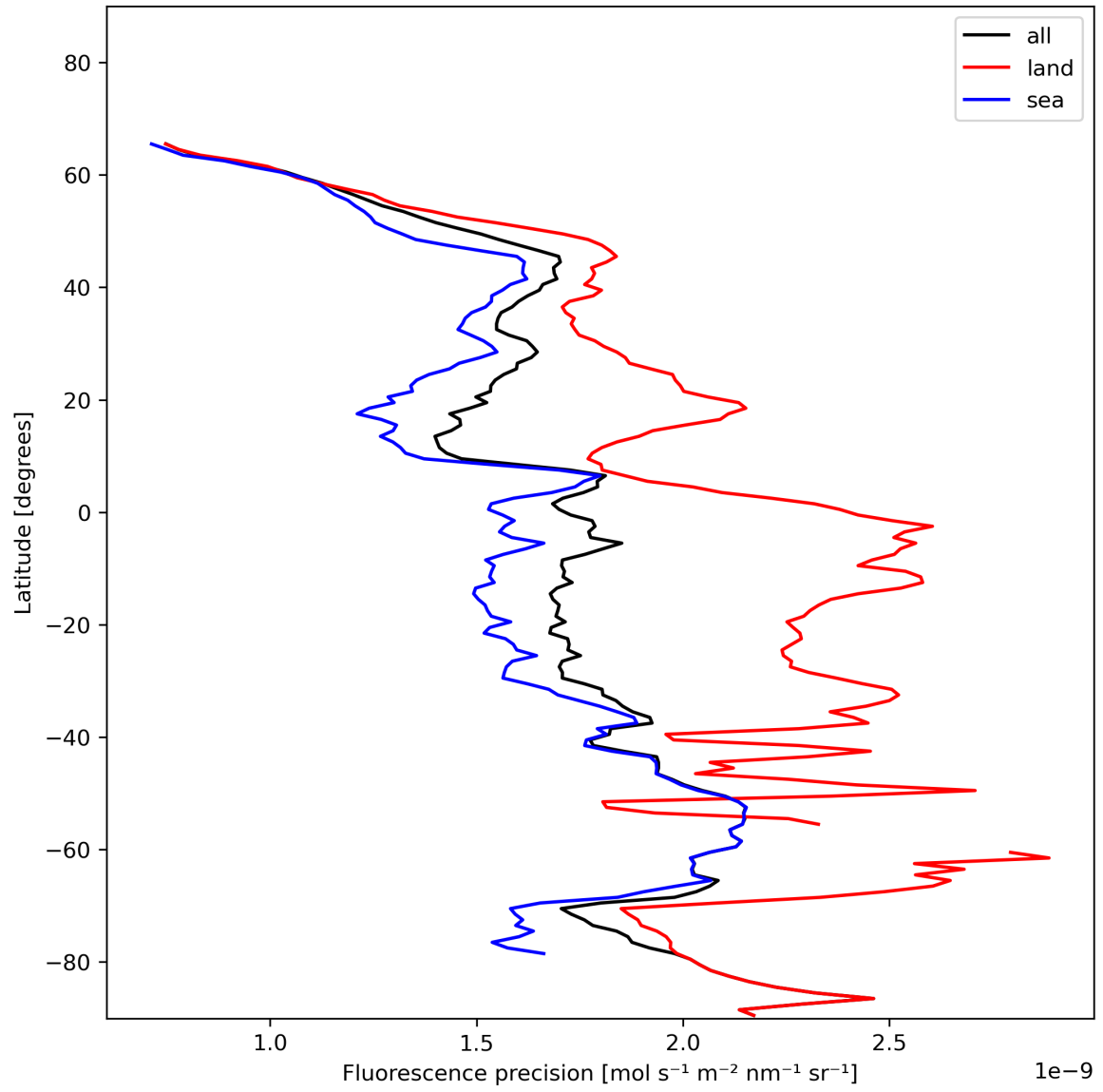
Figure 24: Zonal average of “Fluorescence precision” for 2024-01-06 to 2024-01-08.
