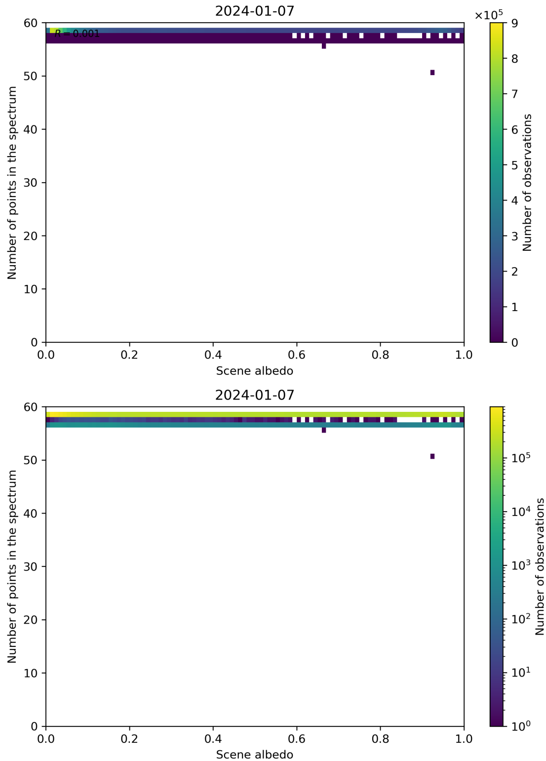
Figure 106: Scatter density plot of “Scene albedo” against “Number of points in the spectrum” for 2024-01-06 to 2024-01-08.
