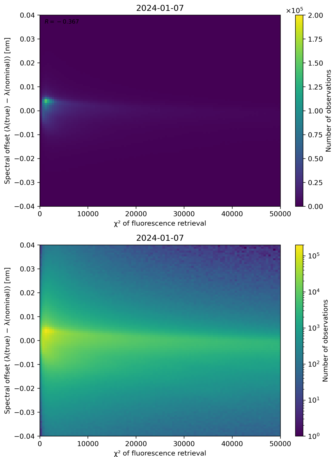
Figure 69: Scatter density plot of " \chi^2 of fluorescence retrieval" against "Spectral offset ( \lambda(\text{true}) - \lambda(\text{nominal}) )" for 2024-01-06 to 2024-01-08.
