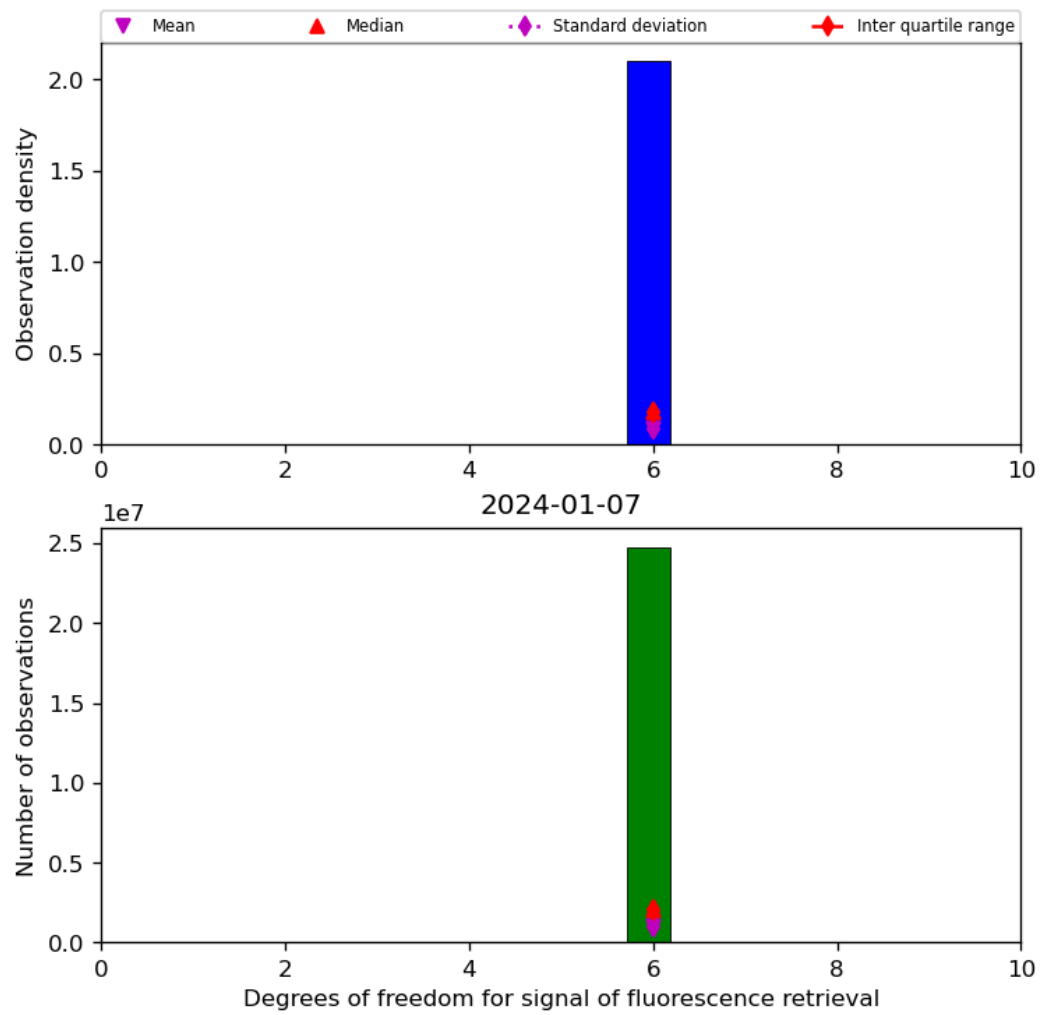
Figure 43: Histogram of “Degrees of freedom for signal of fluorescence retrieval” for 2024-01-06 to 2024-01-08
