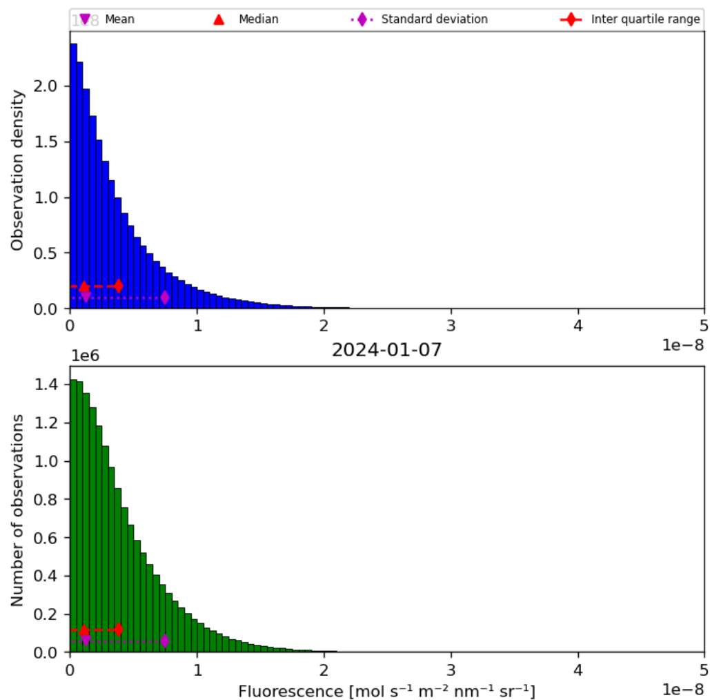
Figure 40: Histogram of “Fluorescence” for 2024-01-06 to 2024-01-08
