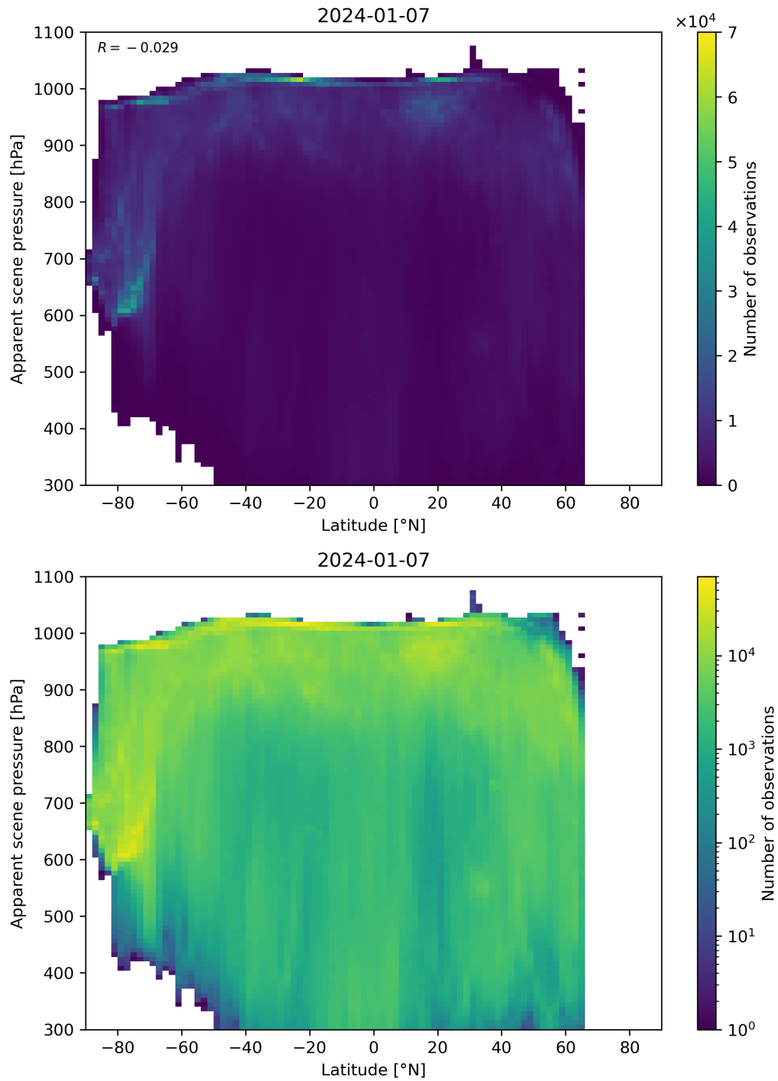
Figure 88: Scatter density plot of “Latitude” against “Apparent scene pressure” for 2024-01-06 to 2024-01-08.
