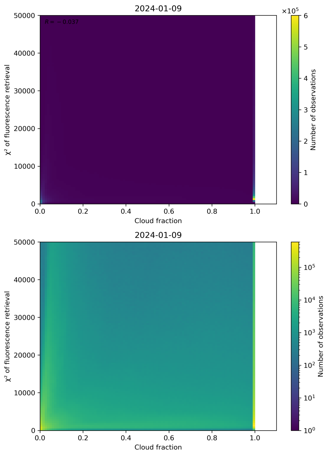
Figure 71: Scatter density plot of “Cloud fraction” against “ \chi^2 of fluorescence retrieval” for 2024-01-08 to 2024-01-10.
