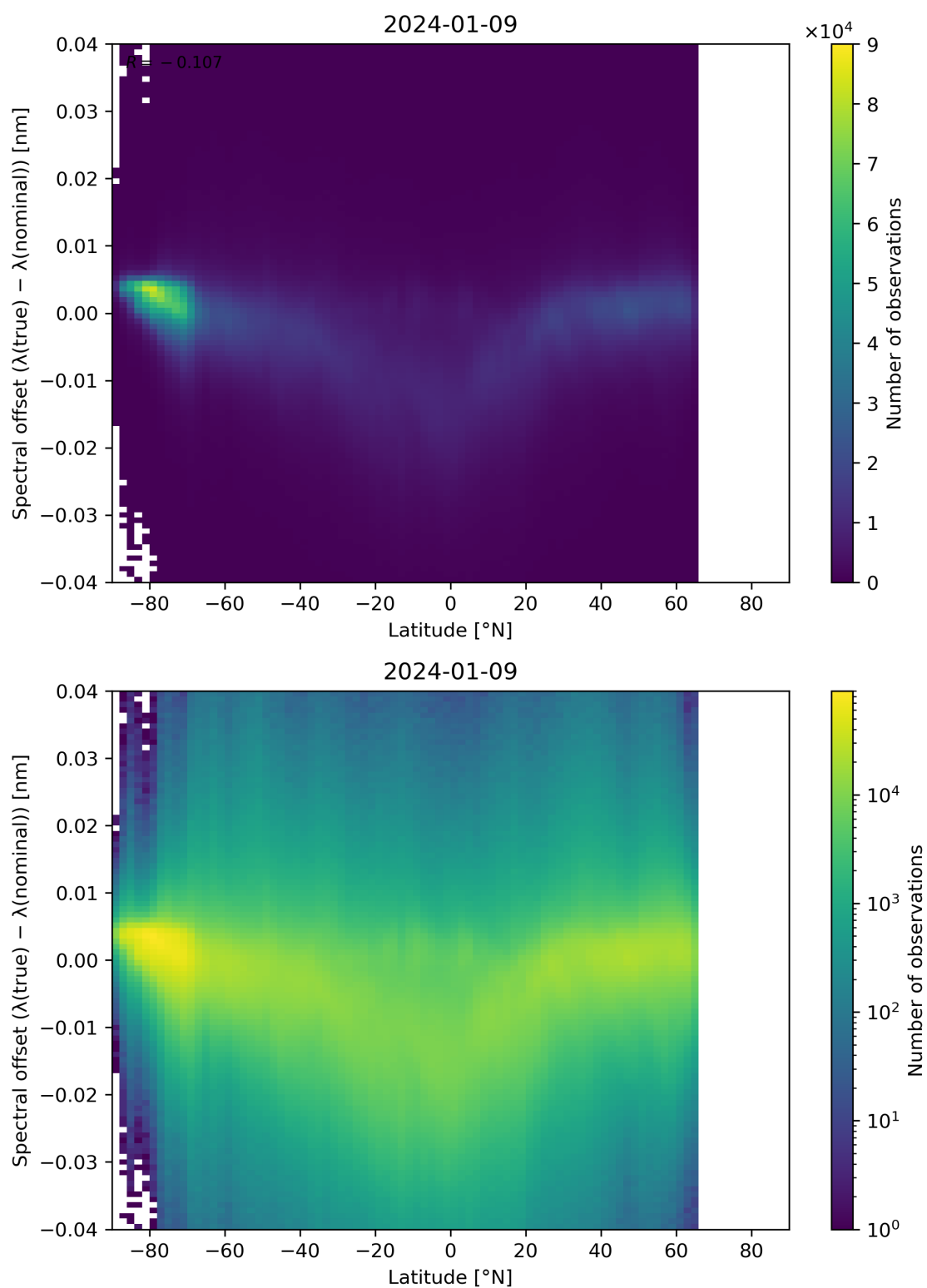
Figure 96: Scatter density plot of “Latitude” against “Spectral offset ( \lambda(\text{true}) - \lambda(\text{nominal}) )” for 2024-01-08 to 2024-01-10.
