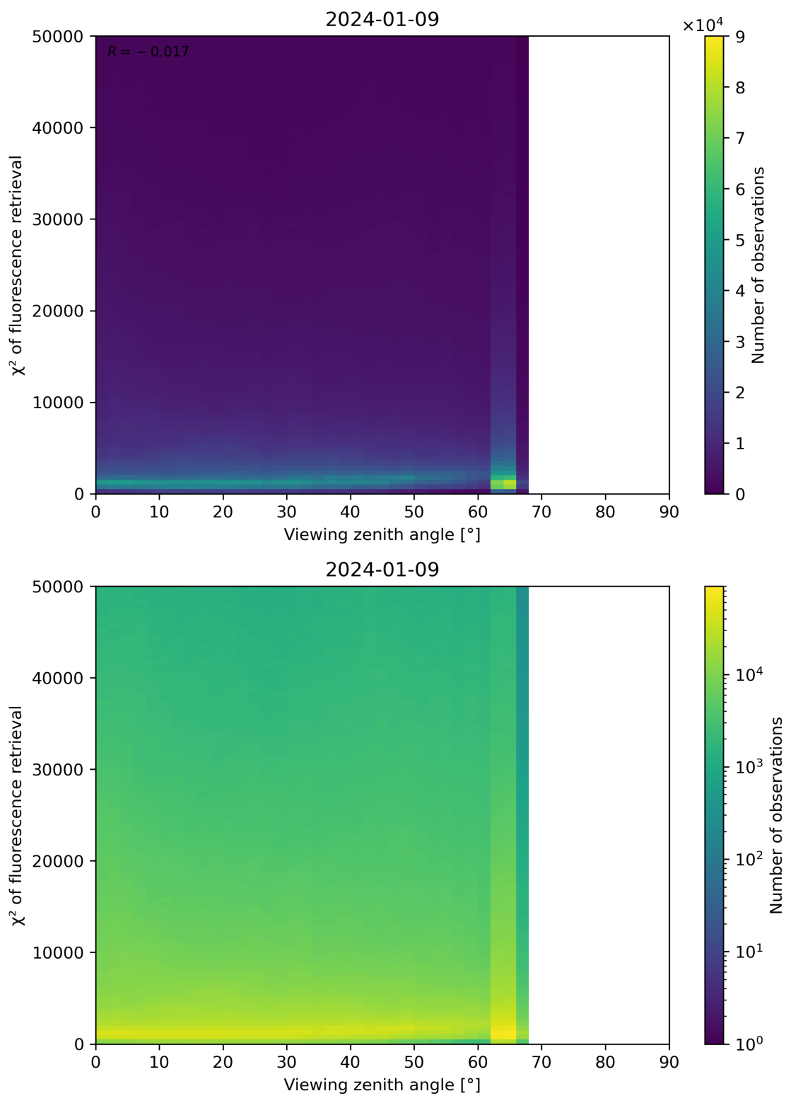
Figure 119: Scatter density plot of “Viewing zenith angle” against “ \chi^2 of fluorescence retrieval” for 2024-01-08 to 2024-01-10.
