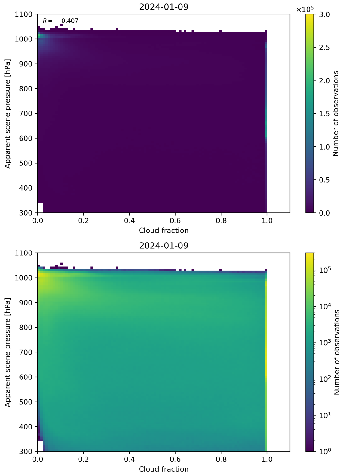
Figure 70: Scatter density plot of “Cloud fraction” against “Apparent scene pressure” for 2024-01-08 to 2024-01-10.
