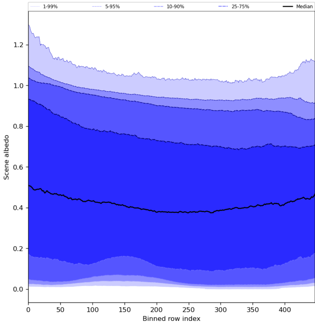
Figure 51: Along track statistics of “Scene albedo” for 2024-01-08 to 2024-01-10
