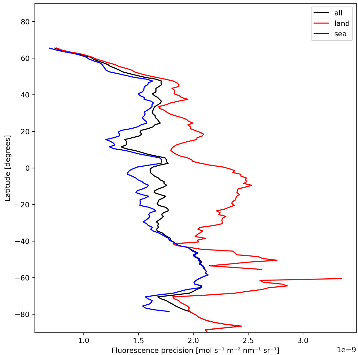
Figure 24: Zonal average of “Fluorescence precision” for 2024-01-08 to 2024-01-10.
