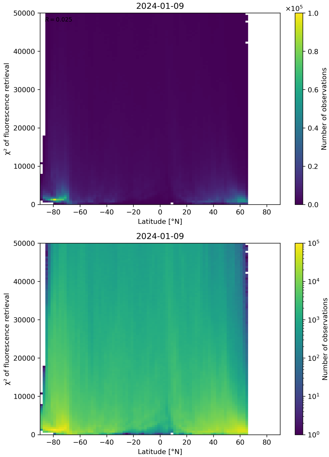
Figure 89: Scatter density plot of “Latitude” against “ \chi^2 of fluorescence retrieval” for 2024-01-08 to 2024-01-10.
