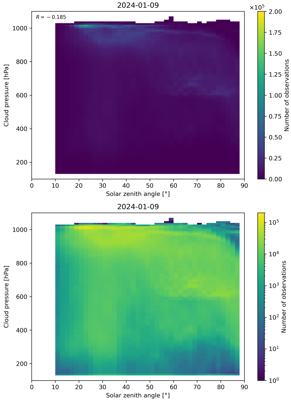
Figure 111: Scatter density plot of “Solar zenith angle” against “Cloud pressure” for 2024-01-08 to 2024-01-10.
