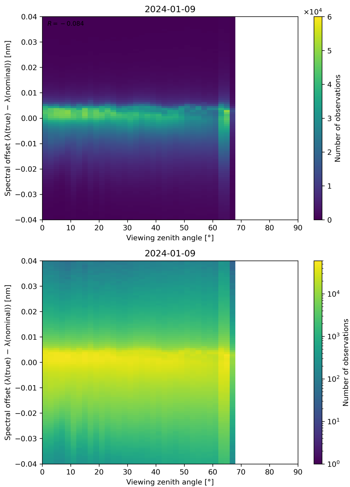
Figure 128: Scatter density plot of “Viewing zenith angle” against “Spectral offset ( \lambda(\text{true}) - \lambda(\text{nominal}) )” for 2024-01-08 to 2024-01-10.
