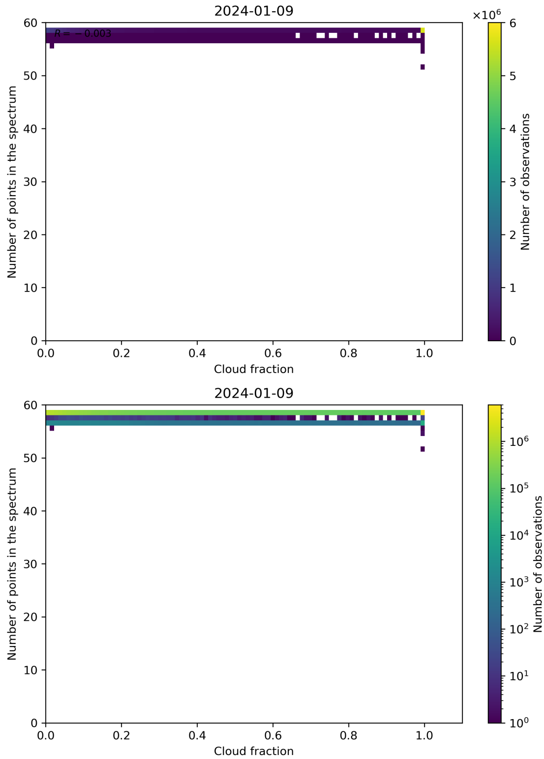
Figure 74: Scatter density plot of “Cloud fraction” against “Number of points in the spectrum” for 2024-01-08 to 2024-01-10.
