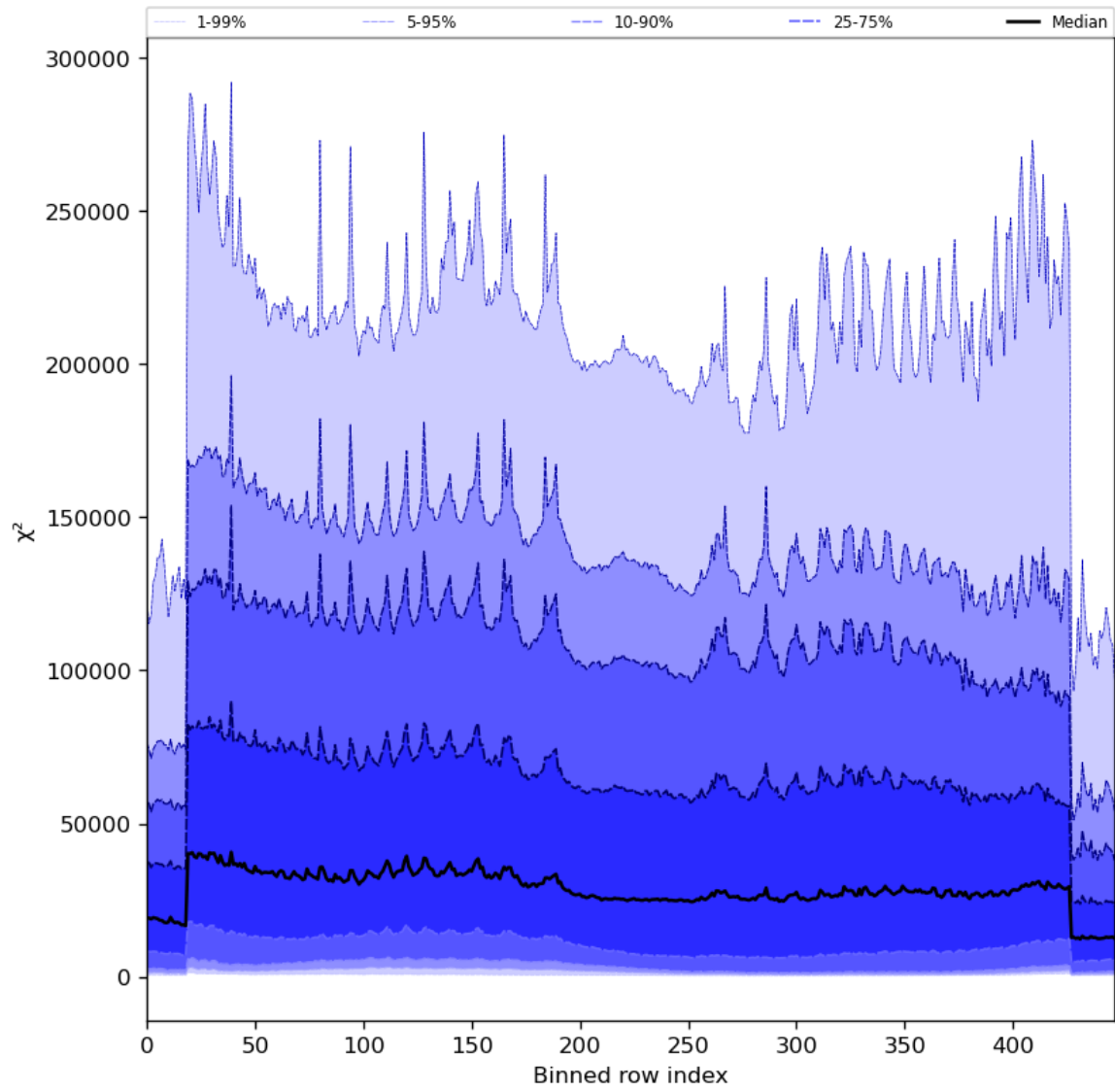
Figure 55: Along track statistics of “ \chi^2 ” for 2024-01-08 to 2024-01-10
