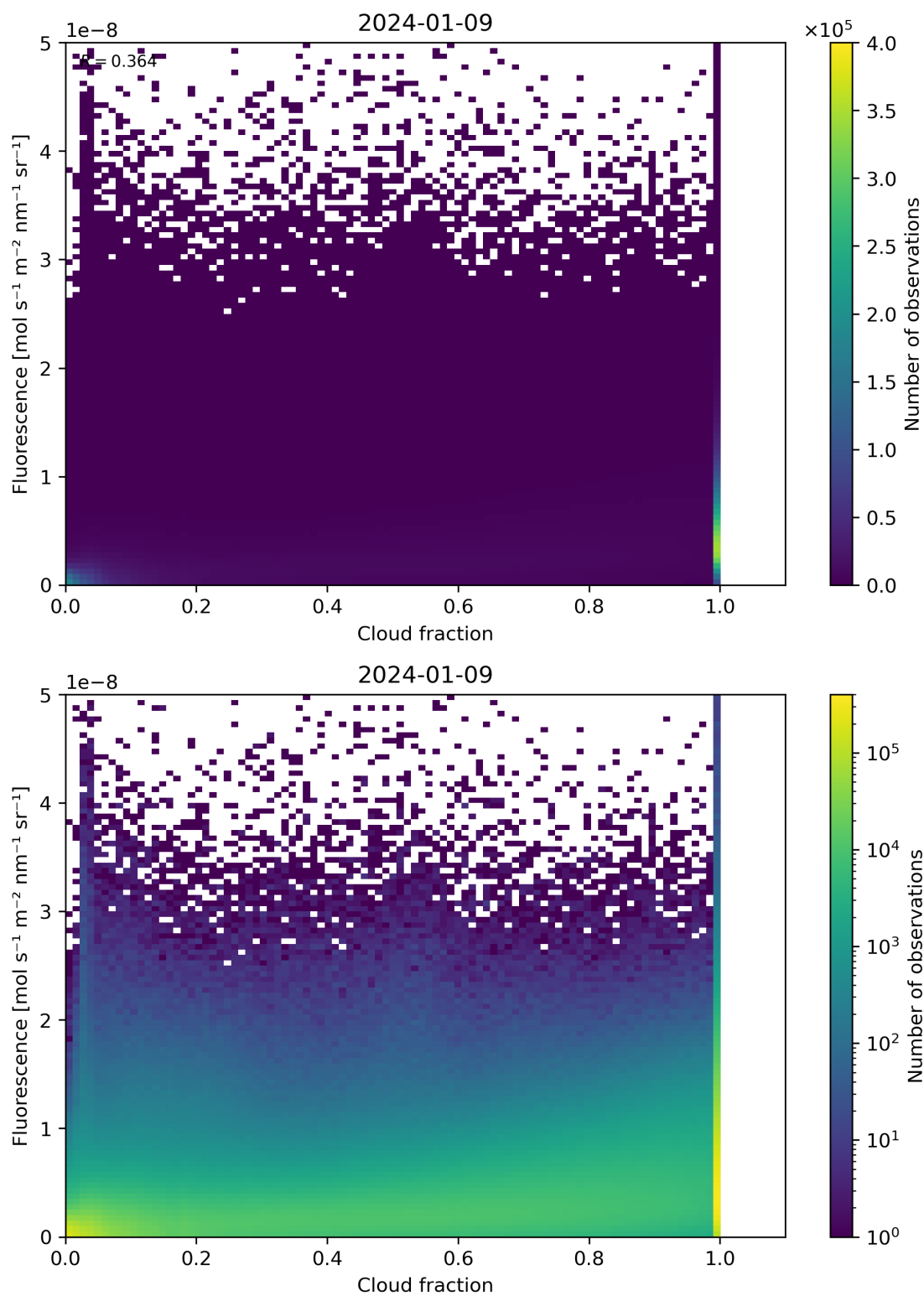
Figure 72: Scatter density plot of “Cloud fraction” against “Fluorescence” for 2024-01-08 to 2024-01-10.
