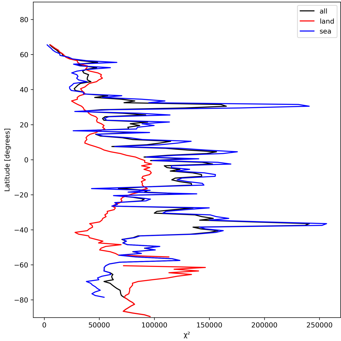
Figure 21: Zonal average of “ \chi^2 ” for 2024-01-08 to 2024-01-10.
