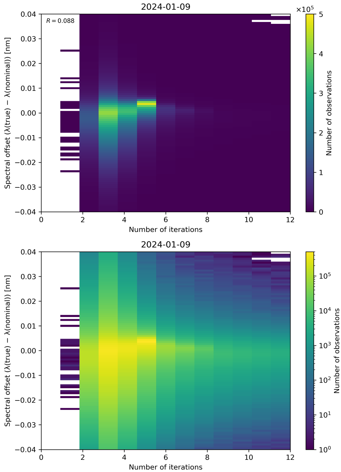
Figure 100: Scatter density plot of “Number of iterations” against “Spectral offset ( \lambda(\text{true}) - \lambda(\text{nominal}) )” for 2024-01-08 to 2024-01-10.
