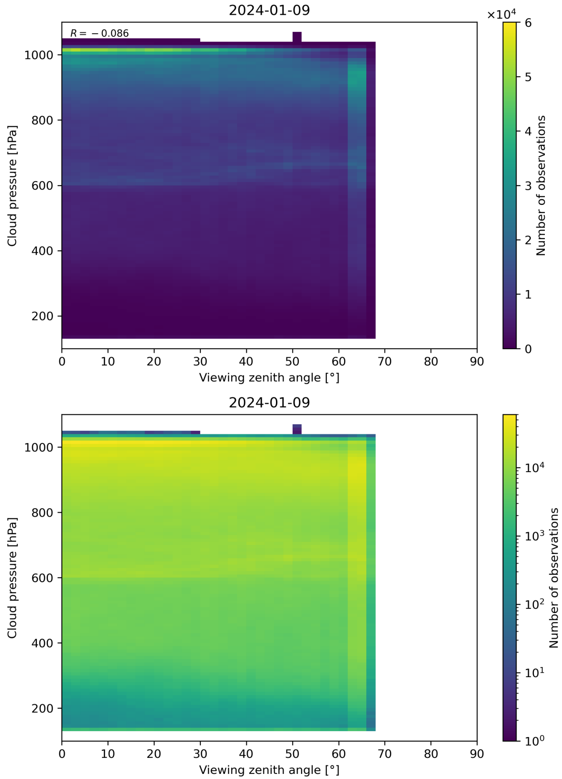
Figure 121: Scatter density plot of “Viewing zenith angle” against “Cloud pressure” for 2024-01-08 to 2024-01-10.
