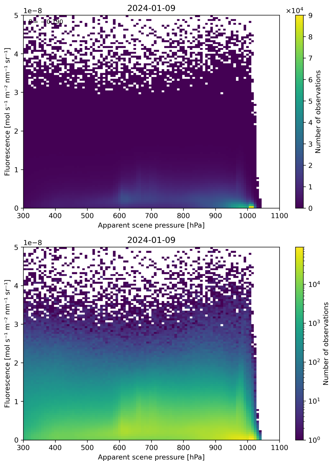
Figure 64: Scatter density plot of “Apparent scene pressure” against “Fluorescence” for 2024-01-08 to 2024-01-10.
