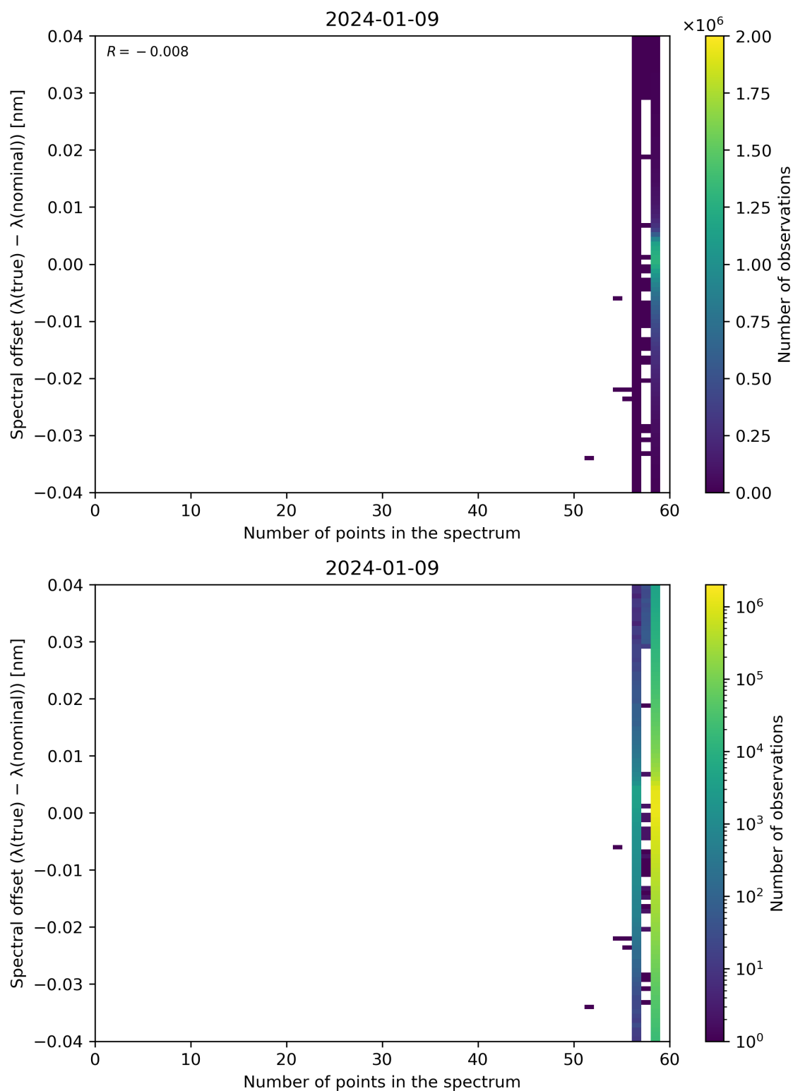
Figure 101: Scatter density plot of “Number of points in the spectrum” against “Spectral offset ( \lambda(\text{true}) - \lambda(\text{nominal}) )” for 2024-01-08 to 2024-01-10.
