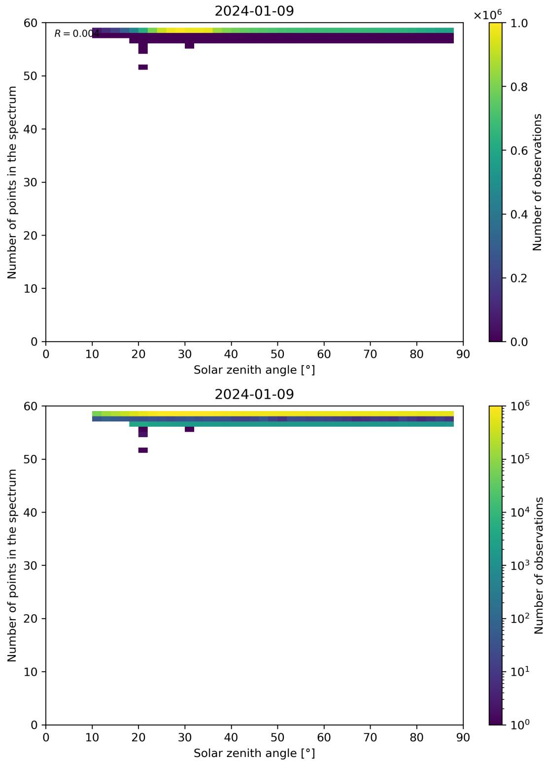
Figure 115: Scatter density plot of “Solar zenith angle” against “Number of points in the spectrum” for 2024-01-08 to 2024-01-10.
