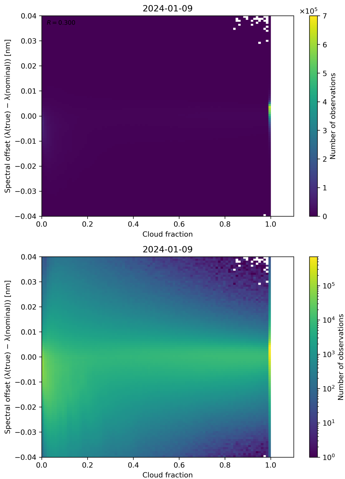
Figure 76: Scatter density plot of “Cloud fraction” against “Spectral offset ( \lambda(\text{true}) - \lambda(\text{nominal}) )” for 2024-01-08 to 2024-01-10.
