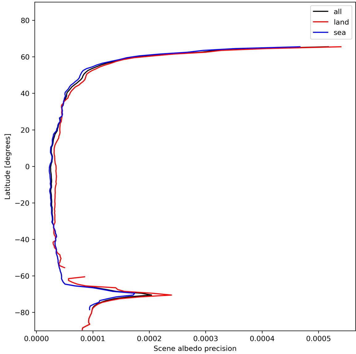
Figure 18: Zonal average of “Scene albedo precision” for 2024-01-08 to 2024-01-10.
