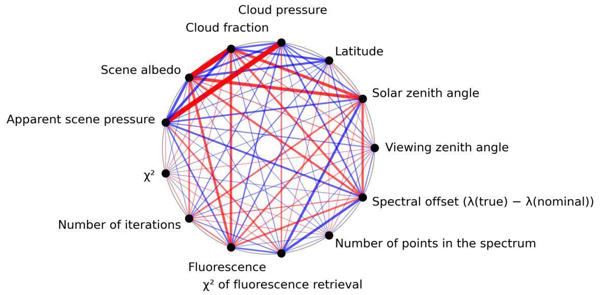
Figure 1: Map of correlation graph for 2024-01-08 to 2024-01-10.
