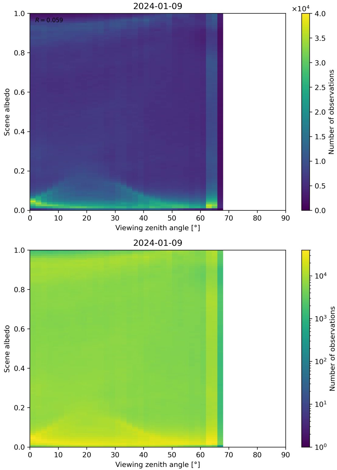
Figure 126: Scatter density plot of “Viewing zenith angle” against “Scene albedo” for 2024-01-08 to 2024-01-10.
