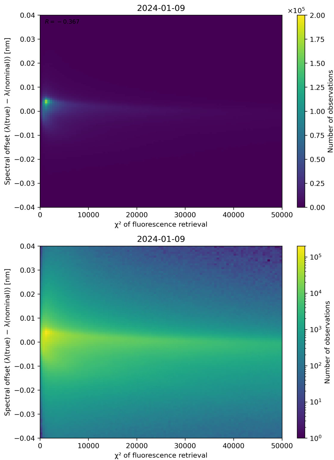
Figure 69: Scatter density plot of " \chi^2 of fluorescence retrieval" against "Spectral offset ( \lambda(\text{true}) - \lambda(\text{nominal}) )" for 2024-01-08 to 2024-01-10.
