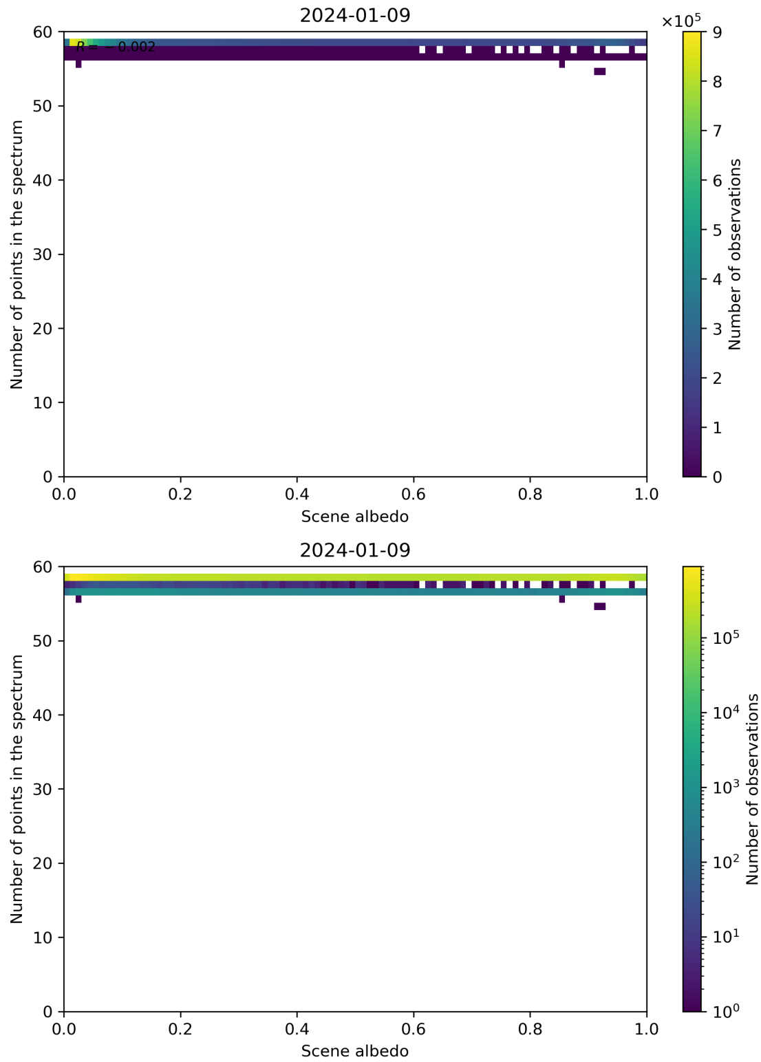
Figure 106: Scatter density plot of “Scene albedo” against “Number of points in the spectrum” for 2024-01-08 to 2024-01-10.
