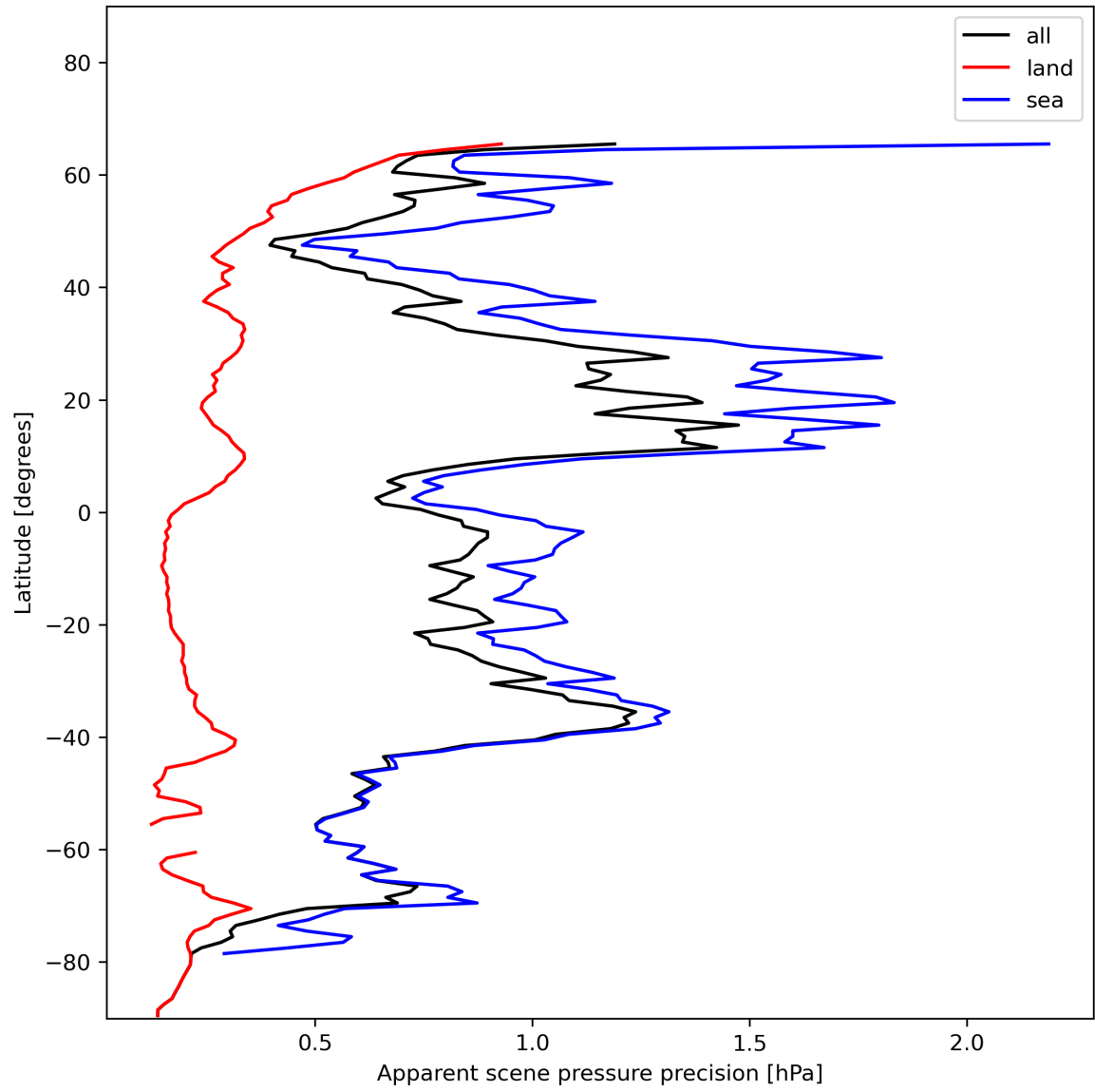
Figure 20: Zonal average of “Apparent scene pressure precision” for 2024-01-08 to 2024-01-10.
