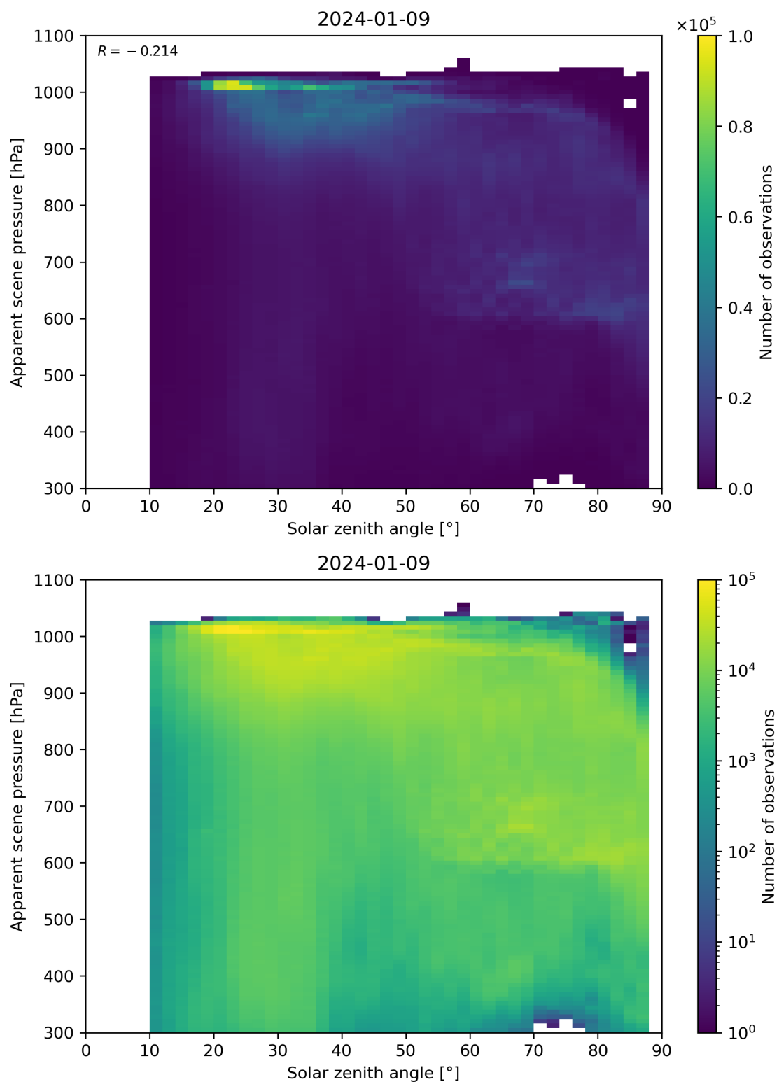
Figure 108: Scatter density plot of “Solar zenith angle” against “Apparent scene pressure” for 2024-01-08 to 2024-01-10.
