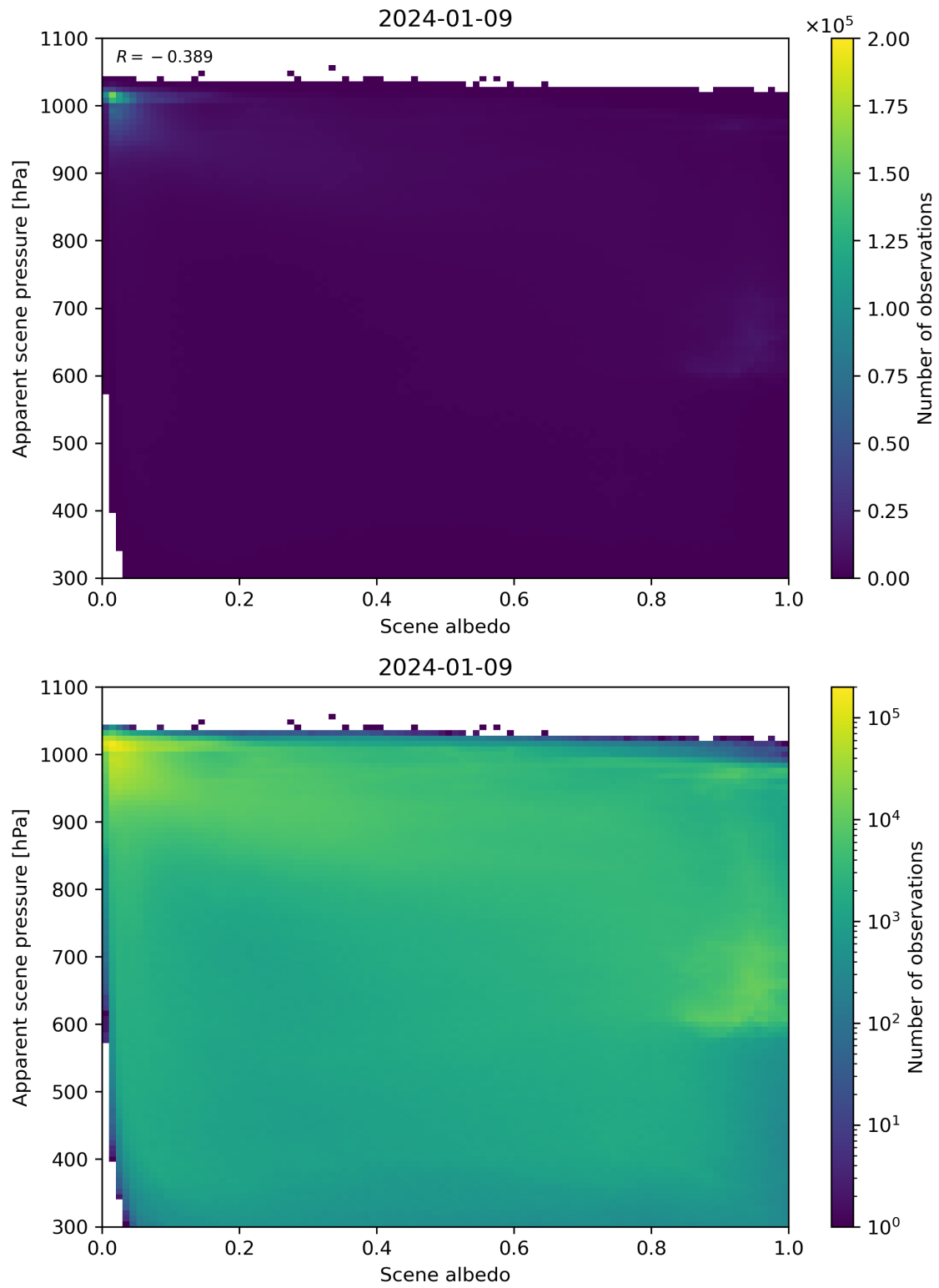
Figure 102: Scatter density plot of “Scene albedo” against “Apparent scene pressure” for 2024-01-08 to 2024-01-10.
