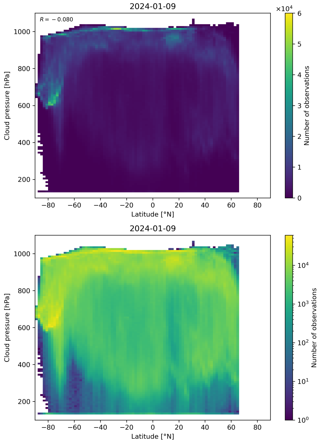
Figure 91: Scatter density plot of “Latitude” against “Cloud pressure” for 2024-01-08 to 2024-01-10.
