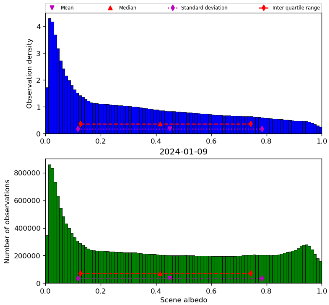
Figure 34: Histogram of “Scene albedo” for 2024-01-08 to 2024-01-10
