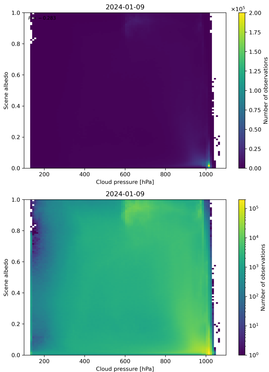
Figure 83: Scatter density plot of “Cloud pressure” against “Scene albedo” for 2024-01-08 to 2024-01-10.
