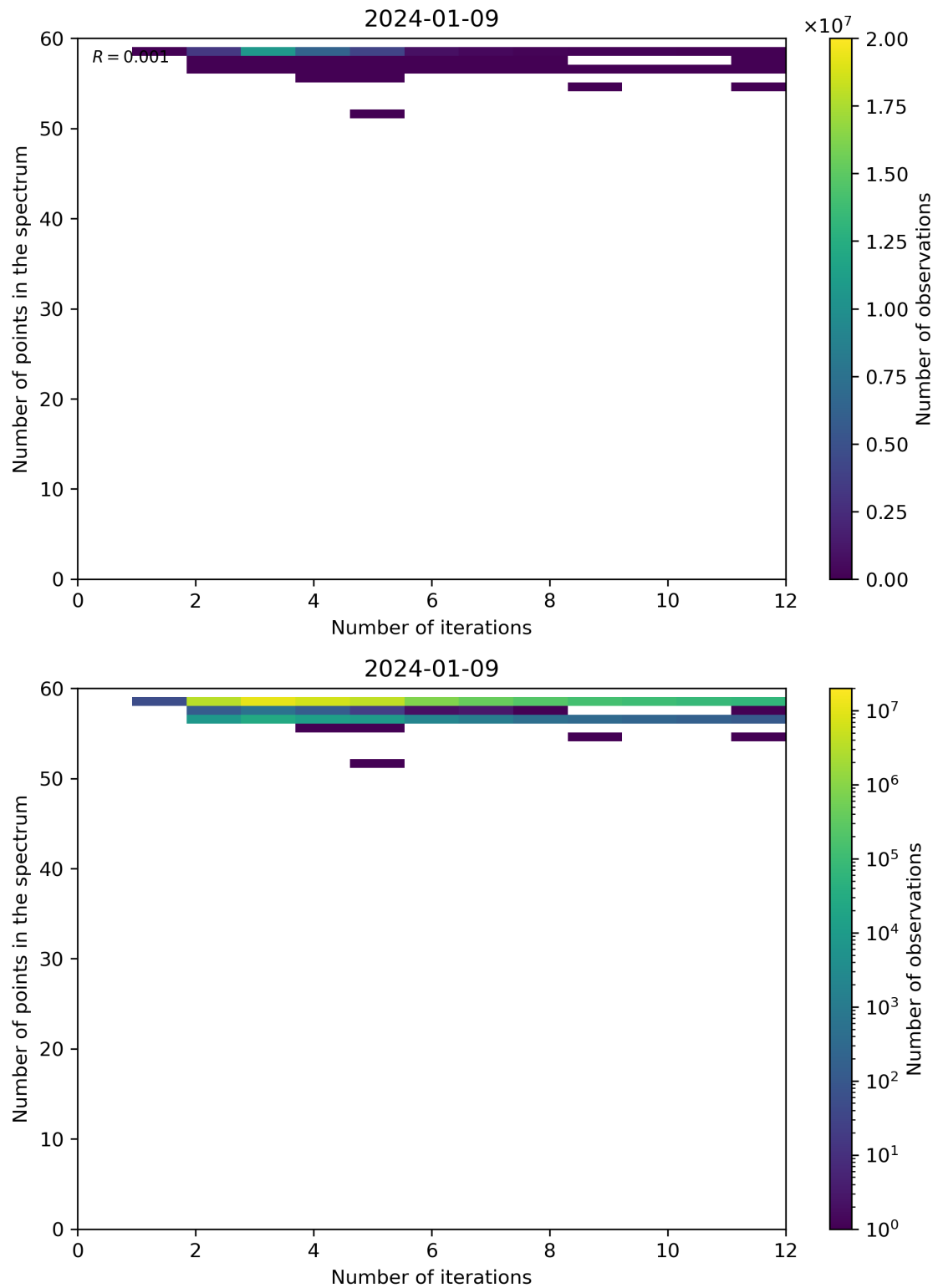
Figure 99: Scatter density plot of “Number of iterations” against “Number of points in the spectrum” for 2024-01-08 to 2024-01-10.
