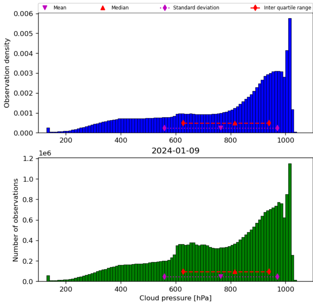
Figure 30: Histogram of “Cloud pressure” for 2024-01-08 to 2024-01-10
