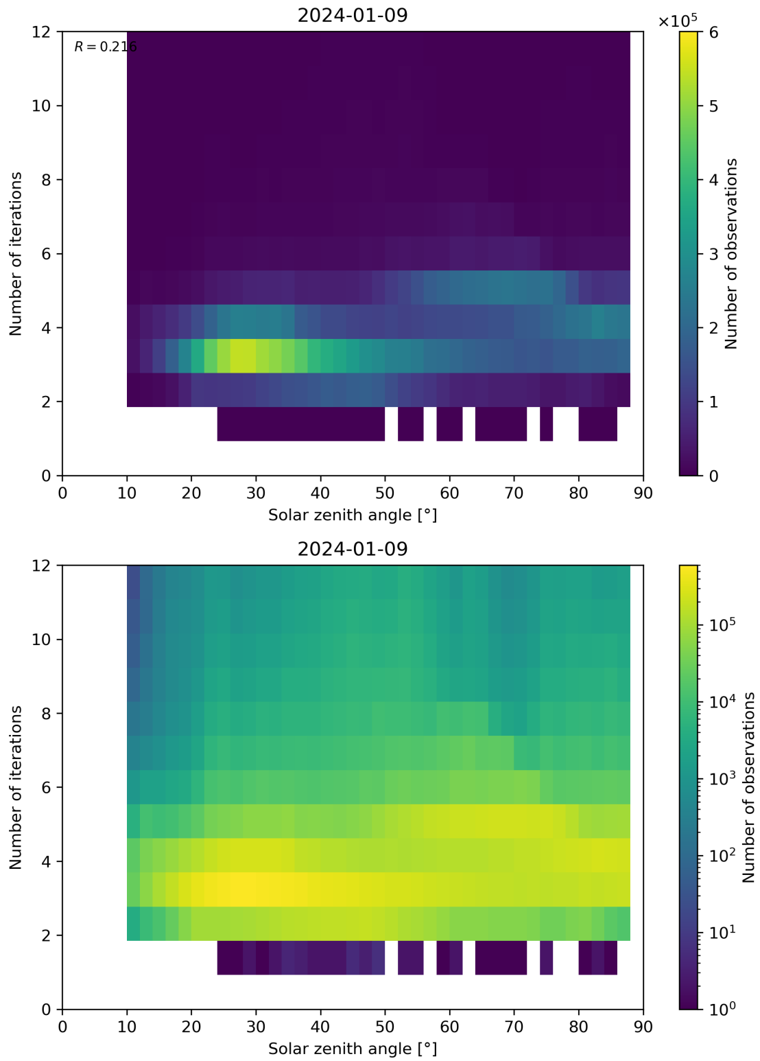
Figure 114: Scatter density plot of “Solar zenith angle” against “Number of iterations” for 2024-01-08 to 2024-01-10.
