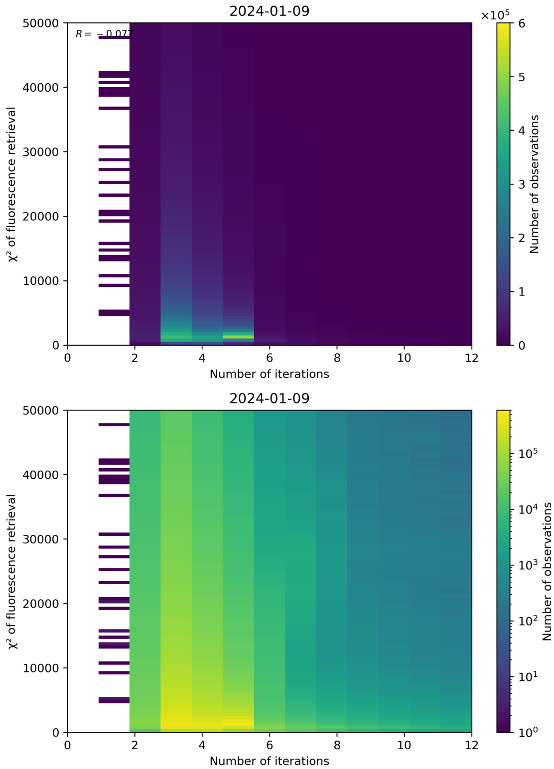
Figure 97: Scatter density plot of “Number of iterations” against “ \chi^2 of fluorescence retrieval” for 2024-01-08 to 2024-01-10.
