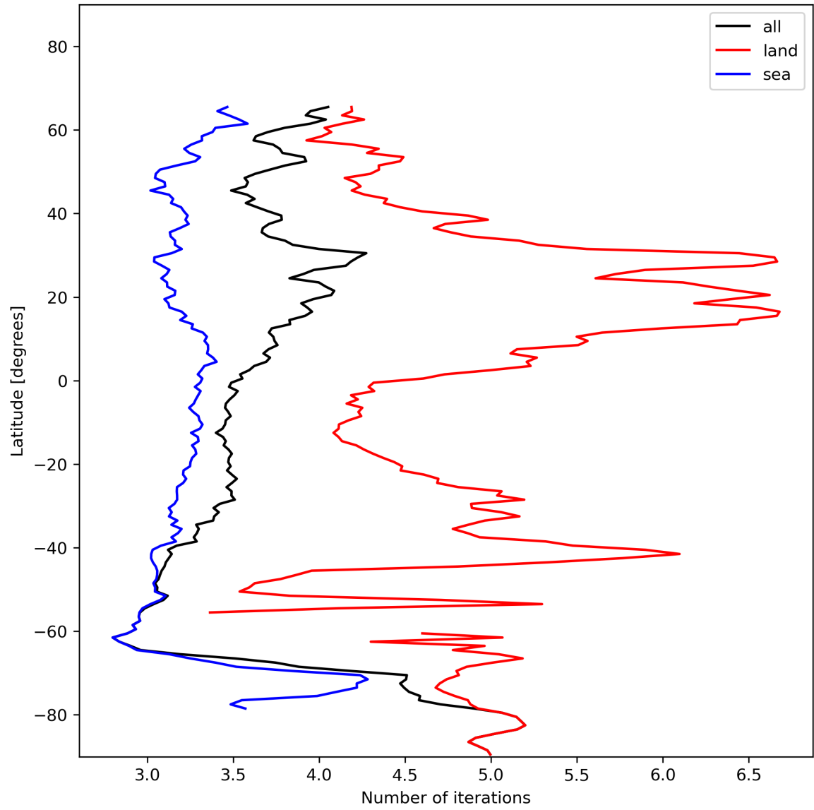
Figure 22: Zonal average of “Number of iterations” for 2024-01-08 to 2024-01-10.
