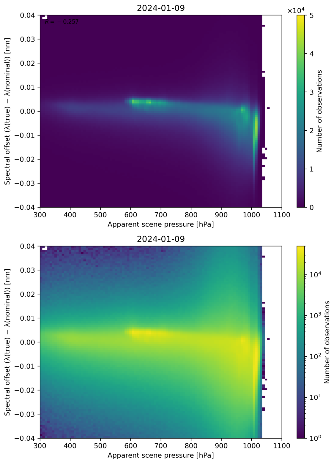
Figure 67: Scatter density plot of “Apparent scene pressure” against “Spectral offset ( \lambda(\text{true}) - \lambda(\text{nominal}) )” for 2024-01-08 to 2024-01-10.
