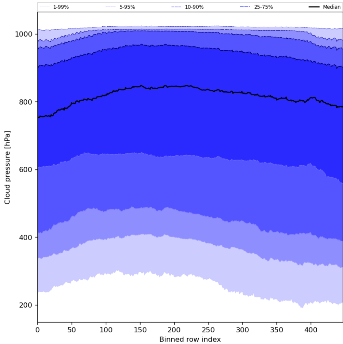
Figure 47: Along track statistics of “Cloud pressure” for 2024-01-08 to 2024-01-10
