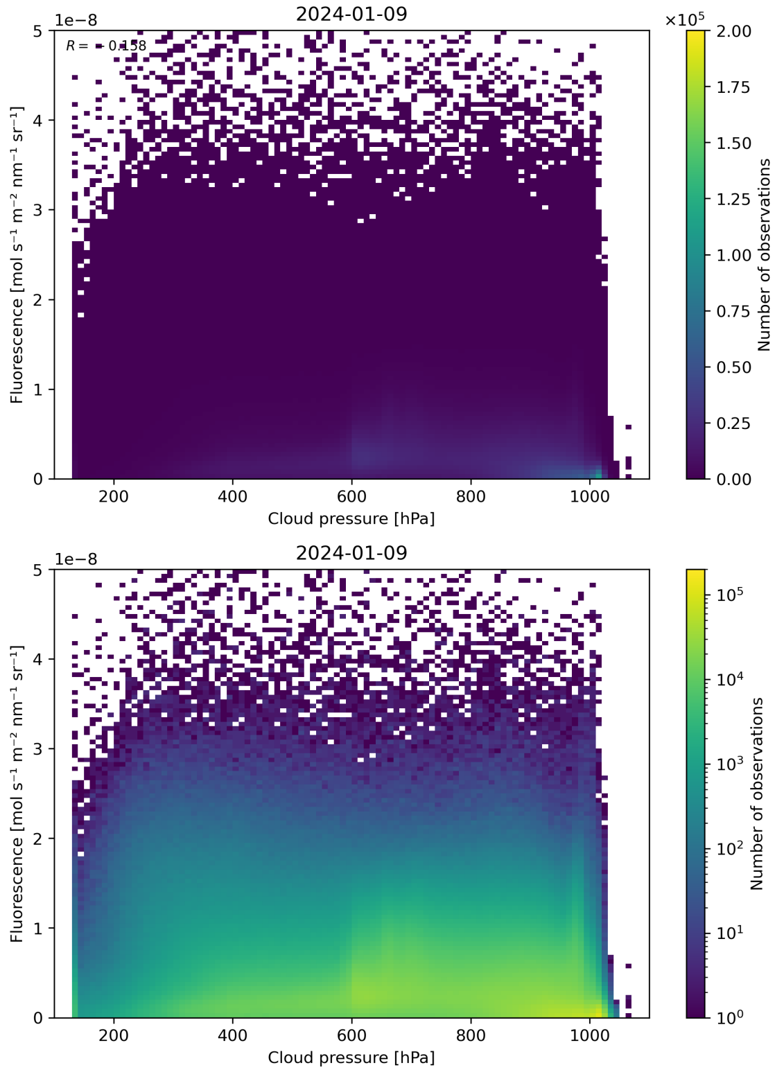
Figure 80: Scatter density plot of “Cloud pressure” against “Fluorescence” for 2024-01-08 to 2024-01-10.
