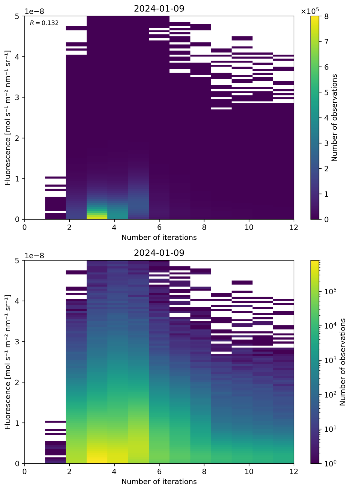
Figure 98: Scatter density plot of “Number of iterations” against “Fluorescence” for 2024-01-08 to 2024-01-10.
