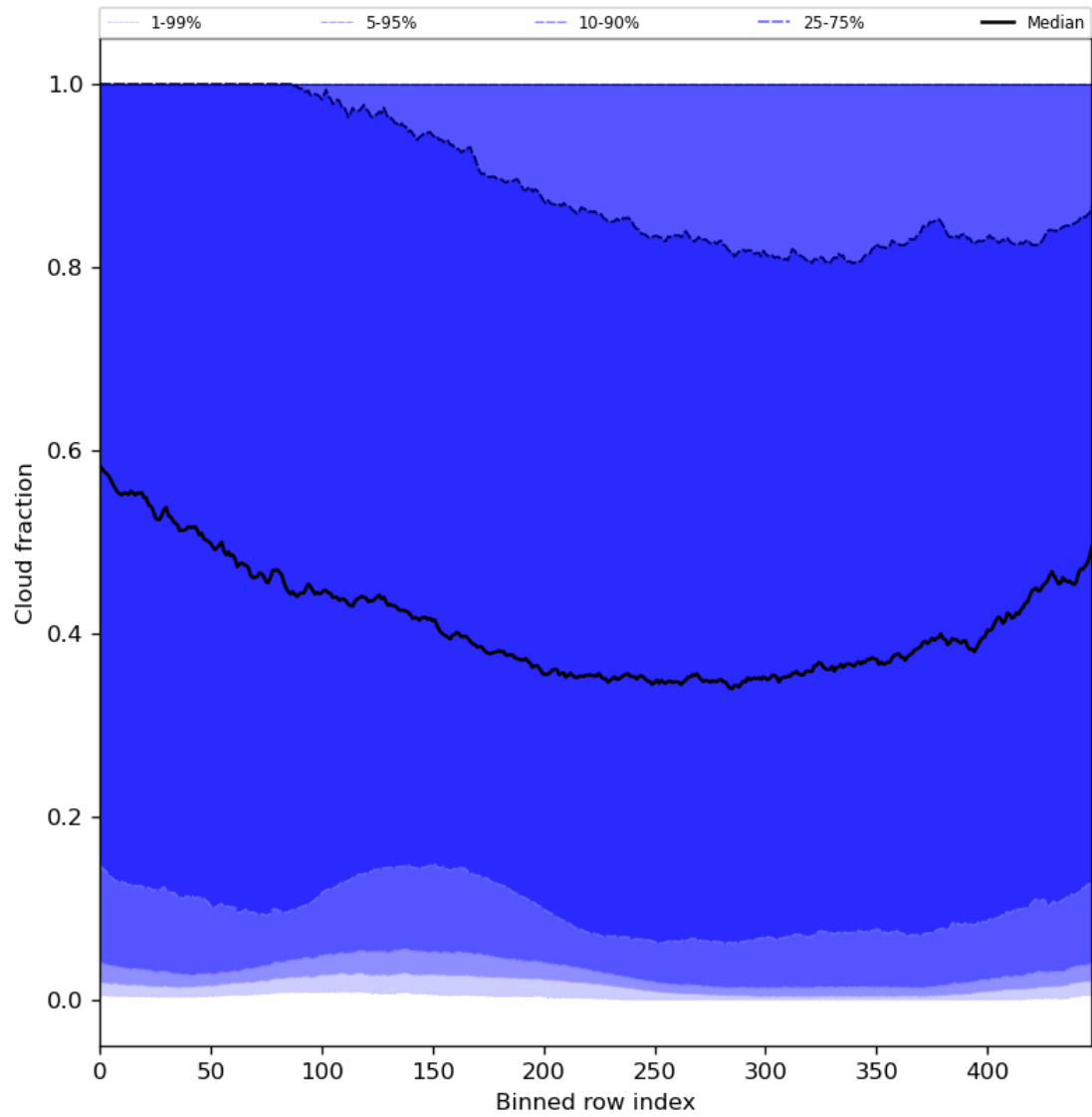
Figure 49: Along track statistics of “Cloud fraction” for 2024-01-08 to 2024-01-10
