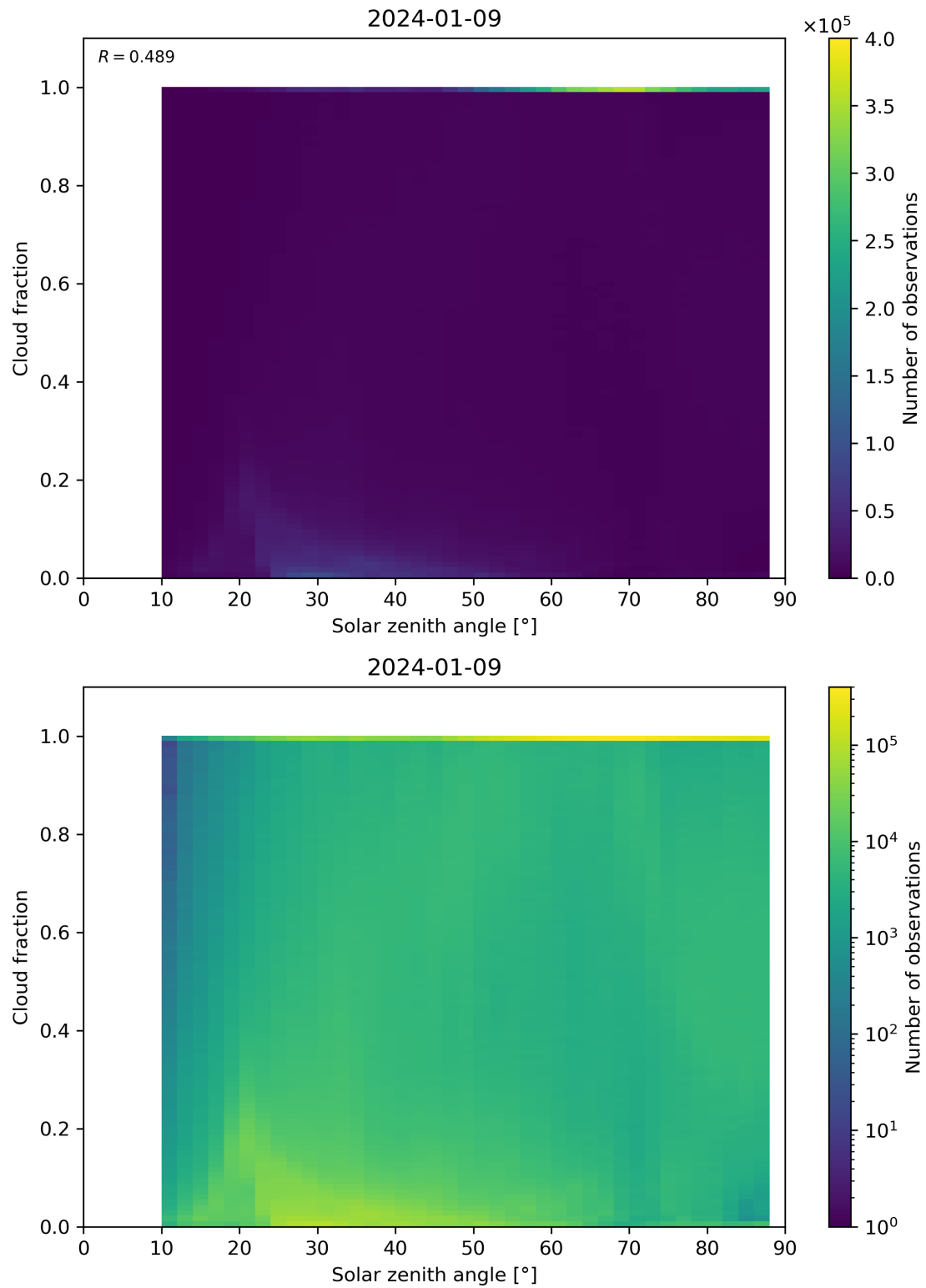
Figure 110: Scatter density plot of “Solar zenith angle” against “Cloud fraction” for 2024-01-08 to 2024-01-10.
