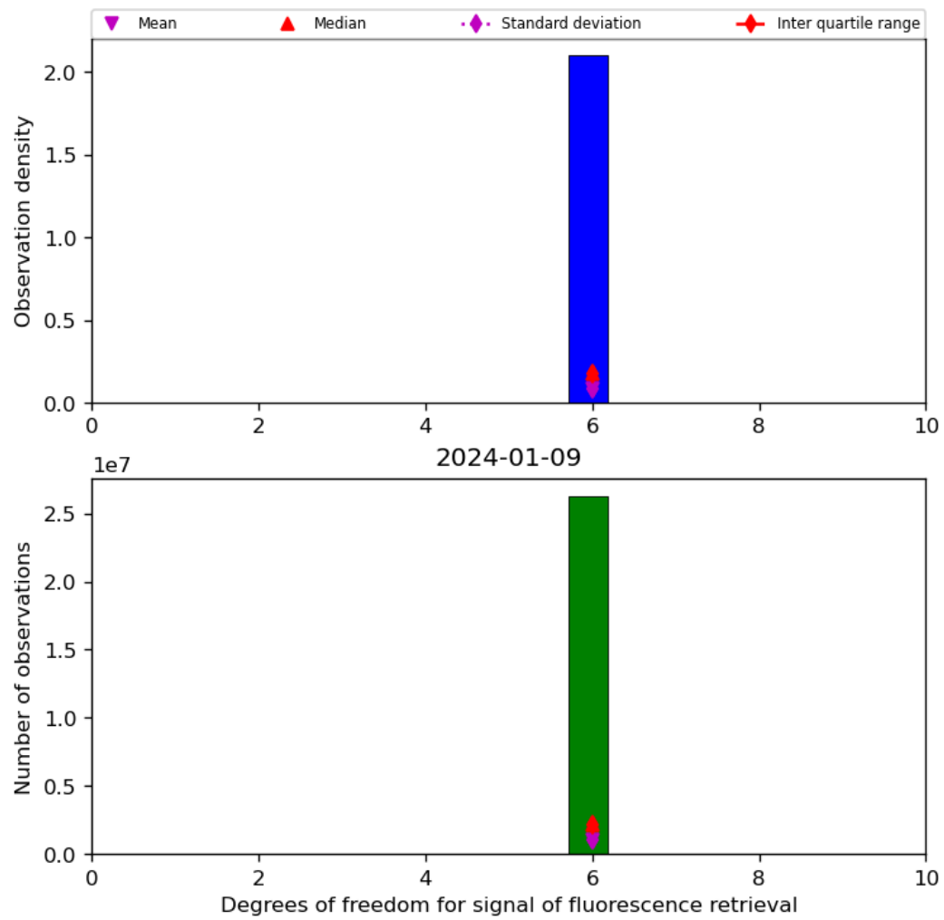
Figure 43: Histogram of “Degrees of freedom for signal of fluorescence retrieval” for 2024-01-08 to 2024-01-10
