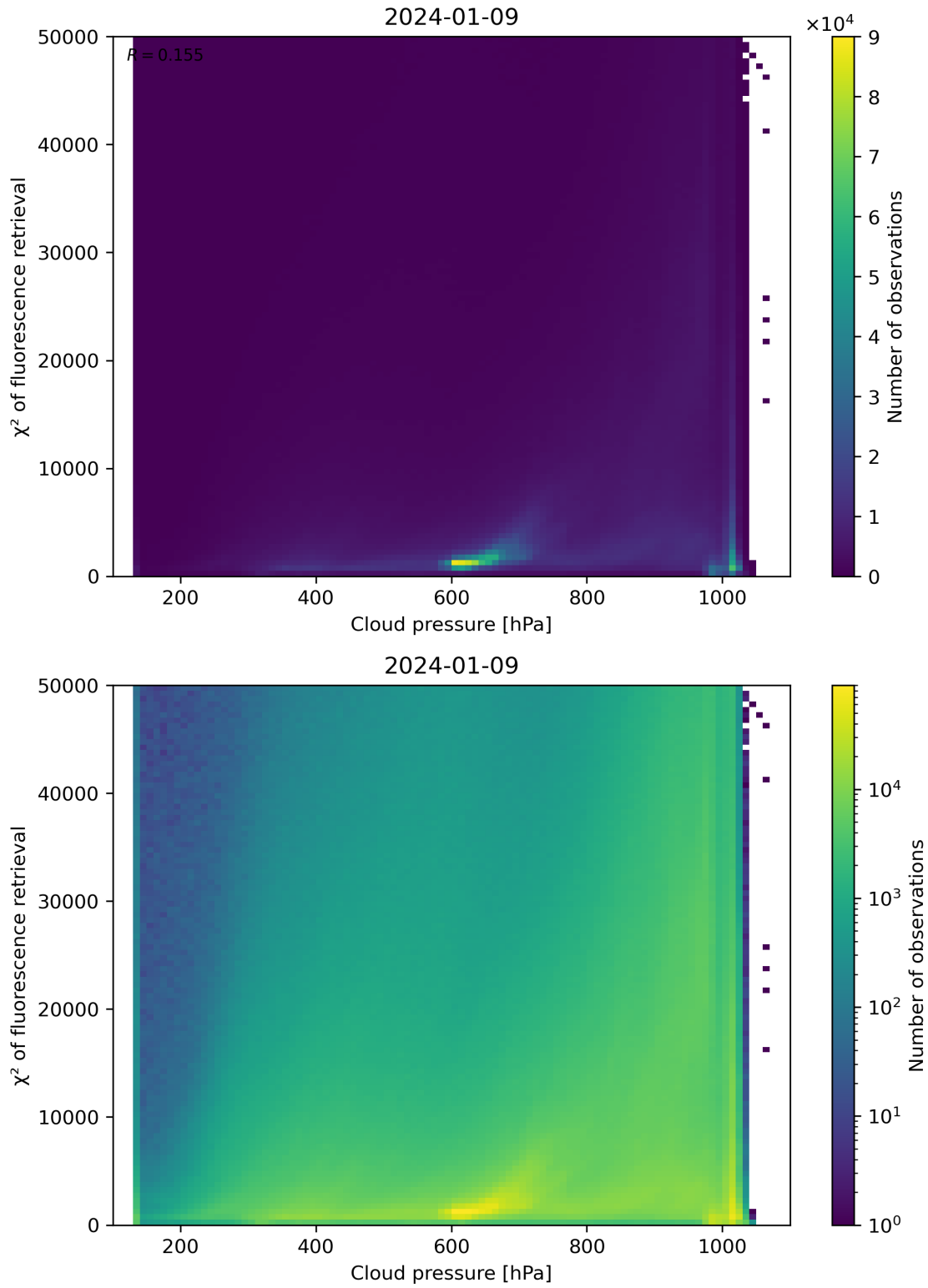
Figure 78: Scatter density plot of “Cloud pressure” against “ \chi^2 of fluorescence retrieval” for 2024-01-08 to 2024-01-10.
