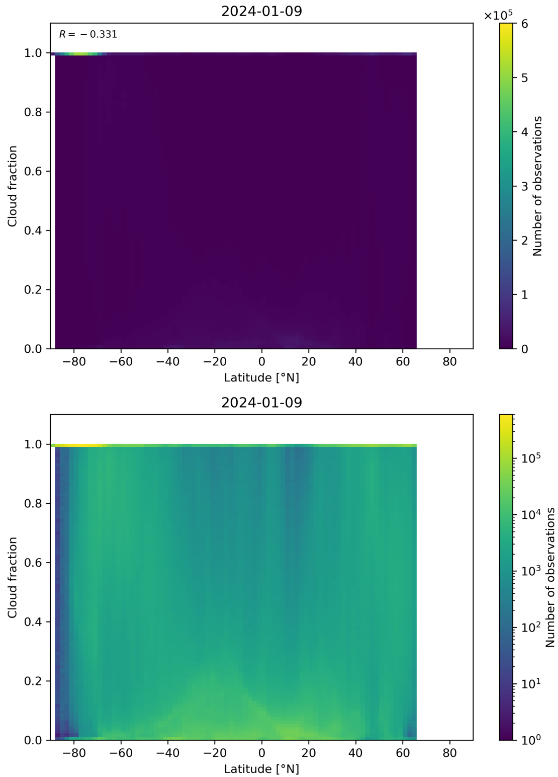
Figure 90: Scatter density plot of “Latitude” against “Cloud fraction” for 2024-01-08 to 2024-01-10.
