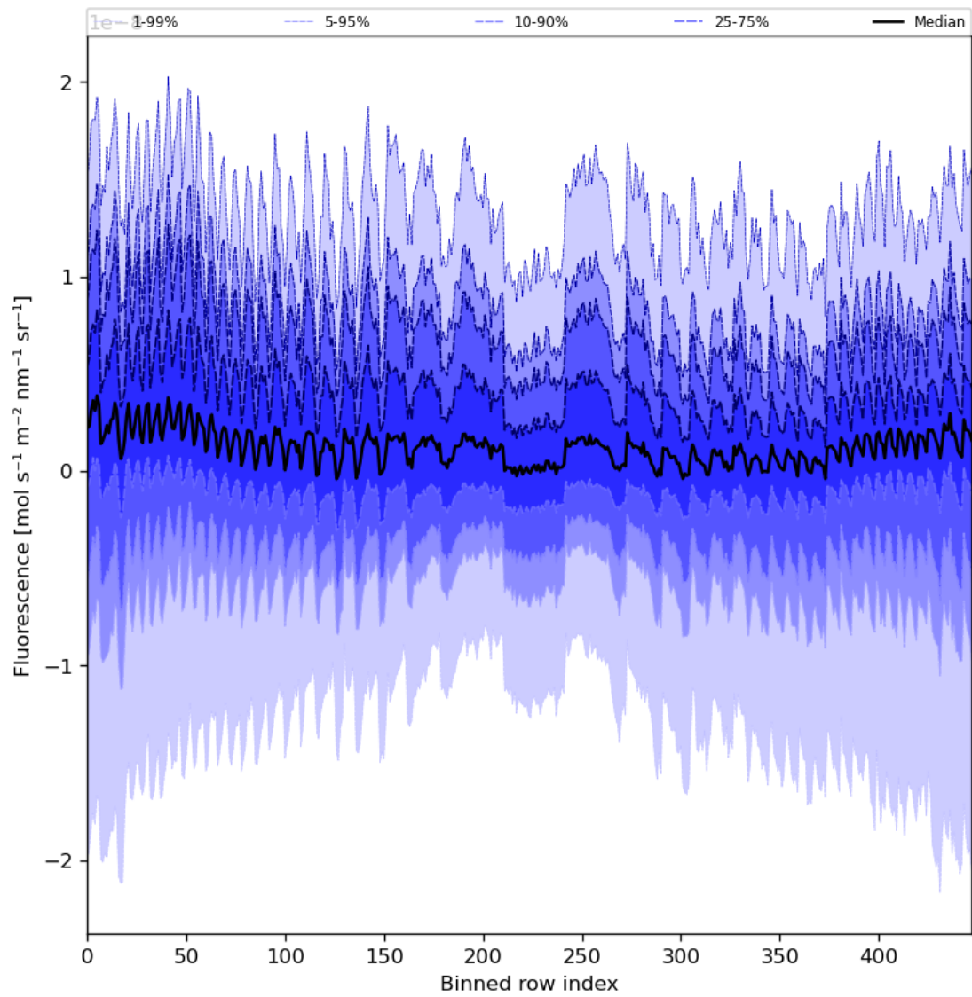
Figure 57: Along track statistics of “Fluorescence” for 2024-01-08 to 2024-01-10
