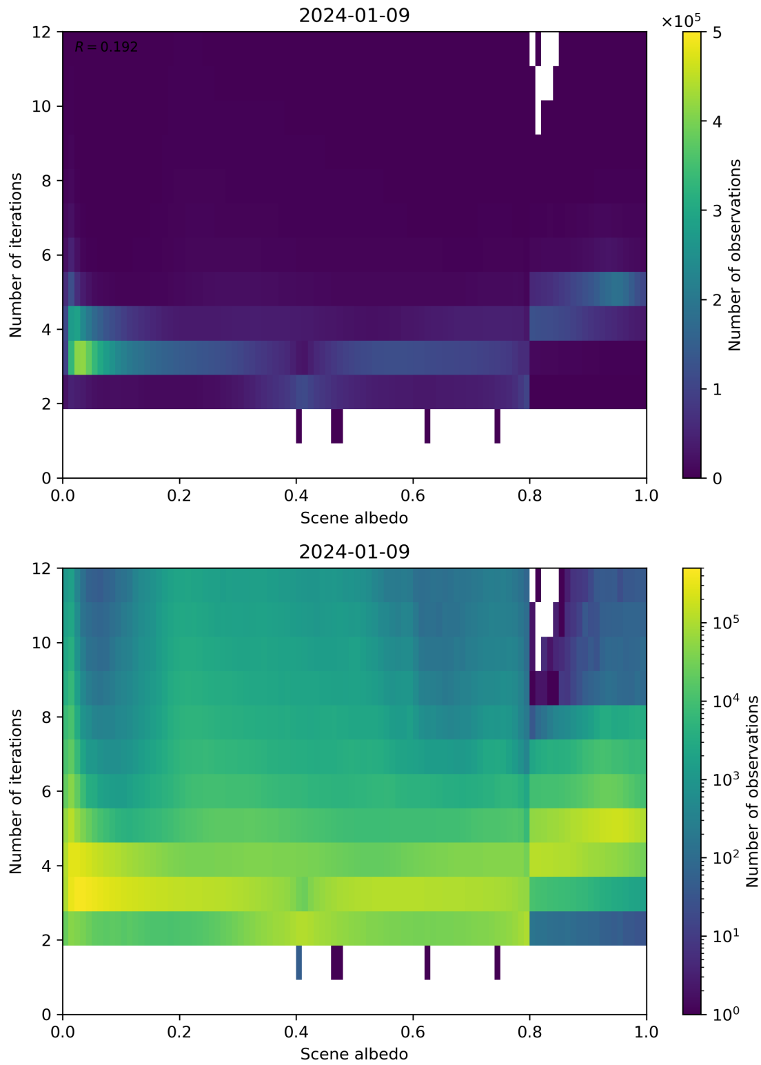
Figure 105: Scatter density plot of “Scene albedo” against “Number of iterations” for 2024-01-08 to 2024-01-10.
