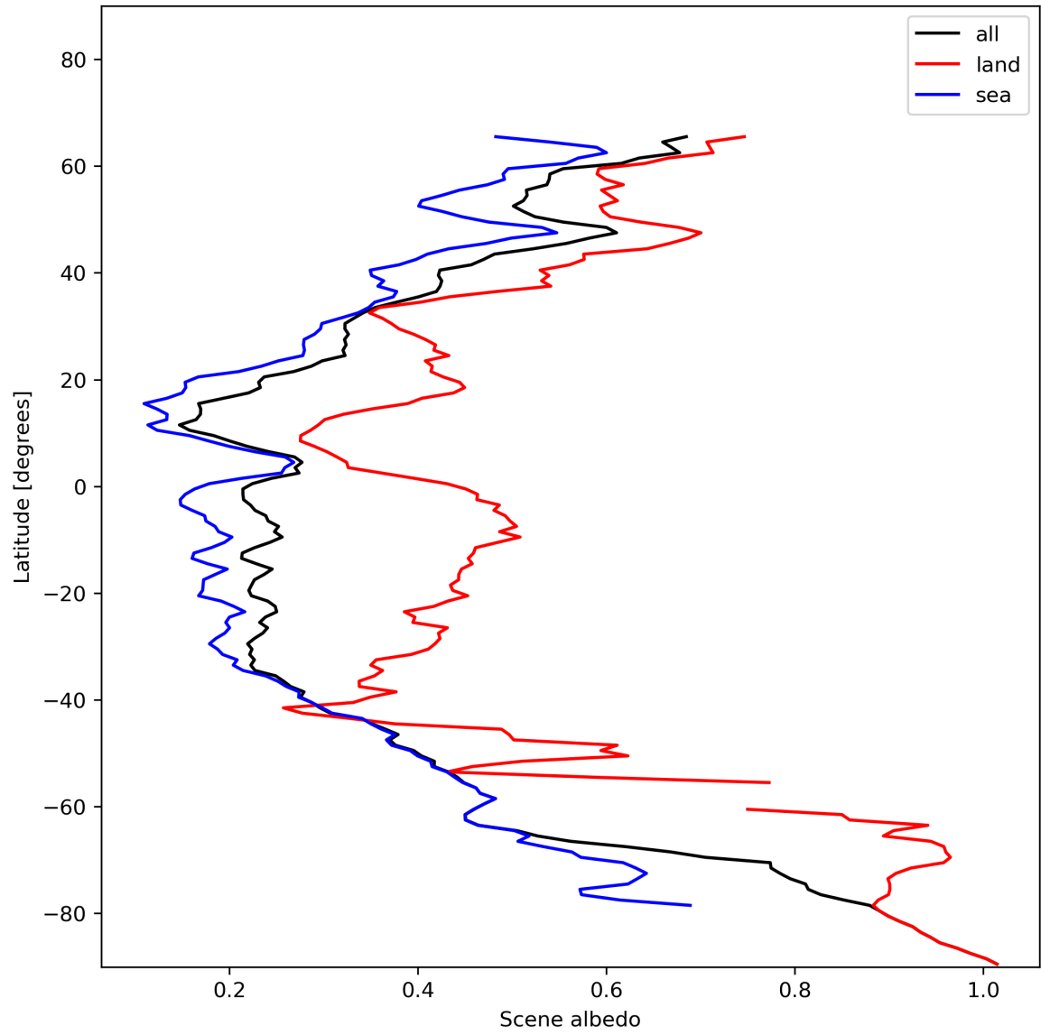
Figure 17: Zonal average of "Scene albedo" for 2024-01-08 to 2024-01-10.
