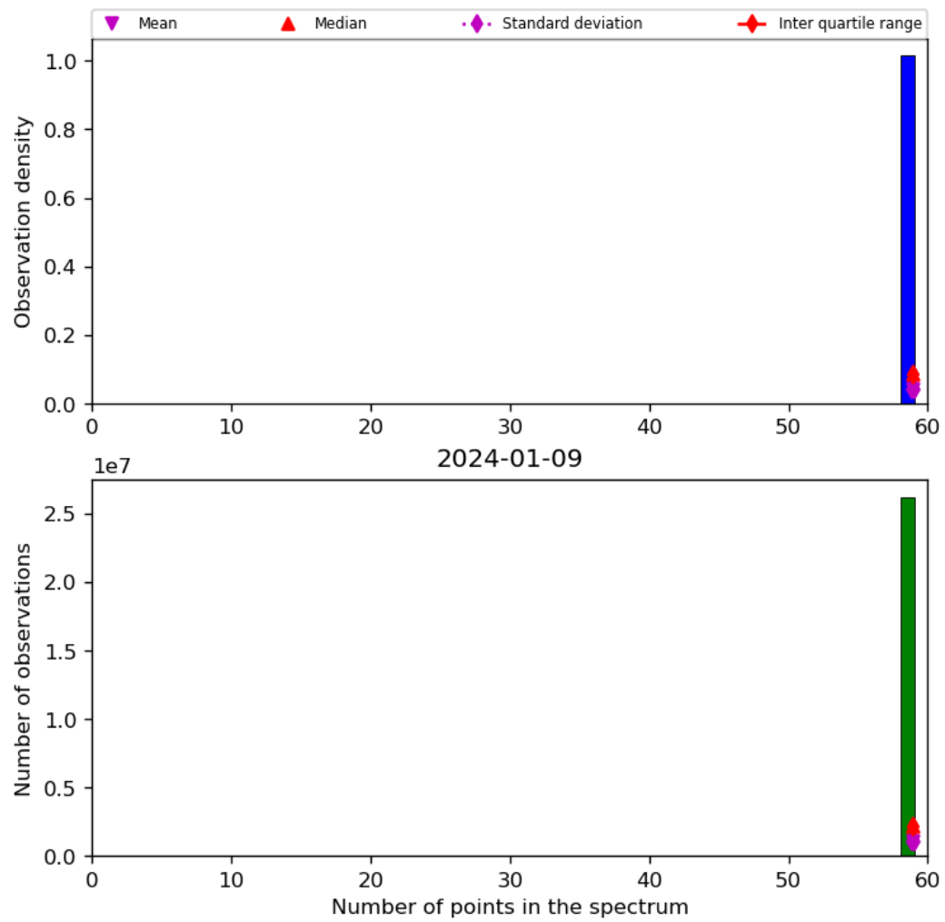
Figure 44: Histogram of “Number of points in the spectrum” for 2024-01-08 to 2024-01-10
