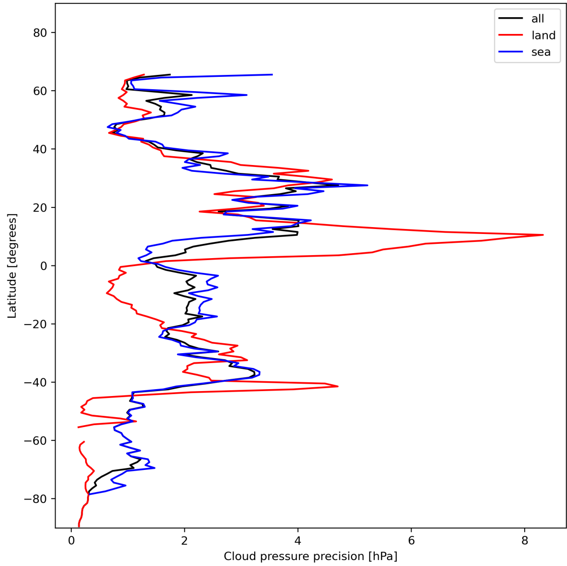
Figure 14: Zonal average of “Cloud pressure precision” for 2024-01-08 to 2024-01-10.
