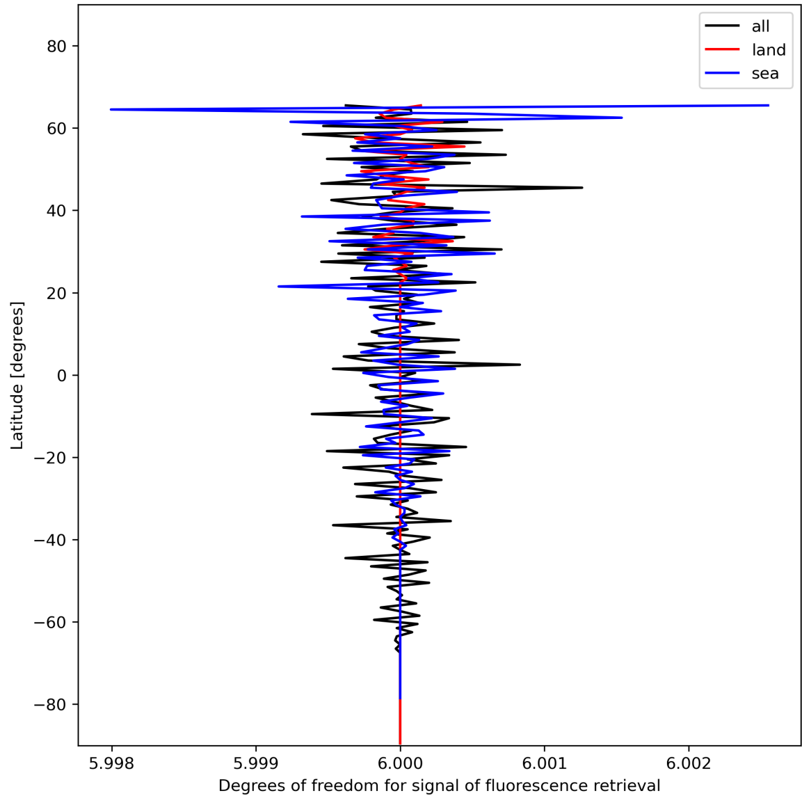
Figure 26: Zonal average of “Degrees of freedom for signal of fluorescence retrieval” for 2024-01-08 to 2024-01-10.
