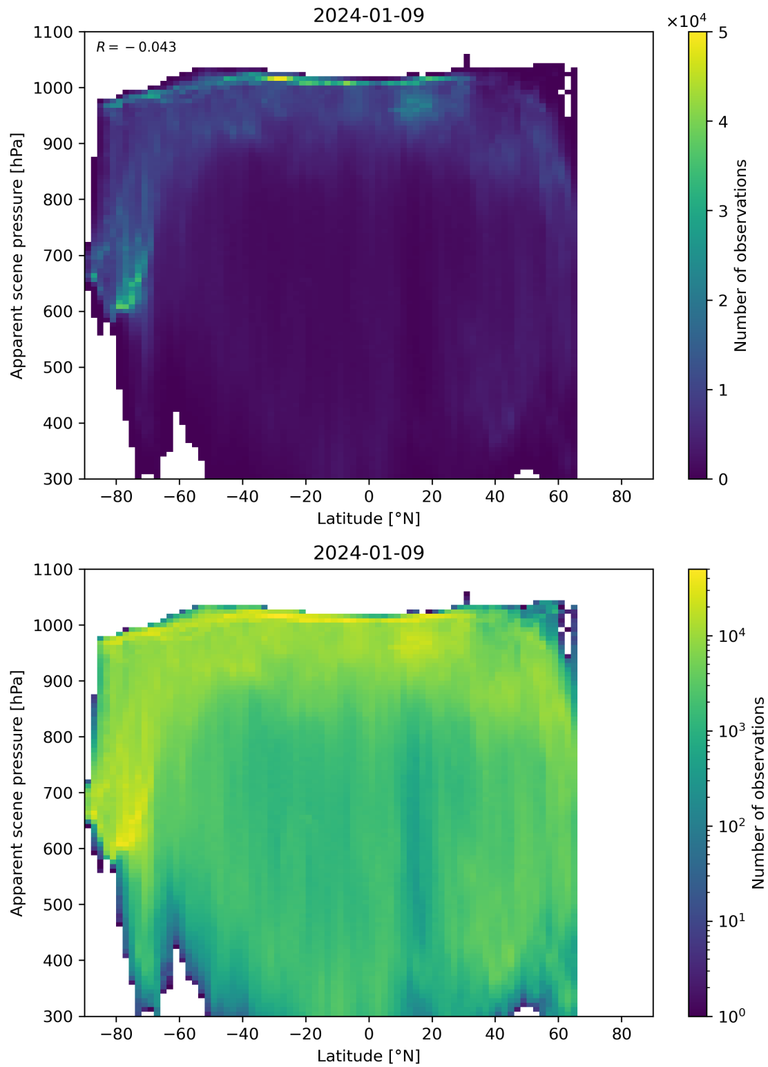
Figure 88: Scatter density plot of “Latitude” against “Apparent scene pressure” for 2024-01-08 to 2024-01-10.
