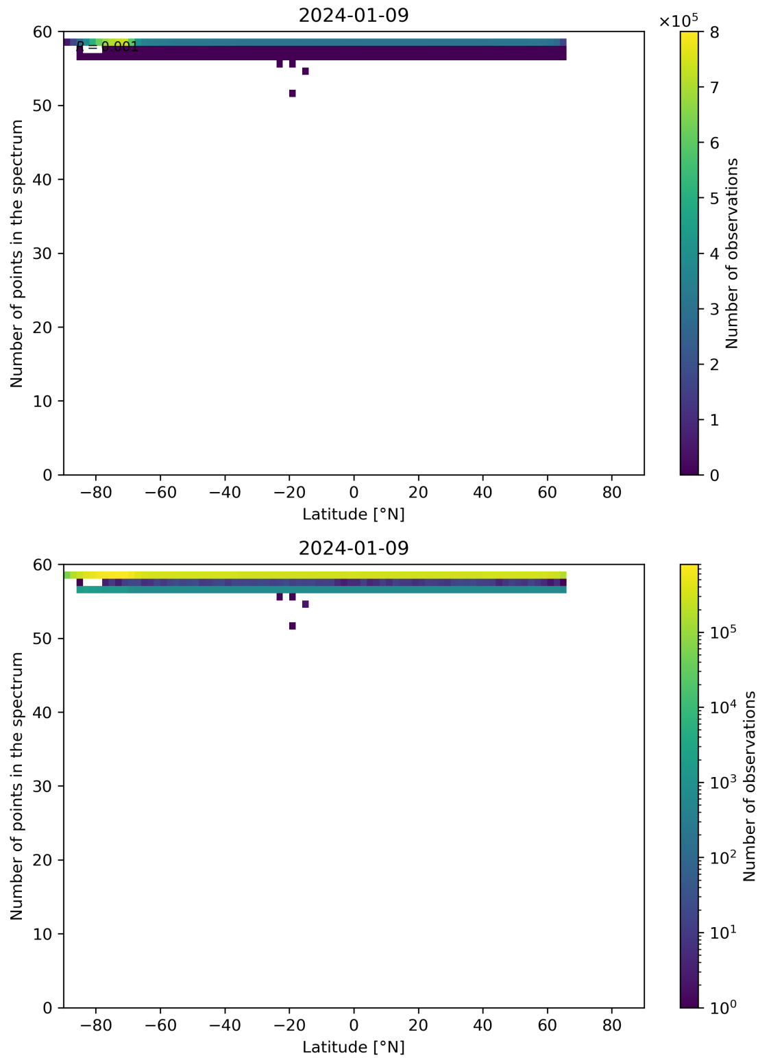
Figure 94: Scatter density plot of “Latitude” against “Number of points in the spectrum” for 2024-01-08 to 2024-01-10.
