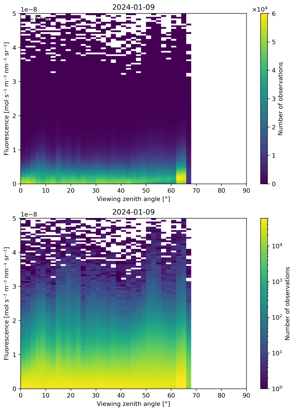
Figure 122: Scatter density plot of “Viewing zenith angle” against “Fluorescence” for 2024-01-08 to 2024-01-10.
