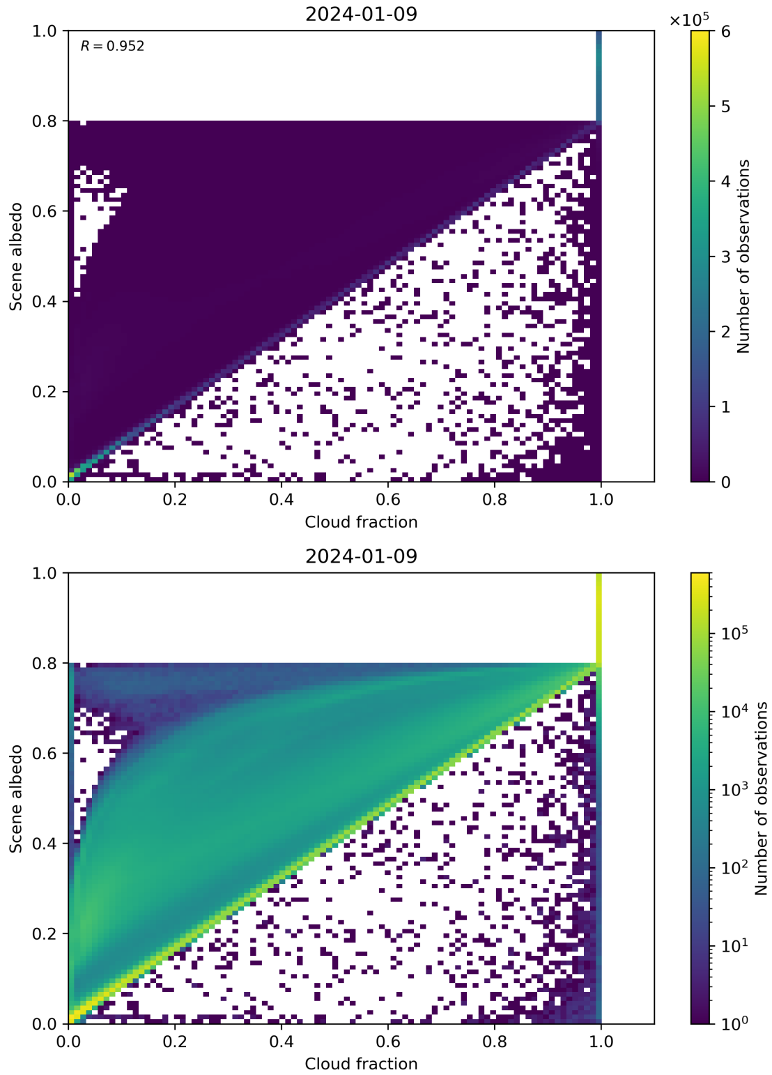
Figure 75: Scatter density plot of “Cloud fraction” against “Scene albedo” for 2024-01-08 to 2024-01-10.
