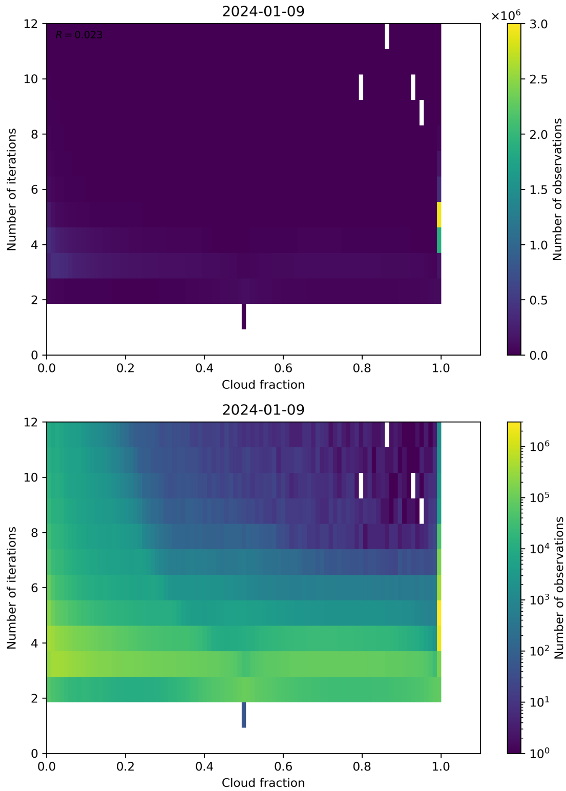
Figure 73: Scatter density plot of “Cloud fraction” against “Number of iterations” for 2024-01-08 to 2024-01-10.
