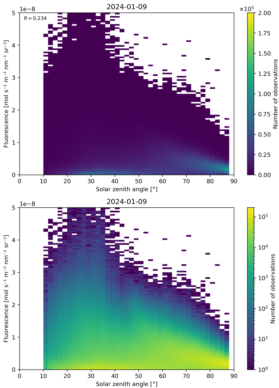
Figure 112: Scatter density plot of “Solar zenith angle” against “Fluorescence” for 2024-01-08 to 2024-01-10.
