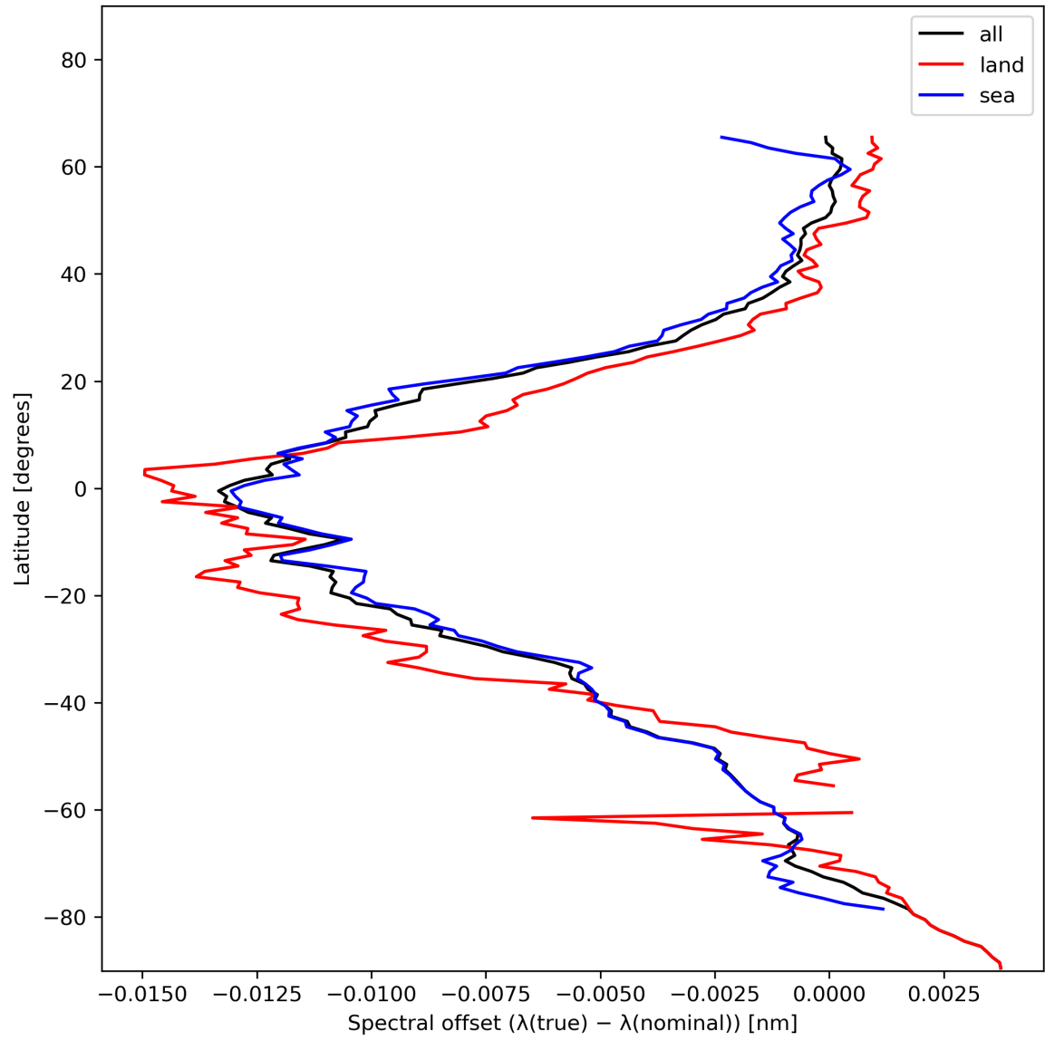
Figure 28: Zonal average of “Spectral offset ( \lambda(\text{true}) - \lambda(\text{nominal}) )” for 2024-01-08 to 2024-01-10.
