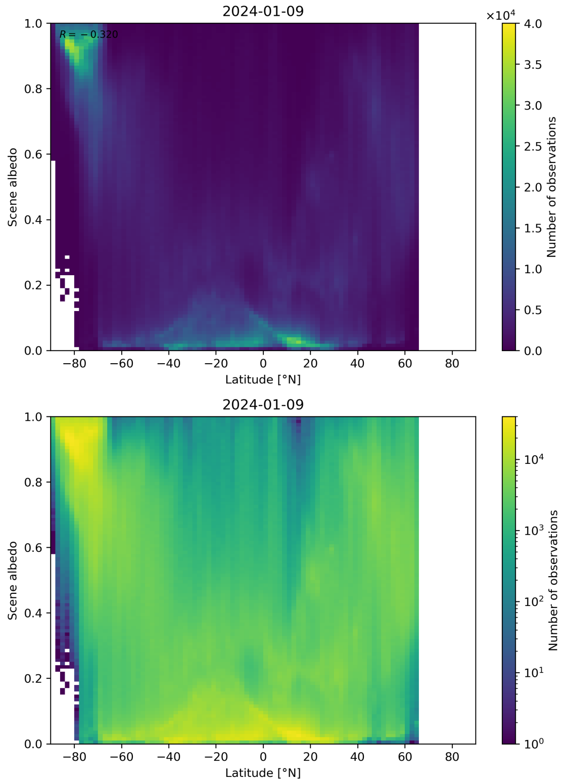
Figure 95: Scatter density plot of “Latitude” against “Scene albedo” for 2024-01-08 to 2024-01-10.
