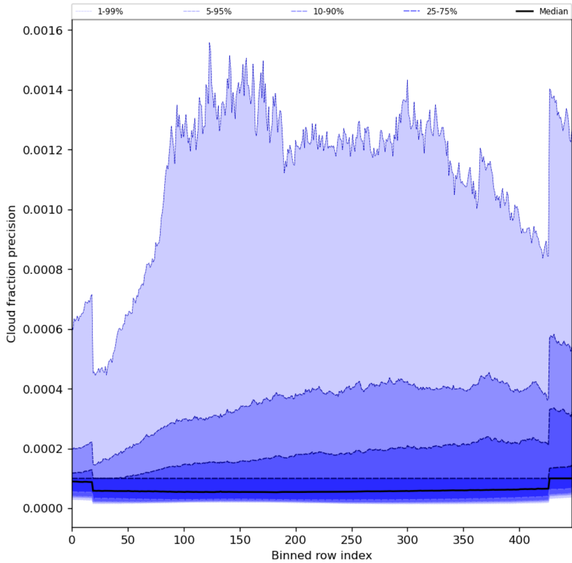
Figure 50: Along track statistics of “Cloud fraction precision” for 2024-01-08 to 2024-01-10
