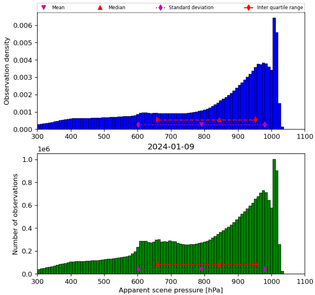
Figure 36: Histogram of “Apparent scene pressure” for 2024-01-08 to 2024-01-10
