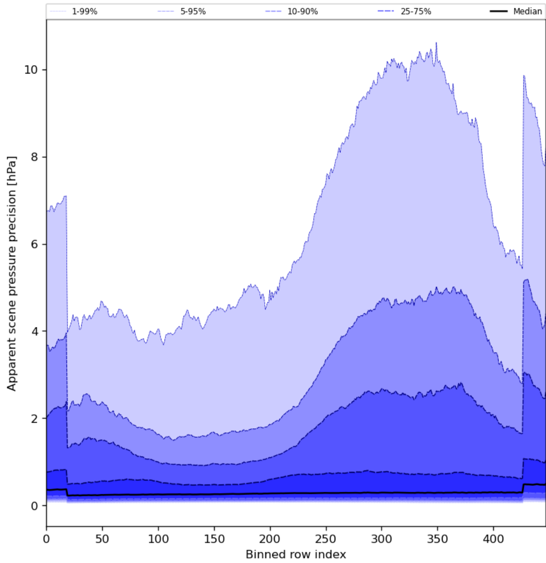
Figure 54: Along track statistics of “Apparent scene pressure precision” for 2024-01-08 to 2024-01-10
