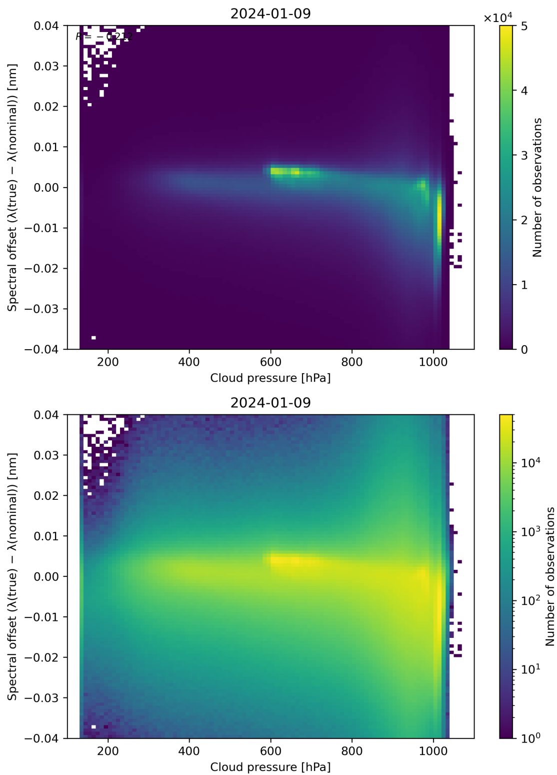
Figure 84: Scatter density plot of “Cloud pressure” against “Spectral offset ( \lambda(\text{true}) - \lambda(\text{nominal}) )” for 2024-01-08 to 2024-01-10.
