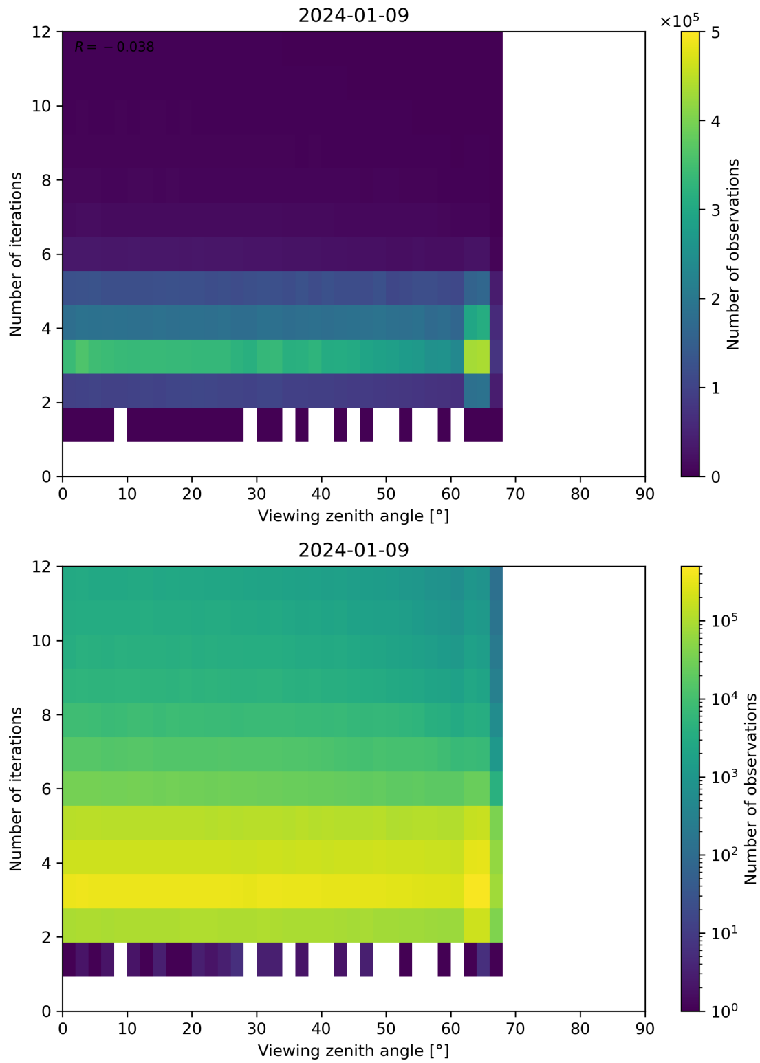
Figure 124: Scatter density plot of “Viewing zenith angle” against “Number of iterations” for 2024-01-08 to 2024-01-10.
