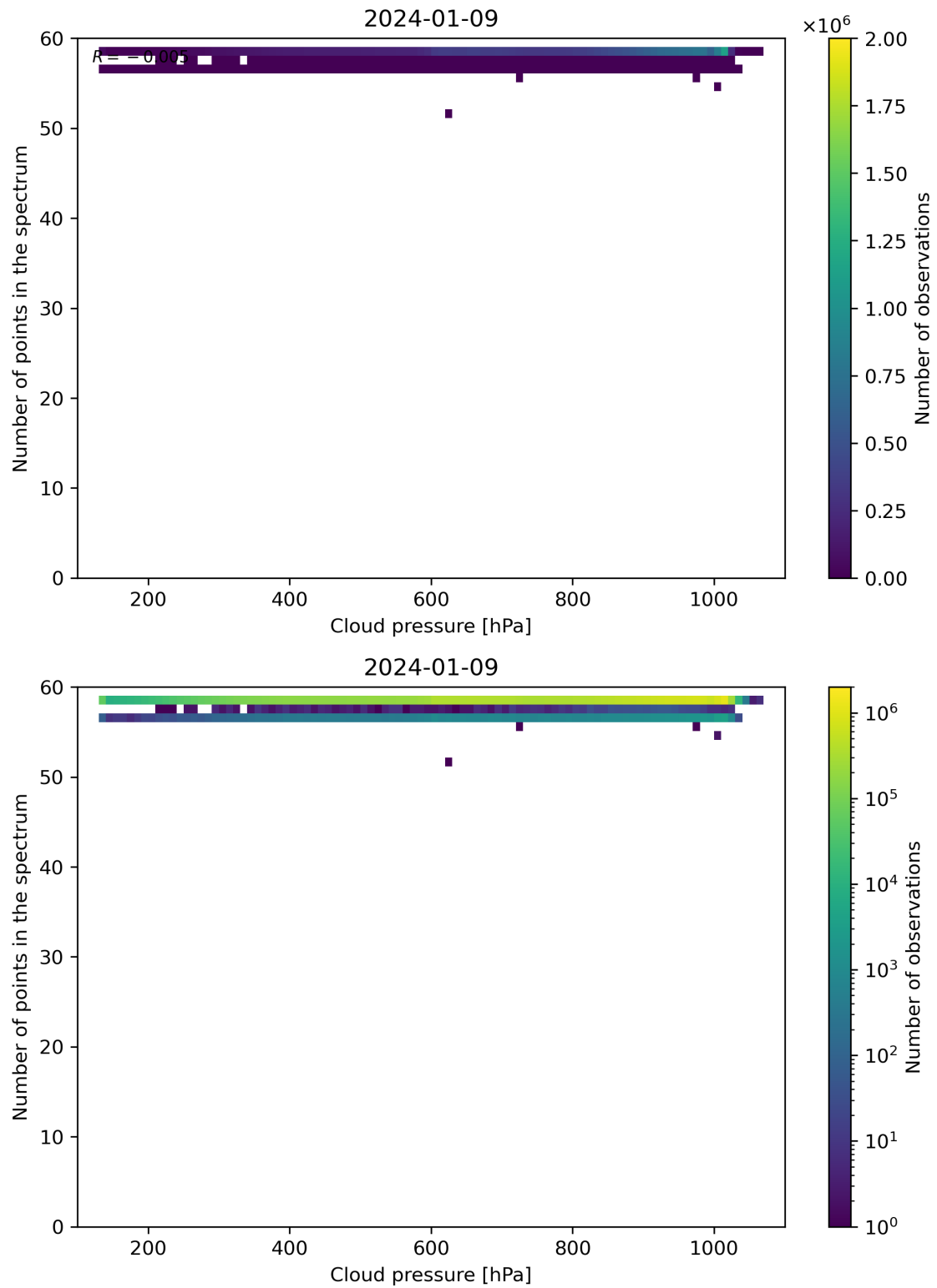
Figure 82: Scatter density plot of “Cloud pressure” against “Number of points in the spectrum” for 2024-01-08 to 2024-01-10.
