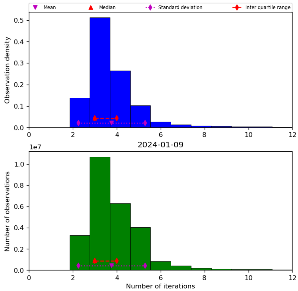
Figure 39: Histogram of “Number of iterations” for 2024-01-08 to 2024-01-10
