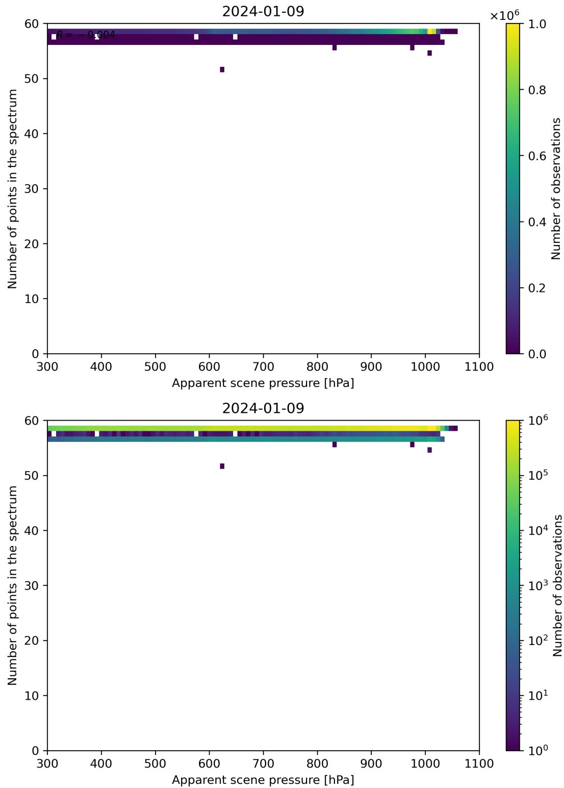
Figure 66: Scatter density plot of “Apparent scene pressure” against “Number of points in the spectrum” for 2024-01-08 to 2024-01-10.
