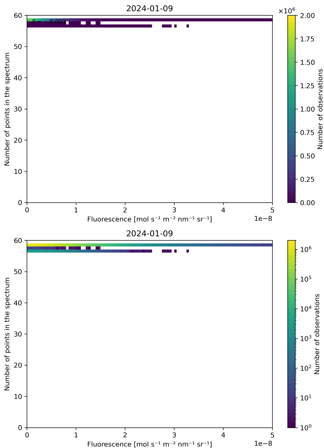
Figure 86: Scatter density plot of “Fluorescence” against “Number of points in the spectrum” for 2024-01-08 to 2024-01-10.
