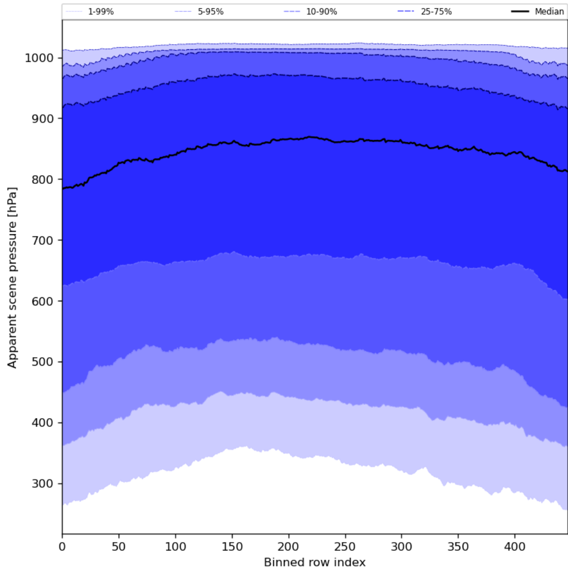
Figure 53: Along track statistics of “Apparent scene pressure” for 2024-01-08 to 2024-01-10
