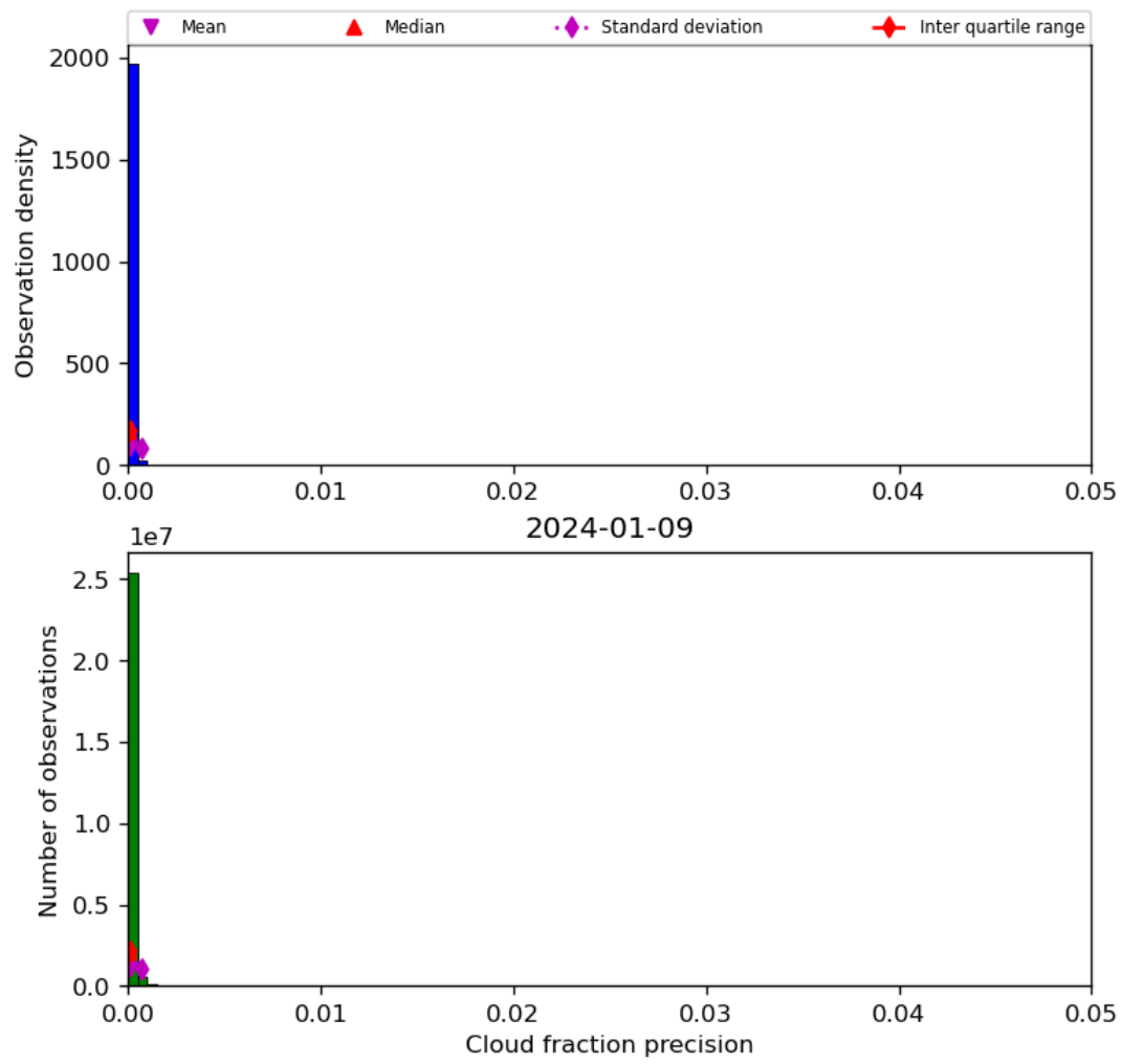
Figure 33: Histogram of “Cloud fraction precision” for 2024-01-08 to 2024-01-10
