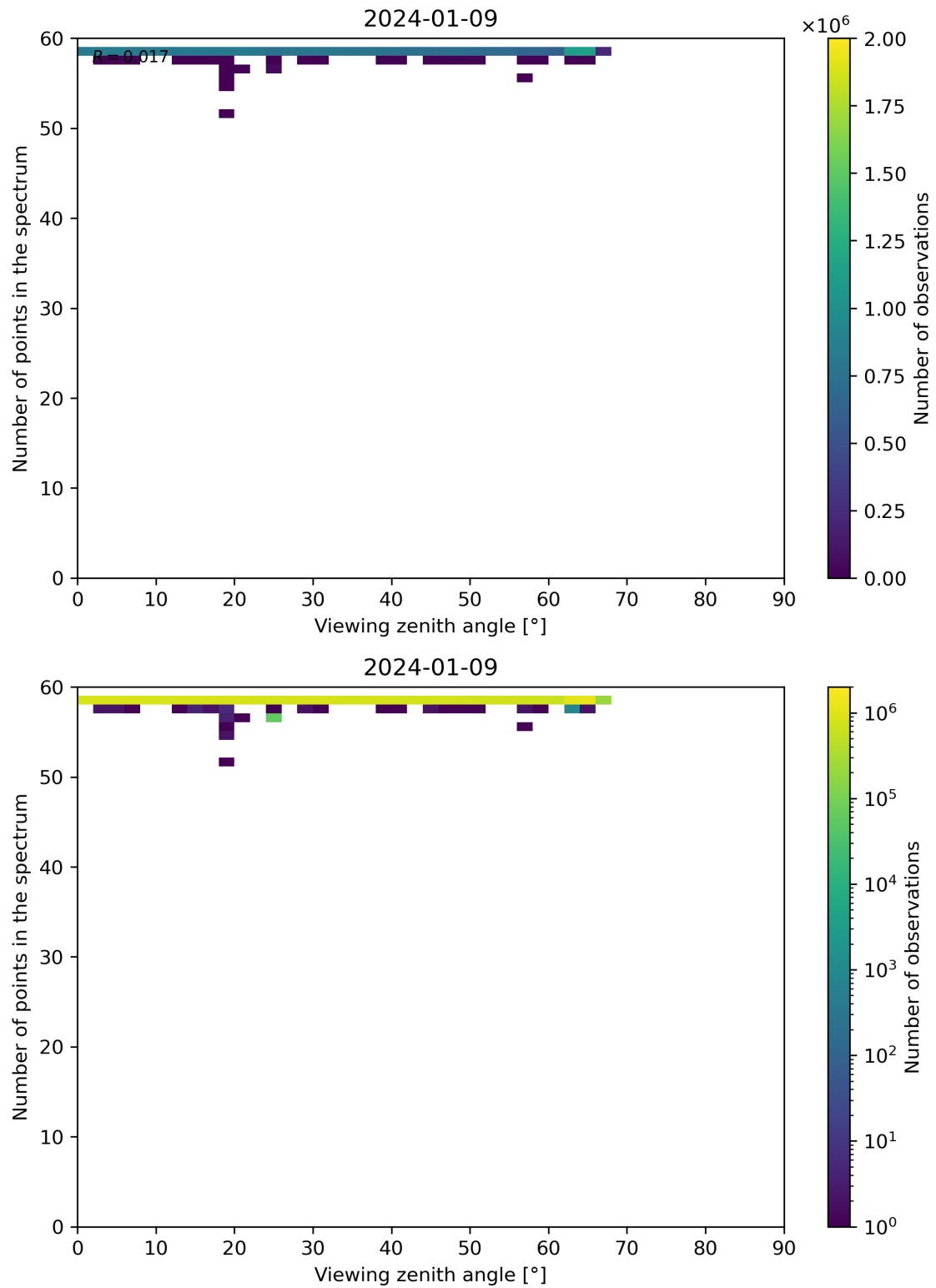
Figure 125: Scatter density plot of “Viewing zenith angle” against “Number of points in the spectrum” for 2024-01-08 to 2024-01-10.
