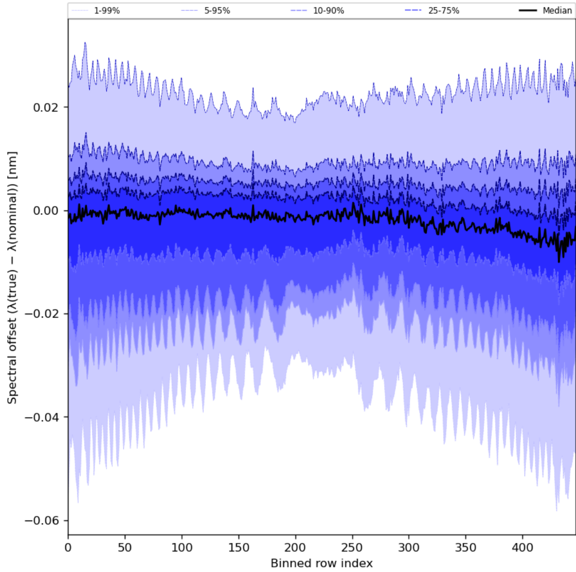
Figure 62: Along track statistics of “Spectral offset ( \lambda(\text{true}) - \lambda(\text{nominal}) )” for 2024-01-08 to 2024-01-10
