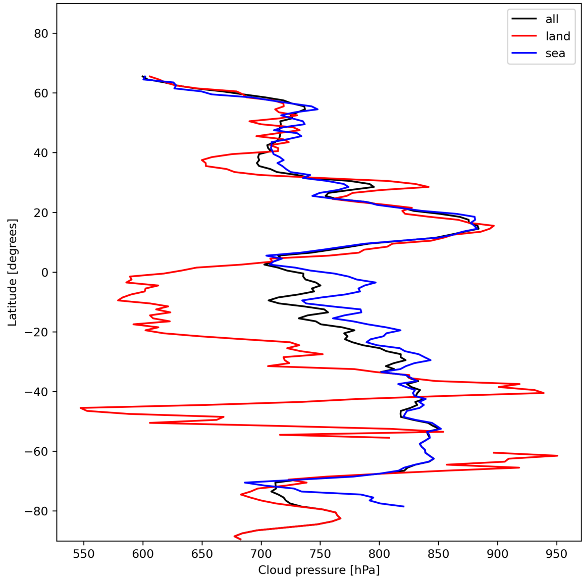
Figure 13: Zonal average of “Cloud pressure” for 2024-01-08 to 2024-01-10.
