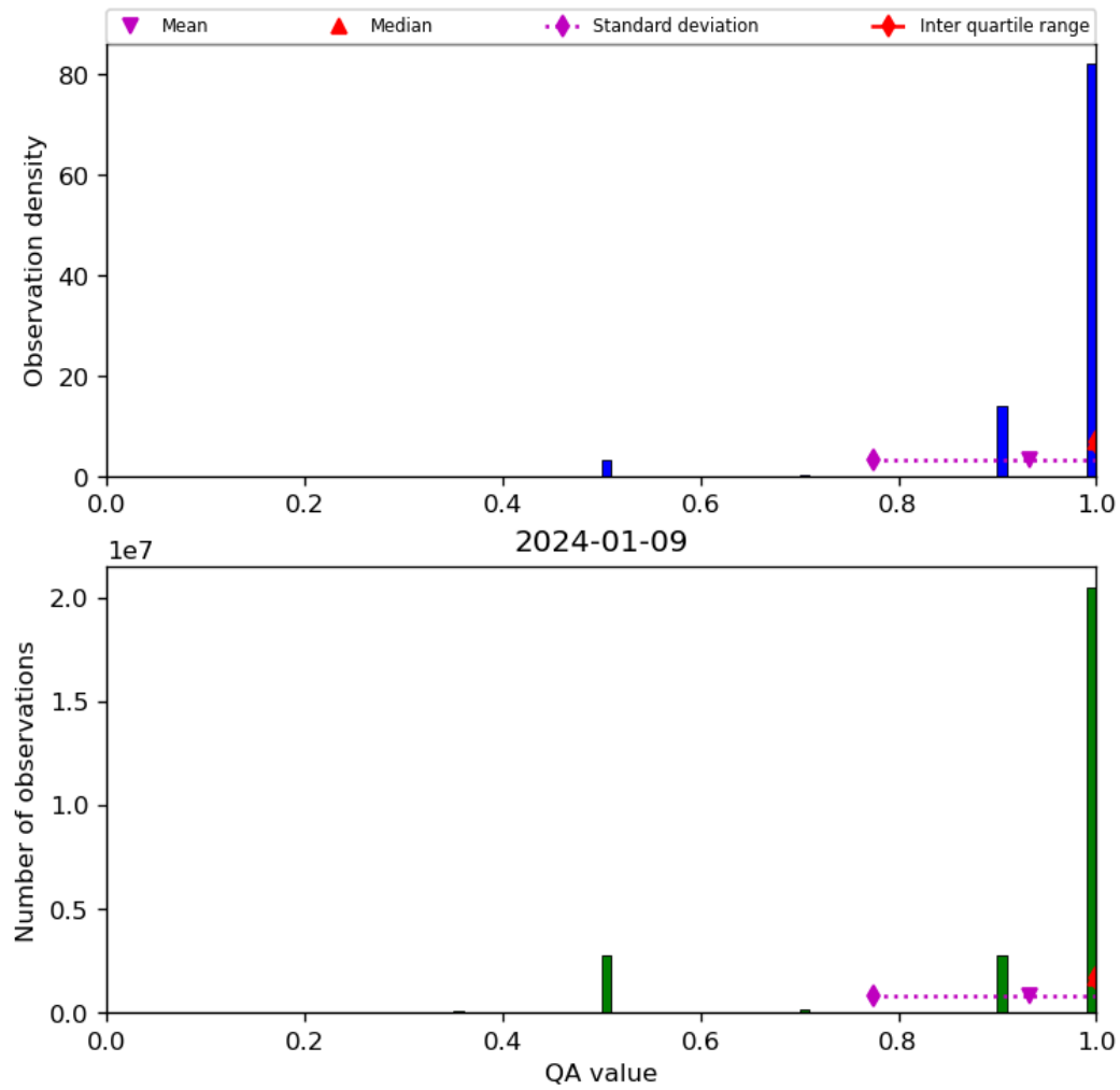
Figure 29: Histogram of “QA value” for 2024-01-08 to 2024-01-10
