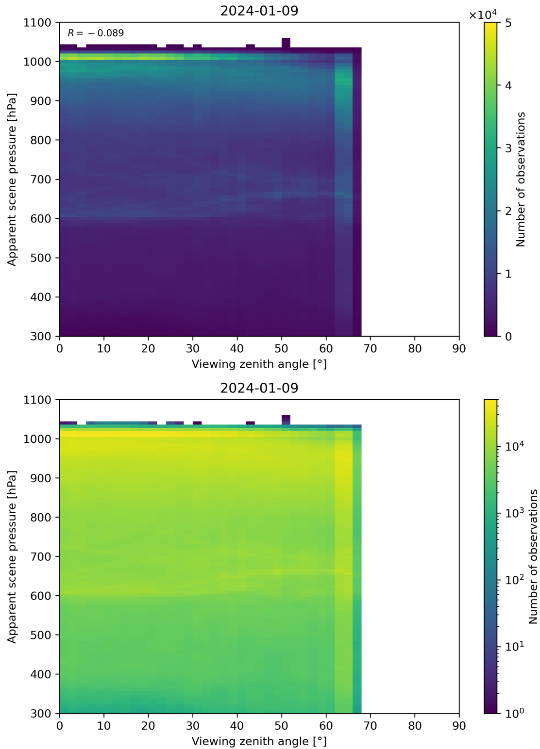
Figure 118: Scatter density plot of “Viewing zenith angle” against “Apparent scene pressure” for 2024-01-08 to 2024-01-10.
