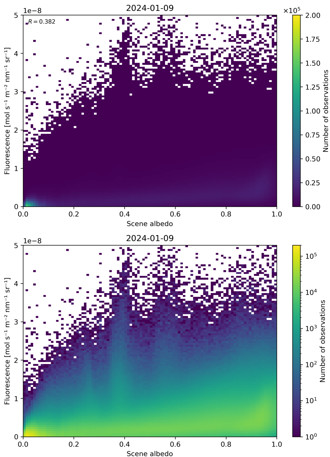
Figure 104: Scatter density plot of “Scene albedo” against “Fluorescence” for 2024-01-08 to 2024-01-10.
