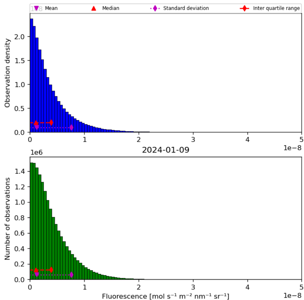
Figure 40: Histogram of “Fluorescence” for 2024-01-08 to 2024-01-10
