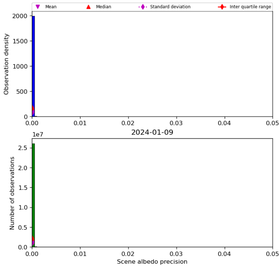
Figure 35: Histogram of “Scene albedo precision” for 2024-01-08 to 2024-01-10
