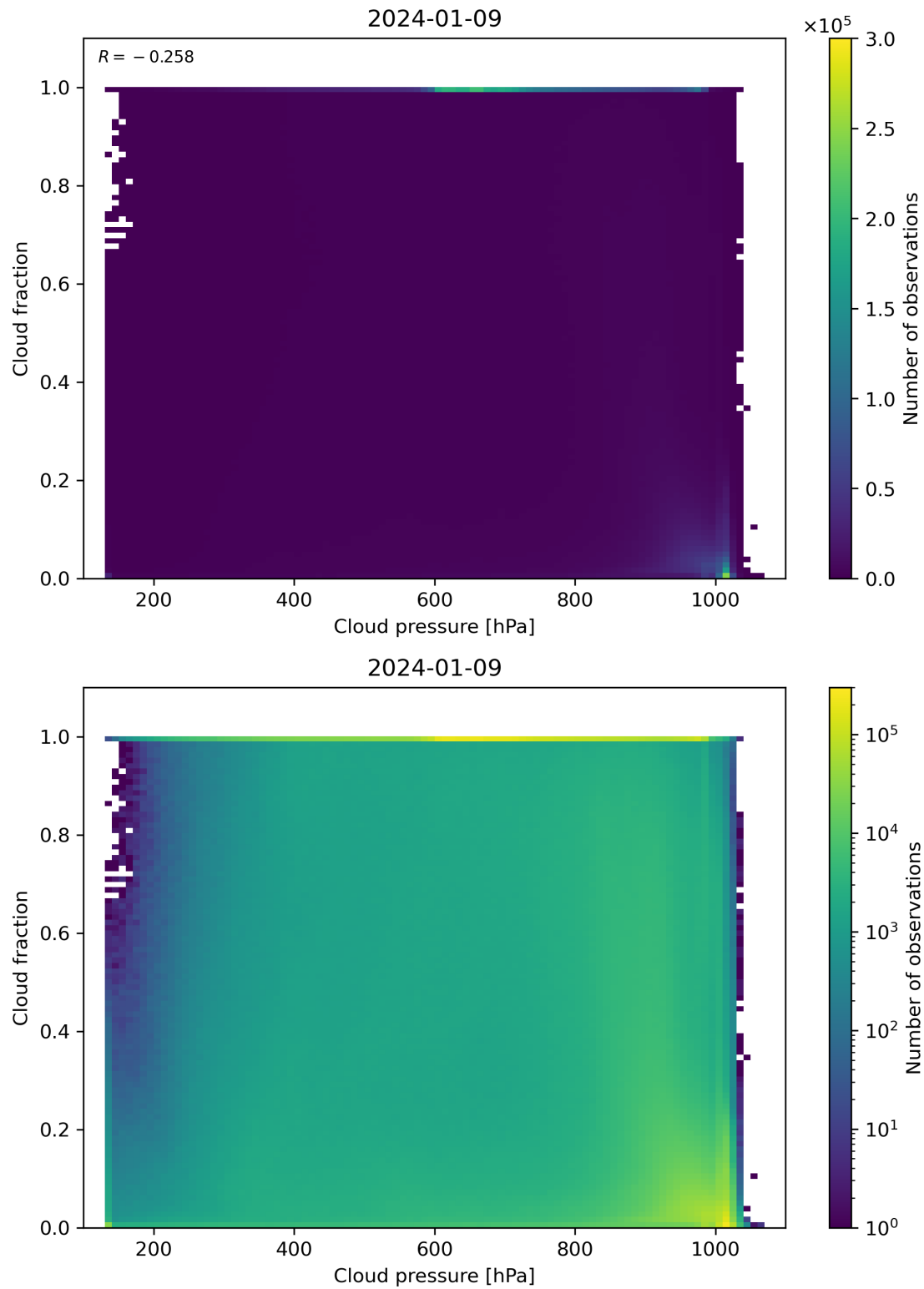
Figure 79: Scatter density plot of “Cloud pressure” against “Cloud fraction” for 2024-01-08 to 2024-01-10.
