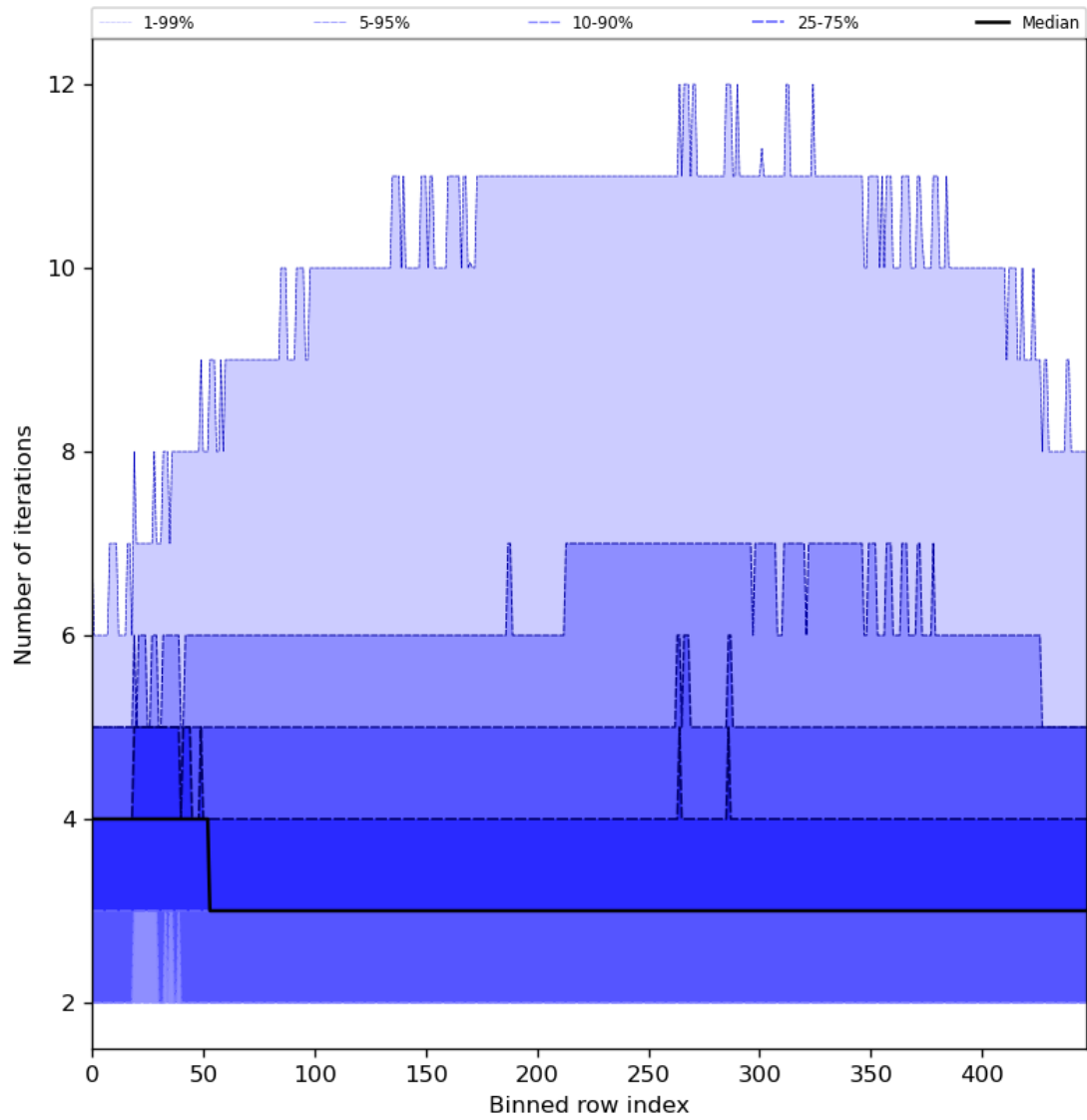
Figure 56: Along track statistics of “Number of iterations” for 2024-01-08 to 2024-01-10
