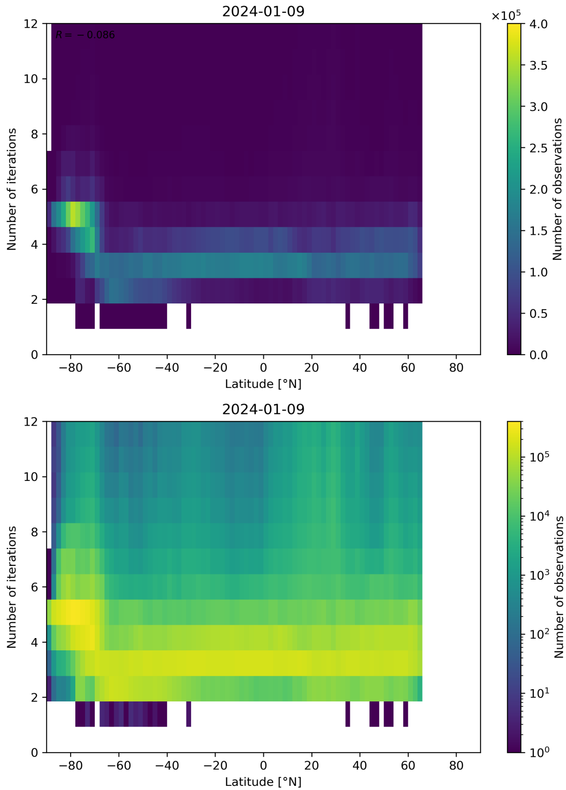
Figure 93: Scatter density plot of “Latitude” against “Number of iterations” for 2024-01-08 to 2024-01-10.
