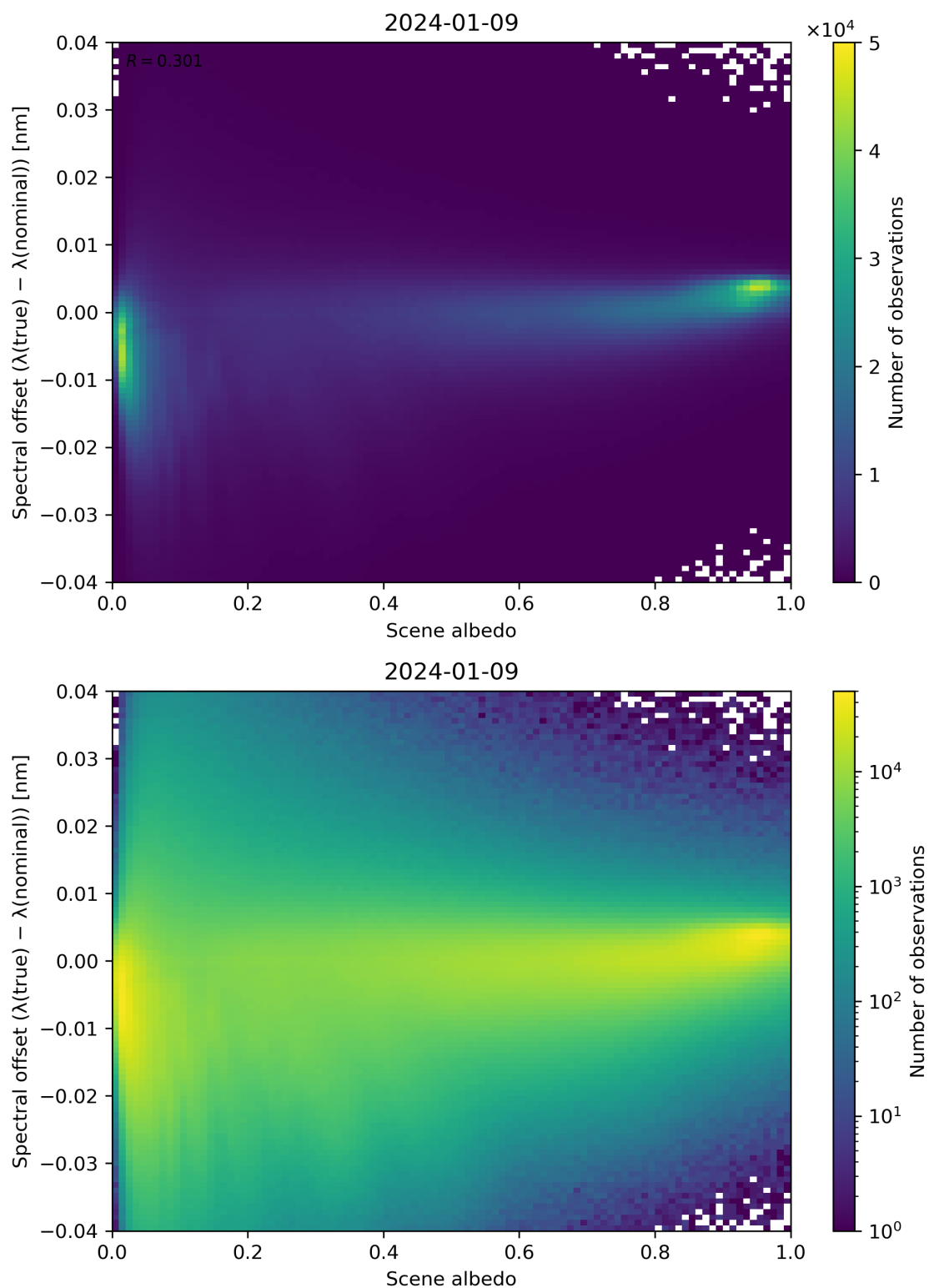
Figure 107: Scatter density plot of “Scene albedo” against “Spectral offset ( \lambda(\text{true}) - \lambda(\text{nominal}) )” for 2024-01-08 to 2024-01-10.
