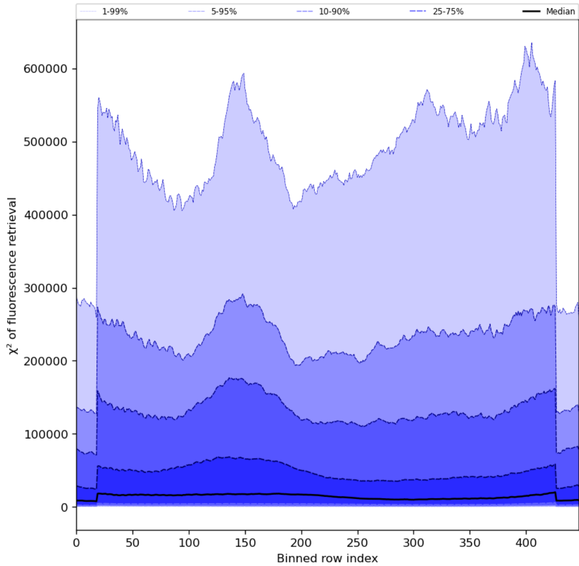
Figure 59: Along track statistics of “ \chi^2 of fluorescence retrieval” for 2024-01-08 to 2024-01-10
