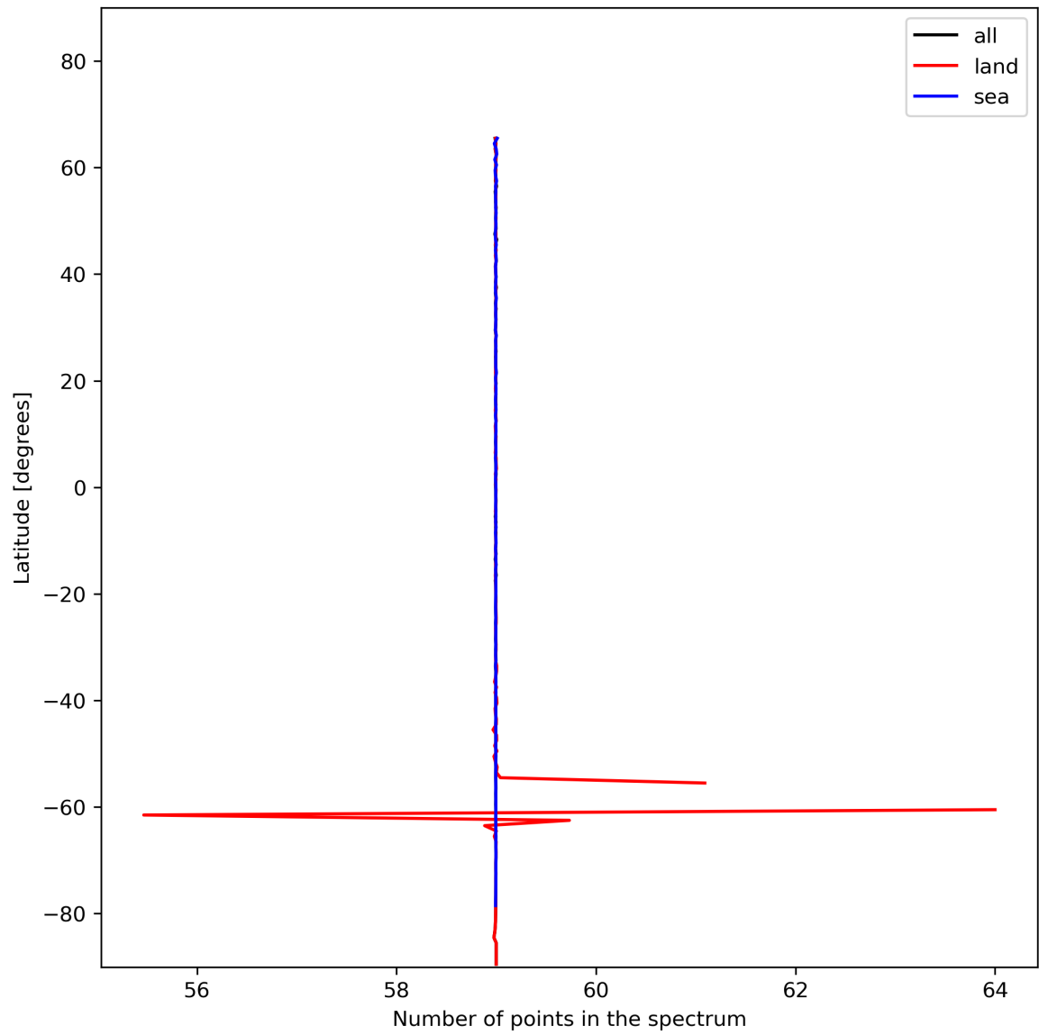
Figure 27: Zonal average of “Number of points in the spectrum” for 2024-01-08 to 2024-01-10.
