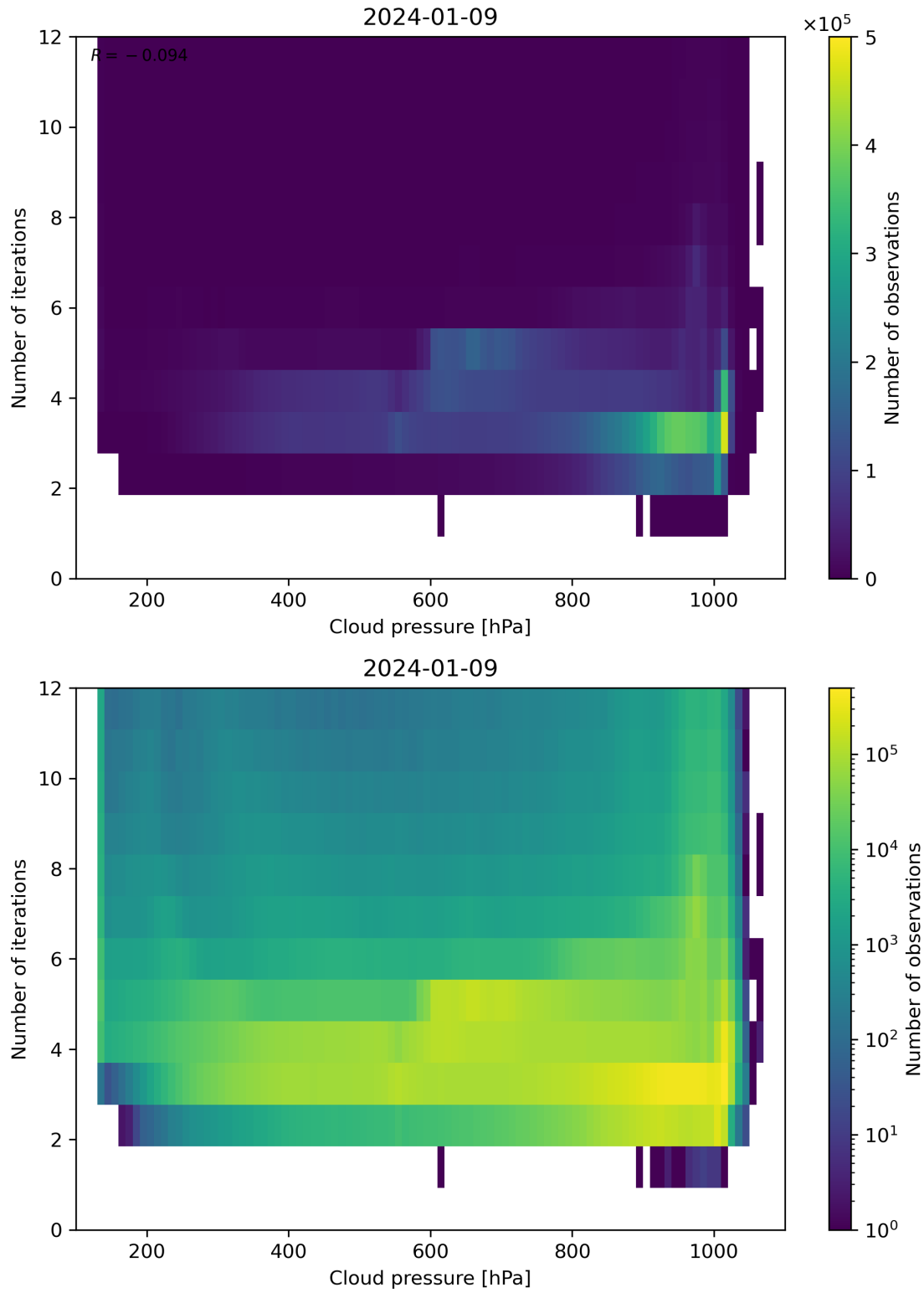
Figure 81: Scatter density plot of “Cloud pressure” against “Number of iterations” for 2024-01-08 to 2024-01-10.
