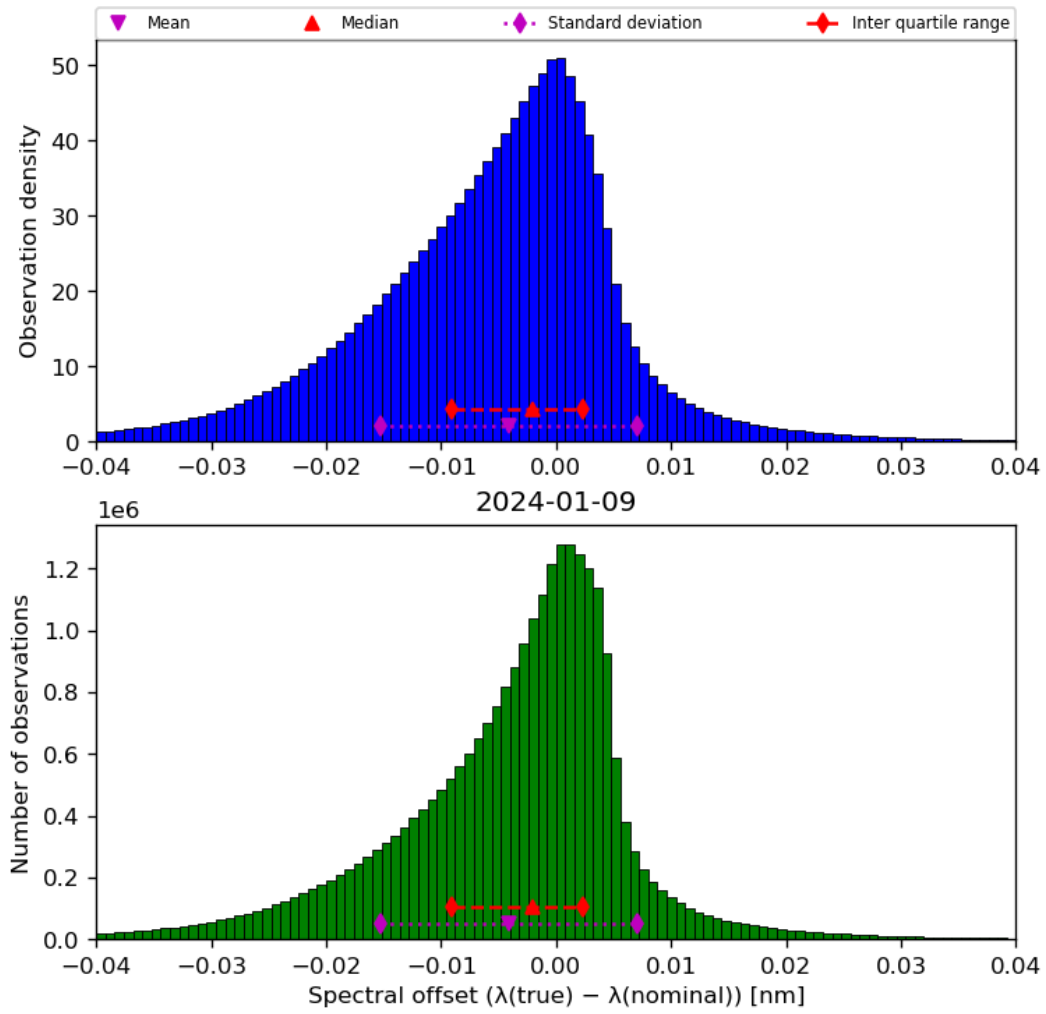
Figure 45: Histogram of “Spectral offset ( \lambda(\text{true}) - \lambda(\text{nominal}) )” for 2024-01-08 to 2024-01-10
