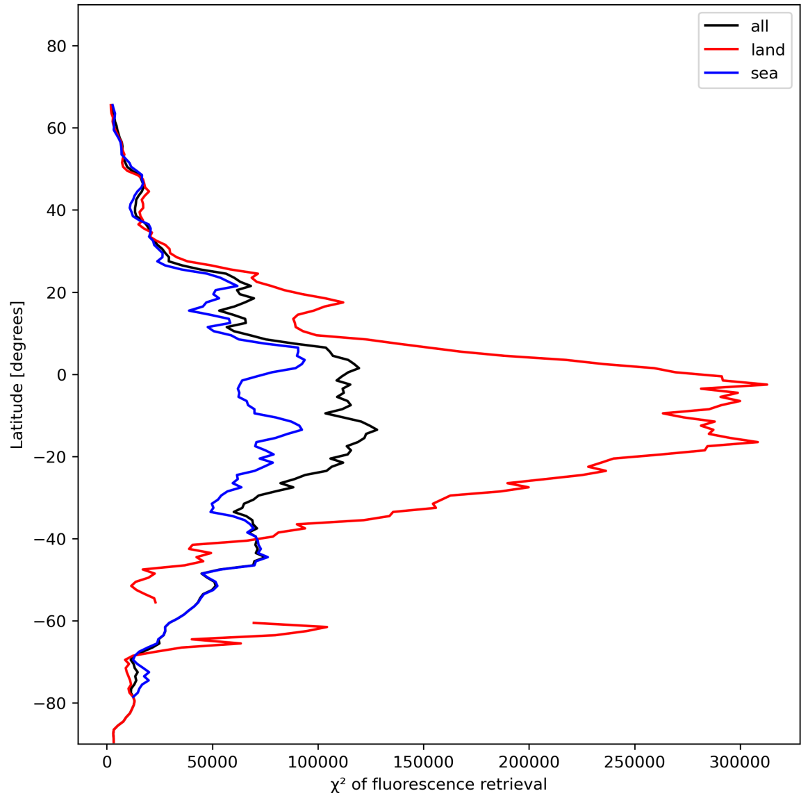
Figure 25: Zonal average of “ \chi^2 of fluorescence retrieval” for 2024-01-08 to 2024-01-10.
