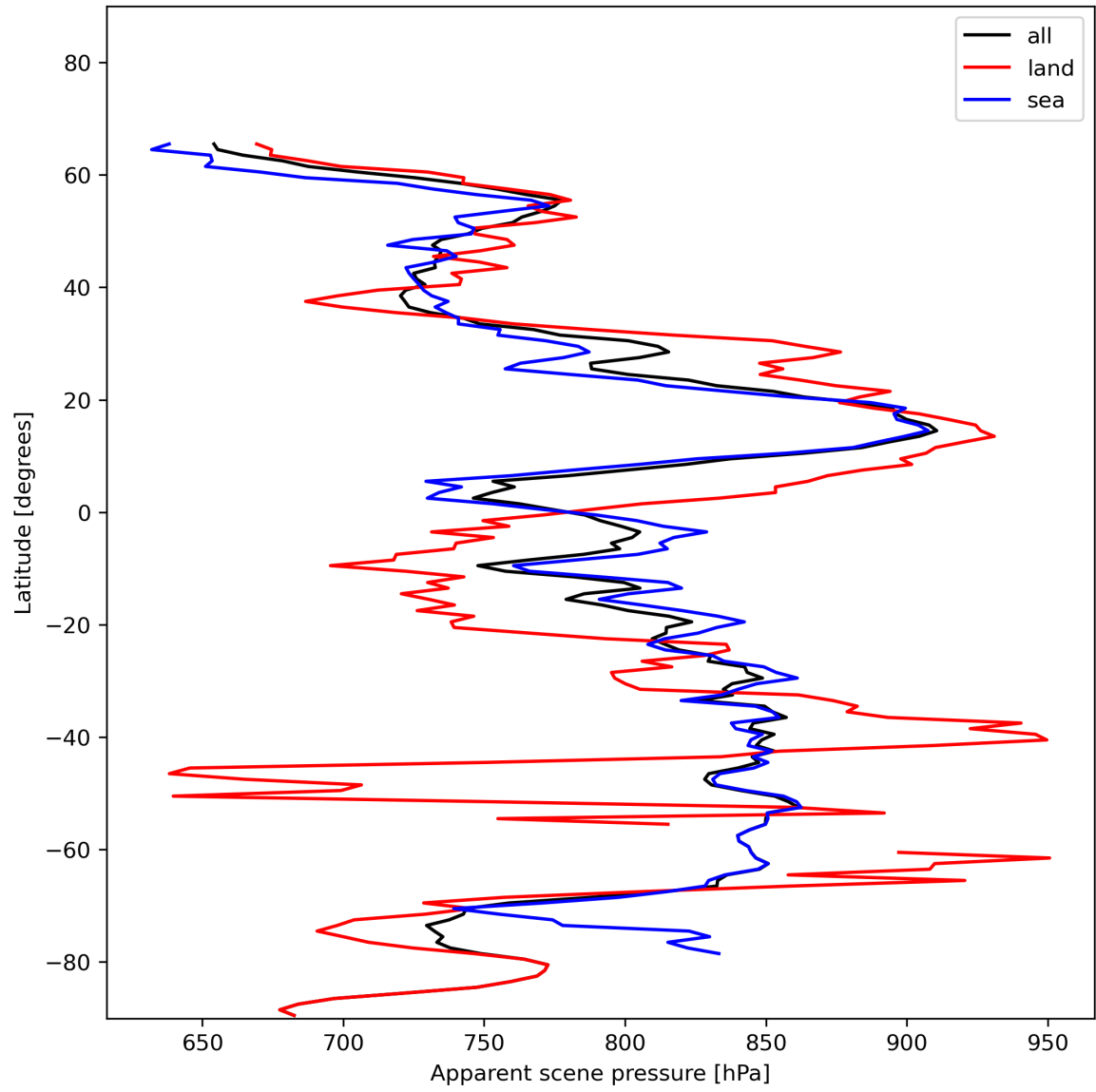
Figure 19: Zonal average of “Apparent scene pressure” for 2024-01-08 to 2024-01-10.
