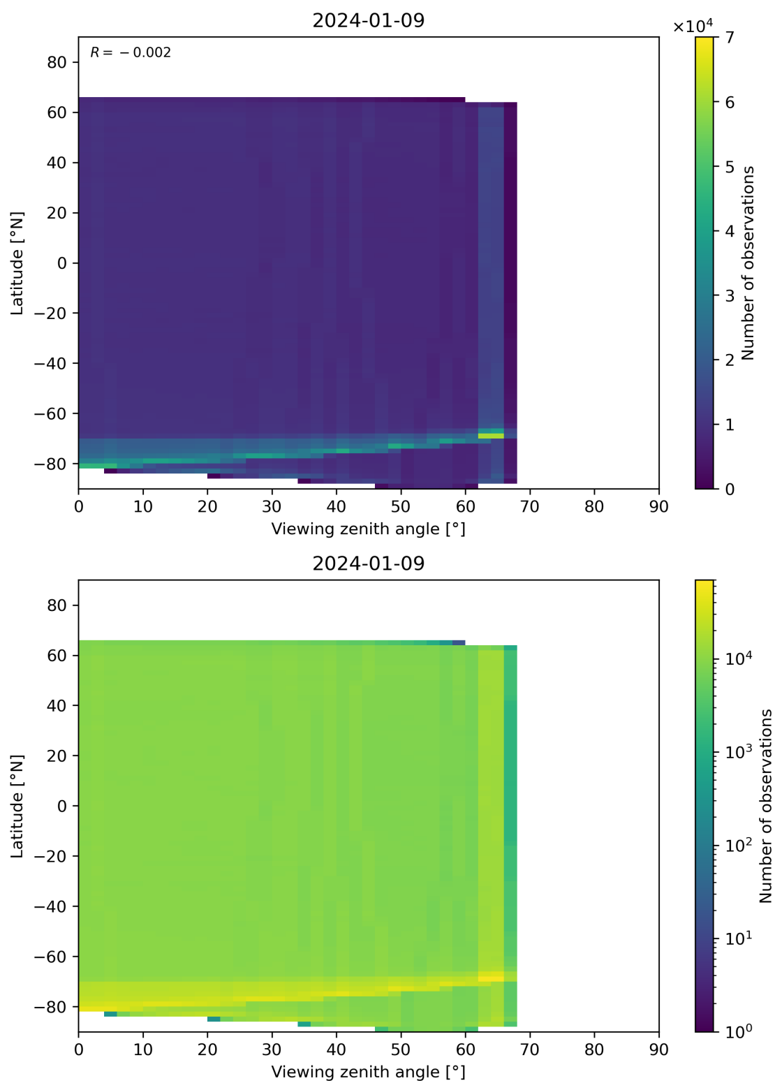
Figure 123: Scatter density plot of “Viewing zenith angle” against “Latitude” for 2024-01-08 to 2024-01-10.
