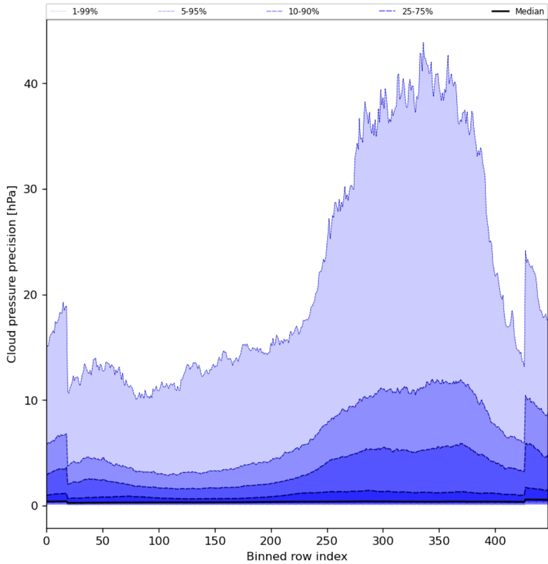
Figure 48: Along track statistics of “Cloud pressure precision” for 2024-01-08 to 2024-01-10
