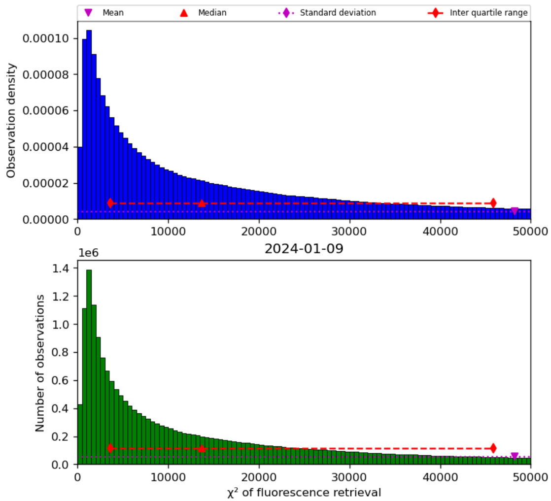
Figure 42: Histogram of “ \chi^2 of fluorescence retrieval” for 2024-01-08 to 2024-01-10
