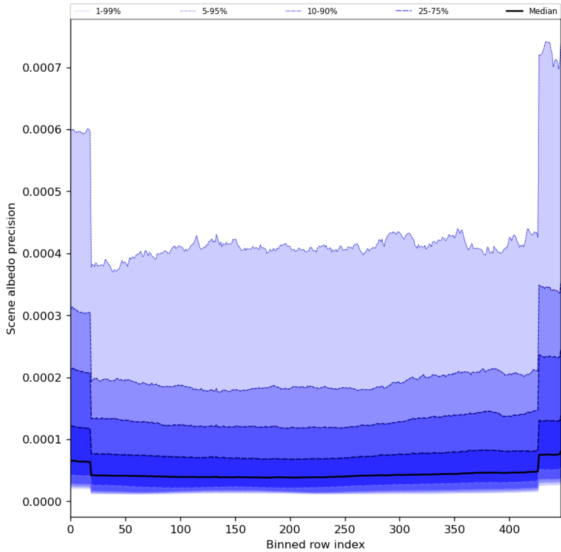
Figure 52: Along track statistics of “Scene albedo precision” for 2024-01-08 to 2024-01-10
