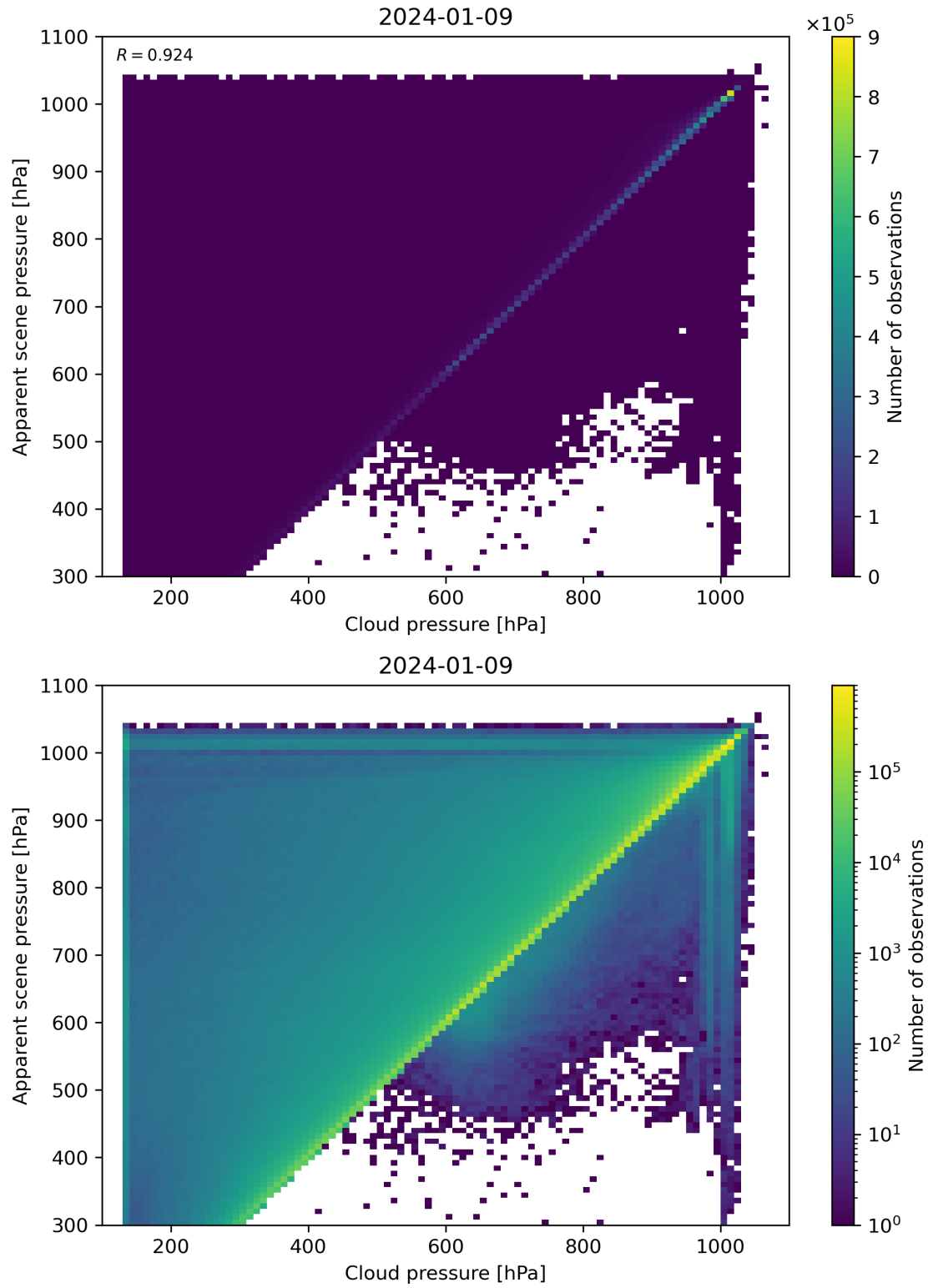
Figure 77: Scatter density plot of “Cloud pressure” against “Apparent scene pressure” for 2024-01-08 to 2024-01-10.
