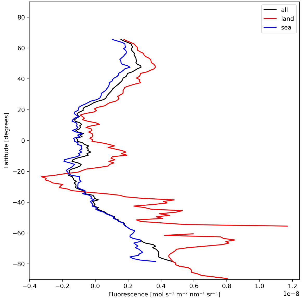
Figure 23: Zonal average of “Fluorescence” for 2024-01-08 to 2024-01-10.
