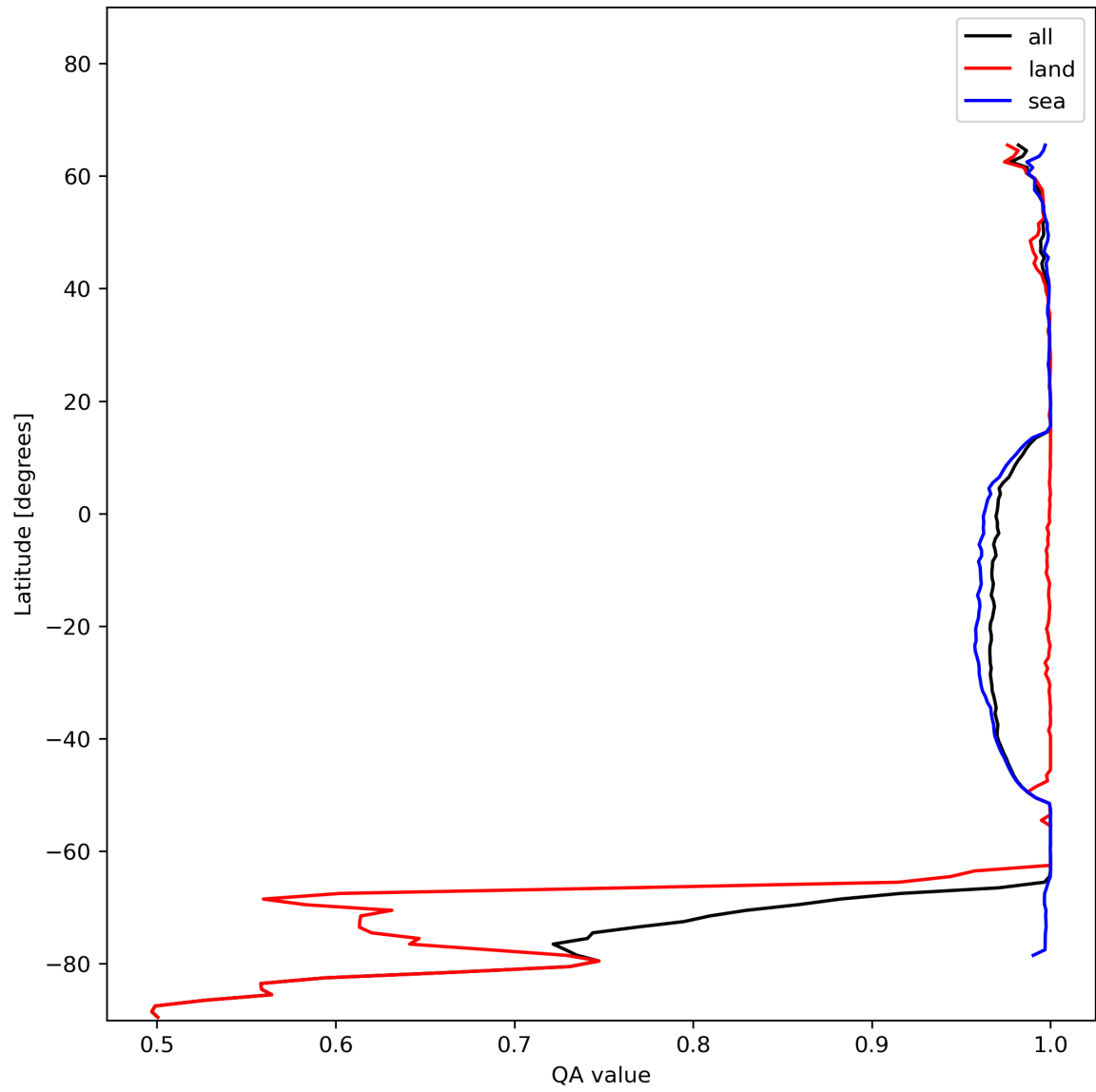
Figure 12: Zonal average of “QA value” for 2024-01-08 to 2024-01-10.
