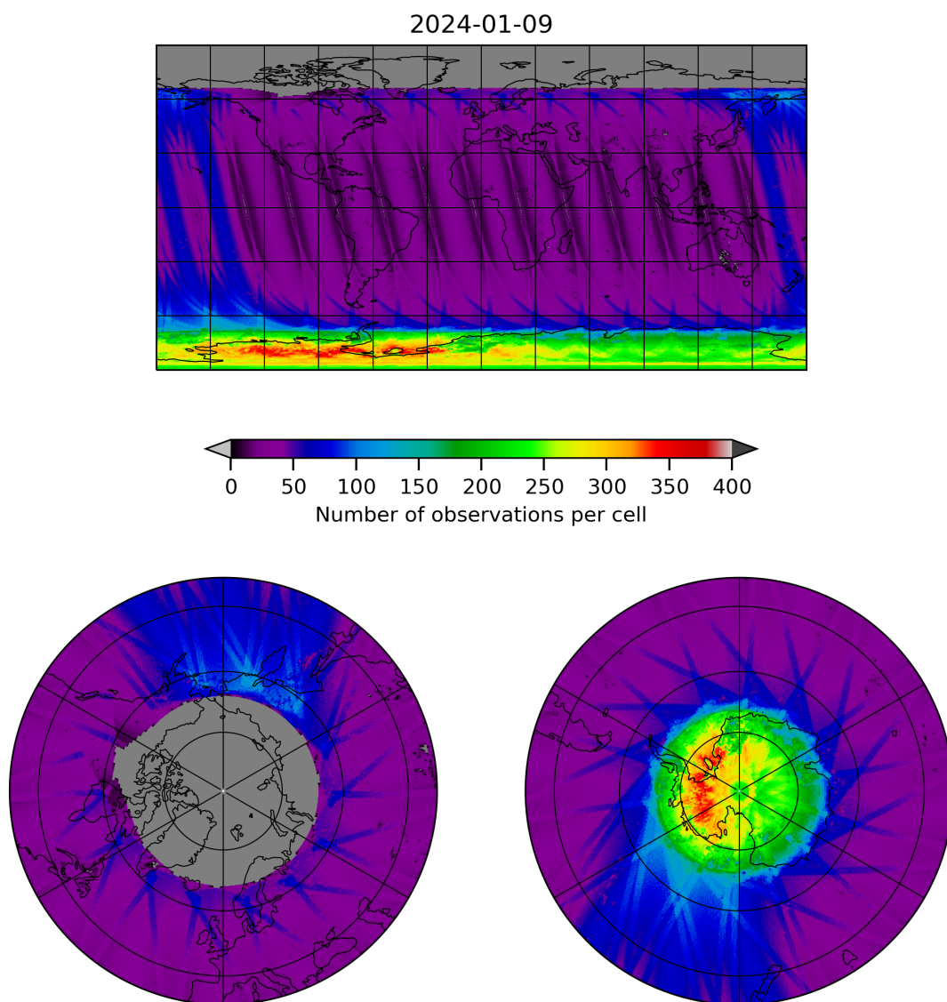
Figure 11: Map of the number of observations for 2024-01-08 to 2024-01-10
