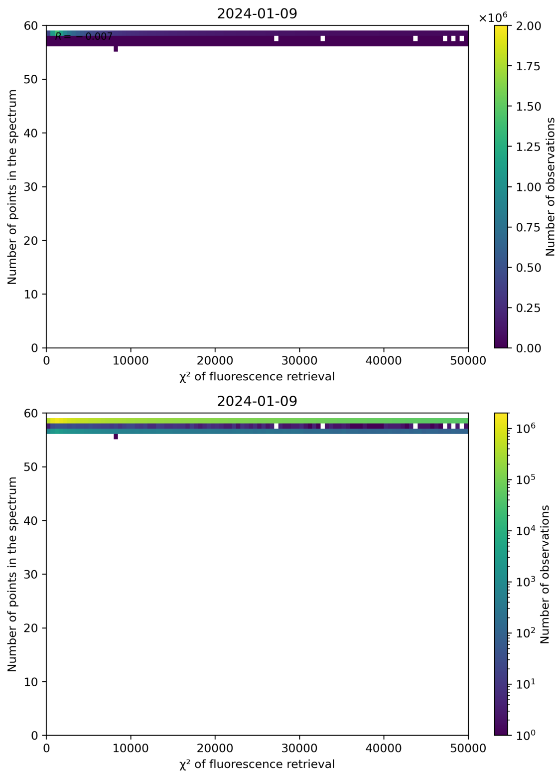
Figure 68: Scatter density plot of “ \chi^2 of fluorescence retrieval” against “Number of points in the spectrum” for 2024-01-08 to 2024-01-10.
