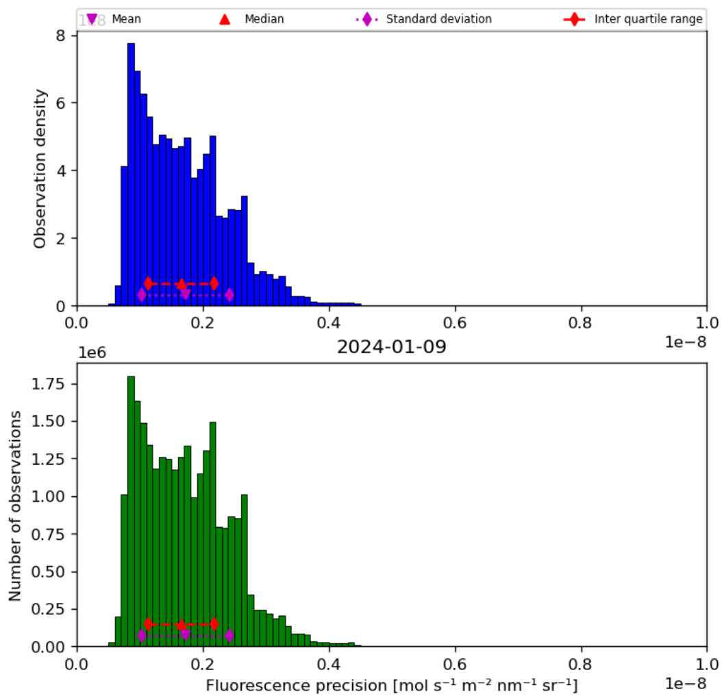
Figure 41: Histogram of “Fluorescence precision” for 2024-01-08 to 2024-01-10
