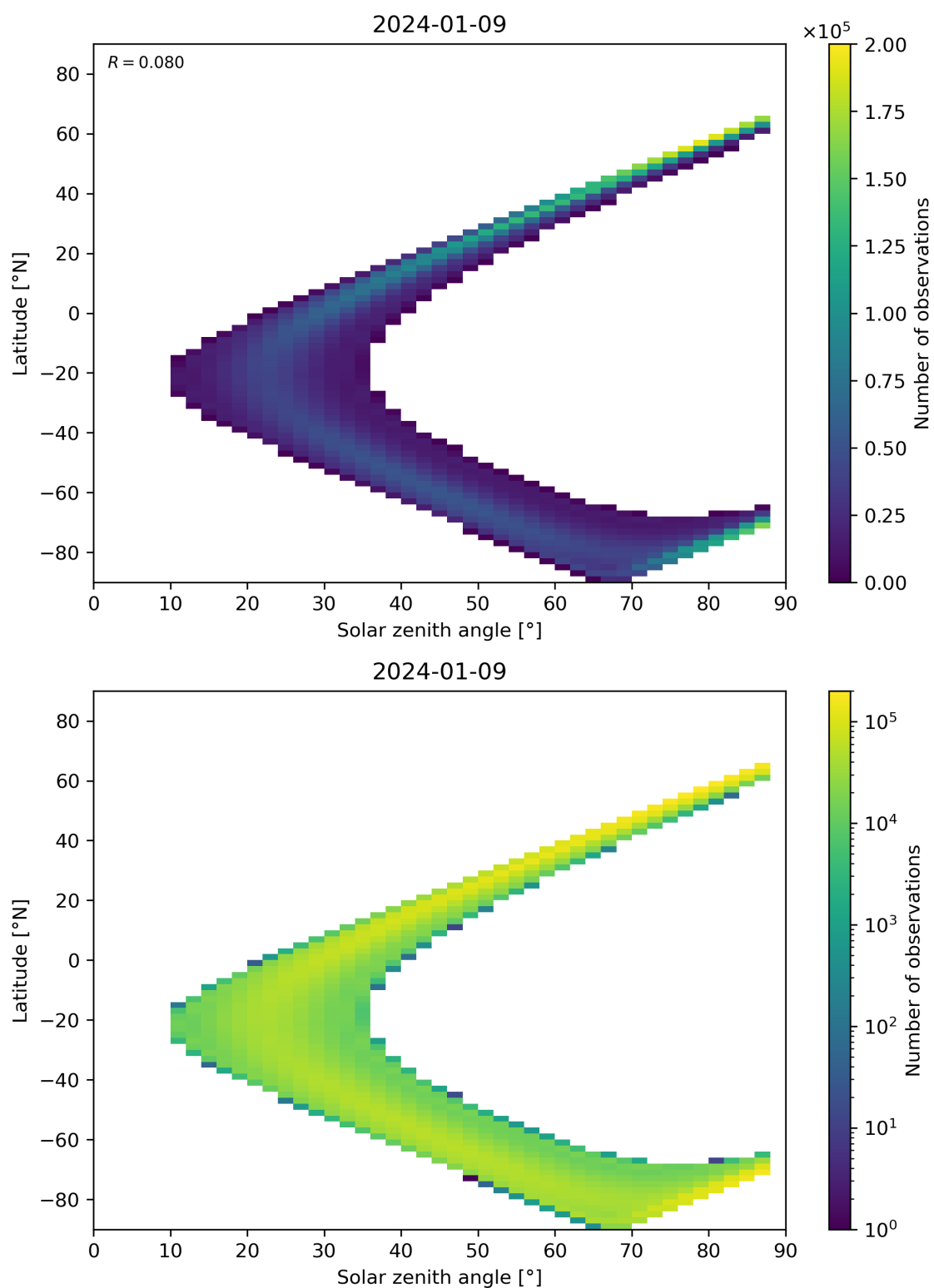
Figure 113: Scatter density plot of “Solar zenith angle” against “Latitude” for 2024-01-08 to 2024-01-10.
