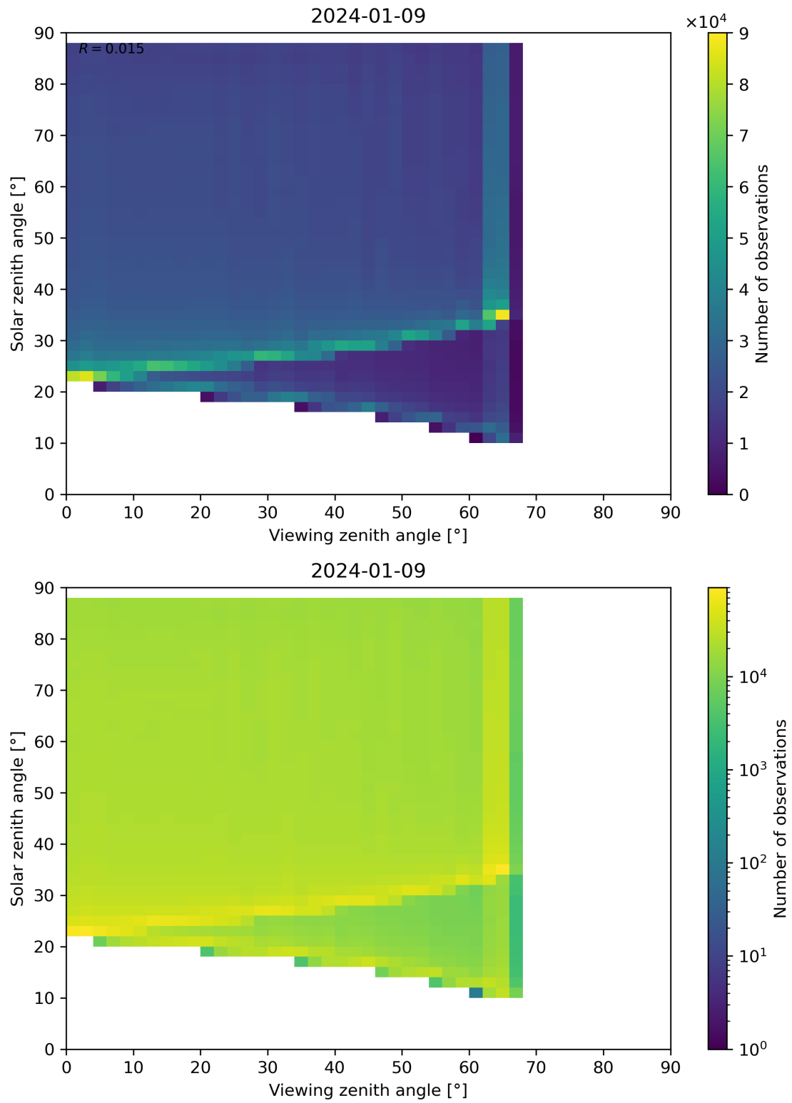
Figure 127: Scatter density plot of “Viewing zenith angle” against “Solar zenith angle” for 2024-01-08 to 2024-01-10.
