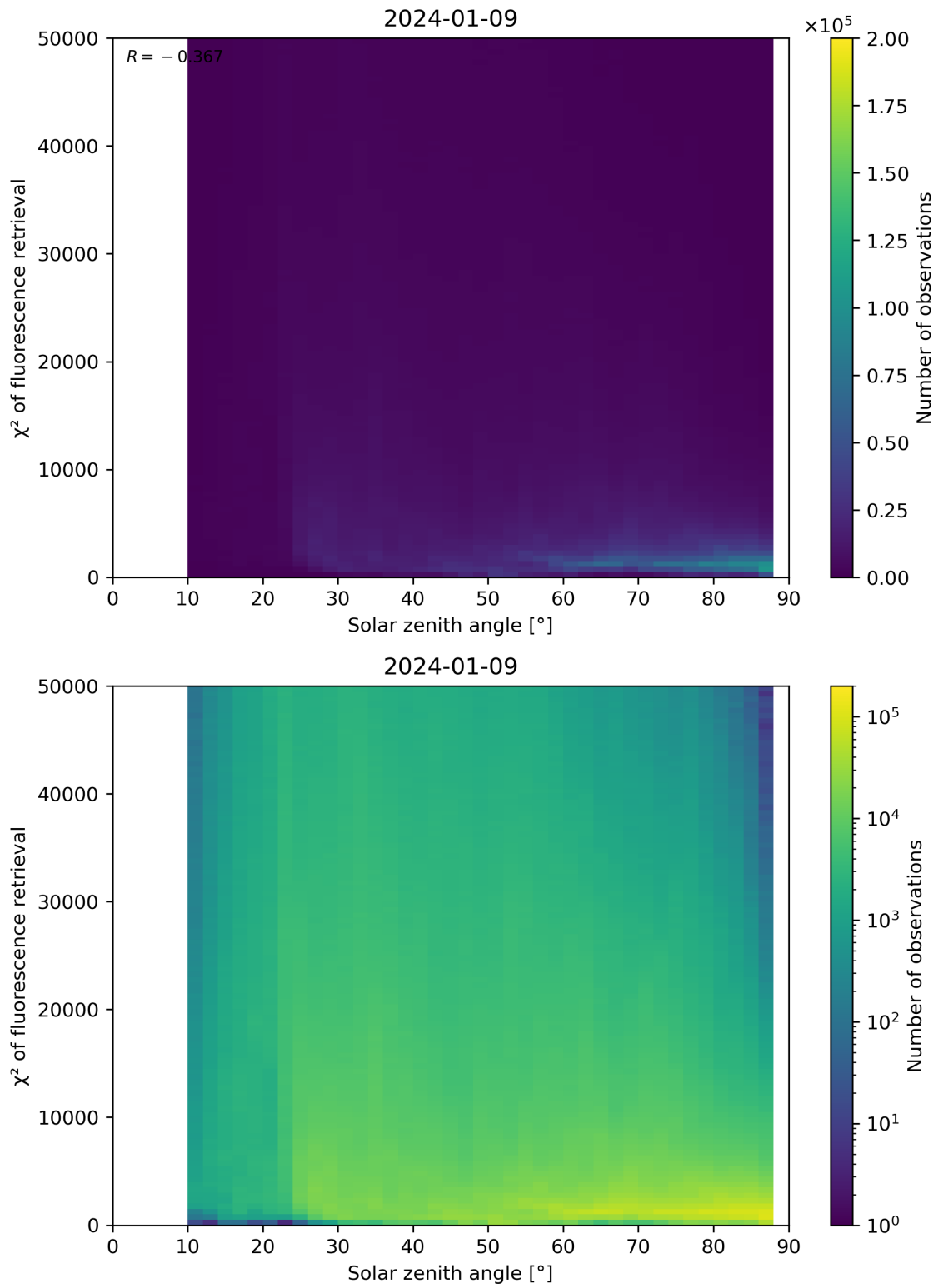
Figure 109: Scatter density plot of “Solar zenith angle” against “ \chi^2 of fluorescence retrieval” for 2024-01-08 to 2024-01-10.
