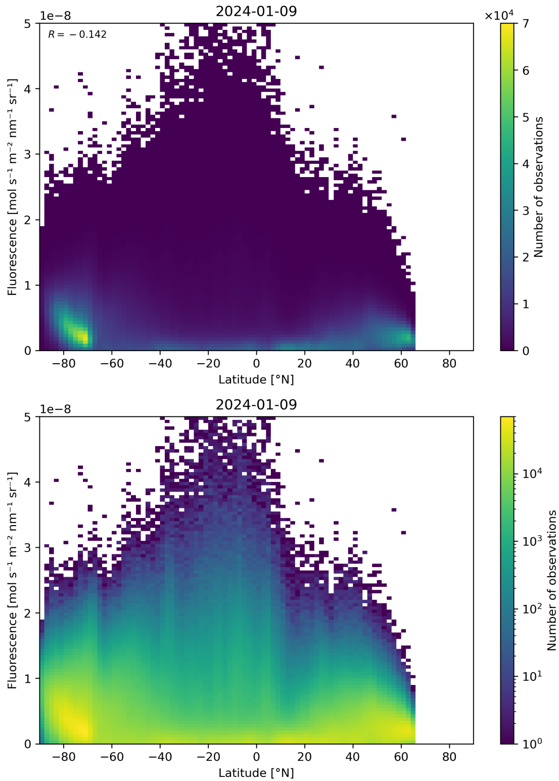
Figure 92: Scatter density plot of “Latitude” against “Fluorescence” for 2024-01-08 to 2024-01-10.
