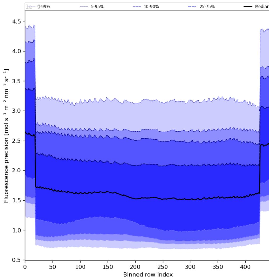
Figure 58: Along track statistics of “Fluorescence precision” for 2024-01-08 to 2024-01-10
