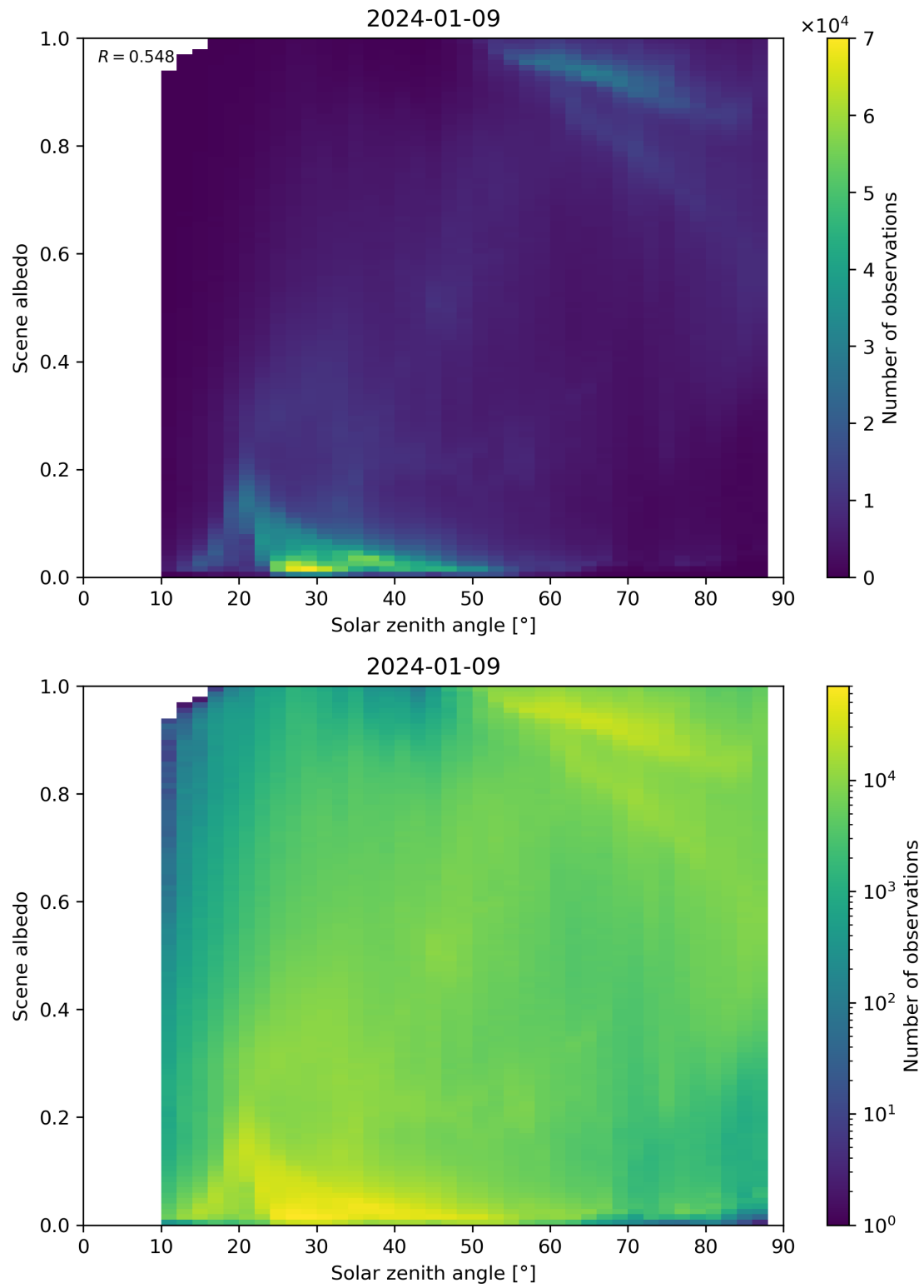
Figure 116: Scatter density plot of “Solar zenith angle” against “Scene albedo” for 2024-01-08 to 2024-01-10.
