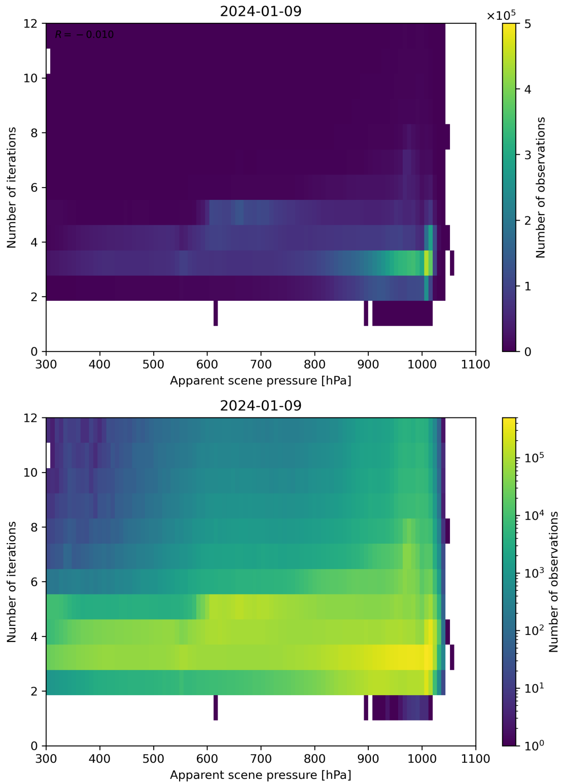
Figure 65: Scatter density plot of “Apparent scene pressure” against “Number of iterations” for 2024-01-08 to 2024-01-10.
