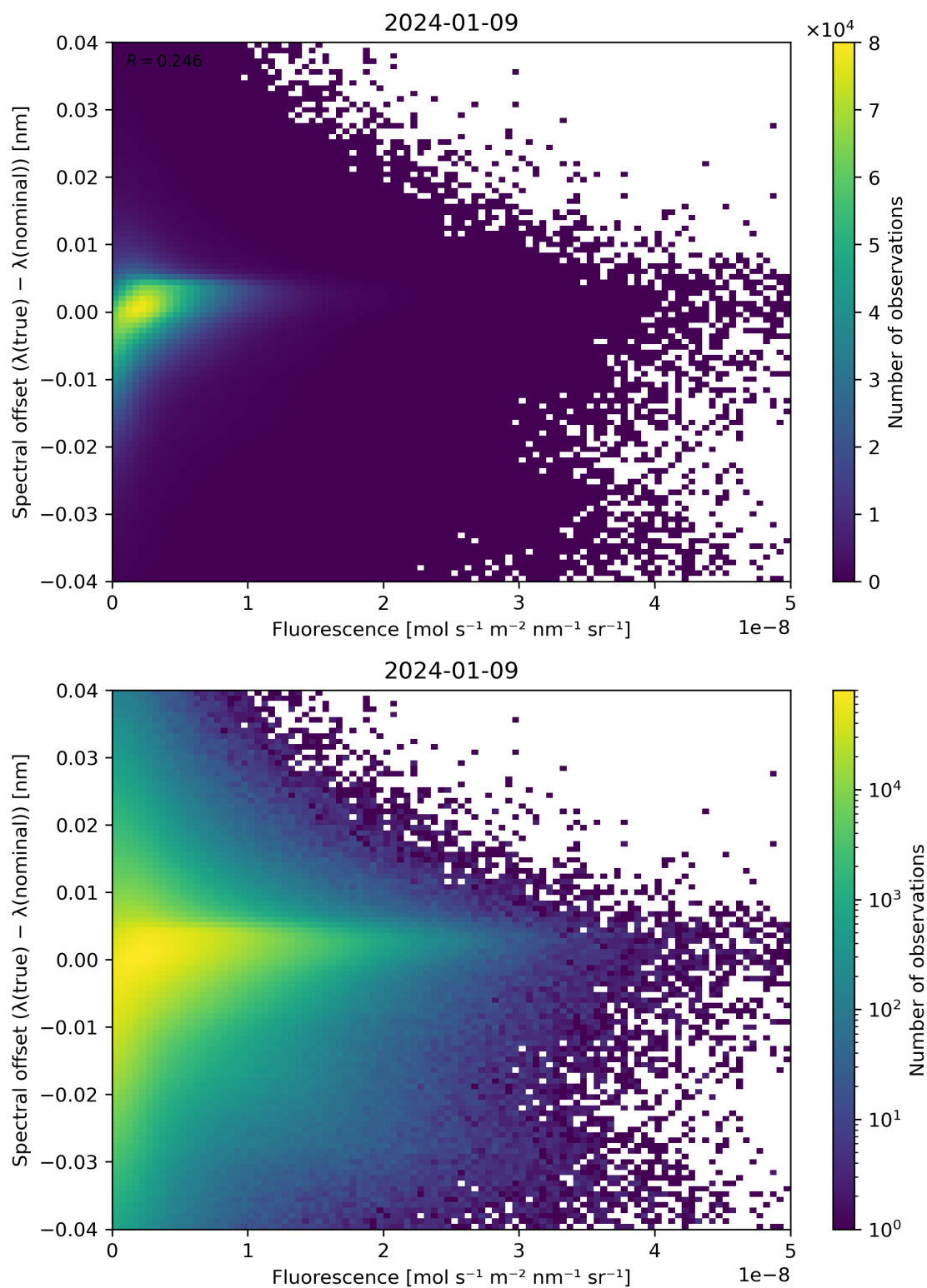
Figure 87: Scatter density plot of “Fluorescence” against “Spectral offset ( \lambda(\text{true}) - \lambda(\text{nominal}) )” for 2024-01-08 to 2024-01-10.
