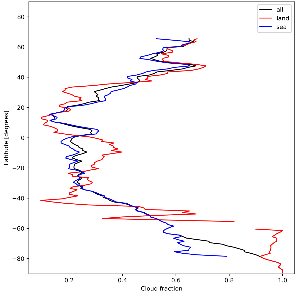
Figure 15: Zonal average of “Cloud fraction” for 2024-01-08 to 2024-01-10.
