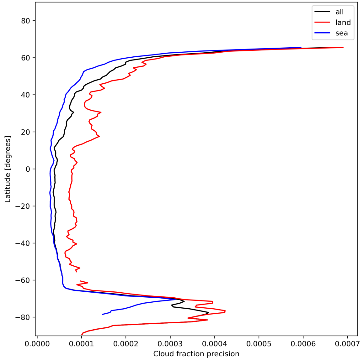
Figure 16: Zonal average of “Cloud fraction precision” for 2024-01-08 to 2024-01-10.
