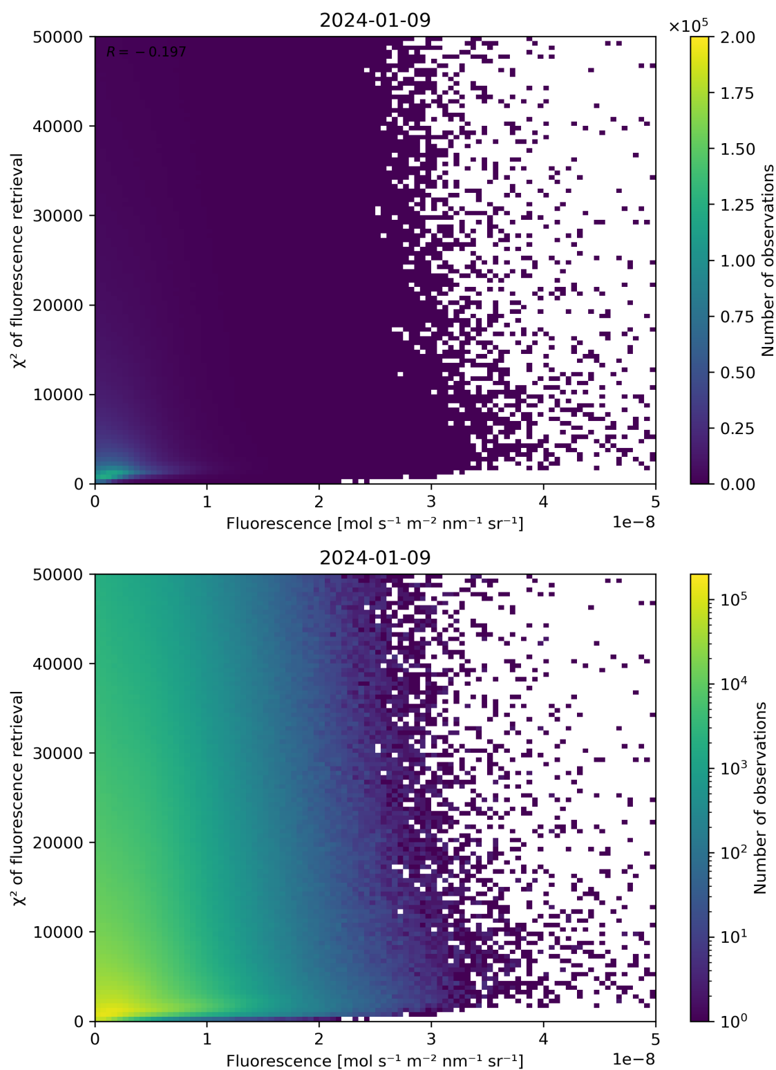
Figure 85: Scatter density plot of “Fluorescence” against “ \chi^2 of fluorescence retrieval” for 2024-01-08 to 2024-01-10.
