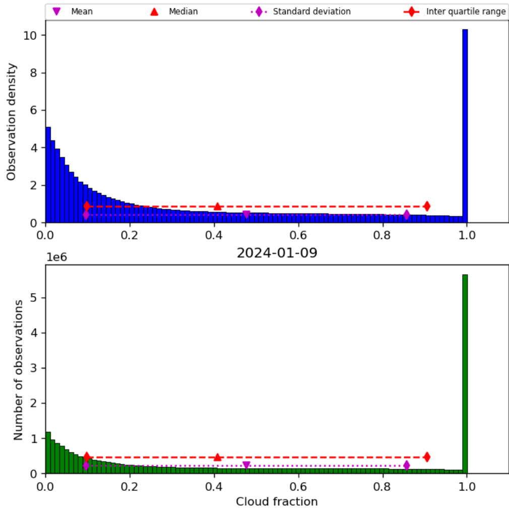
Figure 32: Histogram of “Cloud fraction” for 2024-01-08 to 2024-01-10
