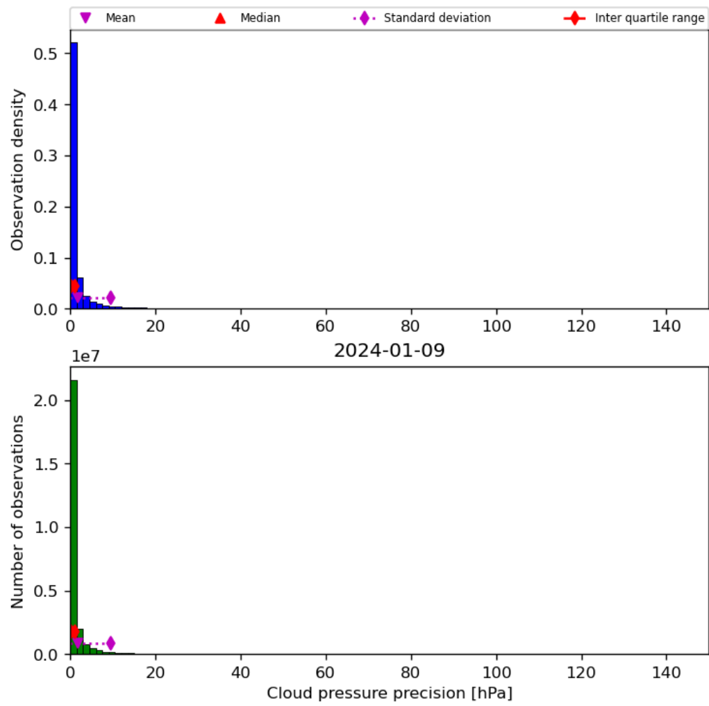
Figure 31: Histogram of “Cloud pressure precision” for 2024-01-08 to 2024-01-10
