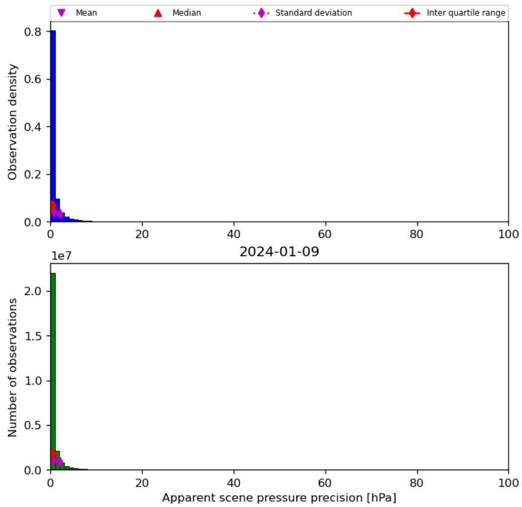
Figure 37: Histogram of “Apparent scene pressure precision” for 2024-01-08 to 2024-01-10
