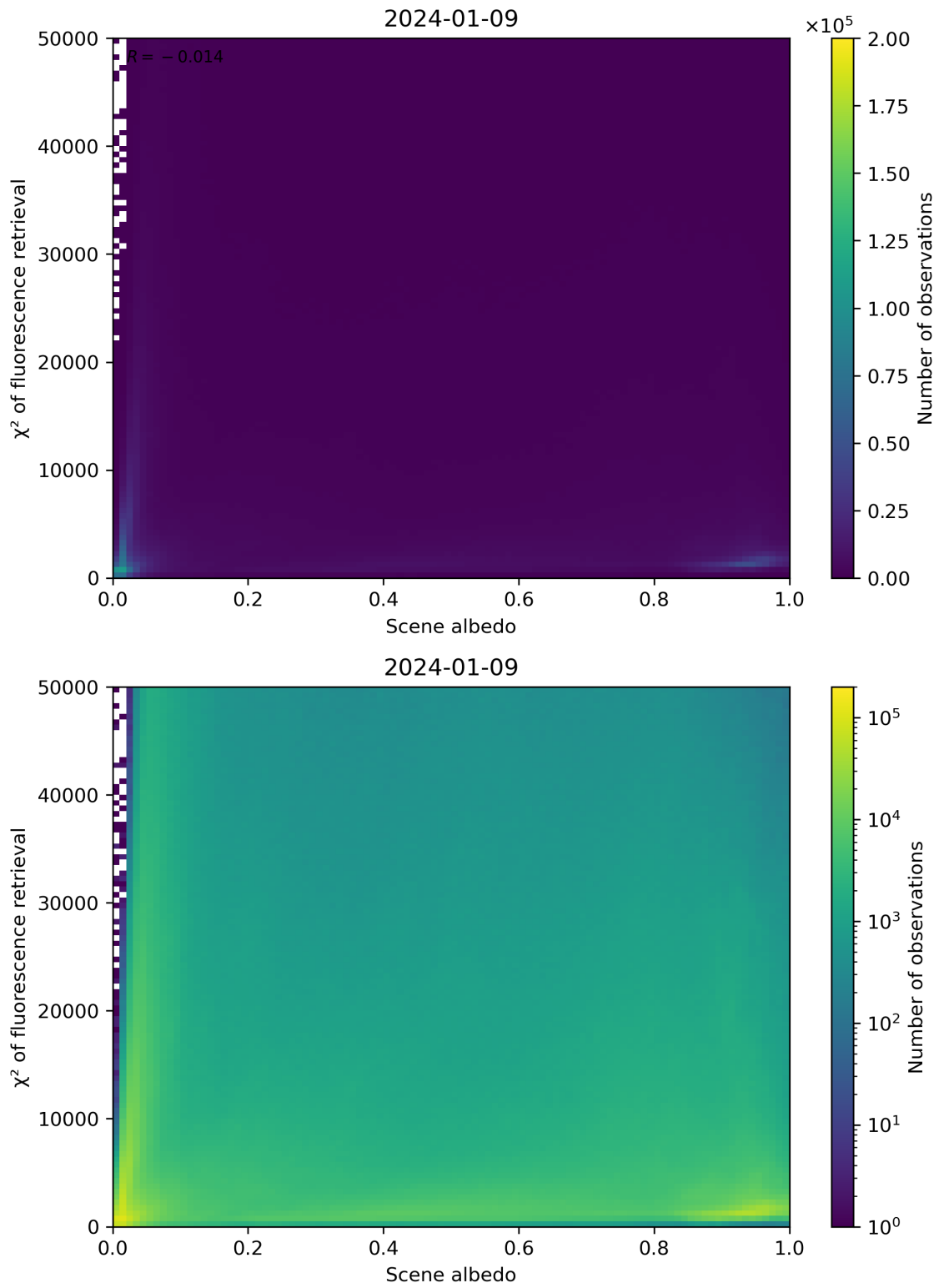
Figure 103: Scatter density plot of “Scene albedo” against “ \chi^2 of fluorescence retrieval” for 2024-01-08 to 2024-01-10.
