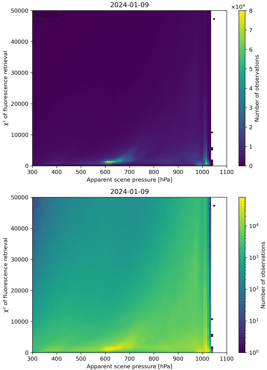
Figure 63: Scatter density plot of “Apparent scene pressure” against “ \chi^2 of fluorescence retrieval” for 2024-01-08 to 2024-01-10.
