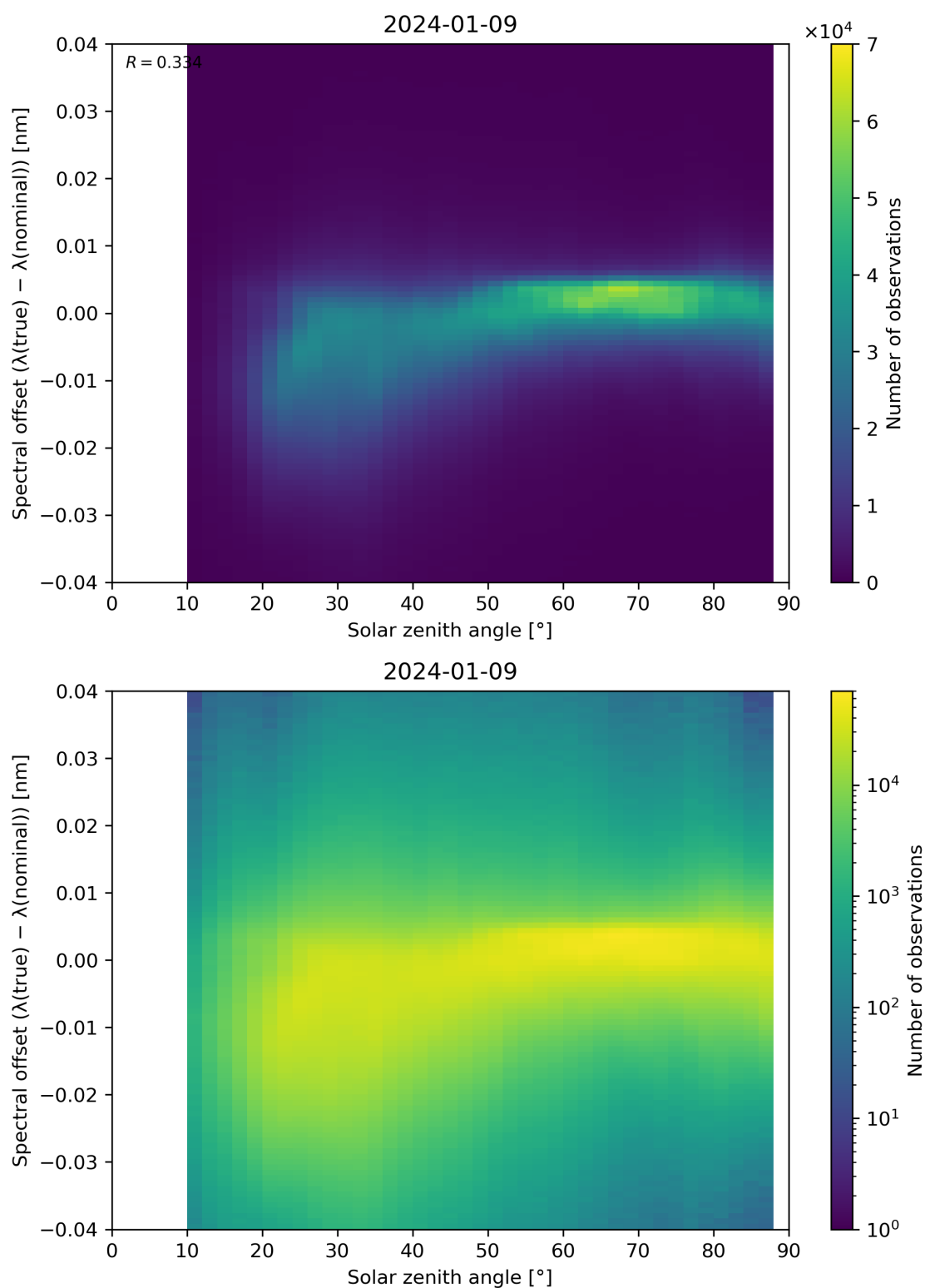
Figure 117: Scatter density plot of “Solar zenith angle” against “Spectral offset ( \lambda(\text{true}) - \lambda(\text{nominal}) )” for 2024-01-08 to 2024-01-10.
