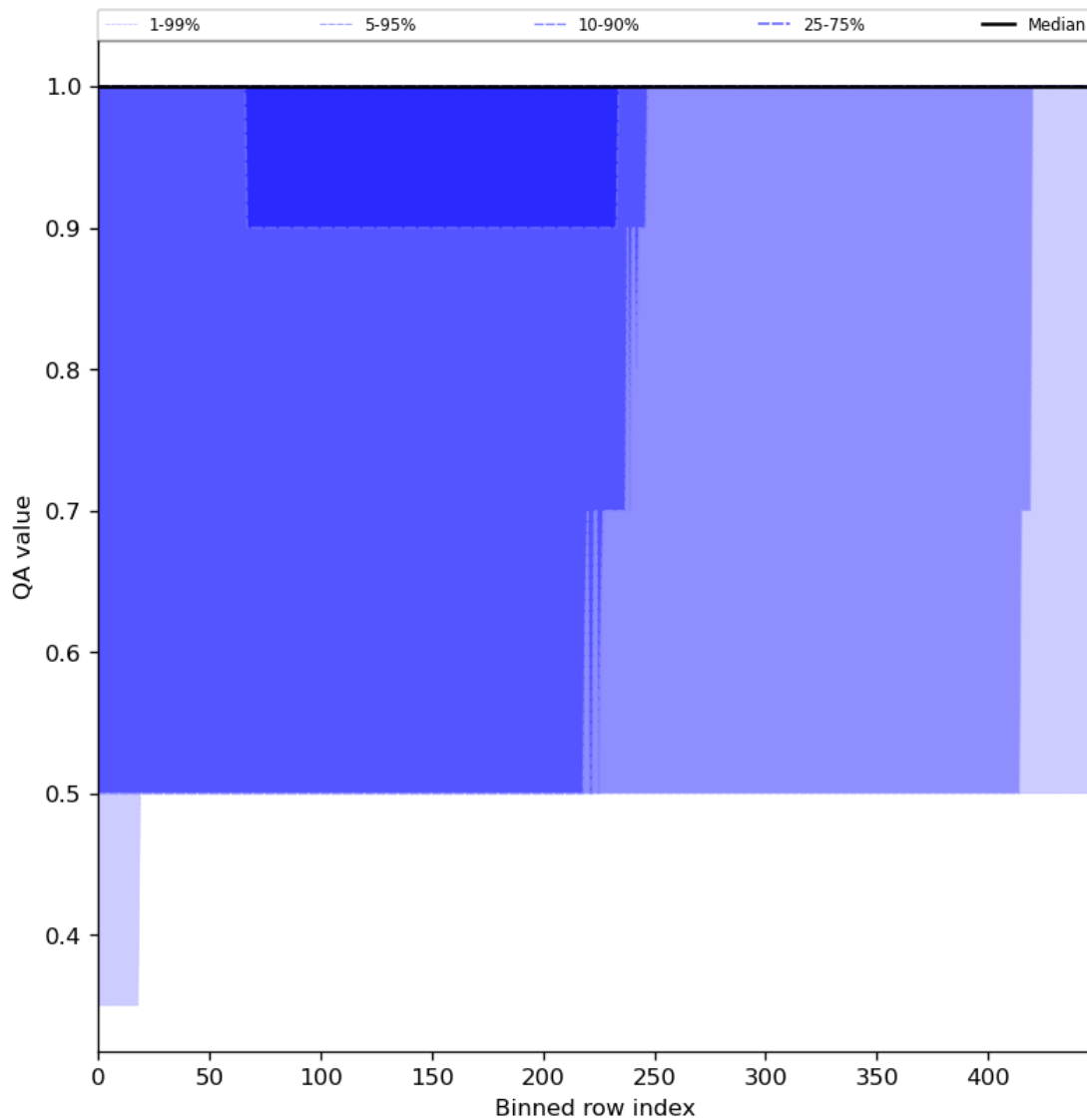
Figure 46: Along track statistics of “QA value” for 2024-01-08 to 2024-01-10
