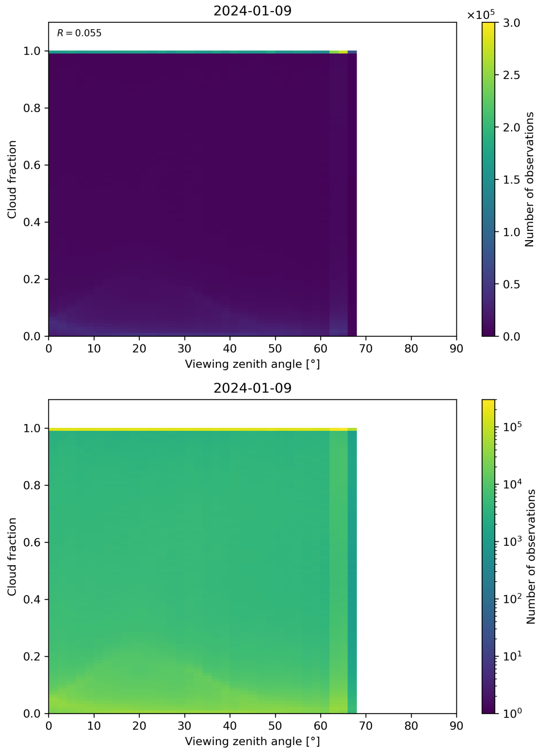
Figure 120: Scatter density plot of “Viewing zenith angle” against “Cloud fraction” for 2024-01-08 to 2024-01-10.
