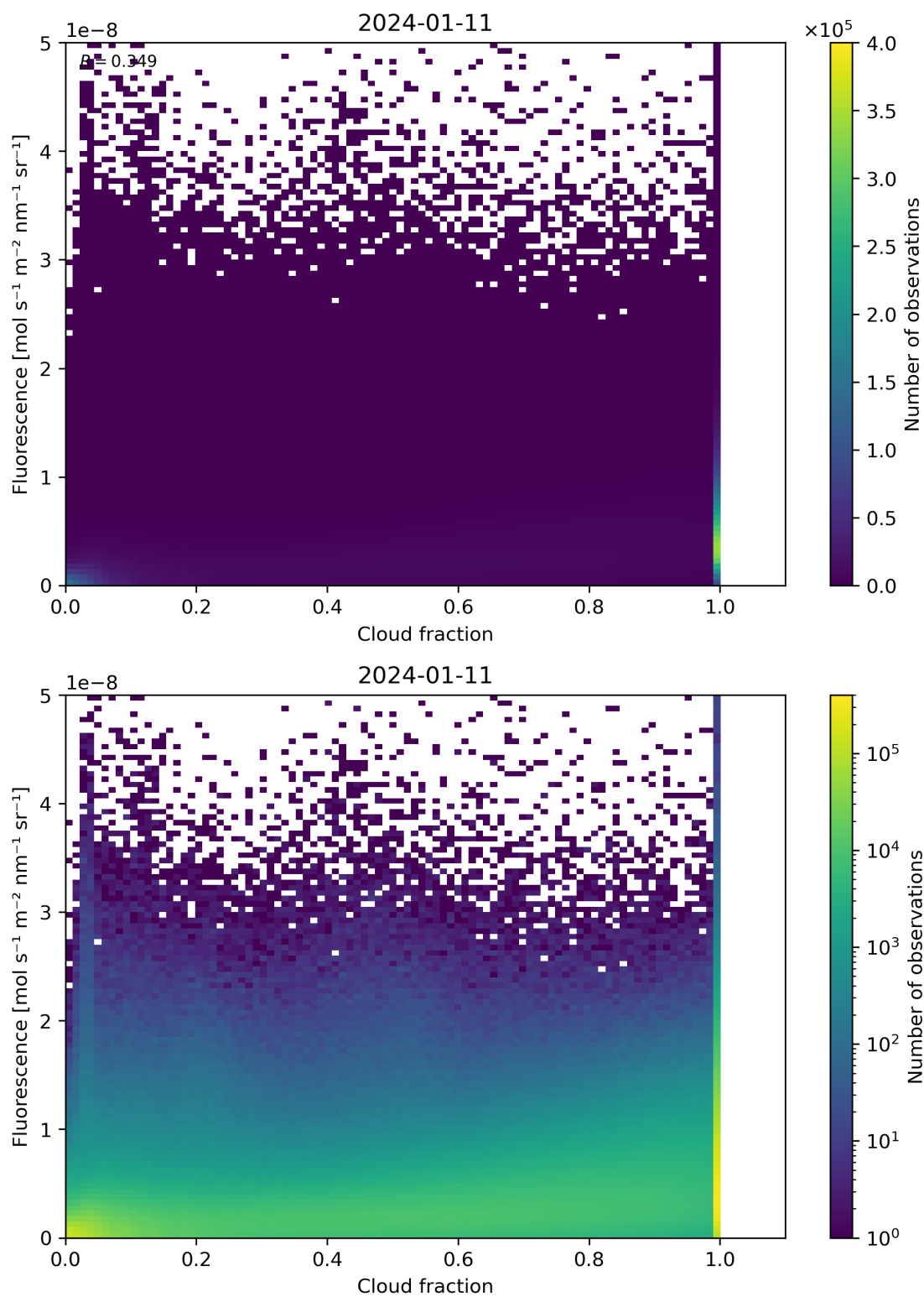
Figure 72: Scatter density plot of “Cloud fraction” against “Fluorescence” for 2024-01-10 to 2024-01-12.
