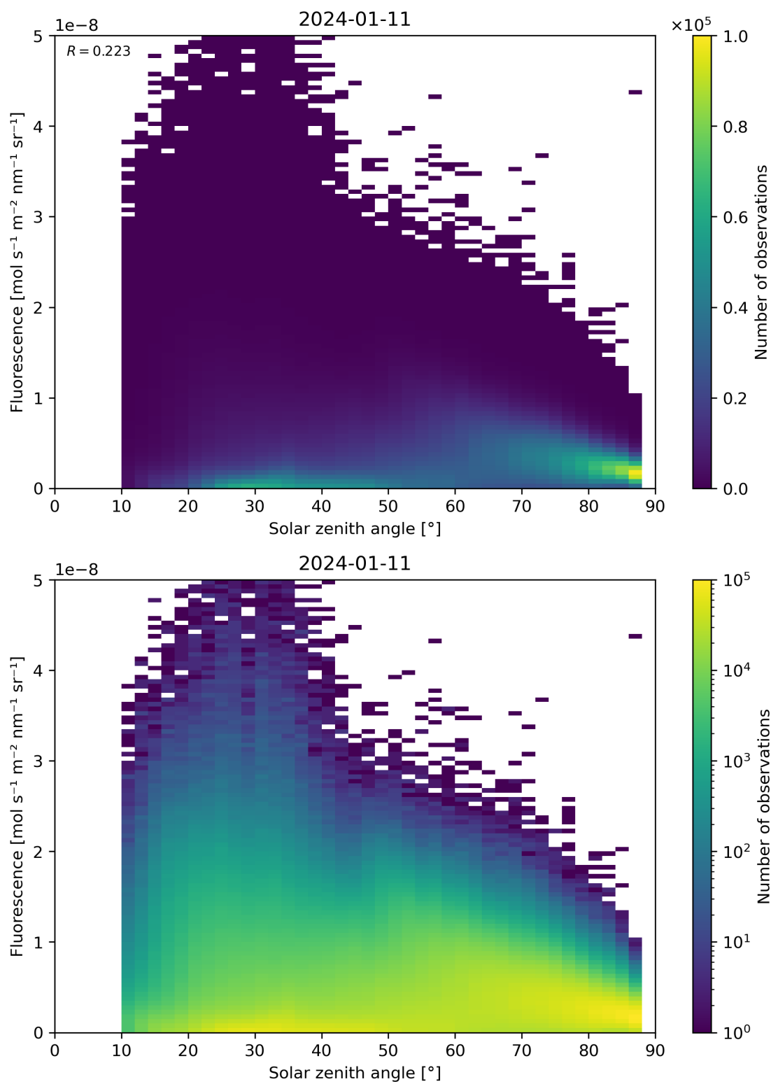
Figure 112: Scatter density plot of “Solar zenith angle” against “Fluorescence” for 2024-01-10 to 2024-01-12.
