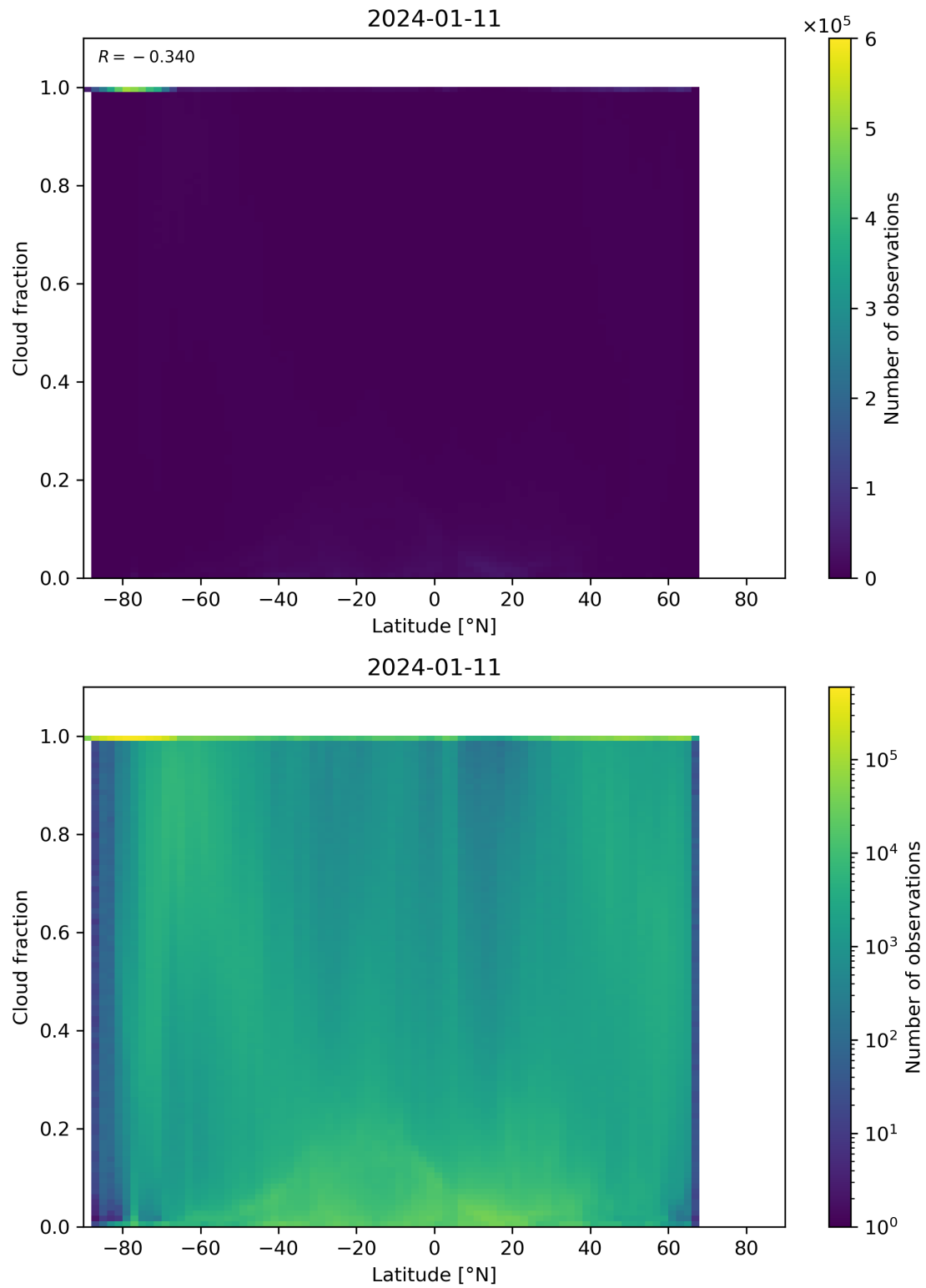
Figure 90: Scatter density plot of “Latitude” against “Cloud fraction” for 2024-01-10 to 2024-01-12.
