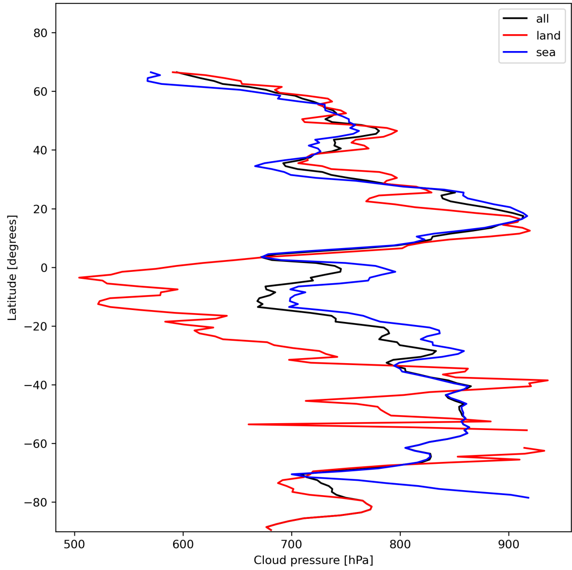
Figure 13: Zonal average of “Cloud pressure” for 2024-01-10 to 2024-01-12.
