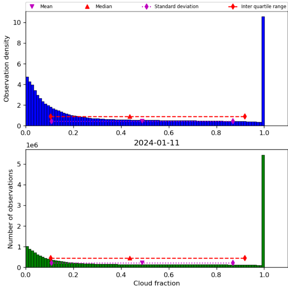
Figure 32: Histogram of “Cloud fraction” for 2024-01-10 to 2024-01-12
