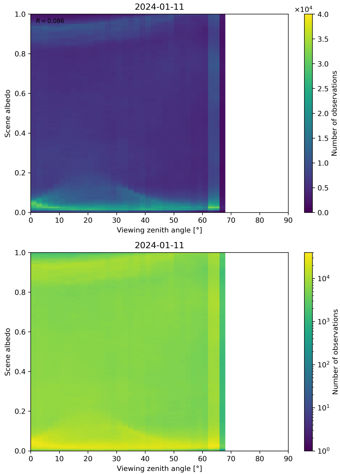
Figure 126: Scatter density plot of “Viewing zenith angle” against “Scene albedo” for 2024-01-10 to 2024-01-12.
