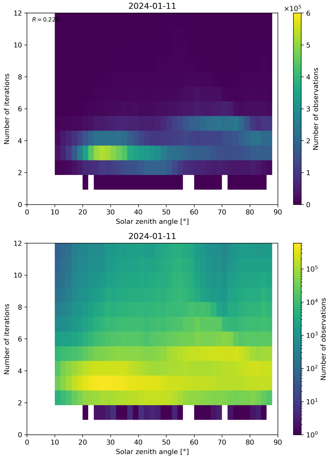
Figure 114: Scatter density plot of “Solar zenith angle” against “Number of iterations” for 2024-01-10 to 2024-01-12.
