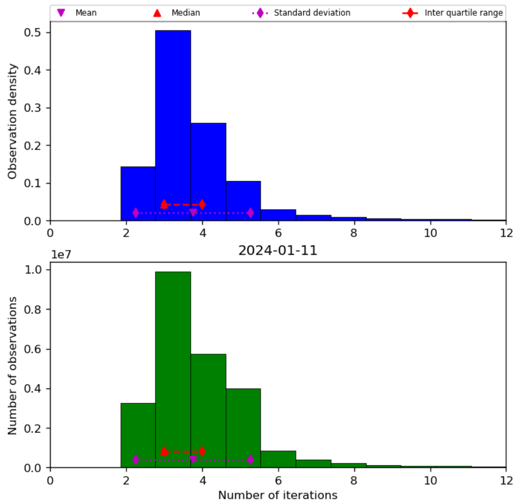
Figure 39: Histogram of “Number of iterations” for 2024-01-10 to 2024-01-12
