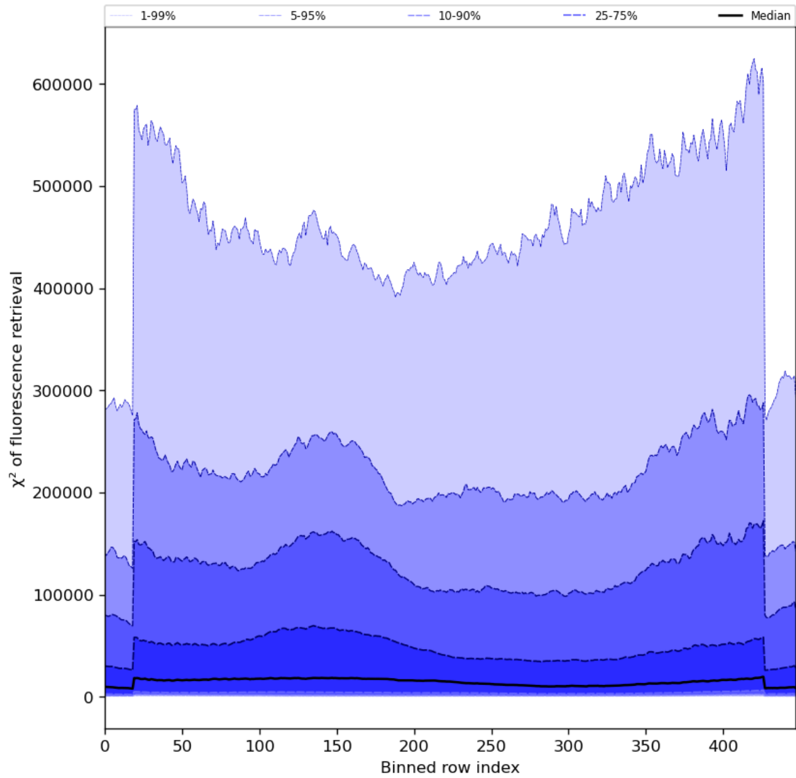
Figure 59: Along track statistics of “ \chi^2 of fluorescence retrieval” for 2024-01-10 to 2024-01-12
