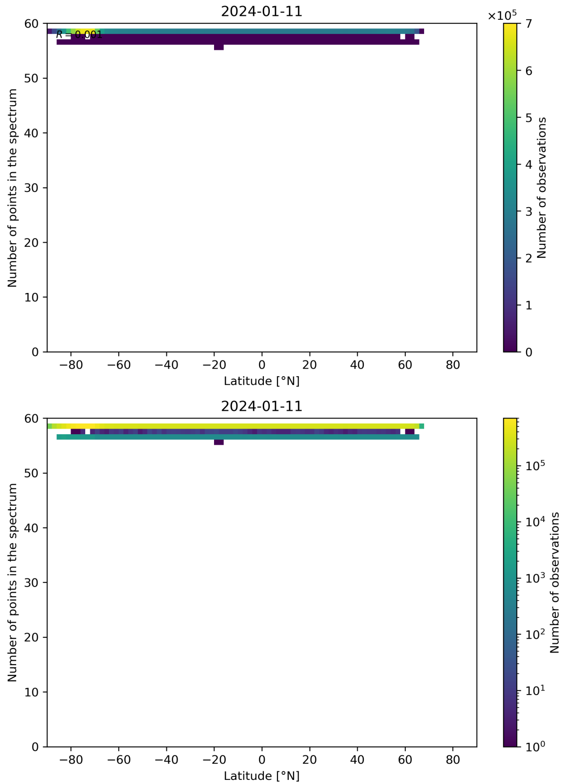
Figure 94: Scatter density plot of “Latitude” against “Number of points in the spectrum” for 2024-01-10 to 2024-01-12.
