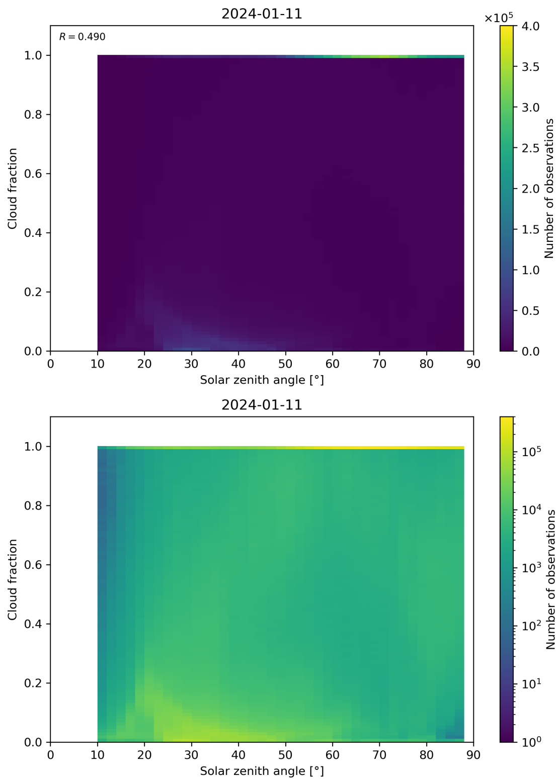
Figure 110: Scatter density plot of “Solar zenith angle” against “Cloud fraction” for 2024-01-10 to 2024-01-12.
