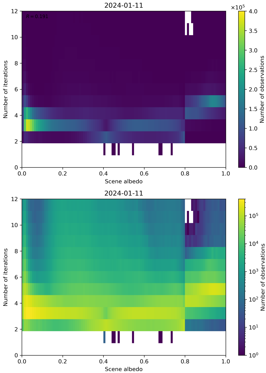
Figure 105: Scatter density plot of “Scene albedo” against “Number of iterations” for 2024-01-10 to 2024-01-12.
