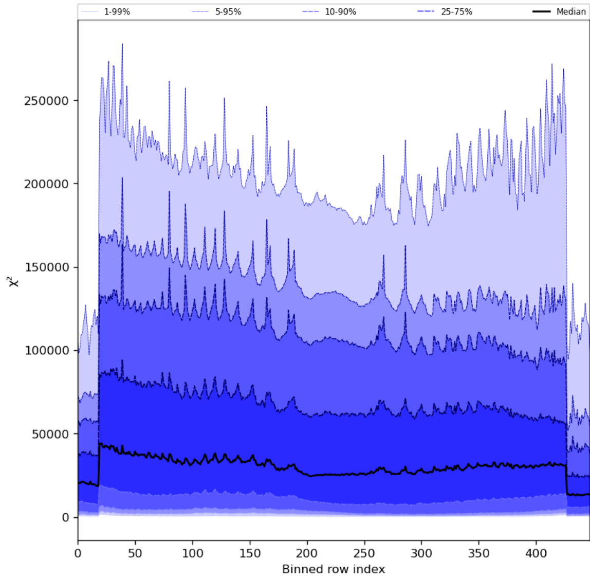
Figure 55: Along track statistics of “ \chi^2 ” for 2024-01-10 to 2024-01-12
