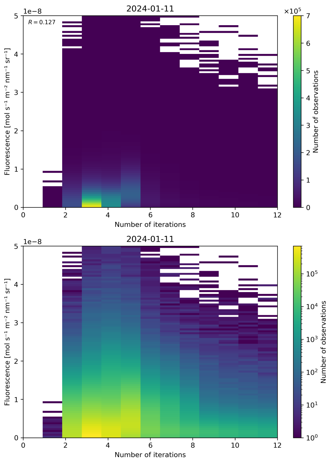
Figure 98: Scatter density plot of “Number of iterations” against “Fluorescence” for 2024-01-10 to 2024-01-12.
