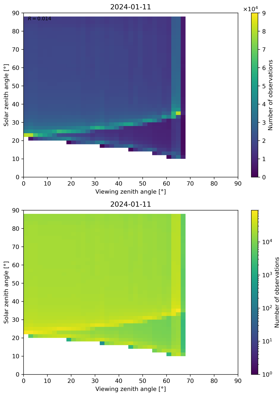
Figure 127: Scatter density plot of “Viewing zenith angle” against “Solar zenith angle” for 2024-01-10 to 2024-01-12.
