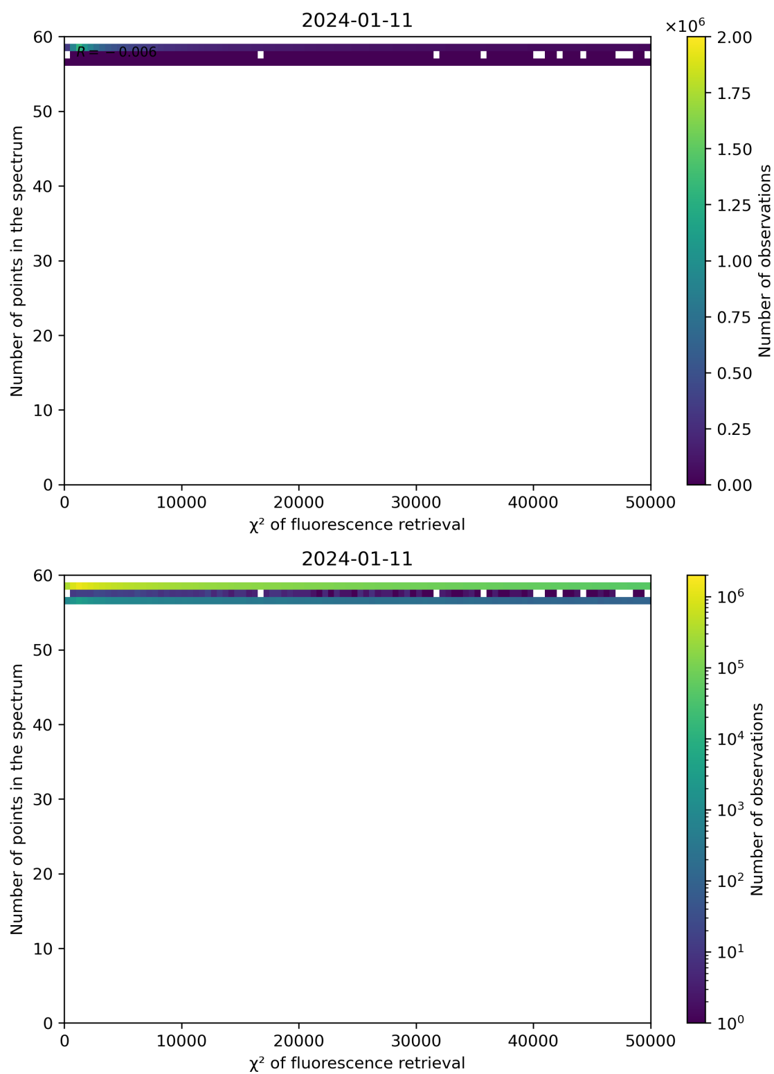
Figure 68: Scatter density plot of " \chi^2 of fluorescence retrieval" against "Number of points in the spectrum" for 2024-01-10 to 2024-01-12.
