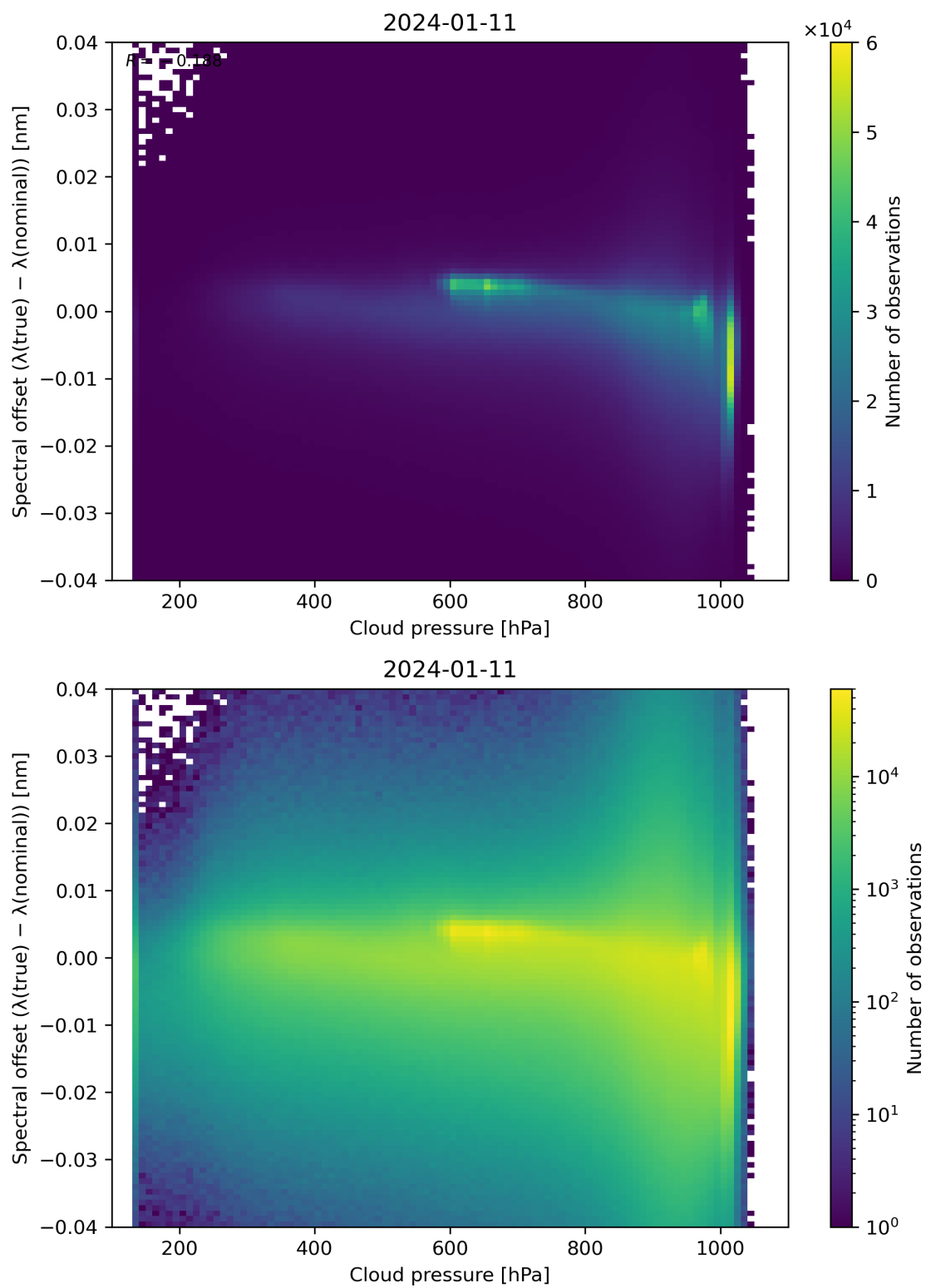
Figure 84: Scatter density plot of “Cloud pressure” against “Spectral offset ( \lambda(\text{true}) - \lambda(\text{nominal}) )” for 2024-01-10 to 2024-01-12.
