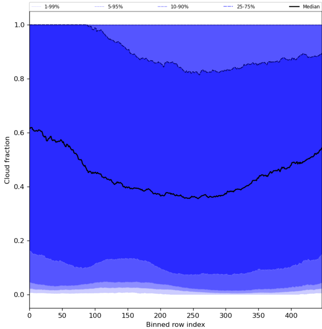
Figure 49: Along track statistics of “Cloud fraction” for 2024-01-10 to 2024-01-12
