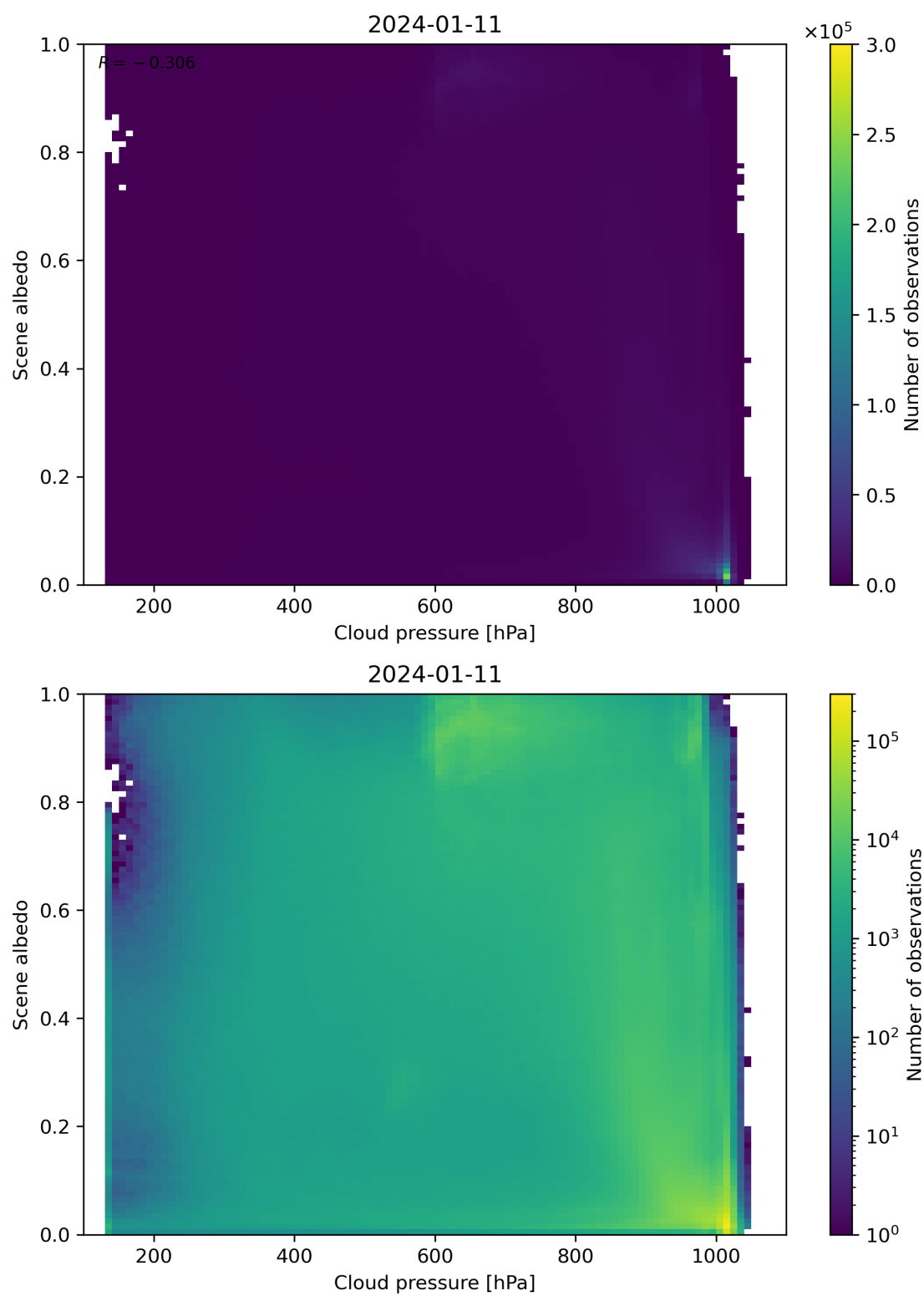
Figure 83: Scatter density plot of “Cloud pressure” against “Scene albedo” for 2024-01-10 to 2024-01-12.
