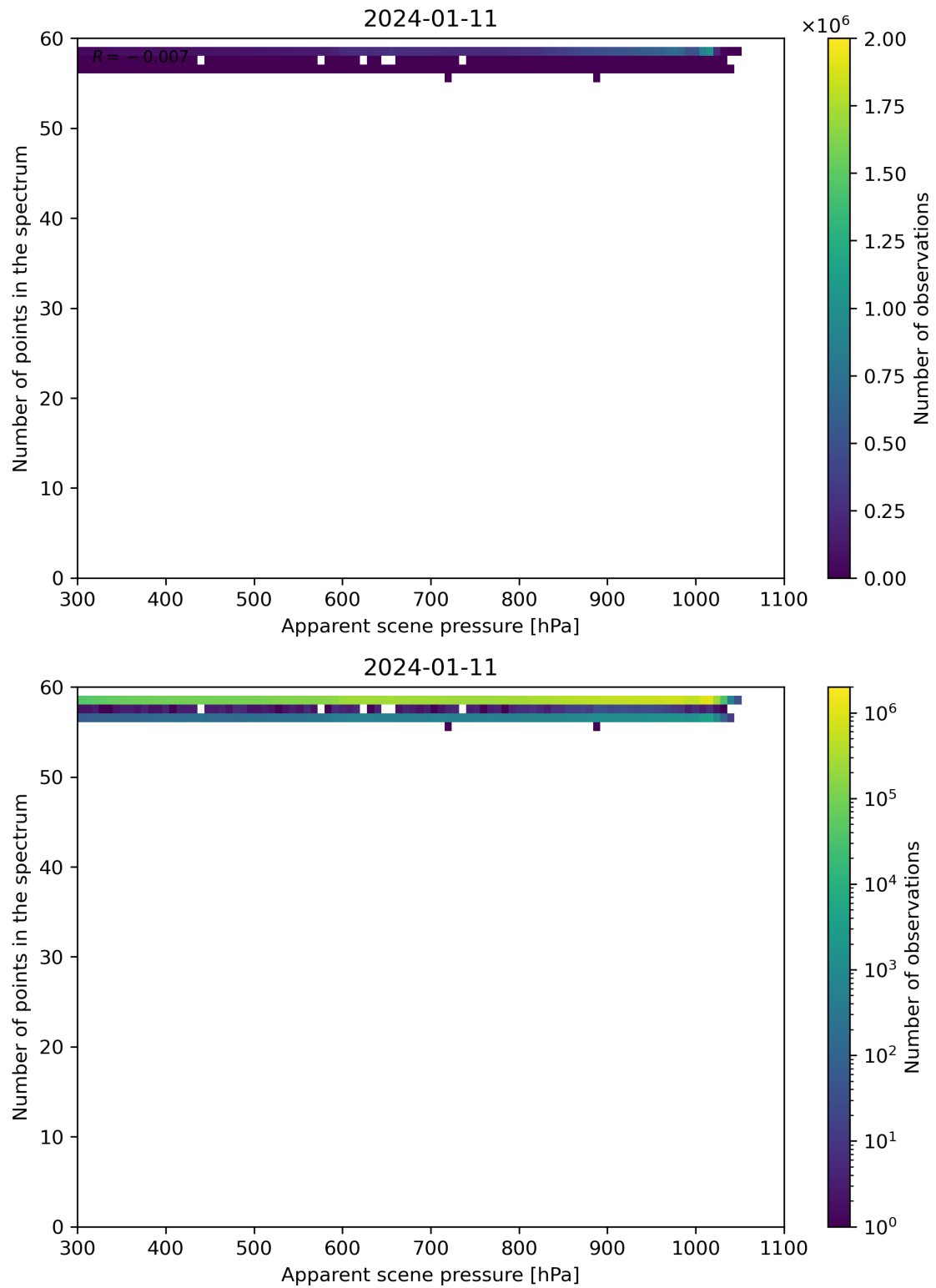
Figure 66: Scatter density plot of “Apparent scene pressure” against “Number of points in the spectrum” for 2024-01-10 to 2024-01-12.
