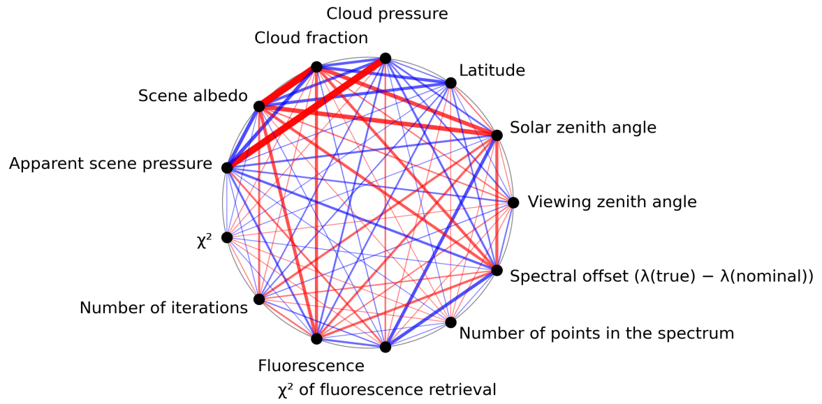
Figure 1: Map of correlation graph for 2024-01-10 to 2024-01-12.
