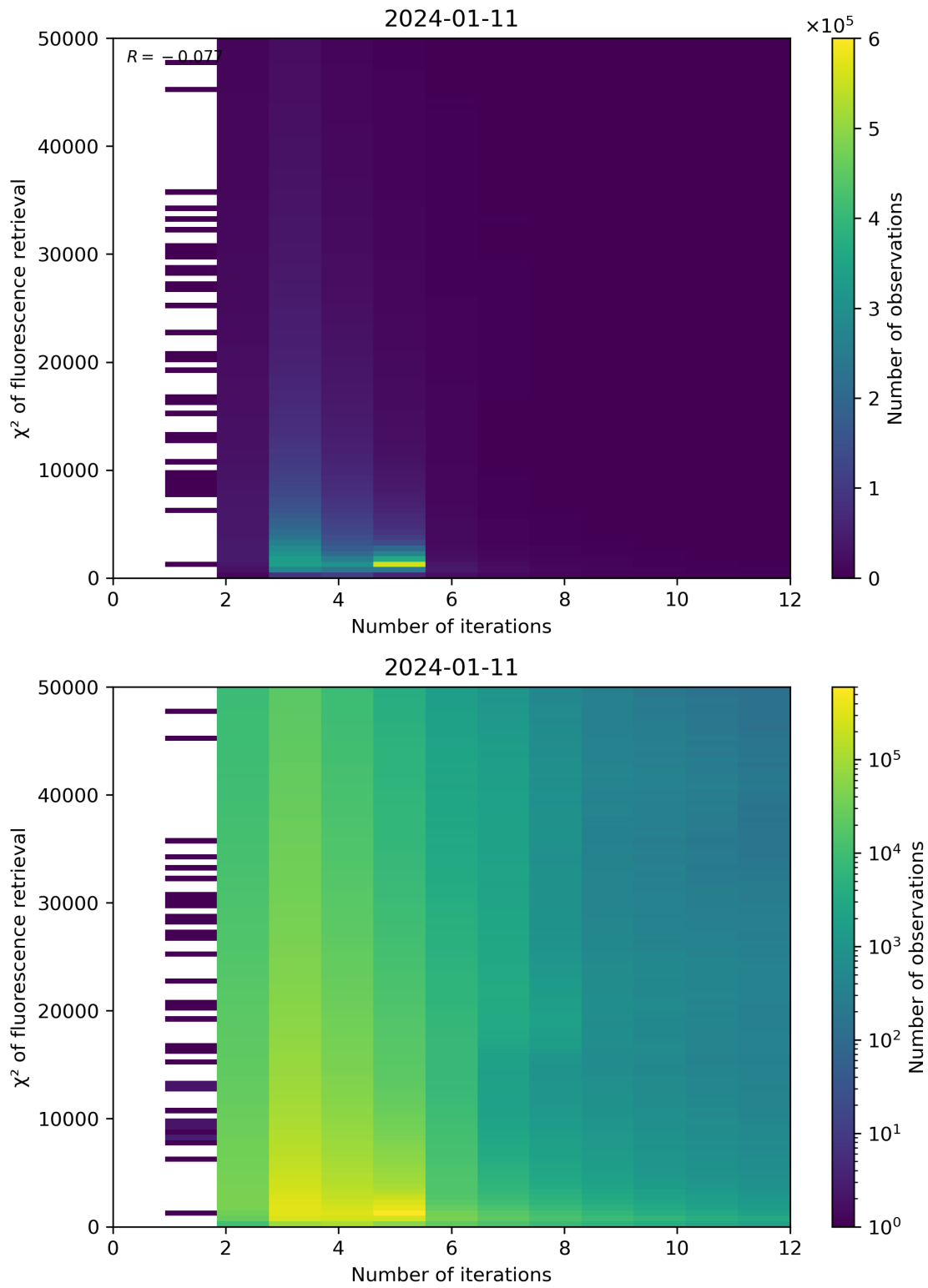
Figure 97: Scatter density plot of “Number of iterations” against “ \chi^2 of fluorescence retrieval” for 2024-01-10 to 2024-01-12.
