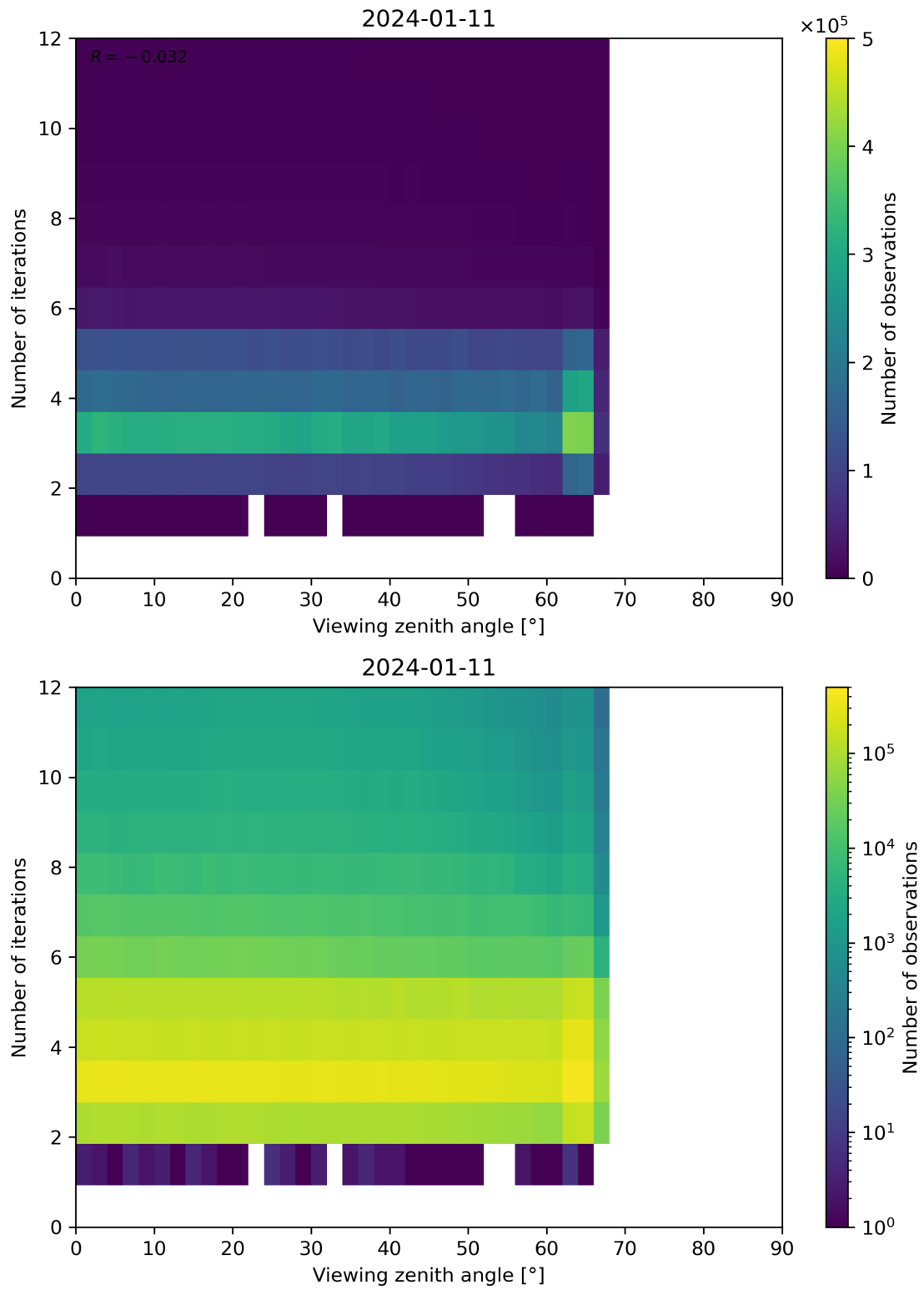
Figure 124: Scatter density plot of “Viewing zenith angle” against “Number of iterations” for 2024-01-10 to 2024-01-12.
