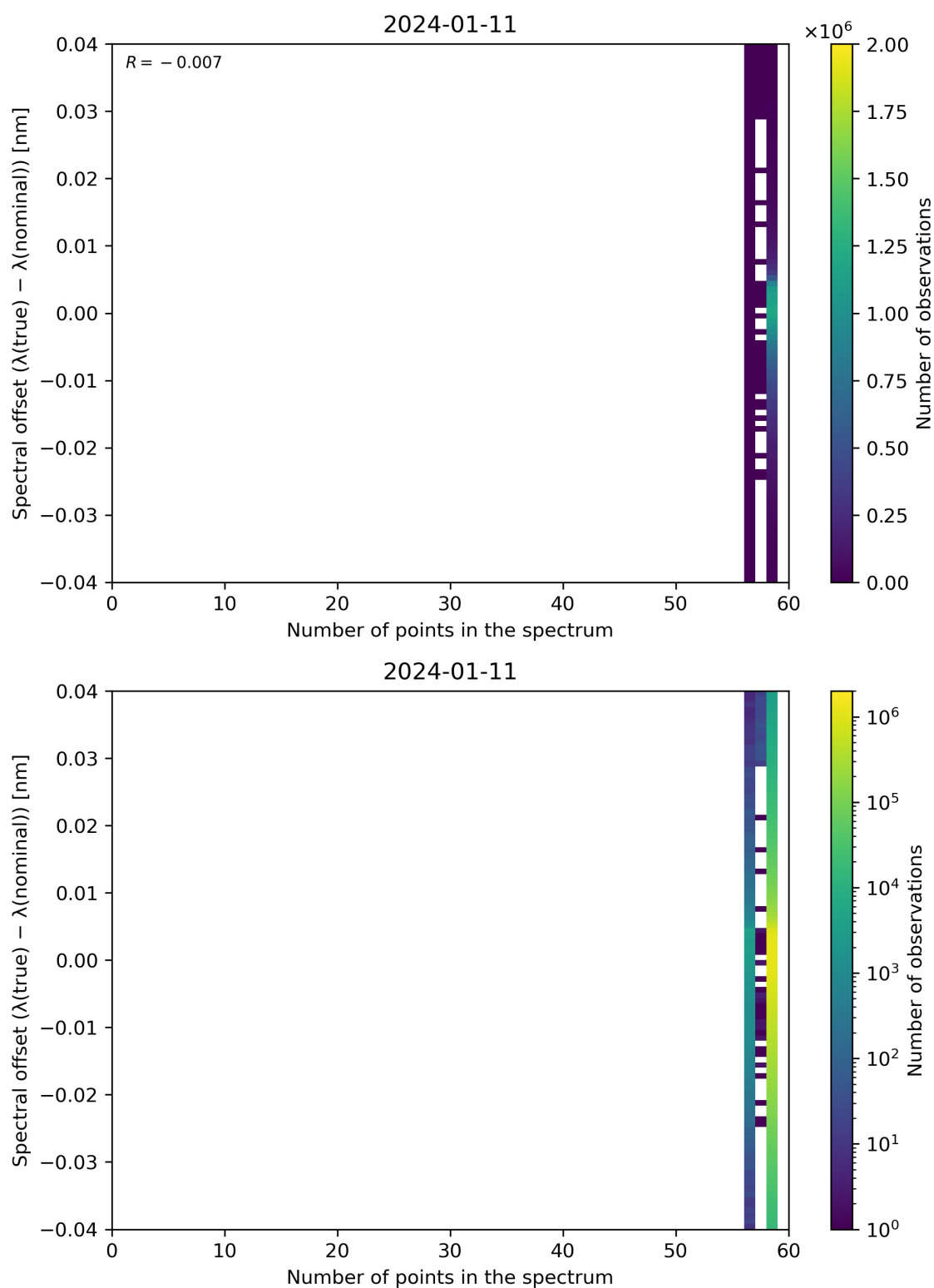
Figure 101: Scatter density plot of “Number of points in the spectrum” against “Spectral offset ( \lambda(\text{true}) - \lambda(\text{nominal}) )” for 2024-01-10 to 2024-01-12.
