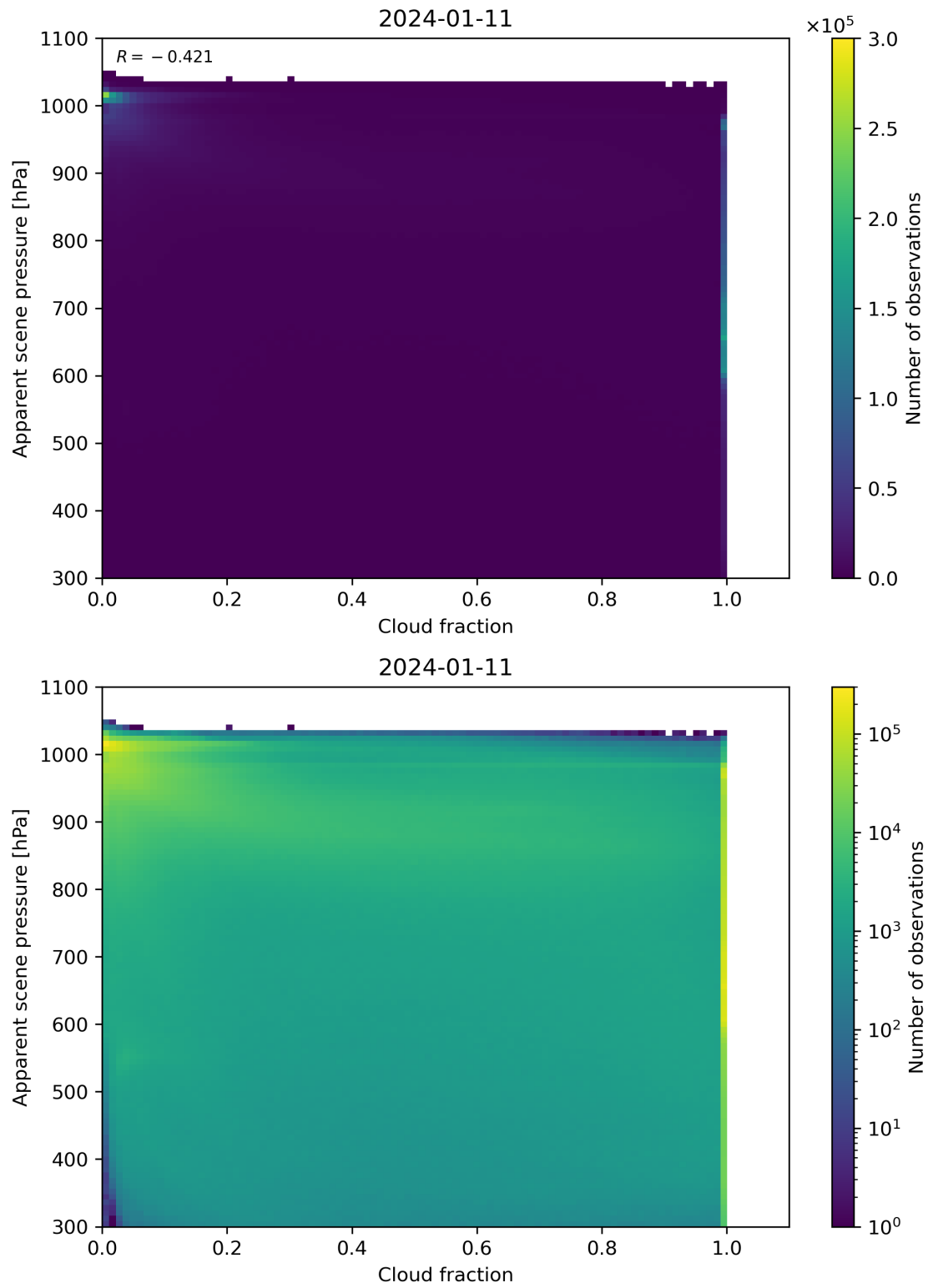
Figure 70: Scatter density plot of “Cloud fraction” against “Apparent scene pressure” for 2024-01-10 to 2024-01-12.
