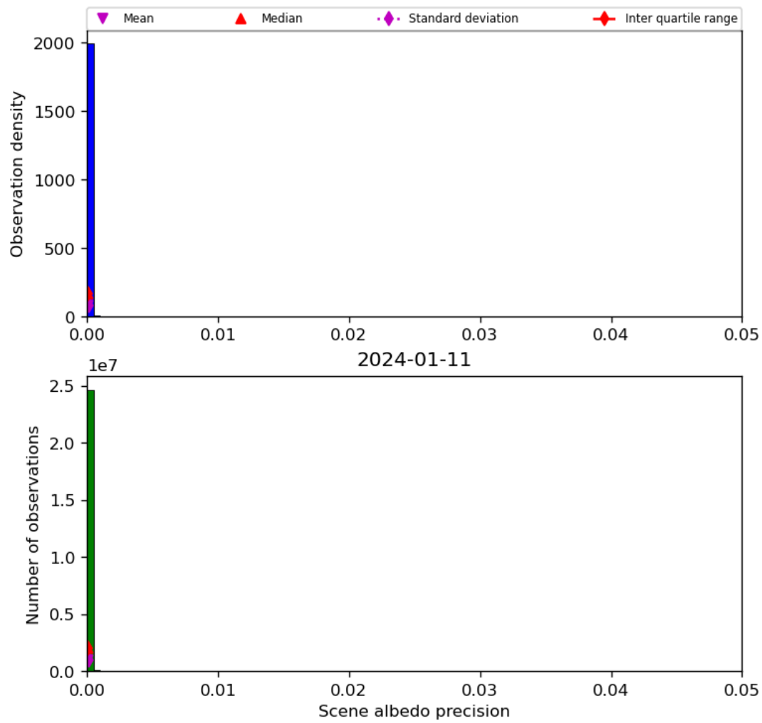
Figure 35: Histogram of “Scene albedo precision” for 2024-01-10 to 2024-01-12
