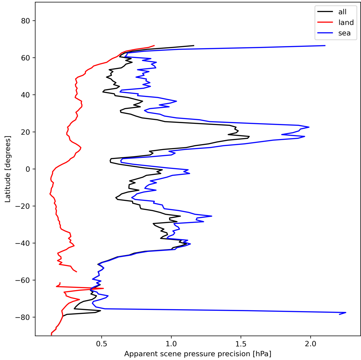
Figure 20: Zonal average of “Apparent scene pressure precision” for 2024-01-10 to 2024-01-12.
