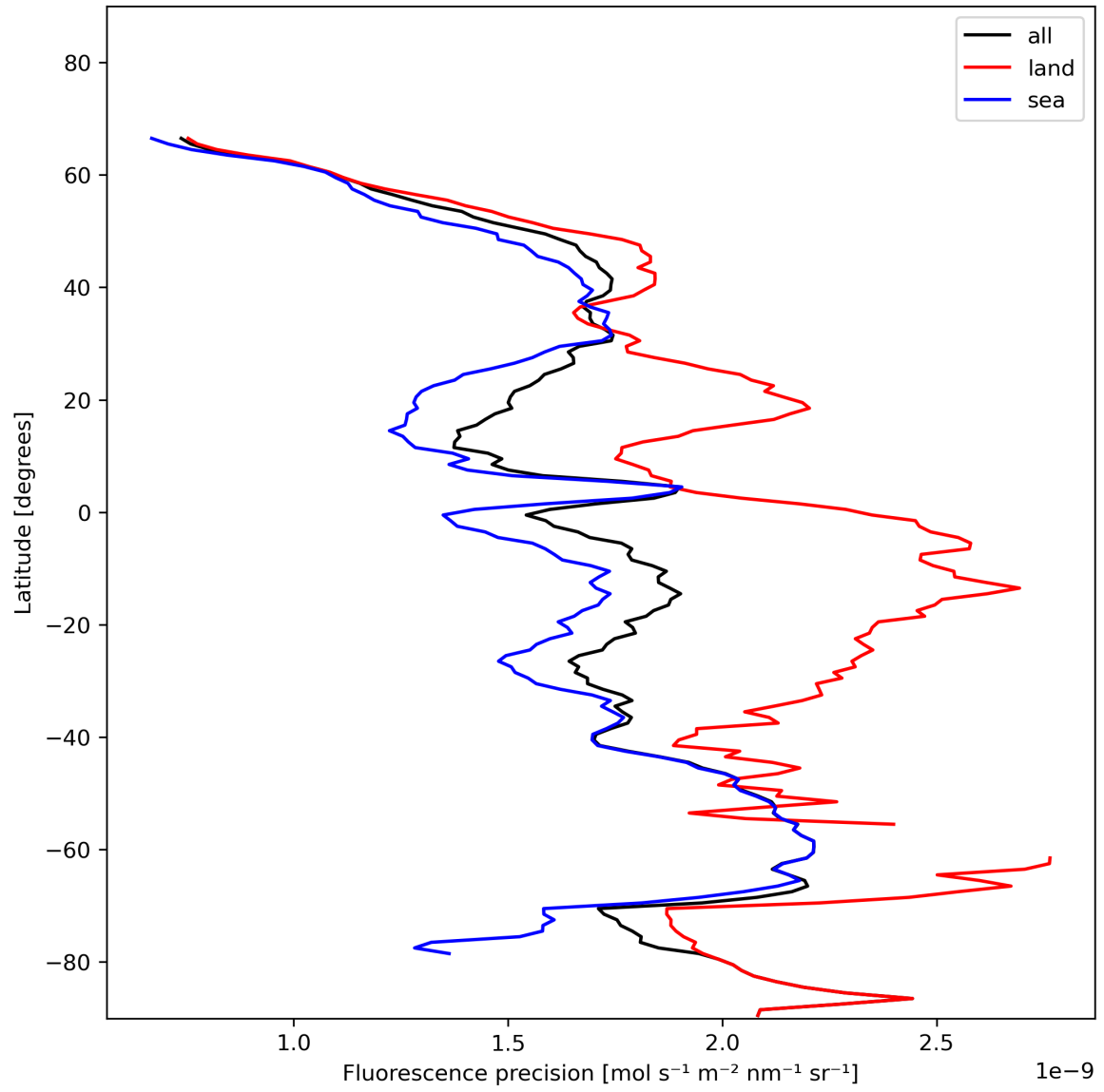
Figure 24: Zonal average of “Fluorescence precision” for 2024-01-10 to 2024-01-12.
