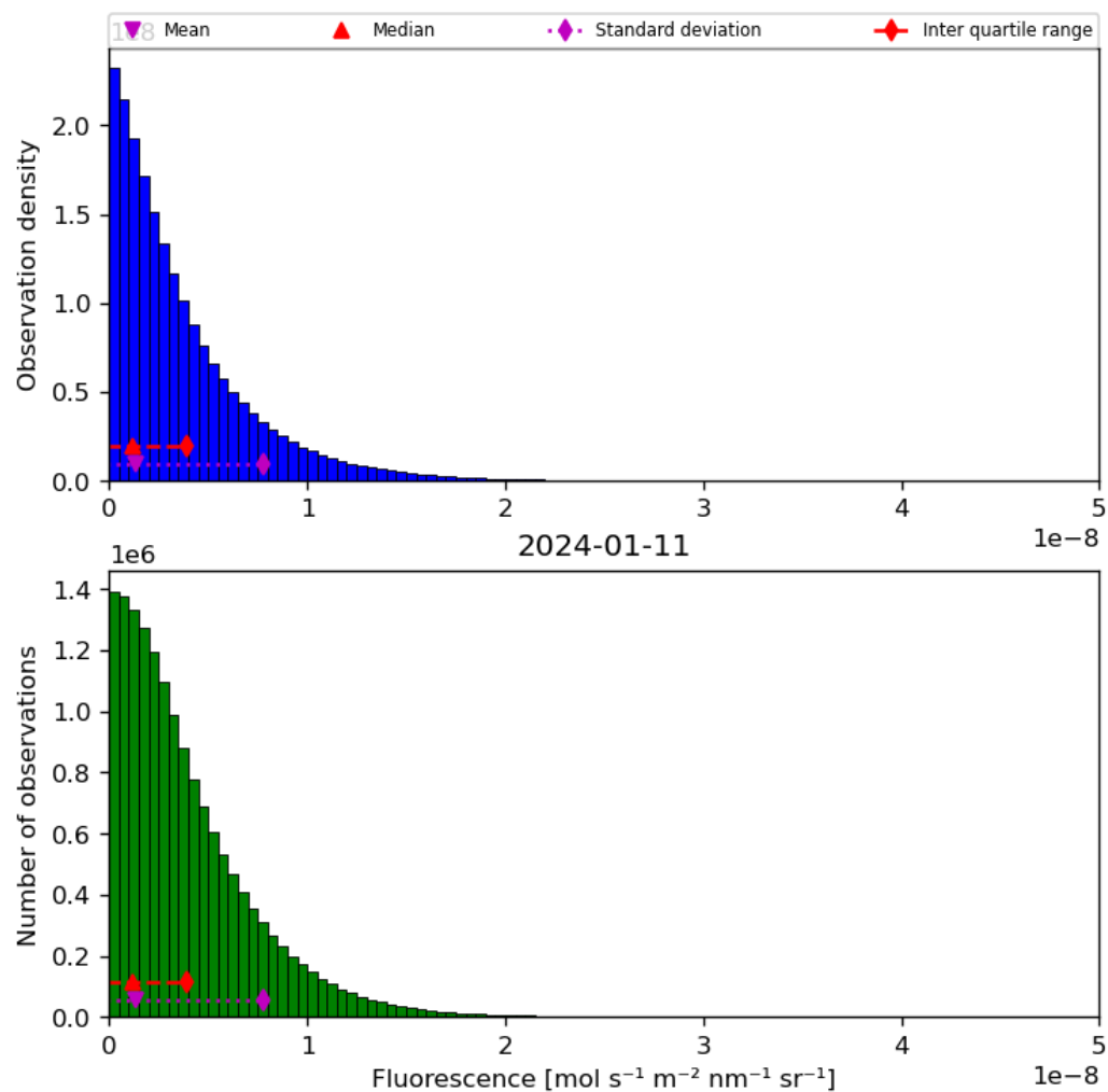
Figure 40: Histogram of “Fluorescence” for 2024-01-10 to 2024-01-12
