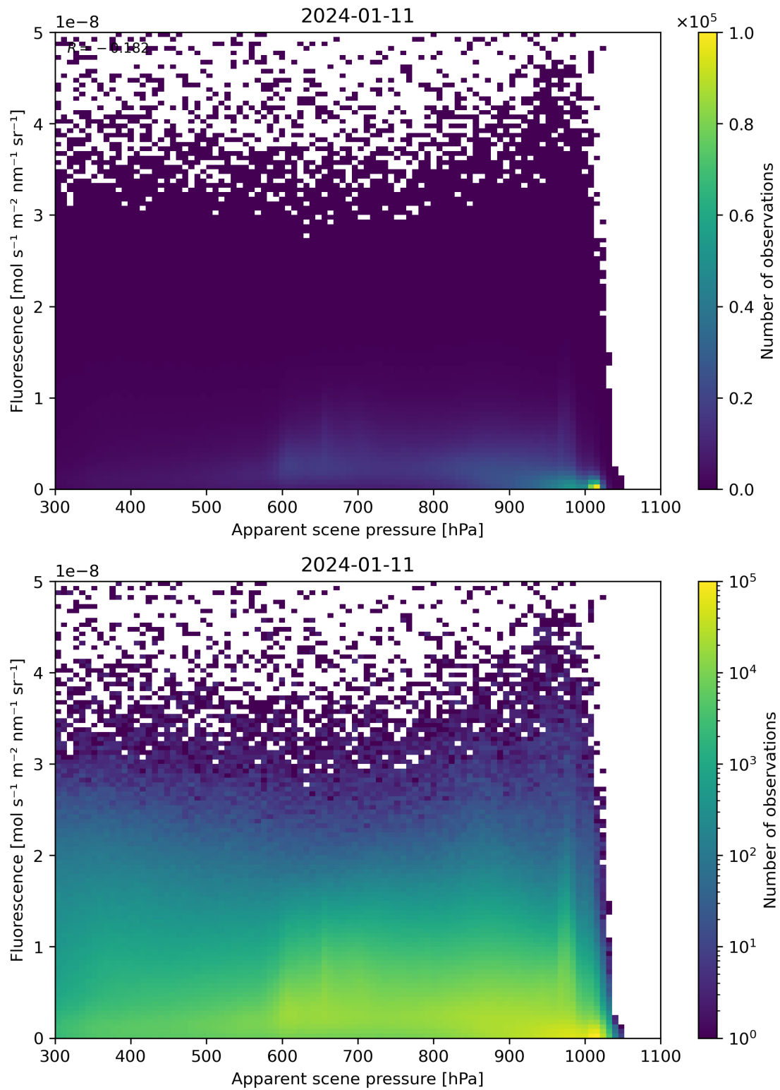
Figure 64: Scatter density plot of “Apparent scene pressure” against “Fluorescence” for 2024-01-10 to 2024-01-12.
