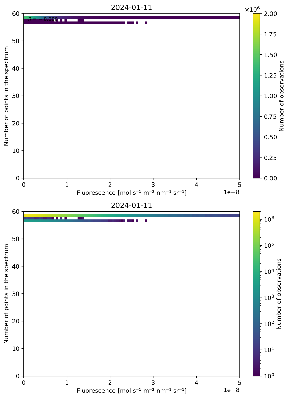
Figure 86: Scatter density plot of “Fluorescence” against “Number of points in the spectrum” for 2024-01-10 to 2024-01-12.
