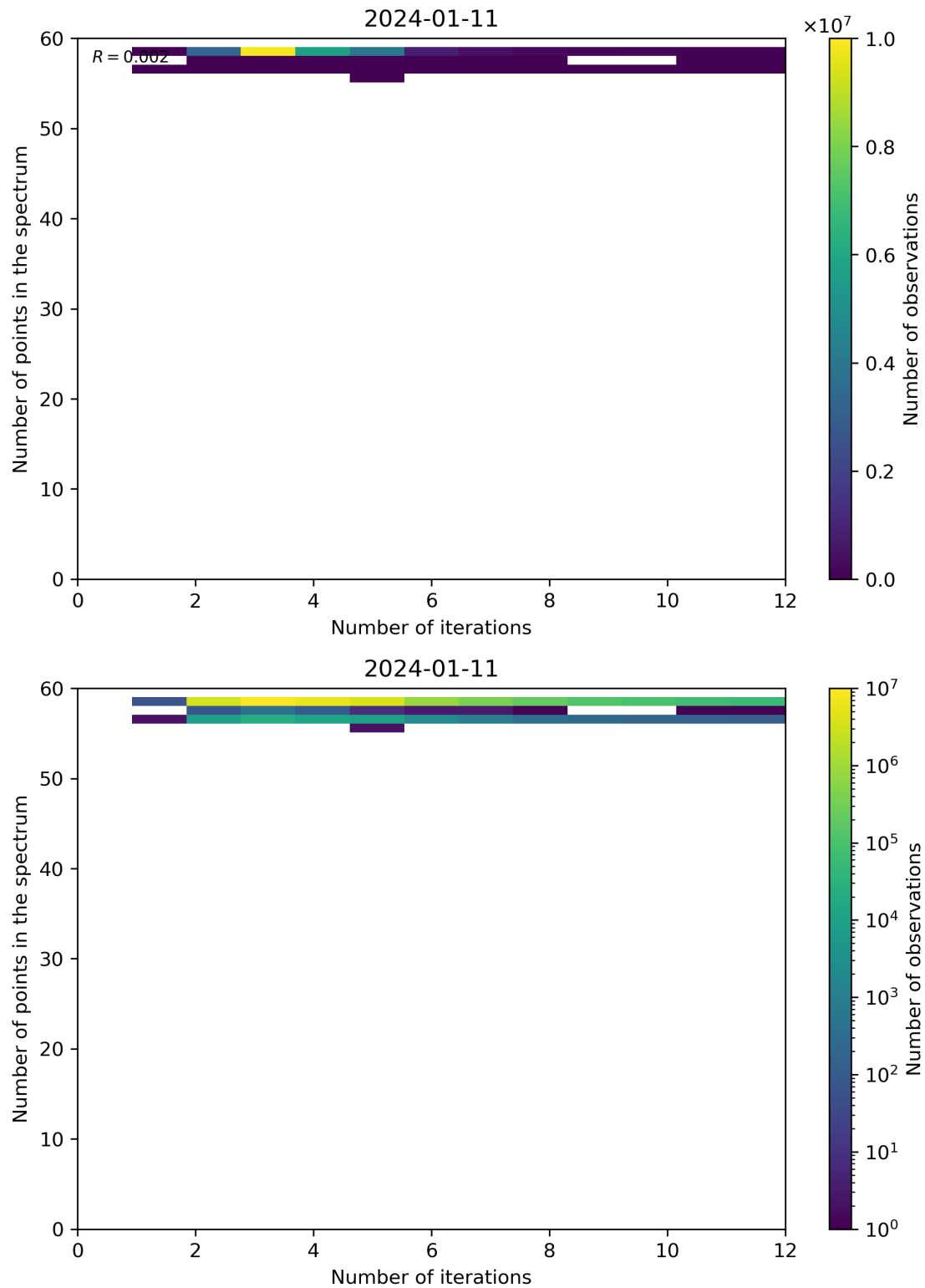
Figure 99: Scatter density plot of “Number of iterations” against “Number of points in the spectrum” for 2024-01-10 to 2024-01-12.
