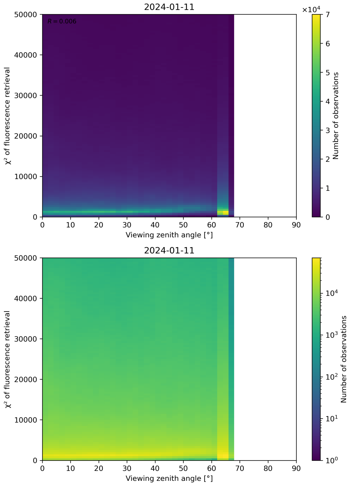
Figure 119: Scatter density plot of “Viewing zenith angle” against “ \chi^2 of fluorescence retrieval” for 2024-01-10 to 2024-01-12.
