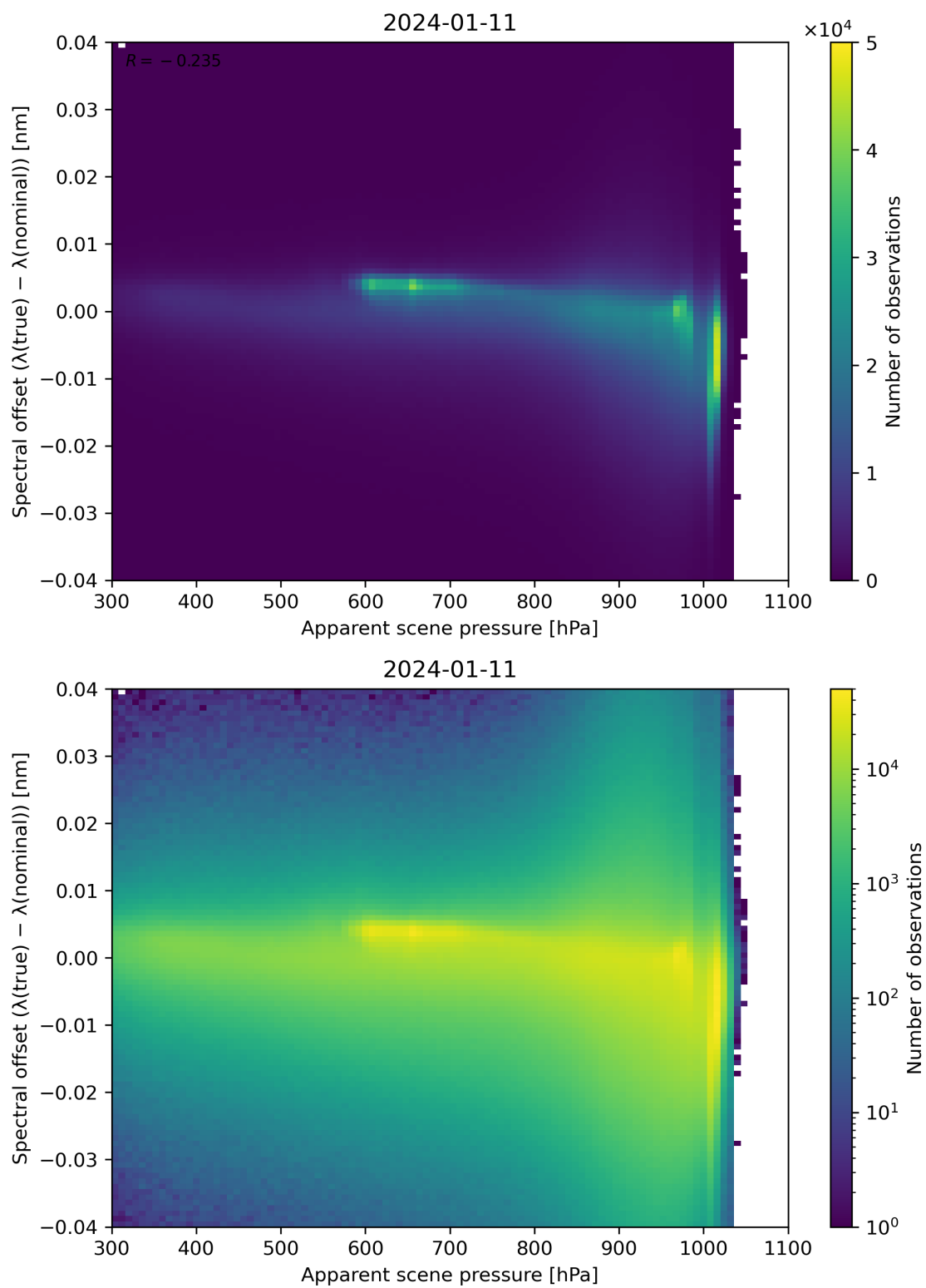
Figure 67: Scatter density plot of “Apparent scene pressure” against “Spectral offset ( \lambda(\text{true}) - \lambda(\text{nominal}) )” for 2024-01-10 to 2024-01-12.
