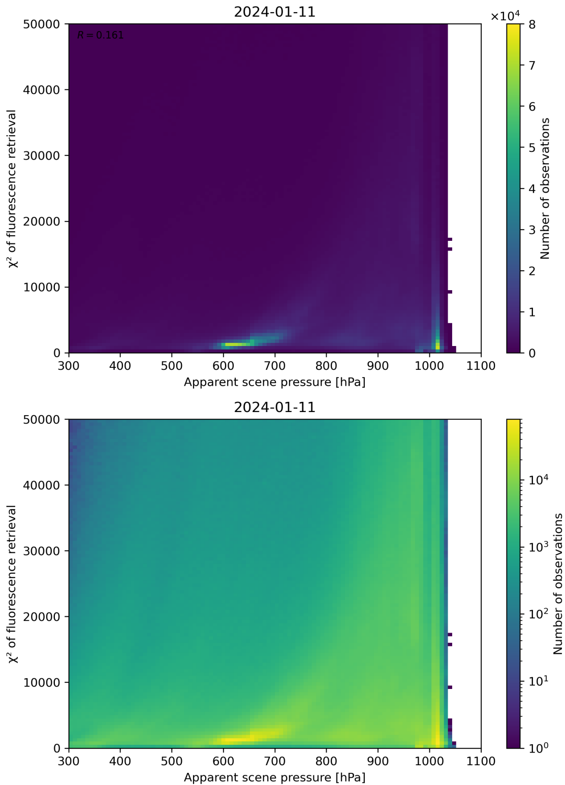
Figure 63: Scatter density plot of “Apparent scene pressure” against “ \chi^2 of fluorescence retrieval” for 2024-01-10 to 2024-01-12.
