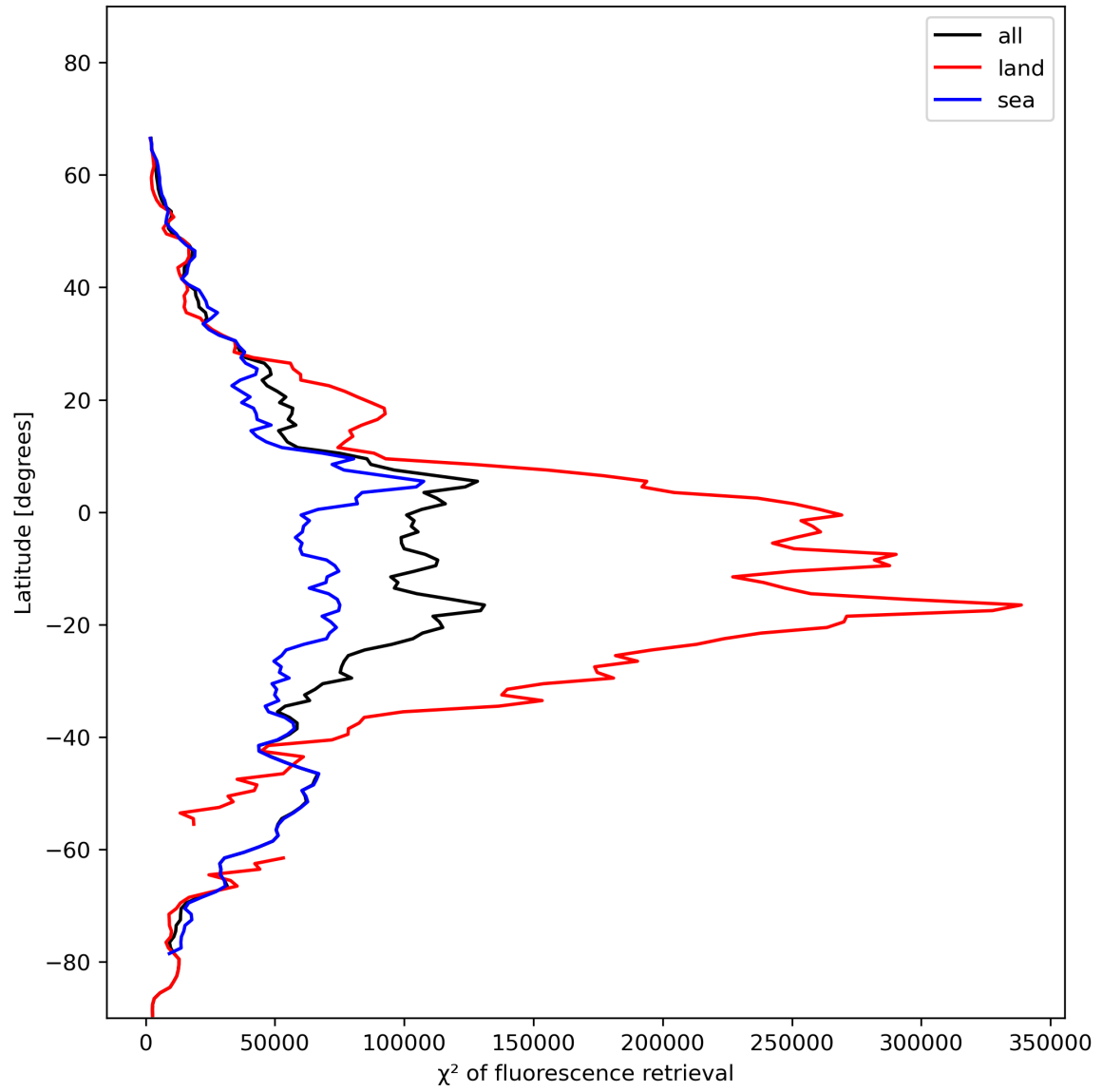
Figure 25: Zonal average of “ \chi^2 of fluorescence retrieval” for 2024-01-10 to 2024-01-12.
