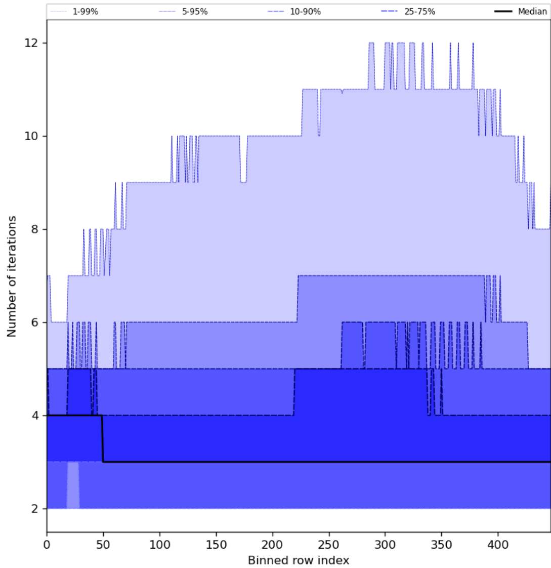
Figure 56: Along track statistics of “Number of iterations” for 2024-01-10 to 2024-01-12
