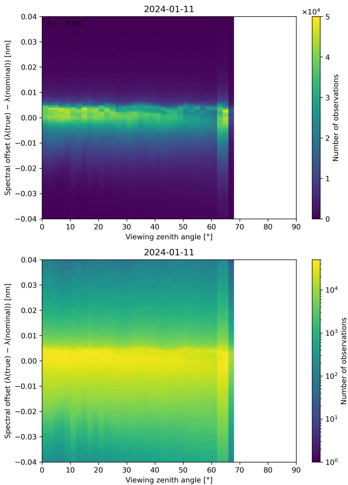
Figure 128: Scatter density plot of “Viewing zenith angle” against “Spectral offset ( \lambda(\text{true}) - \lambda(\text{nominal}) )” for 2024-01-10 to 2024-01-12.
