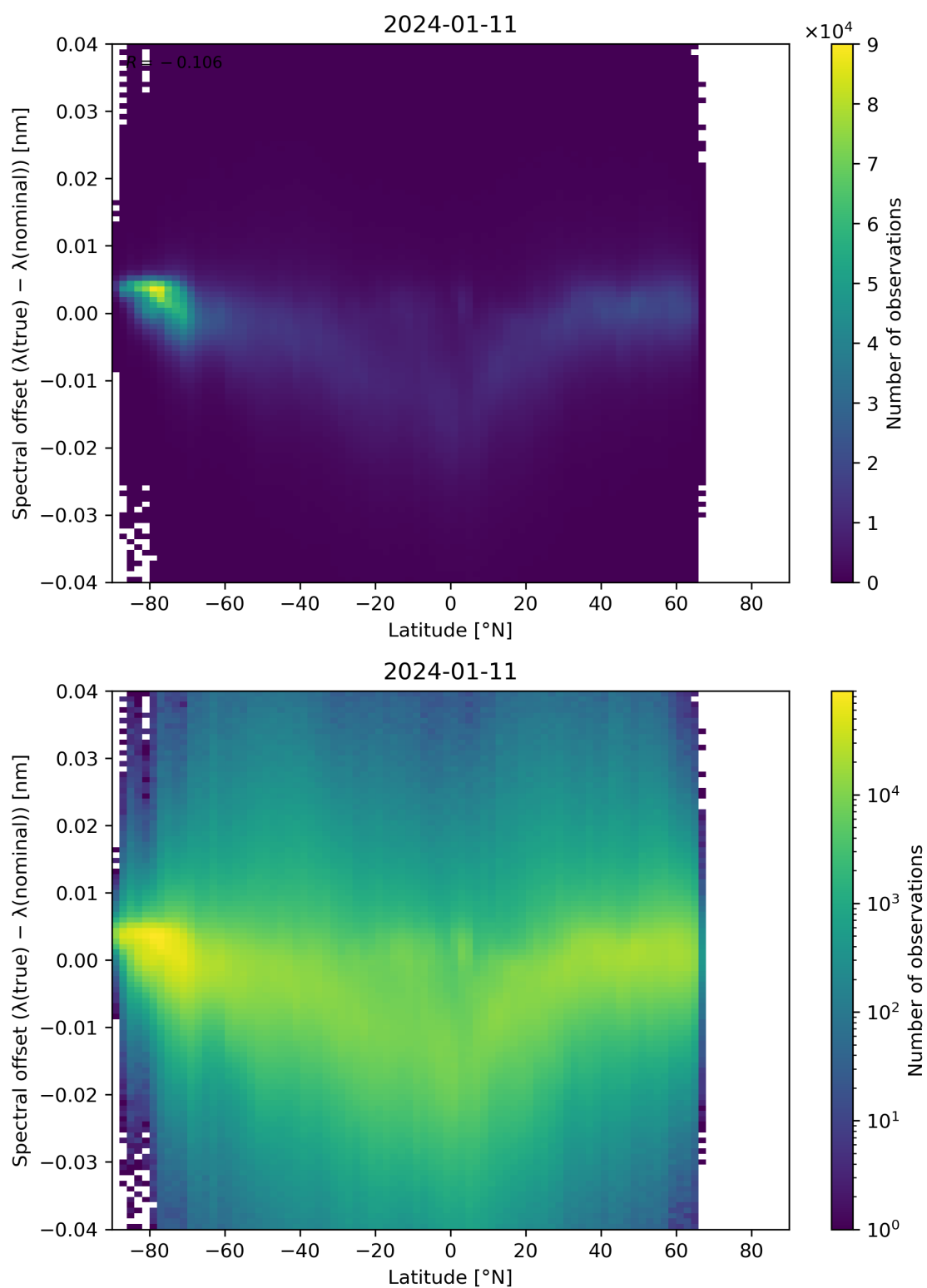
Figure 96: Scatter density plot of “Latitude” against “Spectral offset ( \lambda(\text{true}) - \lambda(\text{nominal}) )” for 2024-01-10 to 2024-01-12.
