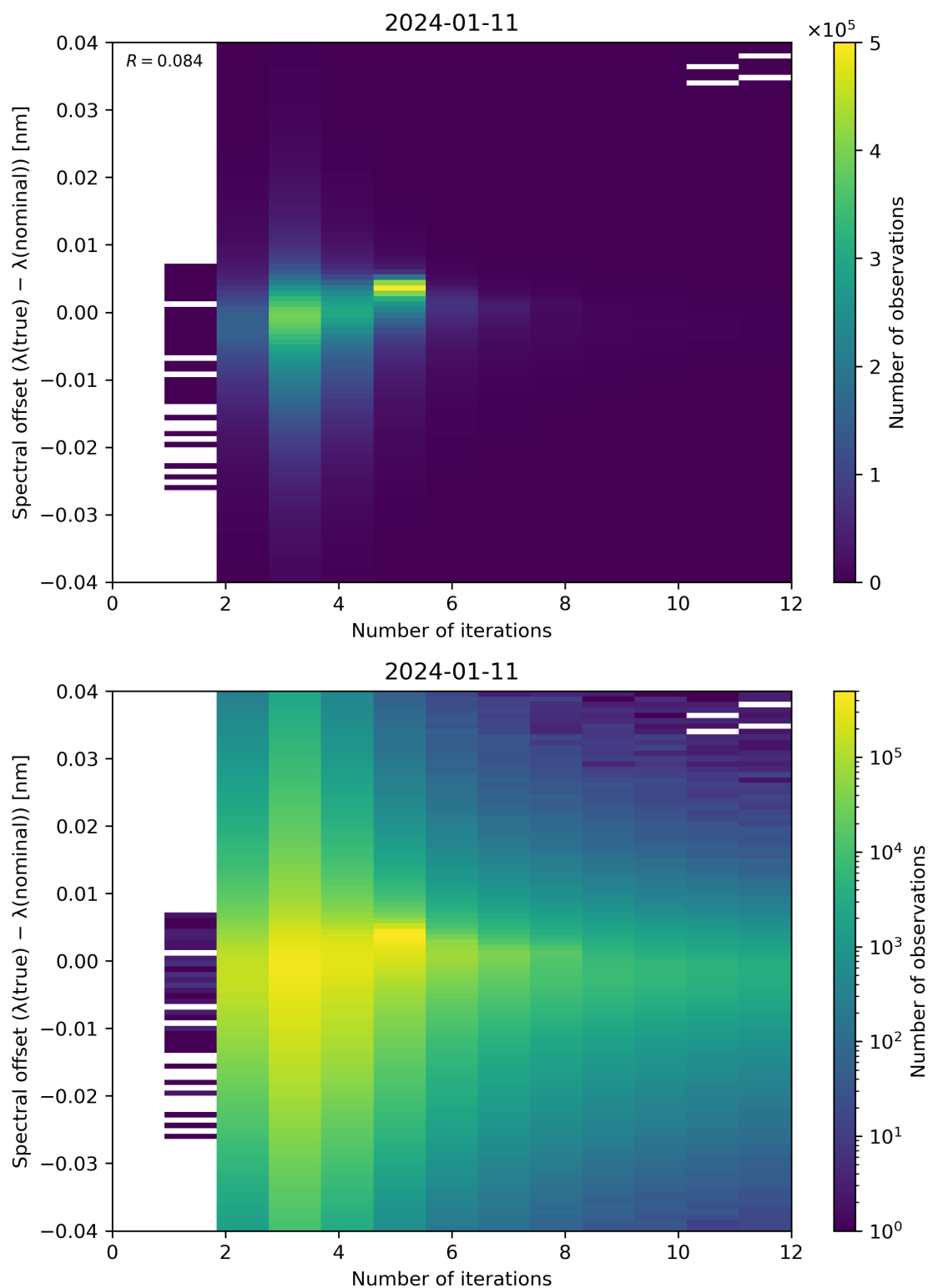
Figure 100: Scatter density plot of “Number of iterations” against “Spectral offset ( \lambda(\text{true}) - \lambda(\text{nominal}) )” for 2024-01-10 to 2024-01-12.
