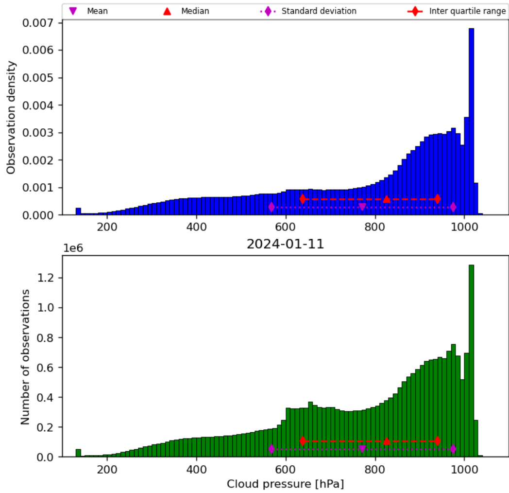
Figure 30: Histogram of “Cloud pressure” for 2024-01-10 to 2024-01-12
