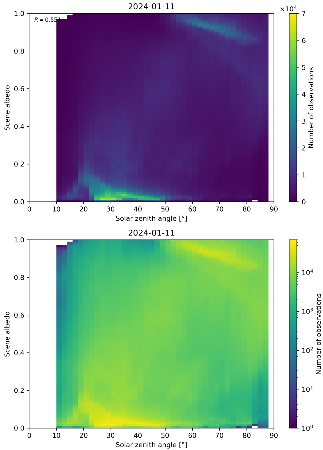
Figure 116: Scatter density plot of “Solar zenith angle” against “Scene albedo” for 2024-01-10 to 2024-01-12.
