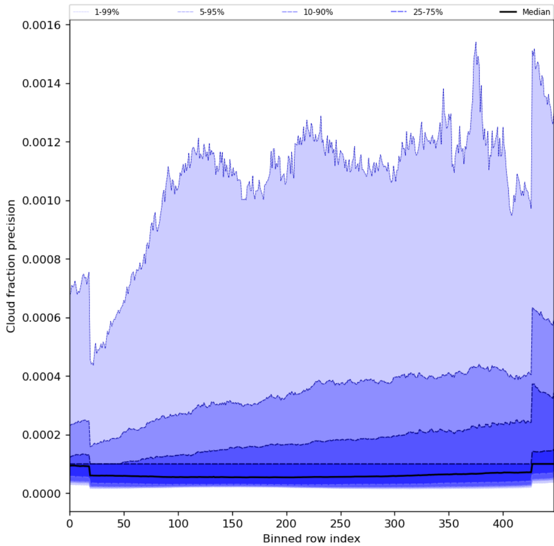
Figure 50: Along track statistics of “Cloud fraction precision” for 2024-01-10 to 2024-01-12
