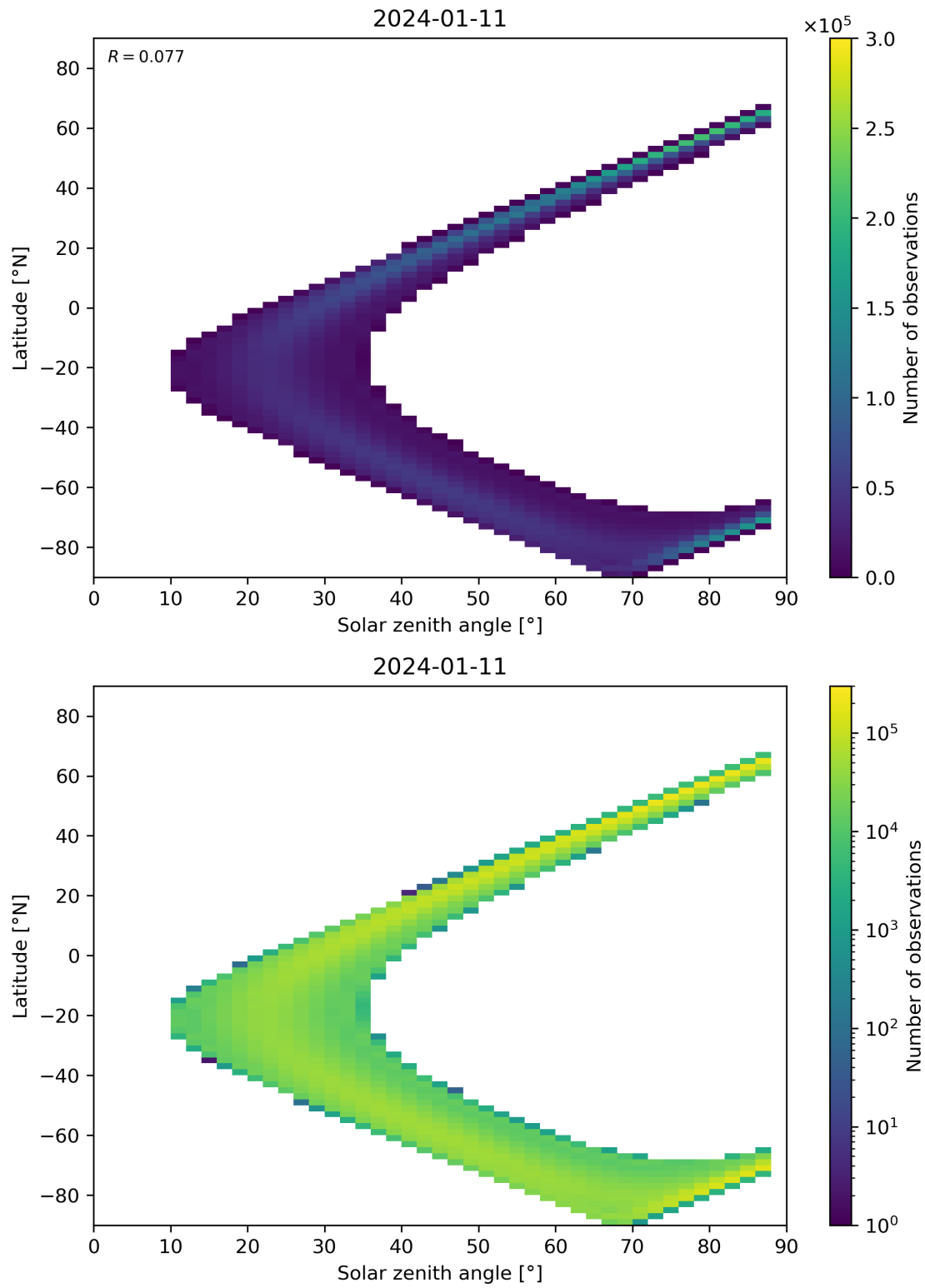
Figure 113: Scatter density plot of “Solar zenith angle” against “Latitude” for 2024-01-10 to 2024-01-12.
