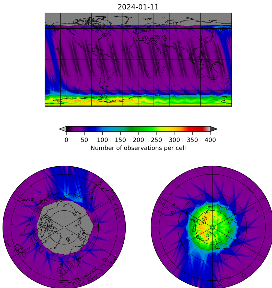
Figure 11: Map of the number of observations for 2024-01-10 to 2024-01-12
