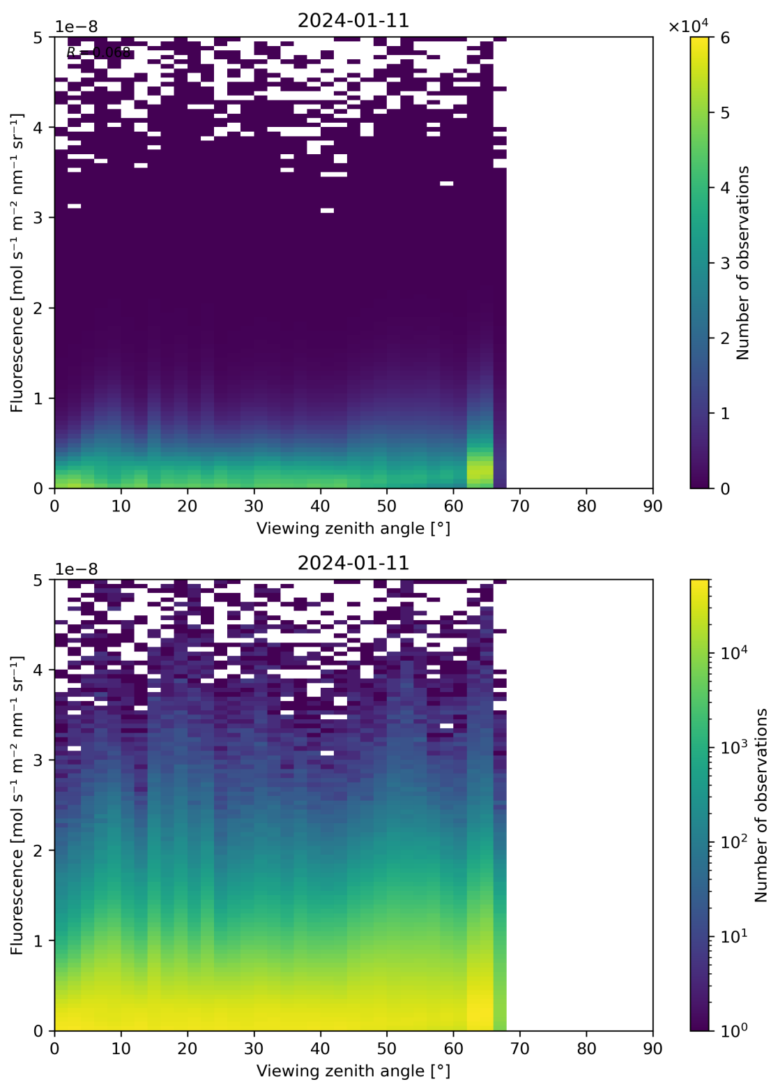
Figure 122: Scatter density plot of “Viewing zenith angle” against “Fluorescence” for 2024-01-10 to 2024-01-12.
