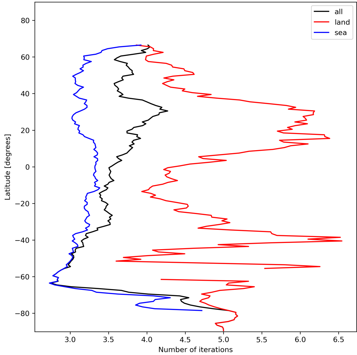
Figure 22: Zonal average of “Number of iterations” for 2024-01-10 to 2024-01-12.
