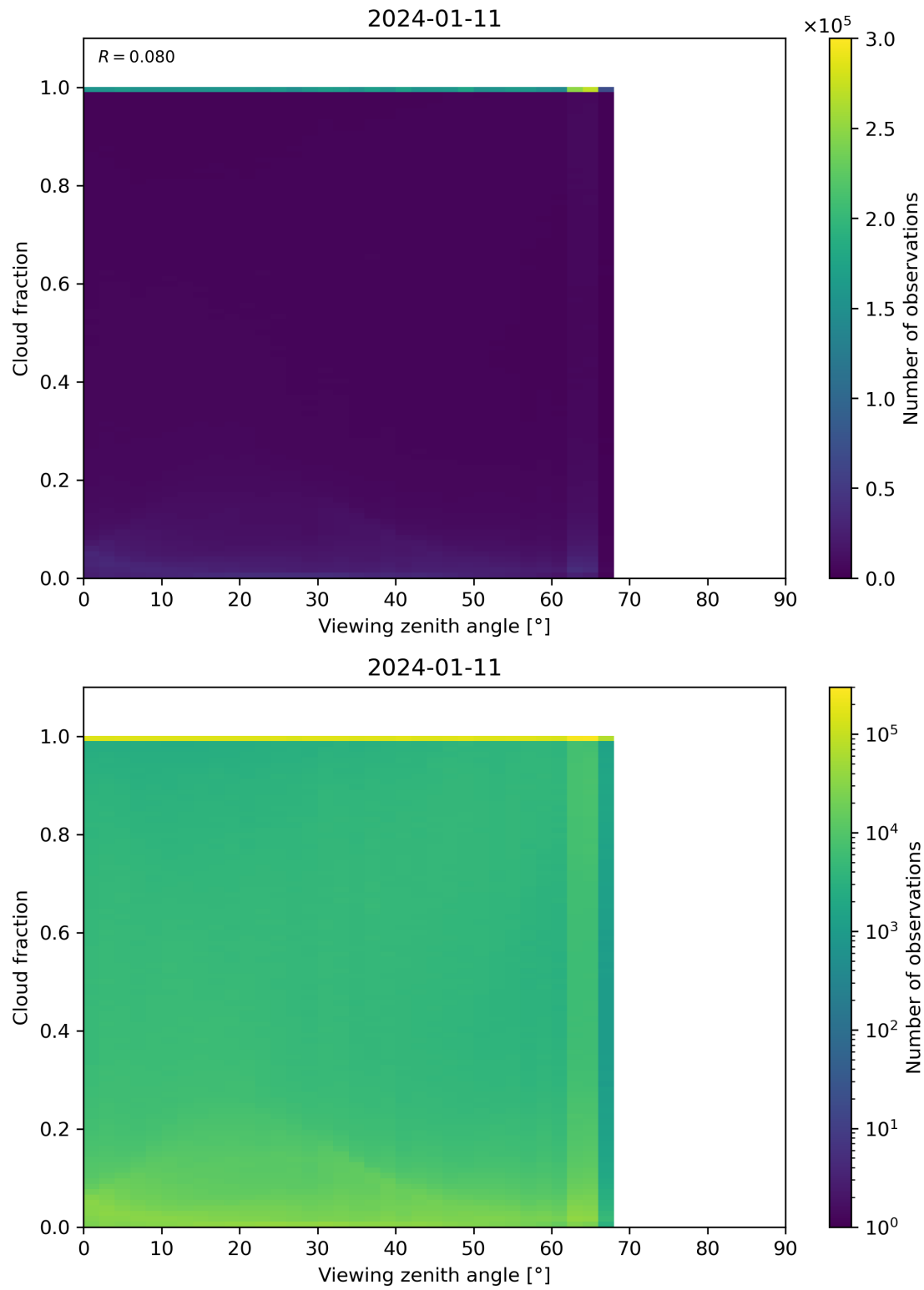
Figure 120: Scatter density plot of “Viewing zenith angle” against “Cloud fraction” for 2024-01-10 to 2024-01-12.
