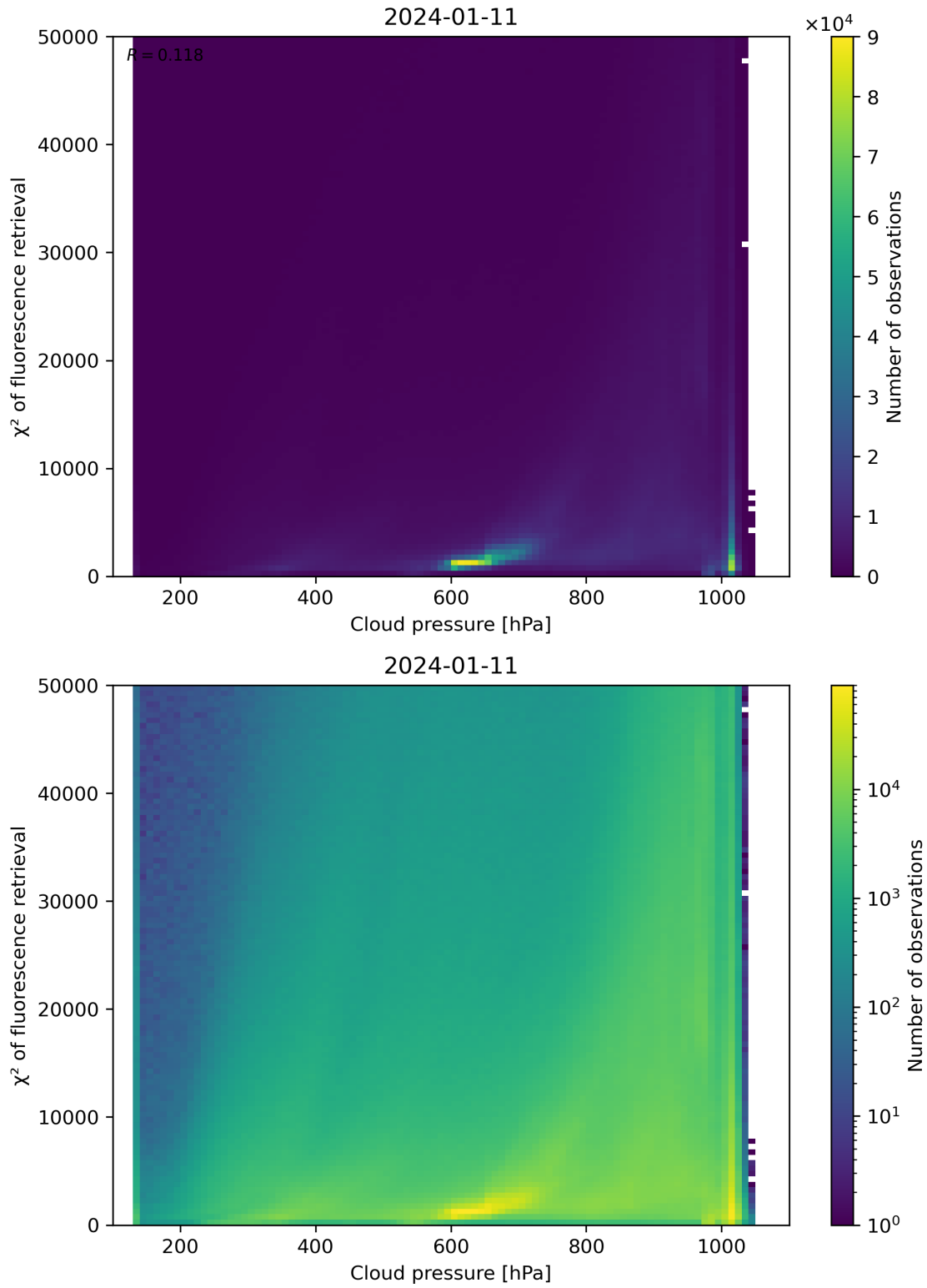
Figure 78: Scatter density plot of “Cloud pressure” against “ \chi^2 of fluorescence retrieval” for 2024-01-10 to 2024-01-12.
