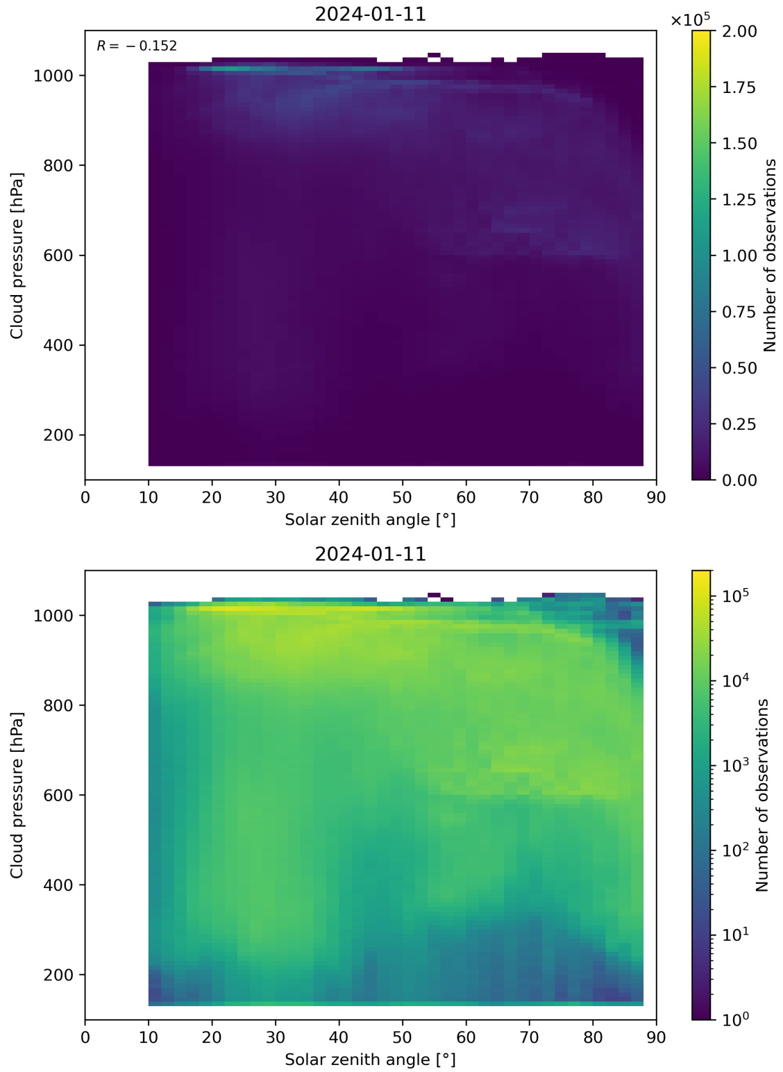
Figure 111: Scatter density plot of “Solar zenith angle” against “Cloud pressure” for 2024-01-10 to 2024-01-12.
