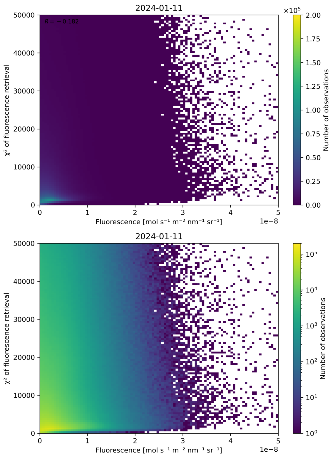
Figure 85: Scatter density plot of “Fluorescence” against “ \chi^2 of fluorescence retrieval” for 2024-01-10 to 2024-01-12.
