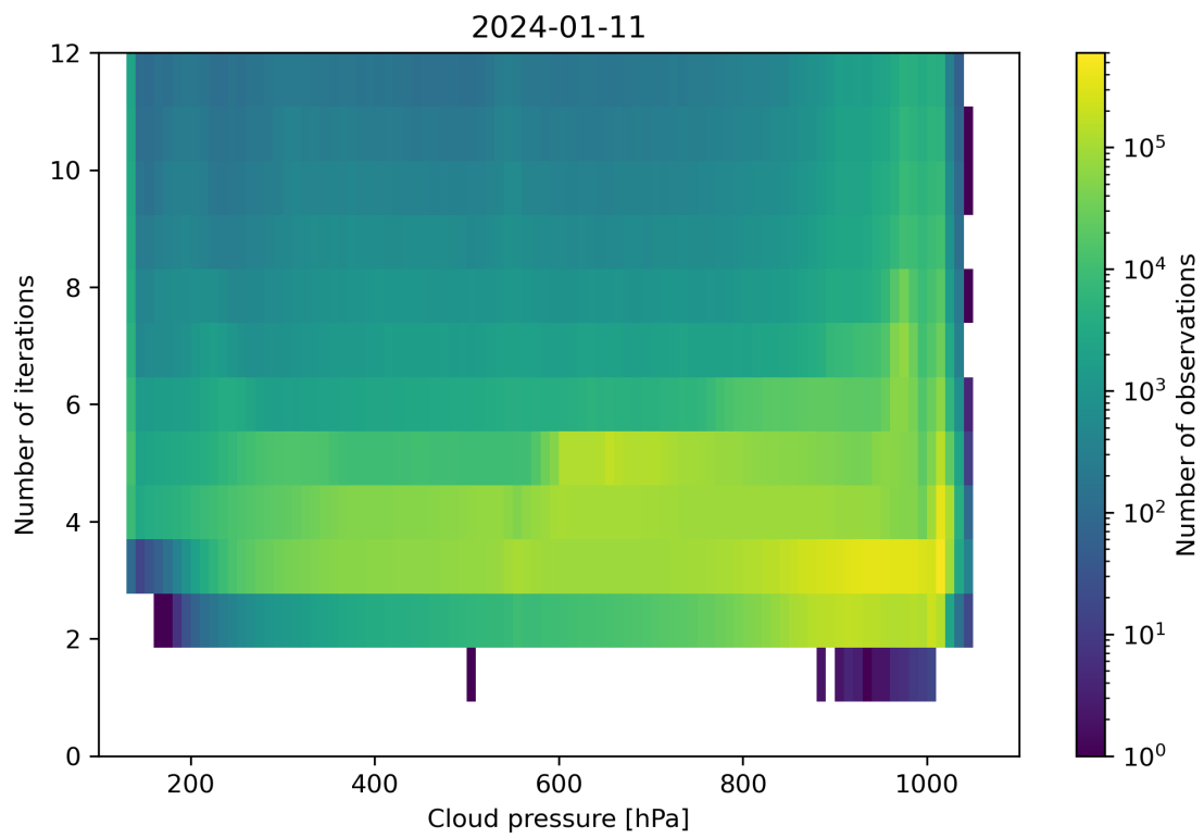
Figure 81: Scatter density plot of “Cloud pressure” against “Number of iterations” for 2024-01-10 to 2024-01-12.
