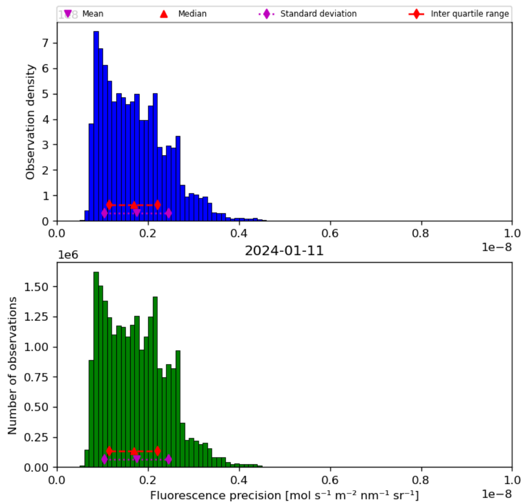
Figure 41: Histogram of “Fluorescence precision” for 2024-01-10 to 2024-01-12
