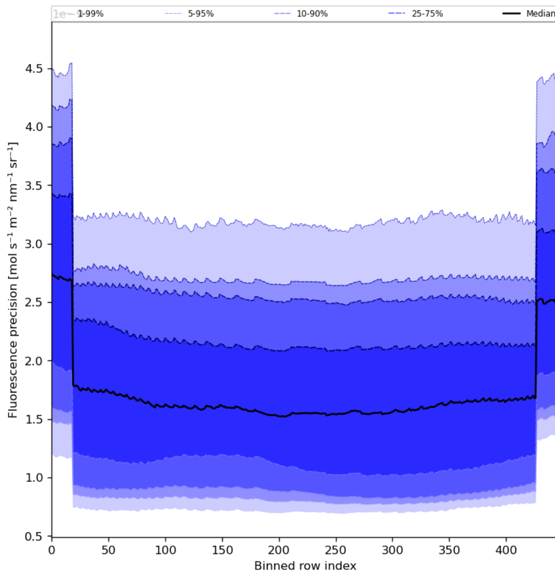
Figure 58: Along track statistics of “Fluorescence precision” for 2024-01-10 to 2024-01-12
