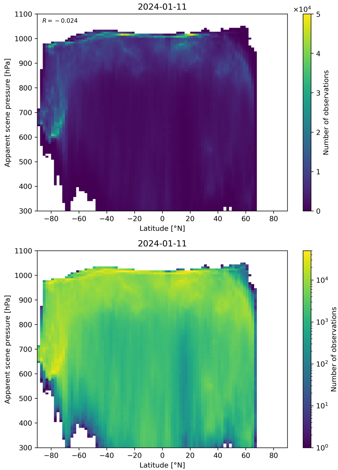
Figure 88: Scatter density plot of “Latitude” against “Apparent scene pressure” for 2024-01-10 to 2024-01-12.
