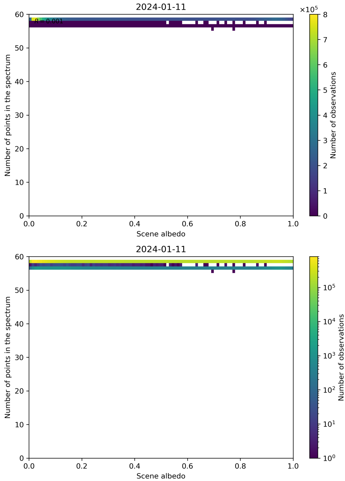
Figure 106: Scatter density plot of “Scene albedo” against “Number of points in the spectrum” for 2024-01-10 to 2024-01-12.
