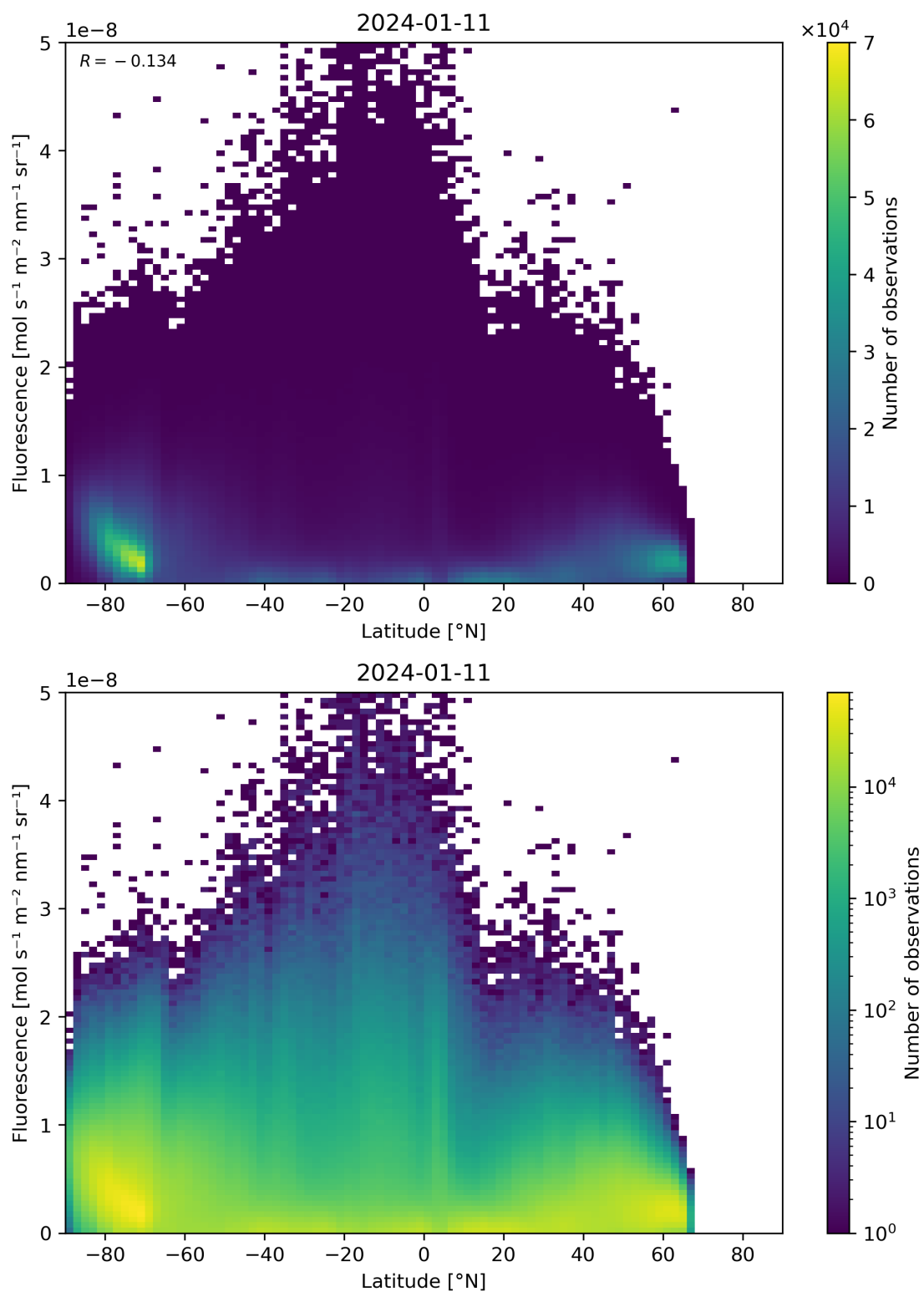
Figure 92: Scatter density plot of “Latitude” against “Fluorescence” for 2024-01-10 to 2024-01-12.
