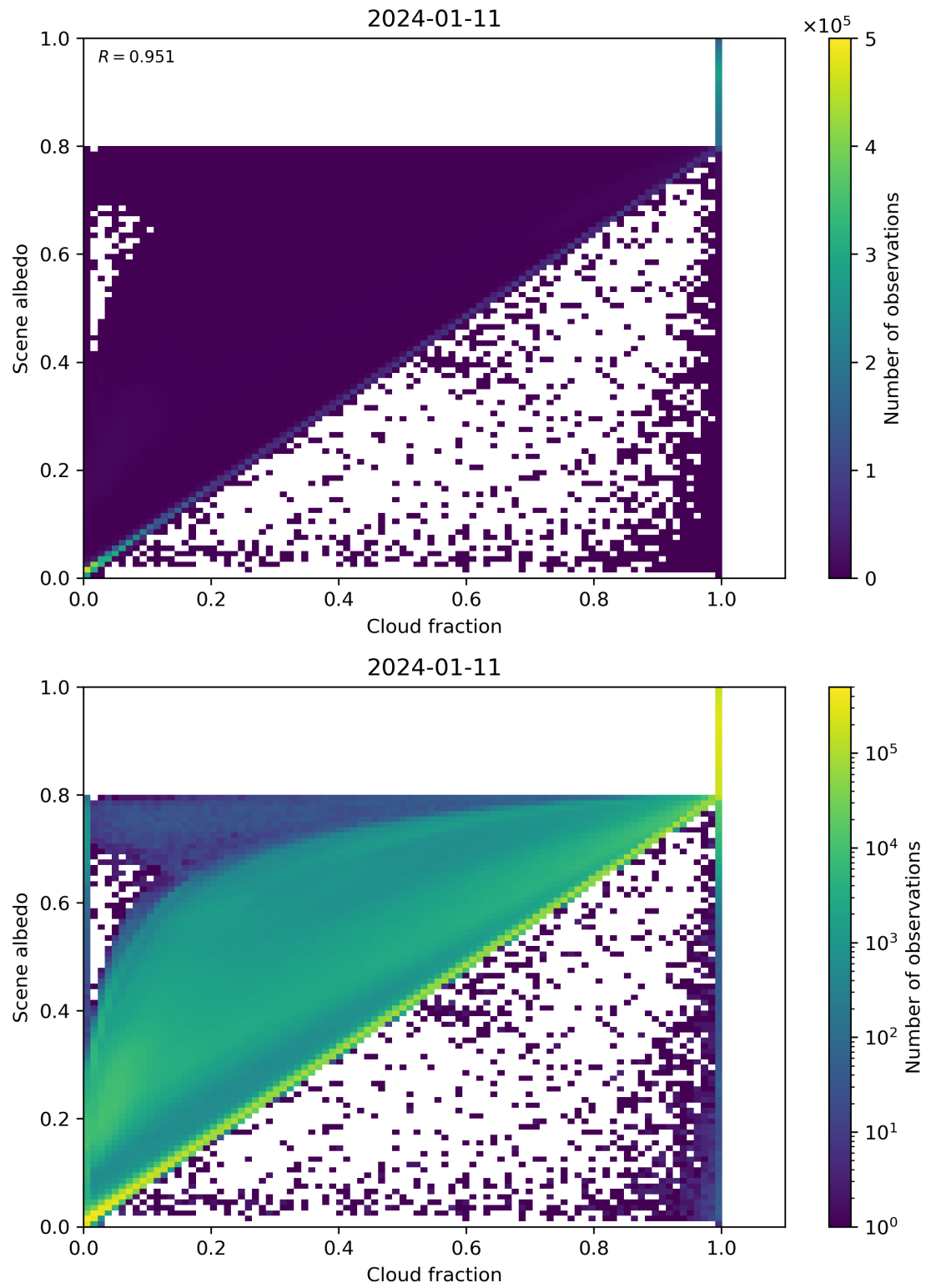
Figure 75: Scatter density plot of “Cloud fraction” against “Scene albedo” for 2024-01-10 to 2024-01-12.
