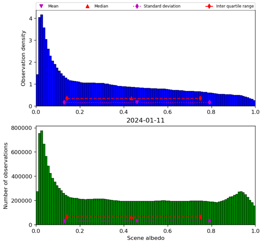
Figure 34: Histogram of “Scene albedo” for 2024-01-10 to 2024-01-12
