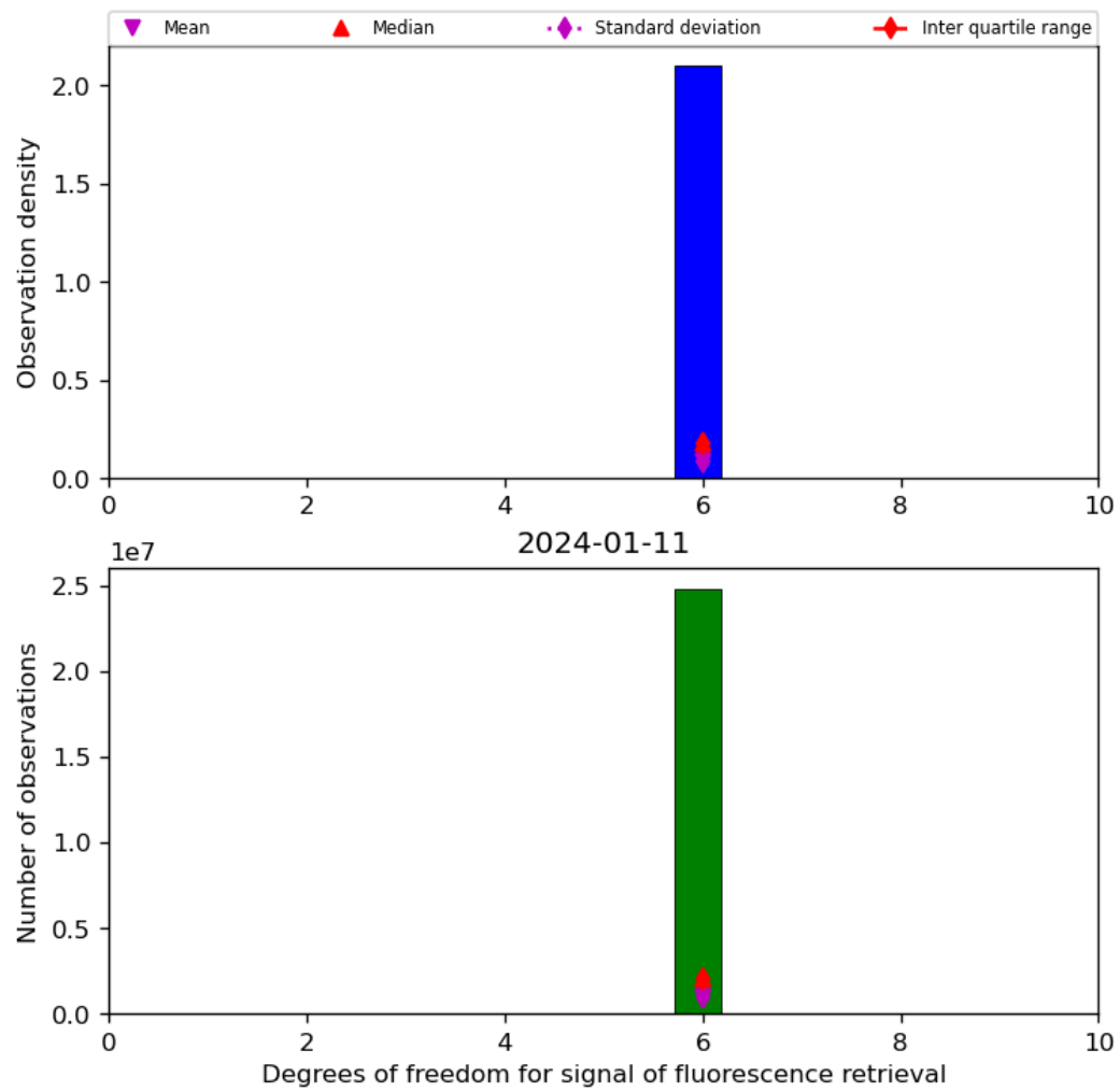
Figure 43: Histogram of “Degrees of freedom for signal of fluorescence retrieval” for 2024-01-10 to 2024-01-12
