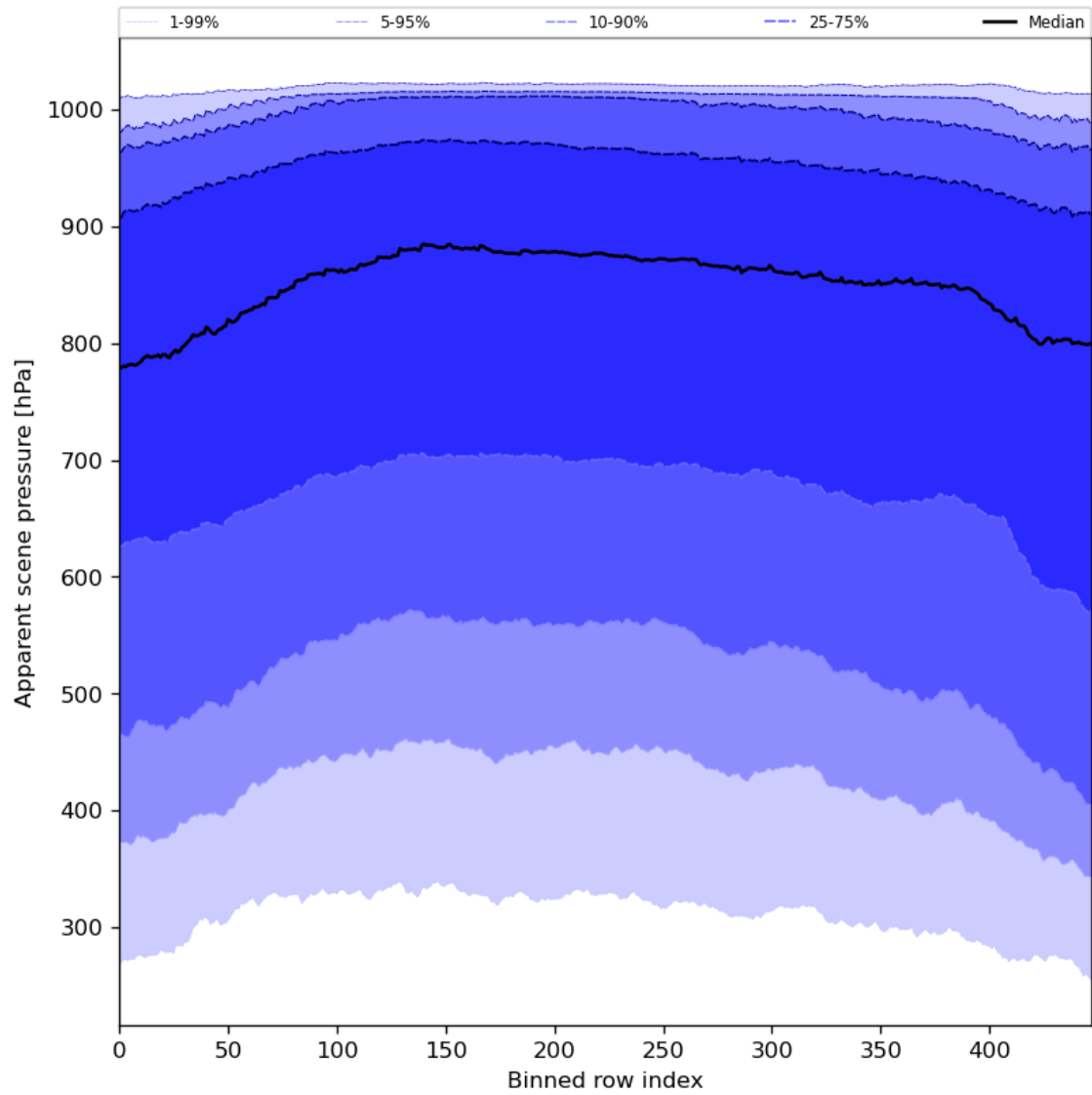
Figure 53: Along track statistics of “Apparent scene pressure” for 2024-01-10 to 2024-01-12
