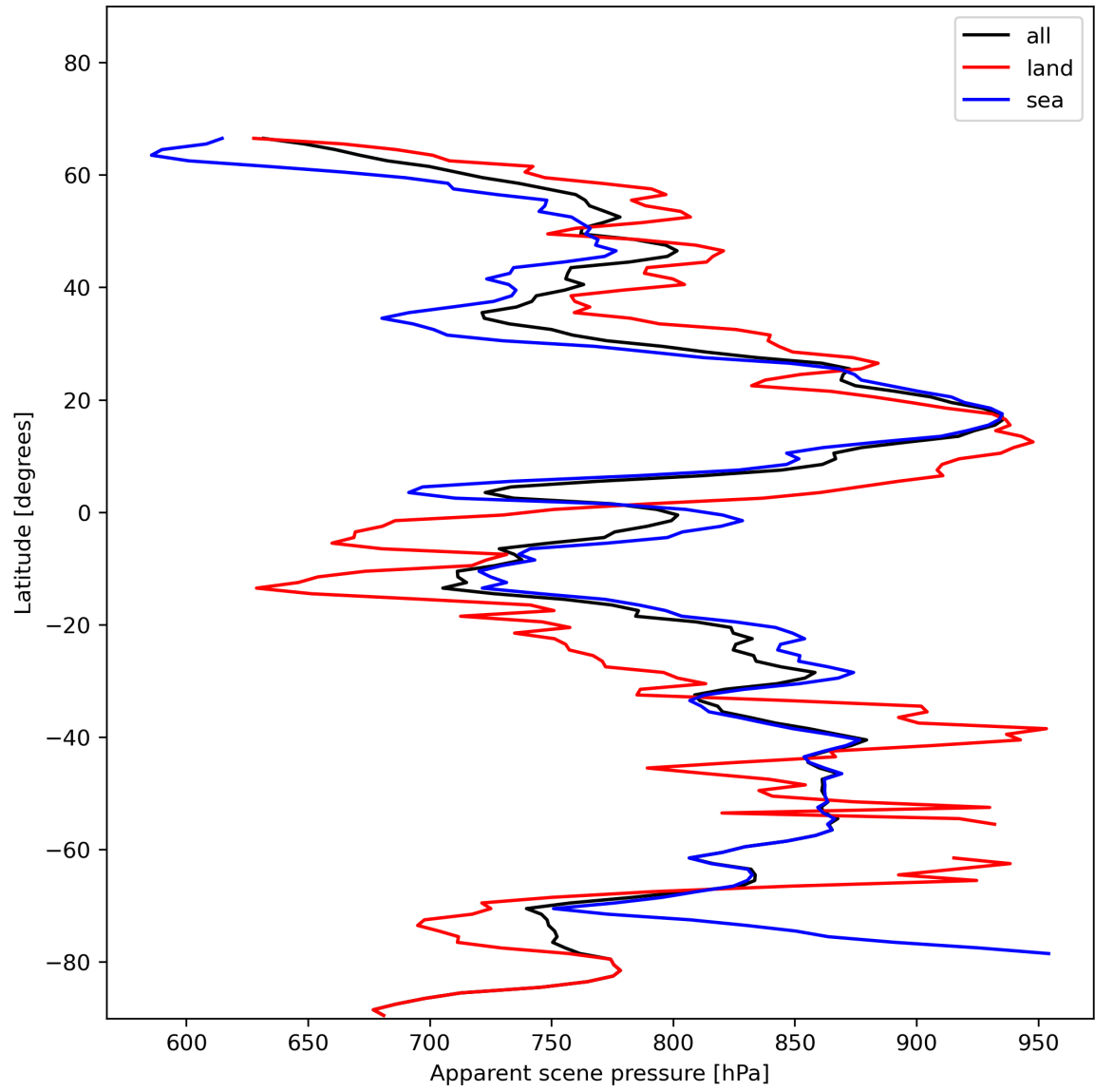
Figure 19: Zonal average of “Apparent scene pressure” for 2024-01-10 to 2024-01-12.
