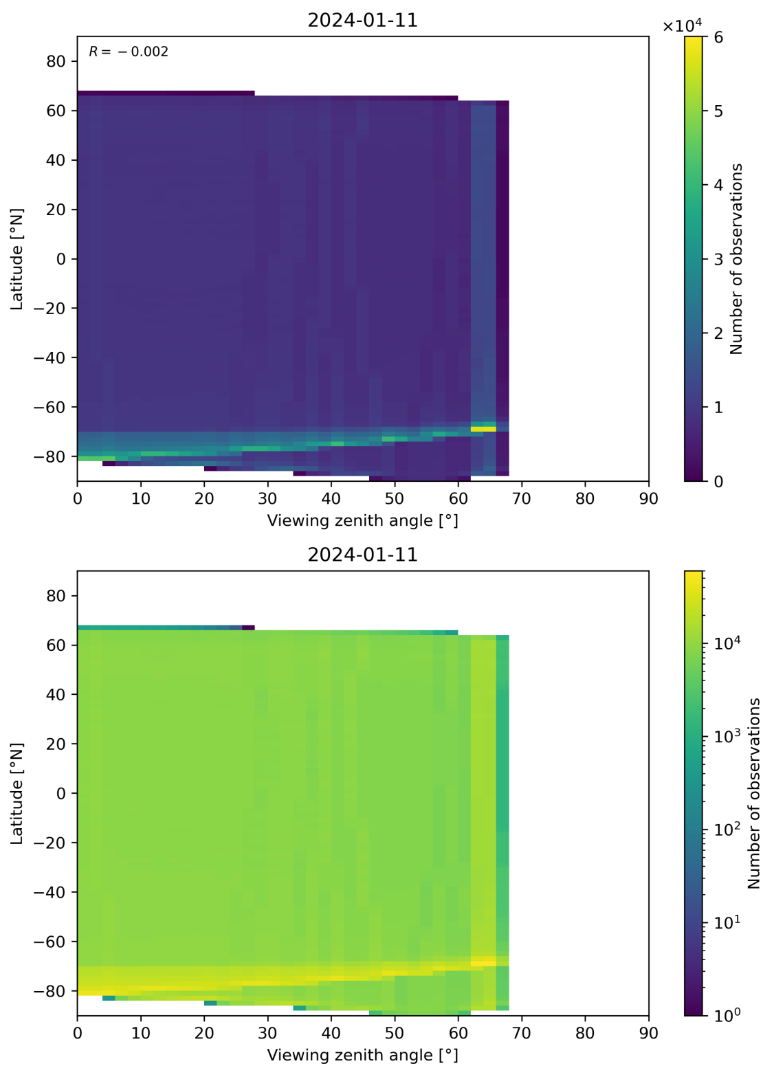
Figure 123: Scatter density plot of “Viewing zenith angle” against “Latitude” for 2024-01-10 to 2024-01-12.
