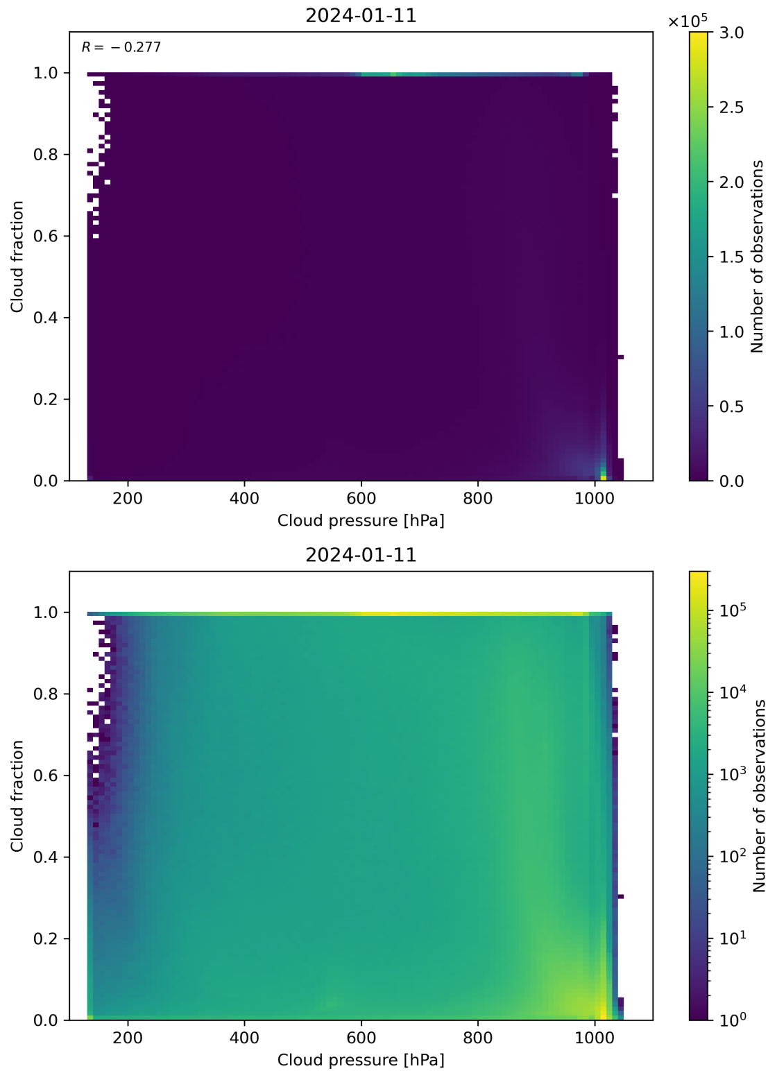
Figure 79: Scatter density plot of “Cloud pressure” against “Cloud fraction” for 2024-01-10 to 2024-01-12.
