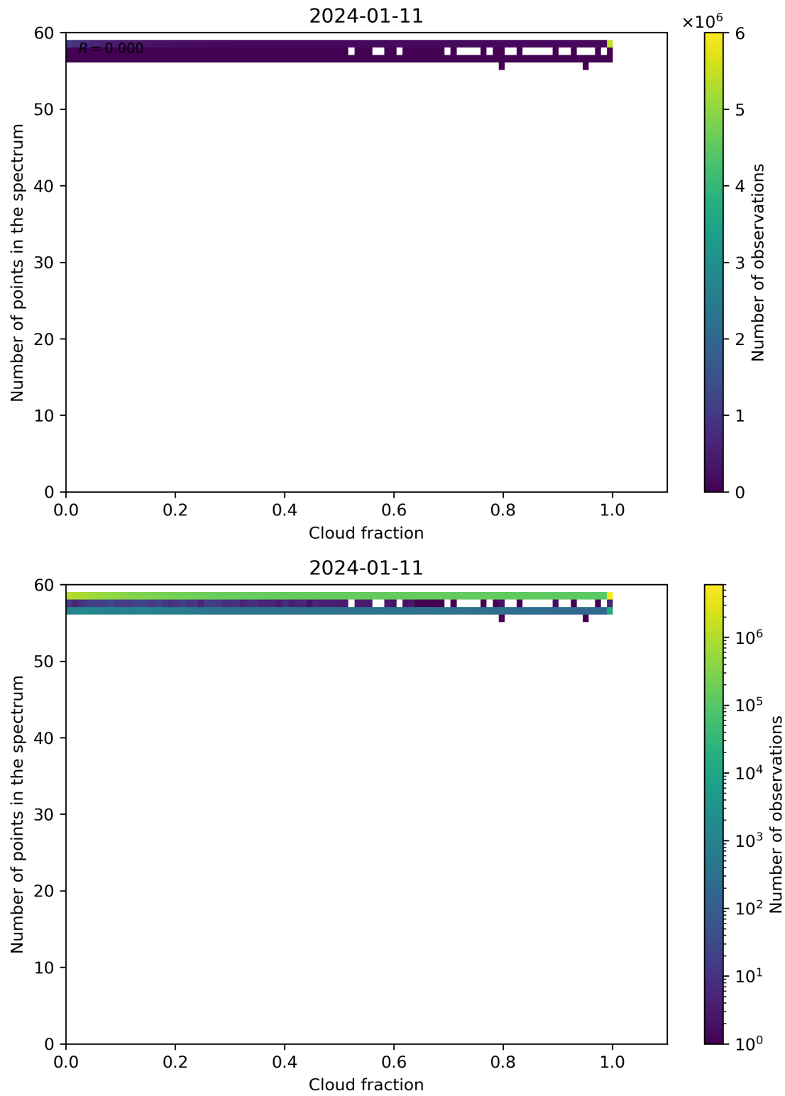
Figure 74: Scatter density plot of “Cloud fraction” against “Number of points in the spectrum” for 2024-01-10 to 2024-01-12.
