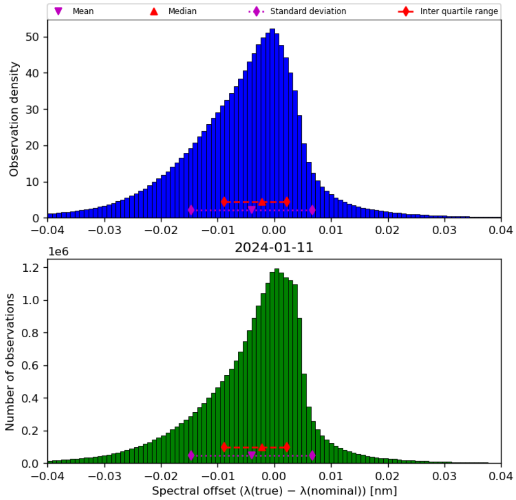
Figure 45: Histogram of “Spectral offset ( \lambda(\text{true}) - \lambda(\text{nominal}) )” for 2024-01-10 to 2024-01-12
