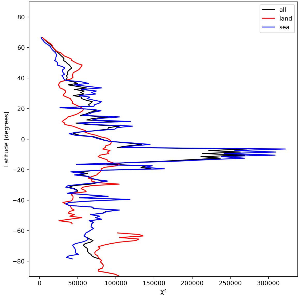
Figure 21: Zonal average of “ \chi^2 ” for 2024-01-10 to 2024-01-12.
