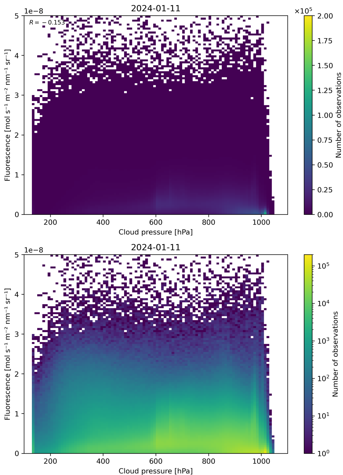
Figure 80: Scatter density plot of “Cloud pressure” against “Fluorescence” for 2024-01-10 to 2024-01-12.
