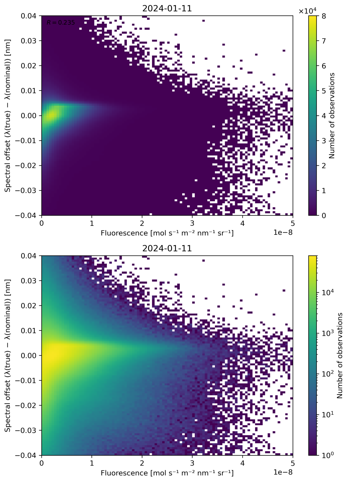
Figure 87: Scatter density plot of “Fluorescence” against “Spectral offset ( \lambda(\text{true}) - \lambda(\text{nominal}) )” for 2024-01-10 to 2024-01-12.
