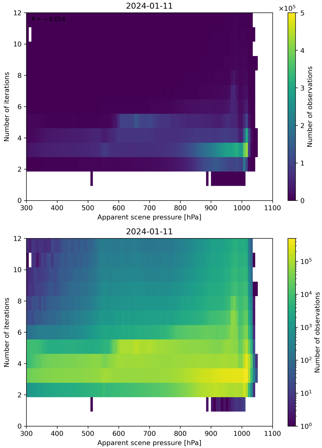
Figure 65: Scatter density plot of “Apparent scene pressure” against “Number of iterations” for 2024-01-10 to 2024-01-12.
