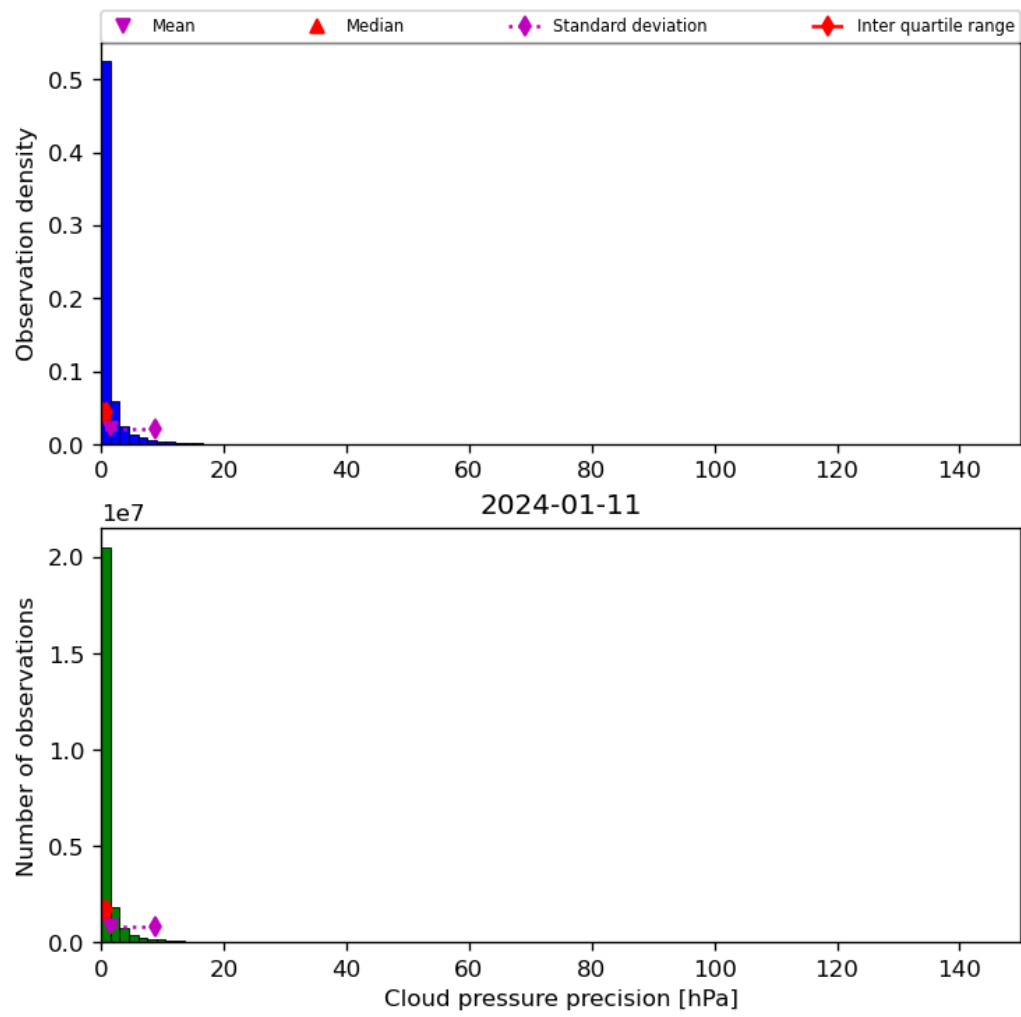
Figure 31: Histogram of “Cloud pressure precision” for 2024-01-10 to 2024-01-12
