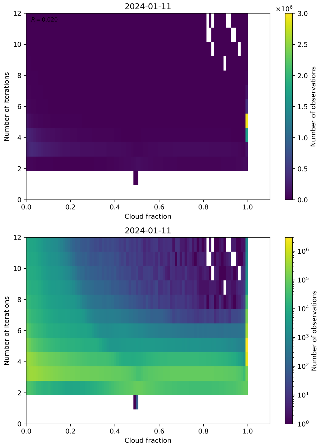
Figure 73: Scatter density plot of “Cloud fraction” against “Number of iterations” for 2024-01-10 to 2024-01-12.
