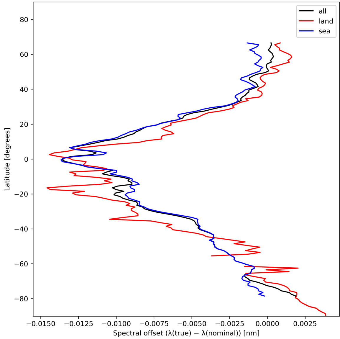
Figure 28: Zonal average of “Spectral offset ( \lambda(\text{true}) - \lambda(\text{nominal}) )” for 2024-01-10 to 2024-01-12.
