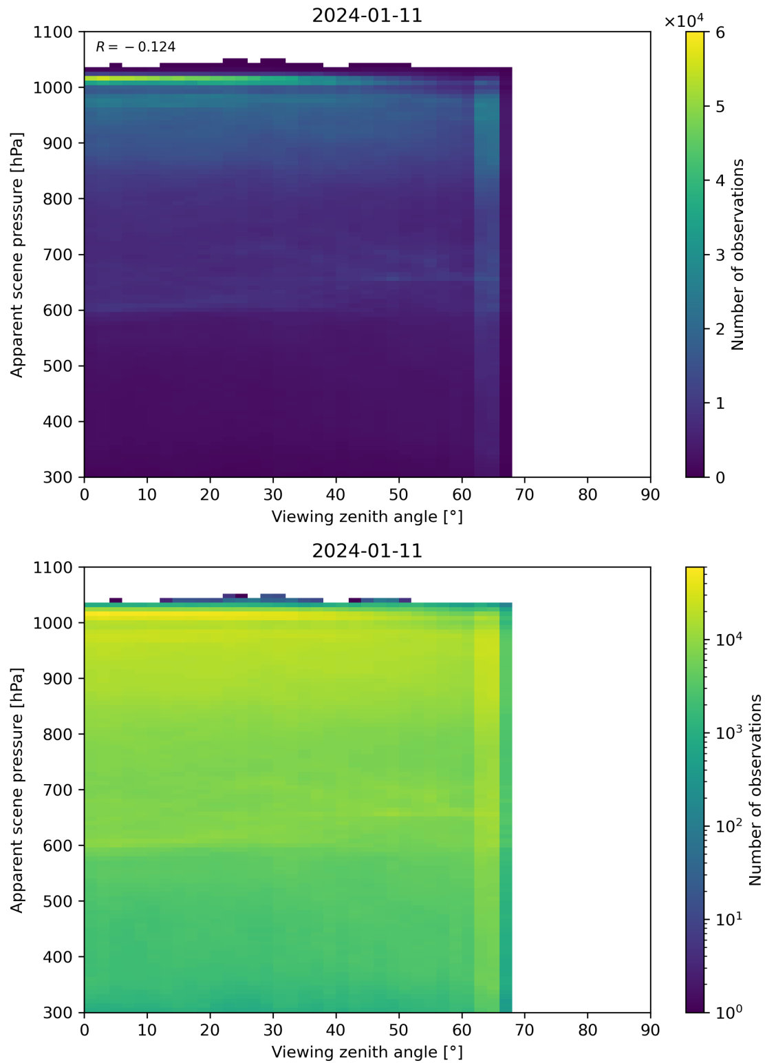
Figure 118: Scatter density plot of “Viewing zenith angle” against “Apparent scene pressure” for 2024-01-10 to 2024-01-12.
