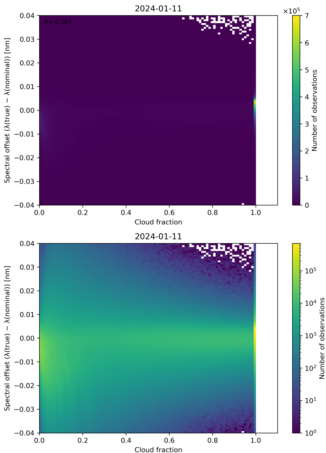
Figure 76: Scatter density plot of “Cloud fraction” against “Spectral offset ( \lambda(\text{true}) - \lambda(\text{nominal}) )” for 2024-01-10 to 2024-01-12.
