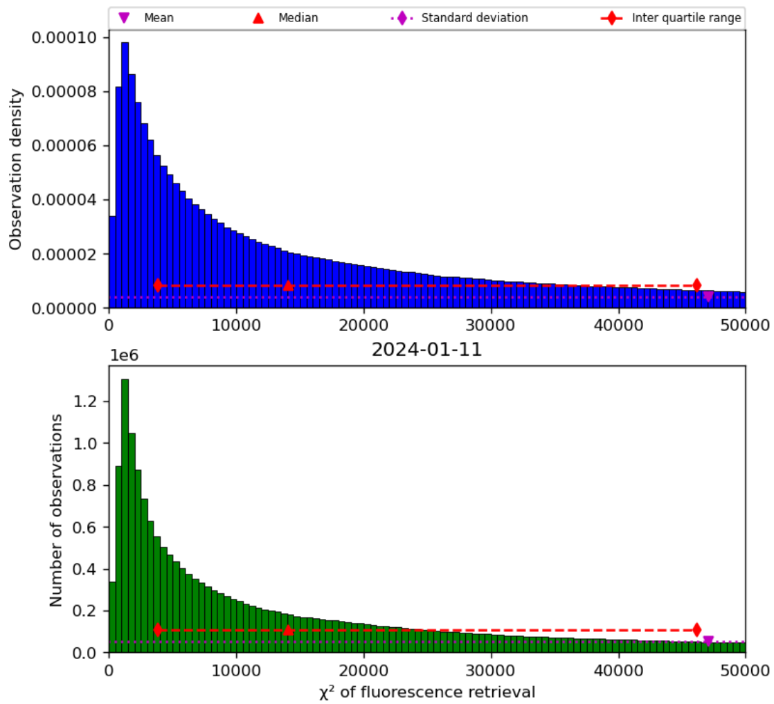
Figure 42: Histogram of “ \chi^2 of fluorescence retrieval” for 2024-01-10 to 2024-01-12
