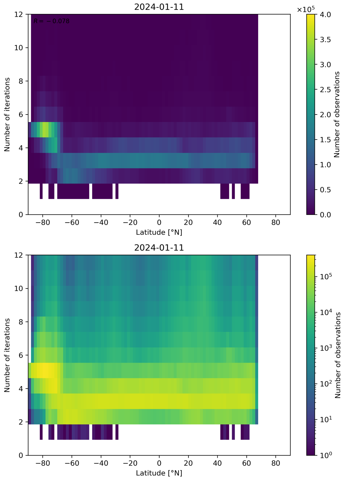
Figure 93: Scatter density plot of “Latitude” against “Number of iterations” for 2024-01-10 to 2024-01-12.
