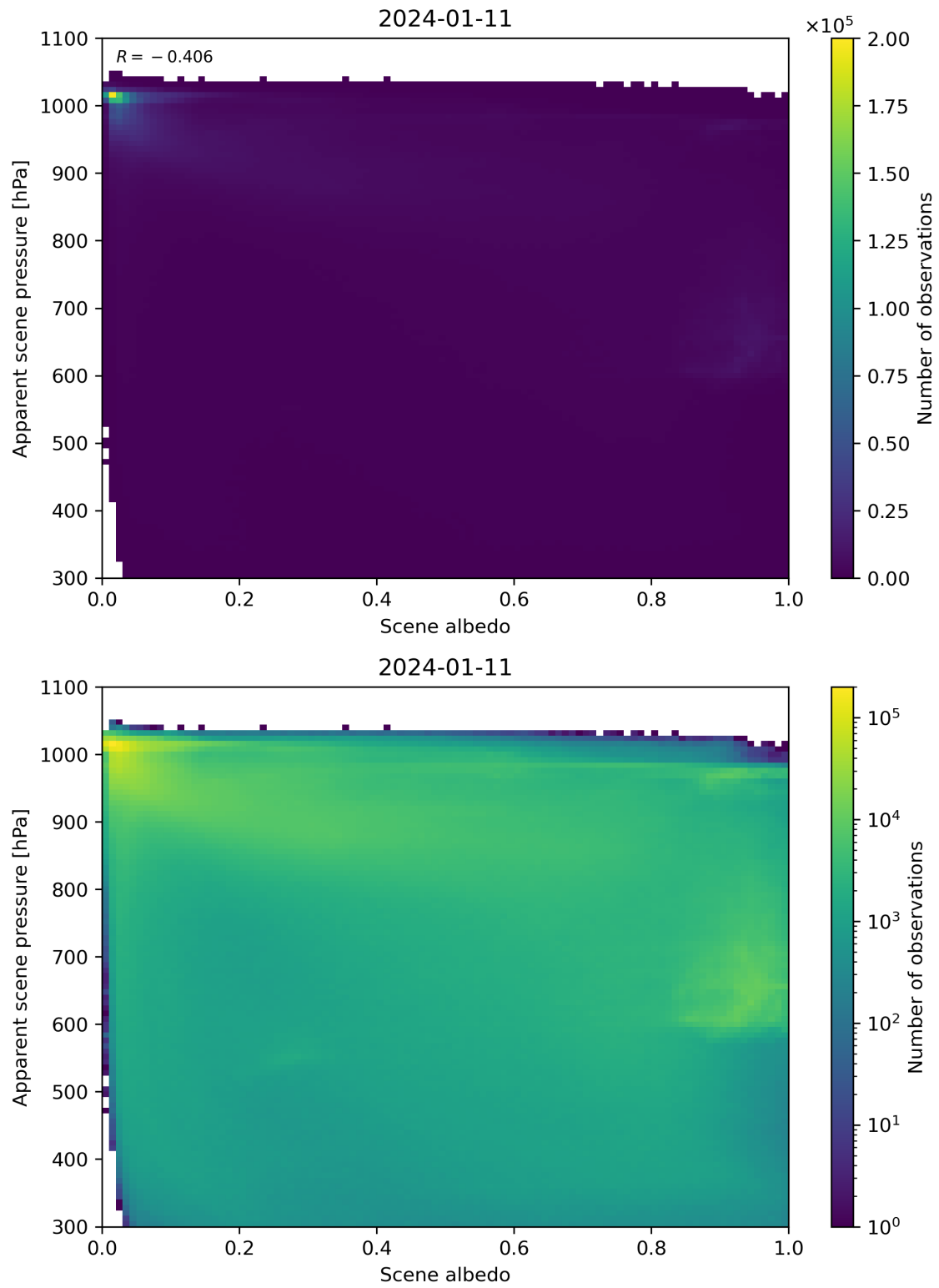
Figure 102: Scatter density plot of “Scene albedo” against “Apparent scene pressure” for 2024-01-10 to 2024-01-12.
