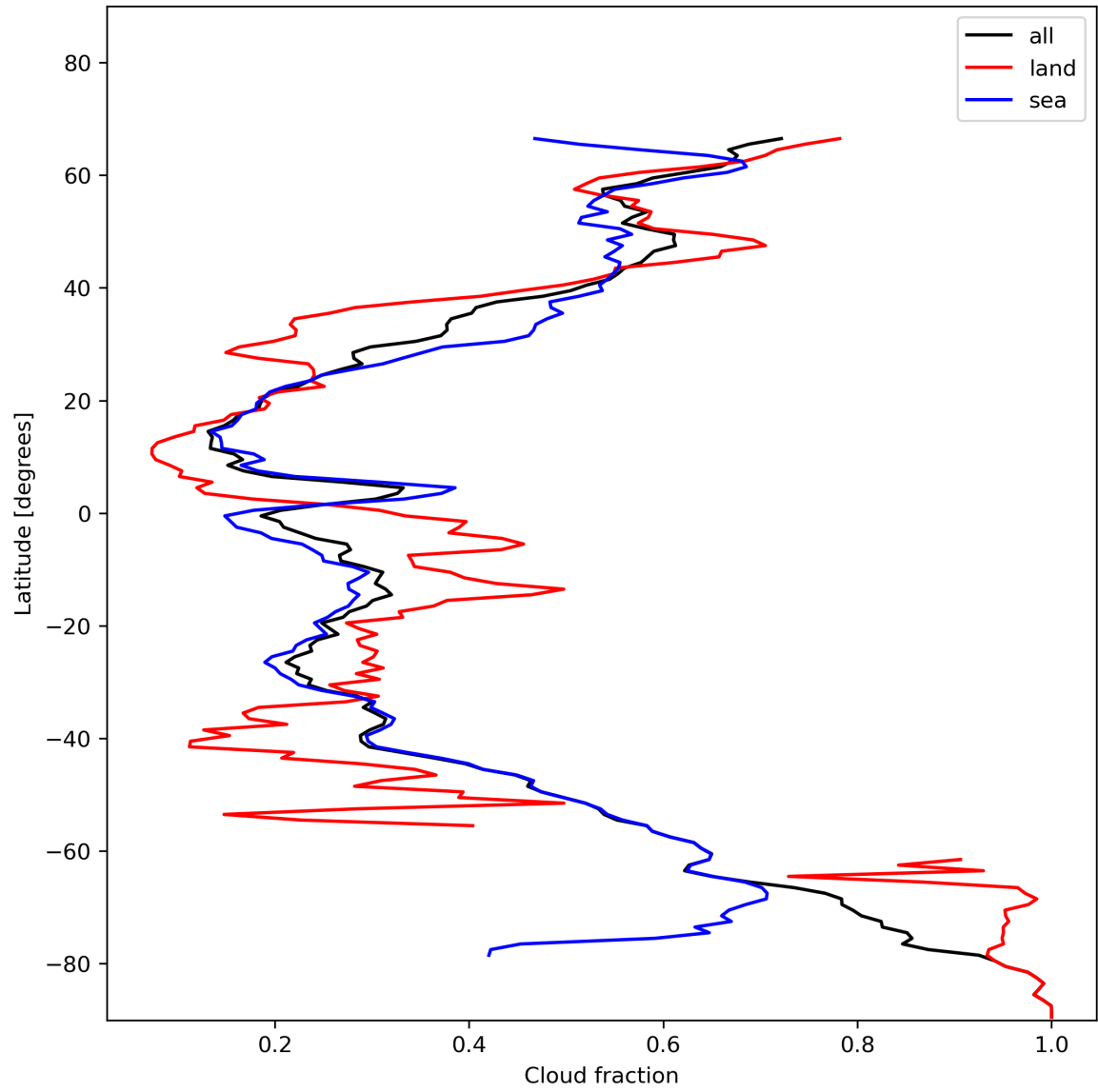
Figure 15: Zonal average of “Cloud fraction” for 2024-01-10 to 2024-01-12.
