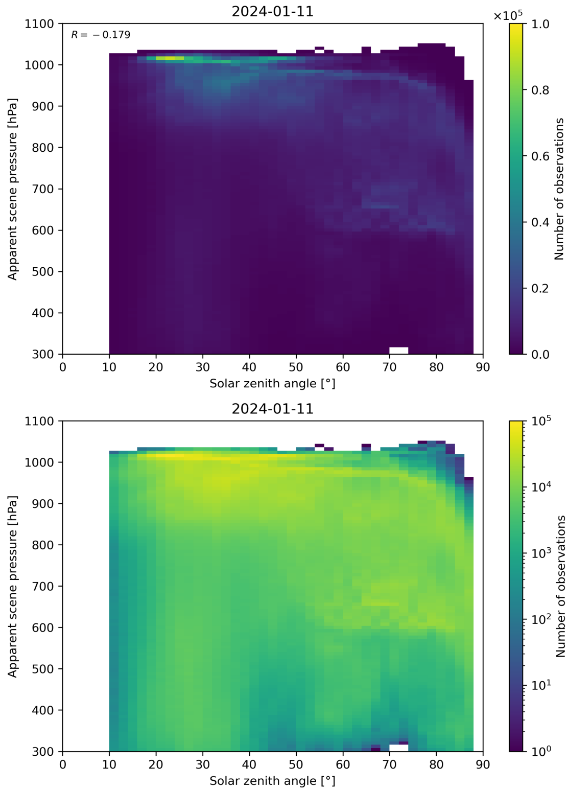
Figure 108: Scatter density plot of “Solar zenith angle” against “Apparent scene pressure” for 2024-01-10 to 2024-01-12.
