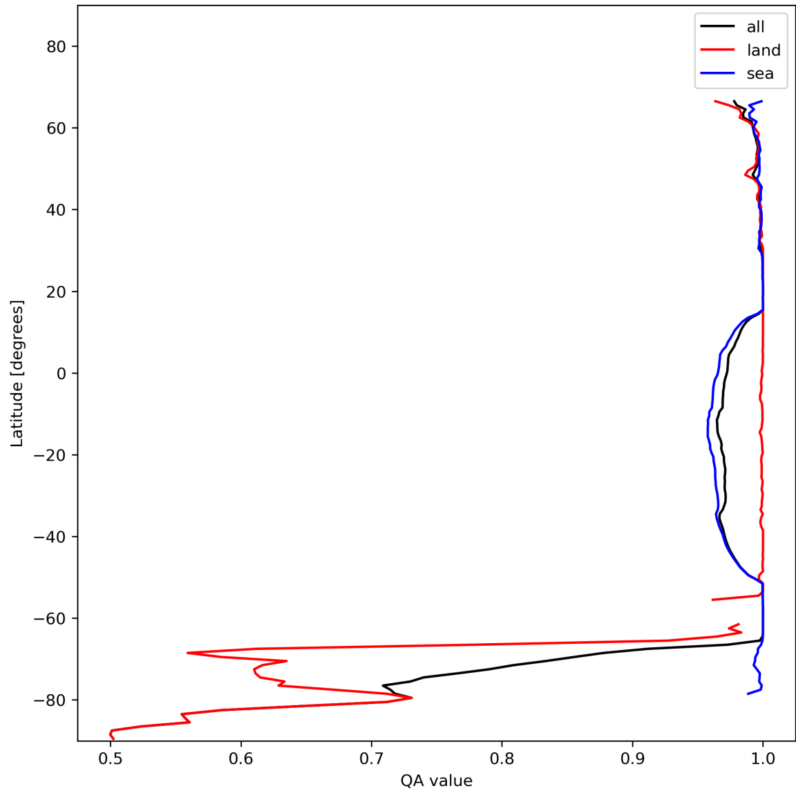
Figure 12: Zonal average of “QA value” for 2024-01-10 to 2024-01-12.
