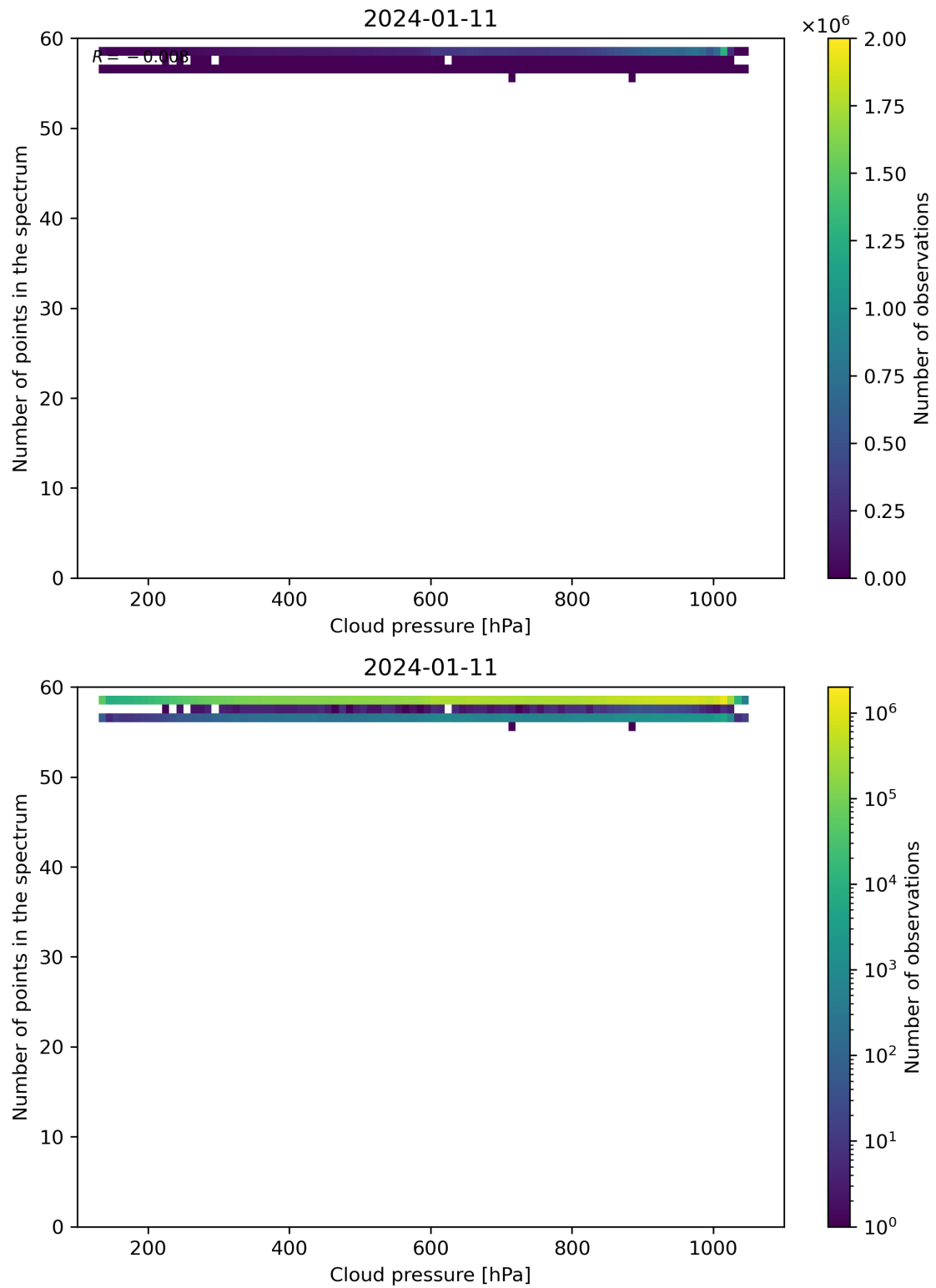
Figure 82: Scatter density plot of “Cloud pressure” against “Number of points in the spectrum” for 2024-01-10 to 2024-01-12.
