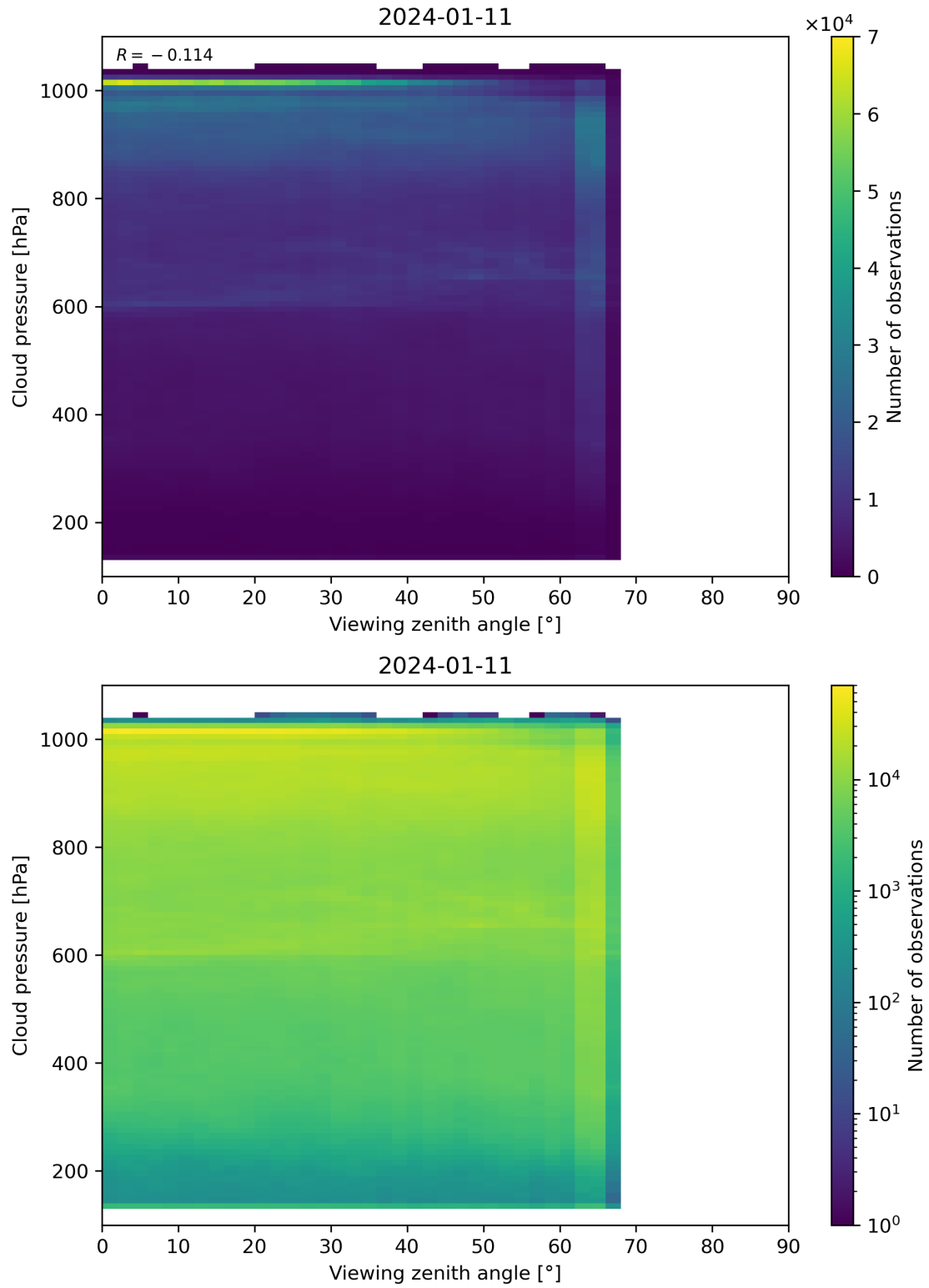
Figure 121: Scatter density plot of “Viewing zenith angle” against “Cloud pressure” for 2024-01-10 to 2024-01-12.
