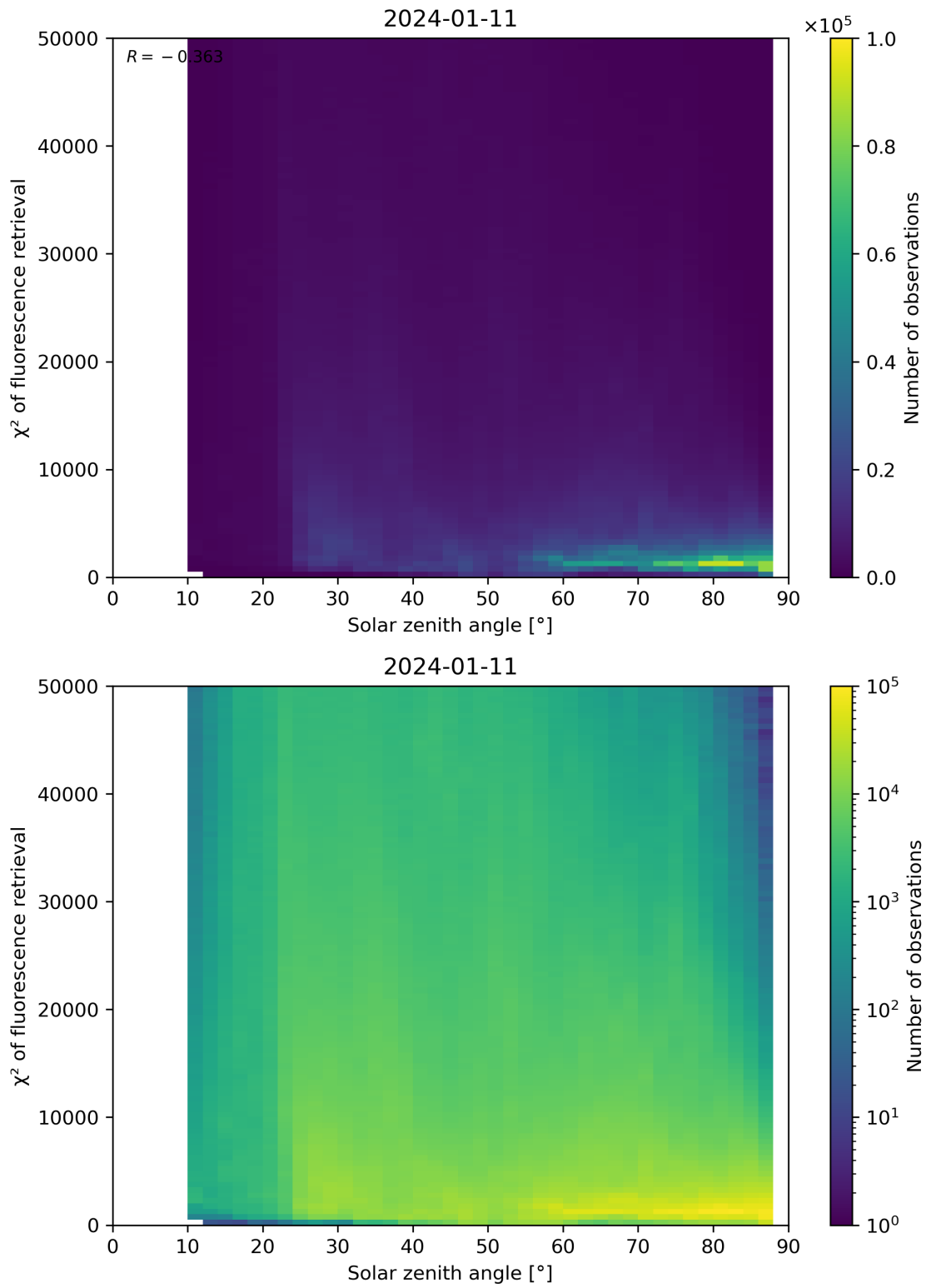
Figure 109: Scatter density plot of “Solar zenith angle” against “ \chi^2 of fluorescence retrieval” for 2024-01-10 to 2024-01-12.
