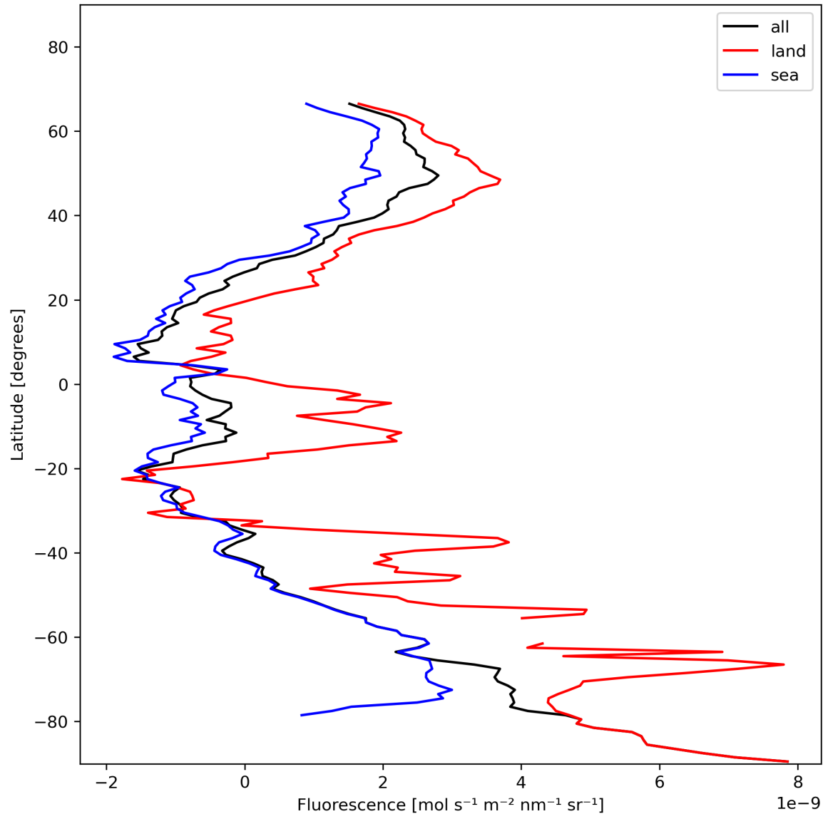
Figure 23: Zonal average of “Fluorescence” for 2024-01-10 to 2024-01-12.
