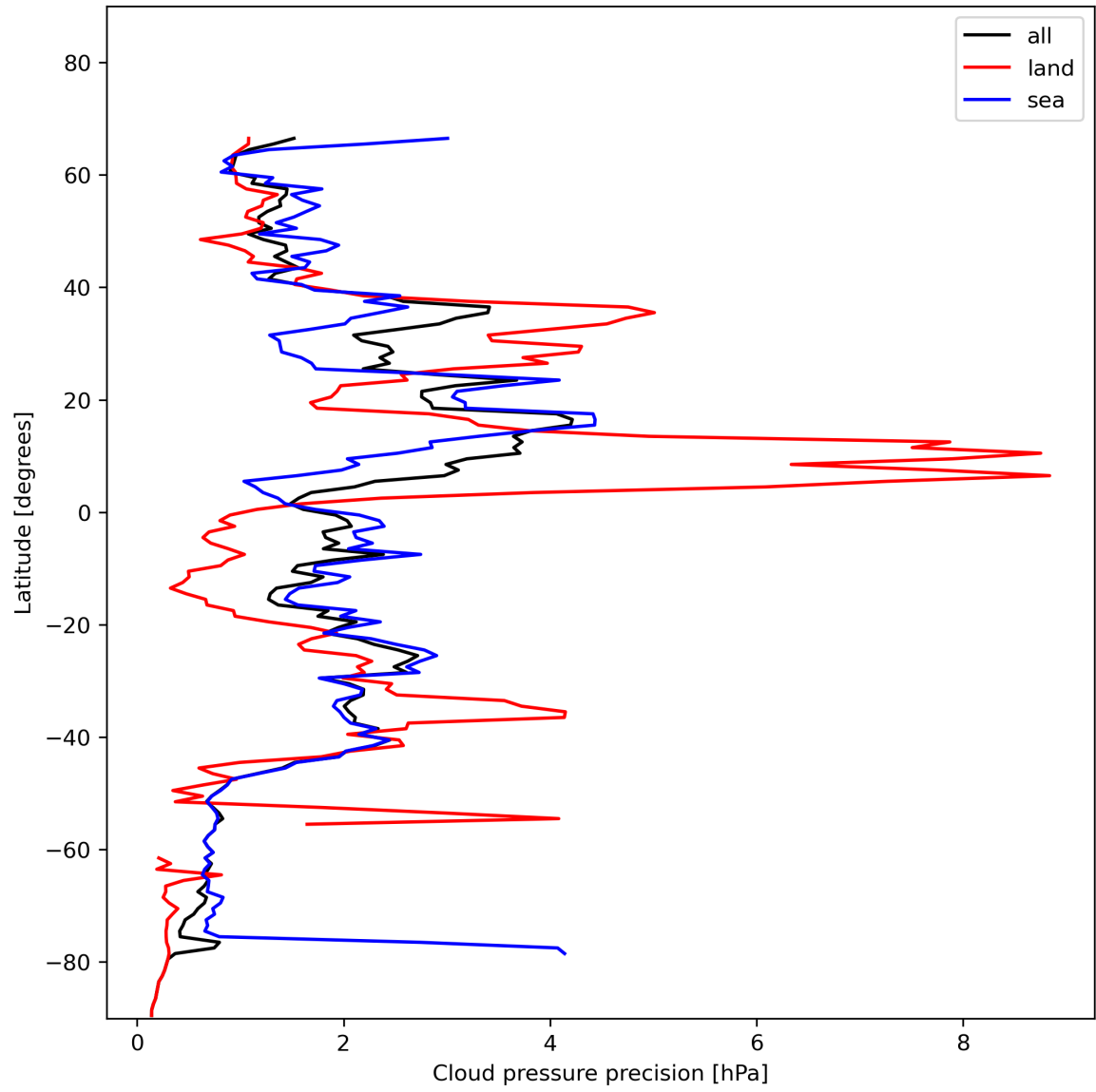
Figure 14: Zonal average of “Cloud pressure precision” for 2024-01-10 to 2024-01-12.
