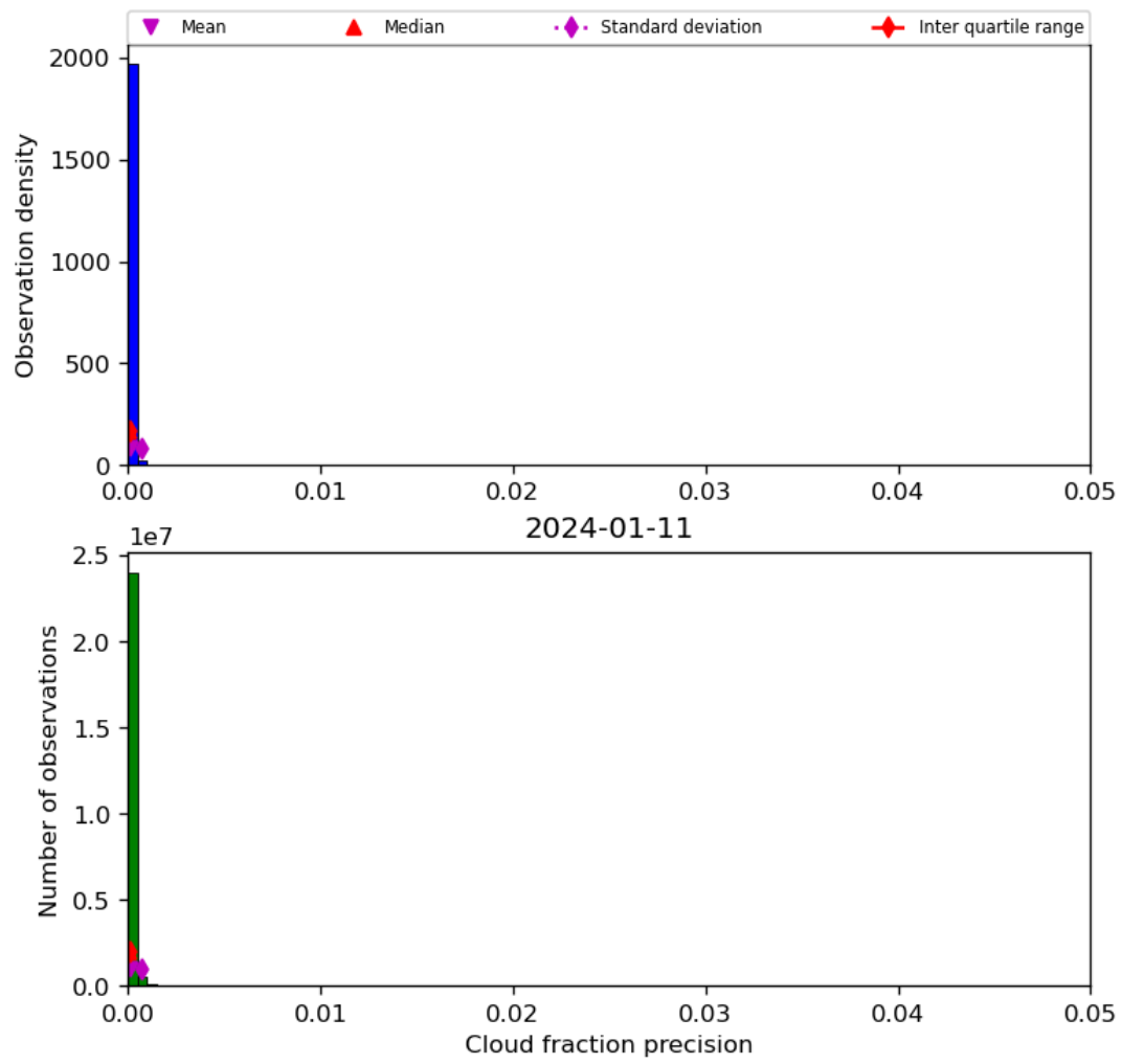
Figure 33: Histogram of “Cloud fraction precision” for 2024-01-10 to 2024-01-12
