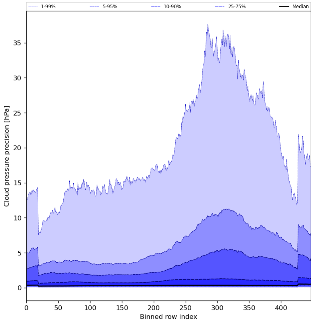
Figure 48: Along track statistics of “Cloud pressure precision” for 2024-01-10 to 2024-01-12
