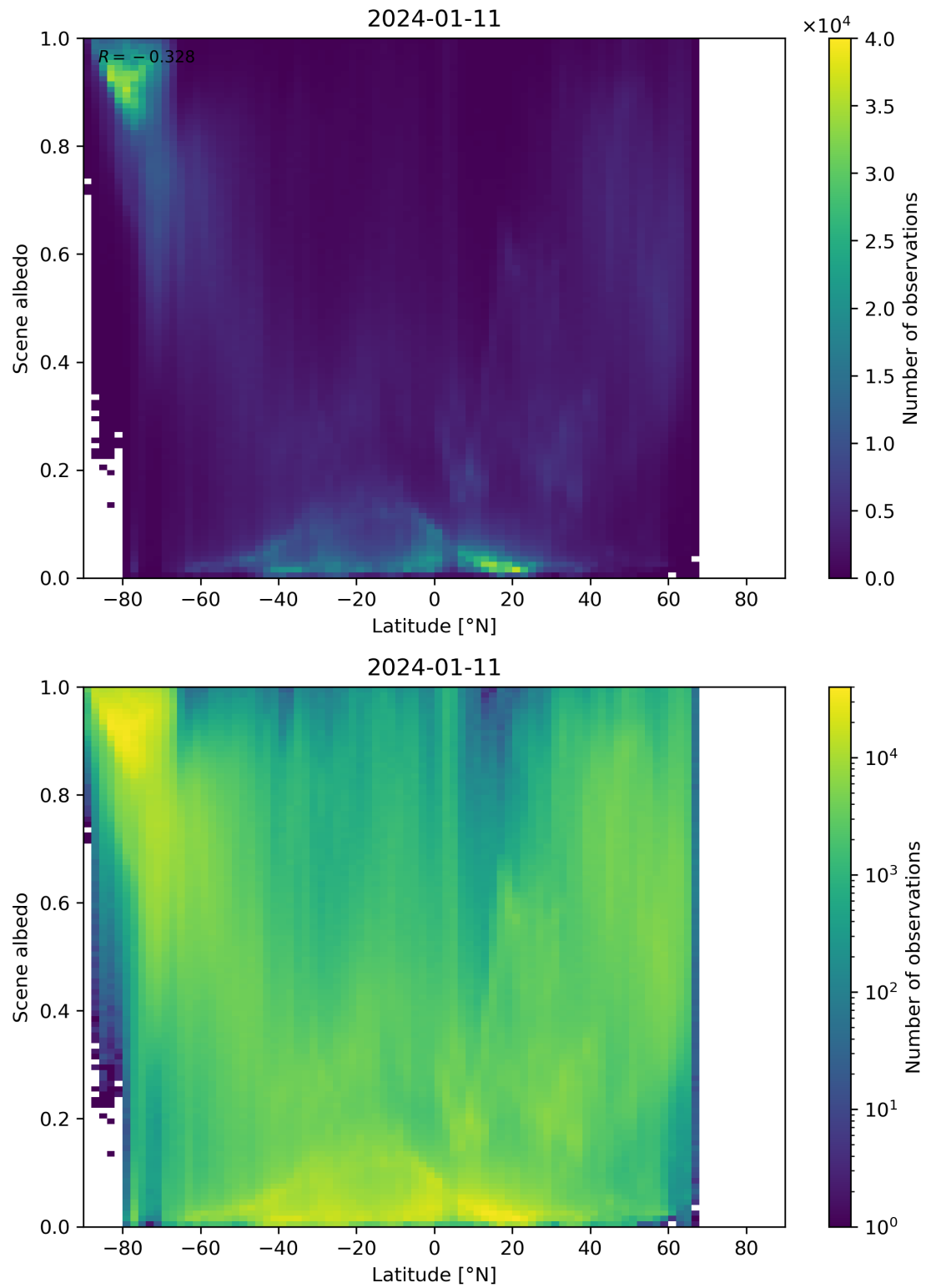
Figure 95: Scatter density plot of “Latitude” against “Scene albedo” for 2024-01-10 to 2024-01-12.
