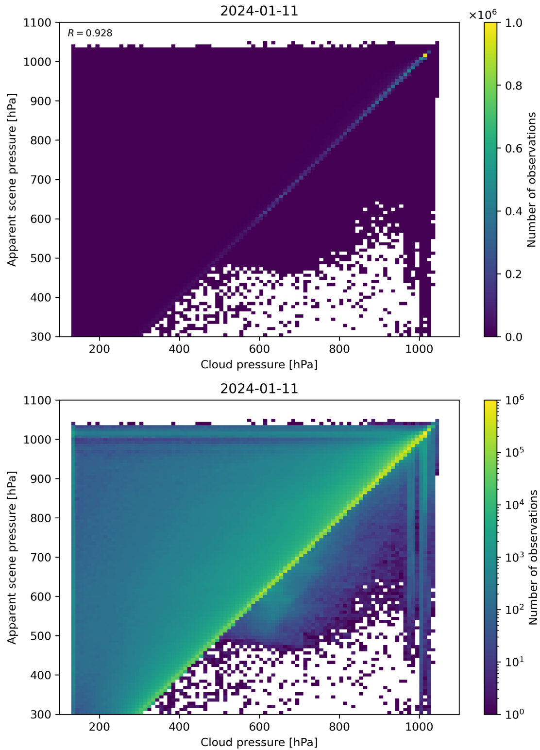
Figure 77: Scatter density plot of “Cloud pressure” against “Apparent scene pressure” for 2024-01-10 to 2024-01-12.
