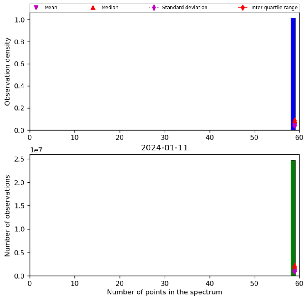
Figure 44: Histogram of “Number of points in the spectrum” for 2024-01-10 to 2024-01-12
