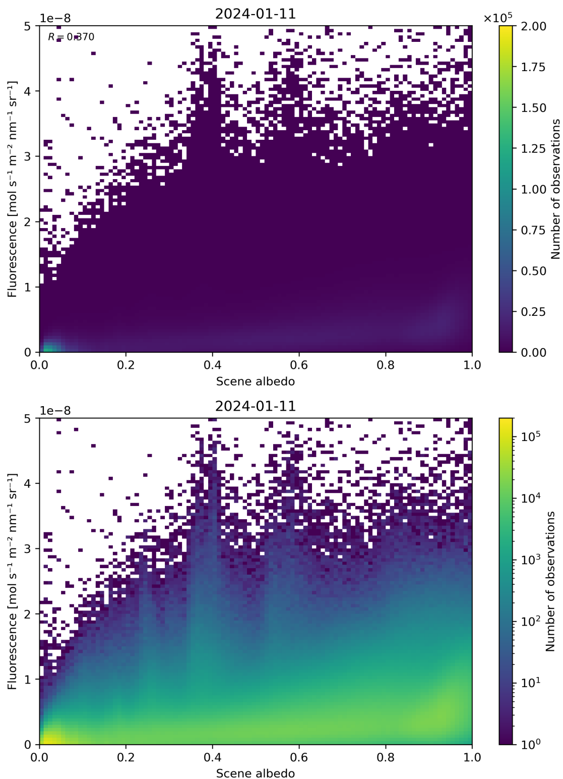
Figure 104: Scatter density plot of “Scene albedo” against “Fluorescence” for 2024-01-10 to 2024-01-12.
