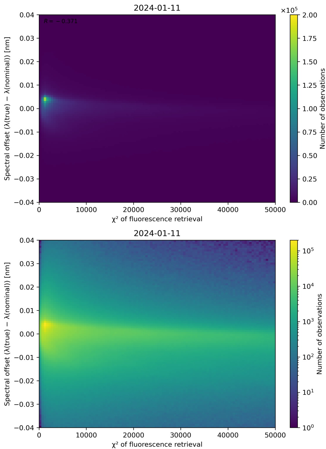
Figure 69: Scatter density plot of " \chi^2 of fluorescence retrieval" against "Spectral offset ( \lambda(\text{true}) - \lambda(\text{nominal}) )" for 2024-01-10 to 2024-01-12.
