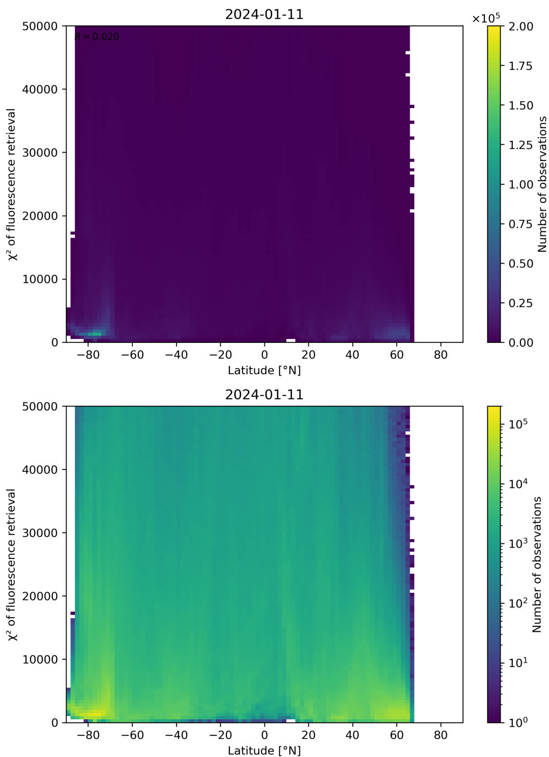
Figure 89: Scatter density plot of “Latitude” against “ \chi^2 of fluorescence retrieval” for 2024-01-10 to 2024-01-12.
