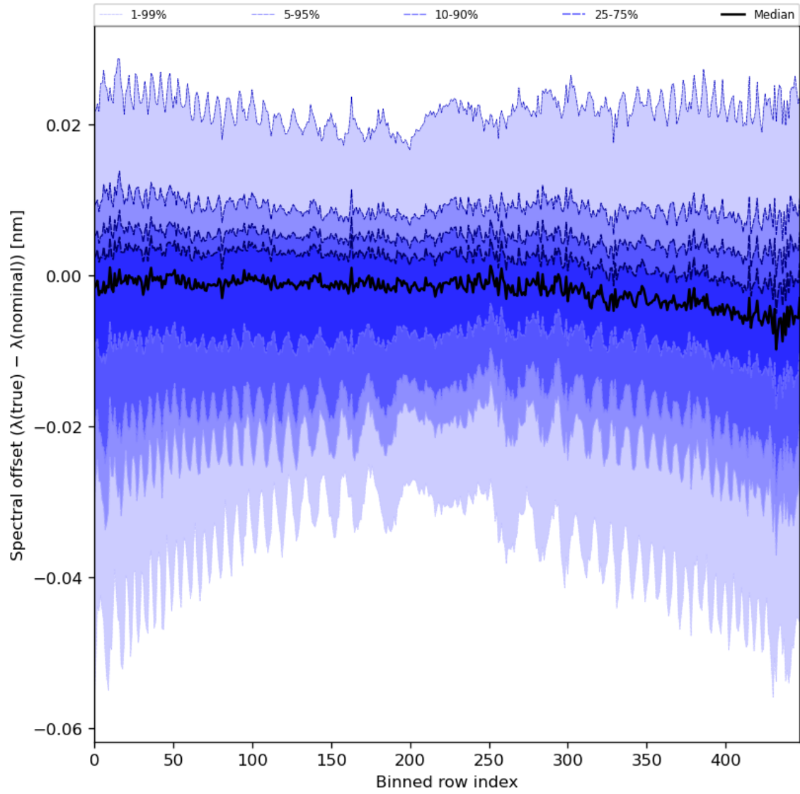
Figure 62: Along track statistics of “Spectral offset ( \lambda(\text{true}) - \lambda(\text{nominal}) )” for 2024-01-10 to 2024-01-12
