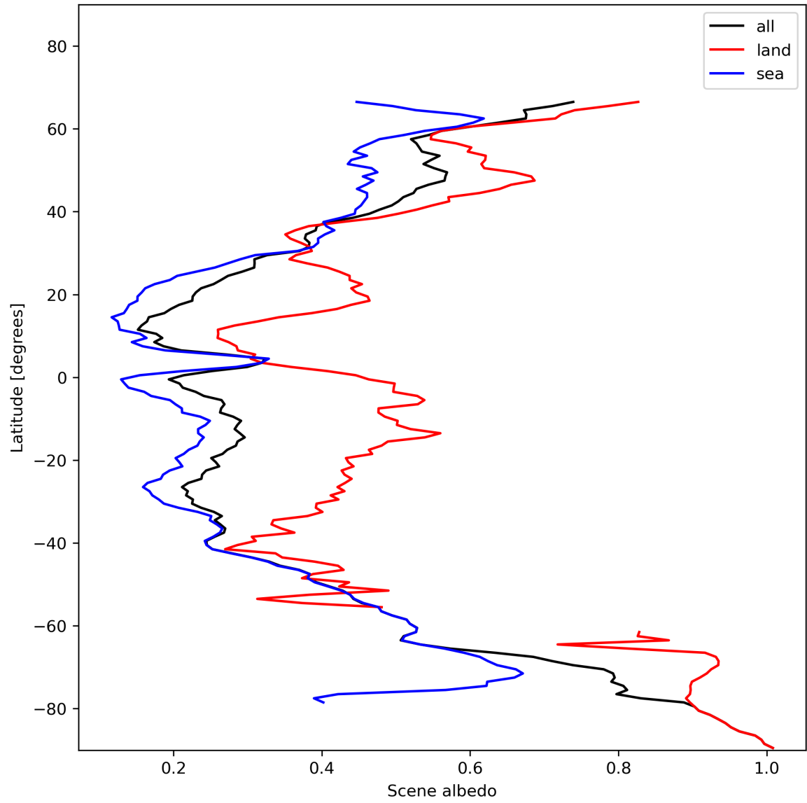
Figure 17: Zonal average of “Scene albedo” for 2024-01-10 to 2024-01-12.
