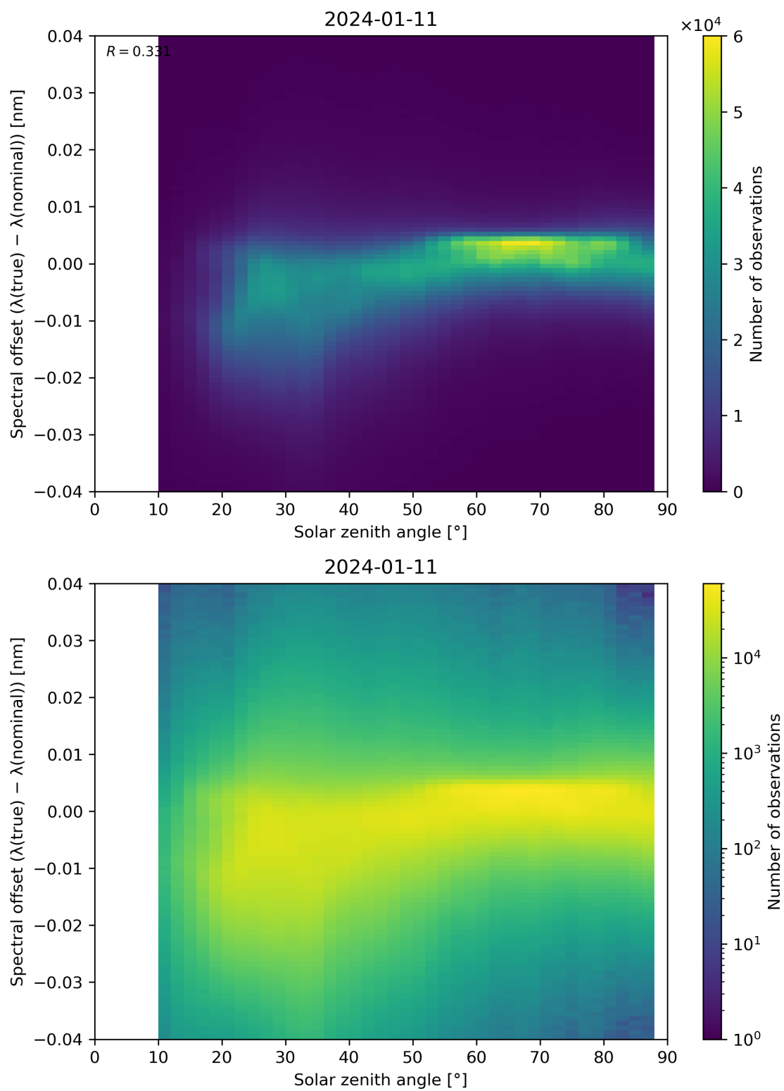
Figure 117: Scatter density plot of “Solar zenith angle” against “Spectral offset ( \lambda(\text{true}) - \lambda(\text{nominal}) )” for 2024-01-10 to 2024-01-12.
