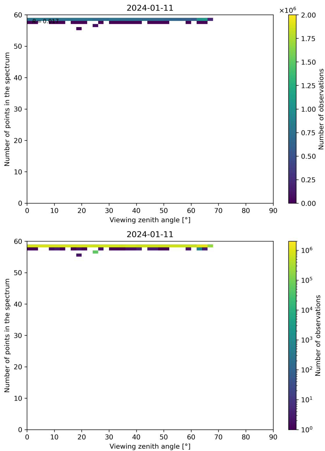
Figure 125: Scatter density plot of “Viewing zenith angle” against “Number of points in the spectrum” for 2024-01-10 to 2024-01-12.
