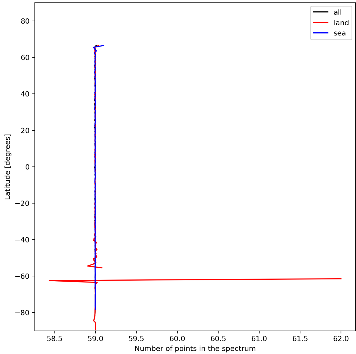
Figure 27: Zonal average of “Number of points in the spectrum” for 2024-01-10 to 2024-01-12.
