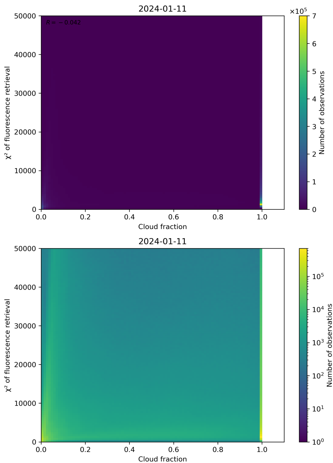
Figure 71: Scatter density plot of “Cloud fraction” against “ \chi^2 of fluorescence retrieval” for 2024-01-10 to 2024-01-12.
