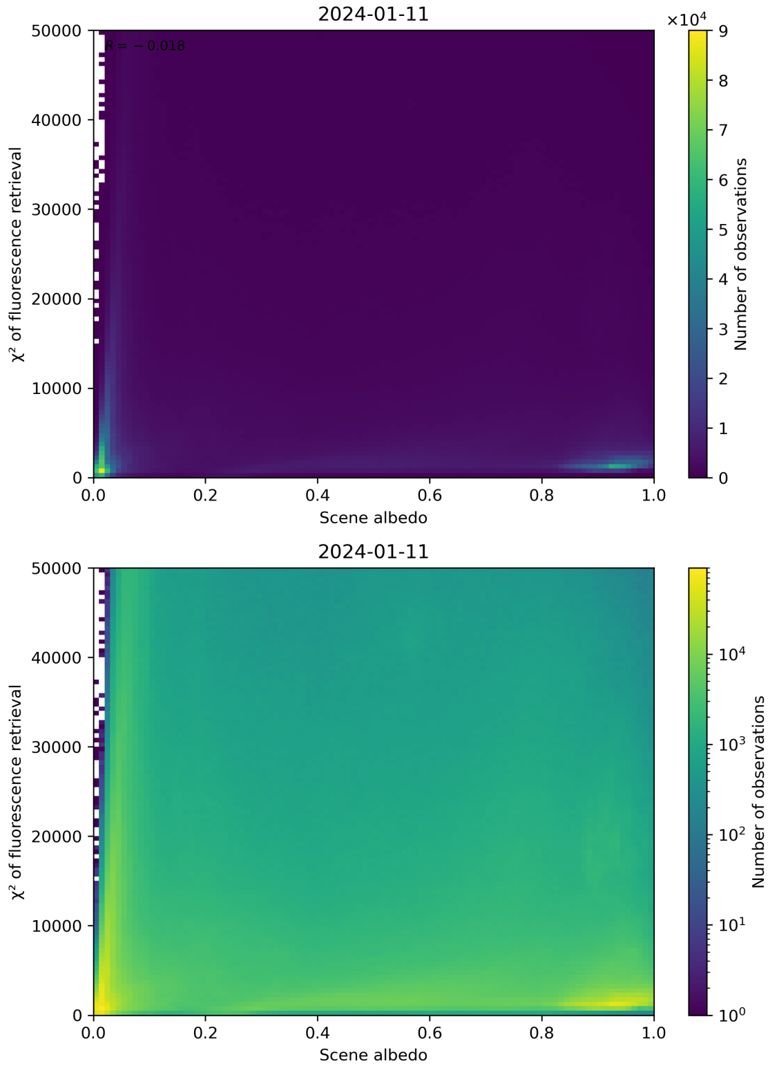
Figure 103: Scatter density plot of “Scene albedo” against “ \chi^2 of fluorescence retrieval” for 2024-01-10 to 2024-01-12.
