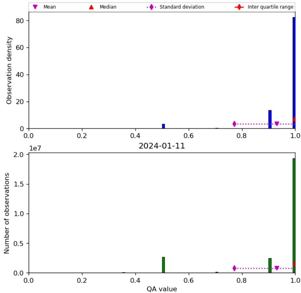
Figure 29: Histogram of “QA value” for 2024-01-10 to 2024-01-12
