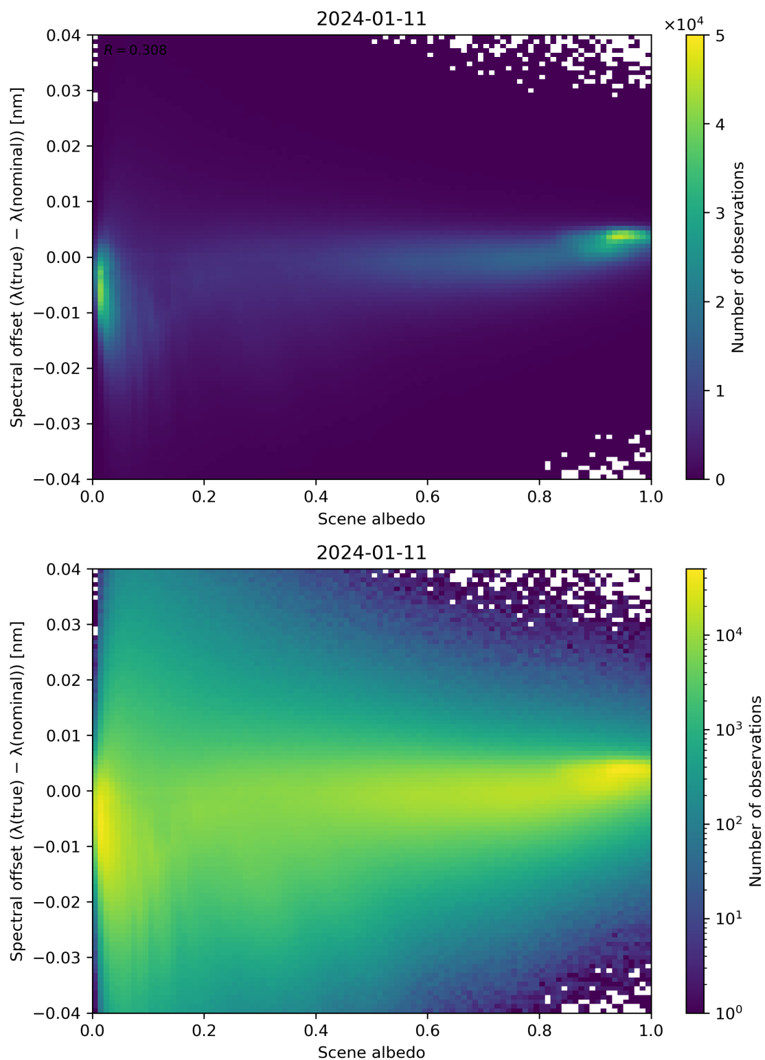
Figure 107: Scatter density plot of “Scene albedo” against “Spectral offset ( \lambda(\text{true}) - \lambda(\text{nominal}) )” for 2024-01-10 to 2024-01-12.
