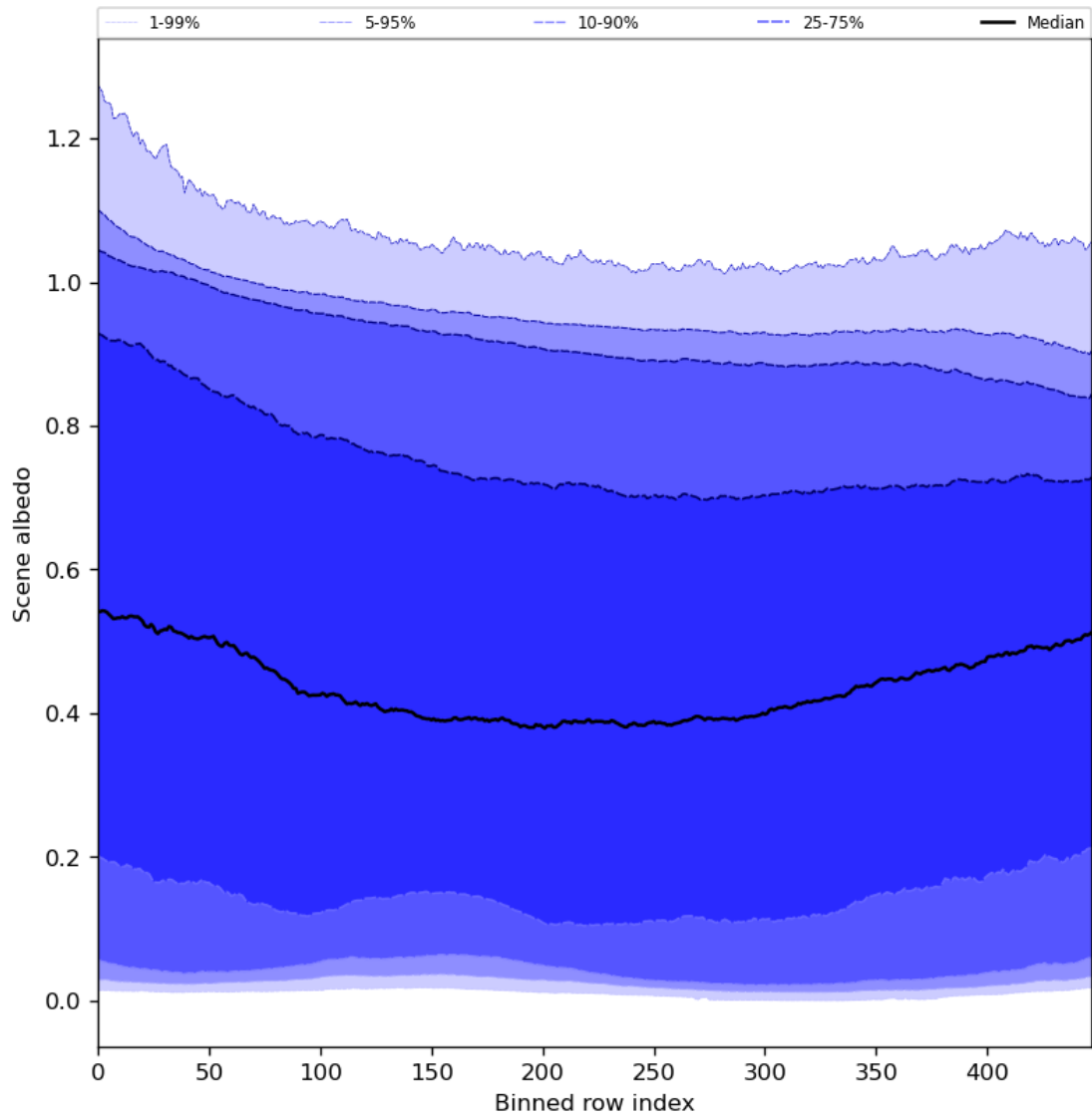
Figure 51: Along track statistics of “Scene albedo” for 2024-01-10 to 2024-01-12
