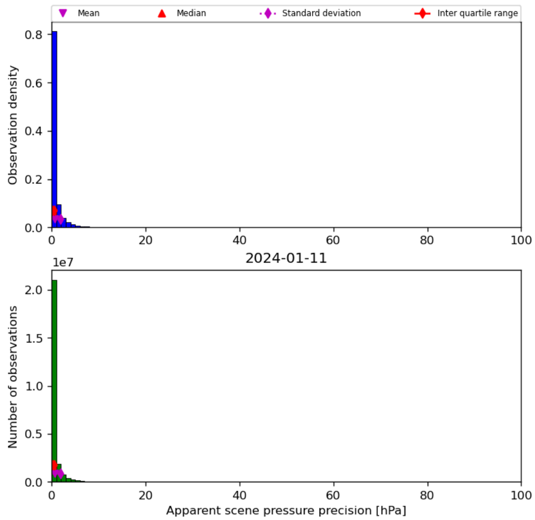
Figure 37: Histogram of “Apparent scene pressure precision” for 2024-01-10 to 2024-01-12
