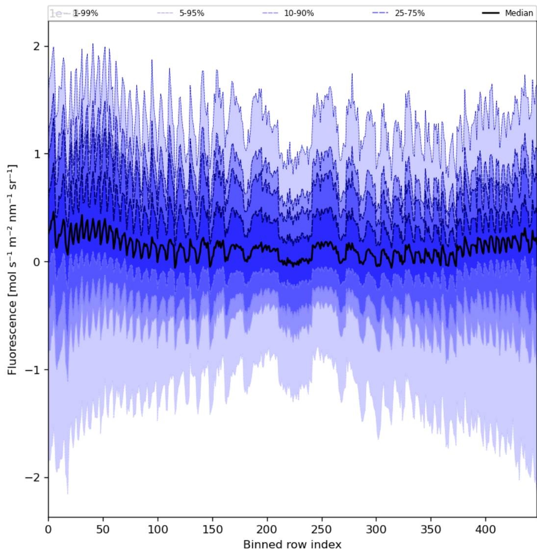
Figure 57: Along track statistics of “Fluorescence” for 2024-01-10 to 2024-01-12
