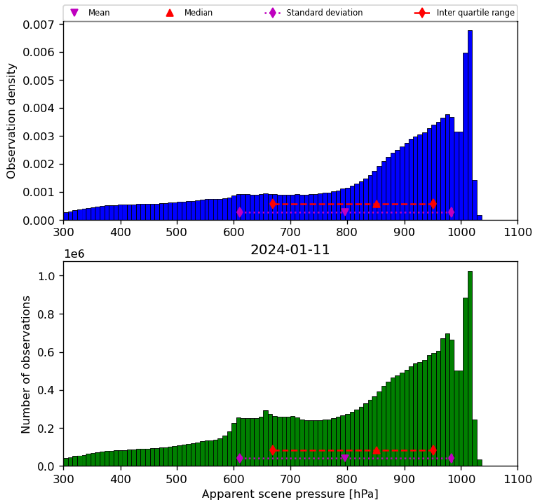
Figure 36: Histogram of “Apparent scene pressure” for 2024-01-10 to 2024-01-12
