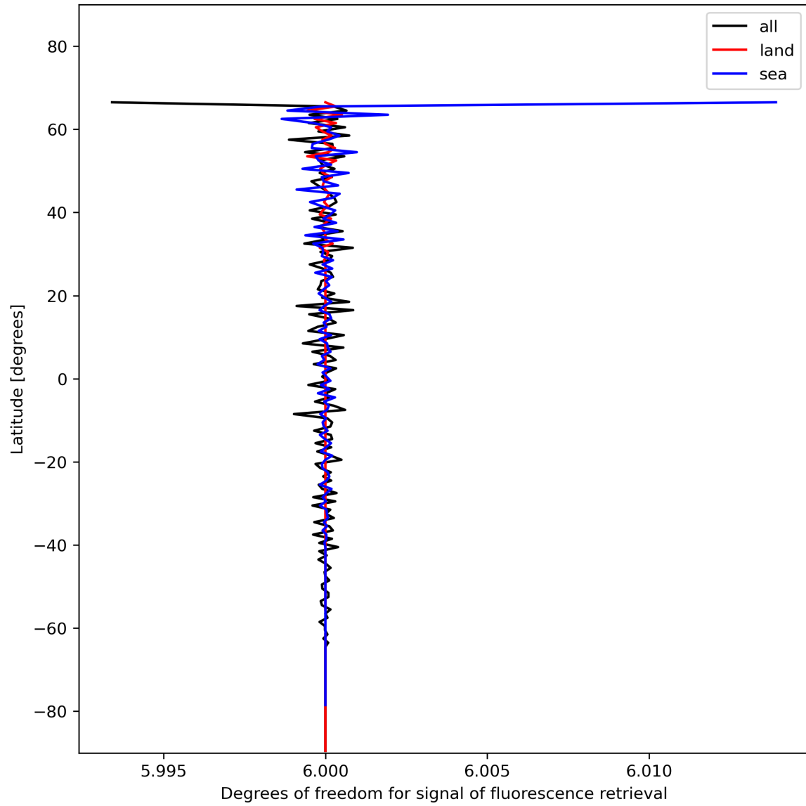
Figure 26: Zonal average of “Degrees of freedom for signal of fluorescence retrieval” for 2024-01-10 to 2024-01-12.
