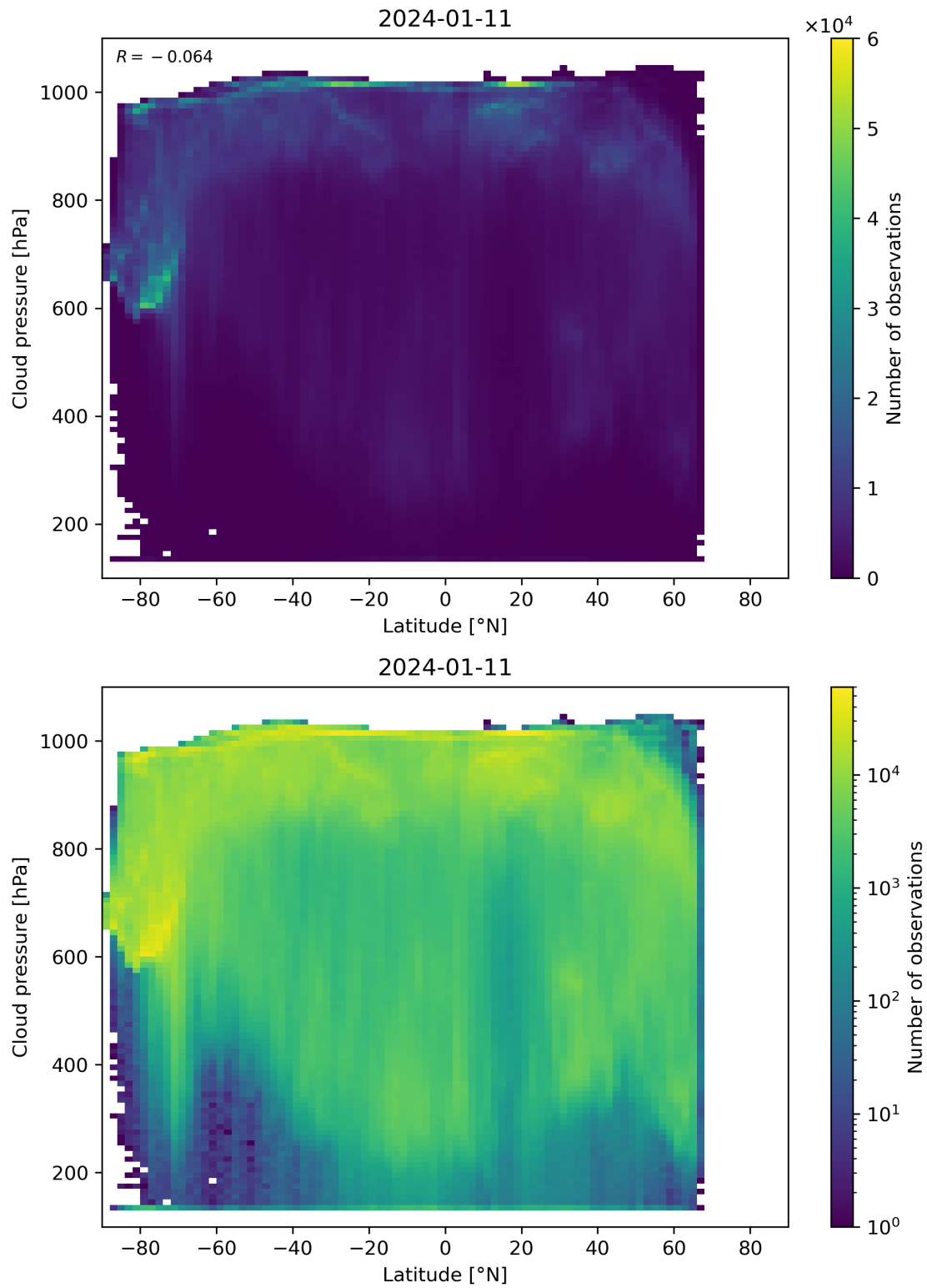
Figure 91: Scatter density plot of “Latitude” against “Cloud pressure” for 2024-01-10 to 2024-01-12.
