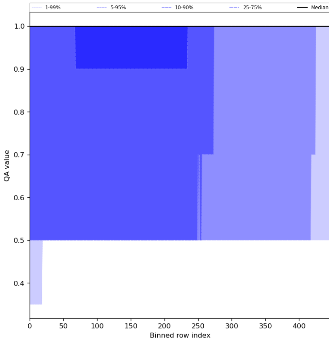
Figure 46: Along track statistics of “QA value” for 2024-01-10 to 2024-01-12
