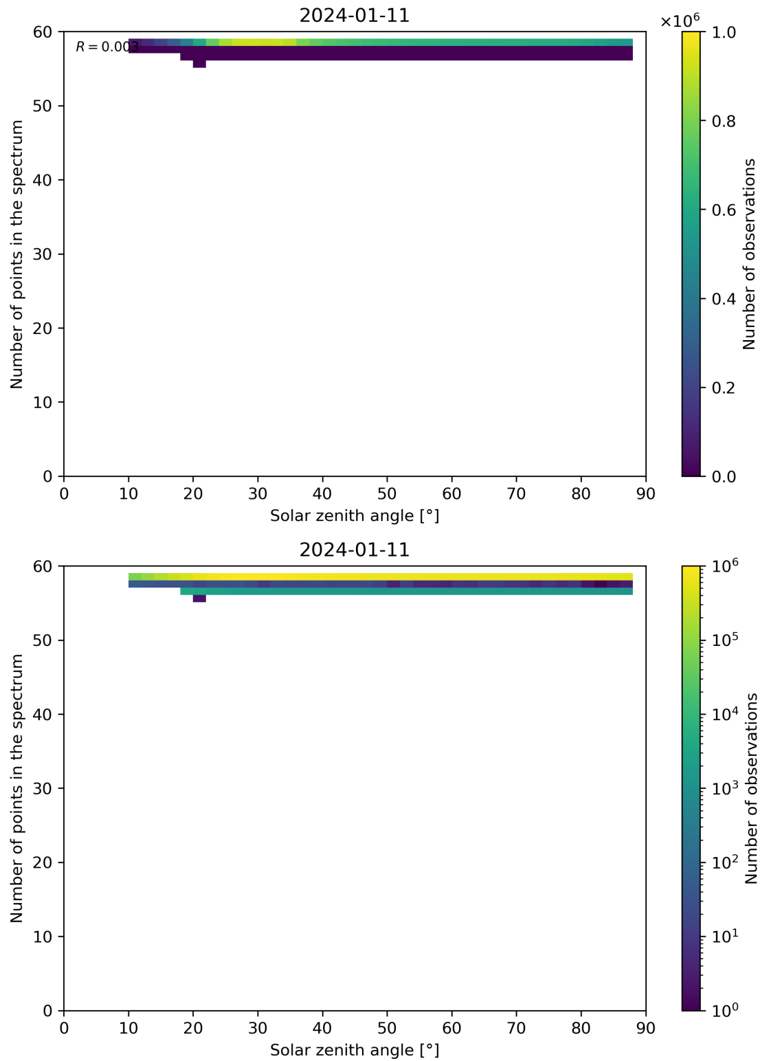
Figure 115: Scatter density plot of “Solar zenith angle” against “Number of points in the spectrum” for 2024-01-10 to 2024-01-12.
