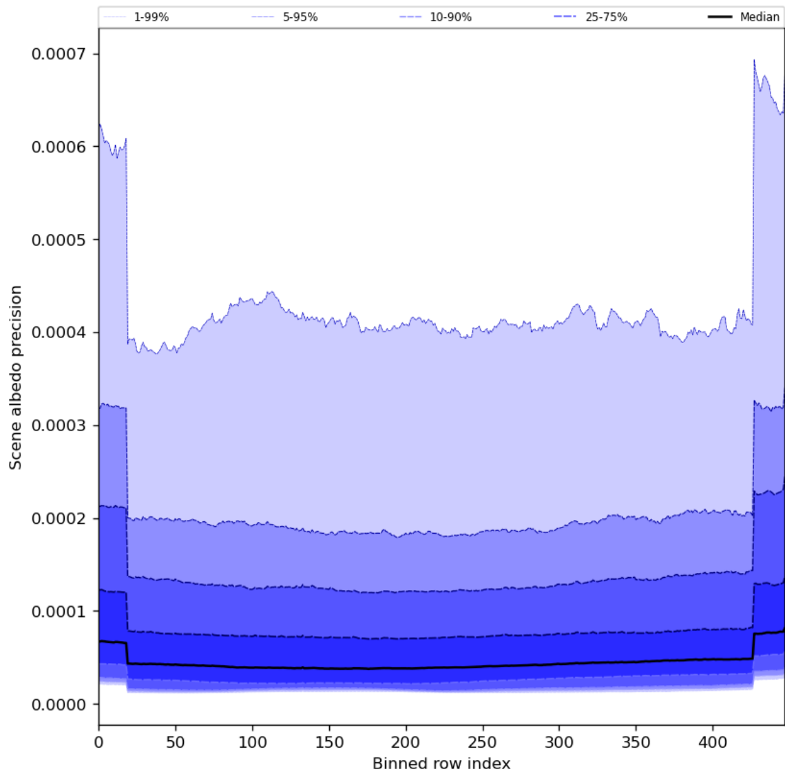
Figure 52: Along track statistics of “Scene albedo precision” for 2024-01-10 to 2024-01-12
