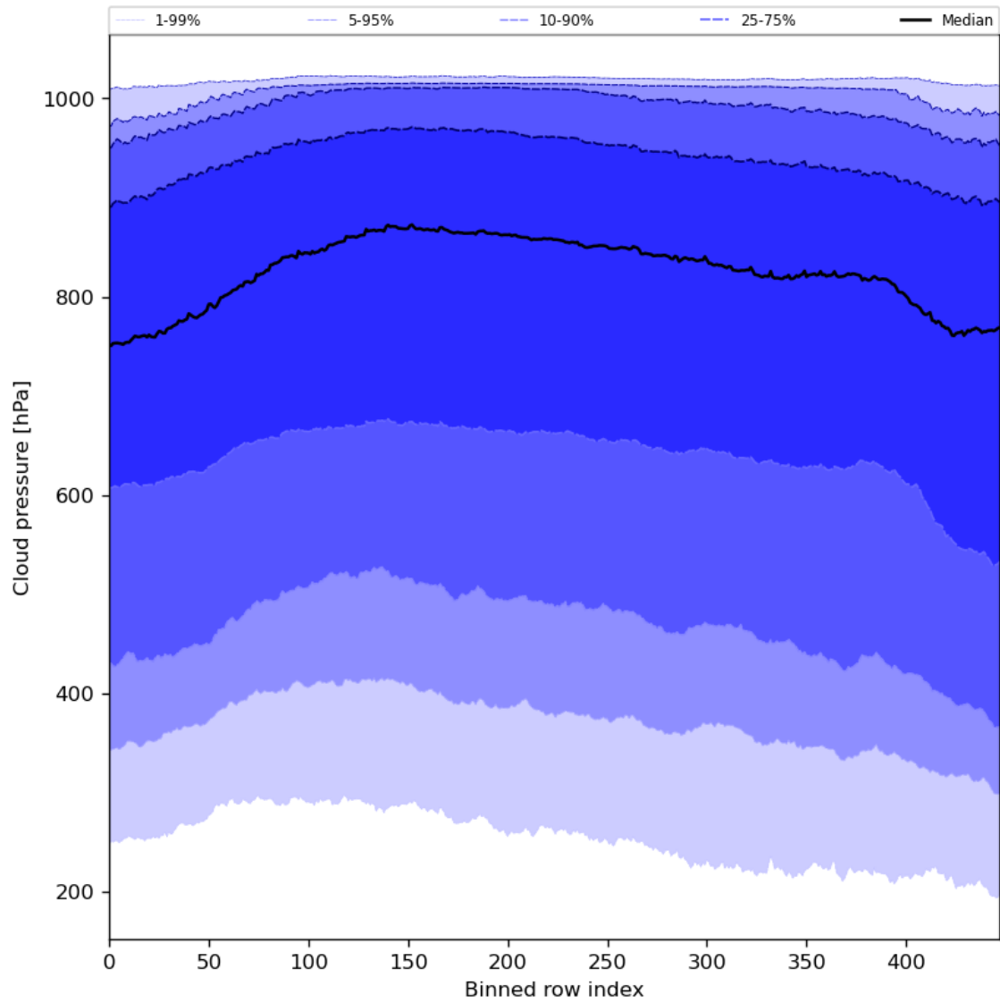
Figure 47: Along track statistics of “Cloud pressure” for 2024-01-10 to 2024-01-12
