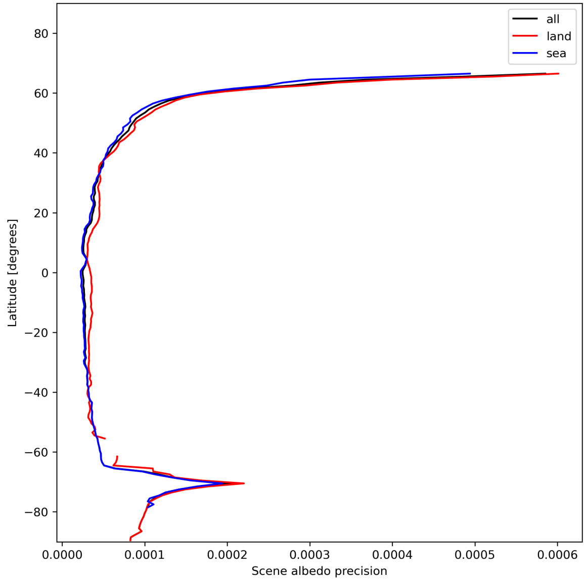
Figure 18: Zonal average of “Scene albedo precision” for 2024-01-10 to 2024-01-12.
