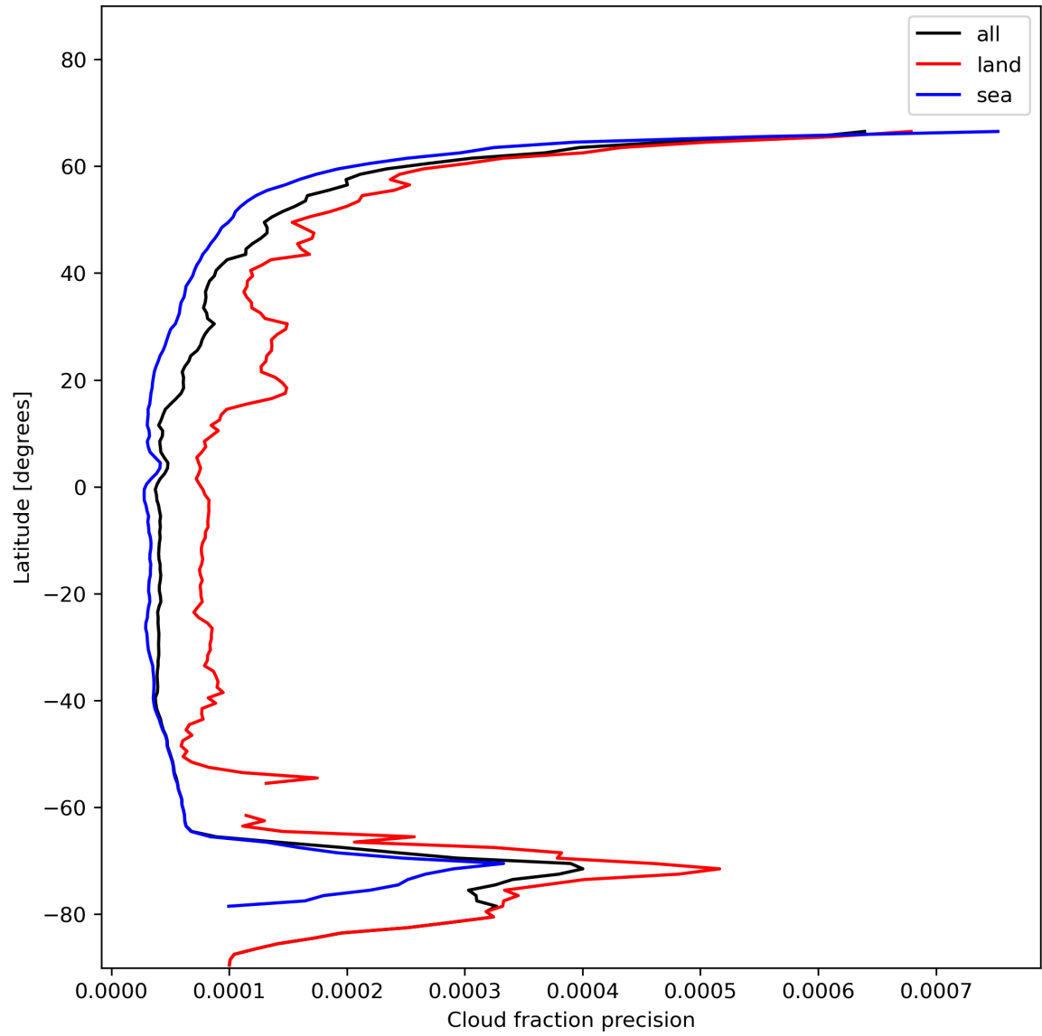
Figure 16: Zonal average of “Cloud fraction precision” for 2024-01-10 to 2024-01-12.
