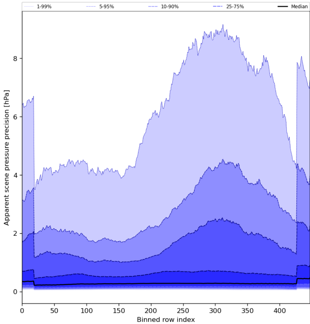
Figure 54: Along track statistics of “Apparent scene pressure precision” for 2024-01-10 to 2024-01-12
