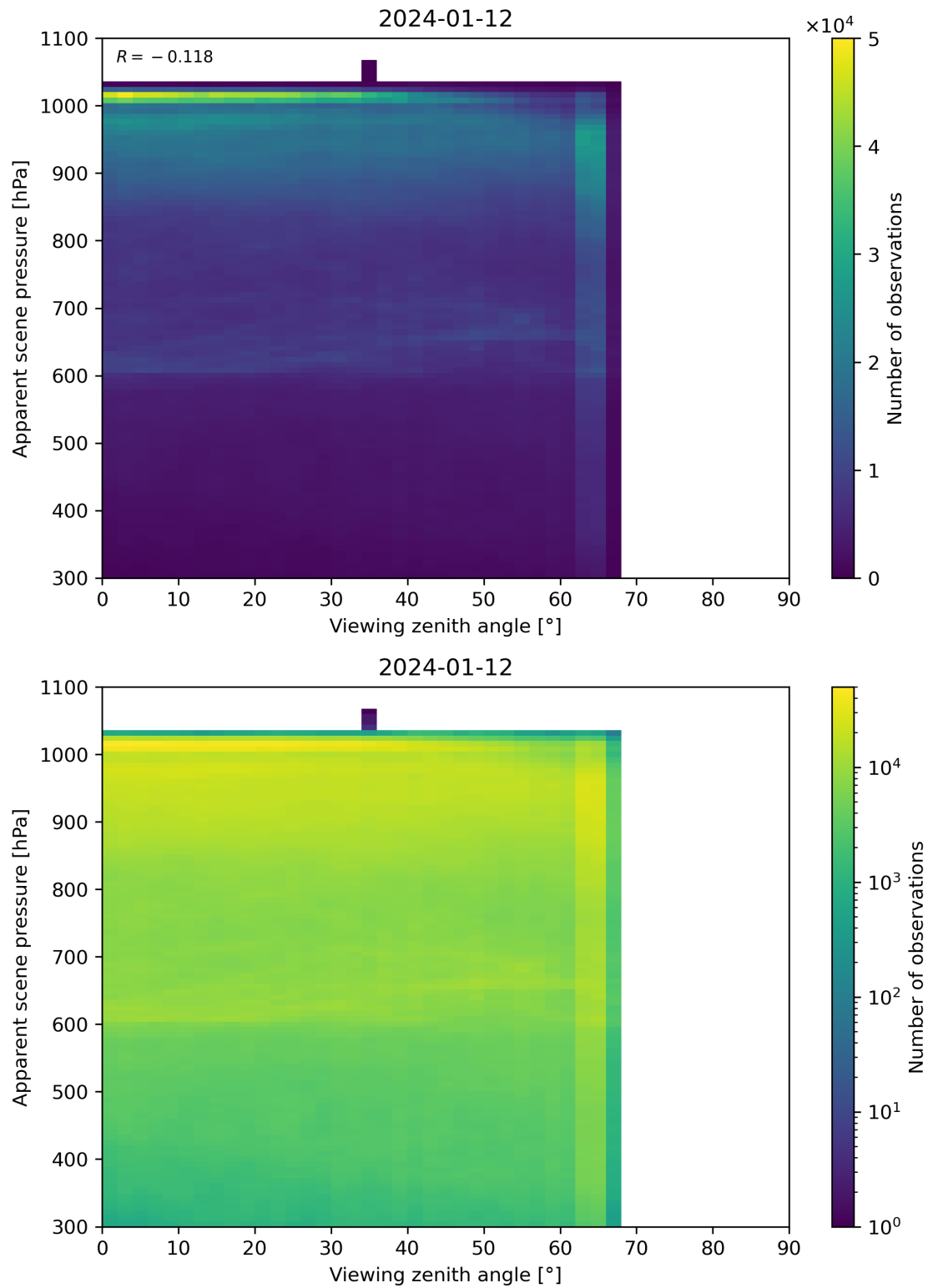
Figure 118: Scatter density plot of “Viewing zenith angle” against “Apparent scene pressure” for 2024-01-11 to 2024-01-13.
