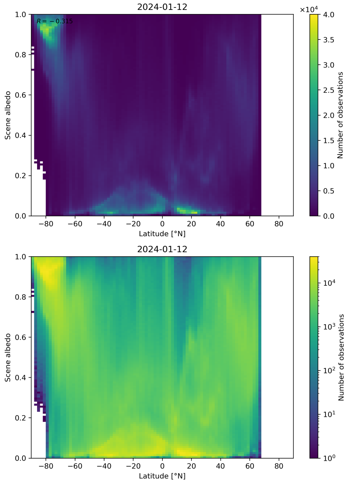
Figure 95: Scatter density plot of “Latitude” against “Scene albedo” for 2024-01-11 to 2024-01-13.
