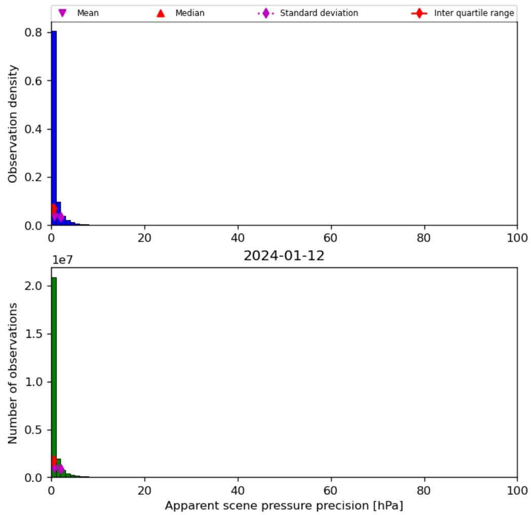
Figure 37: Histogram of “Apparent scene pressure precision” for 2024-01-11 to 2024-01-13
