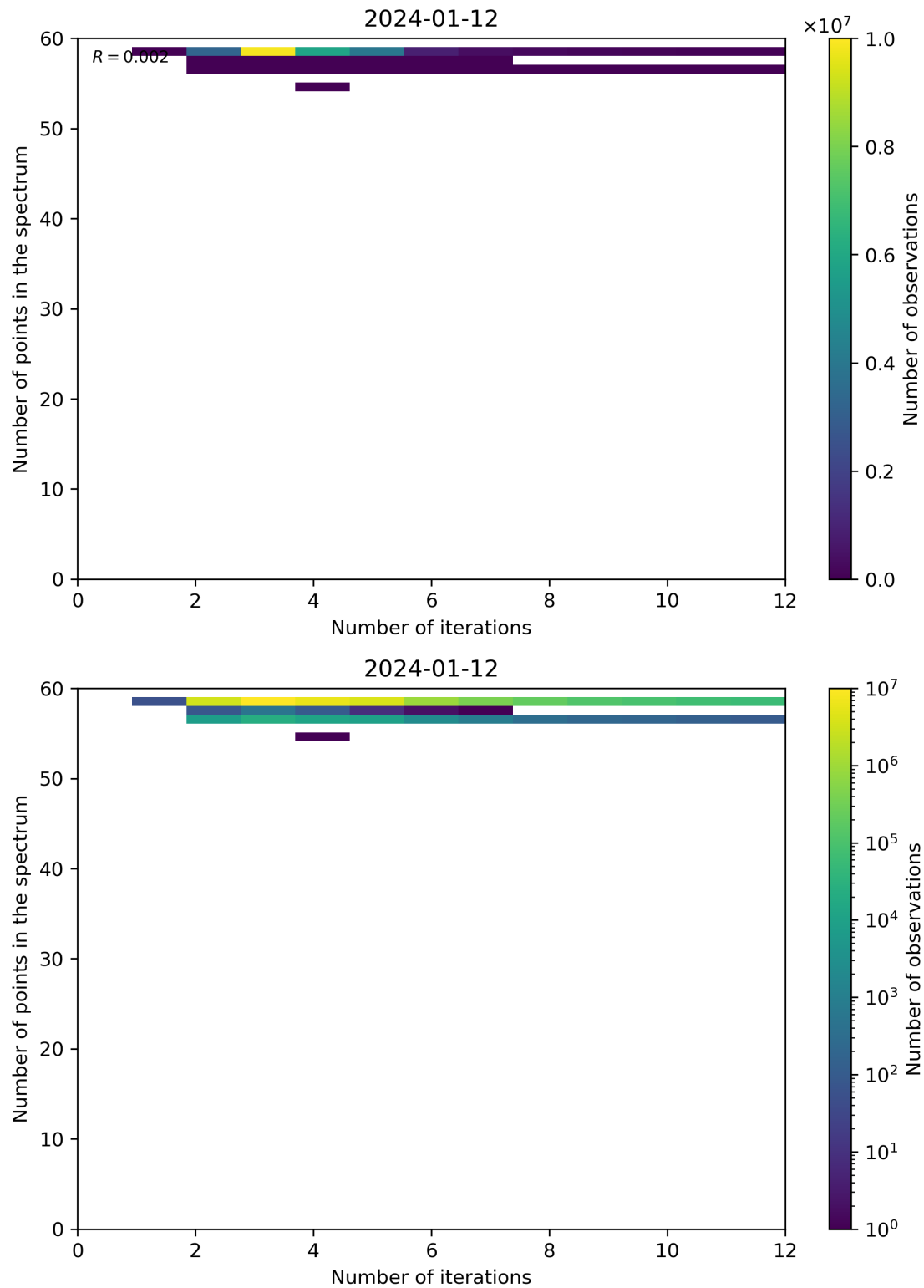
Figure 99: Scatter density plot of “Number of iterations” against “Number of points in the spectrum” for 2024-01-11 to 2024-01-13.
