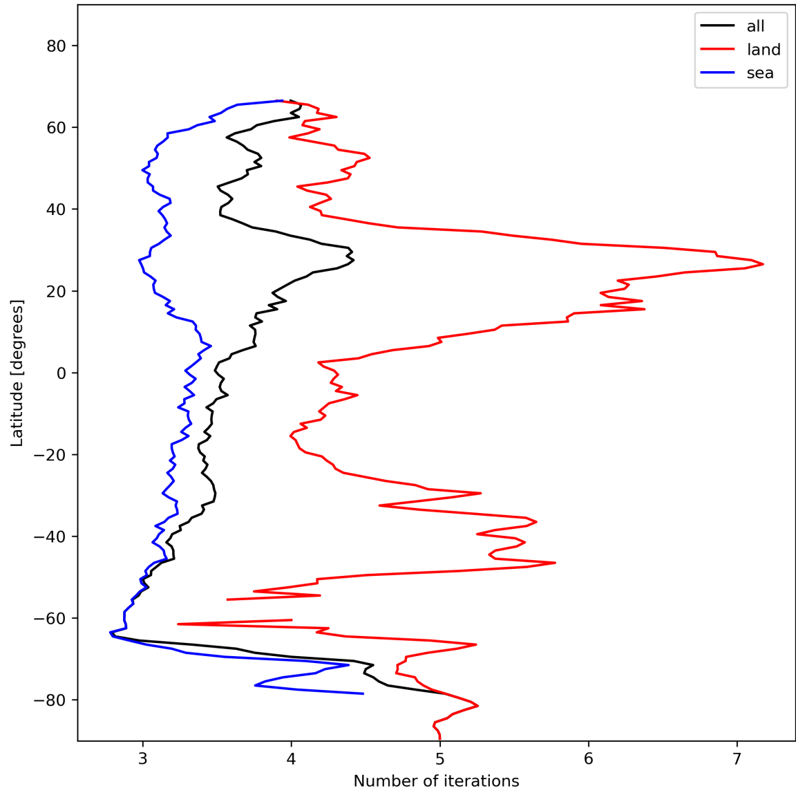
Figure 22: Zonal average of “Number of iterations” for 2024-01-11 to 2024-01-13.
