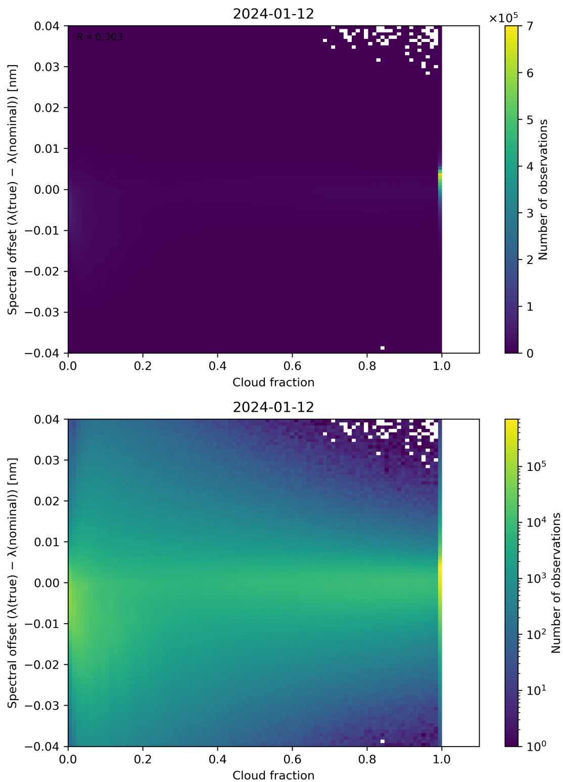
Figure 76: Scatter density plot of “Cloud fraction” against “Spectral offset ( \lambda(\text{true}) - \lambda(\text{nominal}) )” for 2024-01-11 to 2024-01-13.
