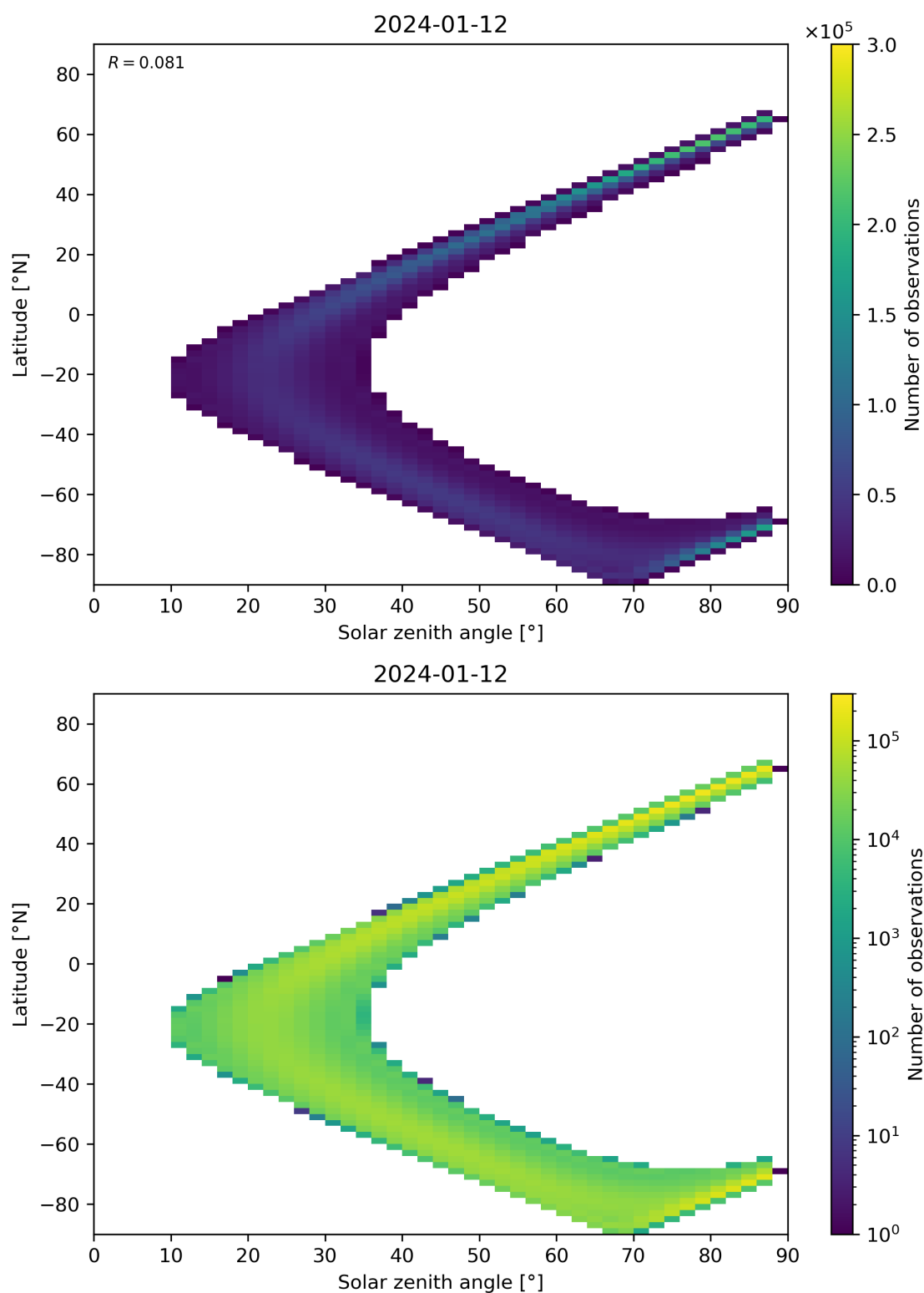
Figure 113: Scatter density plot of “Solar zenith angle” against “Latitude” for 2024-01-11 to 2024-01-13.
