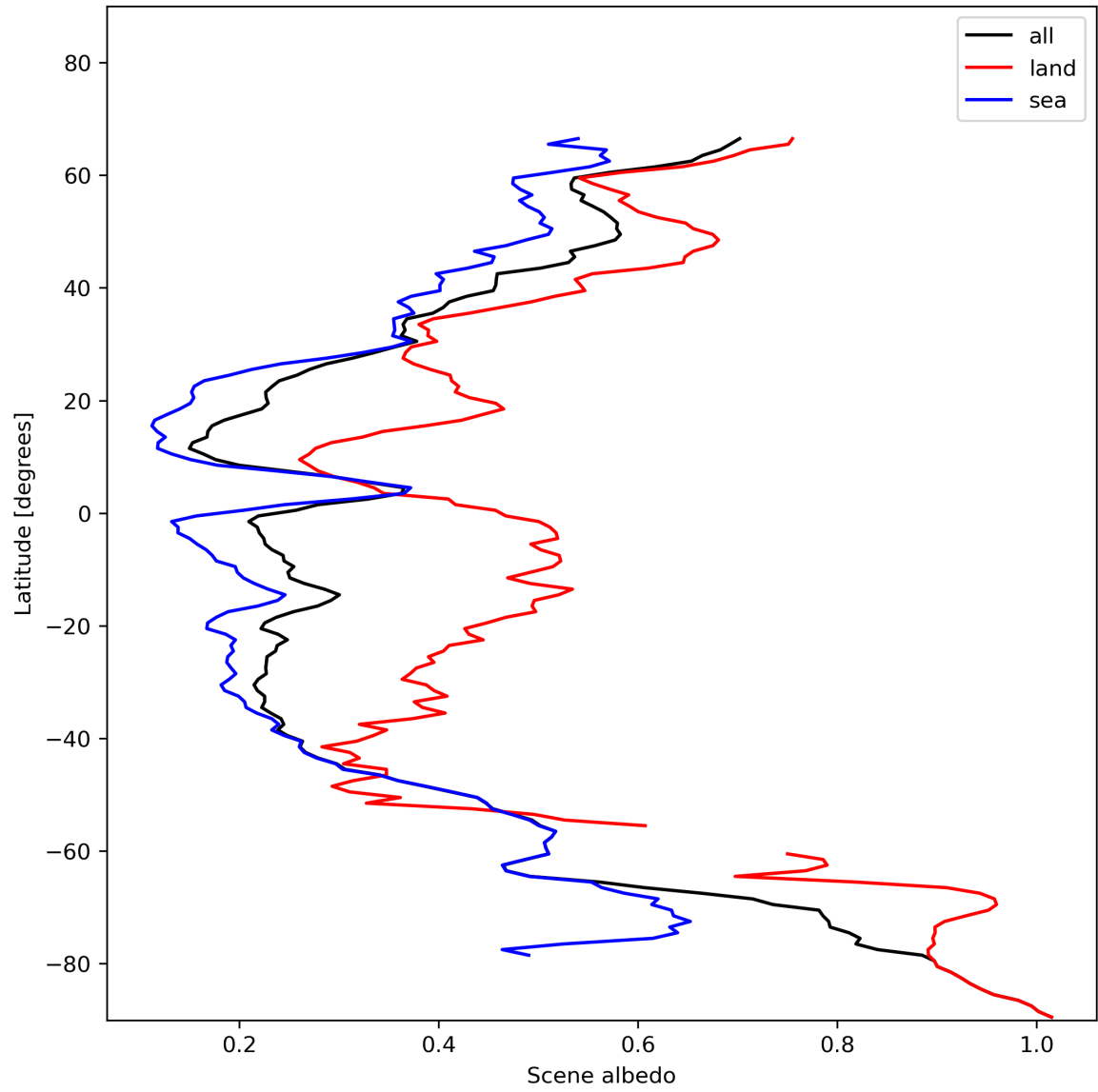
Figure 17: Zonal average of “Scene albedo” for 2024-01-11 to 2024-01-13.
