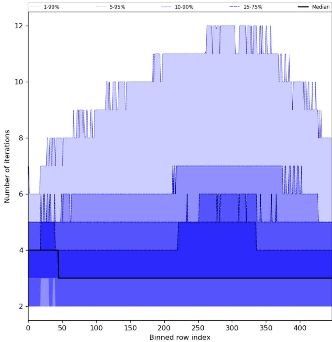
Figure 56: Along track statistics of “Number of iterations” for 2024-01-11 to 2024-01-13
