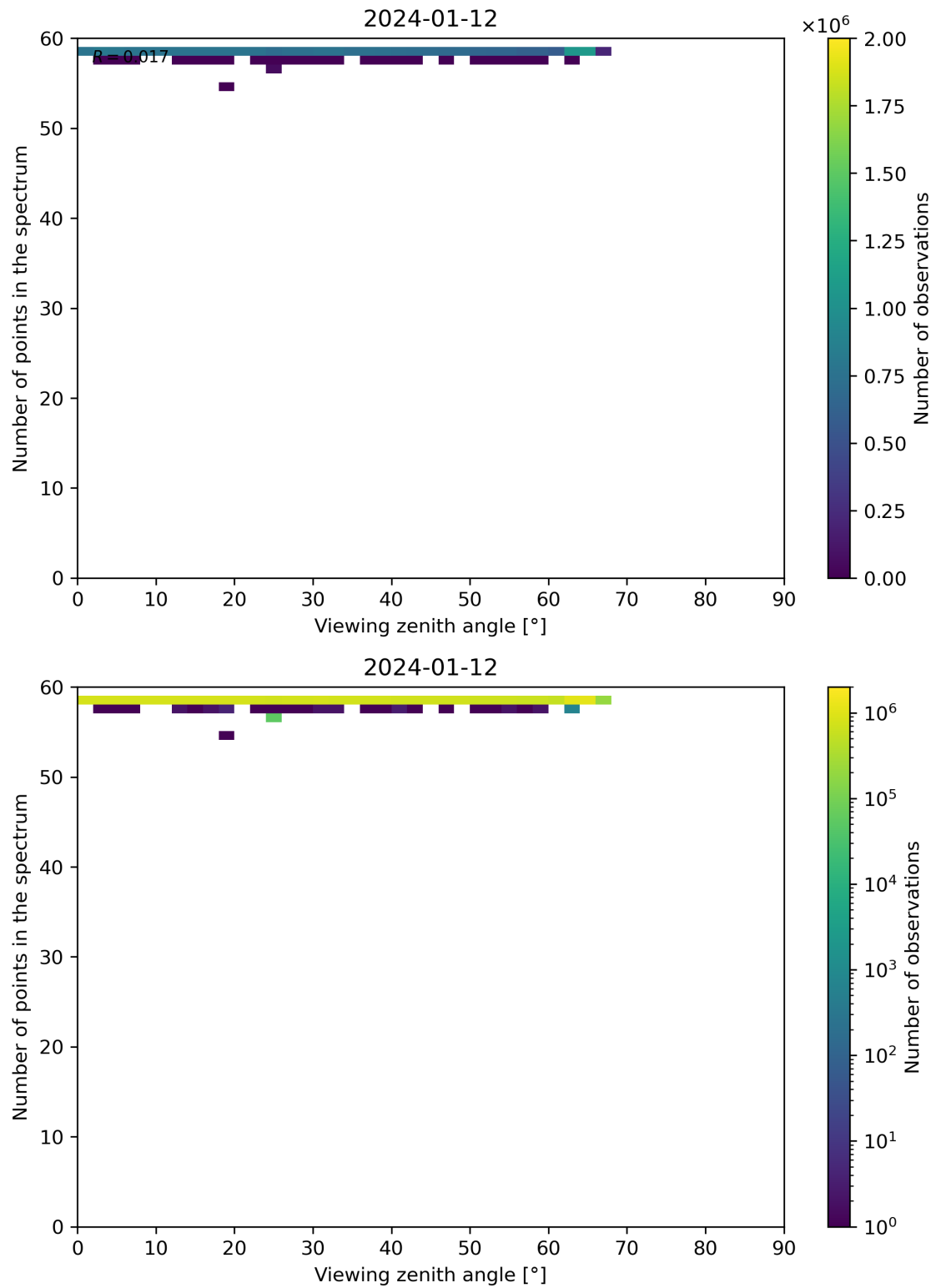
Figure 125: Scatter density plot of “Viewing zenith angle” against “Number of points in the spectrum” for 2024-01-11 to 2024-01-13.
