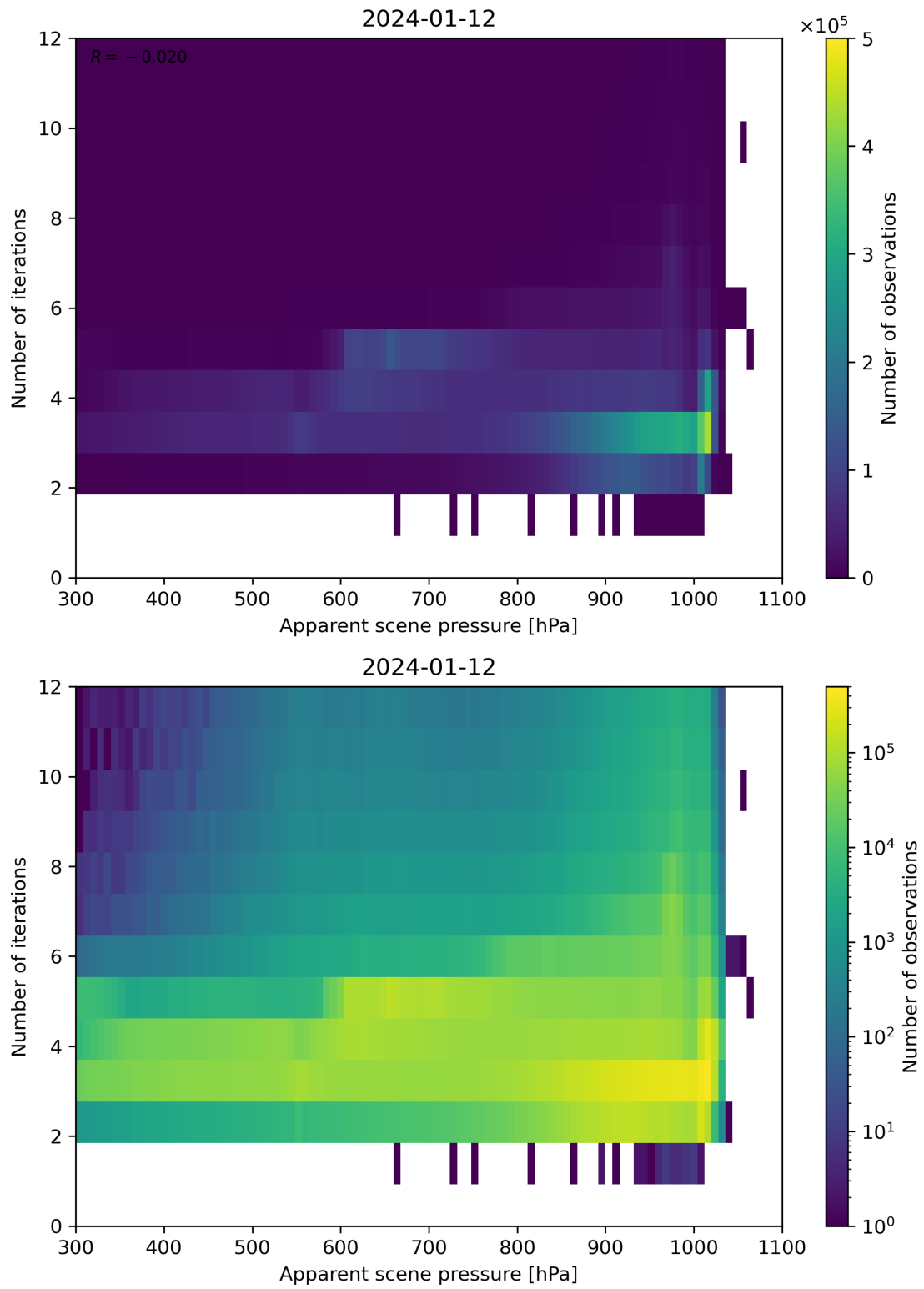
Figure 65: Scatter density plot of “Apparent scene pressure” against “Number of iterations” for 2024-01-11 to 2024-01-13.
