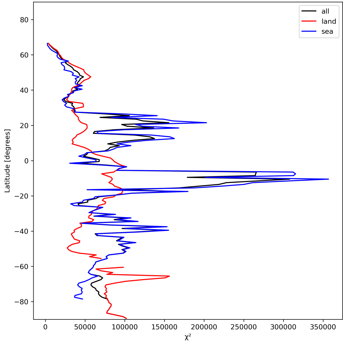
Figure 21: Zonal average of “ \chi^2 ” for 2024-01-11 to 2024-01-13.
