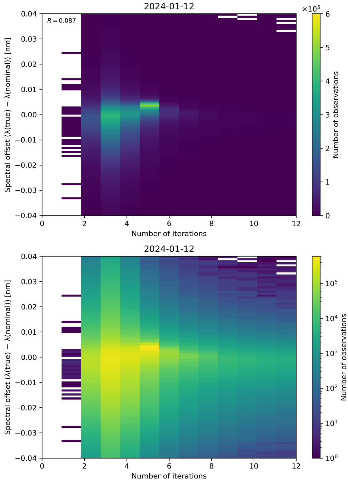
Figure 100: Scatter density plot of “Number of iterations” against “Spectral offset ( \lambda(\text{true}) - \lambda(\text{nominal}) )” for 2024-01-11 to 2024-01-13.
