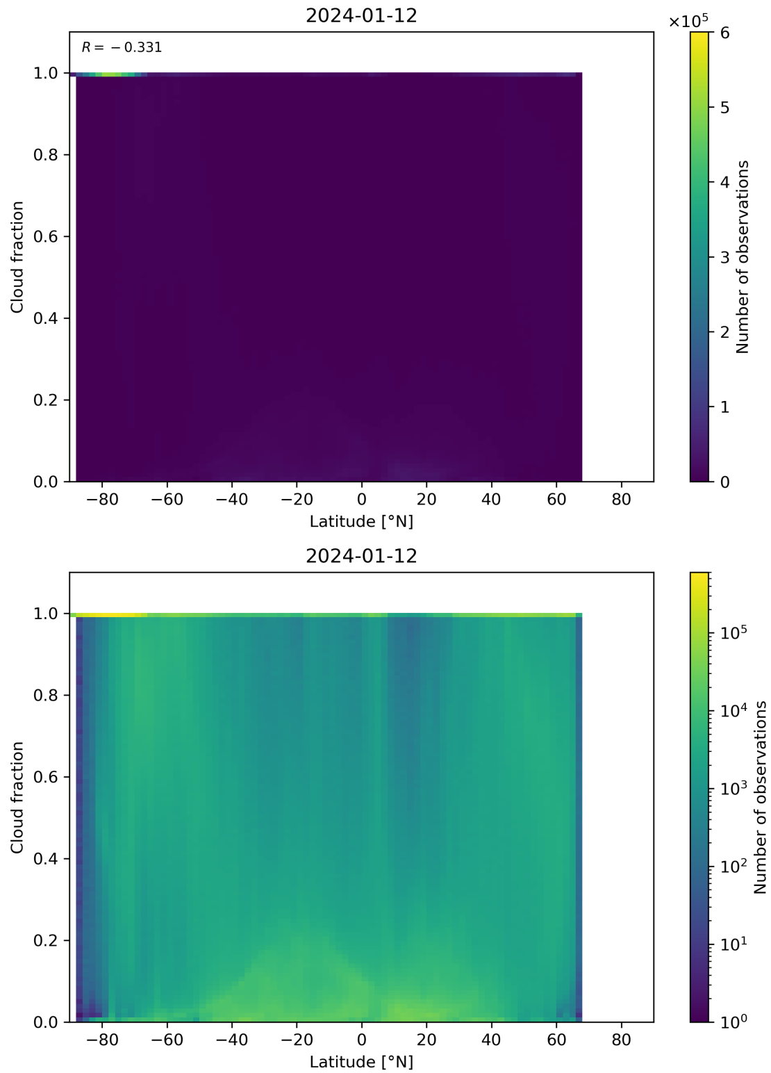
Figure 90: Scatter density plot of “Latitude” against “Cloud fraction” for 2024-01-11 to 2024-01-13.
