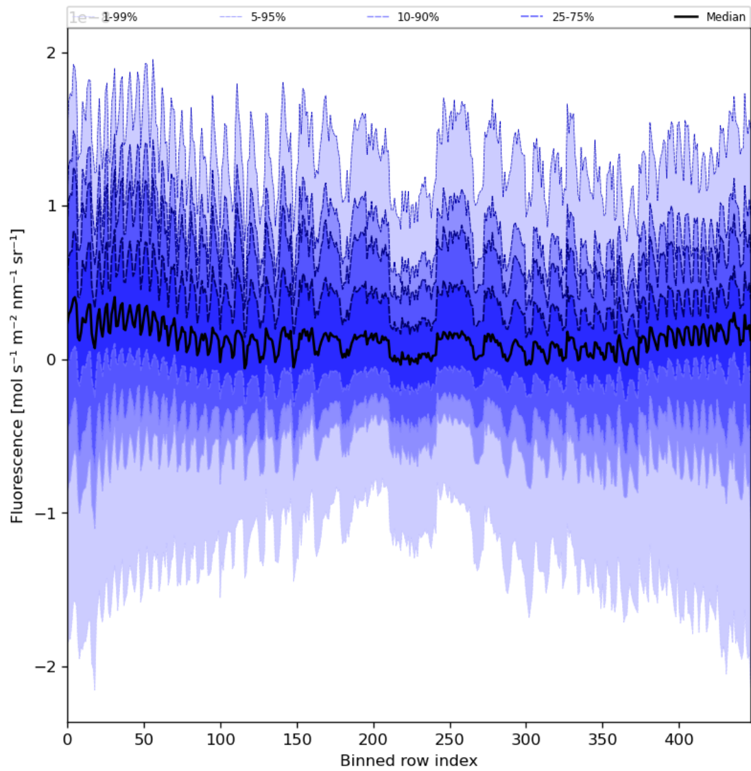
Figure 57: Along track statistics of “Fluorescence” for 2024-01-11 to 2024-01-13
