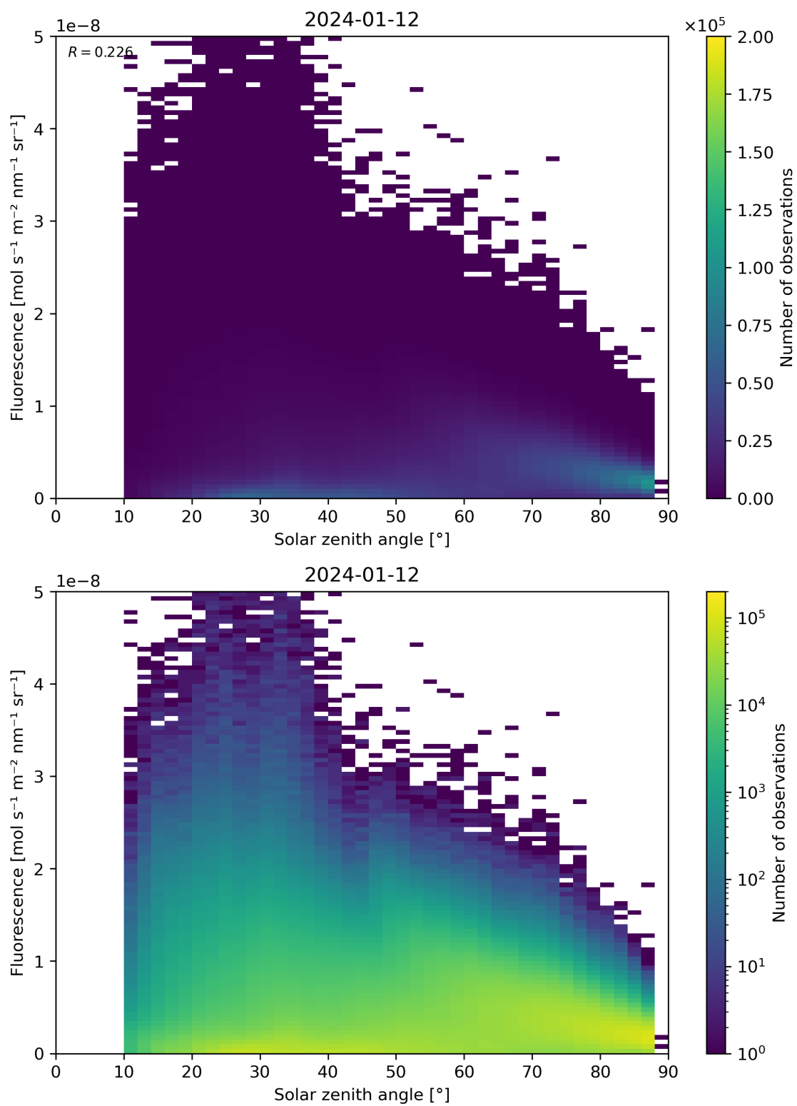
Figure 112: Scatter density plot of “Solar zenith angle” against “Fluorescence” for 2024-01-11 to 2024-01-13.
