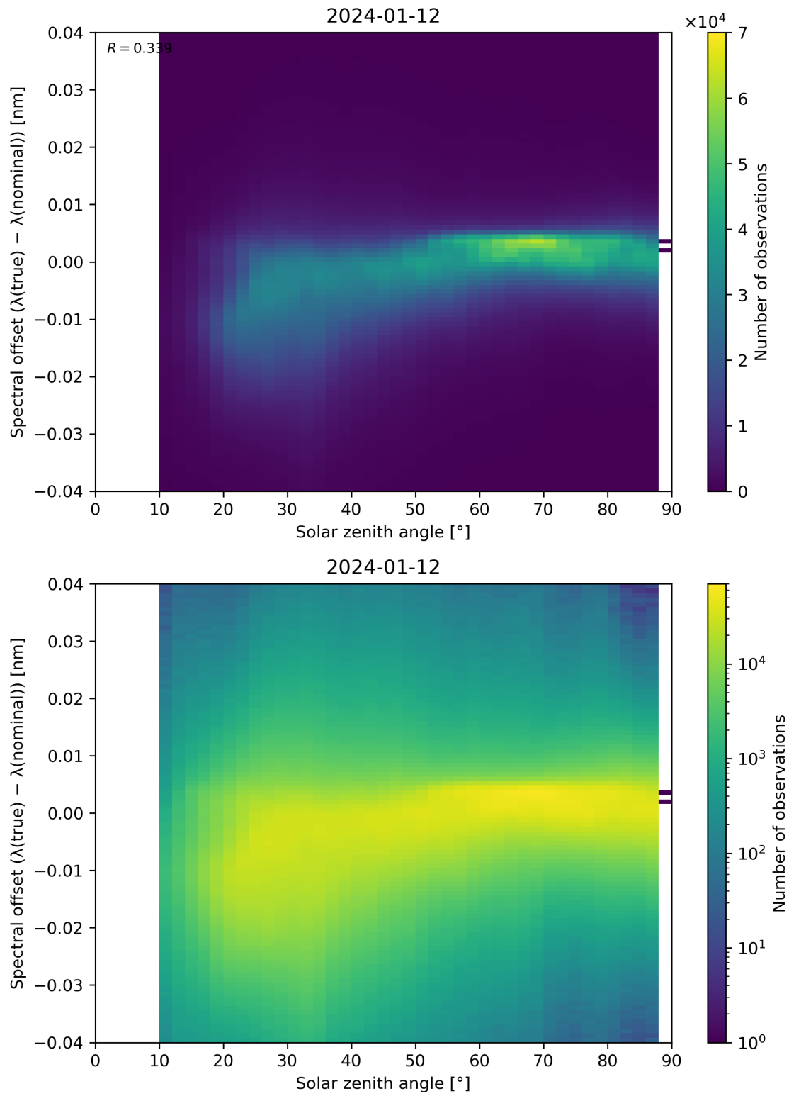
Figure 117: Scatter density plot of “Solar zenith angle” against “Spectral offset ( \lambda(\text{true}) - \lambda(\text{nominal}) )” for 2024-01-11 to 2024-01-13.
