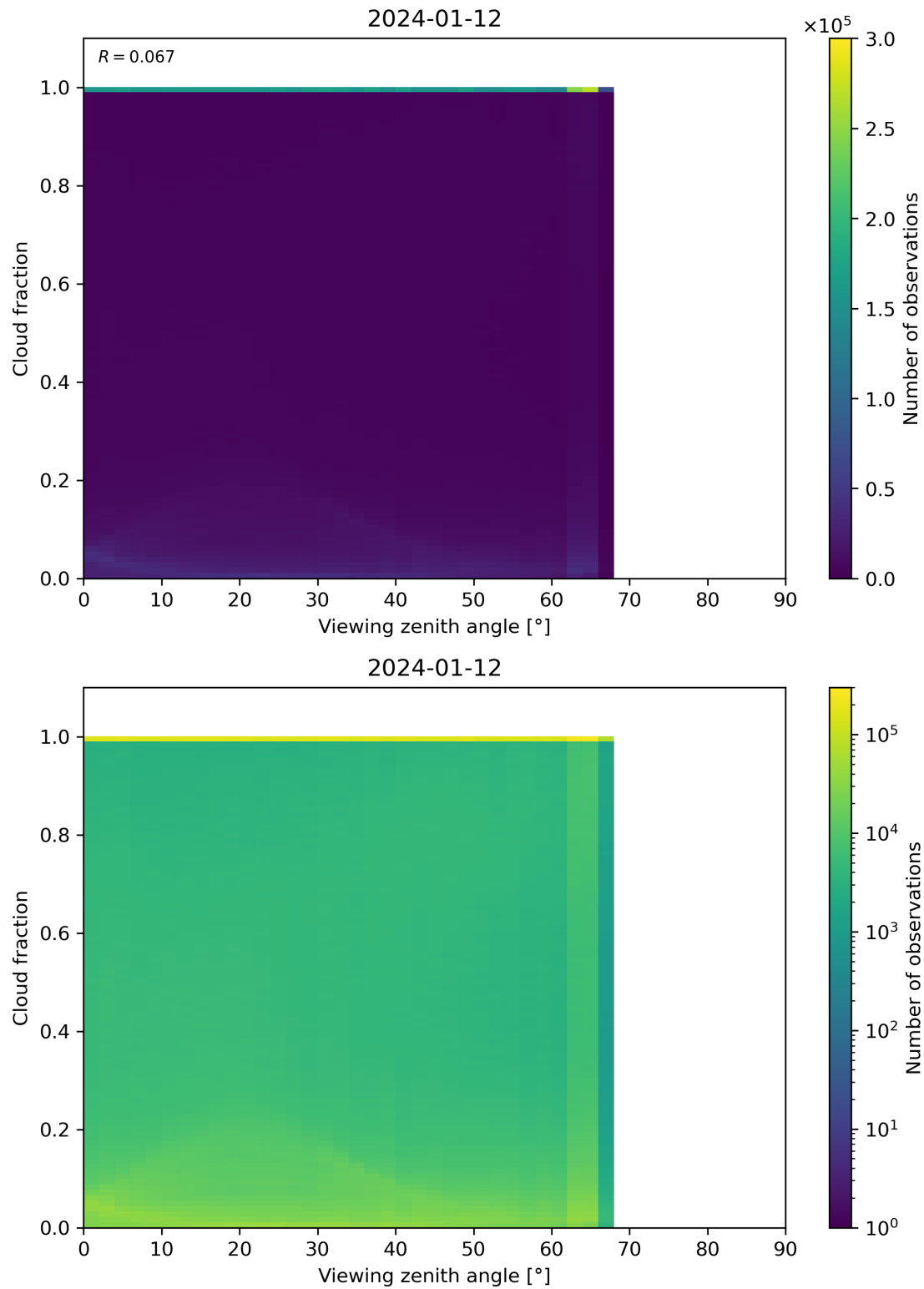
Figure 120: Scatter density plot of “Viewing zenith angle” against “Cloud fraction” for 2024-01-11 to 2024-01-13.
