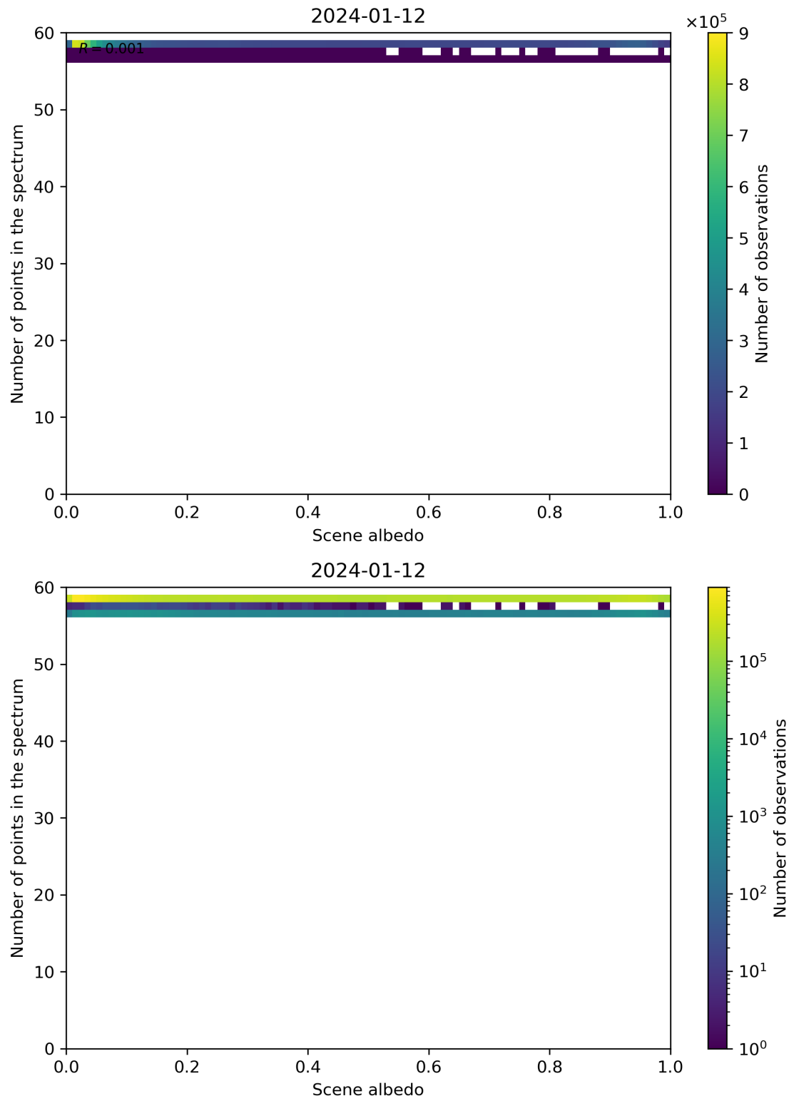
Figure 106: Scatter density plot of “Scene albedo” against “Number of points in the spectrum” for 2024-01-11 to 2024-01-13.
