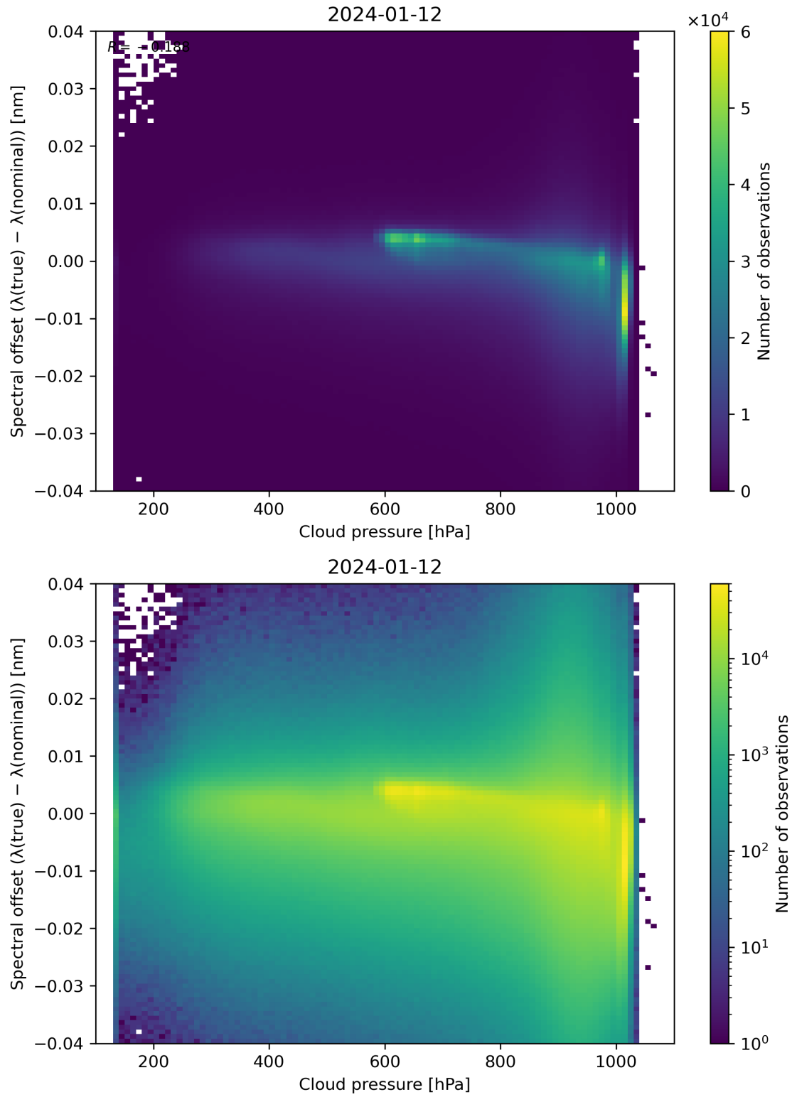
Figure 84: Scatter density plot of “Cloud pressure” against “Spectral offset ( \lambda(\text{true}) - \lambda(\text{nominal}) )” for 2024-01-11 to 2024-01-13.
