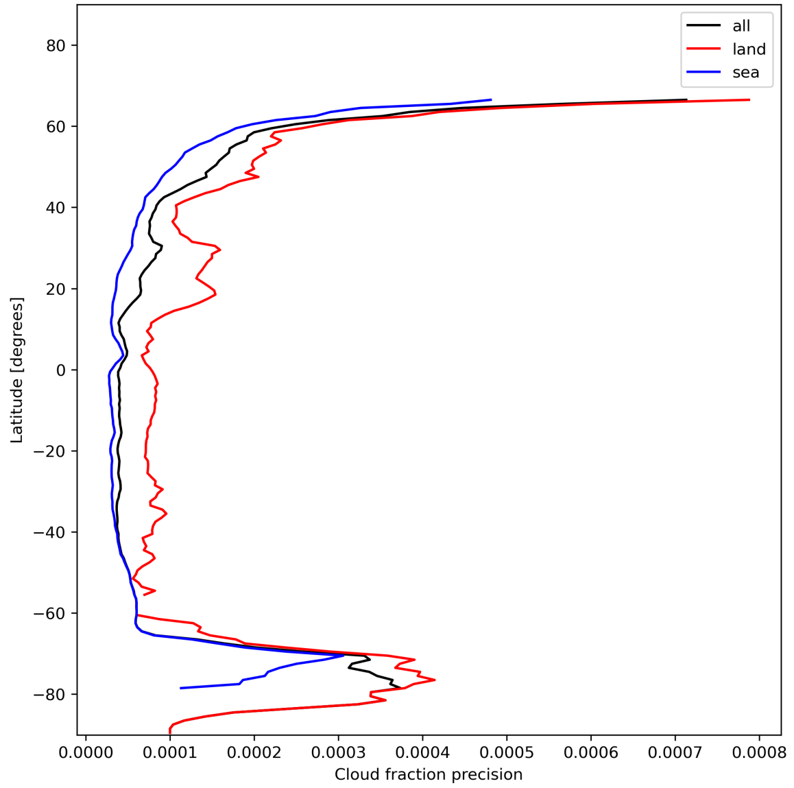
Figure 16: Zonal average of “Cloud fraction precision” for 2024-01-11 to 2024-01-13.
