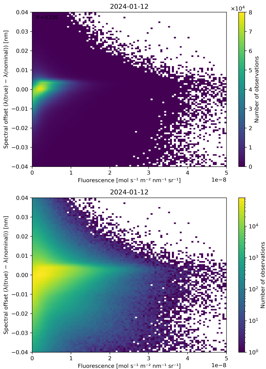
Figure 87: Scatter density plot of “Fluorescence” against “Spectral offset ( \lambda(\text{true}) - \lambda(\text{nominal}) )” for 2024-01-11 to 2024-01-13.
