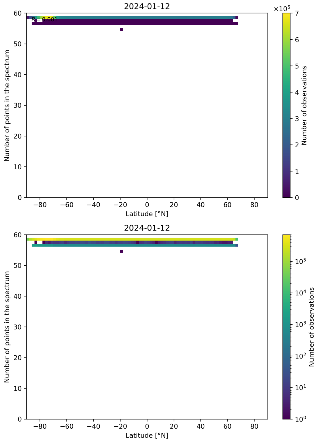
Figure 94: Scatter density plot of “Latitude” against “Number of points in the spectrum” for 2024-01-11 to 2024-01-13.
