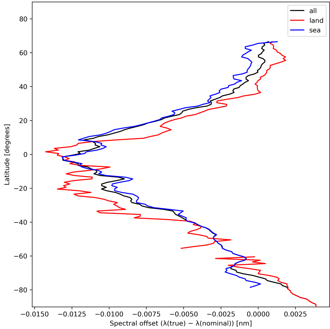
Figure 28: Zonal average of “Spectral offset ( \lambda(\text{true}) - \lambda(\text{nominal}) )” for 2024-01-11 to 2024-01-13.
