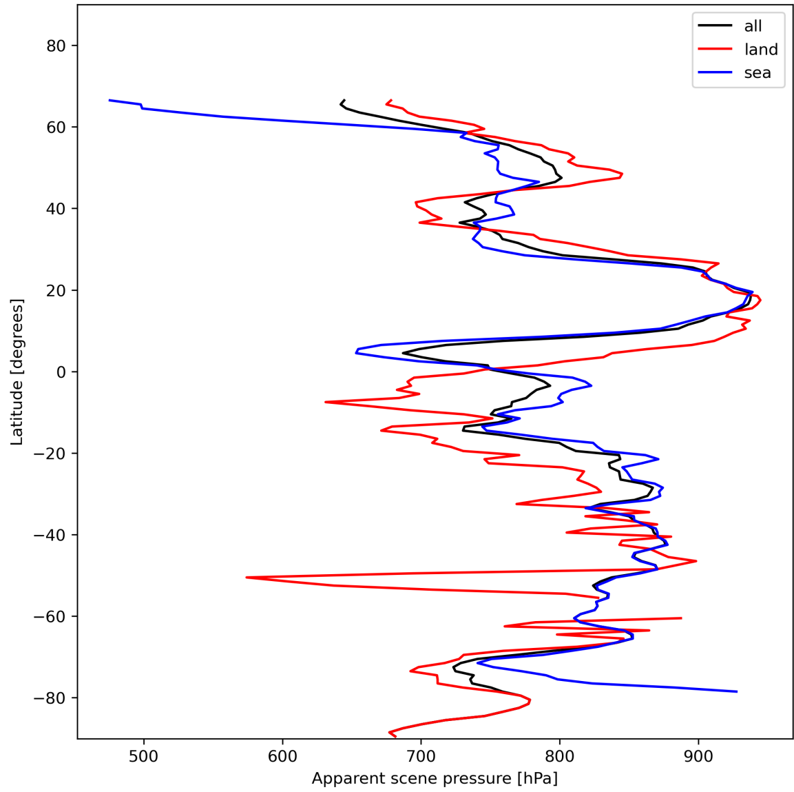
Figure 19: Zonal average of “Apparent scene pressure” for 2024-01-11 to 2024-01-13.
