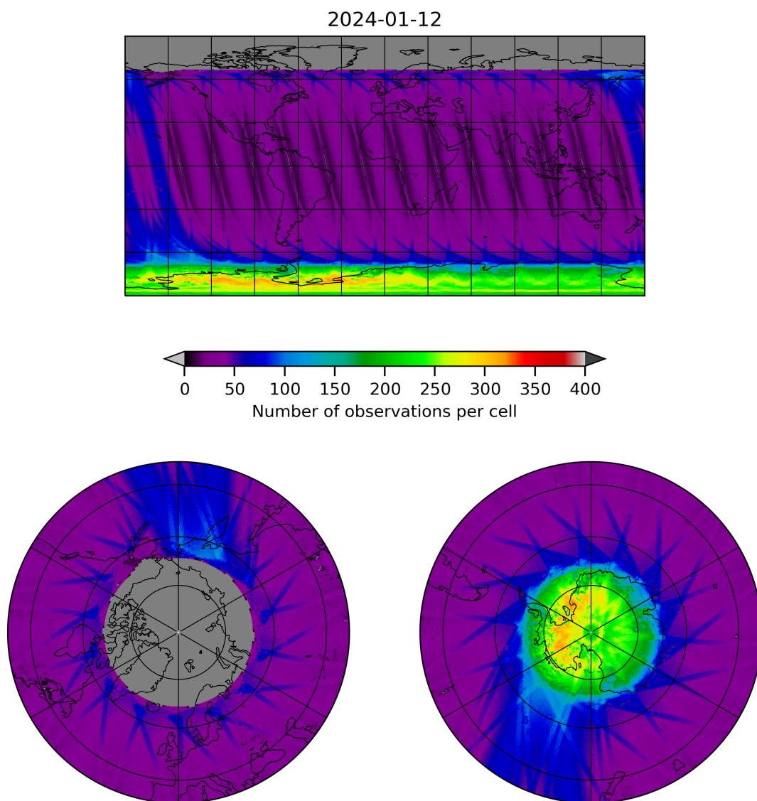
Figure 11: Map of the number of observations for 2024-01-11 to 2024-01-13
