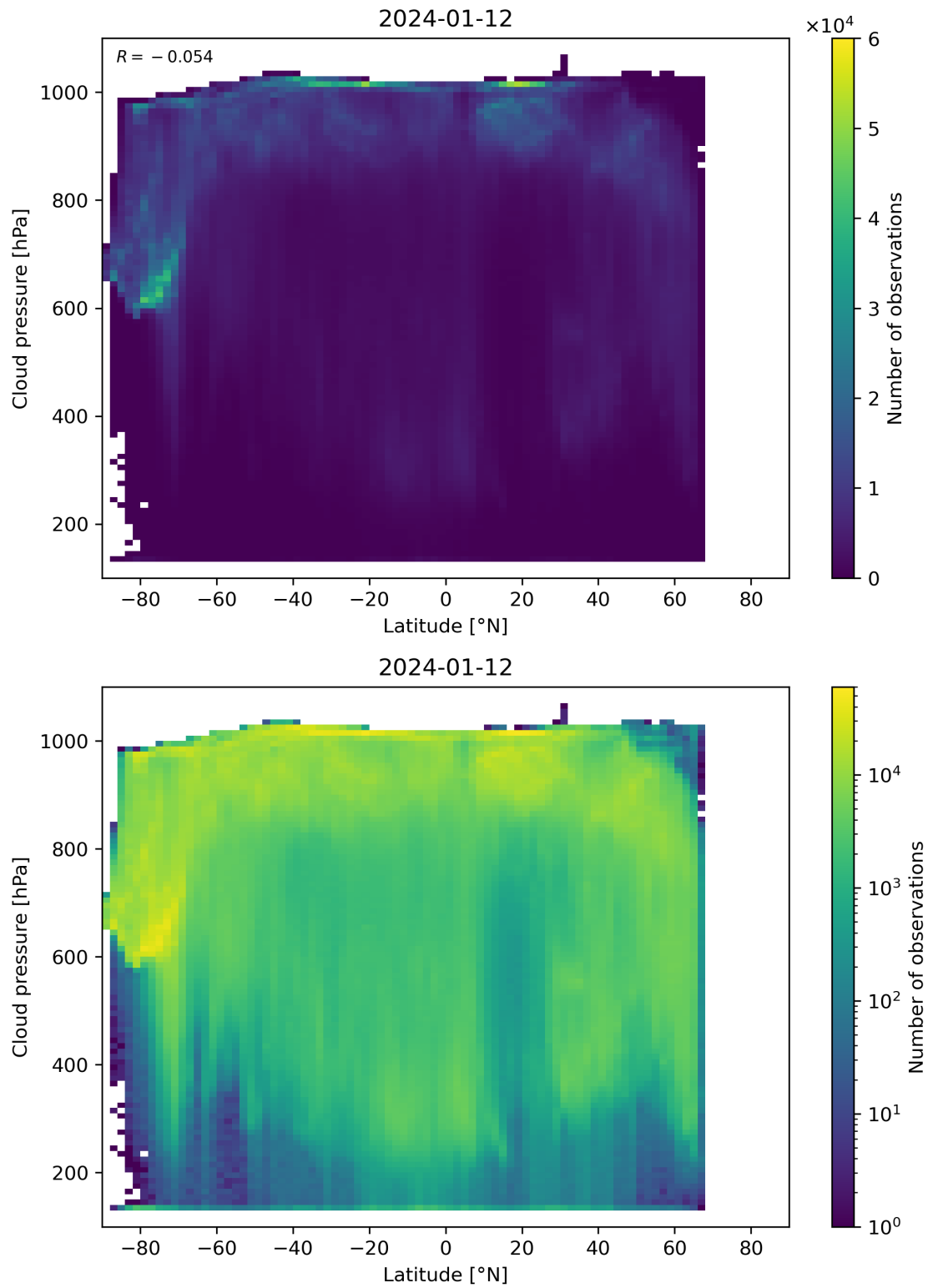
Figure 91: Scatter density plot of “Latitude” against “Cloud pressure” for 2024-01-11 to 2024-01-13.
