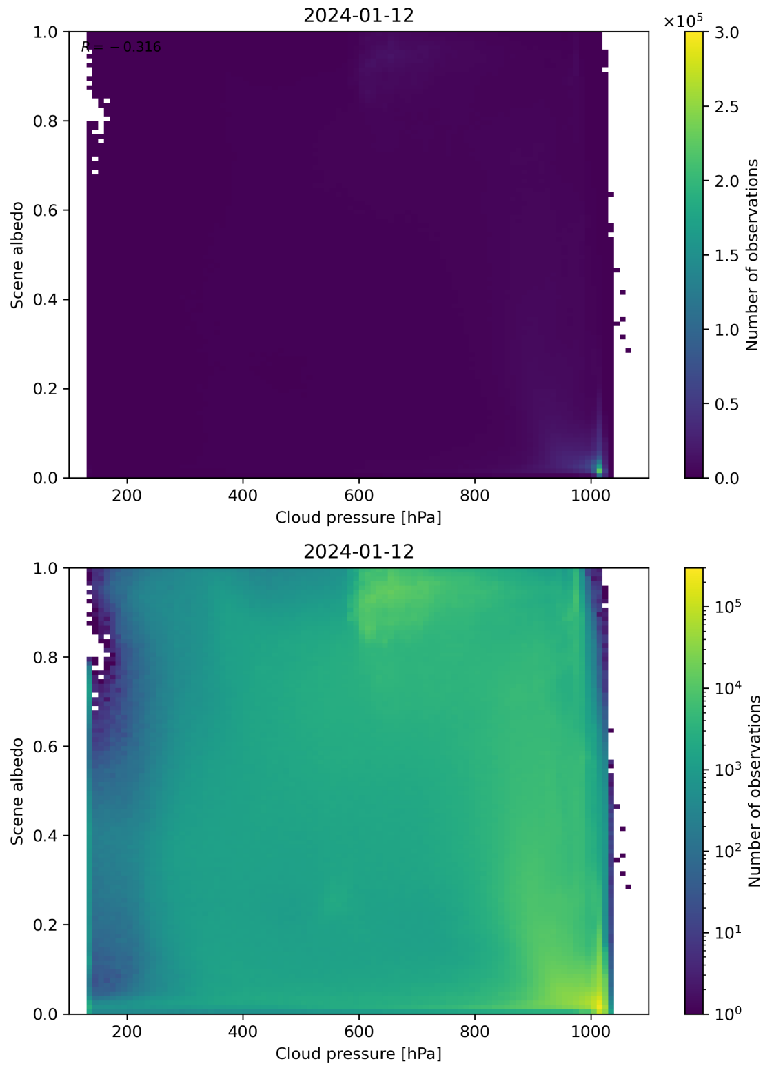
Figure 83: Scatter density plot of “Cloud pressure” against “Scene albedo” for 2024-01-11 to 2024-01-13.
