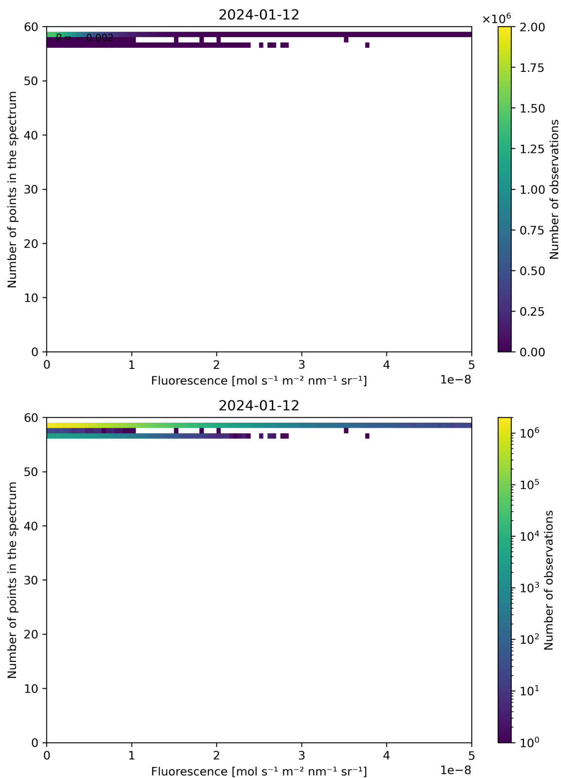
Figure 86: Scatter density plot of “Fluorescence” against “Number of points in the spectrum” for 2024-01-11 to 2024-01-13.
