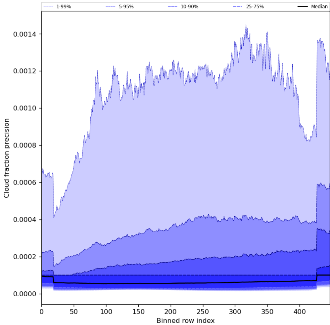
Figure 50: Along track statistics of “Cloud fraction precision” for 2024-01-11 to 2024-01-13
