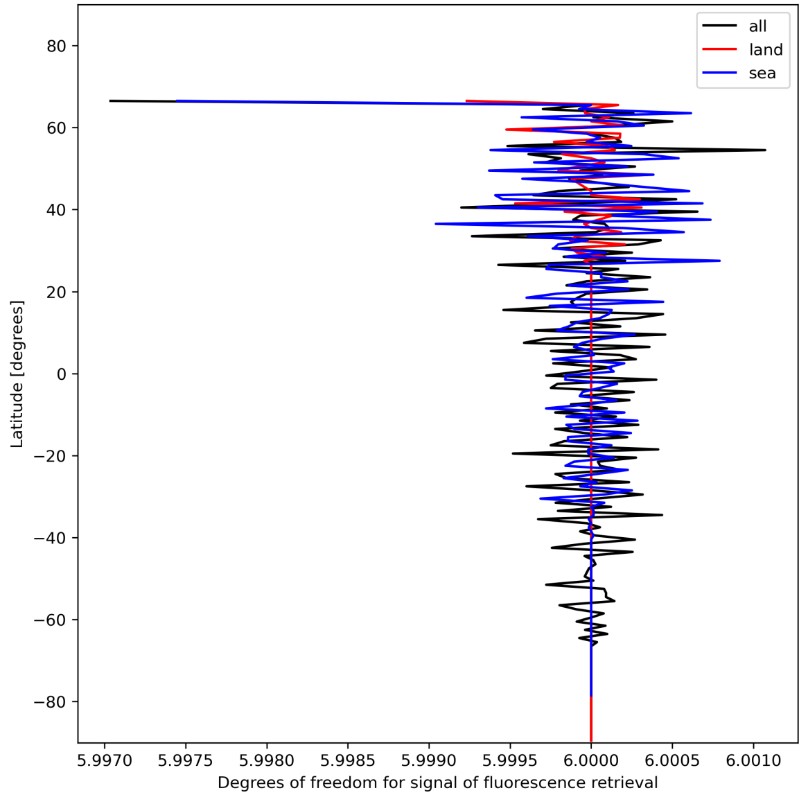
Figure 26: Zonal average of “Degrees of freedom for signal of fluorescence retrieval” for 2024-01-11 to 2024-01-13.
