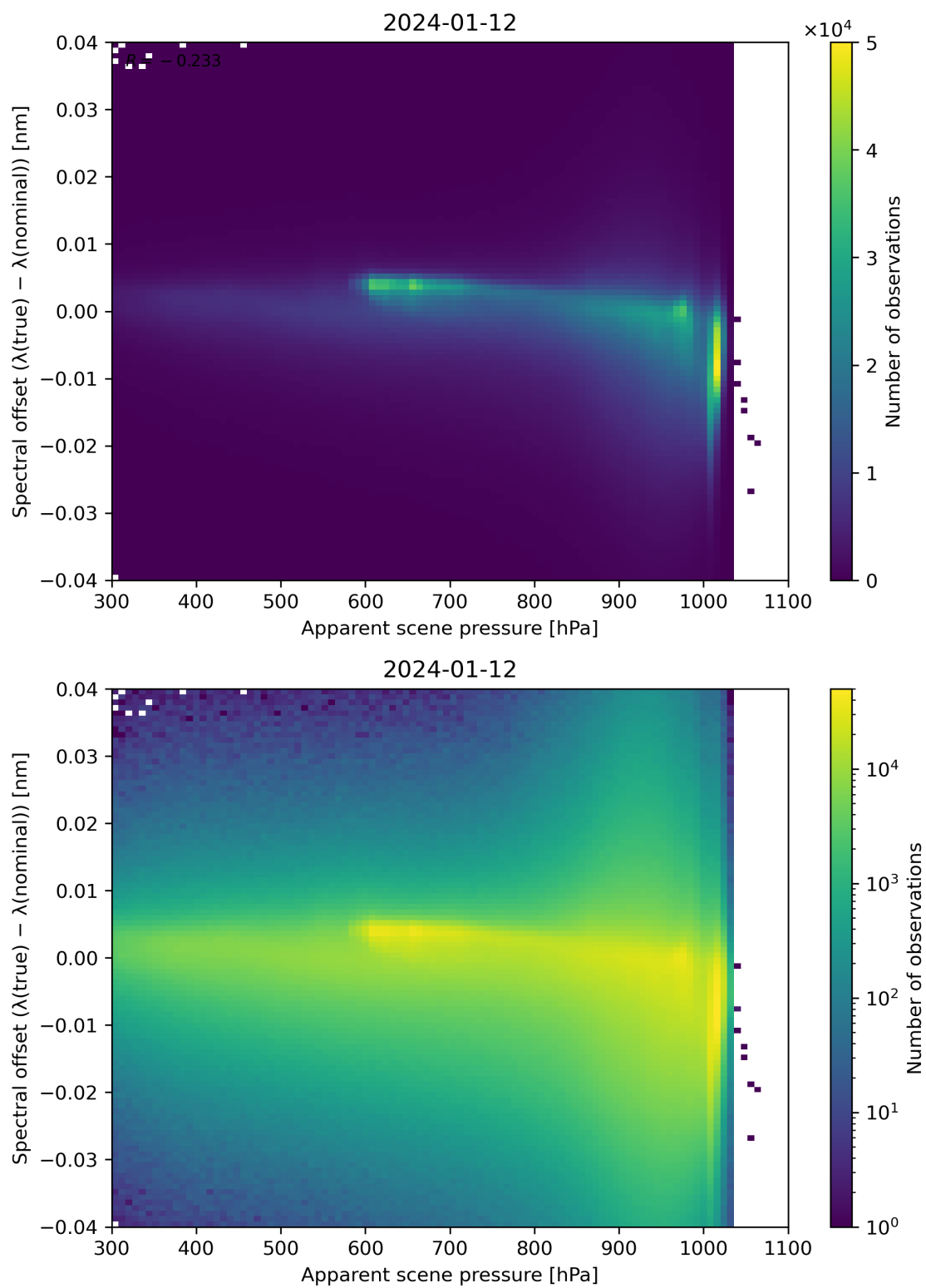
Figure 67: Scatter density plot of “Apparent scene pressure” against “Spectral offset ( \lambda(\text{true}) - \lambda(\text{nominal}) )” for 2024-01-11 to 2024-01-13.
