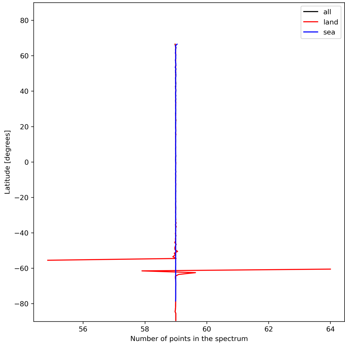
Figure 27: Zonal average of “Number of points in the spectrum” for 2024-01-11 to 2024-01-13.
