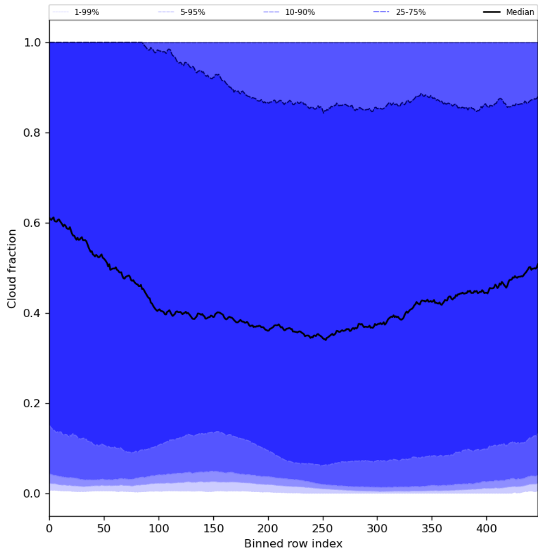
Figure 49: Along track statistics of “Cloud fraction” for 2024-01-11 to 2024-01-13
