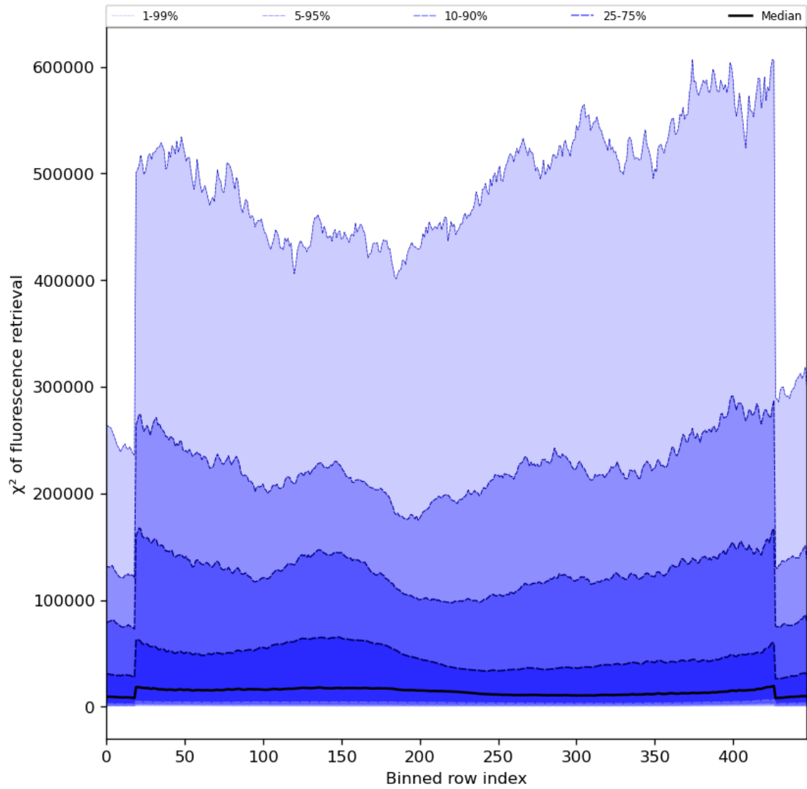
Figure 59: Along track statistics of “ \chi^2 of fluorescence retrieval” for 2024-01-11 to 2024-01-13
