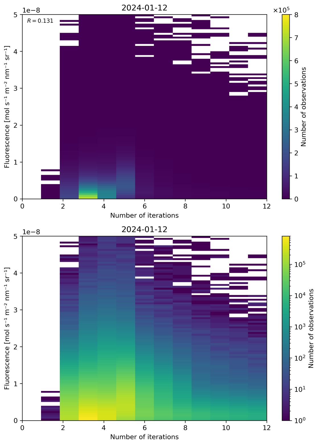
Figure 98: Scatter density plot of “Number of iterations” against “Fluorescence” for 2024-01-11 to 2024-01-13.
