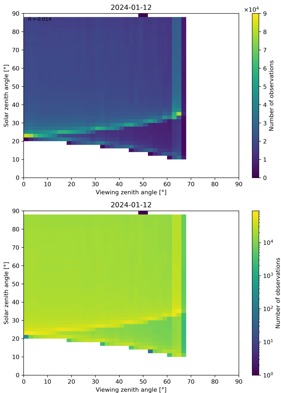
Figure 127: Scatter density plot of “Viewing zenith angle” against “Solar zenith angle” for 2024-01-11 to 2024-01-13.
