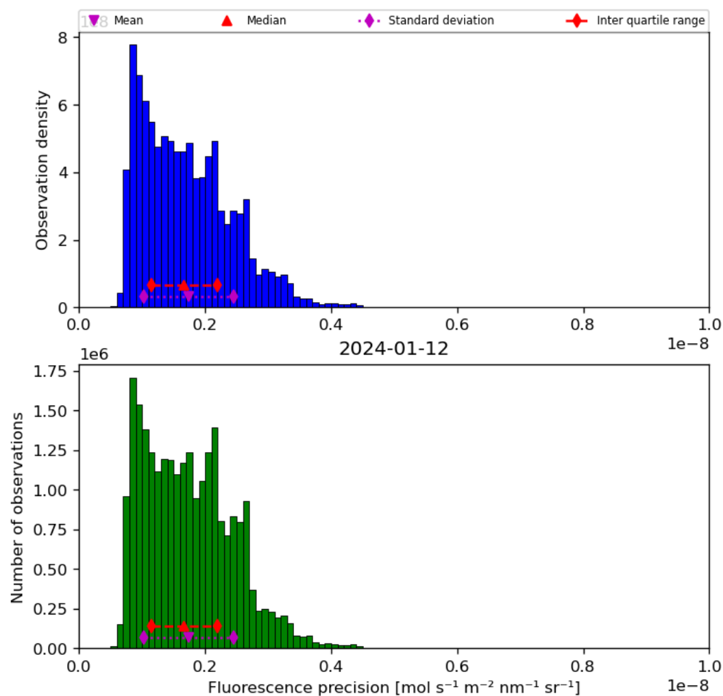
Figure 41: Histogram of “Fluorescence precision” for 2024-01-11 to 2024-01-13
