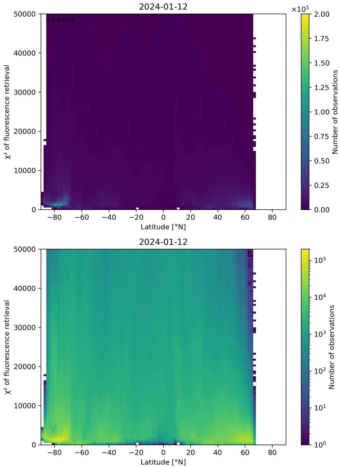
Figure 89: Scatter density plot of “Latitude” against “ \chi^2 of fluorescence retrieval” for 2024-01-11 to 2024-01-13.
