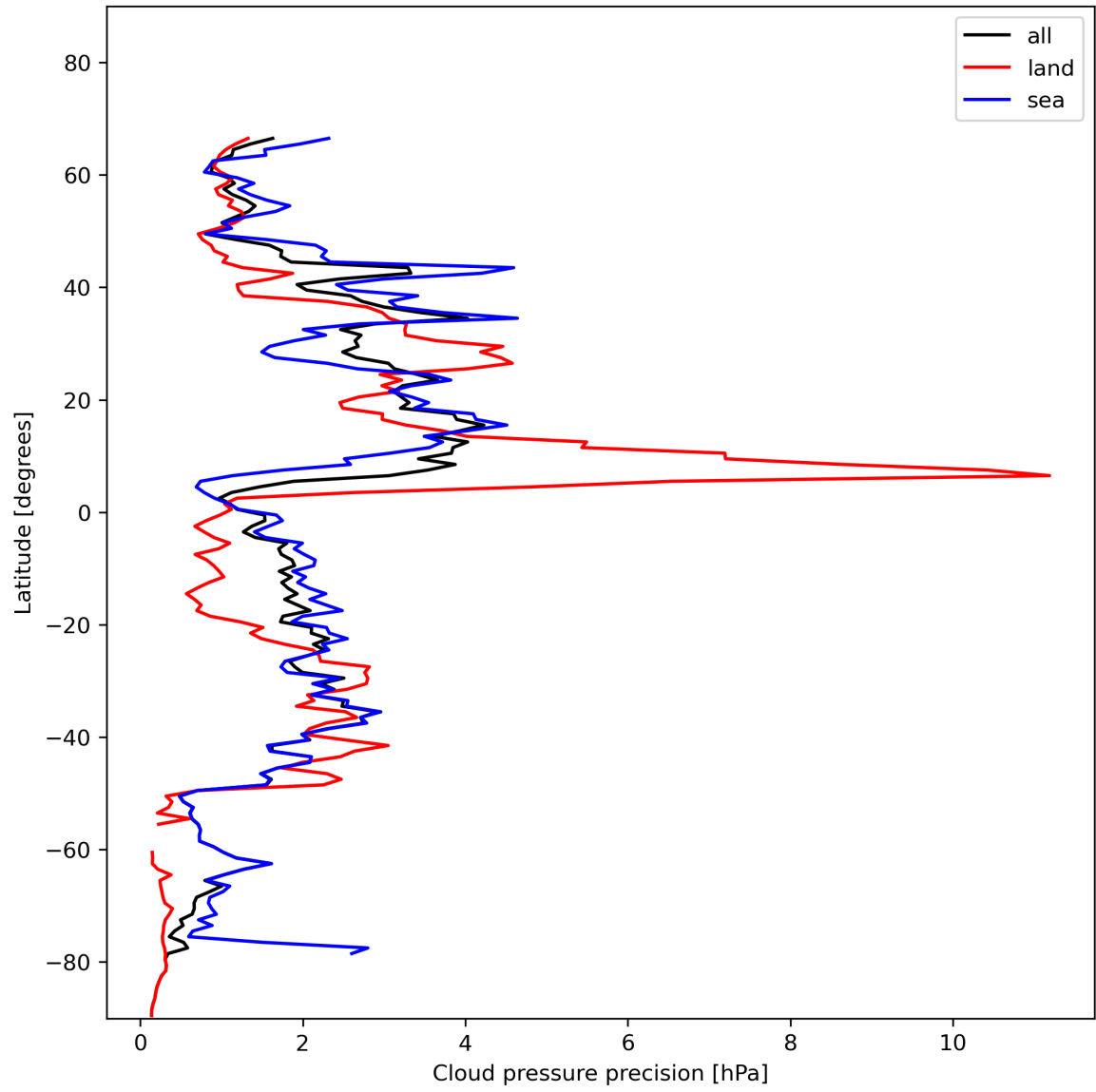
Figure 14: Zonal average of “Cloud pressure precision” for 2024-01-11 to 2024-01-13.
