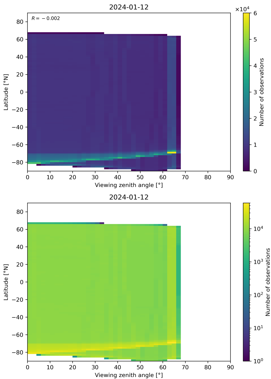
Figure 123: Scatter density plot of “Viewing zenith angle” against “Latitude” for 2024-01-11 to 2024-01-13.
