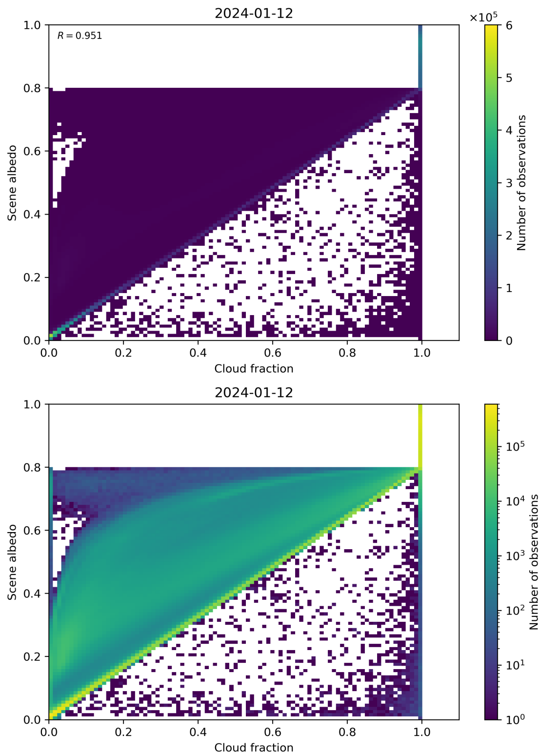
Figure 75: Scatter density plot of “Cloud fraction” against “Scene albedo” for 2024-01-11 to 2024-01-13.
