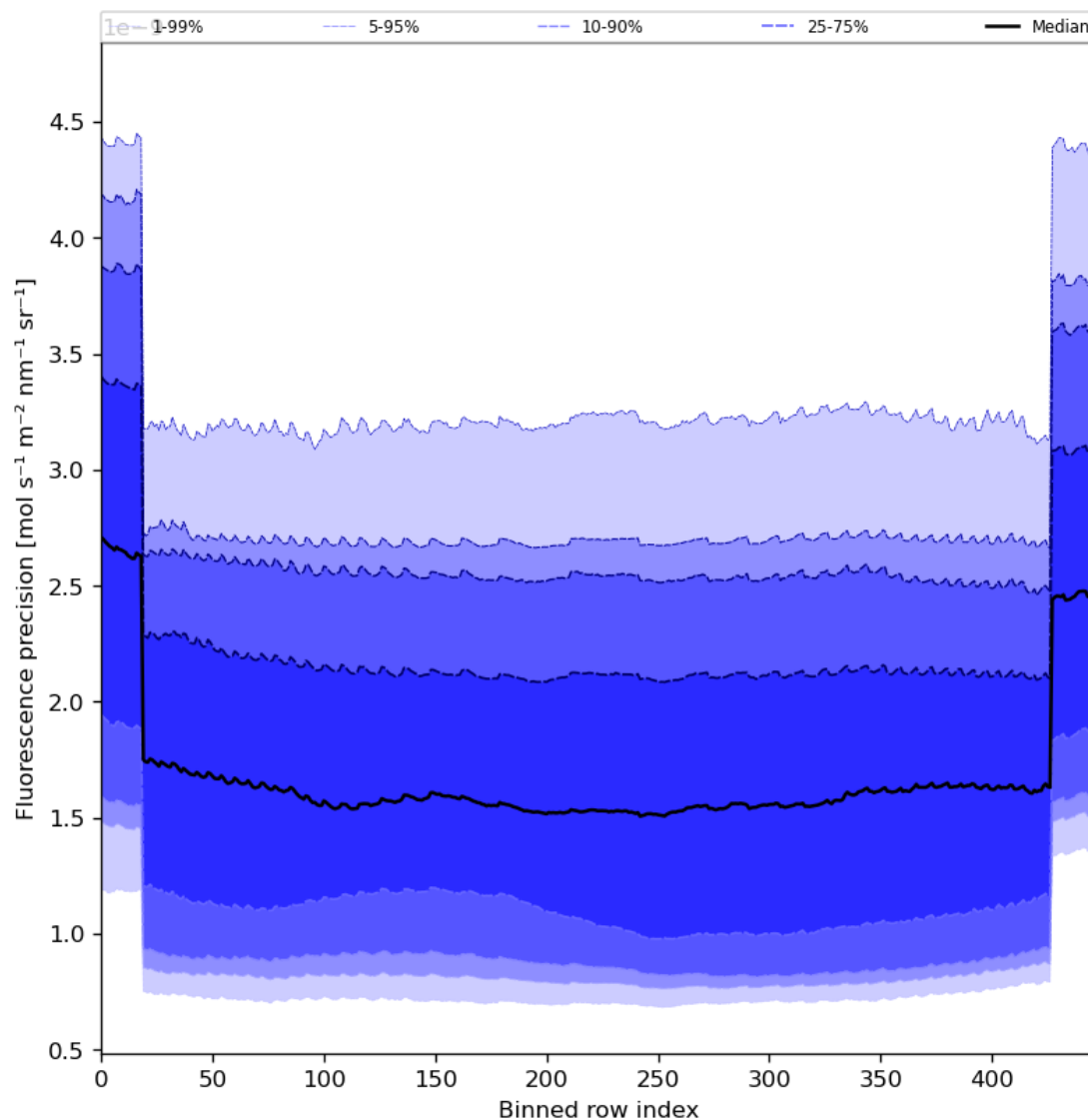
Figure 58: Along track statistics of “Fluorescence precision” for 2024-01-11 to 2024-01-13
