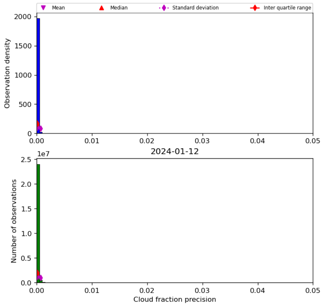
Figure 33: Histogram of “Cloud fraction precision” for 2024-01-11 to 2024-01-13
