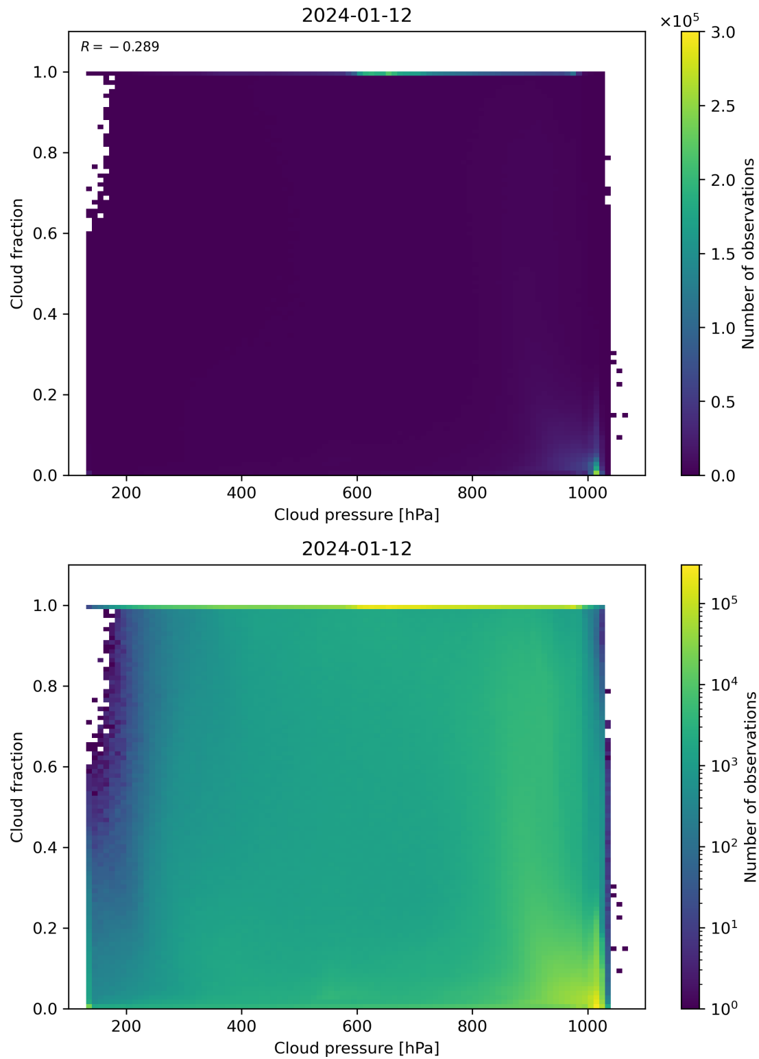
Figure 79: Scatter density plot of “Cloud pressure” against “Cloud fraction” for 2024-01-11 to 2024-01-13.
