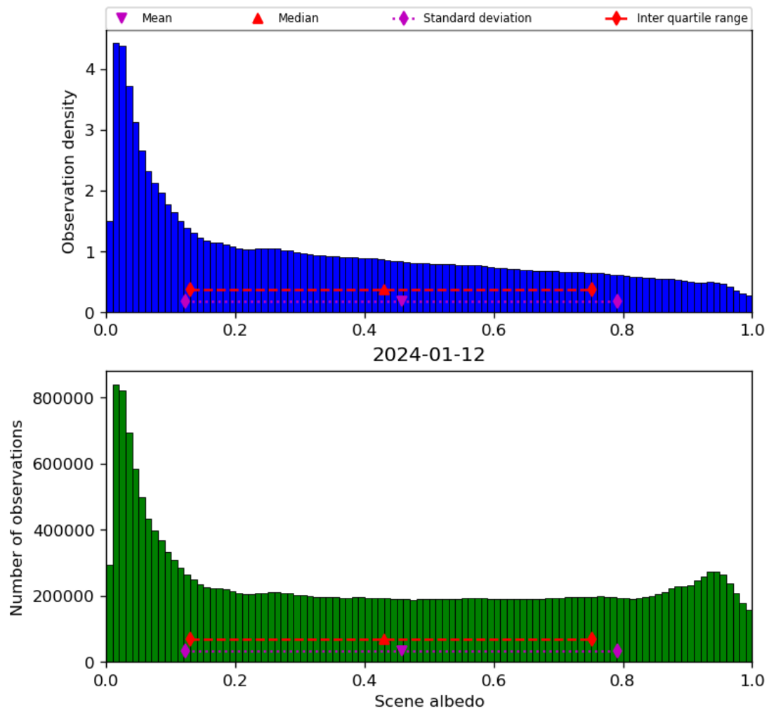
Figure 34: Histogram of “Scene albedo” for 2024-01-11 to 2024-01-13
