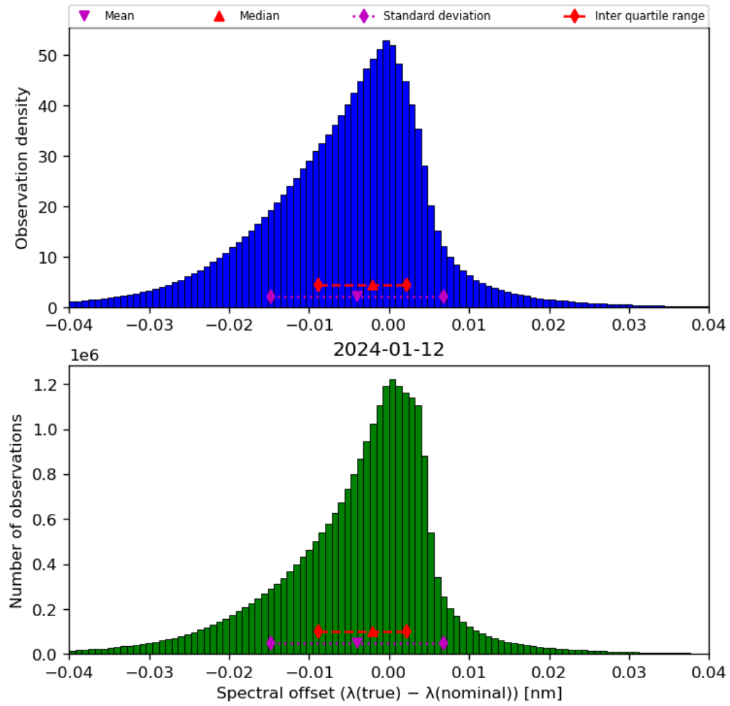
Figure 45: Histogram of “Spectral offset ( \lambda(\text{true}) - \lambda(\text{nominal}) )” for 2024-01-11 to 2024-01-13
