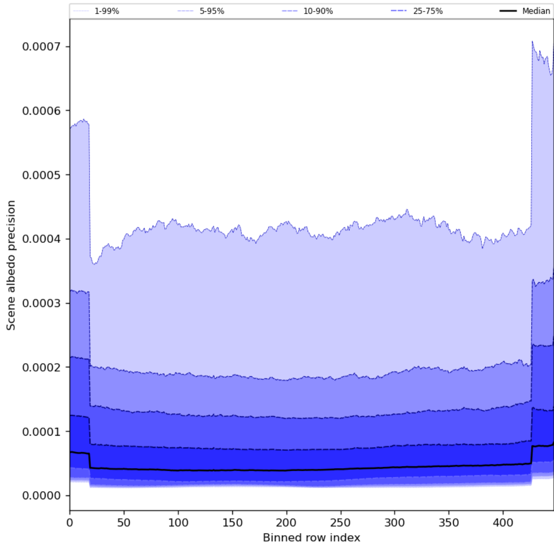
Figure 52: Along track statistics of “Scene albedo precision” for 2024-01-11 to 2024-01-13
