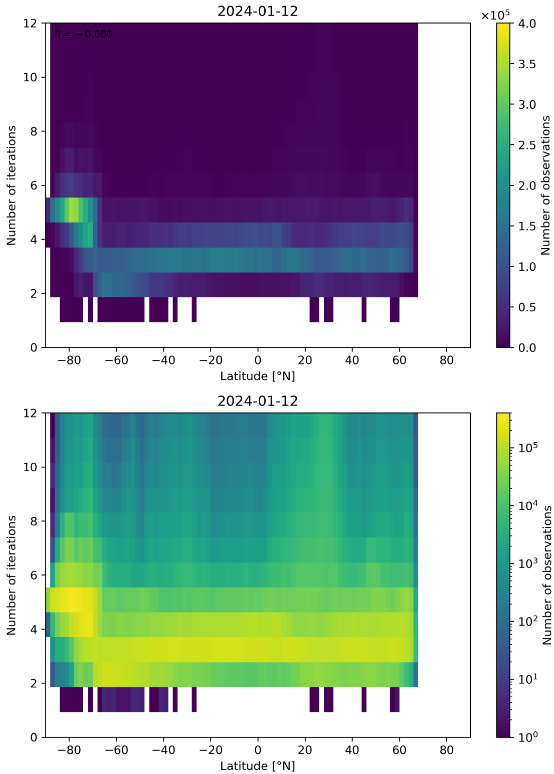
Figure 93: Scatter density plot of “Latitude” against “Number of iterations” for 2024-01-11 to 2024-01-13.
