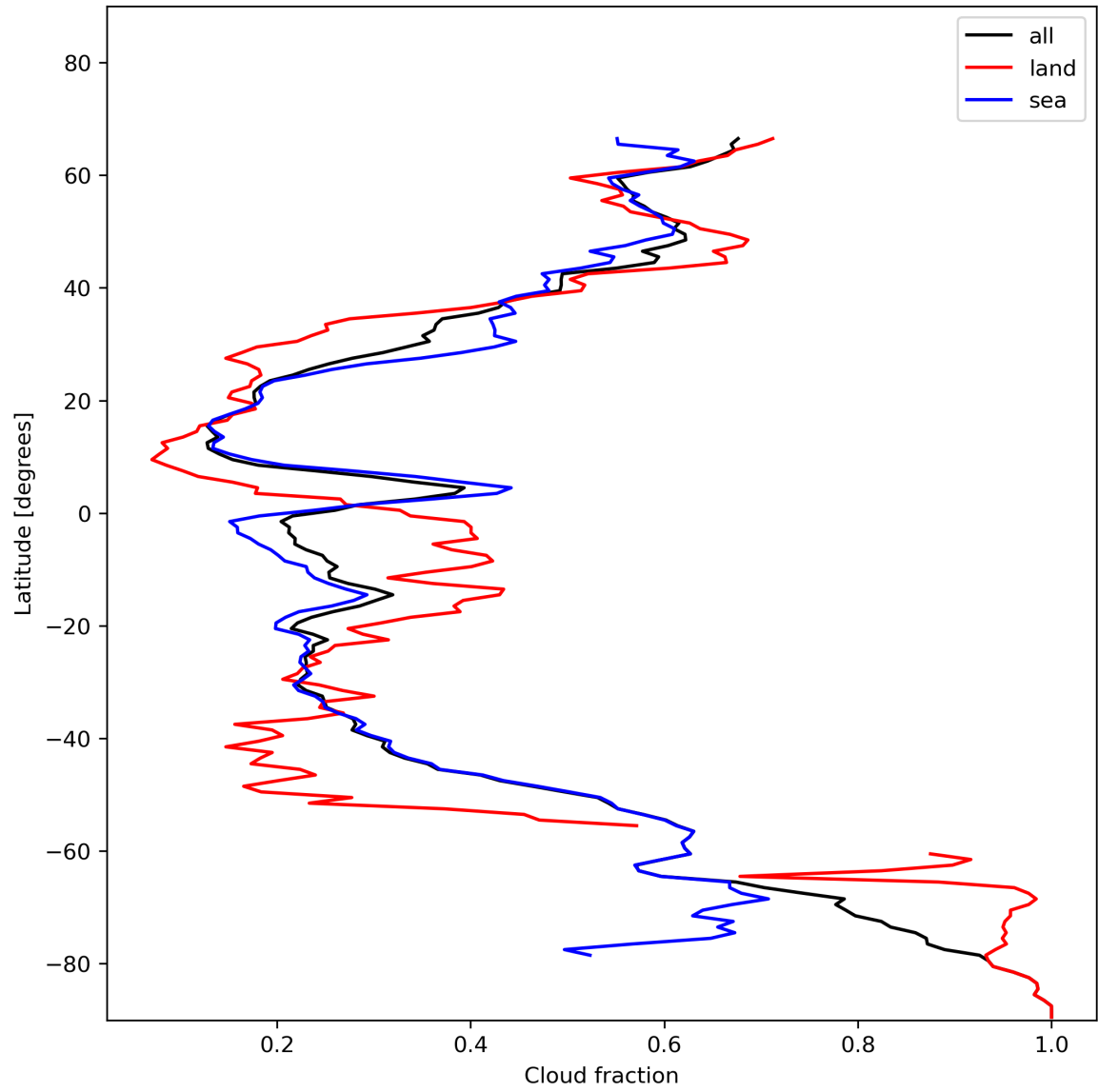
Figure 15: Zonal average of “Cloud fraction” for 2024-01-11 to 2024-01-13.
