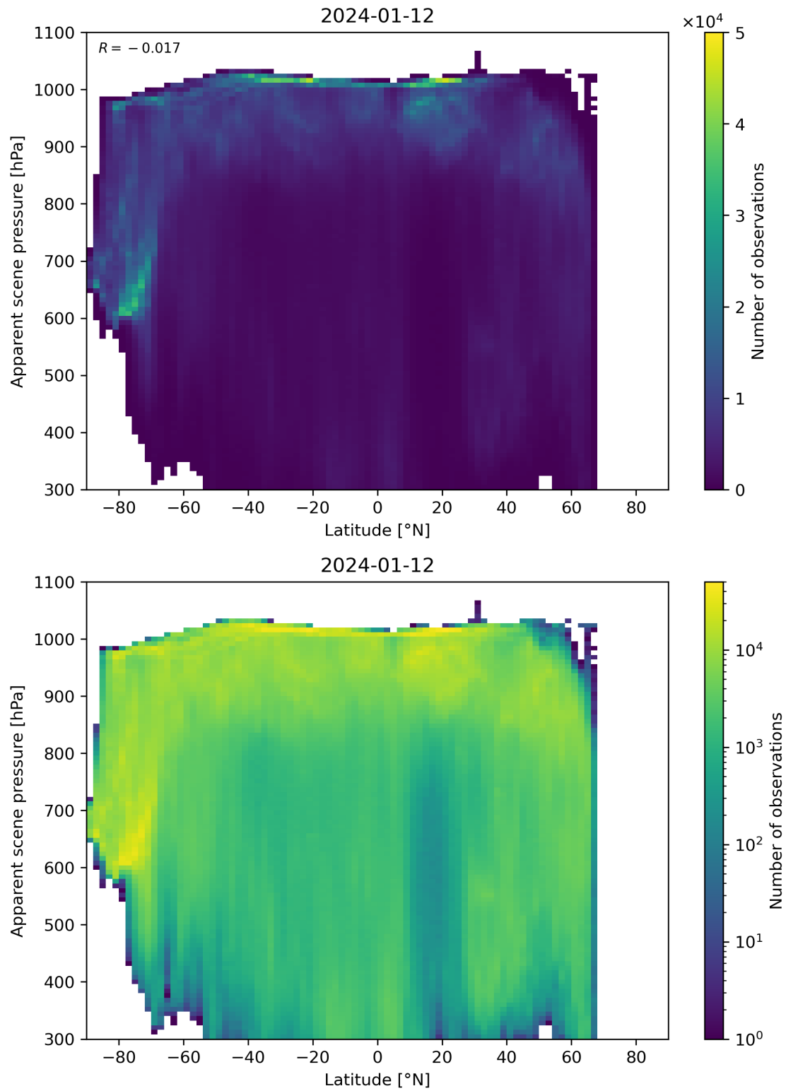
Figure 88: Scatter density plot of “Latitude” against “Apparent scene pressure” for 2024-01-11 to 2024-01-13.
