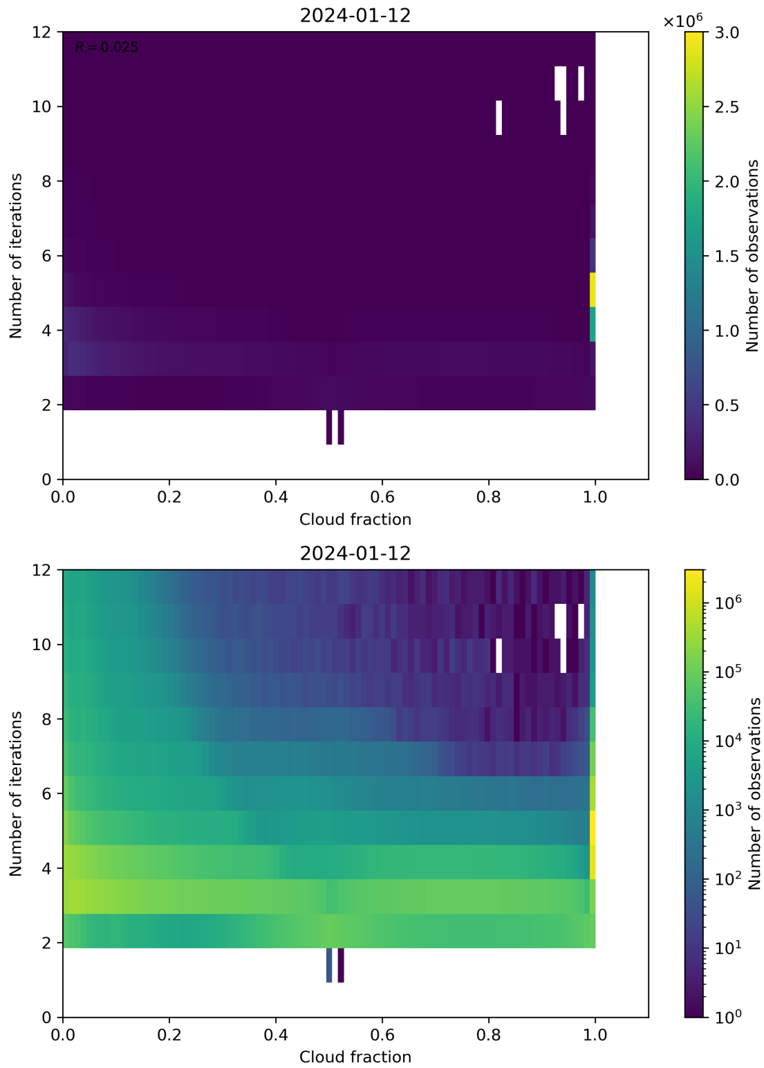
Figure 73: Scatter density plot of “Cloud fraction” against “Number of iterations” for 2024-01-11 to 2024-01-13.
