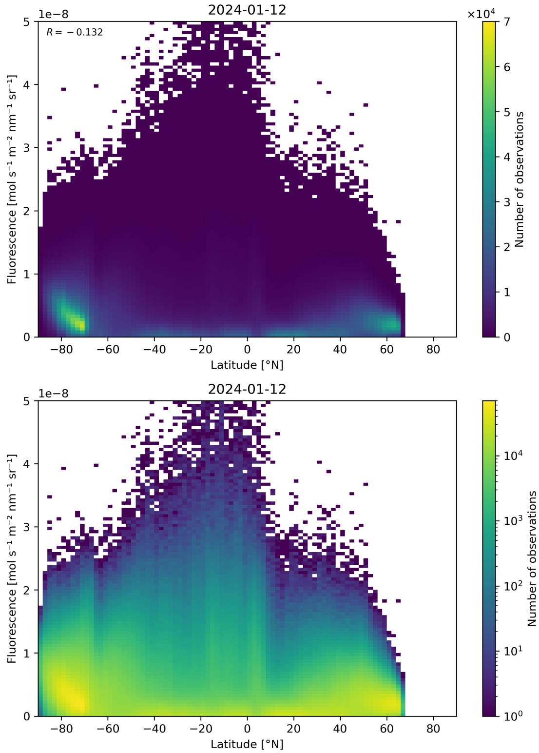
Figure 92: Scatter density plot of “Latitude” against “Fluorescence” for 2024-01-11 to 2024-01-13.
