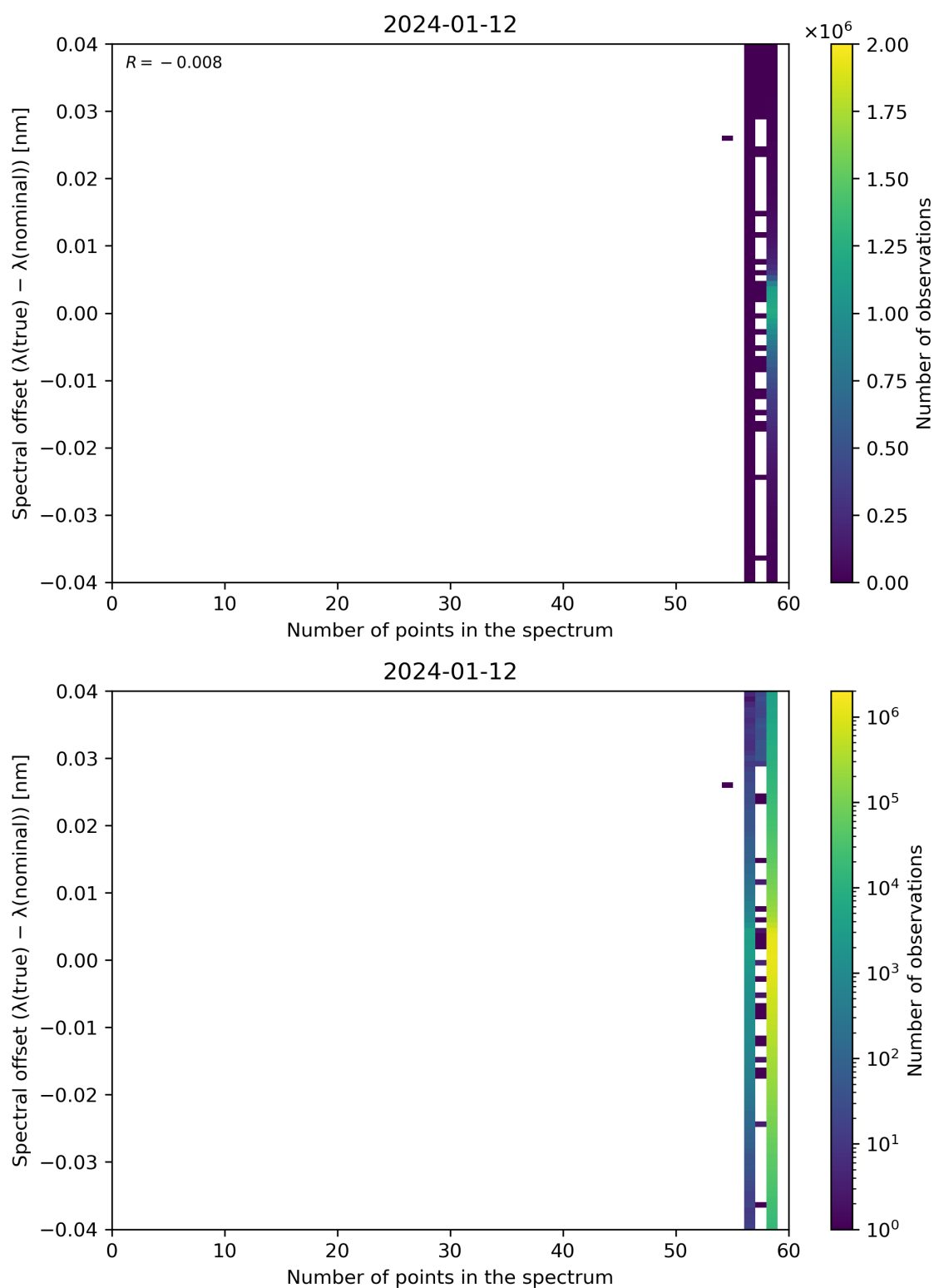
Figure 101: Scatter density plot of “Number of points in the spectrum” against “Spectral offset ( \lambda(\text{true}) - \lambda(\text{nominal}) )” for 2024-01-11 to 2024-01-13.
