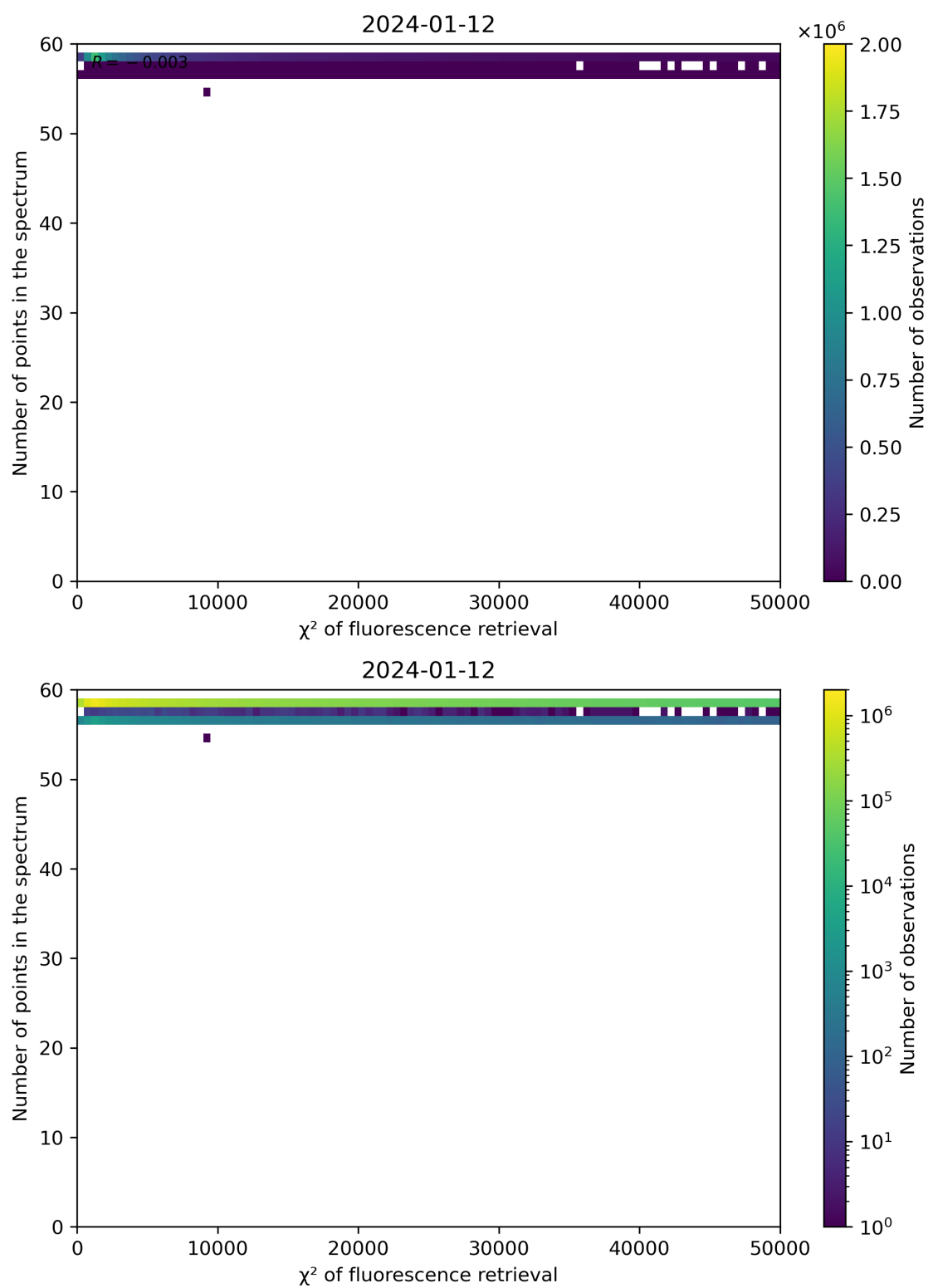
Figure 68: Scatter density plot of “ \chi^2 of fluorescence retrieval” against “Number of points in the spectrum” for 2024-01-11 to 2024-01-13.
