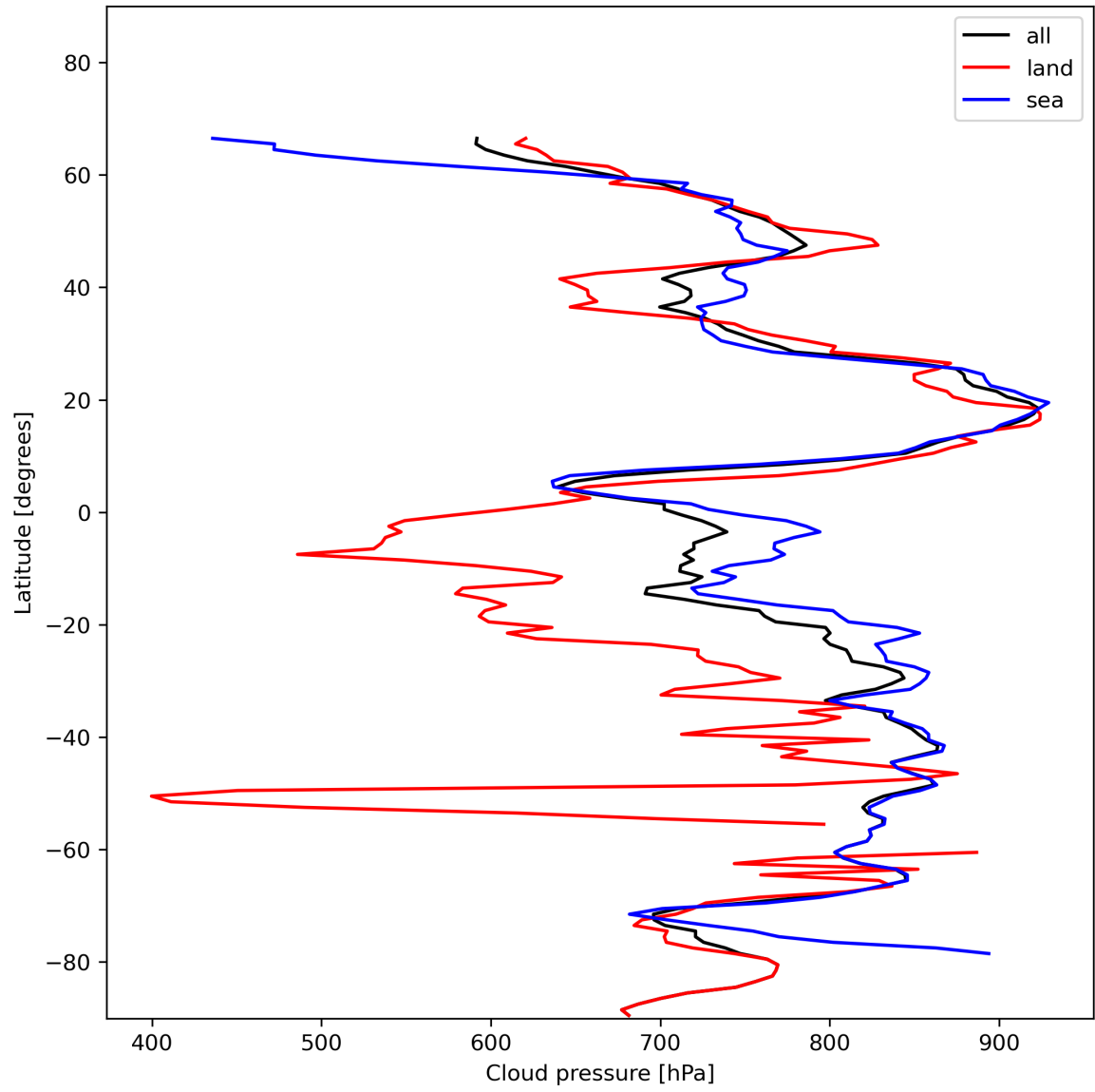
Figure 13: Zonal average of “Cloud pressure” for 2024-01-11 to 2024-01-13.
