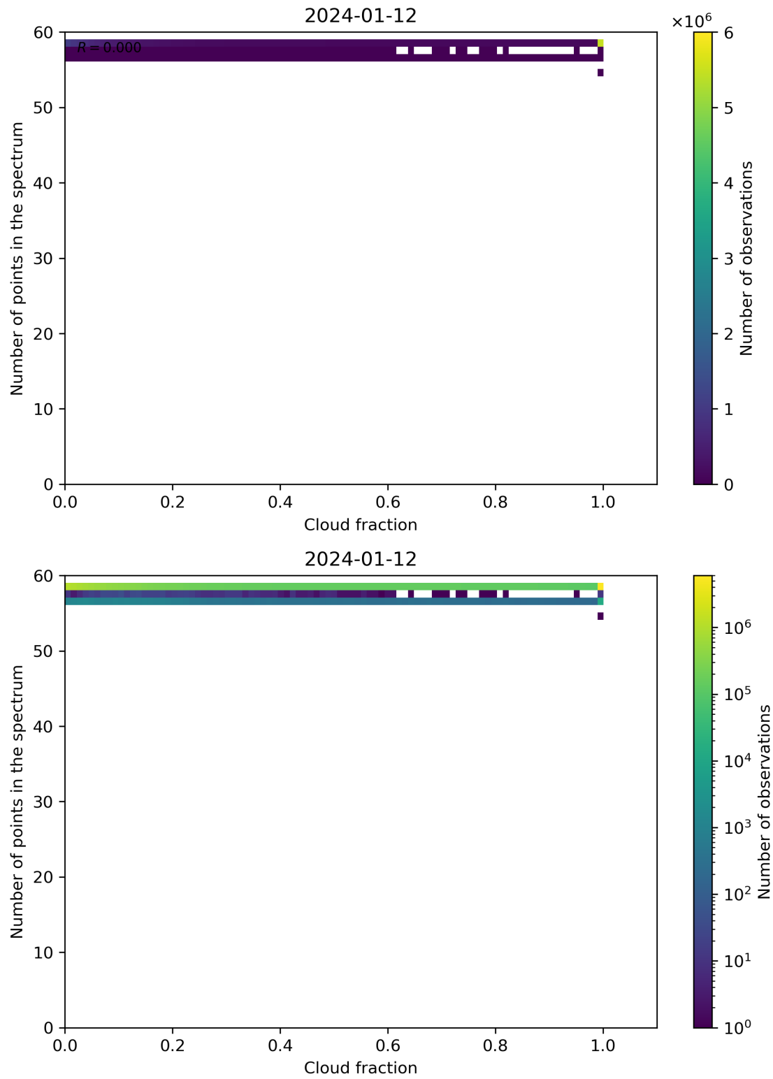
Figure 74: Scatter density plot of “Cloud fraction” against “Number of points in the spectrum” for 2024-01-11 to 2024-01-13.
