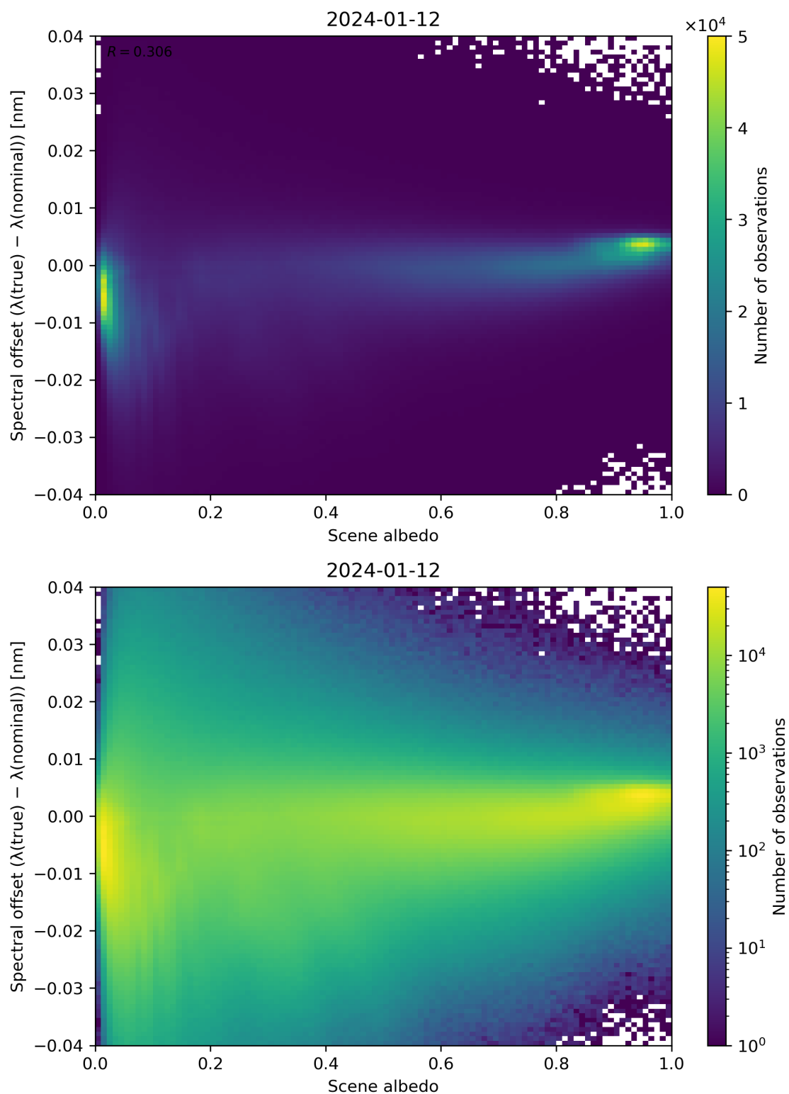
Figure 107: Scatter density plot of “Scene albedo” against “Spectral offset ( \lambda(\text{true}) - \lambda(\text{nominal}) )” for 2024-01-11 to 2024-01-13.
