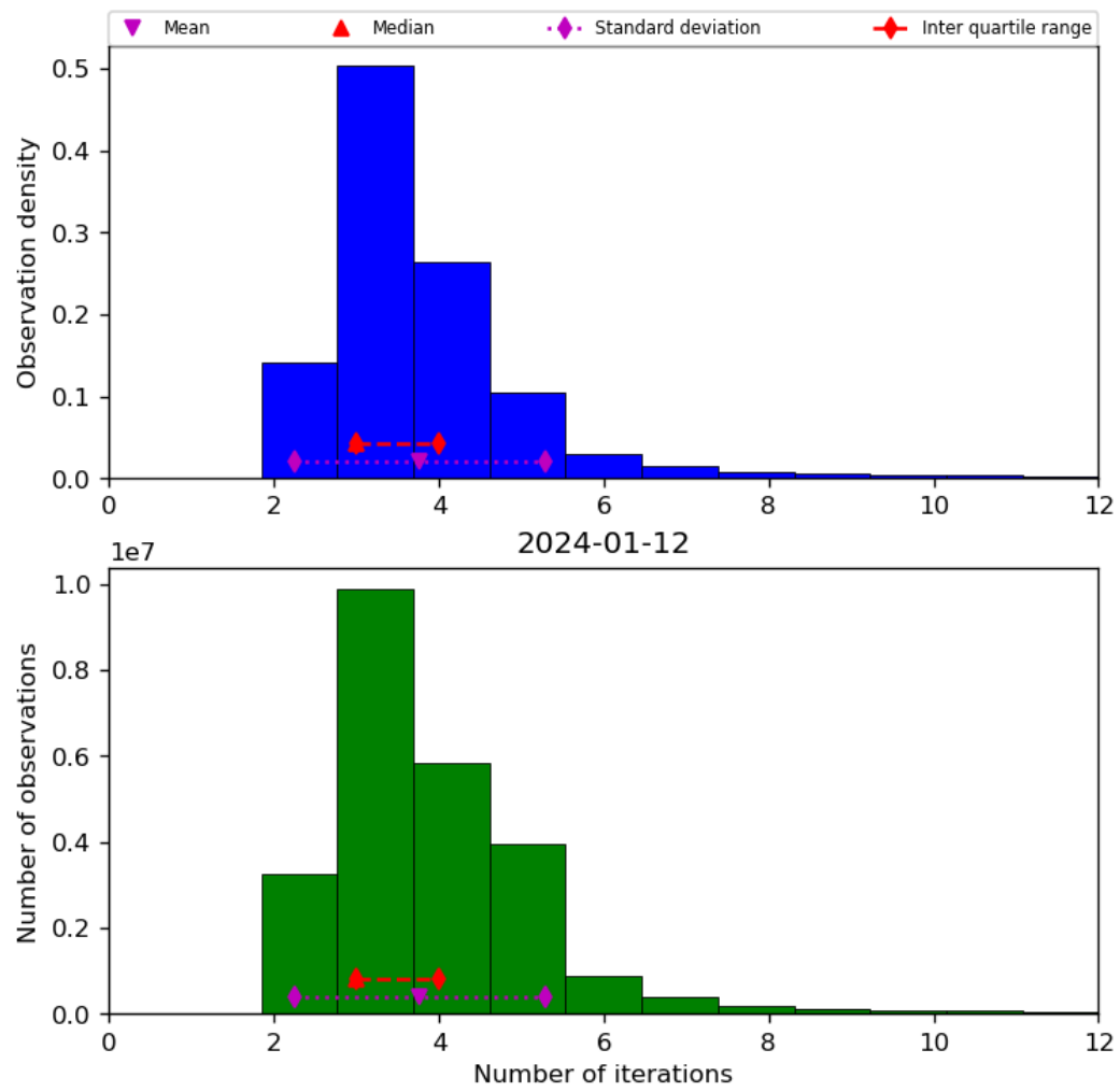
Figure 39: Histogram of “Number of iterations” for 2024-01-11 to 2024-01-13
