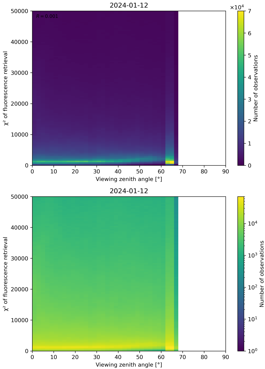
Figure 119: Scatter density plot of “Viewing zenith angle” against “ \chi^2 of fluorescence retrieval” for 2024-01-11 to 2024-01-13.
