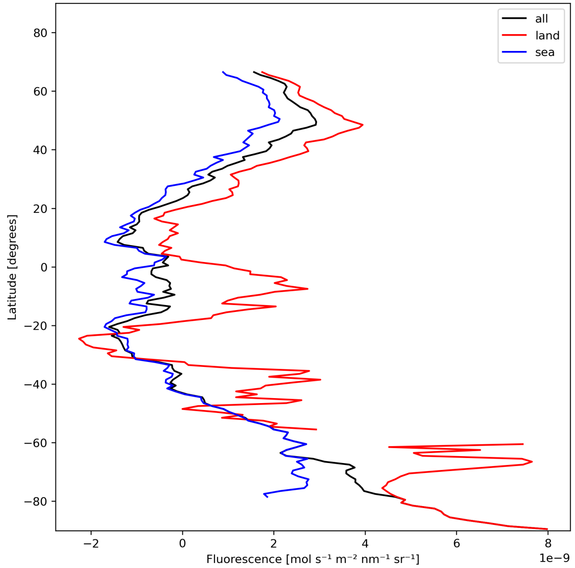
Figure 23: Zonal average of “Fluorescence” for 2024-01-11 to 2024-01-13.
