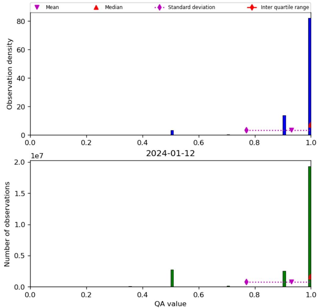
Figure 29: Histogram of “QA value” for 2024-01-11 to 2024-01-13
