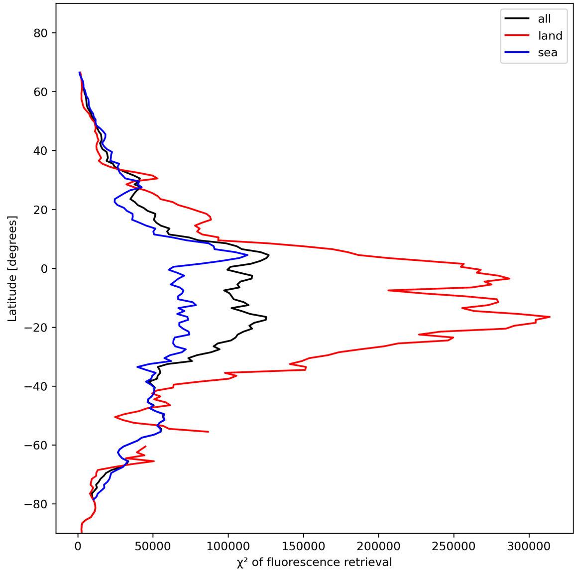
Figure 25: Zonal average of “ \chi^2 of fluorescence retrieval” for 2024-01-11 to 2024-01-13.
