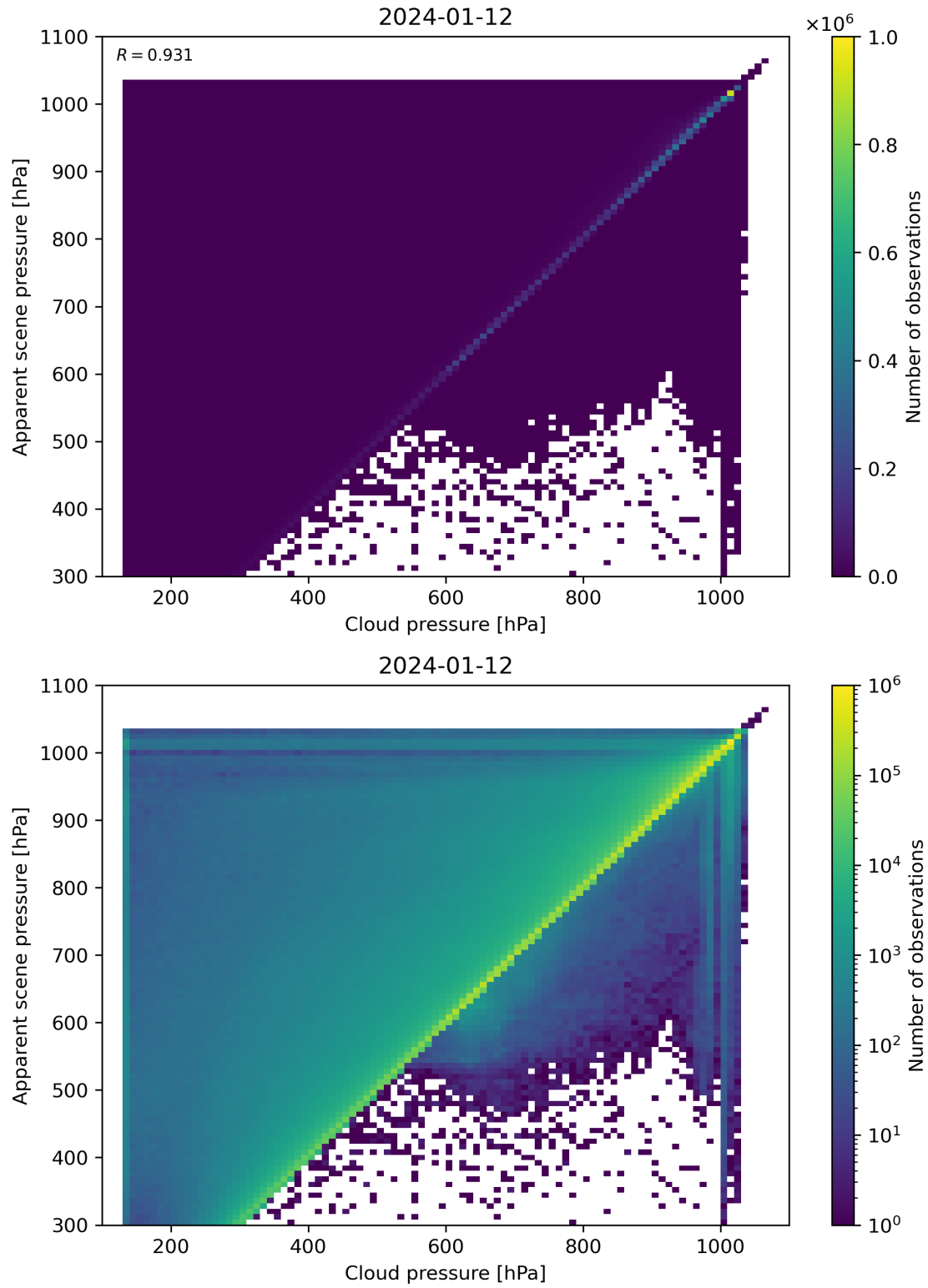
Figure 77: Scatter density plot of “Cloud pressure” against “Apparent scene pressure” for 2024-01-11 to 2024-01-13.
