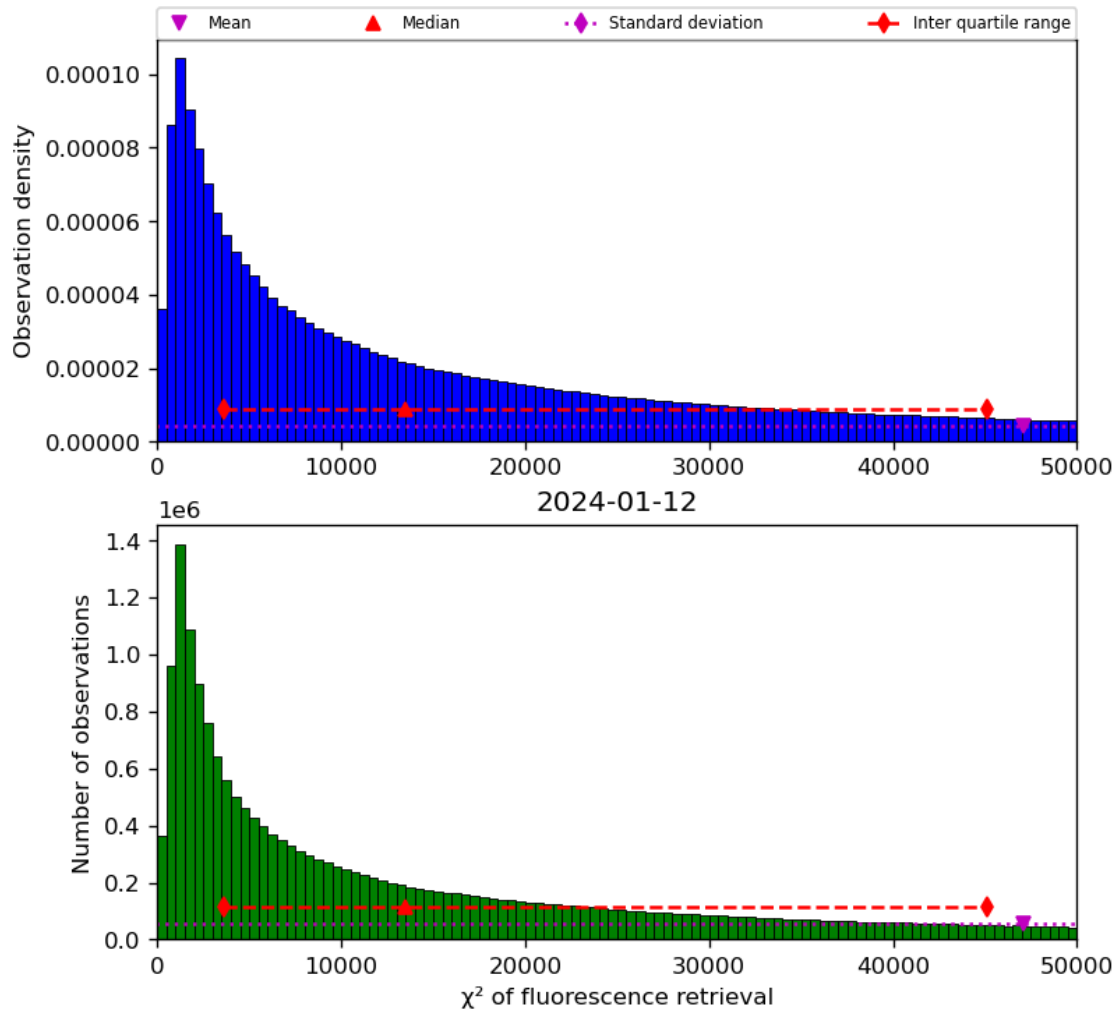
Figure 42: Histogram of “ \chi^2 of fluorescence retrieval” for 2024-01-11 to 2024-01-13
