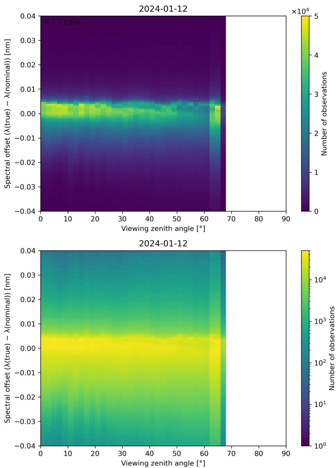
Figure 128: Scatter density plot of “Viewing zenith angle” against “Spectral offset ( \lambda(\text{true}) - \lambda(\text{nominal}) )” for 2024-01-11 to 2024-01-13.
