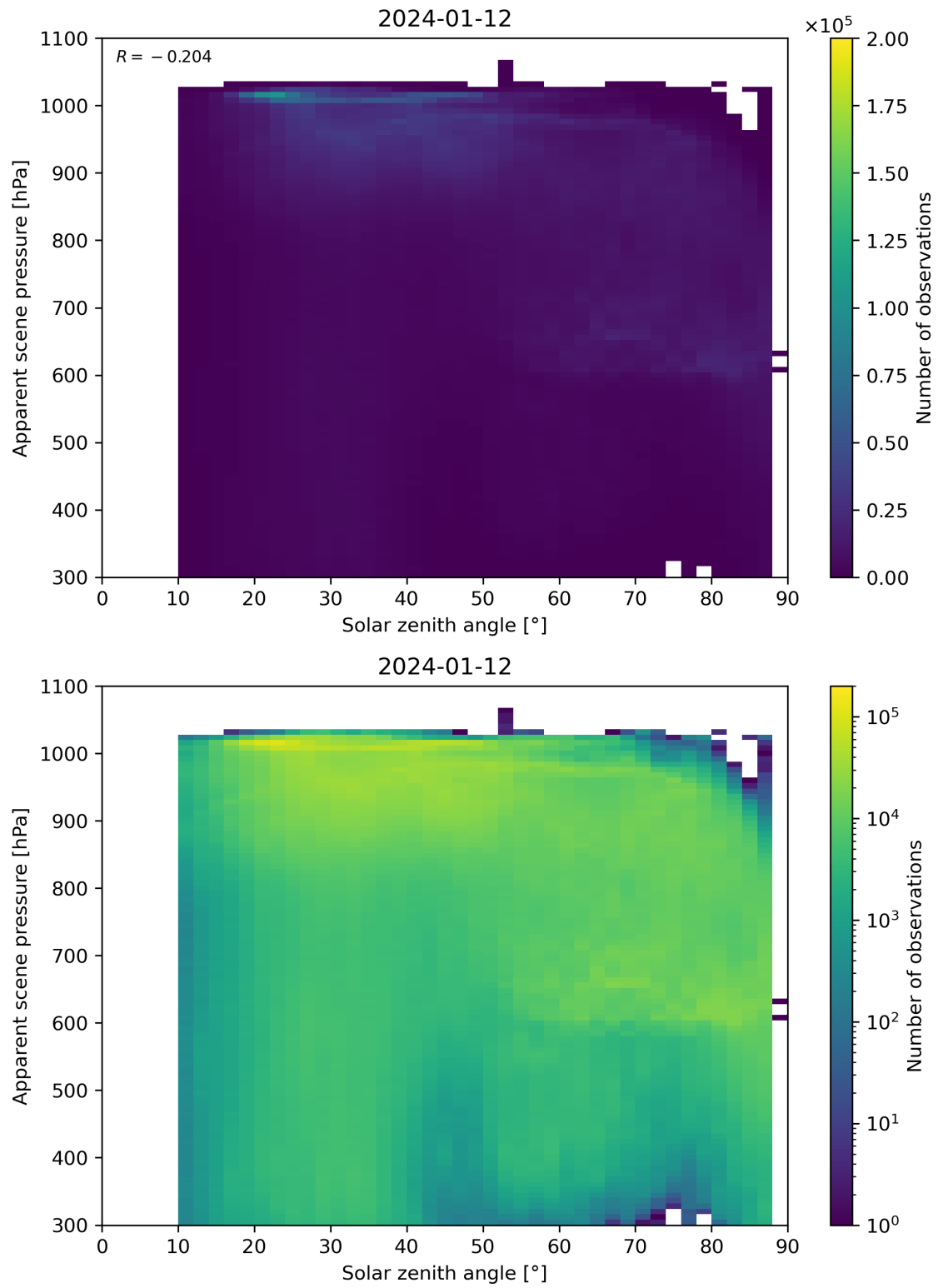
Figure 108: Scatter density plot of “Solar zenith angle” against “Apparent scene pressure” for 2024-01-11 to 2024-01-13.
