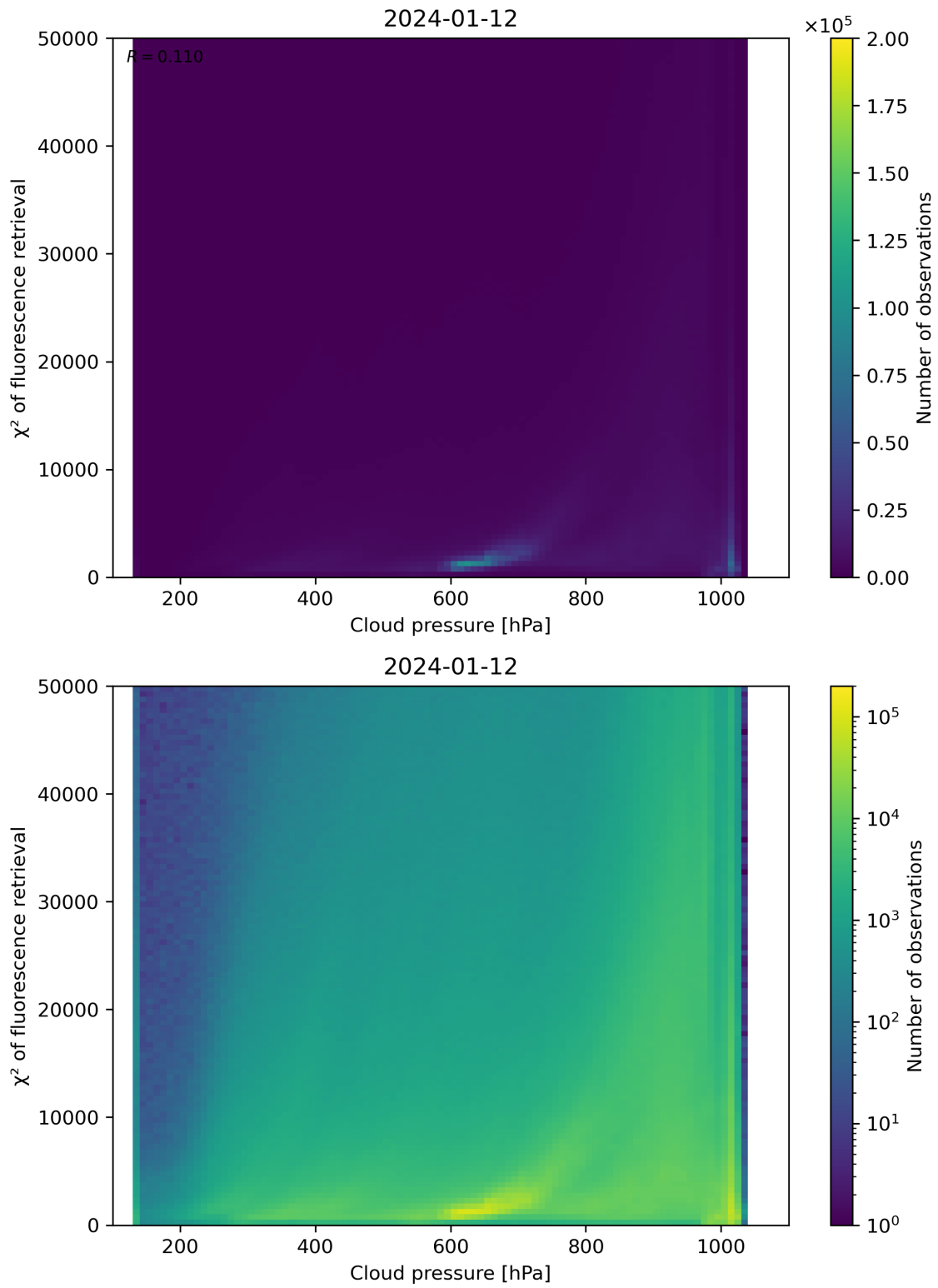
Figure 78: Scatter density plot of “Cloud pressure” against “ \chi^2 of fluorescence retrieval” for 2024-01-11 to 2024-01-13.
