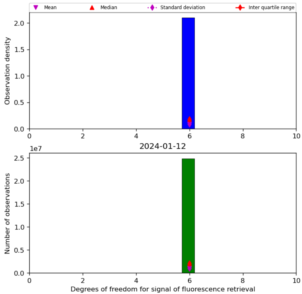
Figure 43: Histogram of “Degrees of freedom for signal of fluorescence retrieval” for 2024-01-11 to 2024-01-13
