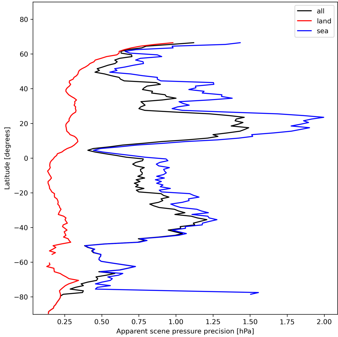
Figure 20: Zonal average of “Apparent scene pressure precision” for 2024-01-11 to 2024-01-13.
