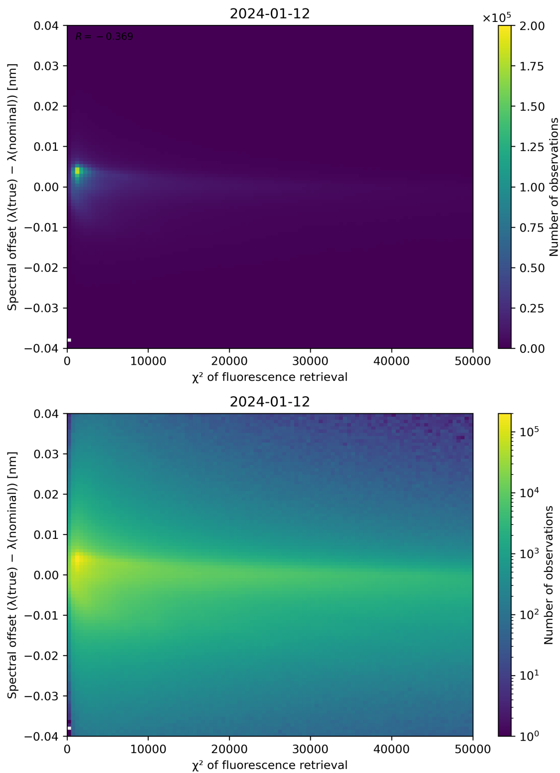
Figure 69: Scatter density plot of “ \chi^2 of fluorescence retrieval” against “Spectral offset ( \lambda(\text{true}) - \lambda(\text{nominal}) )” for 2024-01-11 to 2024-01-13.
