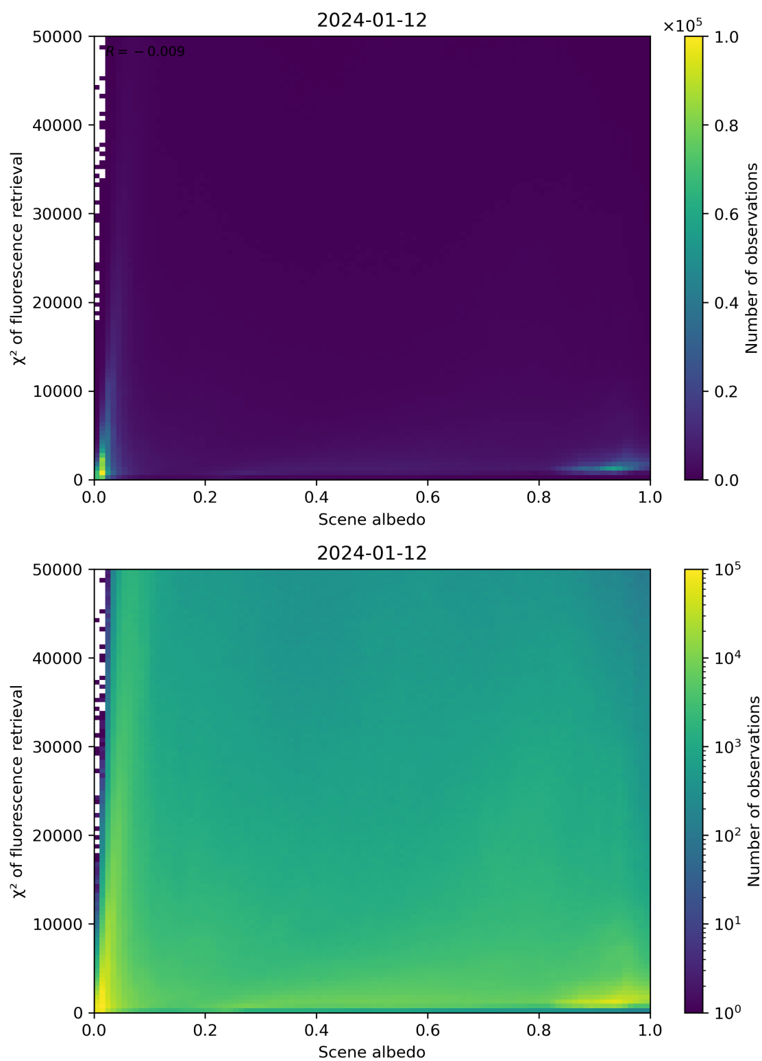
Figure 103: Scatter density plot of “Scene albedo” against “ \chi^2 of fluorescence retrieval” for 2024-01-11 to 2024-01-13.
