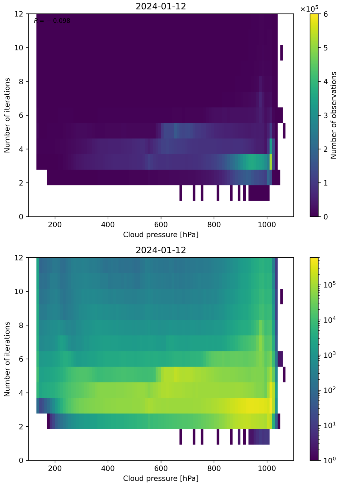
Figure 81: Scatter density plot of “Cloud pressure” against “Number of iterations” for 2024-01-11 to 2024-01-13.
