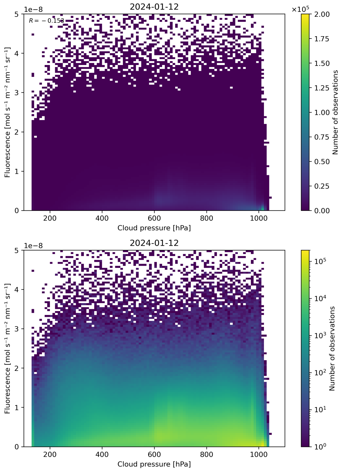
Figure 80: Scatter density plot of “Cloud pressure” against “Fluorescence” for 2024-01-11 to 2024-01-13.
