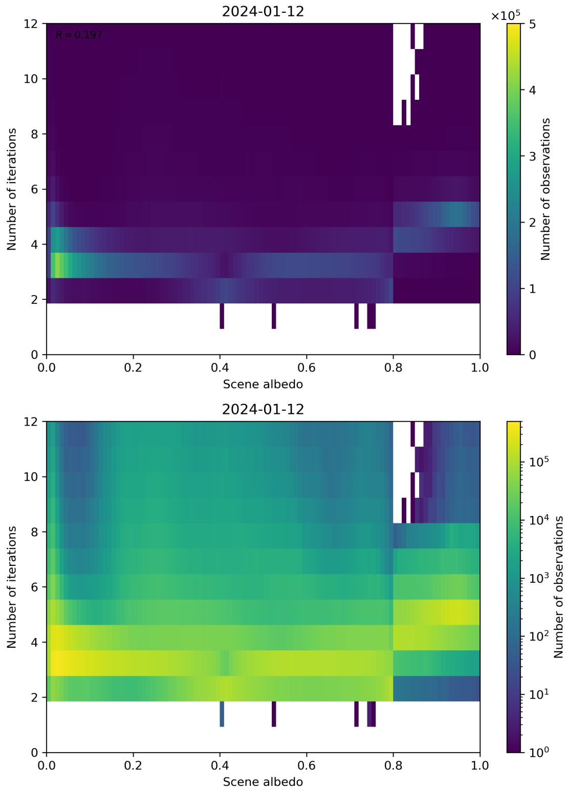
Figure 105: Scatter density plot of “Scene albedo” against “Number of iterations” for 2024-01-11 to 2024-01-13.
