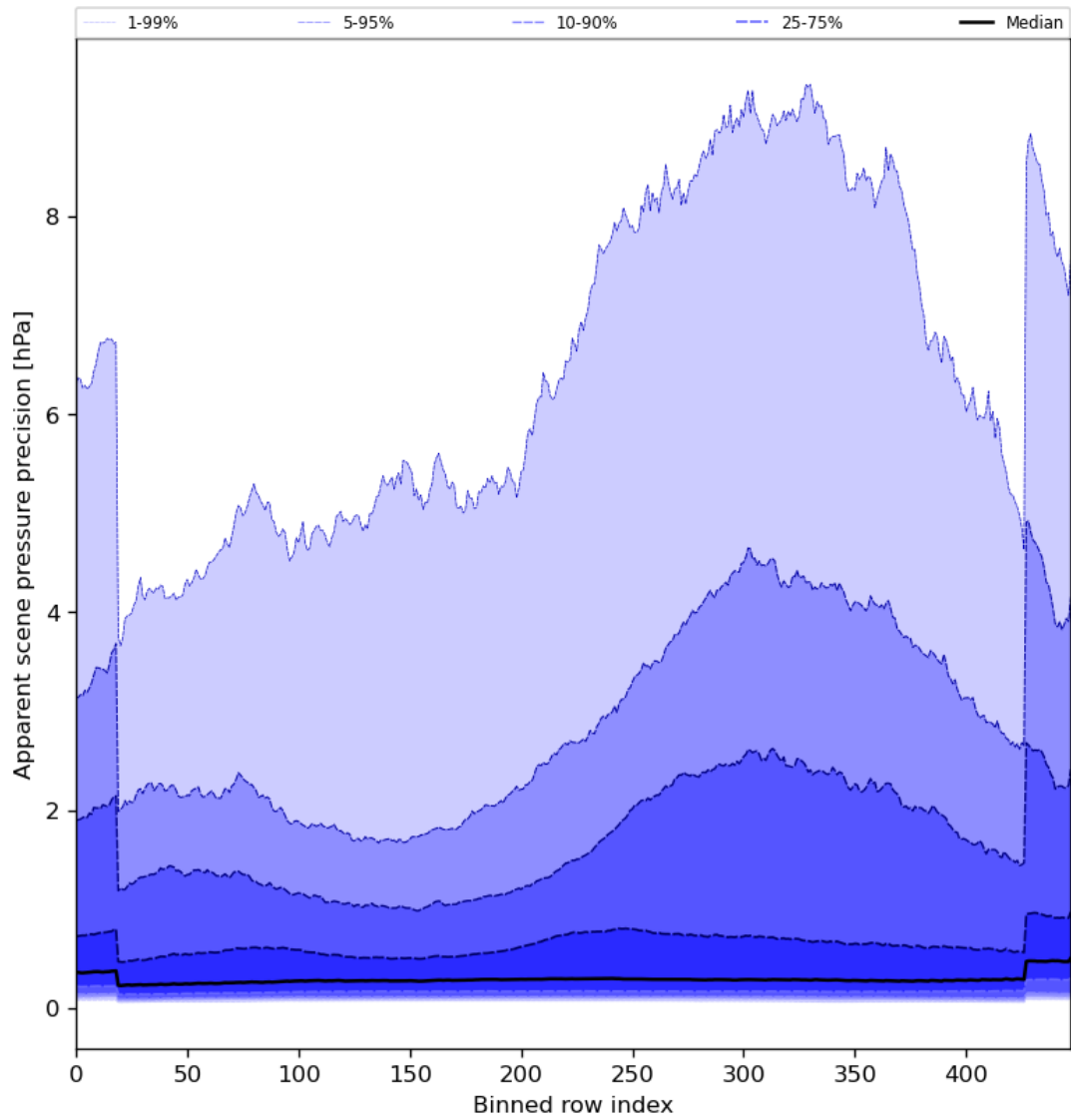
Figure 54: Along track statistics of “Apparent scene pressure precision” for 2024-01-11 to 2024-01-13
