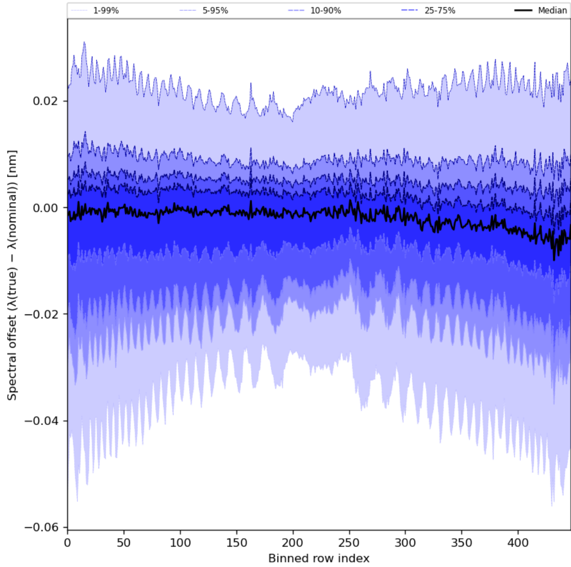
Figure 62: Along track statistics of “Spectral offset ( \lambda(\text{true}) - \lambda(\text{nominal}) )” for 2024-01-11 to 2024-01-13
