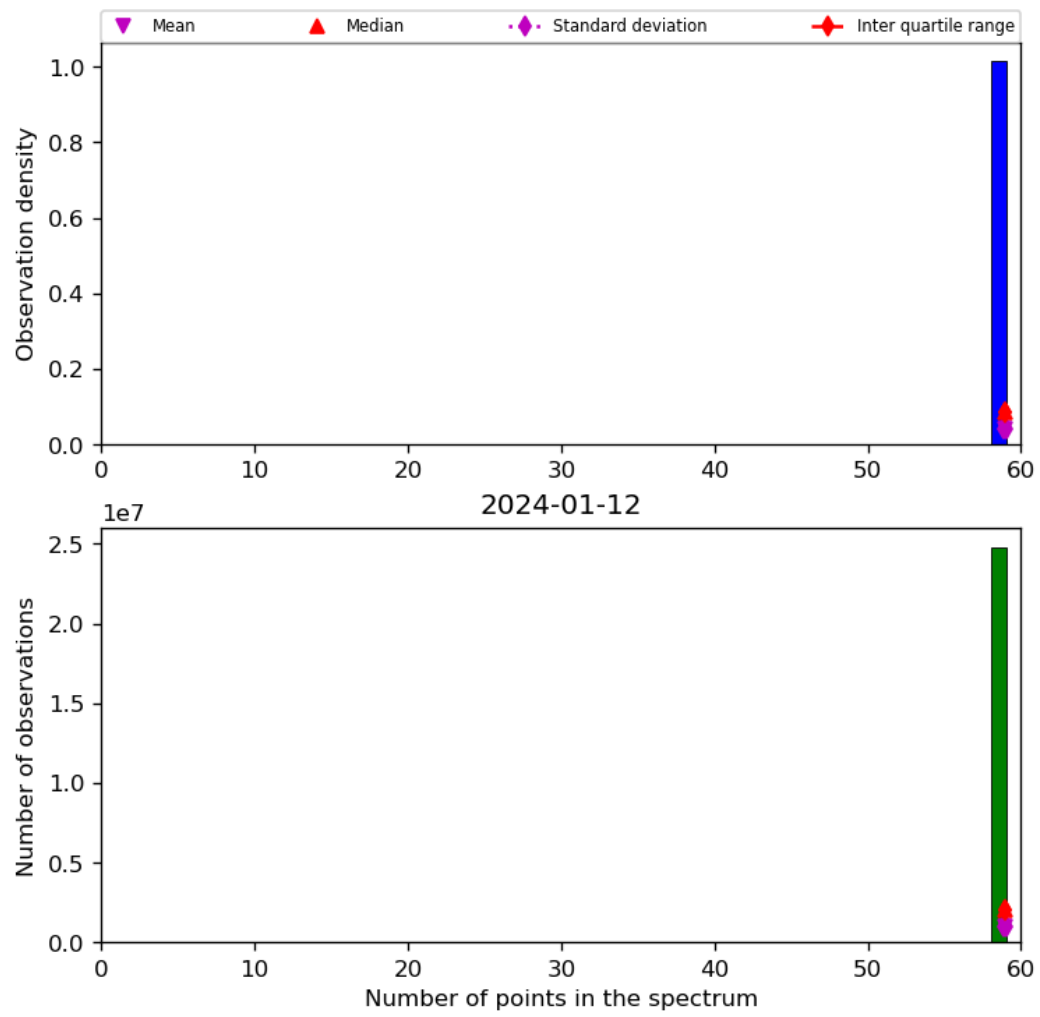
Figure 44: Histogram of “Number of points in the spectrum” for 2024-01-11 to 2024-01-13
