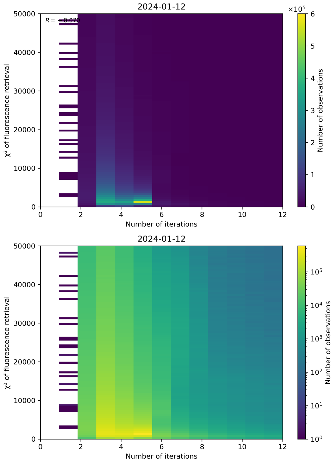
Figure 97: Scatter density plot of “Number of iterations” against “ \chi^2 of fluorescence retrieval” for 2024-01-11 to 2024-01-13.
