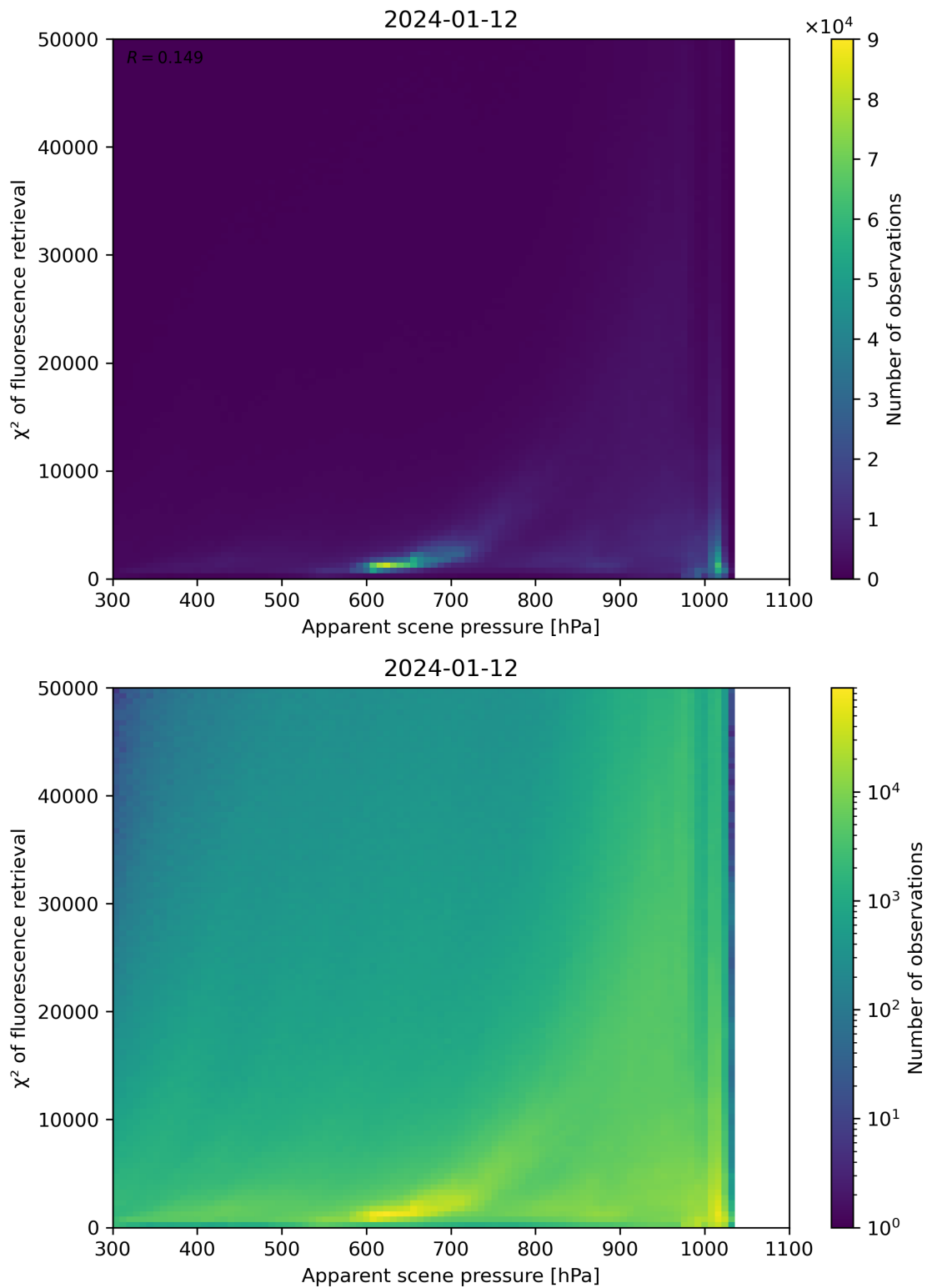
Figure 63: Scatter density plot of “Apparent scene pressure” against “ \chi^2 of fluorescence retrieval” for 2024-01-11 to 2024-01-13.
