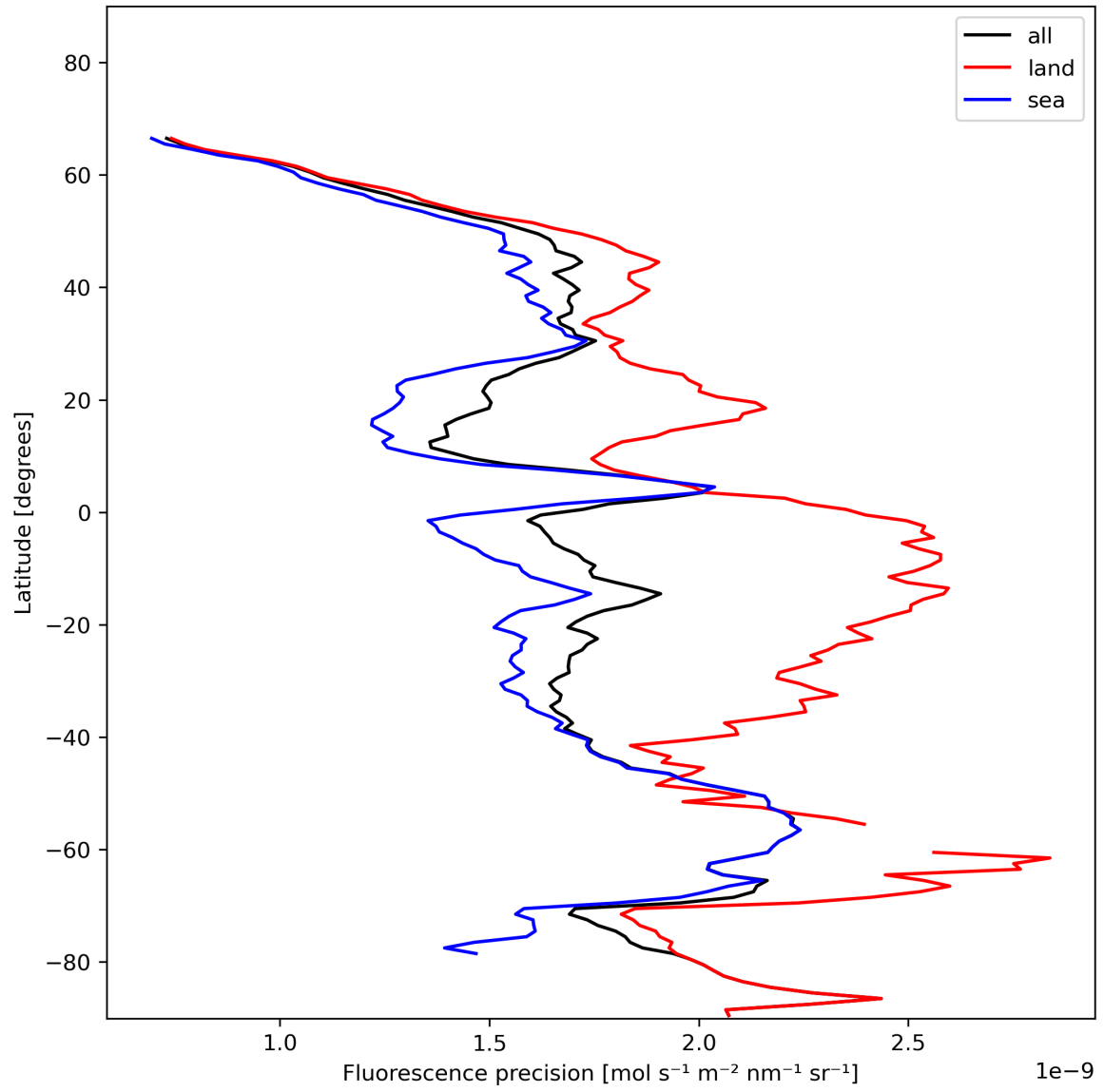
Figure 24: Zonal average of “Fluorescence precision” for 2024-01-11 to 2024-01-13.
