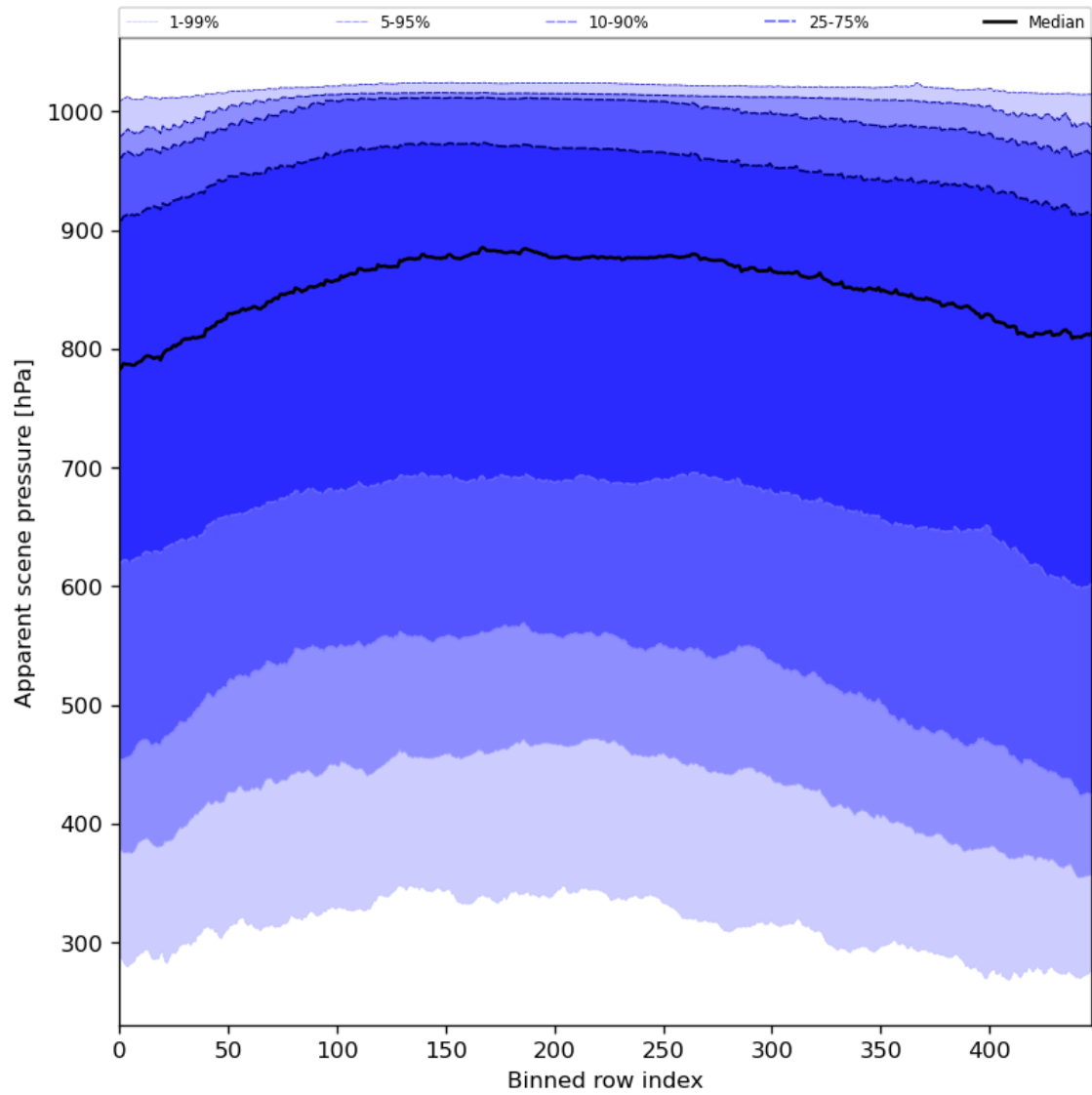
Figure 53: Along track statistics of “Apparent scene pressure” for 2024-01-11 to 2024-01-13
