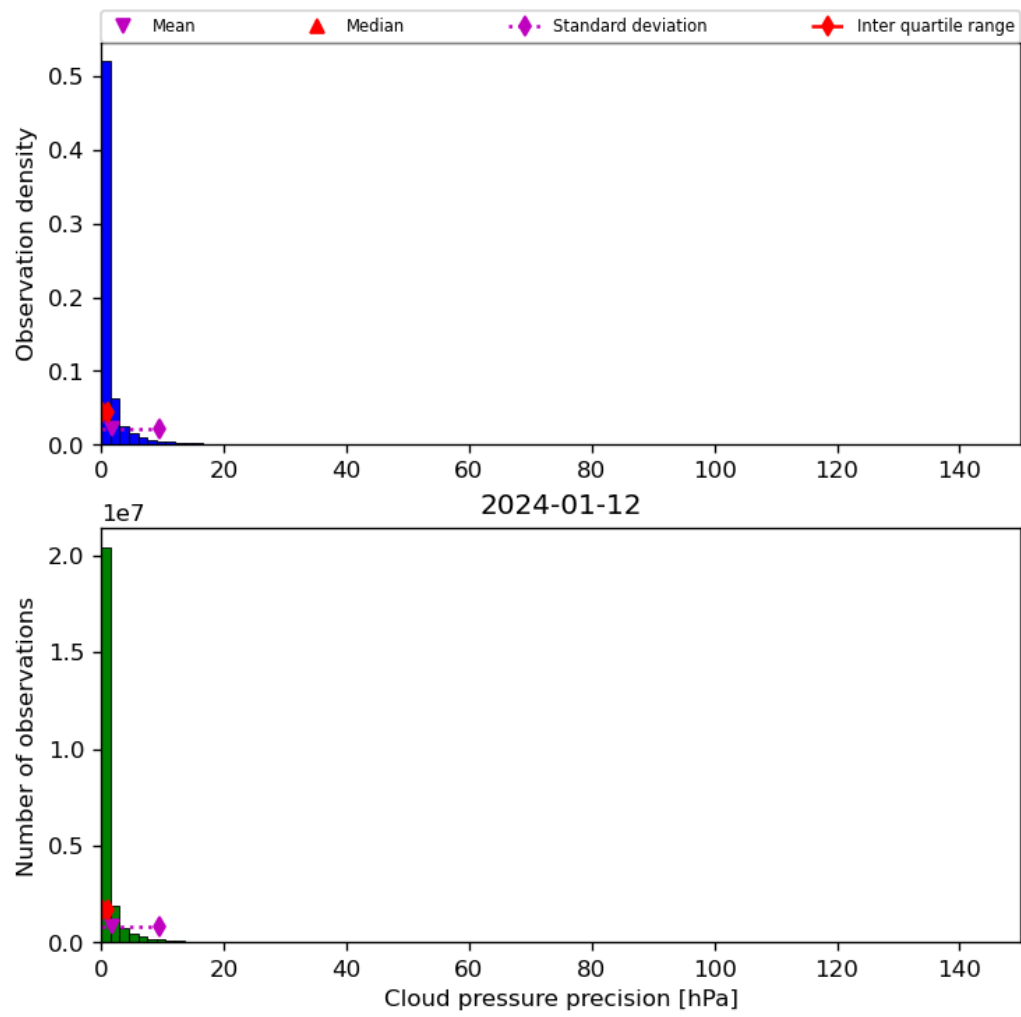
Figure 31: Histogram of “Cloud pressure precision” for 2024-01-11 to 2024-01-13
