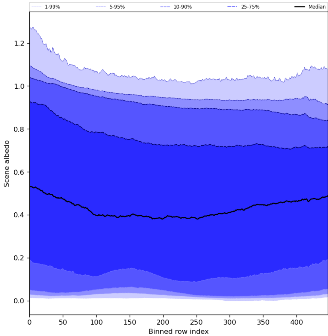
Figure 51: Along track statistics of “Scene albedo” for 2024-01-11 to 2024-01-13
