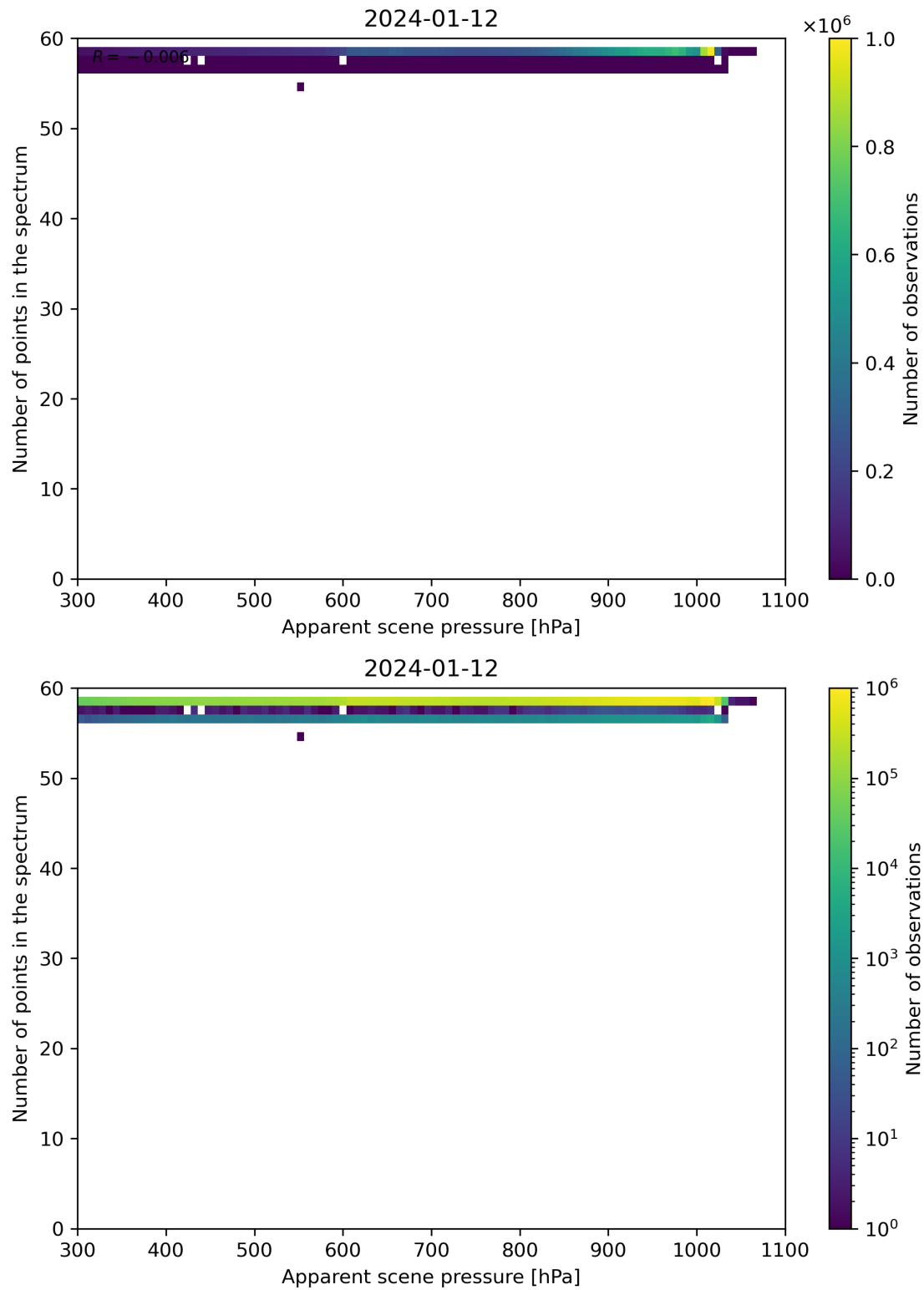
Figure 66: Scatter density plot of “Apparent scene pressure” against “Number of points in the spectrum” for 2024-01-11 to 2024-01-13.
