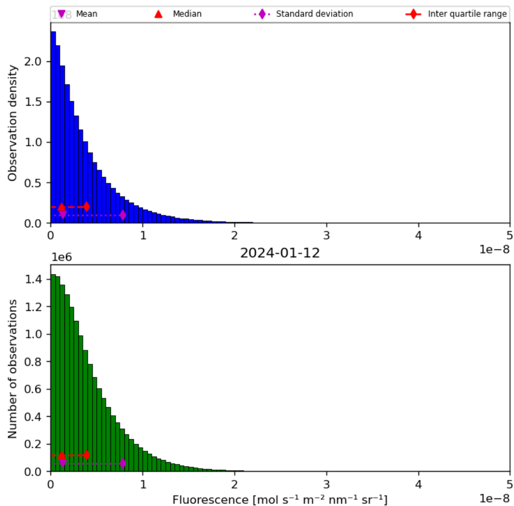
Figure 40: Histogram of “Fluorescence” for 2024-01-11 to 2024-01-13
