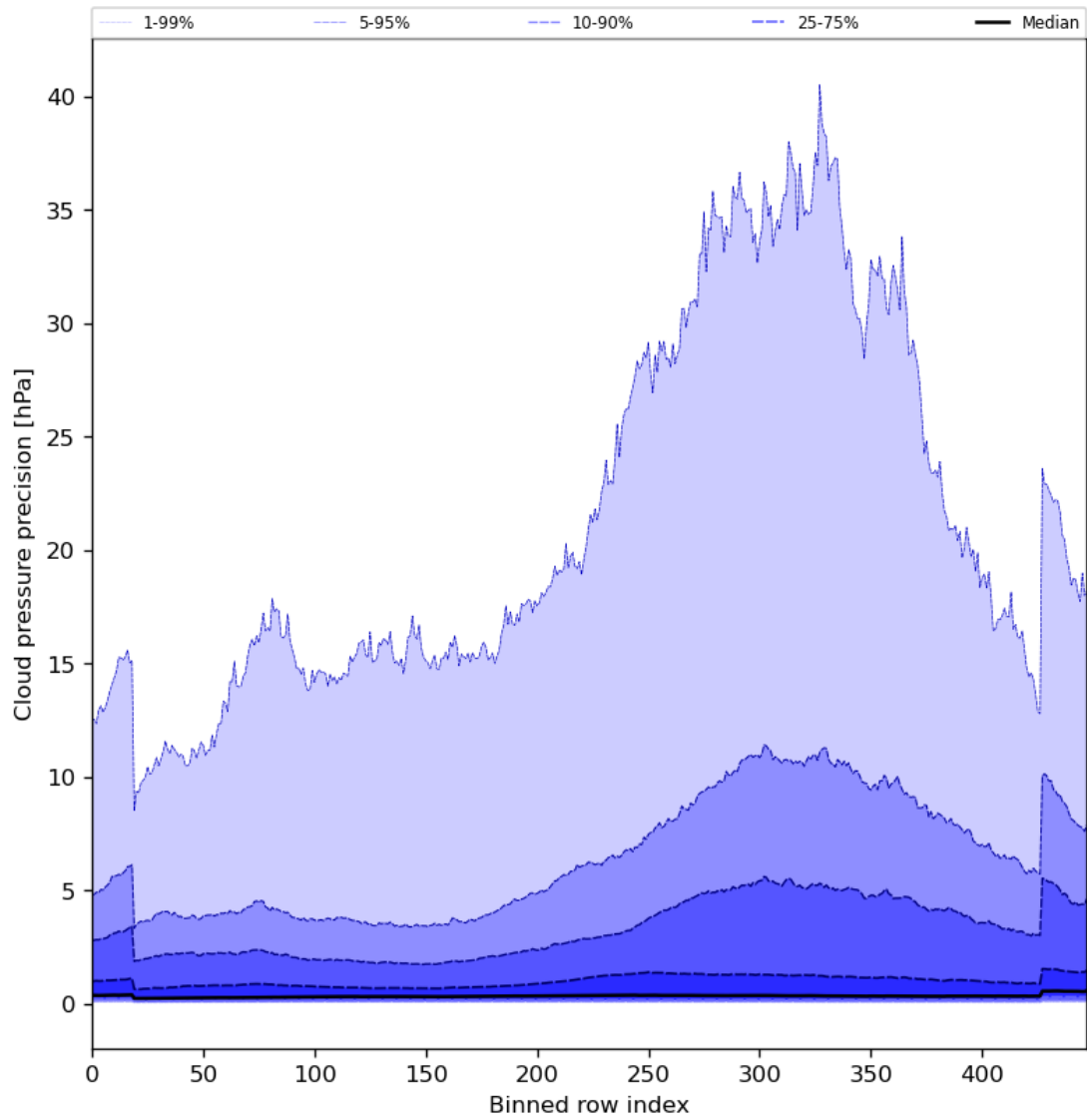
Figure 48: Along track statistics of “Cloud pressure precision” for 2024-01-11 to 2024-01-13
