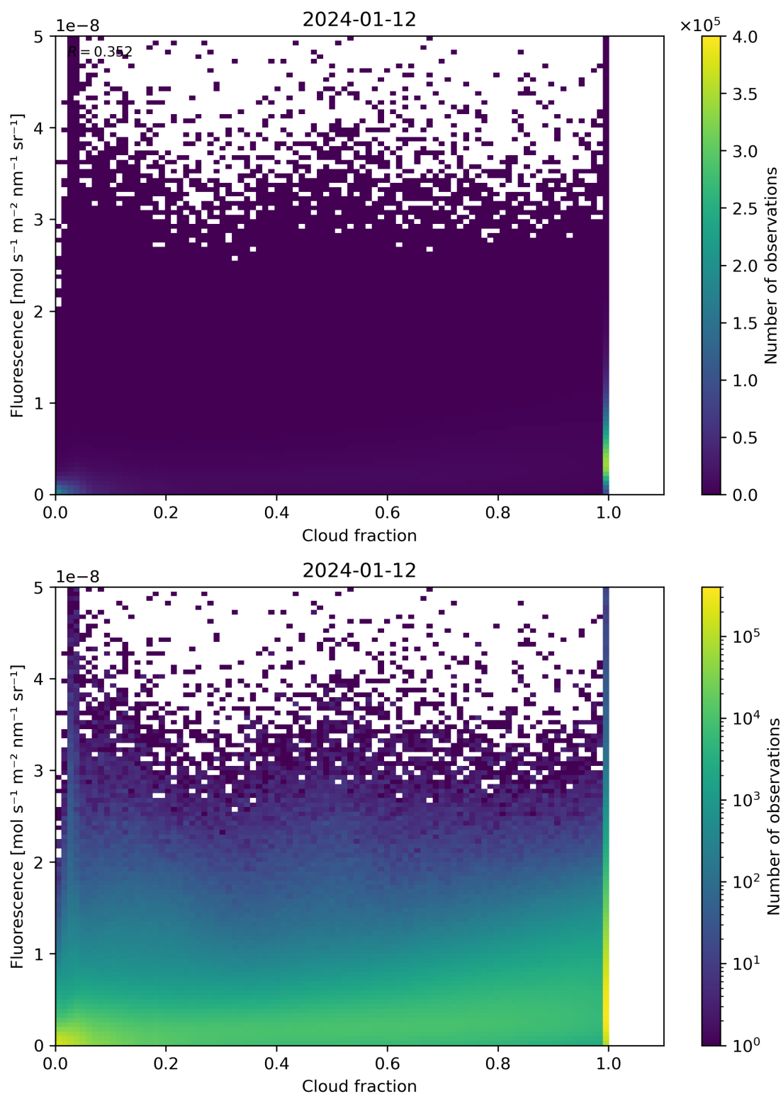
Figure 72: Scatter density plot of “Cloud fraction” against “Fluorescence” for 2024-01-11 to 2024-01-13.
