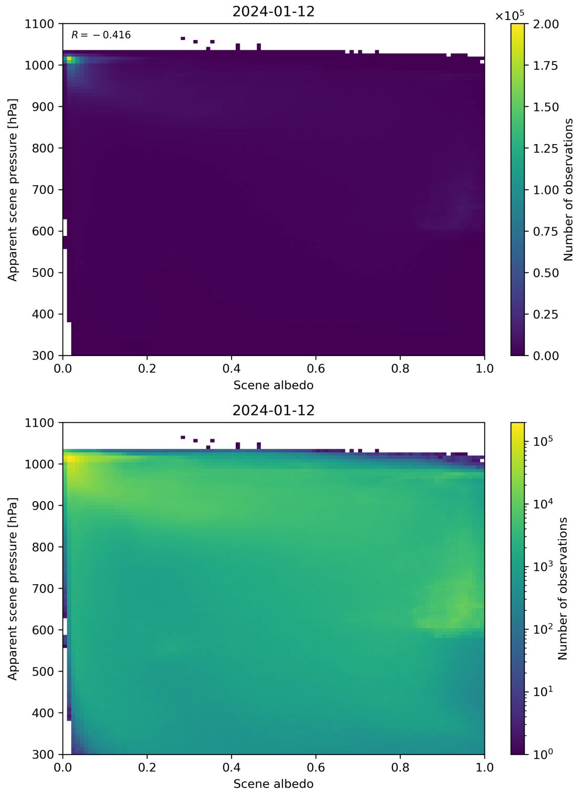
Figure 102: Scatter density plot of “Scene albedo” against “Apparent scene pressure” for 2024-01-11 to 2024-01-13.
