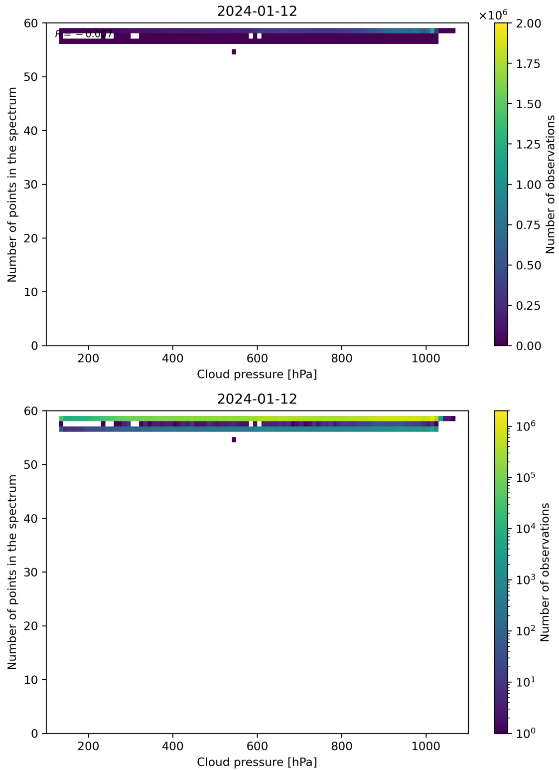
Figure 82: Scatter density plot of “Cloud pressure” against “Number of points in the spectrum” for 2024-01-11 to 2024-01-13.
