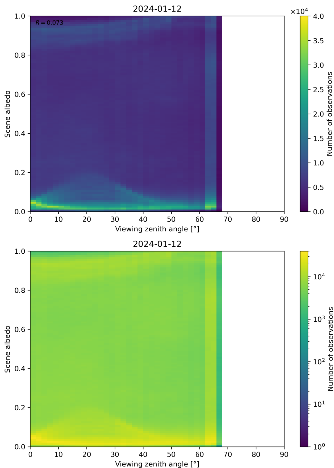
Figure 126: Scatter density plot of “Viewing zenith angle” against “Scene albedo” for 2024-01-11 to 2024-01-13.
