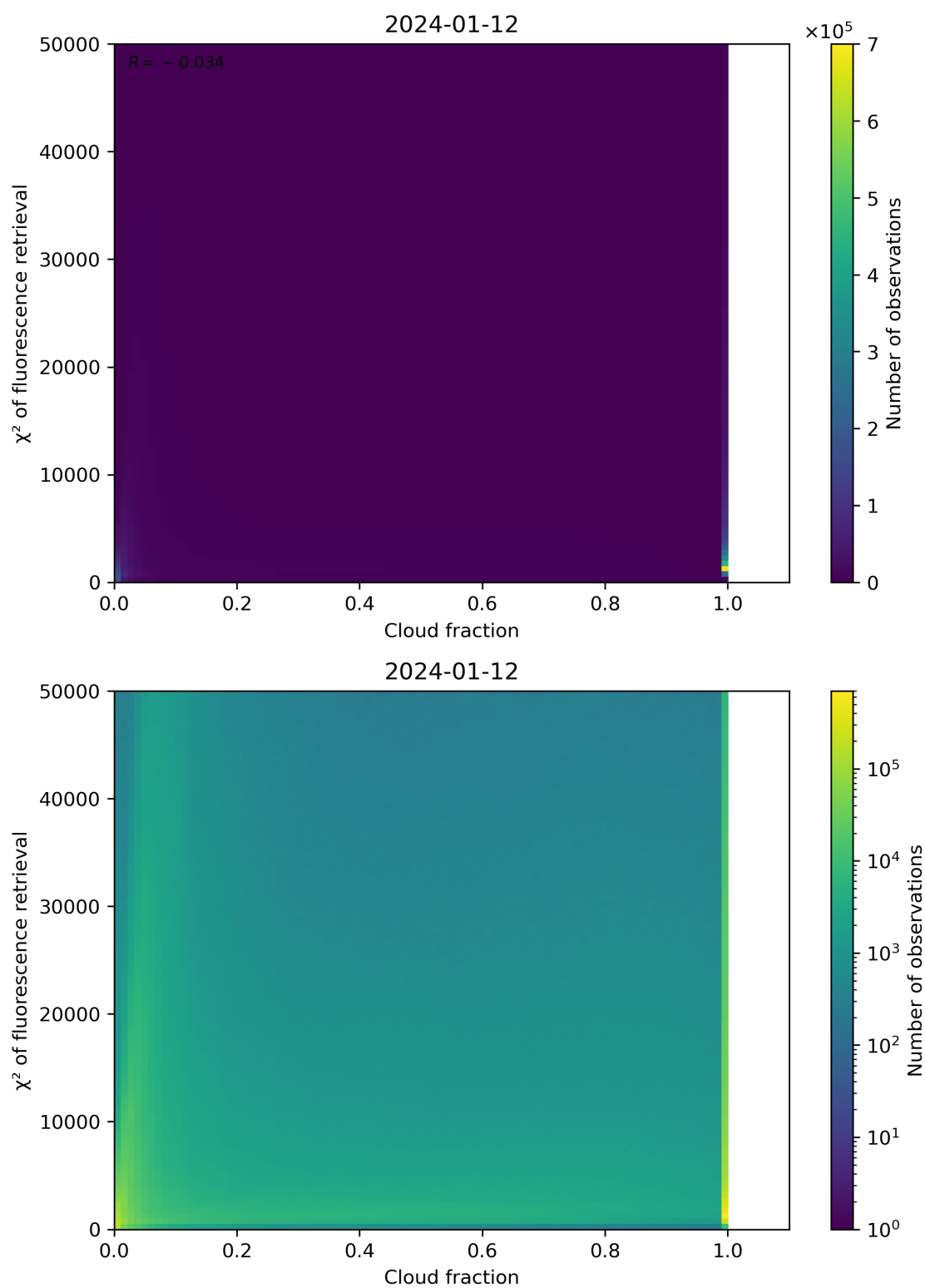
Figure 71: Scatter density plot of “Cloud fraction” against “ \chi^2 of fluorescence retrieval” for 2024-01-11 to 2024-01-13.
