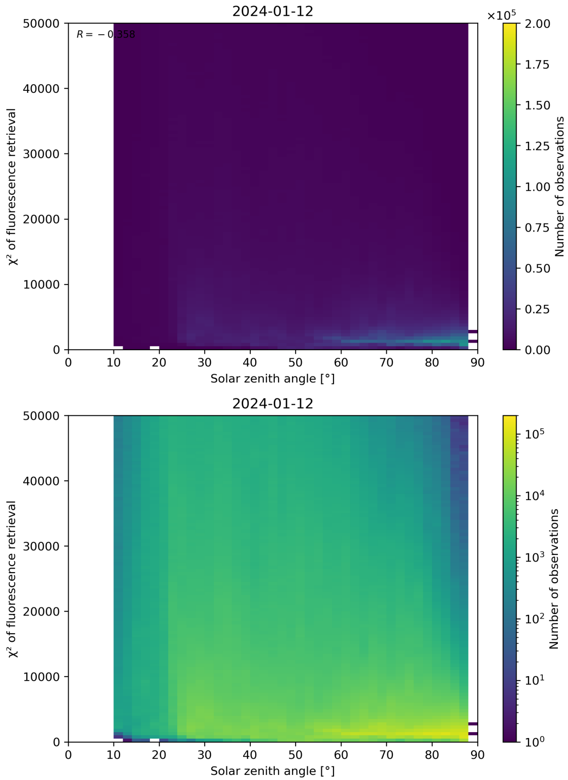
Figure 109: Scatter density plot of “Solar zenith angle” against “ \chi^2 of fluorescence retrieval” for 2024-01-11 to 2024-01-13.
