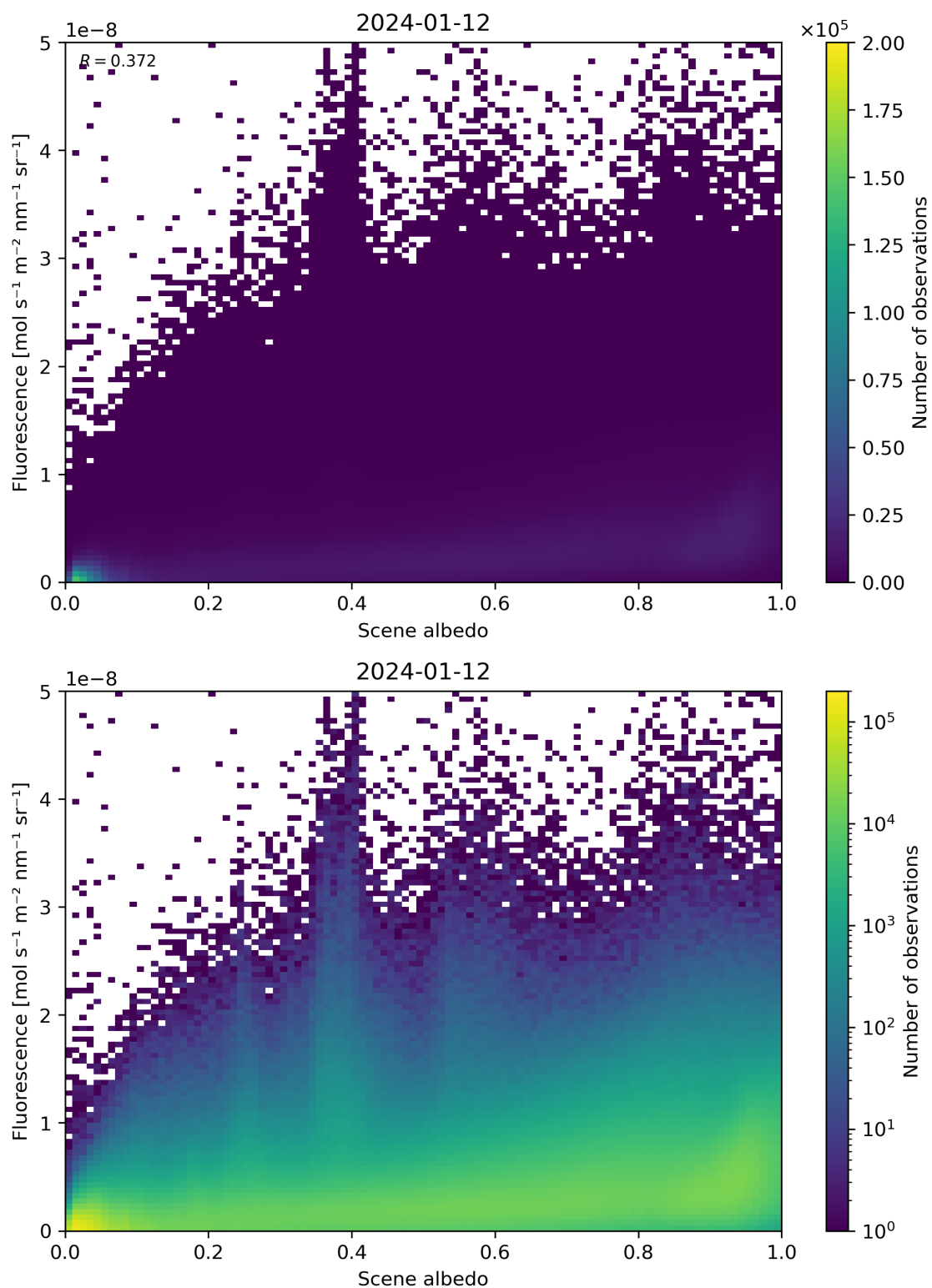
Figure 104: Scatter density plot of “Scene albedo” against “Fluorescence” for 2024-01-11 to 2024-01-13.
