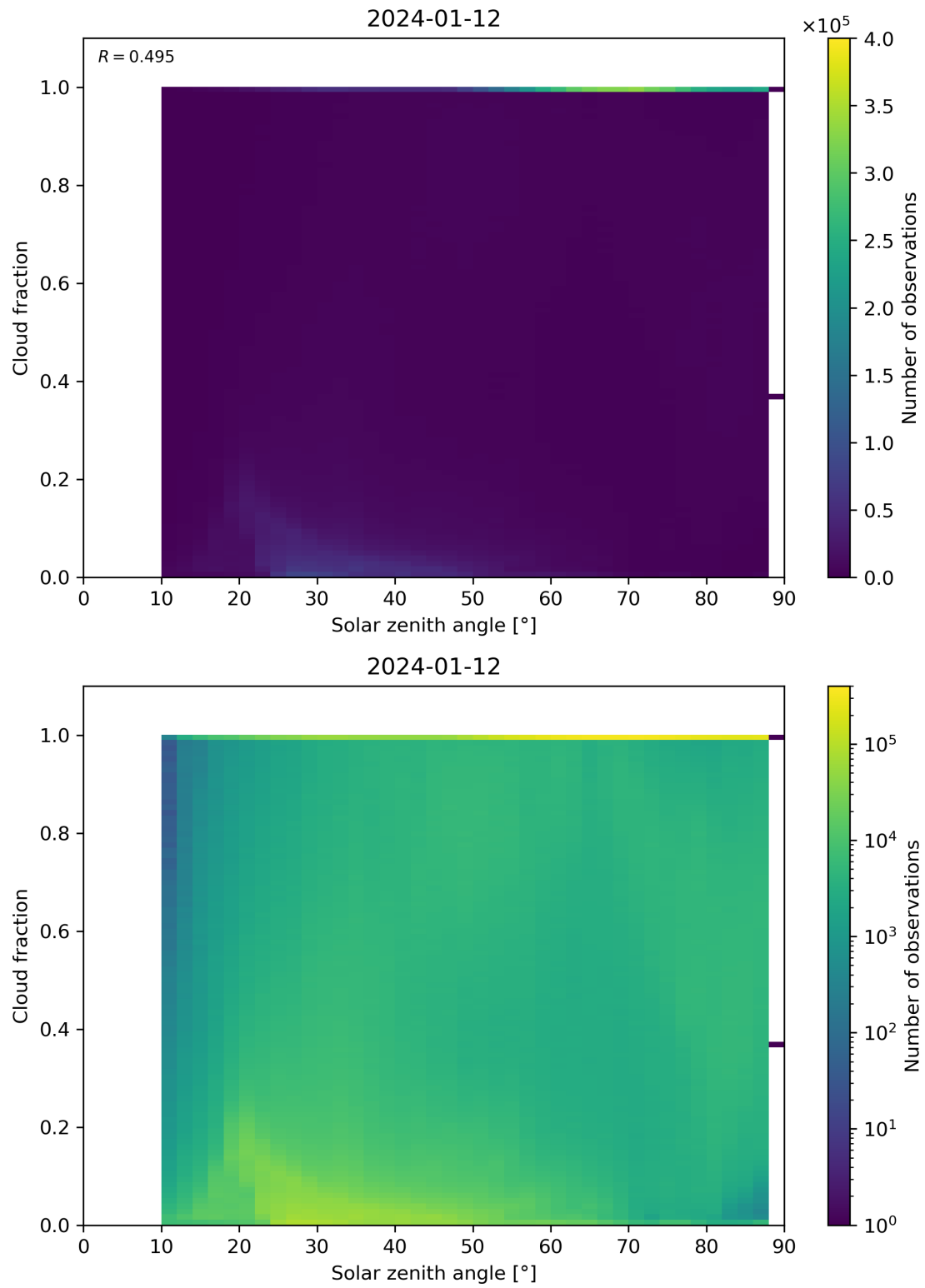
Figure 110: Scatter density plot of “Solar zenith angle” against “Cloud fraction” for 2024-01-11 to 2024-01-13.
