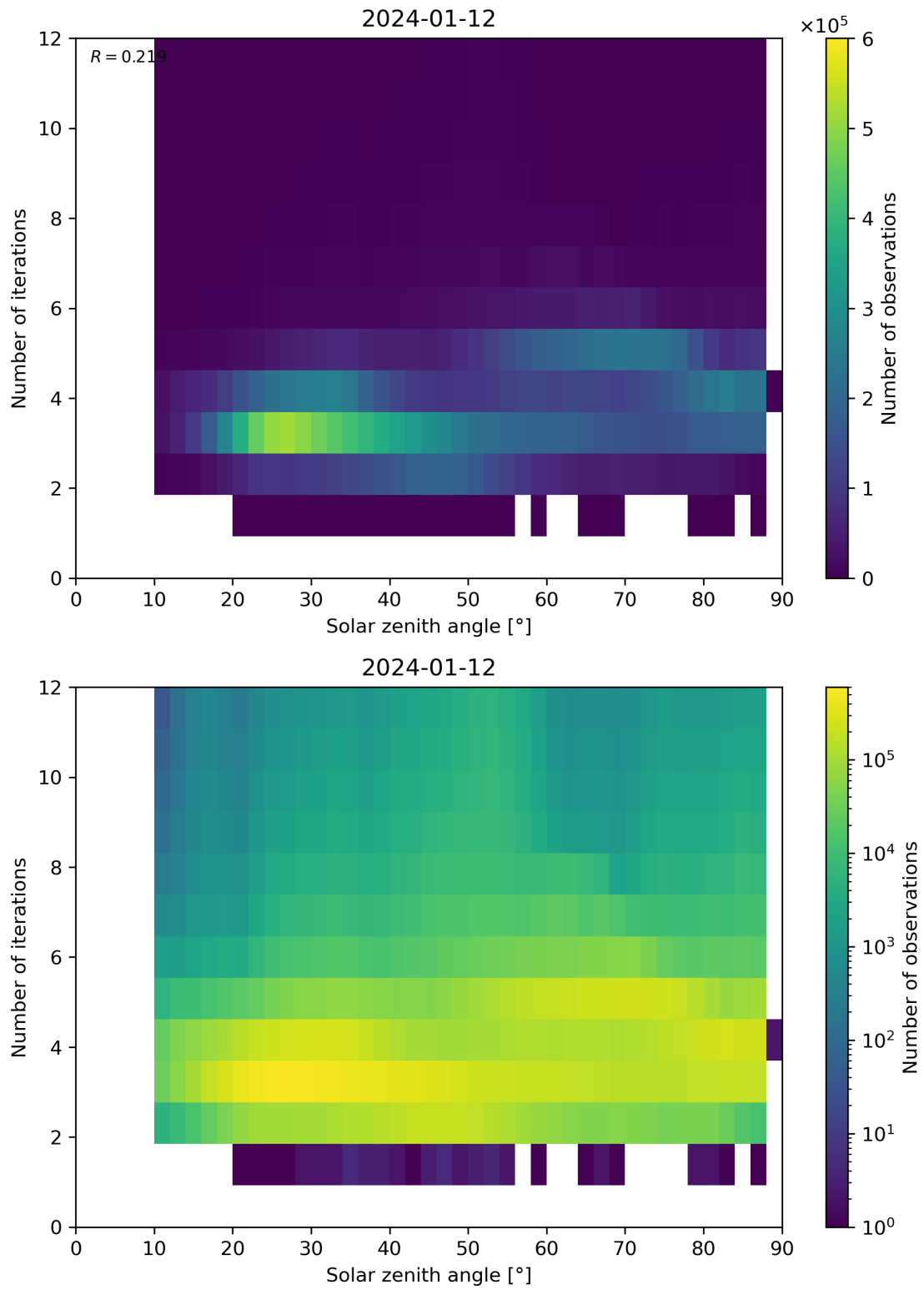
Figure 114: Scatter density plot of “Solar zenith angle” against “Number of iterations” for 2024-01-11 to 2024-01-13.
