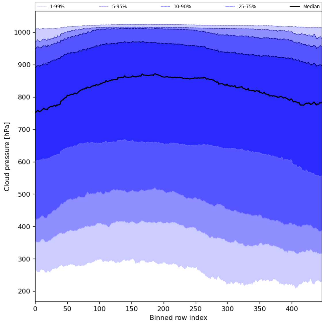
Figure 47: Along track statistics of “Cloud pressure” for 2024-01-11 to 2024-01-13
