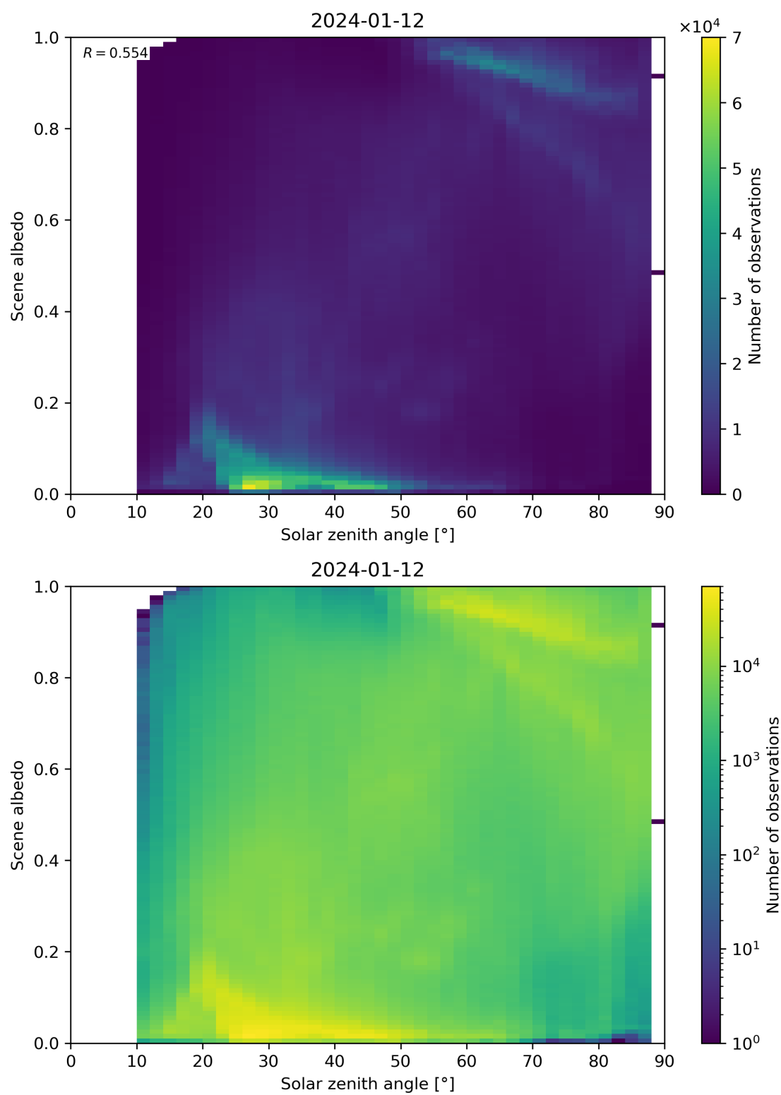
Figure 116: Scatter density plot of “Solar zenith angle” against “Scene albedo” for 2024-01-11 to 2024-01-13.
