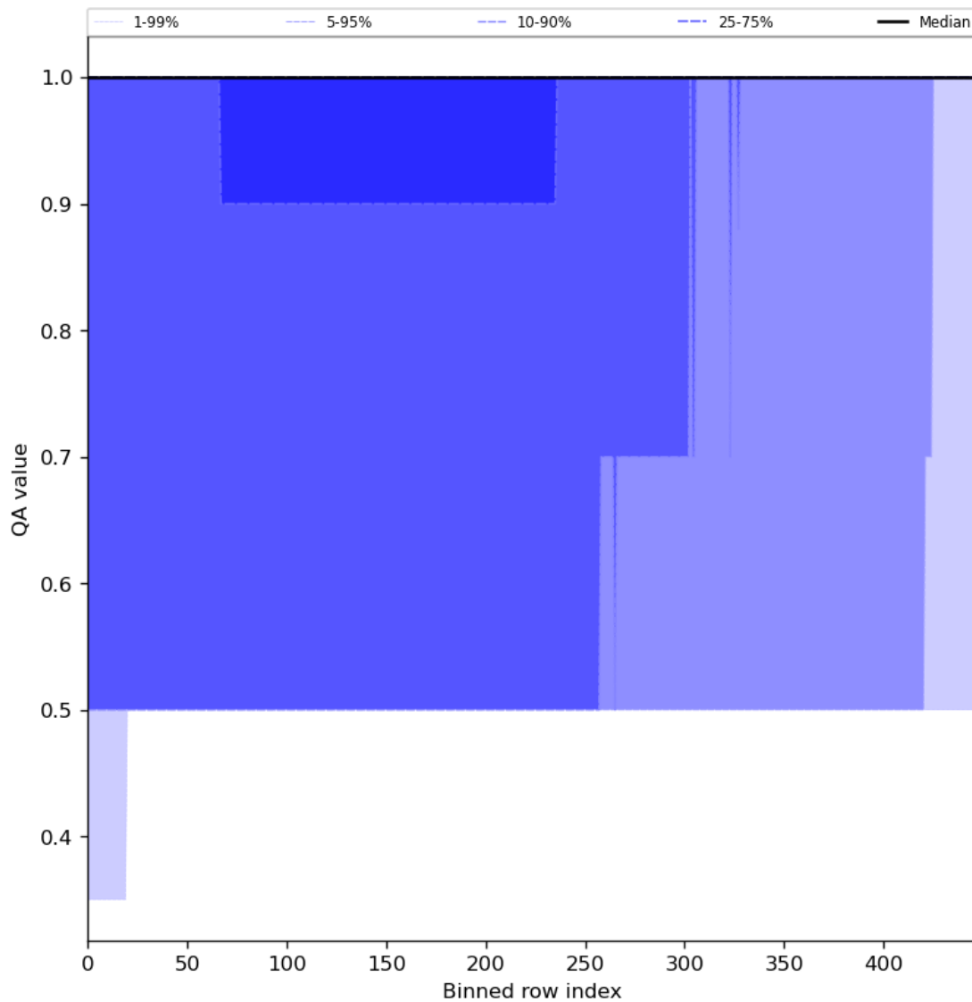
Figure 46: Along track statistics of “QA value” for 2024-01-11 to 2024-01-13
