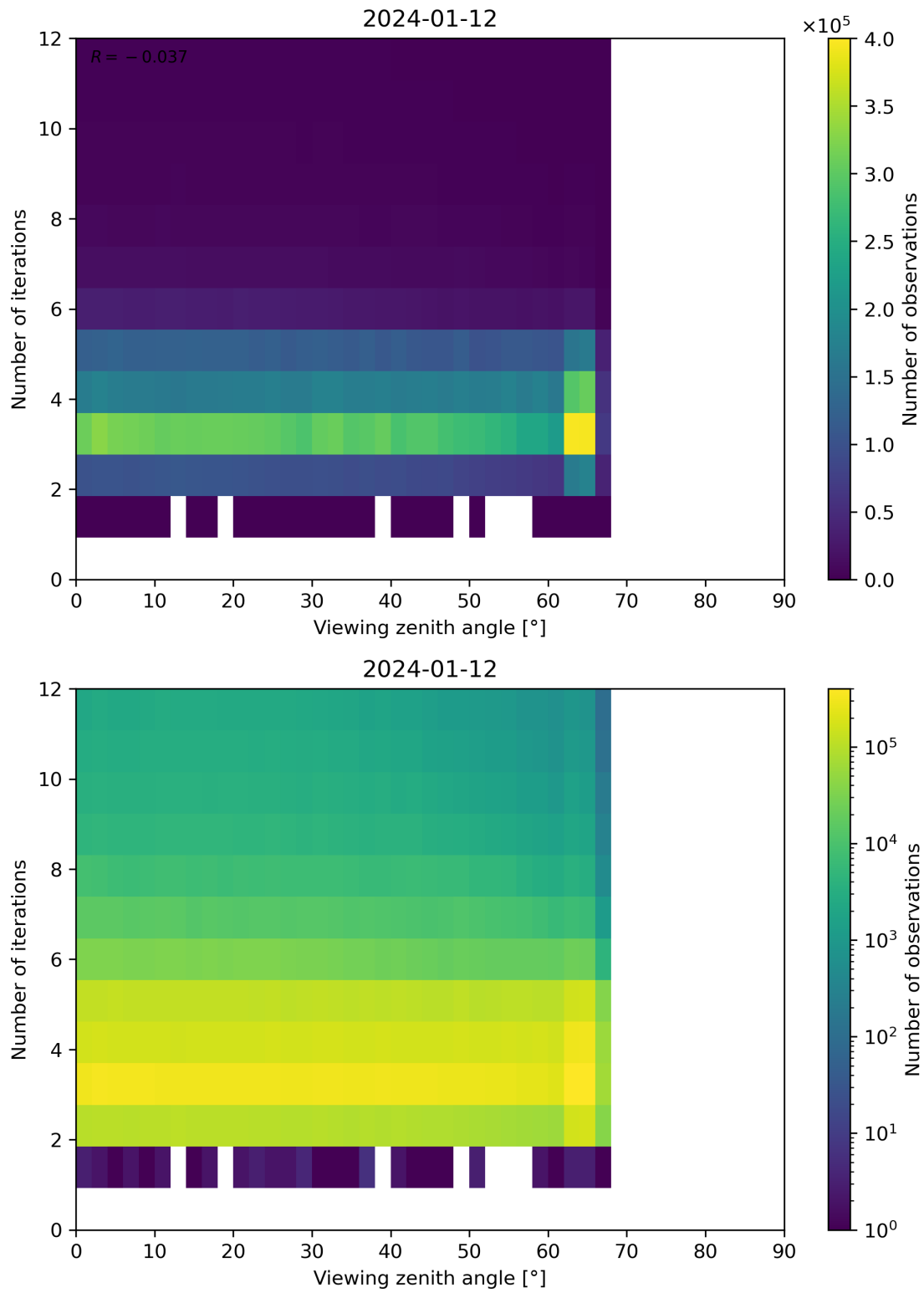
Figure 124: Scatter density plot of “Viewing zenith angle” against “Number of iterations” for 2024-01-11 to 2024-01-13.
