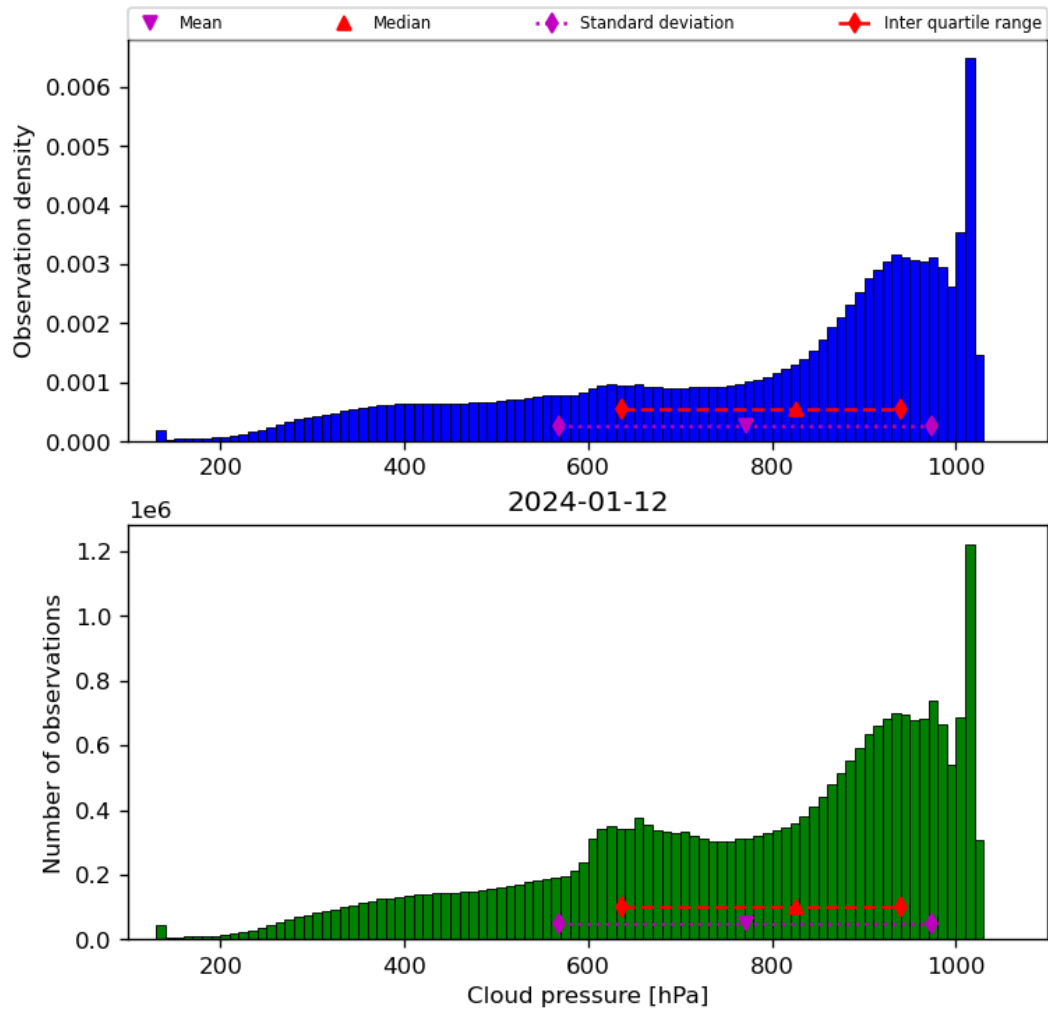
Figure 30: Histogram of “Cloud pressure” for 2024-01-11 to 2024-01-13
