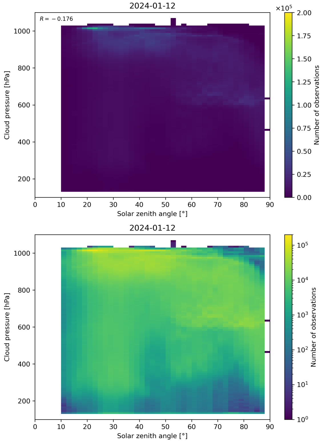
Figure 111: Scatter density plot of “Solar zenith angle” against “Cloud pressure” for 2024-01-11 to 2024-01-13.
