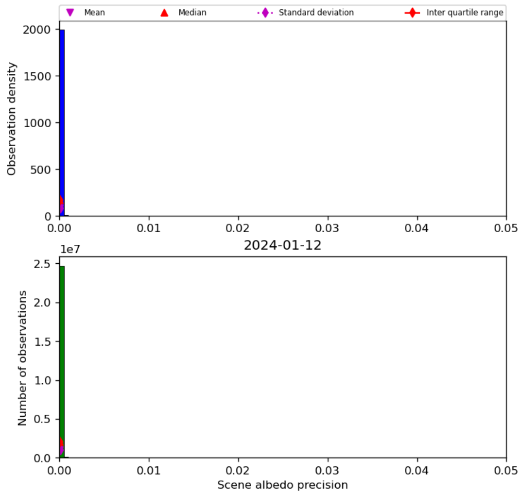
Figure 35: Histogram of “Scene albedo precision” for 2024-01-11 to 2024-01-13
