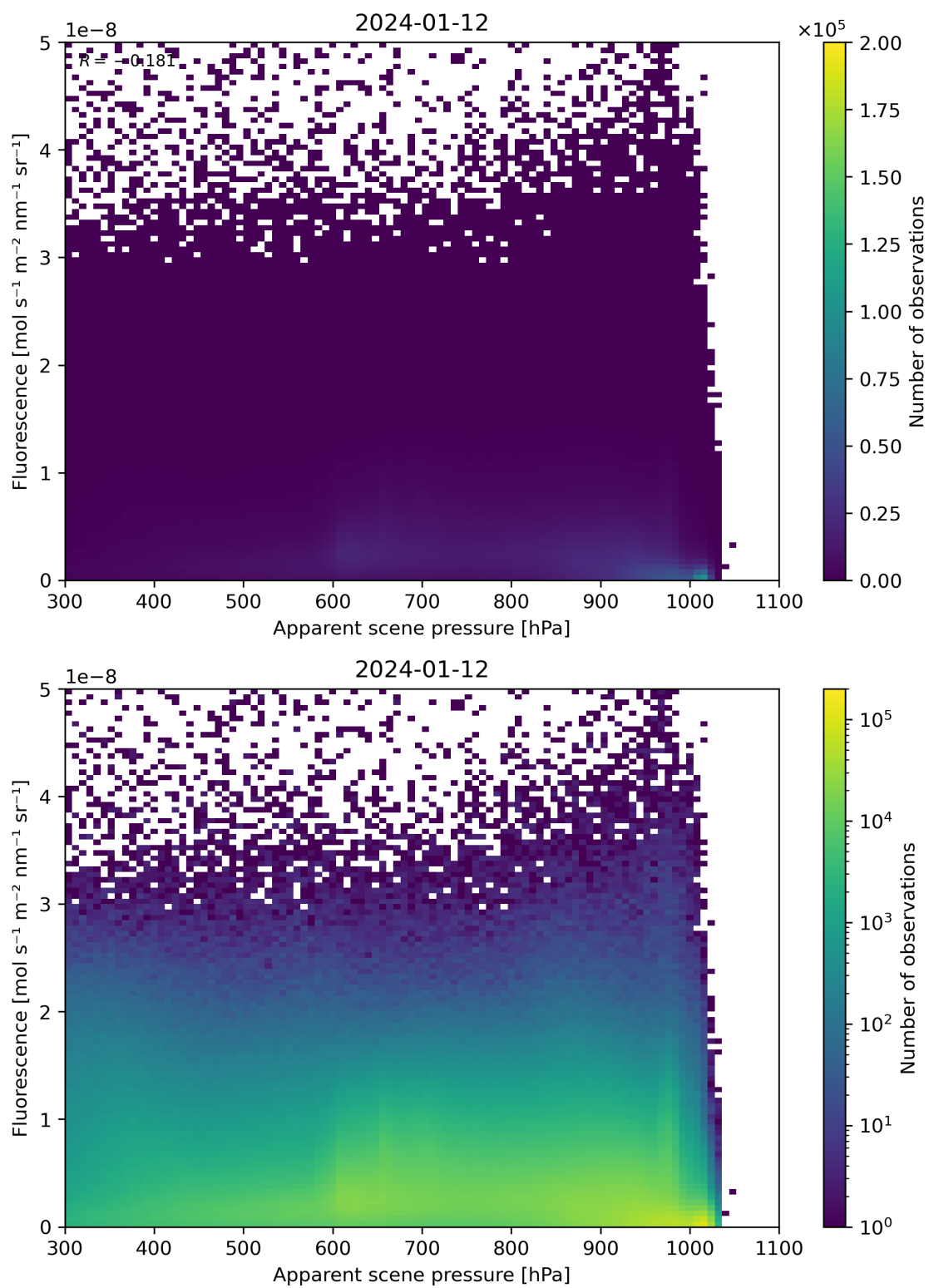
Figure 64: Scatter density plot of “Apparent scene pressure” against “Fluorescence” for 2024-01-11 to 2024-01-13.
