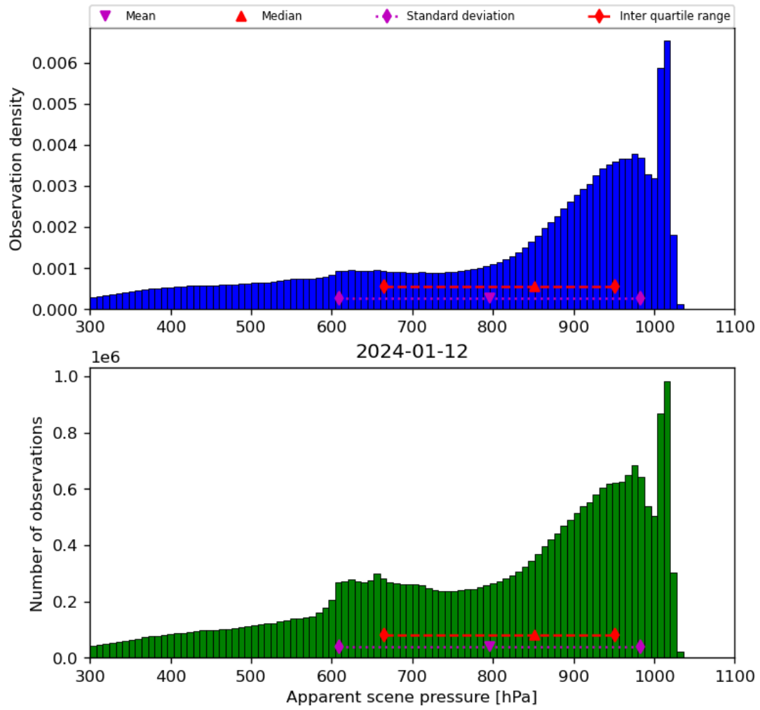
Figure 36: Histogram of “Apparent scene pressure” for 2024-01-11 to 2024-01-13
