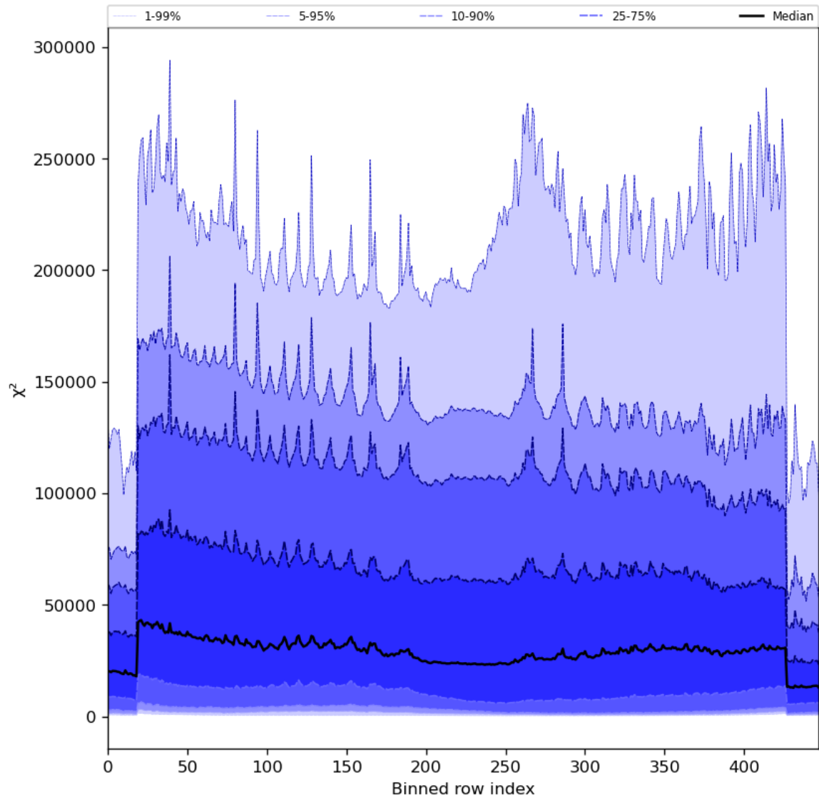
Figure 55: Along track statistics of “ \chi^2 ” for 2024-01-11 to 2024-01-13
