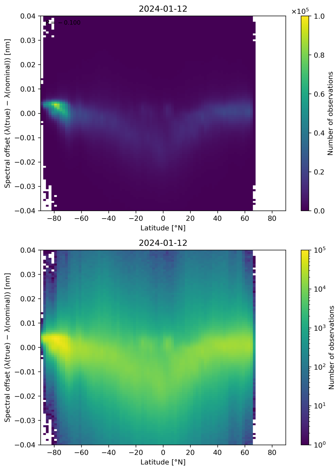
Figure 96: Scatter density plot of “Latitude” against “Spectral offset ( \lambda(\text{true}) - \lambda(\text{nominal}) )” for 2024-01-11 to 2024-01-13.
