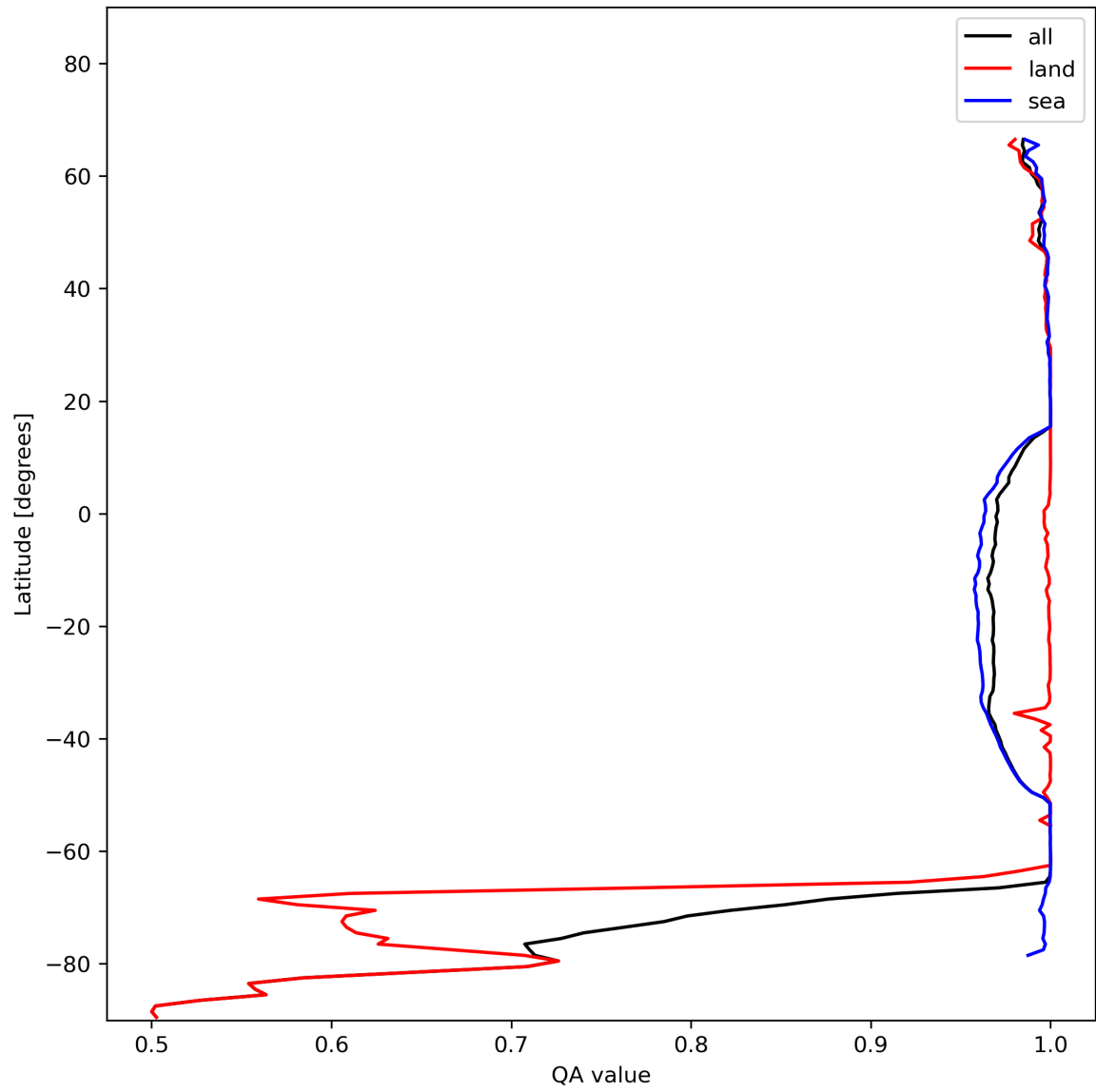
Figure 12: Zonal average of “QA value” for 2024-01-11 to 2024-01-13.
