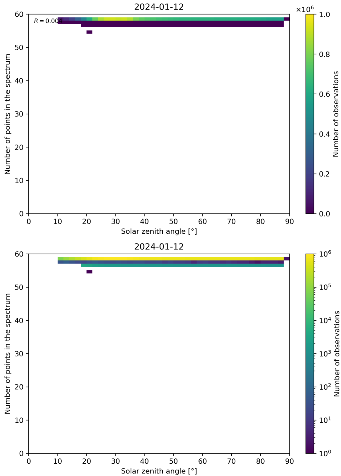
Figure 115: Scatter density plot of “Solar zenith angle” against “Number of points in the spectrum” for 2024-01-11 to 2024-01-13.
