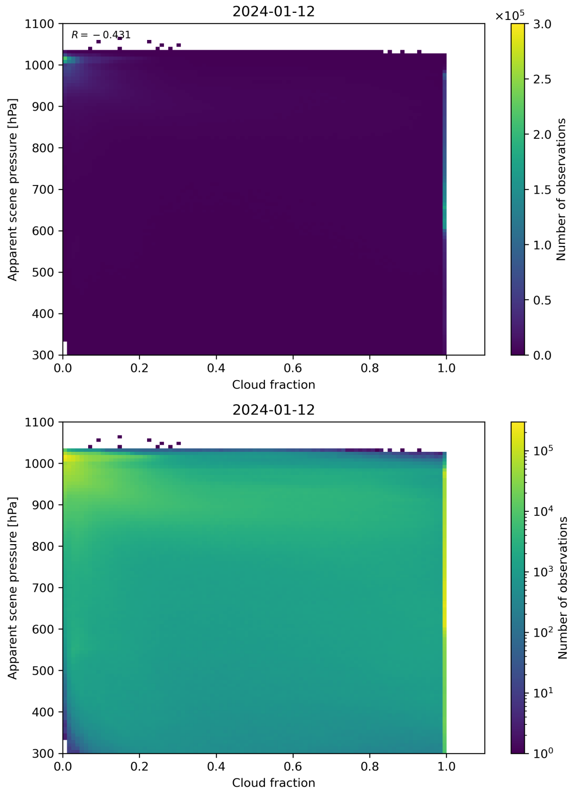
Figure 70: Scatter density plot of “Cloud fraction” against “Apparent scene pressure” for 2024-01-11 to 2024-01-13.
