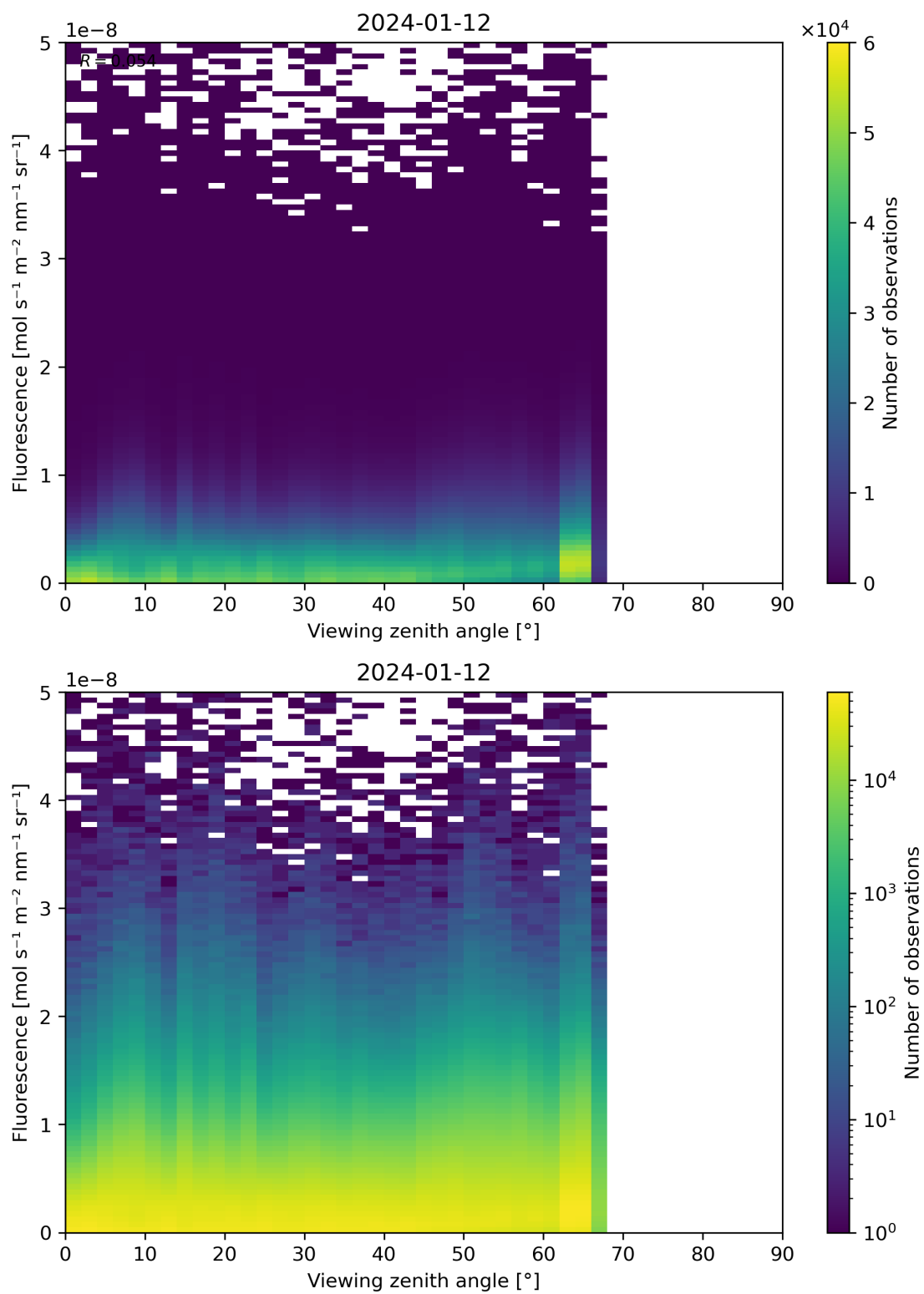
Figure 122: Scatter density plot of “Viewing zenith angle” against “Fluorescence” for 2024-01-11 to 2024-01-13.
