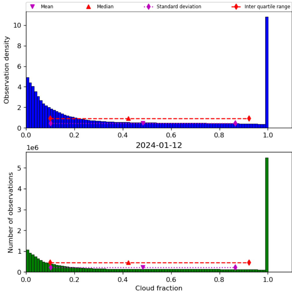
Figure 32: Histogram of “Cloud fraction” for 2024-01-11 to 2024-01-13
