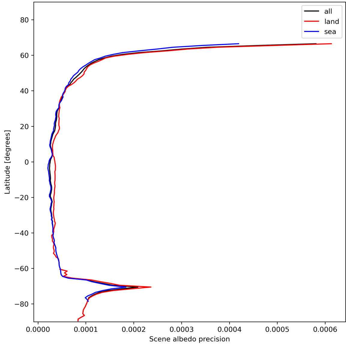
Figure 18: Zonal average of “Scene albedo precision” for 2024-01-11 to 2024-01-13.
