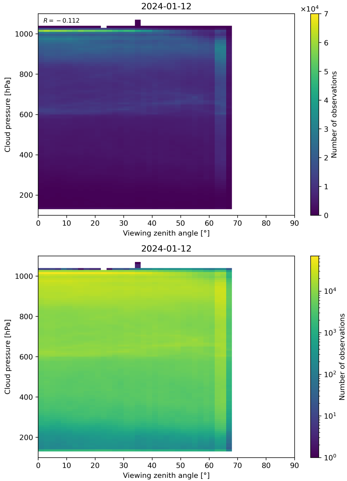
Figure 121: Scatter density plot of “Viewing zenith angle” against “Cloud pressure” for 2024-01-11 to 2024-01-13.
