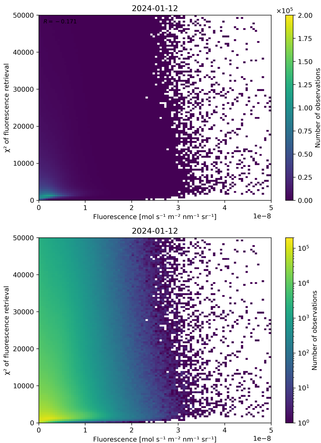
Figure 85: Scatter density plot of “Fluorescence” against “ \chi^2 of fluorescence retrieval” for 2024-01-11 to 2024-01-13.
