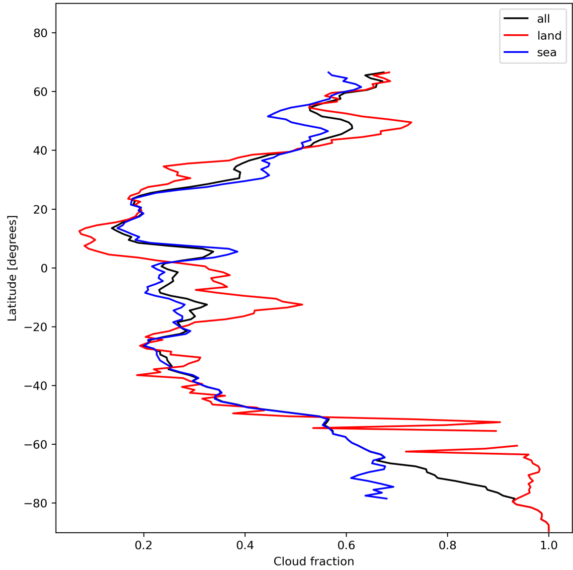
Figure 15: Zonal average of “Cloud fraction” for 2024-01-13 to 2024-01-15.
