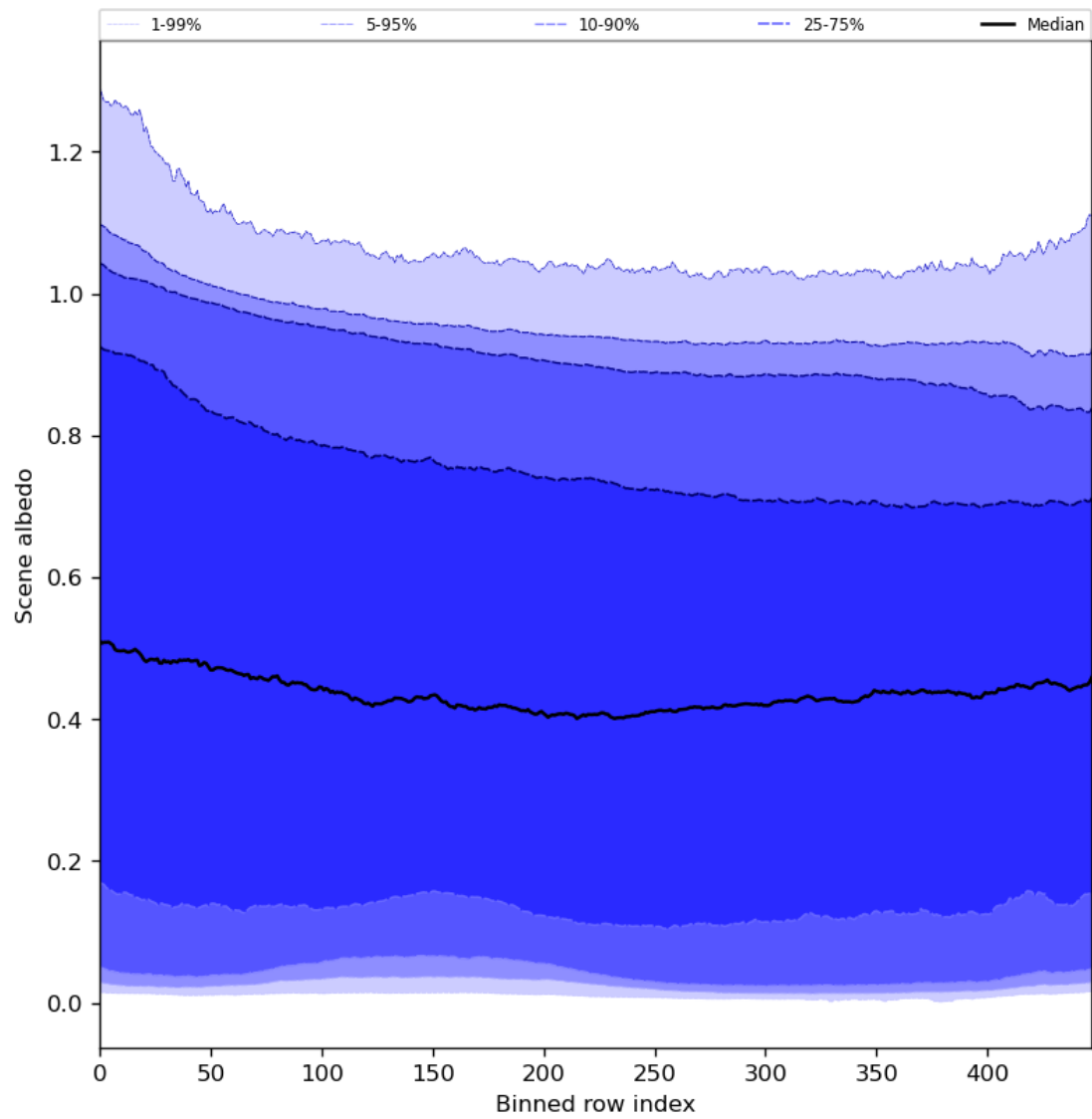
Figure 51: Along track statistics of “Scene albedo” for 2024-01-13 to 2024-01-15
