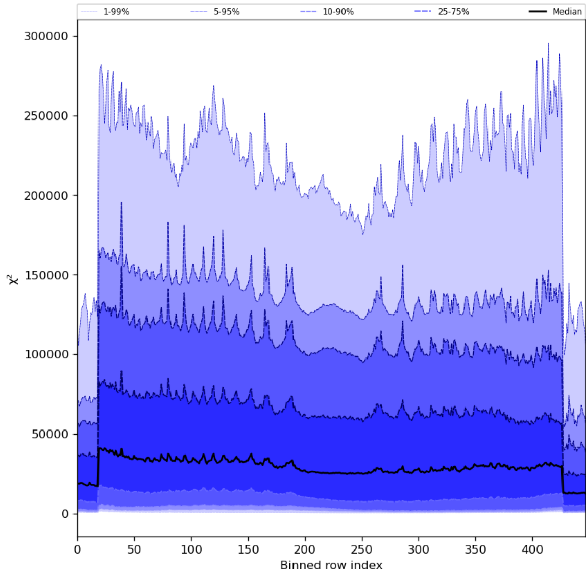
Figure 55: Along track statistics of “ \chi^2 ” for 2024-01-13 to 2024-01-15
