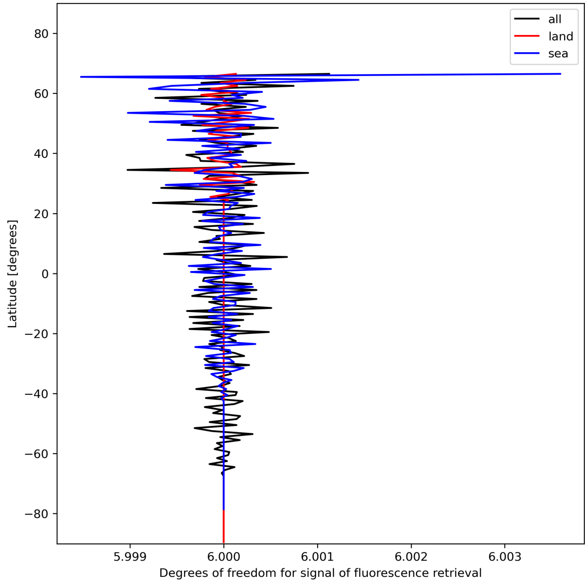
Figure 26: Zonal average of “Degrees of freedom for signal of fluorescence retrieval” for 2024-01-13 to 2024-01-15.
