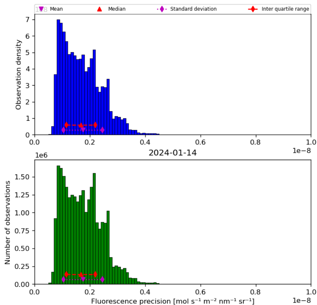
Figure 41: Histogram of “Fluorescence precision” for 2024-01-13 to 2024-01-15
