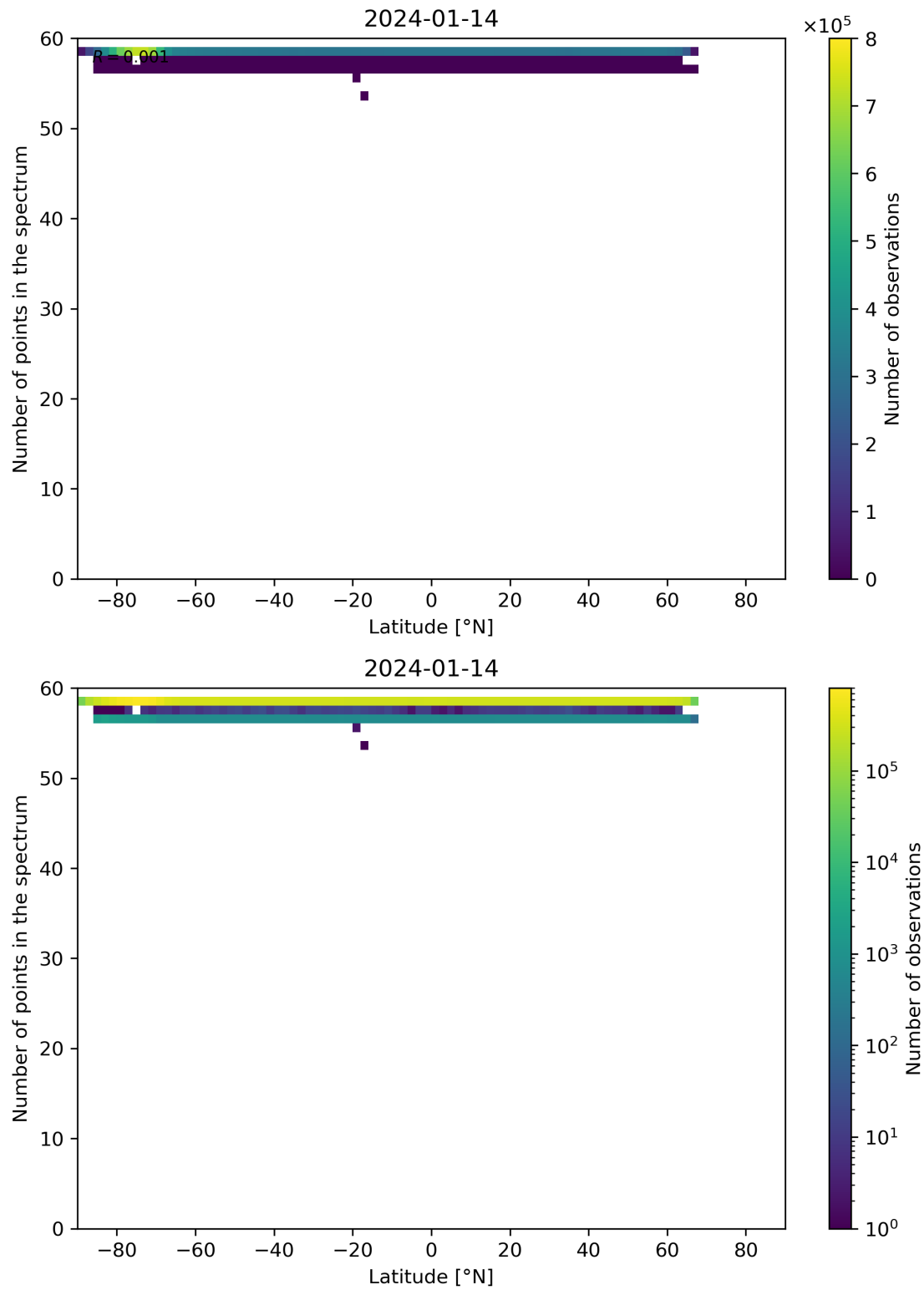
Figure 94: Scatter density plot of “Latitude” against “Number of points in the spectrum” for 2024-01-13 to 2024-01-15.
