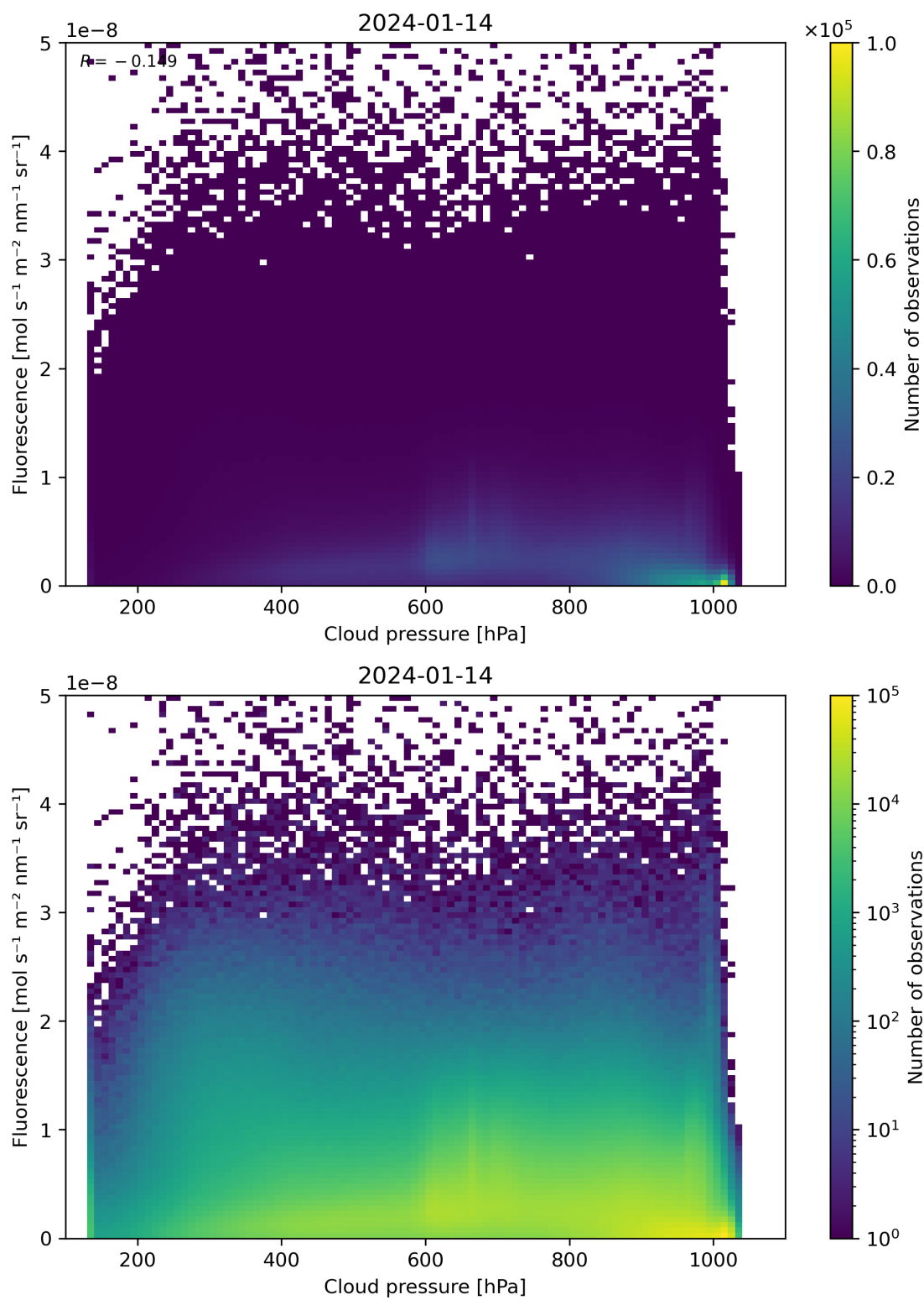
Figure 80: Scatter density plot of “Cloud pressure” against “Fluorescence” for 2024-01-13 to 2024-01-15.
