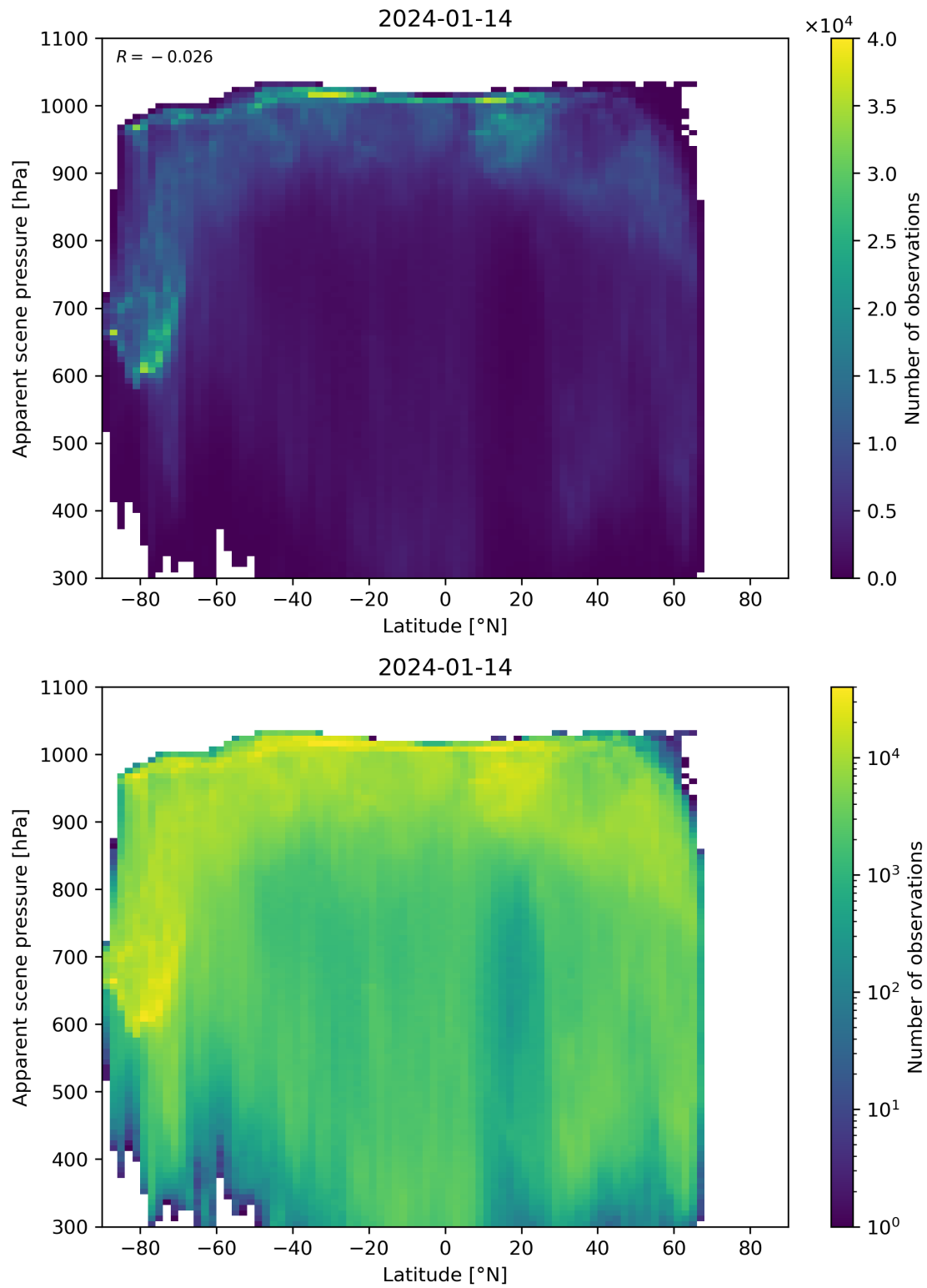
Figure 88: Scatter density plot of “Latitude” against “Apparent scene pressure” for 2024-01-13 to 2024-01-15.
