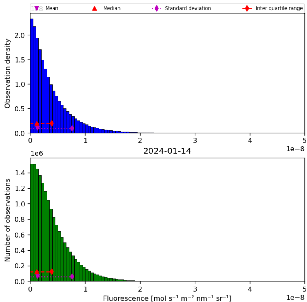
Figure 40: Histogram of “Fluorescence” for 2024-01-13 to 2024-01-15
