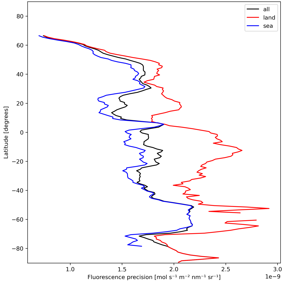
Figure 24: Zonal average of “Fluorescence precision” for 2024-01-13 to 2024-01-15.
