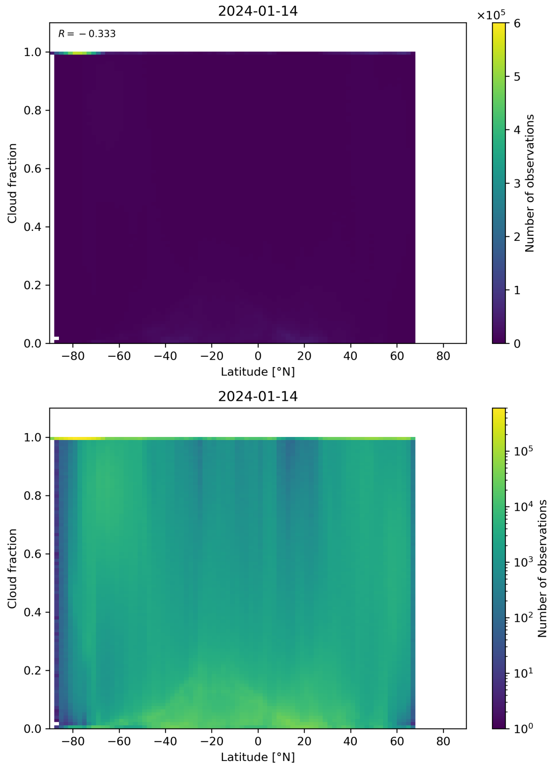
Figure 90: Scatter density plot of “Latitude” against “Cloud fraction” for 2024-01-13 to 2024-01-15.
