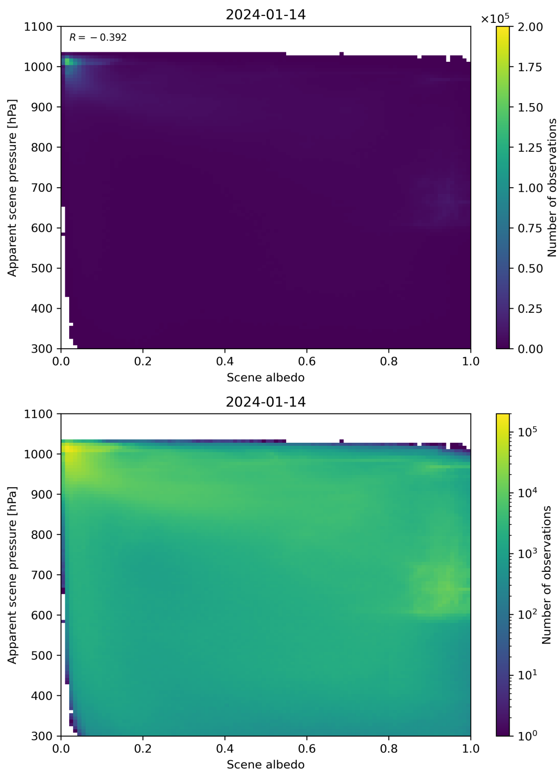
Figure 102: Scatter density plot of “Scene albedo” against “Apparent scene pressure” for 2024-01-13 to 2024-01-15.
