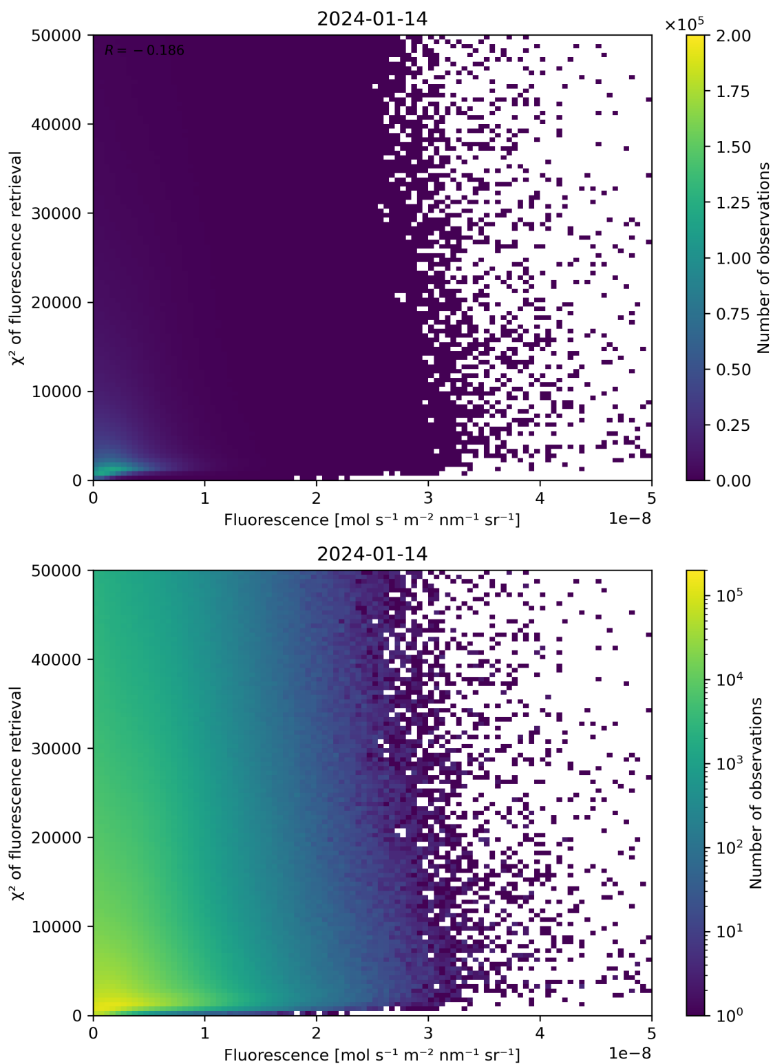
Figure 85: Scatter density plot of “Fluorescence” against “ \chi^2 of fluorescence retrieval” for 2024-01-13 to 2024-01-15.
