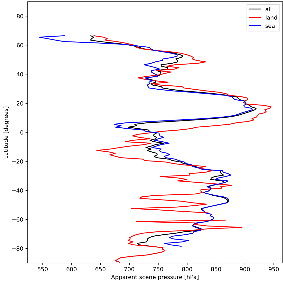
Figure 19: Zonal average of “Apparent scene pressure” for 2024-01-13 to 2024-01-15.
