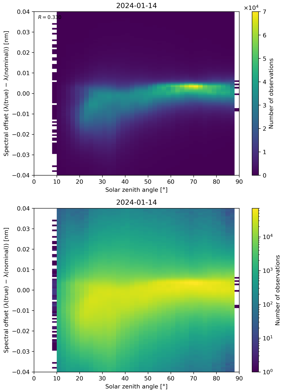
Figure 117: Scatter density plot of “Solar zenith angle” against “Spectral offset ( \lambda(\text{true}) - \lambda(\text{nominal}) )” for 2024-01-13 to 2024-01-15.
