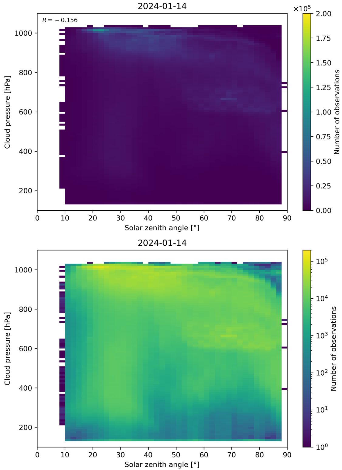
Figure 111: Scatter density plot of “Solar zenith angle” against “Cloud pressure” for 2024-01-13 to 2024-01-15.
