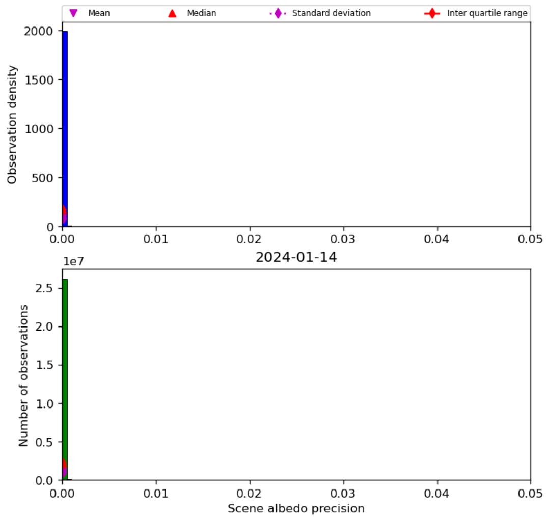
Figure 35: Histogram of “Scene albedo precision” for 2024-01-13 to 2024-01-15
