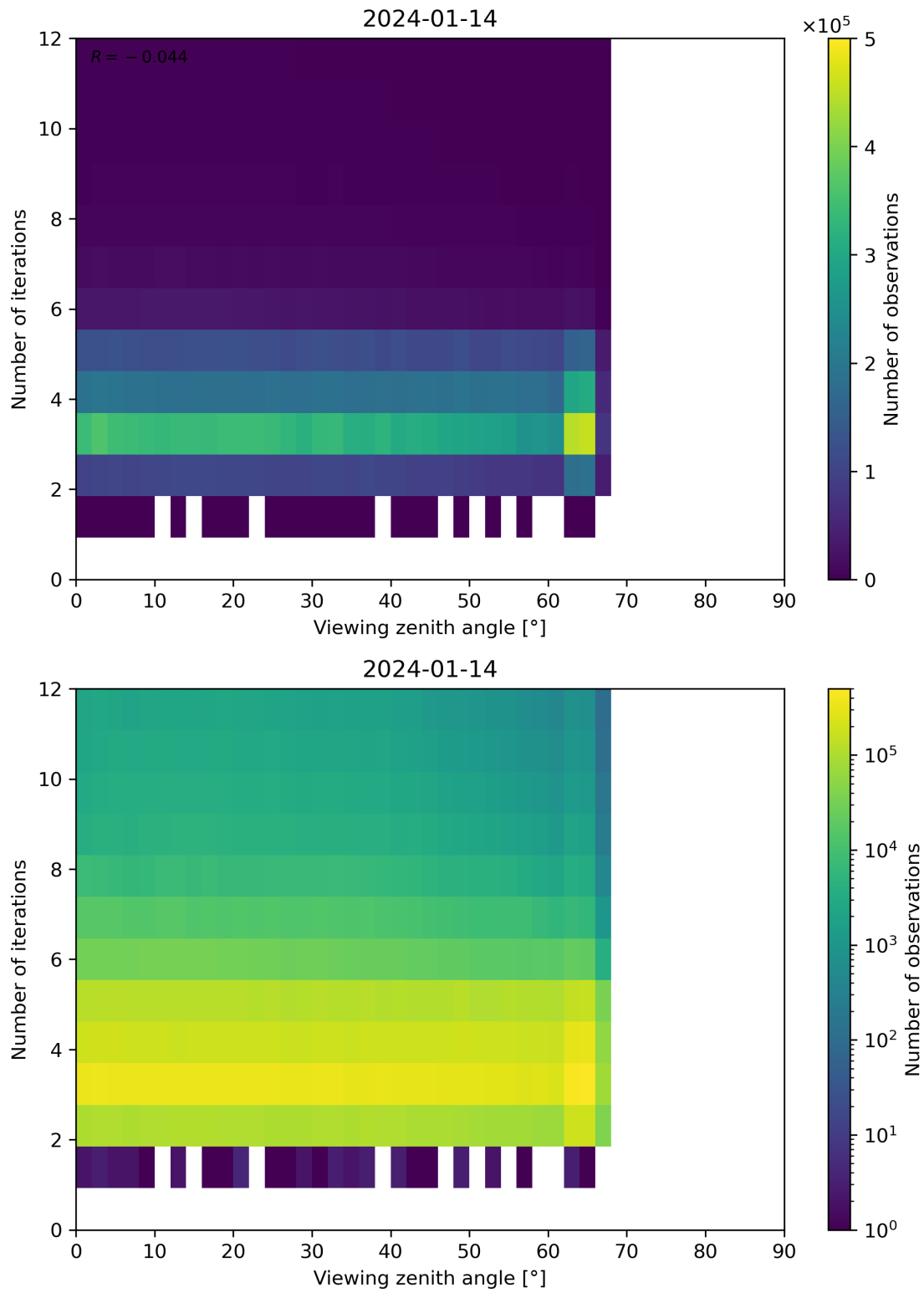
Figure 124: Scatter density plot of “Viewing zenith angle” against “Number of iterations” for 2024-01-13 to 2024-01-15.
