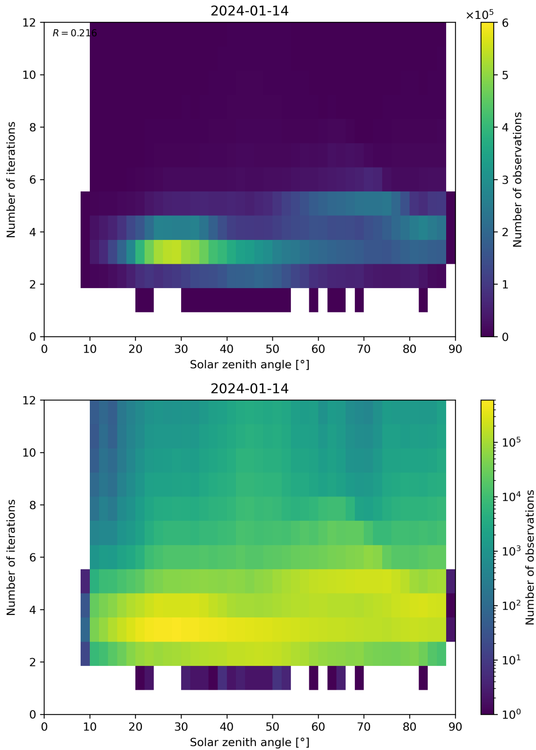
Figure 114: Scatter density plot of “Solar zenith angle” against “Number of iterations” for 2024-01-13 to 2024-01-15.
