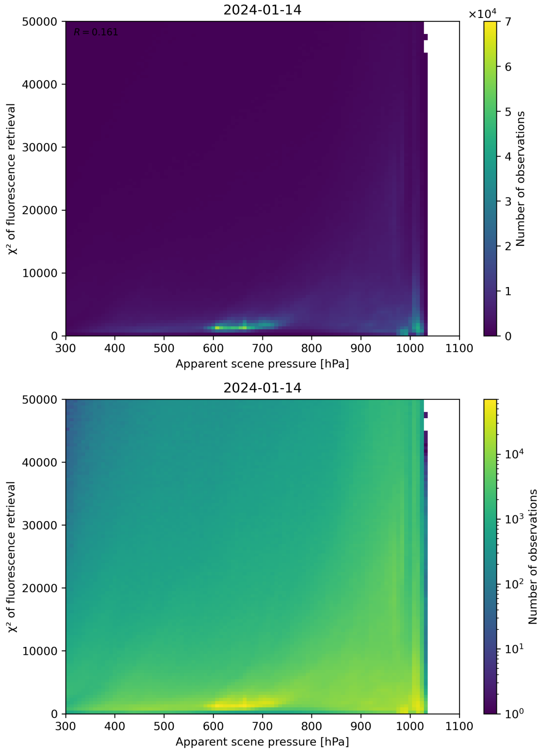
Figure 63: Scatter density plot of “Apparent scene pressure” against “ \chi^2 of fluorescence retrieval” for 2024-01-13 to 2024-01-15.
