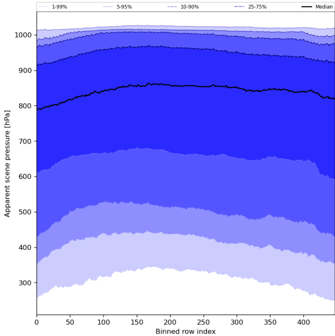
Figure 53: Along track statistics of “Apparent scene pressure” for 2024-01-13 to 2024-01-15
