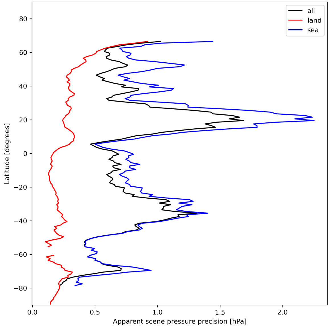
Figure 20: Zonal average of “Apparent scene pressure precision” for 2024-01-13 to 2024-01-15.
