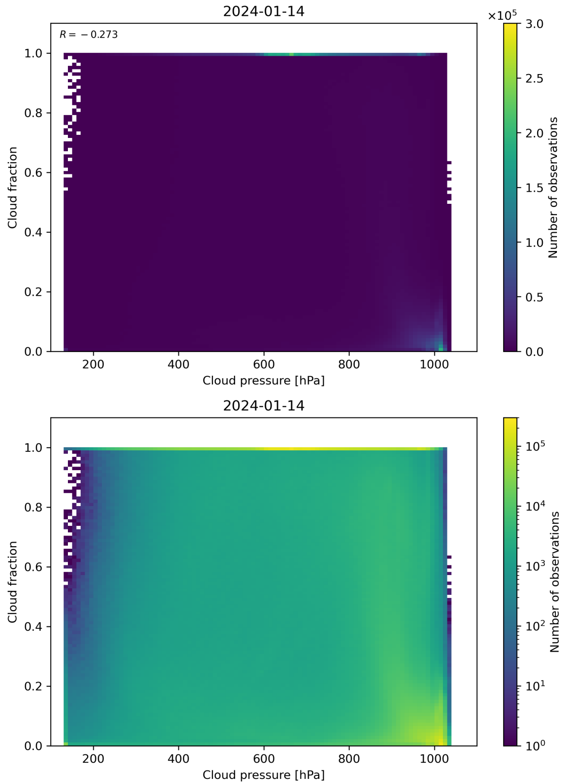
Figure 79: Scatter density plot of “Cloud pressure” against “Cloud fraction” for 2024-01-13 to 2024-01-15.
