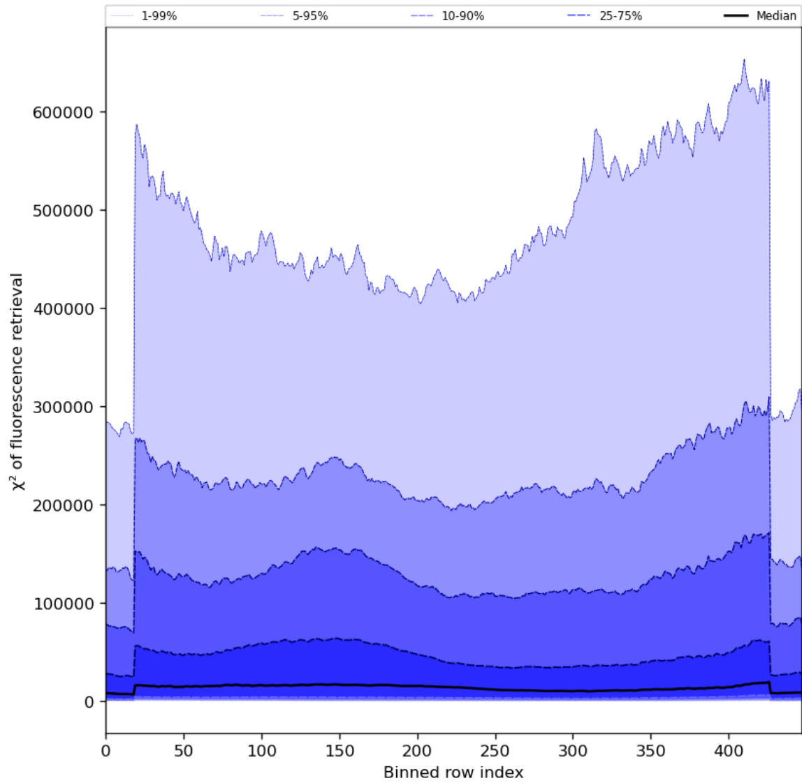
Figure 59: Along track statistics of “ \chi^2 of fluorescence retrieval” for 2024-01-13 to 2024-01-15
