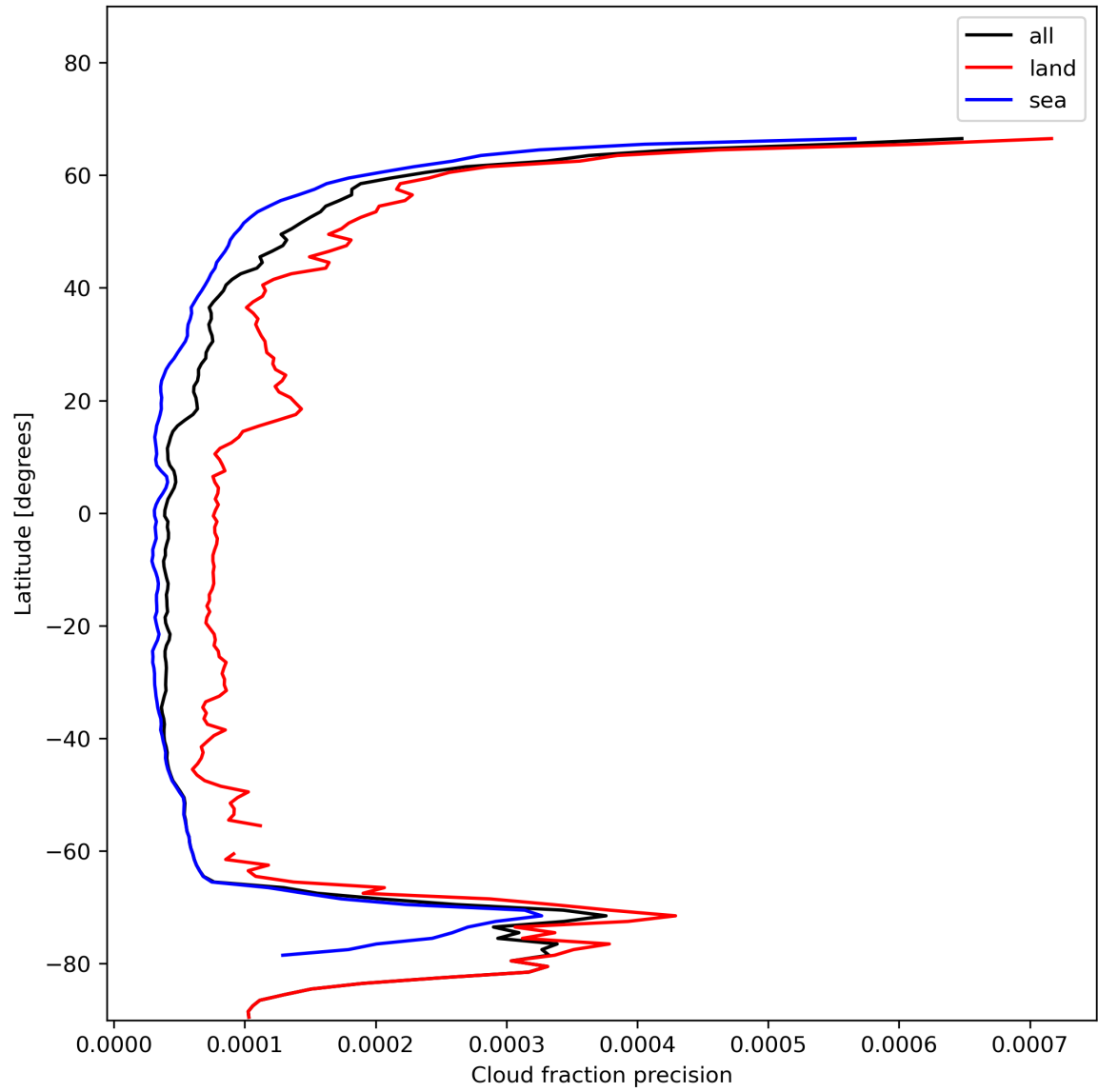
Figure 16: Zonal average of “Cloud fraction precision” for 2024-01-13 to 2024-01-15.
