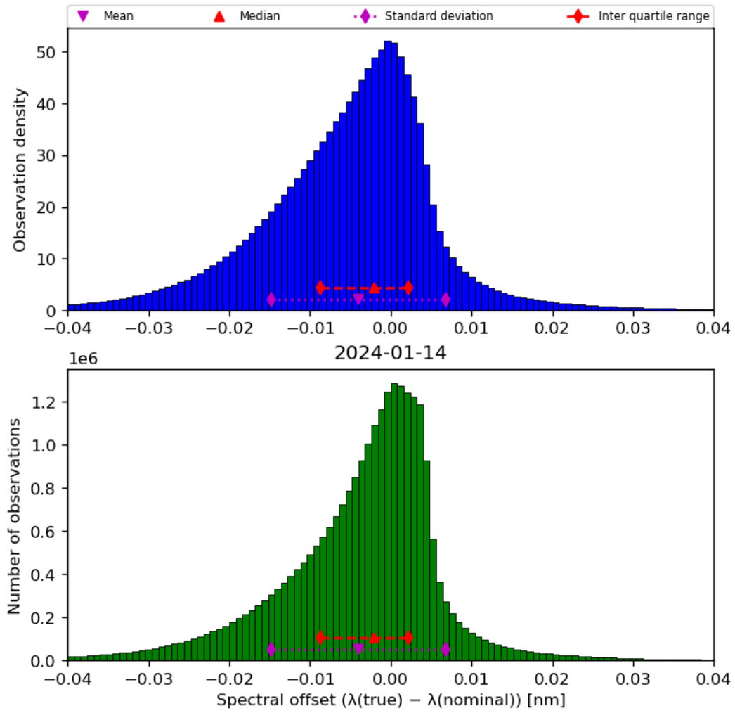
Figure 45: Histogram of “Spectral offset ( \lambda(\text{true}) - \lambda(\text{nominal}) )” for 2024-01-13 to 2024-01-15
