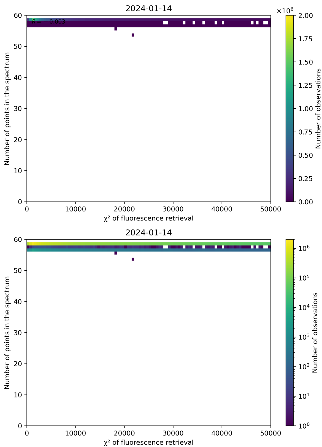
Figure 68: Scatter density plot of “ \chi^2 of fluorescence retrieval” against “Number of points in the spectrum” for 2024-01-13 to 2024-01-15.
