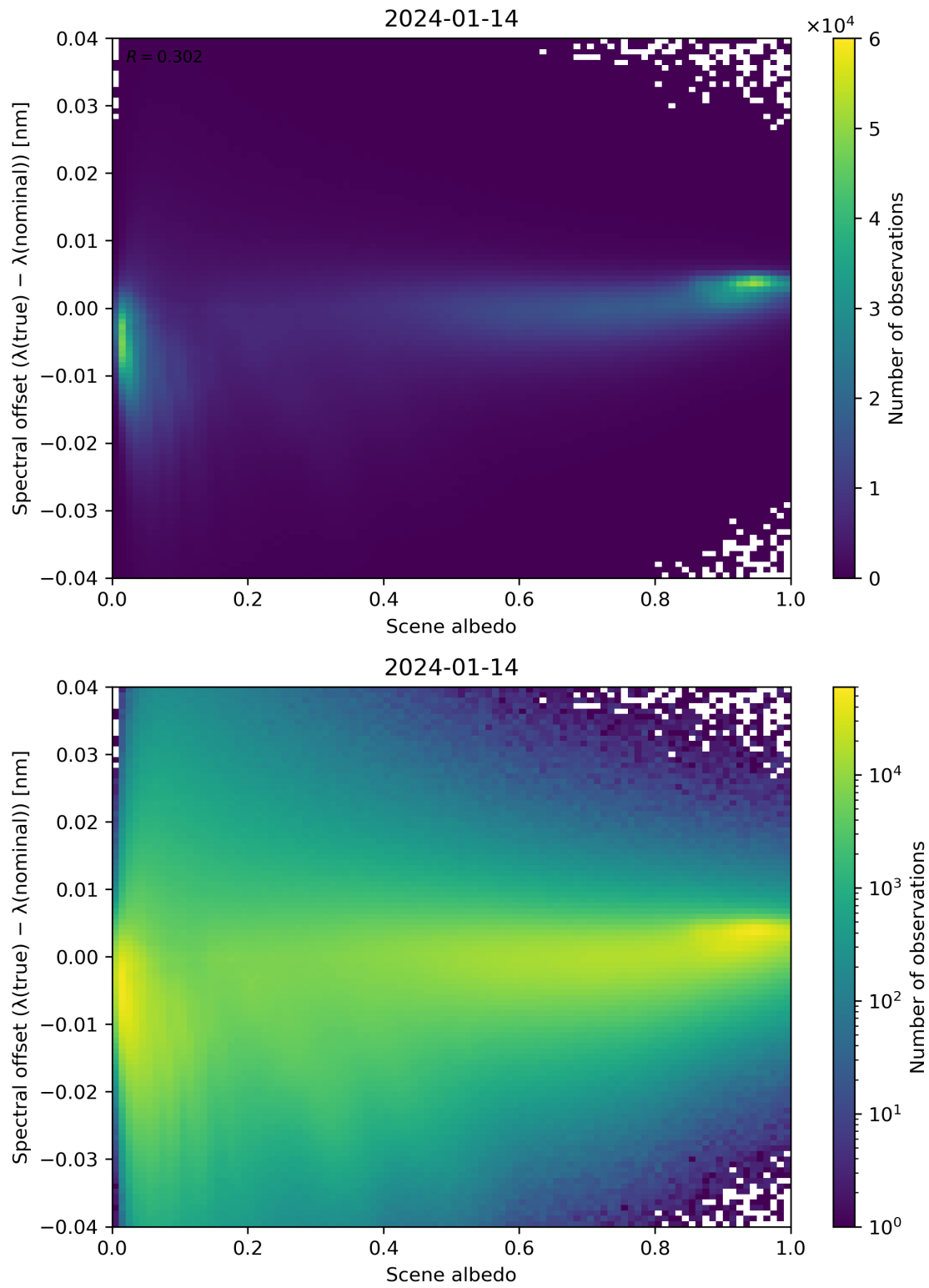
Figure 107: Scatter density plot of “Scene albedo” against “Spectral offset ( \lambda(\text{true}) - \lambda(\text{nominal}) )” for 2024-01-13 to 2024-01-15.
