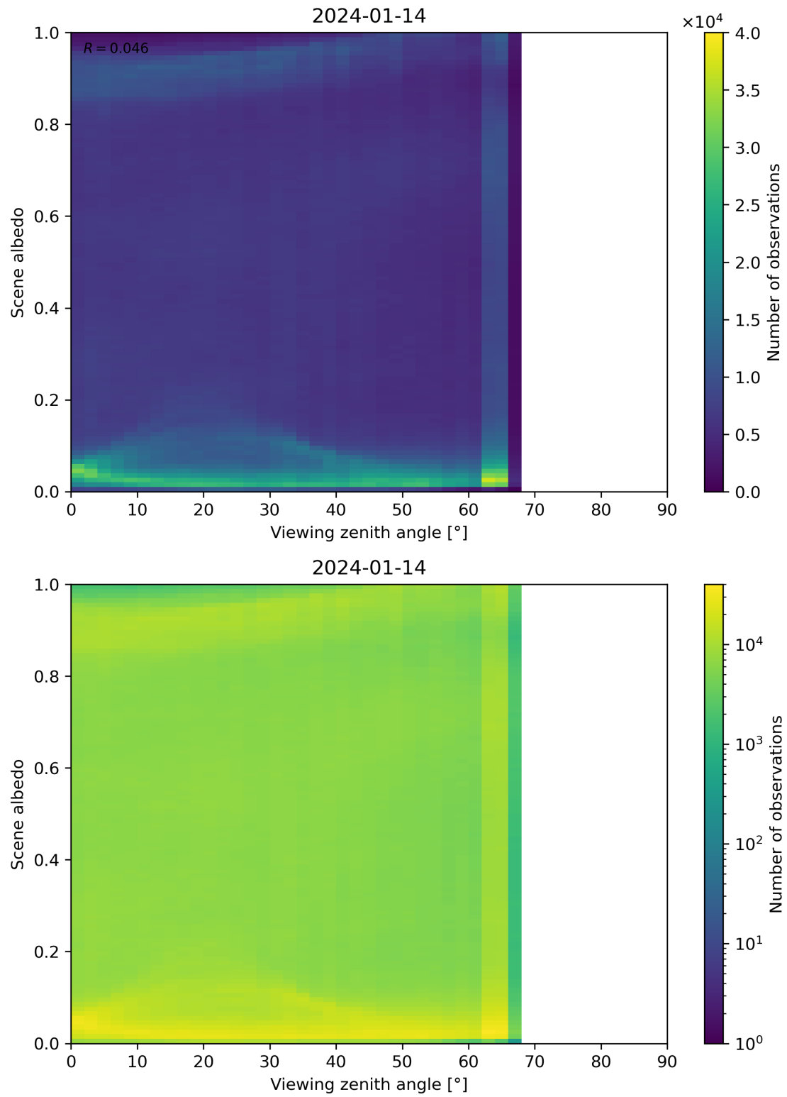
Figure 126: Scatter density plot of “Viewing zenith angle” against “Scene albedo” for 2024-01-13 to 2024-01-15.
