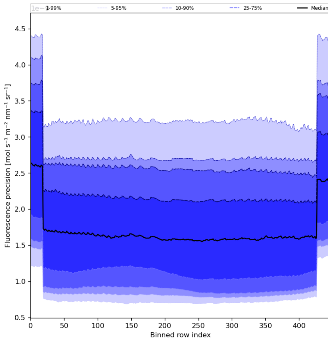
Figure 58: Along track statistics of “Fluorescence precision” for 2024-01-13 to 2024-01-15
