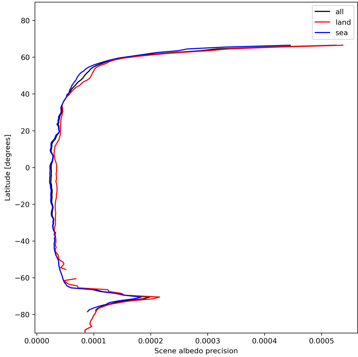
Figure 18: Zonal average of “Scene albedo precision” for 2024-01-13 to 2024-01-15.
