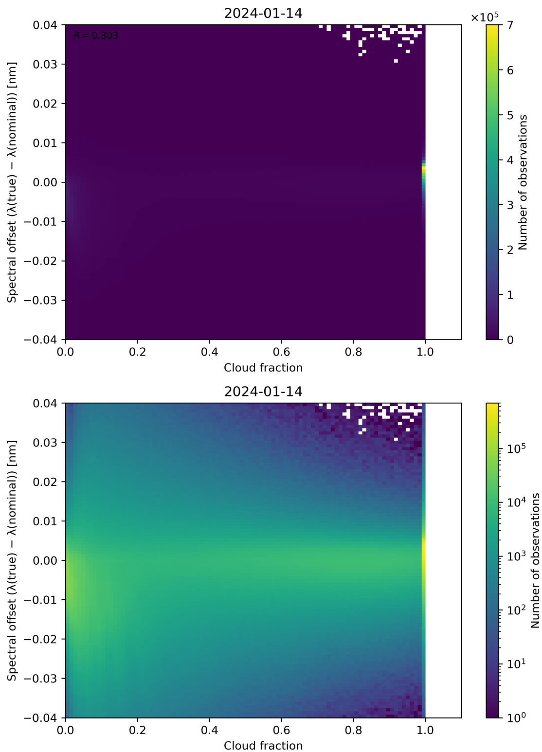
Figure 76: Scatter density plot of “Cloud fraction” against “Spectral offset ( \lambda(\text{true}) - \lambda(\text{nominal}) )” for 2024-01-13 to 2024-01-15.
