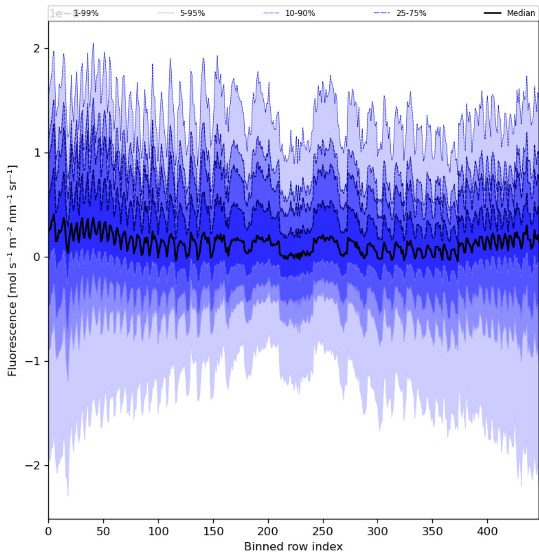
Figure 57: Along track statistics of “Fluorescence” for 2024-01-13 to 2024-01-15
