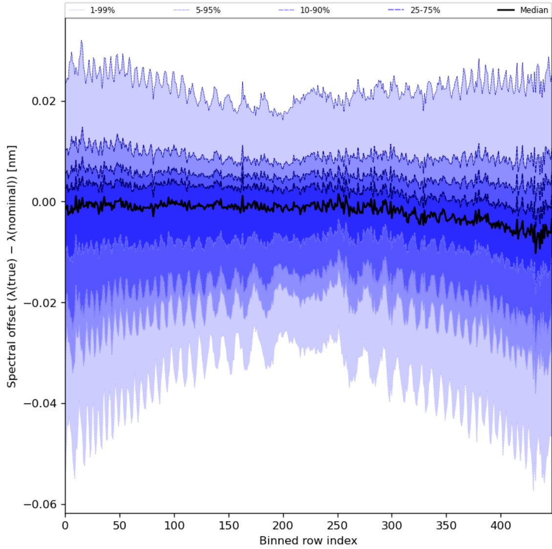
Figure 62: Along track statistics of “Spectral offset ( \lambda(\text{true}) - \lambda(\text{nominal}) )” for 2024-01-13 to 2024-01-15
