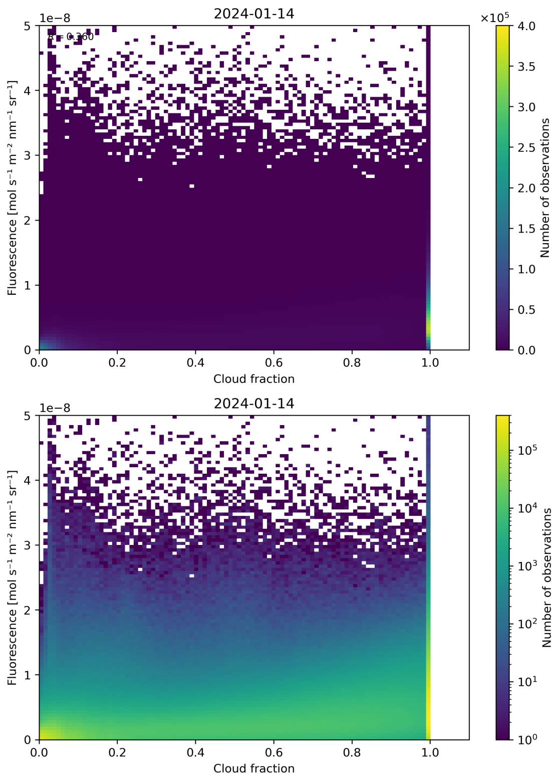
Figure 72: Scatter density plot of “Cloud fraction” against “Fluorescence” for 2024-01-13 to 2024-01-15.
