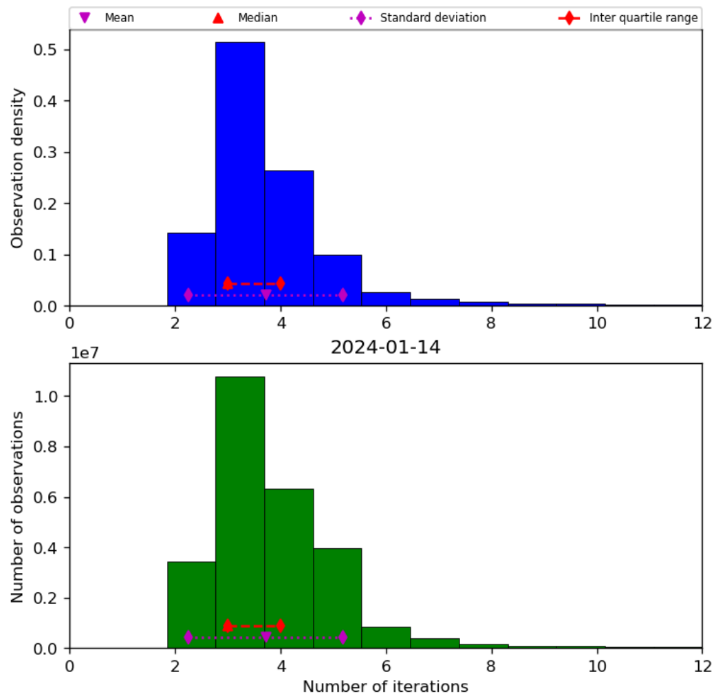
Figure 39: Histogram of “Number of iterations” for 2024-01-13 to 2024-01-15
