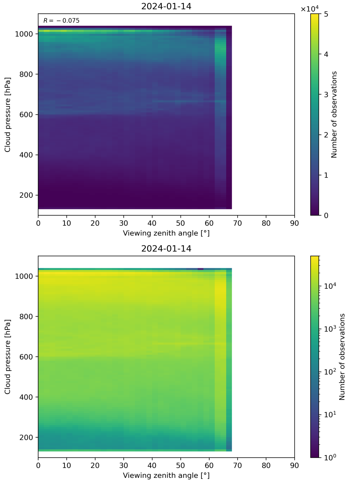
Figure 121: Scatter density plot of “Viewing zenith angle” against “Cloud pressure” for 2024-01-13 to 2024-01-15.
