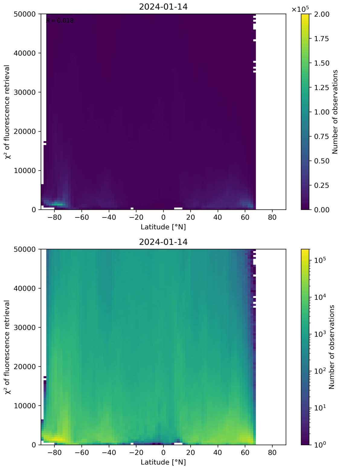
Figure 89: Scatter density plot of “Latitude” against “ \chi^2 of fluorescence retrieval” for 2024-01-13 to 2024-01-15.
