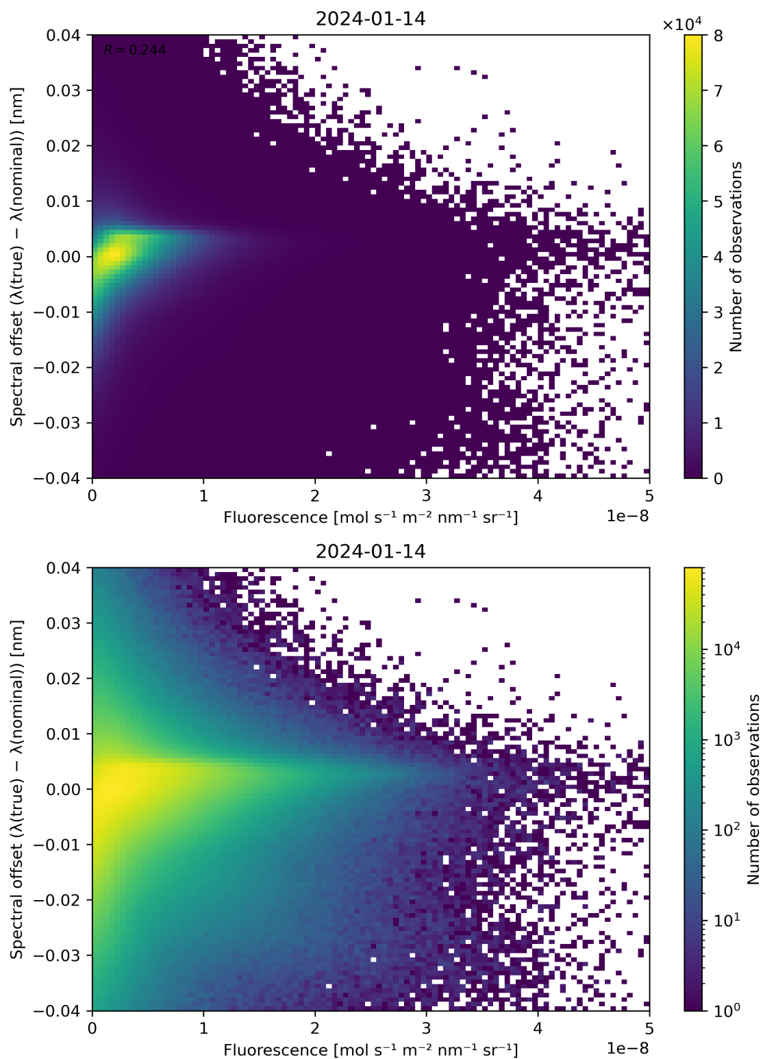
Figure 87: Scatter density plot of “Fluorescence” against “Spectral offset ( \lambda(\text{true}) - \lambda(\text{nominal}) )” for 2024-01-13 to 2024-01-15.
