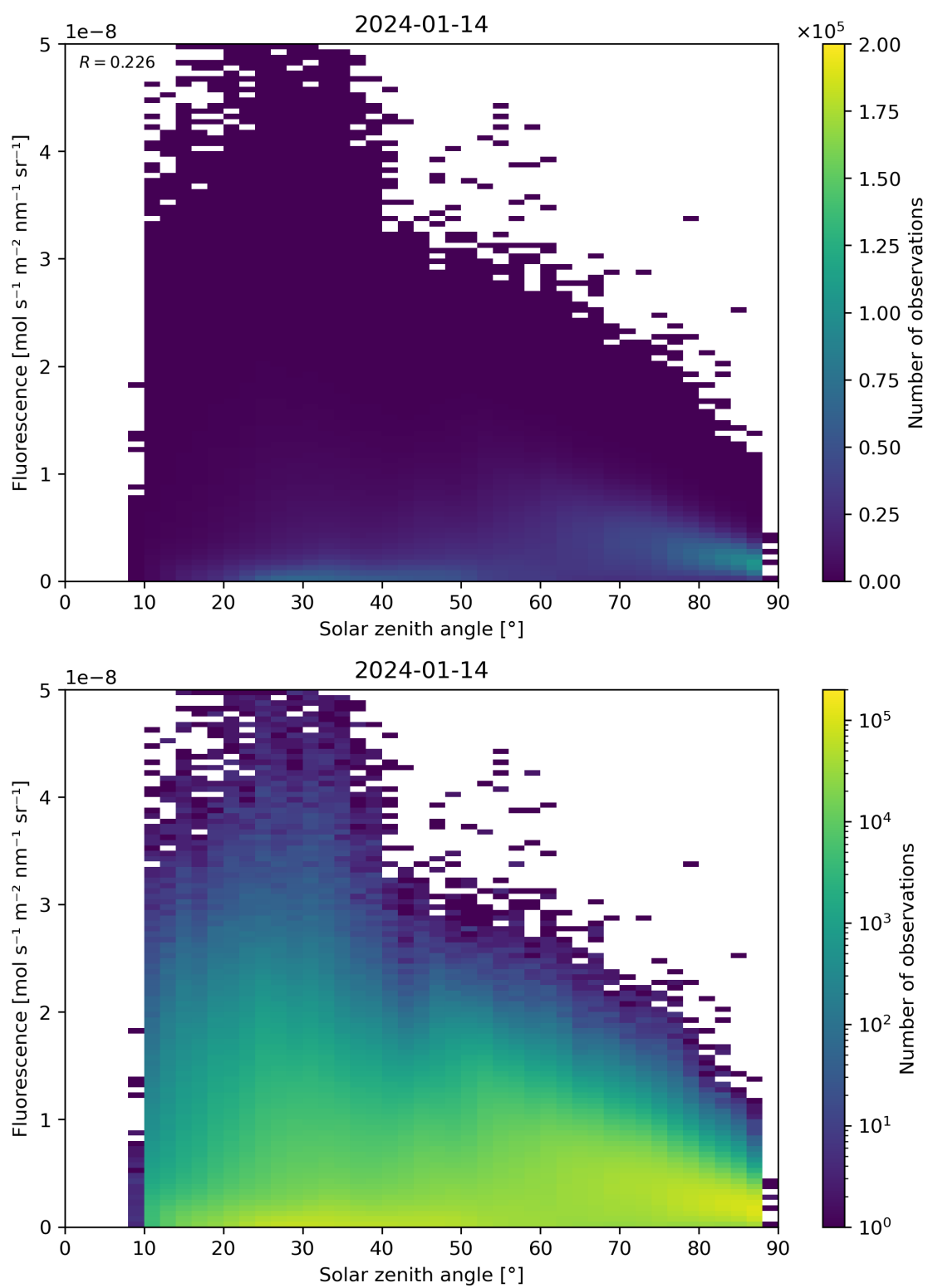
Figure 112: Scatter density plot of “Solar zenith angle” against “Fluorescence” for 2024-01-13 to 2024-01-15.
