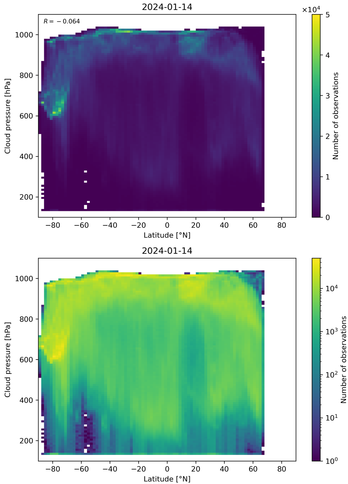
Figure 91: Scatter density plot of “Latitude” against “Cloud pressure” for 2024-01-13 to 2024-01-15.
