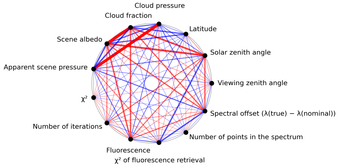
Figure 1: Map of correlation graph for 2024-01-13 to 2024-01-15.
