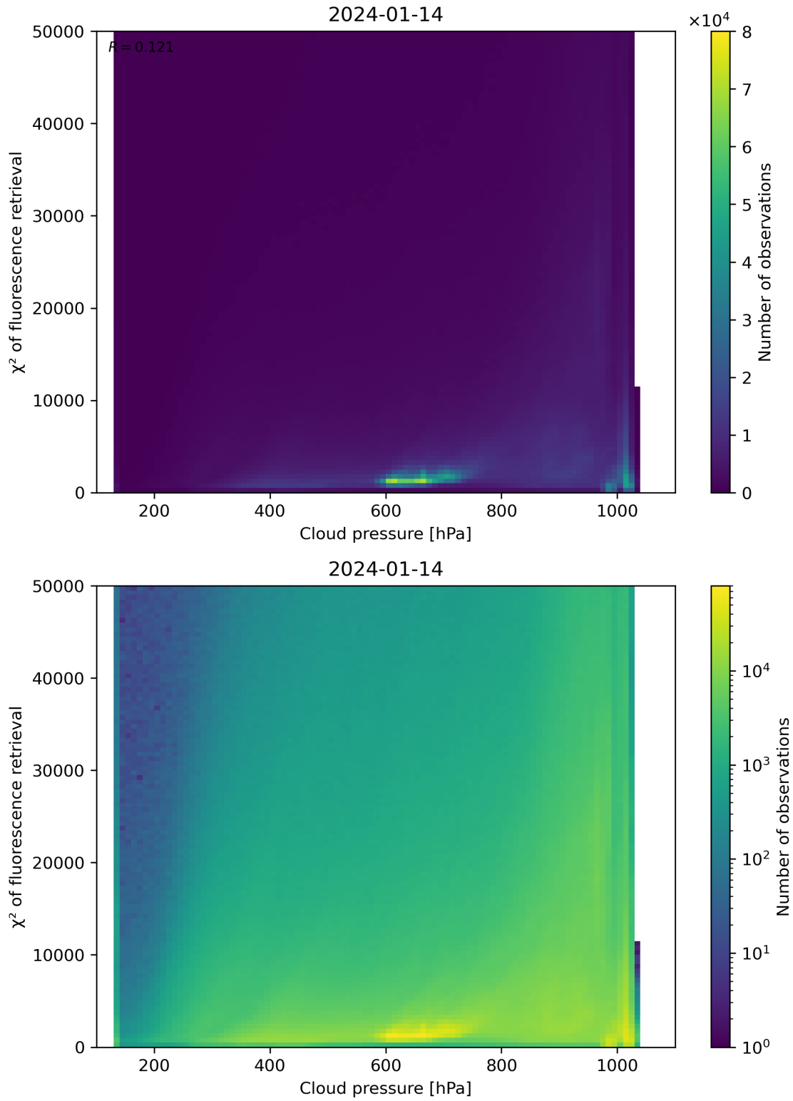
Figure 78: Scatter density plot of “Cloud pressure” against “ \chi^2 of fluorescence retrieval” for 2024-01-13 to 2024-01-15.
