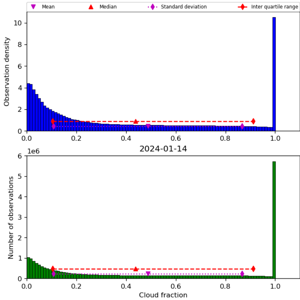
Figure 32: Histogram of “Cloud fraction” for 2024-01-13 to 2024-01-15
