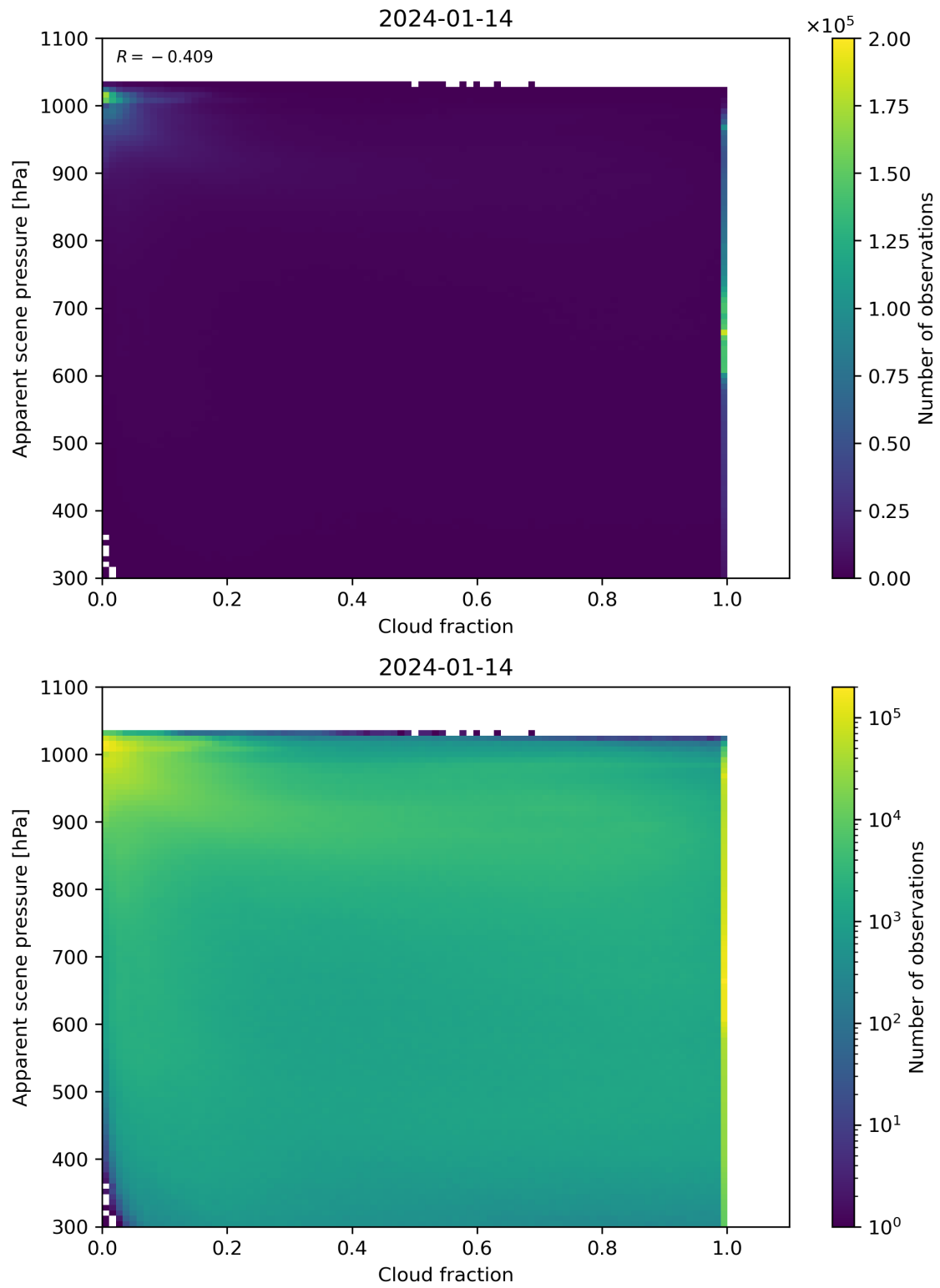
Figure 70: Scatter density plot of “Cloud fraction” against “Apparent scene pressure” for 2024-01-13 to 2024-01-15.
