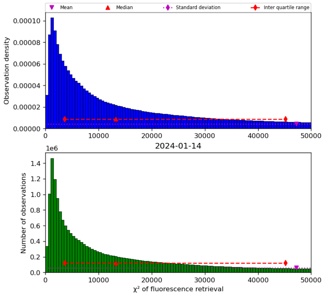
Figure 42: Histogram of “ \chi^2 of fluorescence retrieval” for 2024-01-13 to 2024-01-15
