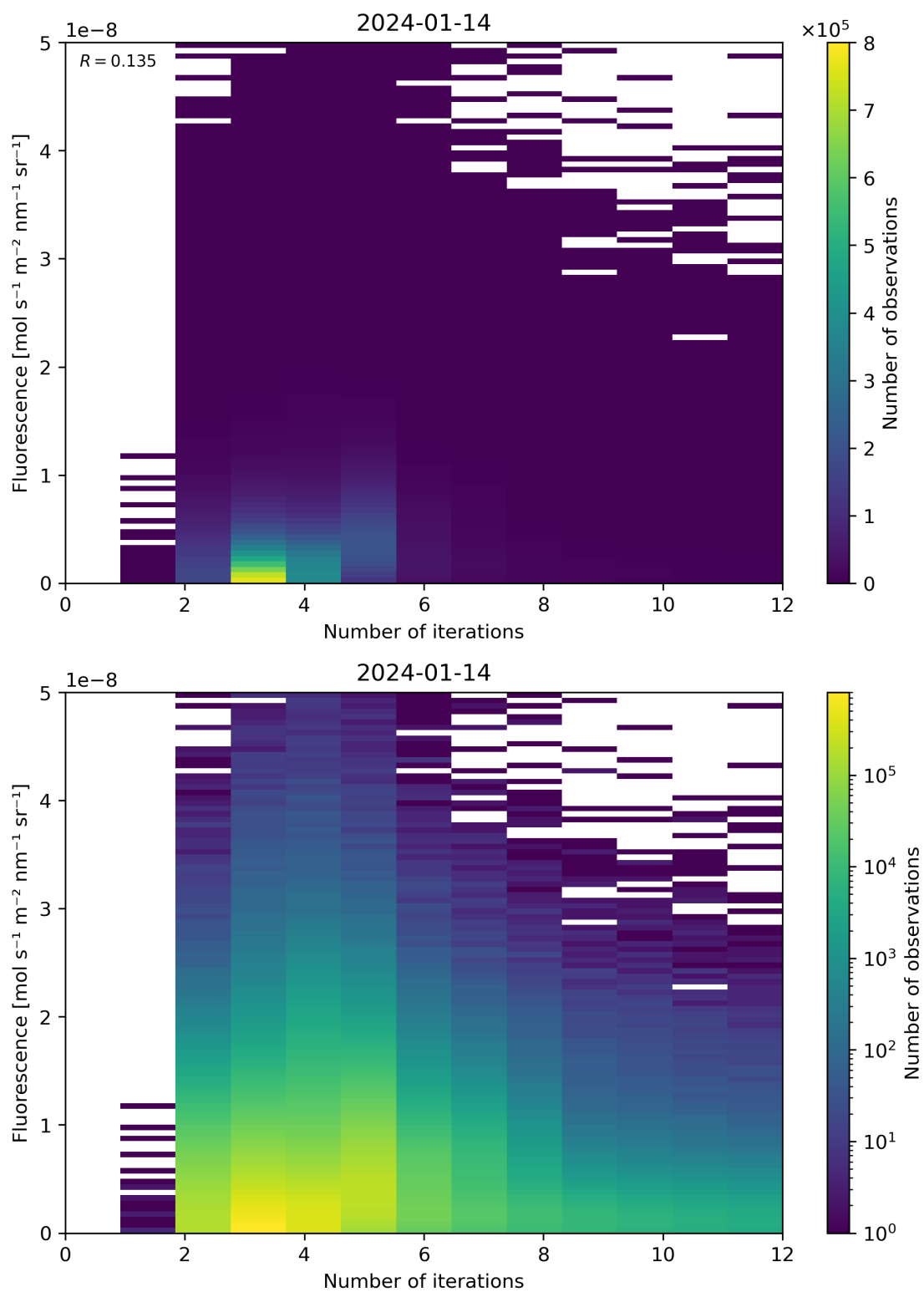
Figure 98: Scatter density plot of “Number of iterations” against “Fluorescence” for 2024-01-13 to 2024-01-15.
