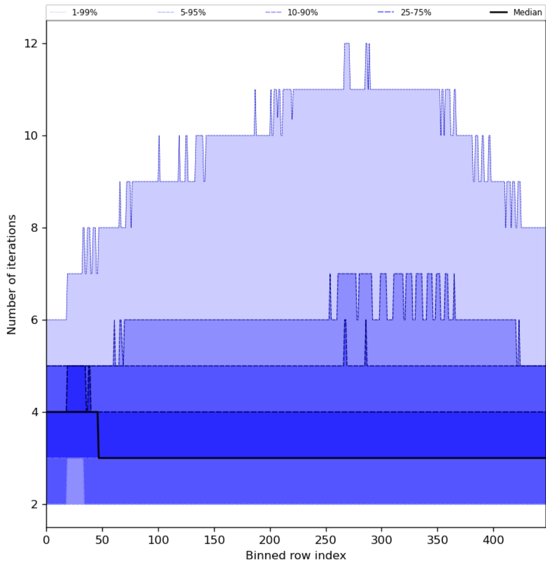
Figure 56: Along track statistics of “Number of iterations” for 2024-01-13 to 2024-01-15
