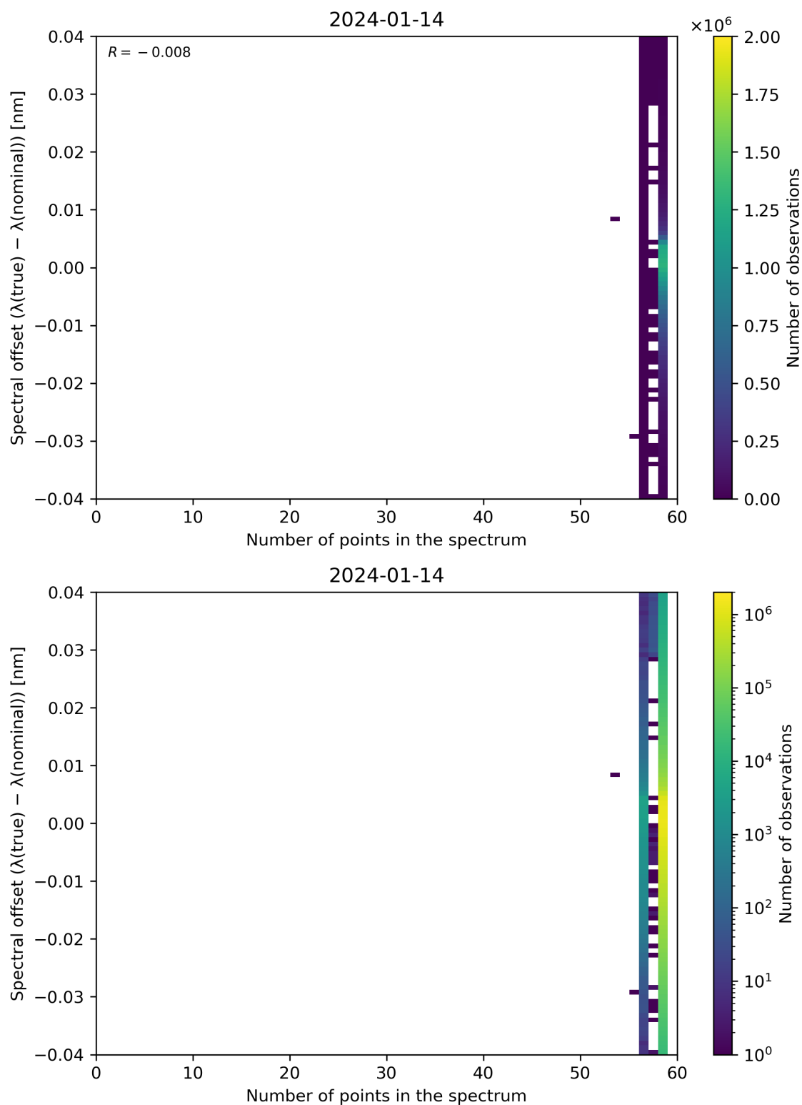
Figure 101: Scatter density plot of “Number of points in the spectrum” against “Spectral offset ( \lambda(\text{true}) - \lambda(\text{nominal}) )” for 2024-01-13 to 2024-01-15.
