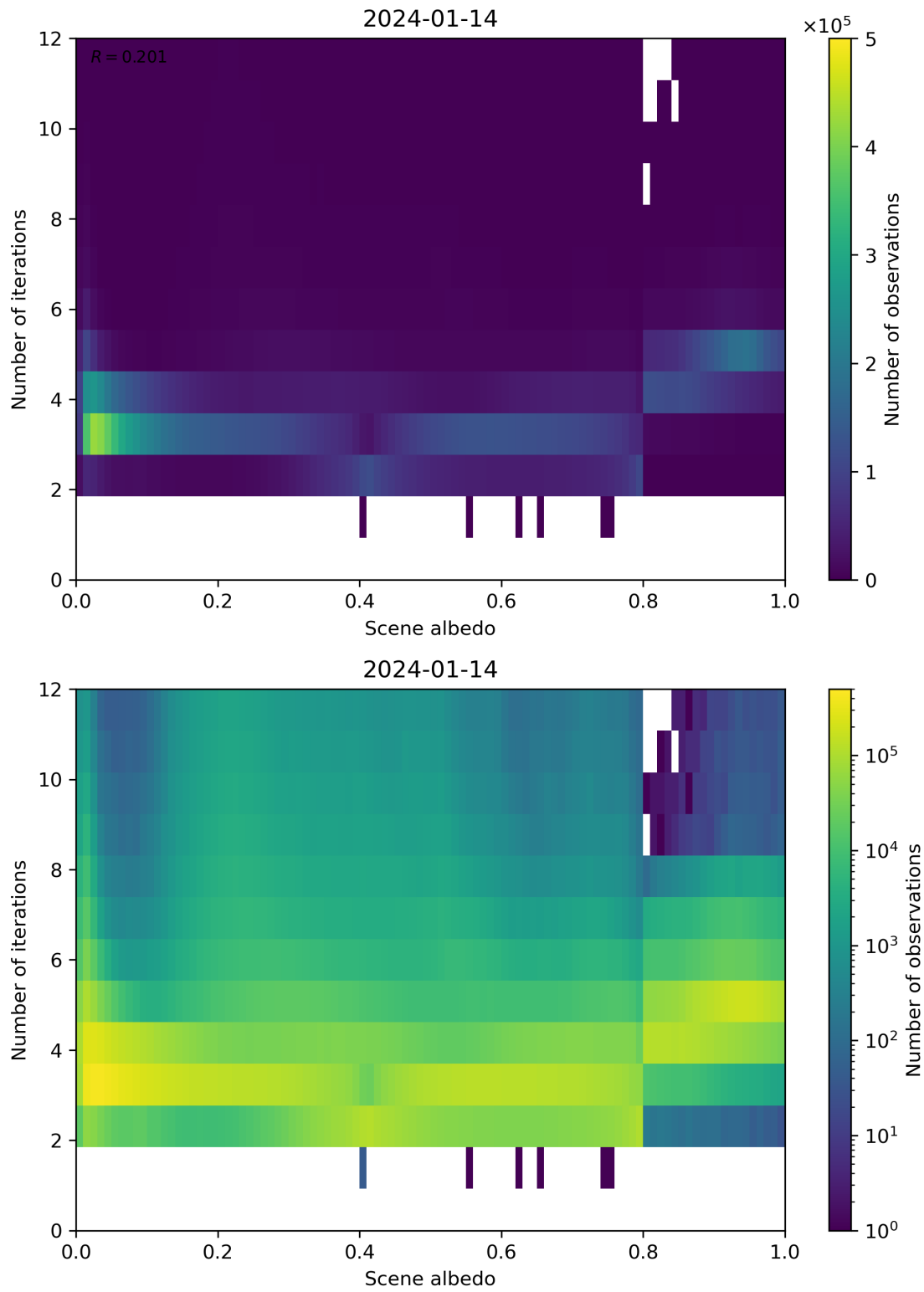
Figure 105: Scatter density plot of “Scene albedo” against “Number of iterations” for 2024-01-13 to 2024-01-15.
