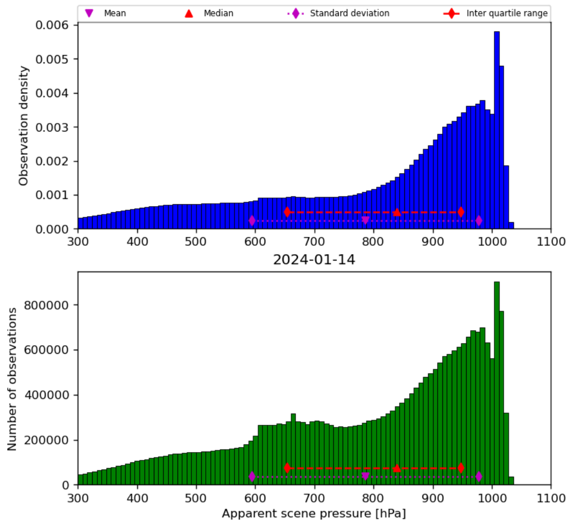
Figure 36: Histogram of “Apparent scene pressure” for 2024-01-13 to 2024-01-15
