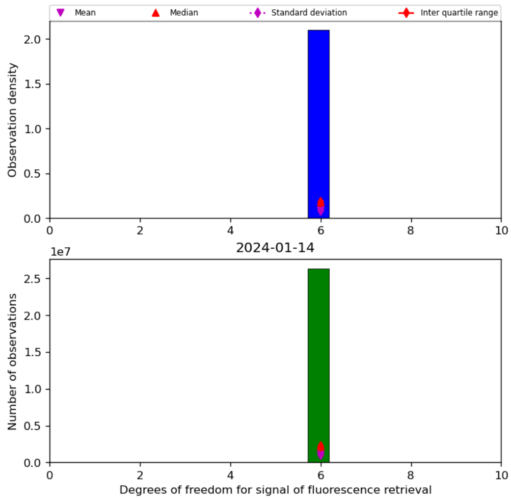
Figure 43: Histogram of “Degrees of freedom for signal of fluorescence retrieval” for 2024-01-13 to 2024-01-15
