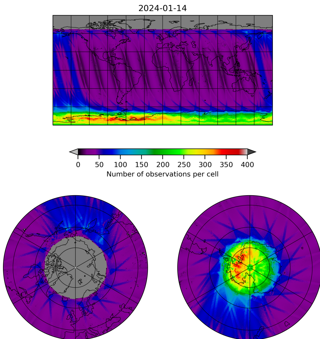
Figure 11: Map of the number of observations for 2024-01-13 to 2024-01-15
