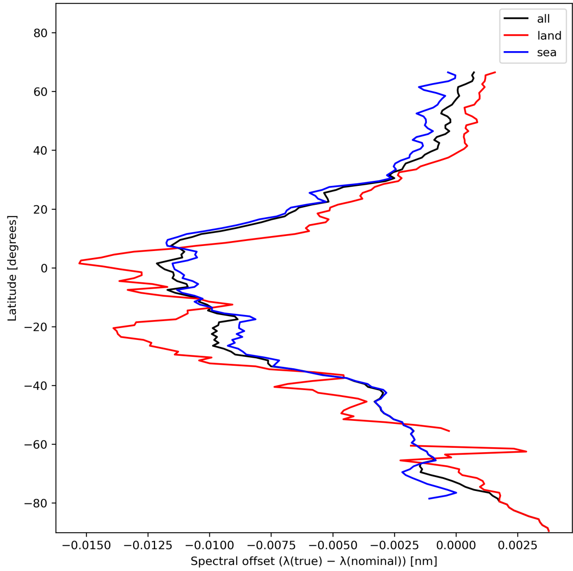
Figure 28: Zonal average of “Spectral offset ( \lambda(\text{true}) - \lambda(\text{nominal}) )” for 2024-01-13 to 2024-01-15.
