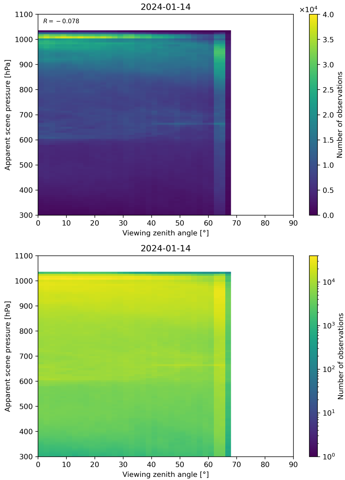
Figure 118: Scatter density plot of “Viewing zenith angle” against “Apparent scene pressure” for 2024-01-13 to 2024-01-15.
