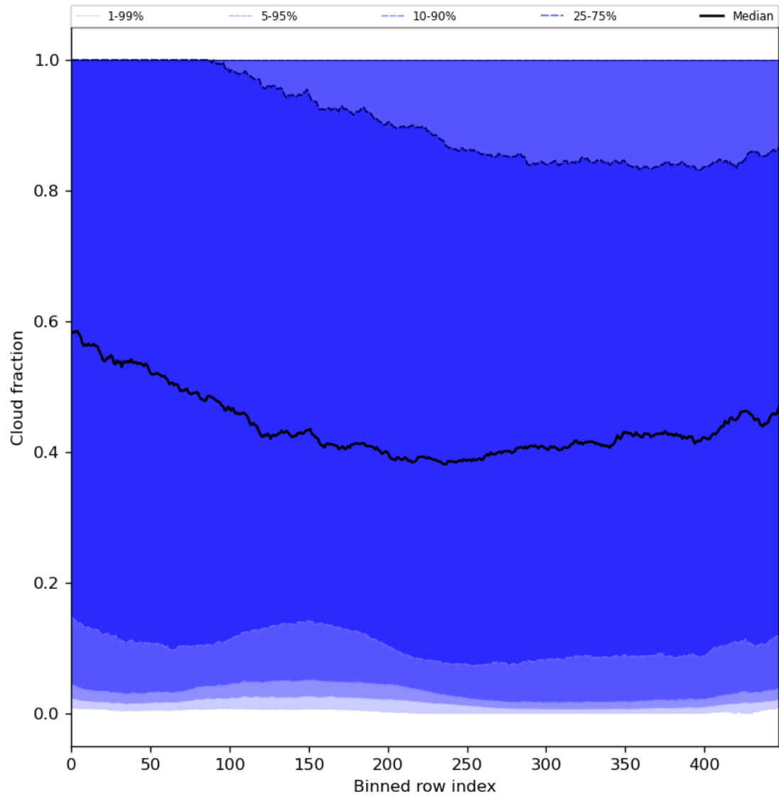
Figure 49: Along track statistics of “Cloud fraction” for 2024-01-13 to 2024-01-15
