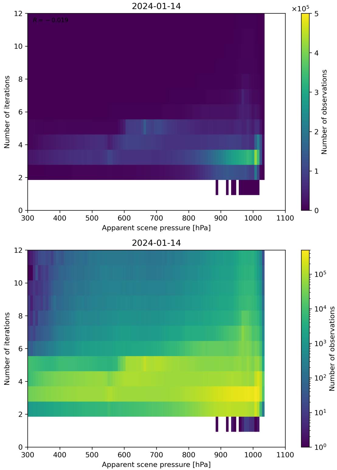
Figure 65: Scatter density plot of “Apparent scene pressure” against “Number of iterations” for 2024-01-13 to 2024-01-15.
