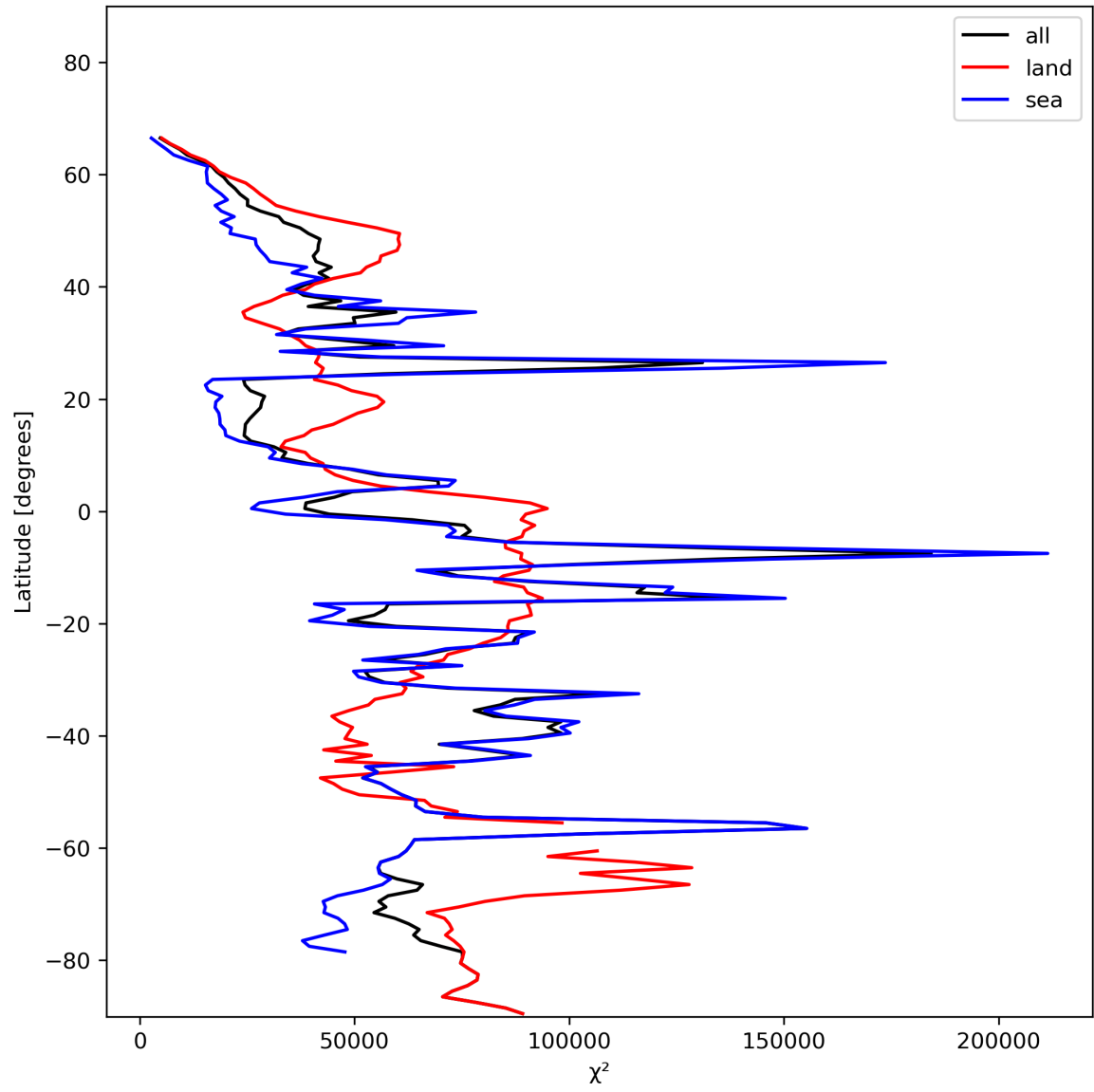
Figure 21: Zonal average of “ \chi^2 ” for 2024-01-13 to 2024-01-15.
