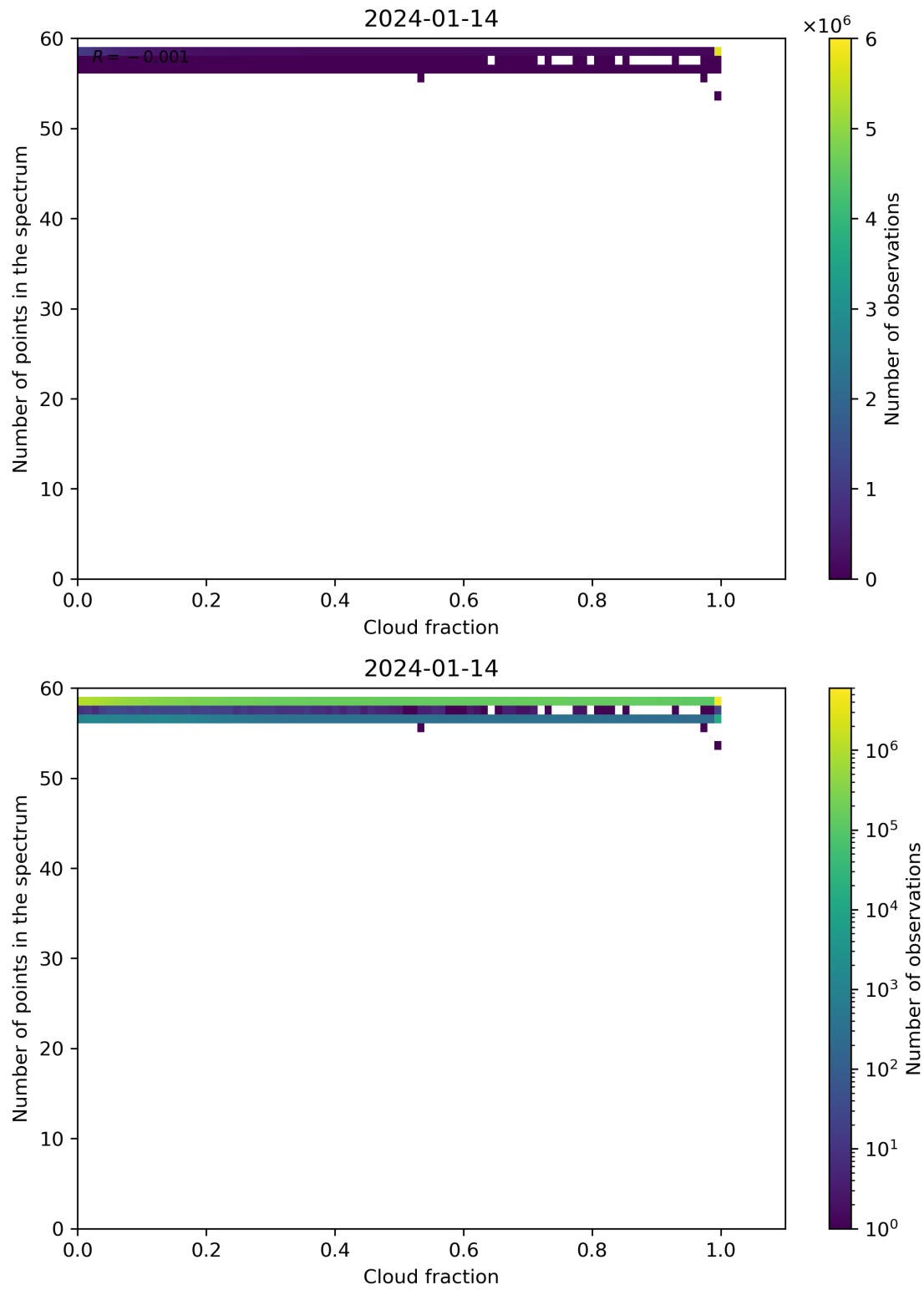
Figure 74: Scatter density plot of “Cloud fraction” against “Number of points in the spectrum” for 2024-01-13 to 2024-01-15.
