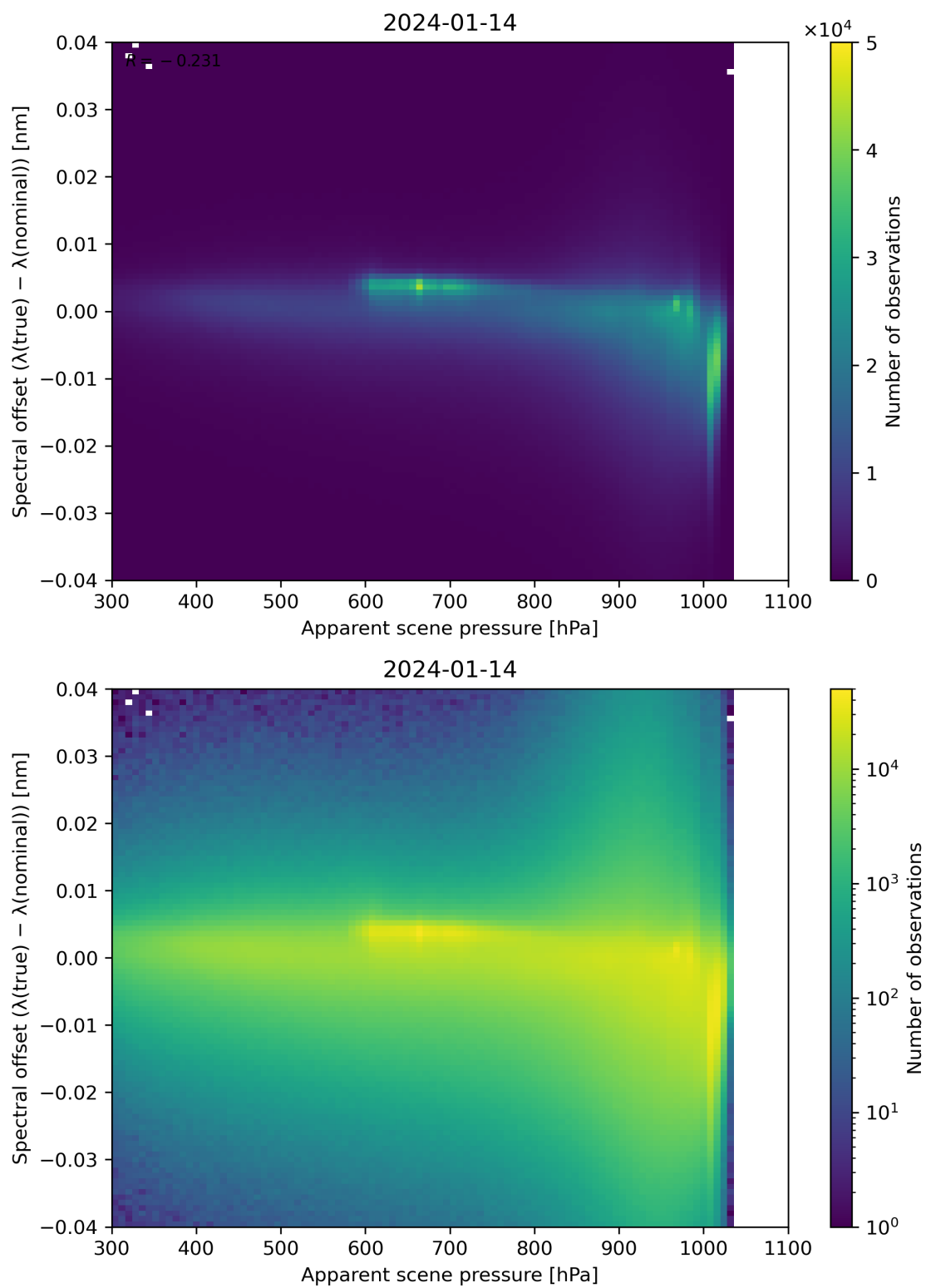
Figure 67: Scatter density plot of “Apparent scene pressure” against “Spectral offset ( \lambda(\text{true}) - \lambda(\text{nominal}) )” for 2024-01-13 to 2024-01-15.
