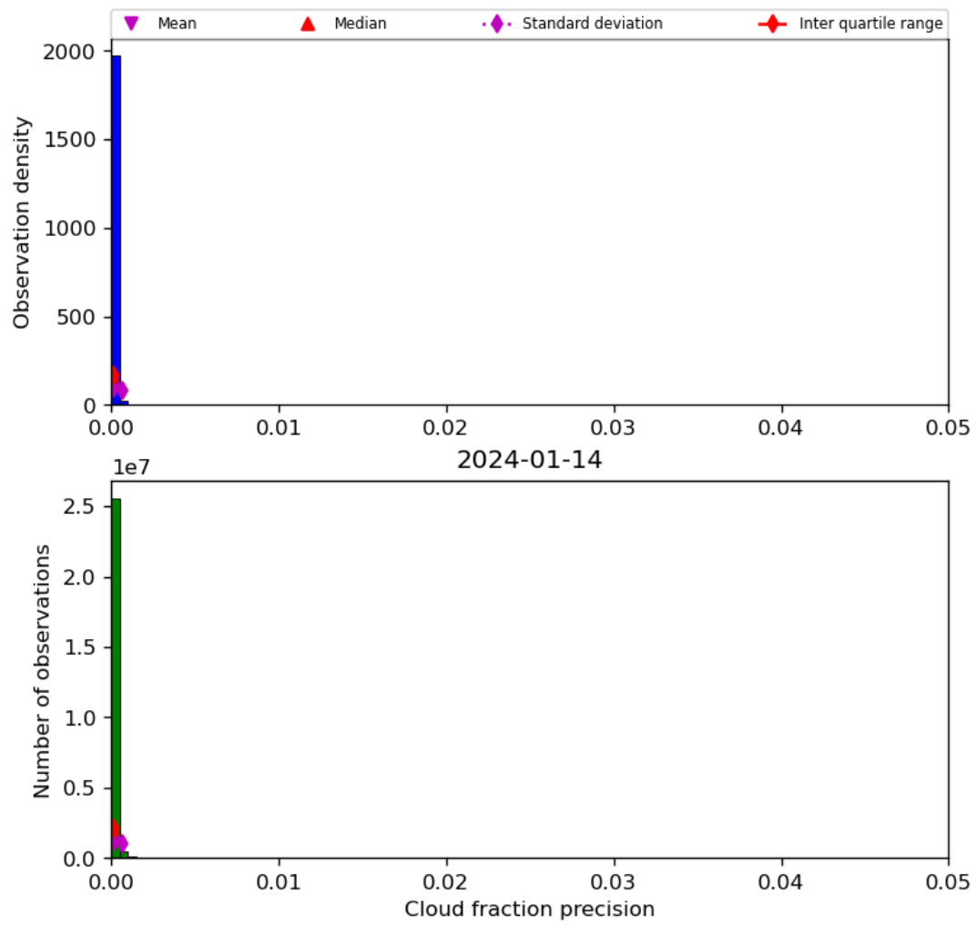
Figure 33: Histogram of “Cloud fraction precision” for 2024-01-13 to 2024-01-15
