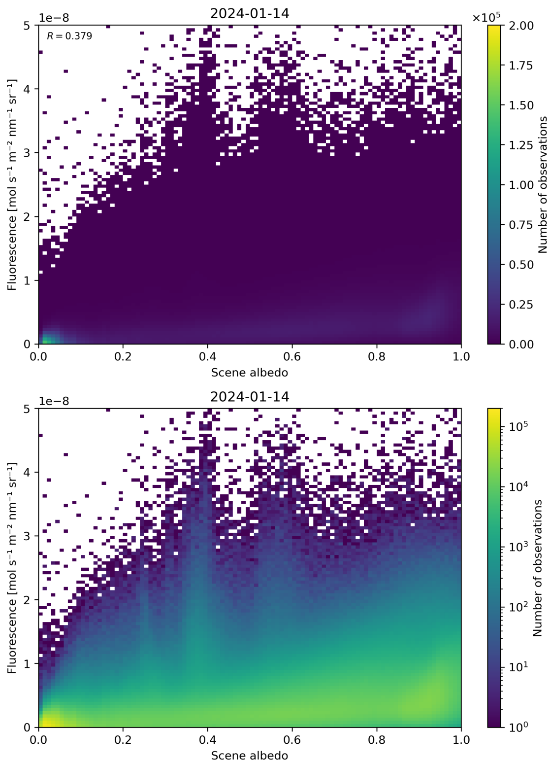
Figure 104: Scatter density plot of “Scene albedo” against “Fluorescence” for 2024-01-13 to 2024-01-15.
