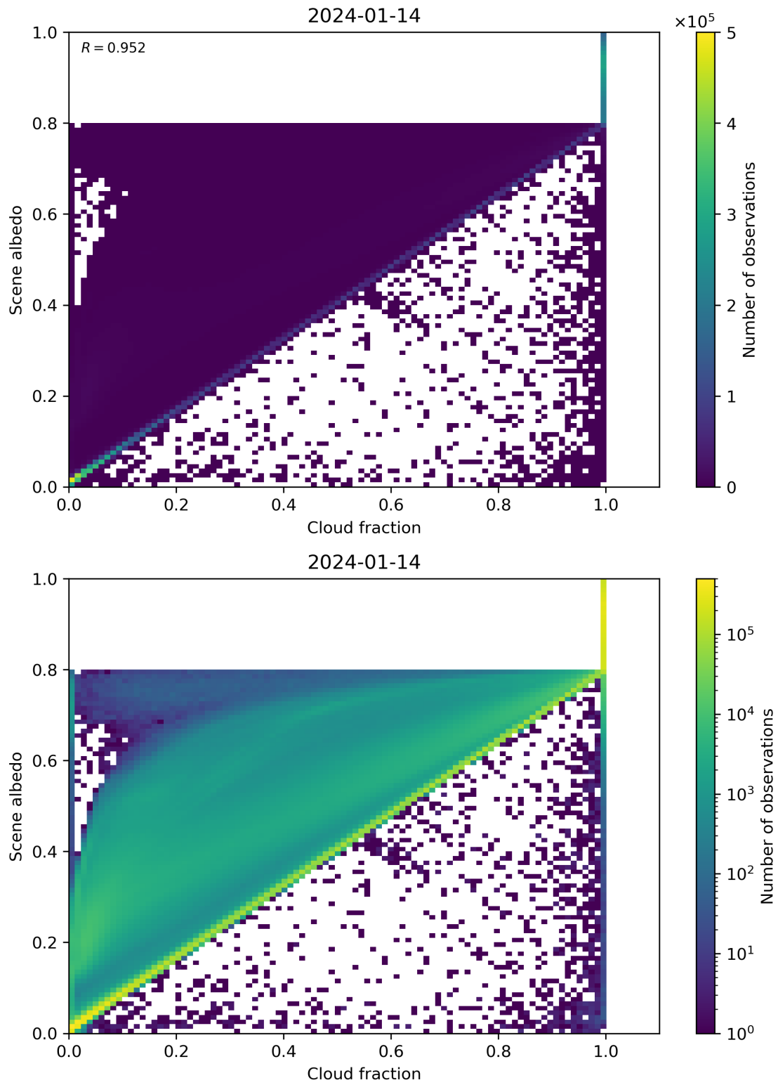
Figure 75: Scatter density plot of “Cloud fraction” against “Scene albedo” for 2024-01-13 to 2024-01-15.
