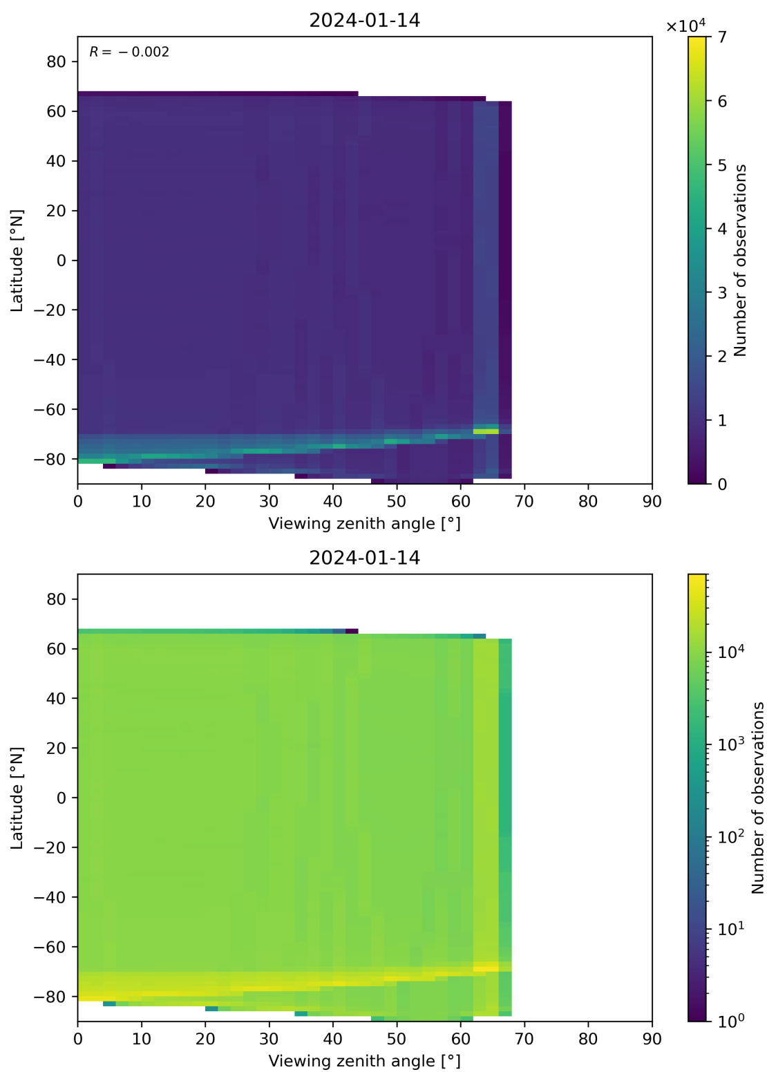
Figure 123: Scatter density plot of “Viewing zenith angle” against “Latitude” for 2024-01-13 to 2024-01-15.
