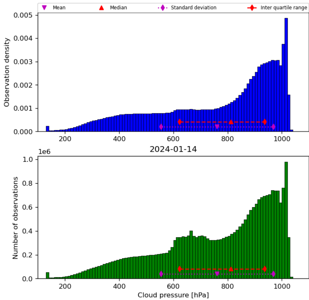
Figure 30: Histogram of “Cloud pressure” for 2024-01-13 to 2024-01-15
