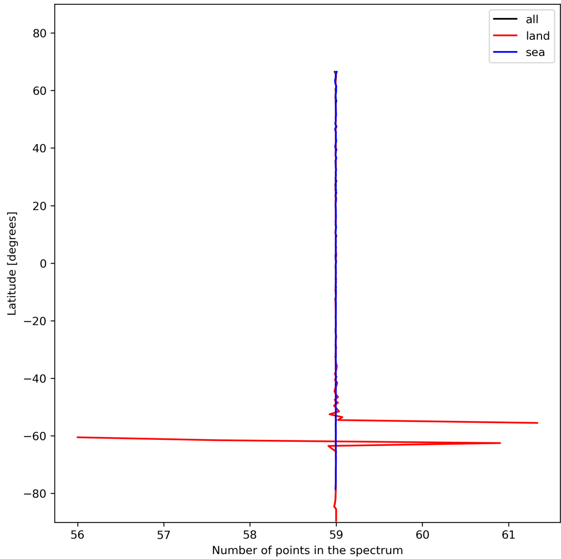
Figure 27: Zonal average of “Number of points in the spectrum” for 2024-01-13 to 2024-01-15.
