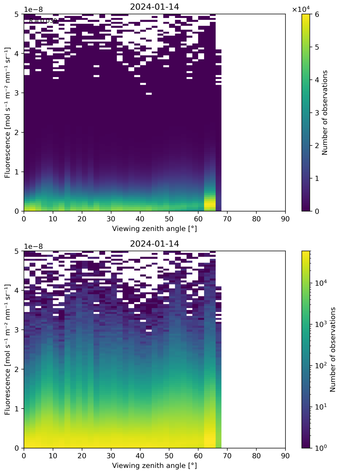
Figure 122: Scatter density plot of “Viewing zenith angle” against “Fluorescence” for 2024-01-13 to 2024-01-15.
