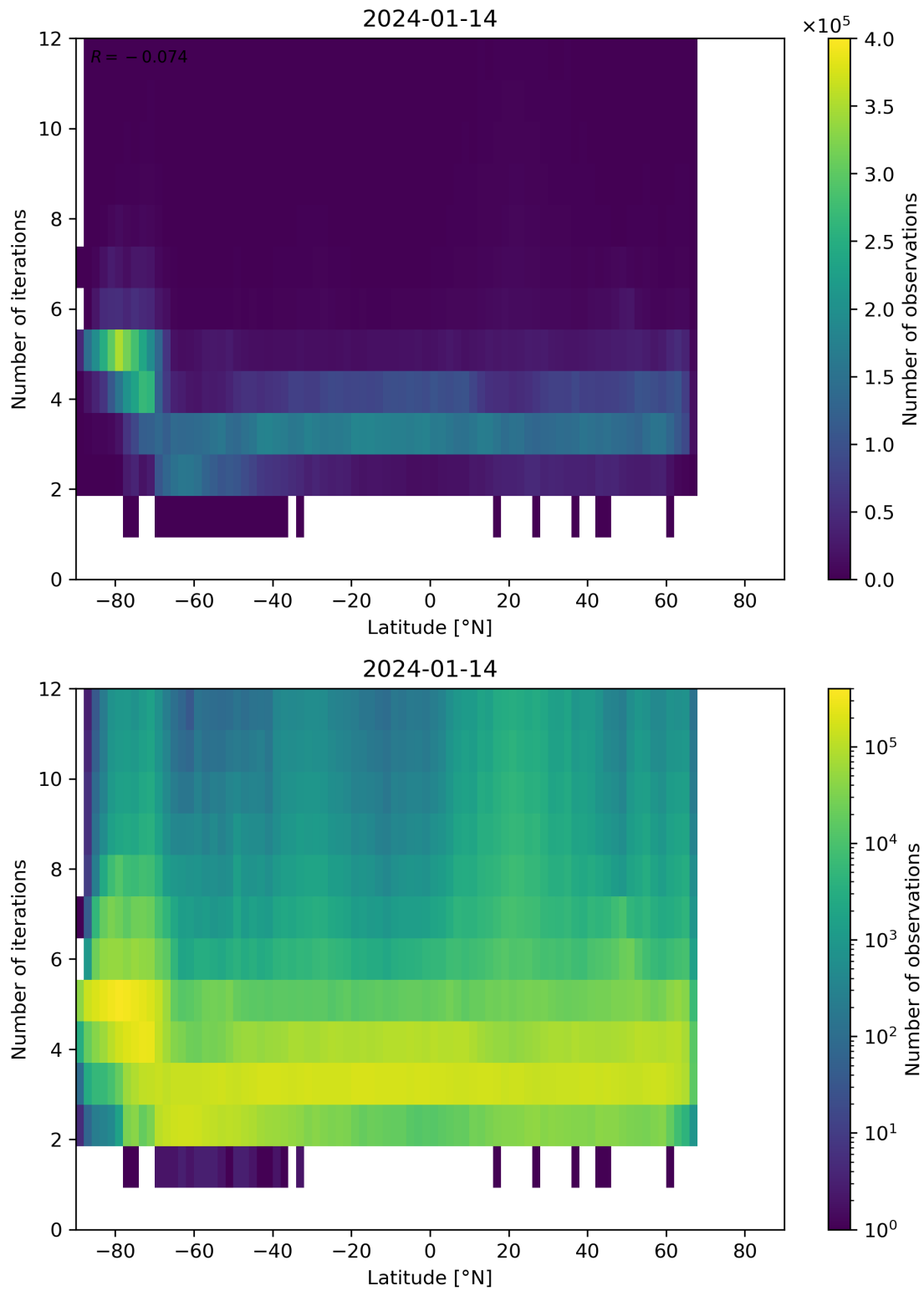
Figure 93: Scatter density plot of “Latitude” against “Number of iterations” for 2024-01-13 to 2024-01-15.
