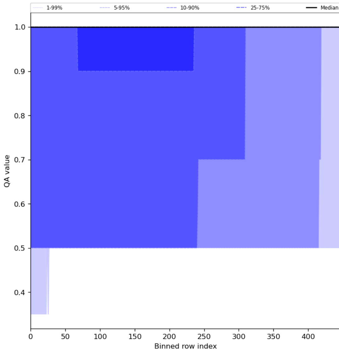
Figure 46: Along track statistics of “QA value” for 2024-01-13 to 2024-01-15
