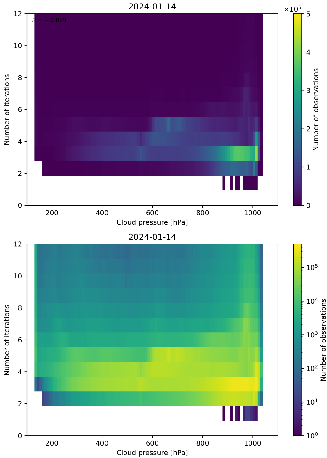
Figure 81: Scatter density plot of “Cloud pressure” against “Number of iterations” for 2024-01-13 to 2024-01-15.
