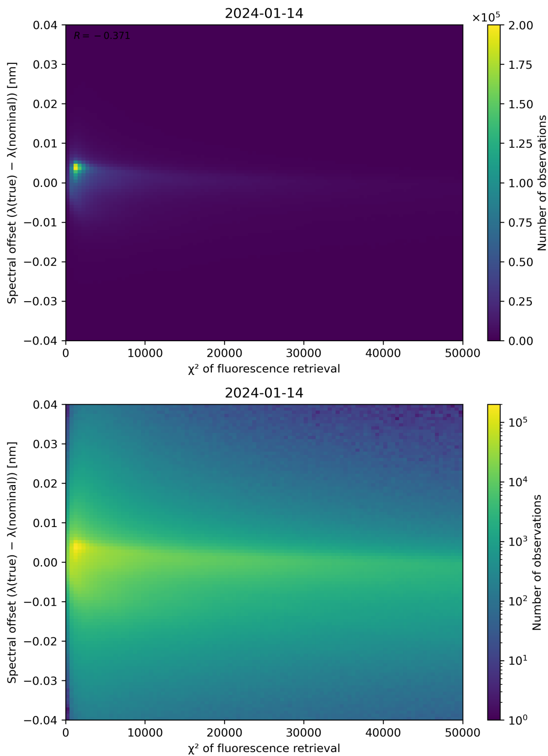
Figure 69: Scatter density plot of " \chi^2 of fluorescence retrieval" against "Spectral offset ( \lambda(\text{true}) - \lambda(\text{nominal}) )" for 2024-01-13 to 2024-01-15.
