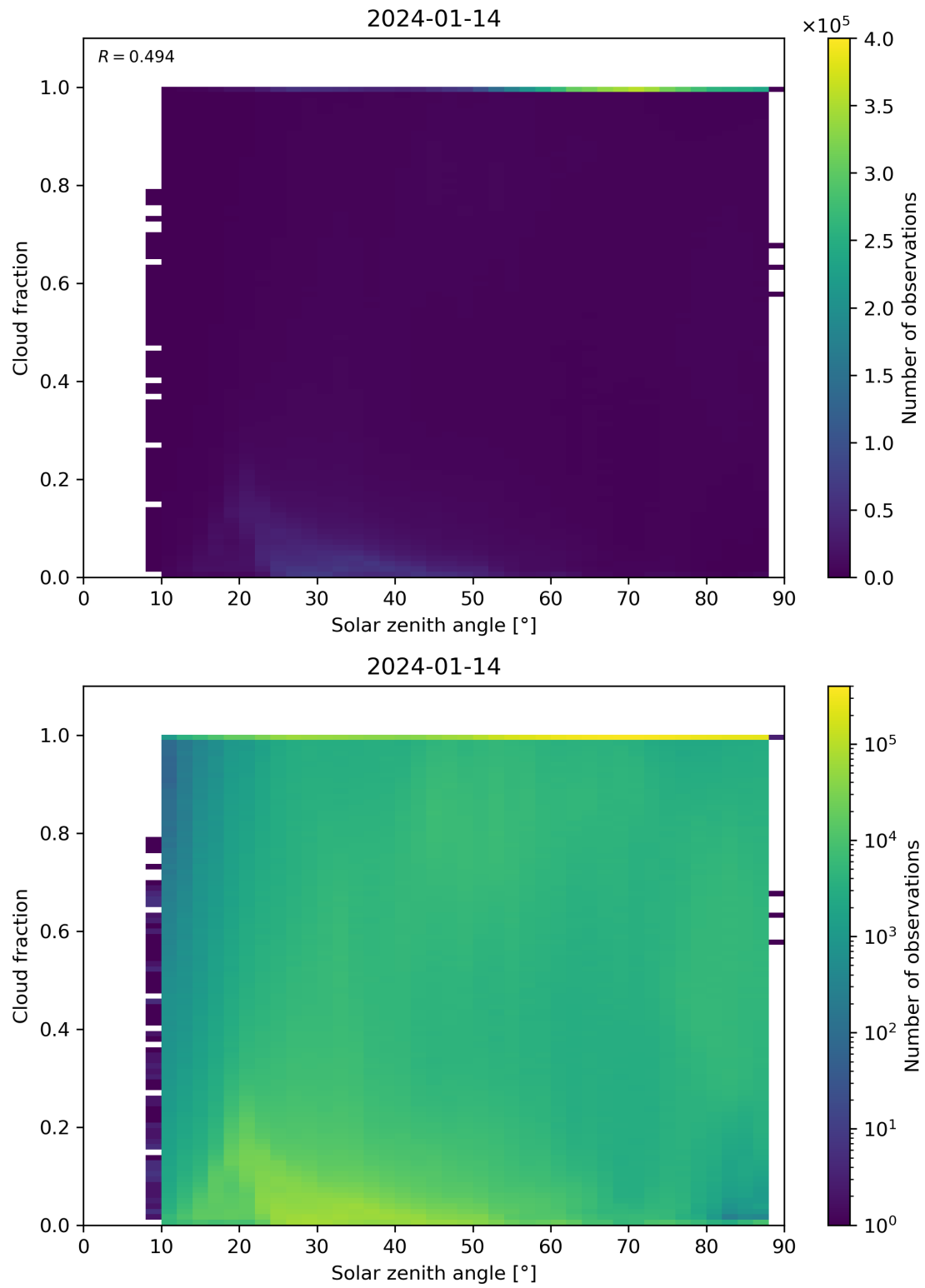
Figure 110: Scatter density plot of “Solar zenith angle” against “Cloud fraction” for 2024-01-13 to 2024-01-15.
