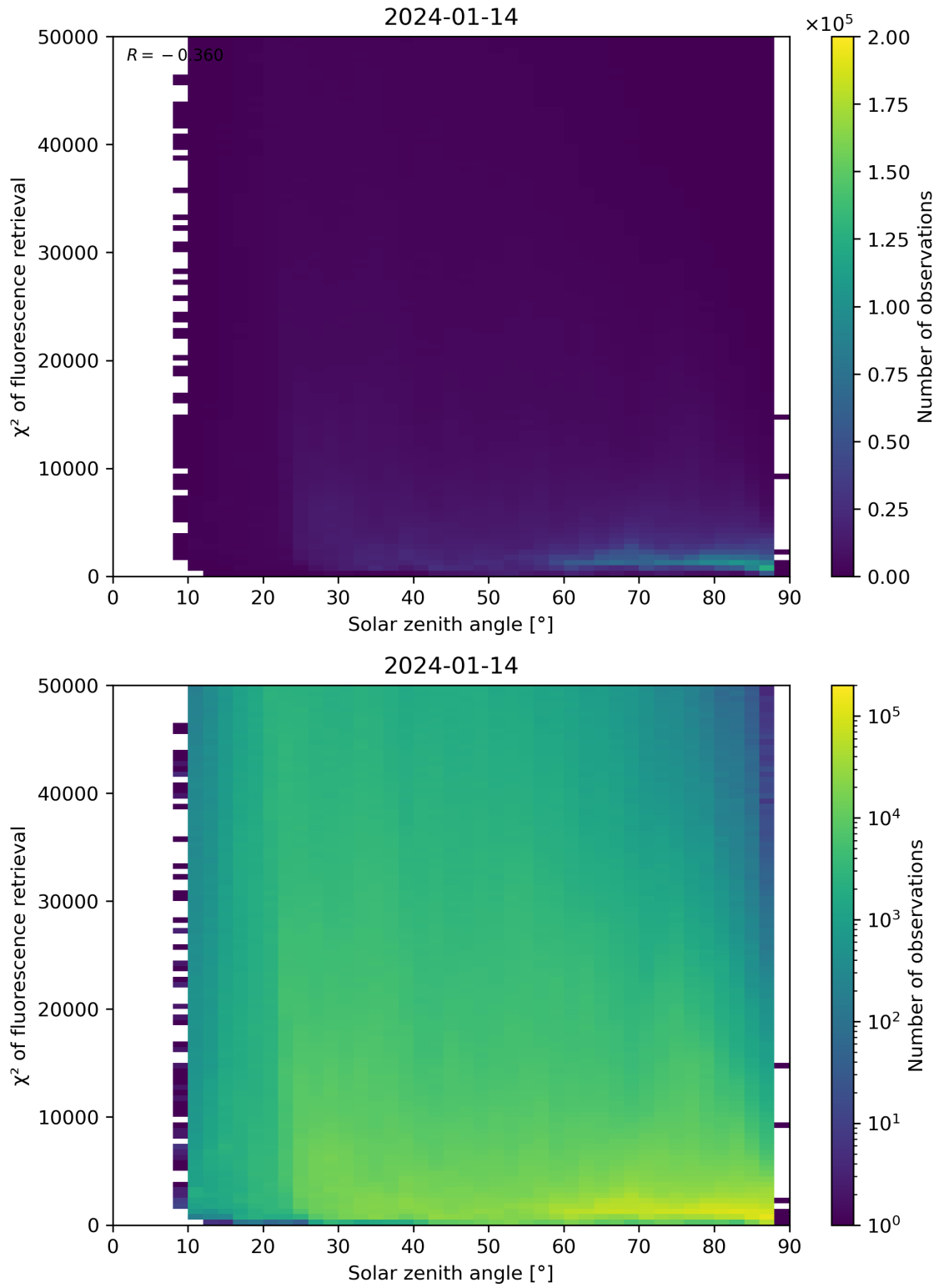
Figure 109: Scatter density plot of “Solar zenith angle” against “ \chi^2 of fluorescence retrieval” for 2024-01-13 to 2024-01-15.
