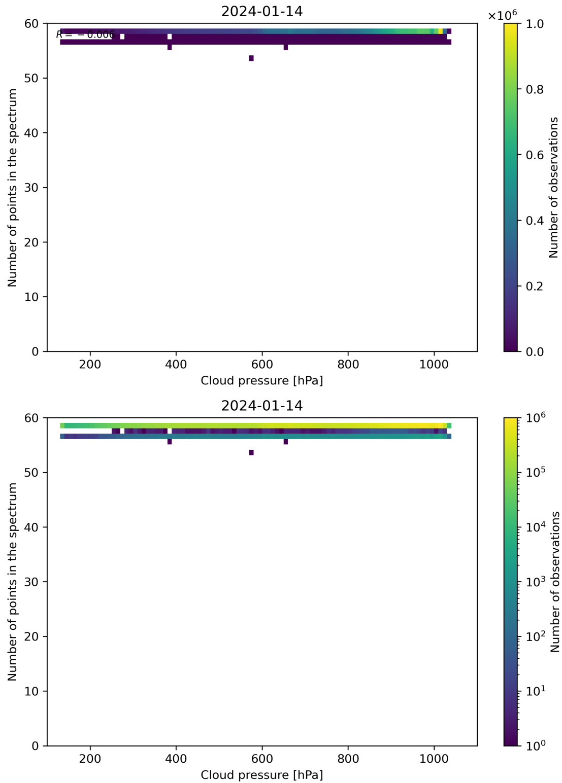
Figure 82: Scatter density plot of “Cloud pressure” against “Number of points in the spectrum” for 2024-01-13 to 2024-01-15.
