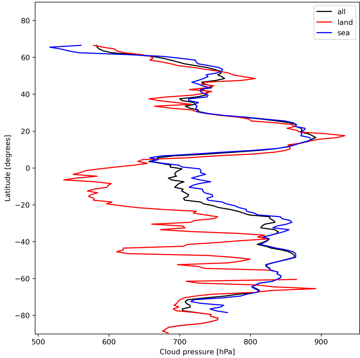
Figure 13: Zonal average of “Cloud pressure” for 2024-01-13 to 2024-01-15.
