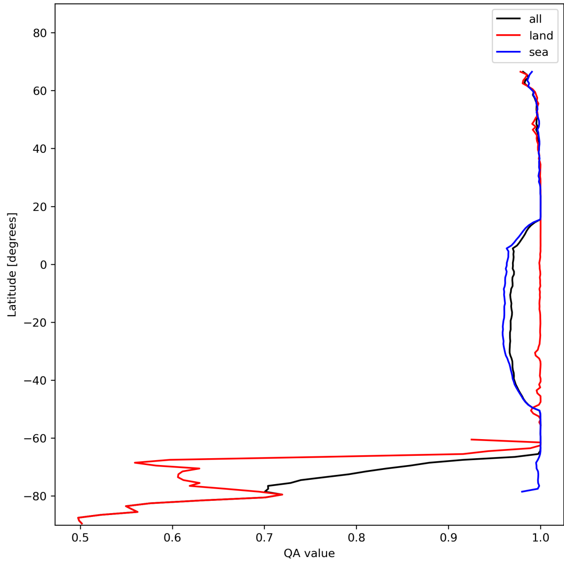
Figure 12: Zonal average of “QA value” for 2024-01-13 to 2024-01-15.
