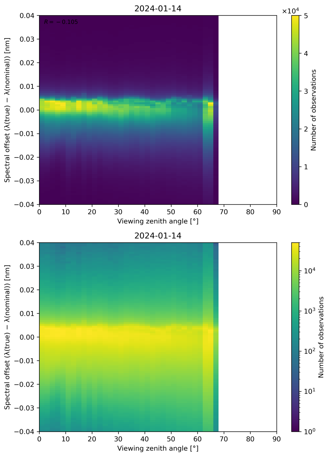
Figure 128: Scatter density plot of “Viewing zenith angle” against “Spectral offset ( \lambda(\text{true}) - \lambda(\text{nominal}) )” for 2024-01-13 to 2024-01-15.
