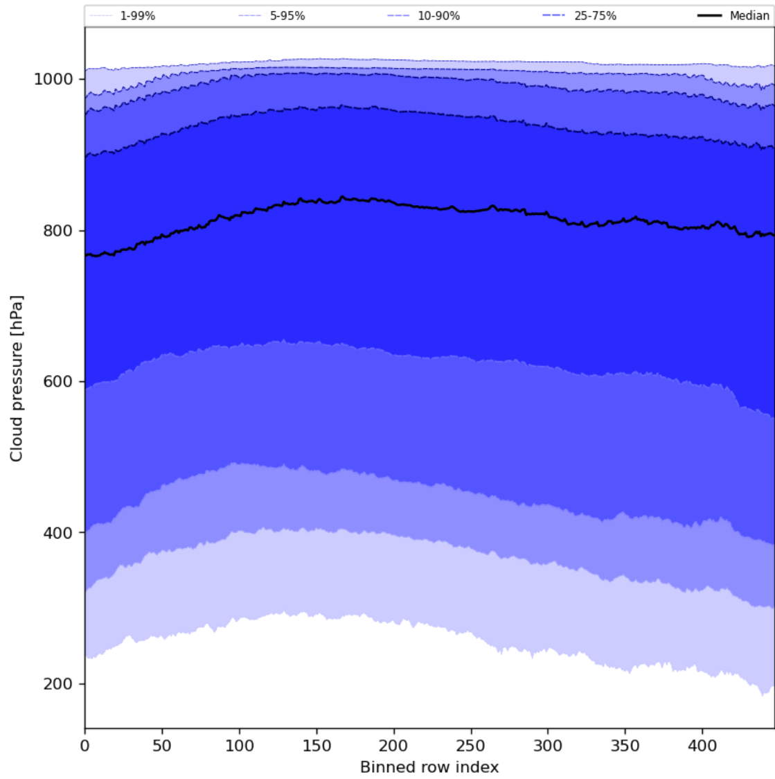
Figure 47: Along track statistics of “Cloud pressure” for 2024-01-13 to 2024-01-15
