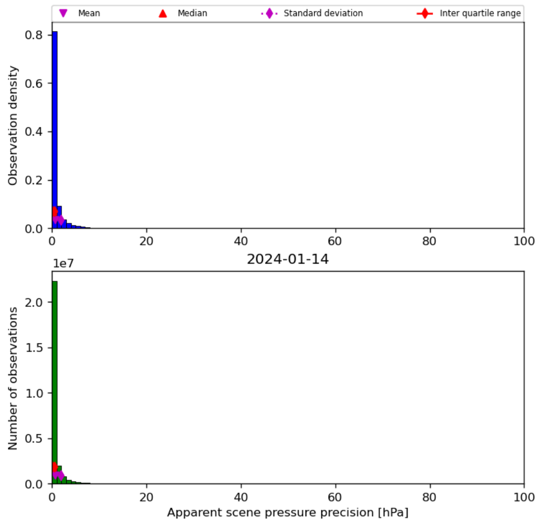
Figure 37: Histogram of "Apparent scene pressure precision" for 2024-01-13 to 2024-01-15
