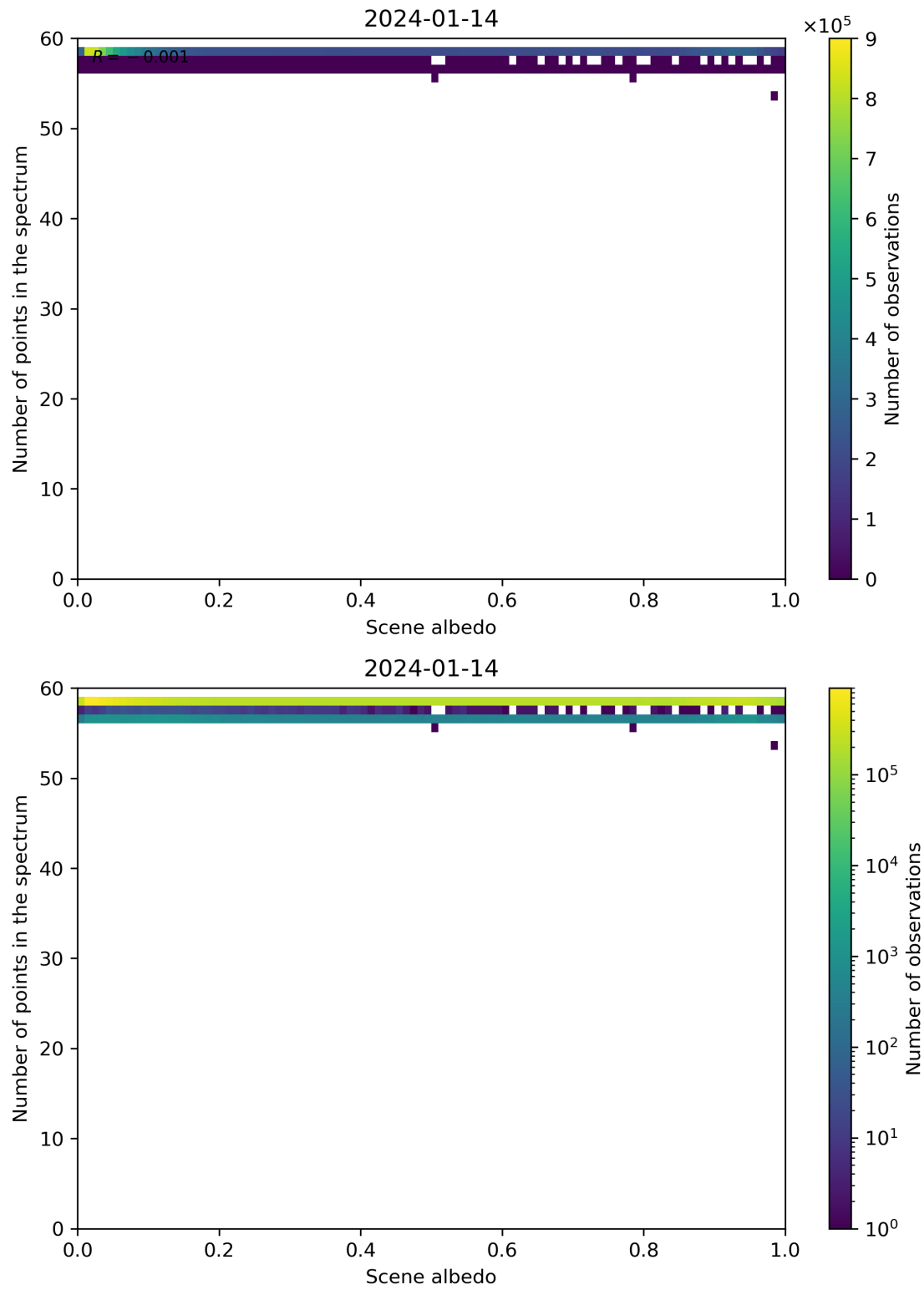
Figure 106: Scatter density plot of “Scene albedo” against “Number of points in the spectrum” for 2024-01-13 to 2024-01-15.
