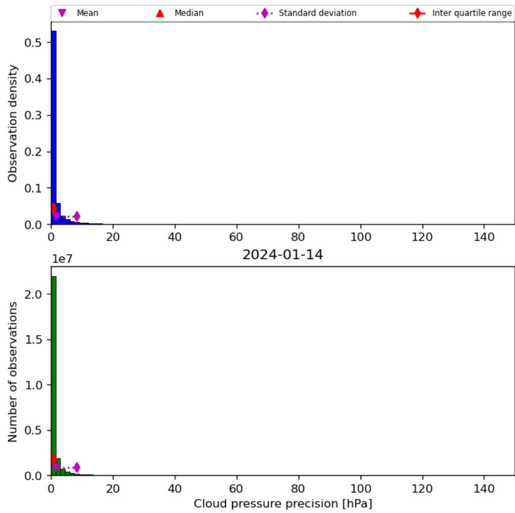
Figure 31: Histogram of “Cloud pressure precision” for 2024-01-13 to 2024-01-15
