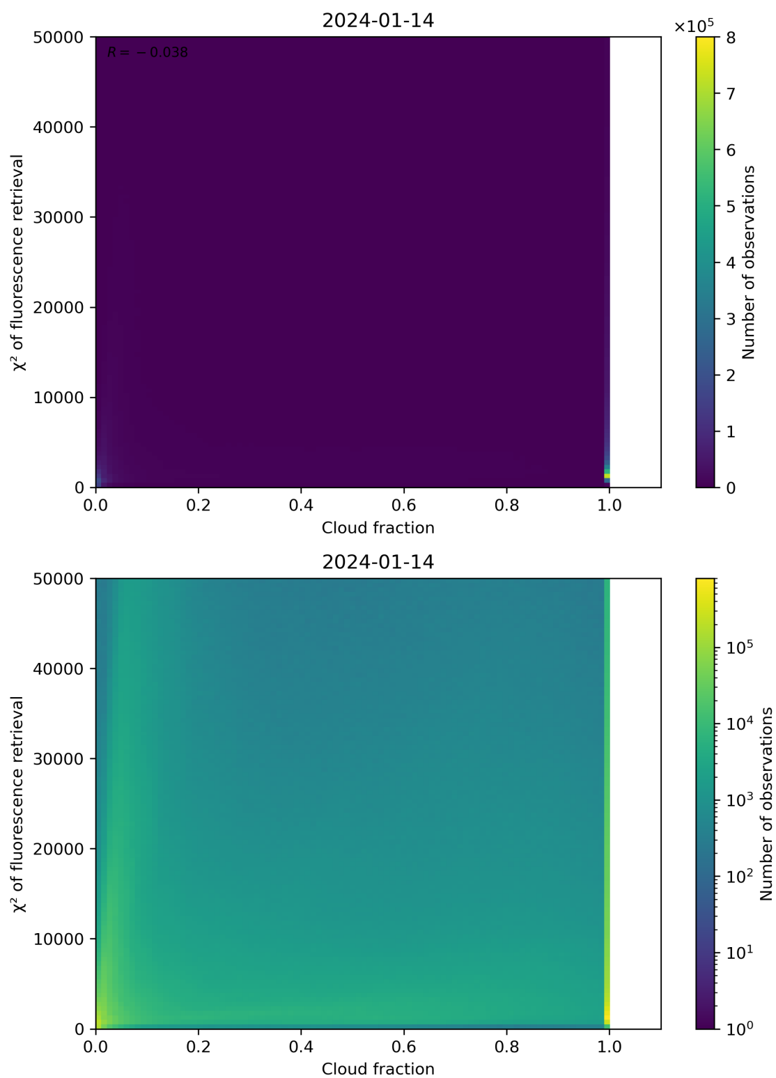
Figure 71: Scatter density plot of “Cloud fraction” against “ \chi^2 of fluorescence retrieval” for 2024-01-13 to 2024-01-15.
