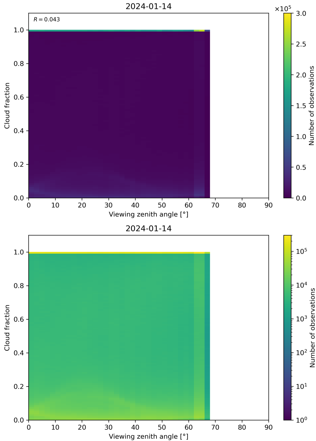
Figure 120: Scatter density plot of “Viewing zenith angle” against “Cloud fraction” for 2024-01-13 to 2024-01-15.
