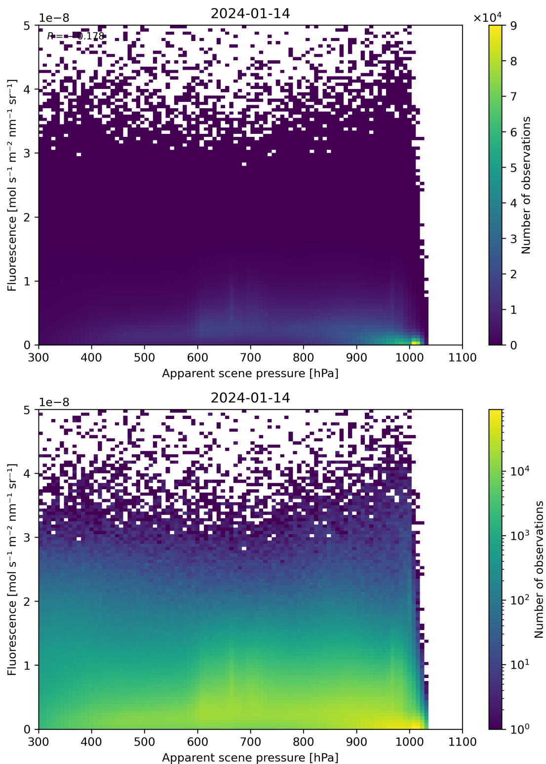
Figure 64: Scatter density plot of “Apparent scene pressure” against “Fluorescence” for 2024-01-13 to 2024-01-15.
