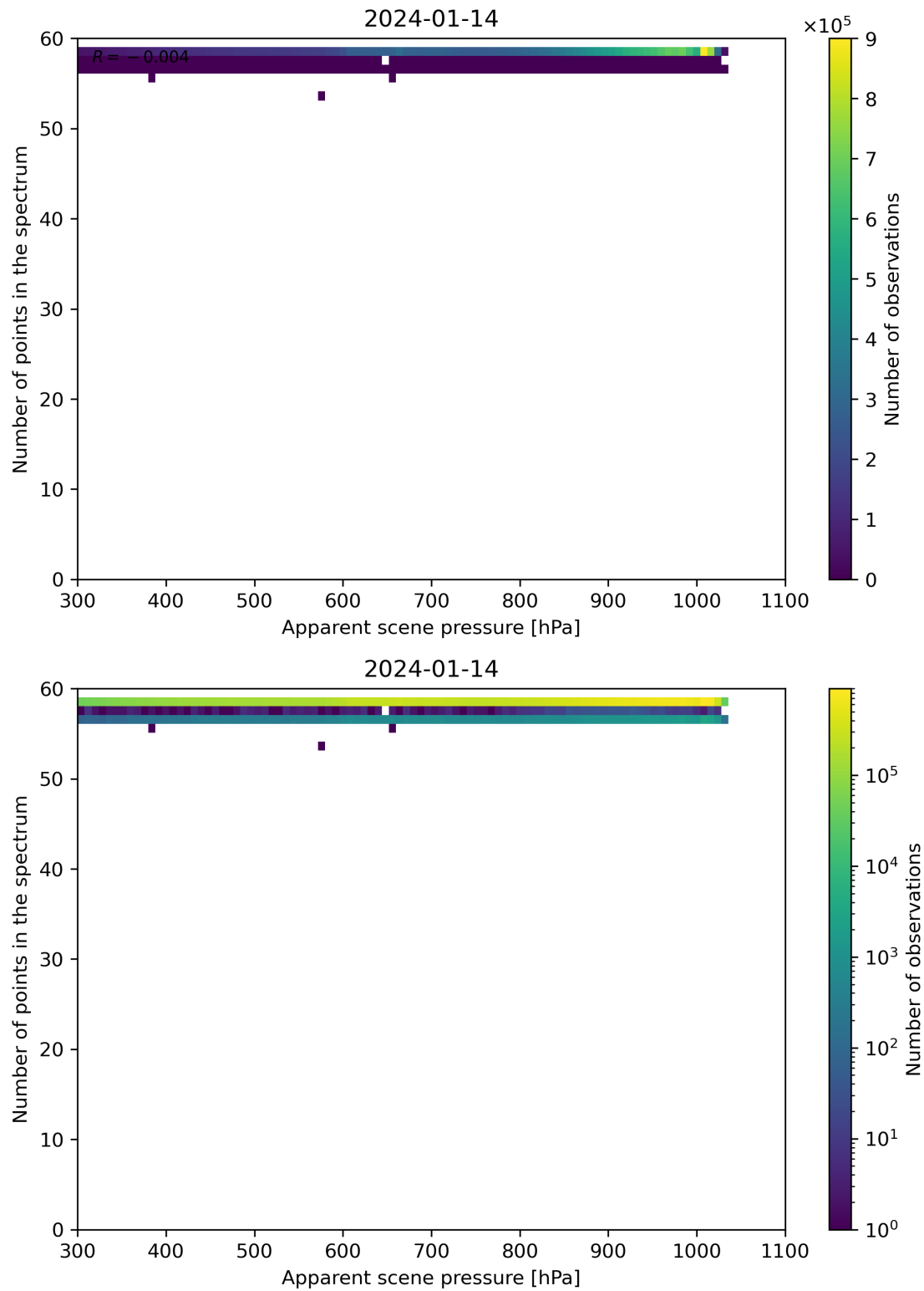
Figure 66: Scatter density plot of “Apparent scene pressure” against “Number of points in the spectrum” for 2024-01-13 to 2024-01-15.
