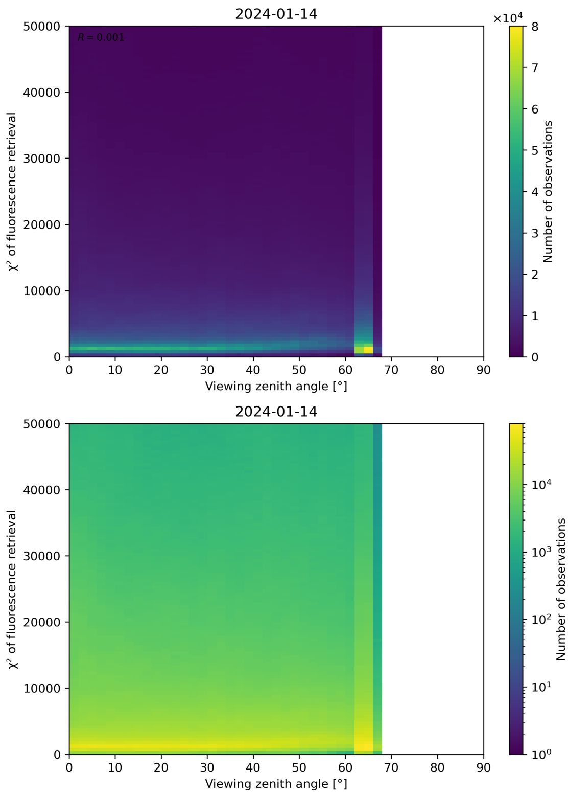
Figure 119: Scatter density plot of “Viewing zenith angle” against “ \chi^2 of fluorescence retrieval” for 2024-01-13 to 2024-01-15.
