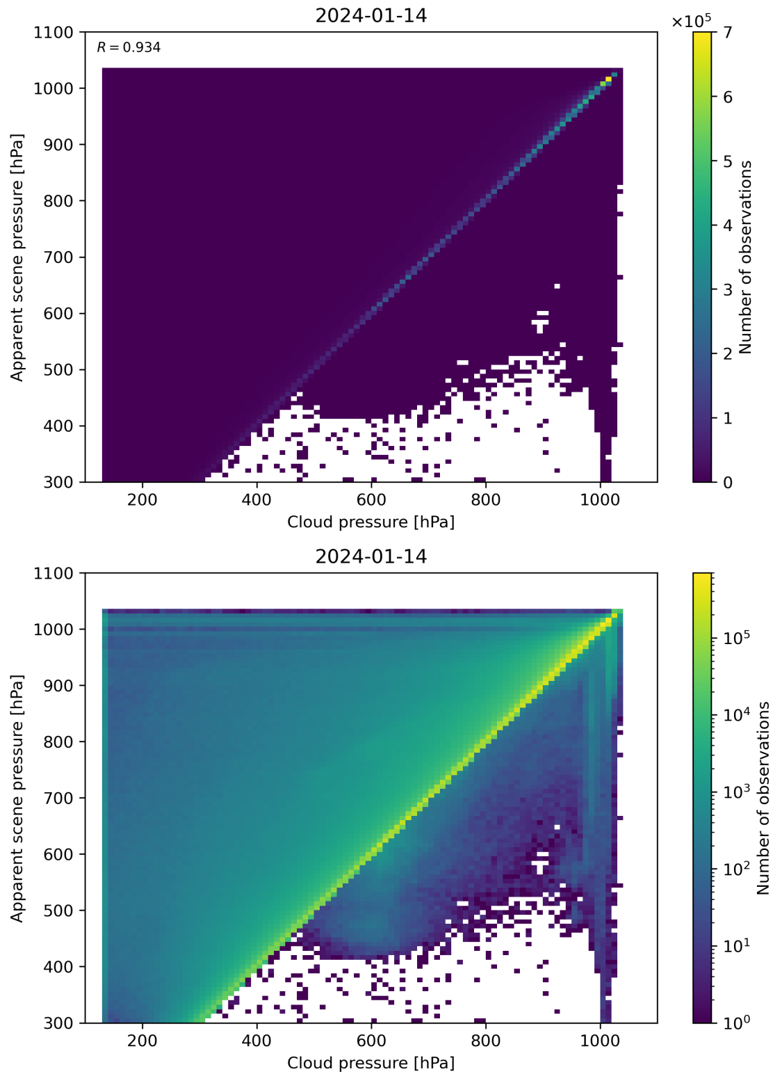
Figure 77: Scatter density plot of “Cloud pressure” against “Apparent scene pressure” for 2024-01-13 to 2024-01-15.
