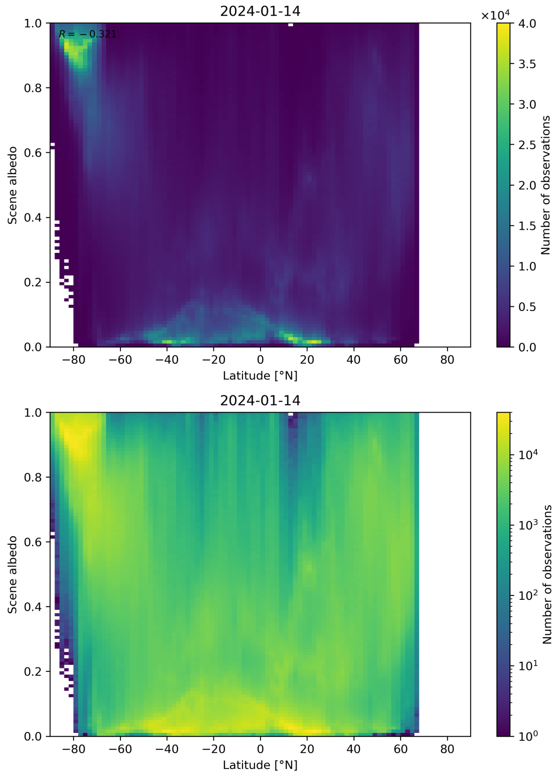
Figure 95: Scatter density plot of “Latitude” against “Scene albedo” for 2024-01-13 to 2024-01-15.
