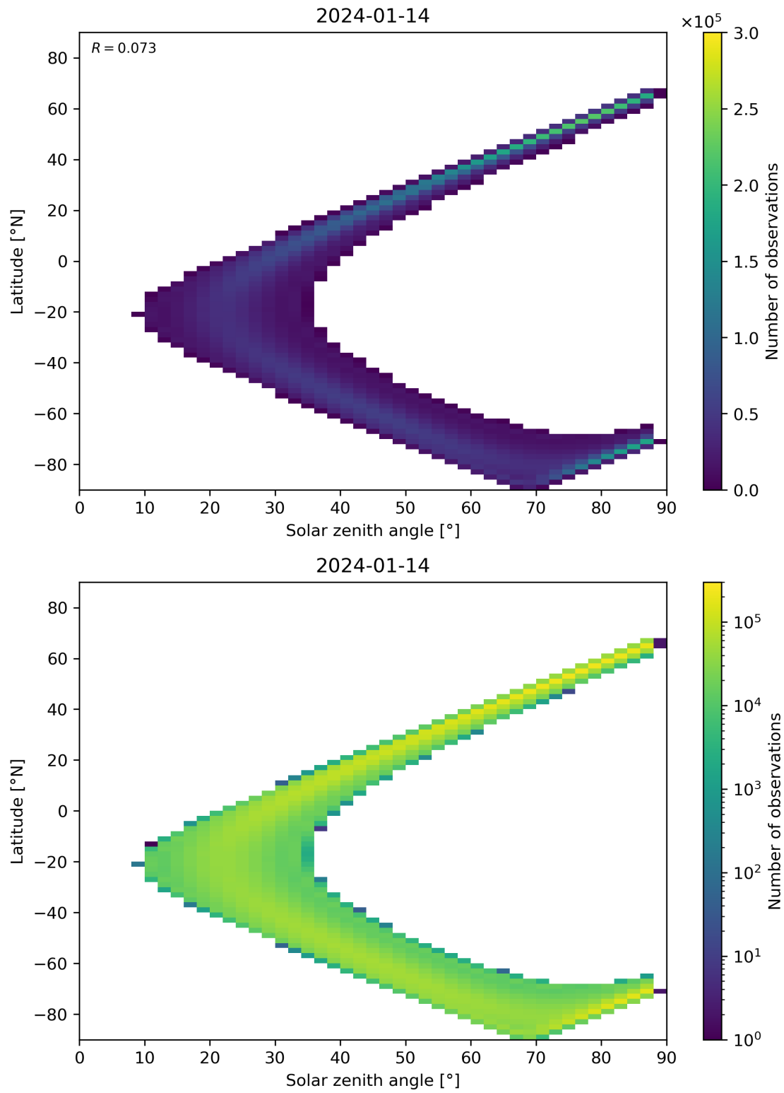
Figure 113: Scatter density plot of “Solar zenith angle” against “Latitude” for 2024-01-13 to 2024-01-15.
