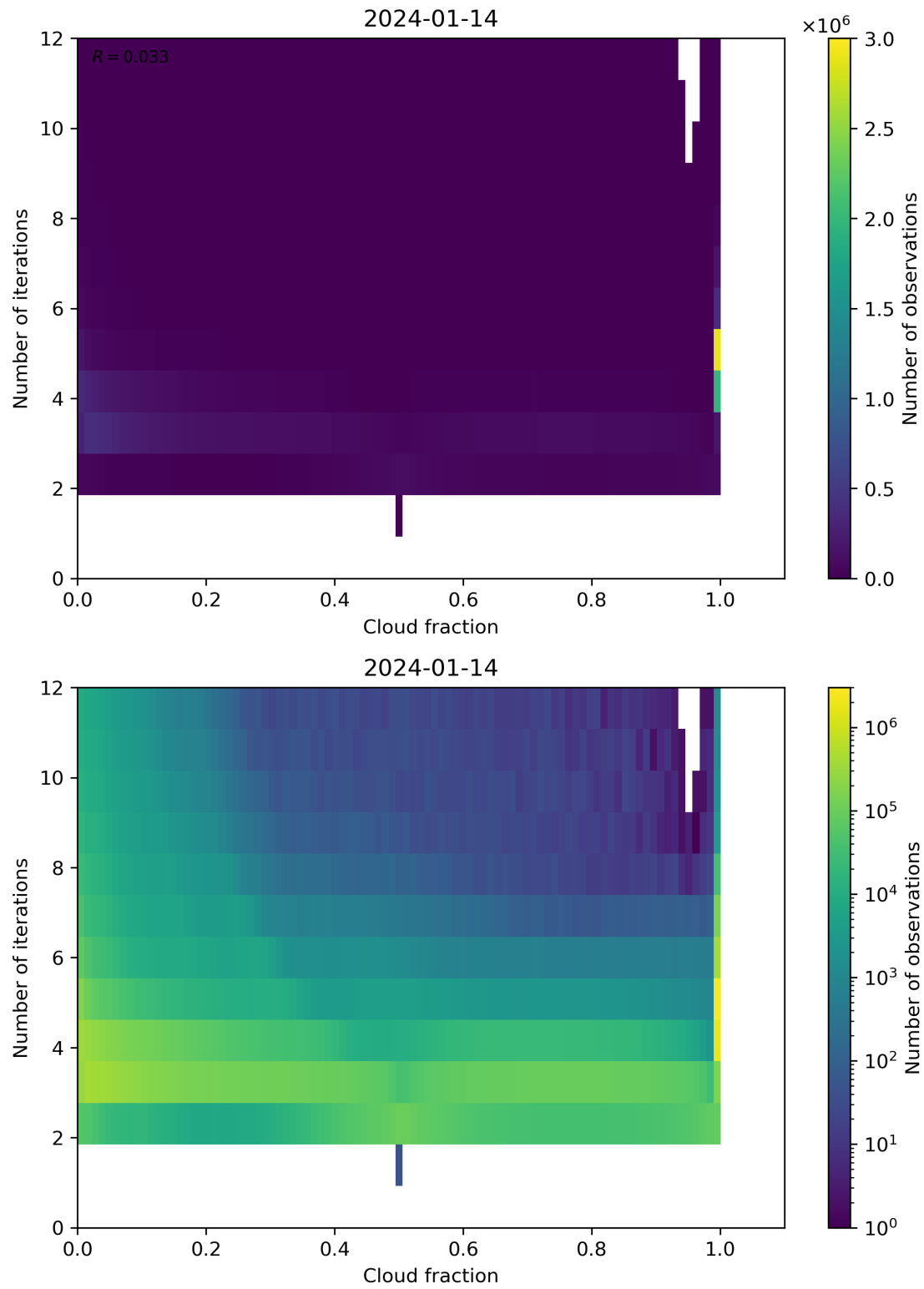
Figure 73: Scatter density plot of “Cloud fraction” against “Number of iterations” for 2024-01-13 to 2024-01-15.
