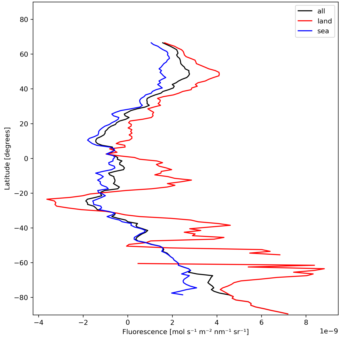
Figure 23: Zonal average of “Fluorescence” for 2024-01-13 to 2024-01-15.
