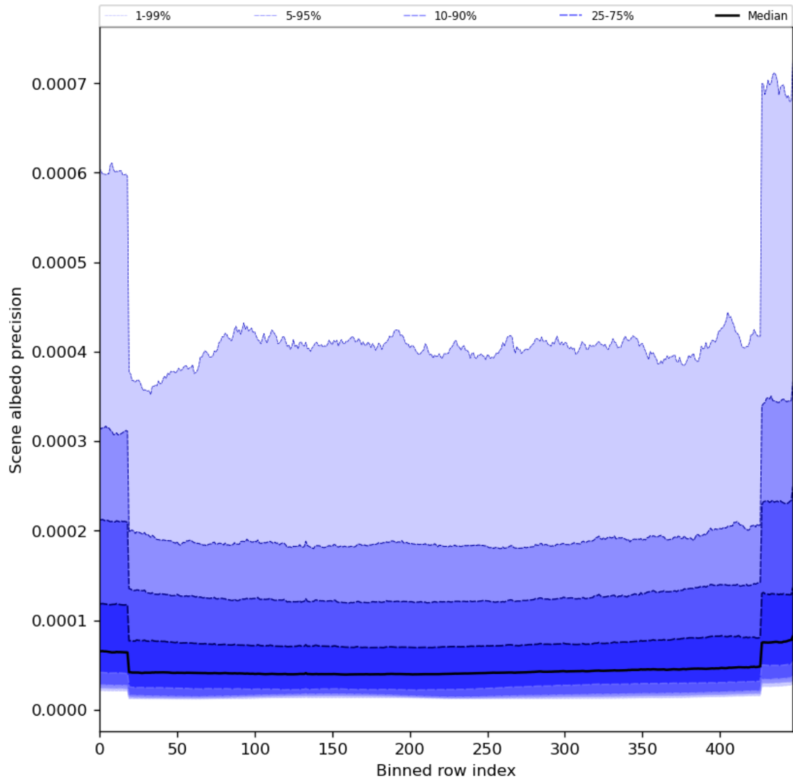
Figure 52: Along track statistics of “Scene albedo precision” for 2024-01-13 to 2024-01-15
