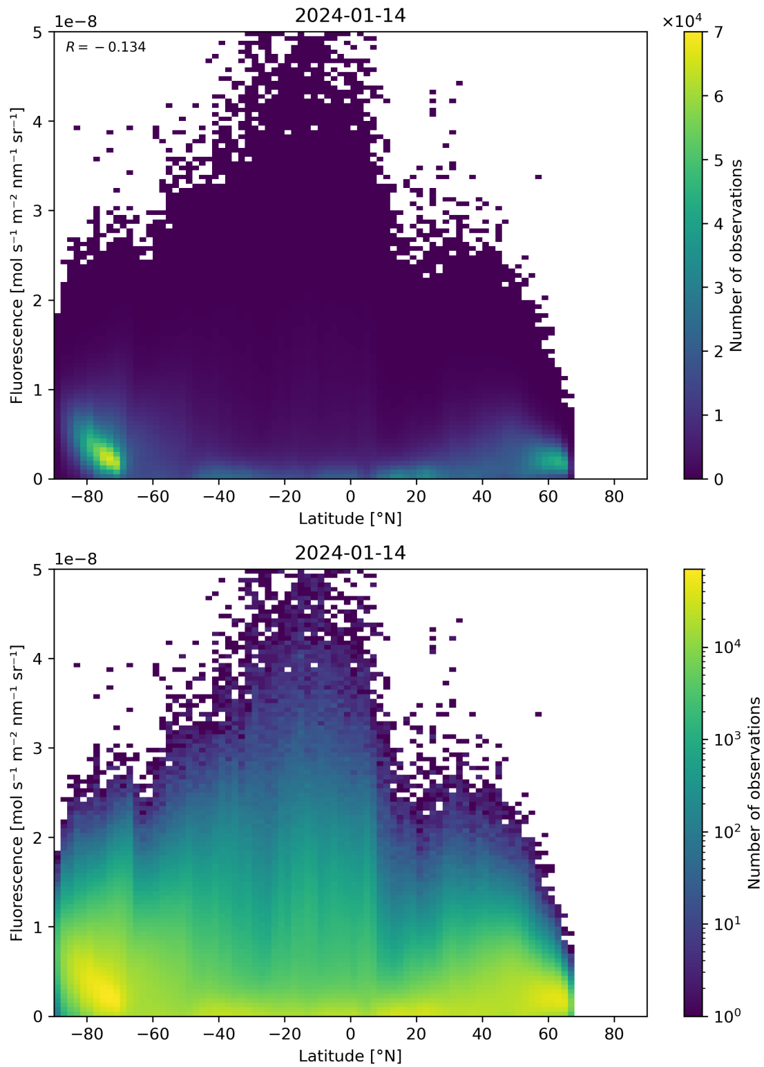
Figure 92: Scatter density plot of “Latitude” against “Fluorescence” for 2024-01-13 to 2024-01-15.
