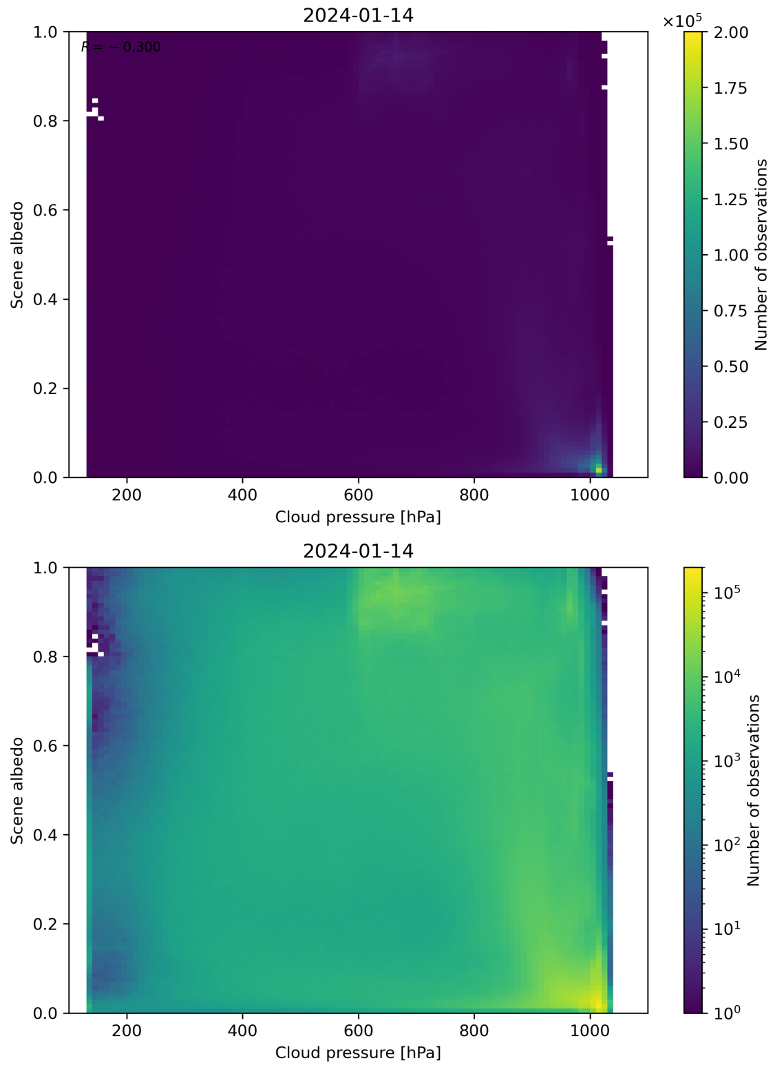
Figure 83: Scatter density plot of “Cloud pressure” against “Scene albedo” for 2024-01-13 to 2024-01-15.
