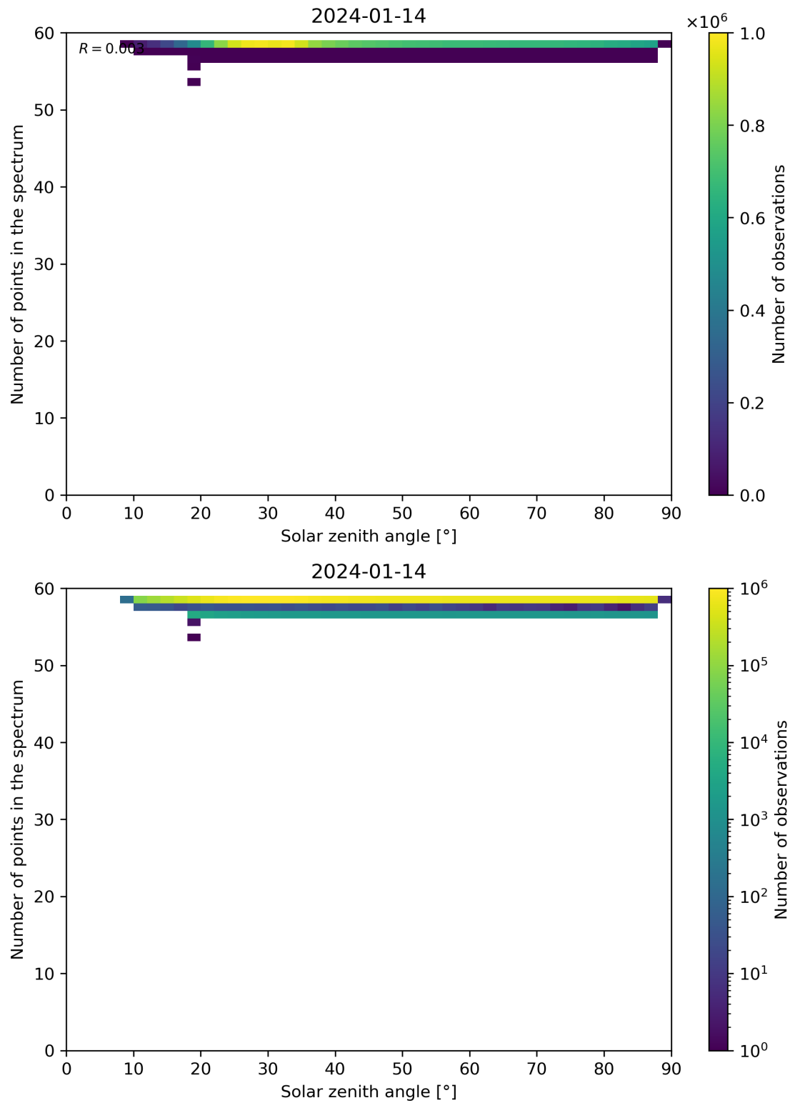
Figure 115: Scatter density plot of “Solar zenith angle” against “Number of points in the spectrum” for 2024-01-13 to 2024-01-15.
