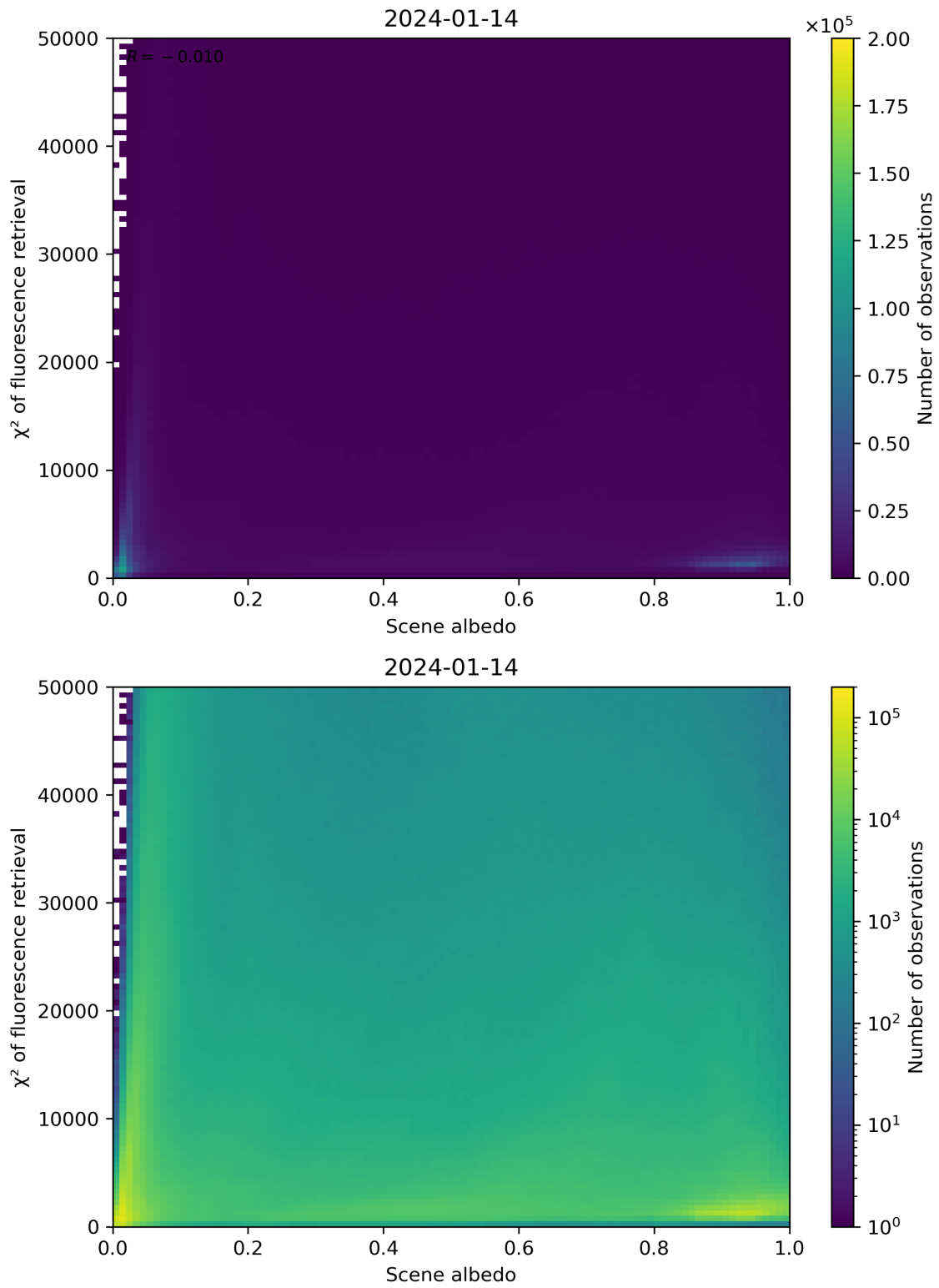
Figure 103: Scatter density plot of “Scene albedo” against “ \chi^2 of fluorescence retrieval” for 2024-01-13 to 2024-01-15.
