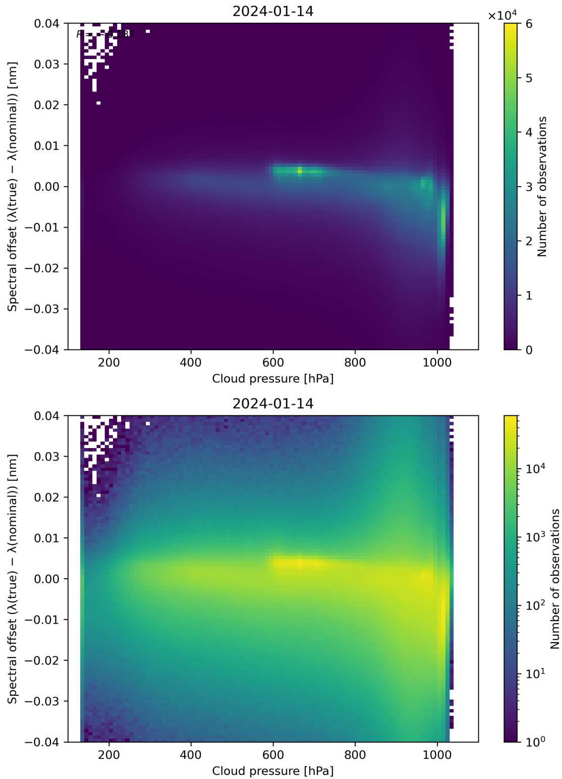
Figure 84: Scatter density plot of “Cloud pressure” against “Spectral offset ( \lambda(\text{true}) - \lambda(\text{nominal}) )” for 2024-01-13 to 2024-01-15.
