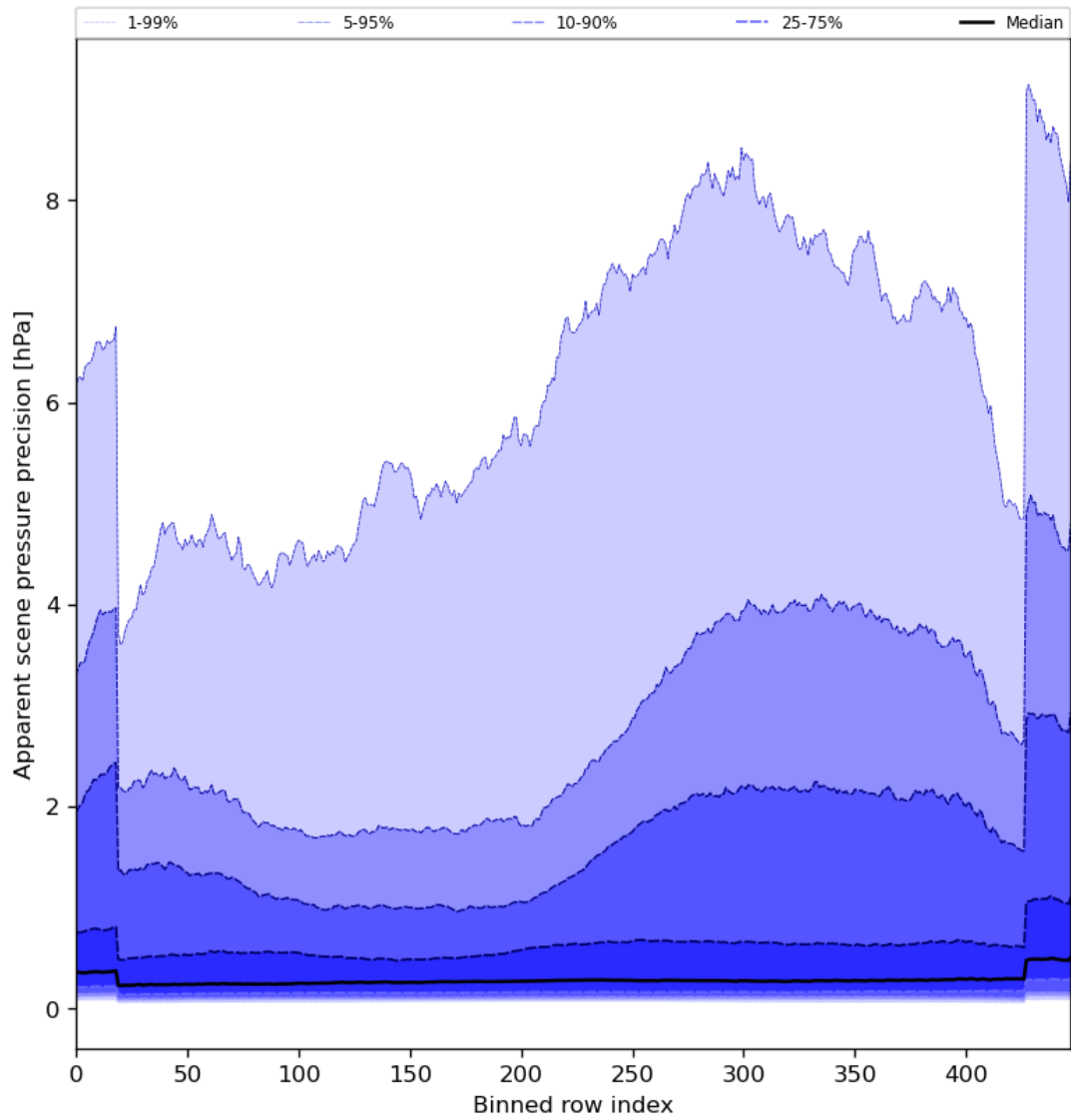
Figure 54: Along track statistics of “Apparent scene pressure precision” for 2024-01-13 to 2024-01-15
