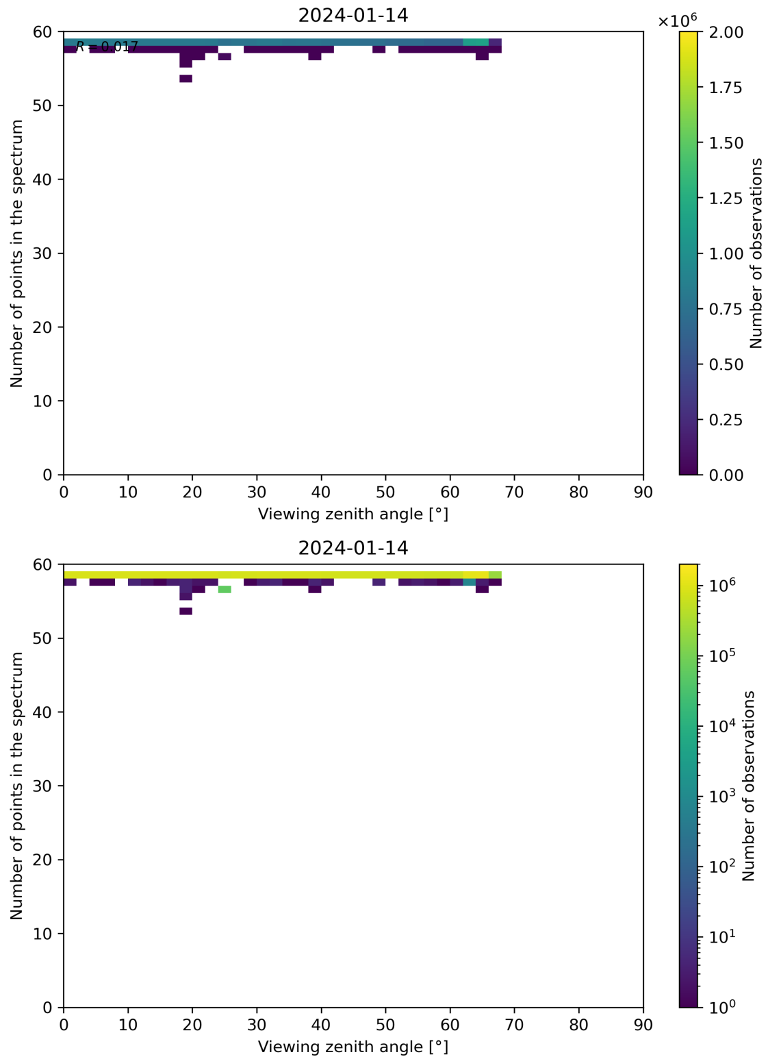
Figure 125: Scatter density plot of “Viewing zenith angle” against “Number of points in the spectrum” for 2024-01-13 to 2024-01-15.
