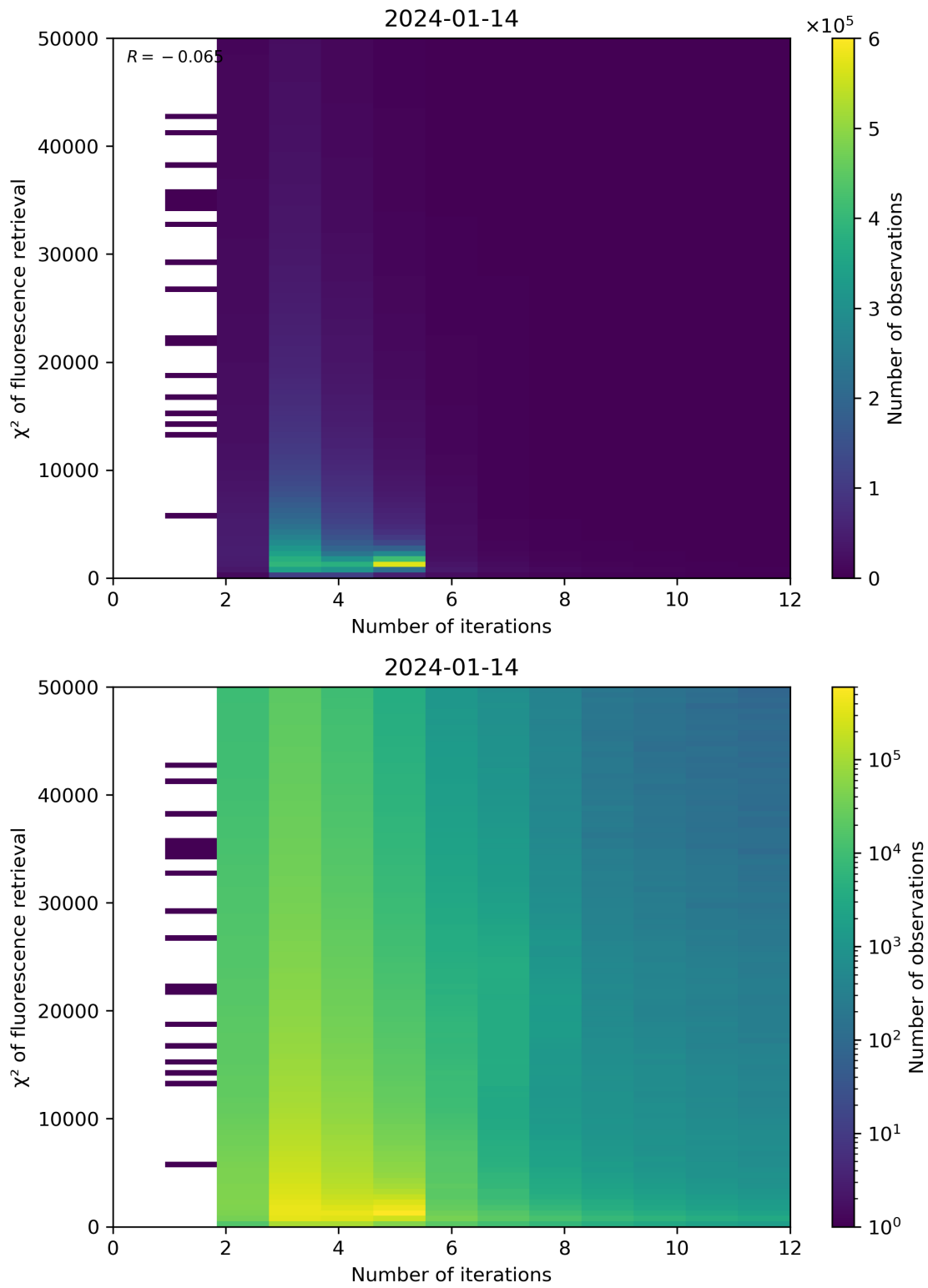
Figure 97: Scatter density plot of “Number of iterations” against “ \chi^2 of fluorescence retrieval” for 2024-01-13 to 2024-01-15.
