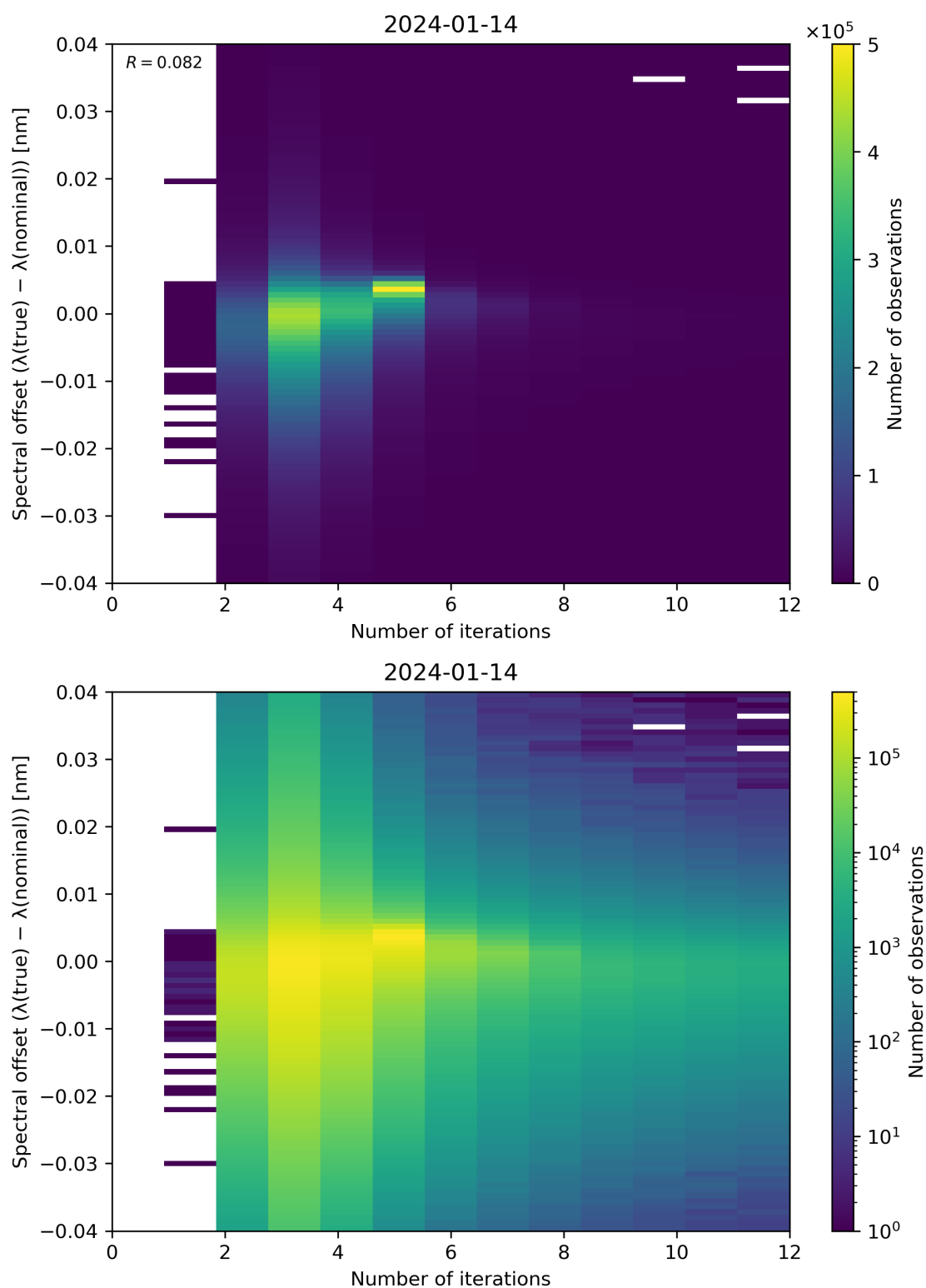
Figure 100: Scatter density plot of “Number of iterations” against “Spectral offset ( \lambda(\text{true}) - \lambda(\text{nominal}) )” for 2024-01-13 to 2024-01-15.
