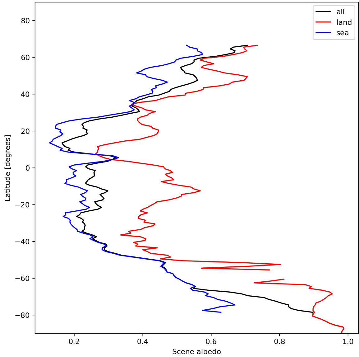
Figure 17: Zonal average of “Scene albedo” for 2024-01-13 to 2024-01-15.
