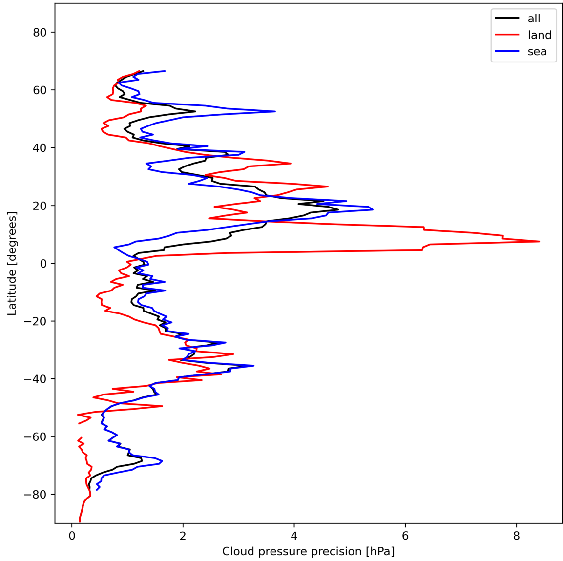
Figure 14: Zonal average of “Cloud pressure precision” for 2024-01-13 to 2024-01-15.
