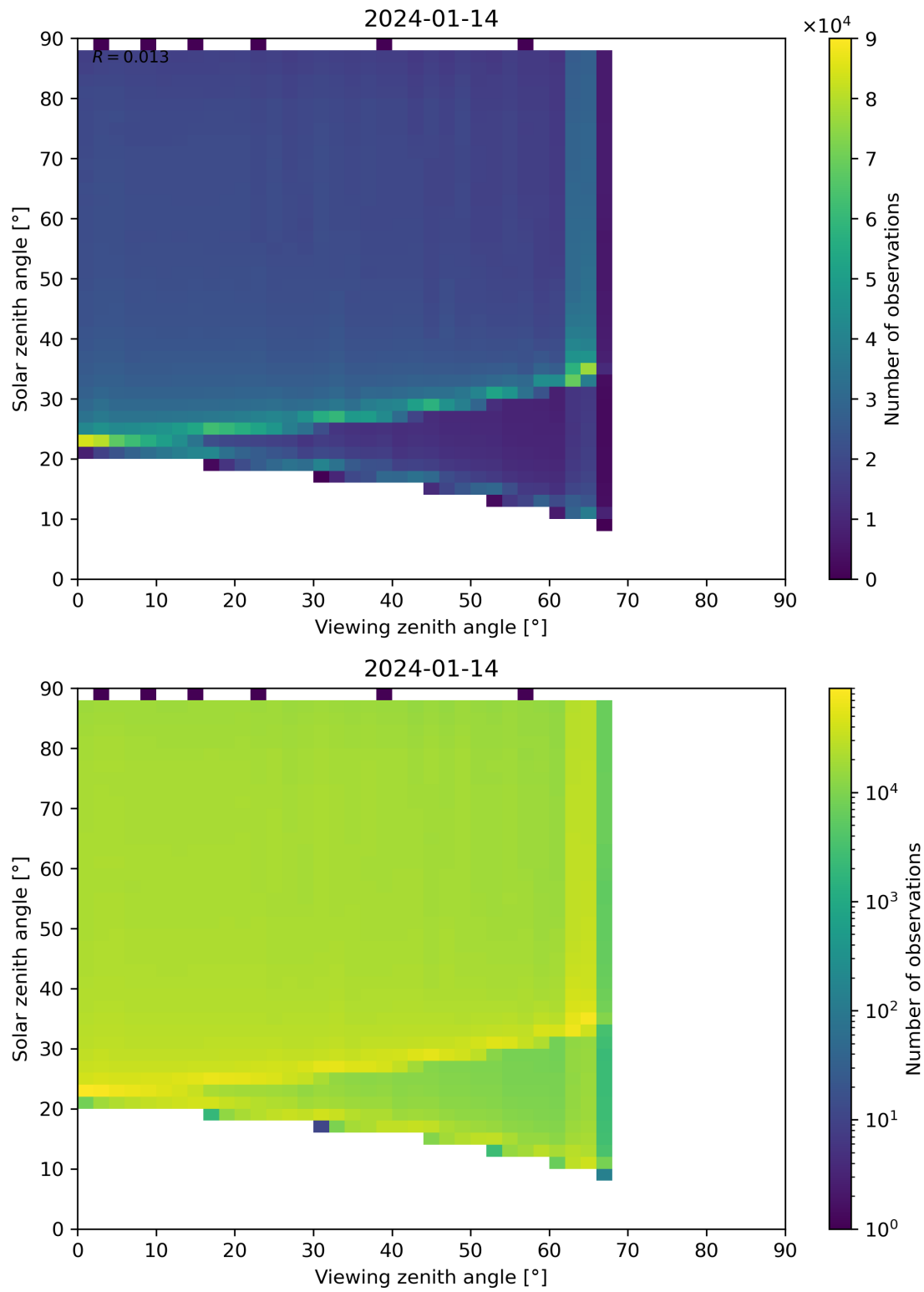
Figure 127: Scatter density plot of “Viewing zenith angle” against “Solar zenith angle” for 2024-01-13 to 2024-01-15.
