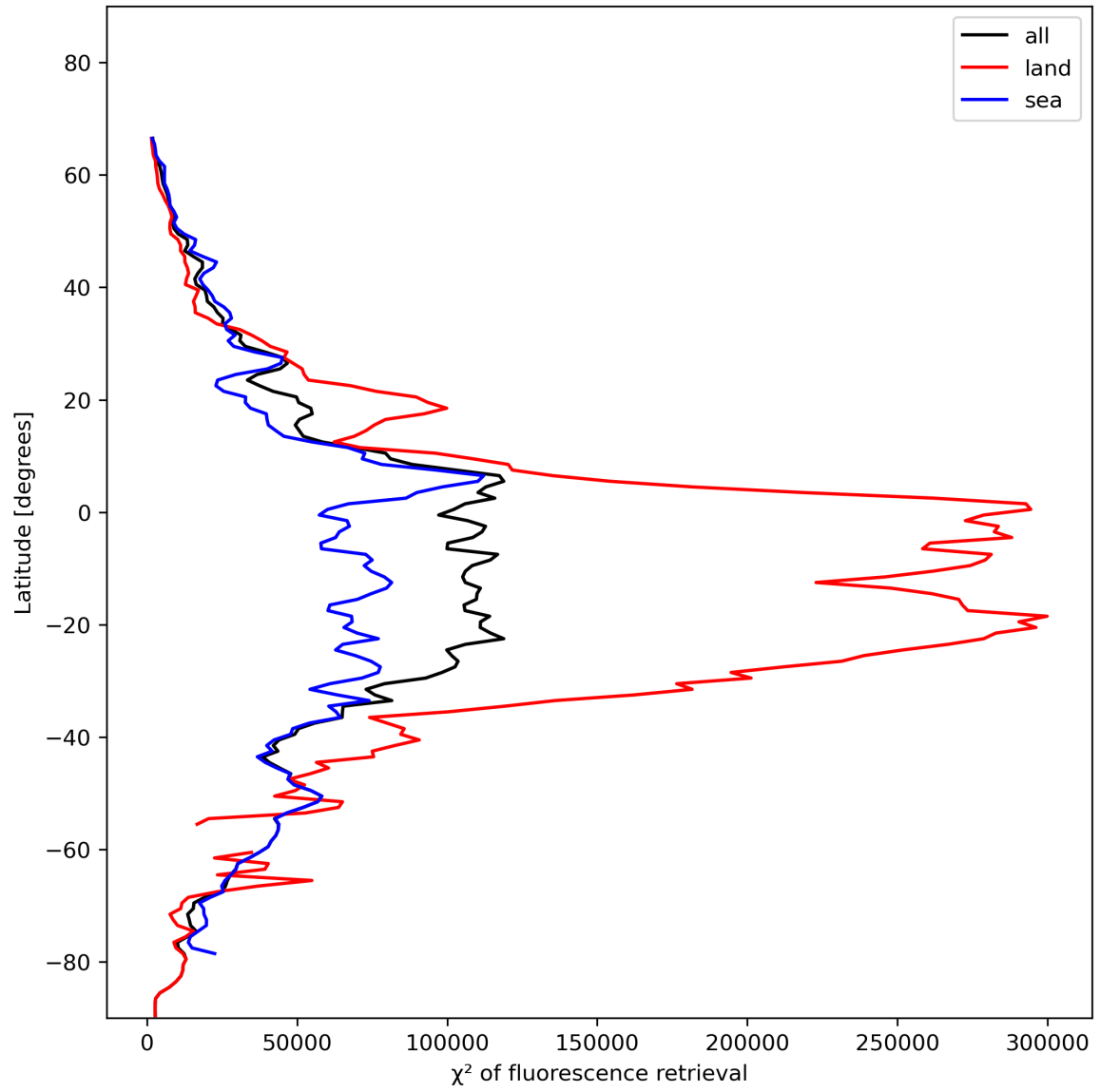
Figure 25: Zonal average of “ \chi^2 of fluorescence retrieval” for 2024-01-13 to 2024-01-15.
