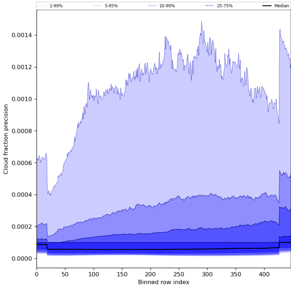
Figure 50: Along track statistics of “Cloud fraction precision” for 2024-01-13 to 2024-01-15
