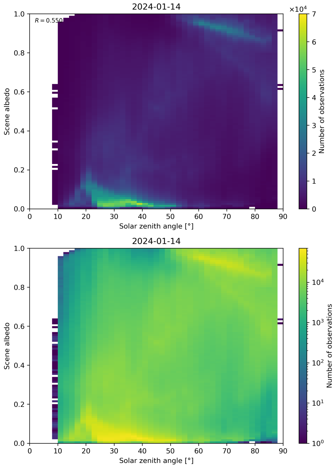
Figure 116: Scatter density plot of “Solar zenith angle” against “Scene albedo” for 2024-01-13 to 2024-01-15.
