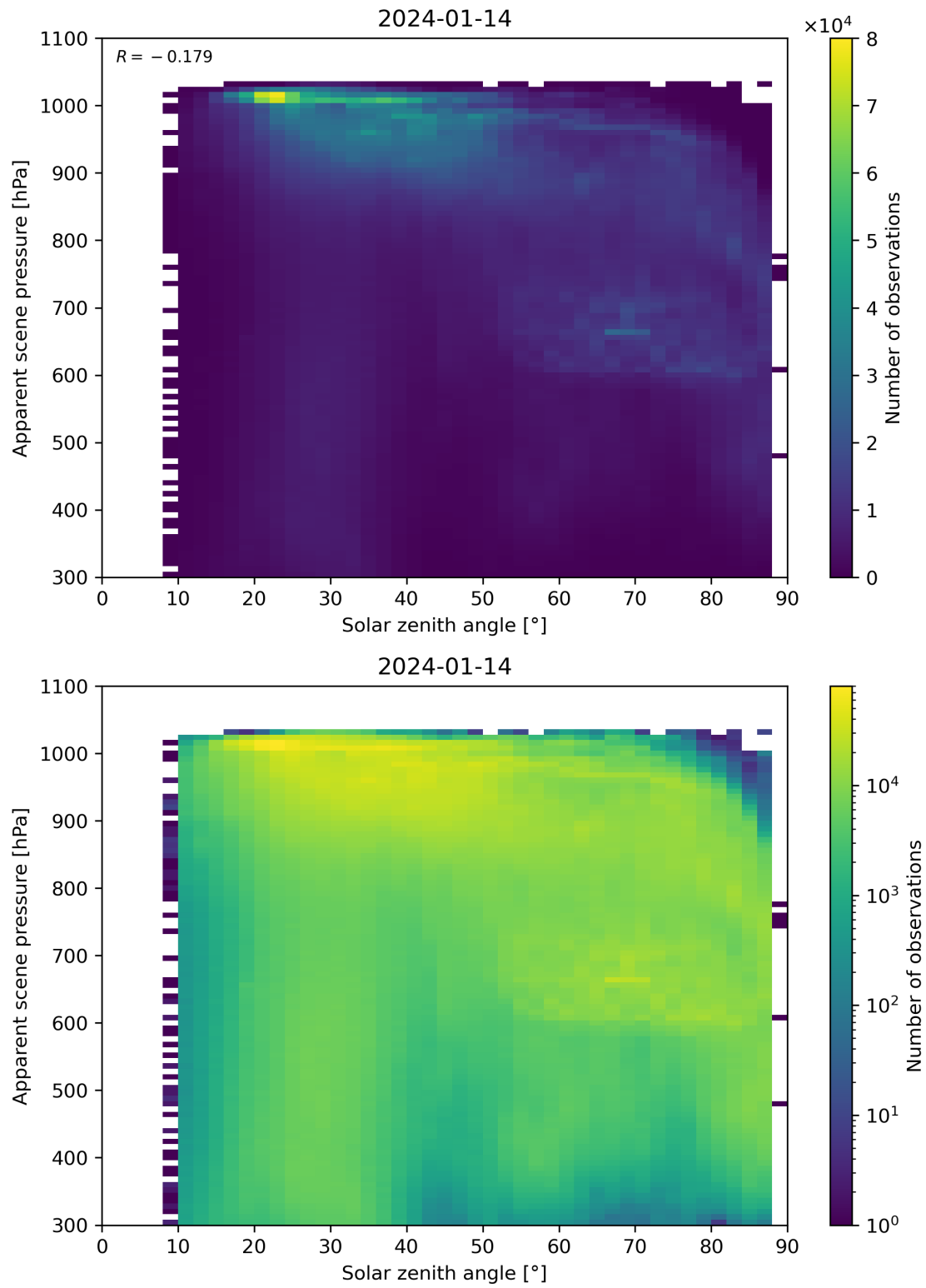
Figure 108: Scatter density plot of “Solar zenith angle” against “Apparent scene pressure” for 2024-01-13 to 2024-01-15.
