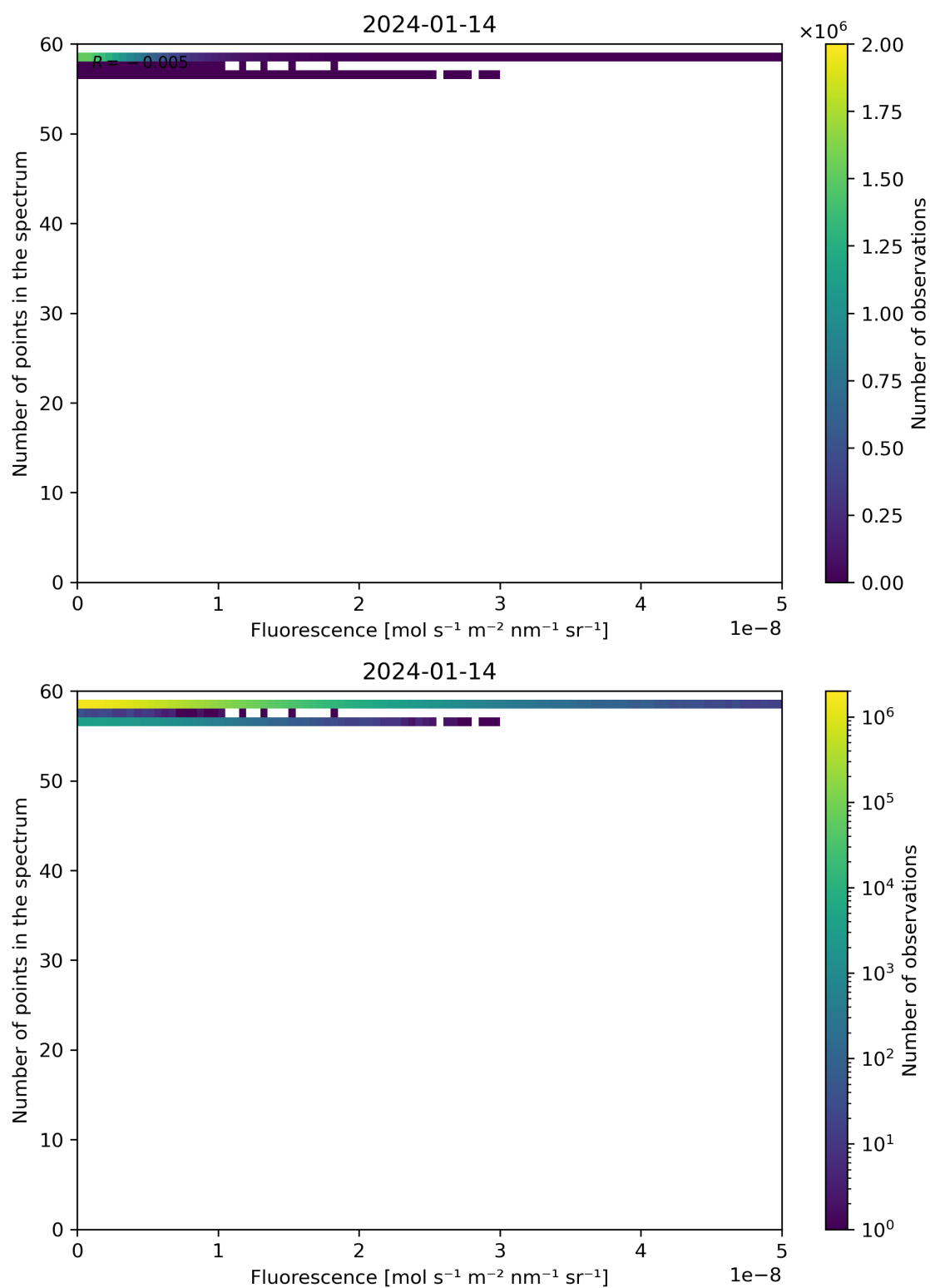
Figure 86: Scatter density plot of “Fluorescence” against “Number of points in the spectrum” for 2024-01-13 to 2024-01-15.
