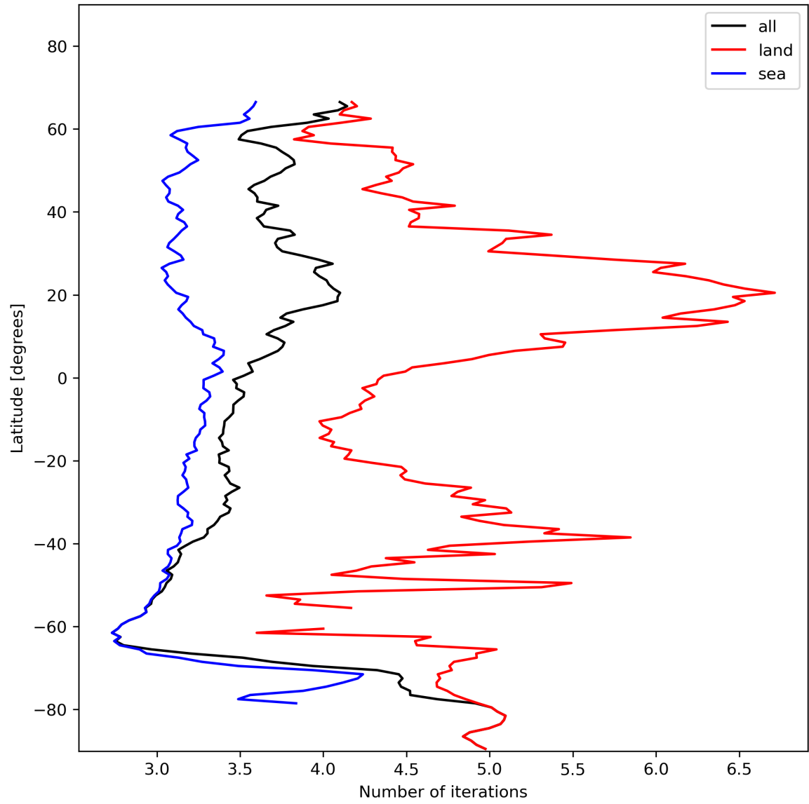
Figure 22: Zonal average of “Number of iterations” for 2024-01-13 to 2024-01-15.
