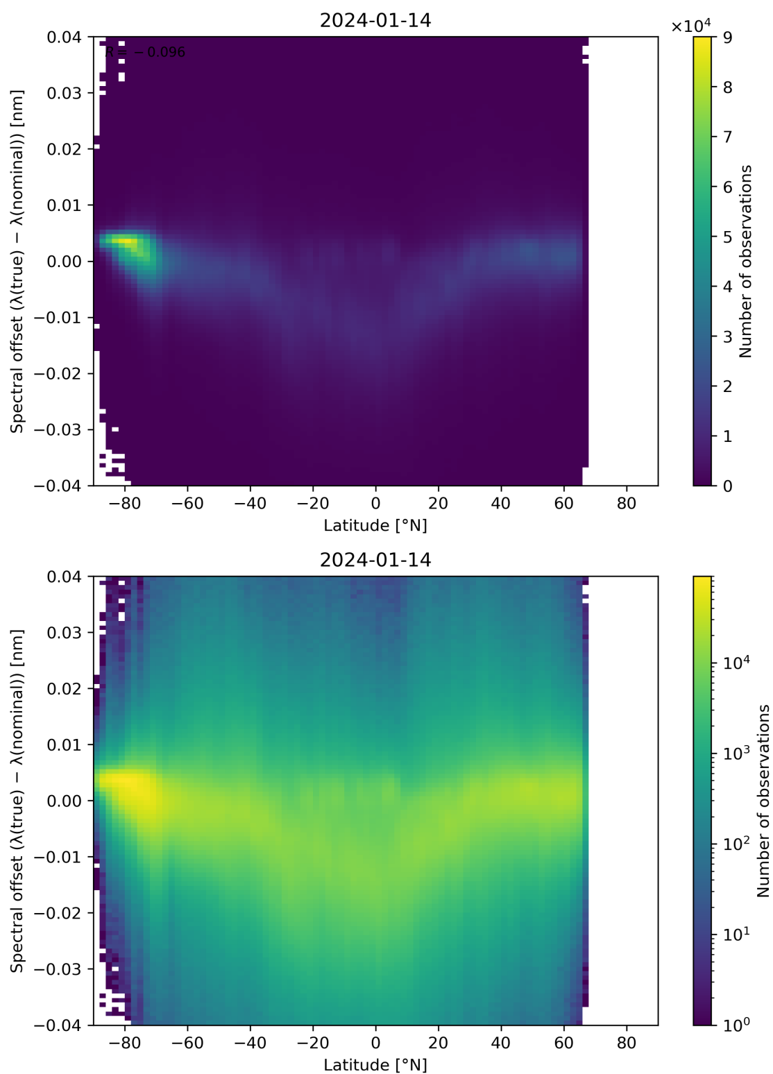
Figure 96: Scatter density plot of “Latitude” against “Spectral offset ( \lambda(\text{true}) - \lambda(\text{nominal}) )” for 2024-01-13 to 2024-01-15.
