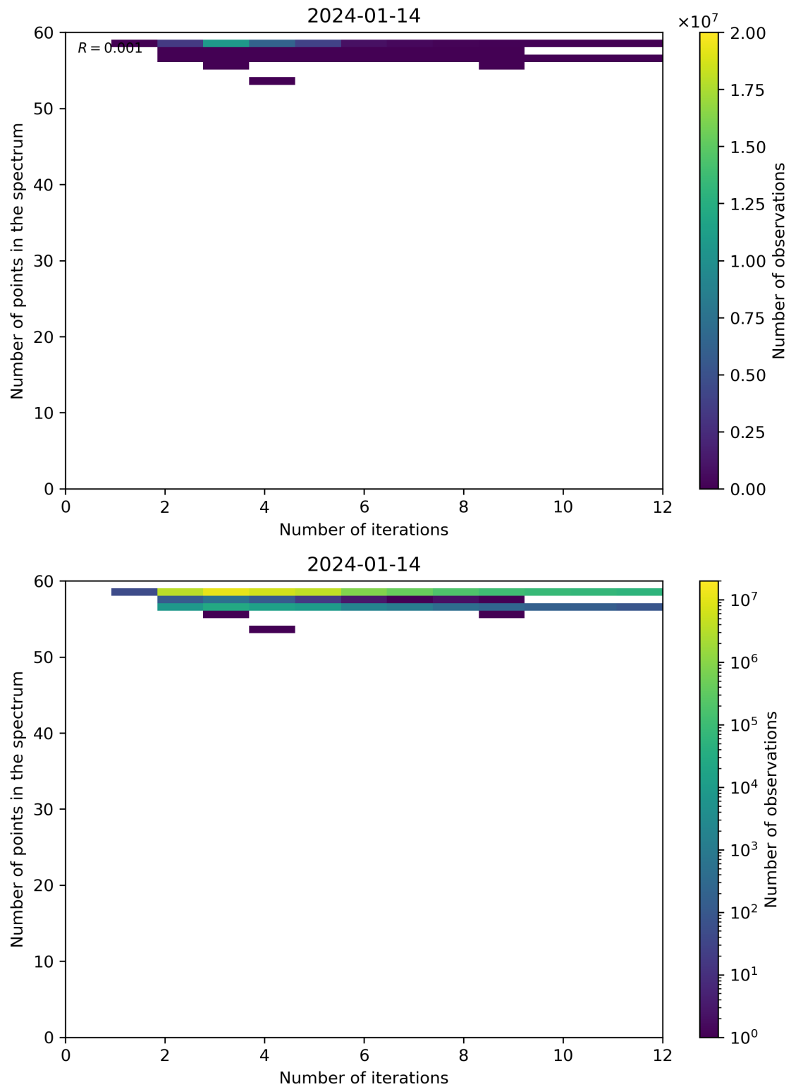
Figure 99: Scatter density plot of “Number of iterations” against “Number of points in the spectrum” for 2024-01-13 to 2024-01-15.
