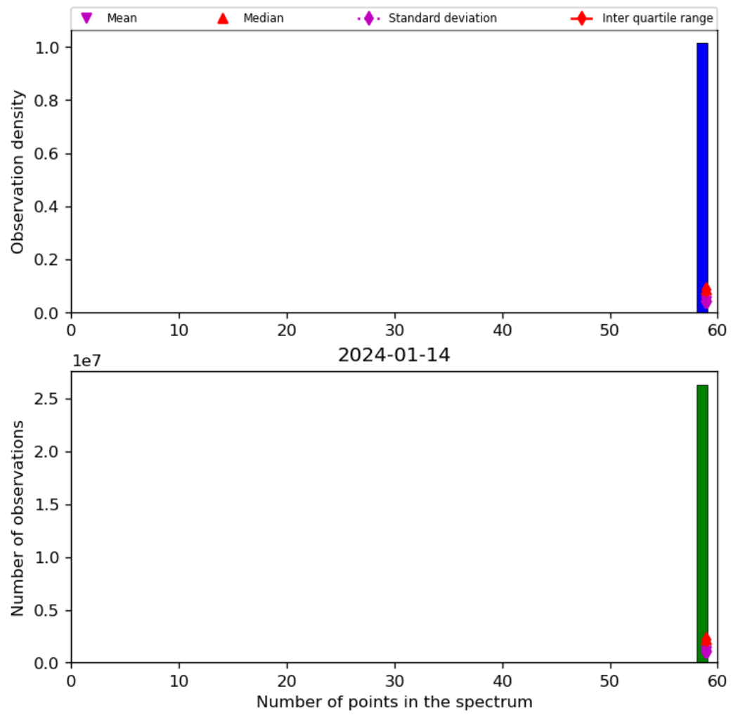
Figure 44: Histogram of “Number of points in the spectrum” for 2024-01-13 to 2024-01-15
