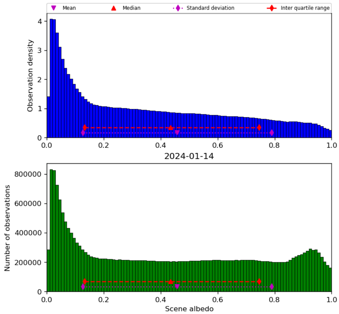
Figure 34: Histogram of “Scene albedo” for 2024-01-13 to 2024-01-15
