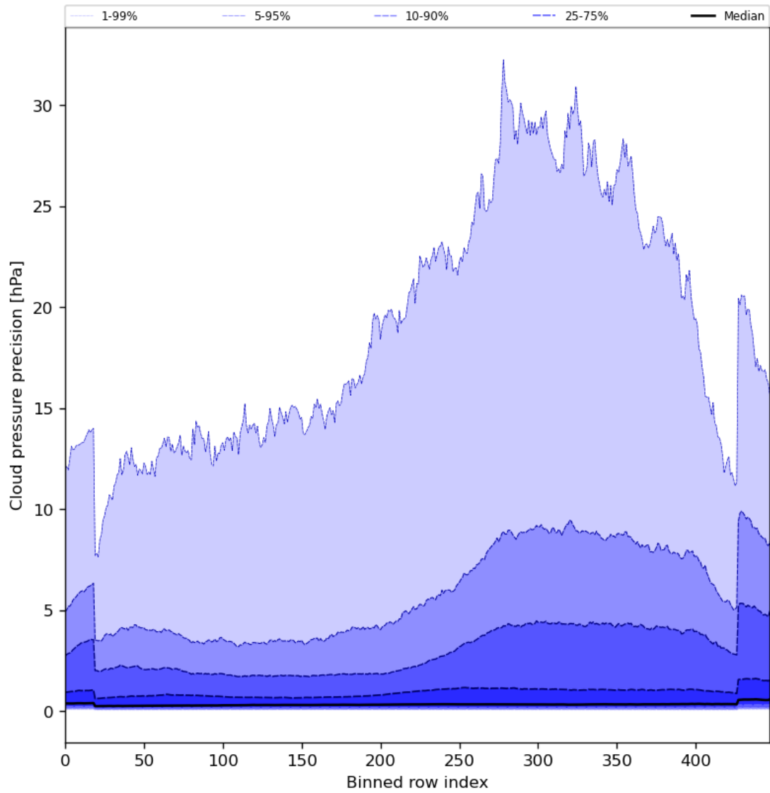
Figure 48: Along track statistics of “Cloud pressure precision” for 2024-01-13 to 2024-01-15
