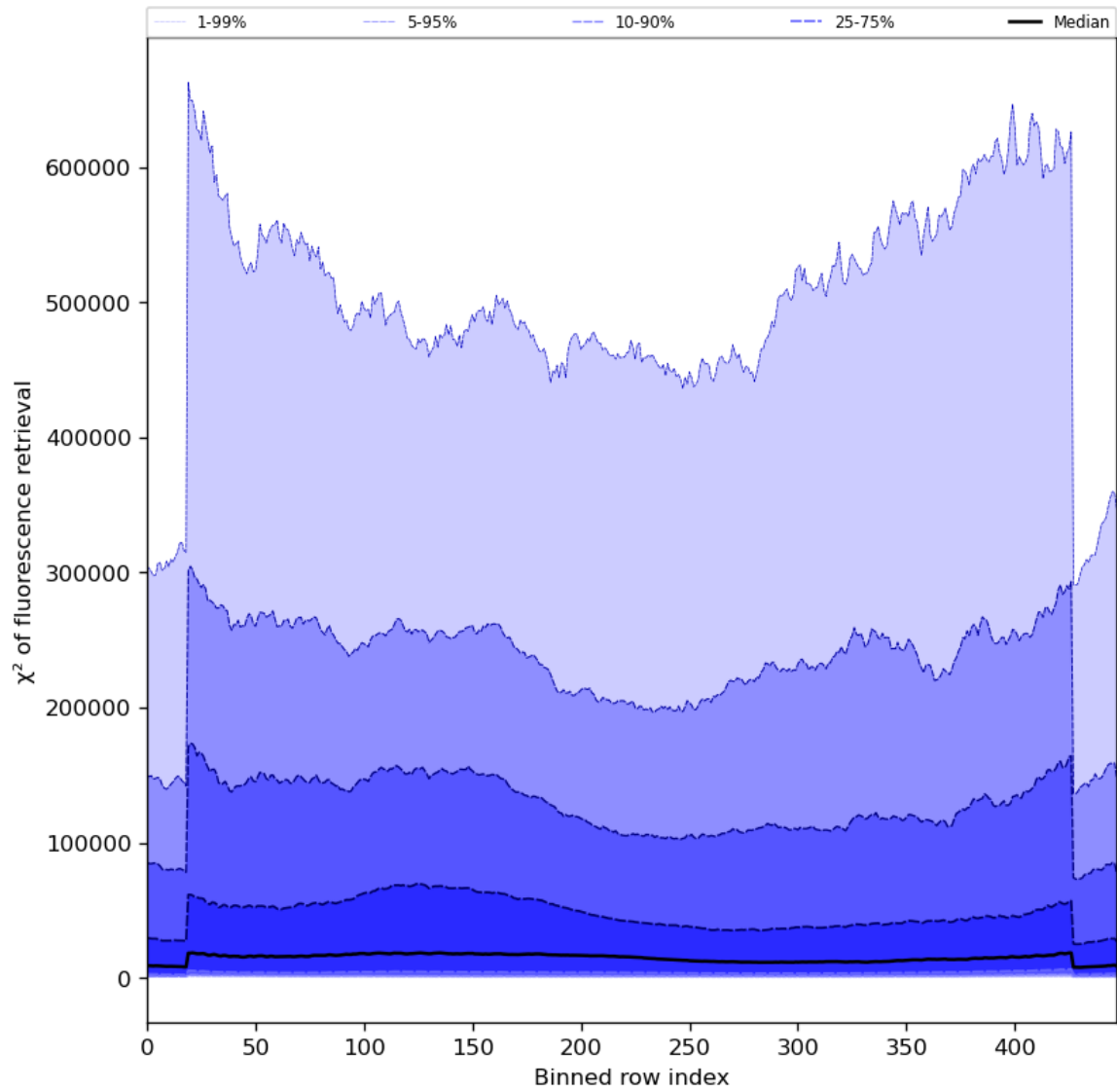
Figure 59: Along track statistics of “ \chi^2 of fluorescence retrieval” for 2024-01-16 to 2024-01-18
