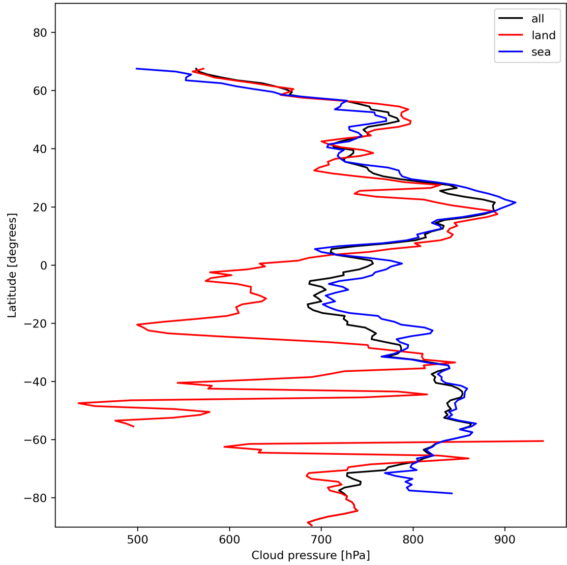
Figure 13: Zonal average of “Cloud pressure” for 2024-01-16 to 2024-01-18.
