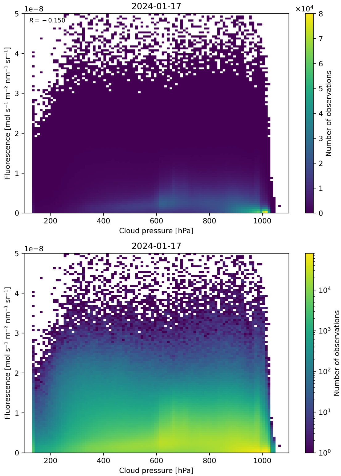
Figure 80: Scatter density plot of “Cloud pressure” against “Fluorescence” for 2024-01-16 to 2024-01-18.
