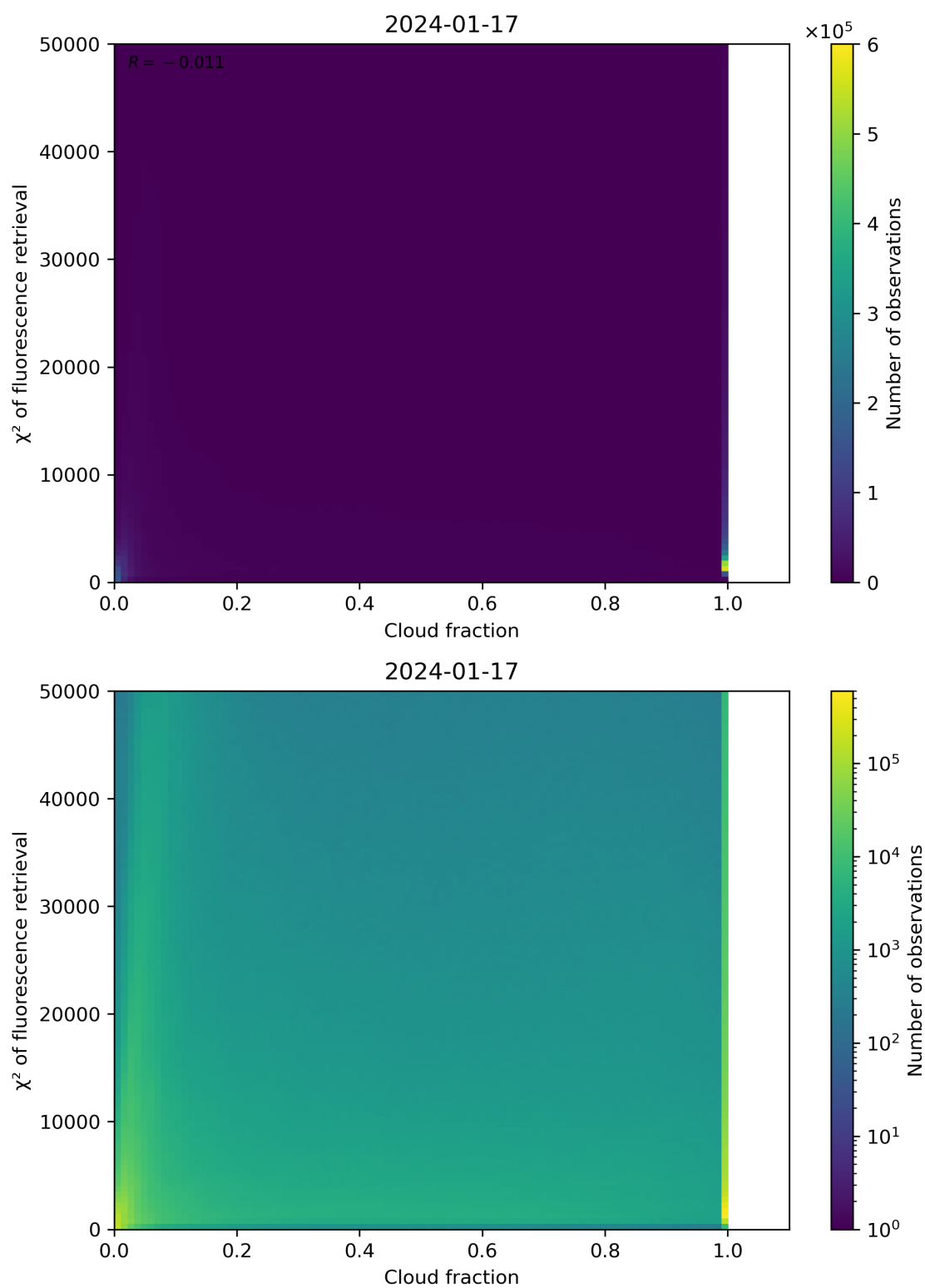
Figure 71: Scatter density plot of “Cloud fraction” against “ \chi^2 of fluorescence retrieval” for 2024-01-16 to 2024-01-18.
