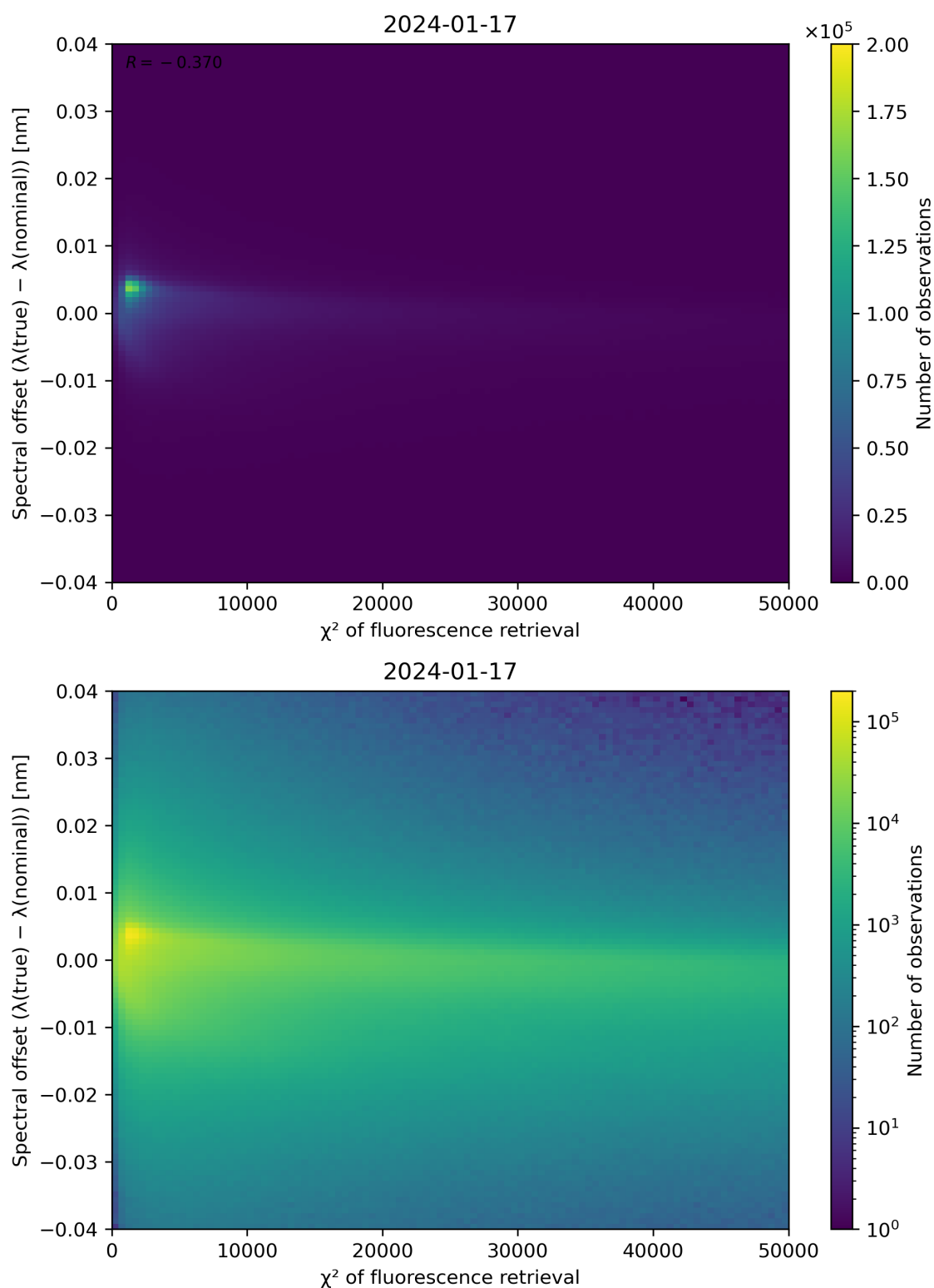
Figure 69: Scatter density plot of " \chi^2 of fluorescence retrieval" against "Spectral offset ( \lambda(\text{true}) - \lambda(\text{nominal}) )" for 2024-01-16 to 2024-01-18.
