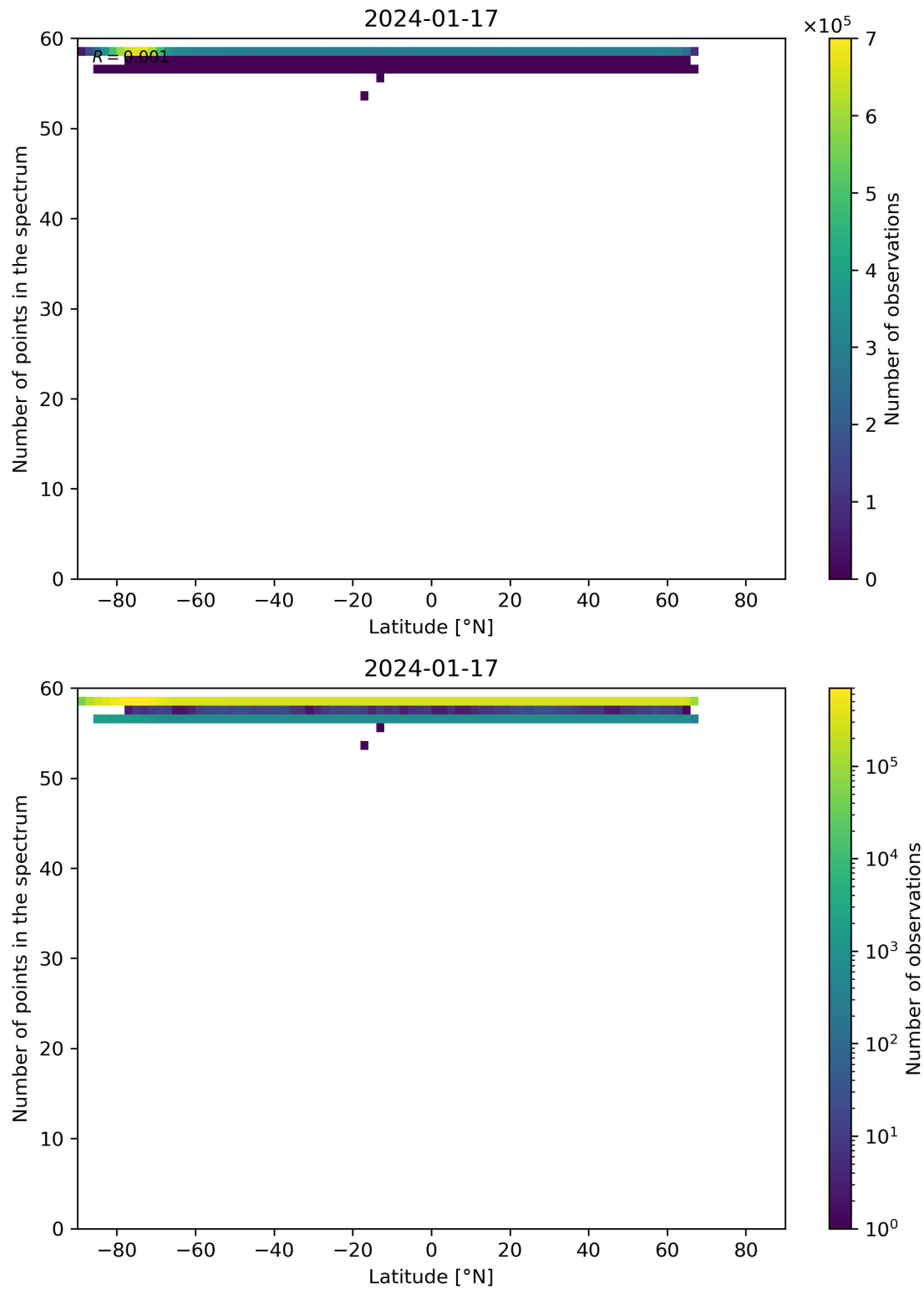
Figure 94: Scatter density plot of “Latitude” against “Number of points in the spectrum” for 2024-01-16 to 2024-01-18.
