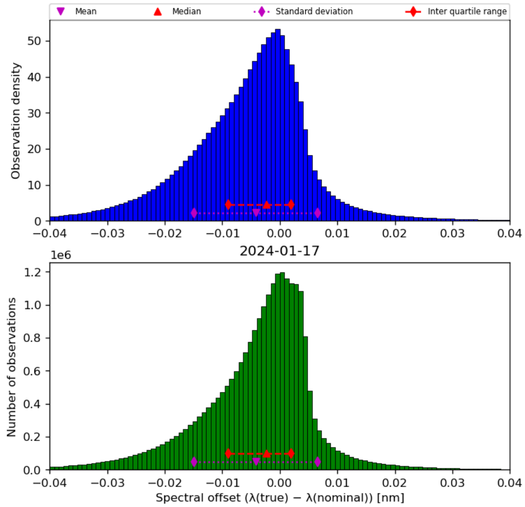
Figure 45: Histogram of “Spectral offset ( \lambda(\text{true}) - \lambda(\text{nominal}) )” for 2024-01-16 to 2024-01-18
