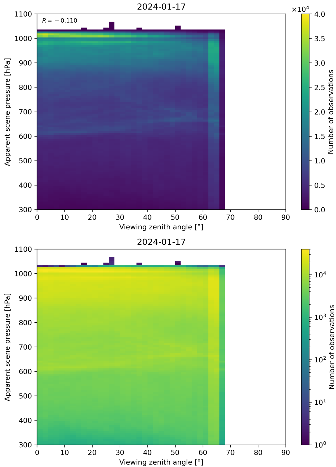
Figure 118: Scatter density plot of “Viewing zenith angle” against “Apparent scene pressure” for 2024-01-16 to 2024-01-18.
