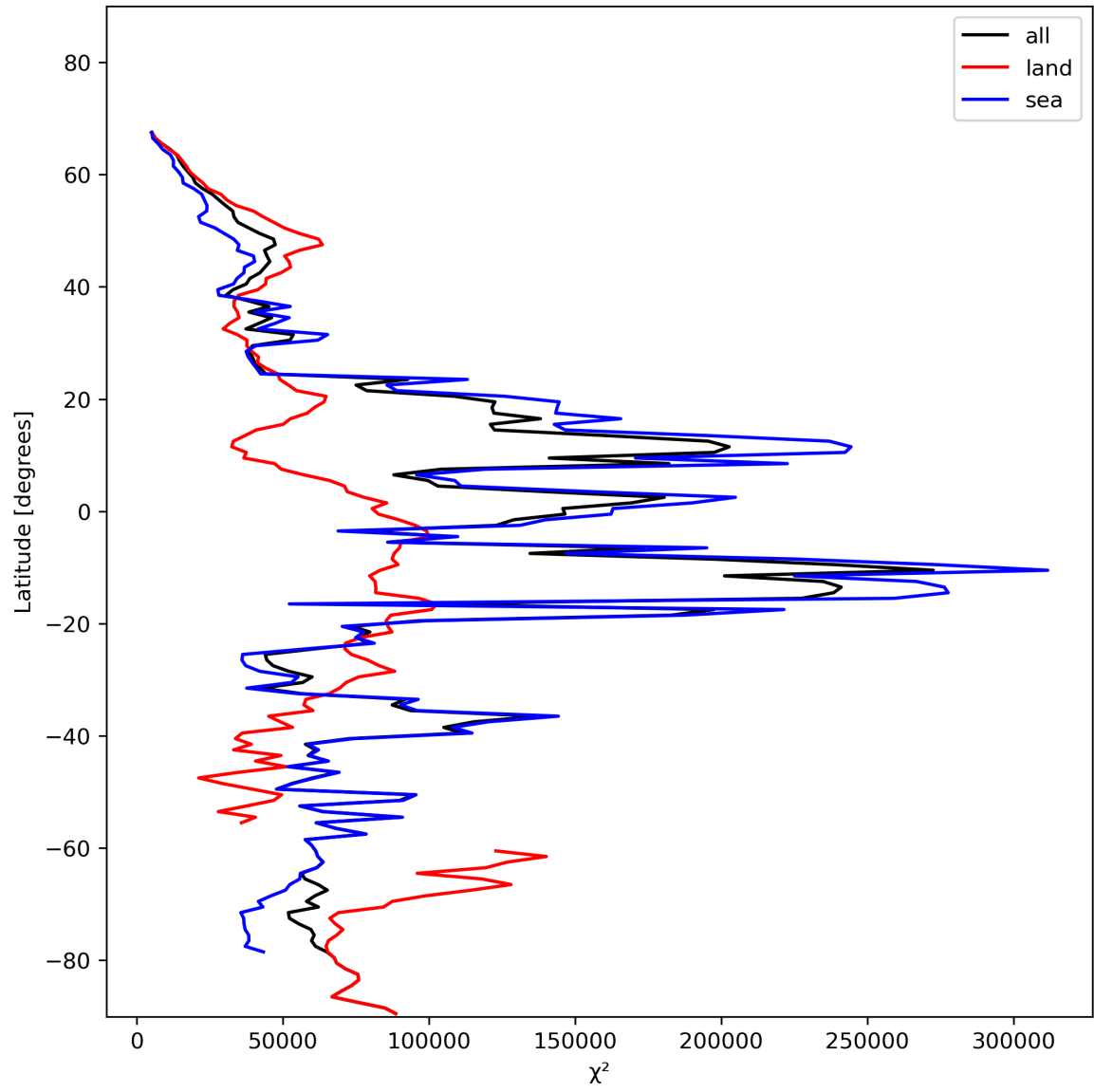
Figure 21: Zonal average of “ \chi^2 ” for 2024-01-16 to 2024-01-18.
