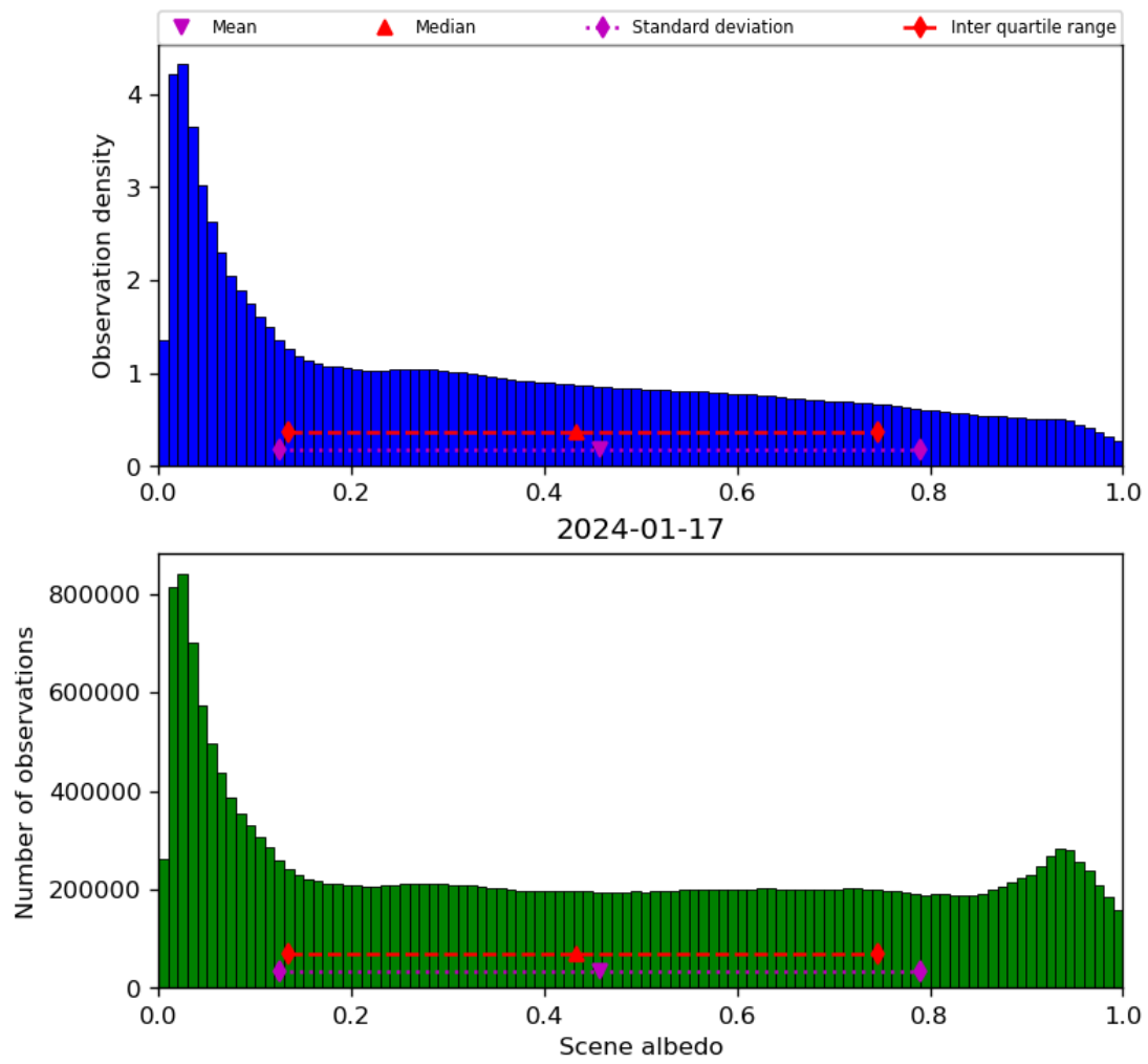
Figure 34: Histogram of “Scene albedo” for 2024-01-16 to 2024-01-18
