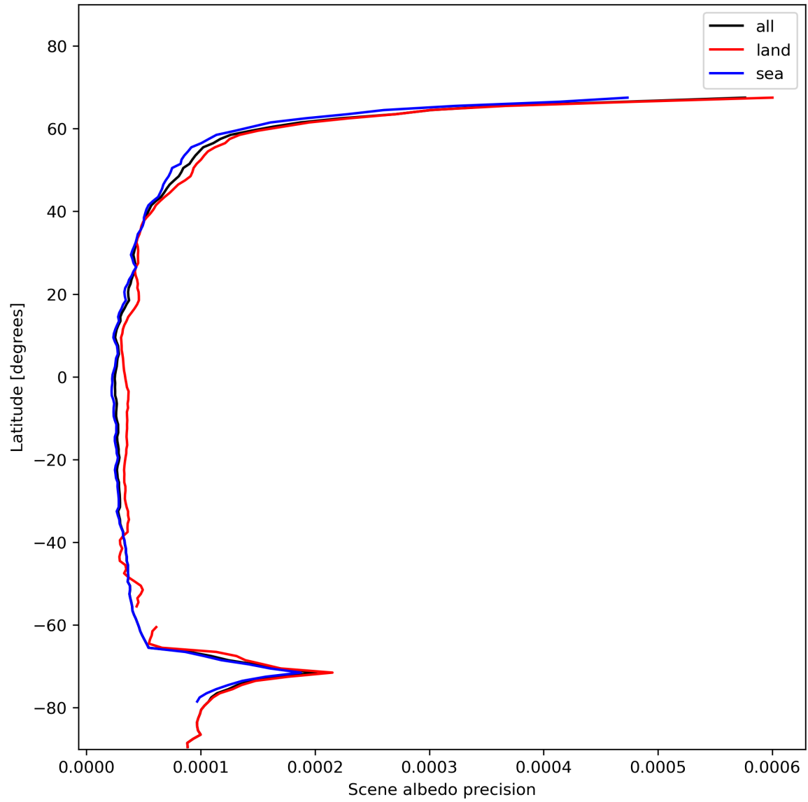
Figure 18: Zonal average of “Scene albedo precision” for 2024-01-16 to 2024-01-18.
