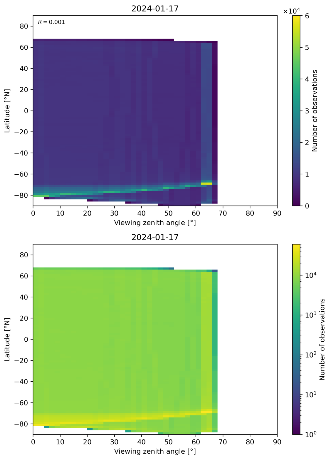
Figure 123: Scatter density plot of “Viewing zenith angle” against “Latitude” for 2024-01-16 to 2024-01-18.
