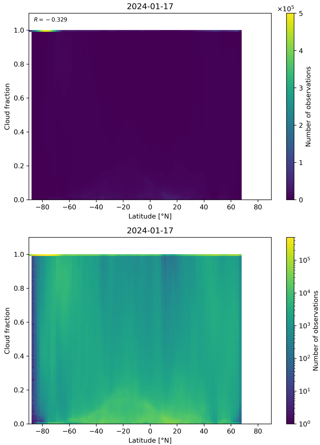
Figure 90: Scatter density plot of “Latitude” against “Cloud fraction” for 2024-01-16 to 2024-01-18.
