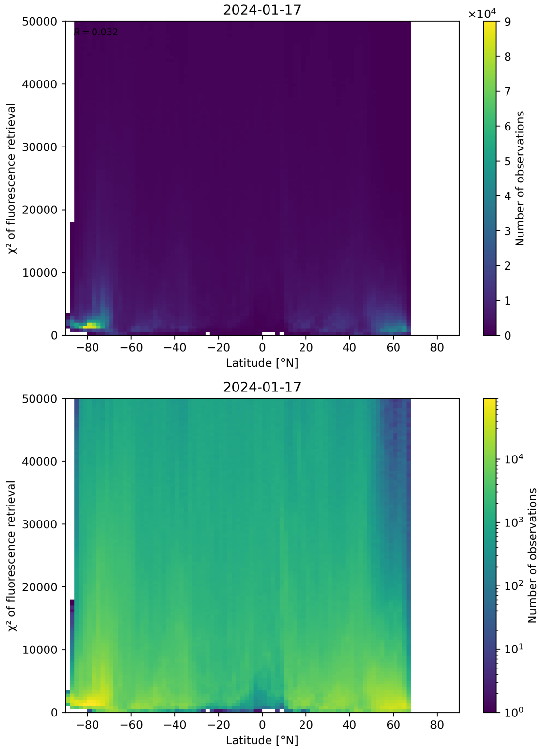
Figure 89: Scatter density plot of “Latitude” against “ \chi^2 of fluorescence retrieval” for 2024-01-16 to 2024-01-18.
