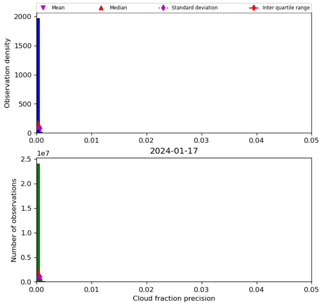
Figure 33: Histogram of “Cloud fraction precision” for 2024-01-16 to 2024-01-18
