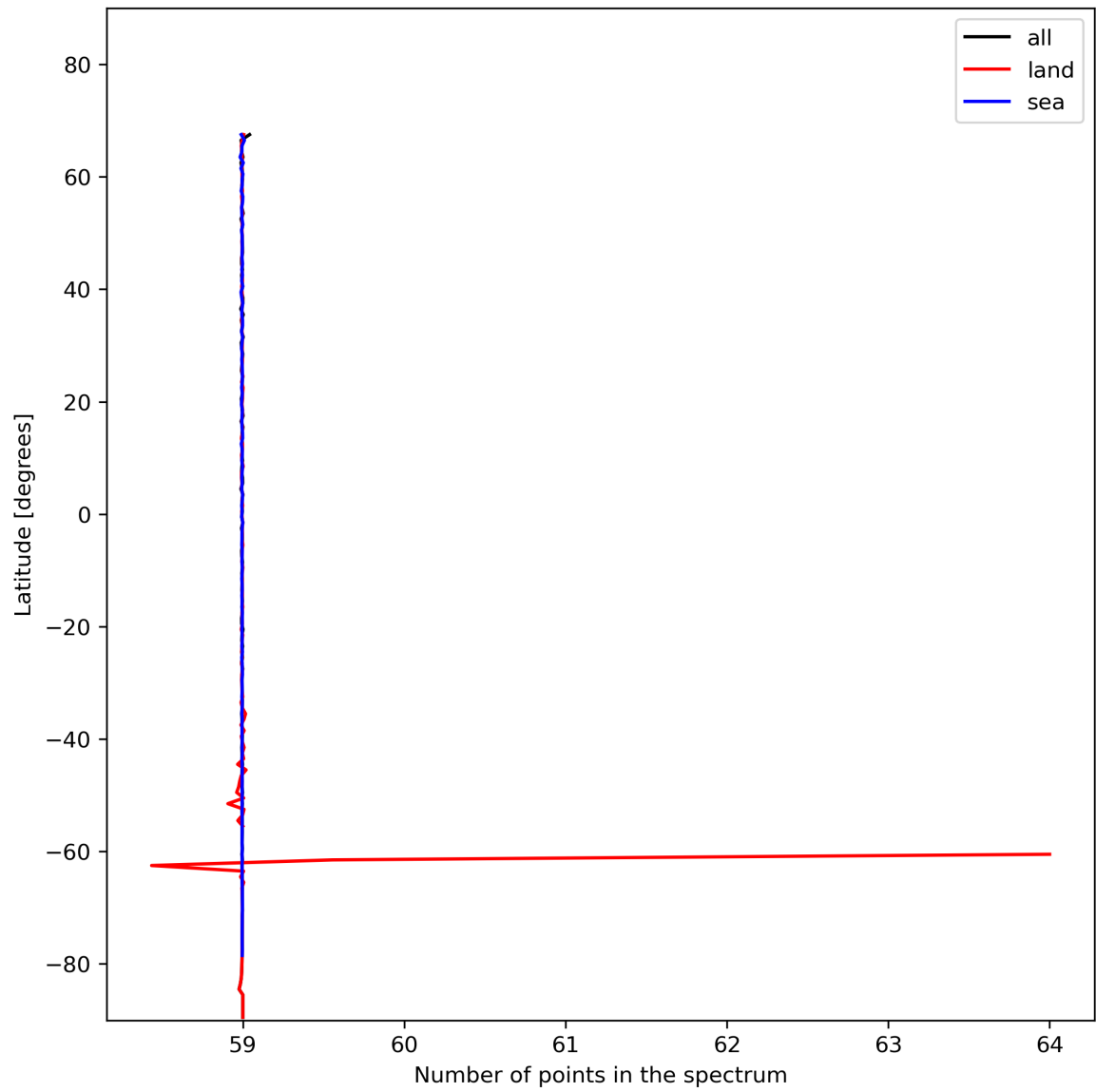
Figure 27: Zonal average of “Number of points in the spectrum” for 2024-01-16 to 2024-01-18.
