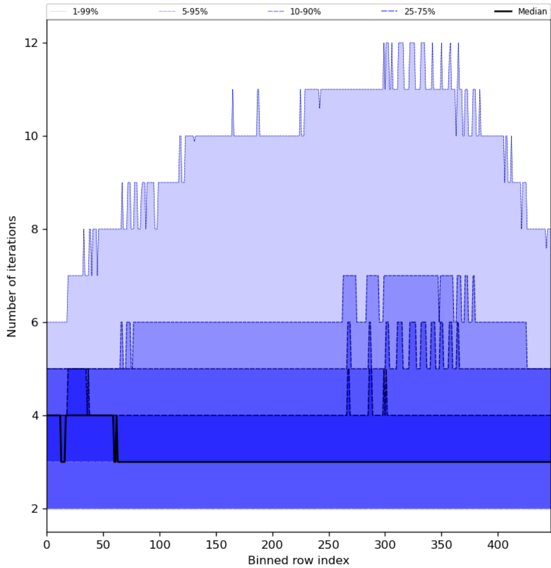
Figure 56: Along track statistics of “Number of iterations” for 2024-01-16 to 2024-01-18
