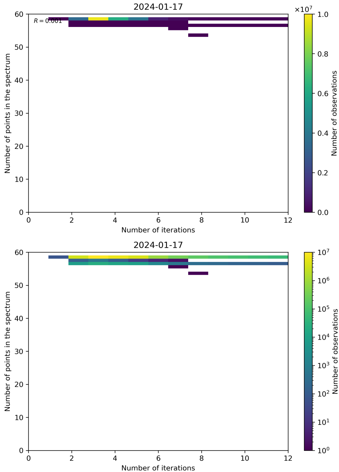
Figure 99: Scatter density plot of “Number of iterations” against “Number of points in the spectrum” for 2024-01-16 to 2024-01-18.
