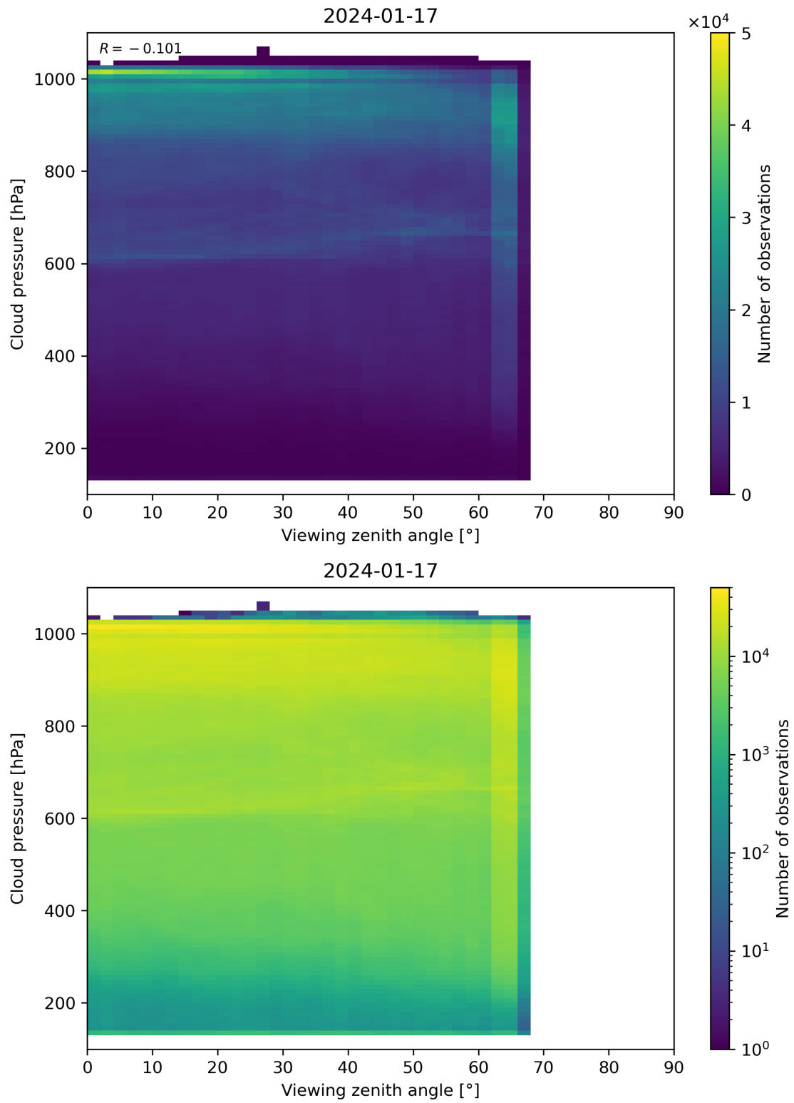
Figure 121: Scatter density plot of “Viewing zenith angle” against “Cloud pressure” for 2024-01-16 to 2024-01-18.
