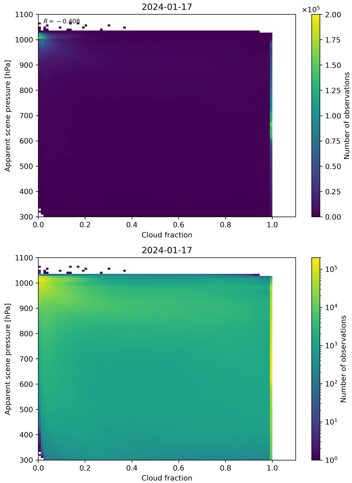
Figure 70: Scatter density plot of “Cloud fraction” against “Apparent scene pressure” for 2024-01-16 to 2024-01-18.
