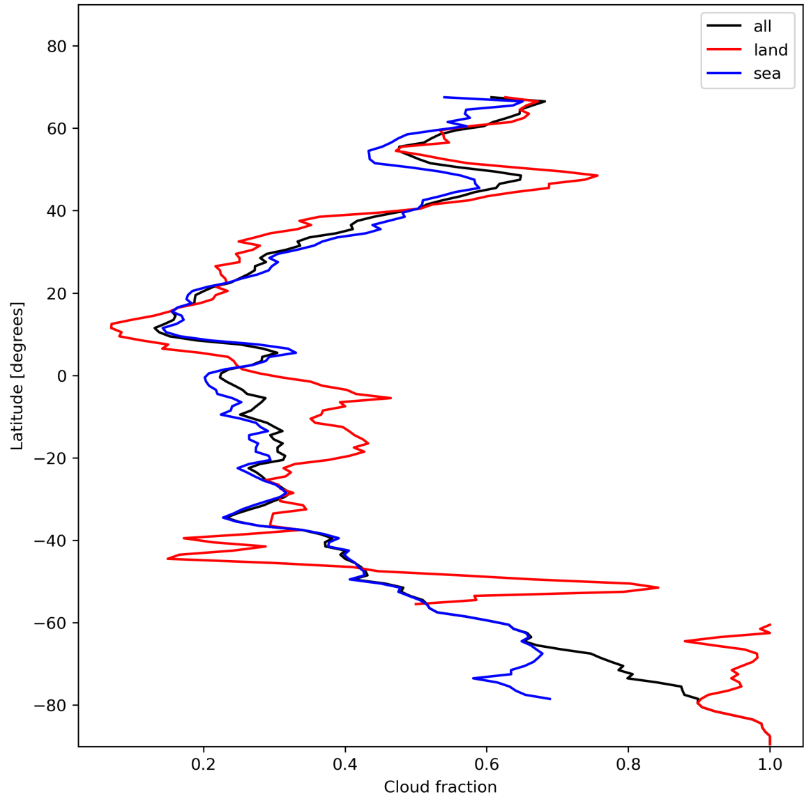
Figure 15: Zonal average of “Cloud fraction” for 2024-01-16 to 2024-01-18.
