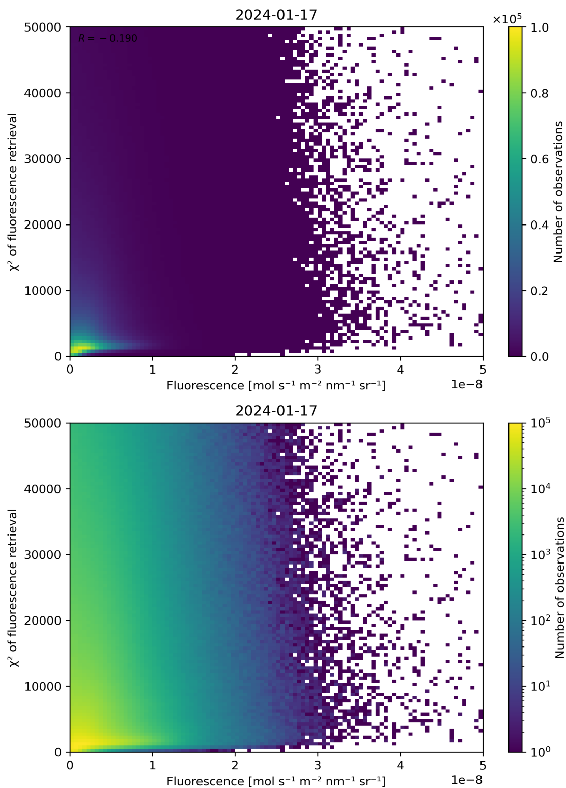
Figure 85: Scatter density plot of “Fluorescence” against “ \chi^2 of fluorescence retrieval” for 2024-01-16 to 2024-01-18.
