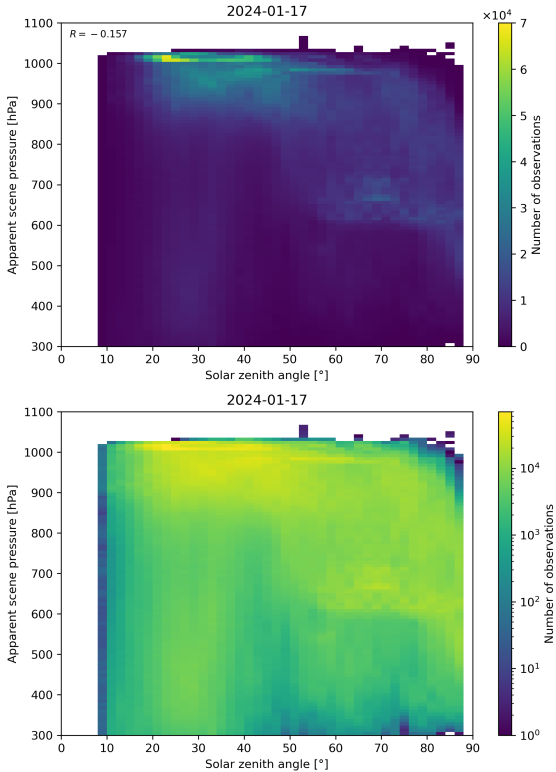
Figure 108: Scatter density plot of “Solar zenith angle” against “Apparent scene pressure” for 2024-01-16 to 2024-01-18.
