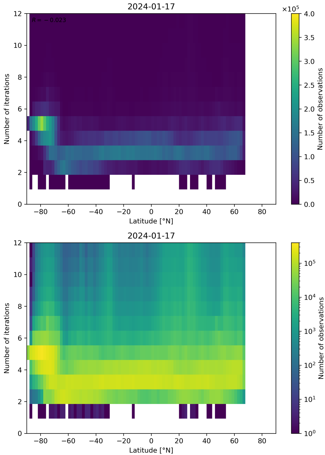
Figure 93: Scatter density plot of “Latitude” against “Number of iterations” for 2024-01-16 to 2024-01-18.
