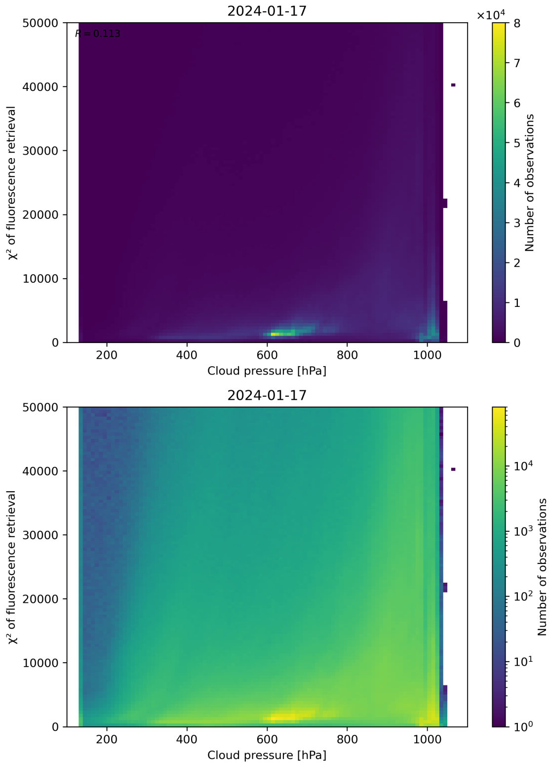
Figure 78: Scatter density plot of “Cloud pressure” against “ \chi^2 of fluorescence retrieval” for 2024-01-16 to 2024-01-18.
