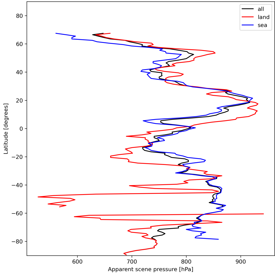
Figure 19: Zonal average of “Apparent scene pressure” for 2024-01-16 to 2024-01-18.
