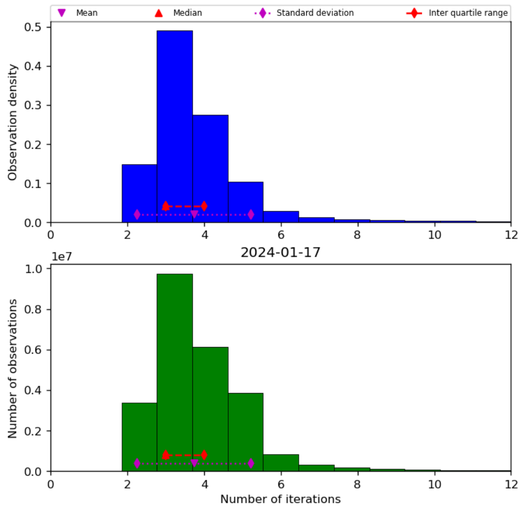
Figure 39: Histogram of “Number of iterations” for 2024-01-16 to 2024-01-18
