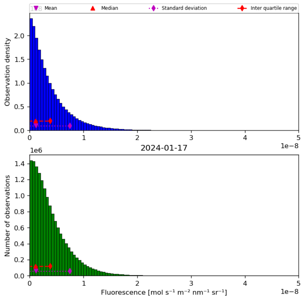
Figure 40: Histogram of “Fluorescence” for 2024-01-16 to 2024-01-18
