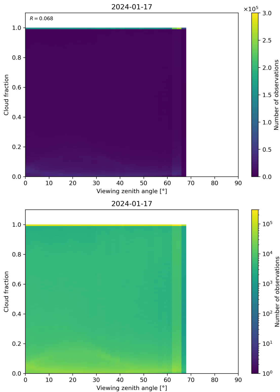
Figure 120: Scatter density plot of “Viewing zenith angle” against “Cloud fraction” for 2024-01-16 to 2024-01-18.
