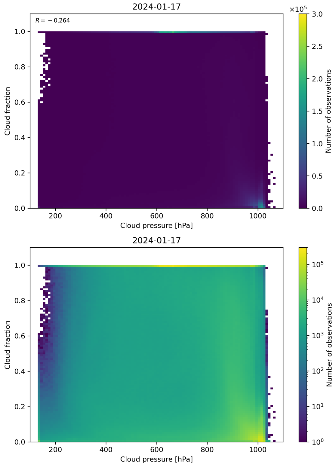
Figure 79: Scatter density plot of “Cloud pressure” against “Cloud fraction” for 2024-01-16 to 2024-01-18.
