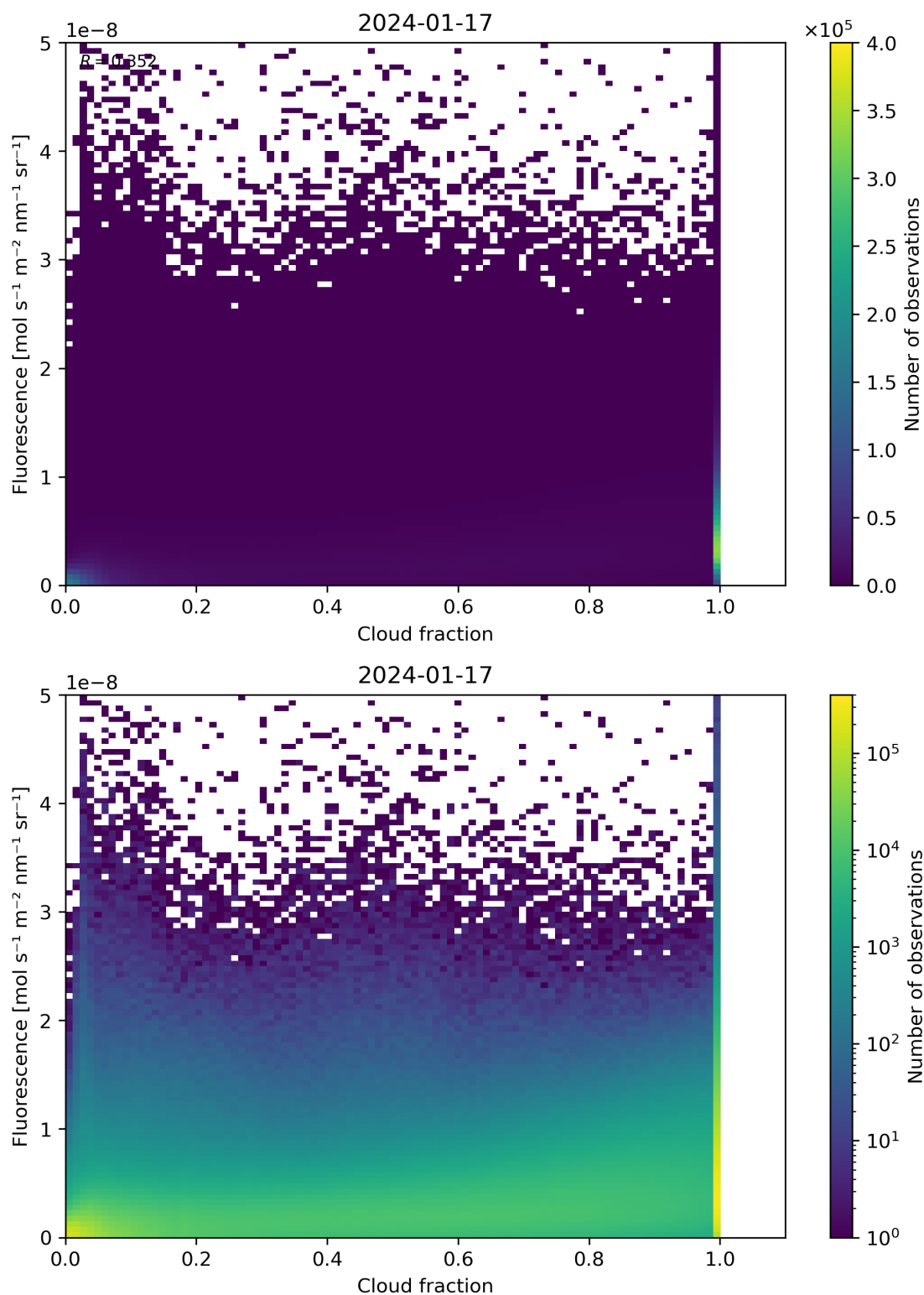
Figure 72: Scatter density plot of “Cloud fraction” against “Fluorescence” for 2024-01-16 to 2024-01-18.
