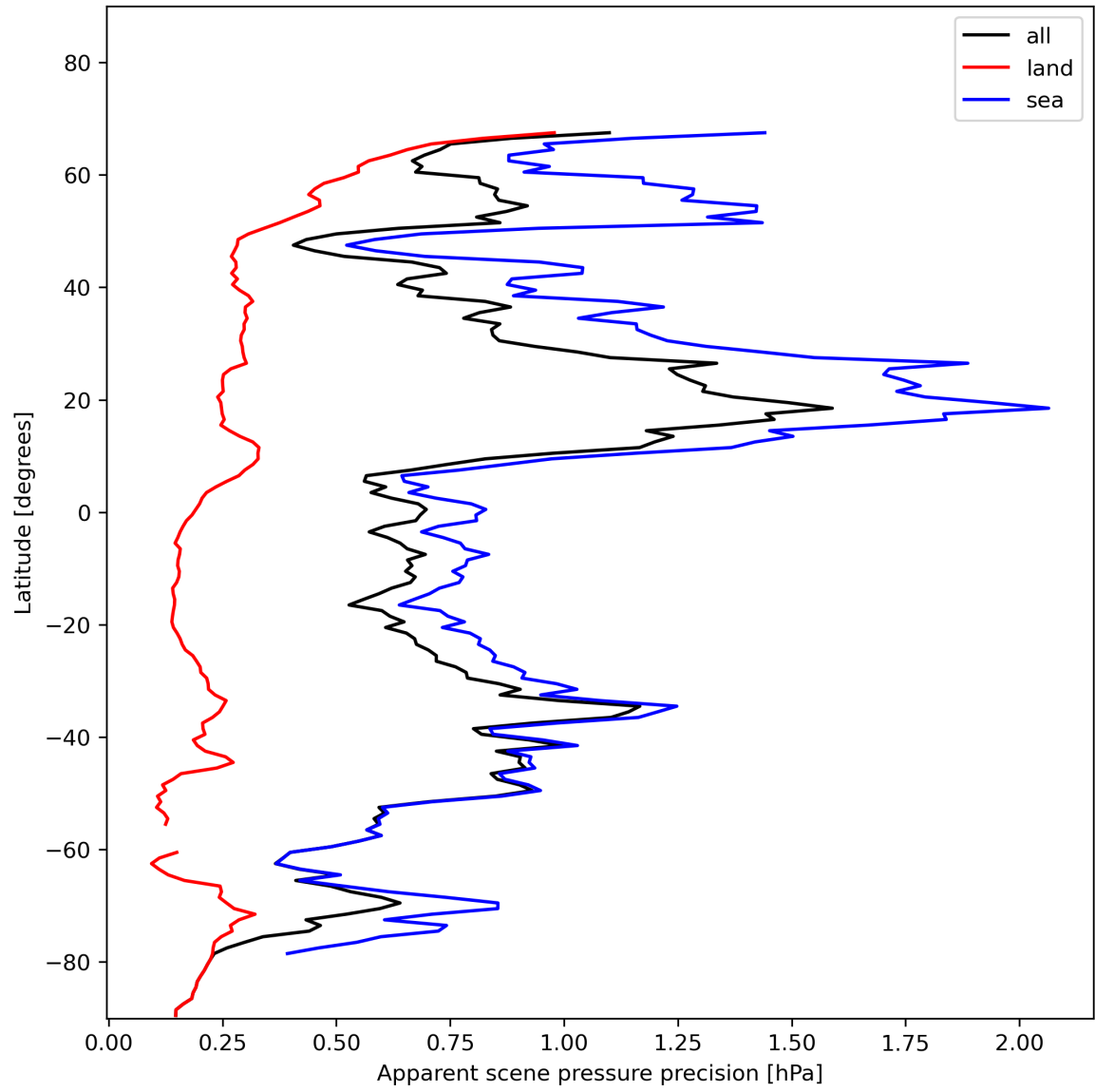
Figure 20: Zonal average of “Apparent scene pressure precision” for 2024-01-16 to 2024-01-18.
