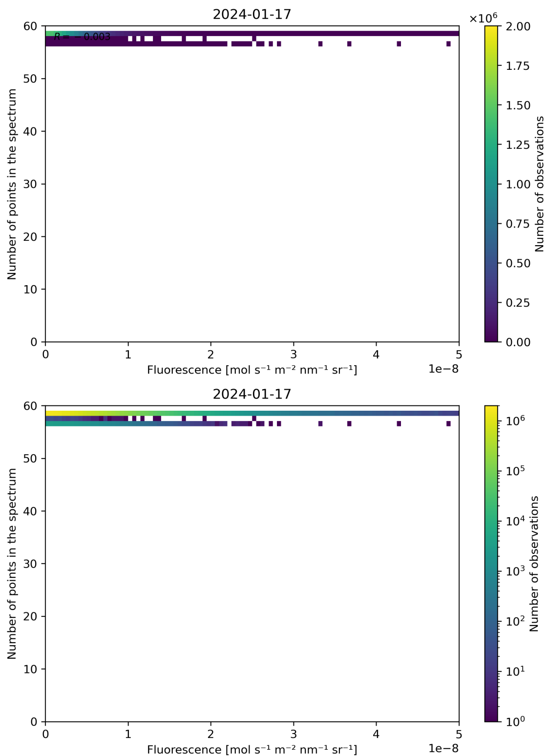
Figure 86: Scatter density plot of “Fluorescence” against “Number of points in the spectrum” for 2024-01-16 to 2024-01-18.
