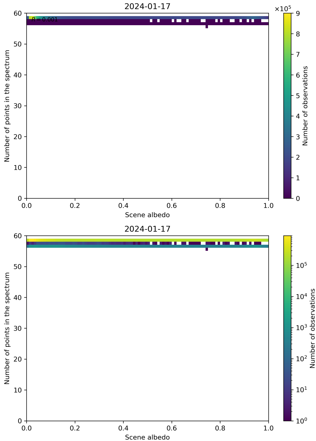
Figure 106: Scatter density plot of “Scene albedo” against “Number of points in the spectrum” for 2024-01-16 to 2024-01-18.
