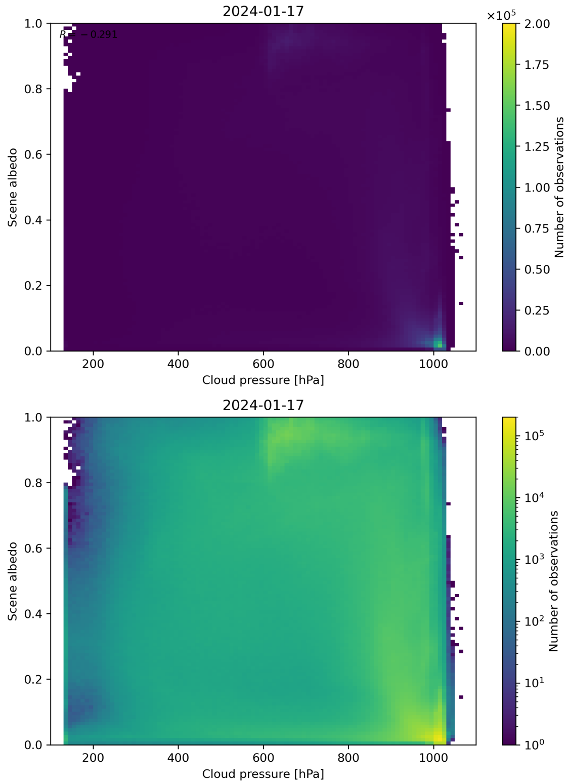
Figure 83: Scatter density plot of “Cloud pressure” against “Scene albedo” for 2024-01-16 to 2024-01-18.
