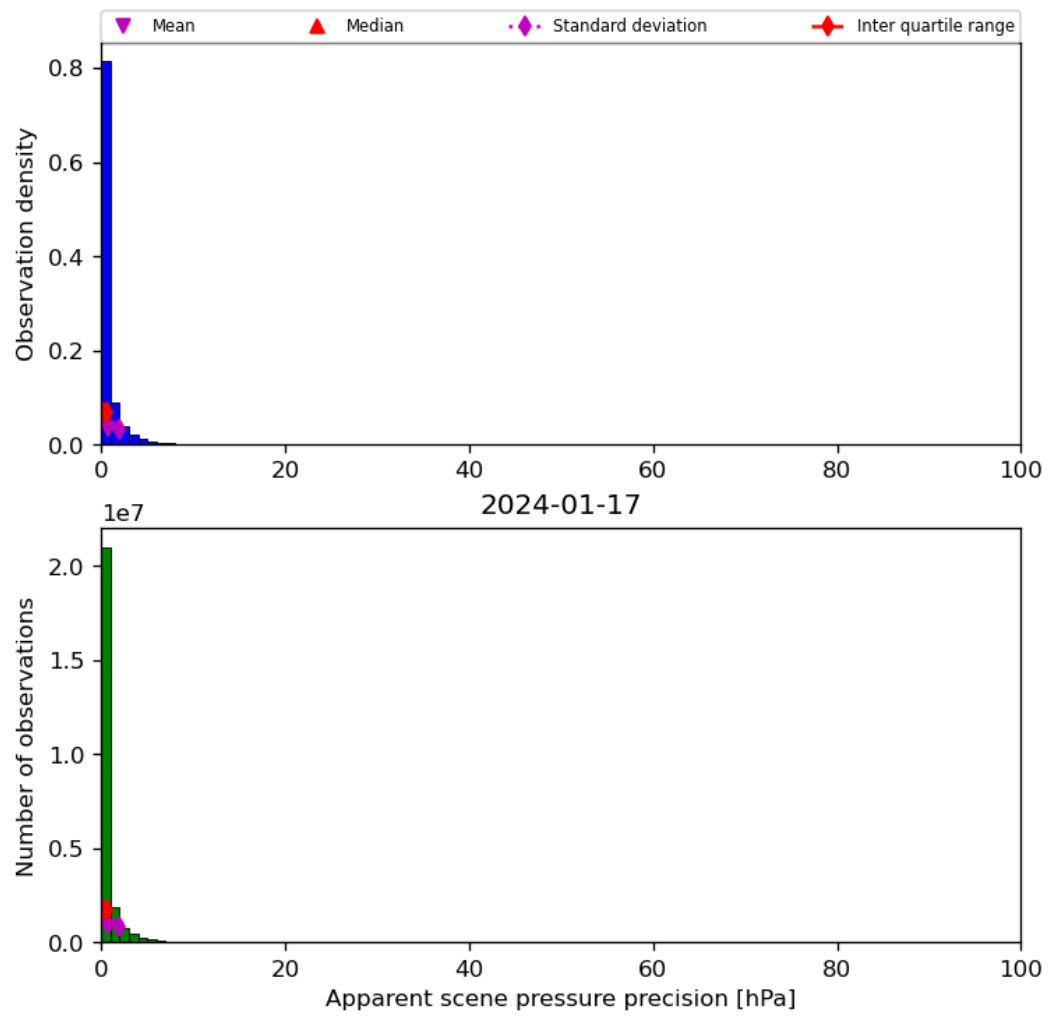
Figure 37: Histogram of “Apparent scene pressure precision” for 2024-01-16 to 2024-01-18
