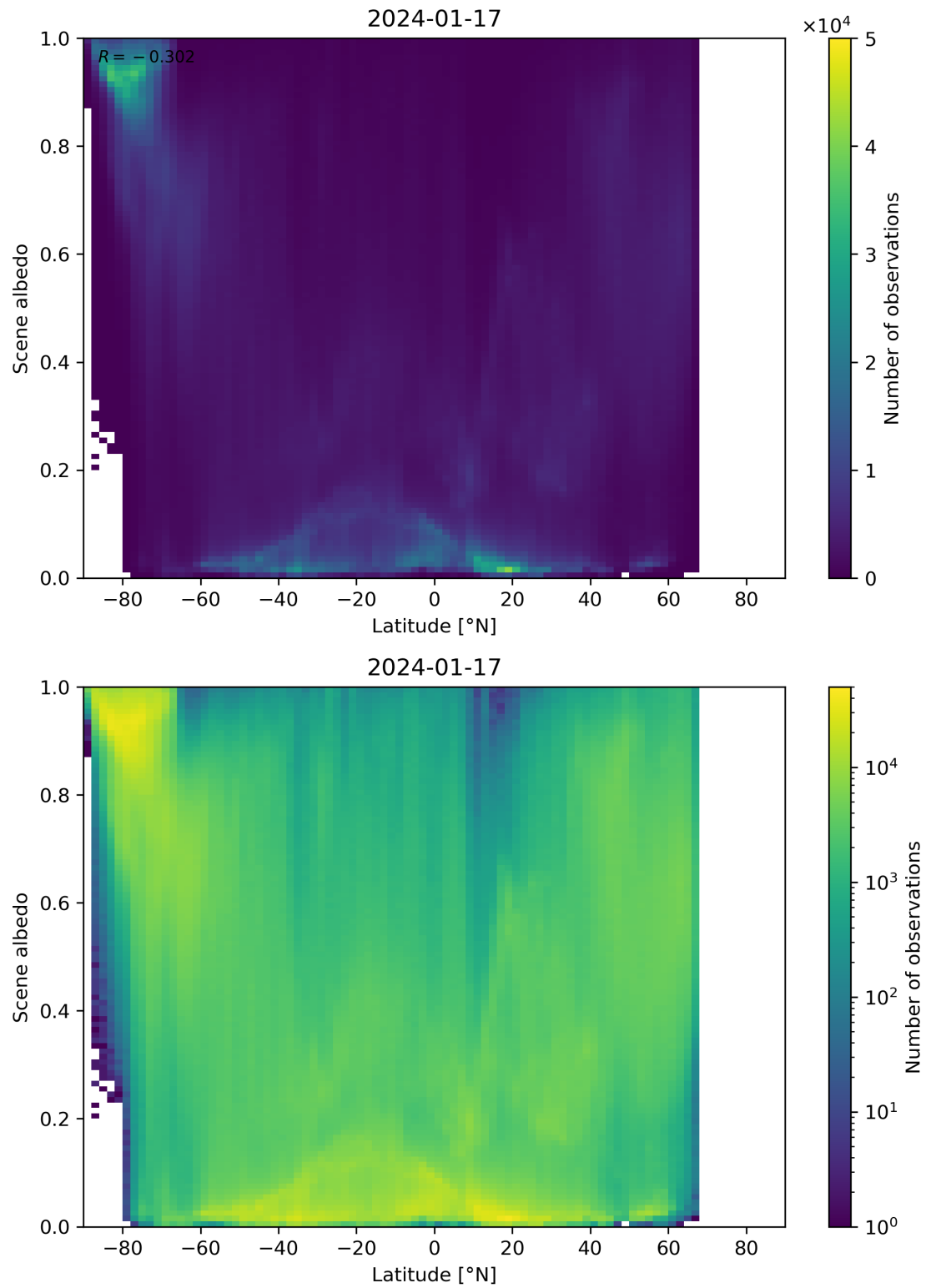
Figure 95: Scatter density plot of “Latitude” against “Scene albedo” for 2024-01-16 to 2024-01-18.
