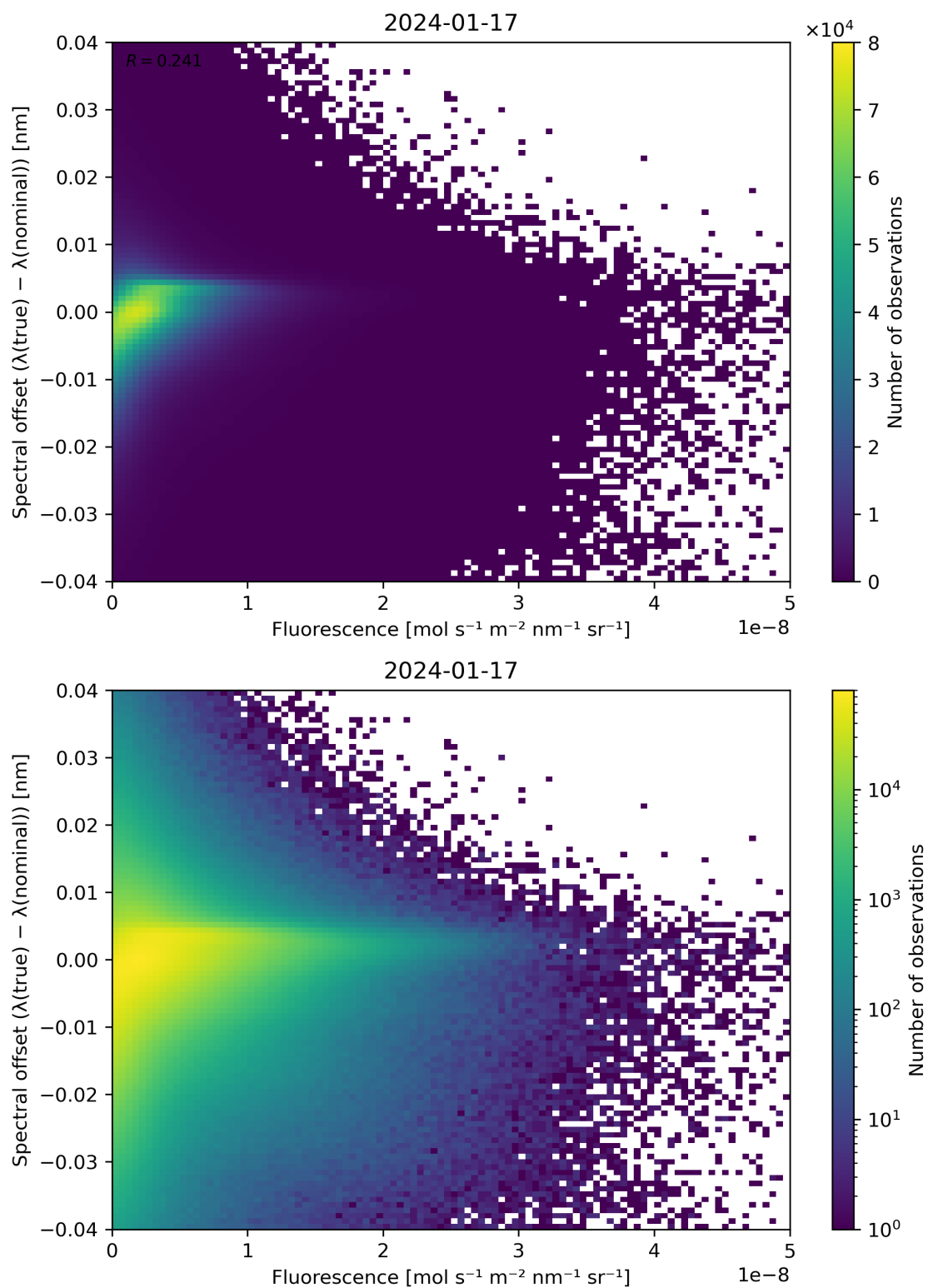
Figure 87: Scatter density plot of “Fluorescence” against “Spectral offset ( \lambda(\text{true}) - \lambda(\text{nominal}) )” for 2024-01-16 to 2024-01-18.
