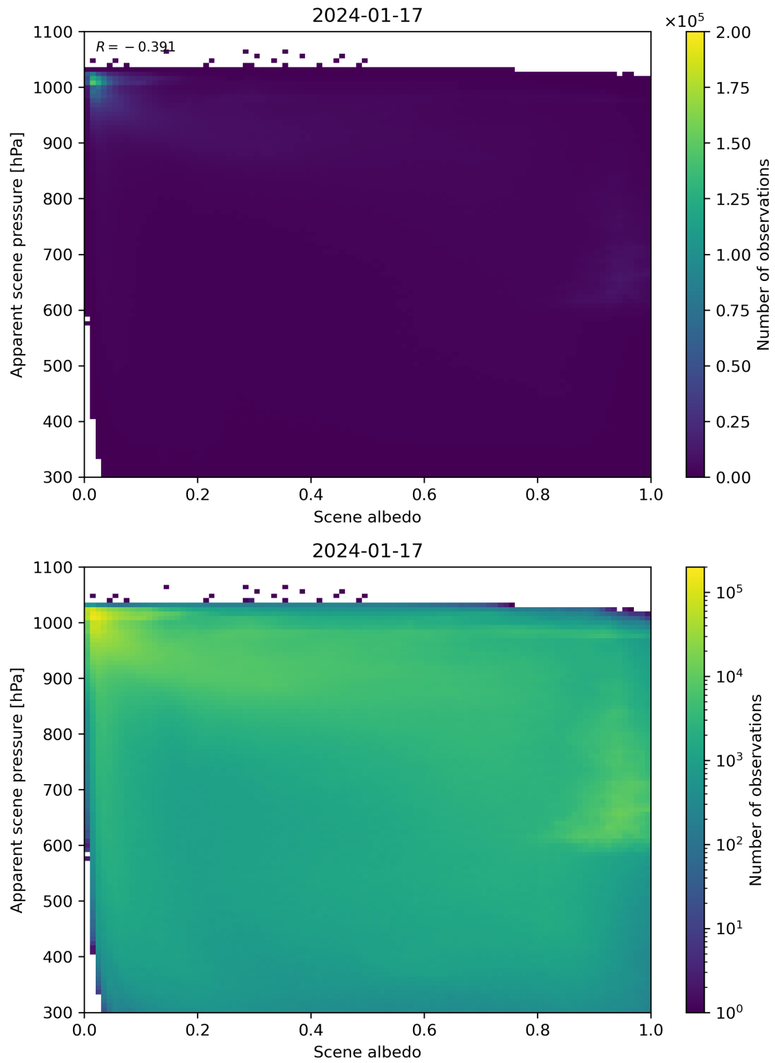
Figure 102: Scatter density plot of “Scene albedo” against “Apparent scene pressure” for 2024-01-16 to 2024-01-18.
