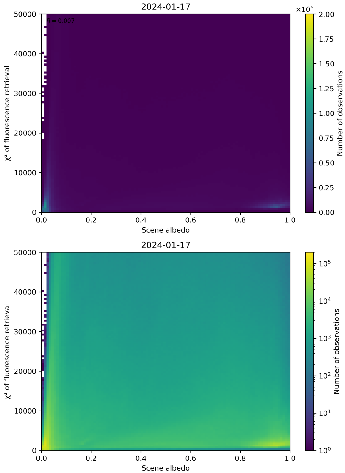
Figure 103: Scatter density plot of “Scene albedo” against “ \chi^2 of fluorescence retrieval” for 2024-01-16 to 2024-01-18.
