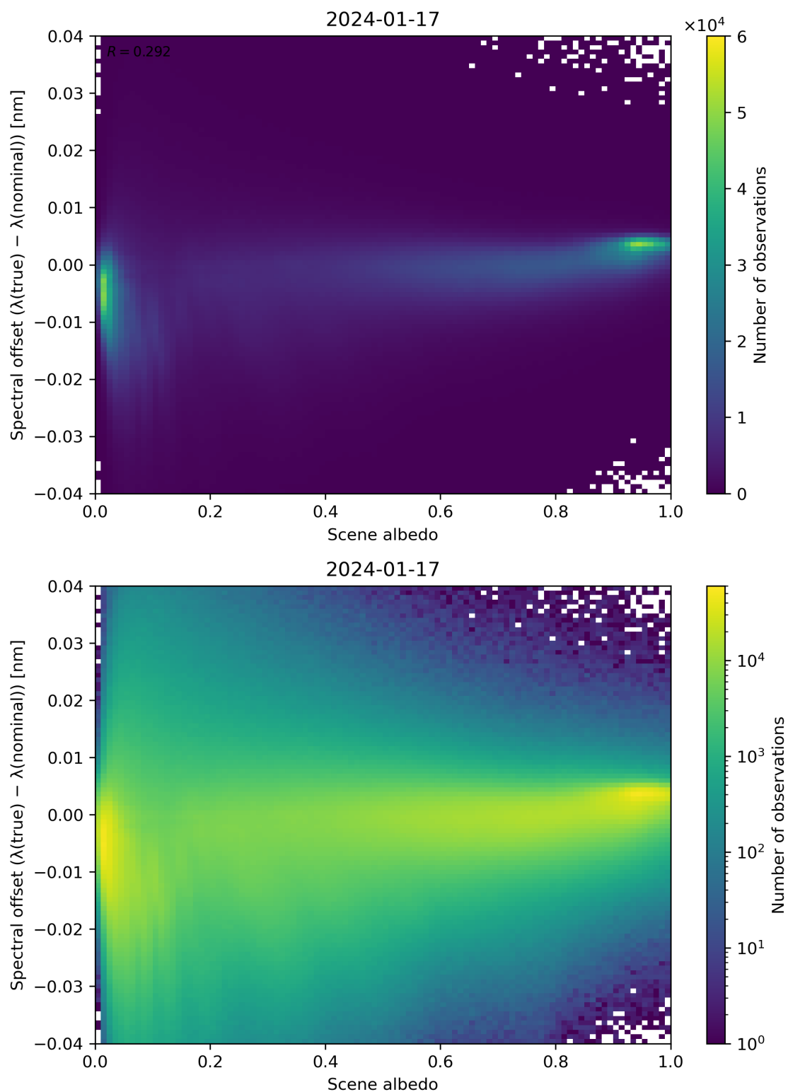
Figure 107: Scatter density plot of “Scene albedo” against “Spectral offset ( \lambda(\text{true}) - \lambda(\text{nominal}) )” for 2024-01-16 to 2024-01-18.
