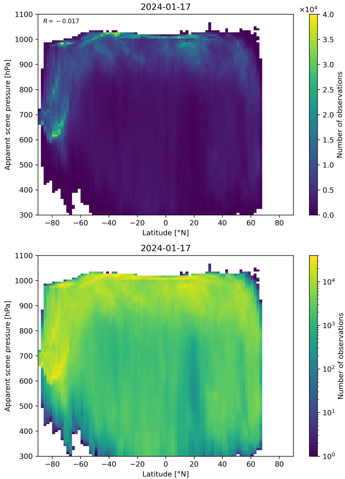
Figure 88: Scatter density plot of “Latitude” against “Apparent scene pressure” for 2024-01-16 to 2024-01-18.
