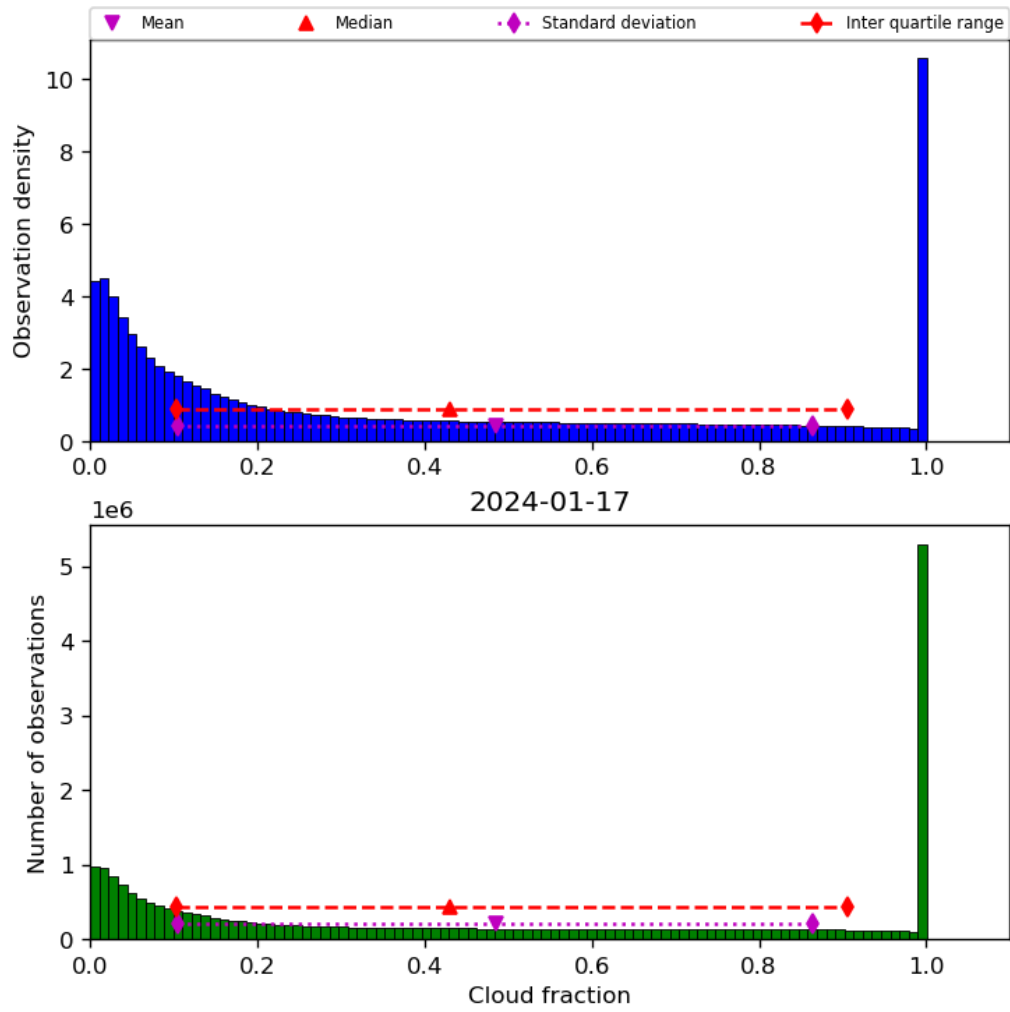
Figure 32: Histogram of “Cloud fraction” for 2024-01-16 to 2024-01-18
