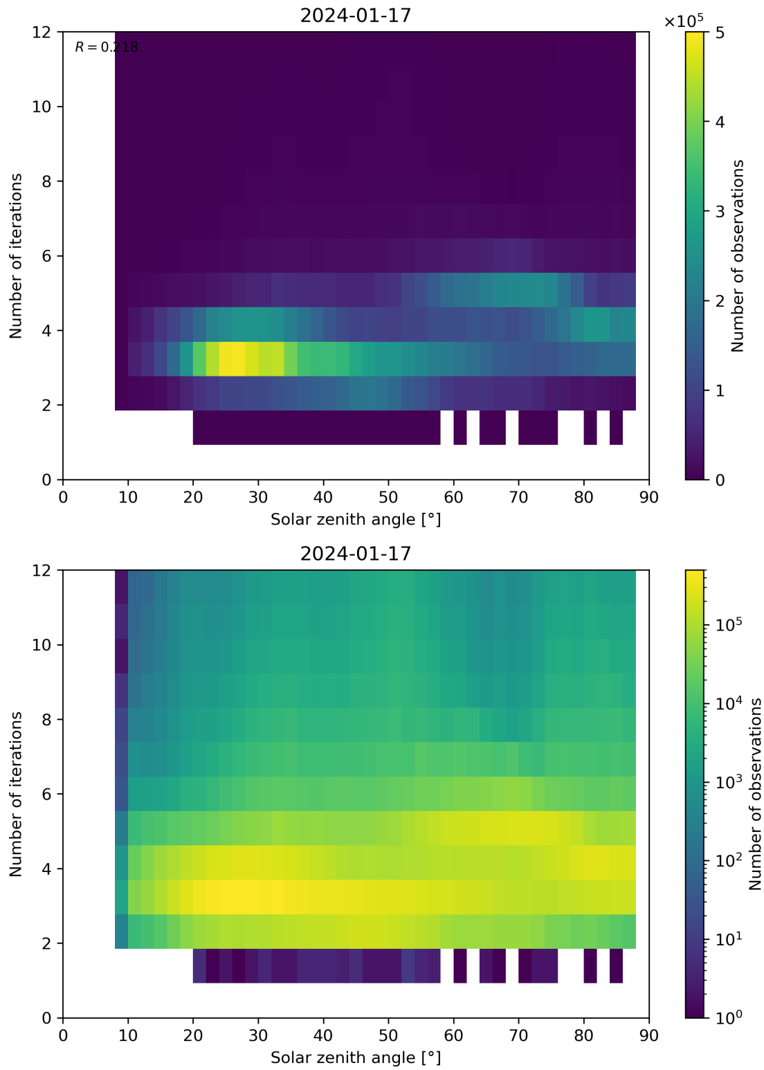
Figure 114: Scatter density plot of “Solar zenith angle” against “Number of iterations” for 2024-01-16 to 2024-01-18.
