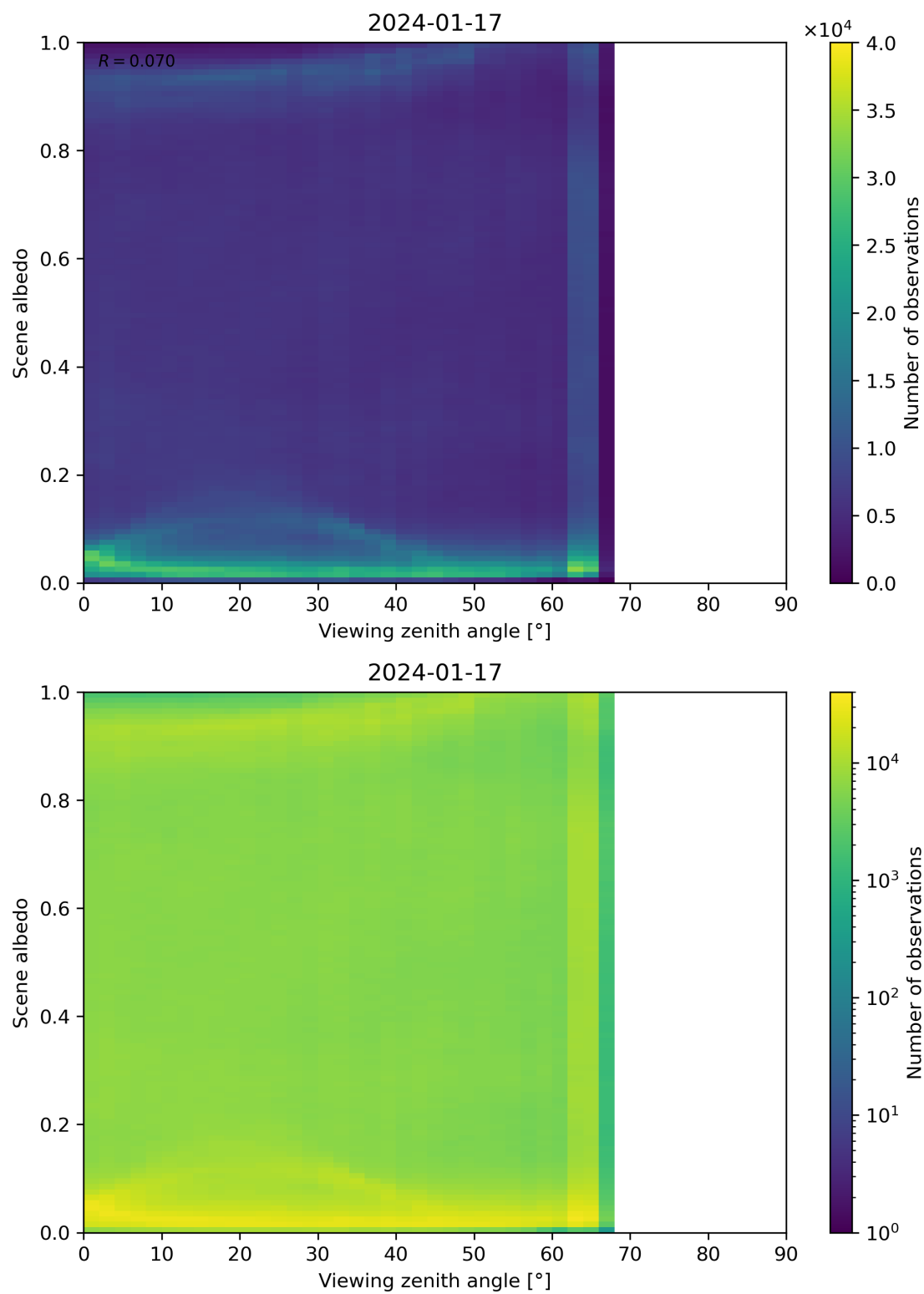
Figure 126: Scatter density plot of “Viewing zenith angle” against “Scene albedo” for 2024-01-16 to 2024-01-18.
