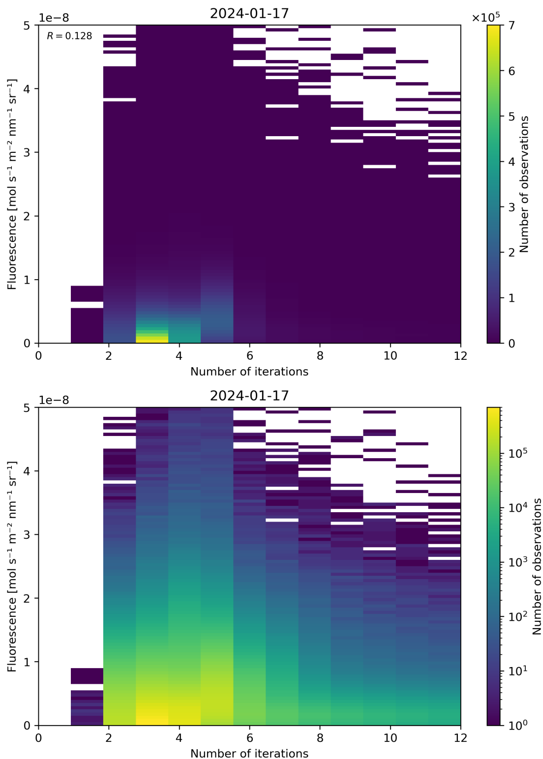
Figure 98: Scatter density plot of “Number of iterations” against “Fluorescence” for 2024-01-16 to 2024-01-18.
