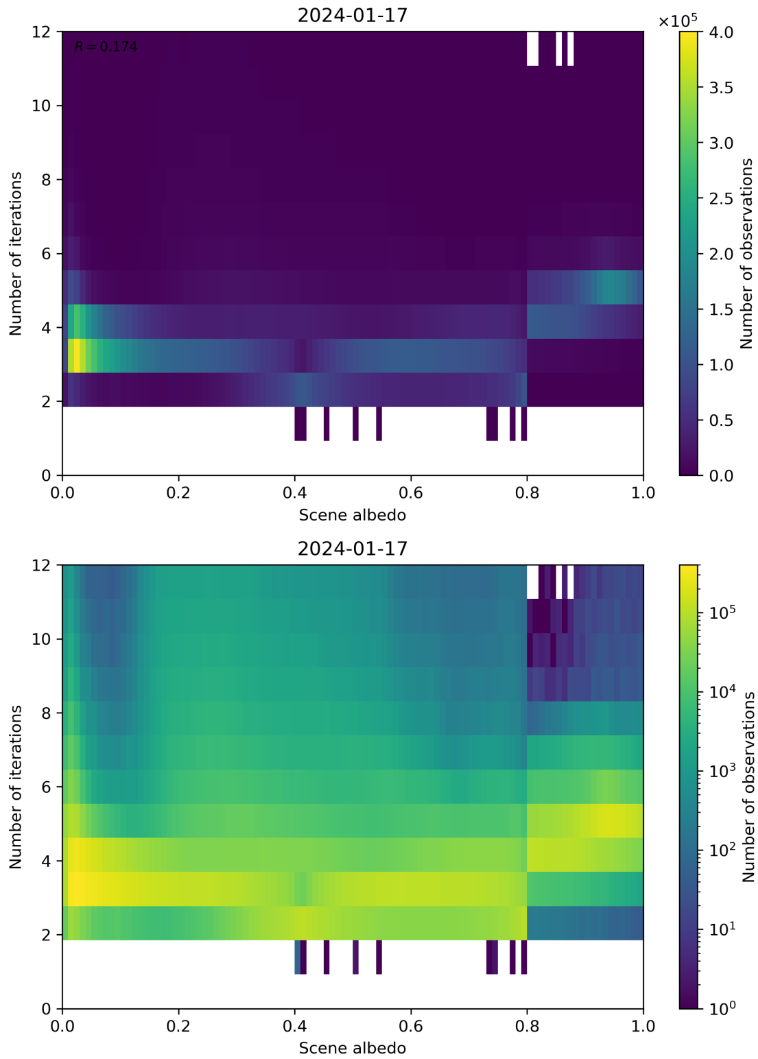
Figure 105: Scatter density plot of “Scene albedo” against “Number of iterations” for 2024-01-16 to 2024-01-18.
