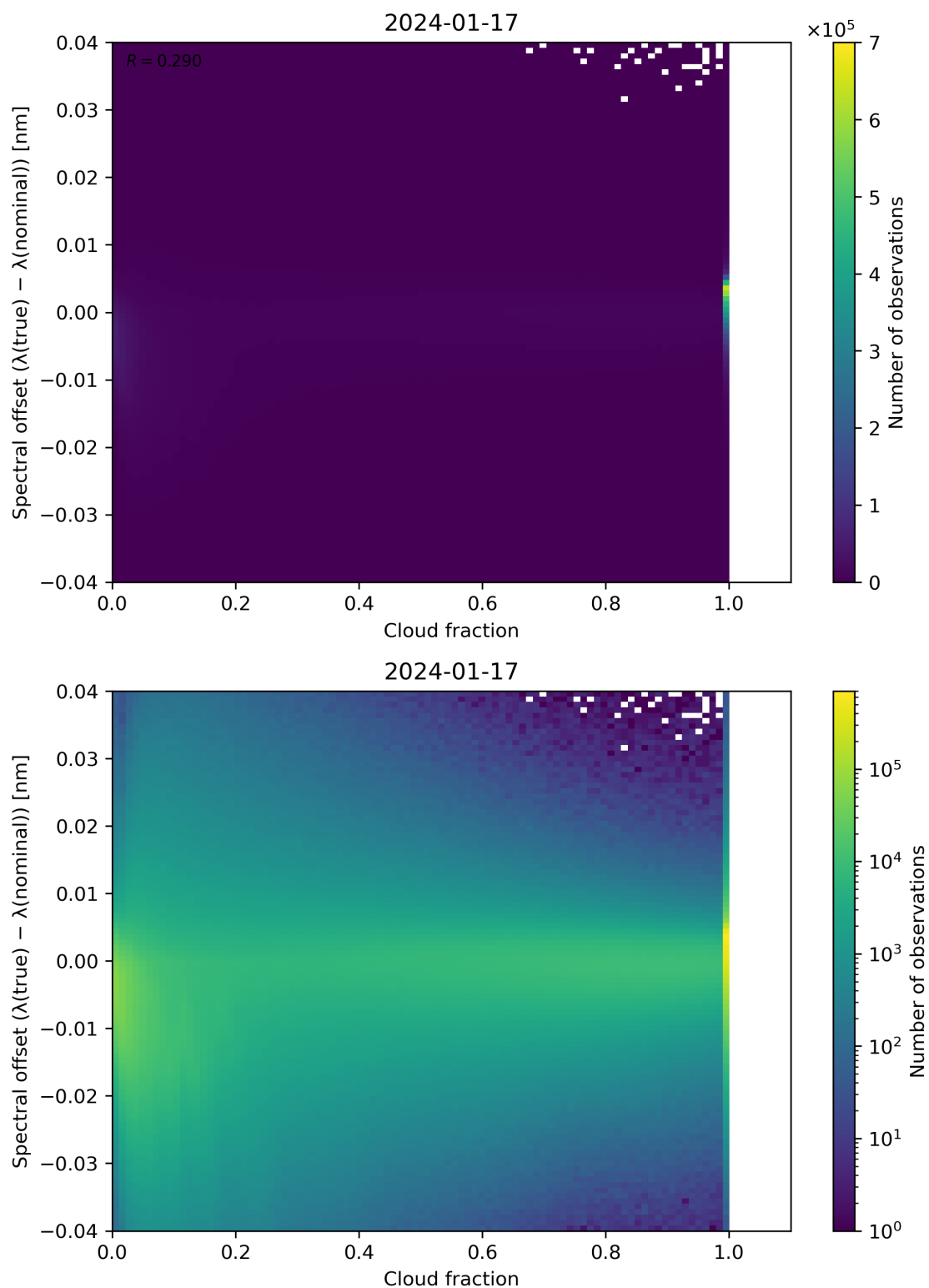
Figure 76: Scatter density plot of “Cloud fraction” against “Spectral offset ( \lambda(\text{true}) - \lambda(\text{nominal}) )” for 2024-01-16 to 2024-01-18.
