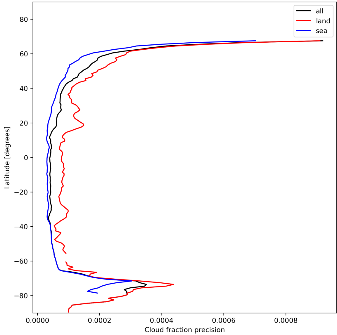
Figure 16: Zonal average of “Cloud fraction precision” for 2024-01-16 to 2024-01-18.
