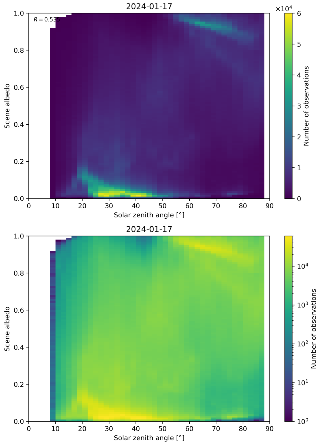
Figure 116: Scatter density plot of “Solar zenith angle” against “Scene albedo” for 2024-01-16 to 2024-01-18.
