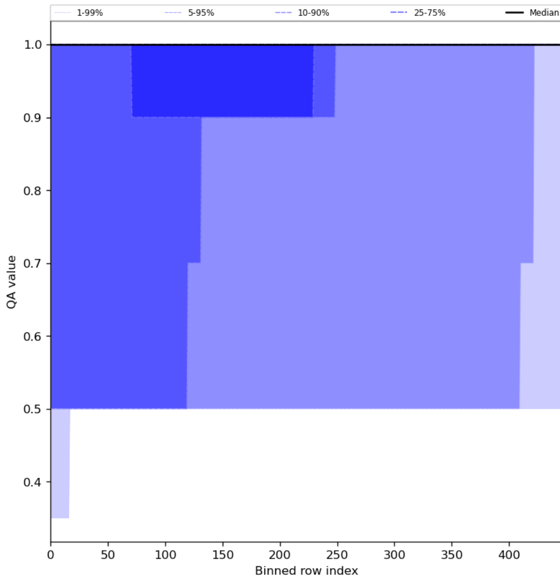
Figure 46: Along track statistics of “QA value” for 2024-01-16 to 2024-01-18
