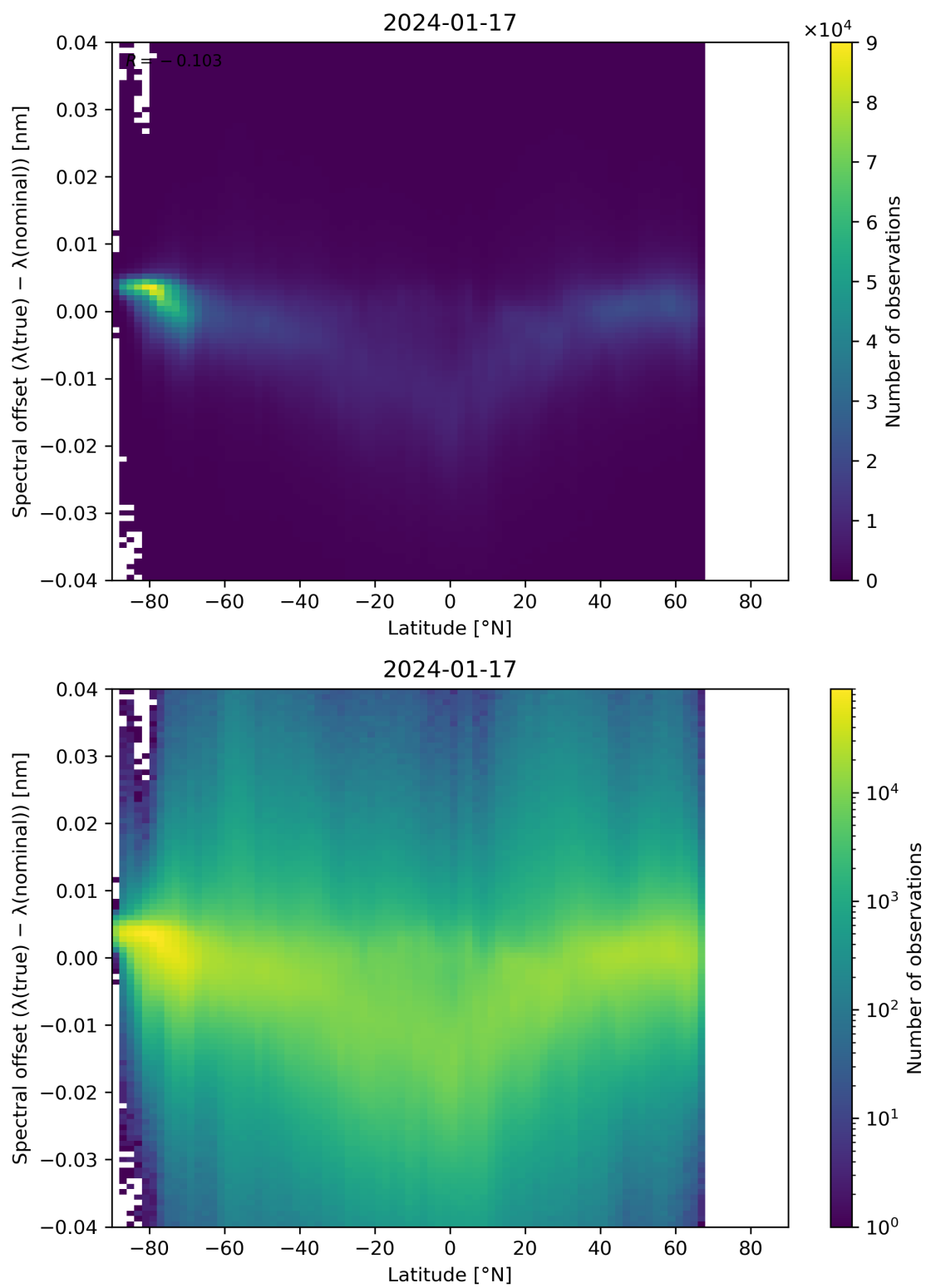
Figure 96: Scatter density plot of “Latitude” against “Spectral offset ( \lambda(\text{true}) - \lambda(\text{nominal}) )” for 2024-01-16 to 2024-01-18.
