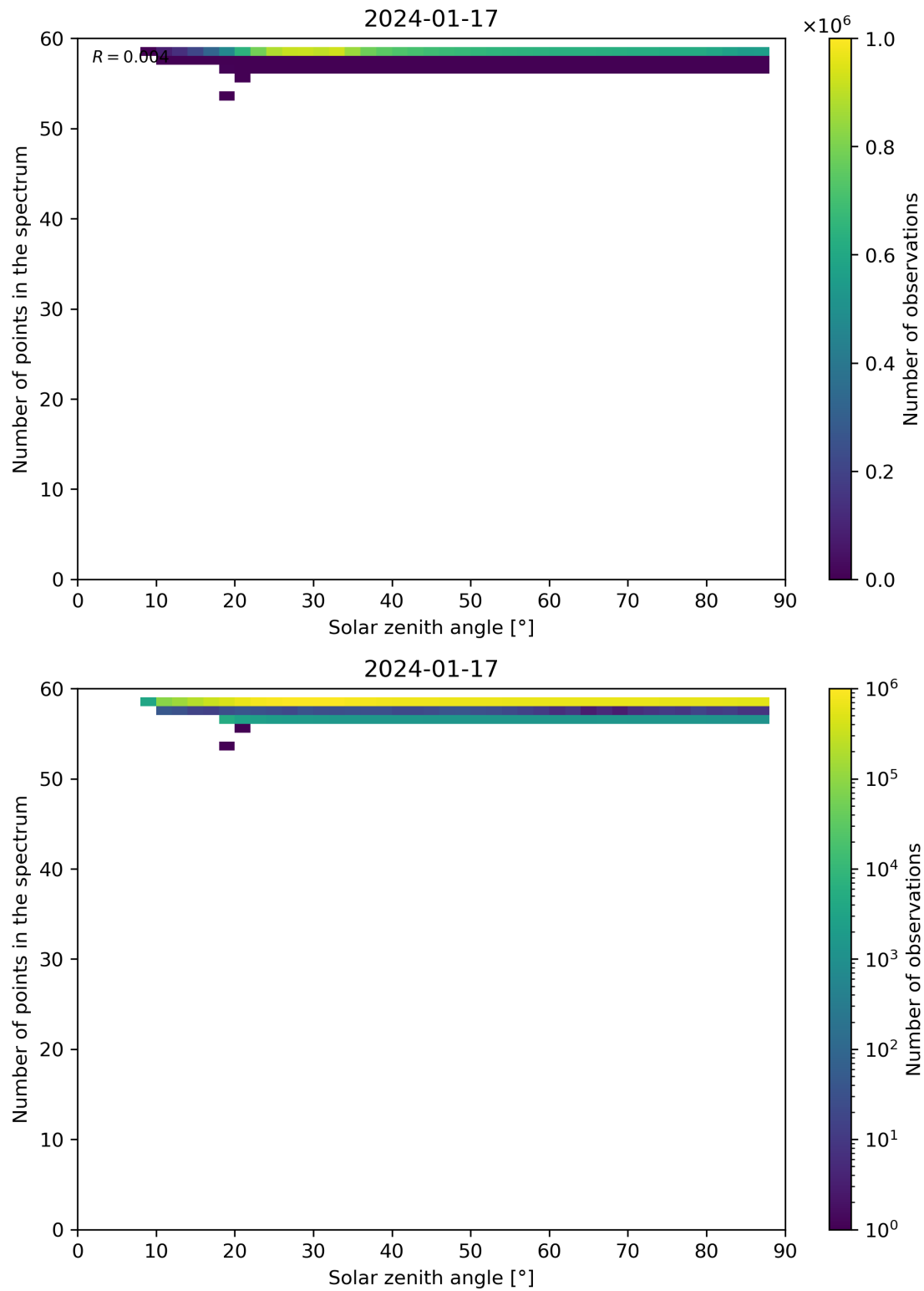
Figure 115: Scatter density plot of “Solar zenith angle” against “Number of points in the spectrum” for 2024-01-16 to 2024-01-18.
