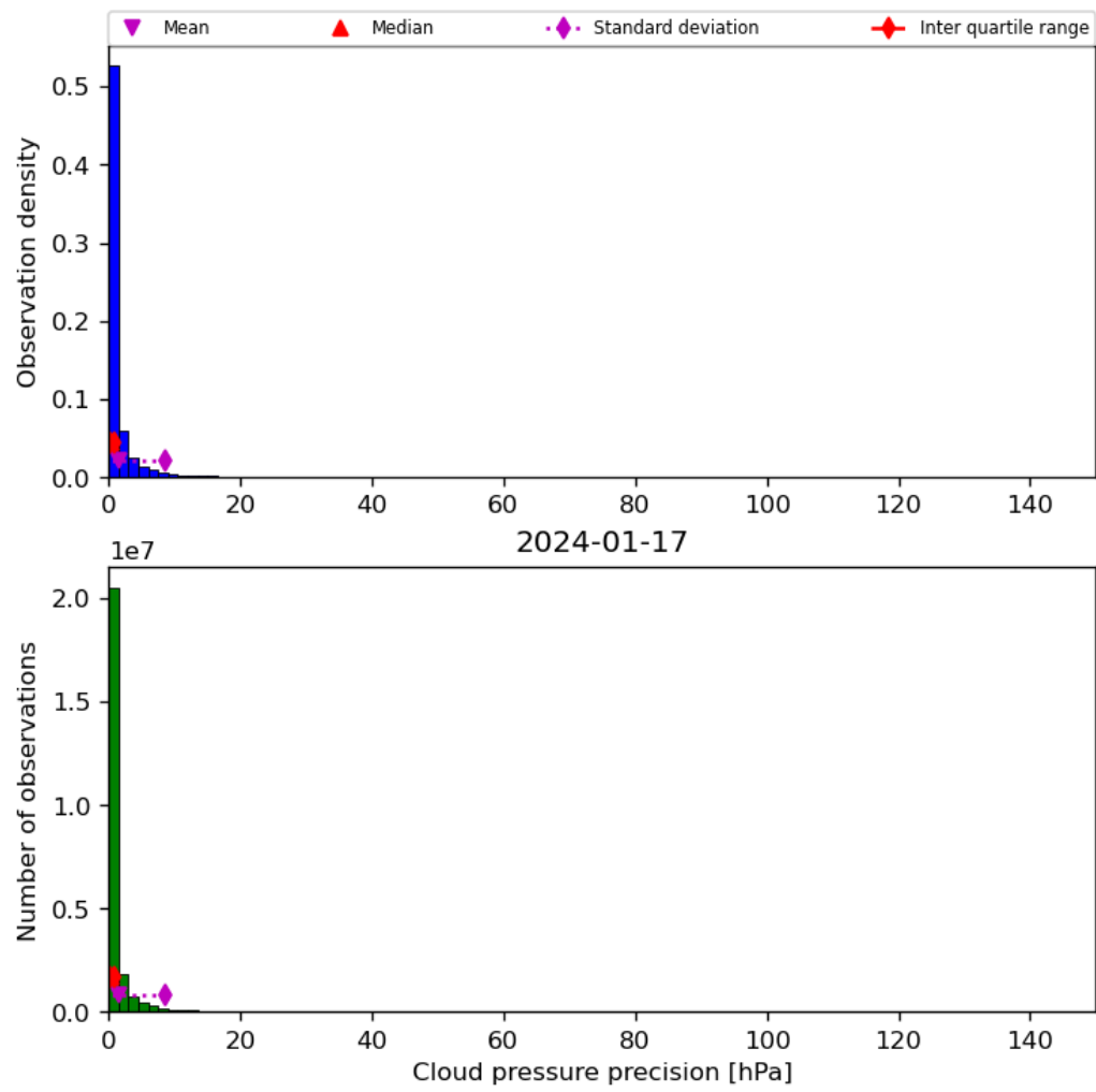
Figure 31: Histogram of “Cloud pressure precision” for 2024-01-16 to 2024-01-18
