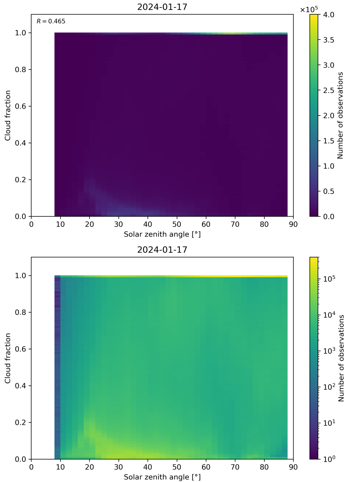
Figure 110: Scatter density plot of “Solar zenith angle” against “Cloud fraction” for 2024-01-16 to 2024-01-18.
