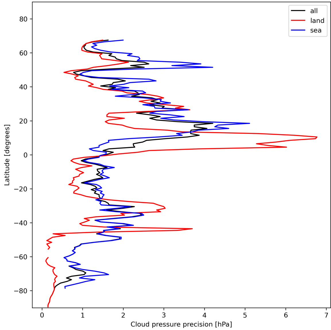
Figure 14: Zonal average of “Cloud pressure precision” for 2024-01-16 to 2024-01-18.
