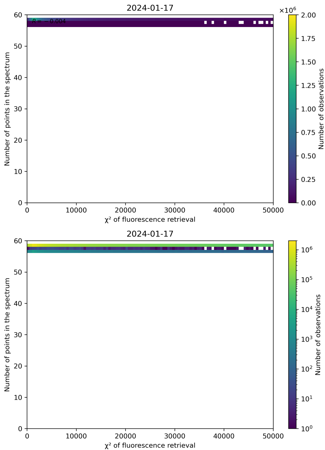
Figure 68: Scatter density plot of " \chi^2 of fluorescence retrieval" against "Number of points in the spectrum" for 2024-01-16 to 2024-01-18.
