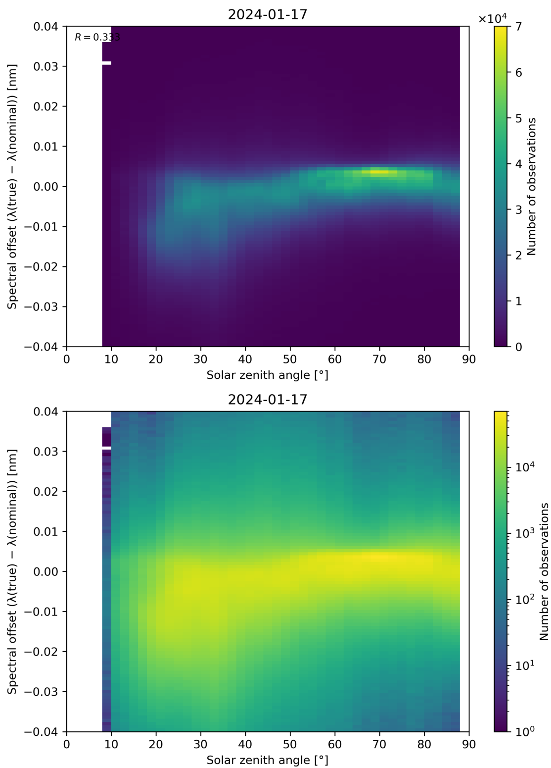
Figure 117: Scatter density plot of “Solar zenith angle” against “Spectral offset ( \lambda(\text{true}) - \lambda(\text{nominal}) )” for 2024-01-16 to 2024-01-18.
