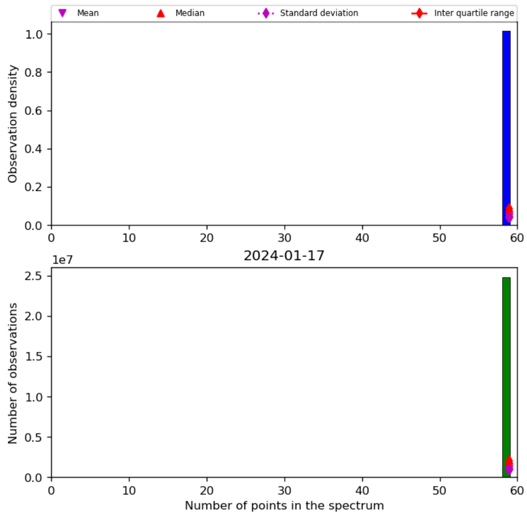
Figure 44: Histogram of “Number of points in the spectrum” for 2024-01-16 to 2024-01-18
