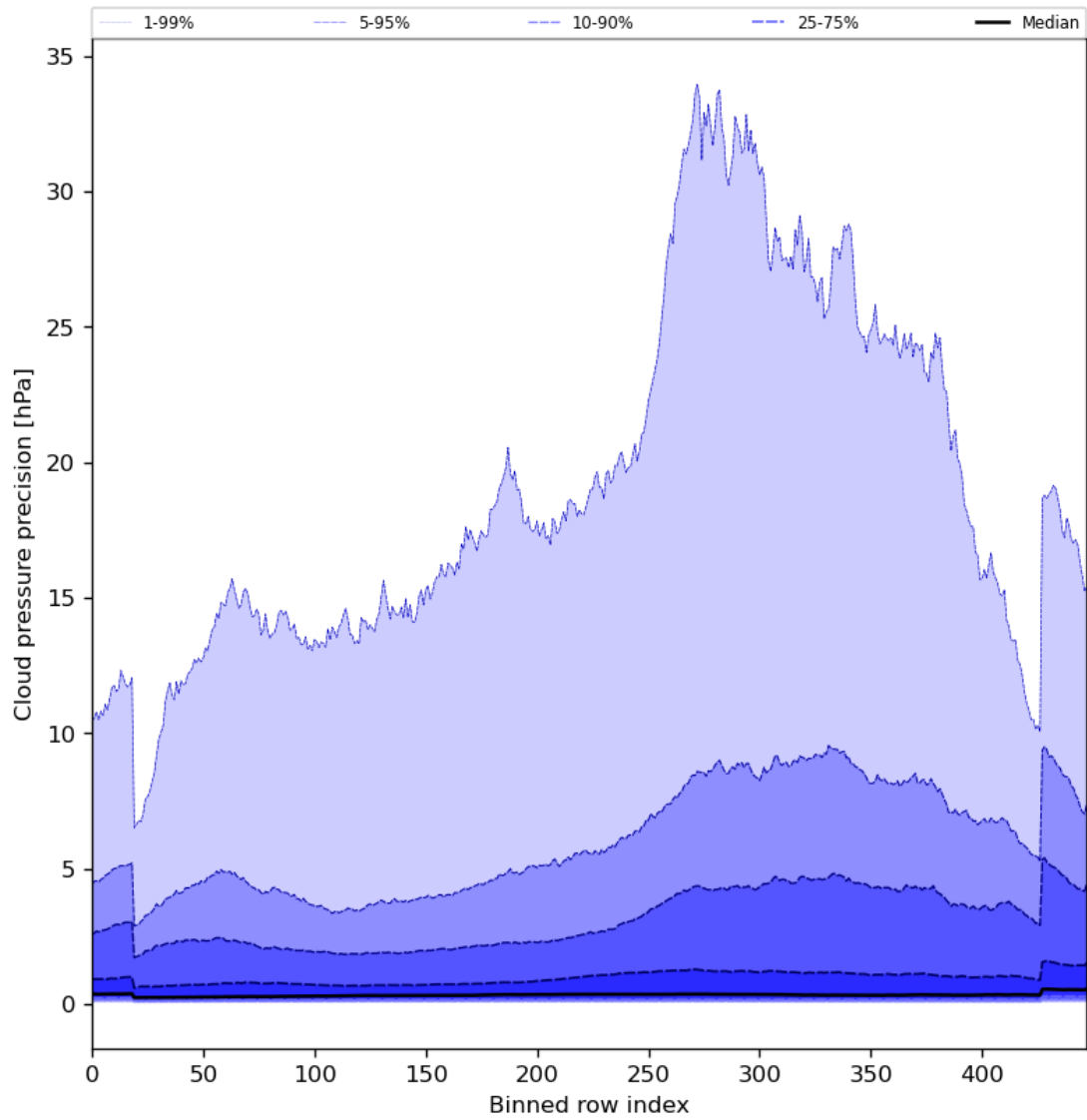
Figure 48: Along track statistics of “Cloud pressure precision” for 2024-01-16 to 2024-01-18
