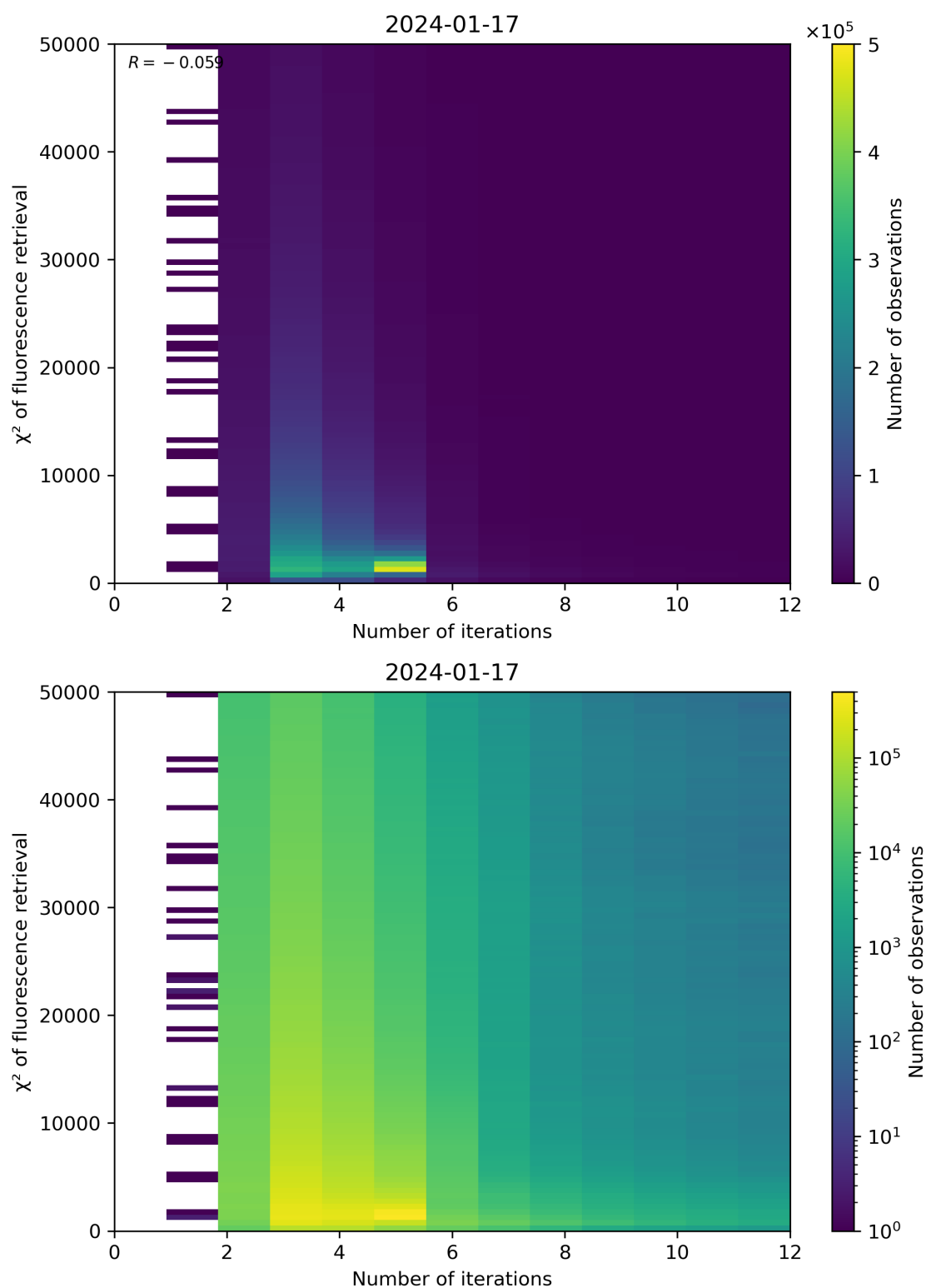
Figure 97: Scatter density plot of “Number of iterations” against “ \chi^2 of fluorescence retrieval” for 2024-01-16 to 2024-01-18.
