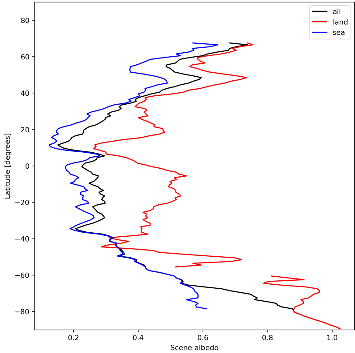
Figure 17: Zonal average of “Scene albedo” for 2024-01-16 to 2024-01-18.
