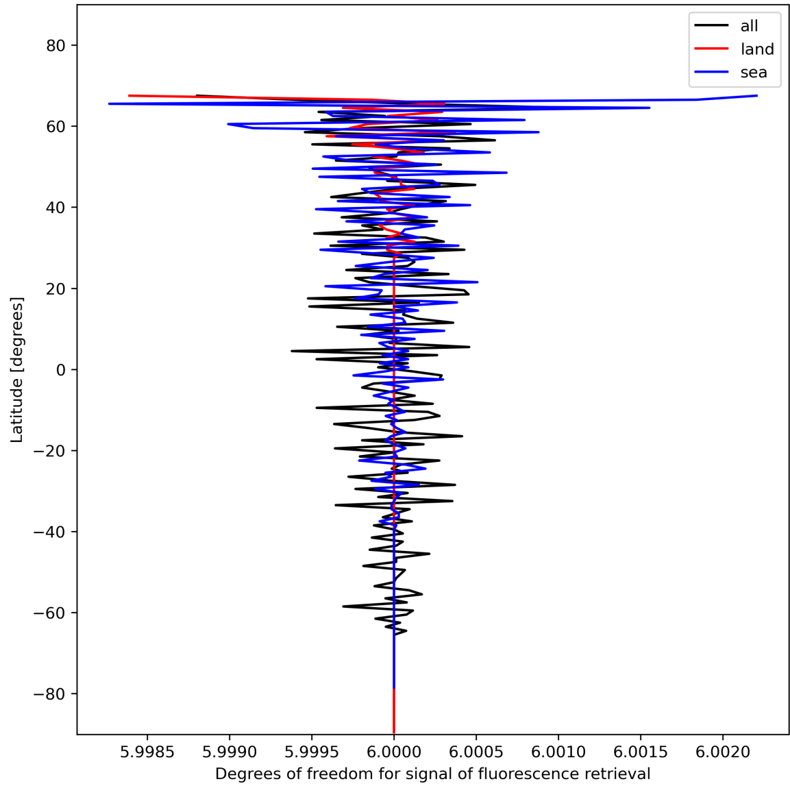
Figure 26: Zonal average of “Degrees of freedom for signal of fluorescence retrieval” for 2024-01-16 to 2024-01-18.
