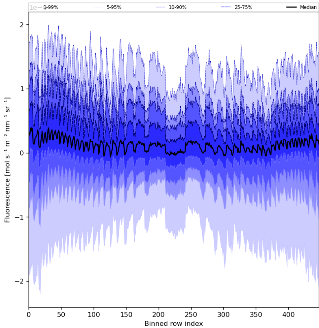
Figure 57: Along track statistics of “Fluorescence” for 2024-01-16 to 2024-01-18
