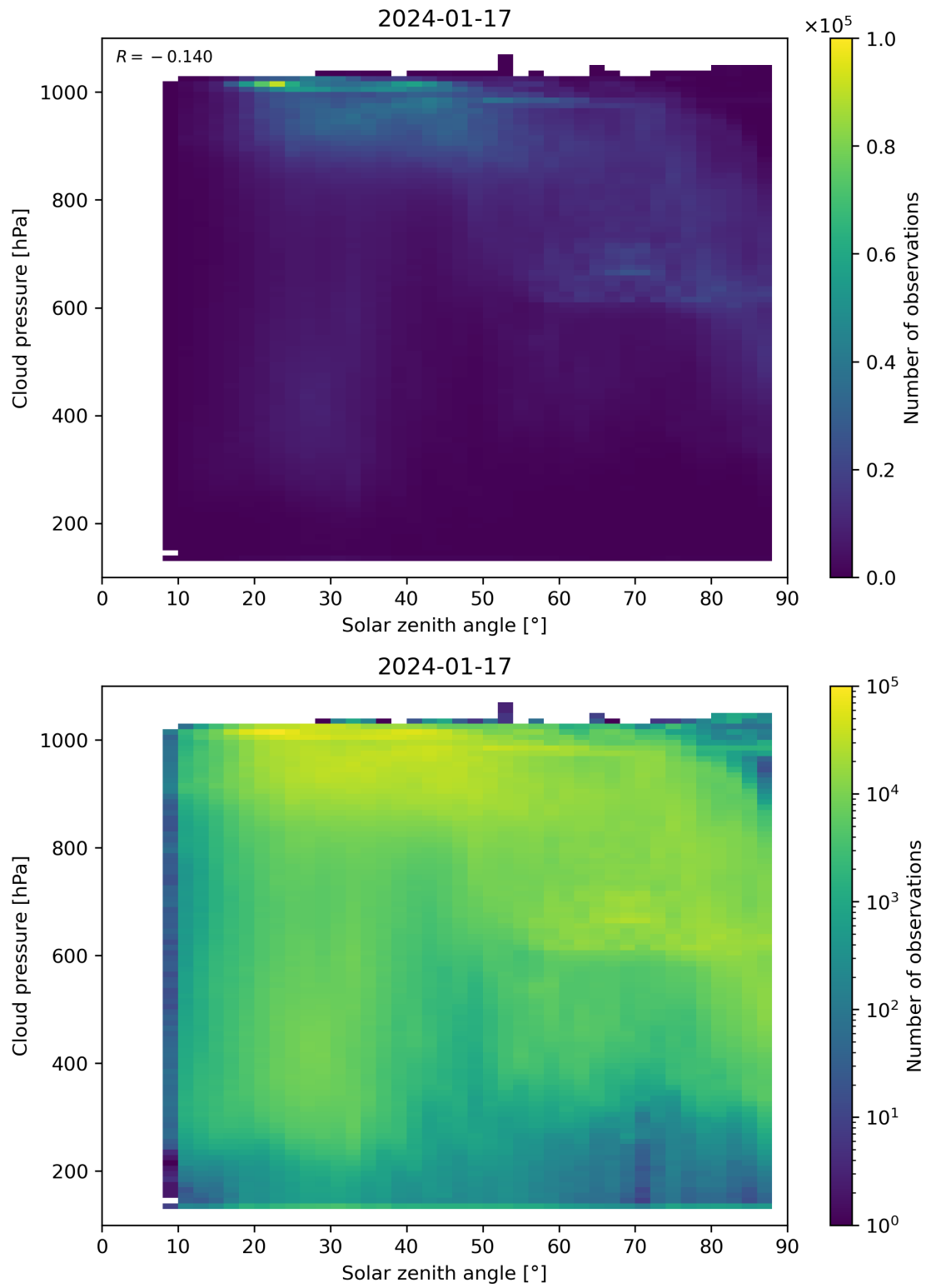
Figure 111: Scatter density plot of “Solar zenith angle” against “Cloud pressure” for 2024-01-16 to 2024-01-18.
