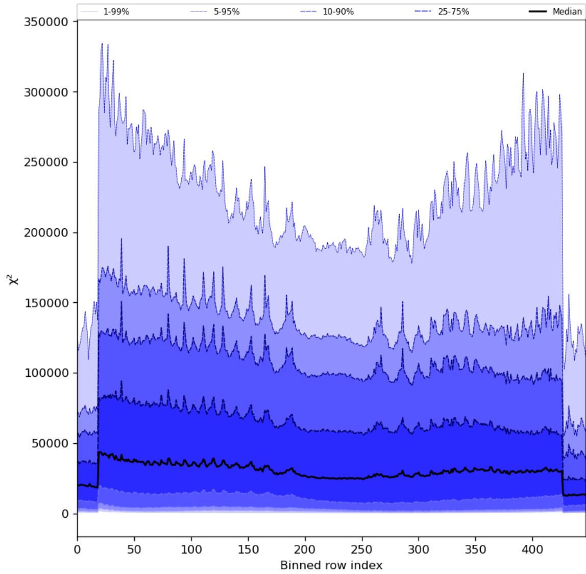
Figure 55: Along track statistics of “ \chi^2 ” for 2024-01-16 to 2024-01-18
