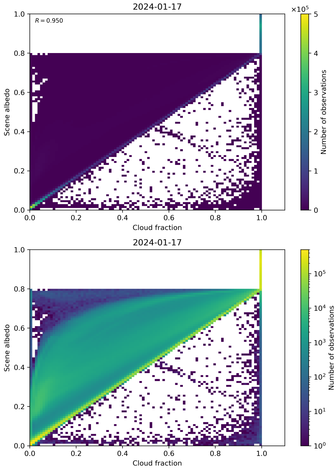
Figure 75: Scatter density plot of “Cloud fraction” against “Scene albedo” for 2024-01-16 to 2024-01-18.
