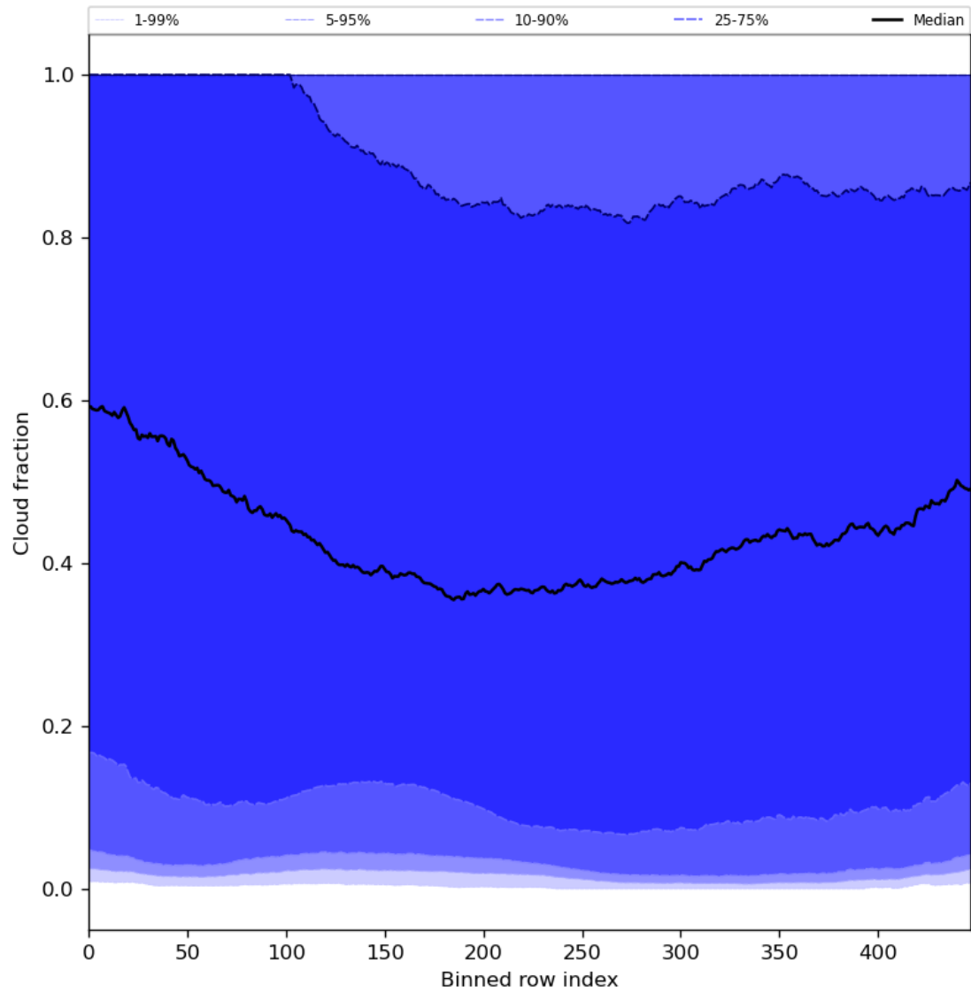
Figure 49: Along track statistics of “Cloud fraction” for 2024-01-16 to 2024-01-18
