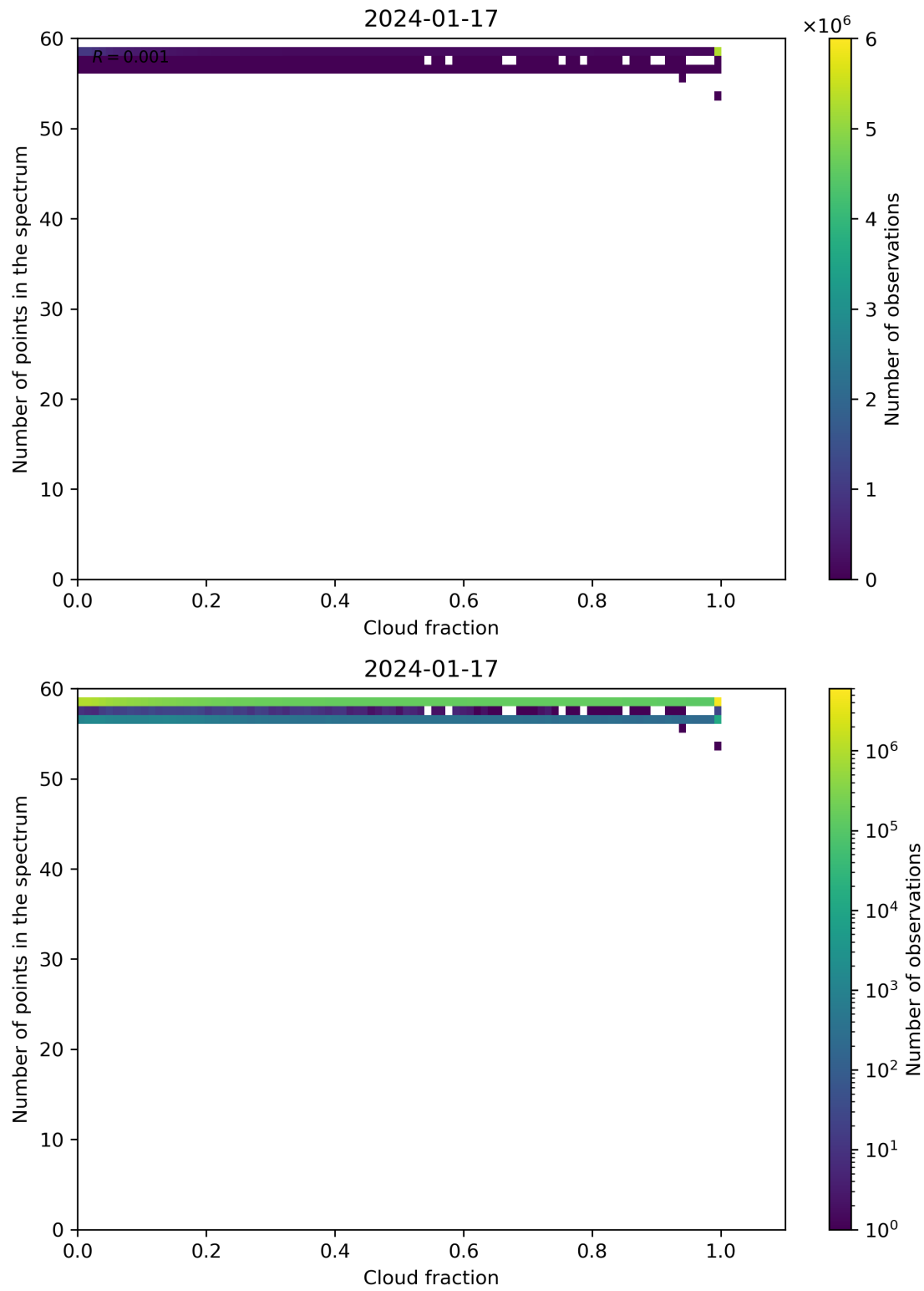
Figure 74: Scatter density plot of “Cloud fraction” against “Number of points in the spectrum” for 2024-01-16 to 2024-01-18.
