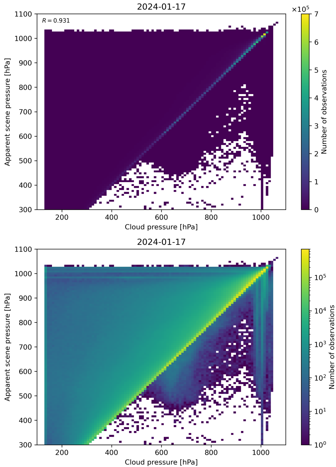
Figure 77: Scatter density plot of “Cloud pressure” against “Apparent scene pressure” for 2024-01-16 to 2024-01-18.
