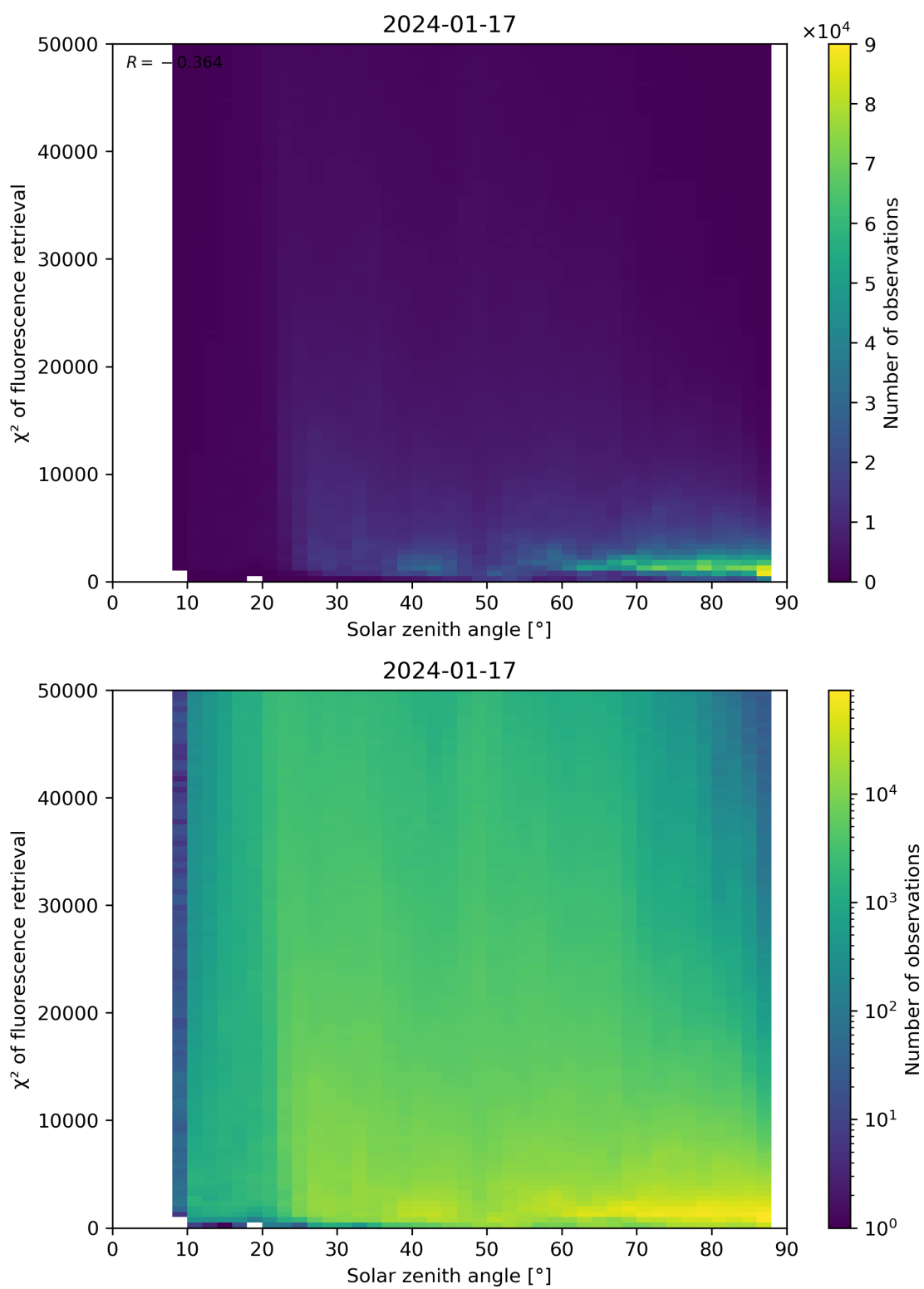
Figure 109: Scatter density plot of “Solar zenith angle” against “ \chi^2 of fluorescence retrieval” for 2024-01-16 to 2024-01-18.
