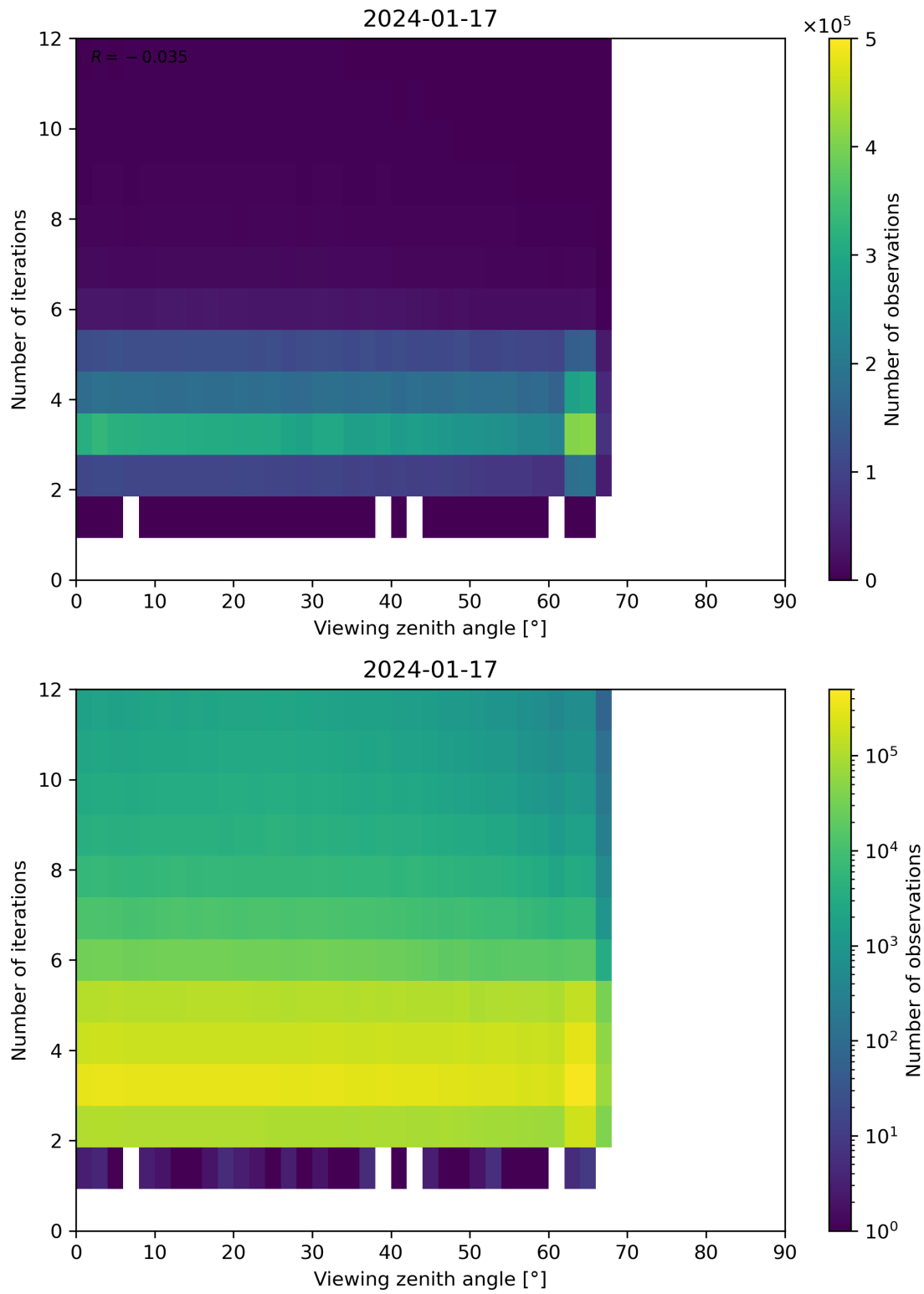
Figure 124: Scatter density plot of “Viewing zenith angle” against “Number of iterations” for 2024-01-16 to 2024-01-18.
