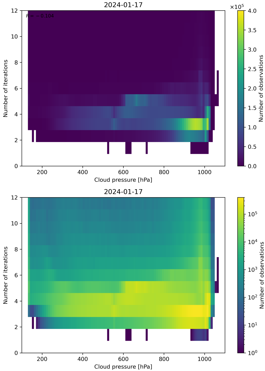
Figure 81: Scatter density plot of “Cloud pressure” against “Number of iterations” for 2024-01-16 to 2024-01-18.
