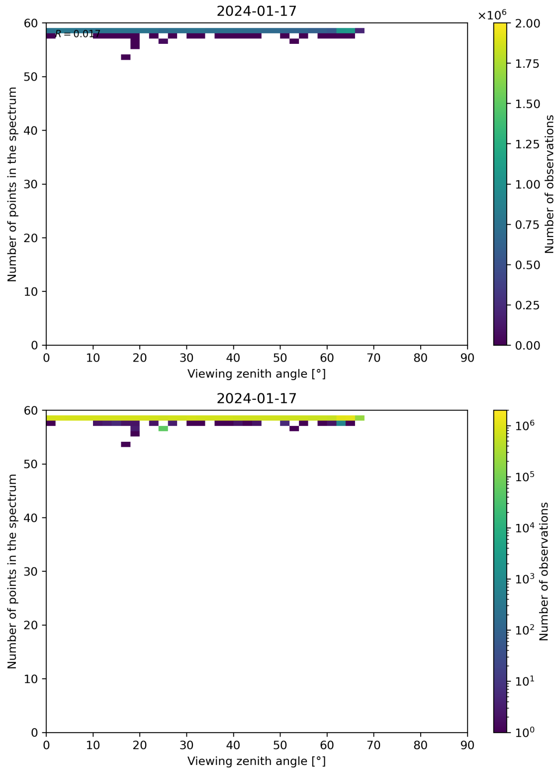
Figure 125: Scatter density plot of “Viewing zenith angle” against “Number of points in the spectrum” for 2024-01-16 to 2024-01-18.
