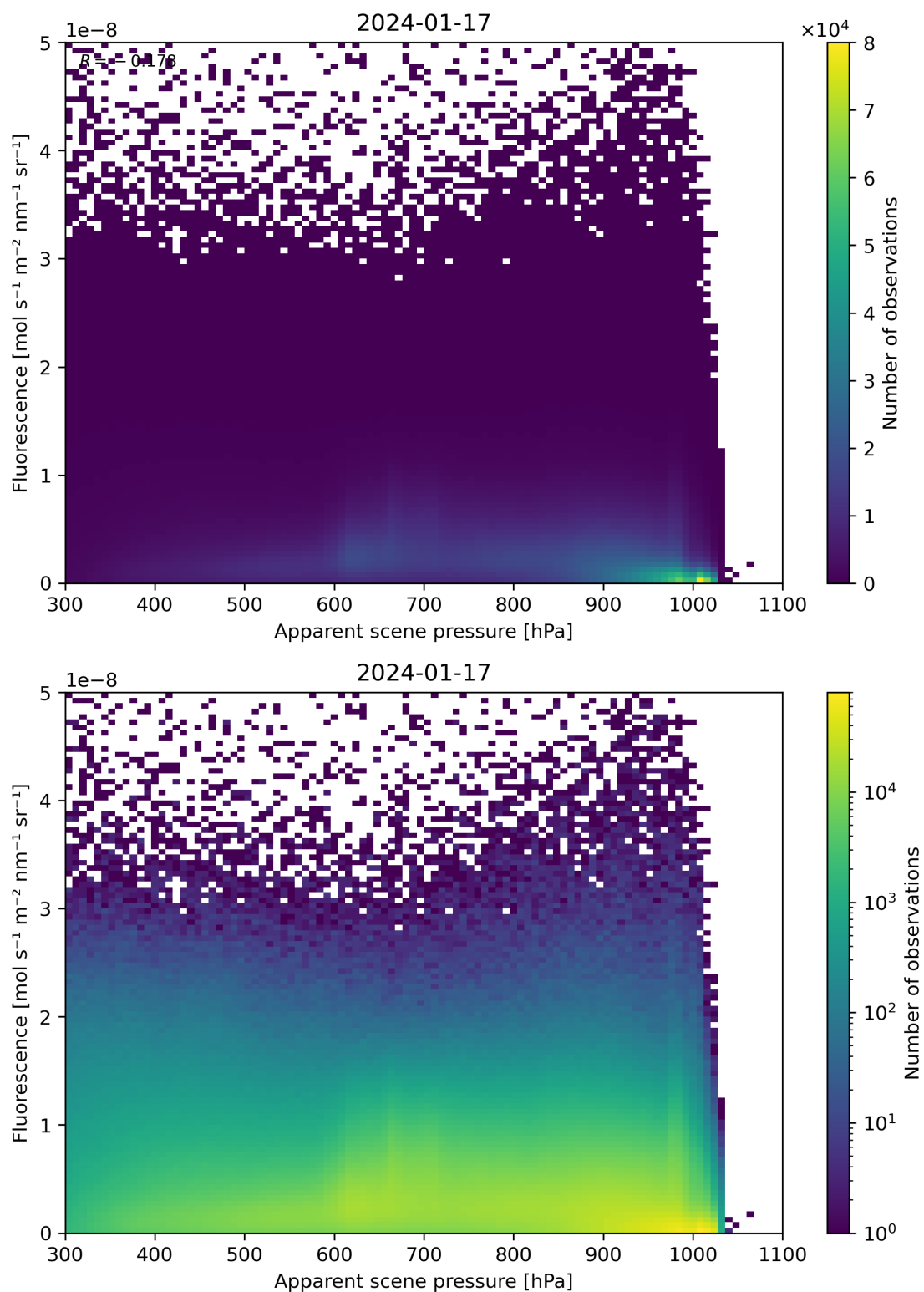
Figure 64: Scatter density plot of “Apparent scene pressure” against “Fluorescence” for 2024-01-16 to 2024-01-18.
