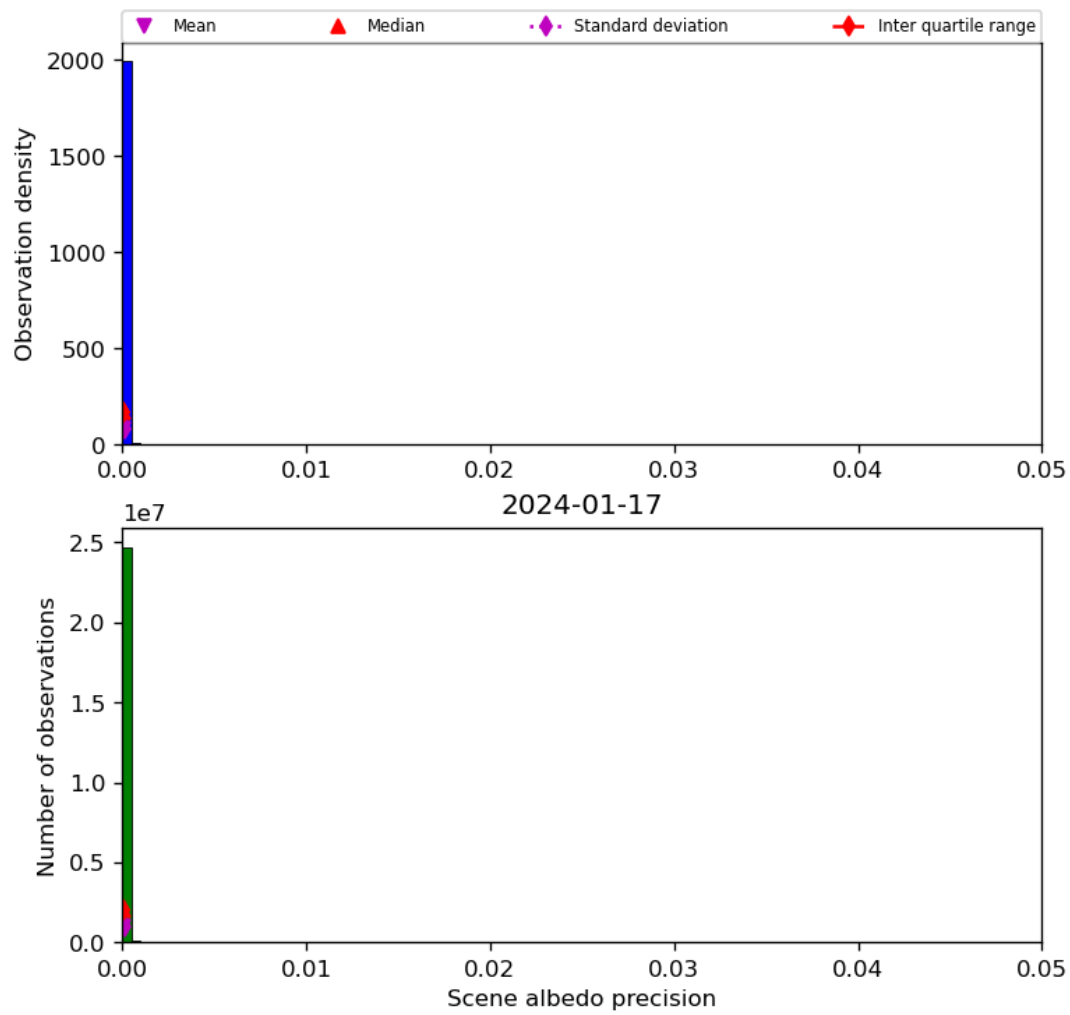
Figure 35: Histogram of “Scene albedo precision” for 2024-01-16 to 2024-01-18
