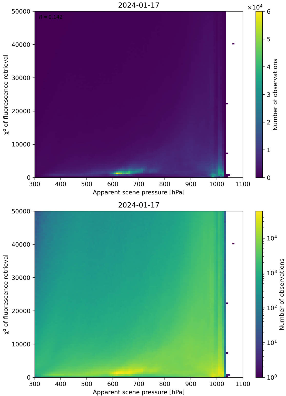
Figure 63: Scatter density plot of “Apparent scene pressure” against “ \chi^2 of fluorescence retrieval” for 2024-01-16 to 2024-01-18.
