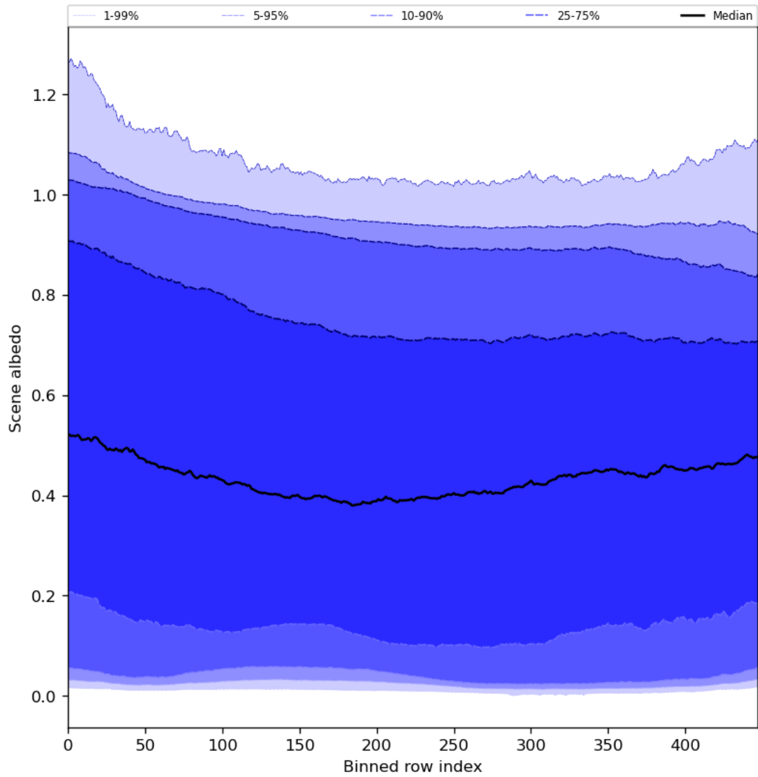
Figure 51: Along track statistics of “Scene albedo” for 2024-01-16 to 2024-01-18
