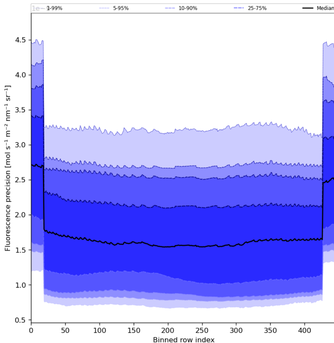
Figure 58: Along track statistics of “Fluorescence precision” for 2024-01-16 to 2024-01-18
