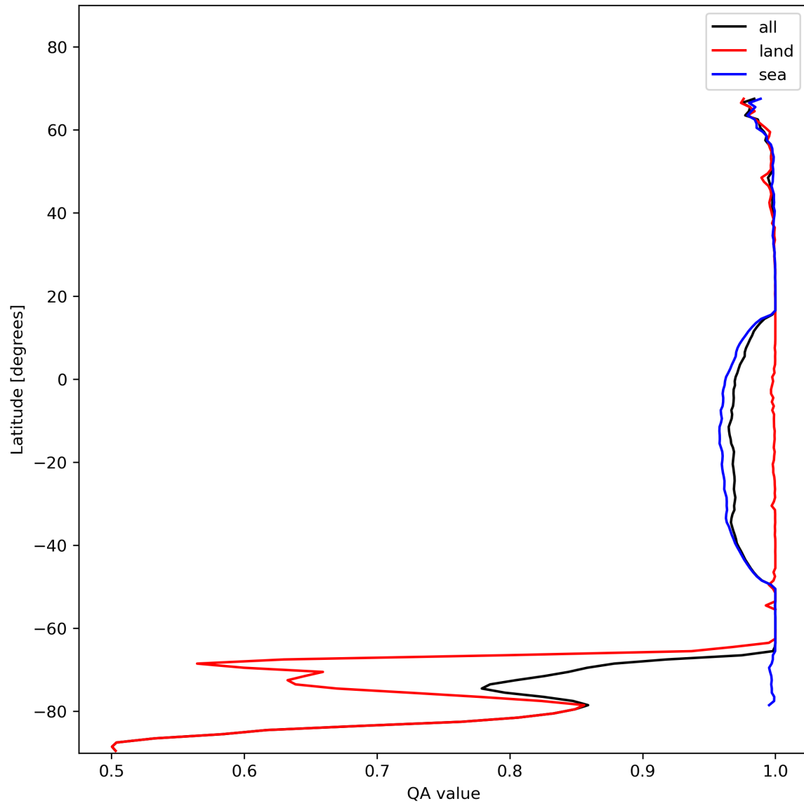
Figure 12: Zonal average of “QA value” for 2024-01-16 to 2024-01-18.
