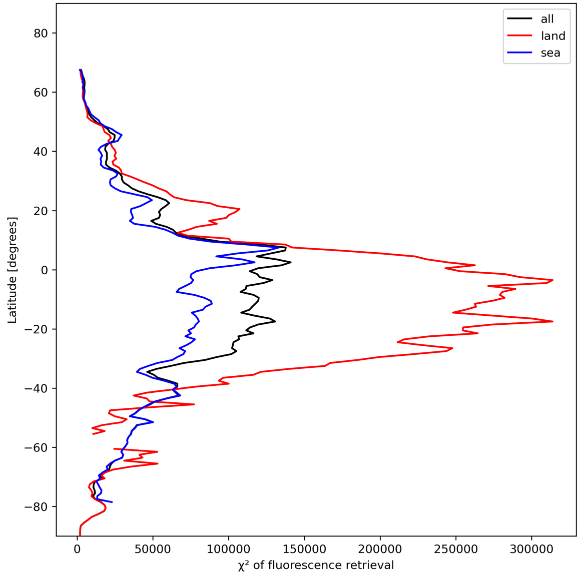
Figure 25: Zonal average of “ \chi^2 of fluorescence retrieval” for 2024-01-16 to 2024-01-18.
