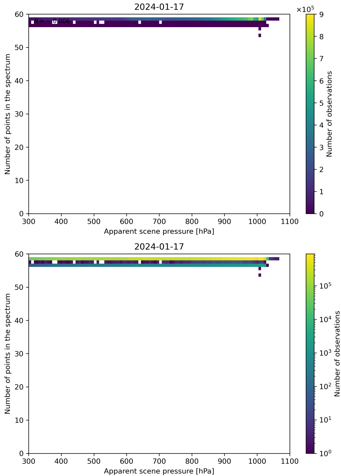
Figure 66: Scatter density plot of “Apparent scene pressure” against “Number of points in the spectrum” for 2024-01-16 to 2024-01-18.
