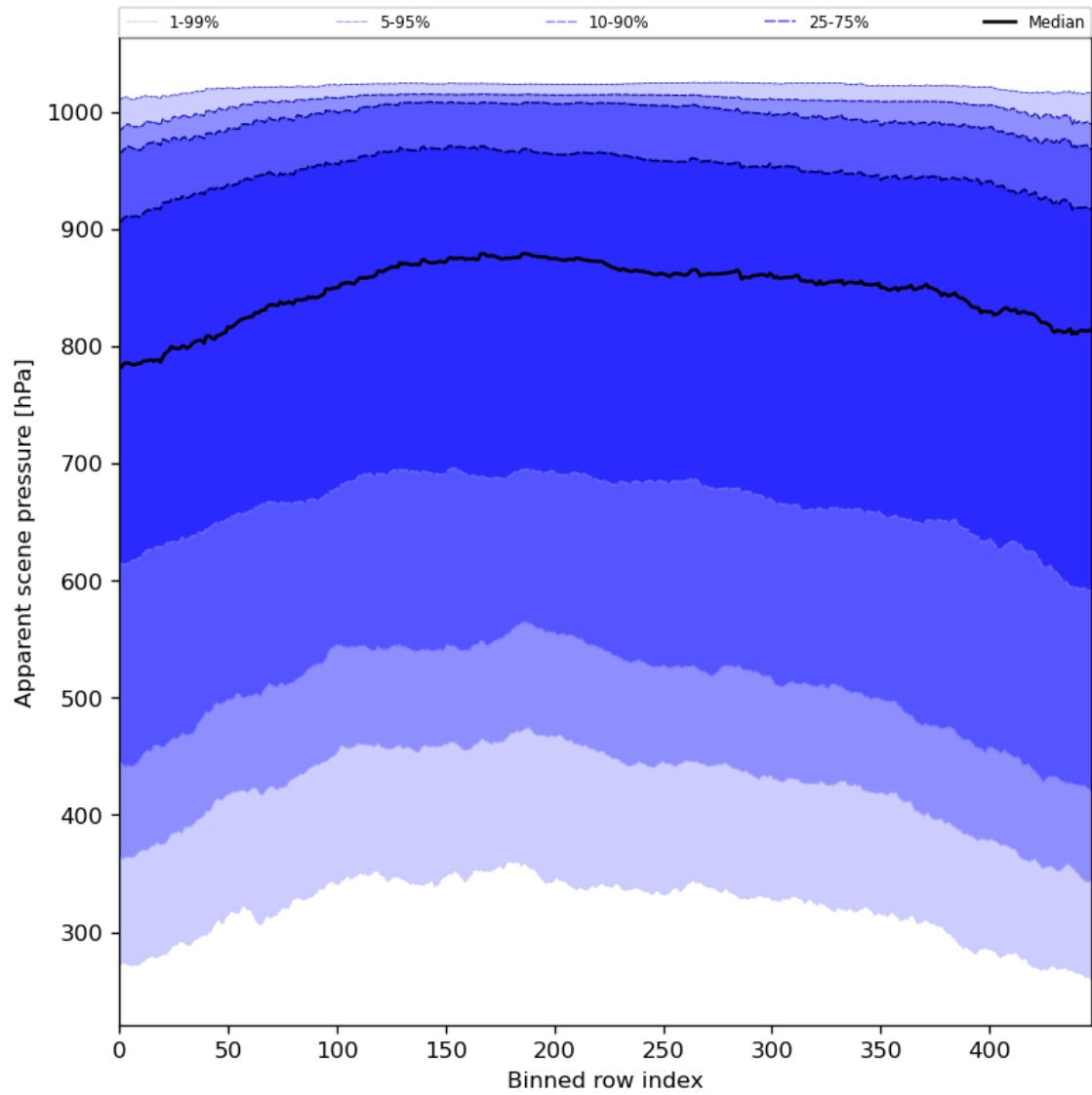
Figure 53: Along track statistics of “Apparent scene pressure” for 2024-01-16 to 2024-01-18
