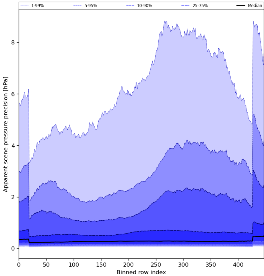
Figure 54: Along track statistics of “Apparent scene pressure precision” for 2024-01-16 to 2024-01-18
