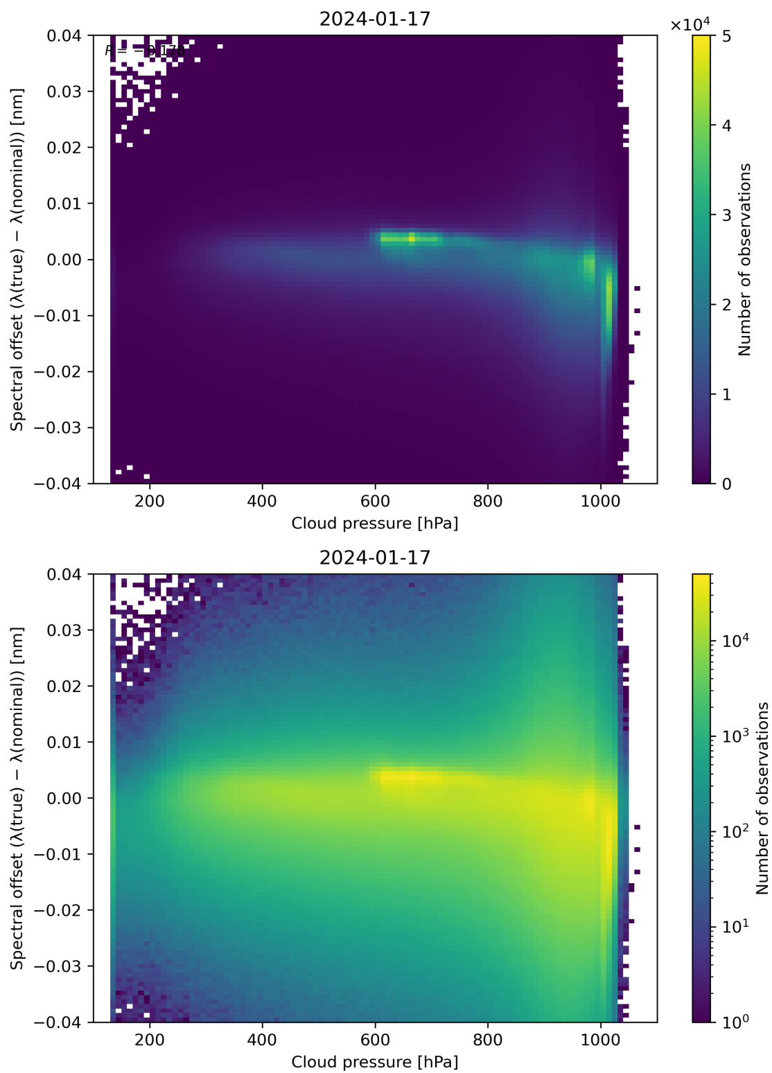
Figure 84: Scatter density plot of “Cloud pressure” against “Spectral offset ( \lambda(\text{true}) - \lambda(\text{nominal}) )” for 2024-01-16 to 2024-01-18.
