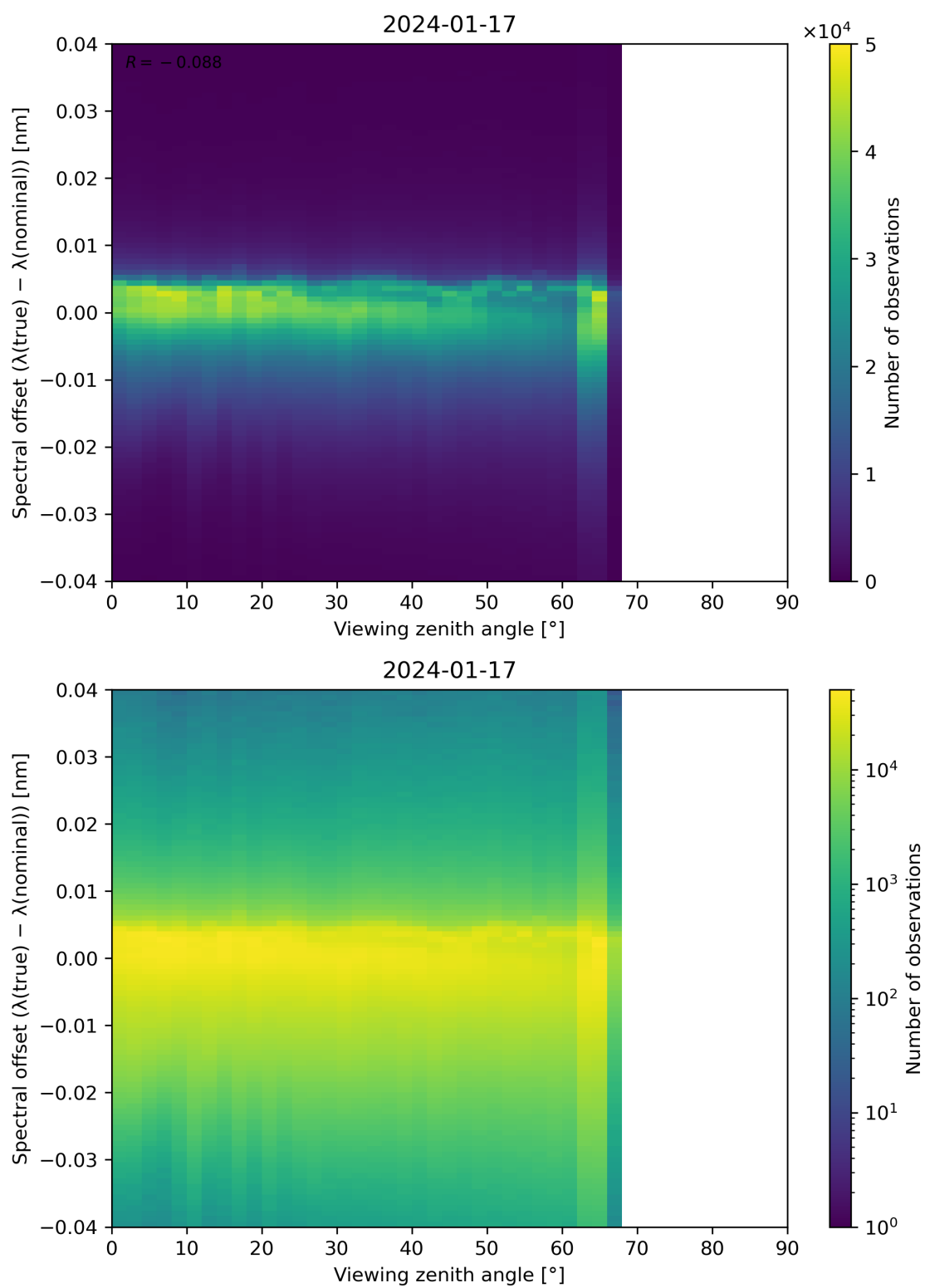
Figure 128: Scatter density plot of “Viewing zenith angle” against “Spectral offset ( \lambda(\text{true}) - \lambda(\text{nominal}) )” for 2024-01-16 to 2024-01-18.
