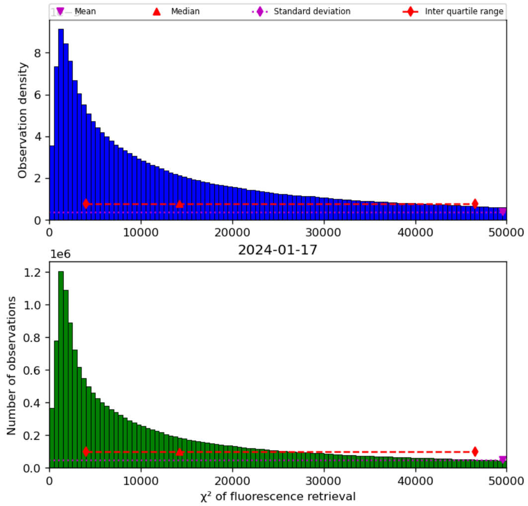
Figure 42: Histogram of “ \chi^2 of fluorescence retrieval” for 2024-01-16 to 2024-01-18
