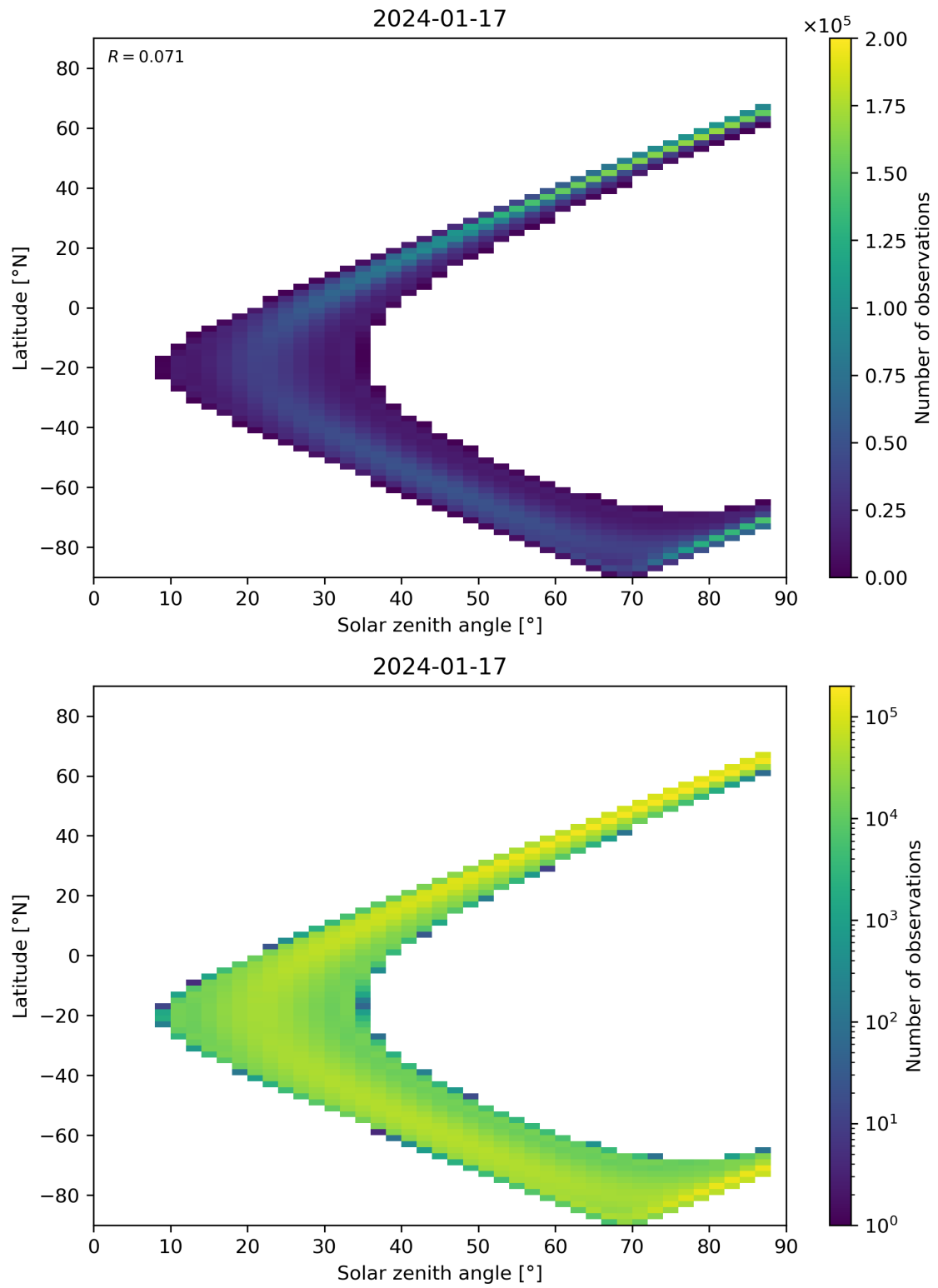
Figure 113: Scatter density plot of “Solar zenith angle” against “Latitude” for 2024-01-16 to 2024-01-18.
