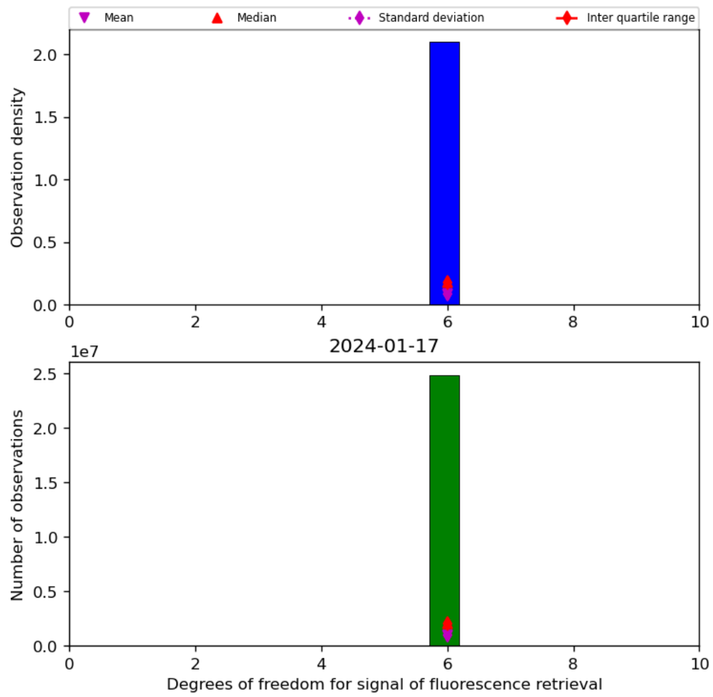
Figure 43: Histogram of “Degrees of freedom for signal of fluorescence retrieval” for 2024-01-16 to 2024-01-18
