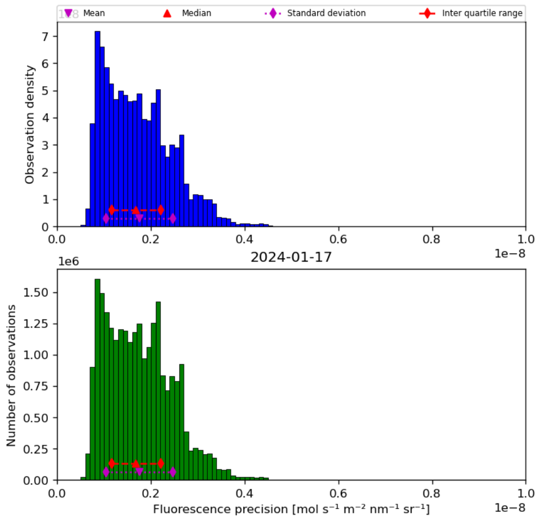
Figure 41: Histogram of “Fluorescence precision” for 2024-01-16 to 2024-01-18
