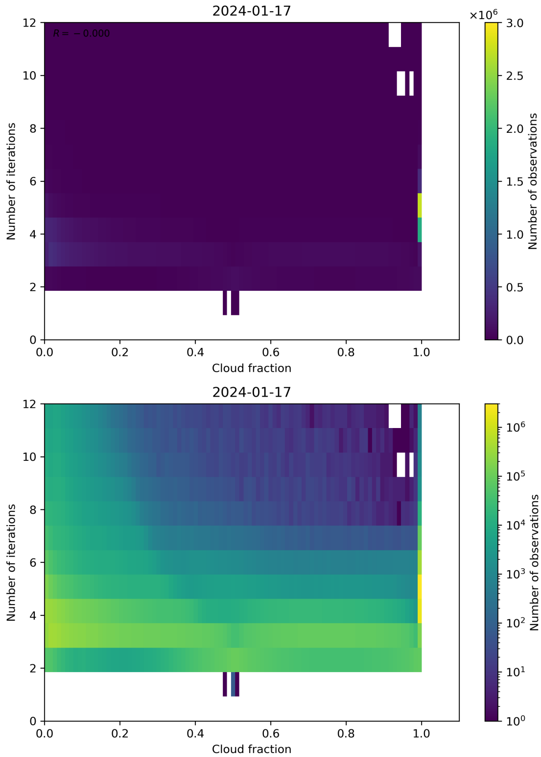
Figure 73: Scatter density plot of “Cloud fraction” against “Number of iterations” for 2024-01-16 to 2024-01-18.
