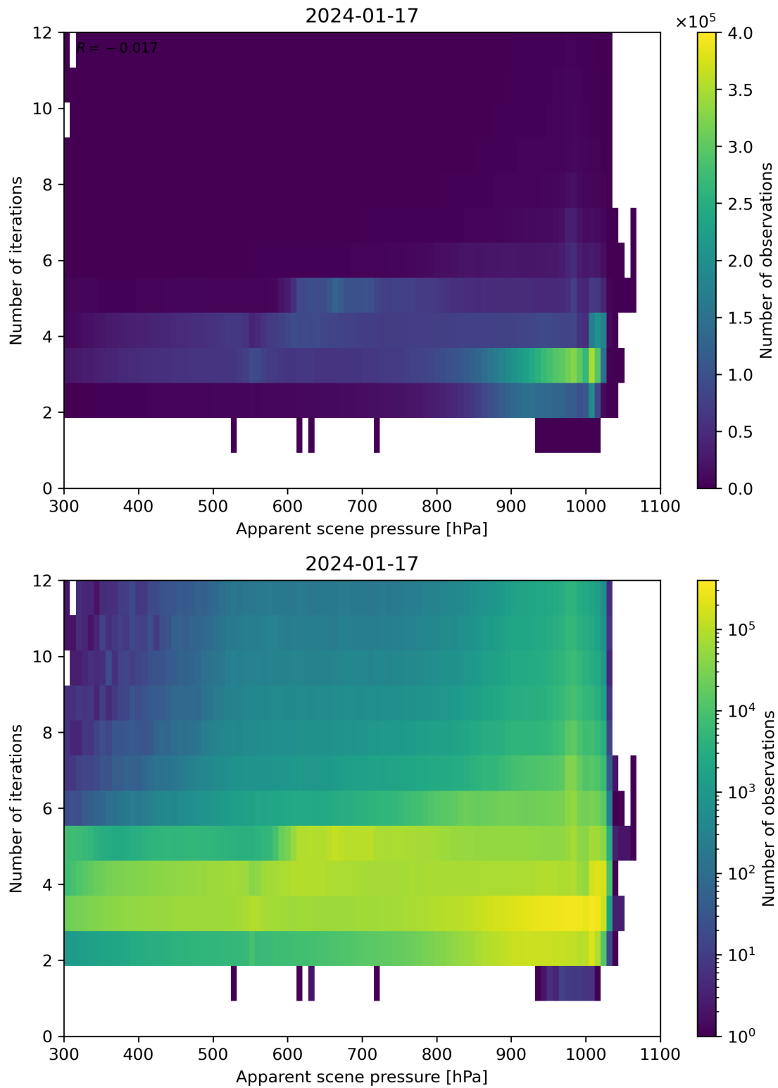
Figure 65: Scatter density plot of “Apparent scene pressure” against “Number of iterations” for 2024-01-16 to 2024-01-18.
