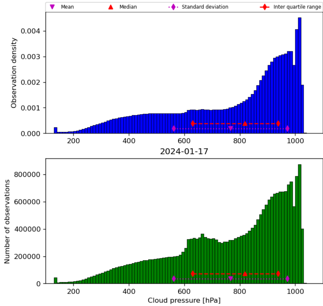
Figure 30: Histogram of “Cloud pressure” for 2024-01-16 to 2024-01-18
