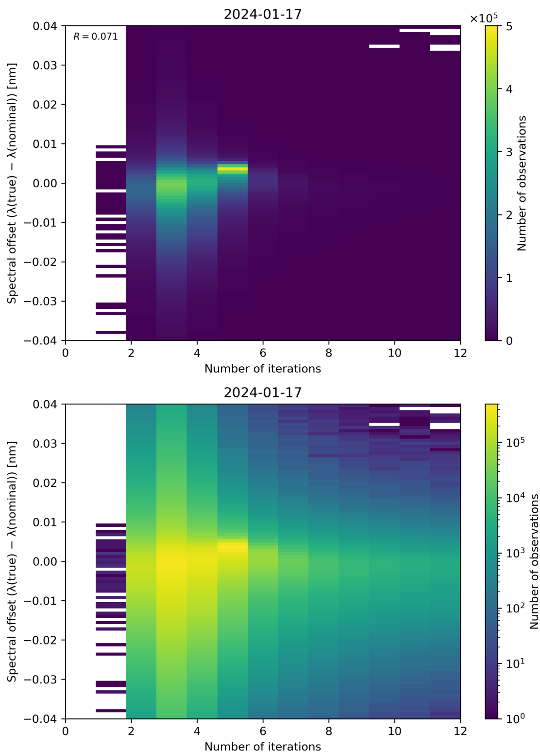
Figure 100: Scatter density plot of “Number of iterations” against “Spectral offset ( \lambda(\text{true}) - \lambda(\text{nominal}) )” for 2024-01-16 to 2024-01-18.
