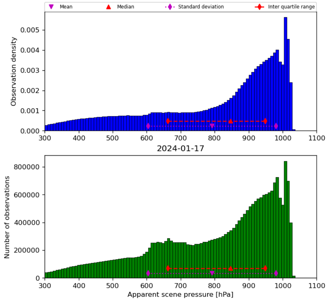
Figure 36: Histogram of “Apparent scene pressure” for 2024-01-16 to 2024-01-18
