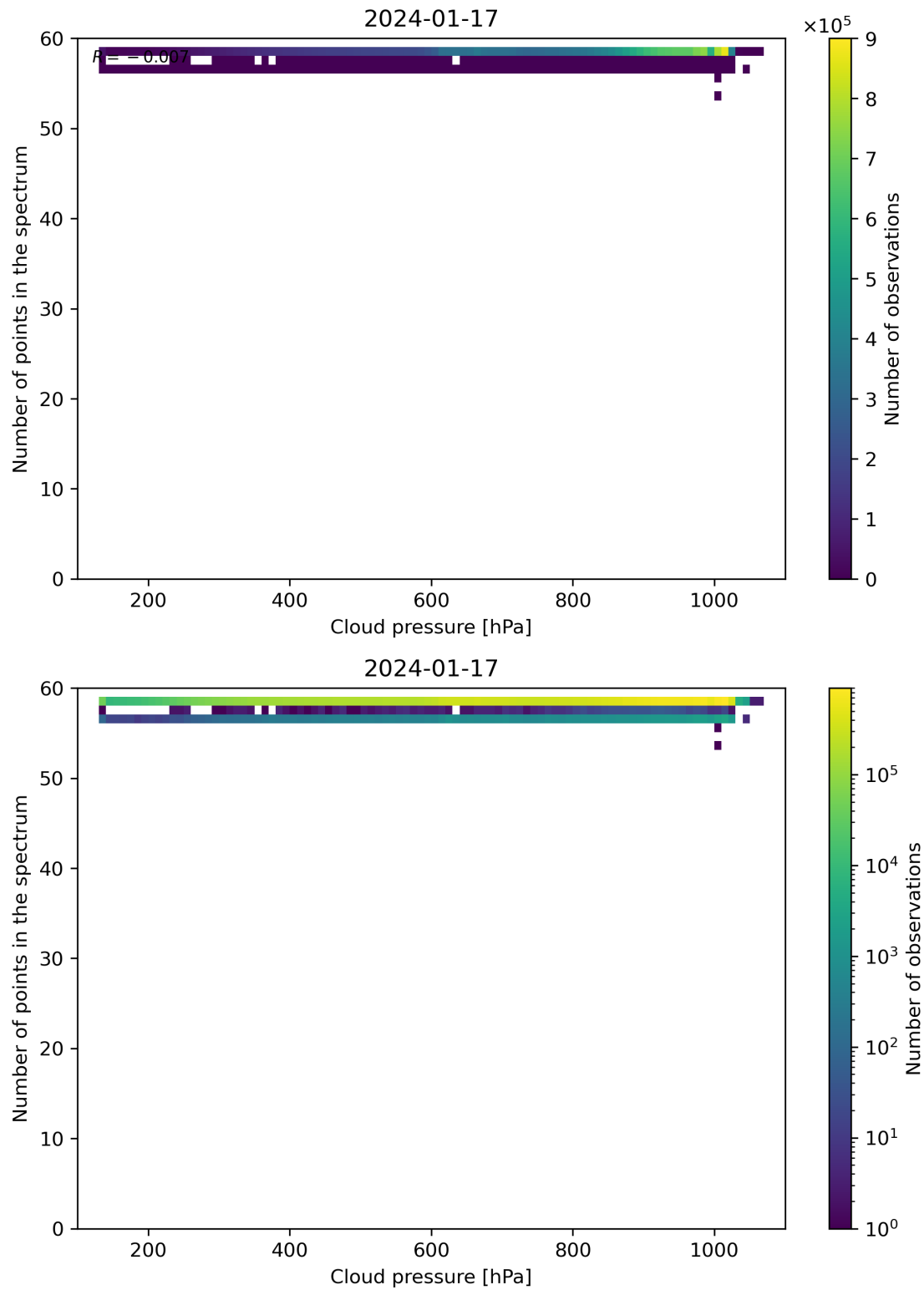
Figure 82: Scatter density plot of “Cloud pressure” against “Number of points in the spectrum” for 2024-01-16 to 2024-01-18.
