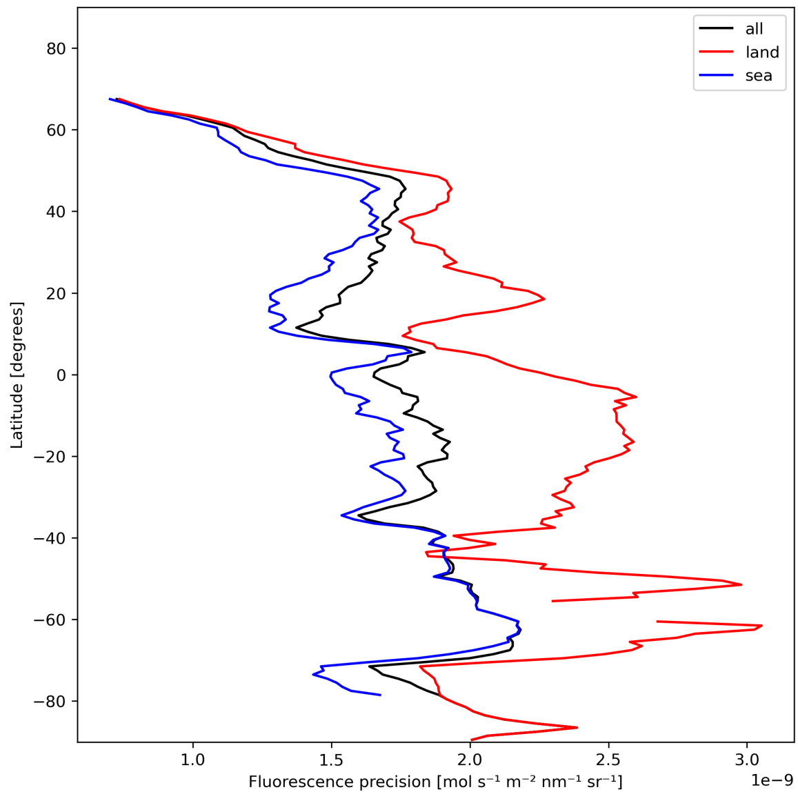
Figure 24: Zonal average of “Fluorescence precision” for 2024-01-16 to 2024-01-18.
