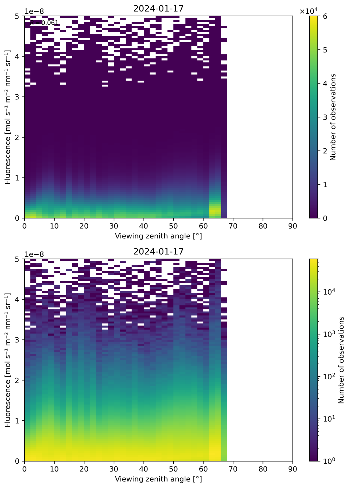
Figure 122: Scatter density plot of “Viewing zenith angle” against “Fluorescence” for 2024-01-16 to 2024-01-18.
