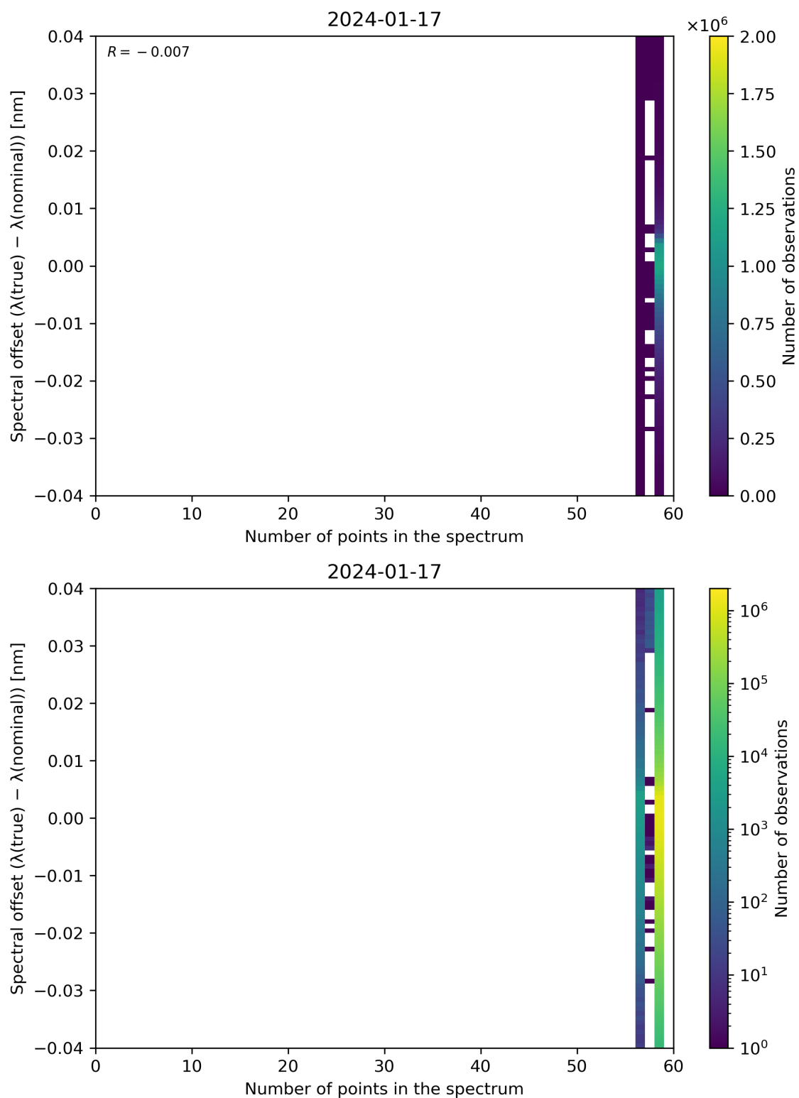
Figure 101: Scatter density plot of “Number of points in the spectrum” against “Spectral offset ( \lambda(\text{true}) - \lambda(\text{nominal}) )” for 2024-01-16 to 2024-01-18.
