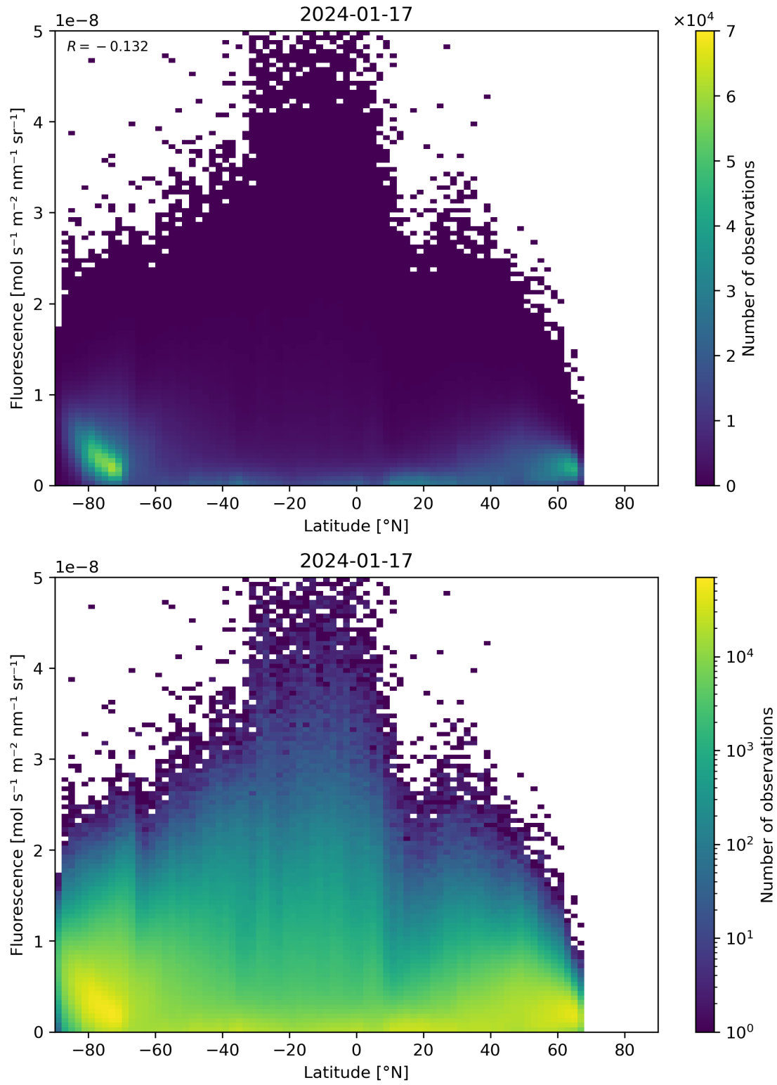
Figure 92: Scatter density plot of “Latitude” against “Fluorescence” for 2024-01-16 to 2024-01-18.
