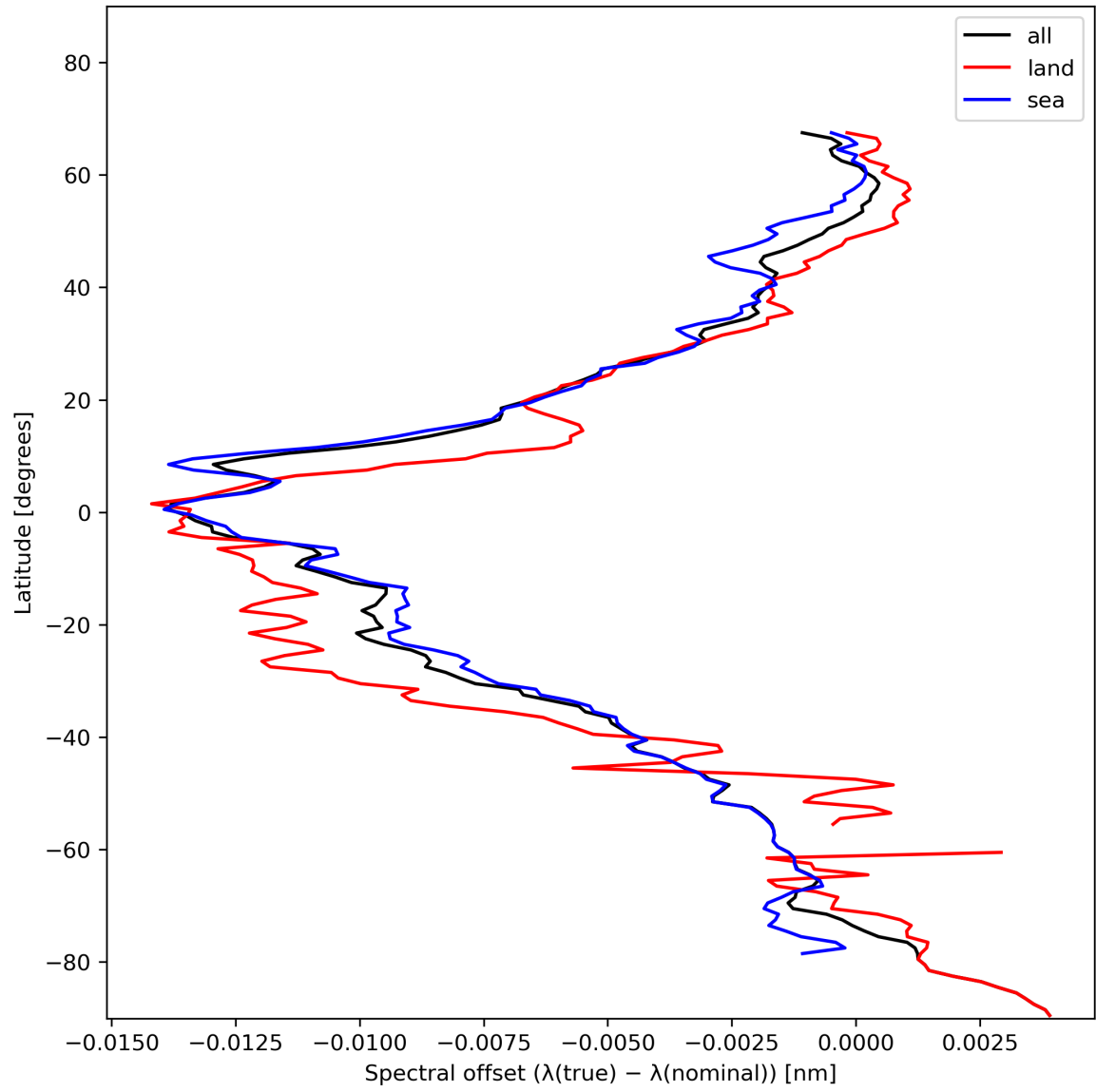
Figure 28: Zonal average of “Spectral offset ( \lambda(\text{true}) - \lambda(\text{nominal}) )” for 2024-01-16 to 2024-01-18.
