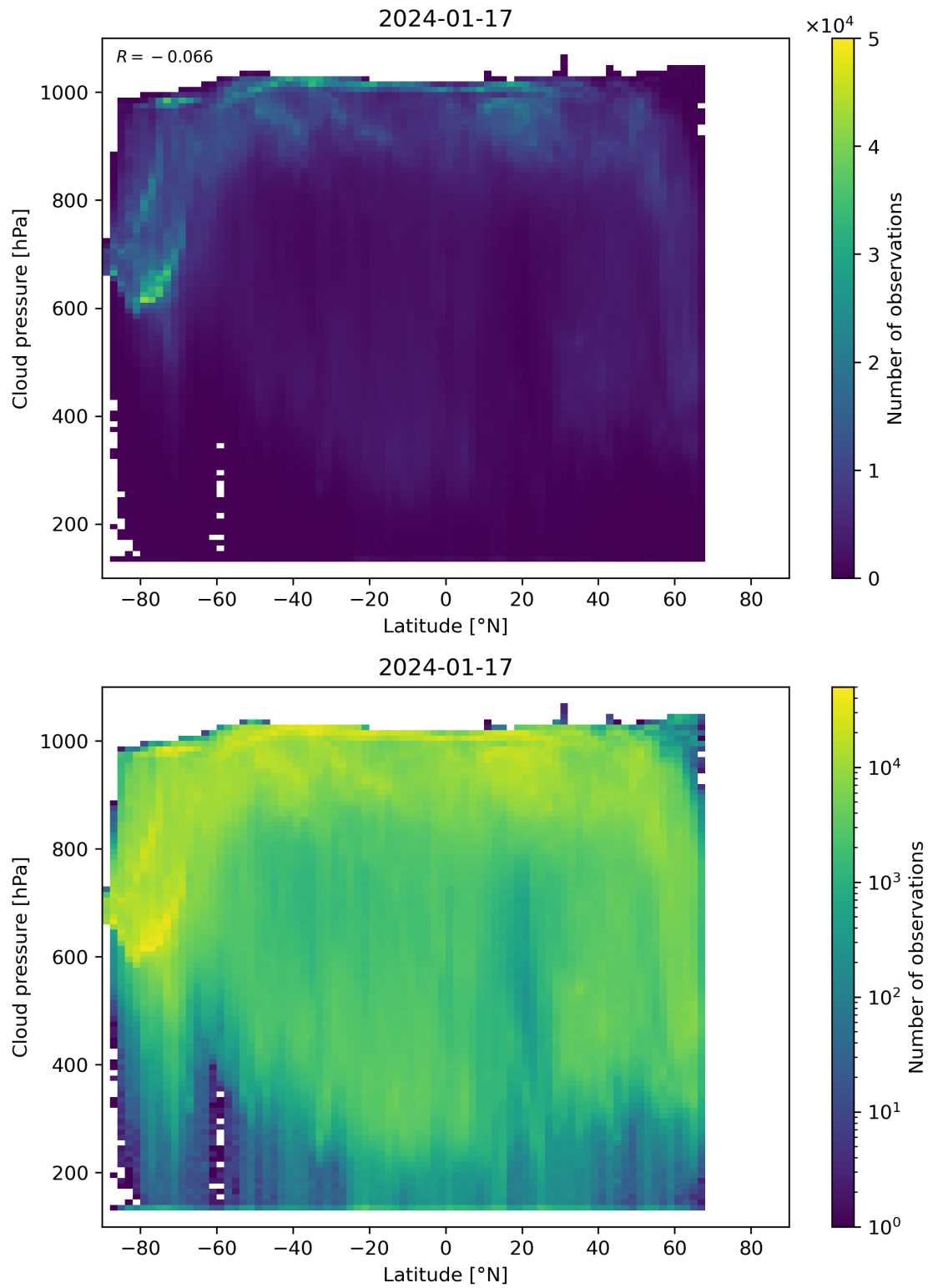
Figure 91: Scatter density plot of “Latitude” against “Cloud pressure” for 2024-01-16 to 2024-01-18.
