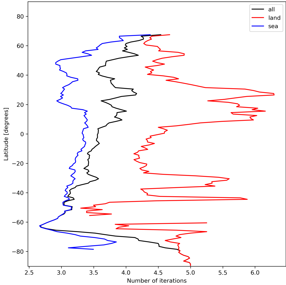
Figure 22: Zonal average of “Number of iterations” for 2024-01-16 to 2024-01-18.
