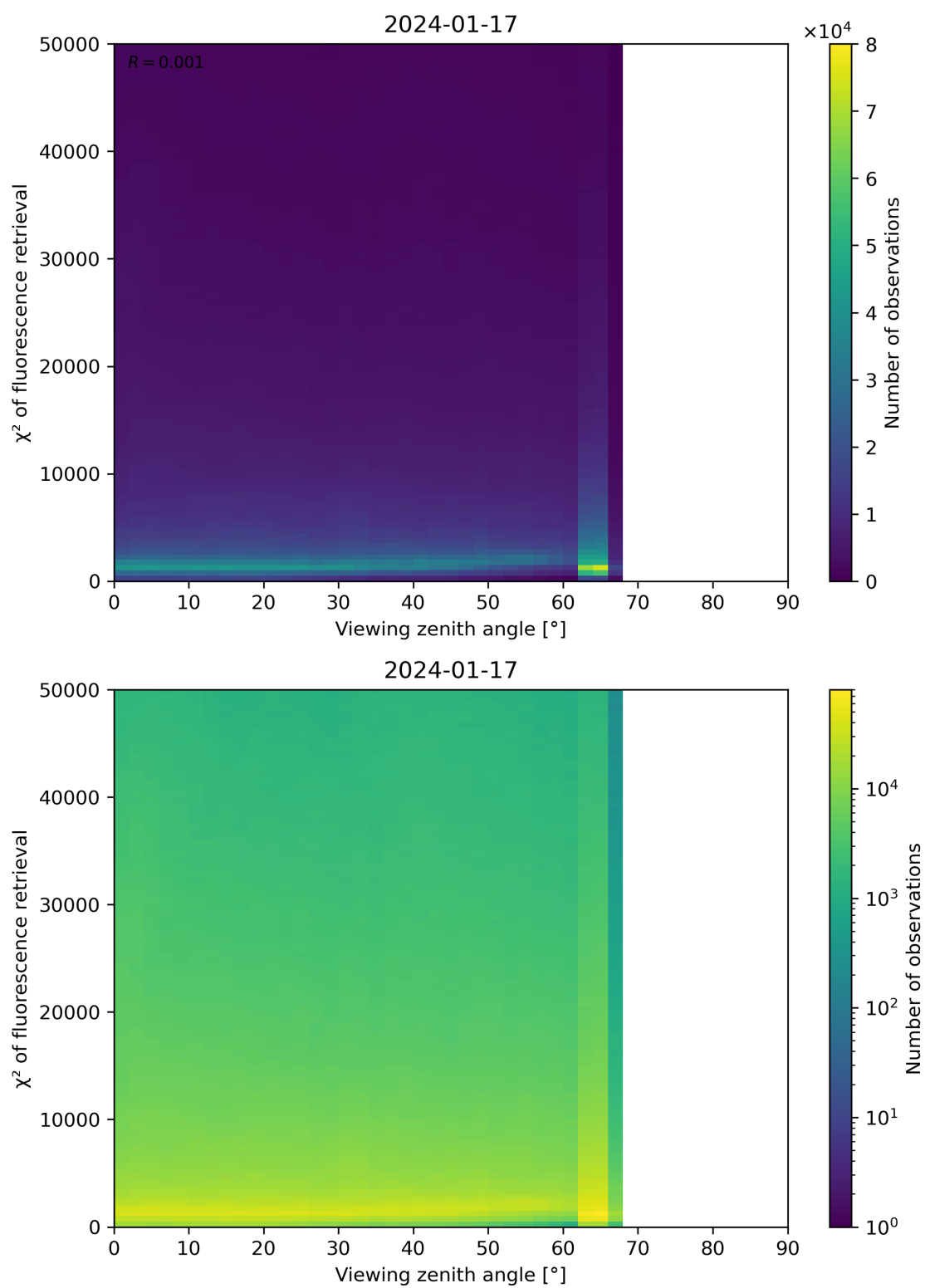
Figure 119: Scatter density plot of “Viewing zenith angle” against “ \chi^2 of fluorescence retrieval” for 2024-01-16 to 2024-01-18.
