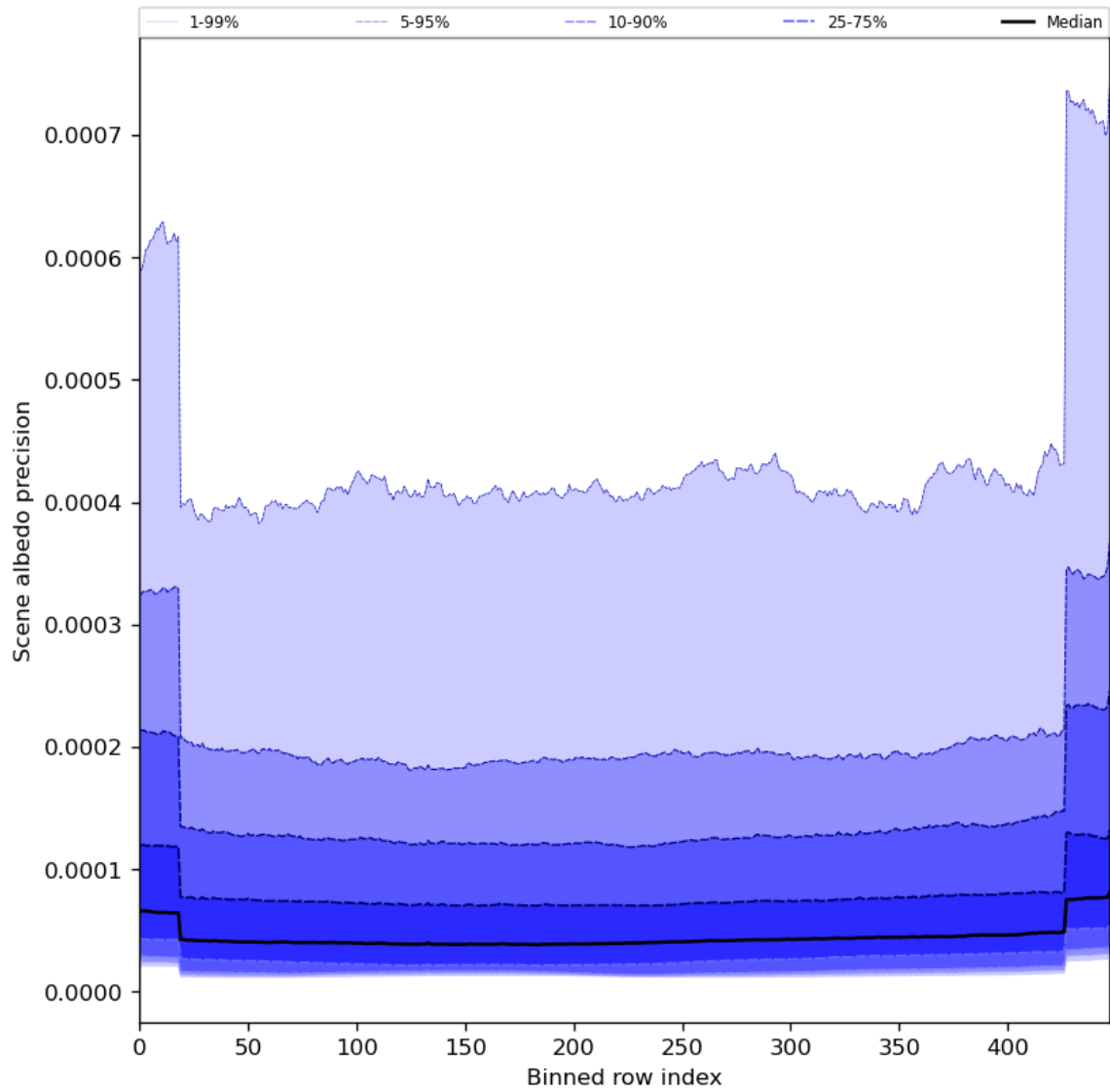
Figure 52: Along track statistics of “Scene albedo precision” for 2024-01-16 to 2024-01-18
