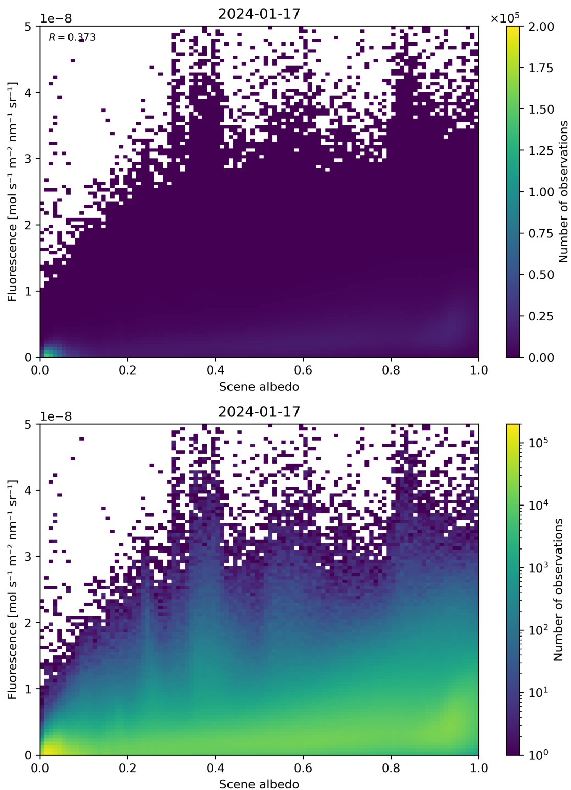
Figure 104: Scatter density plot of “Scene albedo” against “Fluorescence” for 2024-01-16 to 2024-01-18.
