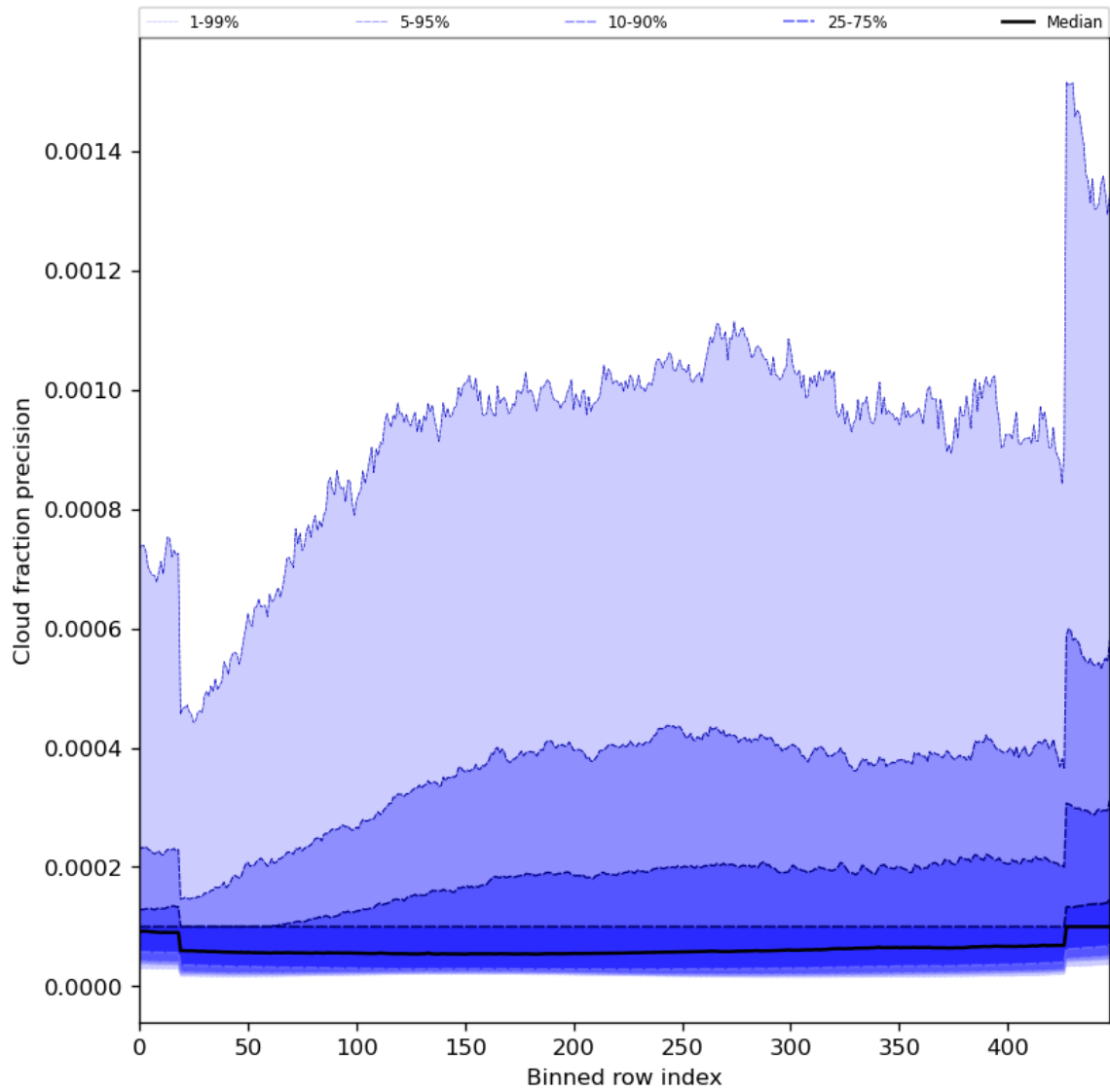
Figure 50: Along track statistics of “Cloud fraction precision” for 2024-01-16 to 2024-01-18
