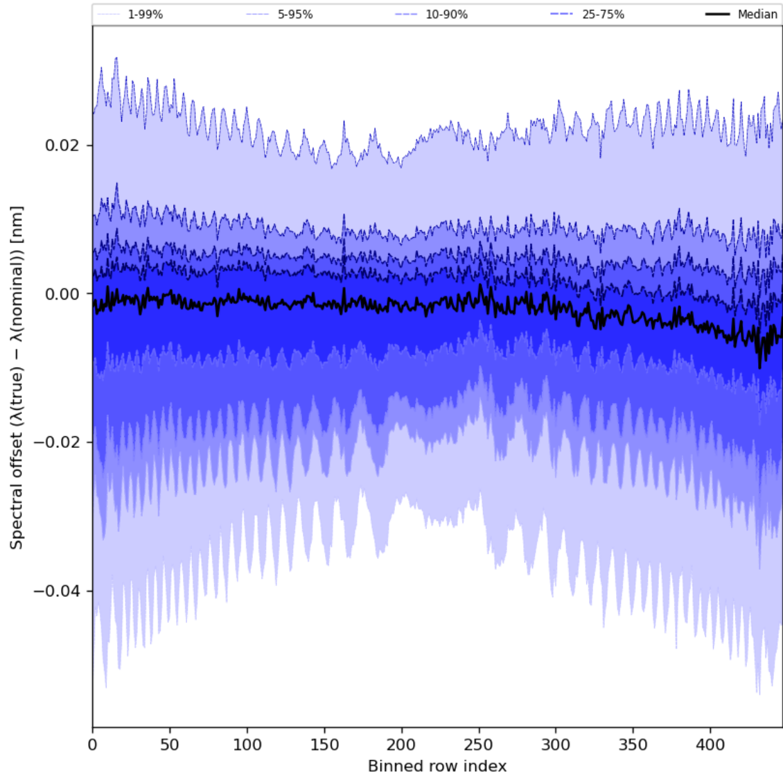
Figure 62: Along track statistics of “Spectral offset ( \lambda(\text{true}) - \lambda(\text{nominal}) )” for 2024-01-16 to 2024-01-18
