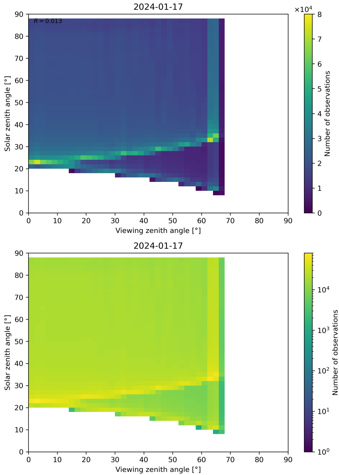
Figure 127: Scatter density plot of “Viewing zenith angle” against “Solar zenith angle” for 2024-01-16 to 2024-01-18.
