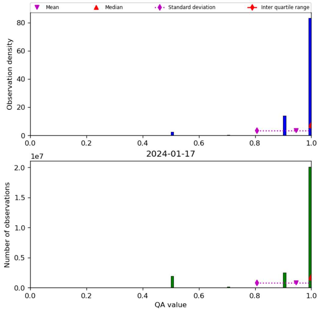
Figure 29: Histogram of “QA value” for 2024-01-16 to 2024-01-18
