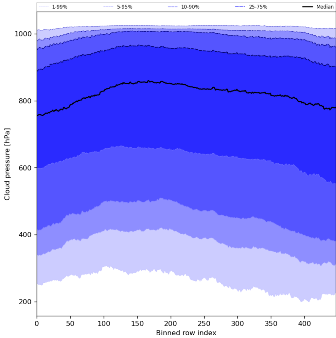
Figure 47: Along track statistics of “Cloud pressure” for 2024-01-16 to 2024-01-18
