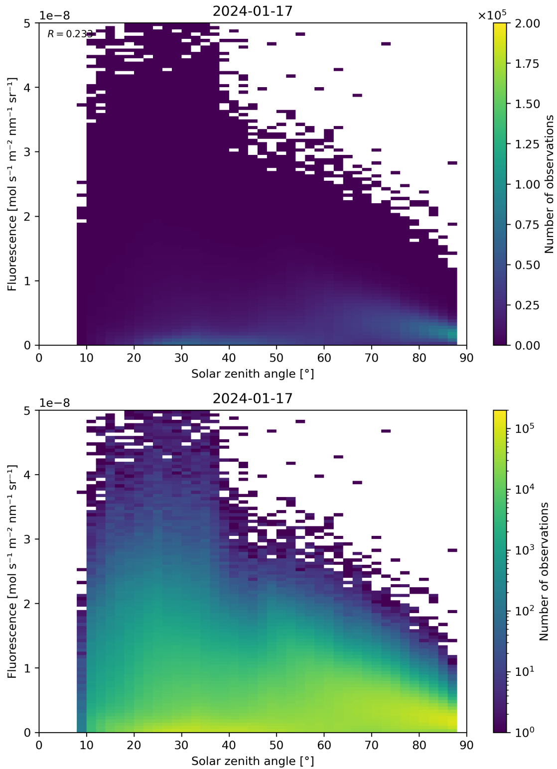
Figure 112: Scatter density plot of “Solar zenith angle” against “Fluorescence” for 2024-01-16 to 2024-01-18.
