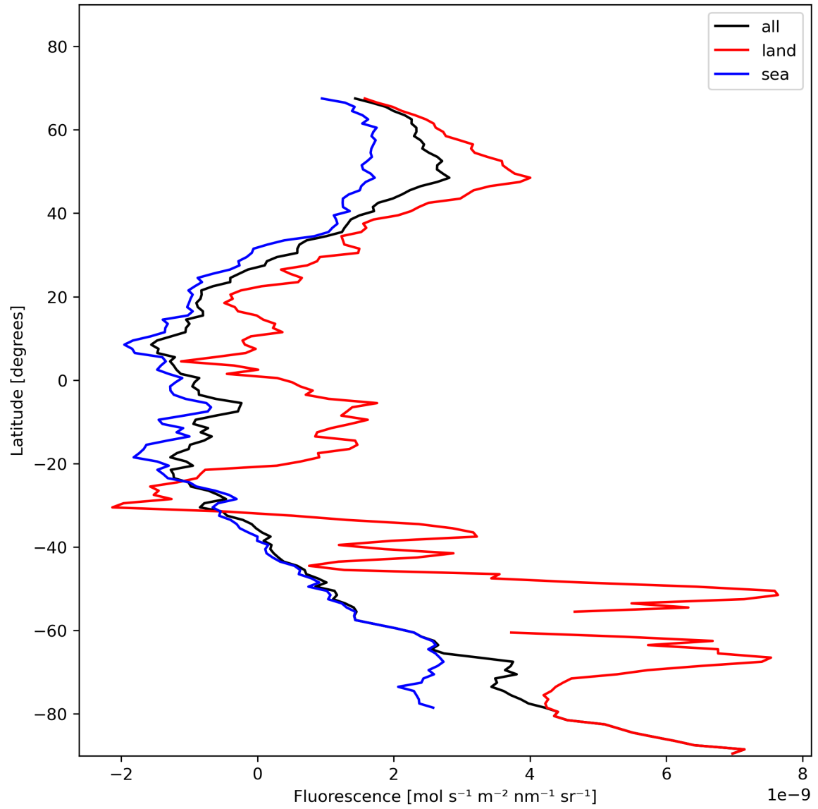
Figure 23: Zonal average of “Fluorescence” for 2024-01-16 to 2024-01-18.
