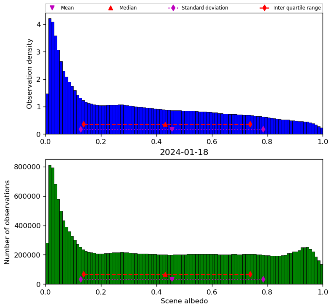
Figure 34: Histogram of “Scene albedo” for 2024-01-17 to 2024-01-19
