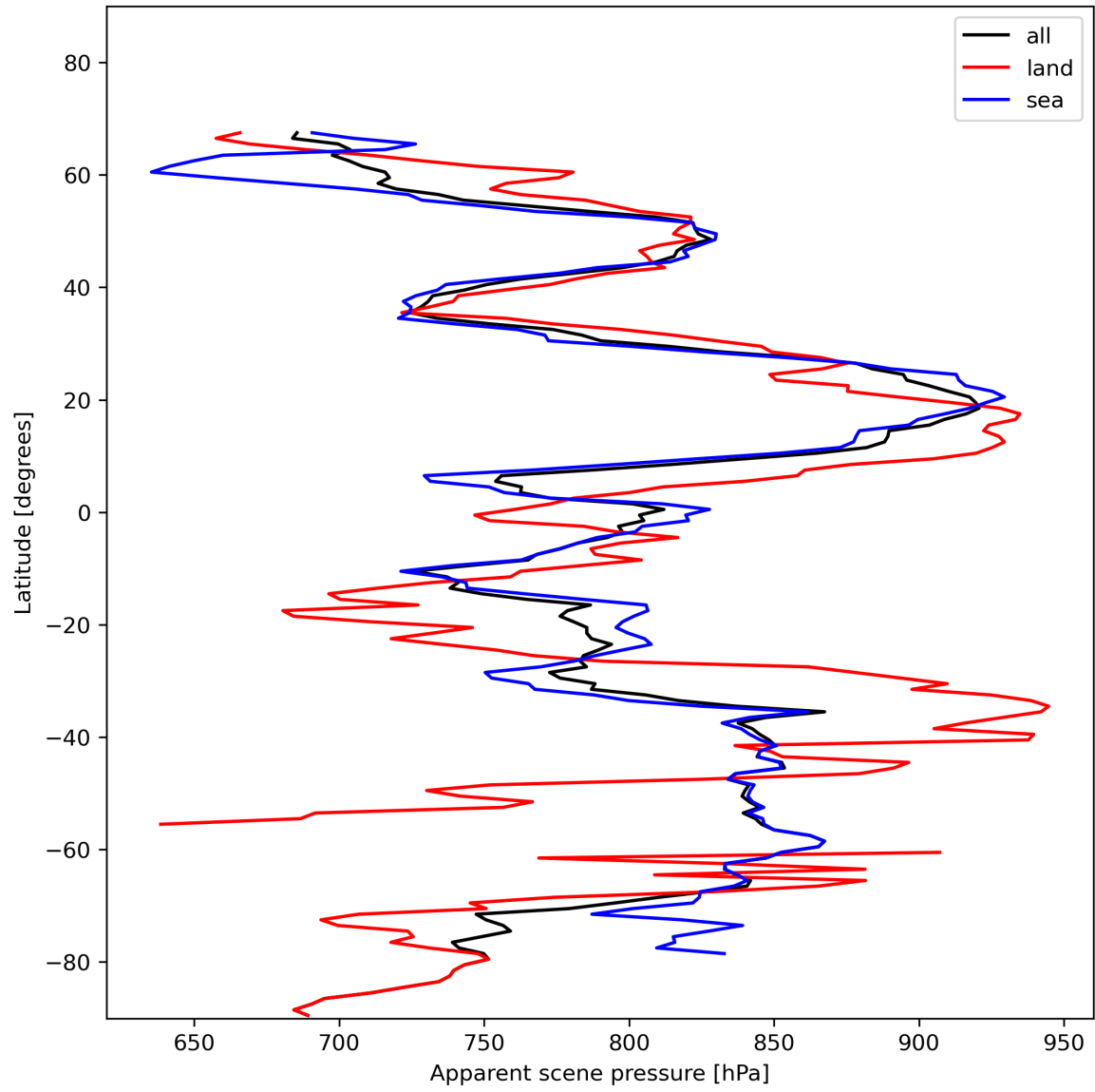
Figure 19: Zonal average of “Apparent scene pressure” for 2024-01-17 to 2024-01-19.
