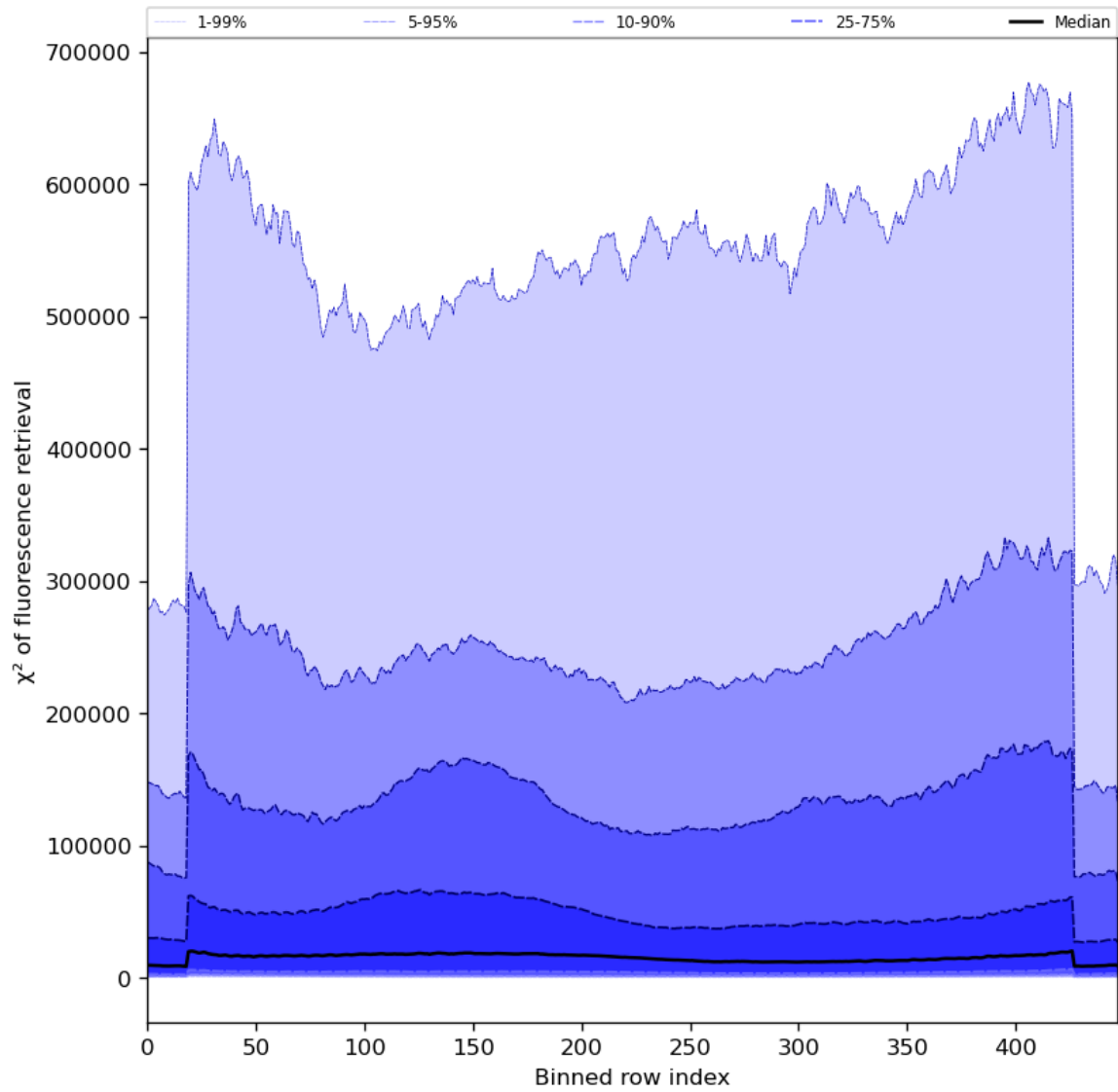
Figure 59: Along track statistics of “ \chi^2 of fluorescence retrieval” for 2024-01-18 to 2024-01-20
