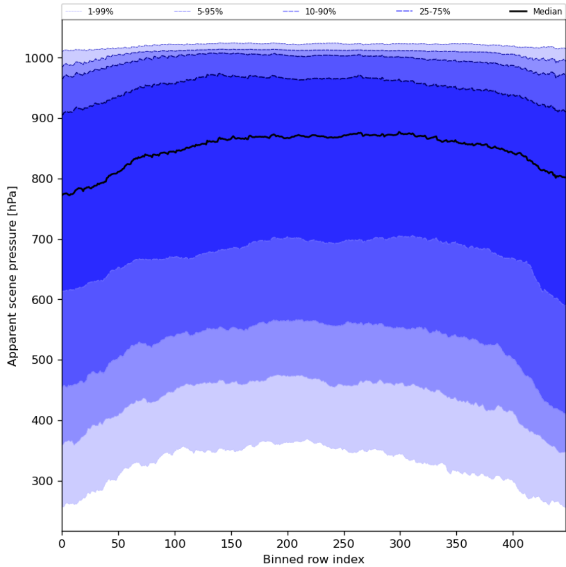
Figure 53: Along track statistics of “Apparent scene pressure” for 2024-01-18 to 2024-01-20
