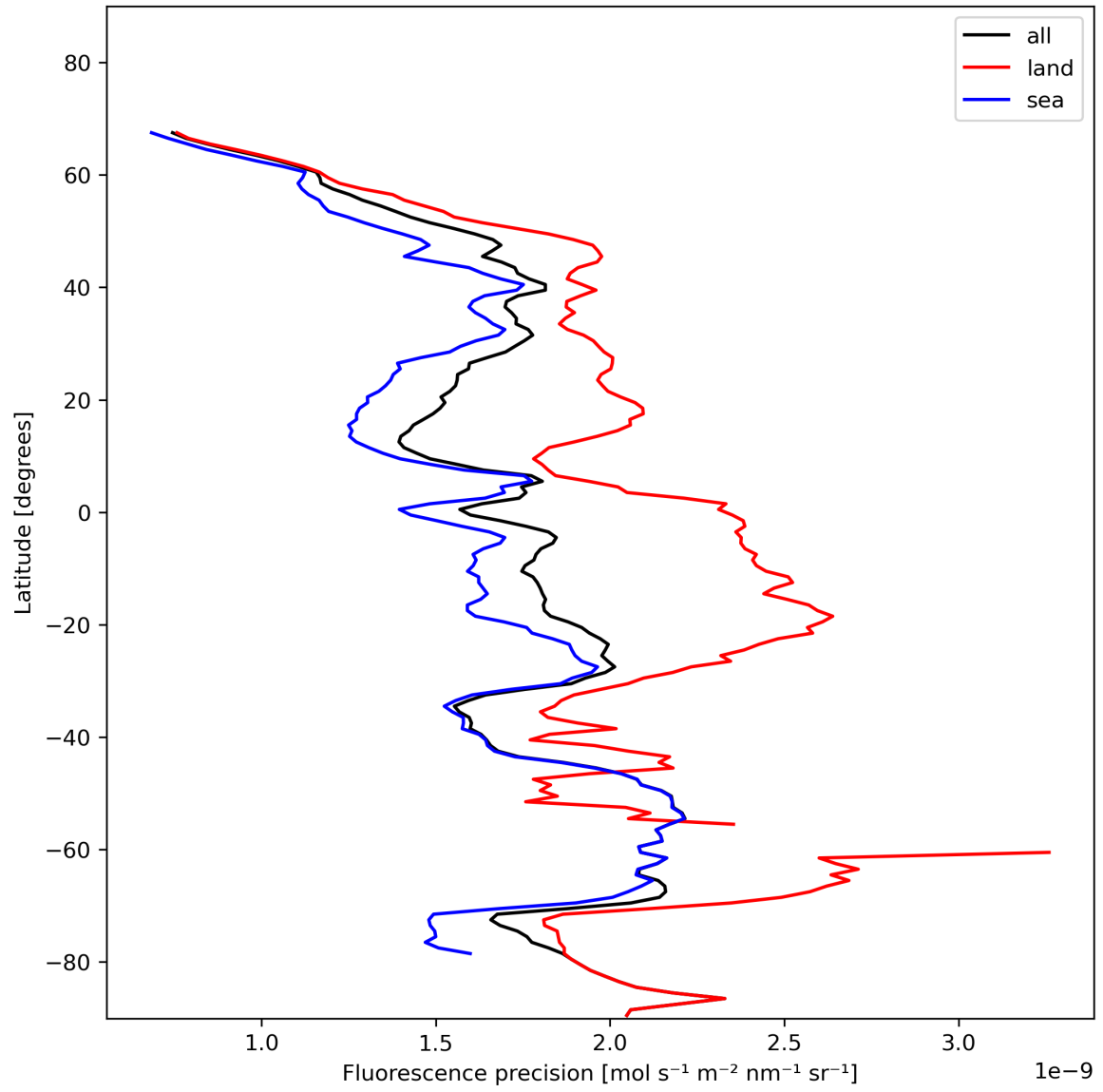
Figure 24: Zonal average of “Fluorescence precision” for 2024-01-18 to 2024-01-20.
