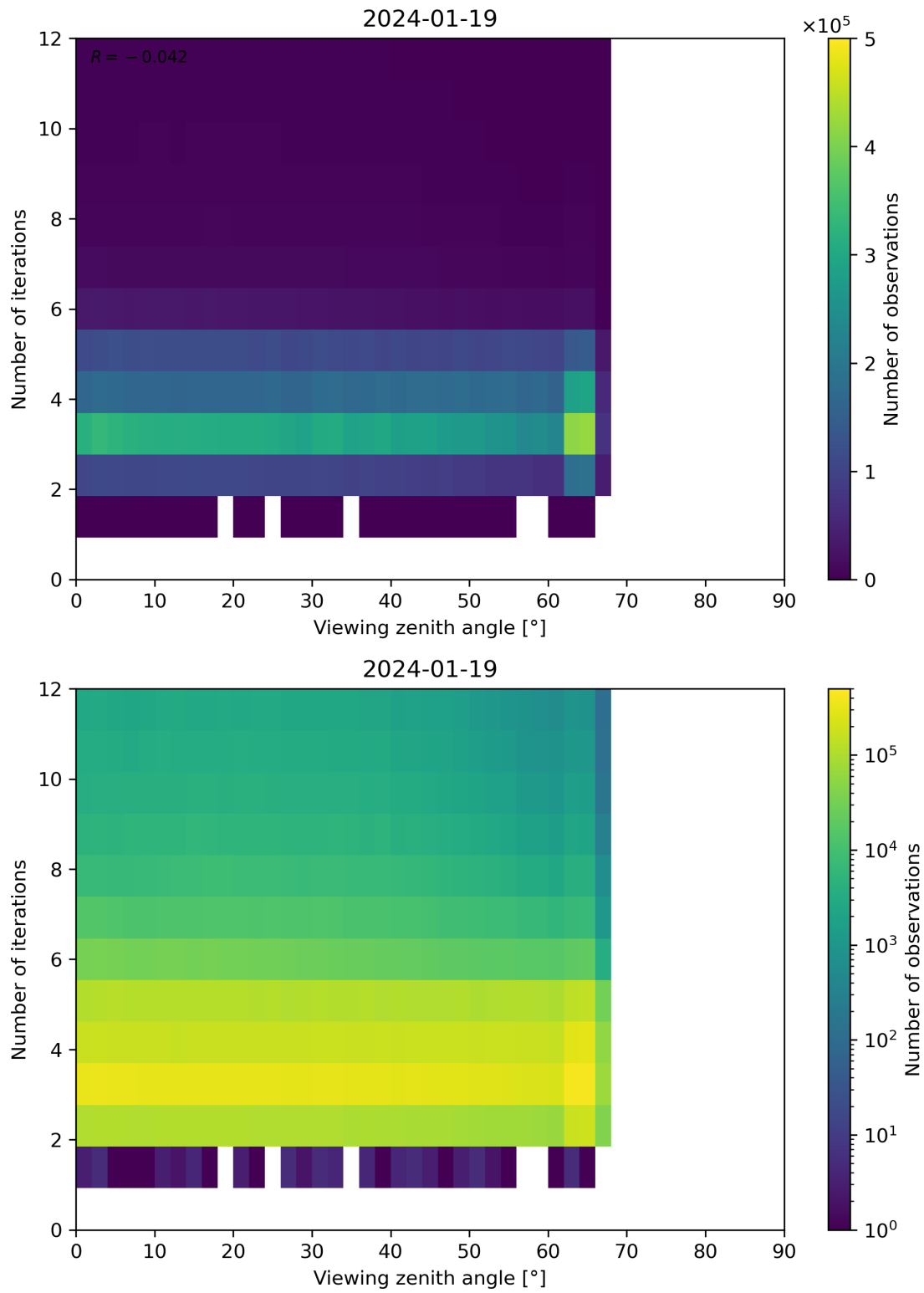
Figure 124: Scatter density plot of “Viewing zenith angle” against “Number of iterations” for 2024-01-18 to 2024-01-20.
