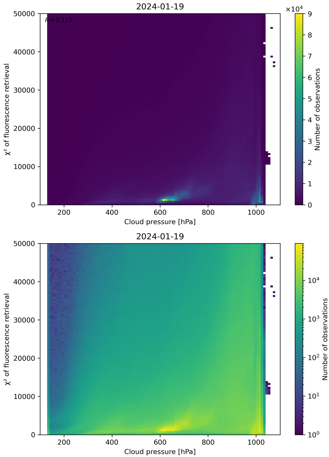
Figure 78: Scatter density plot of “Cloud pressure” against “ \chi^2 of fluorescence retrieval” for 2024-01-18 to 2024-01-20.
