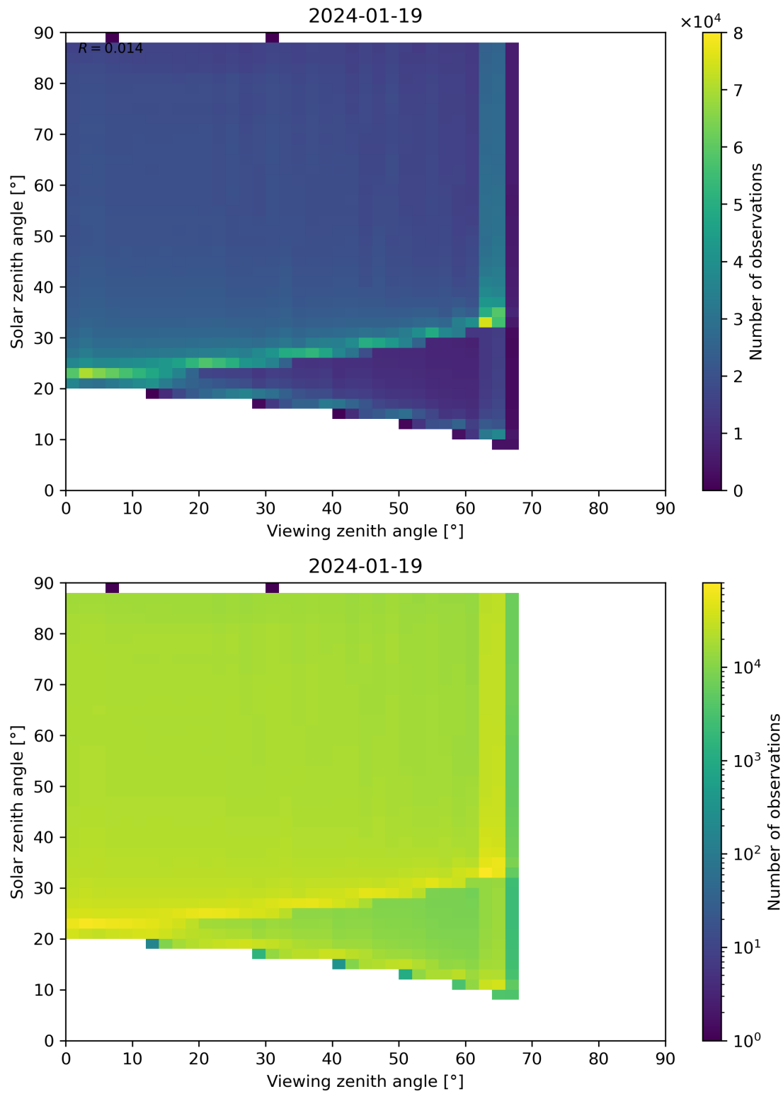
Figure 127: Scatter density plot of “Viewing zenith angle” against “Solar zenith angle” for 2024-01-18 to 2024-01-20.
