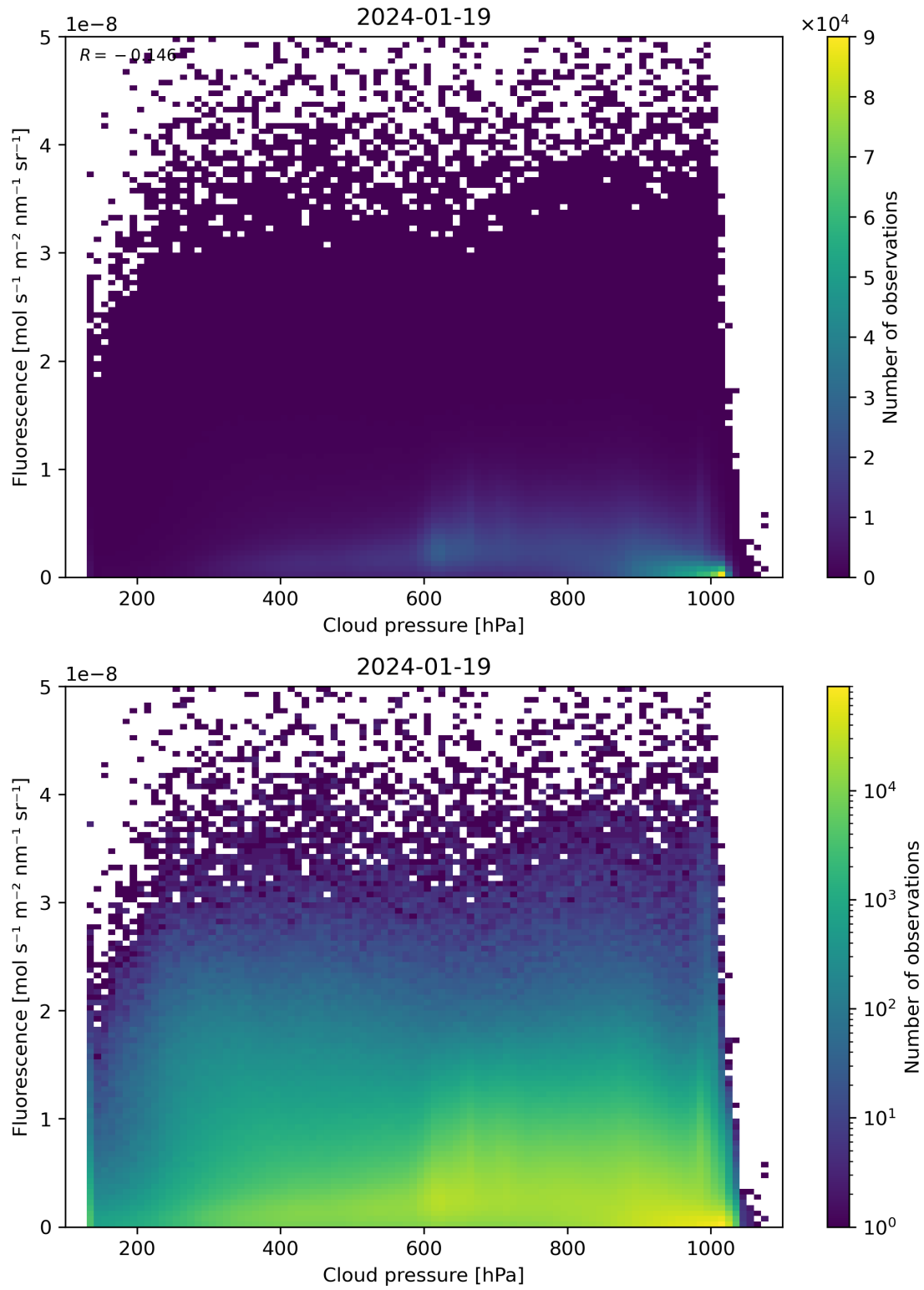
Figure 80: Scatter density plot of “Cloud pressure” against “Fluorescence” for 2024-01-18 to 2024-01-20.
