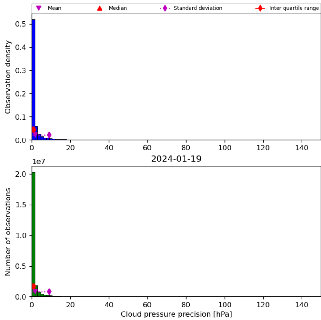
Figure 31: Histogram of “Cloud pressure precision” for 2024-01-18 to 2024-01-20
