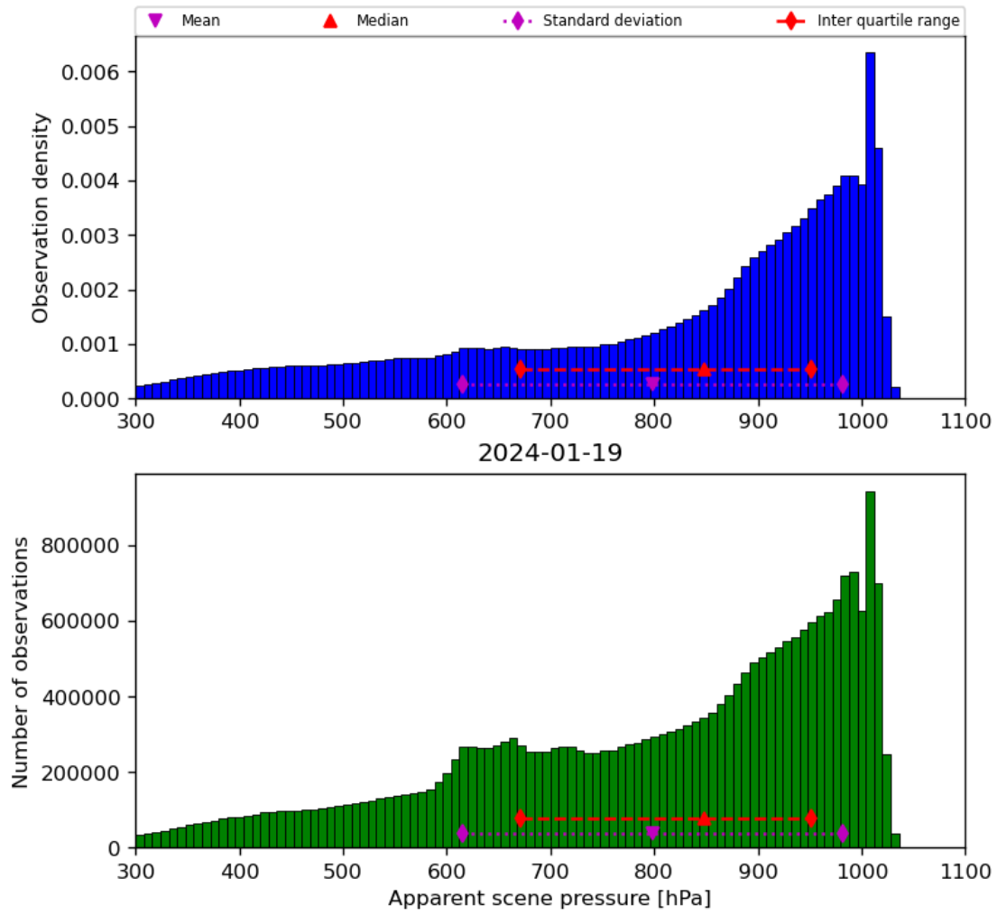
Figure 36: Histogram of “Apparent scene pressure” for 2024-01-18 to 2024-01-20
