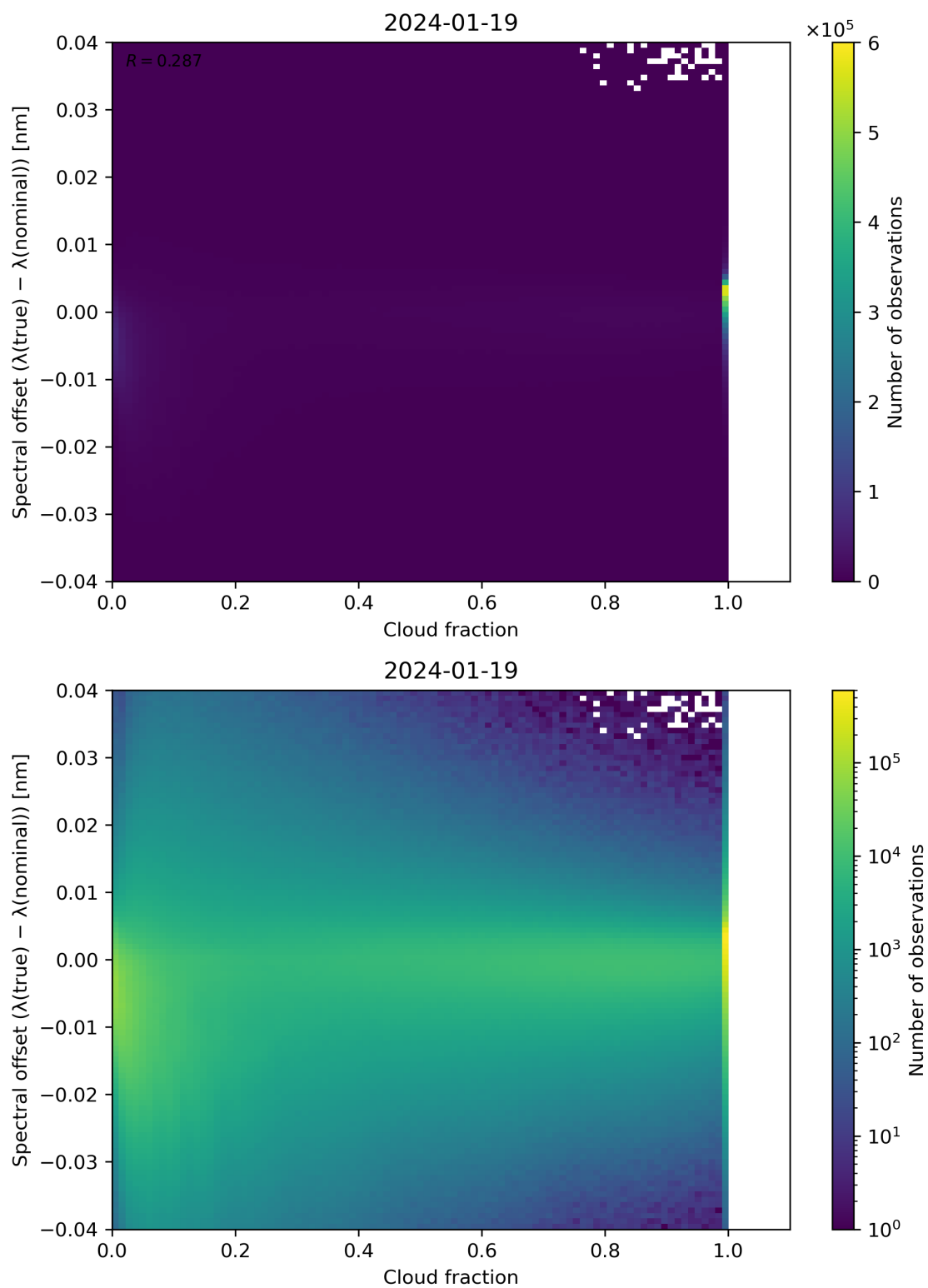
Figure 76: Scatter density plot of “Cloud fraction” against “Spectral offset ( \lambda(\text{true}) - \lambda(\text{nominal}) )” for 2024-01-18 to 2024-01-20.
