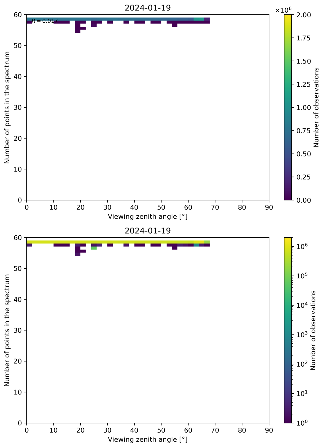
Figure 125: Scatter density plot of “Viewing zenith angle” against “Number of points in the spectrum” for 2024-01-18 to 2024-01-20.
