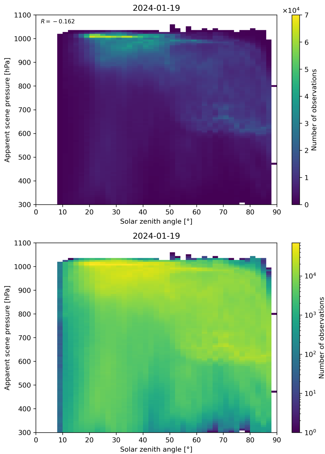
Figure 108: Scatter density plot of “Solar zenith angle” against “Apparent scene pressure” for 2024-01-18 to 2024-01-20.
