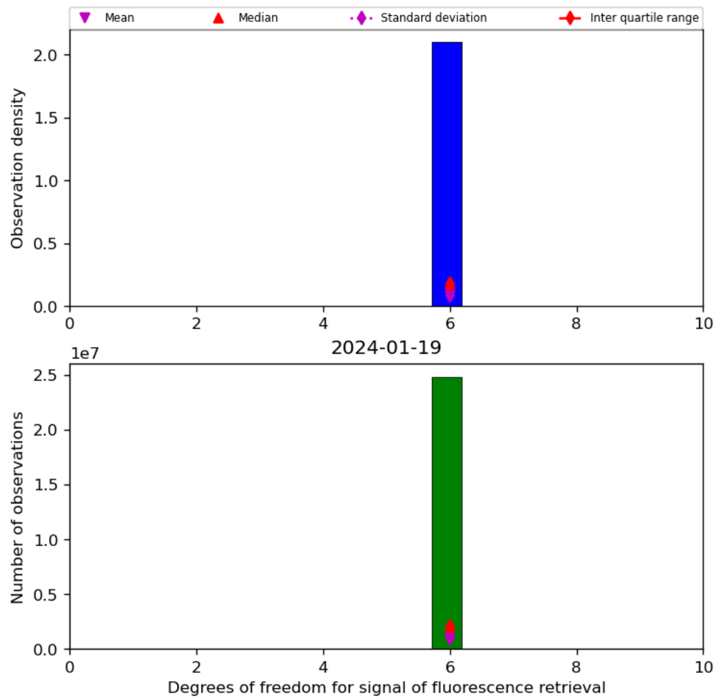
Figure 43: Histogram of “Degrees of freedom for signal of fluorescence retrieval” for 2024-01-18 to 2024-01-20
