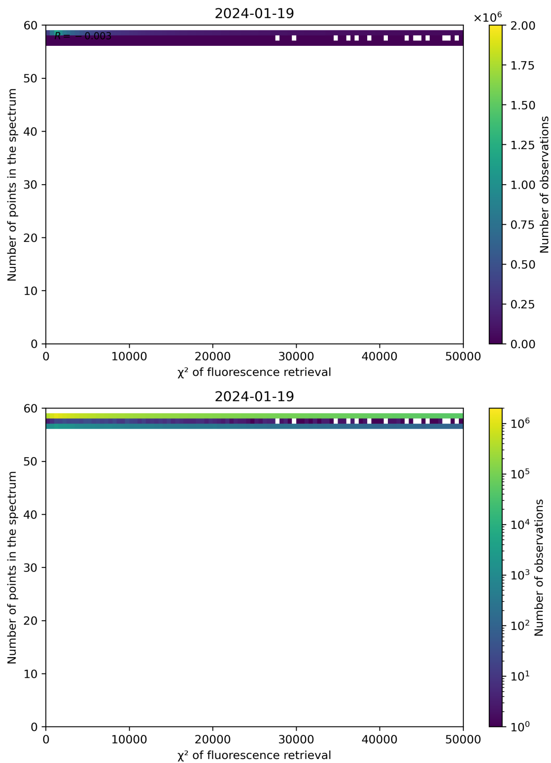
Figure 68: Scatter density plot of " \chi^2 of fluorescence retrieval" against "Number of points in the spectrum" for 2024-01-18 to 2024-01-20.
