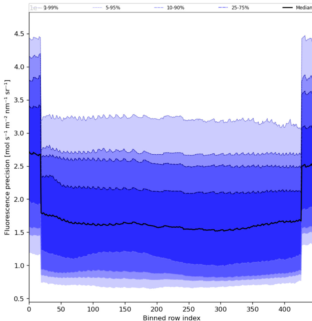
Figure 58: Along track statistics of “Fluorescence precision” for 2024-01-18 to 2024-01-20
