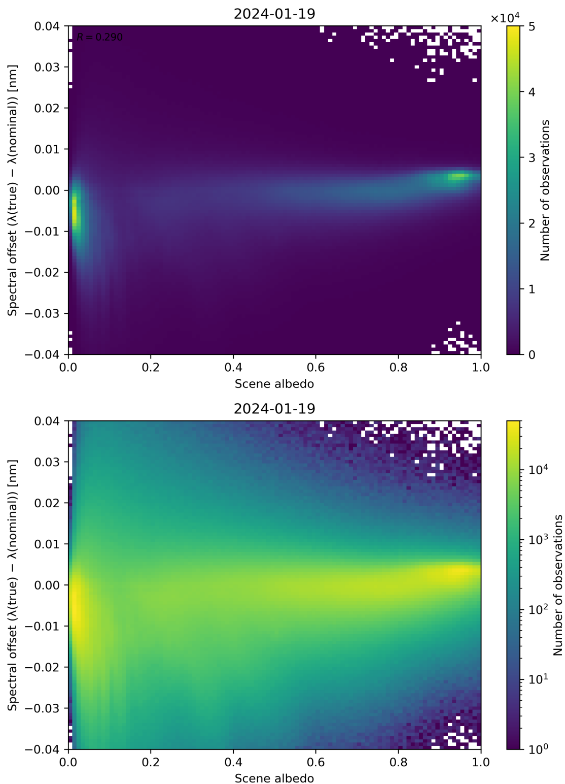
Figure 107: Scatter density plot of “Scene albedo” against “Spectral offset ( \lambda(\text{true}) - \lambda(\text{nominal}) )” for 2024-01-18 to 2024-01-20.
