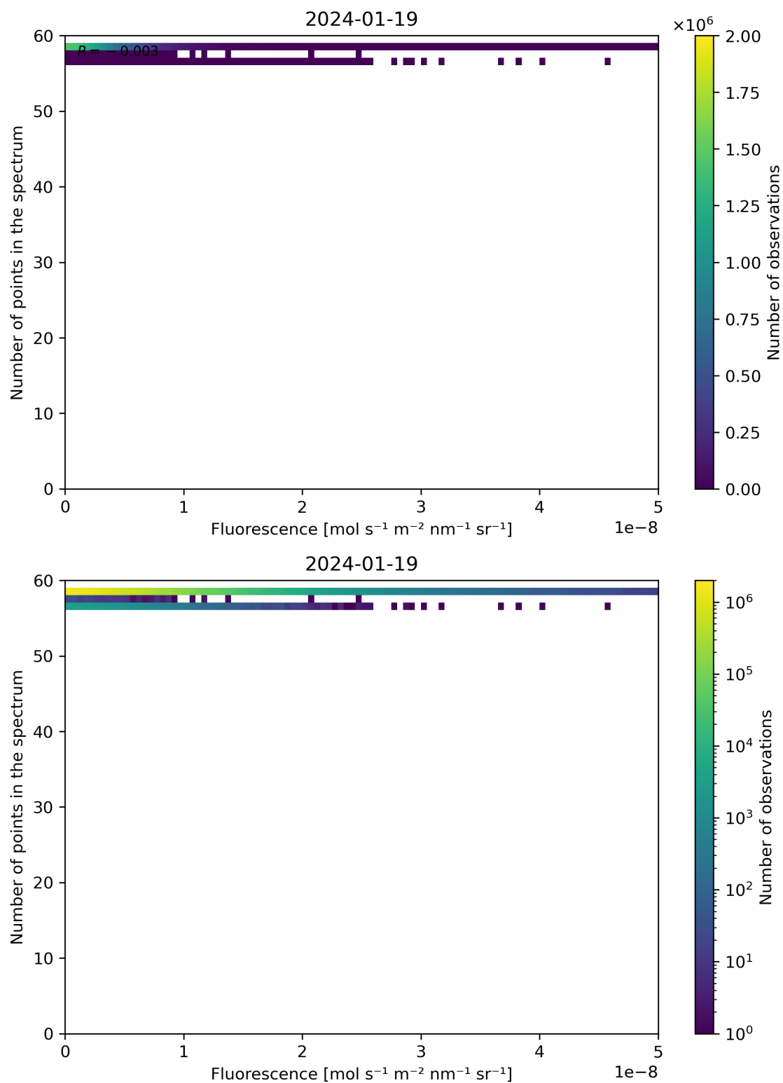
Figure 86: Scatter density plot of “Fluorescence” against “Number of points in the spectrum” for 2024-01-18 to 2024-01-20.
