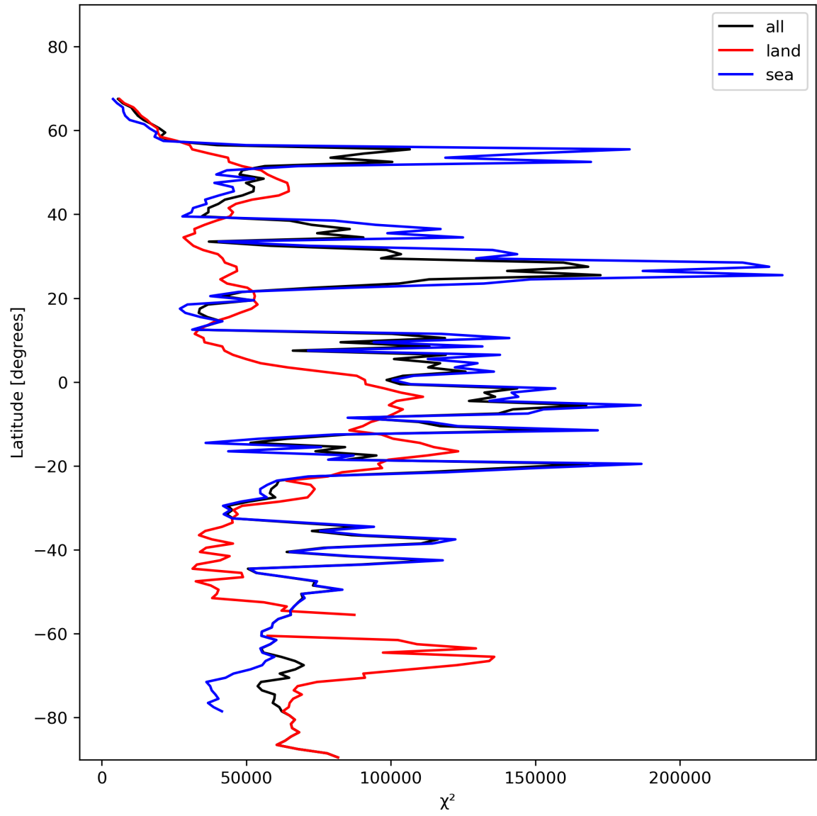
Figure 21: Zonal average of “ \chi^2 ” for 2024-01-18 to 2024-01-20.
