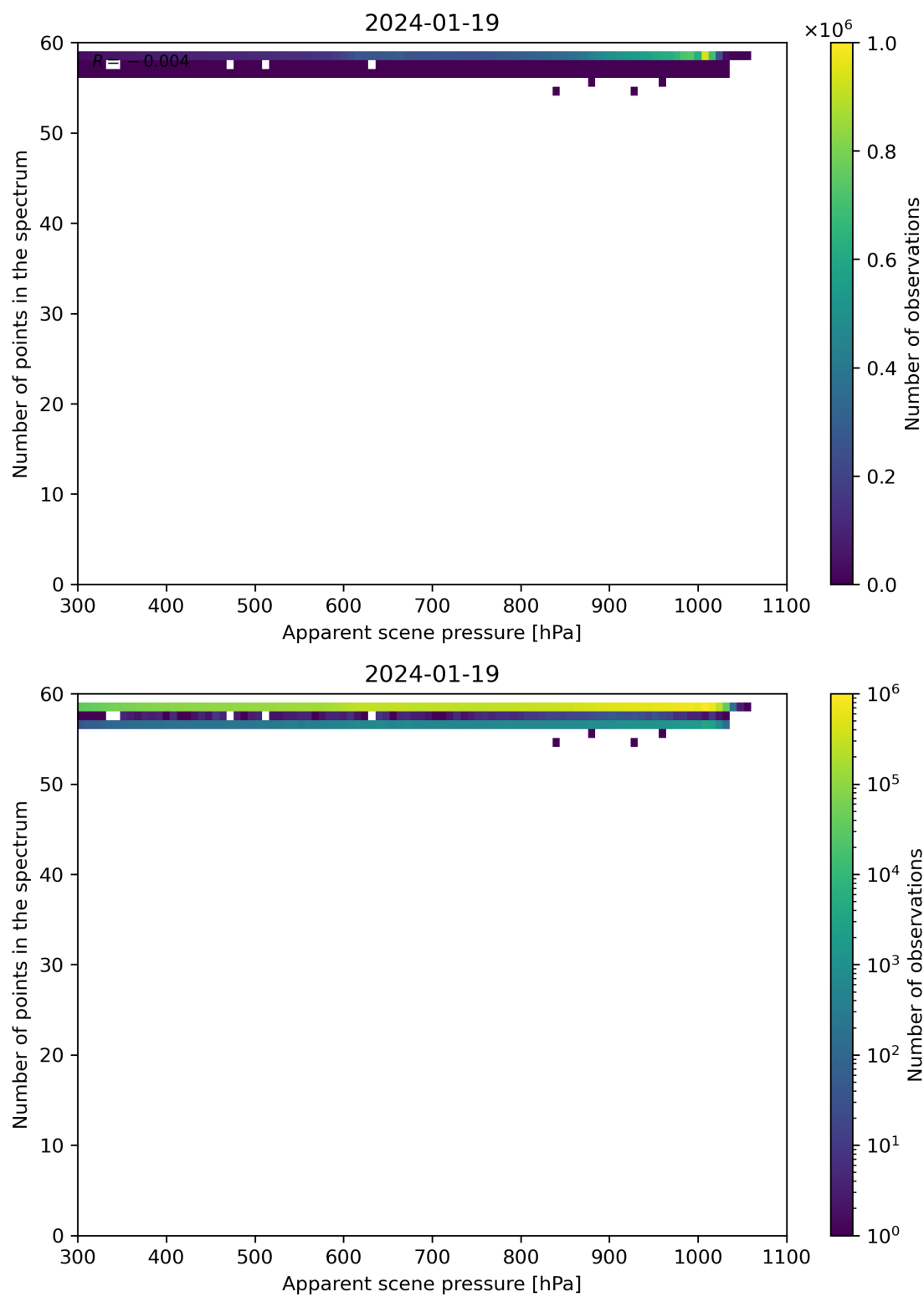
Figure 66: Scatter density plot of “Apparent scene pressure” against “Number of points in the spectrum” for 2024-01-18 to 2024-01-20.
