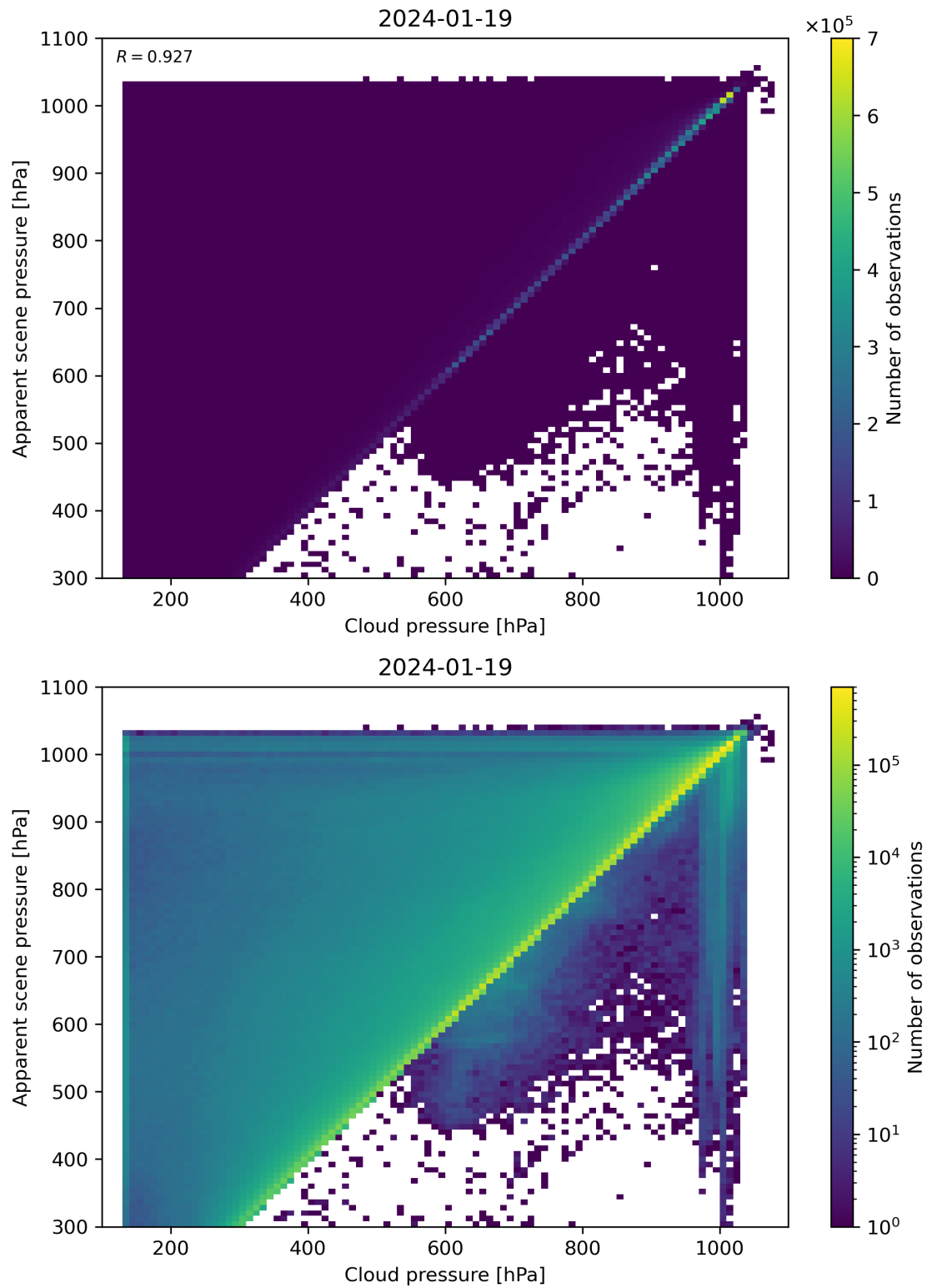
Figure 77: Scatter density plot of “Cloud pressure” against “Apparent scene pressure” for 2024-01-18 to 2024-01-20.
