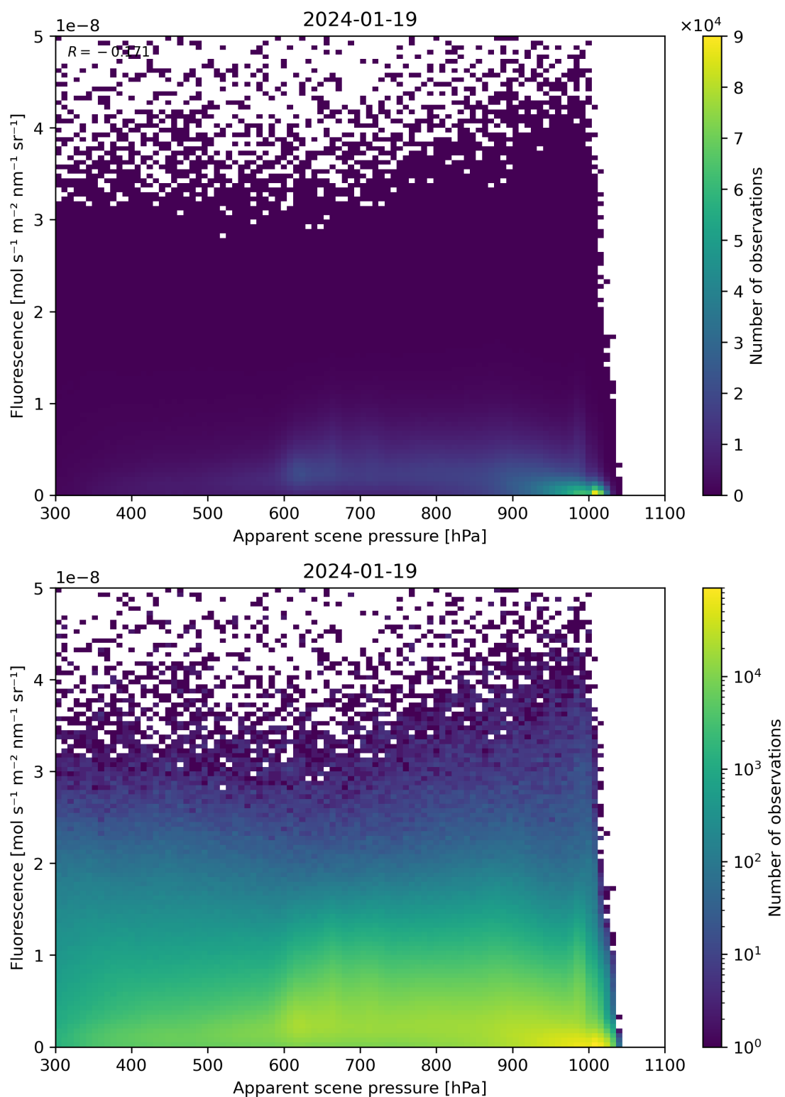
Figure 64: Scatter density plot of “Apparent scene pressure” against “Fluorescence” for 2024-01-18 to 2024-01-20.
