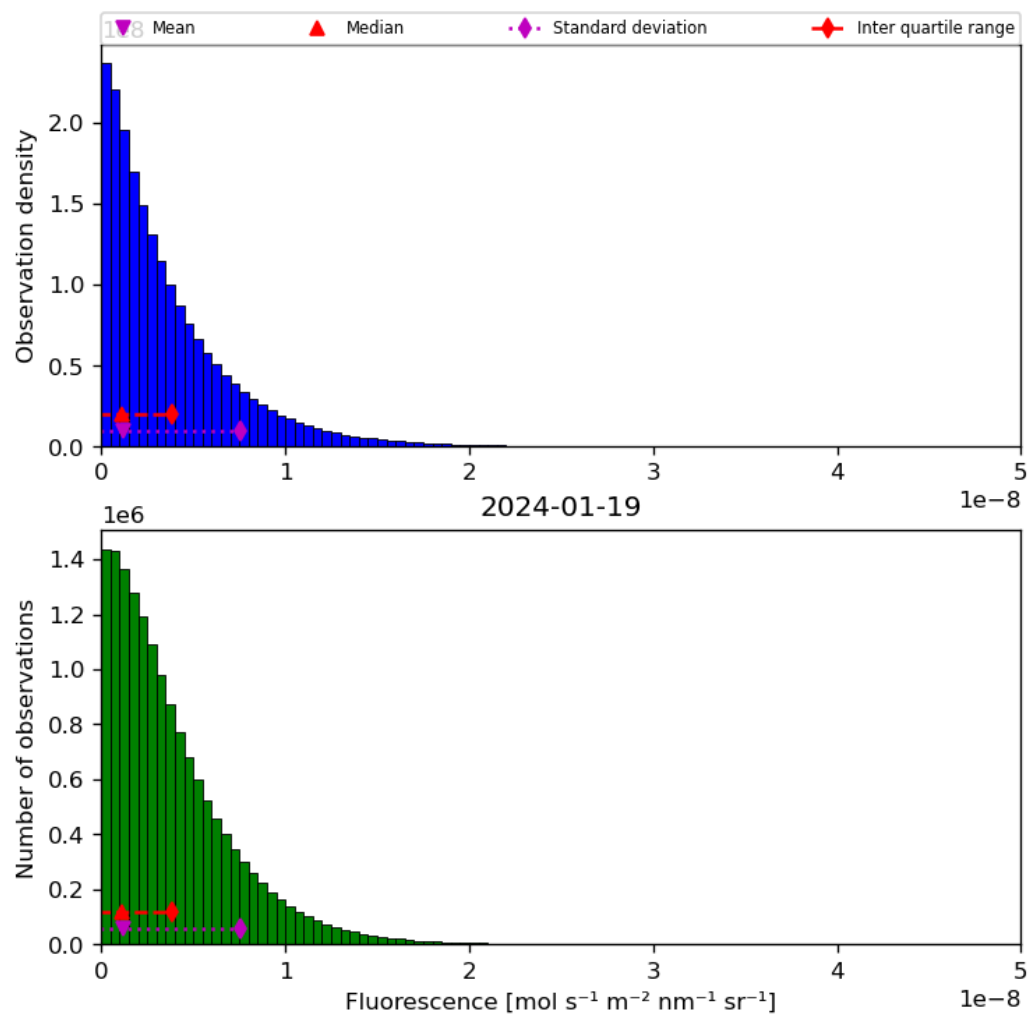
Figure 40: Histogram of “Fluorescence” for 2024-01-18 to 2024-01-20
