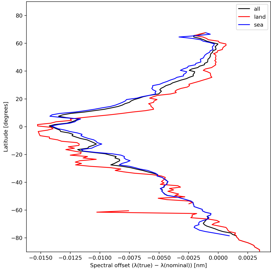
Figure 28: Zonal average of “Spectral offset ( \lambda(\text{true}) - \lambda(\text{nominal}) )” for 2024-01-18 to 2024-01-20.
