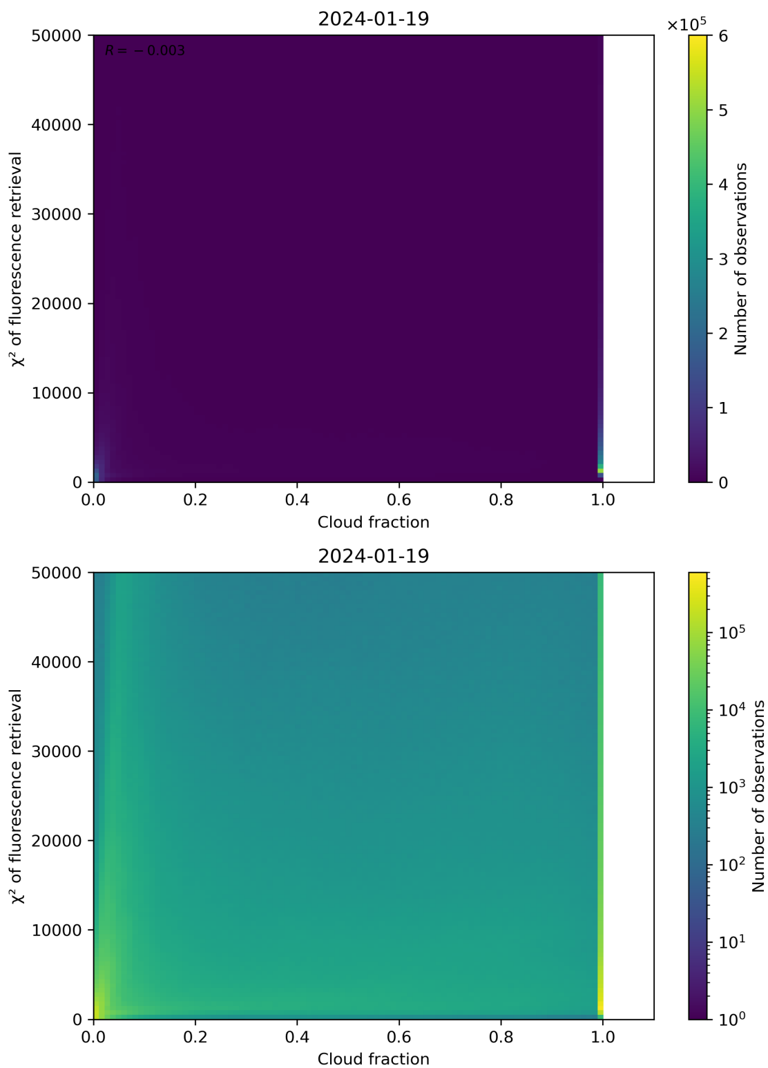
Figure 71: Scatter density plot of “Cloud fraction” against “ \chi^2 of fluorescence retrieval” for 2024-01-18 to 2024-01-20.
