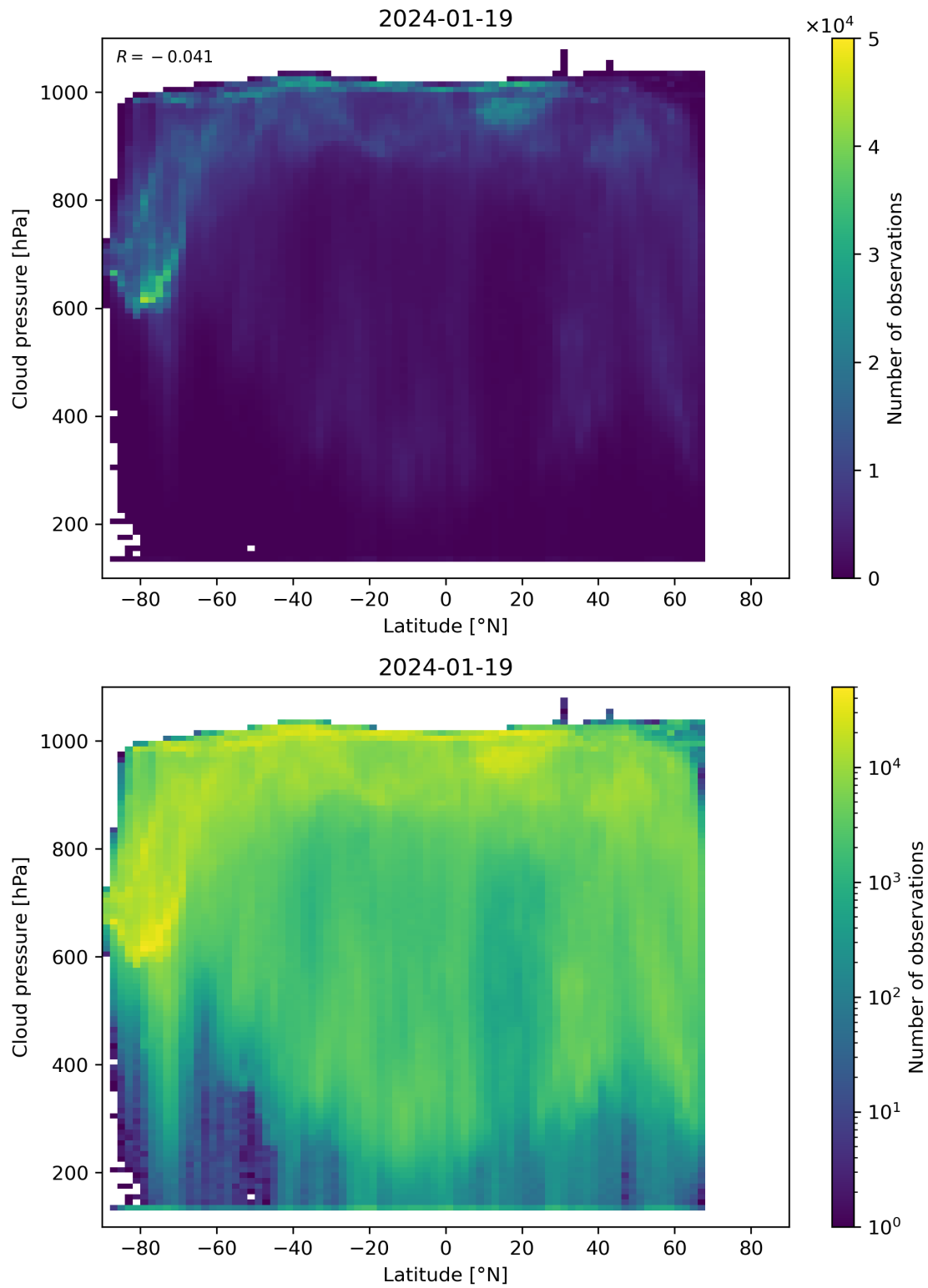
Figure 91: Scatter density plot of “Latitude” against “Cloud pressure” for 2024-01-18 to 2024-01-20.
