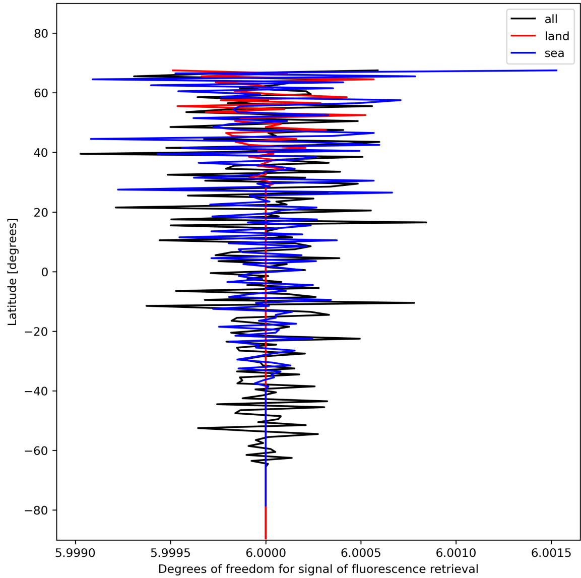
Figure 26: Zonal average of “Degrees of freedom for signal of fluorescence retrieval” for 2024-01-18 to 2024-01-20.
