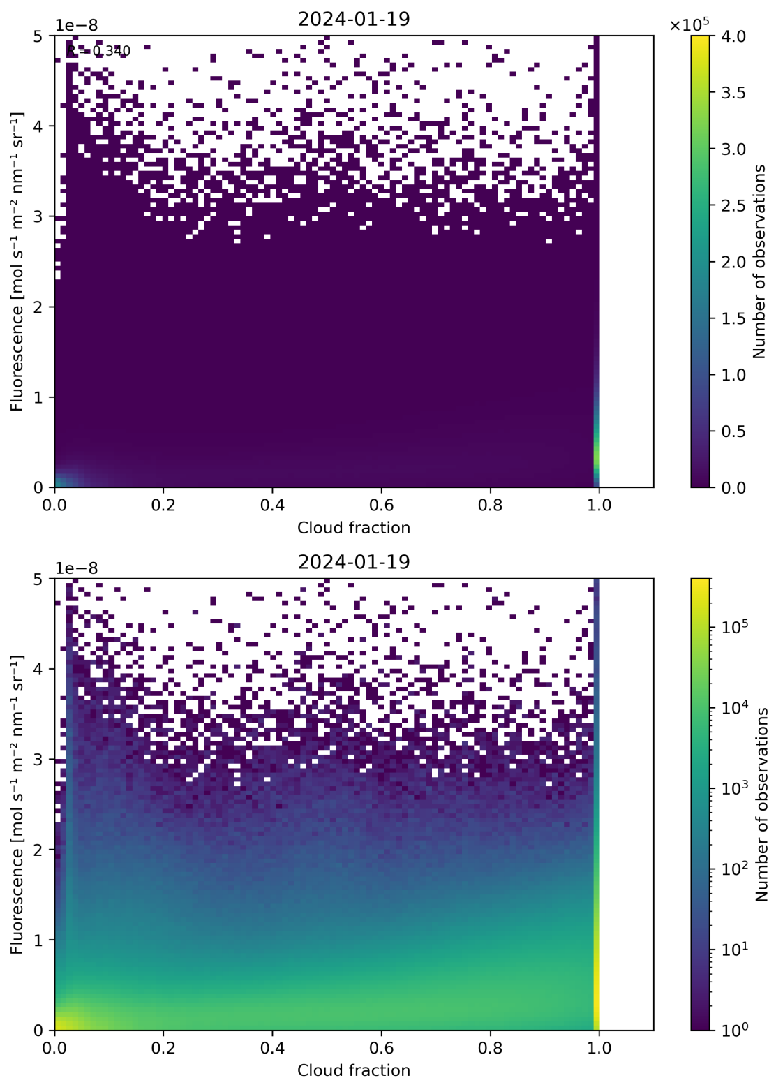
Figure 72: Scatter density plot of “Cloud fraction” against “Fluorescence” for 2024-01-18 to 2024-01-20.
