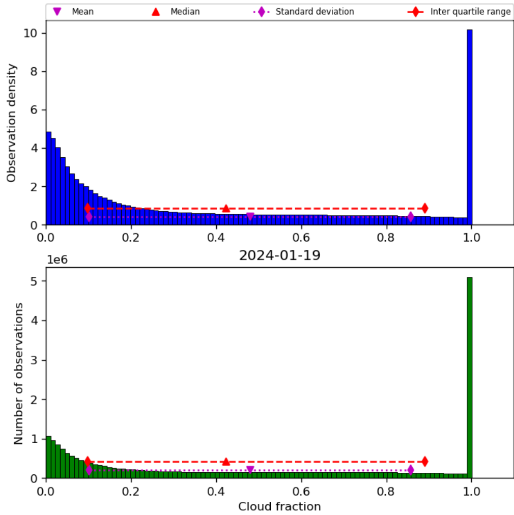
Figure 32: Histogram of “Cloud fraction” for 2024-01-18 to 2024-01-20
