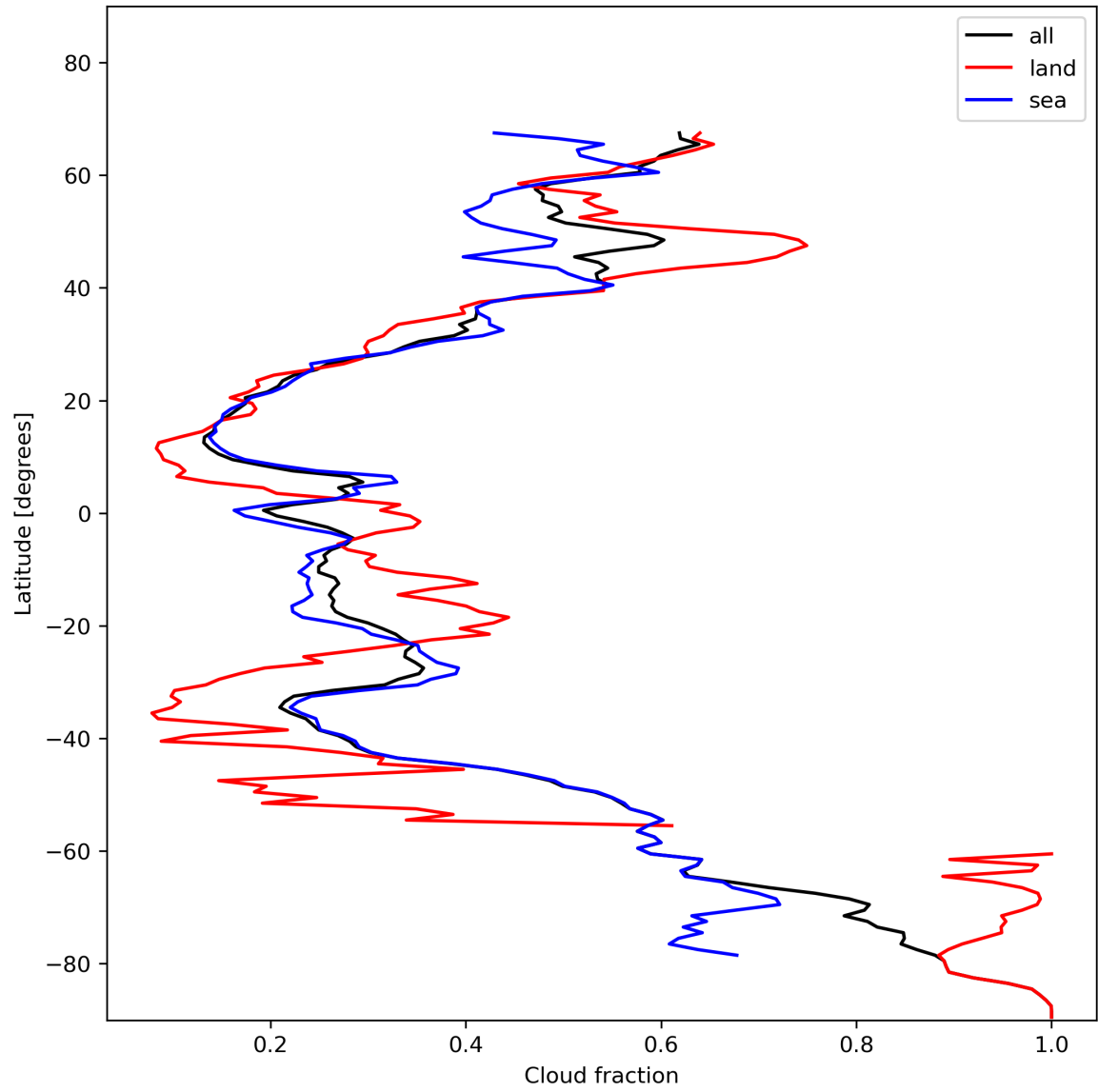
Figure 15: Zonal average of “Cloud fraction” for 2024-01-18 to 2024-01-20.
