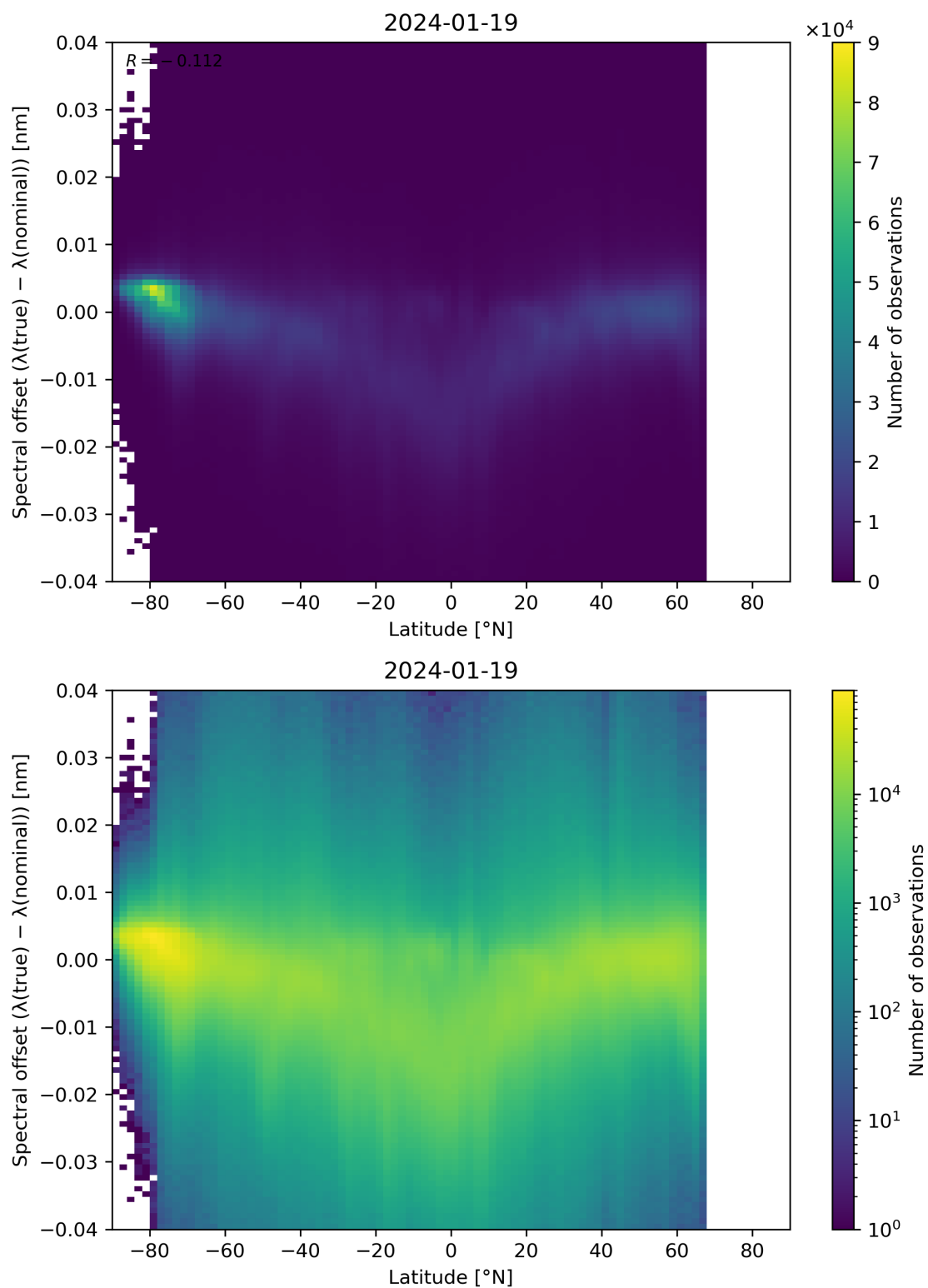
Figure 96: Scatter density plot of “Latitude” against “Spectral offset ( \lambda(\text{true}) - \lambda(\text{nominal}) )” for 2024-01-18 to 2024-01-20.
