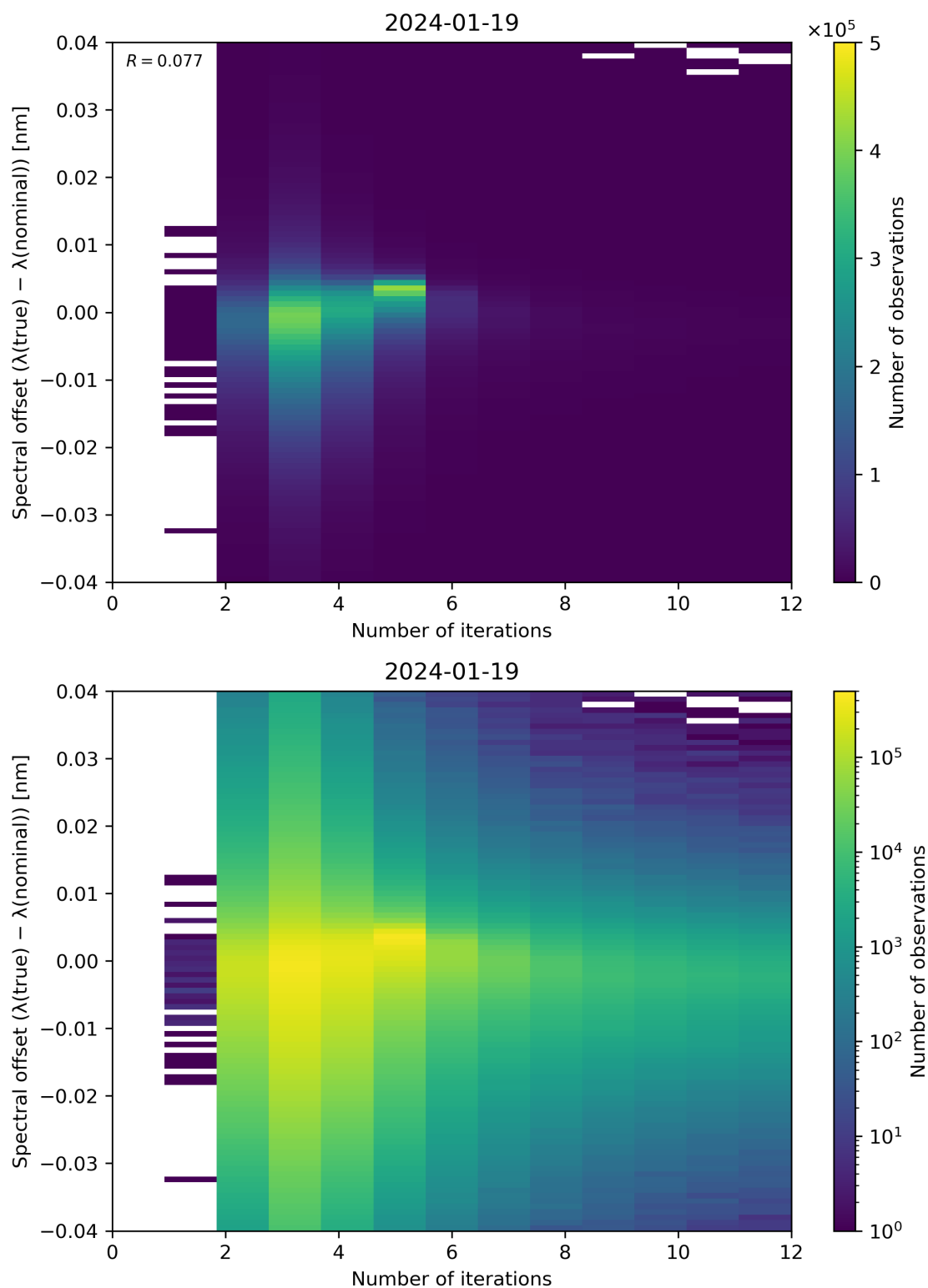
Figure 100: Scatter density plot of “Number of iterations” against “Spectral offset ( \lambda(\text{true}) - \lambda(\text{nominal}) )” for 2024-01-18 to 2024-01-20.
