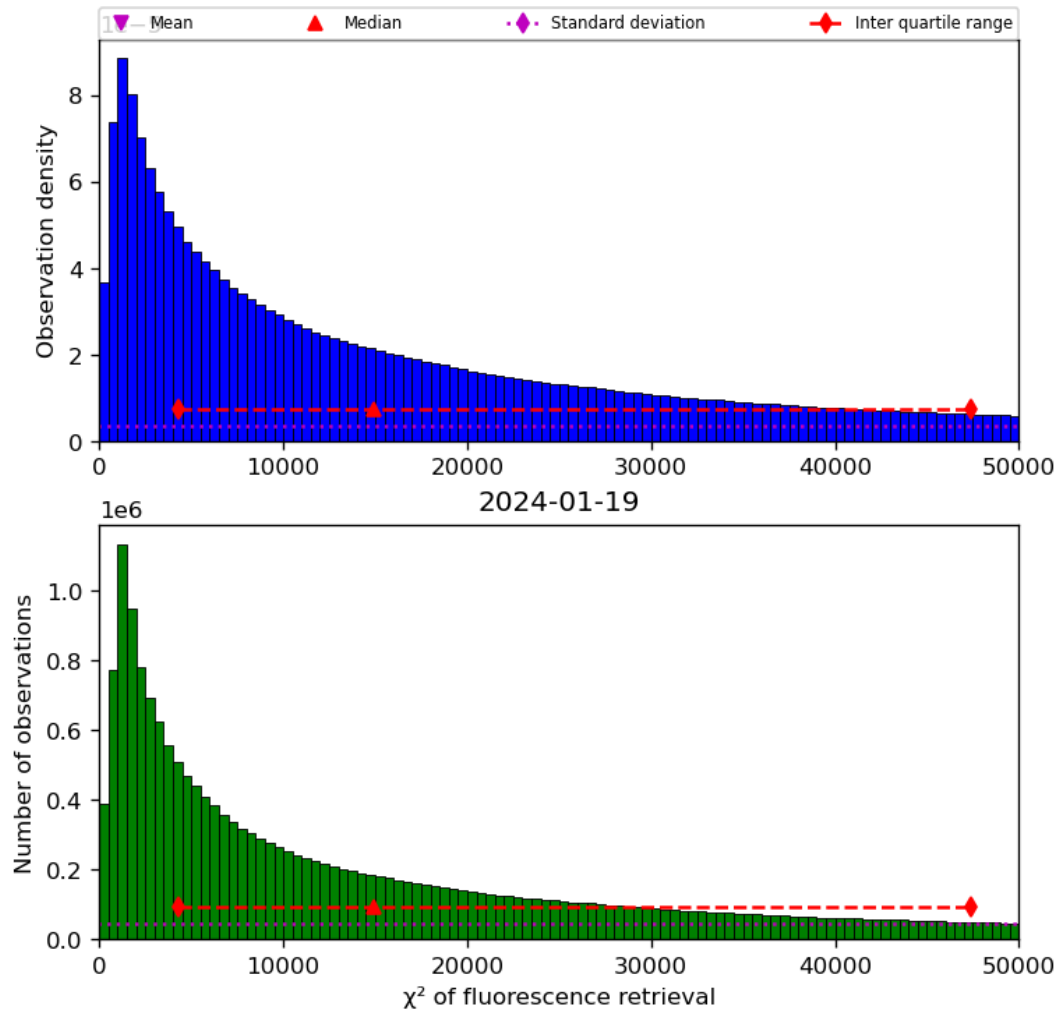
Figure 42: Histogram of “ \chi^2 of fluorescence retrieval” for 2024-01-18 to 2024-01-20
