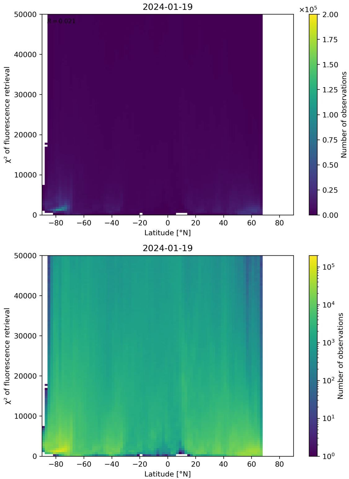
Figure 89: Scatter density plot of “Latitude” against “ \chi^2 of fluorescence retrieval” for 2024-01-18 to 2024-01-20.
