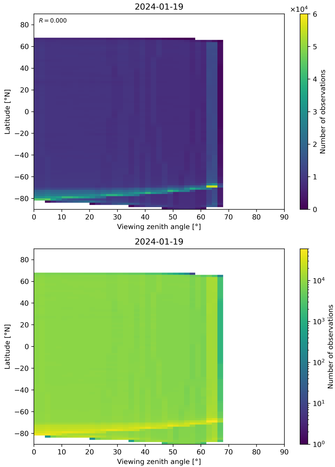
Figure 123: Scatter density plot of “Viewing zenith angle” against “Latitude” for 2024-01-18 to 2024-01-20.
