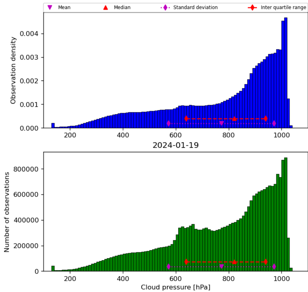
Figure 30: Histogram of “Cloud pressure” for 2024-01-18 to 2024-01-20
