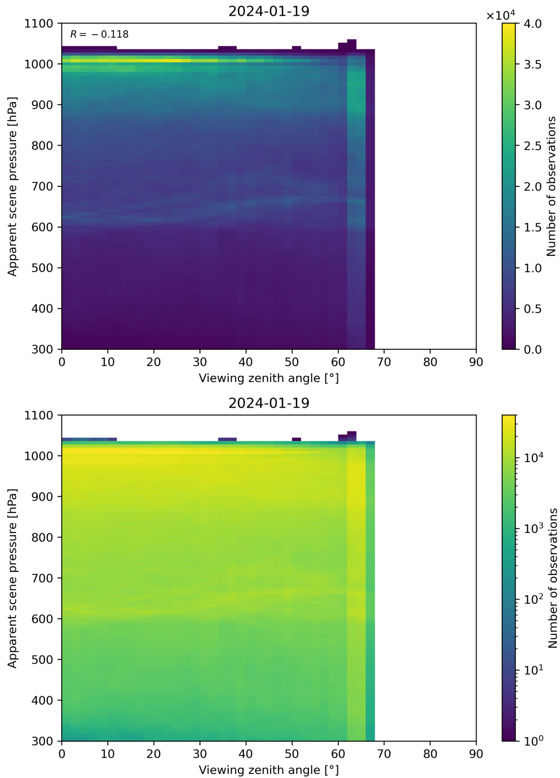
Figure 118: Scatter density plot of “Viewing zenith angle” against “Apparent scene pressure” for 2024-01-18 to 2024-01-20.
