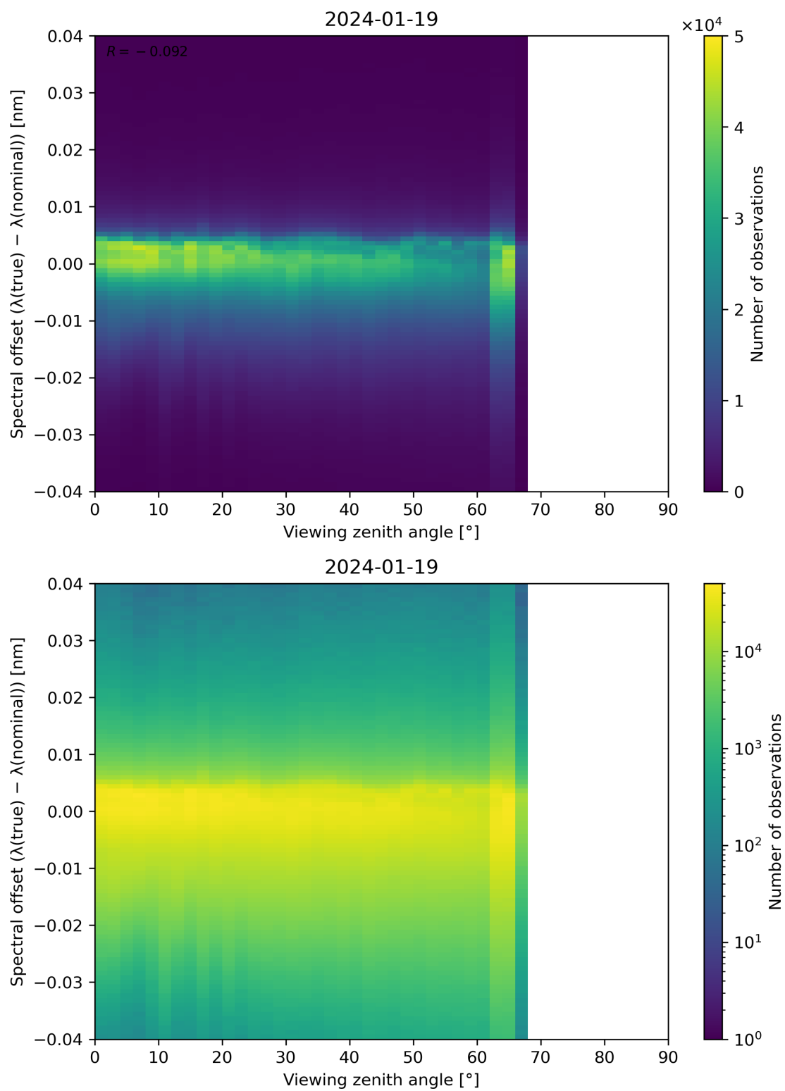
Figure 128: Scatter density plot of “Viewing zenith angle” against “Spectral offset ( \lambda(\text{true}) - \lambda(\text{nominal}) )” for 2024-01-18 to 2024-01-20.
