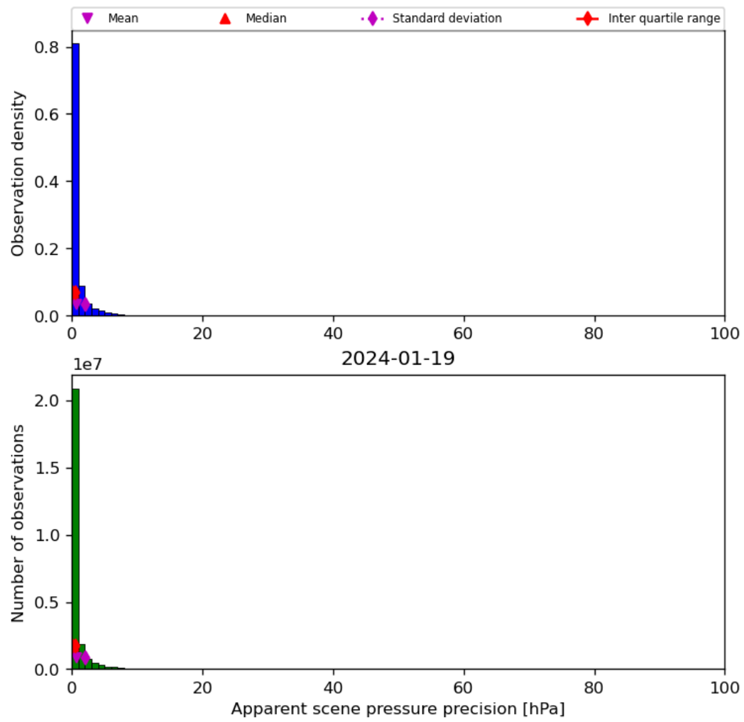
Figure 37: Histogram of “Apparent scene pressure precision” for 2024-01-18 to 2024-01-20
