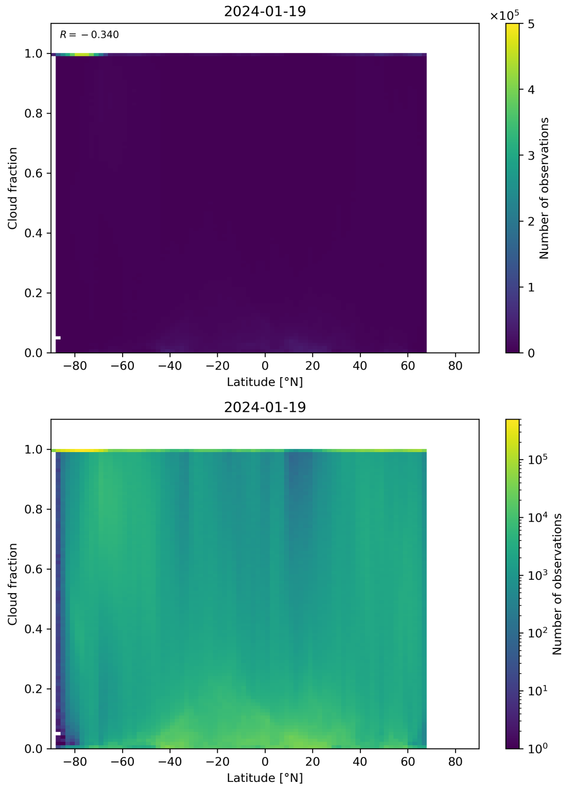
Figure 90: Scatter density plot of “Latitude” against “Cloud fraction” for 2024-01-18 to 2024-01-20.
