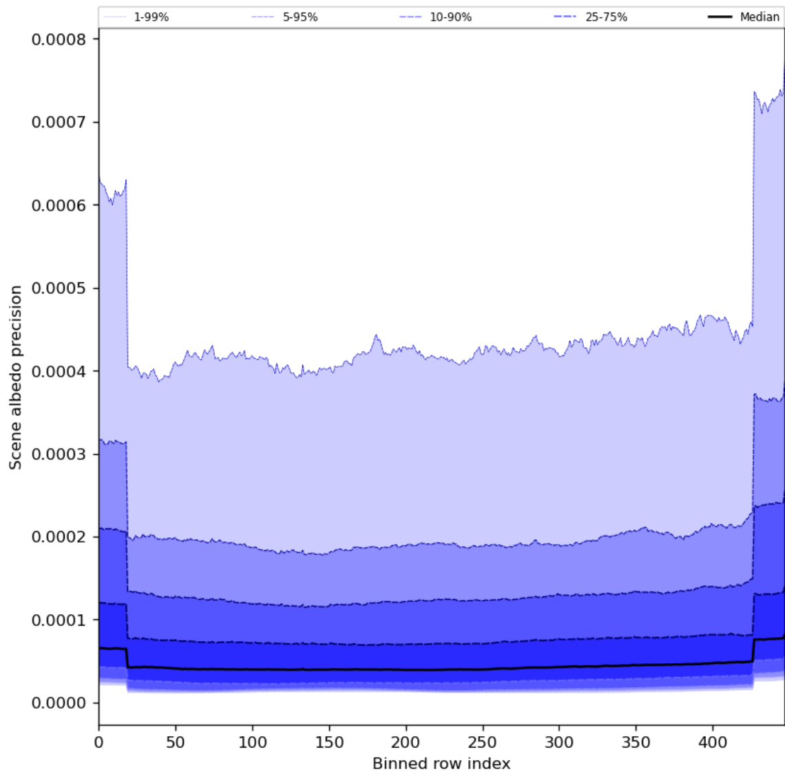
Figure 52: Along track statistics of “Scene albedo precision” for 2024-01-18 to 2024-01-20
