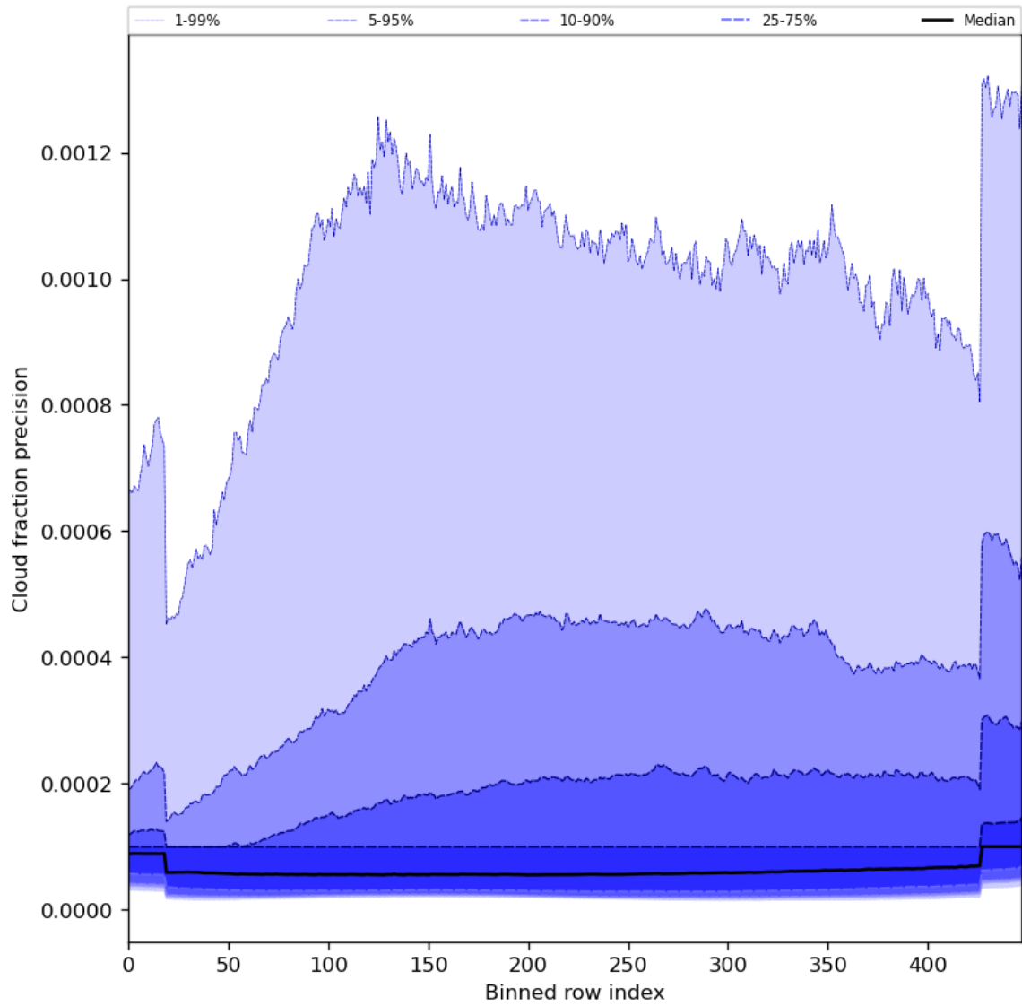
Figure 50: Along track statistics of “Cloud fraction precision” for 2024-01-18 to 2024-01-20
