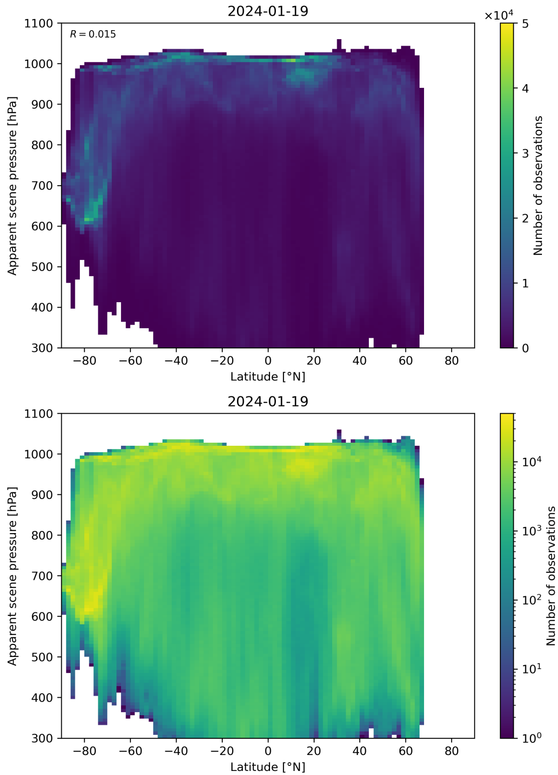
Figure 88: Scatter density plot of “Latitude” against “Apparent scene pressure” for 2024-01-18 to 2024-01-20.
