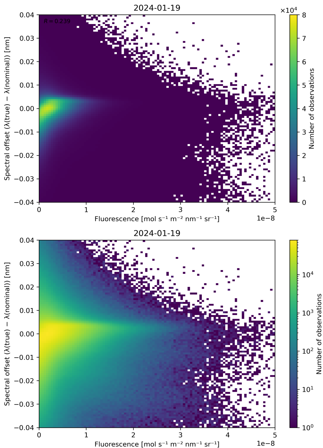
Figure 87: Scatter density plot of “Fluorescence” against “Spectral offset ( \lambda(\text{true}) - \lambda(\text{nominal}) )” for 2024-01-18 to 2024-01-20.
