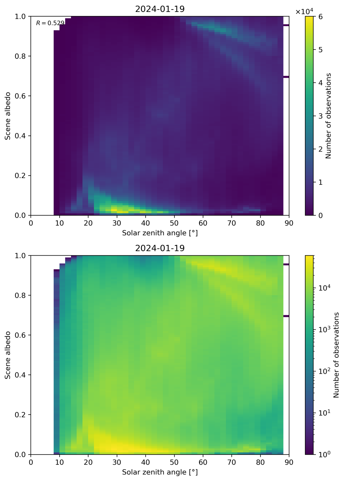
Figure 116: Scatter density plot of “Solar zenith angle” against “Scene albedo” for 2024-01-18 to 2024-01-20.
