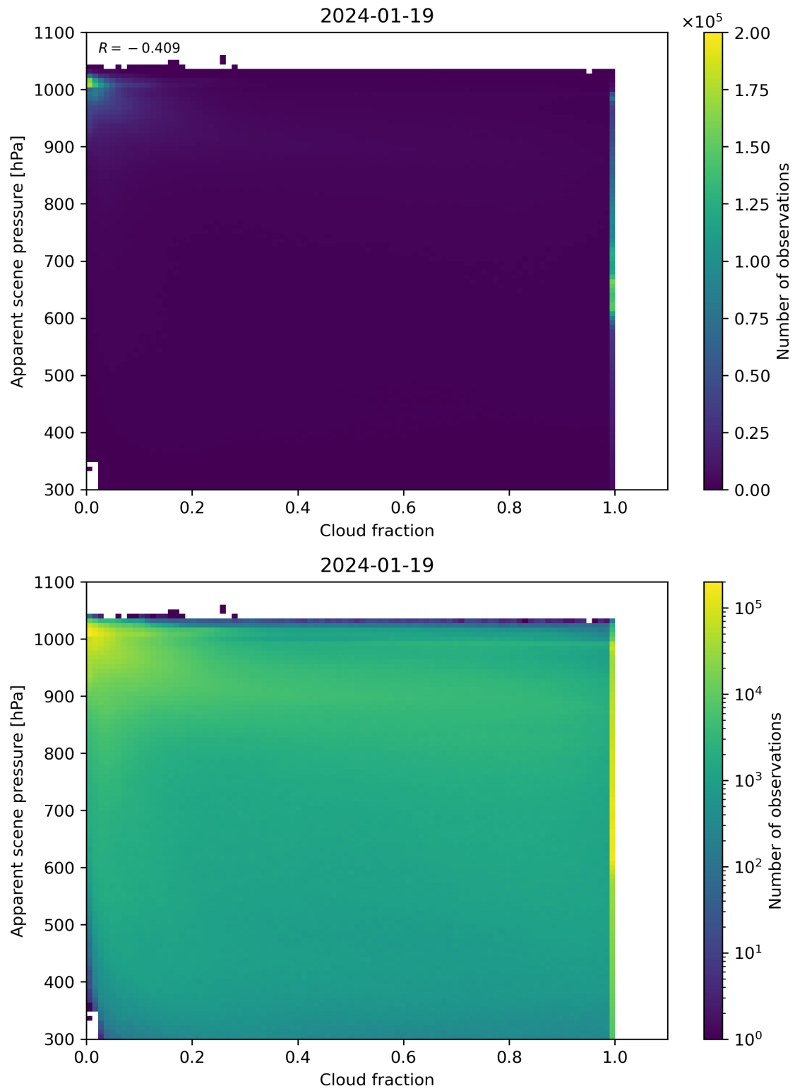
Figure 70: Scatter density plot of “Cloud fraction” against “Apparent scene pressure” for 2024-01-18 to 2024-01-20.
