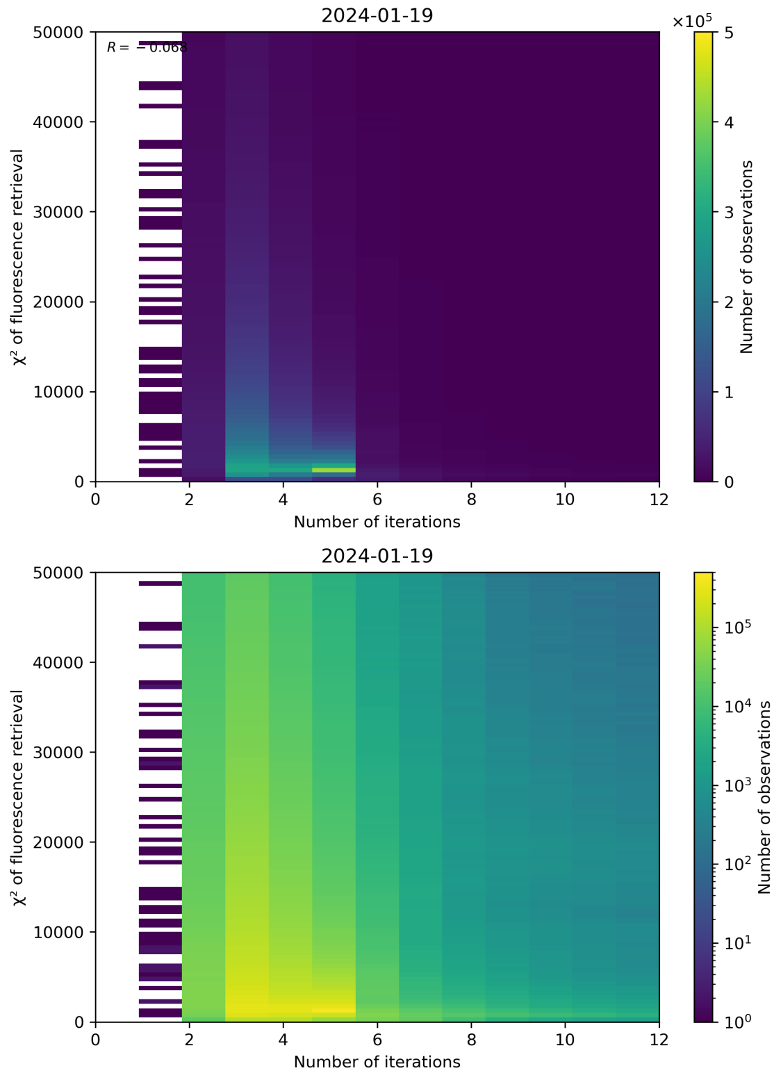
Figure 97: Scatter density plot of “Number of iterations” against “ \chi^2 of fluorescence retrieval” for 2024-01-18 to 2024-01-20.
