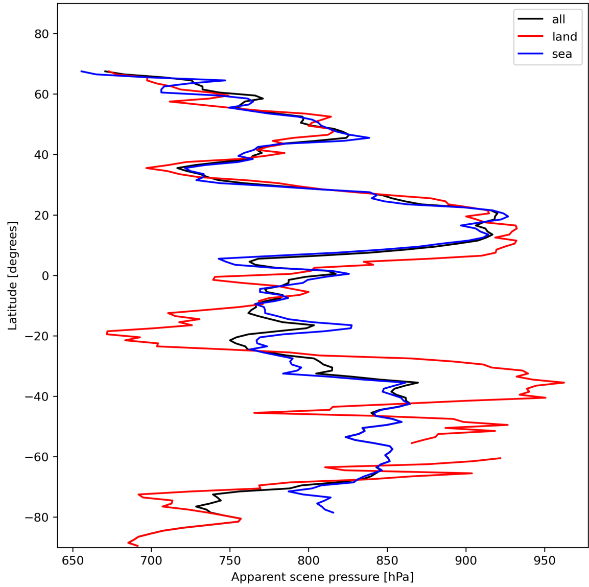
Figure 19: Zonal average of “Apparent scene pressure” for 2024-01-18 to 2024-01-20.
