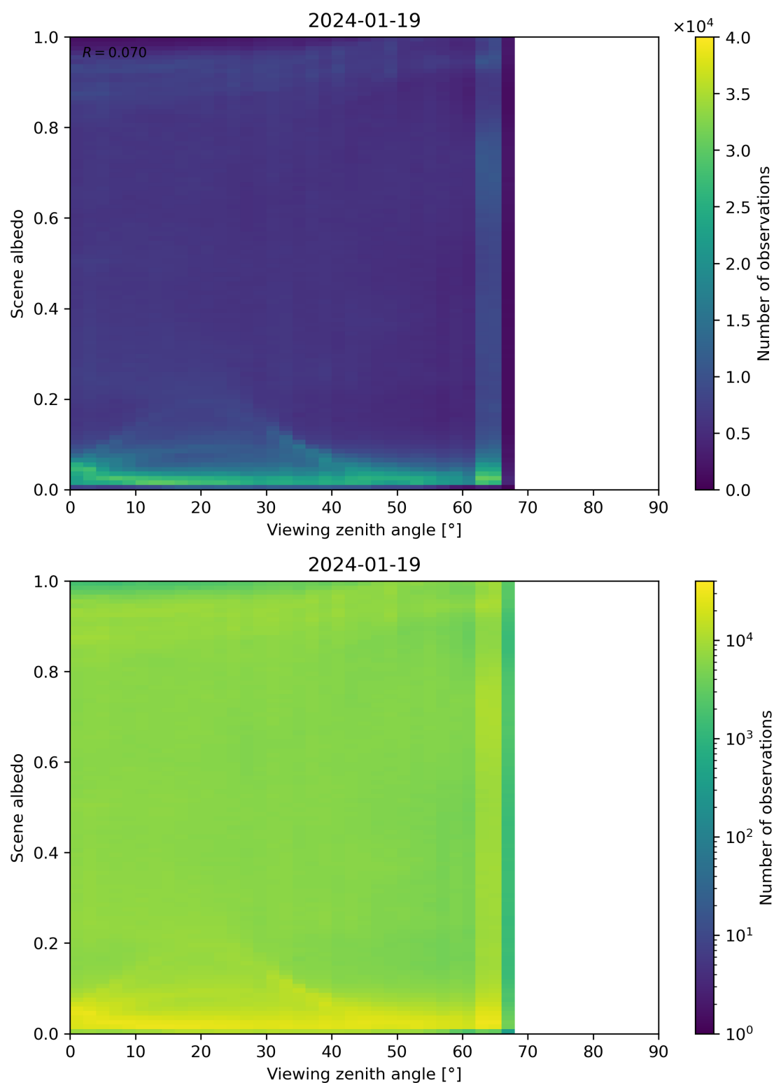
Figure 126: Scatter density plot of “Viewing zenith angle” against “Scene albedo” for 2024-01-18 to 2024-01-20.
