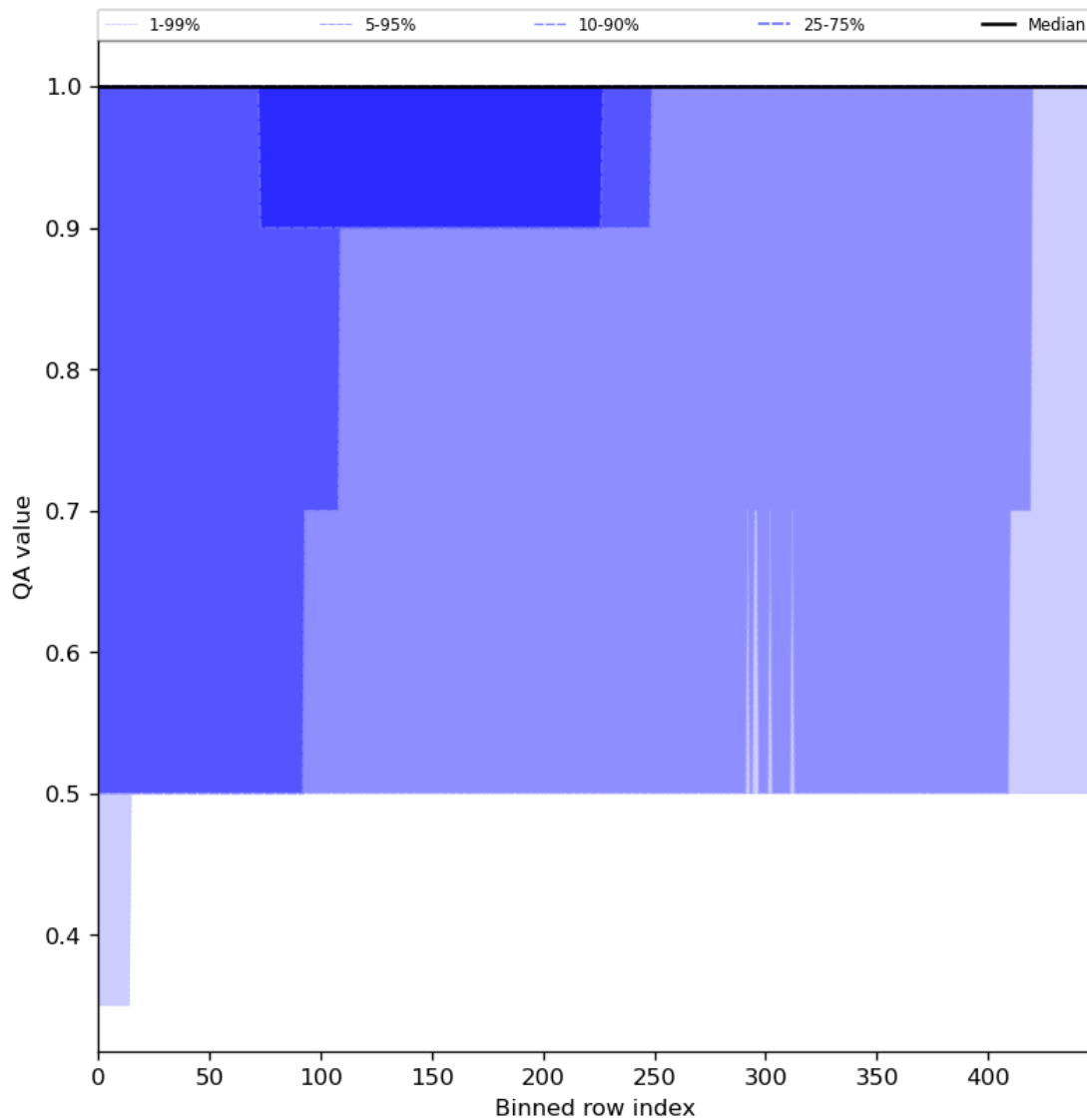
Figure 46: Along track statistics of “QA value” for 2024-01-18 to 2024-01-20
