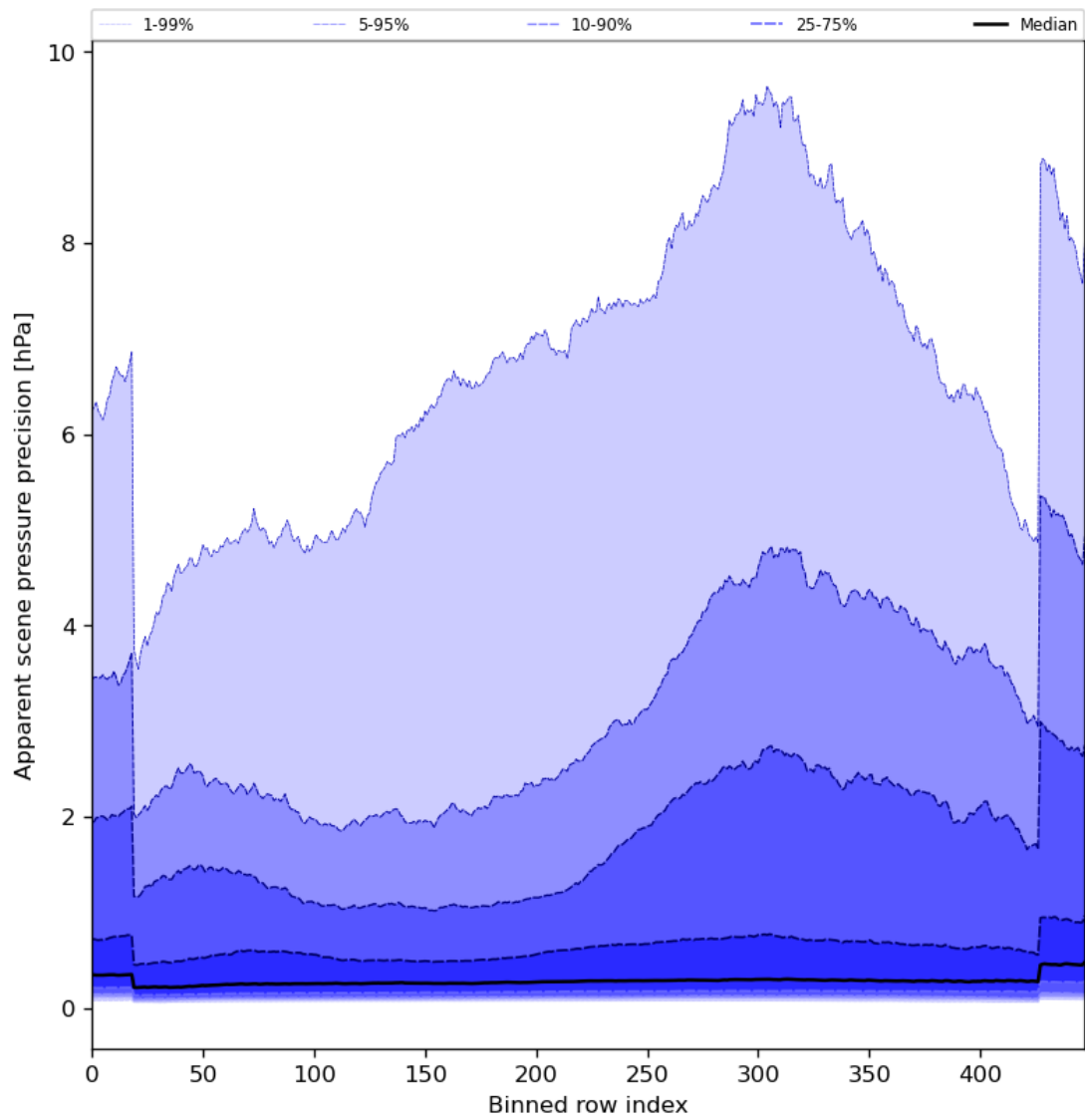
Figure 54: Along track statistics of “Apparent scene pressure precision” for 2024-01-18 to 2024-01-20
