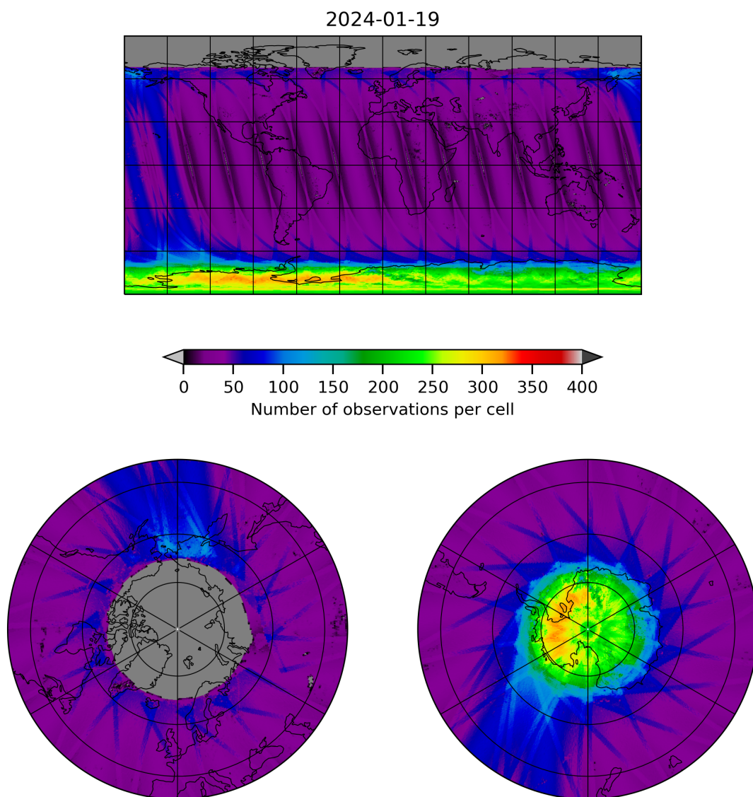
Figure 11: Map of the number of observations for 2024-01-18 to 2024-01-20
