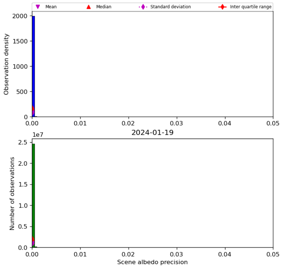
Figure 35: Histogram of “Scene albedo precision” for 2024-01-18 to 2024-01-20
