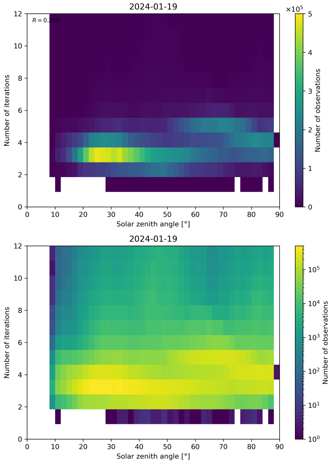
Figure 114: Scatter density plot of “Solar zenith angle” against “Number of iterations” for 2024-01-18 to 2024-01-20.
