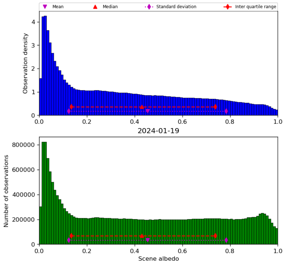
Figure 34: Histogram of “Scene albedo” for 2024-01-18 to 2024-01-20
