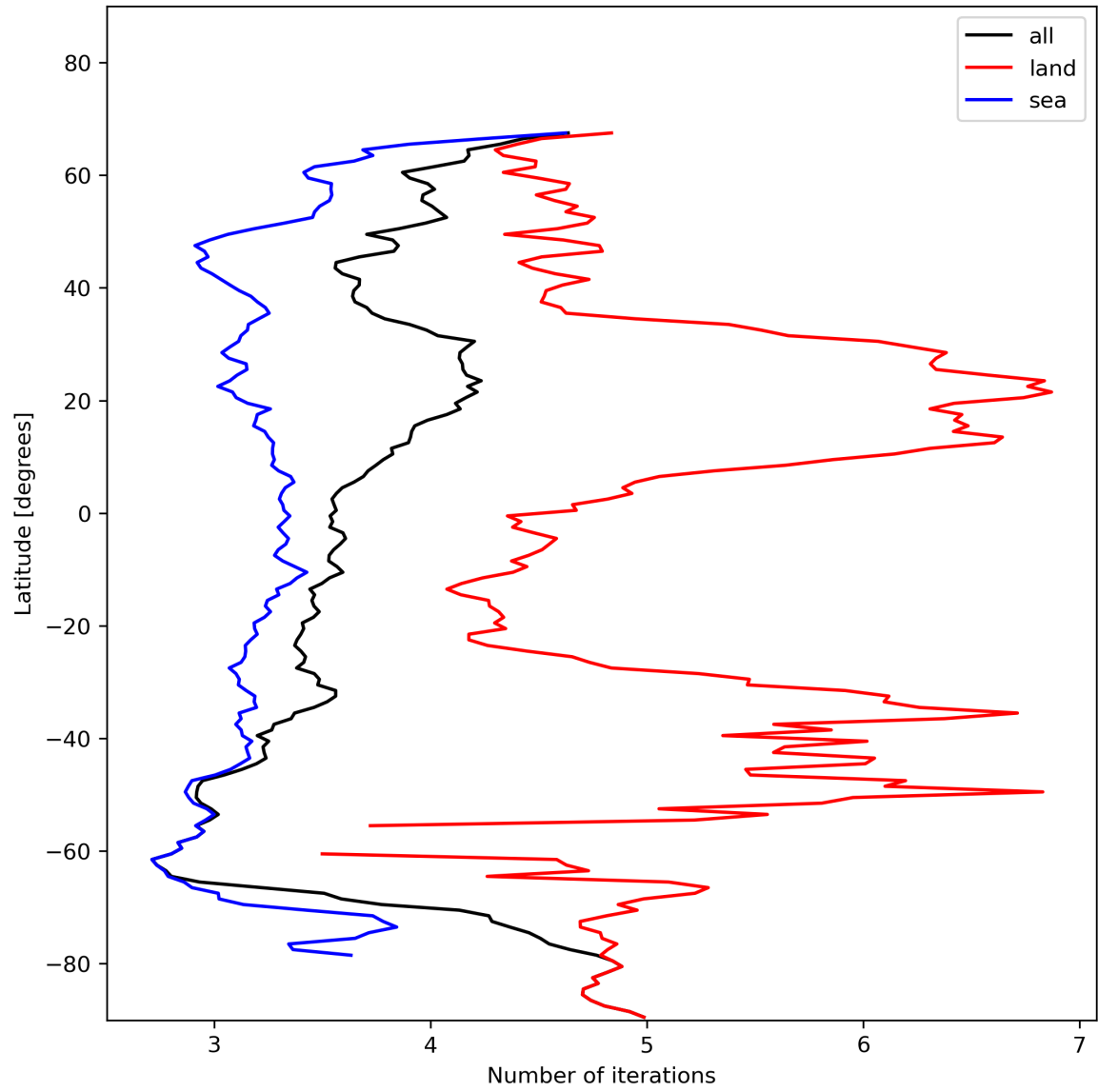
Figure 22: Zonal average of “Number of iterations” for 2024-01-18 to 2024-01-20.
