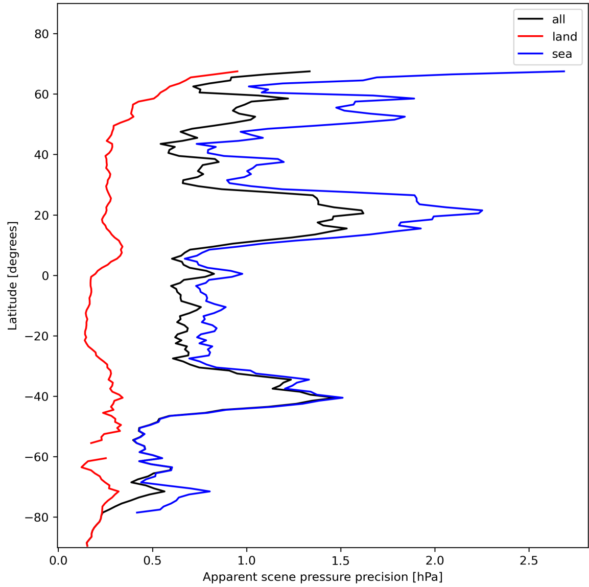
Figure 20: Zonal average of “Apparent scene pressure precision” for 2024-01-18 to 2024-01-20.
