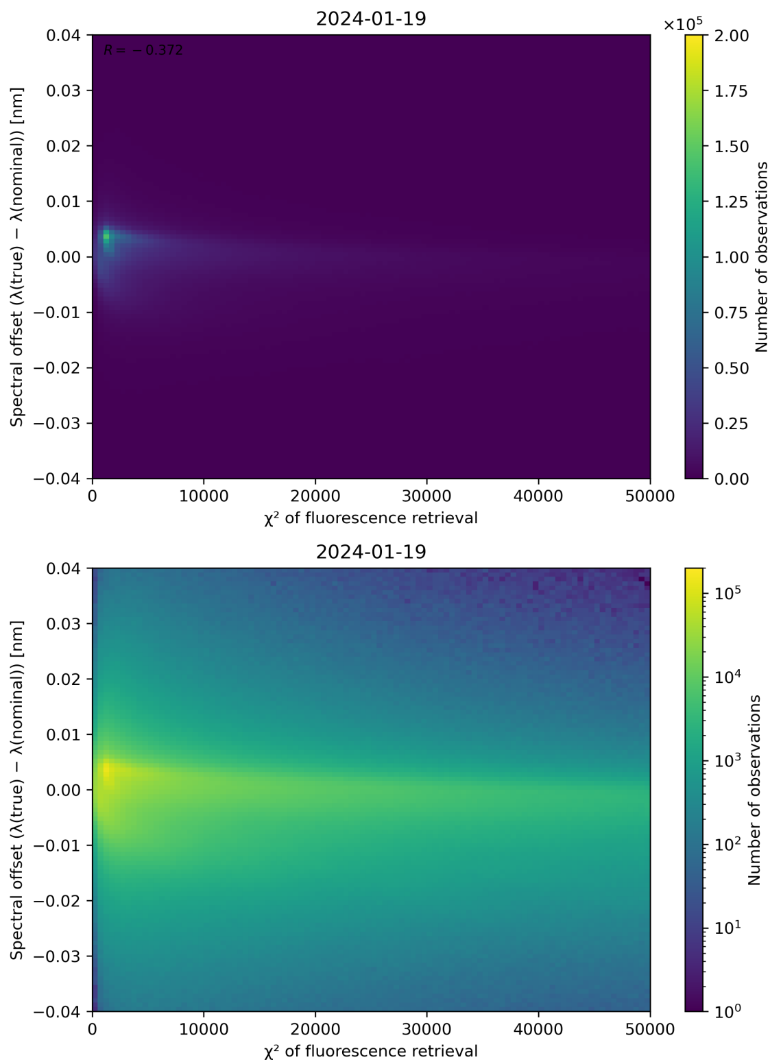
Figure 69: Scatter density plot of " \chi^2 of fluorescence retrieval" against "Spectral offset ( \lambda(\text{true}) - \lambda(\text{nominal}) )" for 2024-01-18 to 2024-01-20.
