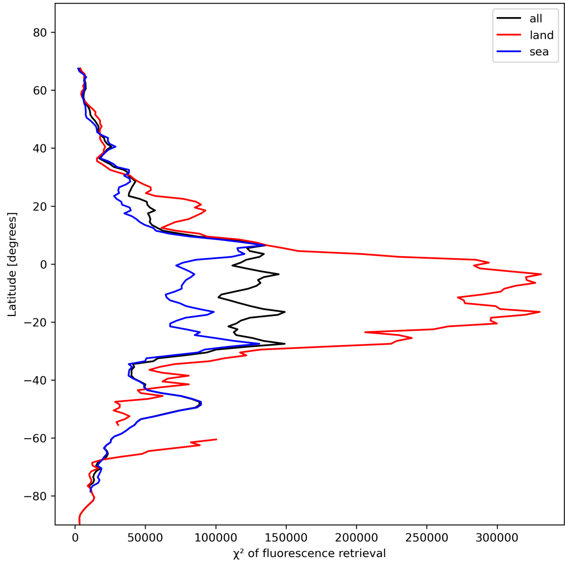
Figure 25: Zonal average of “ \chi^2 of fluorescence retrieval” for 2024-01-18 to 2024-01-20.
