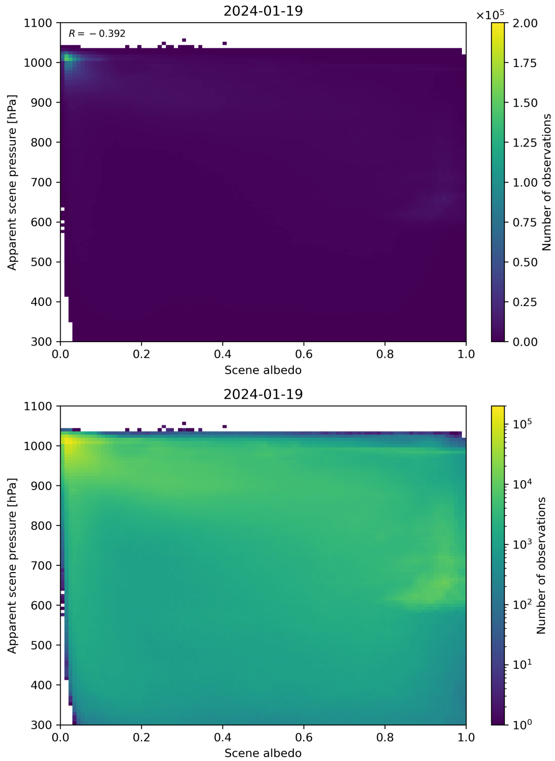
Figure 102: Scatter density plot of “Scene albedo” against “Apparent scene pressure” for 2024-01-18 to 2024-01-20.
