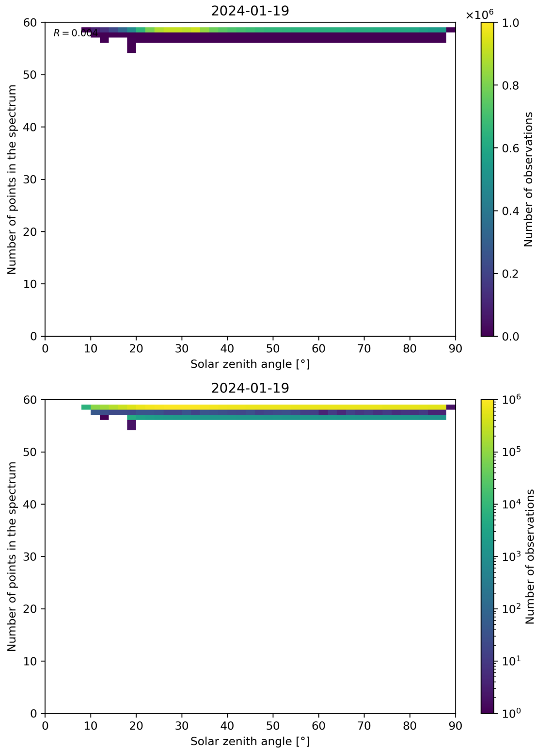
Figure 115: Scatter density plot of “Solar zenith angle” against “Number of points in the spectrum” for 2024-01-18 to 2024-01-20.
