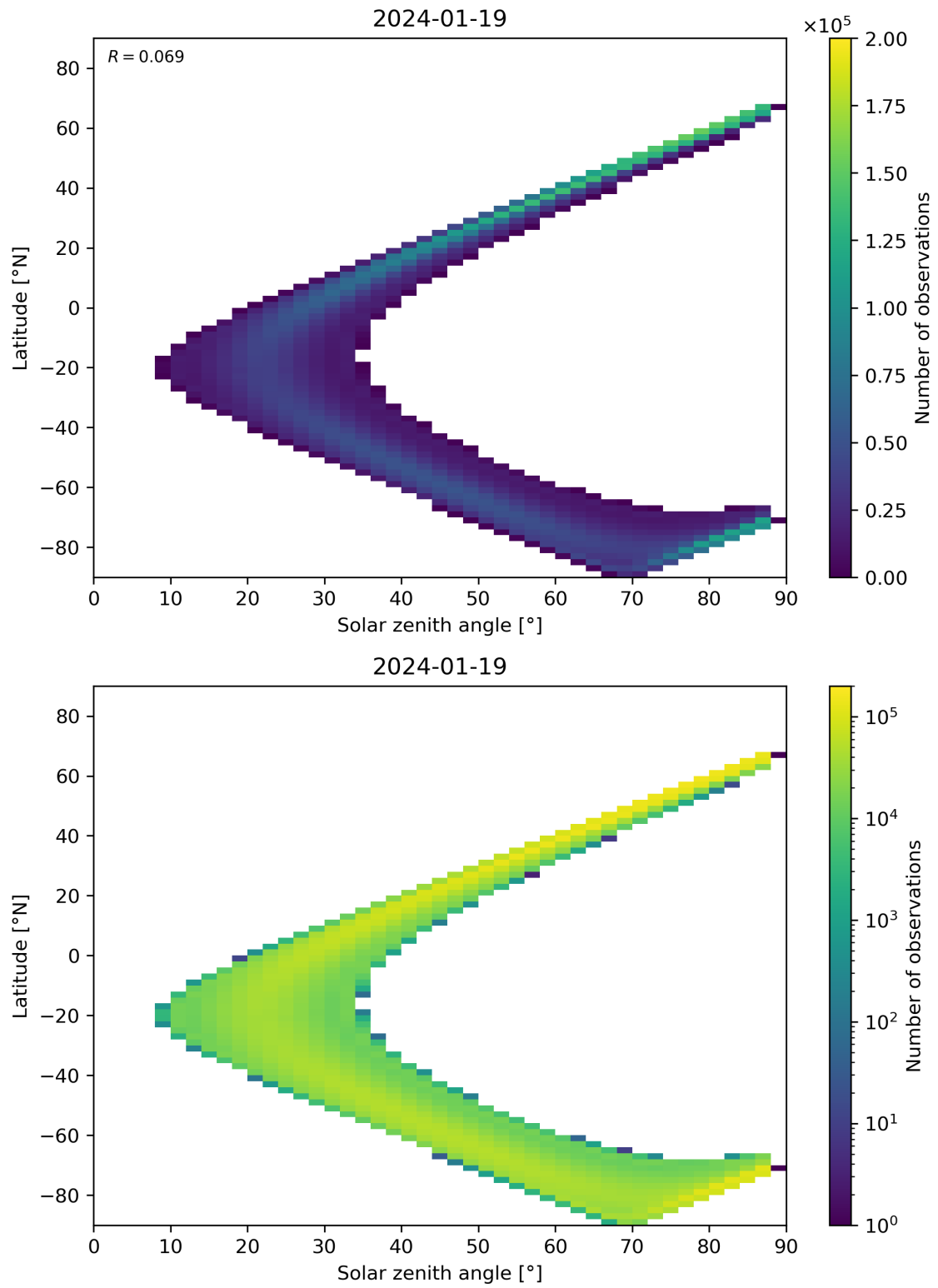
Figure 113: Scatter density plot of “Solar zenith angle” against “Latitude” for 2024-01-18 to 2024-01-20.
