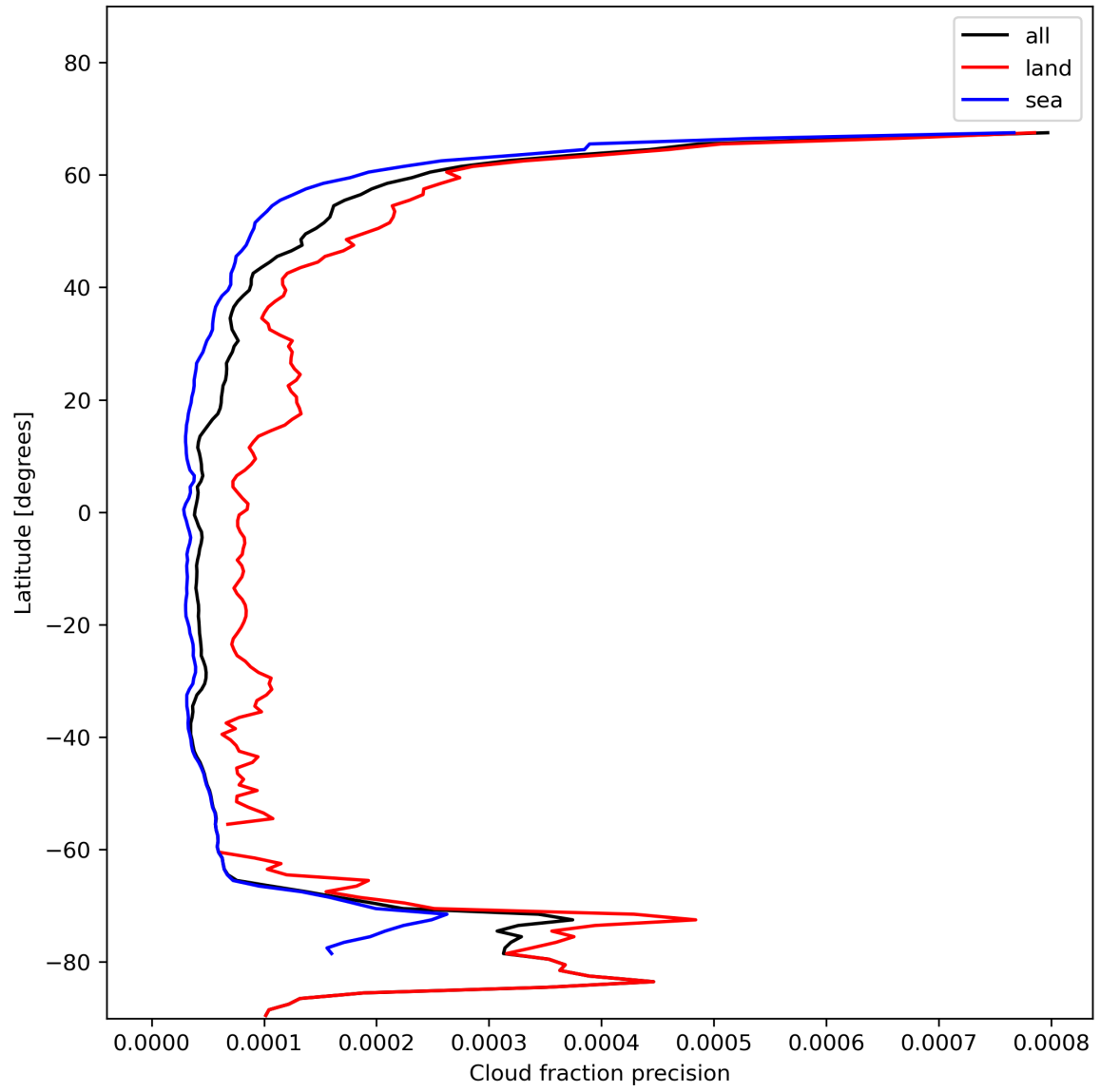
Figure 16: Zonal average of “Cloud fraction precision” for 2024-01-18 to 2024-01-20.
