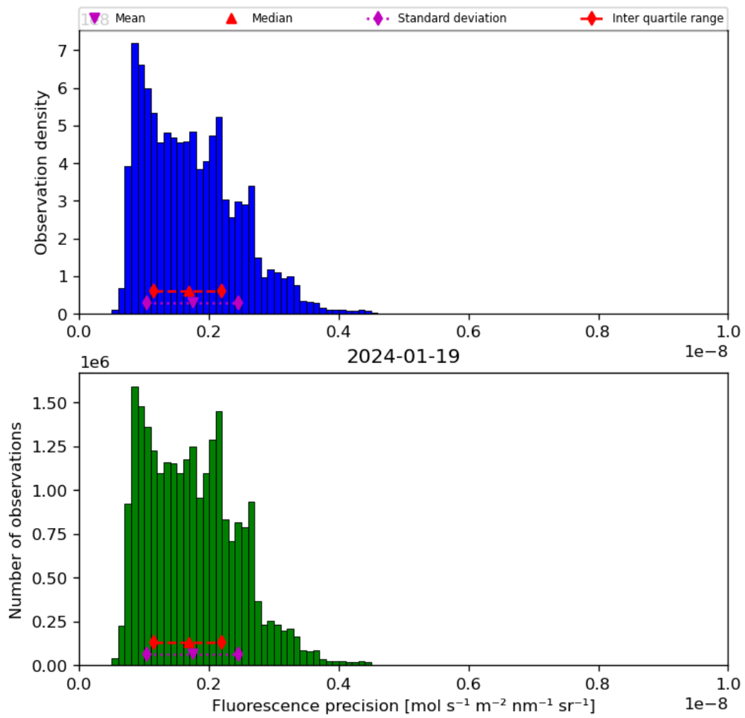
Figure 41: Histogram of “Fluorescence precision” for 2024-01-18 to 2024-01-20
