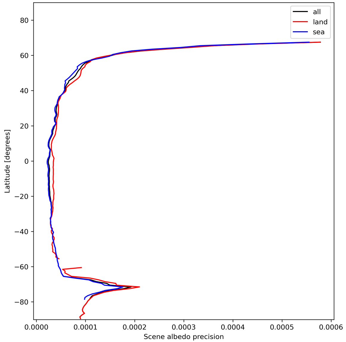
Figure 18: Zonal average of “Scene albedo precision” for 2024-01-18 to 2024-01-20.
