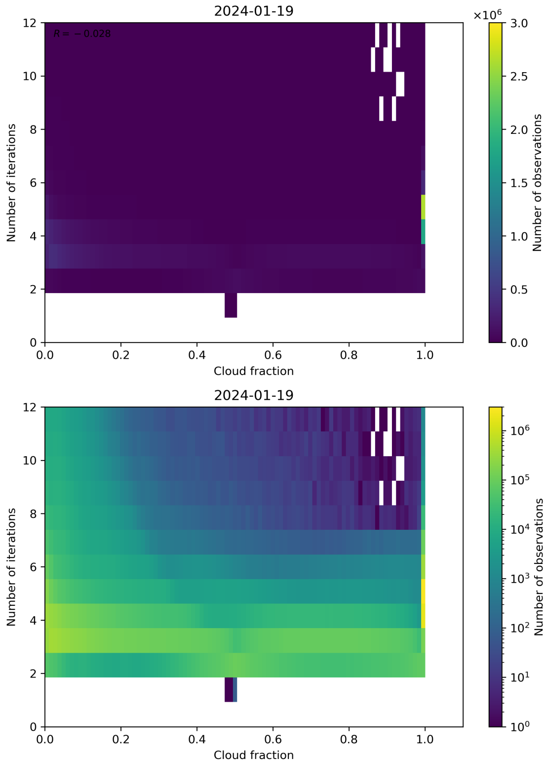
Figure 73: Scatter density plot of “Cloud fraction” against “Number of iterations” for 2024-01-18 to 2024-01-20.
