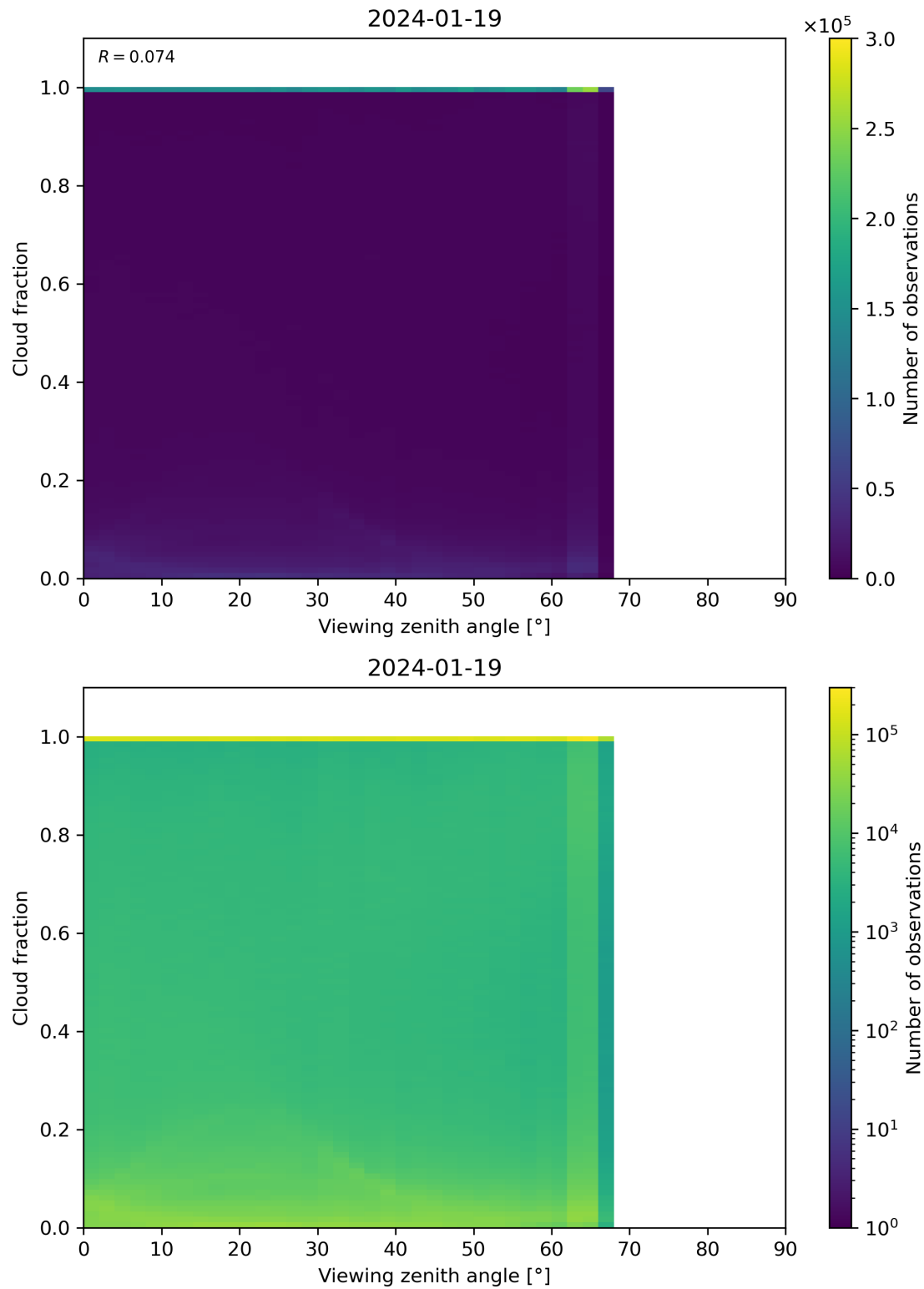
Figure 120: Scatter density plot of “Viewing zenith angle” against “Cloud fraction” for 2024-01-18 to 2024-01-20.
