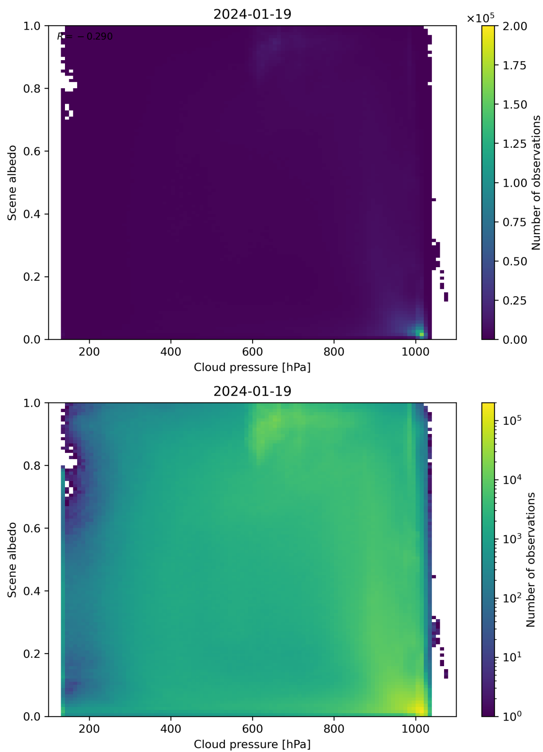
Figure 83: Scatter density plot of “Cloud pressure” against “Scene albedo” for 2024-01-18 to 2024-01-20.
