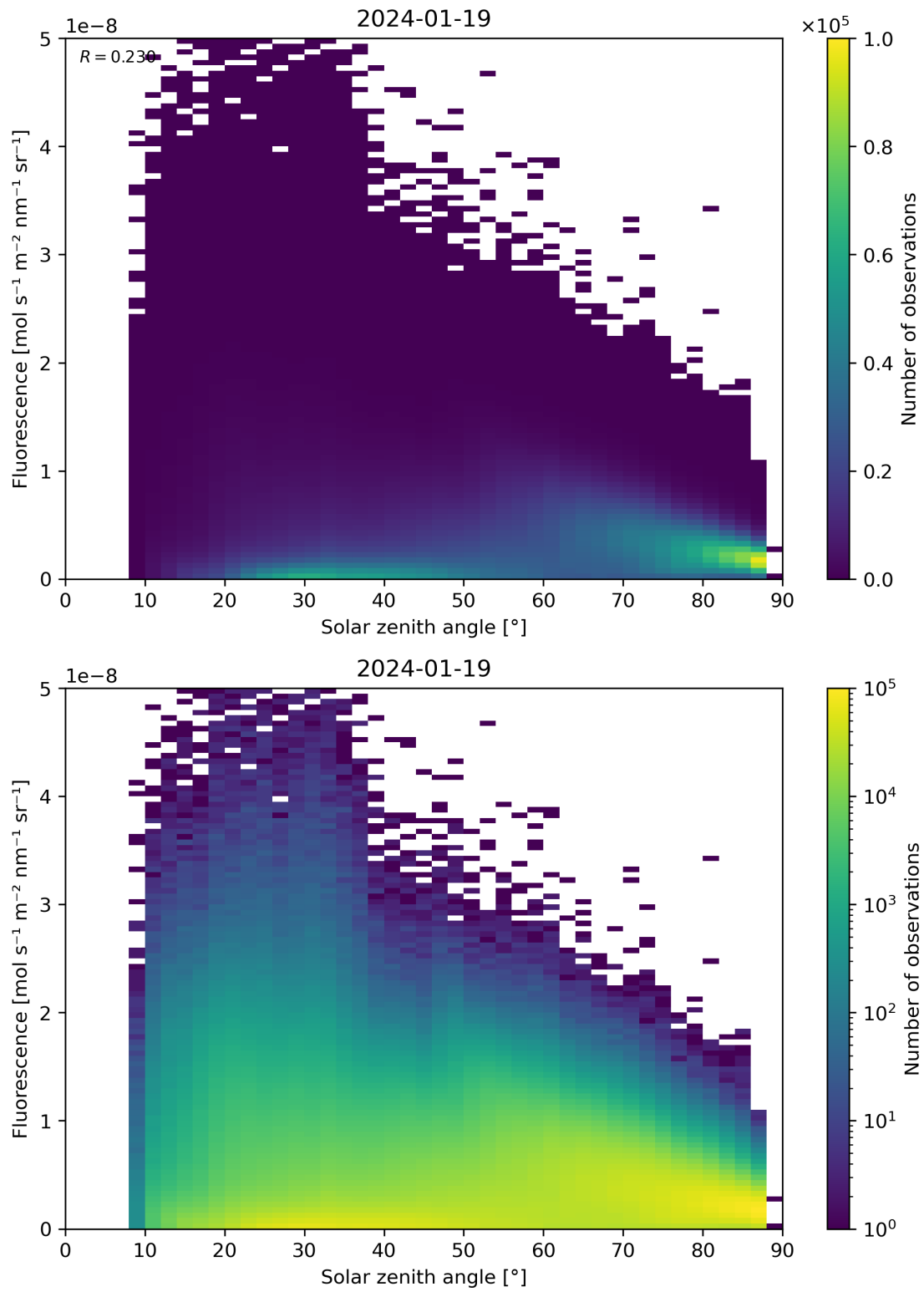
Figure 112: Scatter density plot of “Solar zenith angle” against “Fluorescence” for 2024-01-18 to 2024-01-20.
