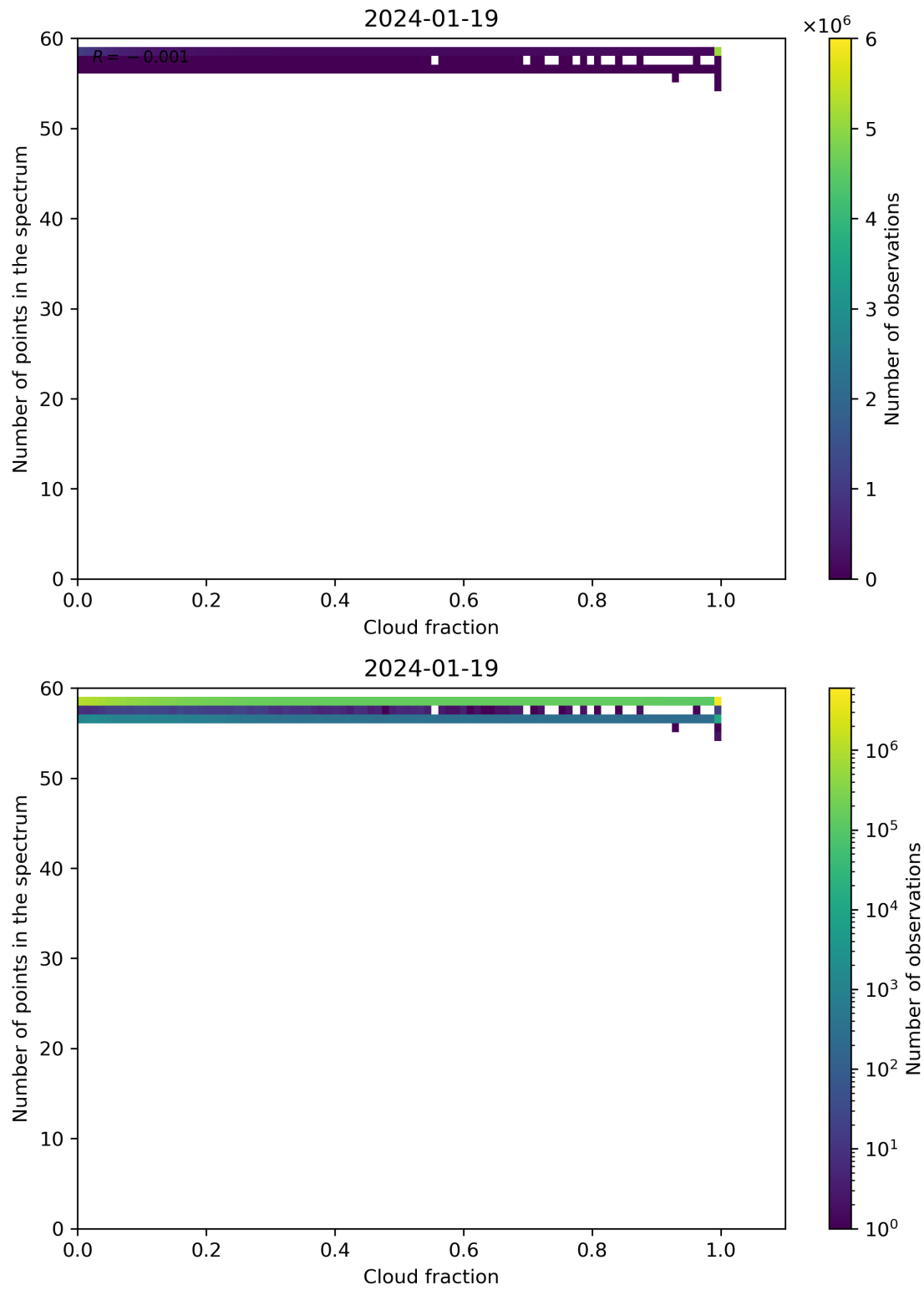
Figure 74: Scatter density plot of “Cloud fraction” against “Number of points in the spectrum” for 2024-01-18 to 2024-01-20.
