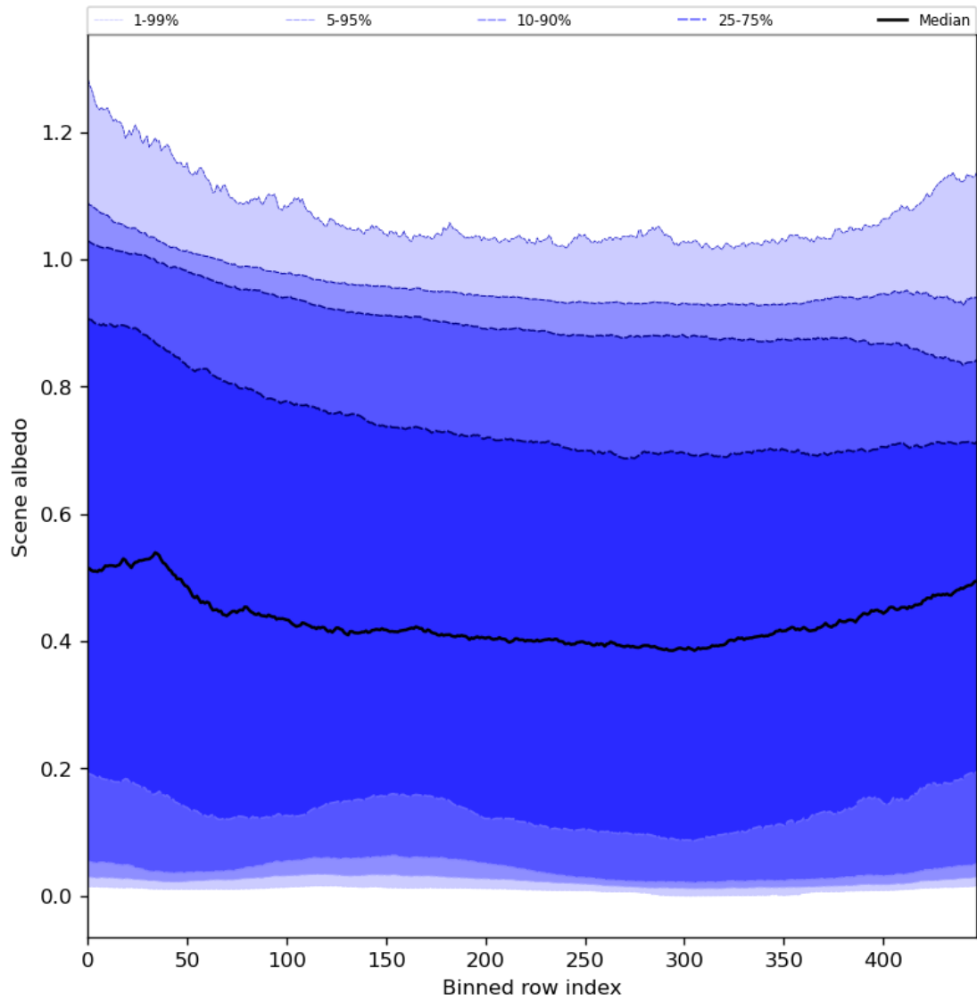
Figure 51: Along track statistics of “Scene albedo” for 2024-01-18 to 2024-01-20
