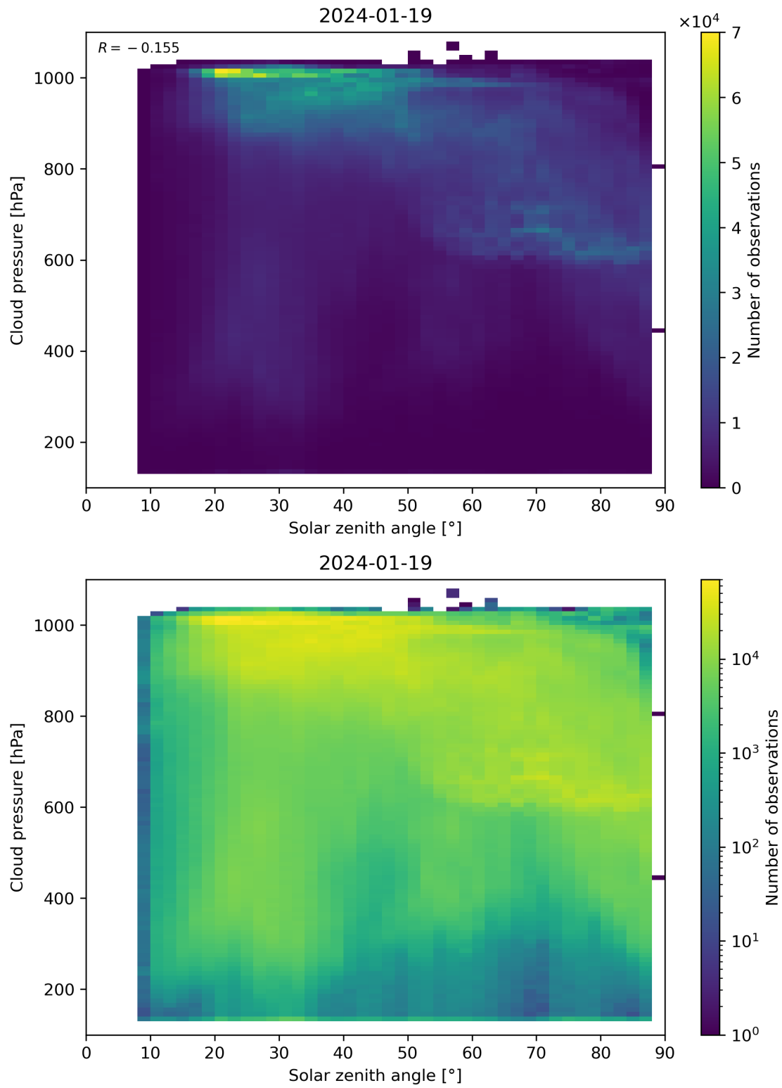
Figure 111: Scatter density plot of “Solar zenith angle” against “Cloud pressure” for 2024-01-18 to 2024-01-20.
