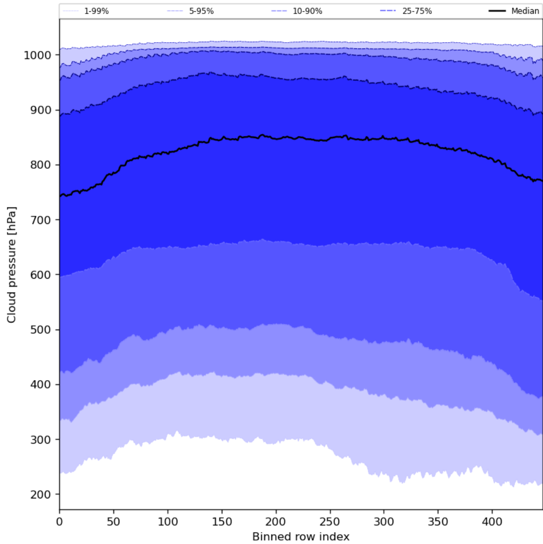
Figure 47: Along track statistics of “Cloud pressure” for 2024-01-18 to 2024-01-20
