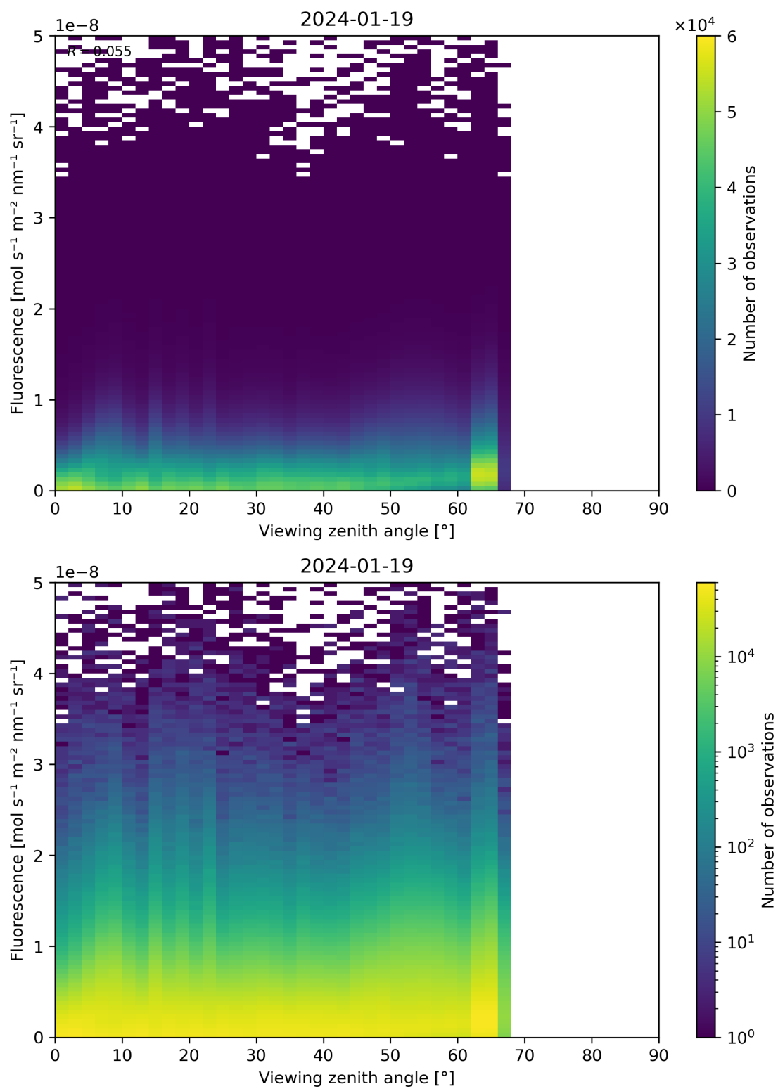
Figure 122: Scatter density plot of “Viewing zenith angle” against “Fluorescence” for 2024-01-18 to 2024-01-20.
