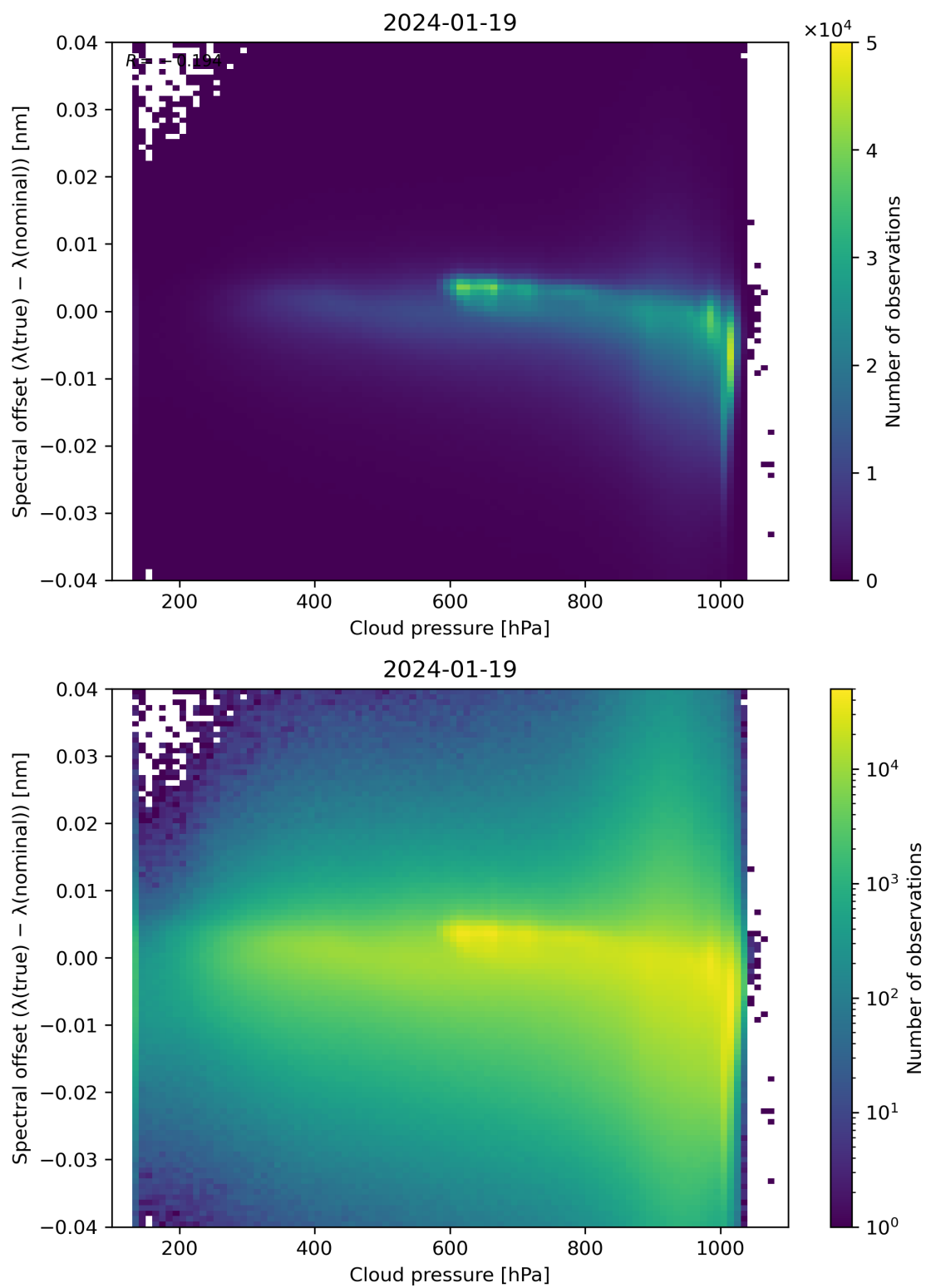
Figure 84: Scatter density plot of “Cloud pressure” against “Spectral offset ( \lambda(\text{true}) - \lambda(\text{nominal}) )” for 2024-01-18 to 2024-01-20.
