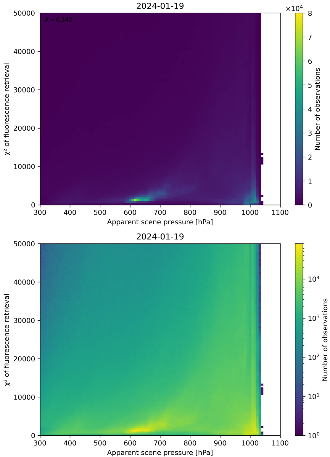
Figure 63: Scatter density plot of “Apparent scene pressure” against “ \chi^2 of fluorescence retrieval” for 2024-01-18 to 2024-01-20.
