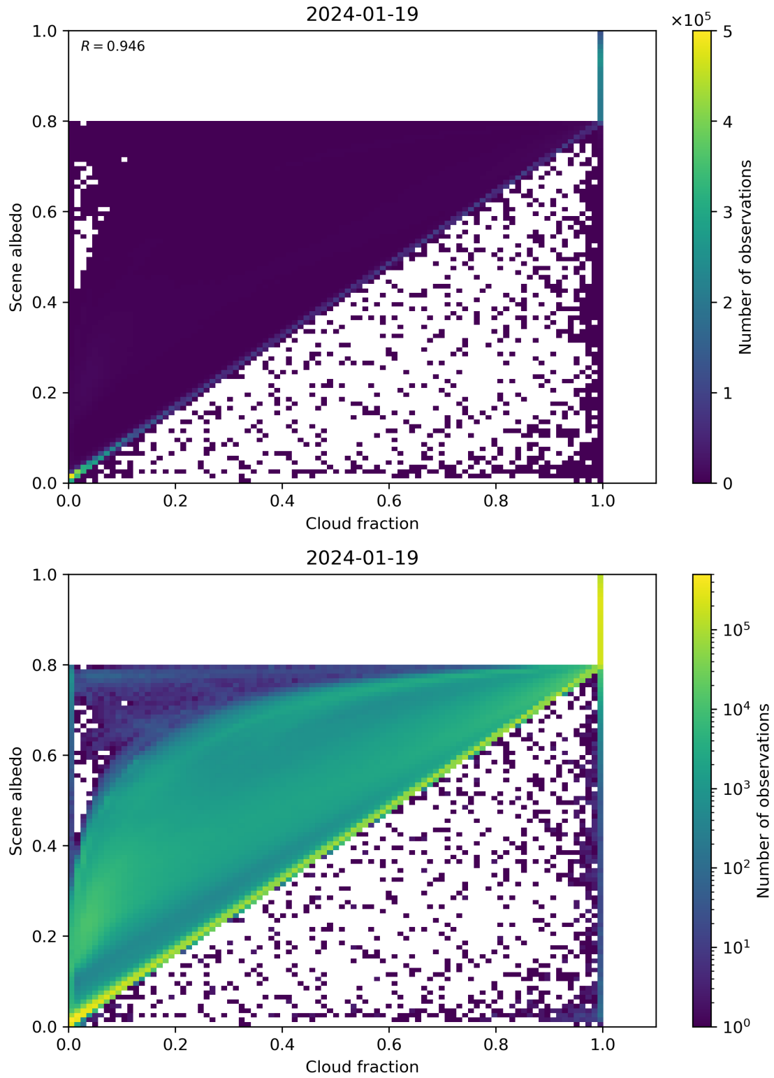
Figure 75: Scatter density plot of “Cloud fraction” against “Scene albedo” for 2024-01-18 to 2024-01-20.
