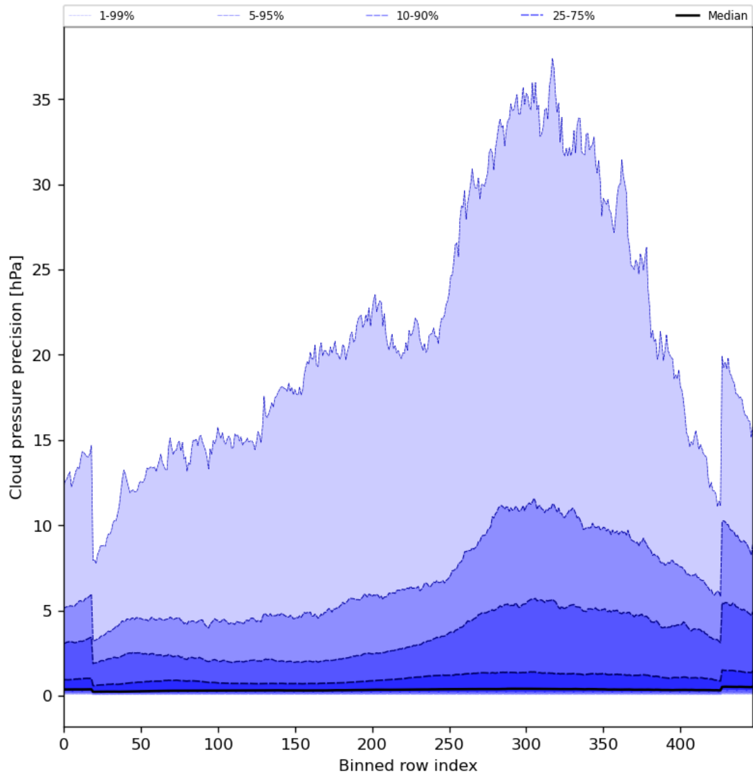
Figure 48: Along track statistics of “Cloud pressure precision” for 2024-01-18 to 2024-01-20
