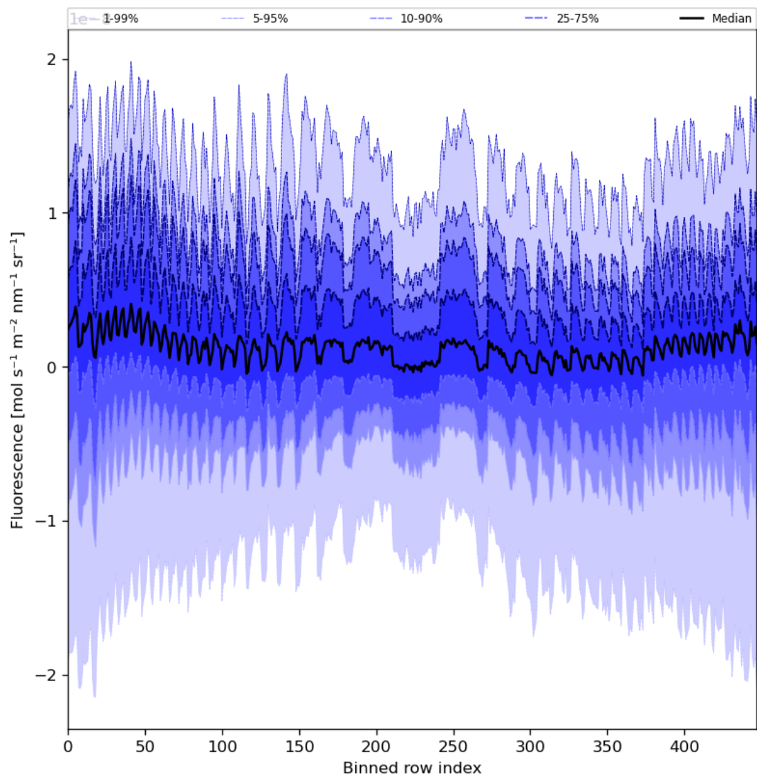
Figure 57: Along track statistics of “Fluorescence” for 2024-01-18 to 2024-01-20
