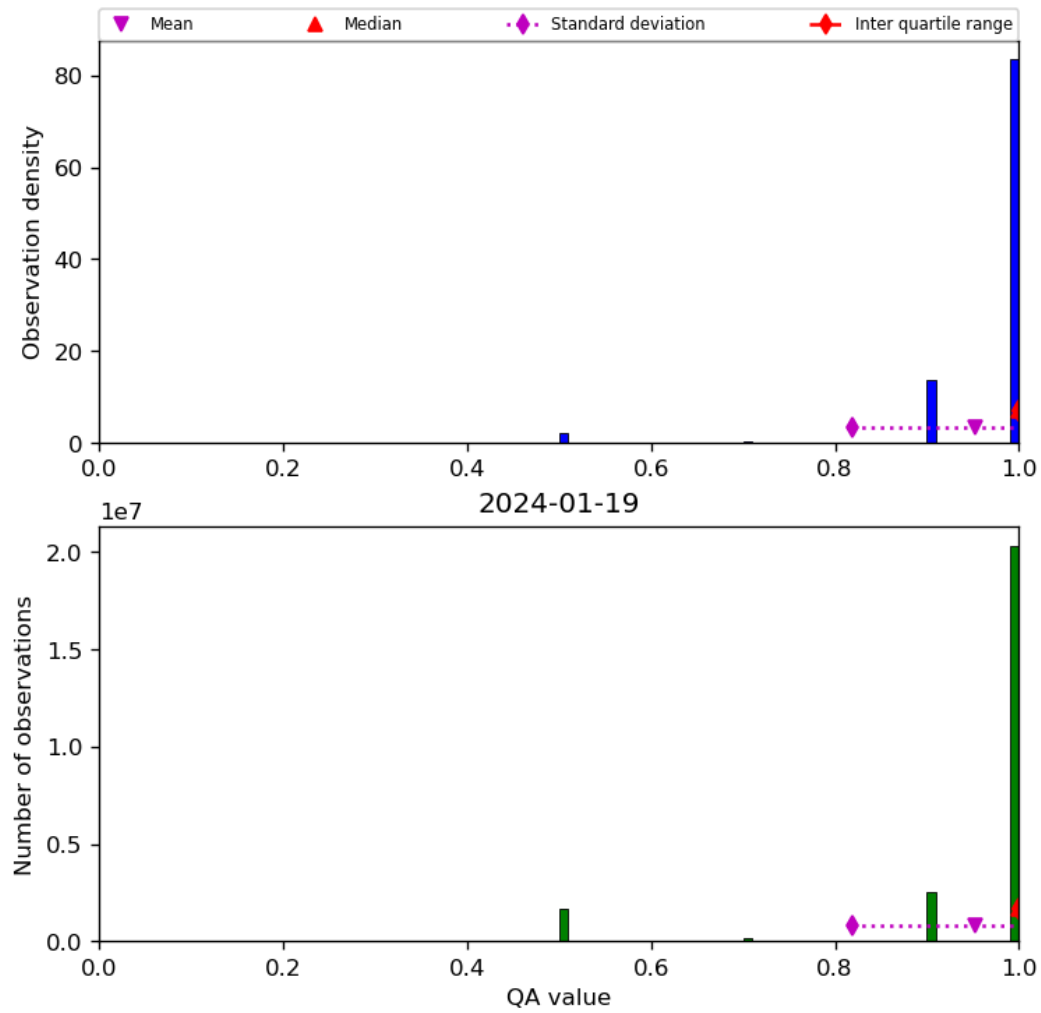
Figure 29: Histogram of “QA value” for 2024-01-18 to 2024-01-20
