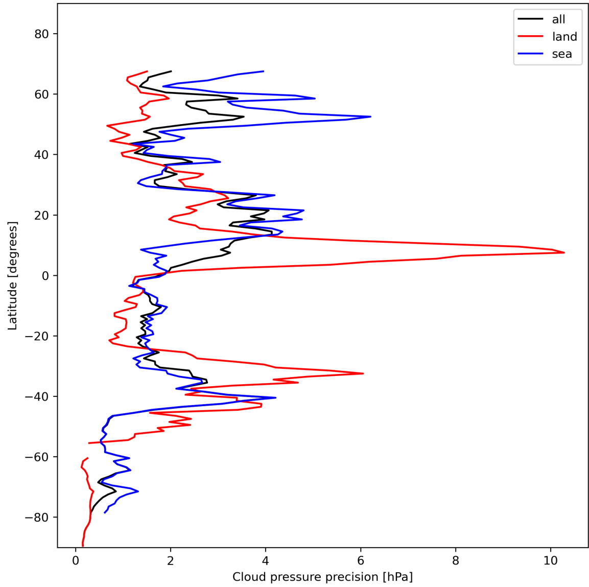
Figure 14: Zonal average of “Cloud pressure precision” for 2024-01-18 to 2024-01-20.
