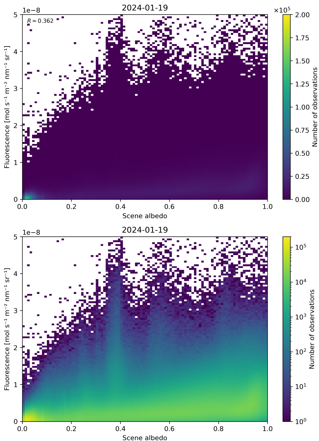
Figure 104: Scatter density plot of “Scene albedo” against “Fluorescence” for 2024-01-18 to 2024-01-20.
