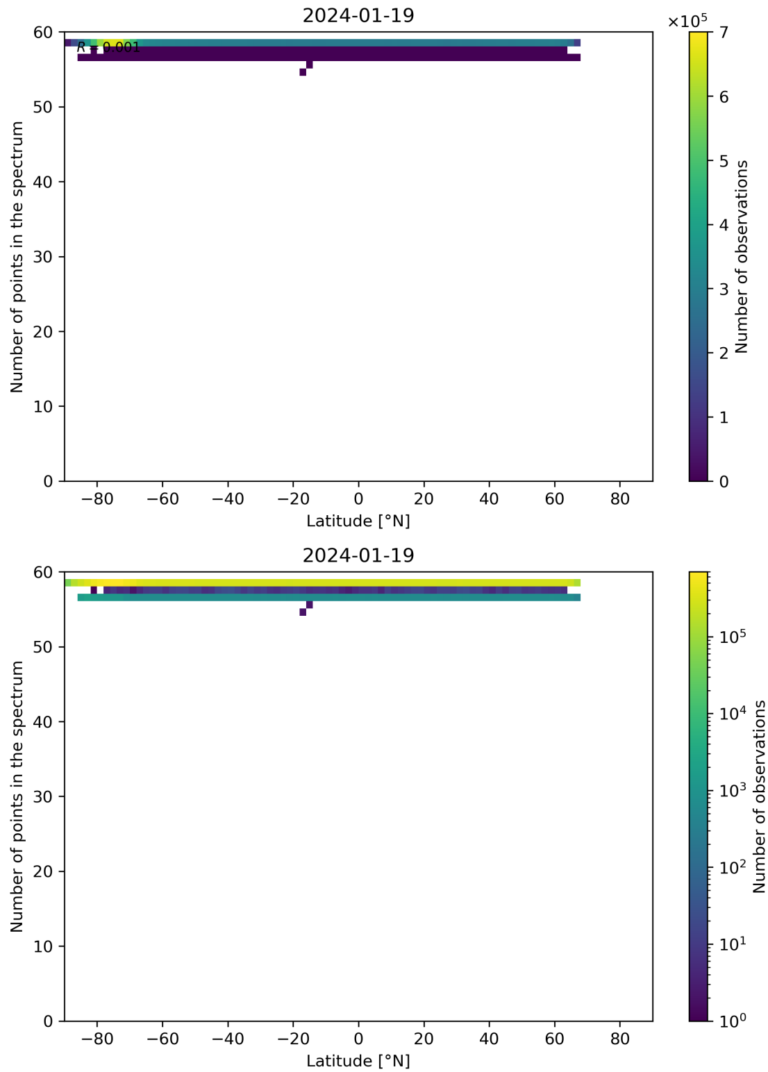
Figure 94: Scatter density plot of “Latitude” against “Number of points in the spectrum” for 2024-01-18 to 2024-01-20.
