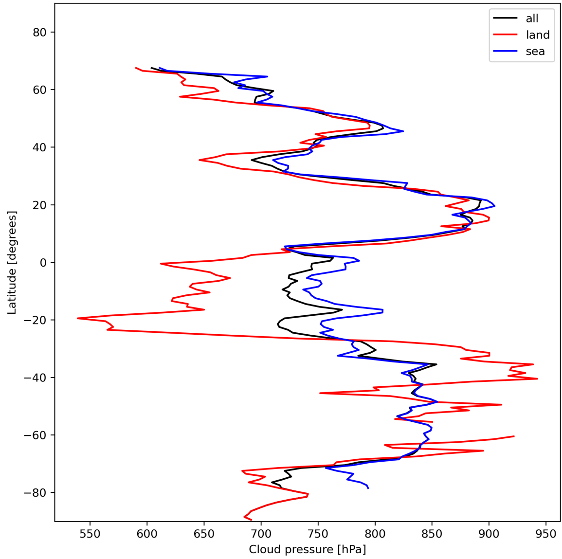
Figure 13: Zonal average of “Cloud pressure” for 2024-01-18 to 2024-01-20.
