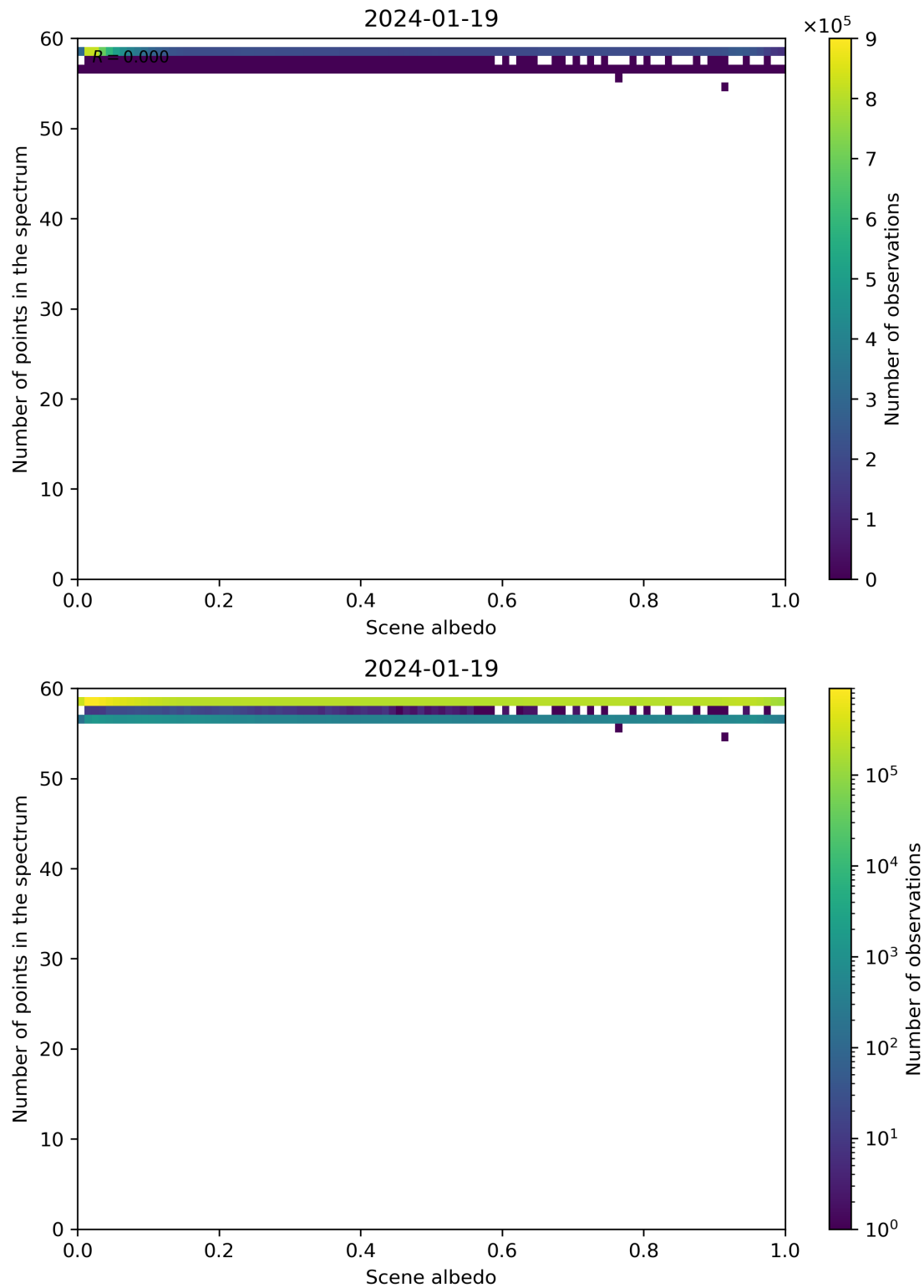
Figure 106: Scatter density plot of “Scene albedo” against “Number of points in the spectrum” for 2024-01-18 to 2024-01-20.
