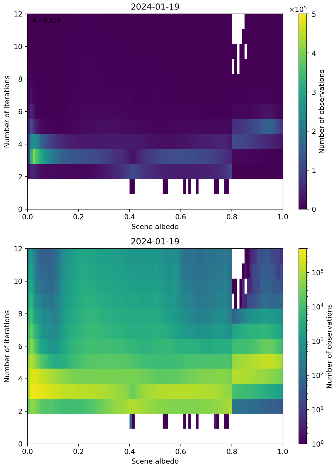
Figure 105: Scatter density plot of “Scene albedo” against “Number of iterations” for 2024-01-18 to 2024-01-20.
