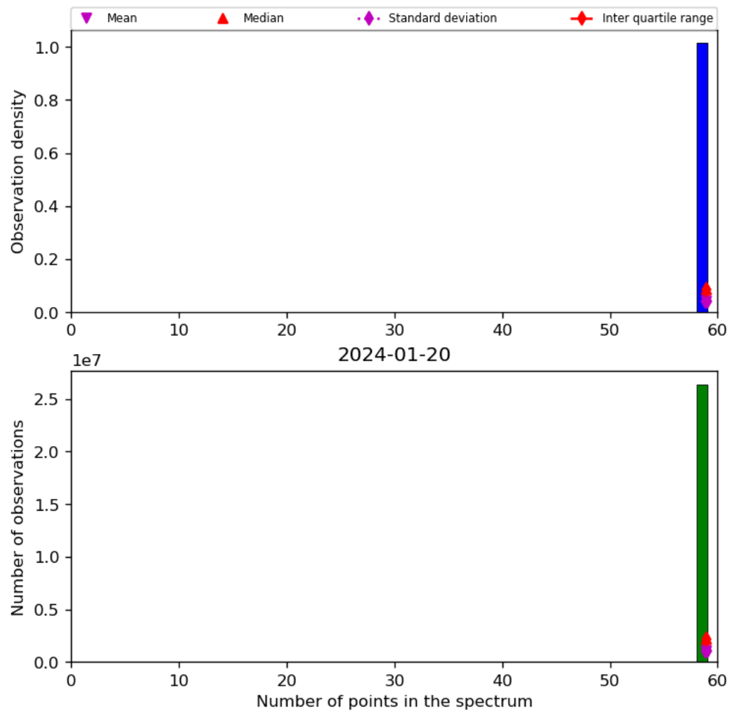
Figure 44: Histogram of “Number of points in the spectrum” for 2024-01-19 to 2024-01-21
