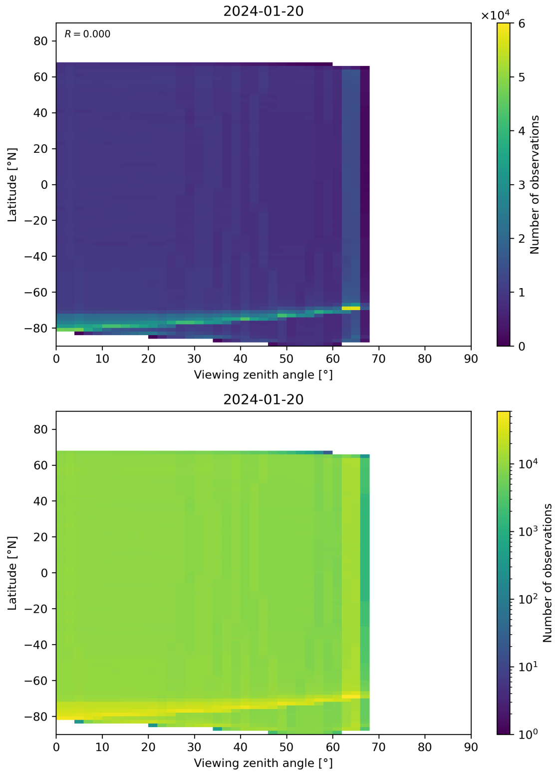
Figure 123: Scatter density plot of “Viewing zenith angle” against “Latitude” for 2024-01-19 to 2024-01-21.
