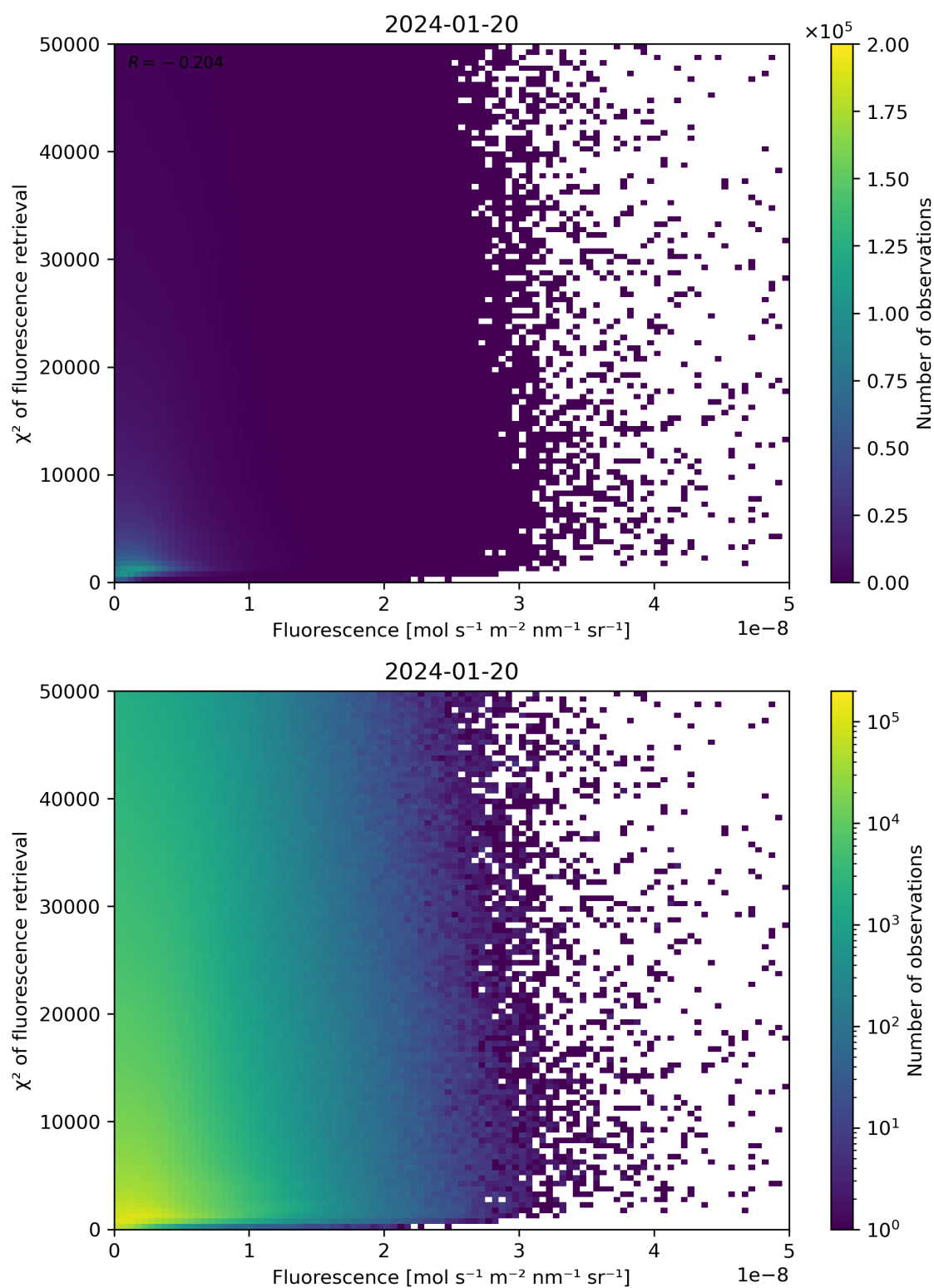
Figure 85: Scatter density plot of “Fluorescence” against “ \chi^2 of fluorescence retrieval” for 2024-01-19 to 2024-01-21.
