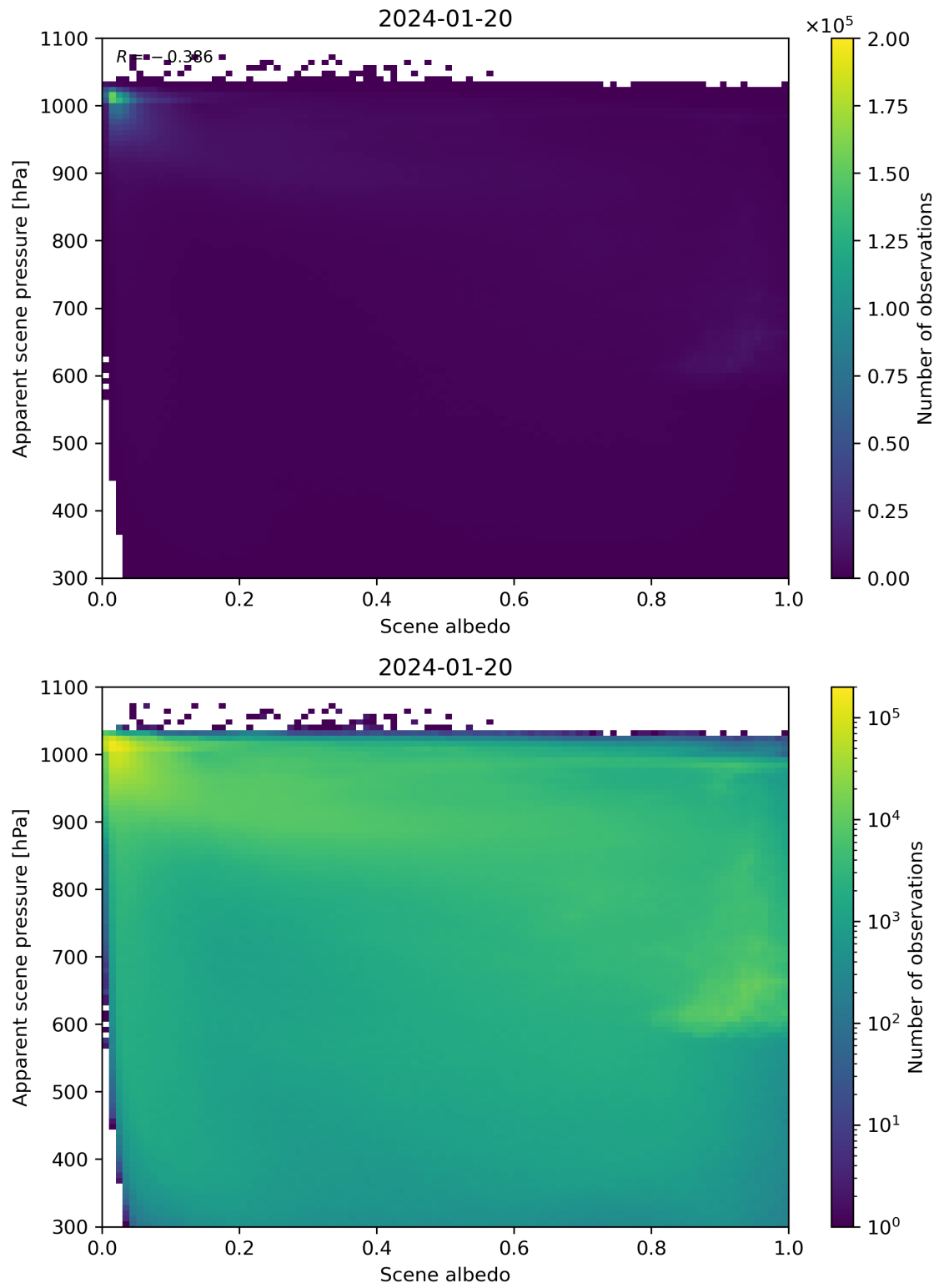
Figure 102: Scatter density plot of “Scene albedo” against “Apparent scene pressure” for 2024-01-19 to 2024-01-21.
