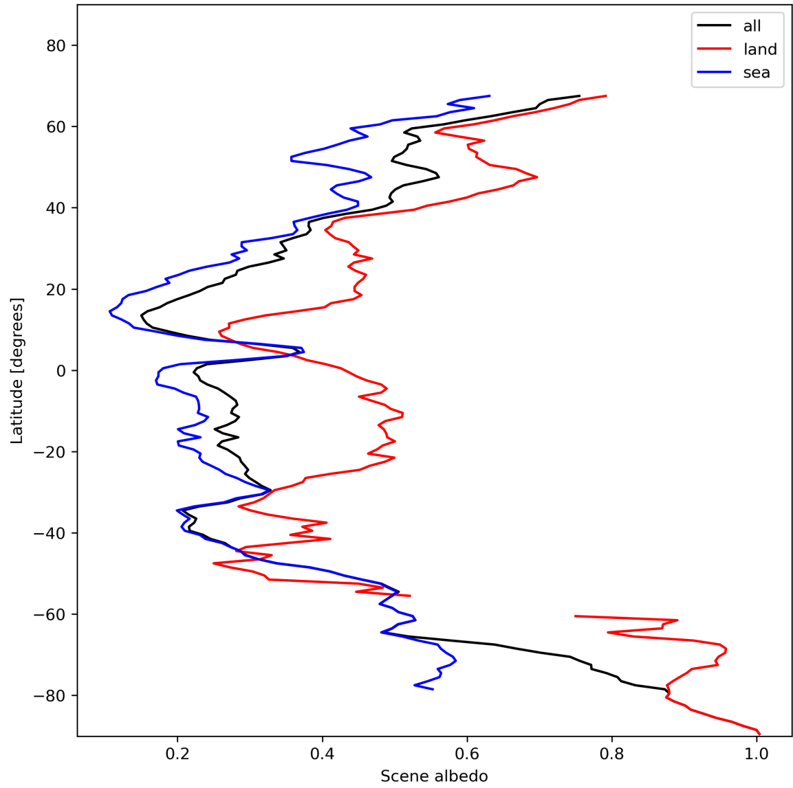
Figure 17: Zonal average of “Scene albedo” for 2024-01-19 to 2024-01-21.
