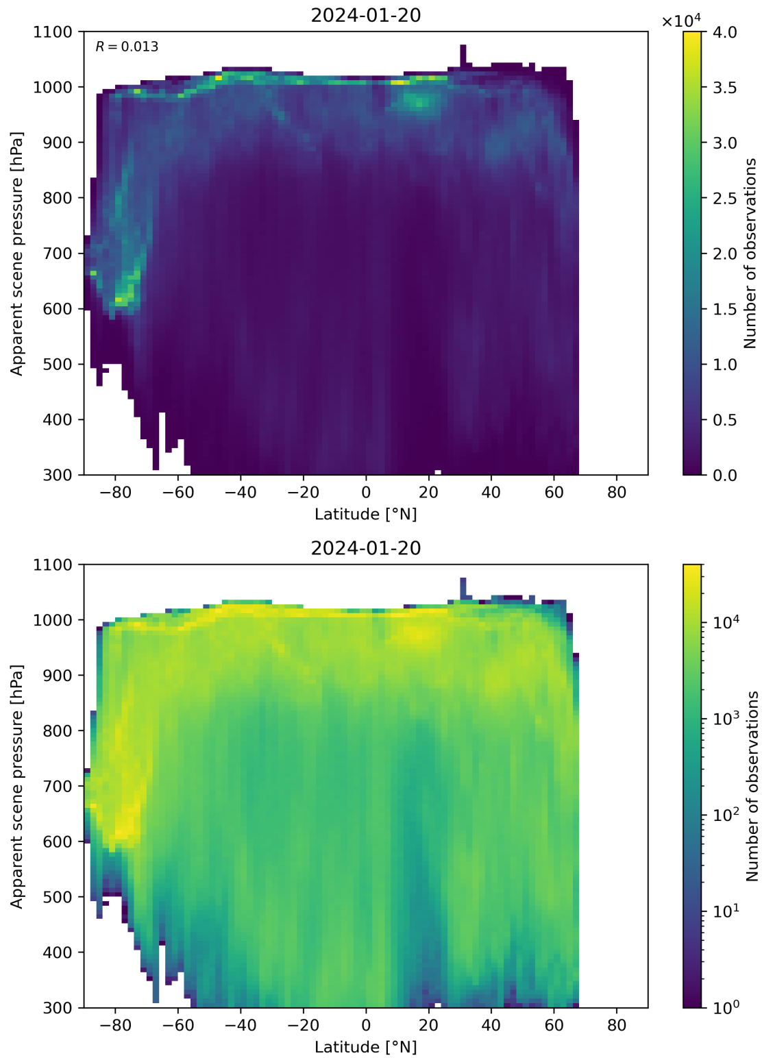
Figure 88: Scatter density plot of “Latitude” against “Apparent scene pressure” for 2024-01-19 to 2024-01-21.
