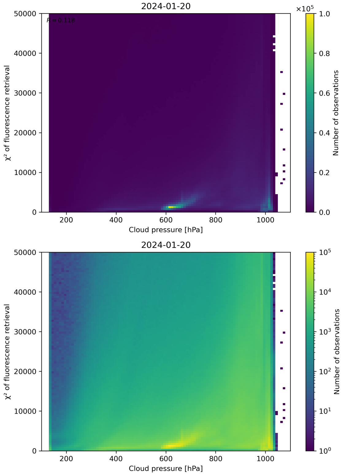
Figure 78: Scatter density plot of “Cloud pressure” against “ \chi^2 of fluorescence retrieval” for 2024-01-19 to 2024-01-21.
