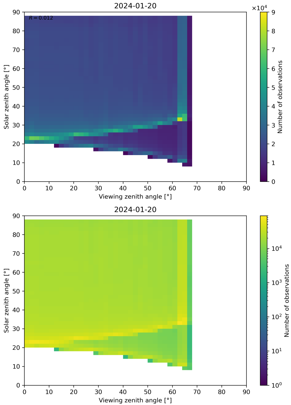
Figure 127: Scatter density plot of “Viewing zenith angle” against “Solar zenith angle” for 2024-01-19 to 2024-01-21.
