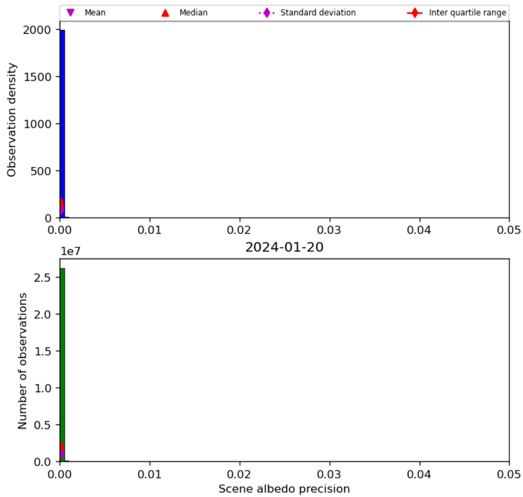
Figure 35: Histogram of “Scene albedo precision” for 2024-01-19 to 2024-01-21
