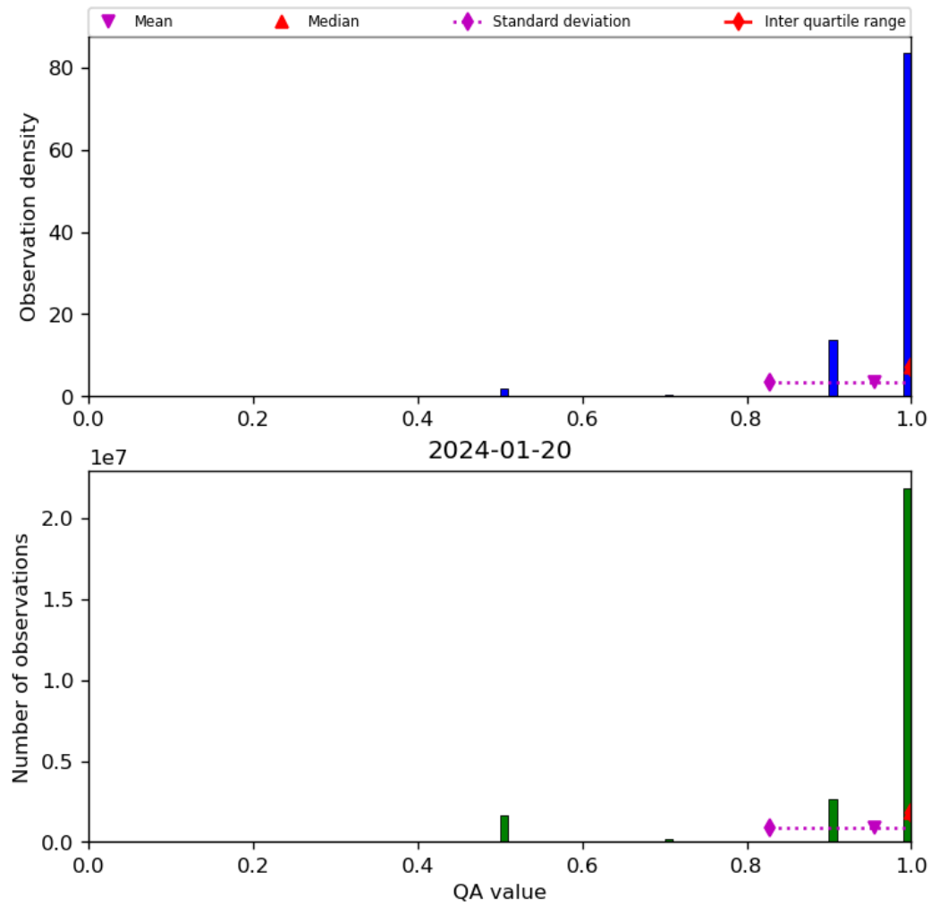
Figure 29: Histogram of “QA value” for 2024-01-19 to 2024-01-21
