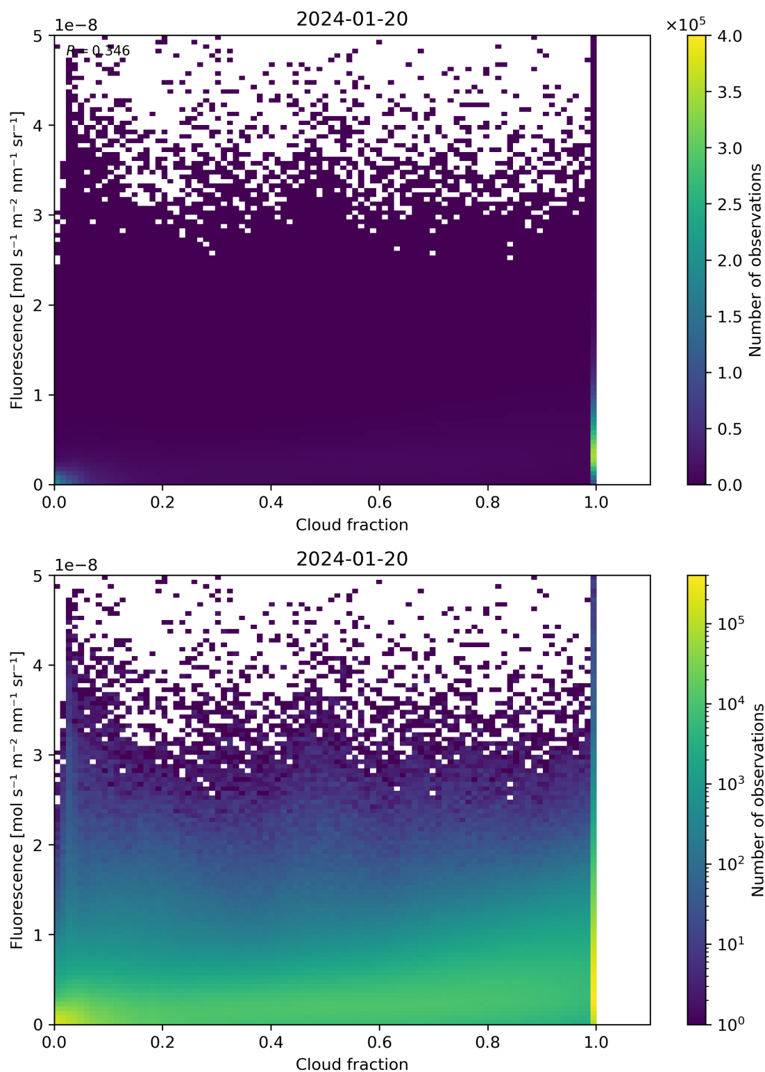
Figure 72: Scatter density plot of “Cloud fraction” against “Fluorescence” for 2024-01-19 to 2024-01-21.
