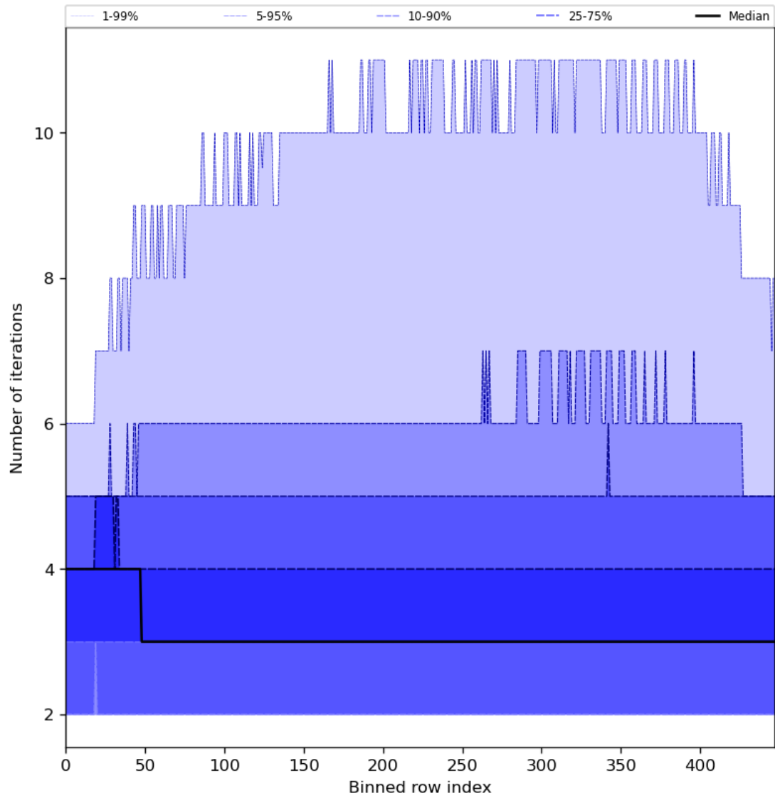
Figure 56: Along track statistics of “Number of iterations” for 2024-01-19 to 2024-01-21
