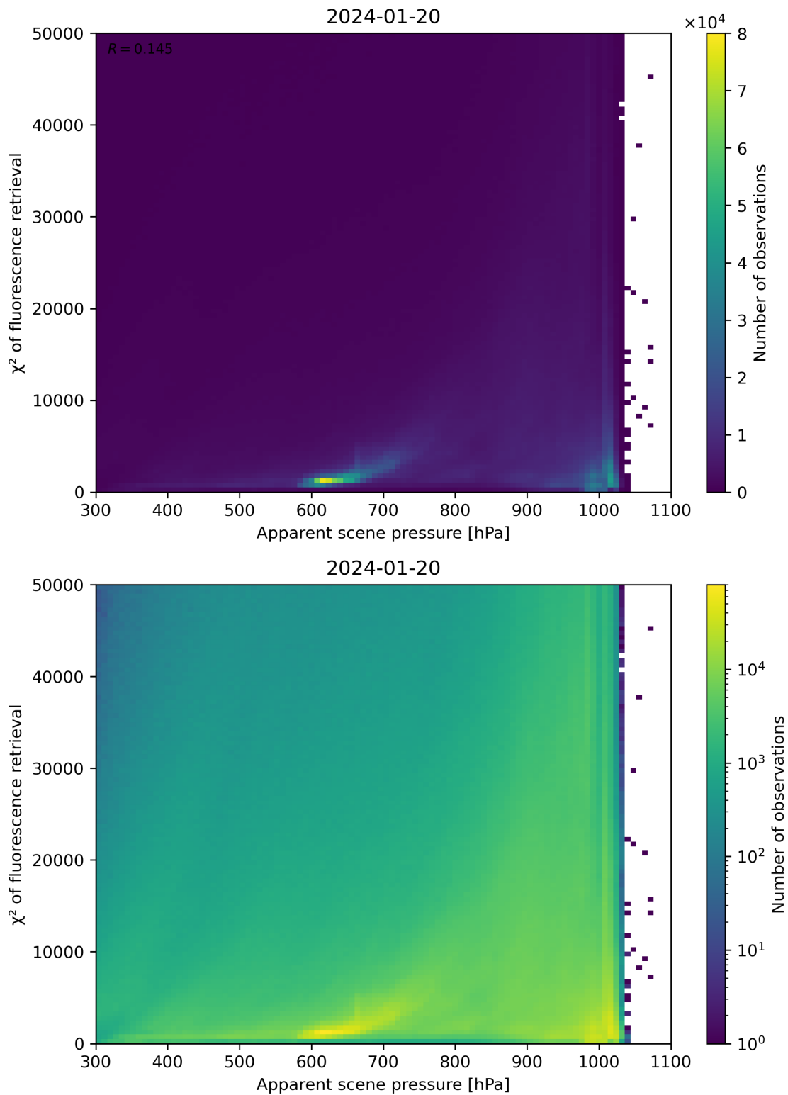
Figure 63: Scatter density plot of “Apparent scene pressure” against “ \chi^2 of fluorescence retrieval” for 2024-01-19 to 2024-01-21.
