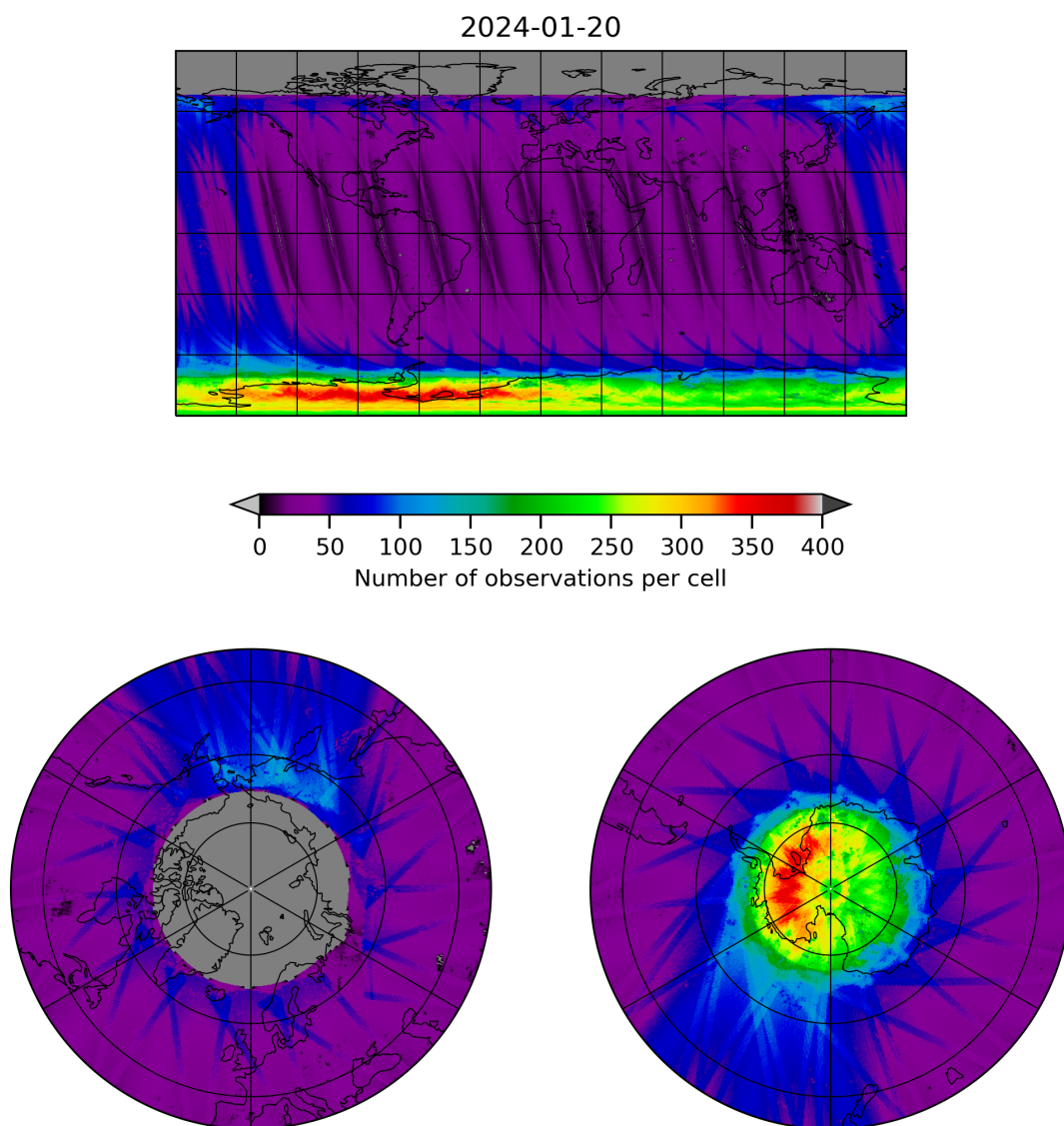
Figure 11: Map of the number of observations for 2024-01-19 to 2024-01-21
