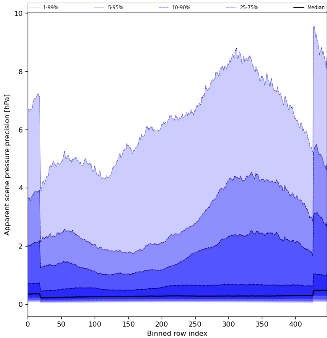
Figure 54: Along track statistics of “Apparent scene pressure precision” for 2024-01-19 to 2024-01-21
