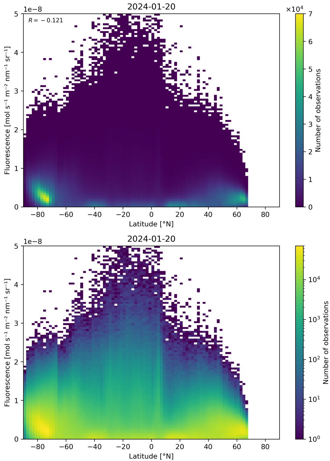
Figure 92: Scatter density plot of “Latitude” against “Fluorescence” for 2024-01-19 to 2024-01-21.
