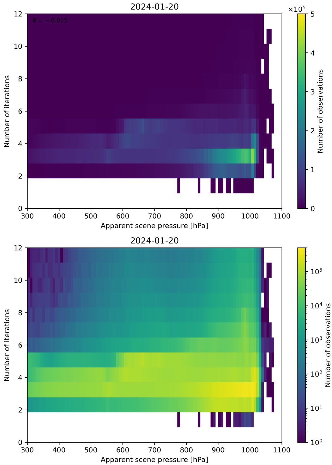
Figure 65: Scatter density plot of “Apparent scene pressure” against “Number of iterations” for 2024-01-19 to 2024-01-21.
