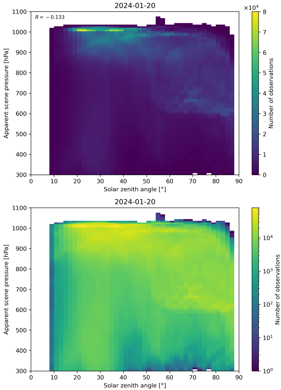
Figure 108: Scatter density plot of “Solar zenith angle” against “Apparent scene pressure” for 2024-01-19 to 2024-01-21.
