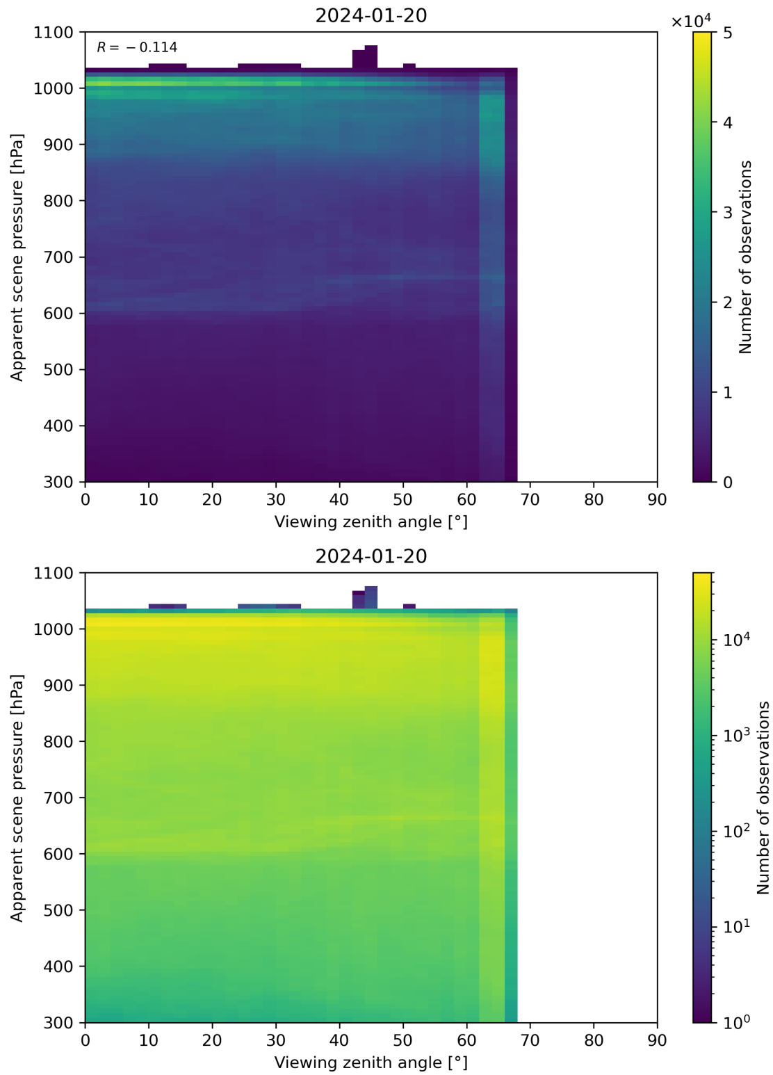
Figure 118: Scatter density plot of “Viewing zenith angle” against “Apparent scene pressure” for 2024-01-19 to 2024-01-21.
