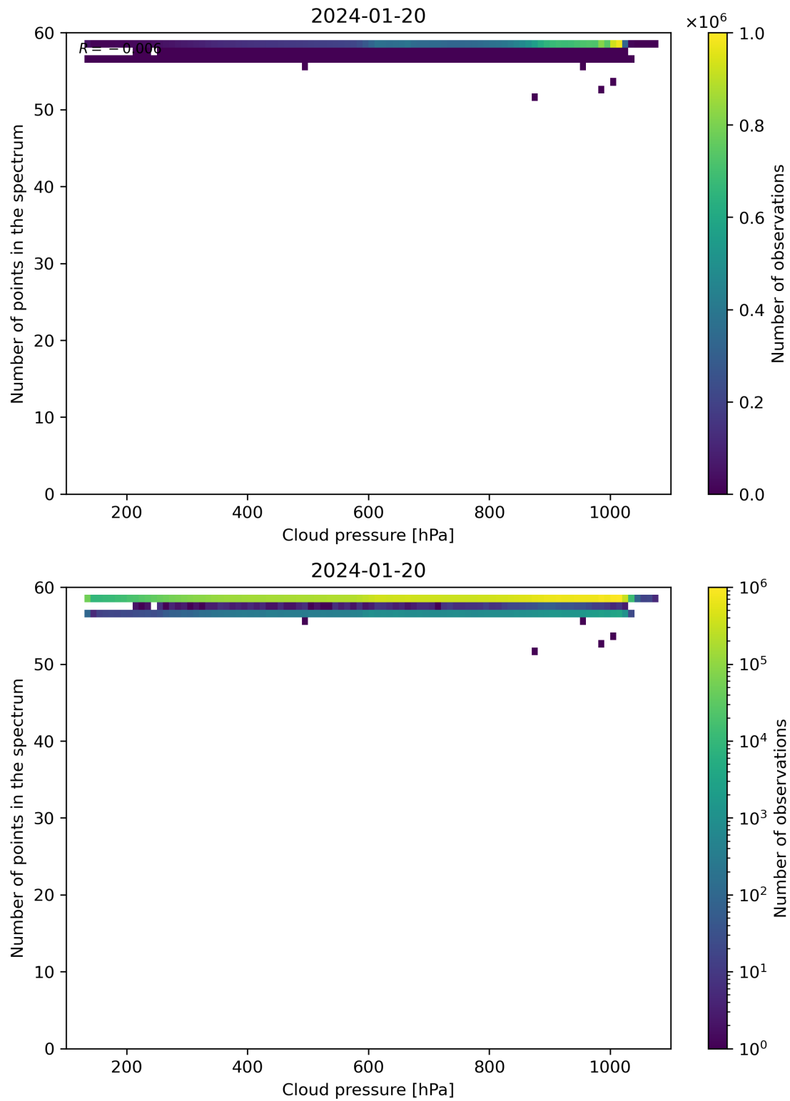
Figure 82: Scatter density plot of “Cloud pressure” against “Number of points in the spectrum” for 2024-01-19 to 2024-01-21.
