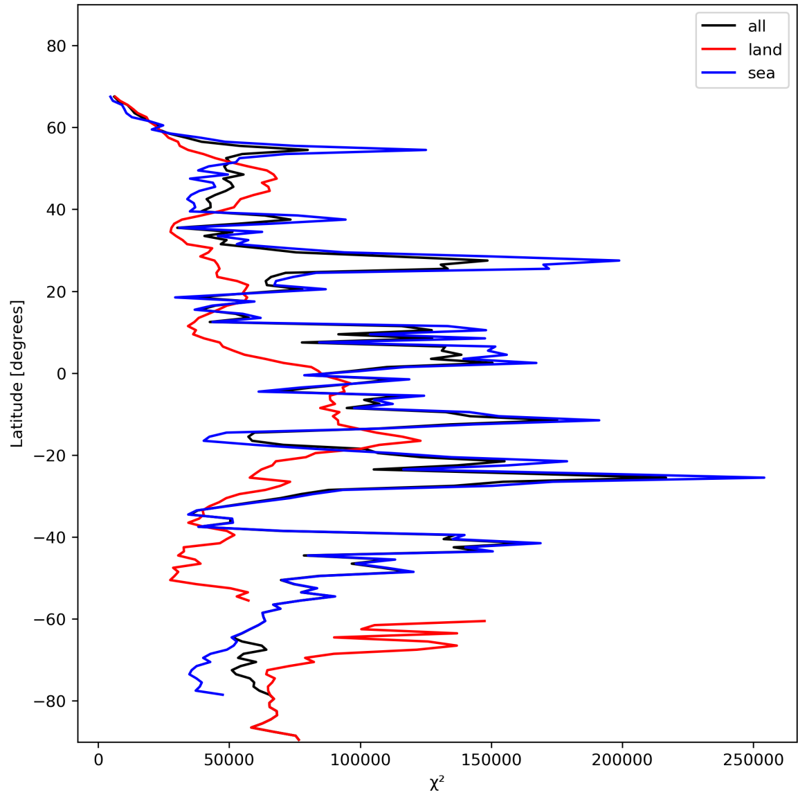
Figure 21: Zonal average of “ \chi^2 ” for 2024-01-19 to 2024-01-21.
