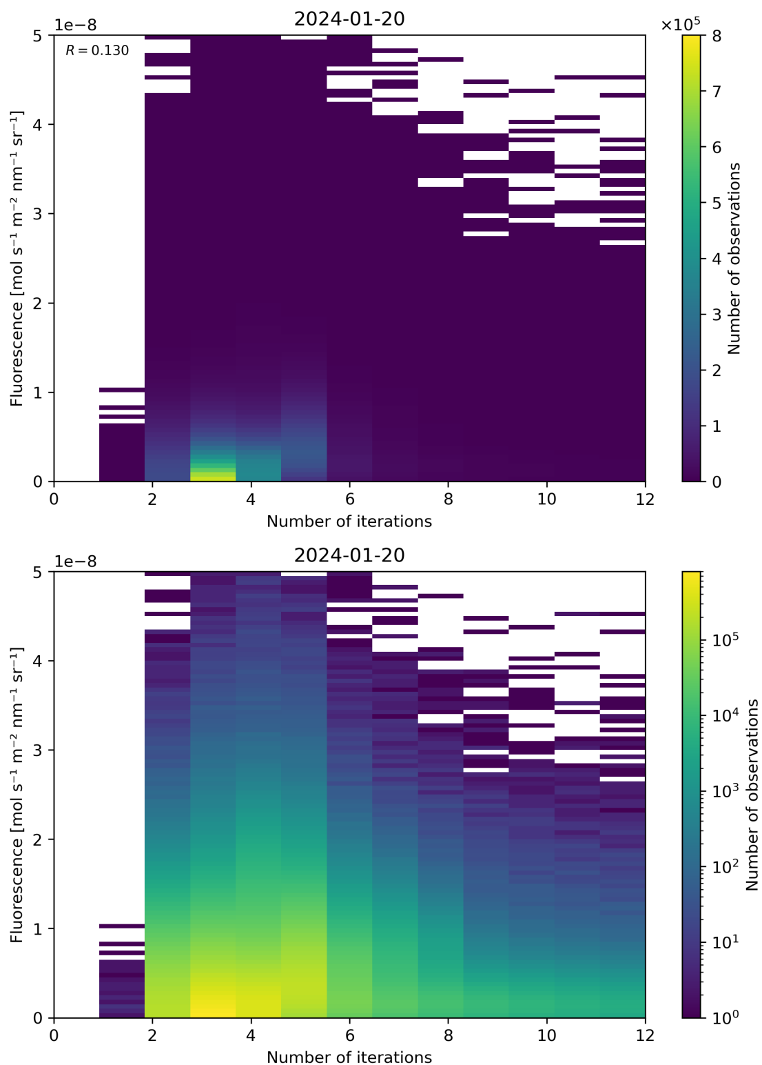
Figure 98: Scatter density plot of “Number of iterations” against “Fluorescence” for 2024-01-19 to 2024-01-21.
