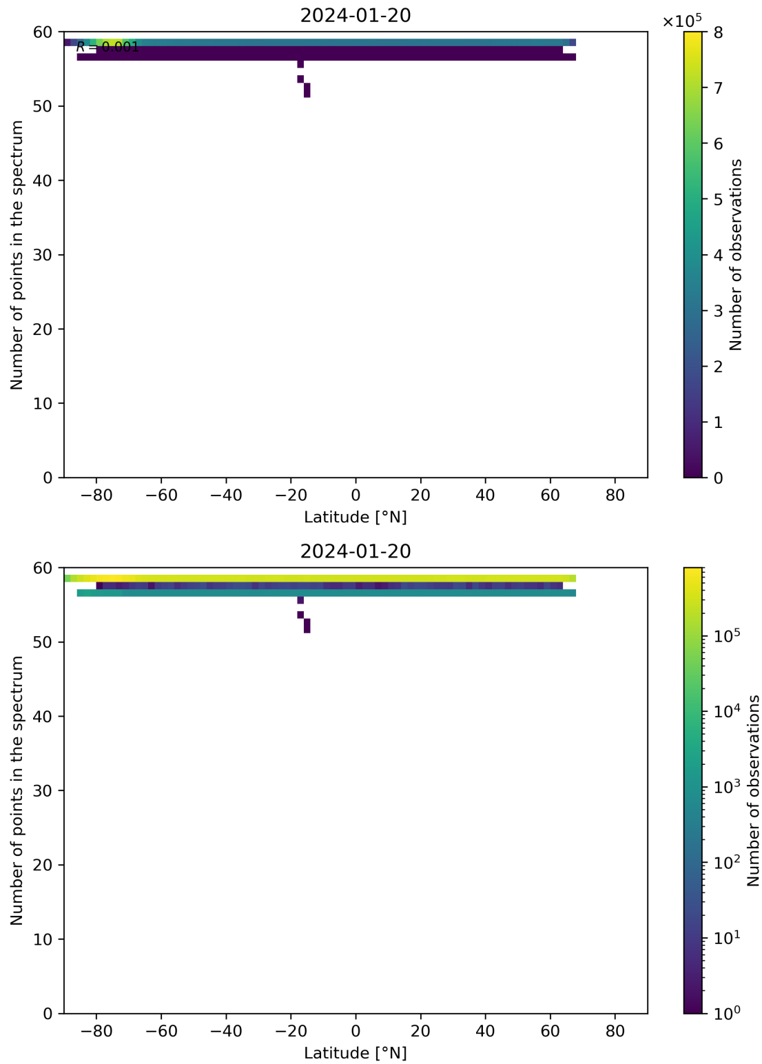
Figure 94: Scatter density plot of “Latitude” against “Number of points in the spectrum” for 2024-01-19 to 2024-01-21.
