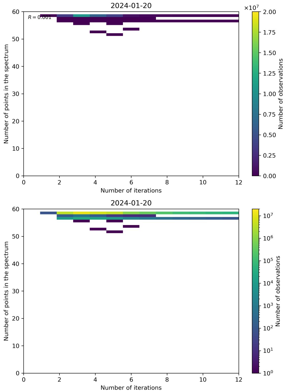
Figure 99: Scatter density plot of “Number of iterations” against “Number of points in the spectrum” for 2024-01-19 to 2024-01-21.
