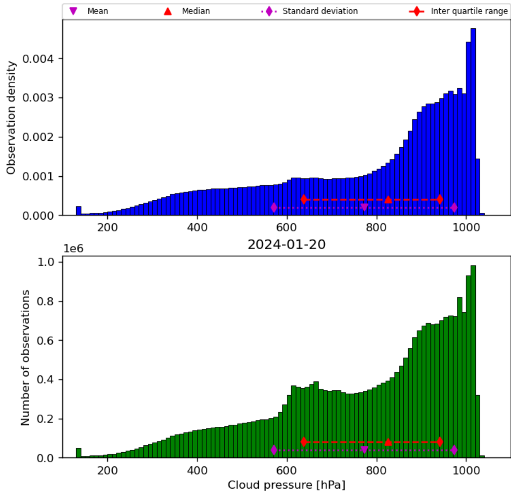
Figure 30: Histogram of “Cloud pressure” for 2024-01-19 to 2024-01-21
