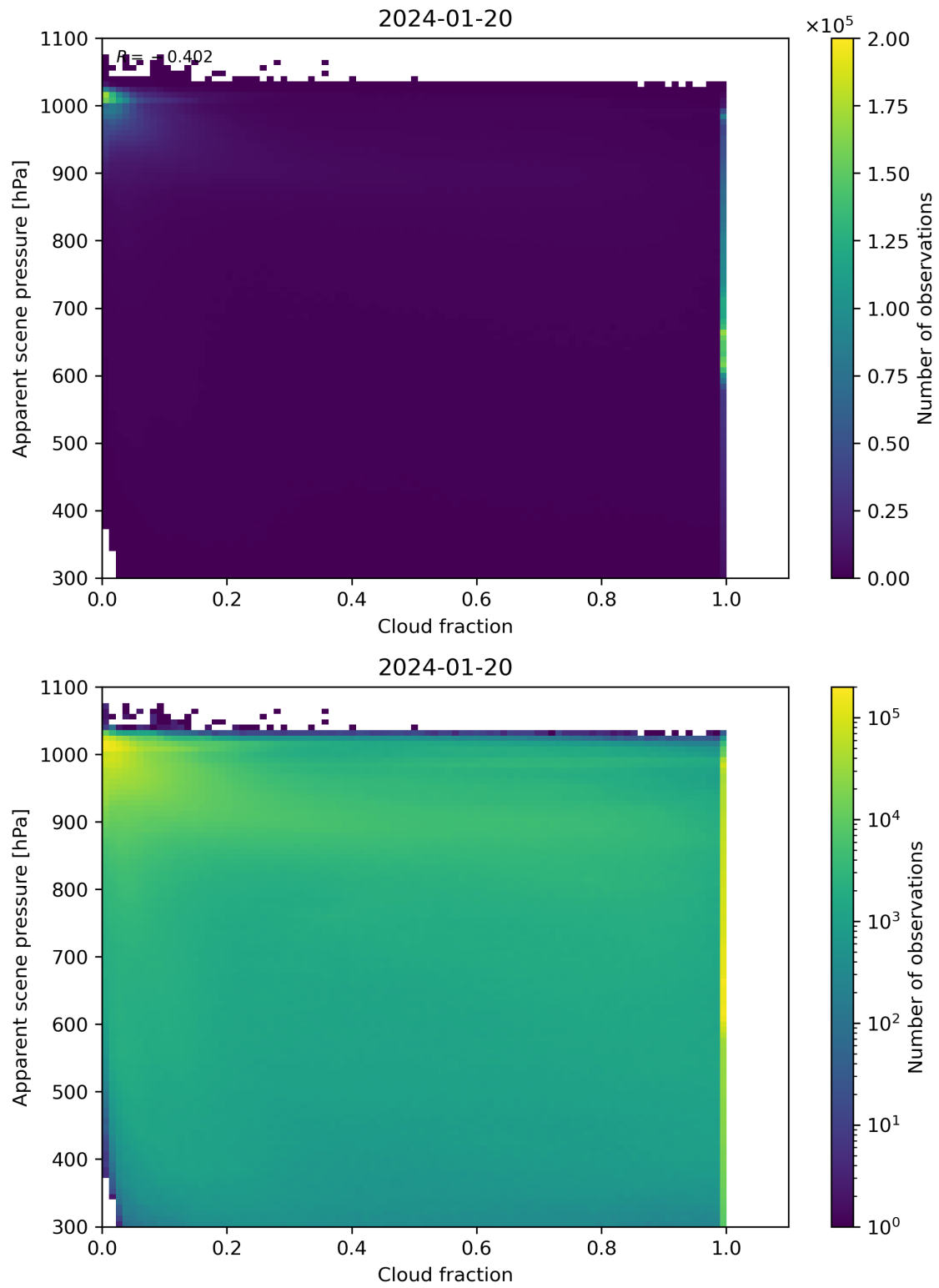
Figure 70: Scatter density plot of “Cloud fraction” against “Apparent scene pressure” for 2024-01-19 to 2024-01-21.
