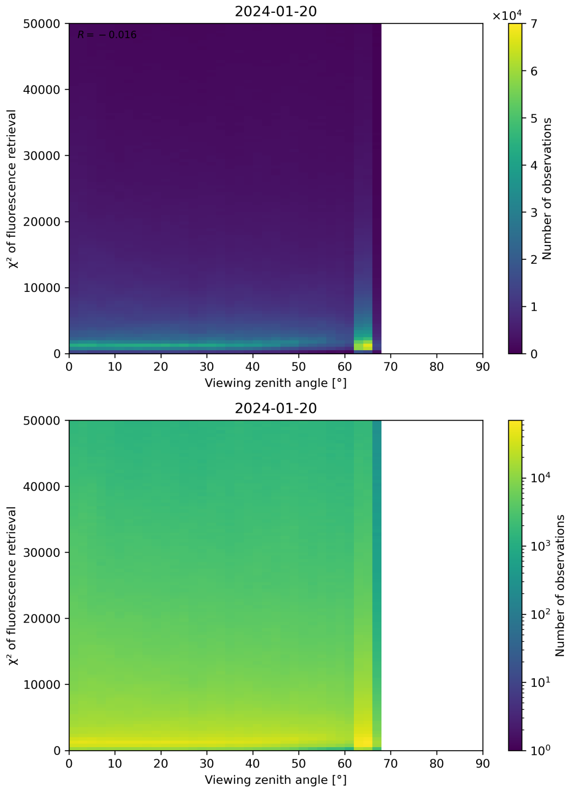
Figure 119: Scatter density plot of “Viewing zenith angle” against “ \chi^2 of fluorescence retrieval” for 2024-01-19 to 2024-01-21.
