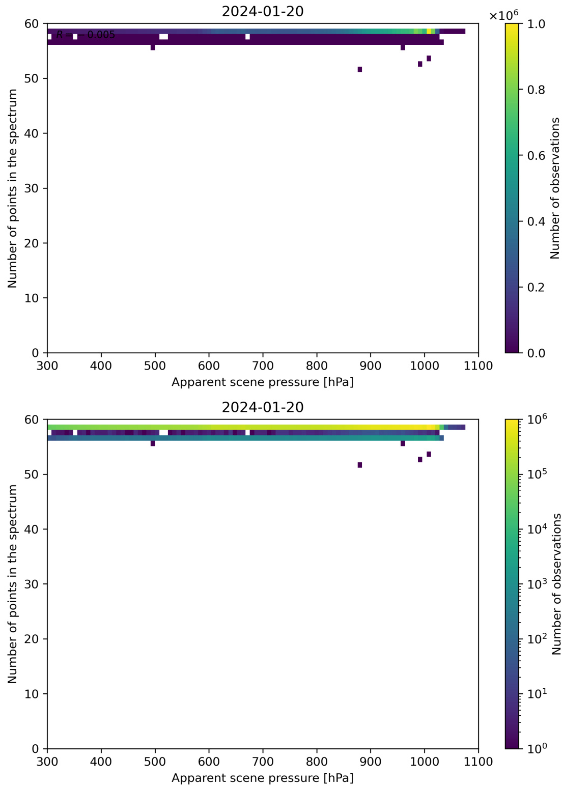
Figure 66: Scatter density plot of “Apparent scene pressure” against “Number of points in the spectrum” for 2024-01-19 to 2024-01-21.
