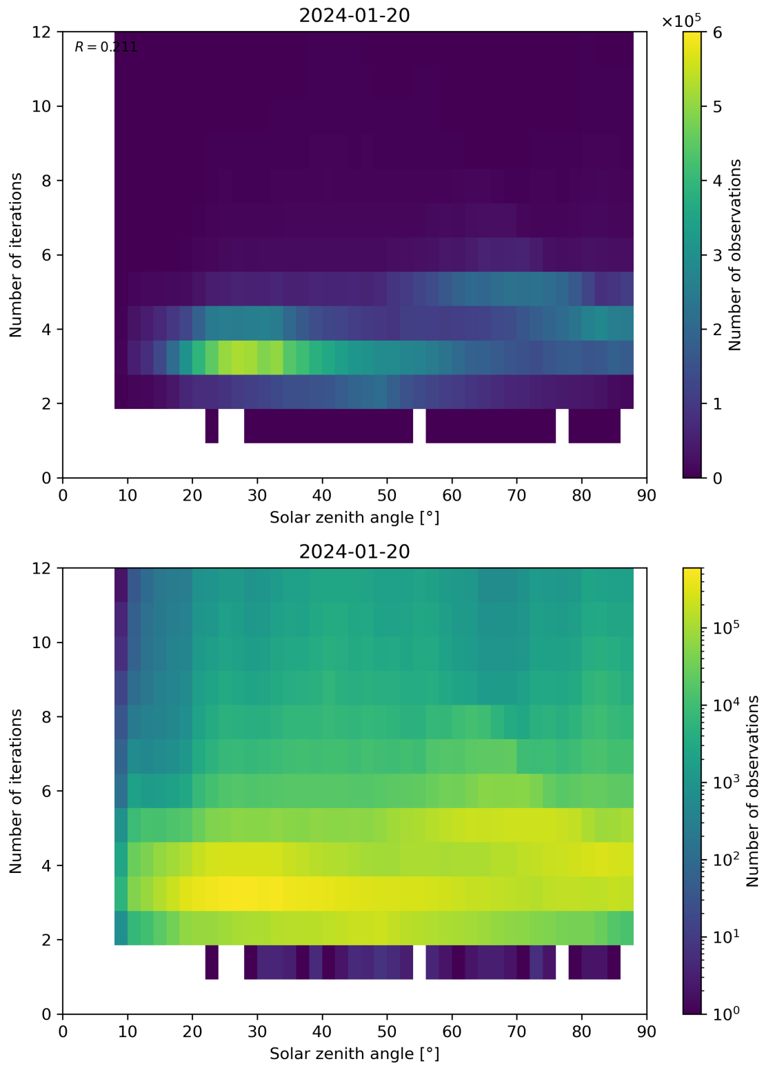
Figure 114: Scatter density plot of “Solar zenith angle” against “Number of iterations” for 2024-01-19 to 2024-01-21.
