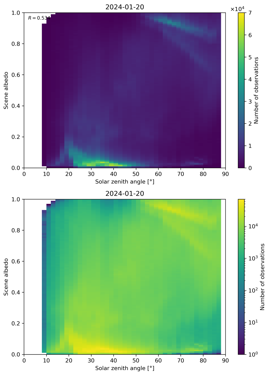
Figure 116: Scatter density plot of “Solar zenith angle” against “Scene albedo” for 2024-01-19 to 2024-01-21.
