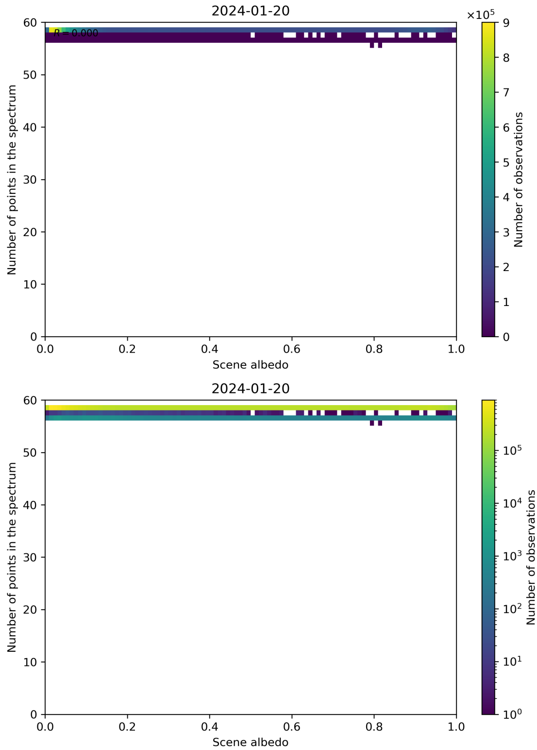
Figure 106: Scatter density plot of “Scene albedo” against “Number of points in the spectrum” for 2024-01-19 to 2024-01-21.
