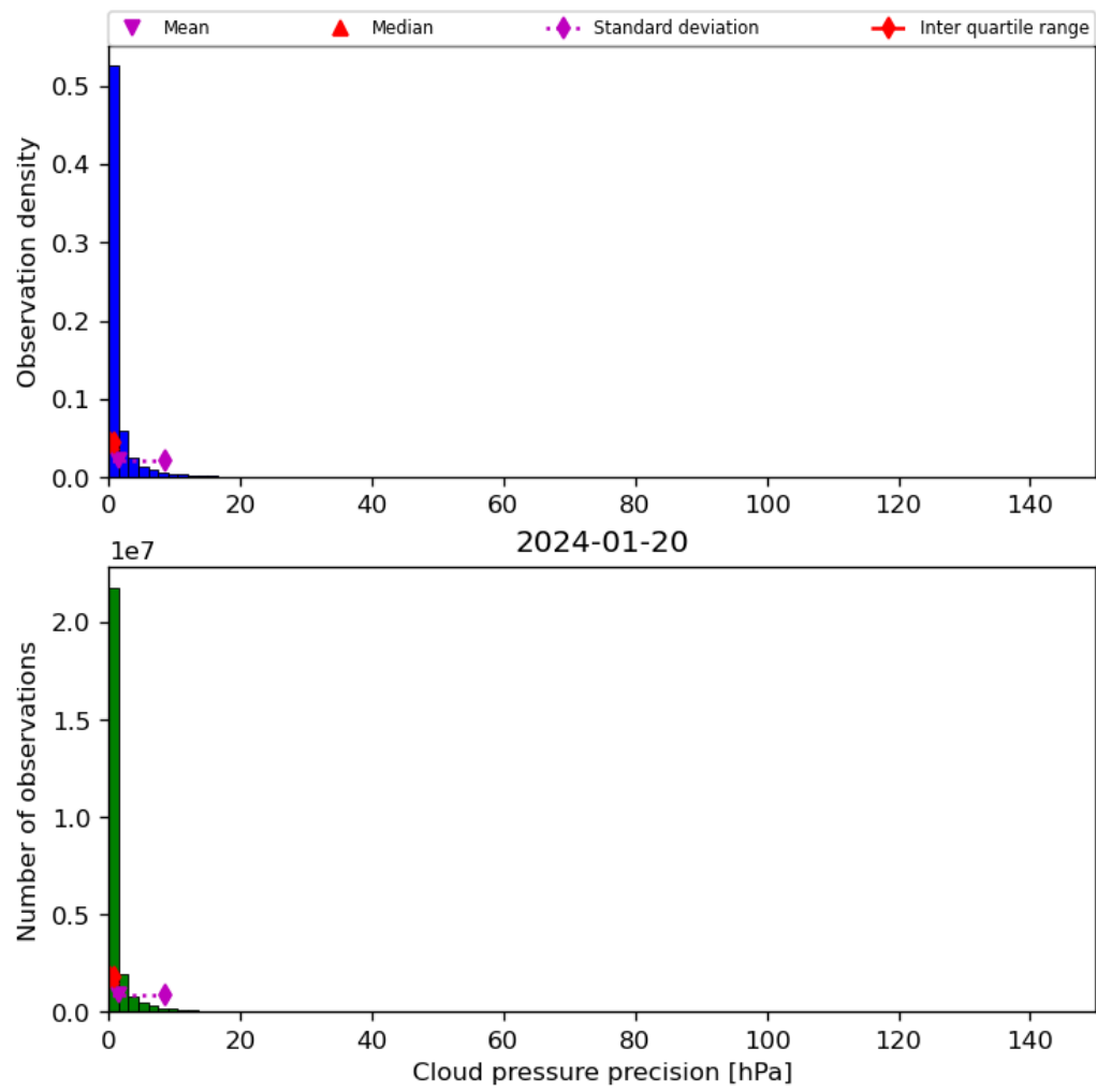
Figure 31: Histogram of “Cloud pressure precision” for 2024-01-19 to 2024-01-21
