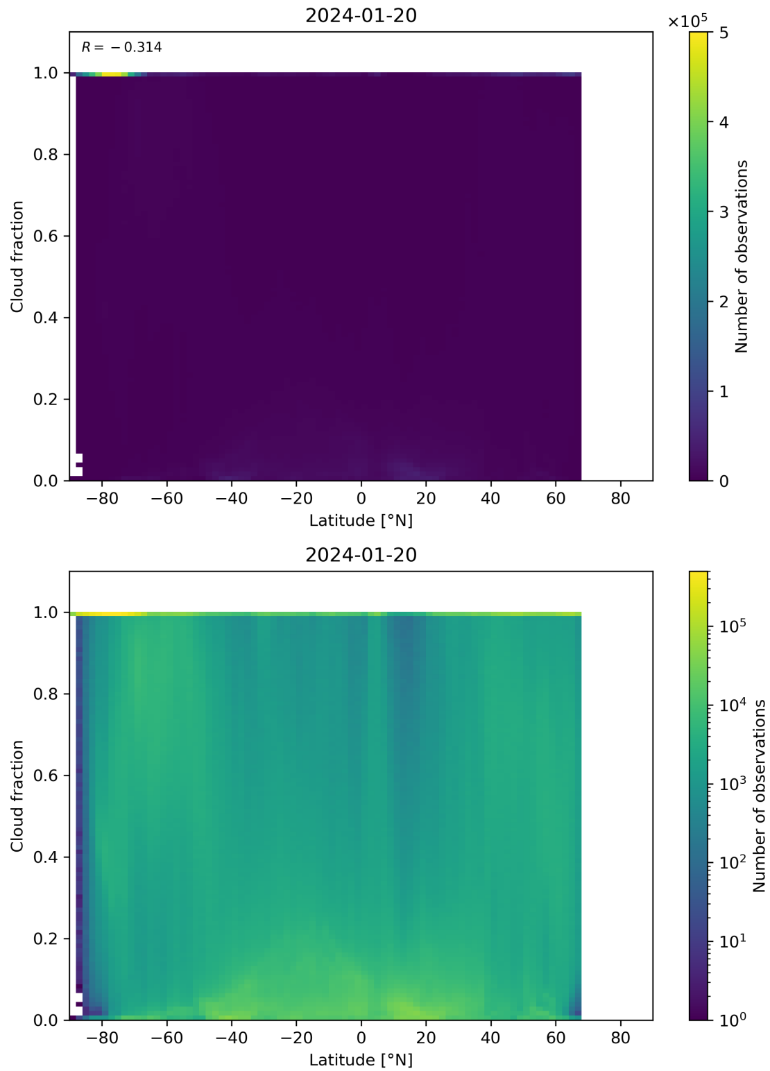
Figure 90: Scatter density plot of “Latitude” against “Cloud fraction” for 2024-01-19 to 2024-01-21.
