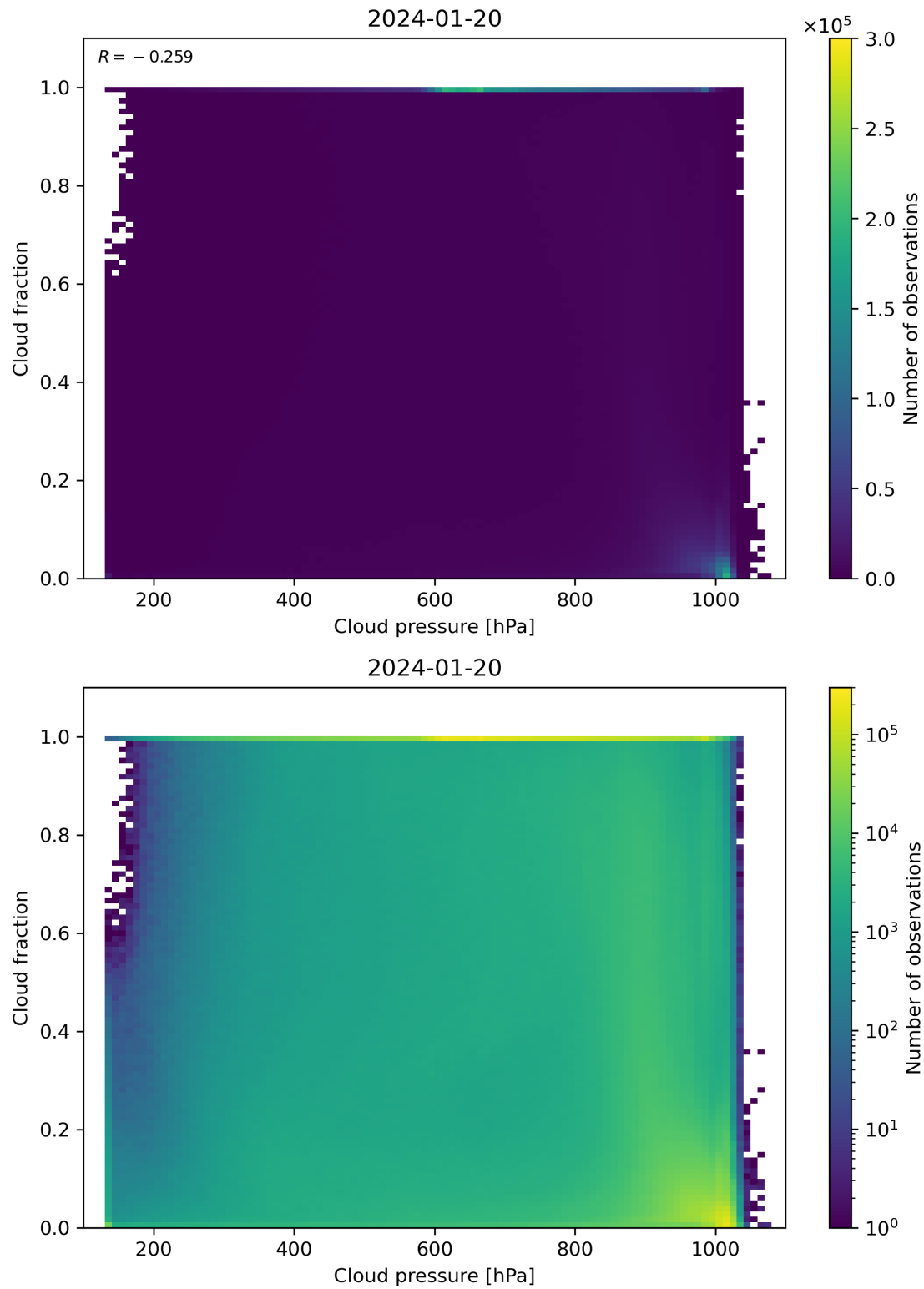
Figure 79: Scatter density plot of “Cloud pressure” against “Cloud fraction” for 2024-01-19 to 2024-01-21.
