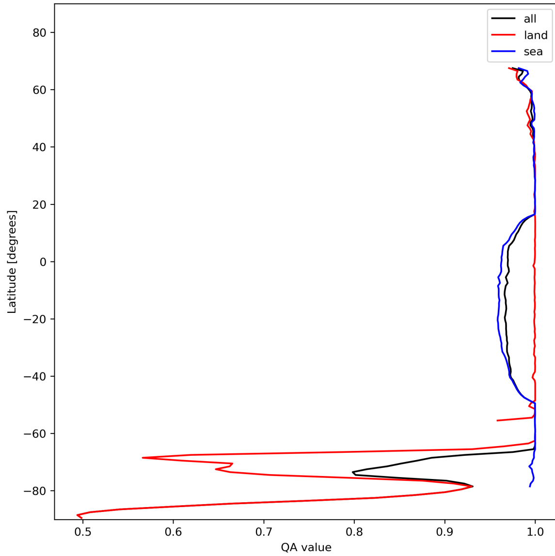
Figure 12: Zonal average of “QA value” for 2024-01-19 to 2024-01-21.
