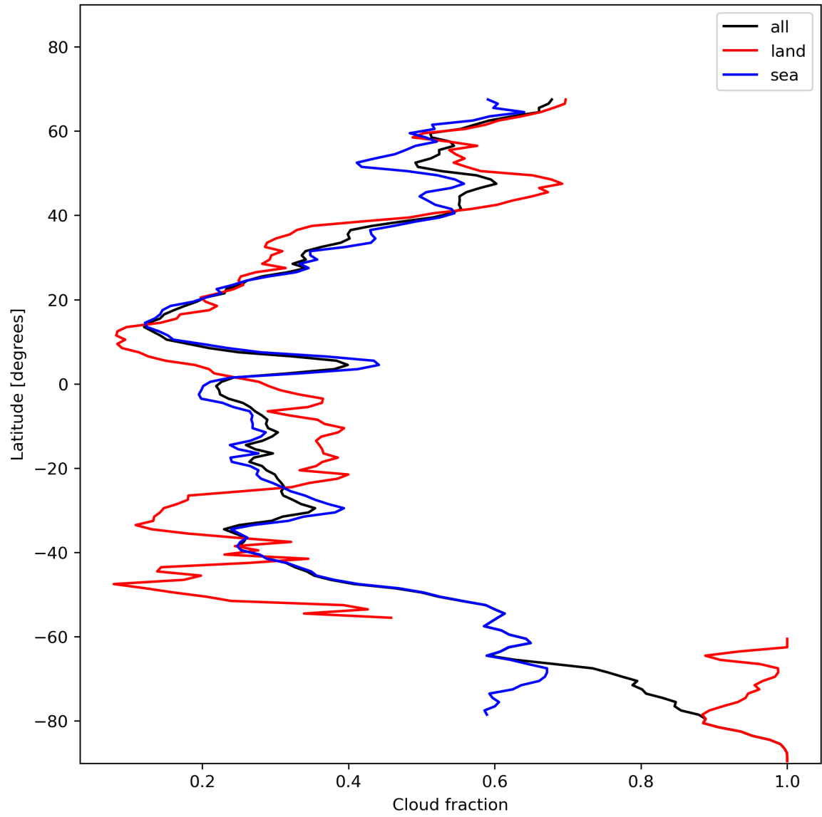
Figure 15: Zonal average of “Cloud fraction” for 2024-01-19 to 2024-01-21.
