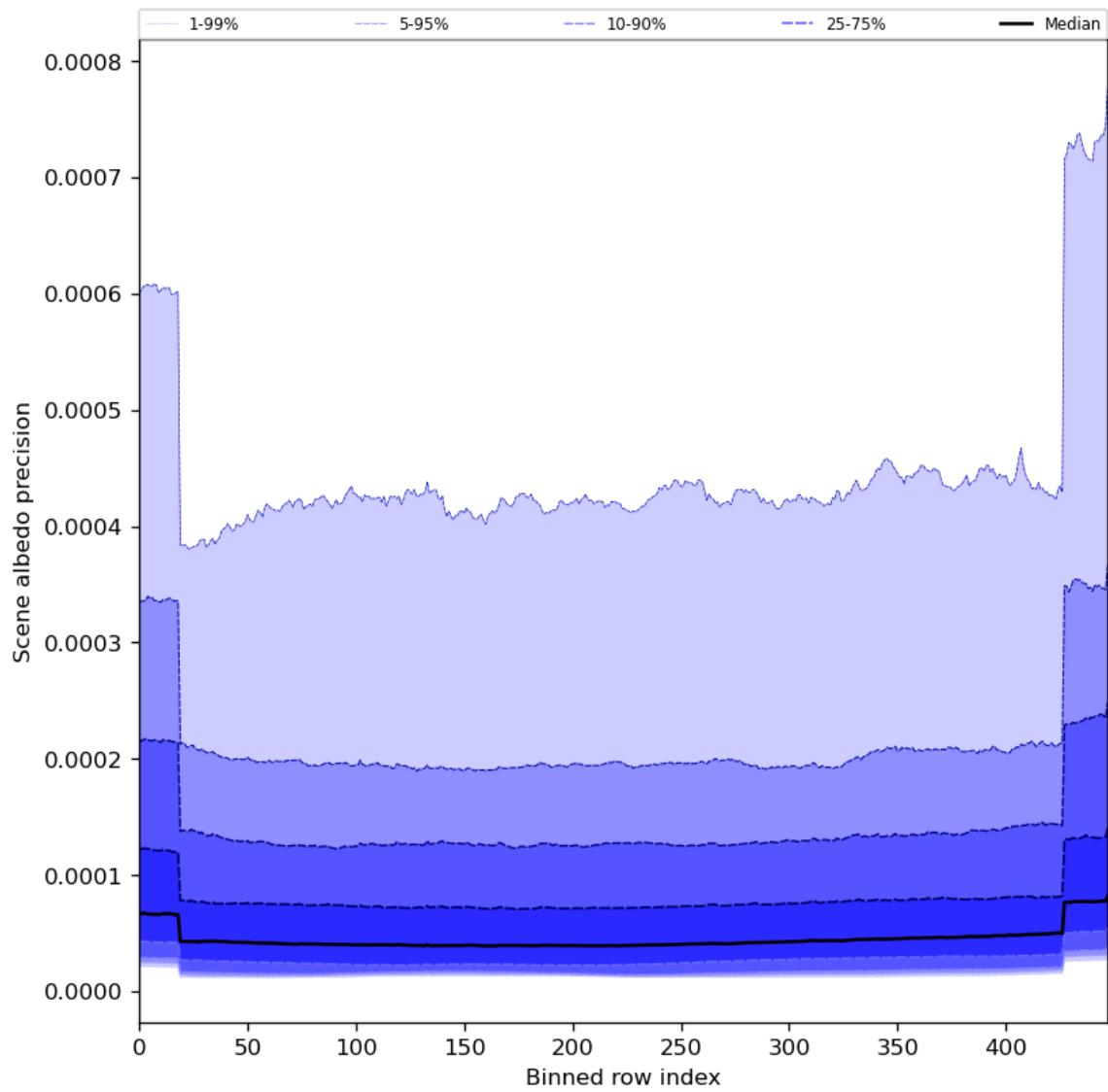
Figure 52: Along track statistics of “Scene albedo precision” for 2024-01-19 to 2024-01-21
