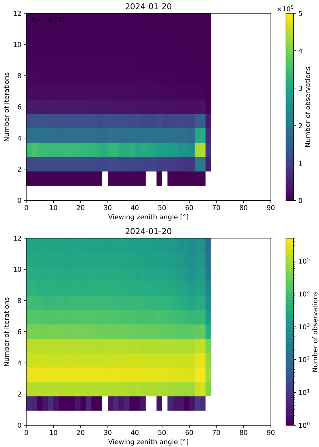
Figure 124: Scatter density plot of “Viewing zenith angle” against “Number of iterations” for 2024-01-19 to 2024-01-21.
