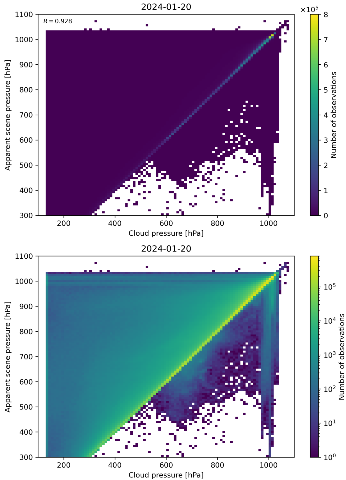
Figure 77: Scatter density plot of “Cloud pressure” against “Apparent scene pressure” for 2024-01-19 to 2024-01-21.
