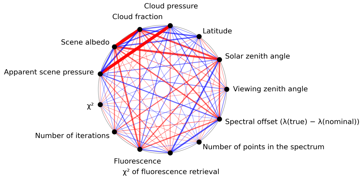
Figure 1: Map of correlation graph for 2024-01-19 to 2024-01-21.
