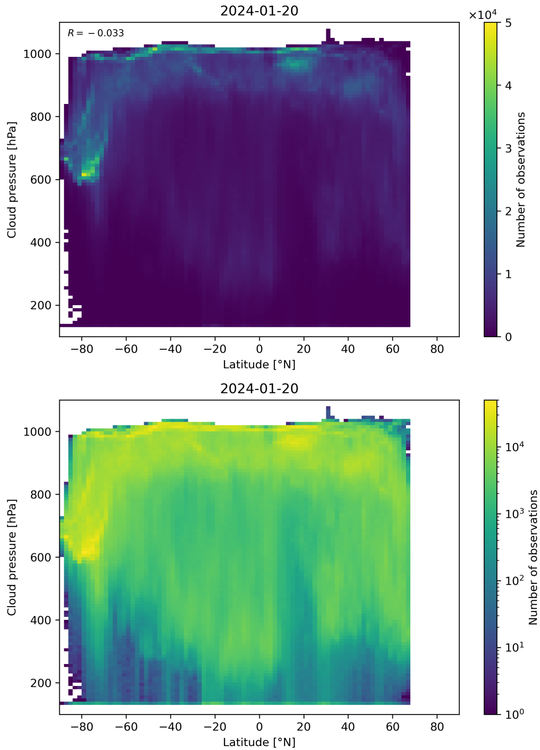
Figure 91: Scatter density plot of “Latitude” against “Cloud pressure” for 2024-01-19 to 2024-01-21.
