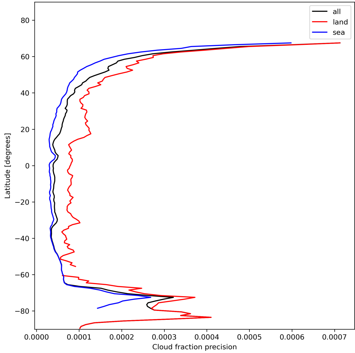
Figure 16: Zonal average of “Cloud fraction precision” for 2024-01-19 to 2024-01-21.
