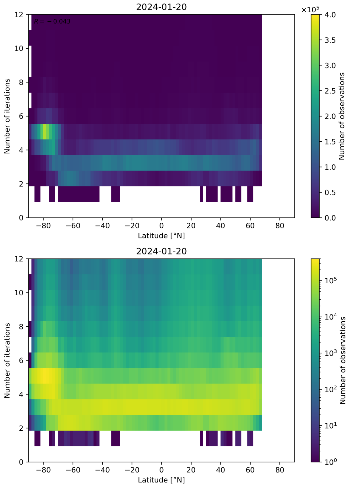
Figure 93: Scatter density plot of “Latitude” against “Number of iterations” for 2024-01-19 to 2024-01-21.
