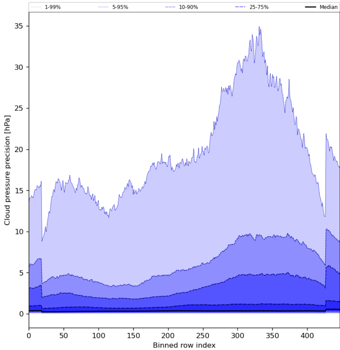
Figure 48: Along track statistics of “Cloud pressure precision” for 2024-01-19 to 2024-01-21
