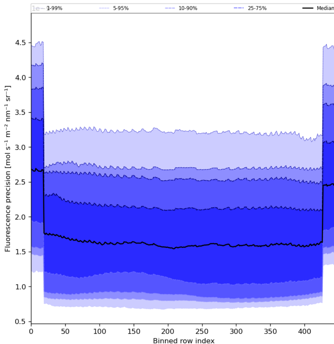
Figure 58: Along track statistics of “Fluorescence precision” for 2024-01-19 to 2024-01-21
