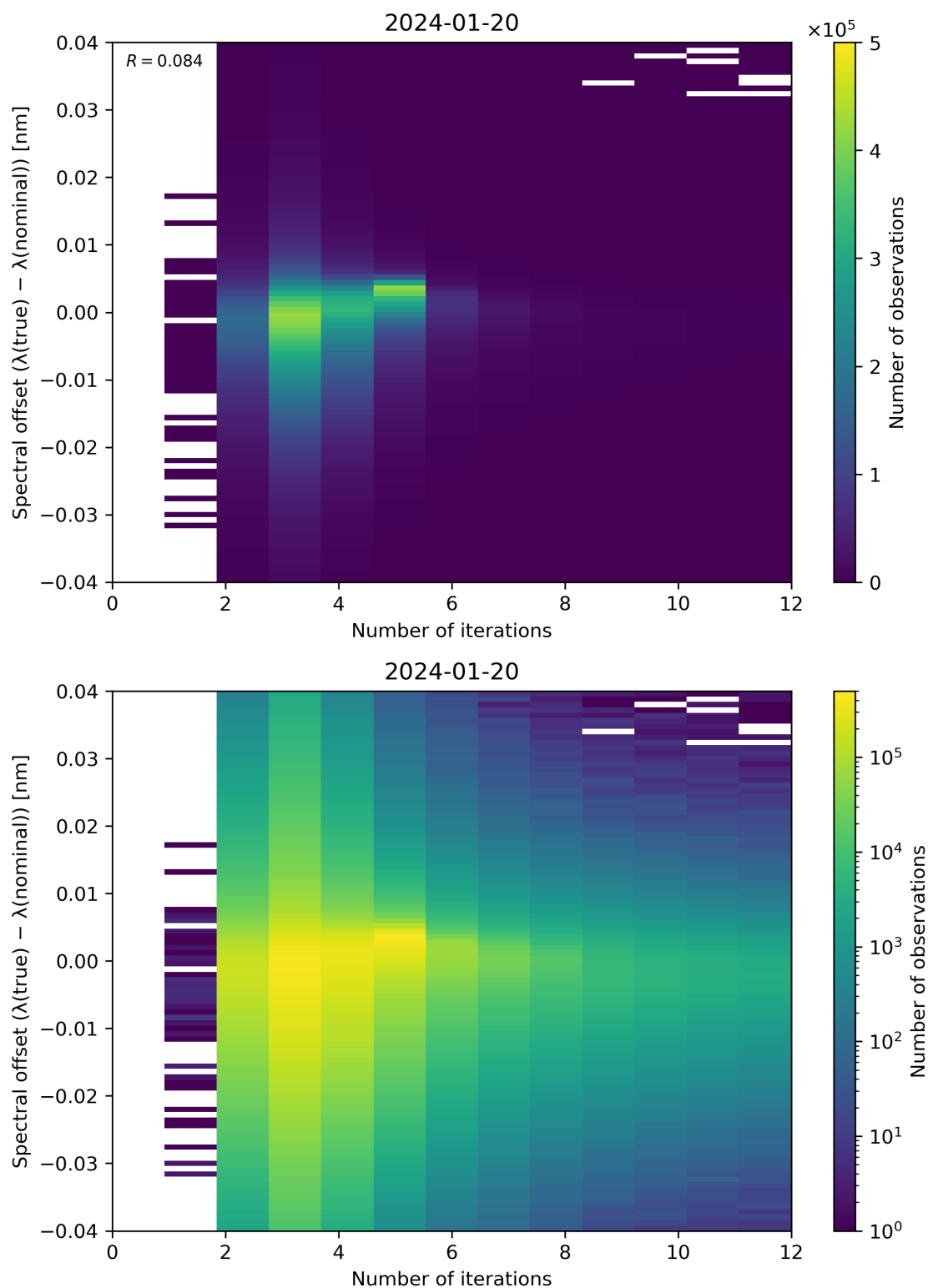
Figure 100: Scatter density plot of “Number of iterations” against “Spectral offset ( \lambda(\text{true}) - \lambda(\text{nominal}) )” for 2024-01-19 to 2024-01-21.
