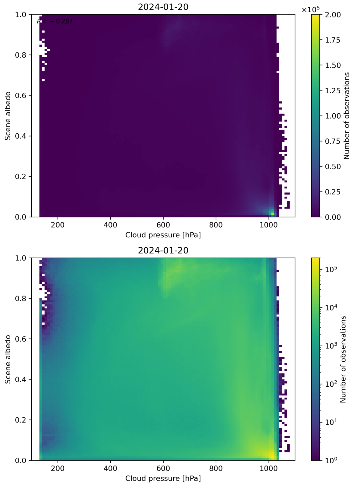
Figure 83: Scatter density plot of “Cloud pressure” against “Scene albedo” for 2024-01-19 to 2024-01-21.
