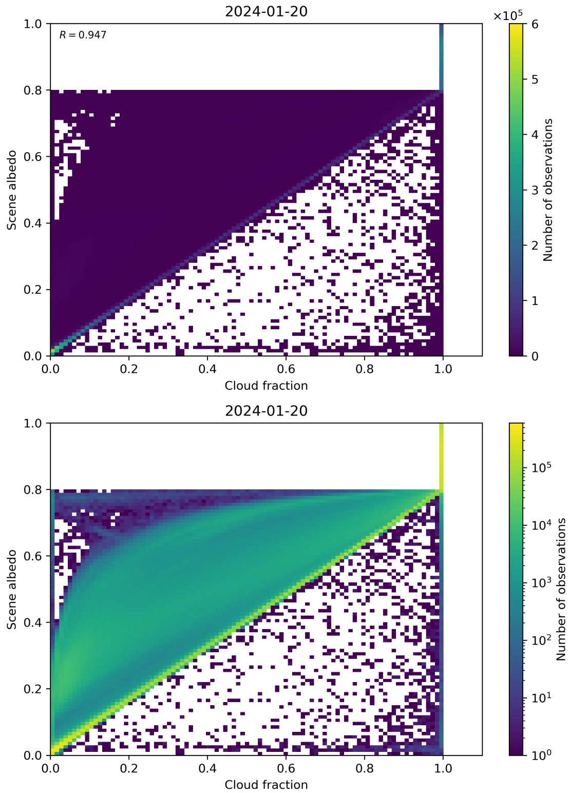
Figure 75: Scatter density plot of “Cloud fraction” against “Scene albedo” for 2024-01-19 to 2024-01-21.
