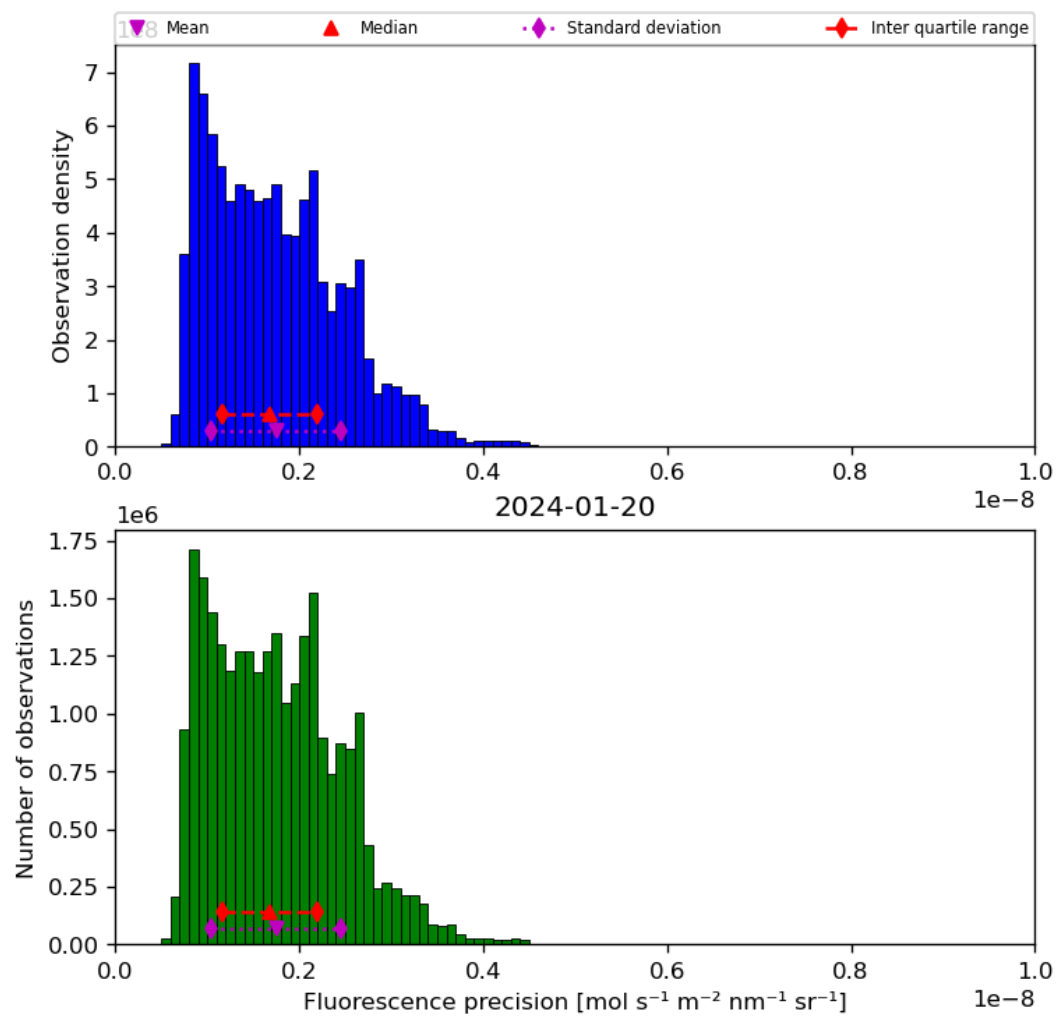
Figure 41: Histogram of “Fluorescence precision” for 2024-01-19 to 2024-01-21
