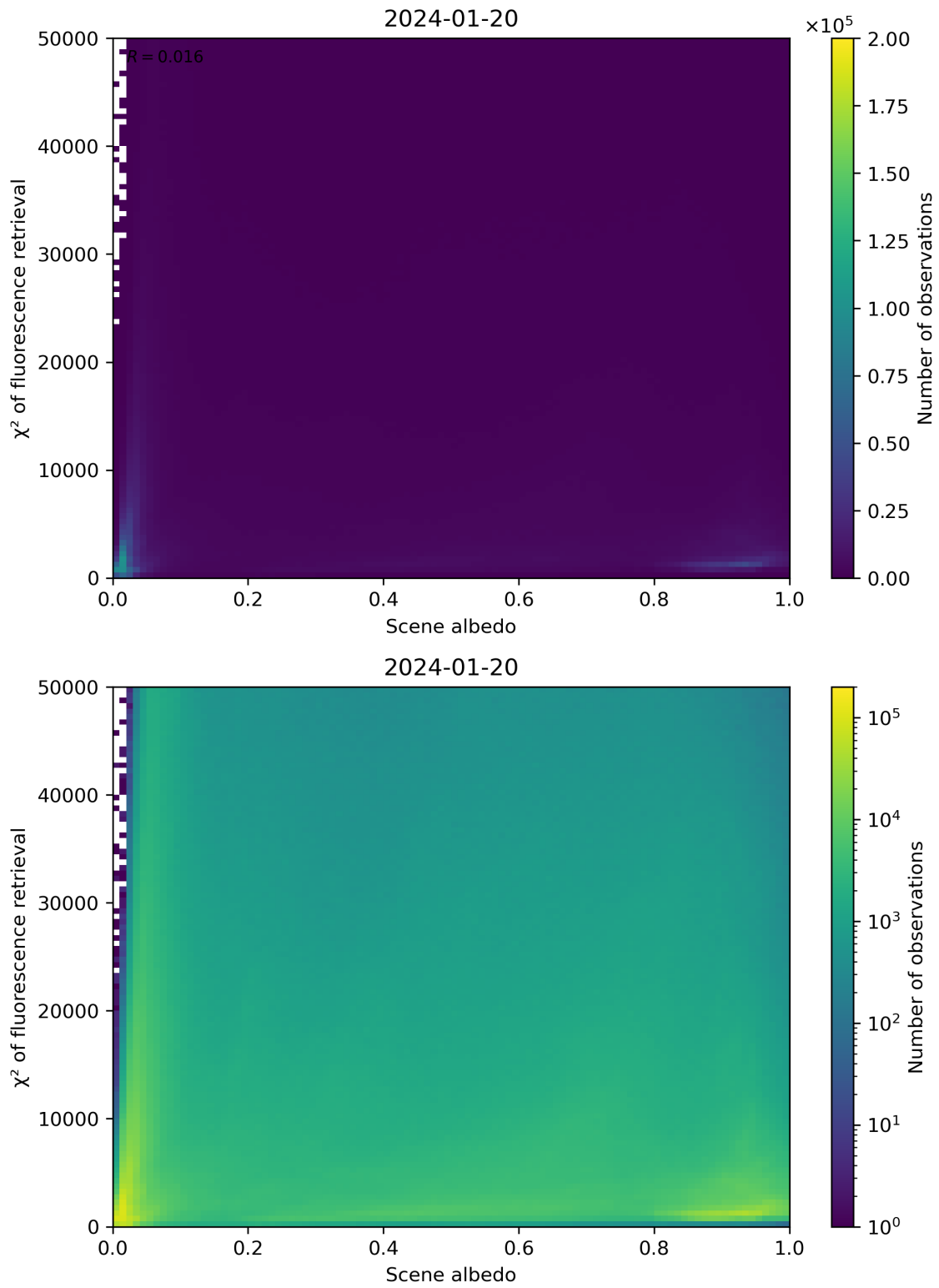
Figure 103: Scatter density plot of “Scene albedo” against “ \chi^2 of fluorescence retrieval” for 2024-01-19 to 2024-01-21.
