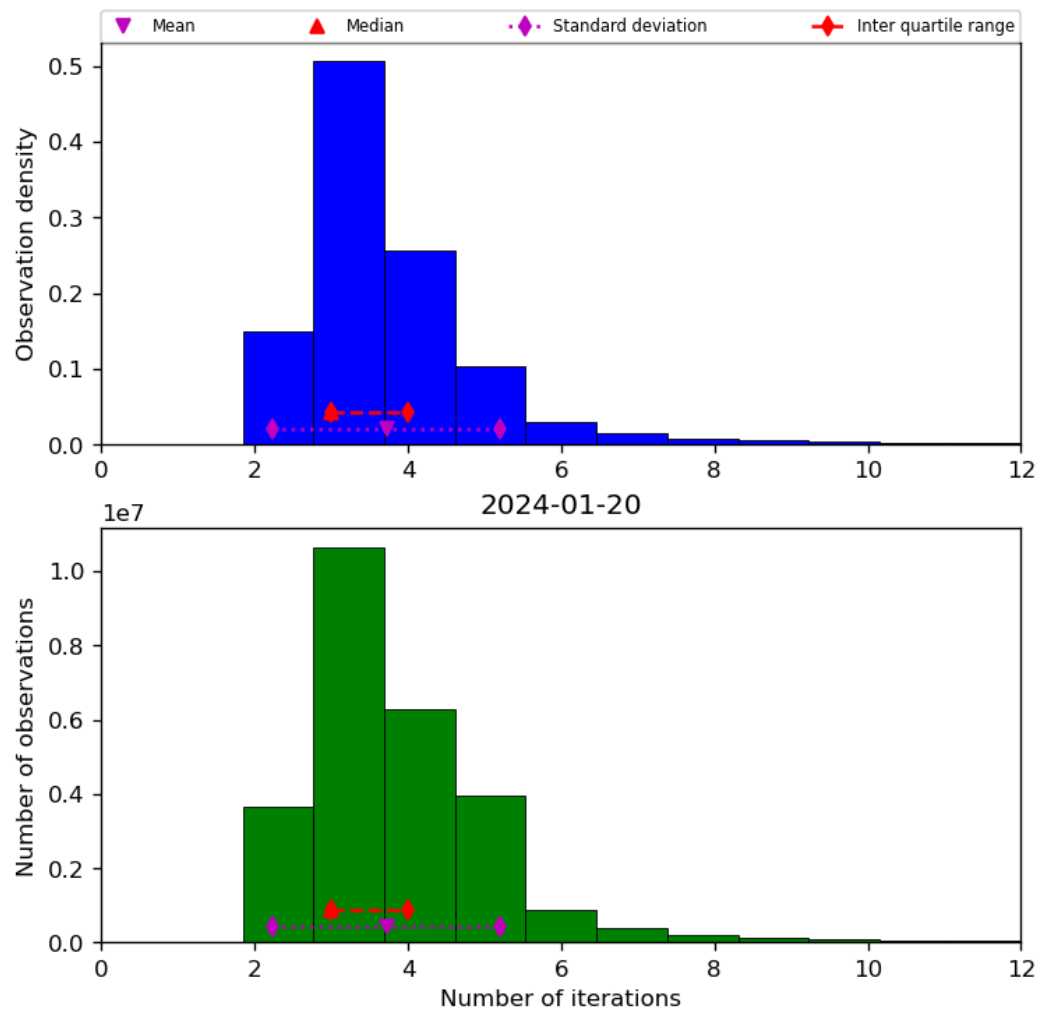
Figure 39: Histogram of “Number of iterations” for 2024-01-19 to 2024-01-21
