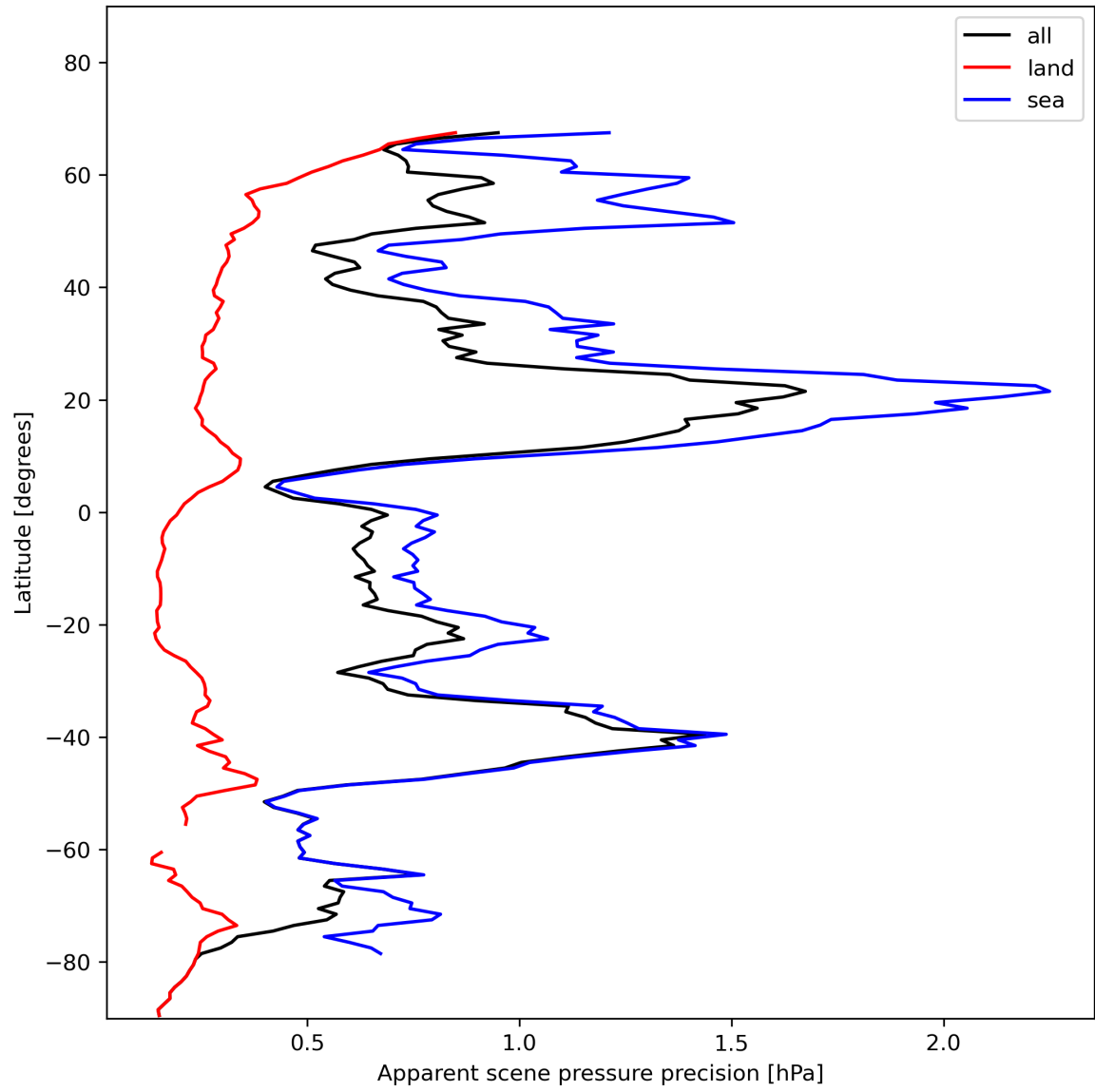
Figure 20: Zonal average of “Apparent scene pressure precision” for 2024-01-19 to 2024-01-21.
