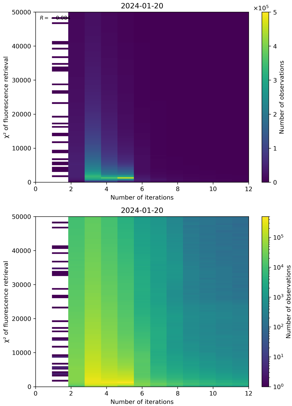
Figure 97: Scatter density plot of “Number of iterations” against “ \chi^2 of fluorescence retrieval” for 2024-01-19 to 2024-01-21.
