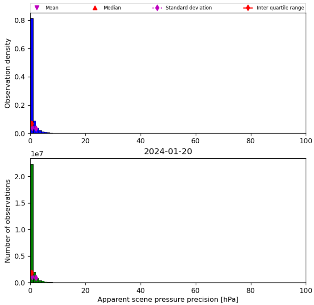
Figure 37: Histogram of “Apparent scene pressure precision” for 2024-01-19 to 2024-01-21
