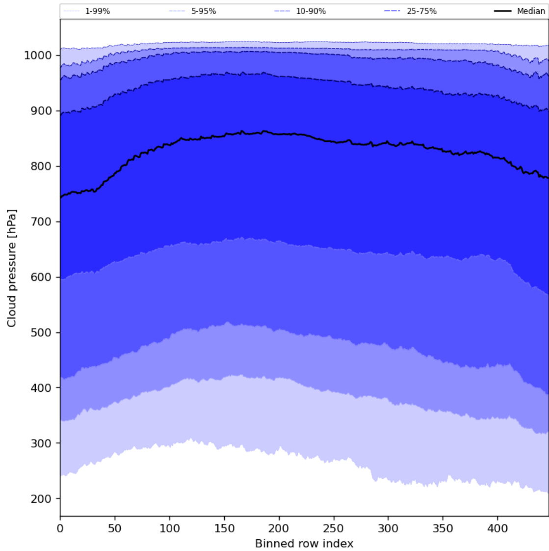
Figure 47: Along track statistics of “Cloud pressure” for 2024-01-19 to 2024-01-21
