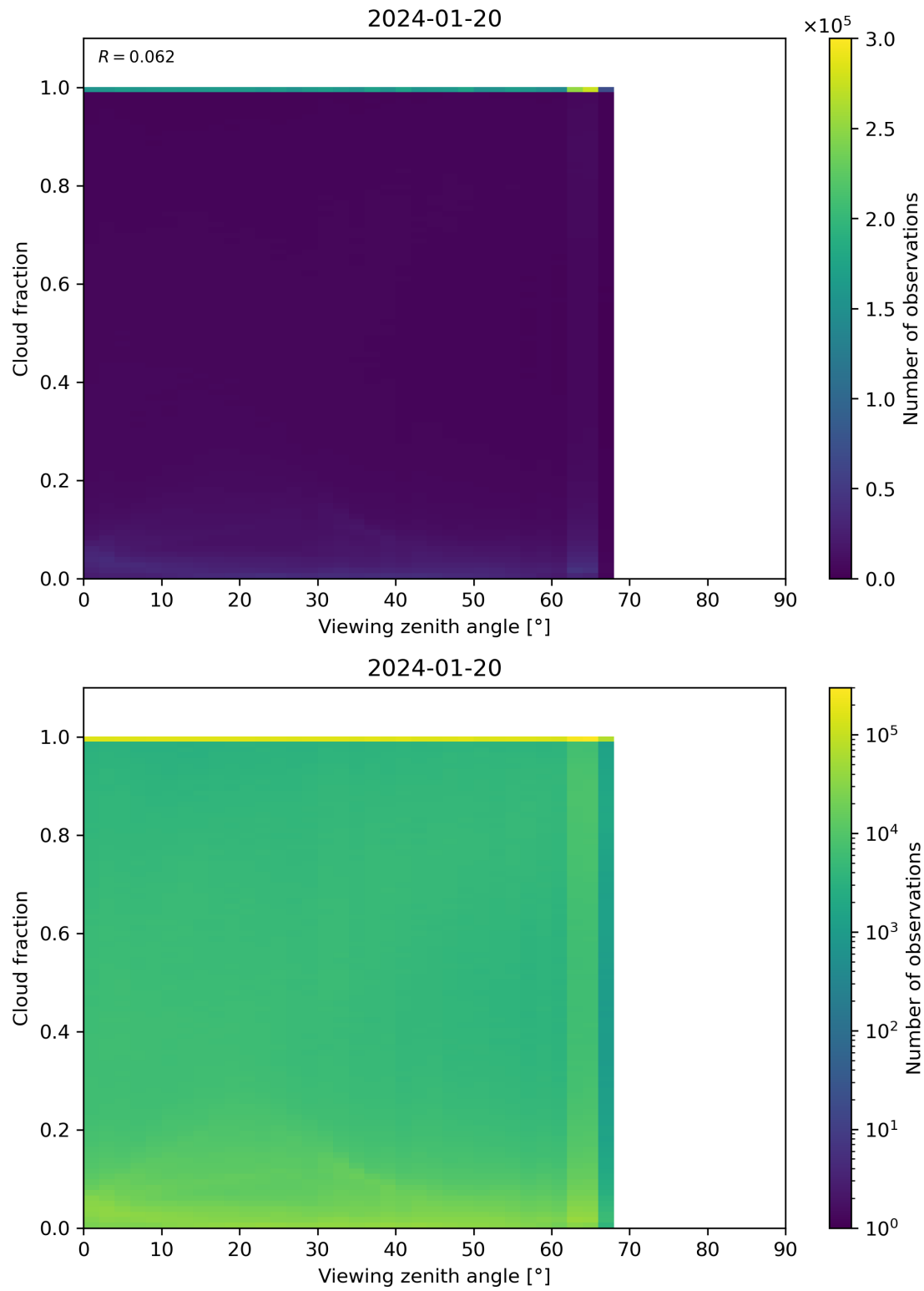
Figure 120: Scatter density plot of “Viewing zenith angle” against “Cloud fraction” for 2024-01-19 to 2024-01-21.
