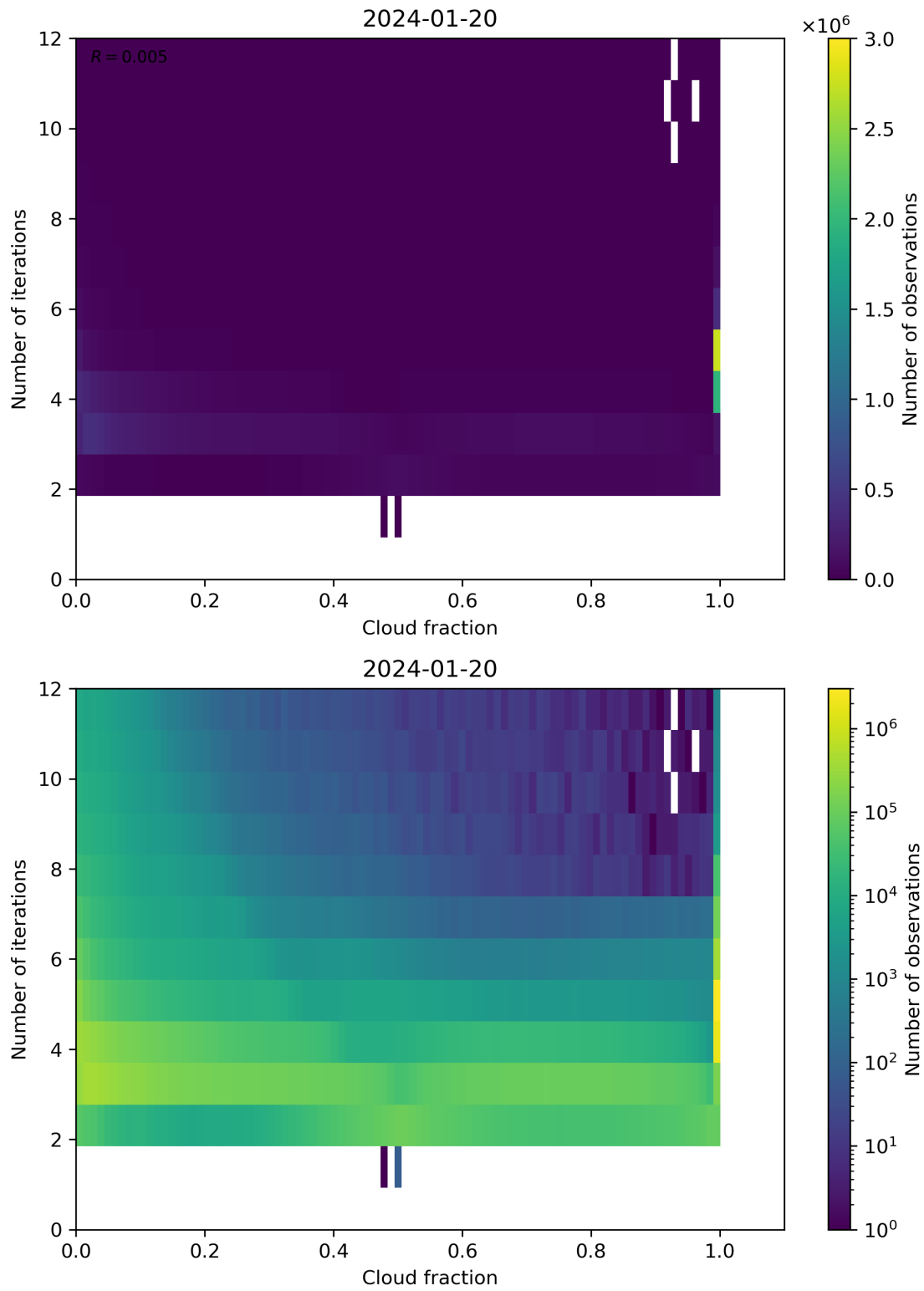
Figure 73: Scatter density plot of “Cloud fraction” against “Number of iterations” for 2024-01-19 to 2024-01-21.
