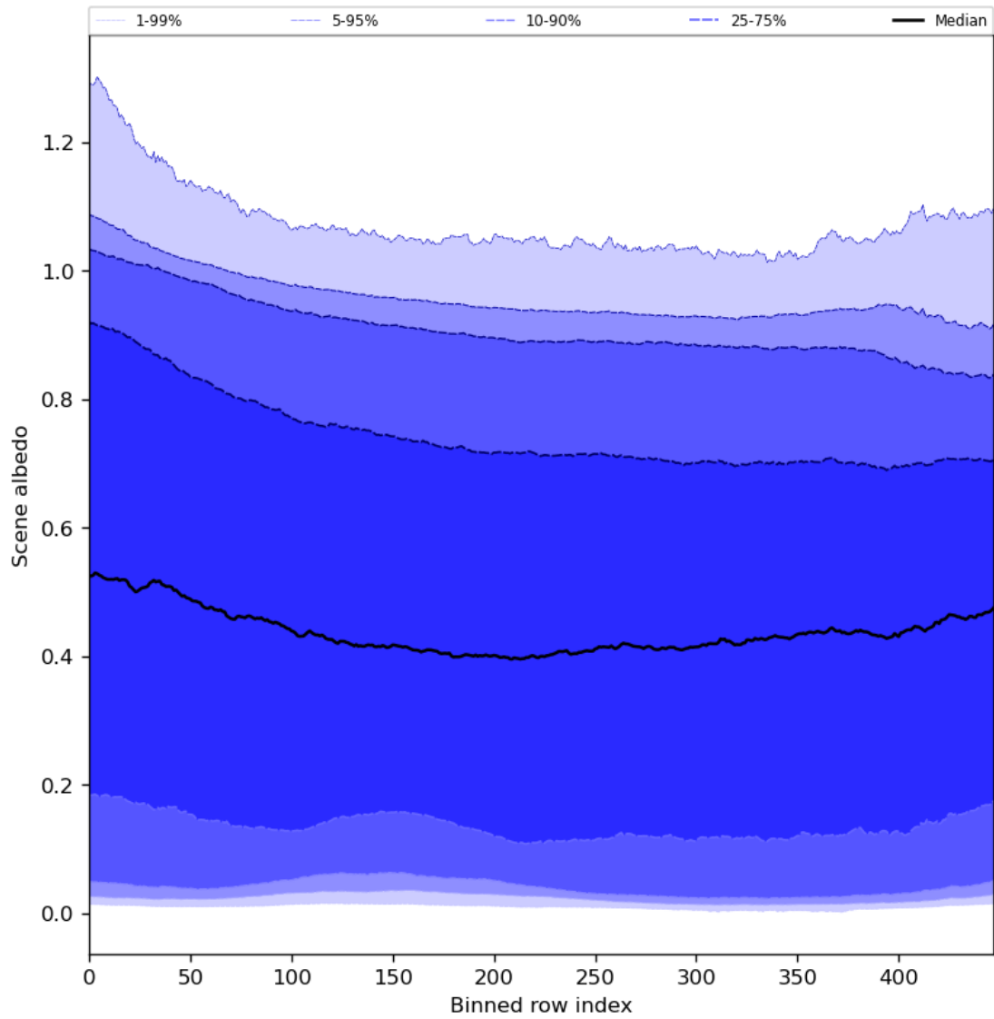
Figure 51: Along track statistics of “Scene albedo” for 2024-01-19 to 2024-01-21
