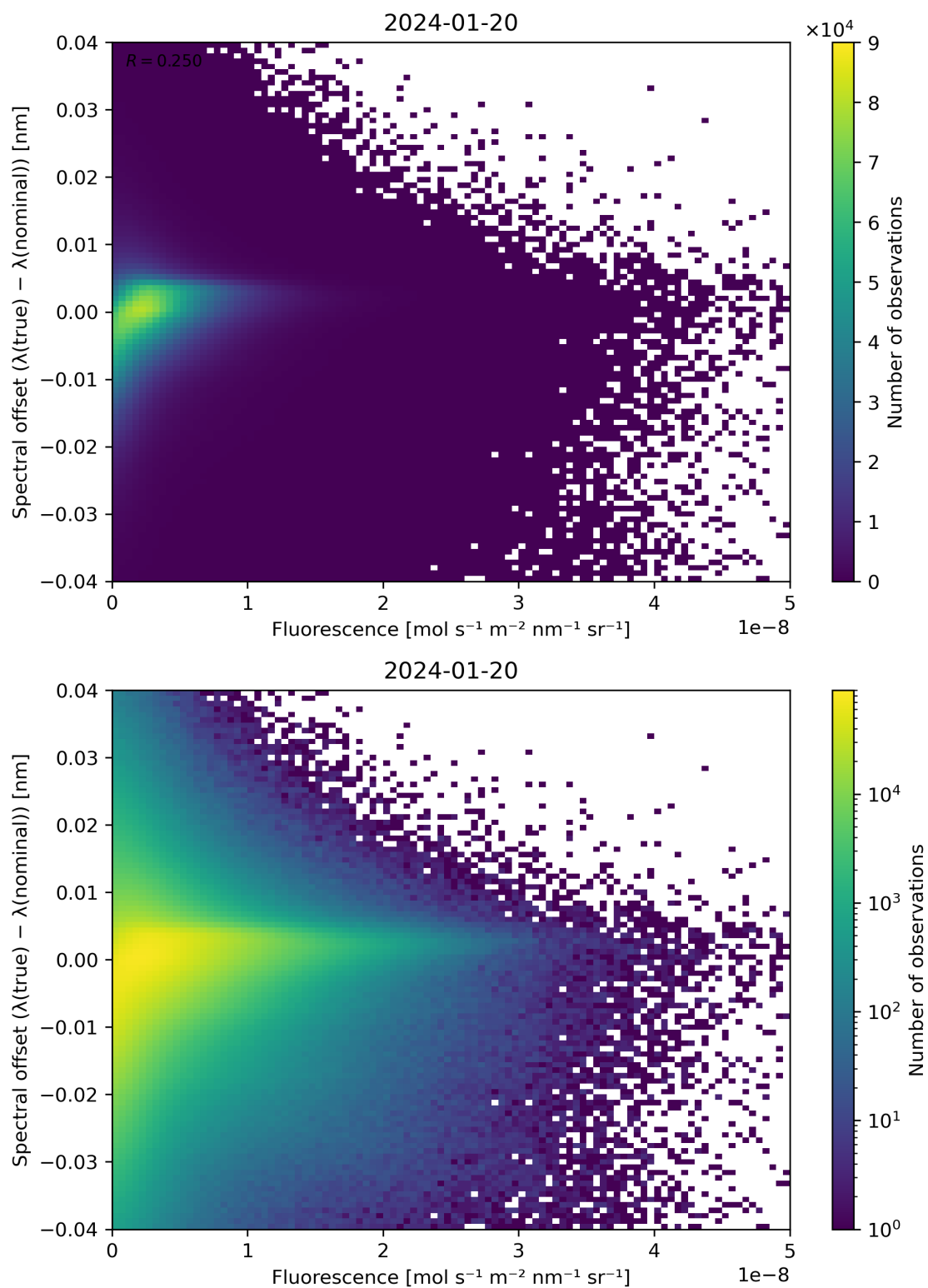
Figure 87: Scatter density plot of “Fluorescence” against “Spectral offset ( \lambda(\text{true}) - \lambda(\text{nominal}) )” for 2024-01-19 to 2024-01-21.
