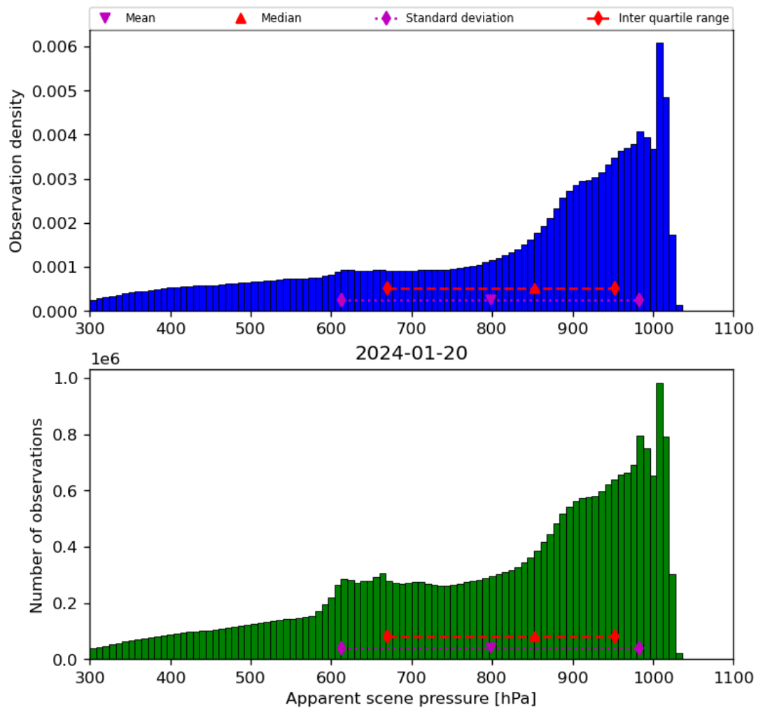
Figure 36: Histogram of “Apparent scene pressure” for 2024-01-19 to 2024-01-21
