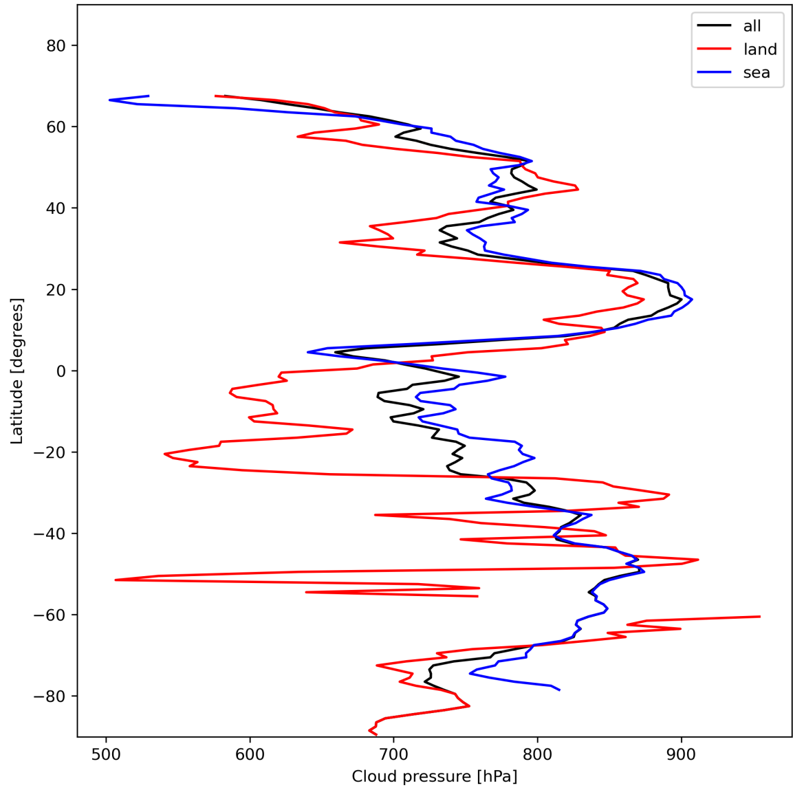
Figure 13: Zonal average of “Cloud pressure” for 2024-01-19 to 2024-01-21.
