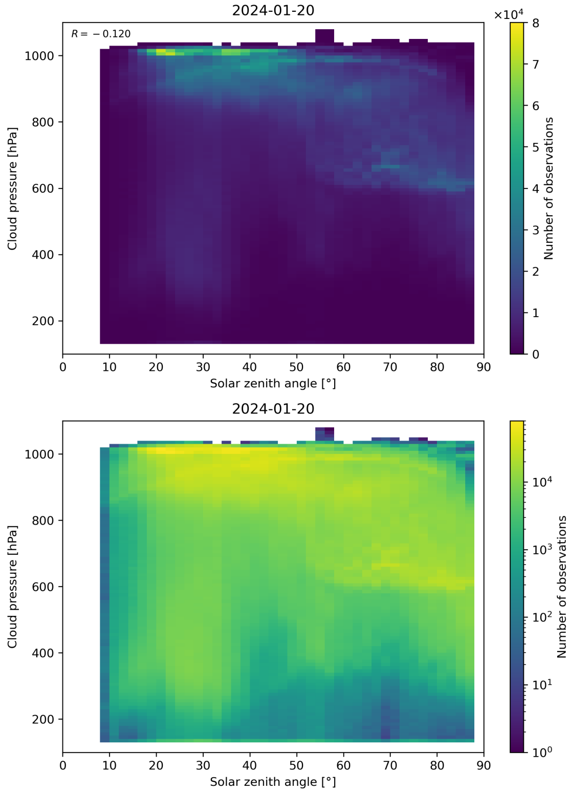
Figure 111: Scatter density plot of “Solar zenith angle” against “Cloud pressure” for 2024-01-19 to 2024-01-21.
