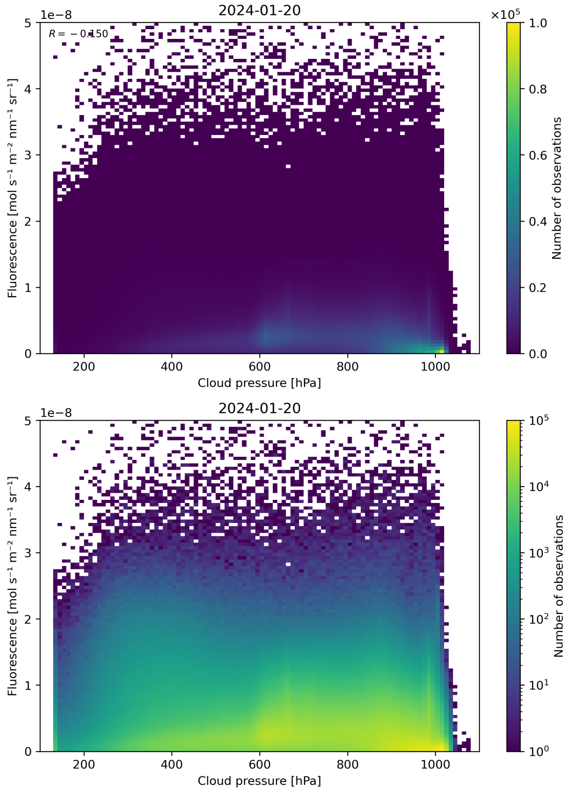
Figure 80: Scatter density plot of “Cloud pressure” against “Fluorescence” for 2024-01-19 to 2024-01-21.
