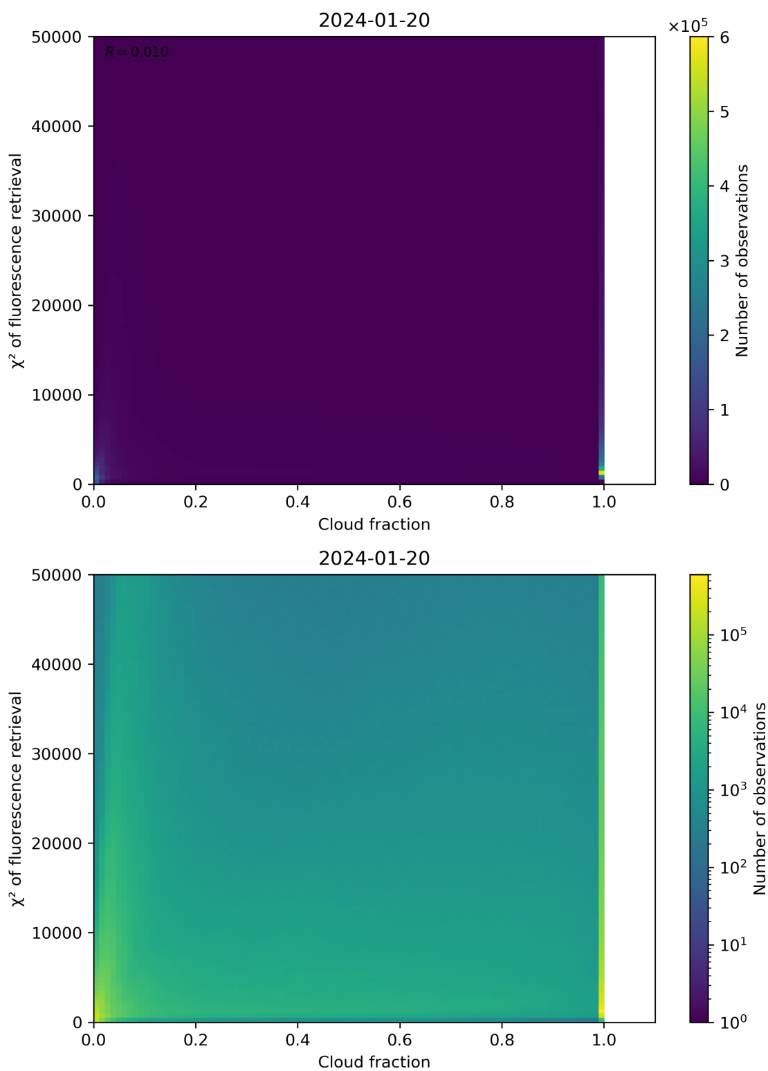
Figure 71: Scatter density plot of “Cloud fraction” against “ \chi^2 of fluorescence retrieval” for 2024-01-19 to 2024-01-21.
