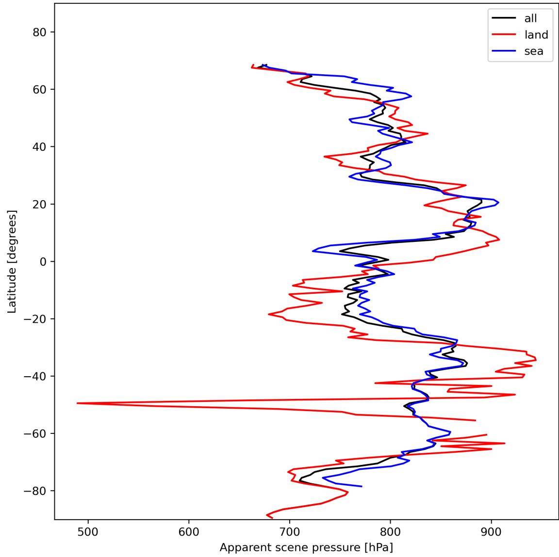
Figure 19: Zonal average of “Apparent scene pressure” for 2024-01-21 to 2024-01-23.
