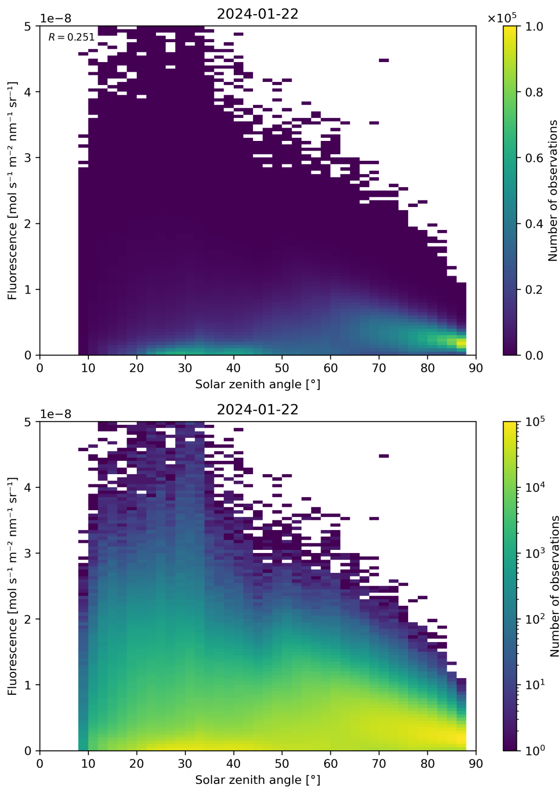
Figure 112: Scatter density plot of “Solar zenith angle” against “Fluorescence” for 2024-01-21 to 2024-01-23.
