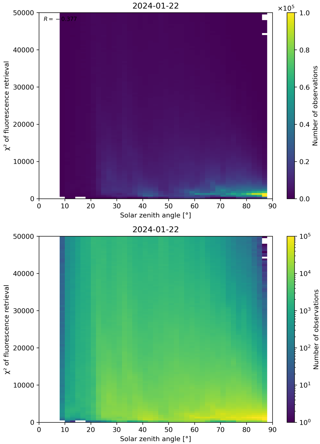
Figure 109: Scatter density plot of “Solar zenith angle” against “ \chi^2 of fluorescence retrieval” for 2024-01-21 to 2024-01-23.
