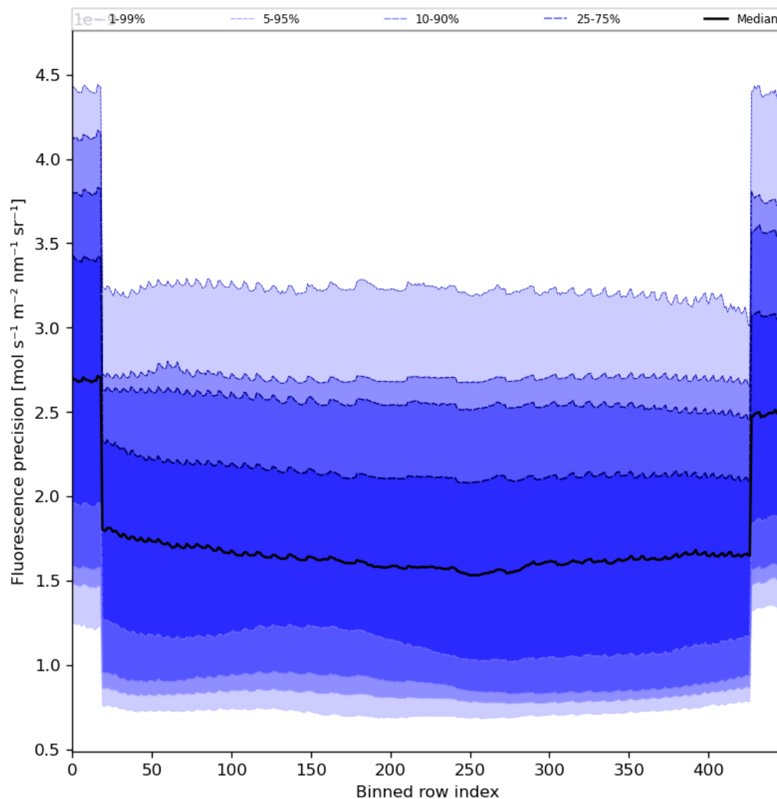
Figure 58: Along track statistics of “Fluorescence precision” for 2024-01-21 to 2024-01-23
