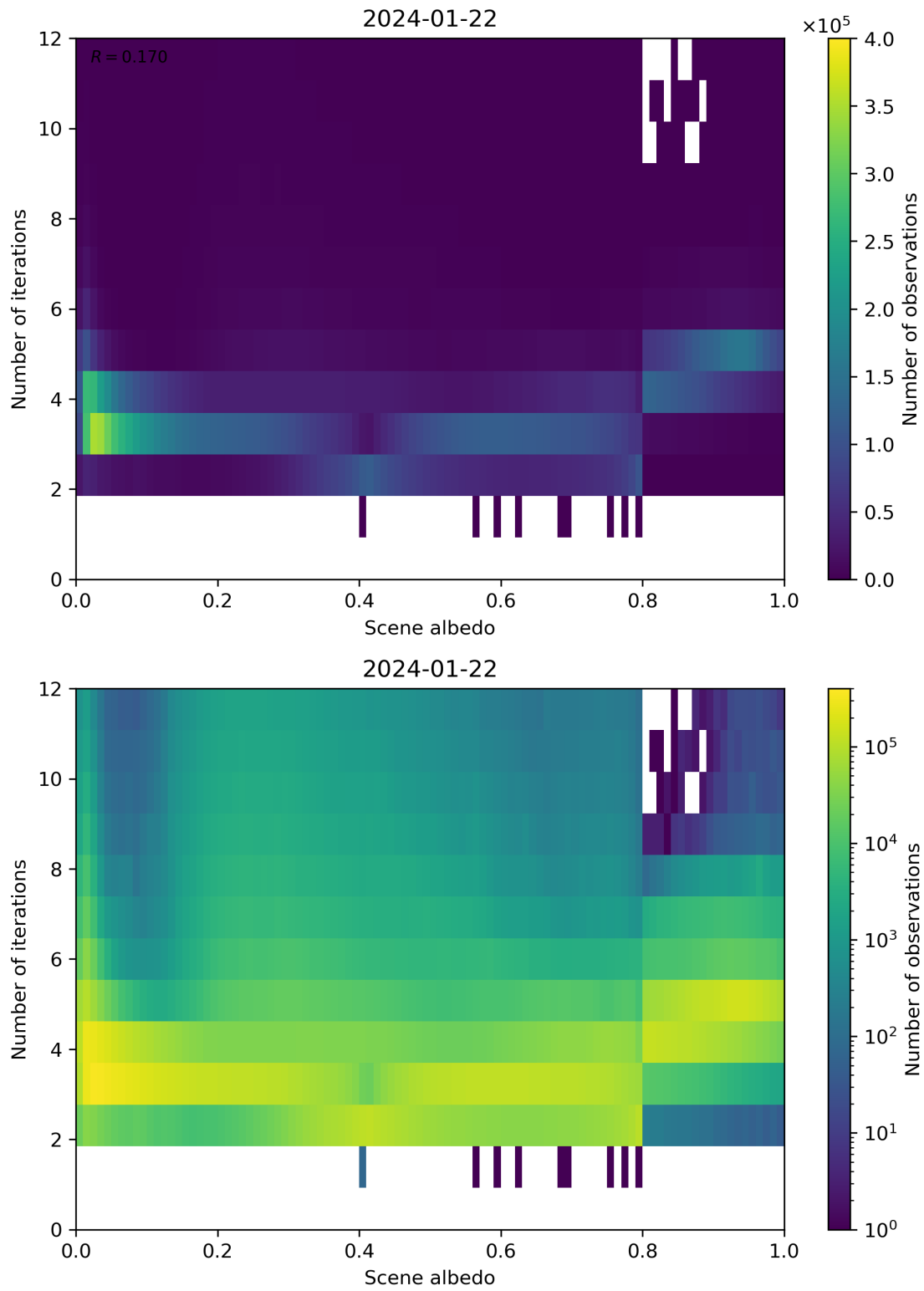
Figure 105: Scatter density plot of “Scene albedo” against “Number of iterations” for 2024-01-21 to 2024-01-23.
