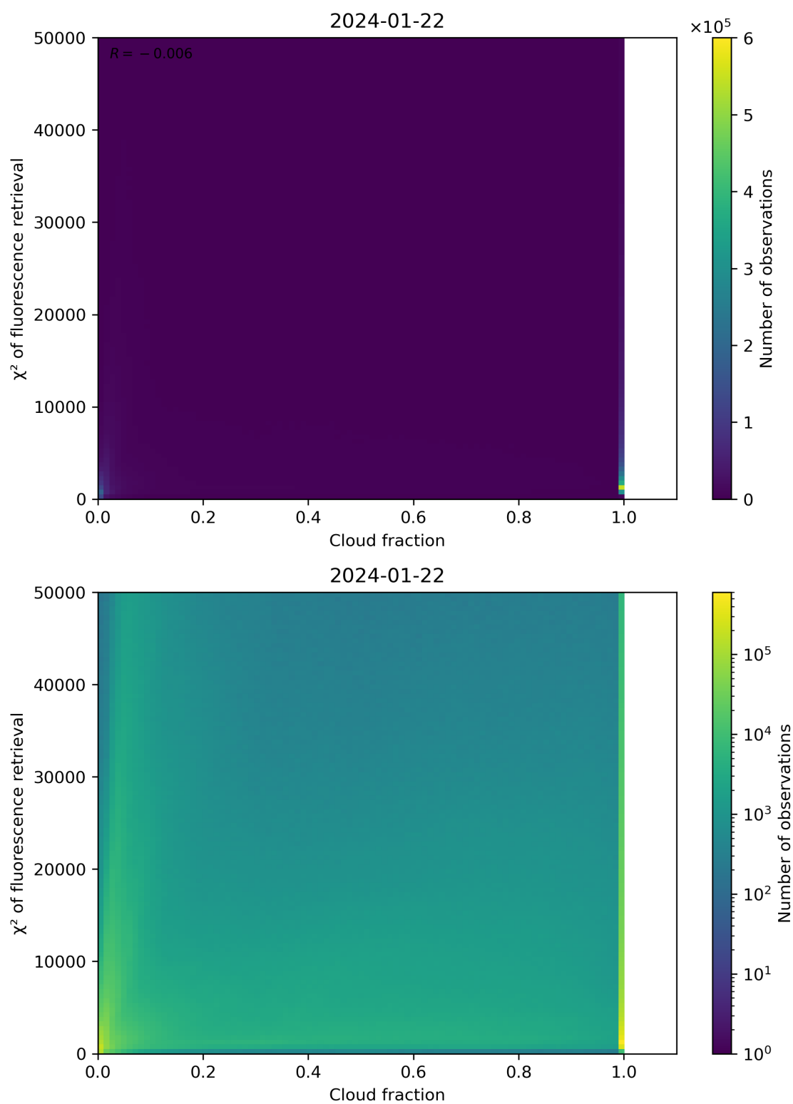
Figure 71: Scatter density plot of “Cloud fraction” against “ \chi^2 of fluorescence retrieval” for 2024-01-21 to 2024-01-23.
