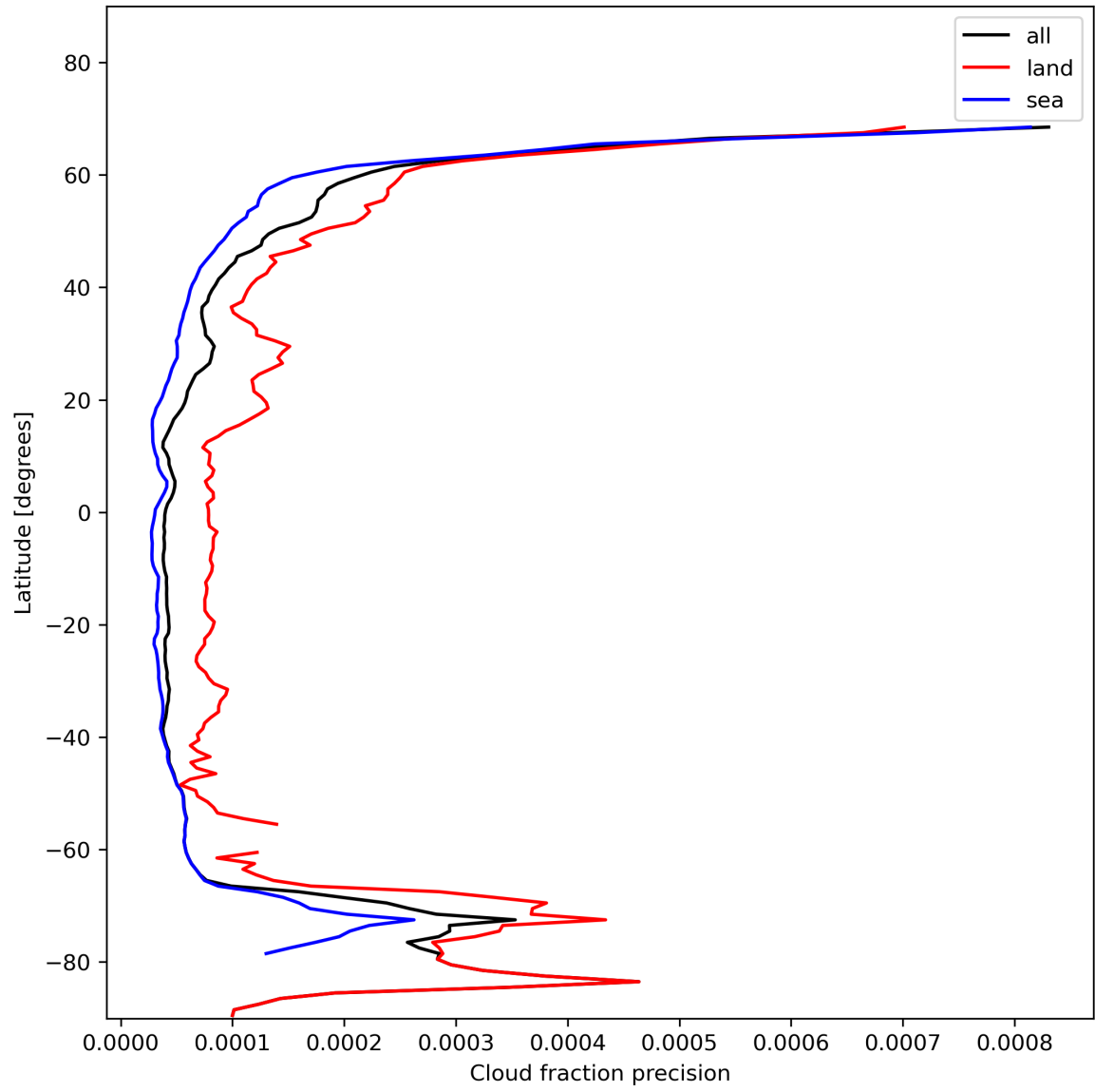
Figure 16: Zonal average of “Cloud fraction precision” for 2024-01-21 to 2024-01-23.
