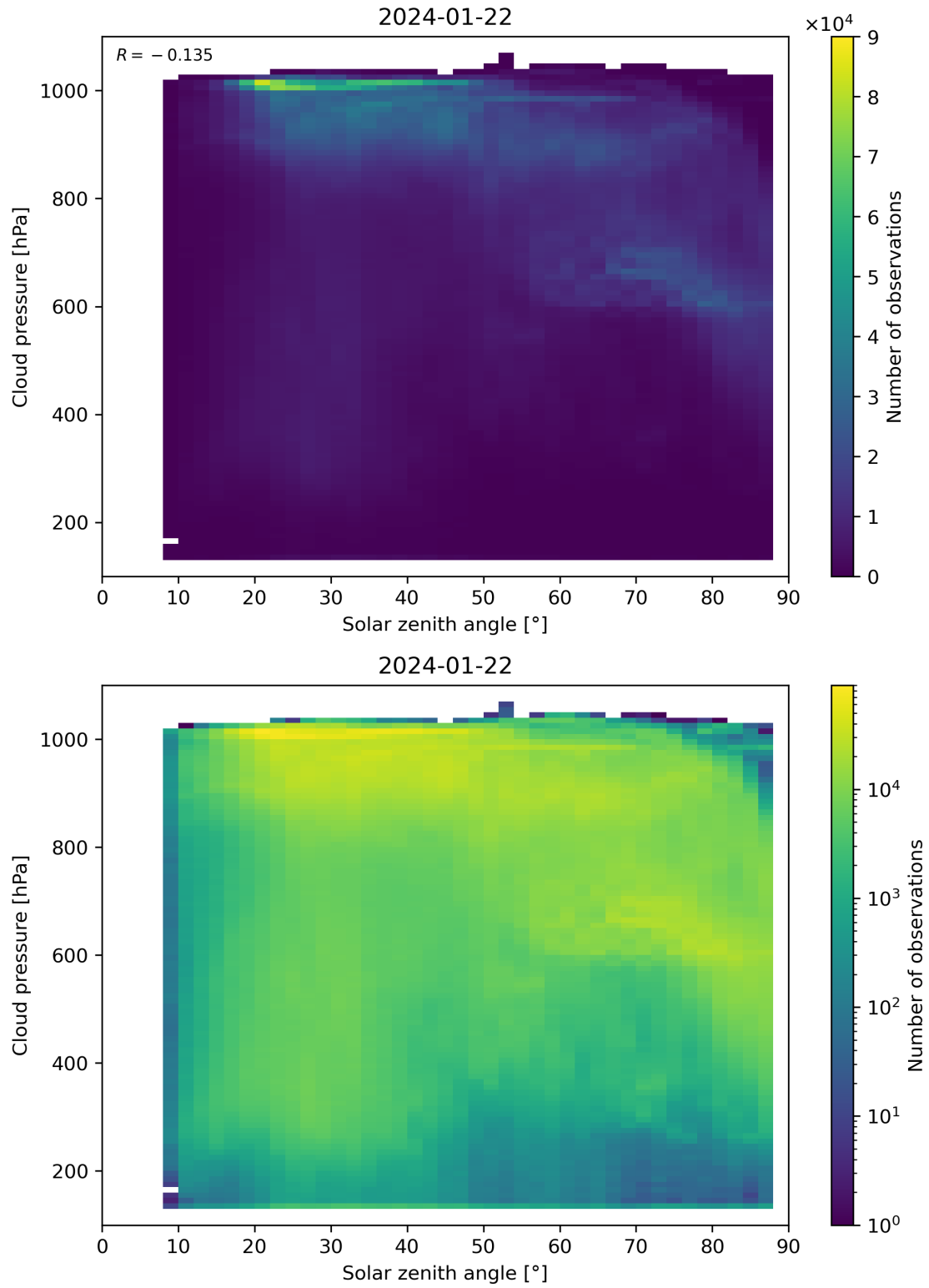
Figure 111: Scatter density plot of “Solar zenith angle” against “Cloud pressure” for 2024-01-21 to 2024-01-23.
