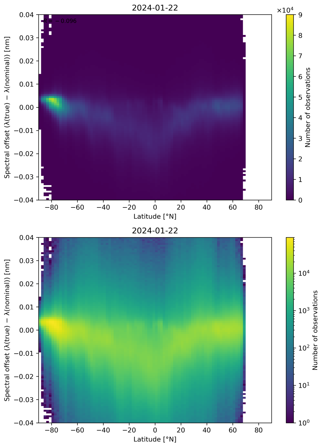
Figure 96: Scatter density plot of “Latitude” against “Spectral offset ( \lambda(\text{true}) - \lambda(\text{nominal}) )” for 2024-01-21 to 2024-01-23.
