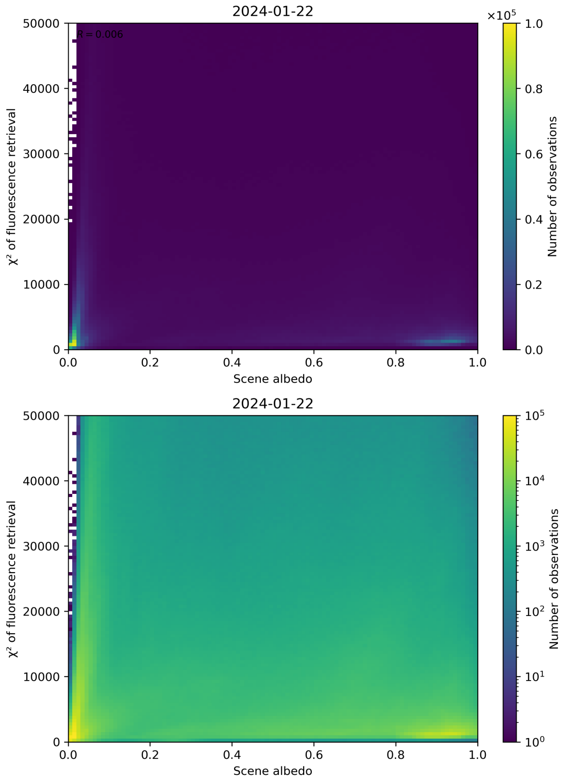
Figure 103: Scatter density plot of “Scene albedo” against “ \chi^2 of fluorescence retrieval” for 2024-01-21 to 2024-01-23.
