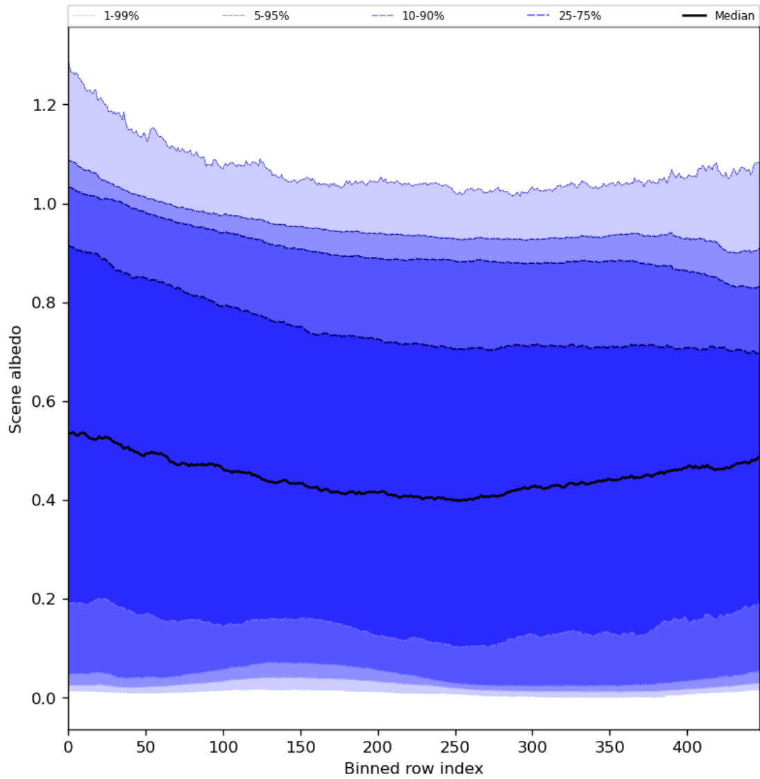
Figure 51: Along track statistics of “Scene albedo” for 2024-01-21 to 2024-01-23
