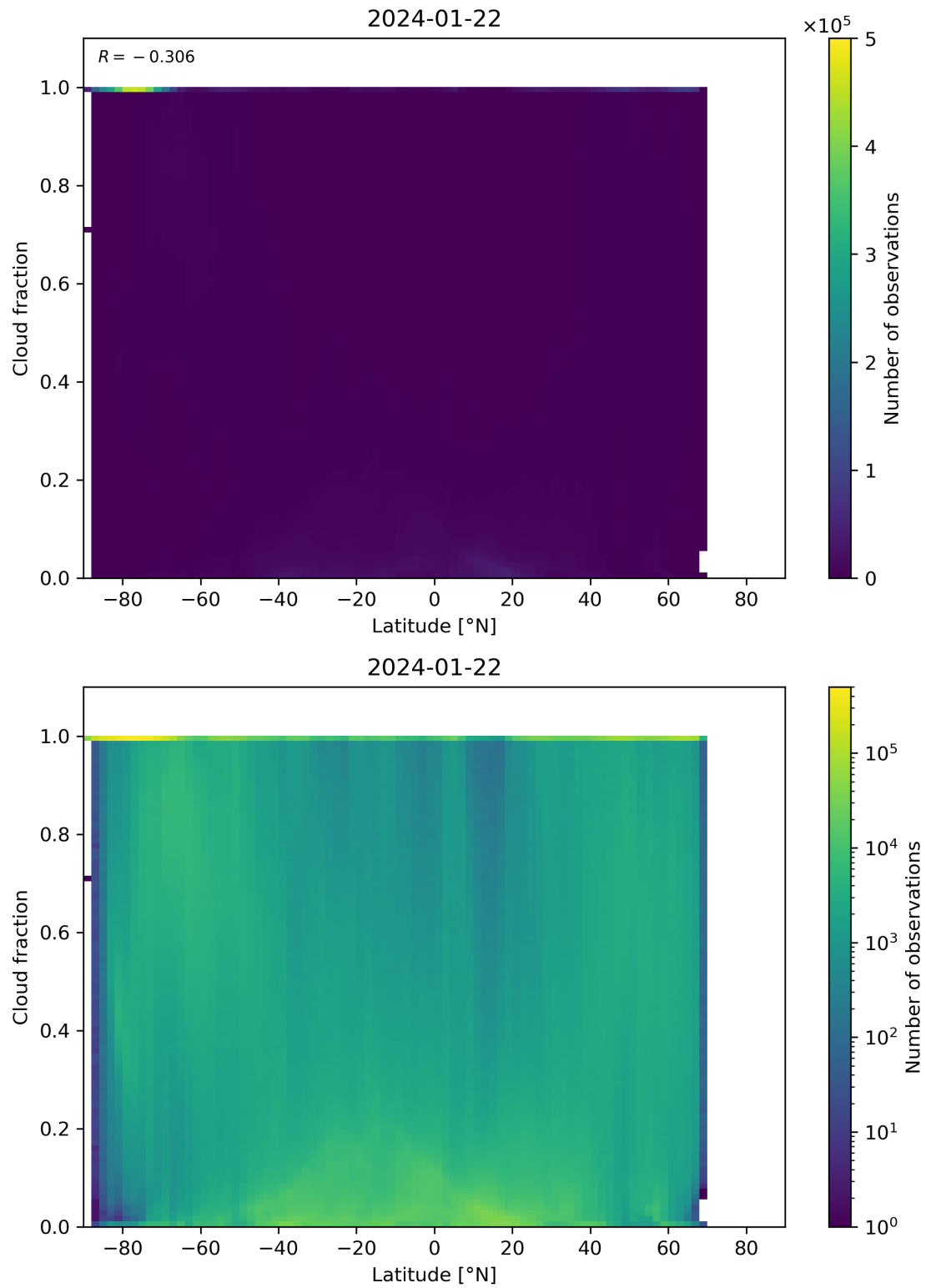
Figure 90: Scatter density plot of “Latitude” against “Cloud fraction” for 2024-01-21 to 2024-01-23.
