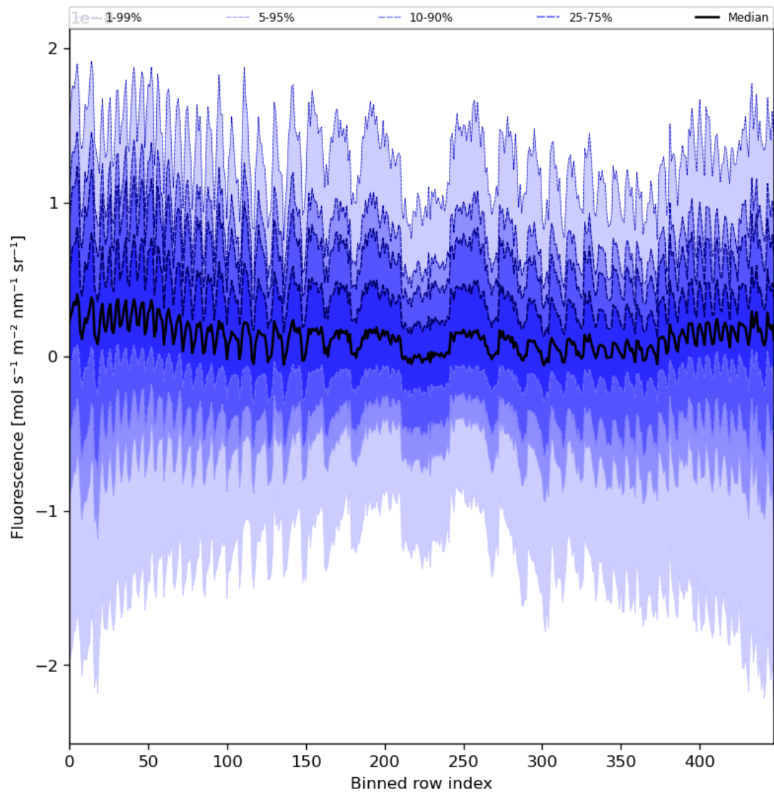
Figure 57: Along track statistics of “Fluorescence” for 2024-01-21 to 2024-01-23
