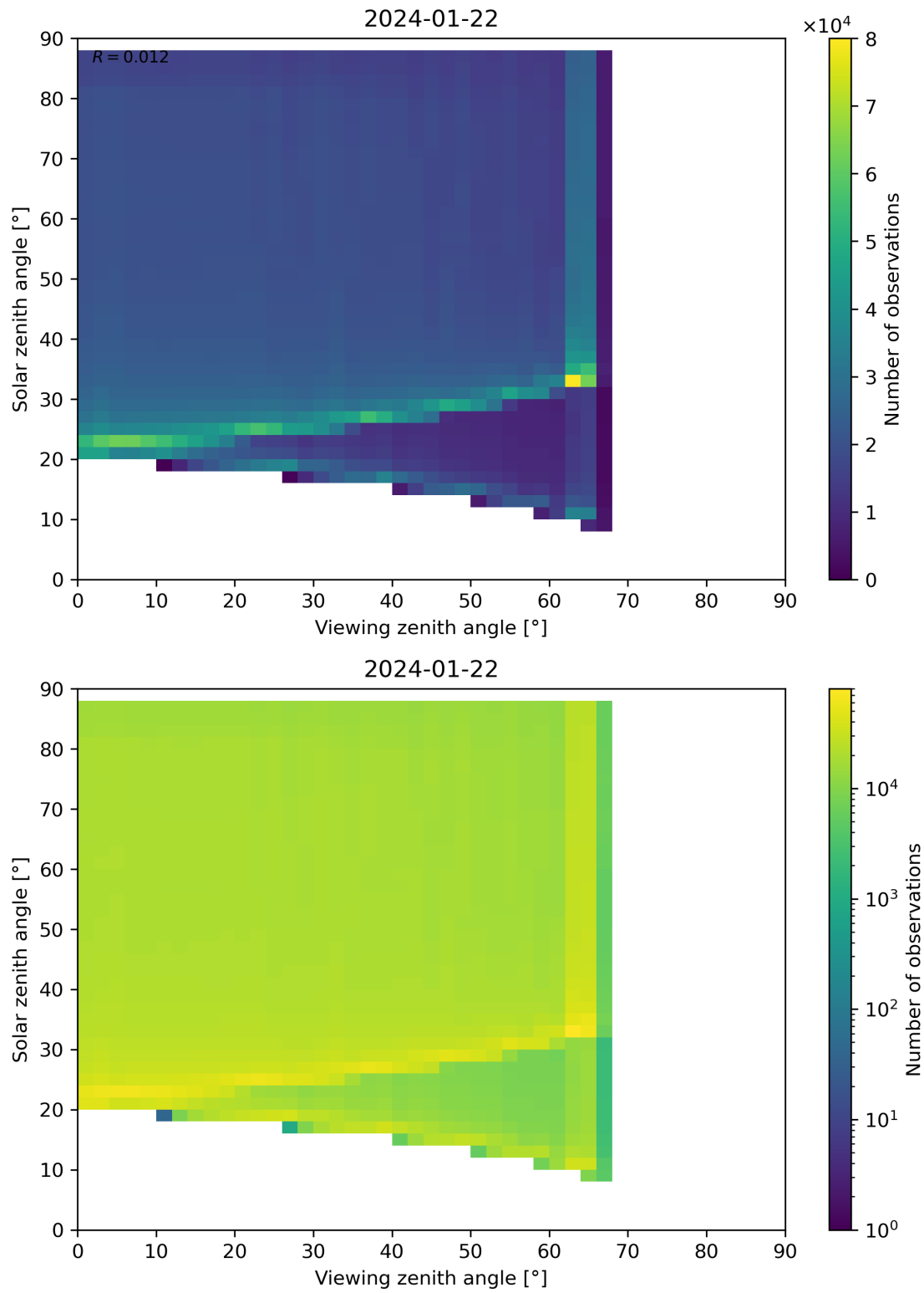
Figure 127: Scatter density plot of “Viewing zenith angle” against “Solar zenith angle” for 2024-01-21 to 2024-01-23.
