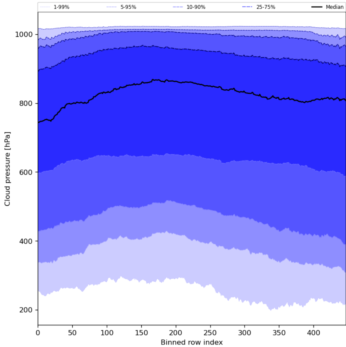
Figure 47: Along track statistics of “Cloud pressure” for 2024-01-21 to 2024-01-23
