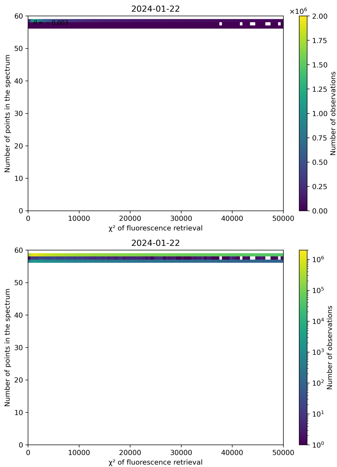
Figure 68: Scatter density plot of " \chi^2 of fluorescence retrieval" against "Number of points in the spectrum" for 2024-01-21 to 2024-01-23.
