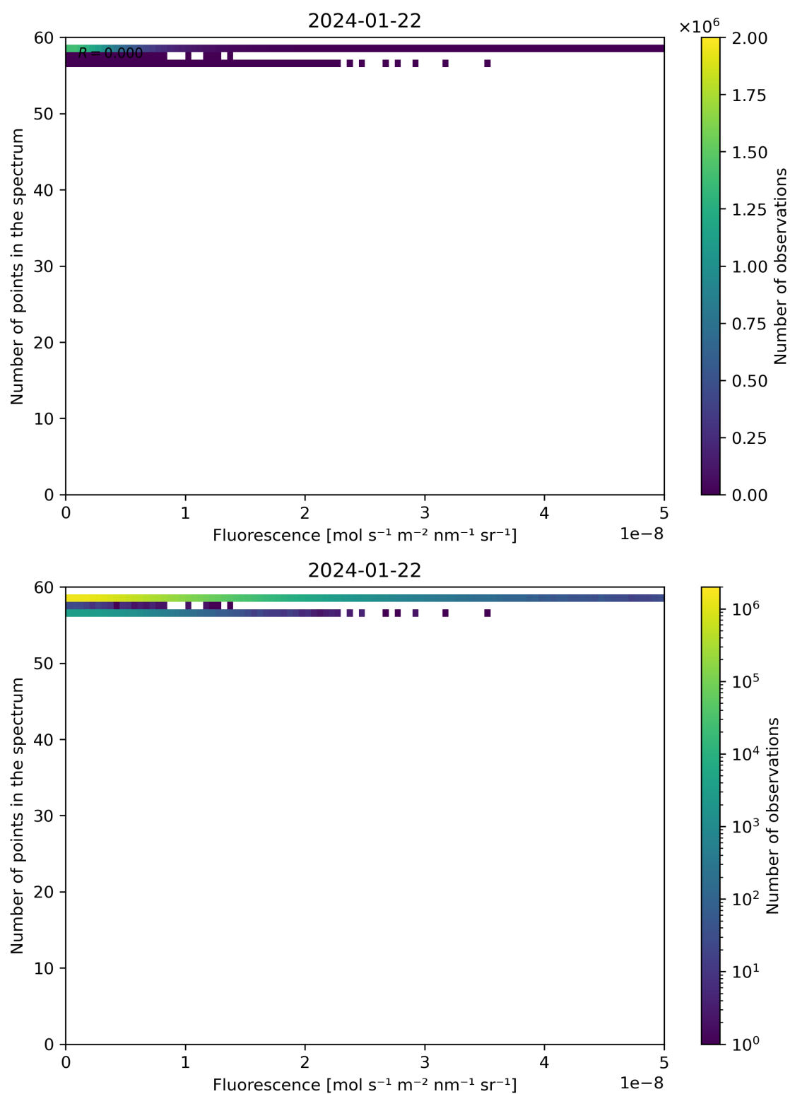
Figure 86: Scatter density plot of “Fluorescence” against “Number of points in the spectrum” for 2024-01-21 to 2024-01-23.
