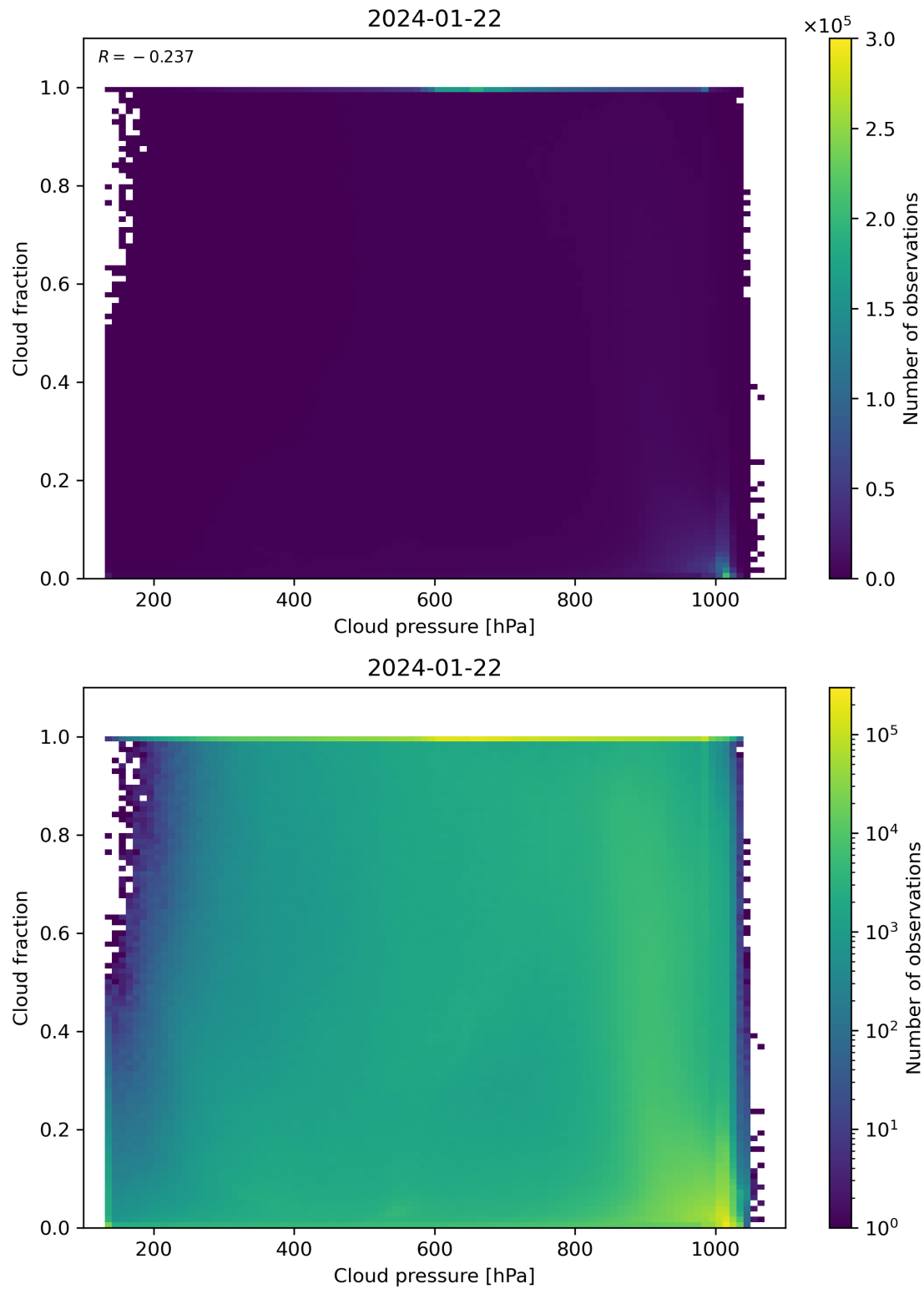
Figure 79: Scatter density plot of “Cloud pressure” against “Cloud fraction” for 2024-01-21 to 2024-01-23.
