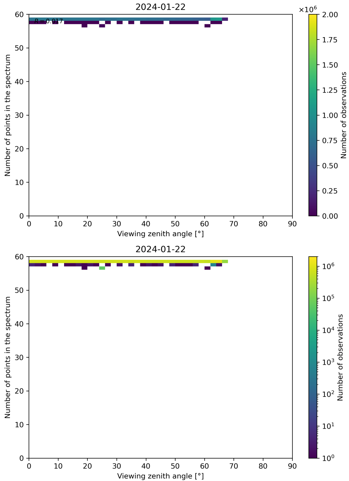
Figure 125: Scatter density plot of “Viewing zenith angle” against “Number of points in the spectrum” for 2024-01-21 to 2024-01-23.
