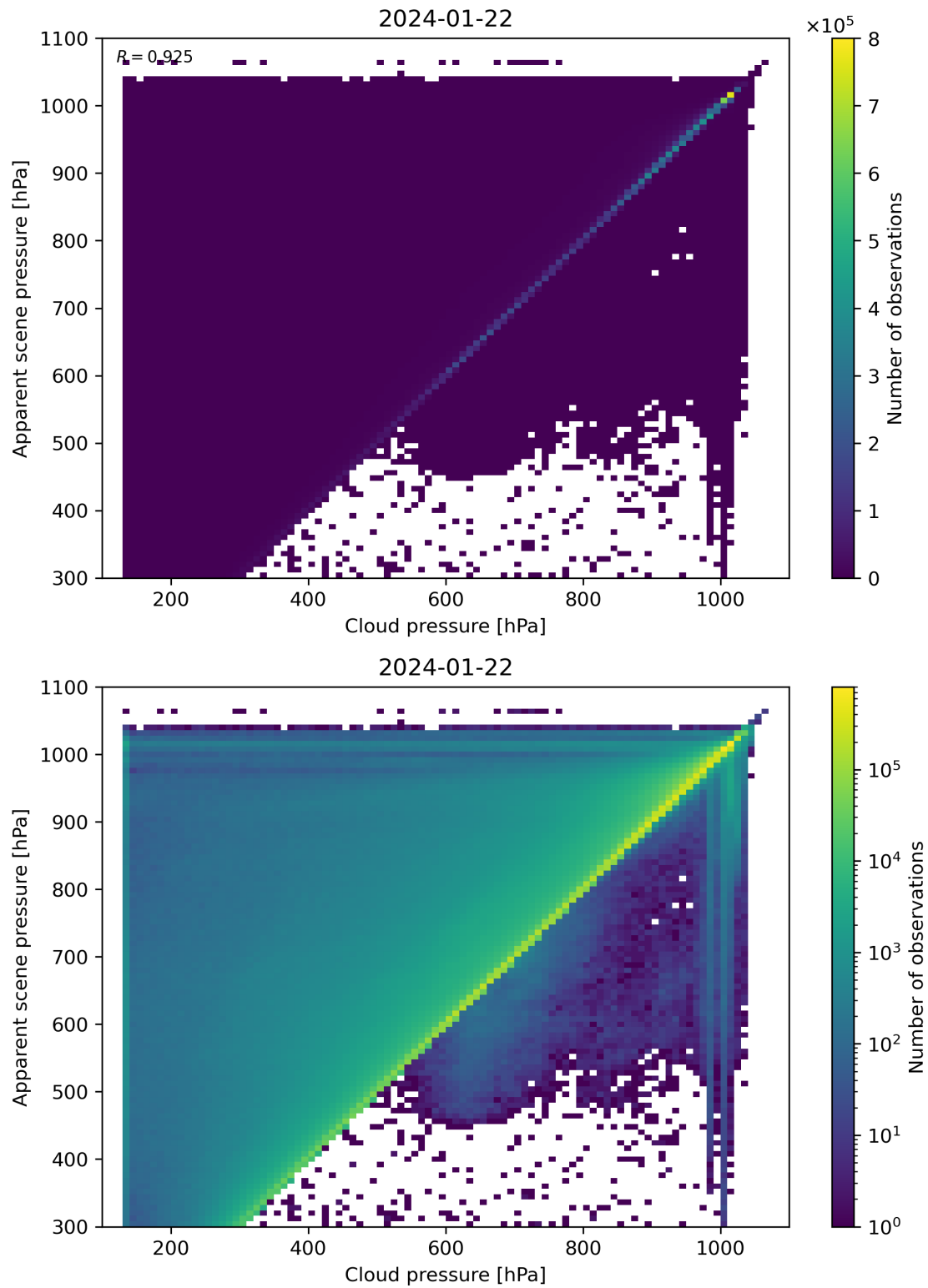
Figure 77: Scatter density plot of “Cloud pressure” against “Apparent scene pressure” for 2024-01-21 to 2024-01-23.
