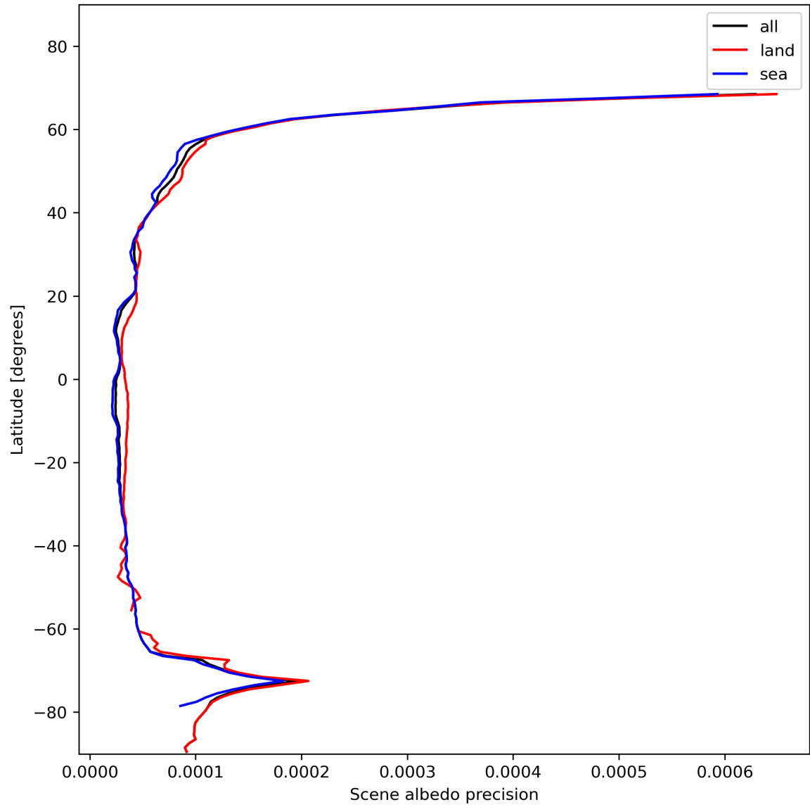
Figure 18: Zonal average of “Scene albedo precision” for 2024-01-21 to 2024-01-23.
