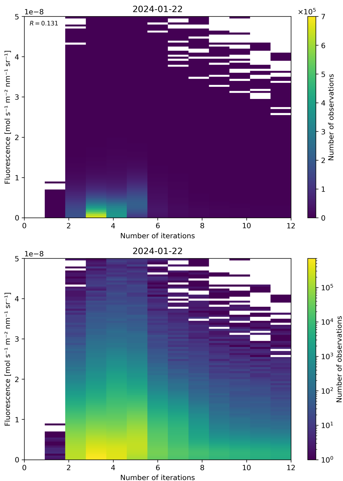
Figure 98: Scatter density plot of “Number of iterations” against “Fluorescence” for 2024-01-21 to 2024-01-23.
