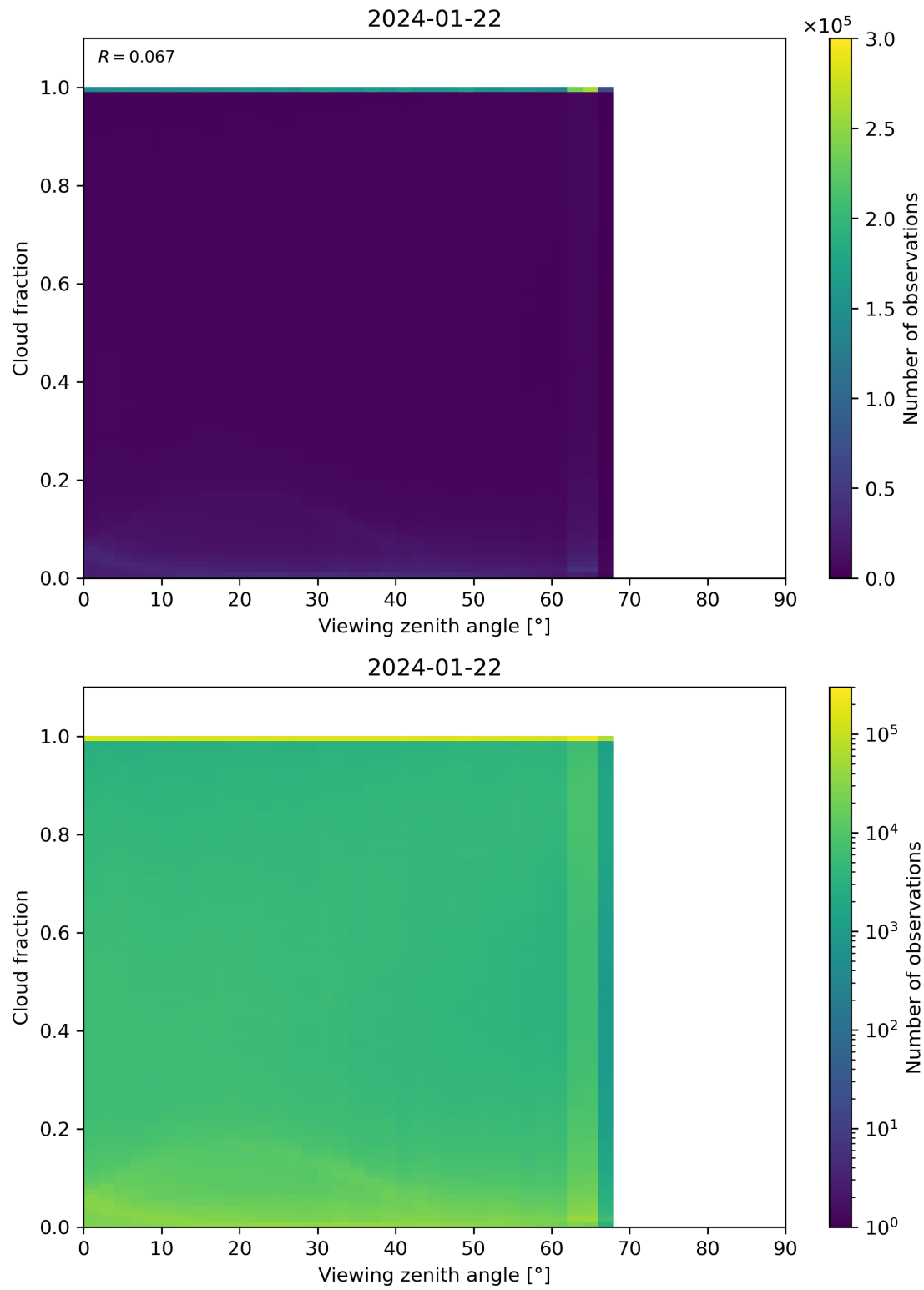
Figure 120: Scatter density plot of “Viewing zenith angle” against “Cloud fraction” for 2024-01-21 to 2024-01-23.
