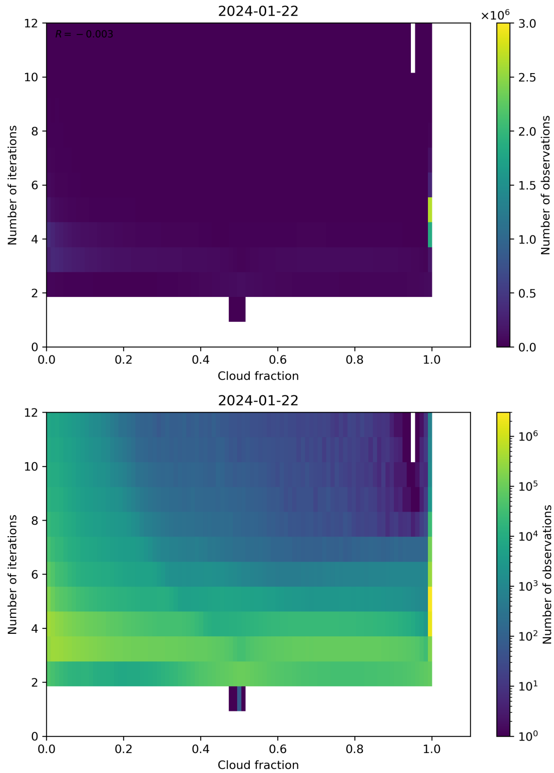
Figure 73: Scatter density plot of “Cloud fraction” against “Number of iterations” for 2024-01-21 to 2024-01-23.
