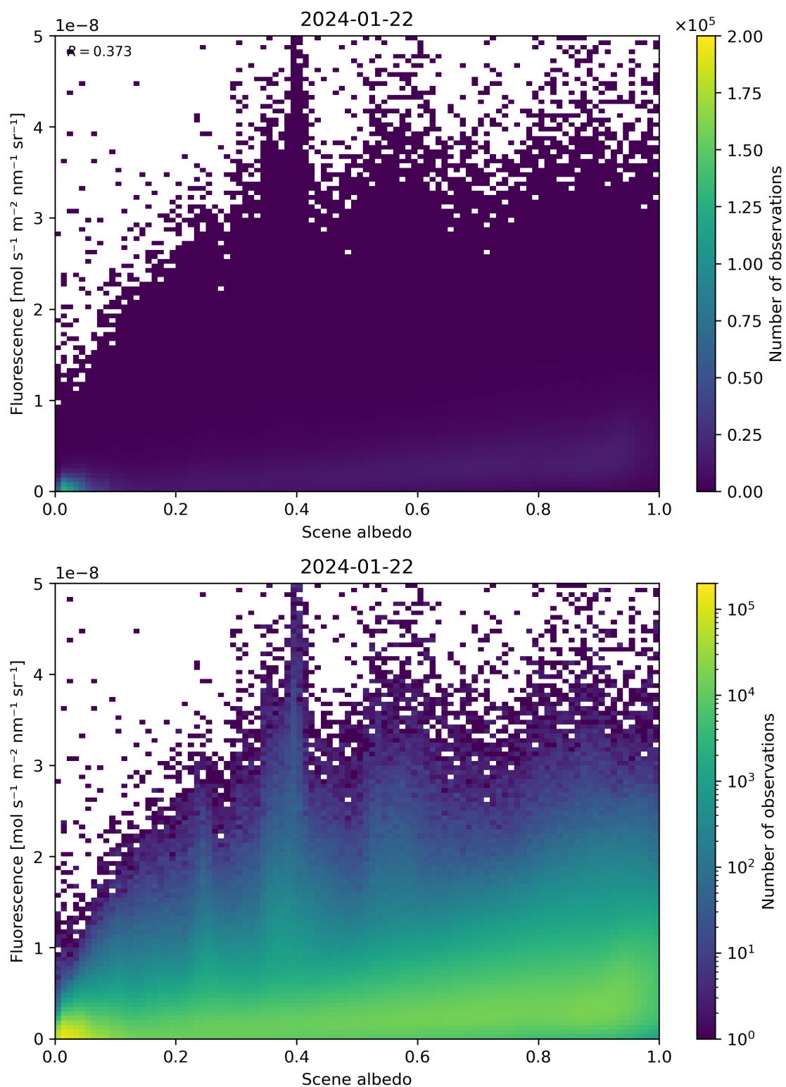
Figure 104: Scatter density plot of “Scene albedo” against “Fluorescence” for 2024-01-21 to 2024-01-23.
