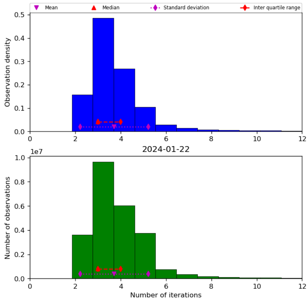
Figure 39: Histogram of “Number of iterations” for 2024-01-21 to 2024-01-23
