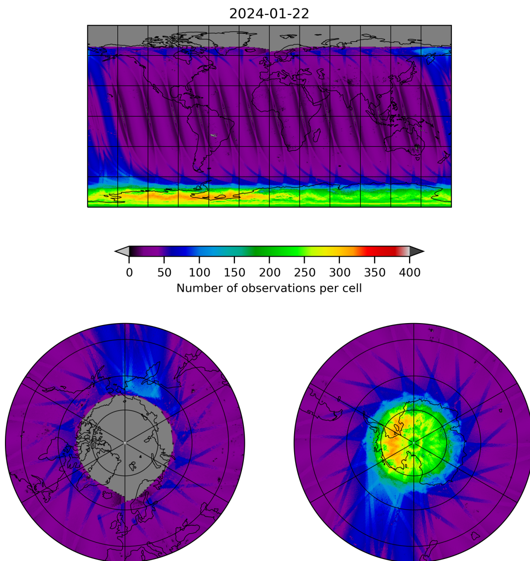
Figure 11: Map of the number of observations for 2024-01-21 to 2024-01-23
