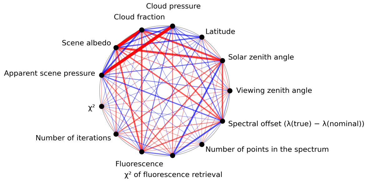
Figure 1: Map of correlation graph for 2024-01-21 to 2024-01-23.
