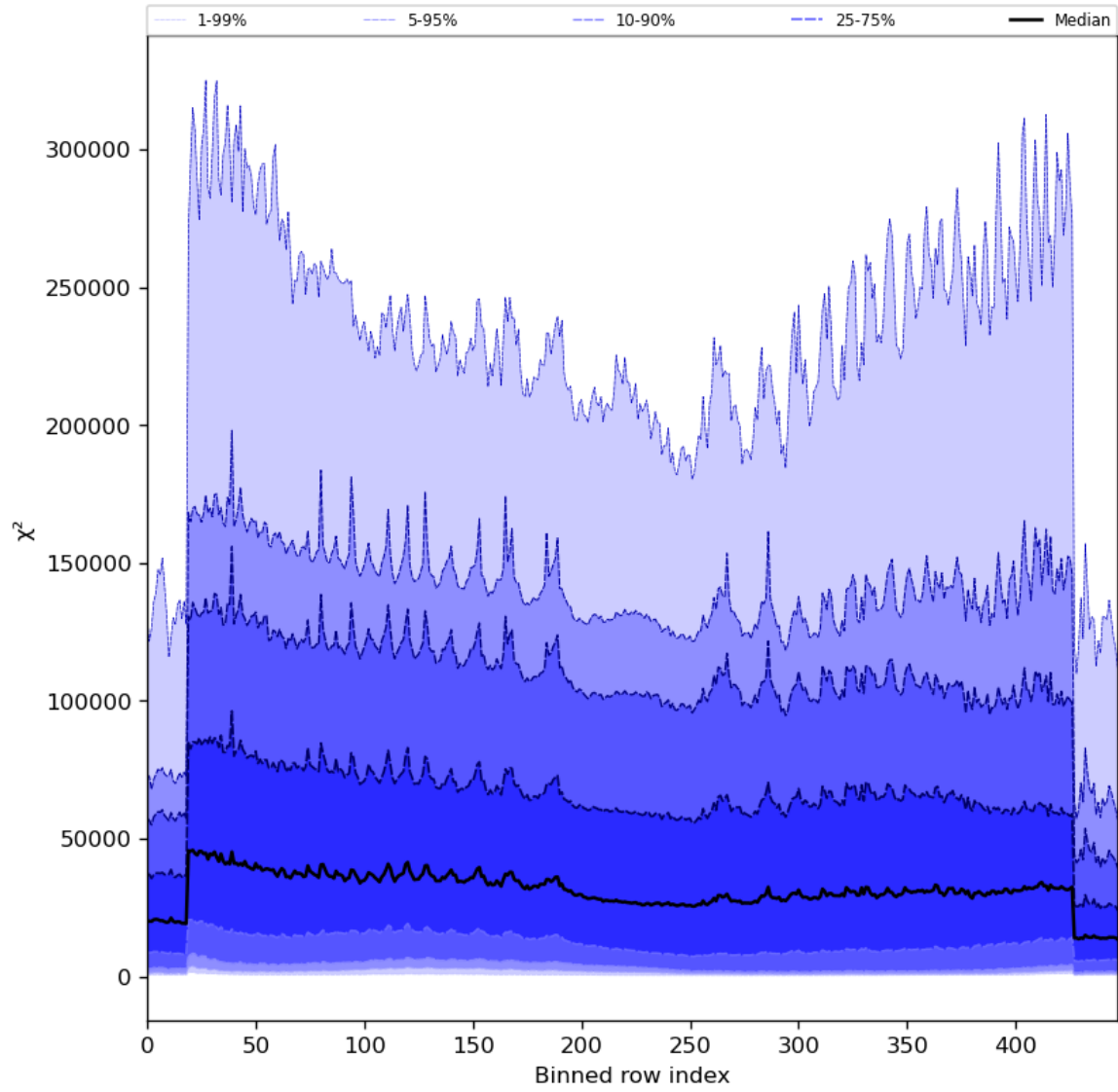
Figure 55: Along track statistics of “ \chi^2 ” for 2024-01-21 to 2024-01-23
