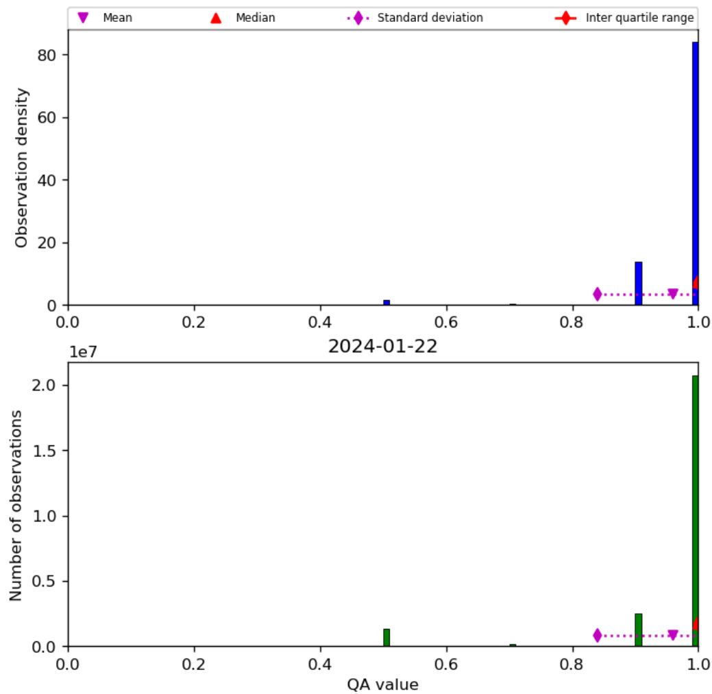
Figure 29: Histogram of “QA value” for 2024-01-21 to 2024-01-23
