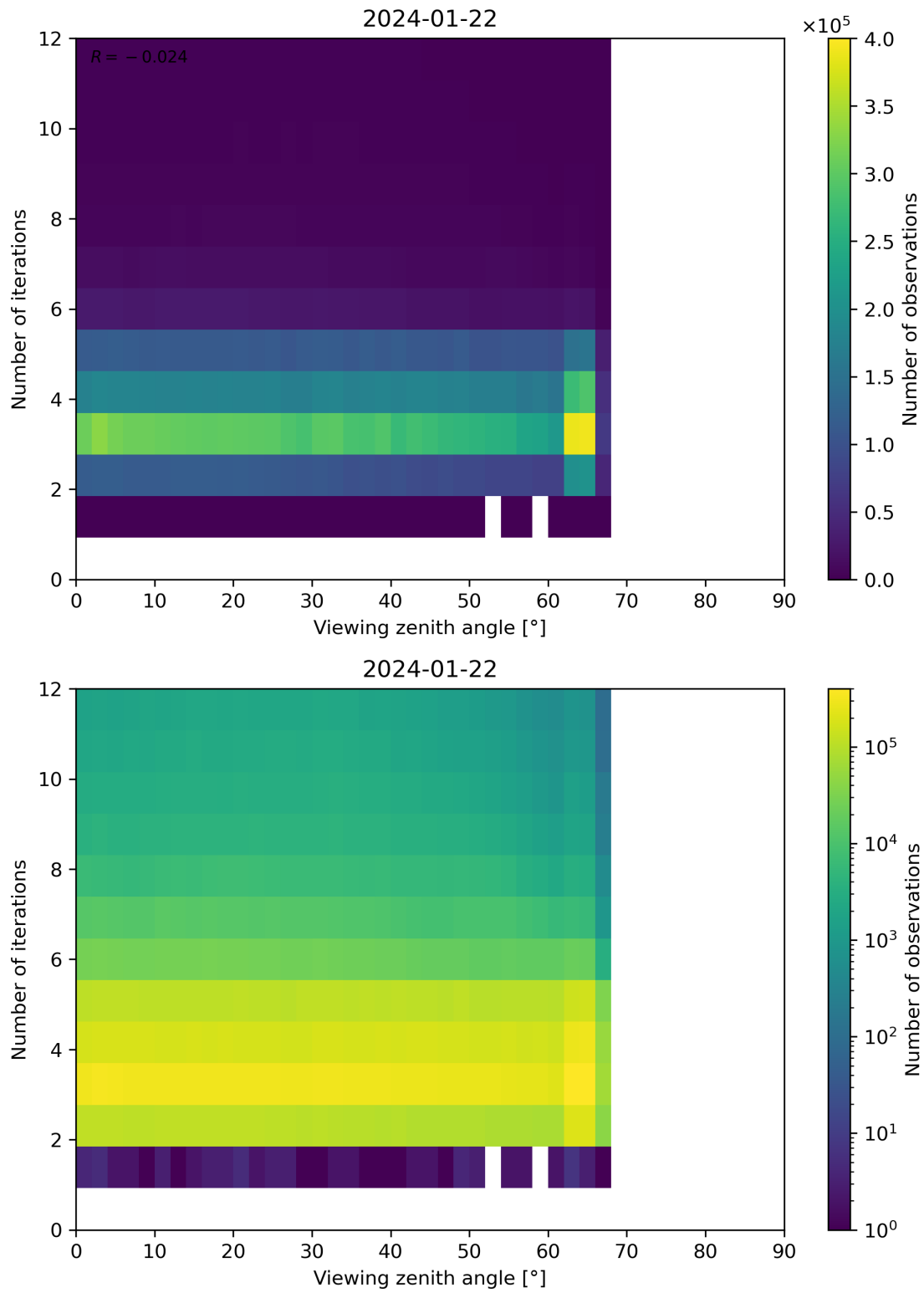
Figure 124: Scatter density plot of “Viewing zenith angle” against “Number of iterations” for 2024-01-21 to 2024-01-23.
