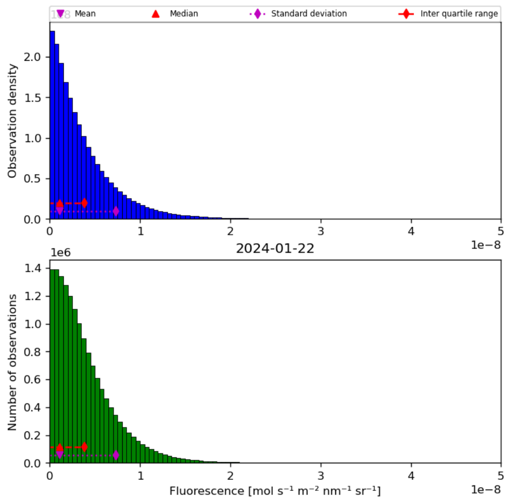
Figure 40: Histogram of “Fluorescence” for 2024-01-21 to 2024-01-23
