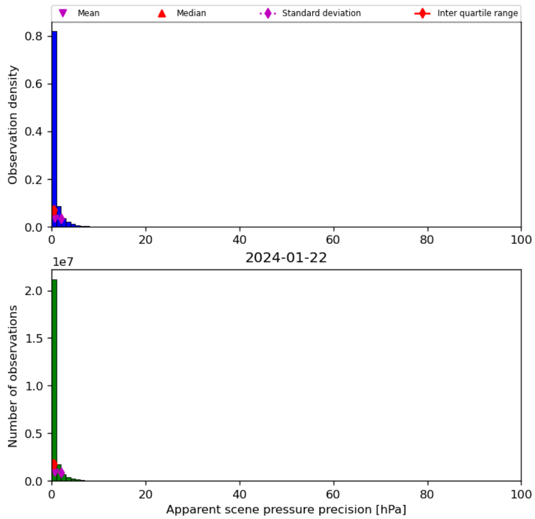
Figure 37: Histogram of “Apparent scene pressure precision” for 2024-01-21 to 2024-01-23
