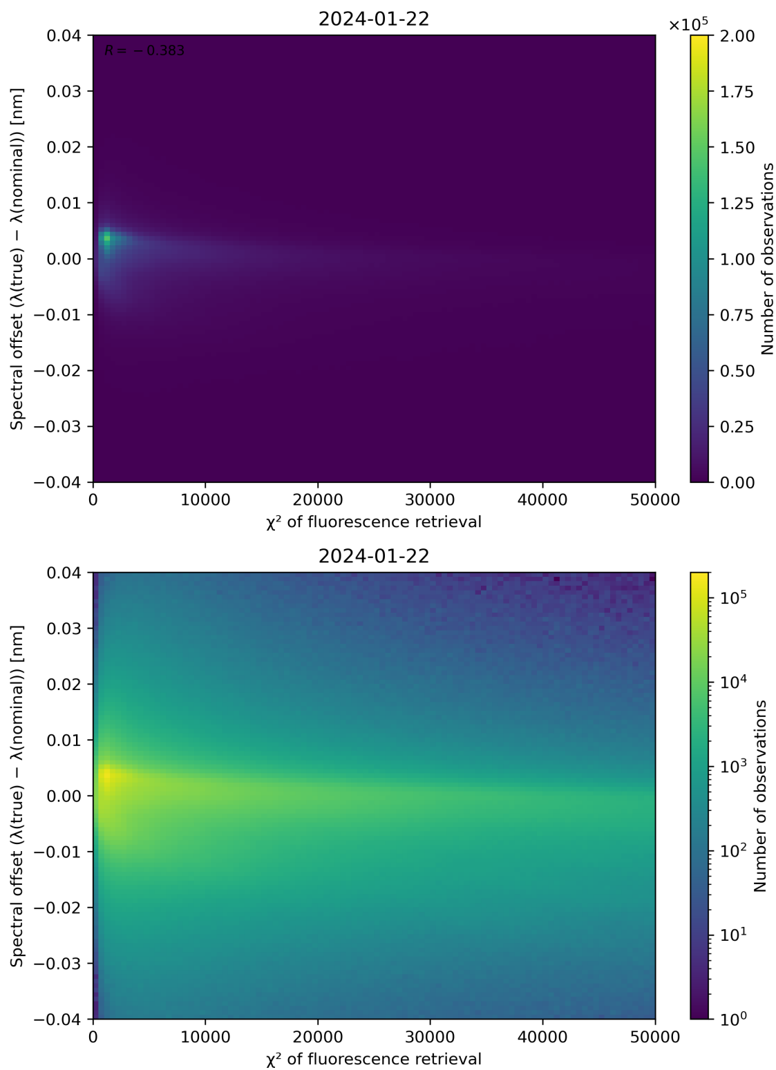
Figure 69: Scatter density plot of " \chi^2 of fluorescence retrieval" against "Spectral offset ( \lambda(\text{true}) - \lambda(\text{nominal}) )" for 2024-01-21 to 2024-01-23.
