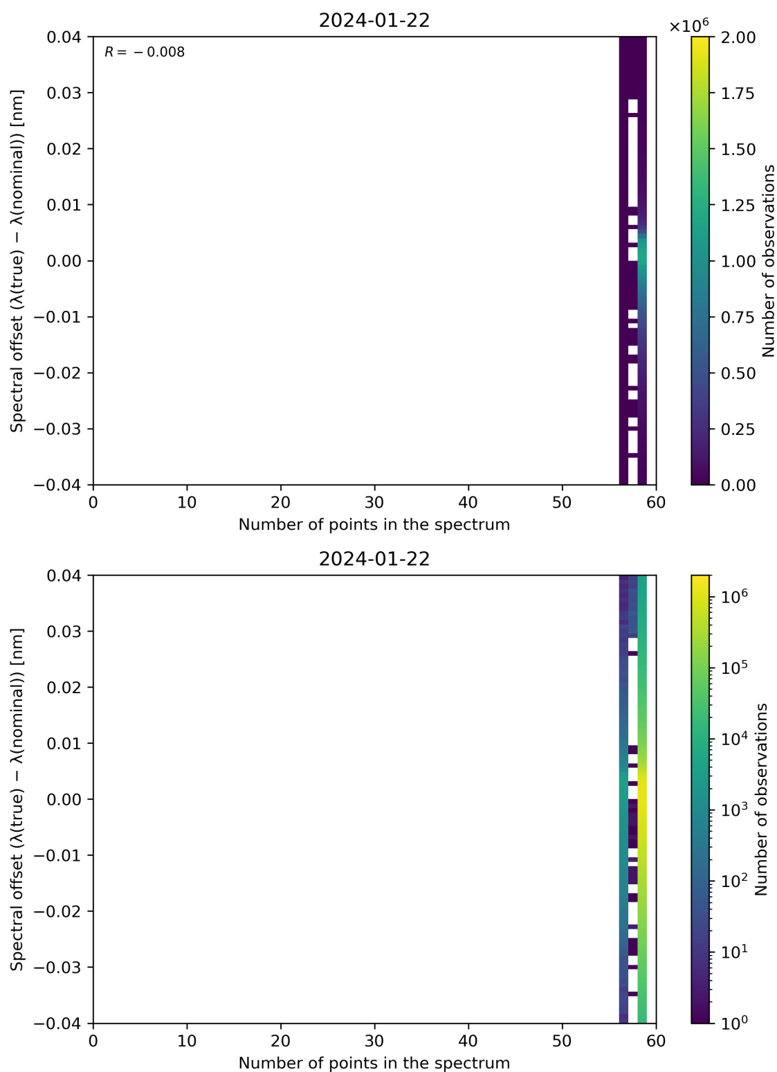
Figure 101: Scatter density plot of “Number of points in the spectrum” against “Spectral offset ( \lambda(\text{true}) - \lambda(\text{nominal}) )” for 2024-01-21 to 2024-01-23.
