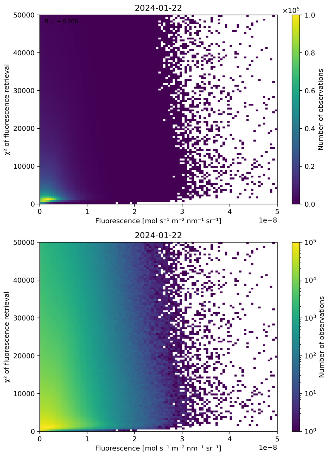
Figure 85: Scatter density plot of “Fluorescence” against “ \chi^2 of fluorescence retrieval” for 2024-01-21 to 2024-01-23.
