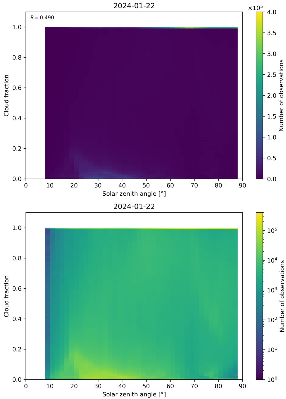
Figure 110: Scatter density plot of “Solar zenith angle” against “Cloud fraction” for 2024-01-21 to 2024-01-23.
