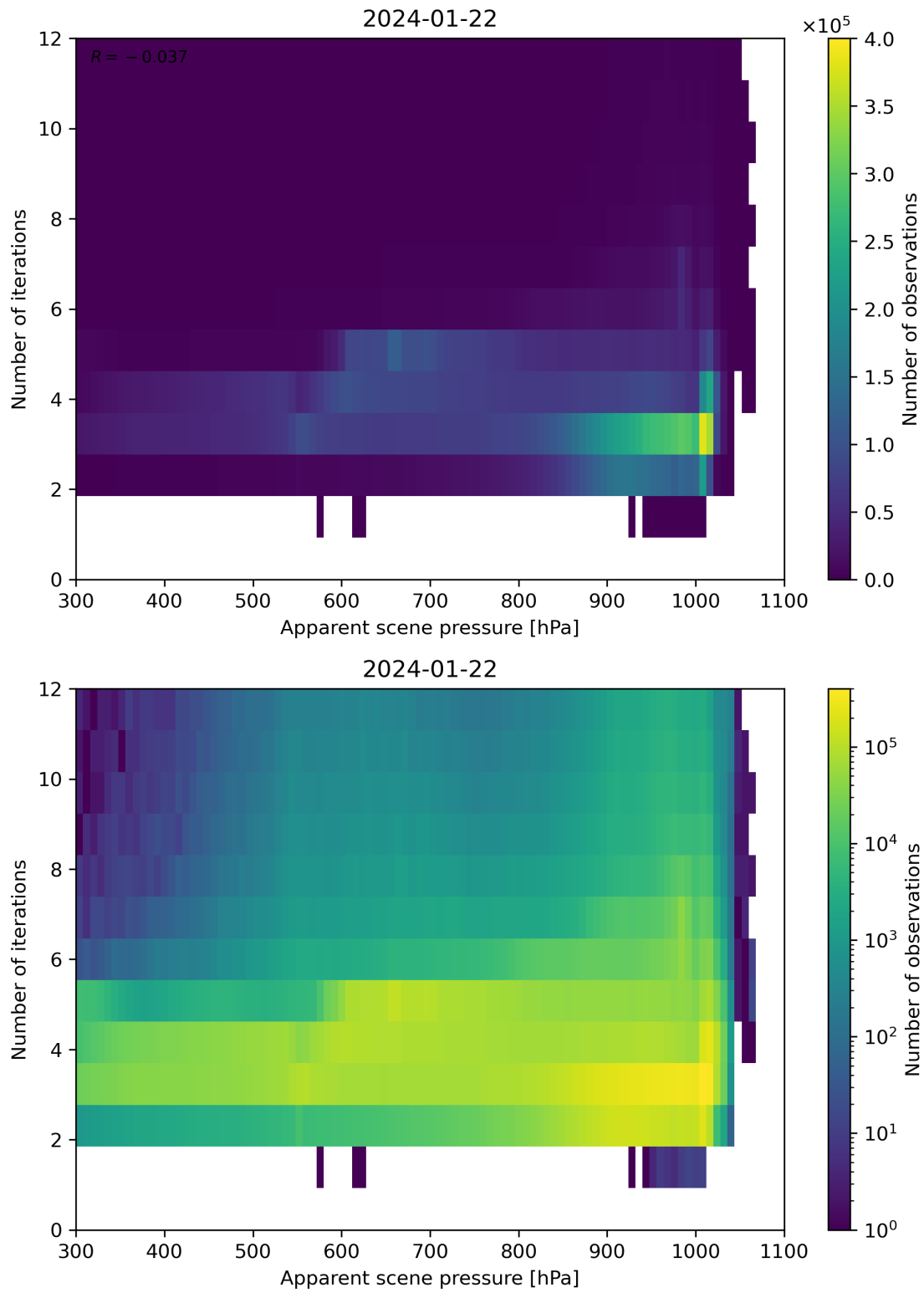
Figure 65: Scatter density plot of “Apparent scene pressure” against “Number of iterations” for 2024-01-21 to 2024-01-23.
