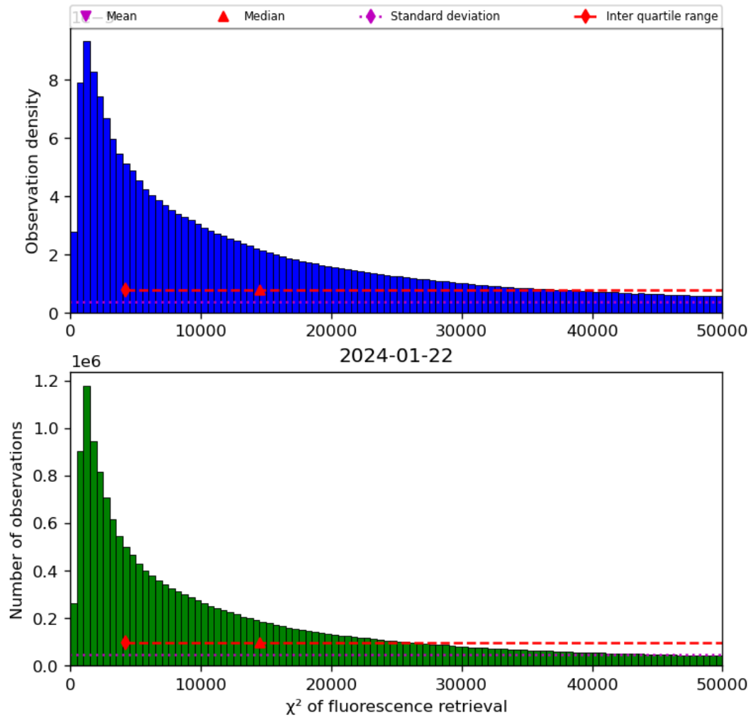
Figure 42: Histogram of “ \chi^2 of fluorescence retrieval” for 2024-01-21 to 2024-01-23
