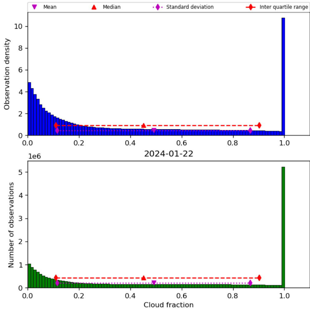
Figure 32: Histogram of “Cloud fraction” for 2024-01-21 to 2024-01-23
