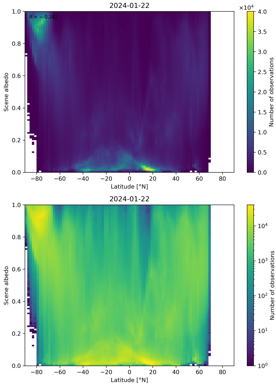
Figure 95: Scatter density plot of “Latitude” against “Scene albedo” for 2024-01-21 to 2024-01-23.
