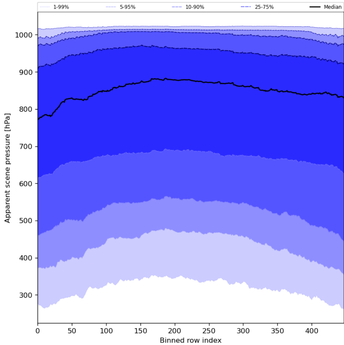
Figure 53: Along track statistics of “Apparent scene pressure” for 2024-01-21 to 2024-01-23
