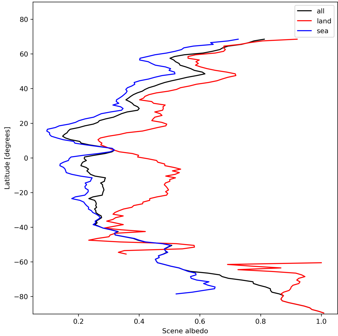
Figure 17: Zonal average of “Scene albedo” for 2024-01-21 to 2024-01-23.
