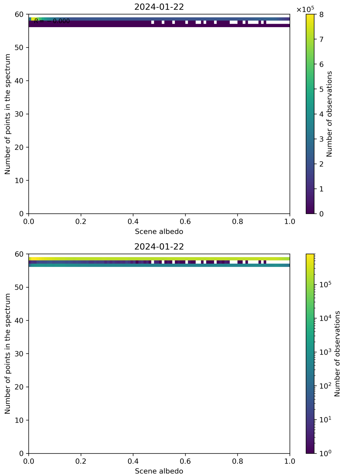
Figure 106: Scatter density plot of “Scene albedo” against “Number of points in the spectrum” for 2024-01-21 to 2024-01-23.
