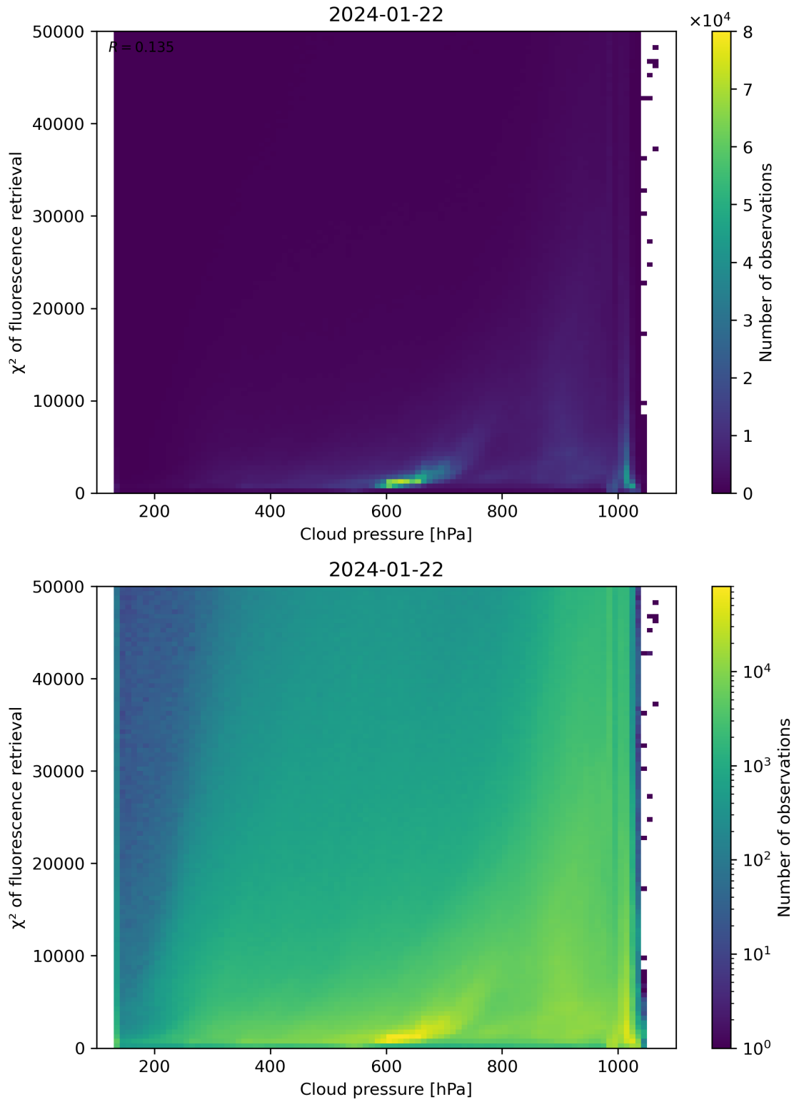
Figure 78: Scatter density plot of “Cloud pressure” against “ \chi^2 of fluorescence retrieval” for 2024-01-21 to 2024-01-23.
