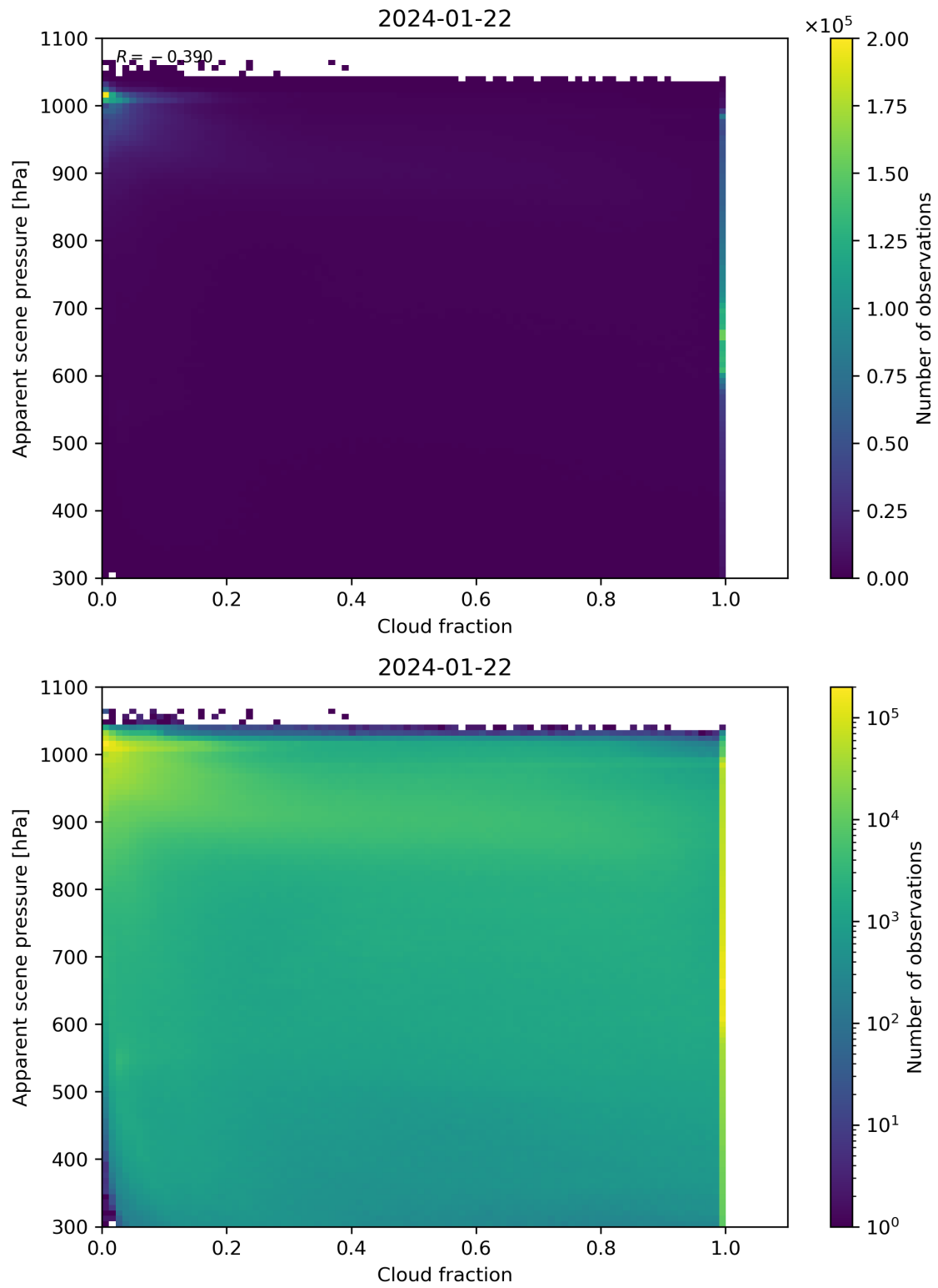
Figure 70: Scatter density plot of “Cloud fraction” against “Apparent scene pressure” for 2024-01-21 to 2024-01-23.
