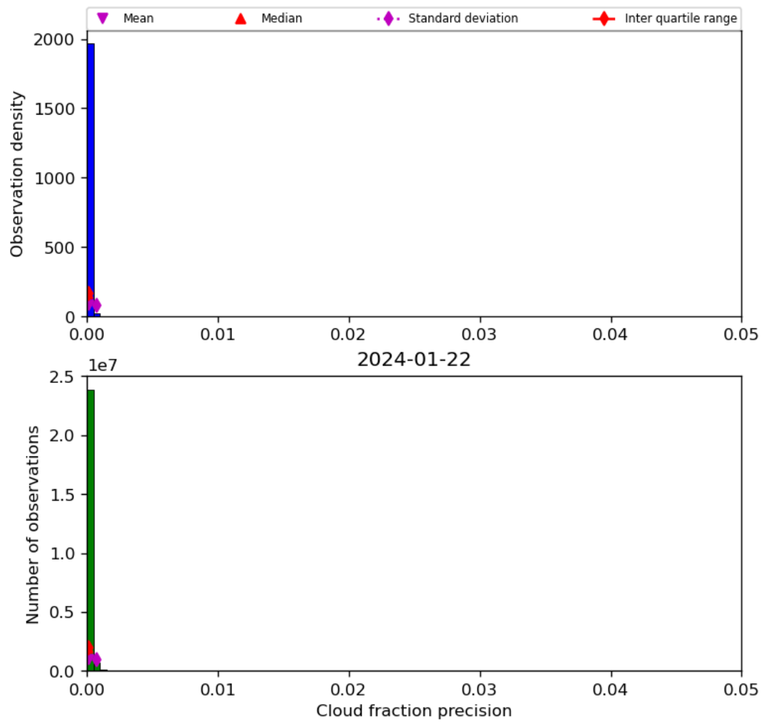
Figure 33: Histogram of “Cloud fraction precision” for 2024-01-21 to 2024-01-23
