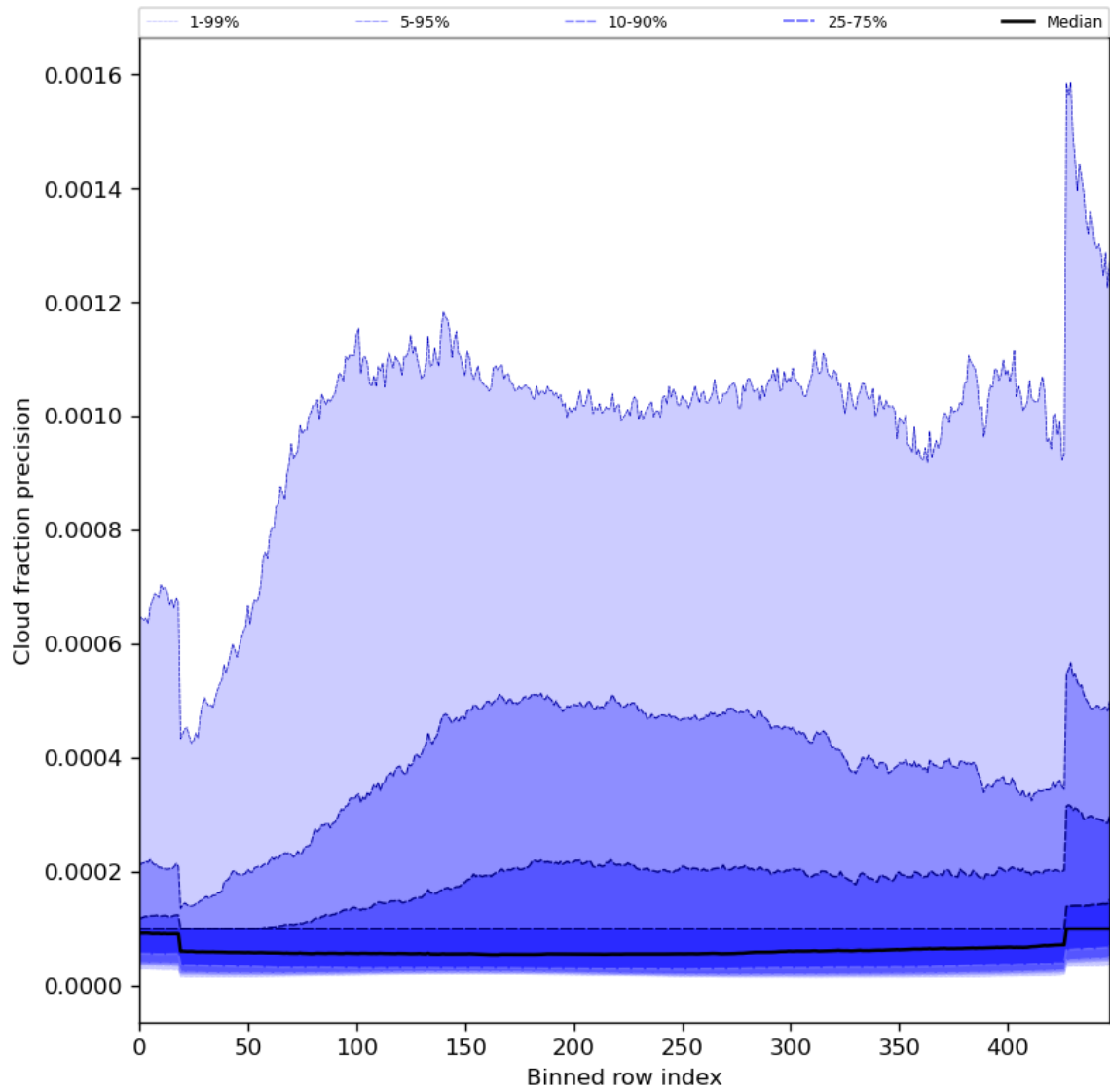
Figure 50: Along track statistics of “Cloud fraction precision” for 2024-01-21 to 2024-01-23
