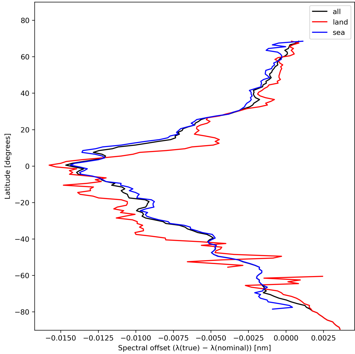
Figure 28: Zonal average of “Spectral offset ( \lambda(\text{true}) - \lambda(\text{nominal}) )” for 2024-01-21 to 2024-01-23.
