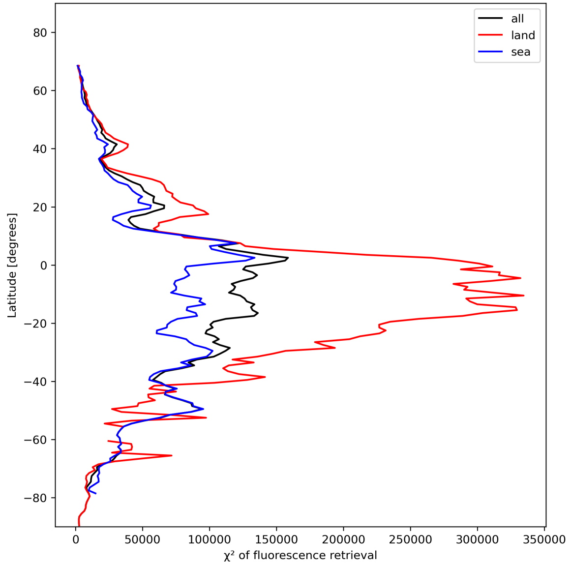
Figure 25: Zonal average of “ \chi^2 of fluorescence retrieval” for 2024-01-21 to 2024-01-23.
