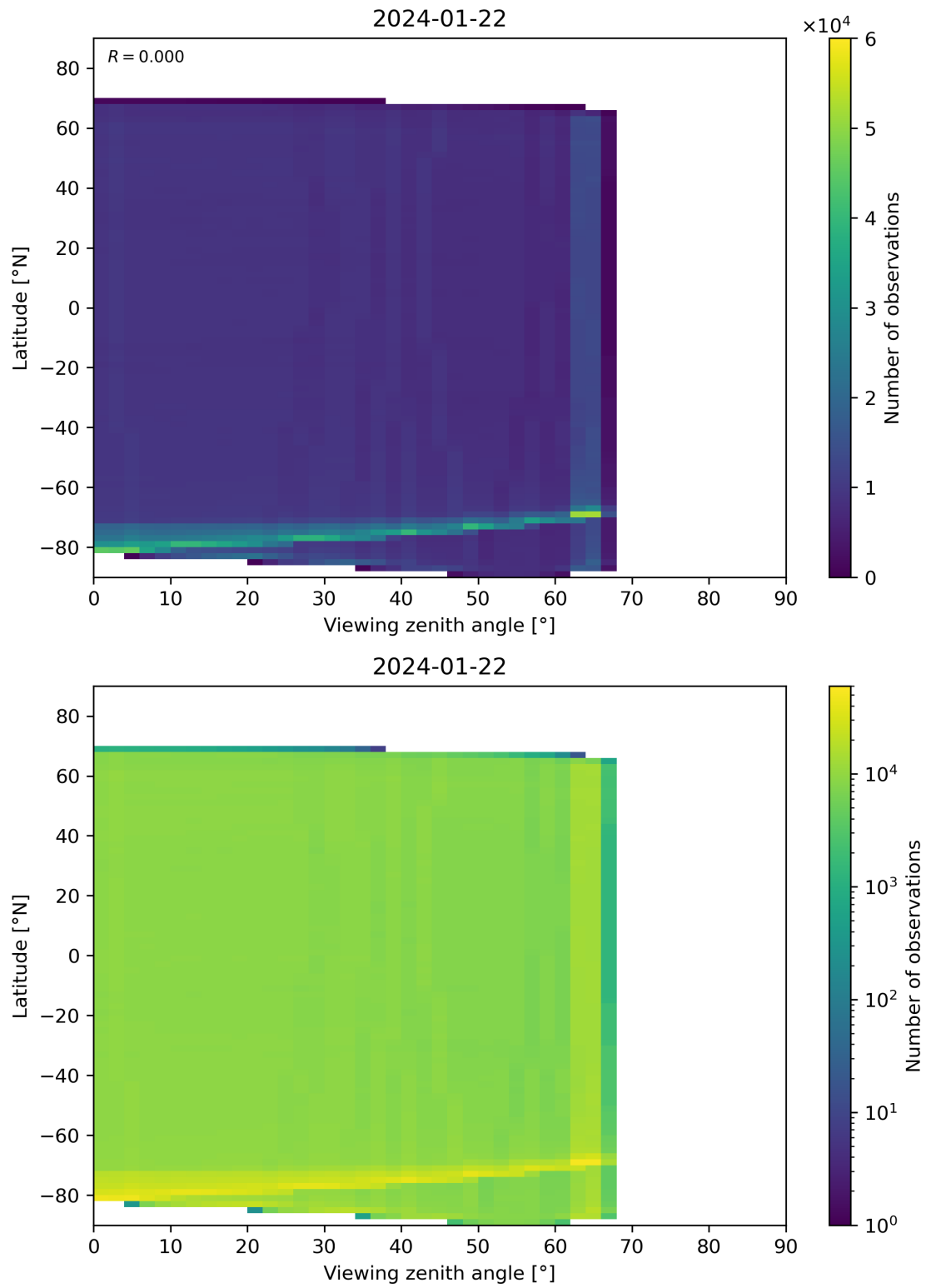
Figure 123: Scatter density plot of “Viewing zenith angle” against “Latitude” for 2024-01-21 to 2024-01-23.
