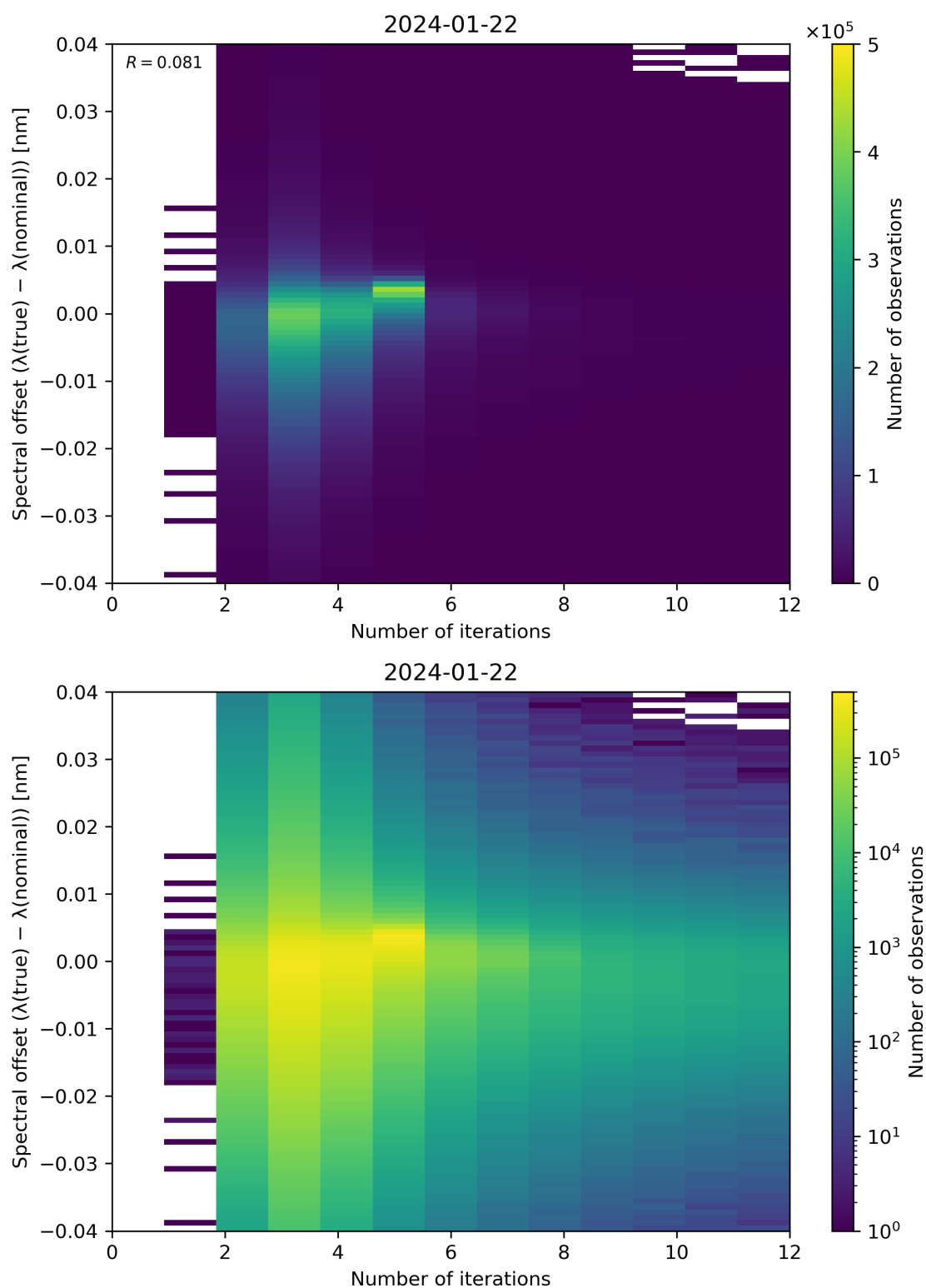
Figure 100: Scatter density plot of “Number of iterations” against “Spectral offset ( \lambda(\text{true}) - \lambda(\text{nominal}) )” for 2024-01-21 to 2024-01-23.
