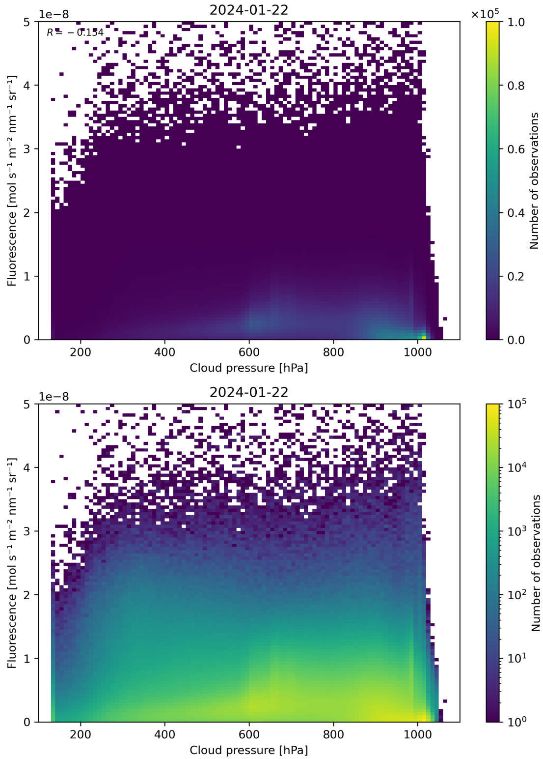
Figure 80: Scatter density plot of “Cloud pressure” against “Fluorescence” for 2024-01-21 to 2024-01-23.
