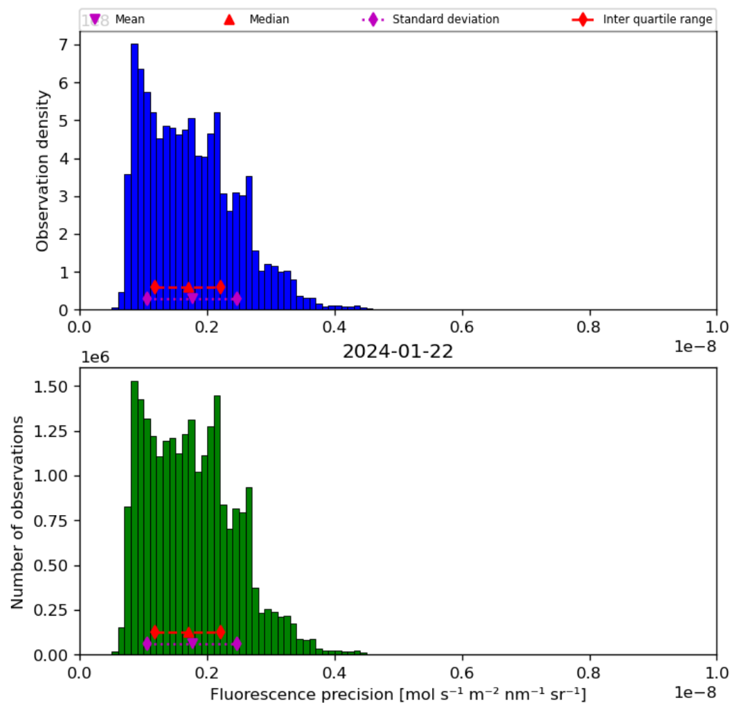
Figure 41: Histogram of “Fluorescence precision” for 2024-01-21 to 2024-01-23
