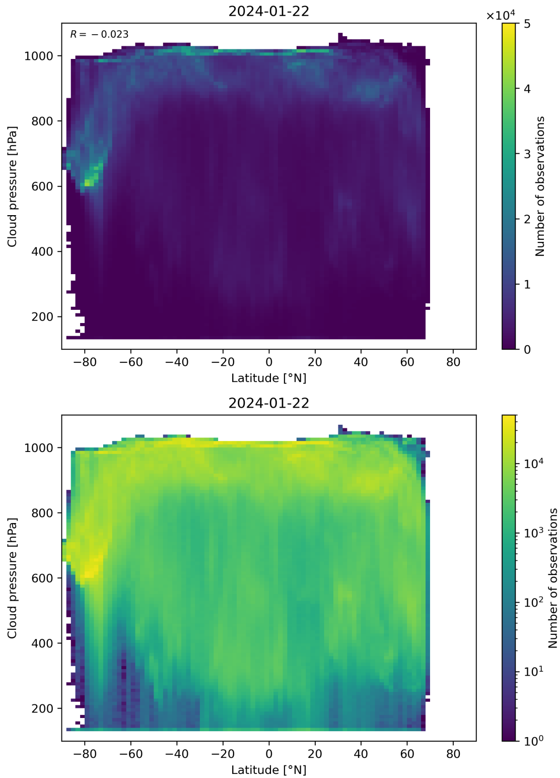
Figure 91: Scatter density plot of “Latitude” against “Cloud pressure” for 2024-01-21 to 2024-01-23.
