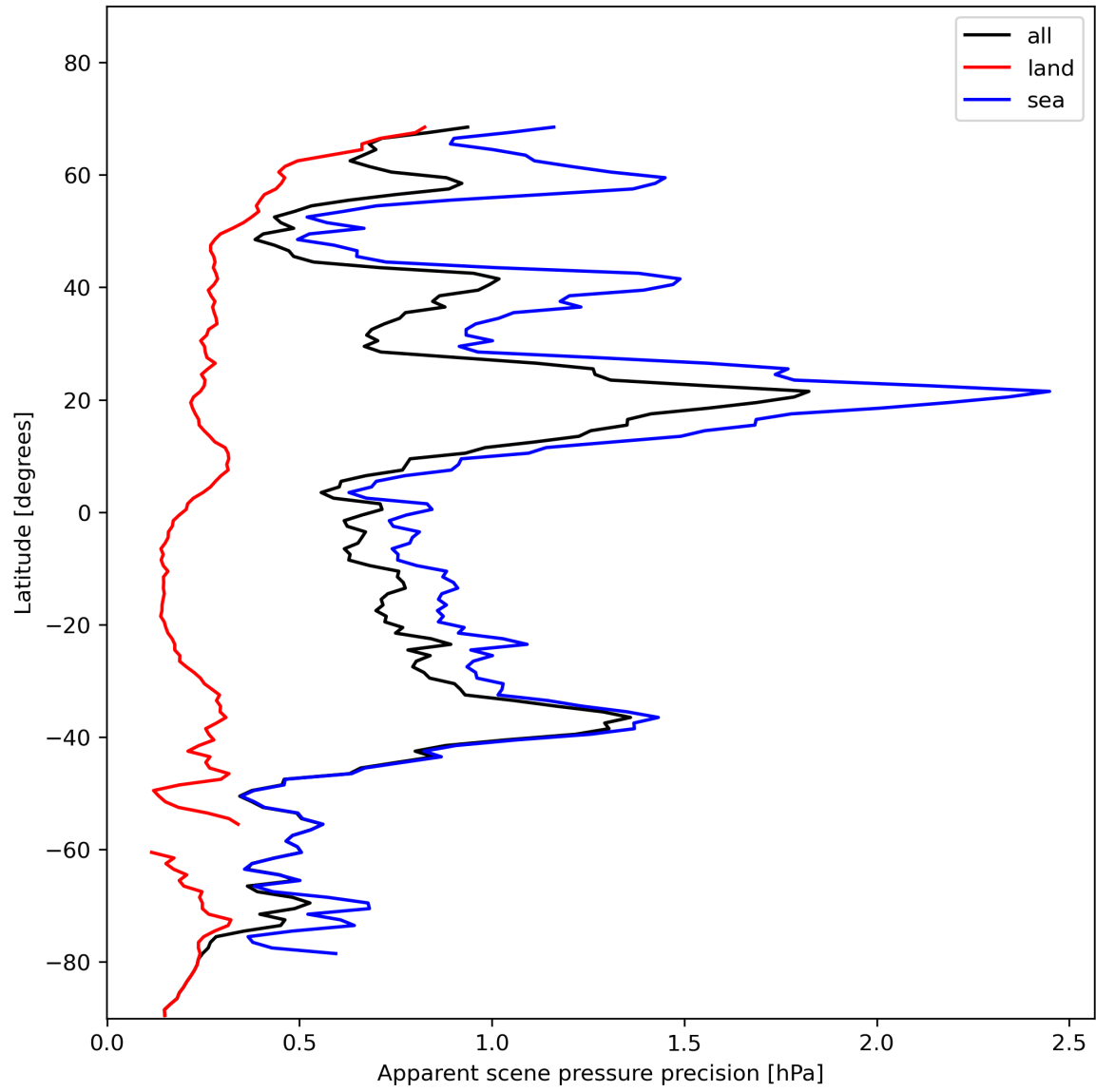
Figure 20: Zonal average of “Apparent scene pressure precision” for 2024-01-21 to 2024-01-23.
