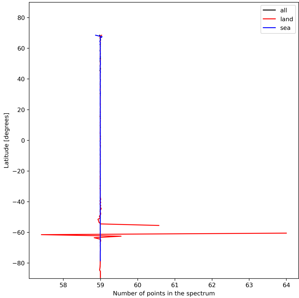
Figure 27: Zonal average of “Number of points in the spectrum” for 2024-01-21 to 2024-01-23.
