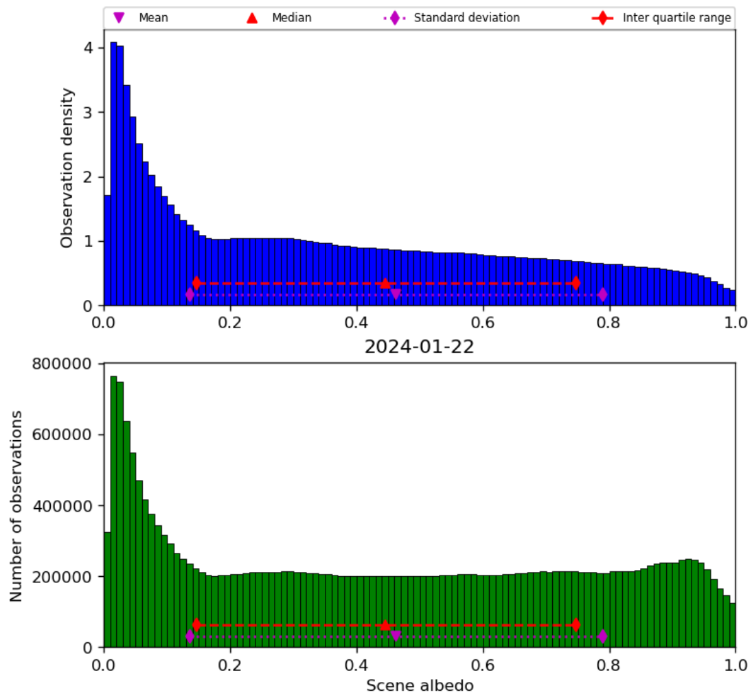
Figure 34: Histogram of “Scene albedo” for 2024-01-21 to 2024-01-23
