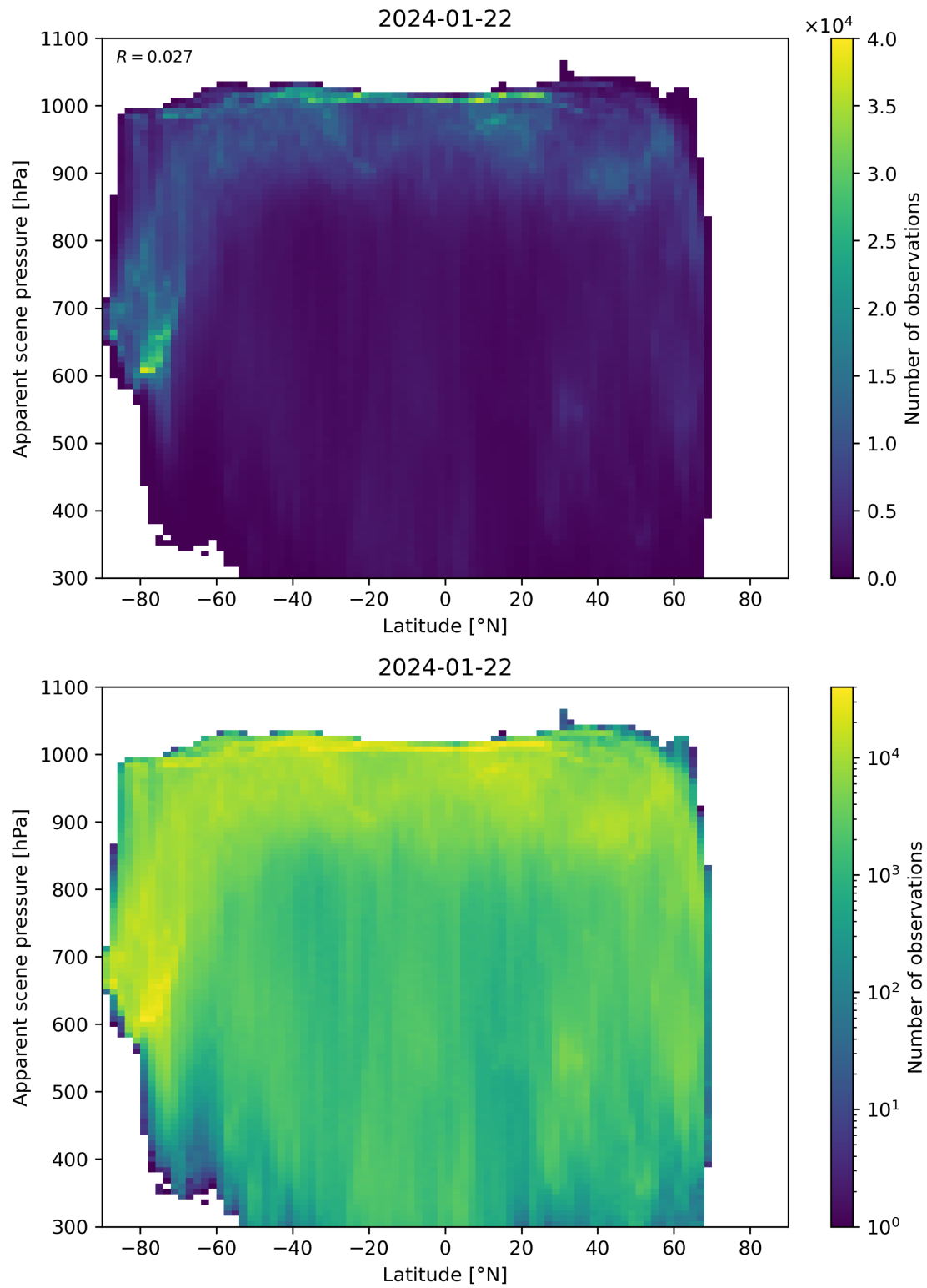
Figure 88: Scatter density plot of “Latitude” against “Apparent scene pressure” for 2024-01-21 to 2024-01-23.
