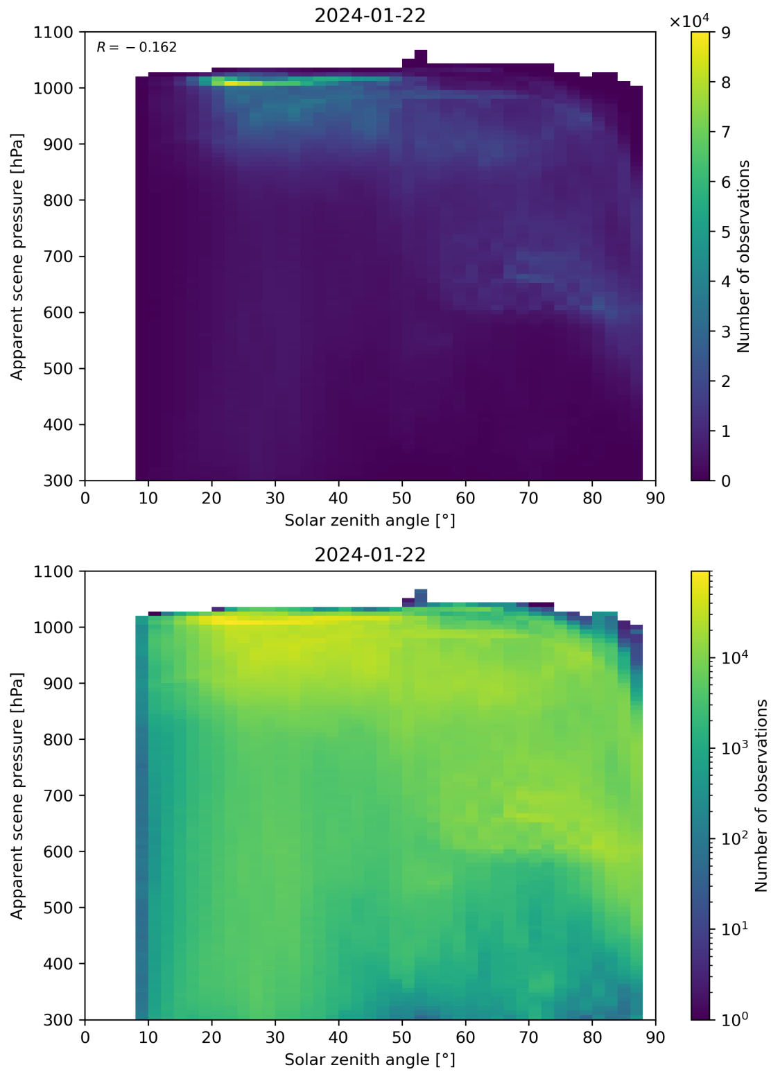
Figure 108: Scatter density plot of “Solar zenith angle” against “Apparent scene pressure” for 2024-01-21 to 2024-01-23.
