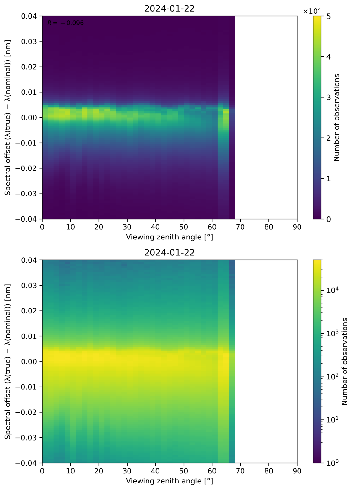
Figure 128: Scatter density plot of “Viewing zenith angle” against “Spectral offset ( \lambda(\text{true}) - \lambda(\text{nominal}) )” for 2024-01-21 to 2024-01-23.
