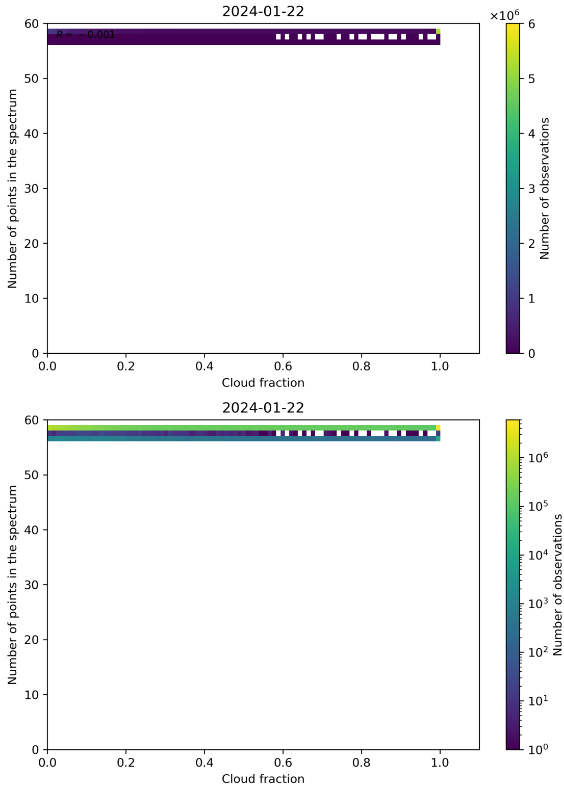
Figure 74: Scatter density plot of “Cloud fraction” against “Number of points in the spectrum” for 2024-01-21 to 2024-01-23.
