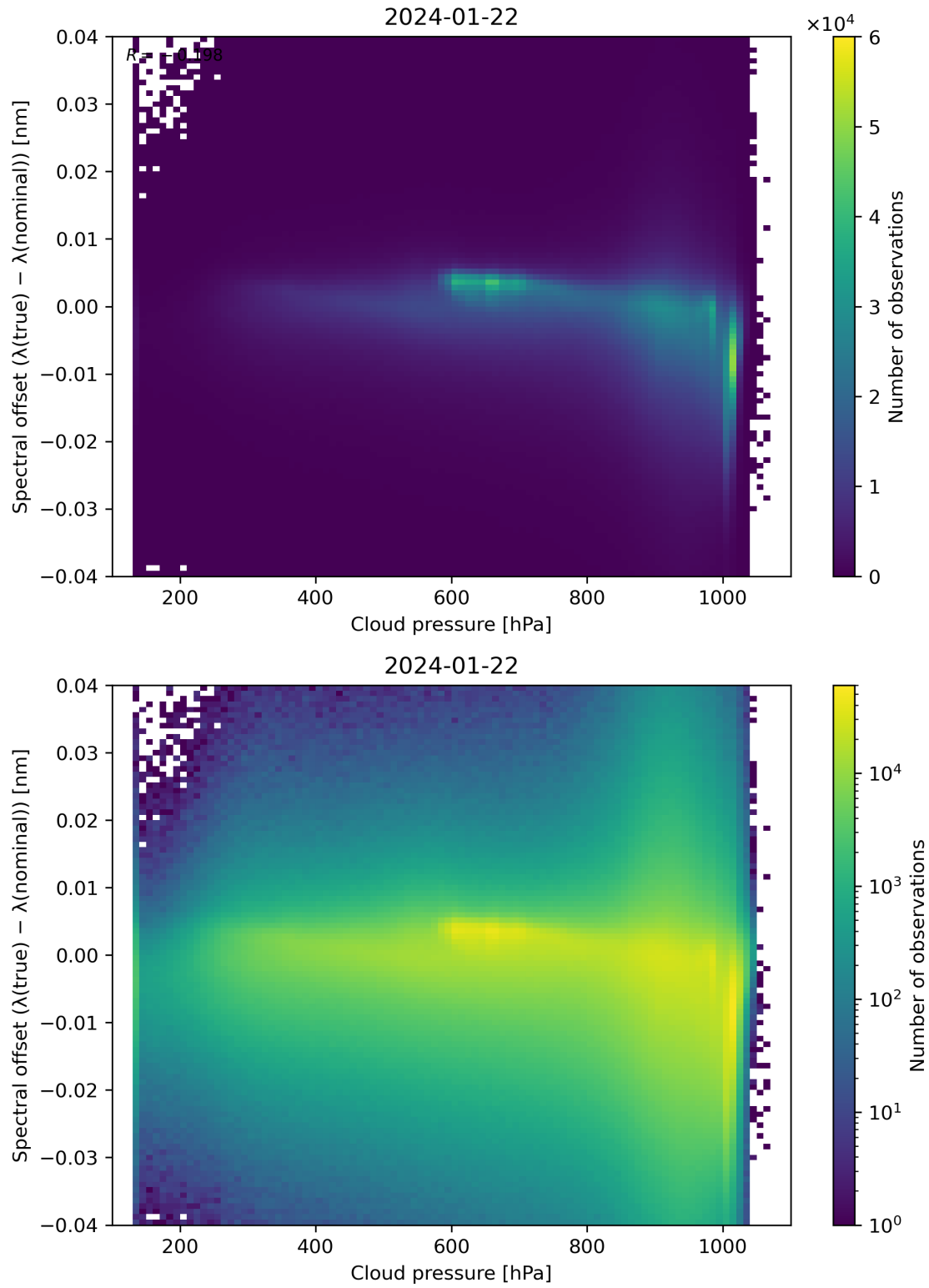
Figure 84: Scatter density plot of “Cloud pressure” against “Spectral offset ( \lambda(\text{true}) - \lambda(\text{nominal}) )” for 2024-01-21 to 2024-01-23.
