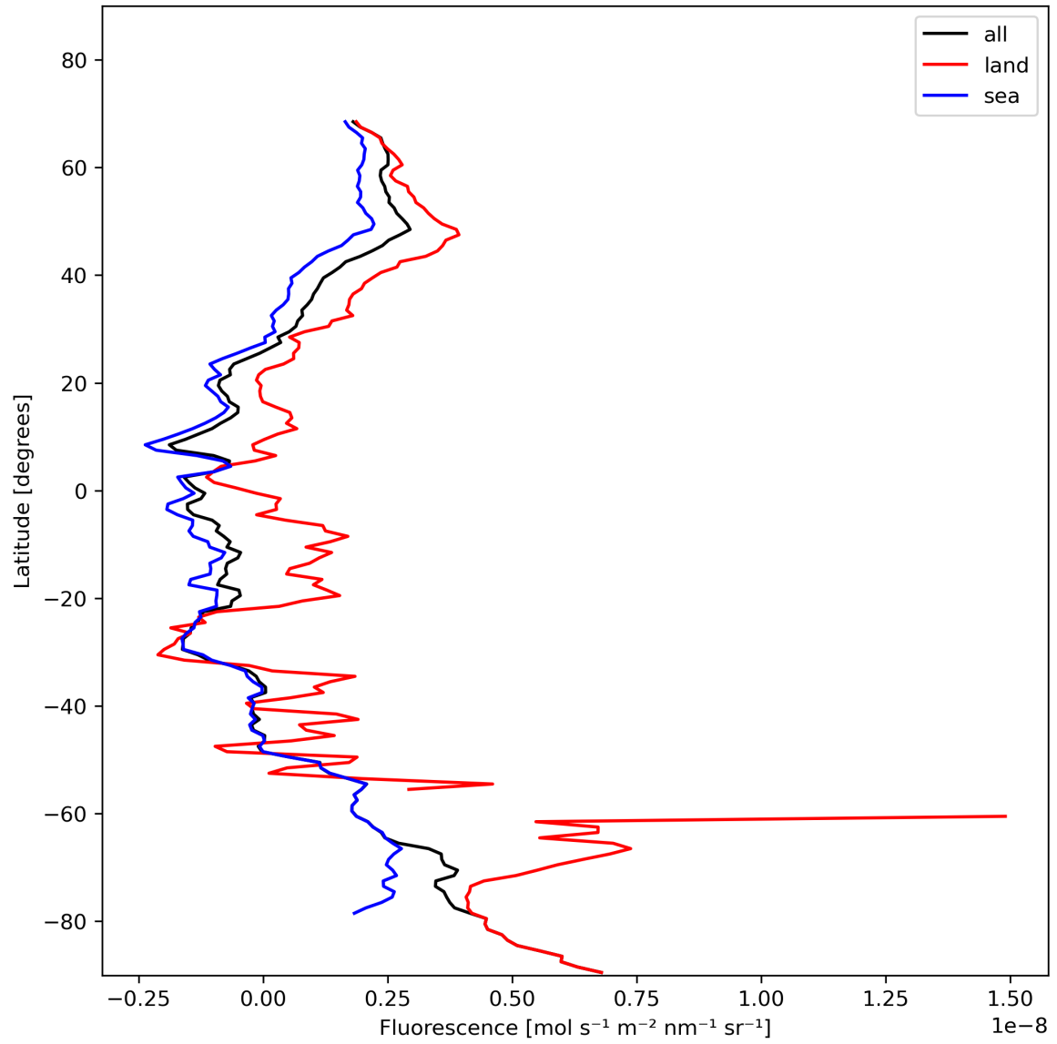
Figure 23: Zonal average of “Fluorescence” for 2024-01-21 to 2024-01-23.
