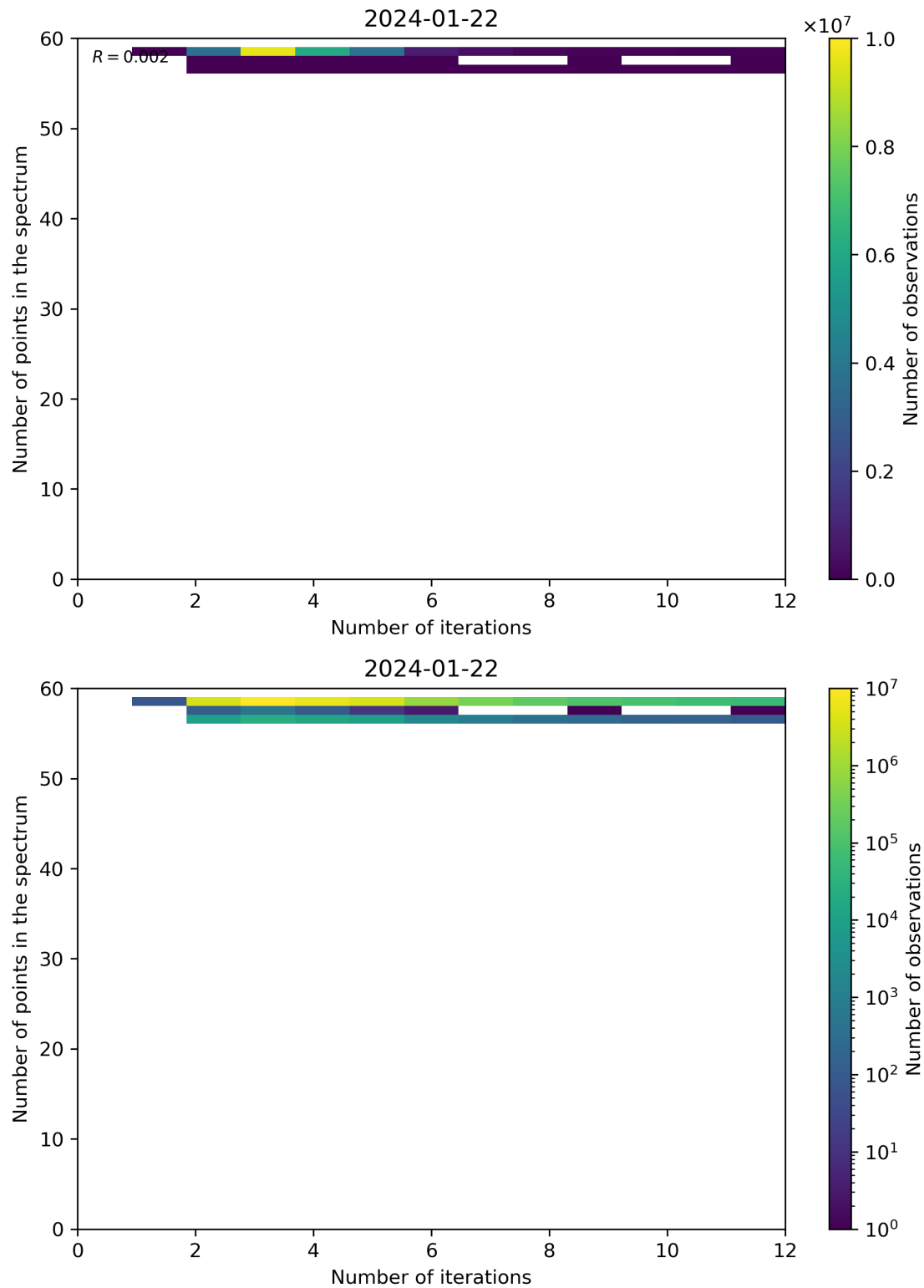
Figure 99: Scatter density plot of “Number of iterations” against “Number of points in the spectrum” for 2024-01-21 to 2024-01-23.
