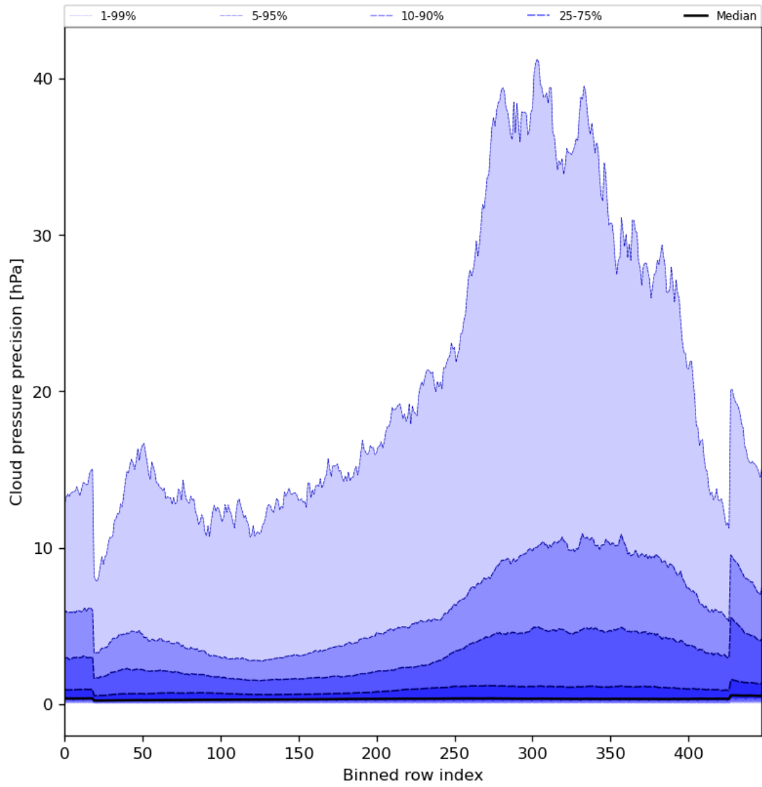
Figure 48: Along track statistics of “Cloud pressure precision” for 2024-01-21 to 2024-01-23
