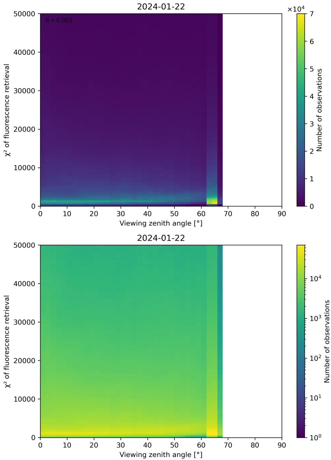
Figure 119: Scatter density plot of “Viewing zenith angle” against “ \chi^2 of fluorescence retrieval” for 2024-01-21 to 2024-01-23.
