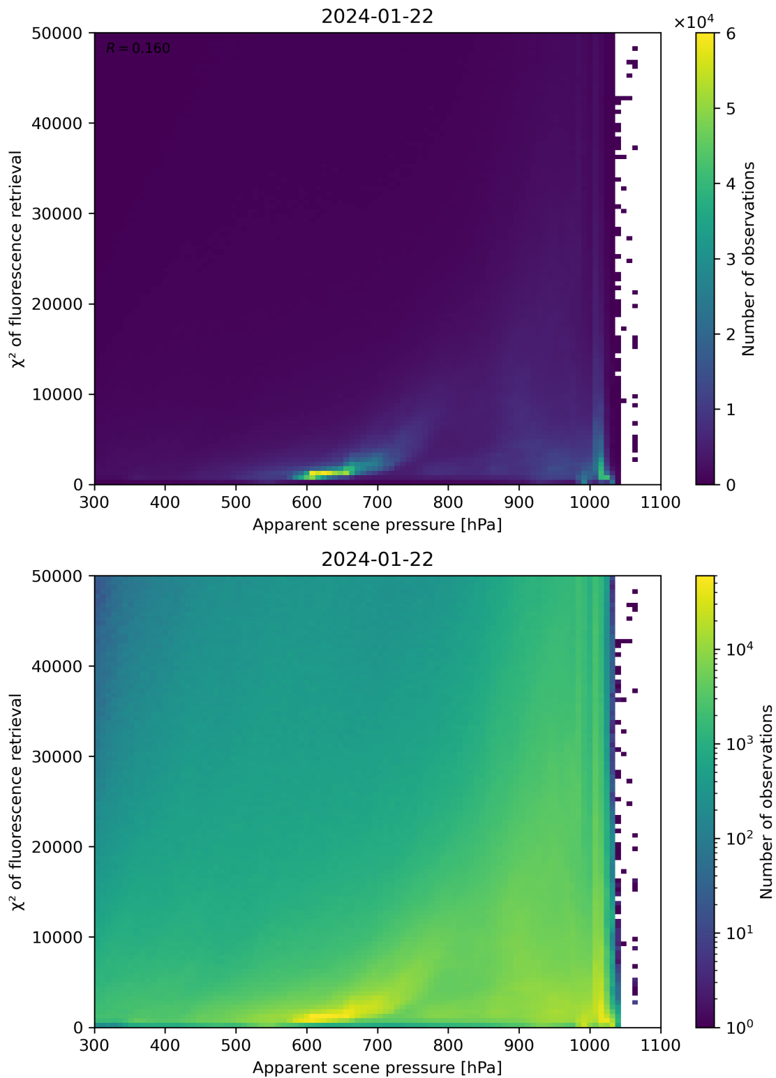
Figure 63: Scatter density plot of “Apparent scene pressure” against “ \chi^2 of fluorescence retrieval” for 2024-01-21 to 2024-01-23.
