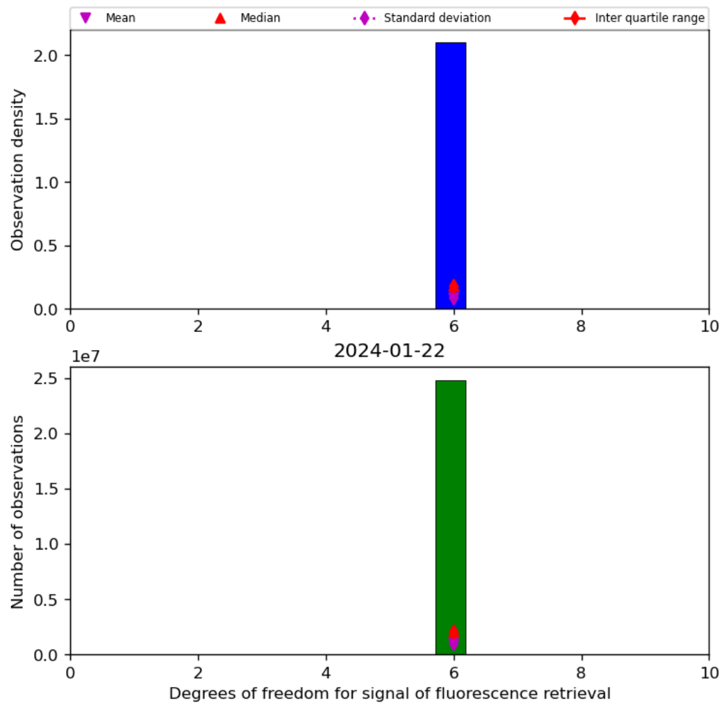
Figure 43: Histogram of “Degrees of freedom for signal of fluorescence retrieval” for 2024-01-21 to 2024-01-23
