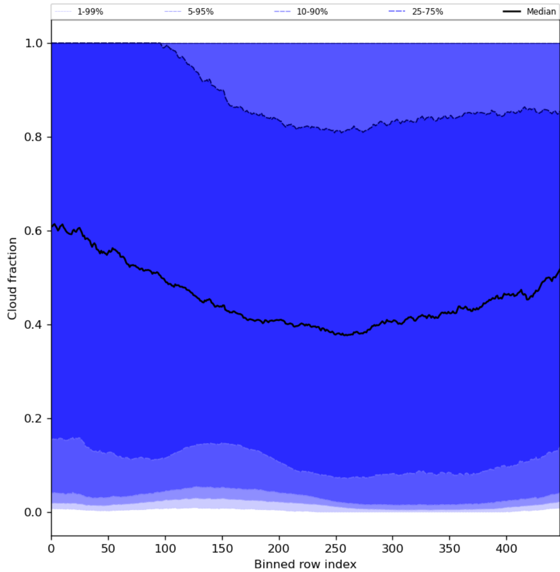
Figure 49: Along track statistics of “Cloud fraction” for 2024-01-21 to 2024-01-23
