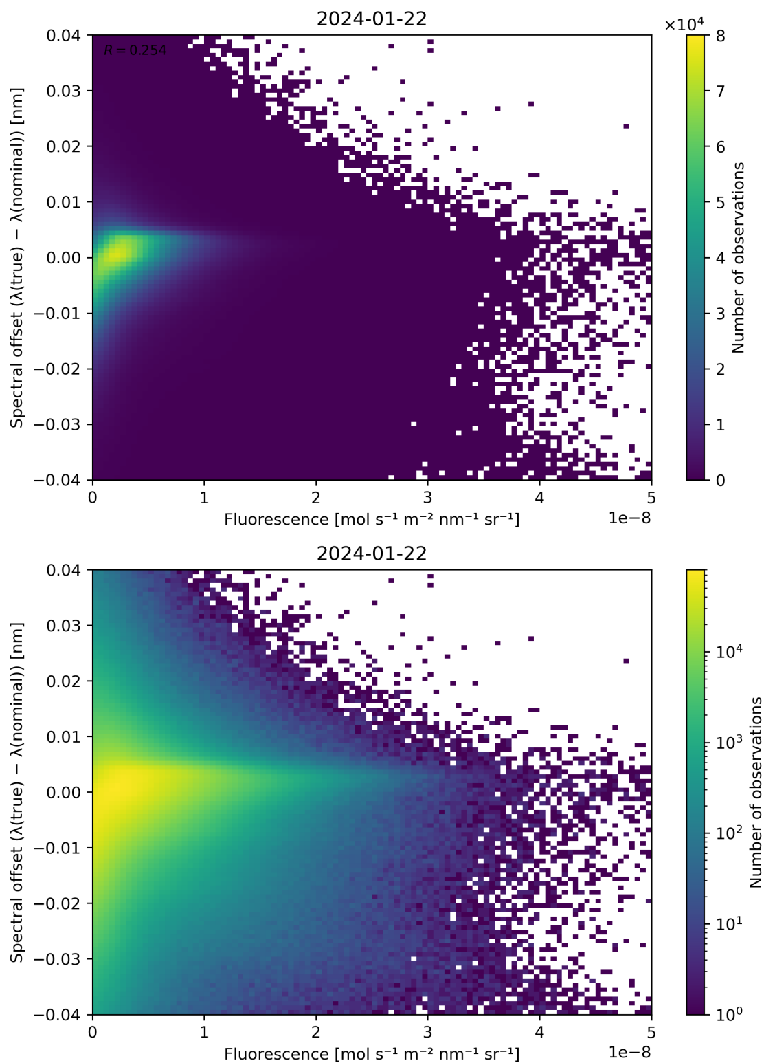
Figure 87: Scatter density plot of “Fluorescence” against “Spectral offset ( \lambda(\text{true}) - \lambda(\text{nominal}) )” for 2024-01-21 to 2024-01-23.
