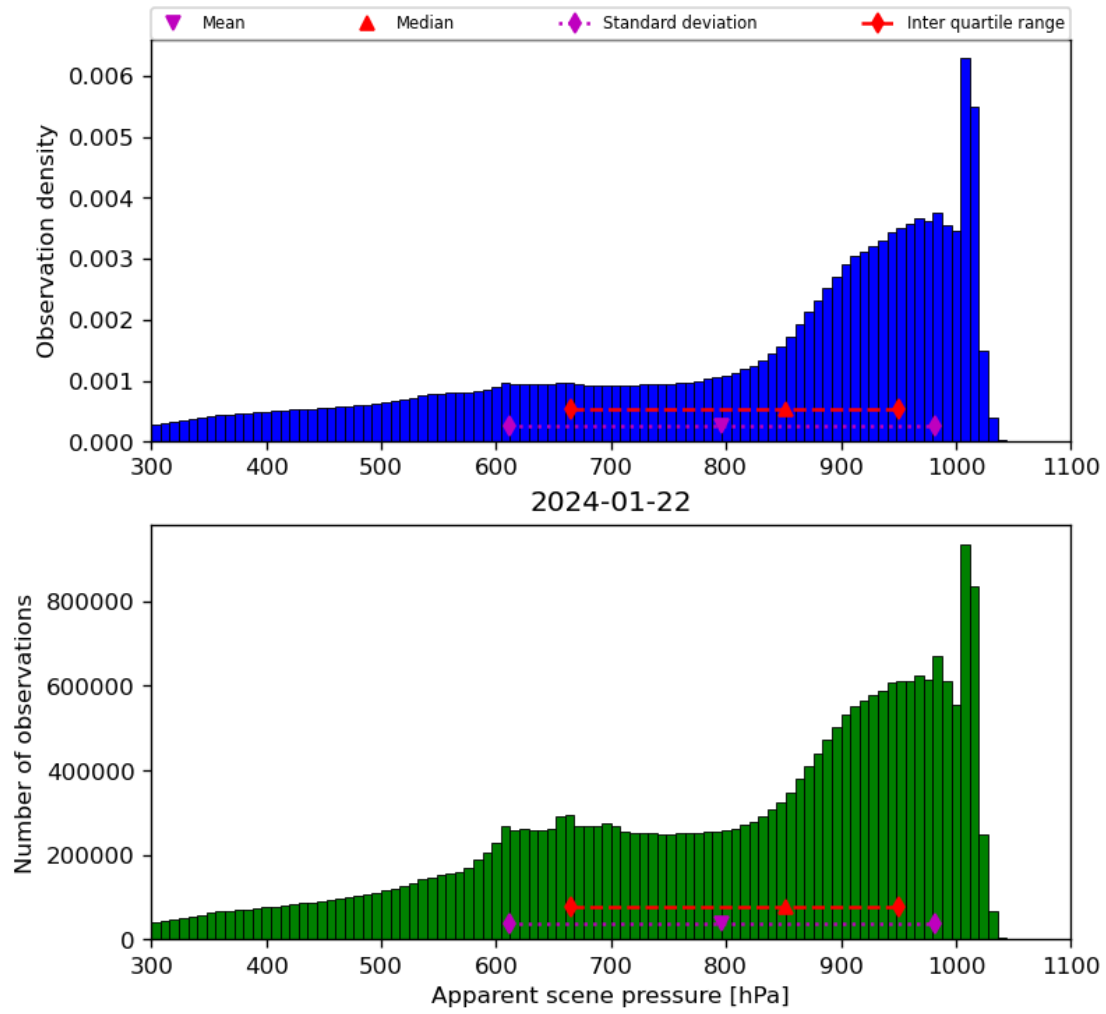
Figure 36: Histogram of “Apparent scene pressure” for 2024-01-21 to 2024-01-23
