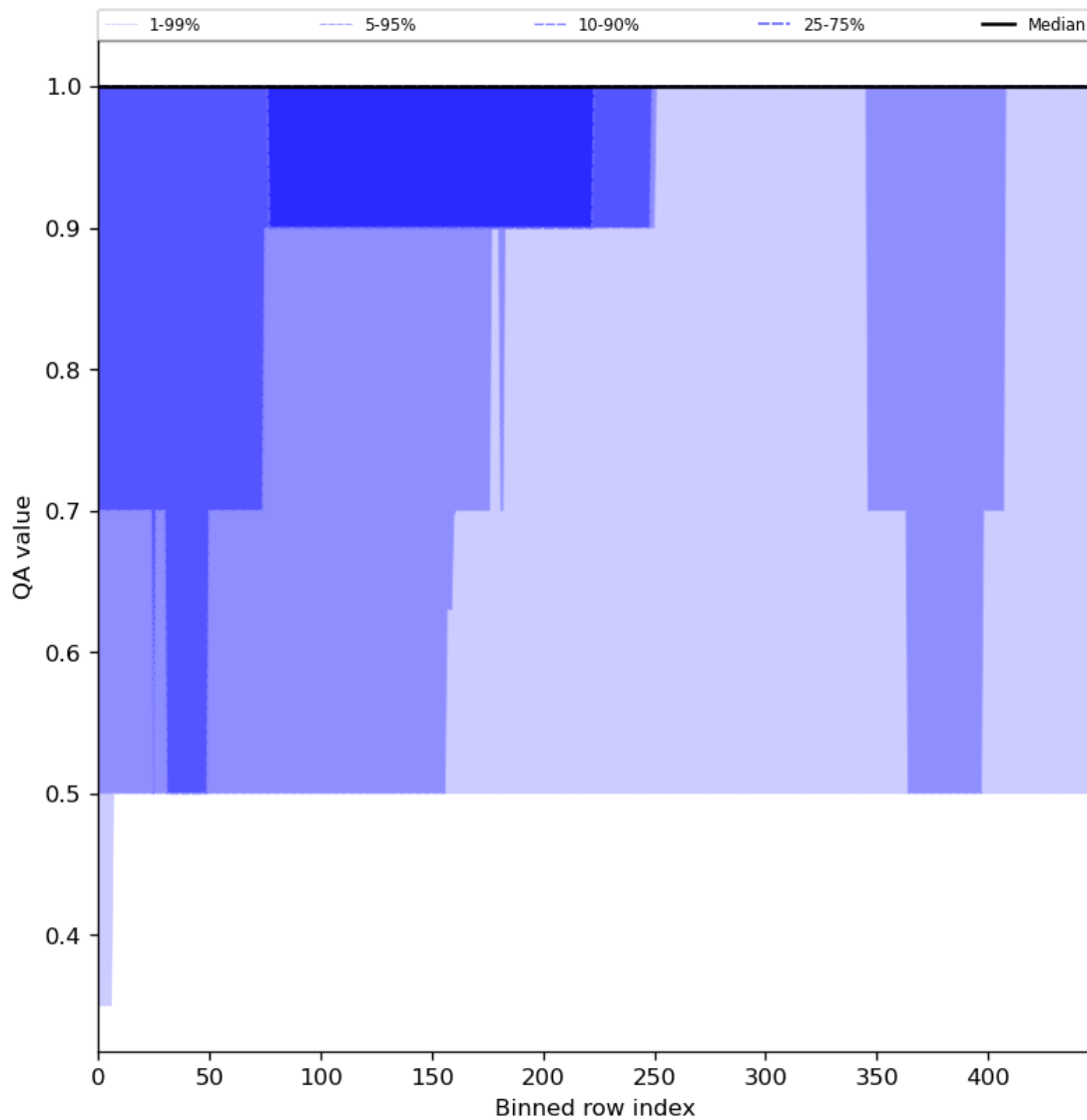
Figure 46: Along track statistics of “QA value” for 2024-01-21 to 2024-01-23
