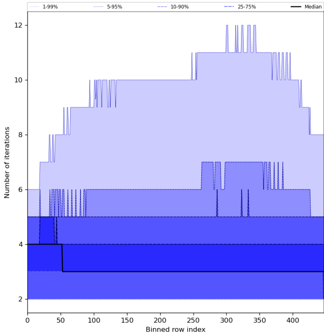
Figure 56: Along track statistics of “Number of iterations” for 2024-01-21 to 2024-01-23
