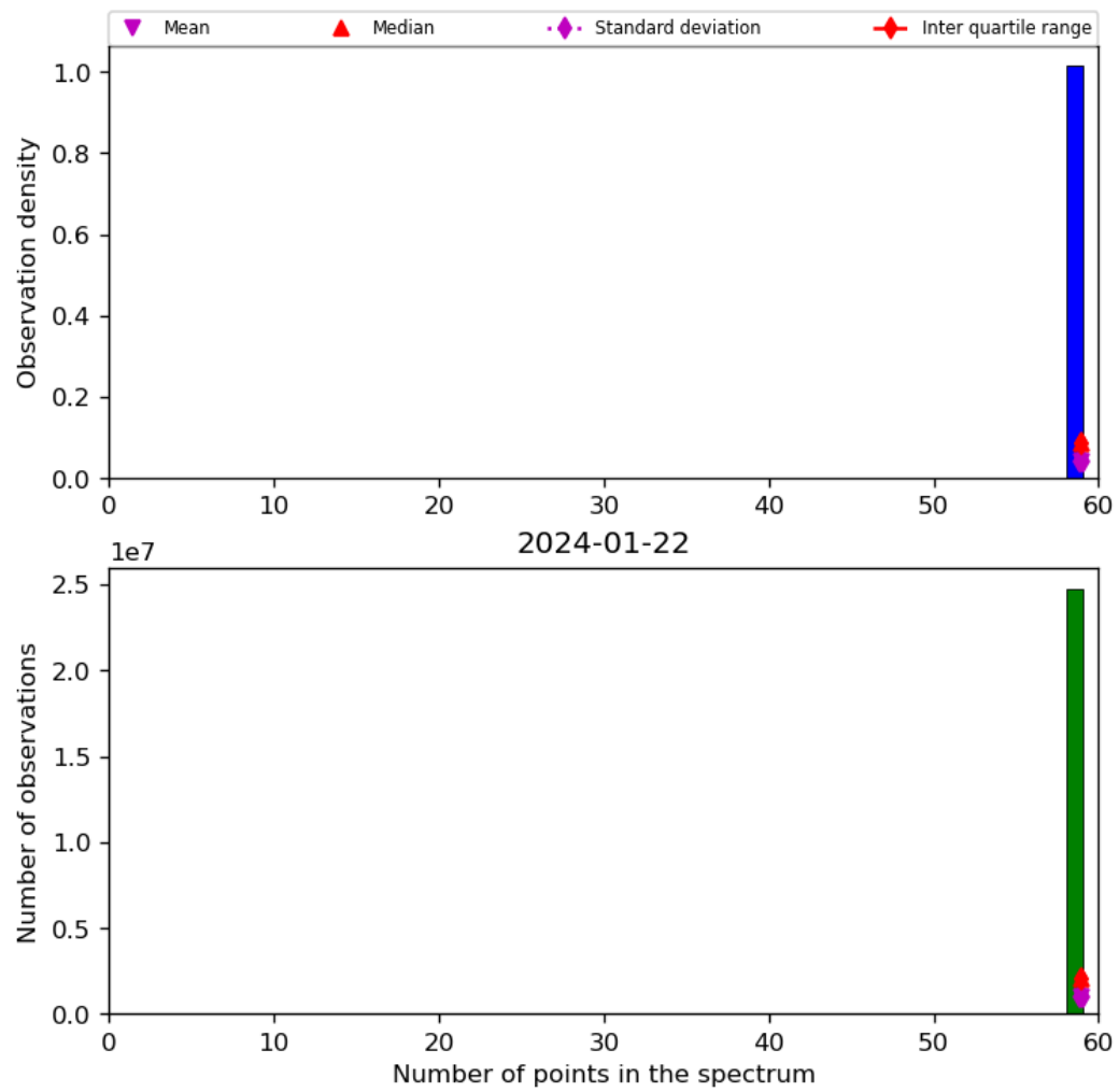
Figure 44: Histogram of “Number of points in the spectrum” for 2024-01-21 to 2024-01-23
