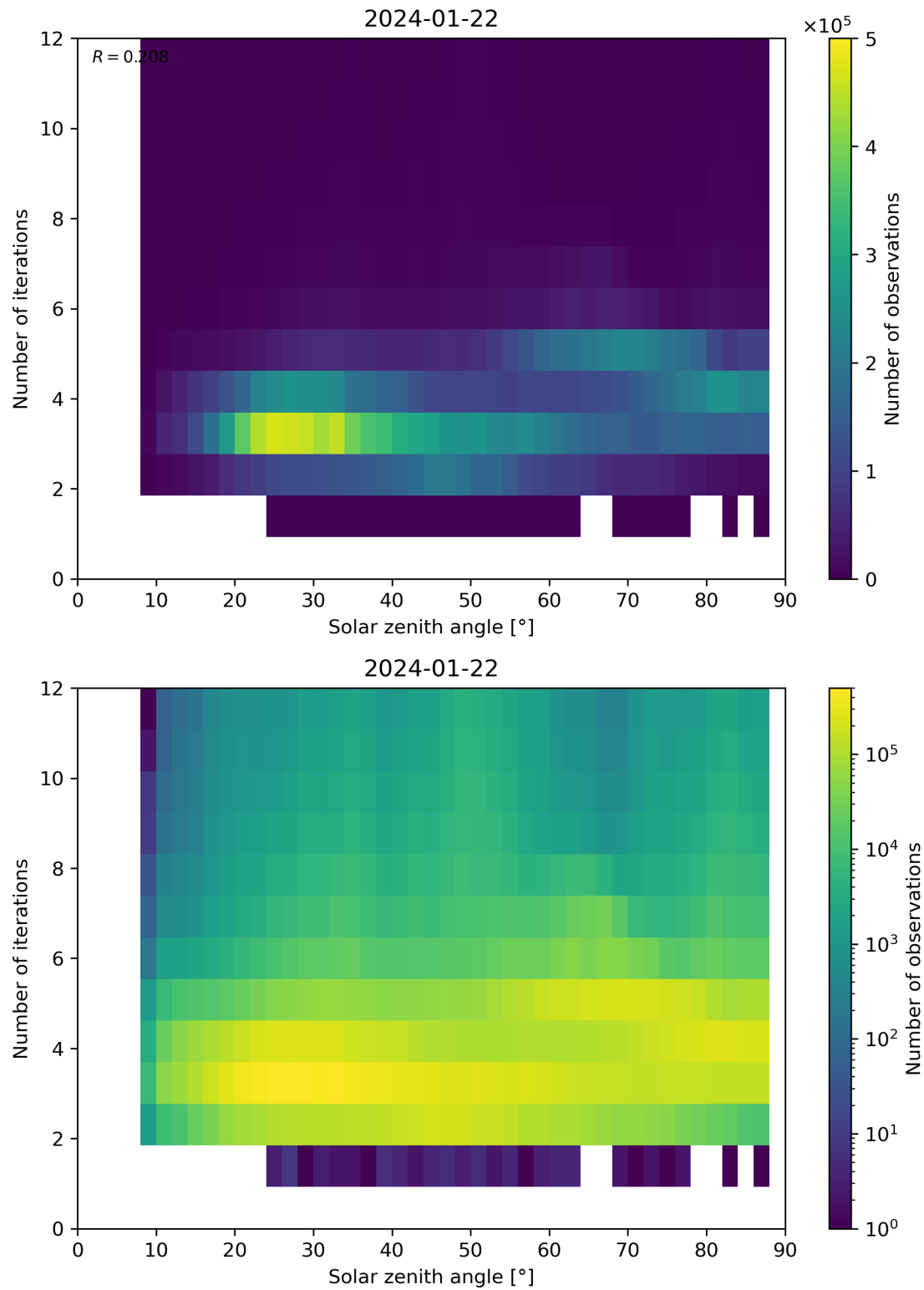
Figure 114: Scatter density plot of “Solar zenith angle” against “Number of iterations” for 2024-01-21 to 2024-01-23.
