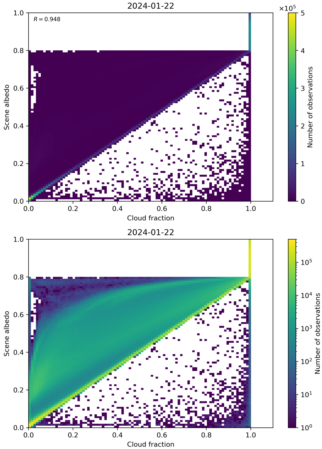
Figure 75: Scatter density plot of “Cloud fraction” against “Scene albedo” for 2024-01-21 to 2024-01-23.
