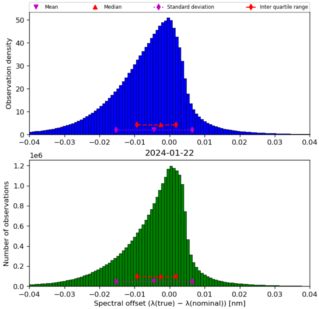
Figure 45: Histogram of “Spectral offset ( \lambda(\text{true}) - \lambda(\text{nominal}) )” for 2024-01-21 to 2024-01-23
