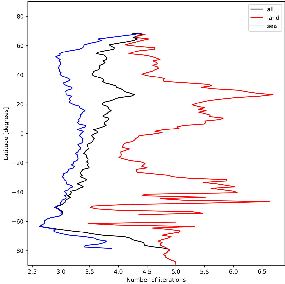
Figure 22: Zonal average of “Number of iterations” for 2024-01-21 to 2024-01-23.
