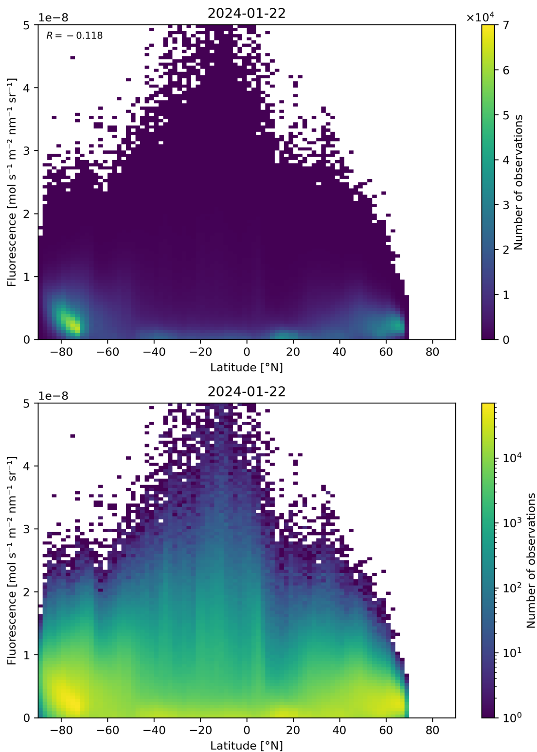
Figure 92: Scatter density plot of “Latitude” against “Fluorescence” for 2024-01-21 to 2024-01-23.
