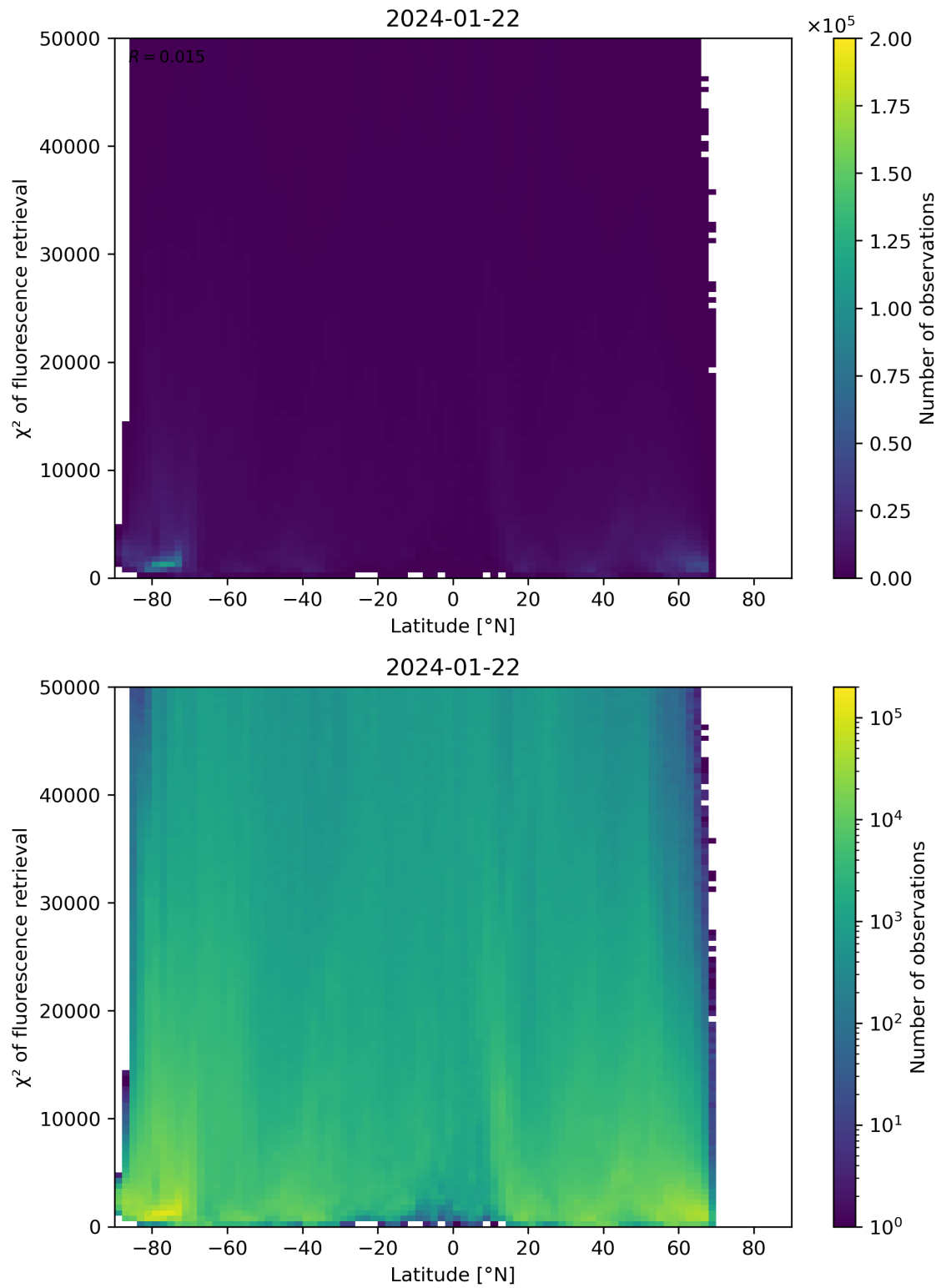
Figure 89: Scatter density plot of “Latitude” against “ \chi^2 of fluorescence retrieval” for 2024-01-21 to 2024-01-23.
