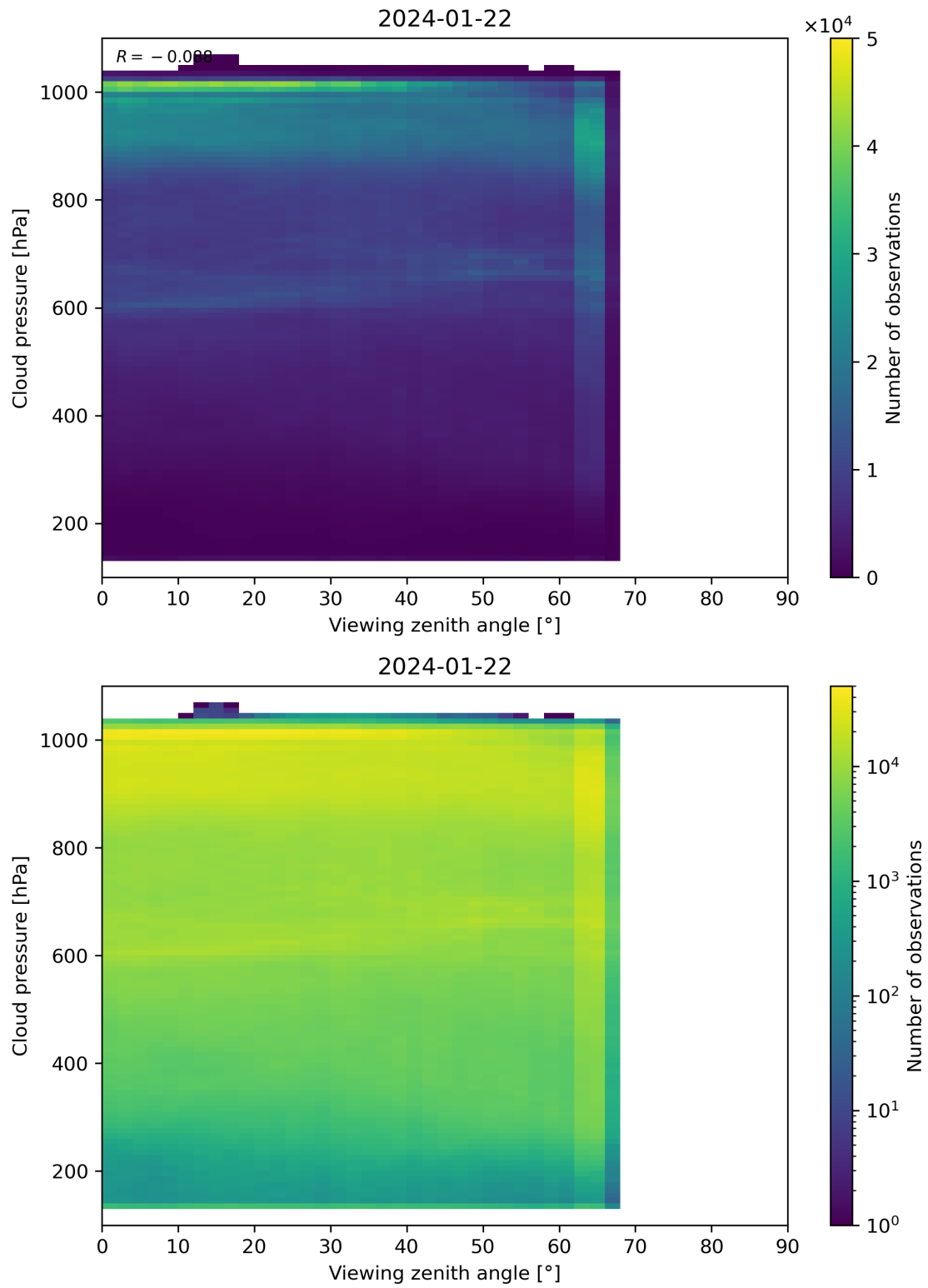
Figure 121: Scatter density plot of “Viewing zenith angle” against “Cloud pressure” for 2024-01-21 to 2024-01-23.
