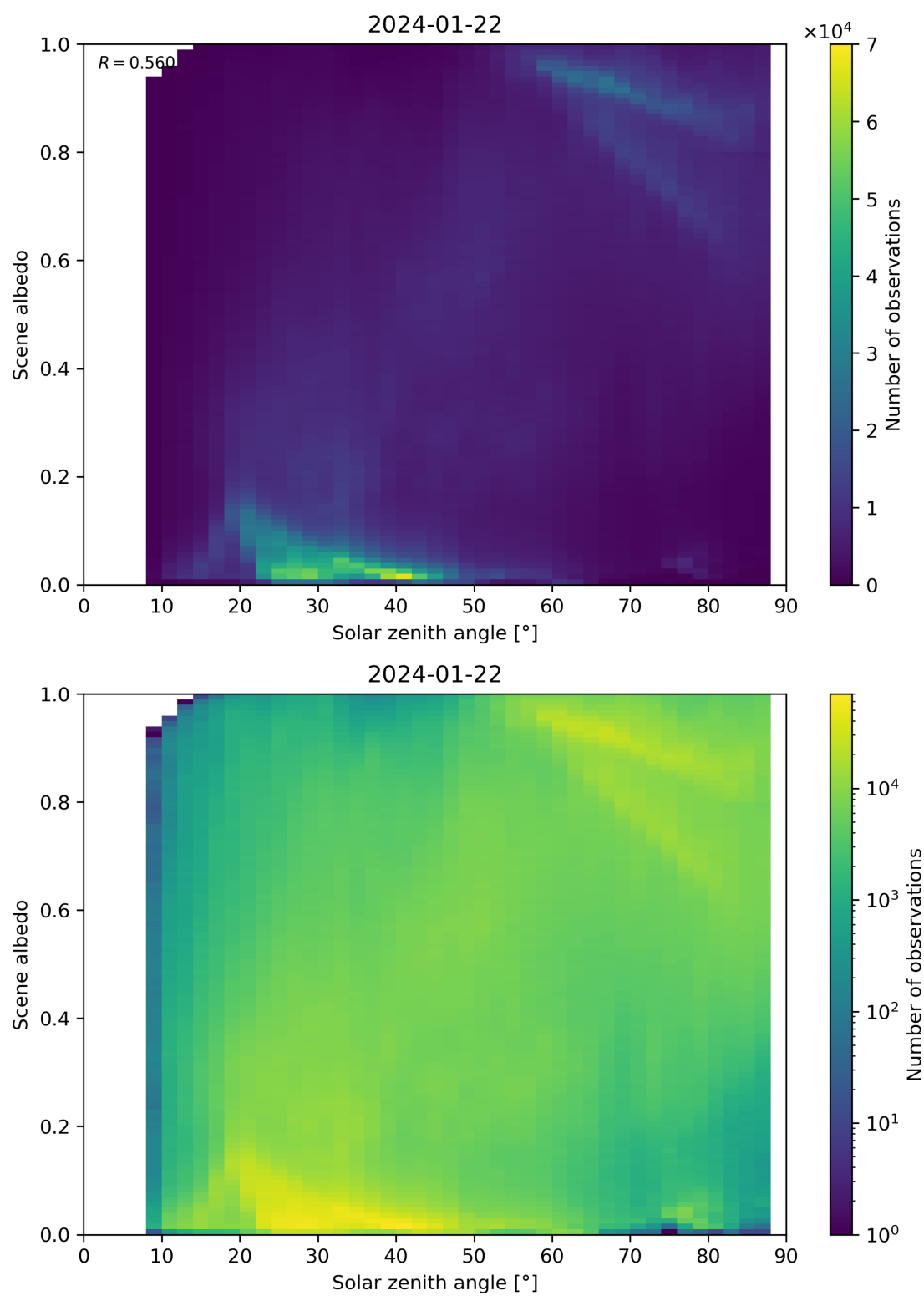
Figure 116: Scatter density plot of “Solar zenith angle” against “Scene albedo” for 2024-01-21 to 2024-01-23.
