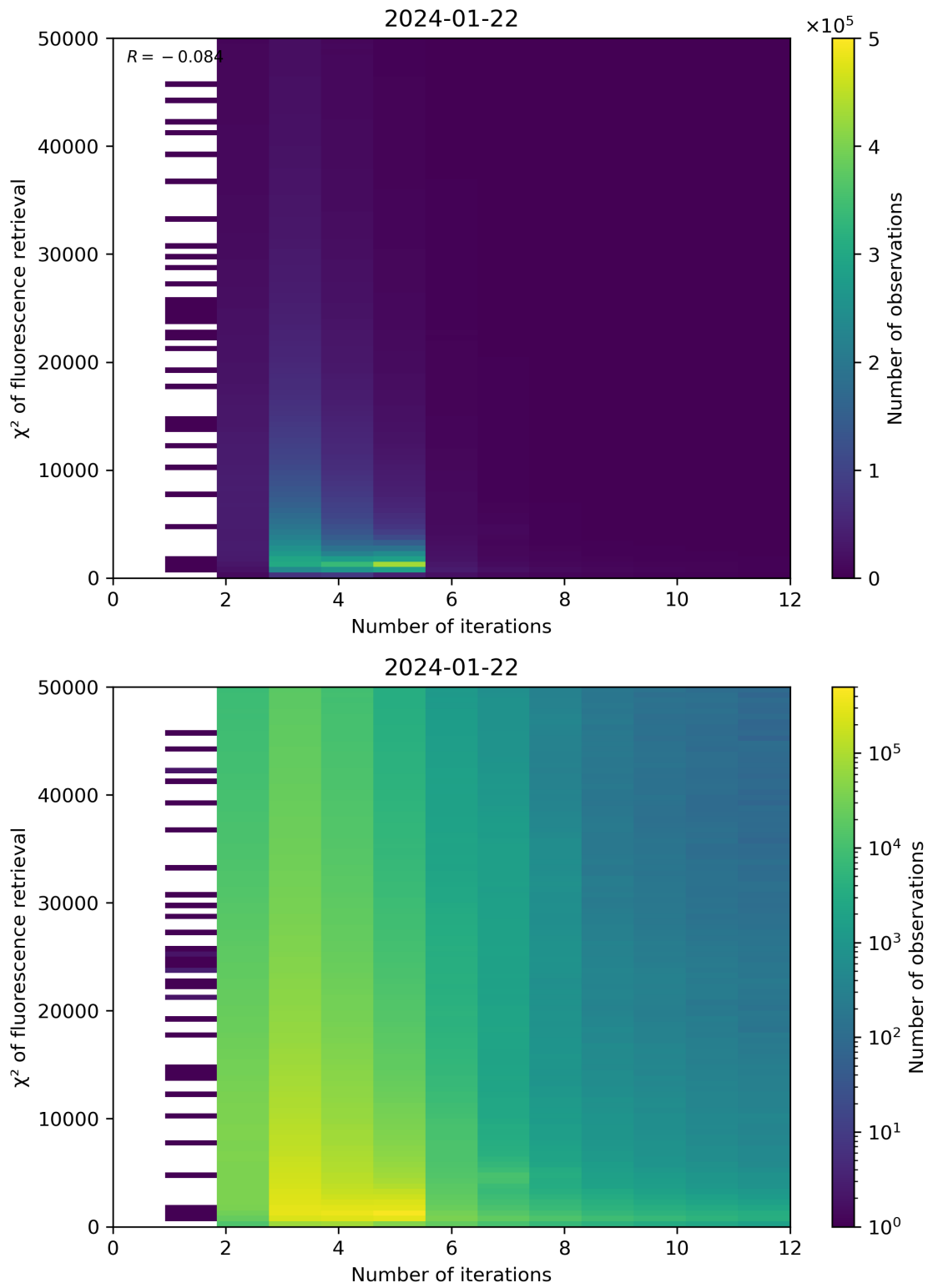
Figure 97: Scatter density plot of “Number of iterations” against “ \chi^2 of fluorescence retrieval” for 2024-01-21 to 2024-01-23.
