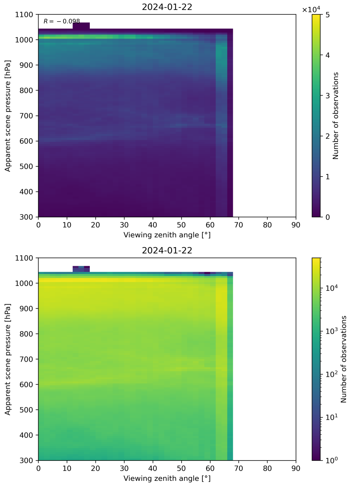
Figure 118: Scatter density plot of “Viewing zenith angle” against “Apparent scene pressure” for 2024-01-21 to 2024-01-23.
