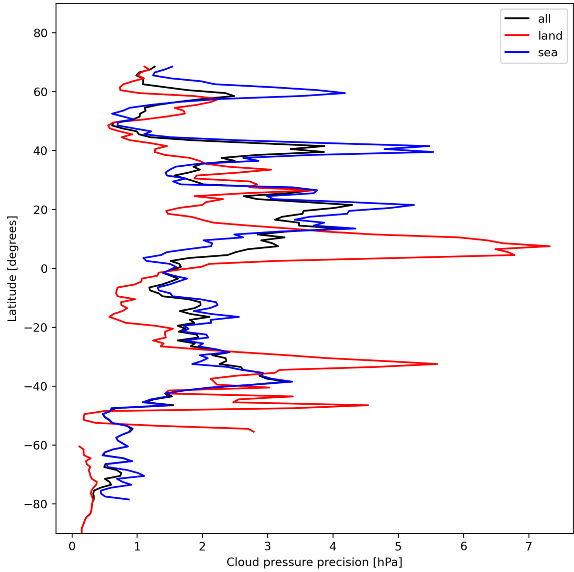
Figure 14: Zonal average of “Cloud pressure precision” for 2024-01-21 to 2024-01-23.
