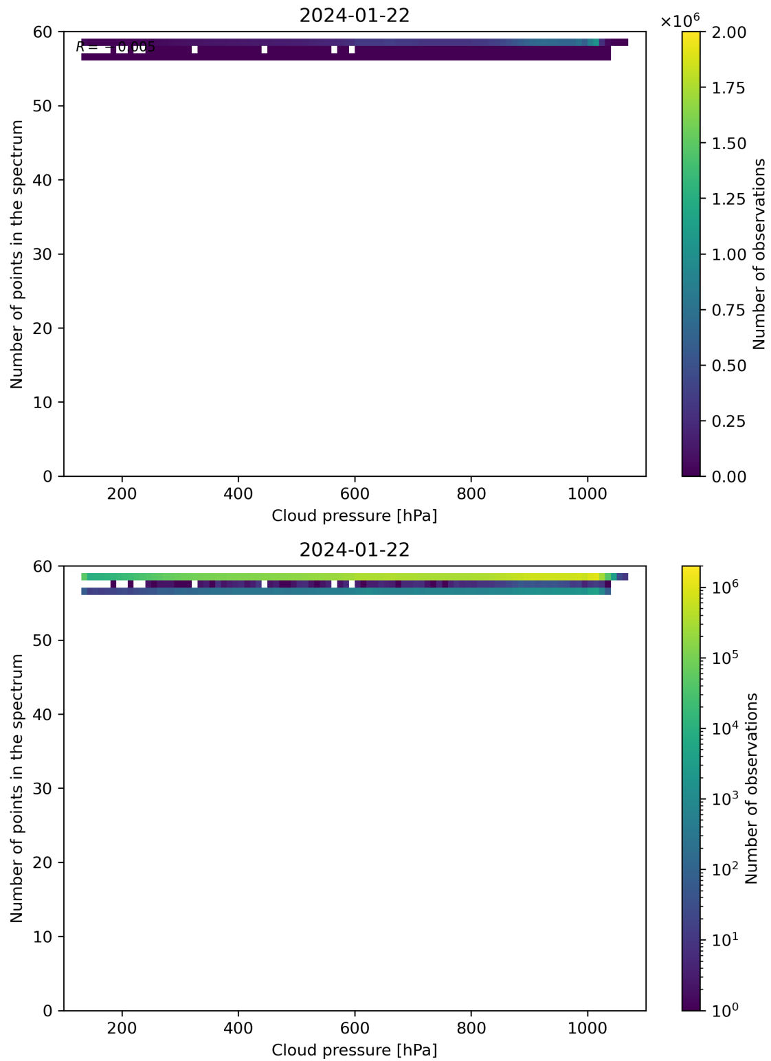
Figure 82: Scatter density plot of “Cloud pressure” against “Number of points in the spectrum” for 2024-01-21 to 2024-01-23.
