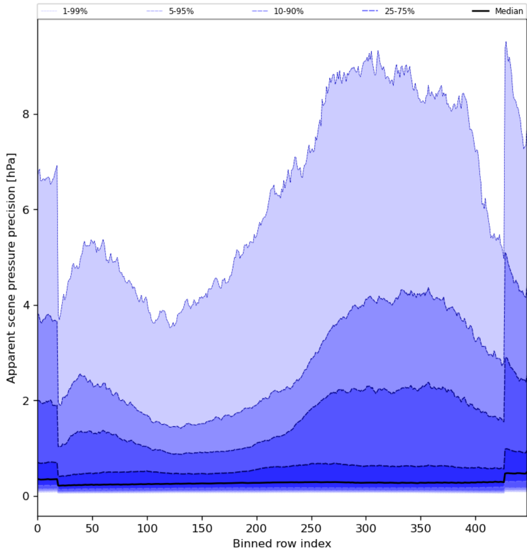
Figure 54: Along track statistics of “Apparent scene pressure precision” for 2024-01-21 to 2024-01-23
