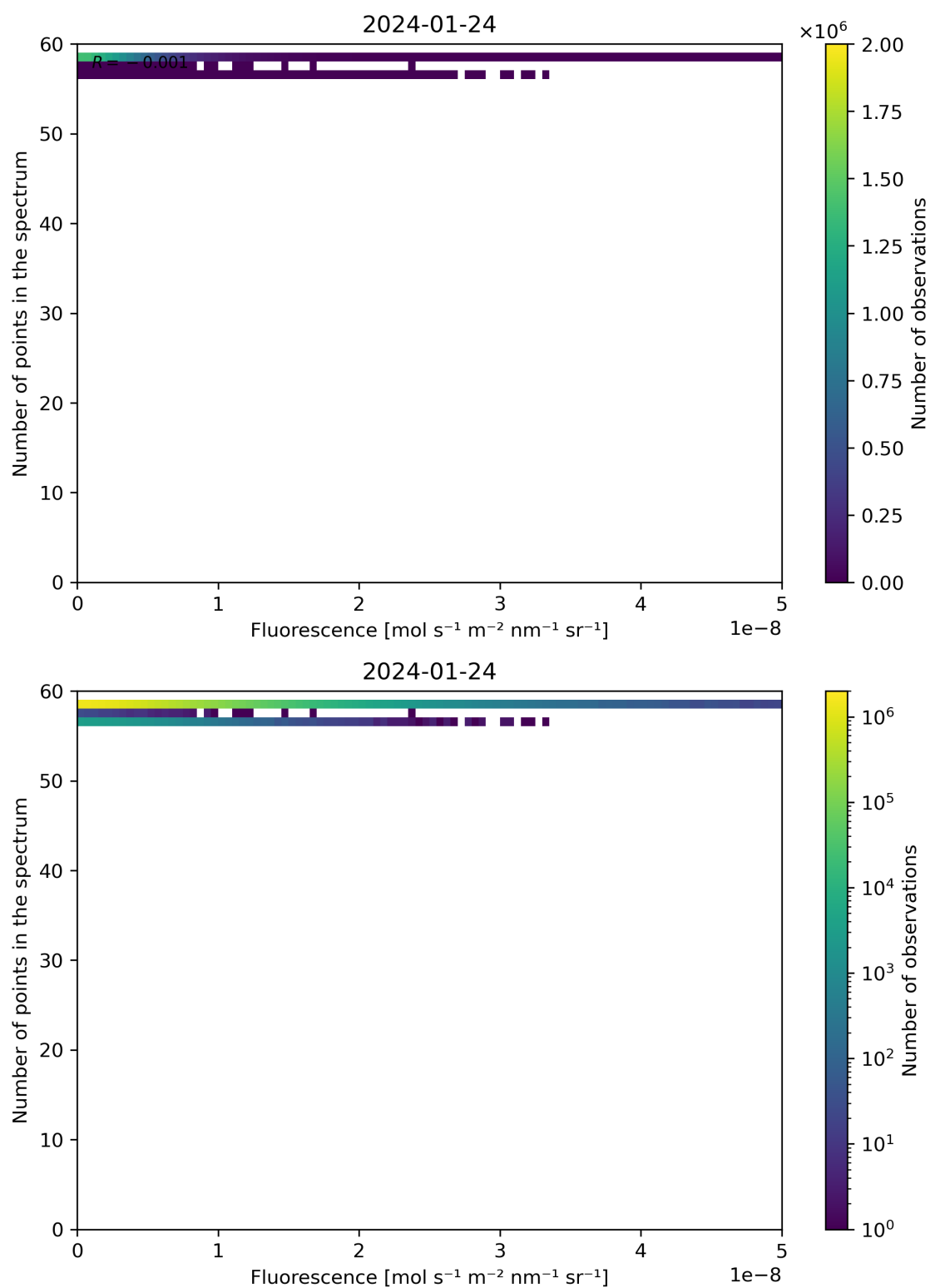
Figure 86: Scatter density plot of “Fluorescence” against “Number of points in the spectrum” for 2024-01-23 to 2024-01-25.
