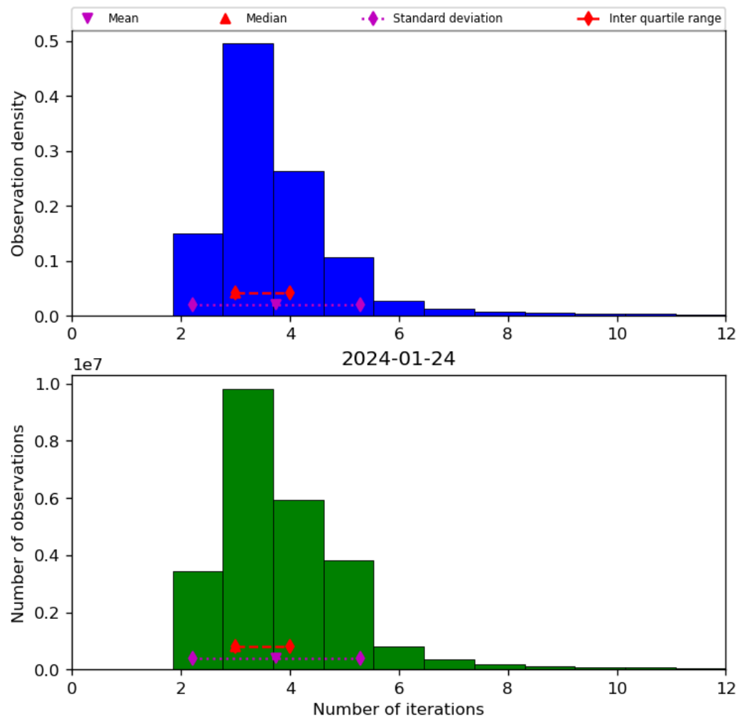
Figure 39: Histogram of “Number of iterations” for 2024-01-23 to 2024-01-25
