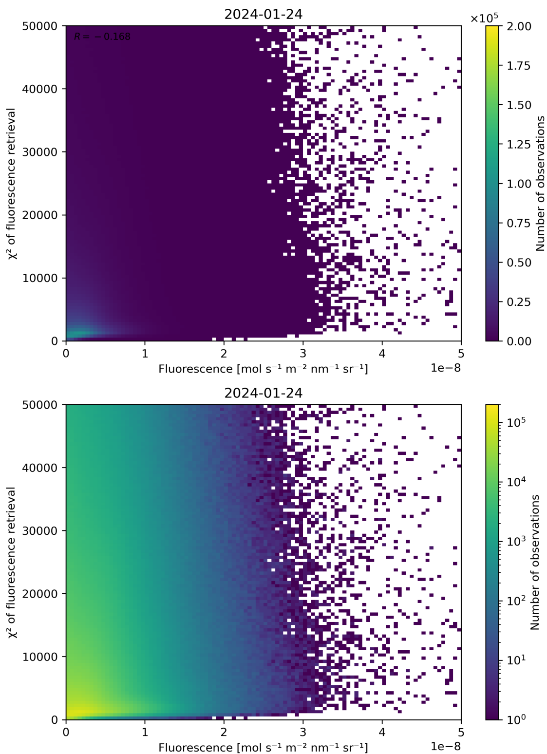
Figure 85: Scatter density plot of “Fluorescence” against “ \chi^2 of fluorescence retrieval” for 2024-01-23 to 2024-01-25.
