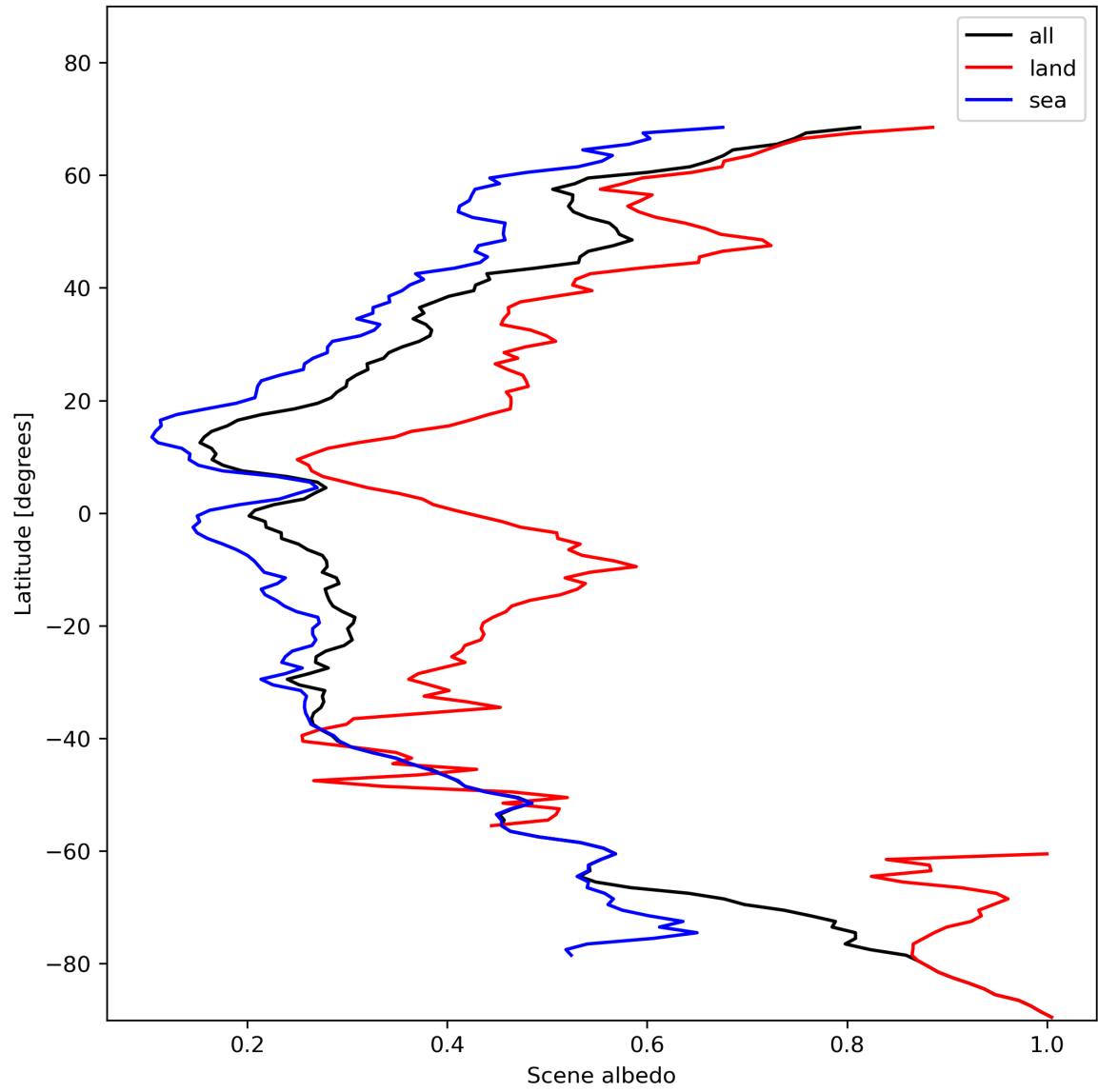
Figure 17: Zonal average of “Scene albedo” for 2024-01-23 to 2024-01-25.
