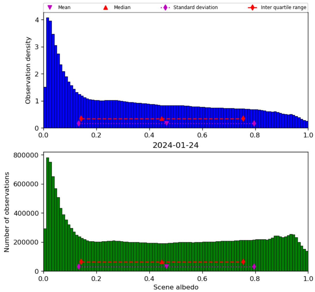
Figure 34: Histogram of “Scene albedo” for 2024-01-23 to 2024-01-25
