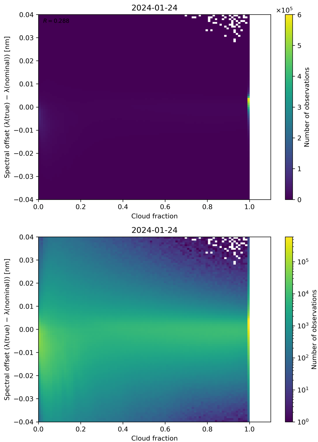
Figure 76: Scatter density plot of “Cloud fraction” against “Spectral offset ( \lambda(\text{true}) - \lambda(\text{nominal}) )” for 2024-01-23 to 2024-01-25.
