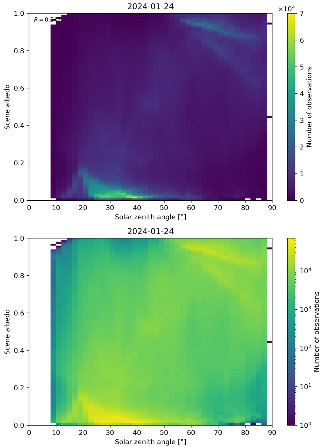
Figure 116: Scatter density plot of “Solar zenith angle” against “Scene albedo” for 2024-01-23 to 2024-01-25.
