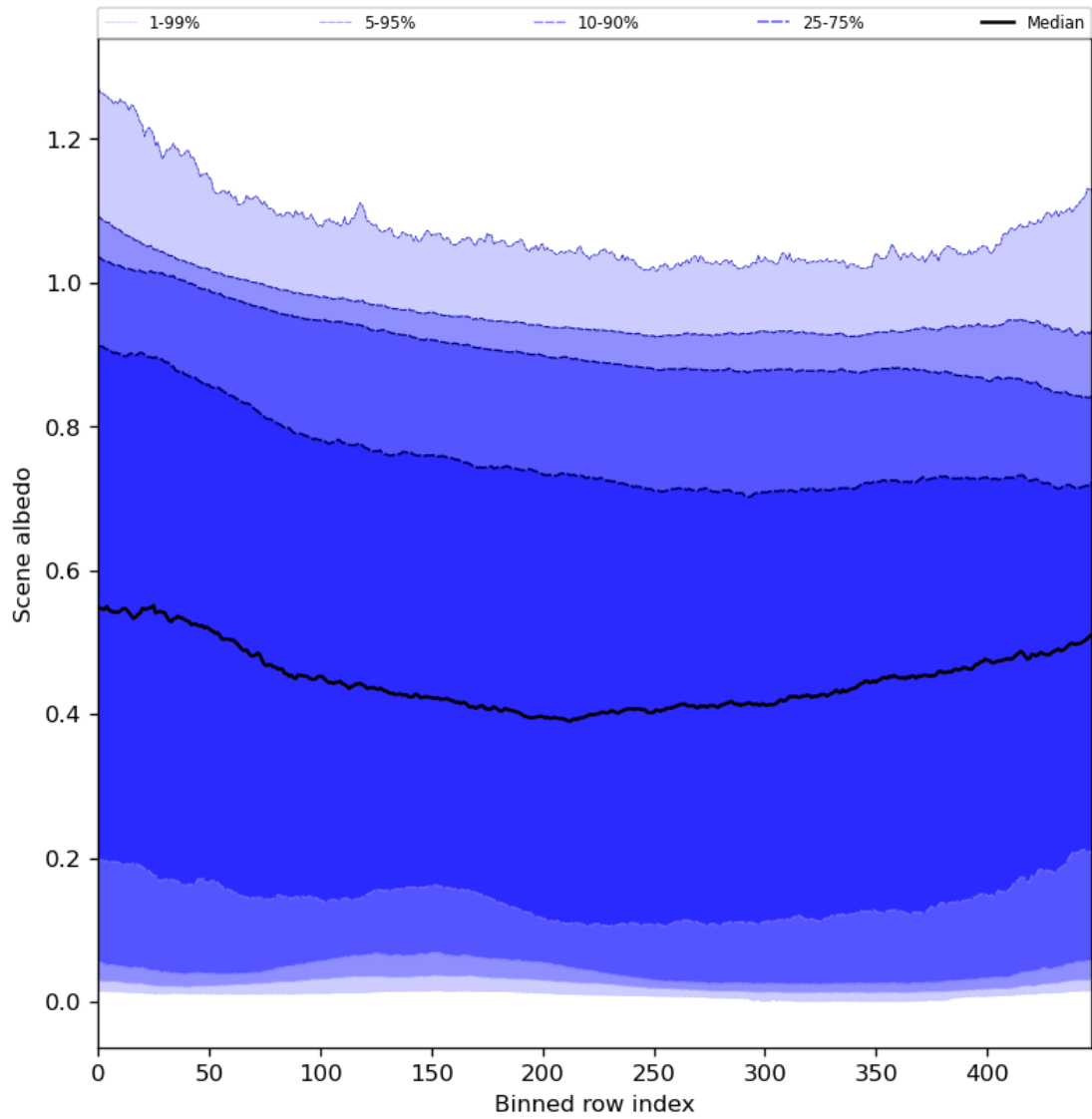
Figure 51: Along track statistics of “Scene albedo” for 2024-01-23 to 2024-01-25
