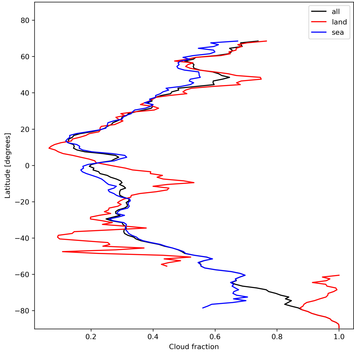
Figure 15: Zonal average of “Cloud fraction” for 2024-01-23 to 2024-01-25.
