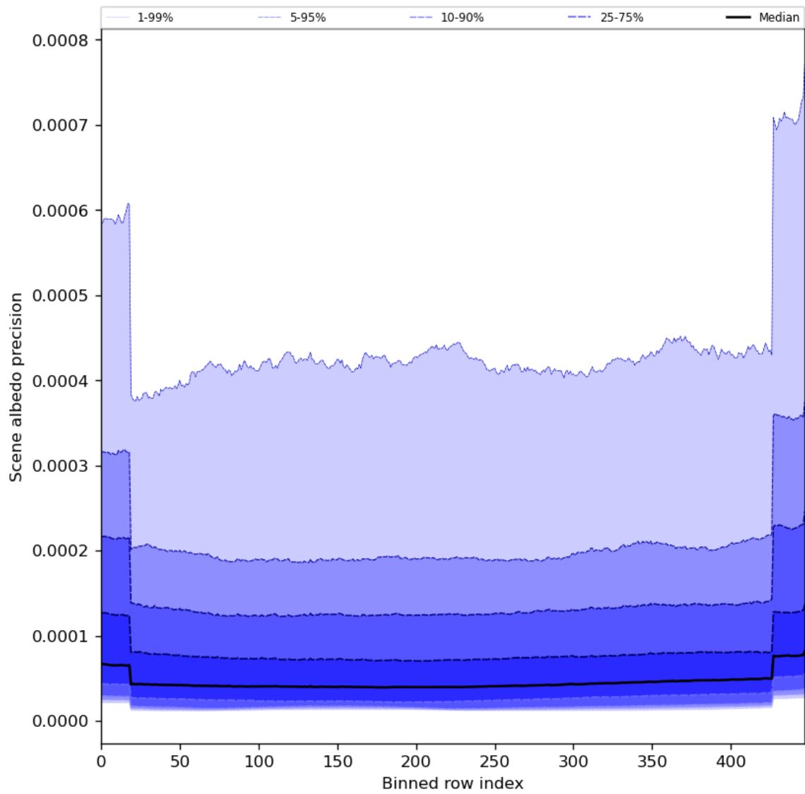
Figure 52: Along track statistics of “Scene albedo precision” for 2024-01-23 to 2024-01-25
