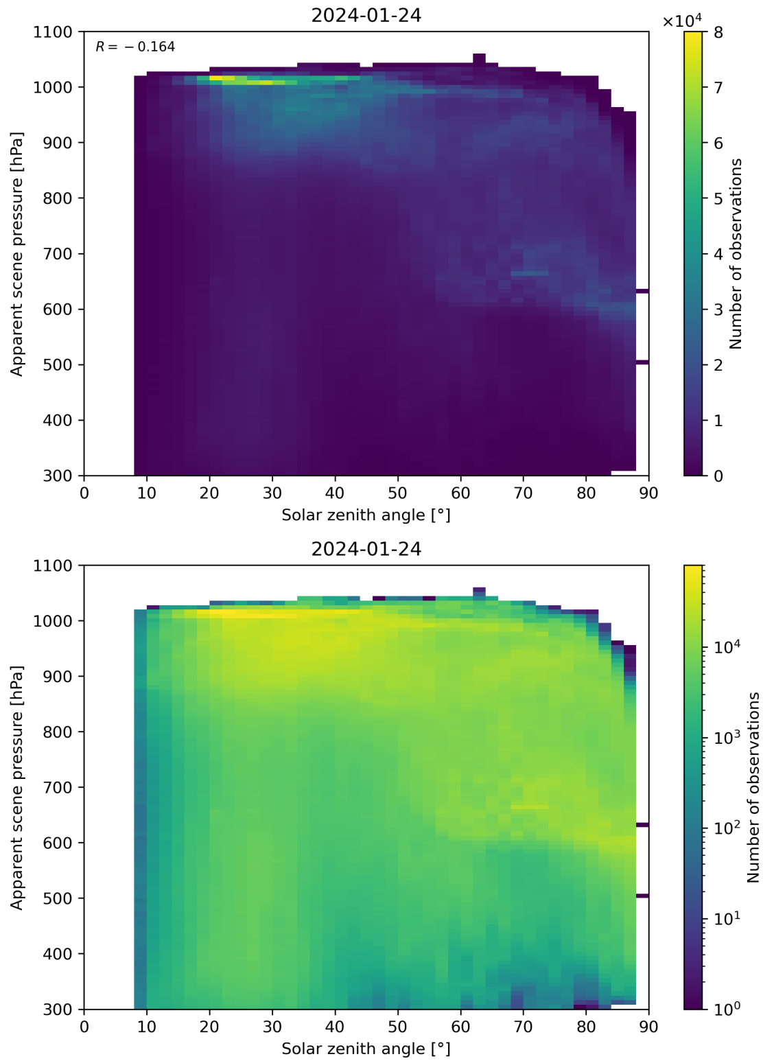
Figure 108: Scatter density plot of “Solar zenith angle” against “Apparent scene pressure” for 2024-01-23 to 2024-01-25.
