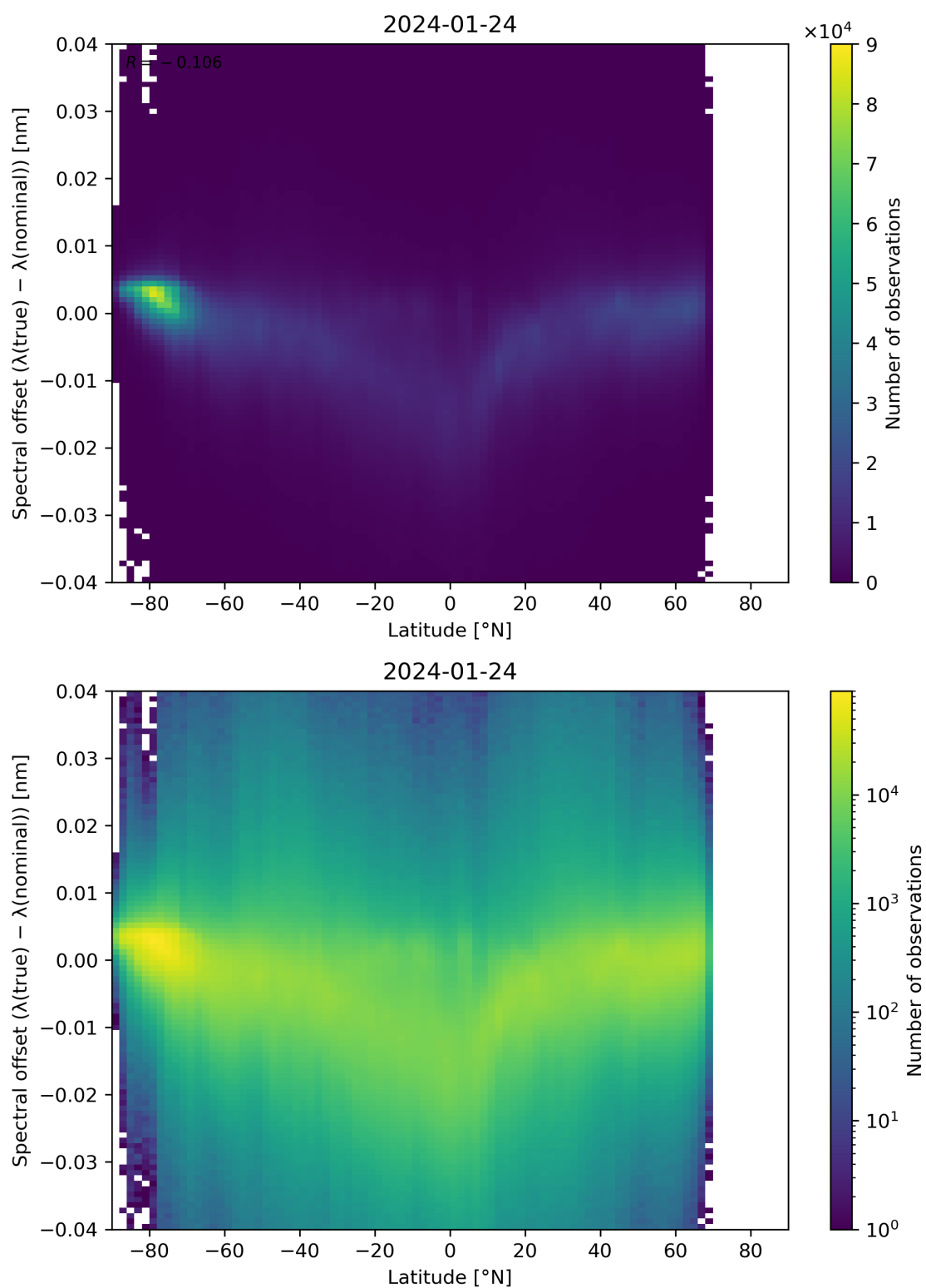
Figure 96: Scatter density plot of “Latitude” against “Spectral offset ( \lambda(\text{true}) - \lambda(\text{nominal}) )” for 2024-01-23 to 2024-01-25.
