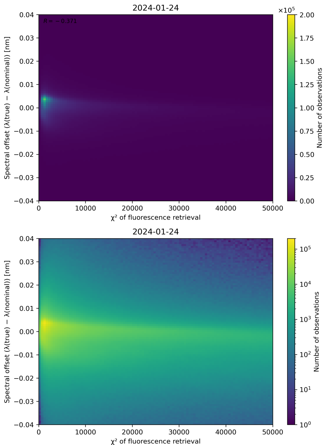
Figure 69: Scatter density plot of " \chi^2 of fluorescence retrieval" against "Spectral offset ( \lambda(\text{true}) - \lambda(\text{nominal}) )" for 2024-01-23 to 2024-01-25.
