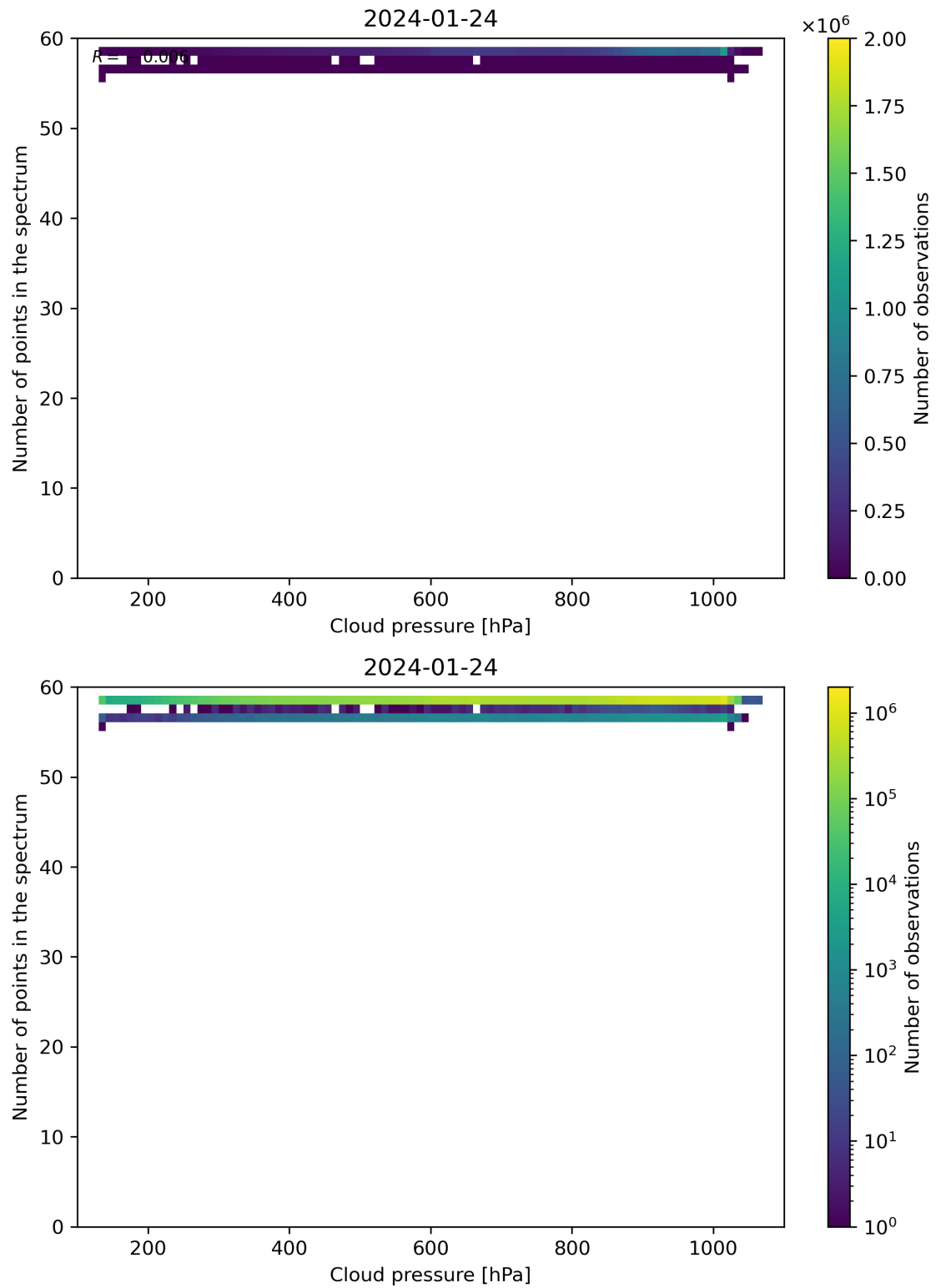
Figure 82: Scatter density plot of “Cloud pressure” against “Number of points in the spectrum” for 2024-01-23 to 2024-01-25.
