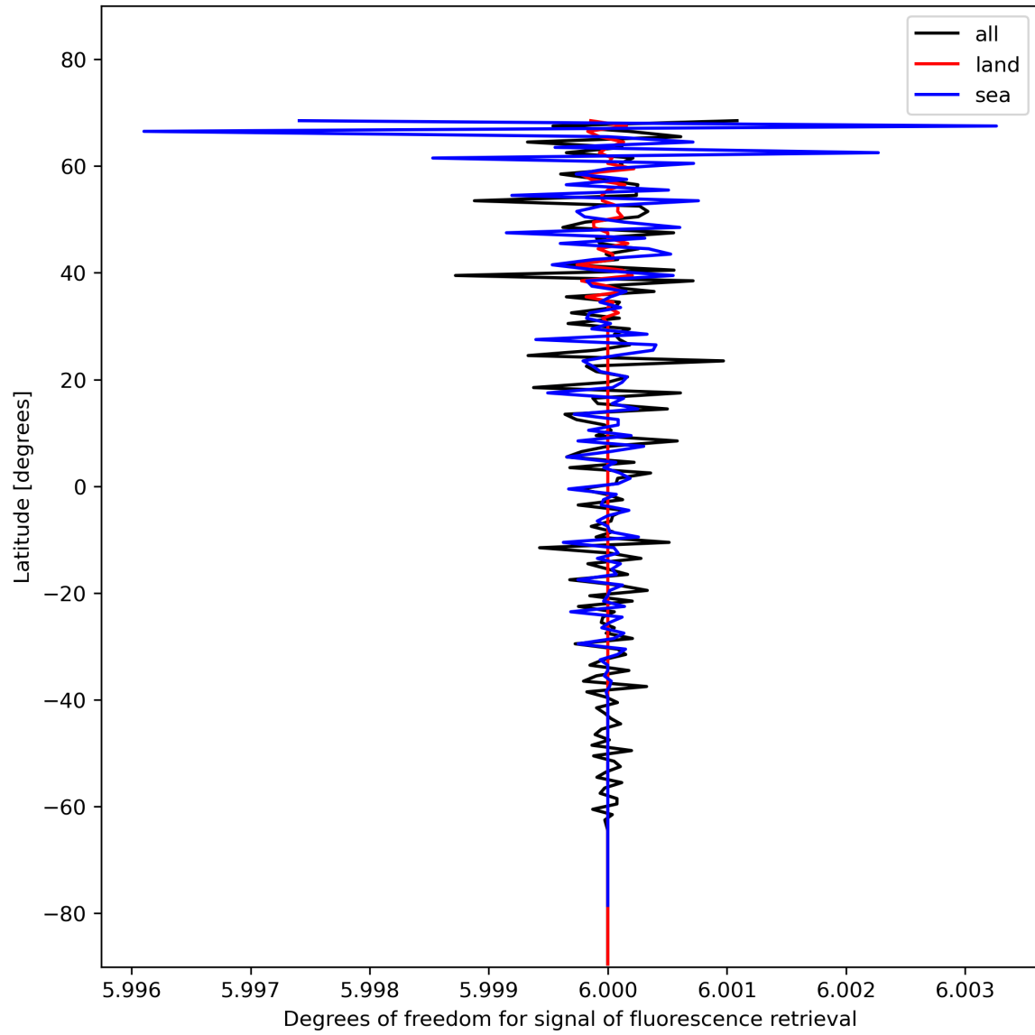
Figure 26: Zonal average of “Degrees of freedom for signal of fluorescence retrieval” for 2024-01-23 to 2024-01-25.
