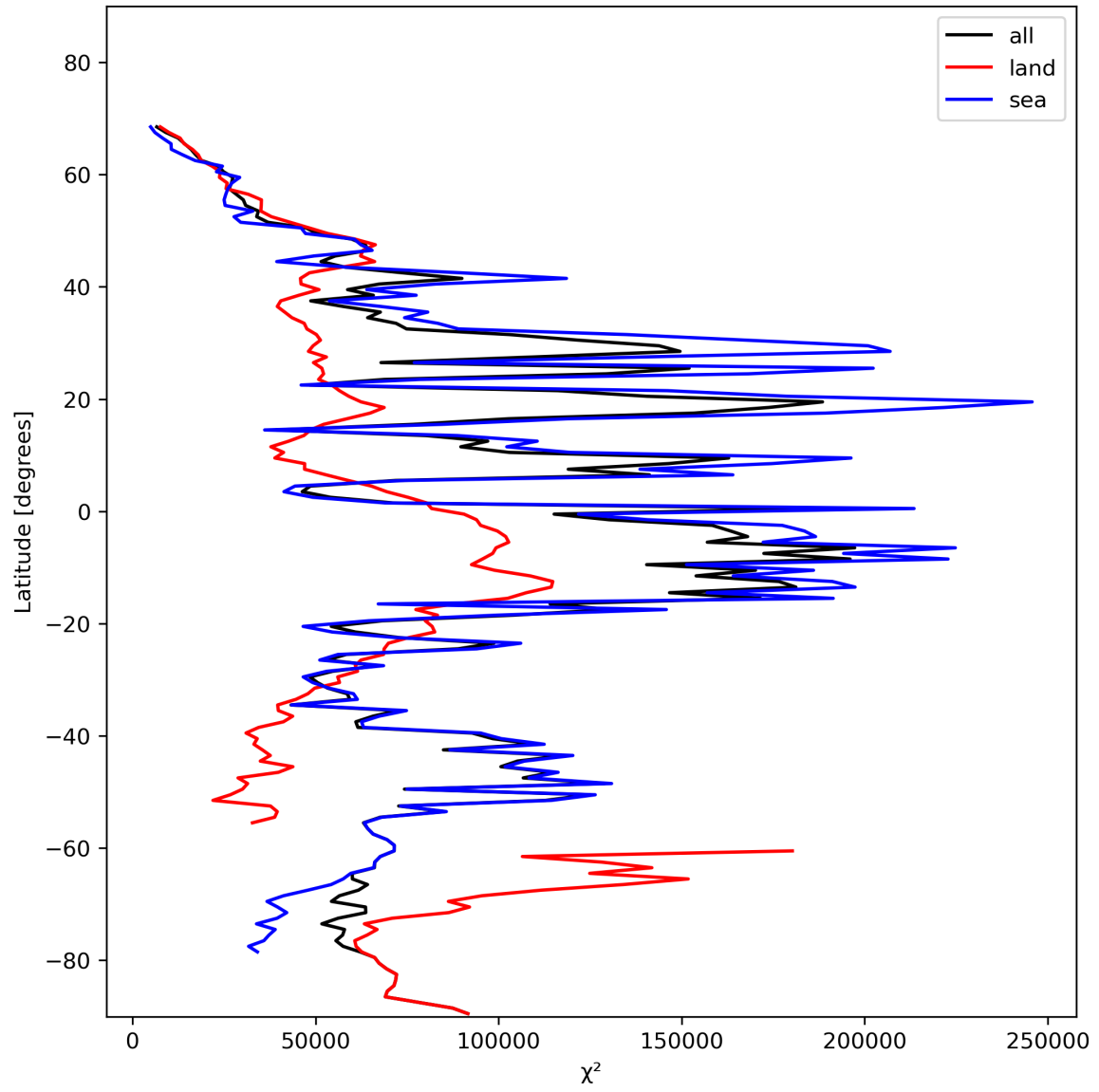
Figure 21: Zonal average of “ \chi^2 ” for 2024-01-23 to 2024-01-25.
