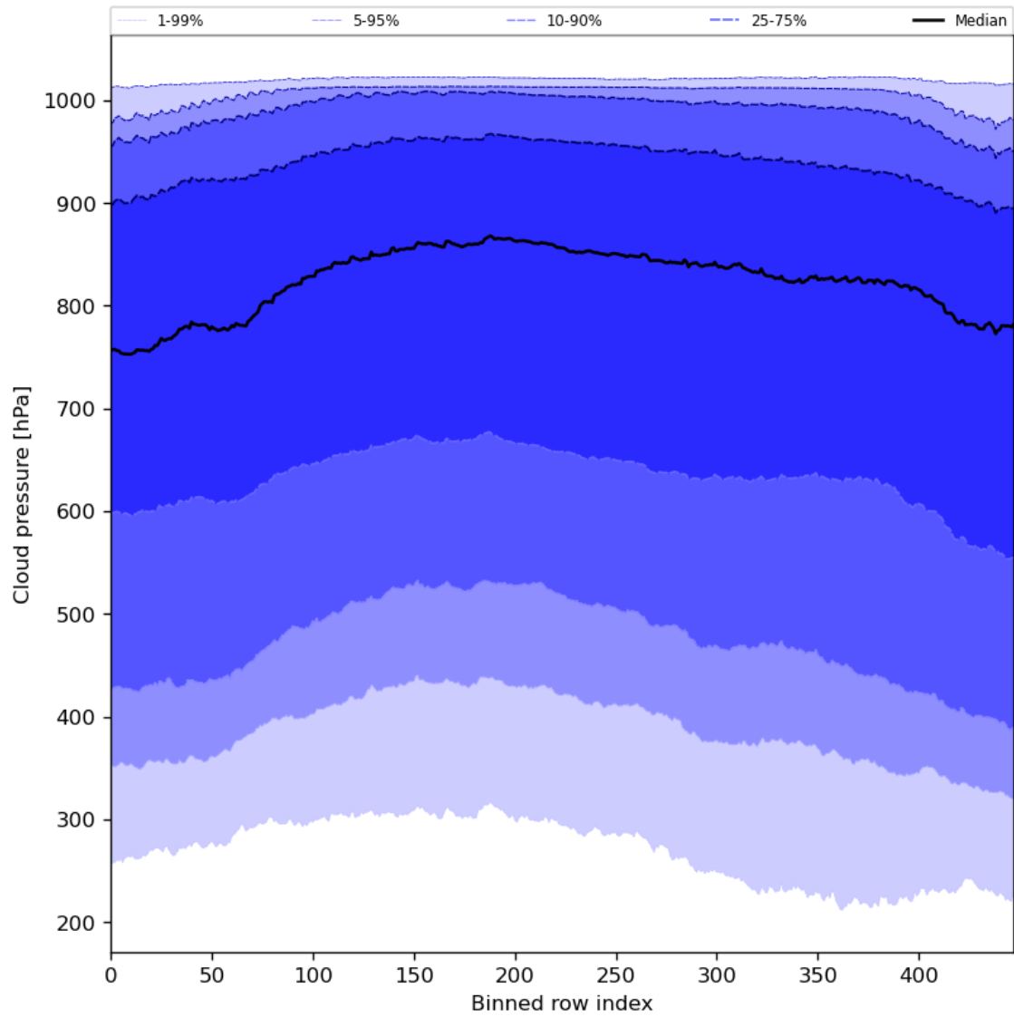
Figure 47: Along track statistics of “Cloud pressure” for 2024-01-23 to 2024-01-25
