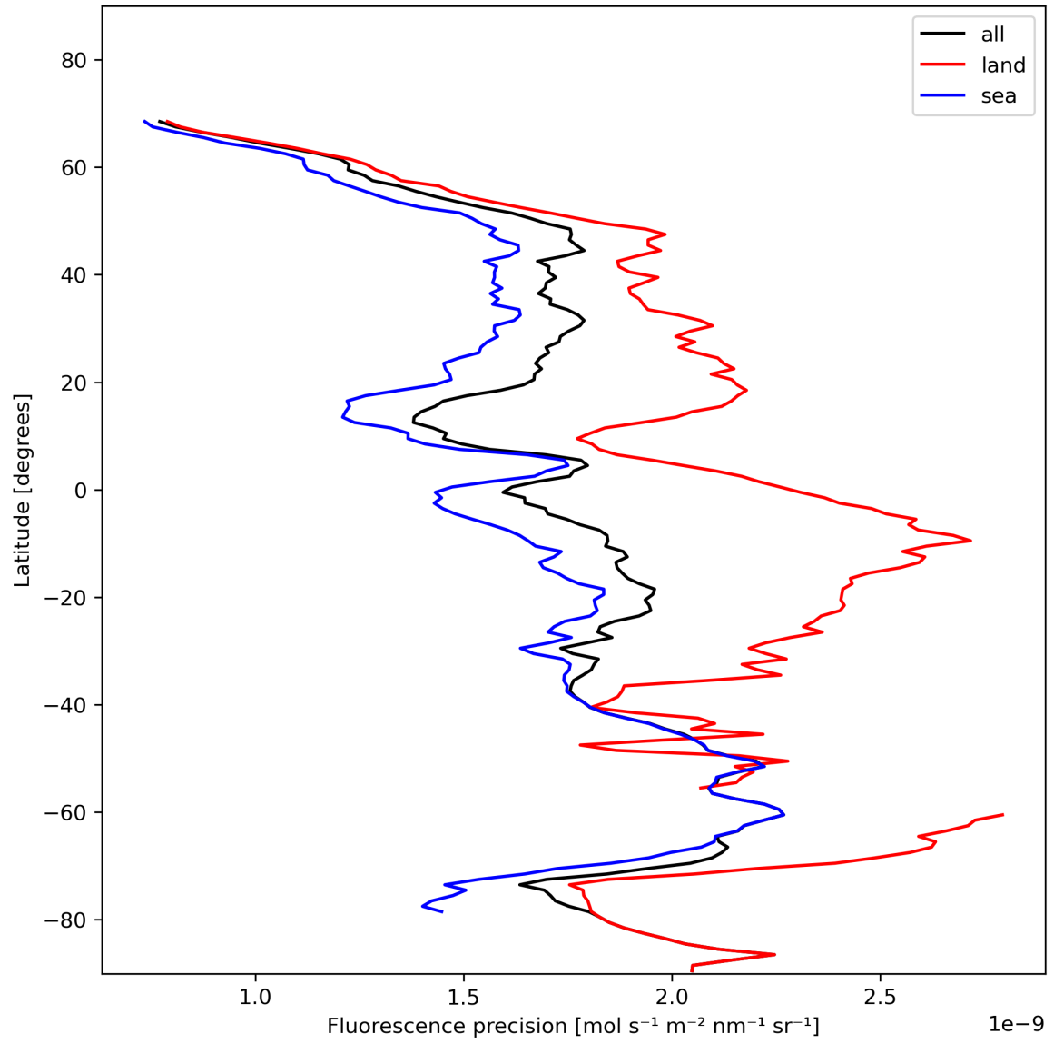
Figure 24: Zonal average of “Fluorescence precision” for 2024-01-23 to 2024-01-25.
