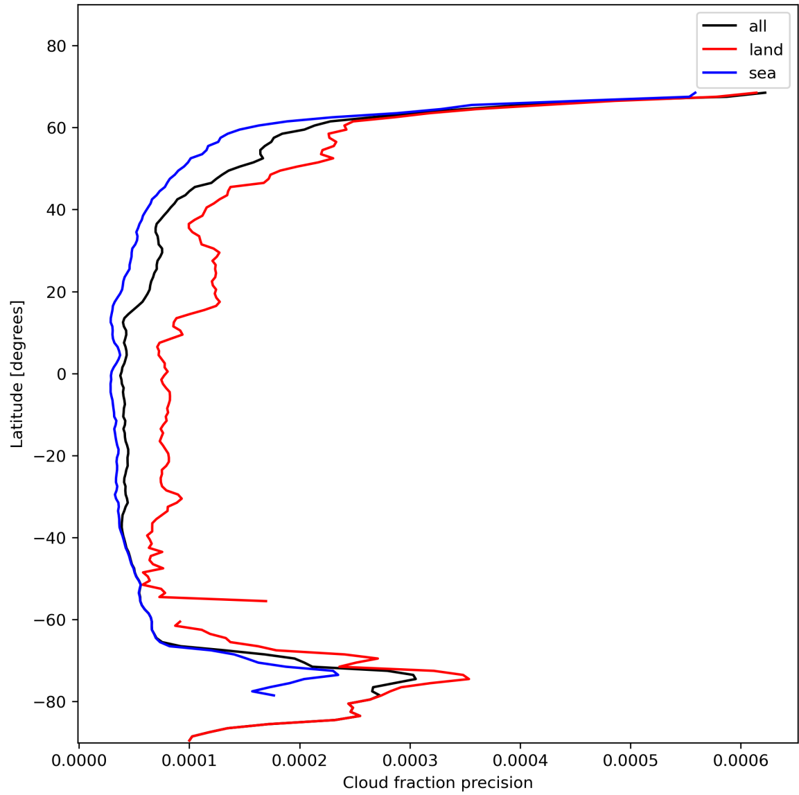
Figure 16: Zonal average of “Cloud fraction precision” for 2024-01-23 to 2024-01-25.
