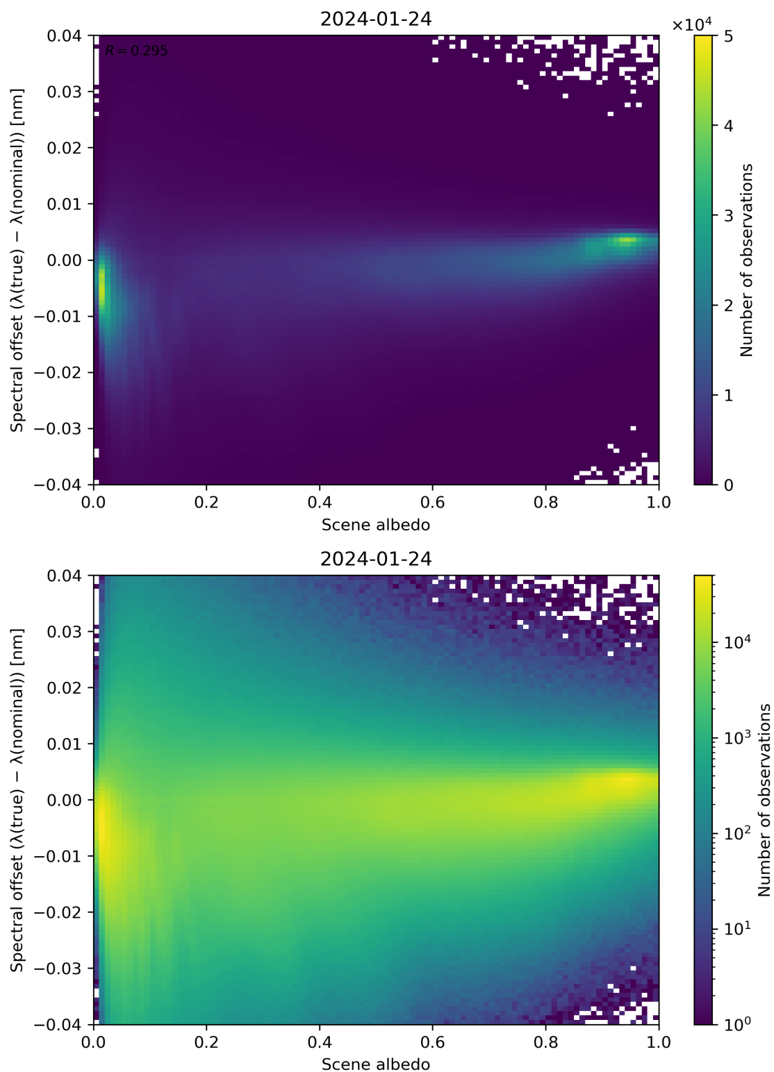
Figure 107: Scatter density plot of “Scene albedo” against “Spectral offset ( \lambda(\text{true}) - \lambda(\text{nominal}) )” for 2024-01-23 to 2024-01-25.
