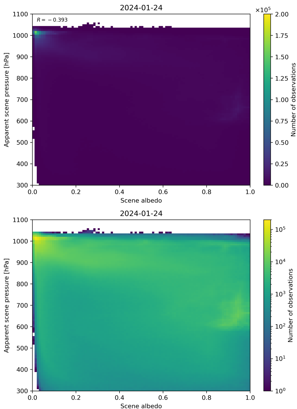
Figure 102: Scatter density plot of “Scene albedo” against “Apparent scene pressure” for 2024-01-23 to 2024-01-25.
