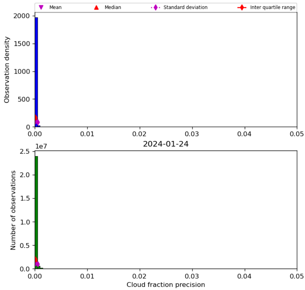
Figure 33: Histogram of “Cloud fraction precision” for 2024-01-23 to 2024-01-25
