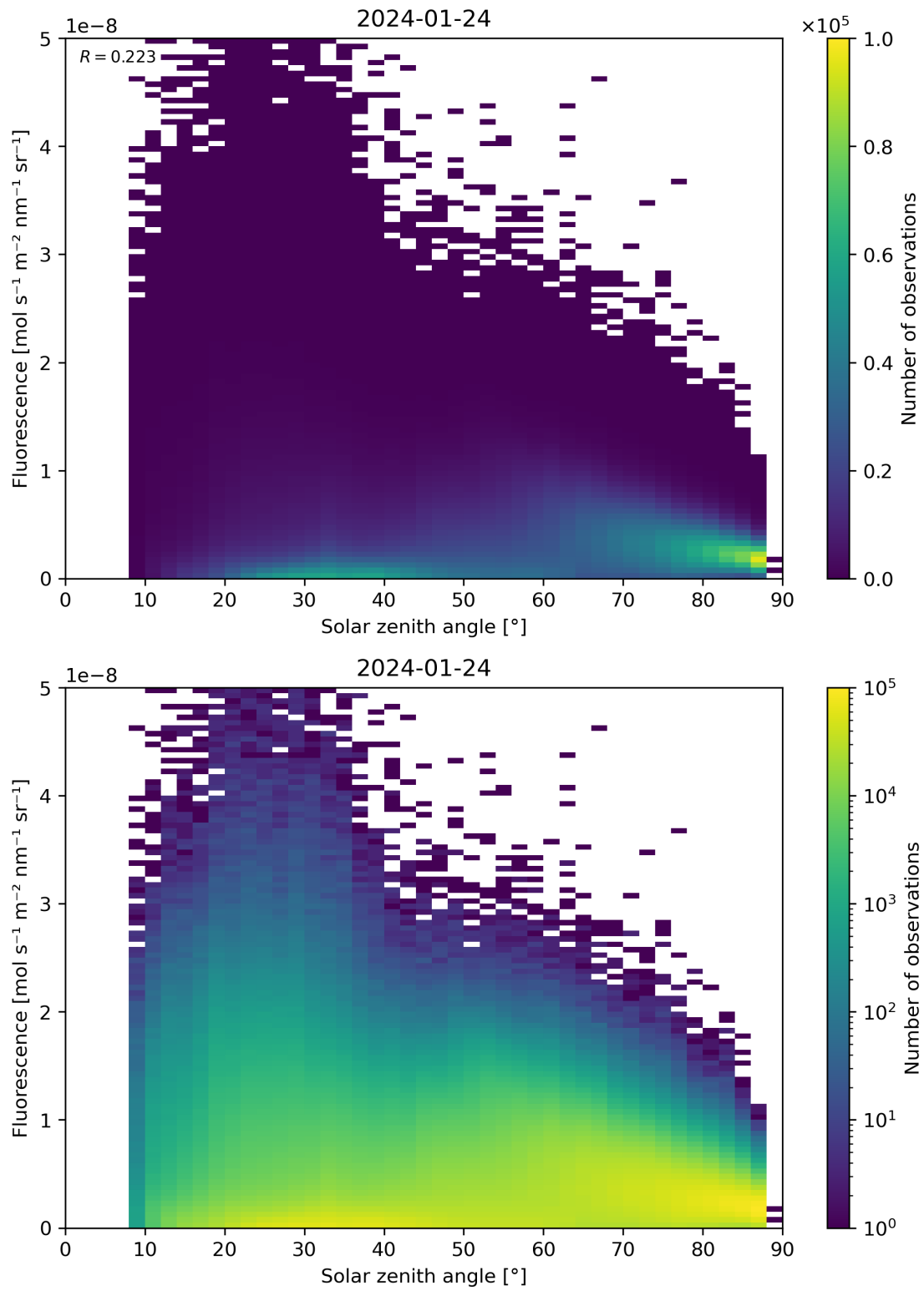
Figure 112: Scatter density plot of “Solar zenith angle” against “Fluorescence” for 2024-01-23 to 2024-01-25.
