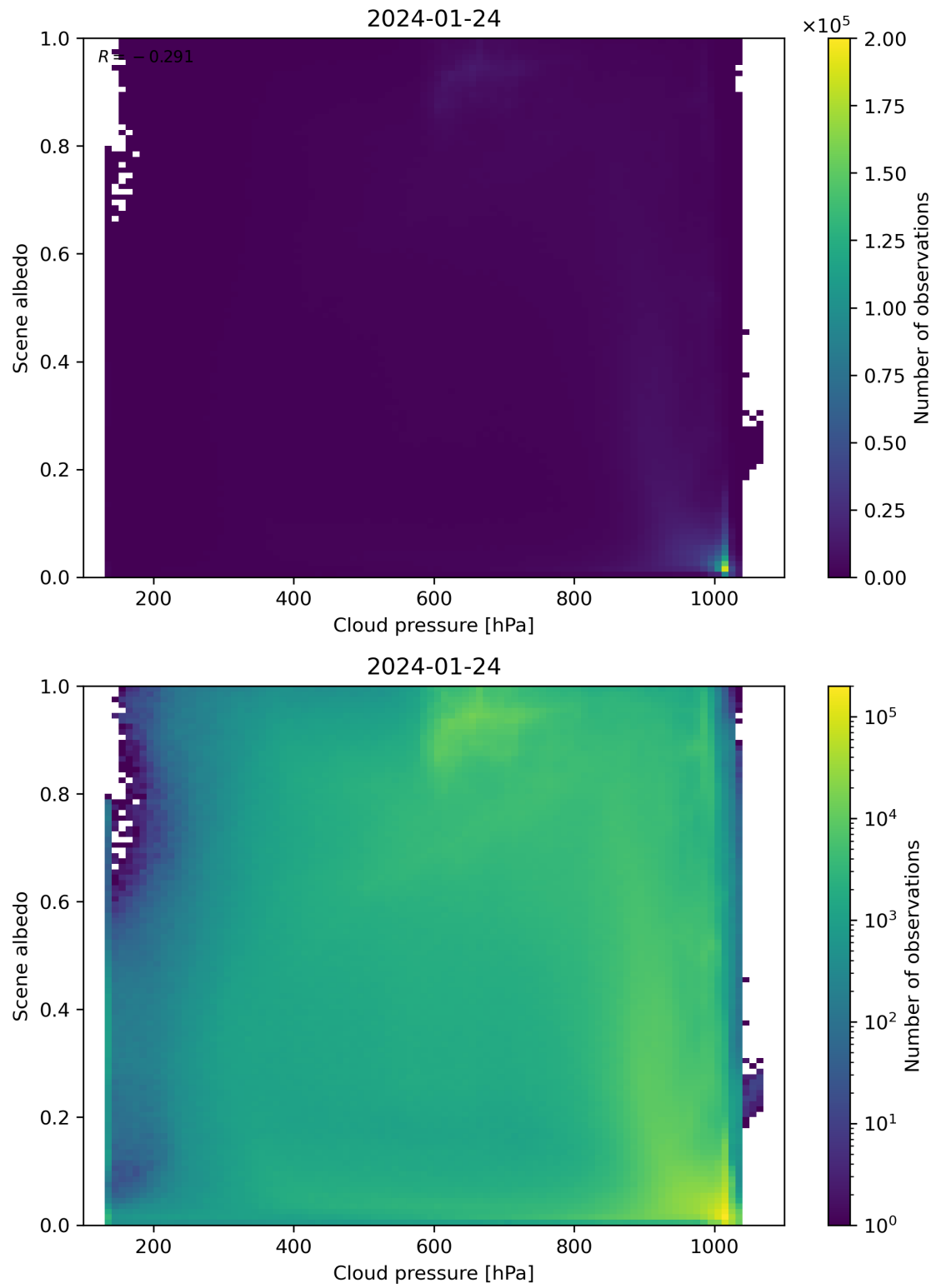
Figure 83: Scatter density plot of “Cloud pressure” against “Scene albedo” for 2024-01-23 to 2024-01-25.
