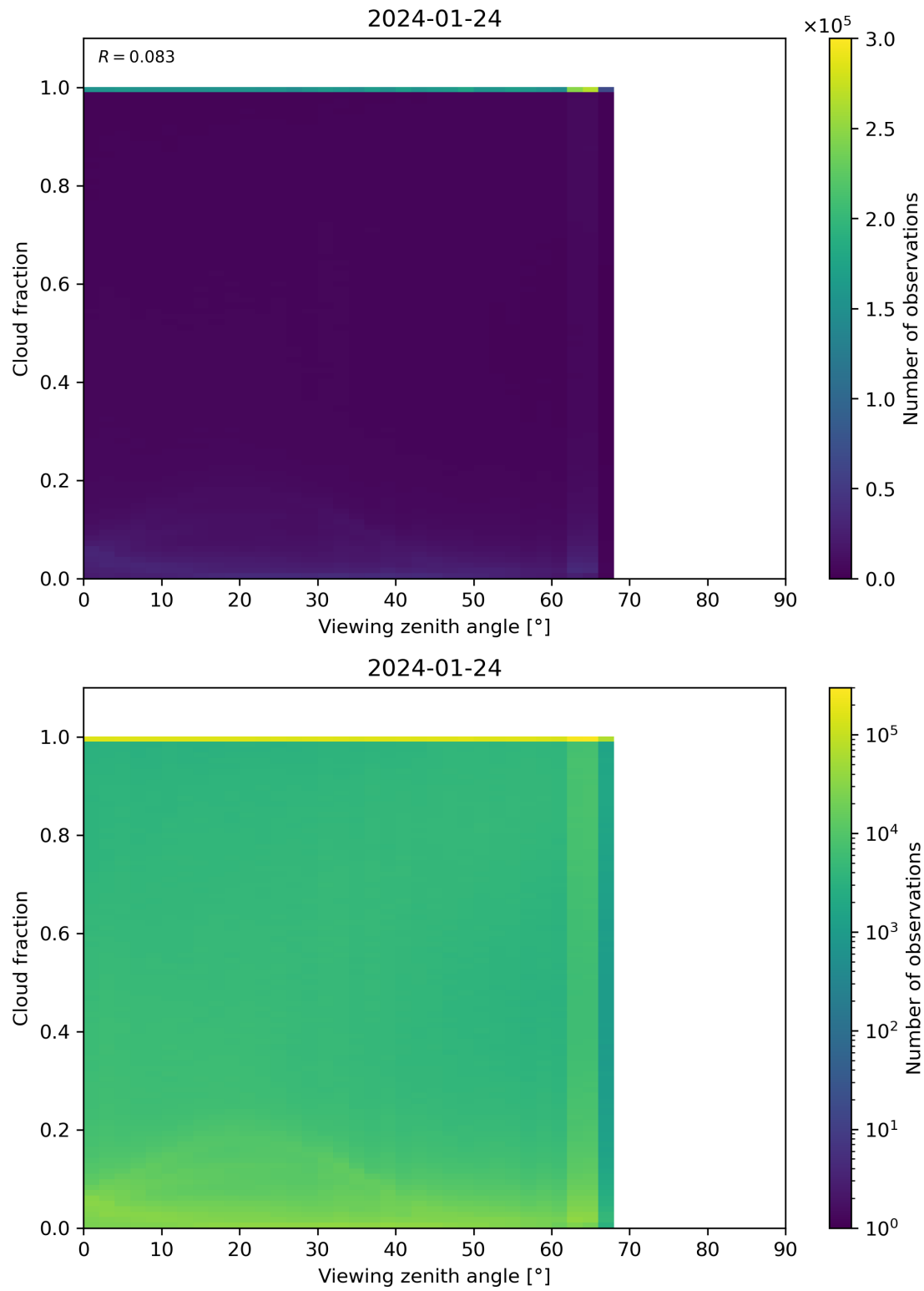
Figure 120: Scatter density plot of “Viewing zenith angle” against “Cloud fraction” for 2024-01-23 to 2024-01-25.
