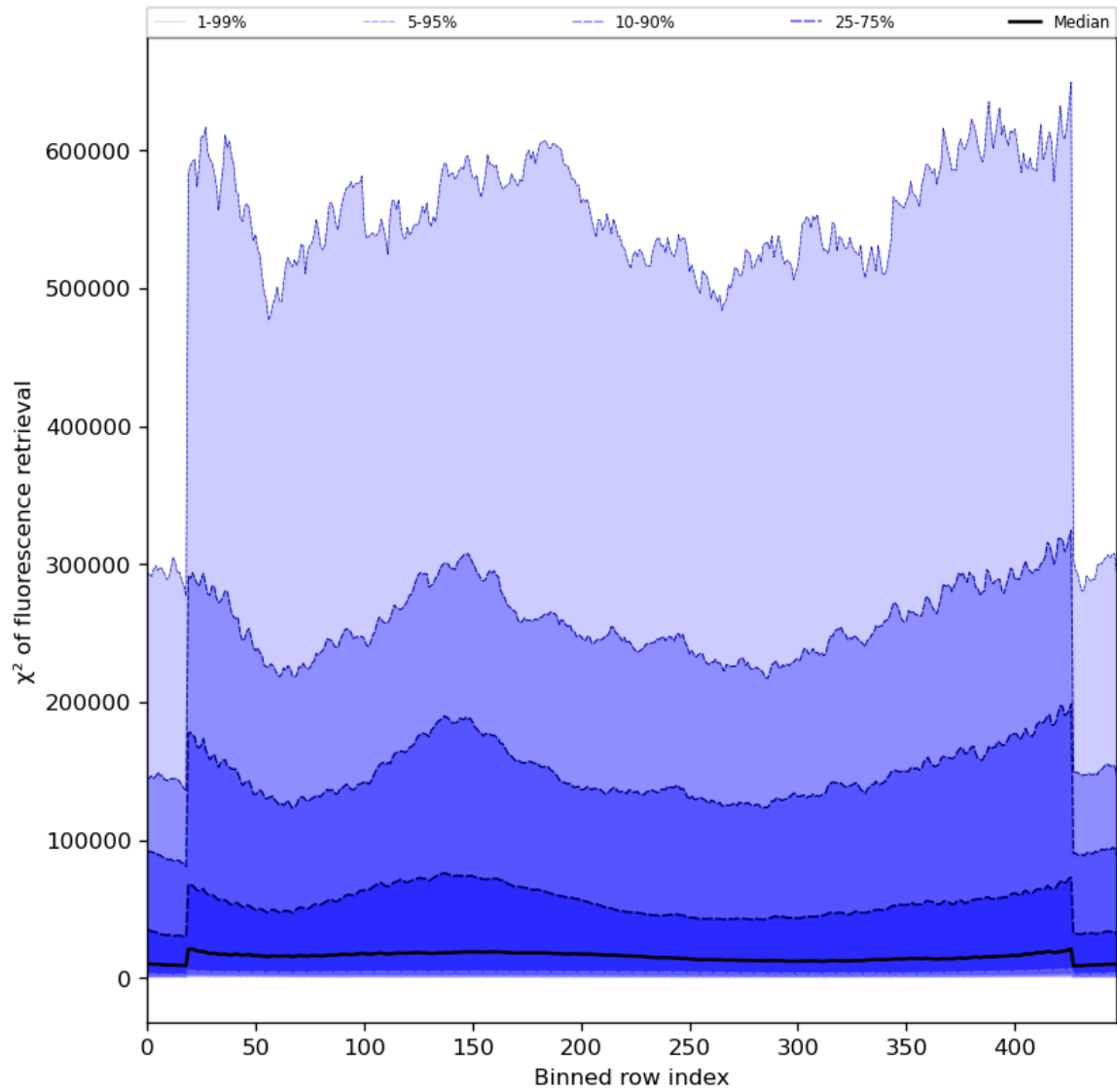
Figure 59: Along track statistics of “ \chi^2 of fluorescence retrieval” for 2024-01-23 to 2024-01-25
