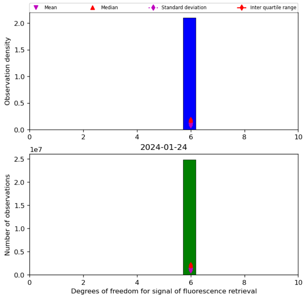
Figure 43: Histogram of “Degrees of freedom for signal of fluorescence retrieval” for 2024-01-23 to 2024-01-25
