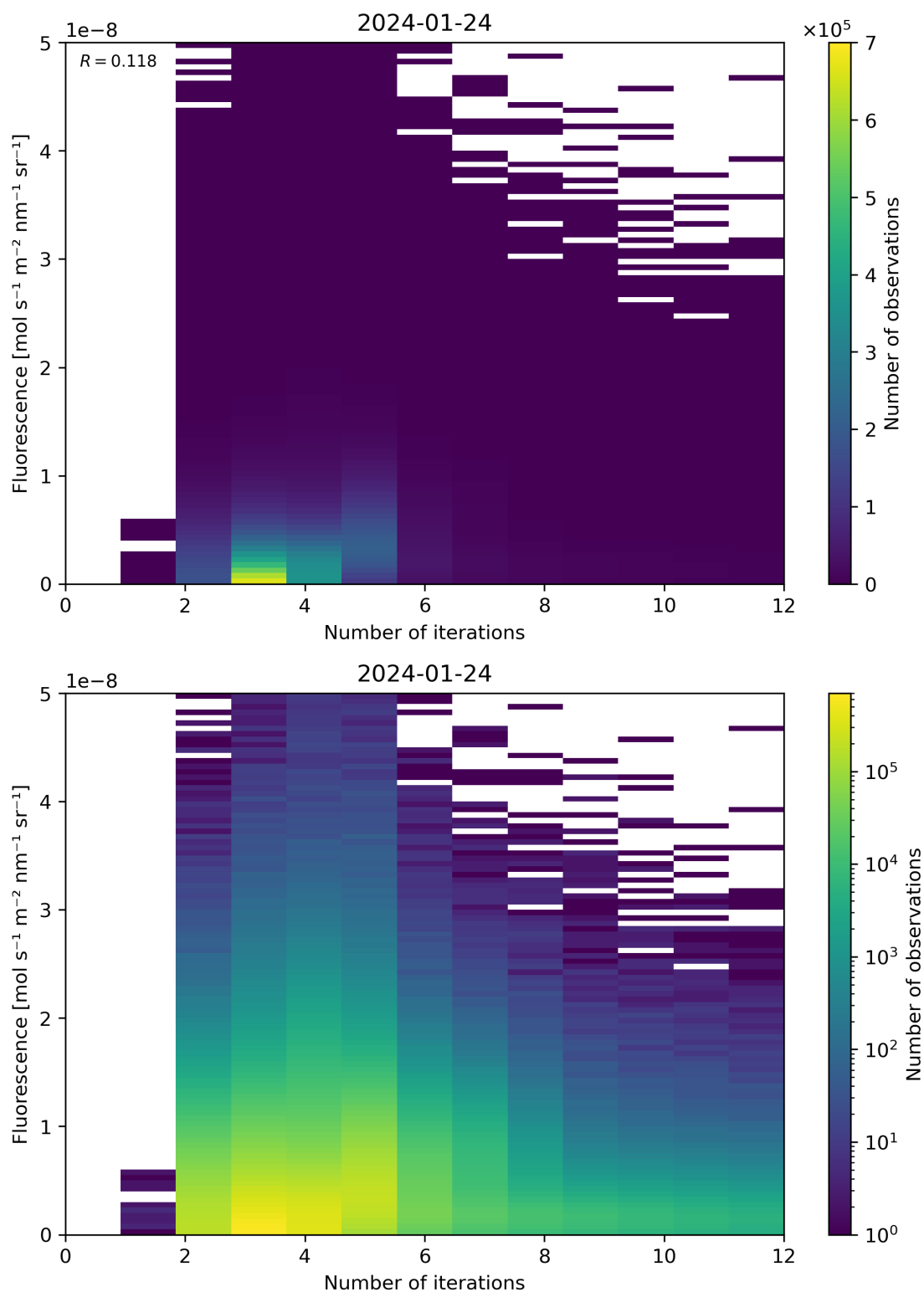
Figure 98: Scatter density plot of “Number of iterations” against “Fluorescence” for 2024-01-23 to 2024-01-25.
