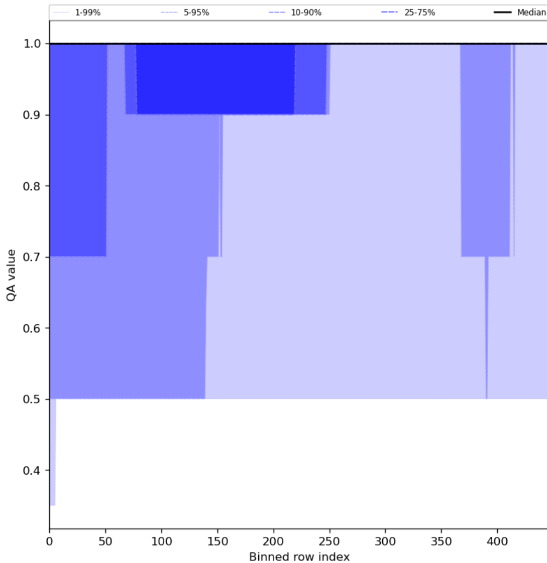
Figure 46: Along track statistics of “QA value” for 2024-01-23 to 2024-01-25
