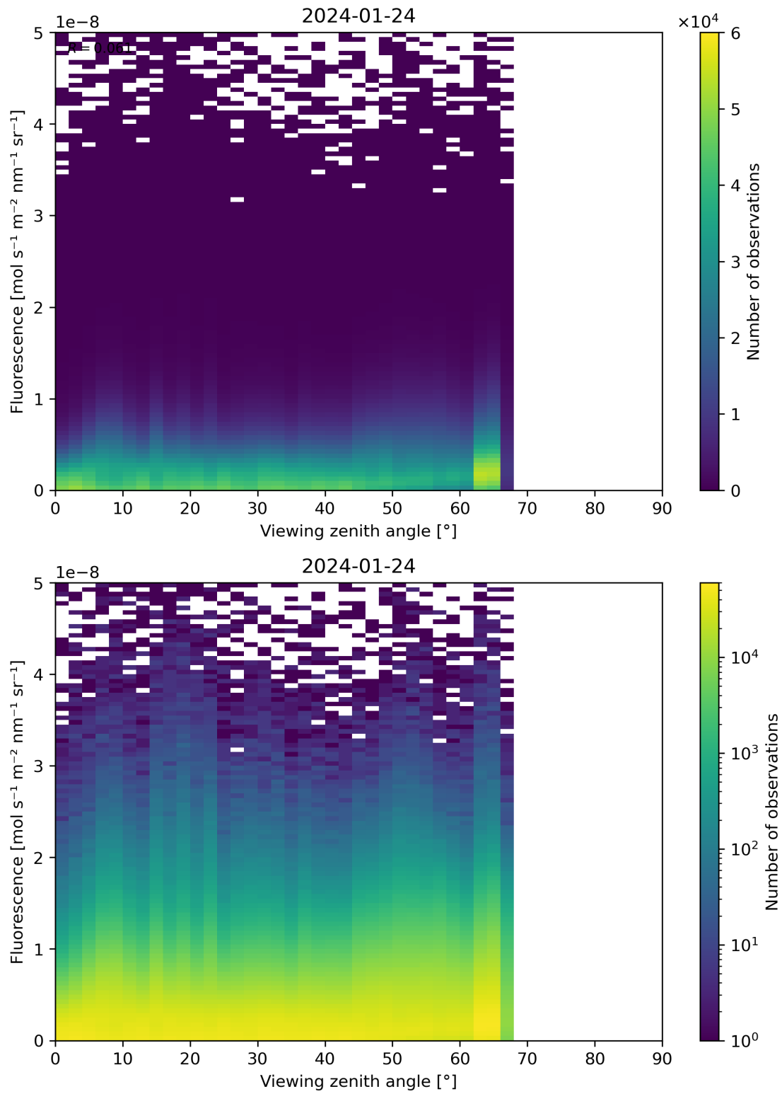
Figure 122: Scatter density plot of “Viewing zenith angle” against “Fluorescence” for 2024-01-23 to 2024-01-25.
