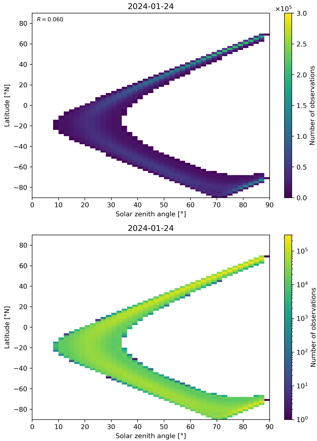
Figure 113: Scatter density plot of “Solar zenith angle” against “Latitude” for 2024-01-23 to 2024-01-25.
