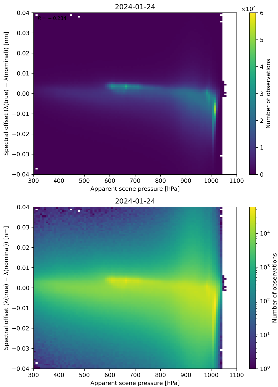
Figure 67: Scatter density plot of “Apparent scene pressure” against “Spectral offset ( \lambda(\text{true}) - \lambda(\text{nominal}) )” for 2024-01-23 to 2024-01-25.
