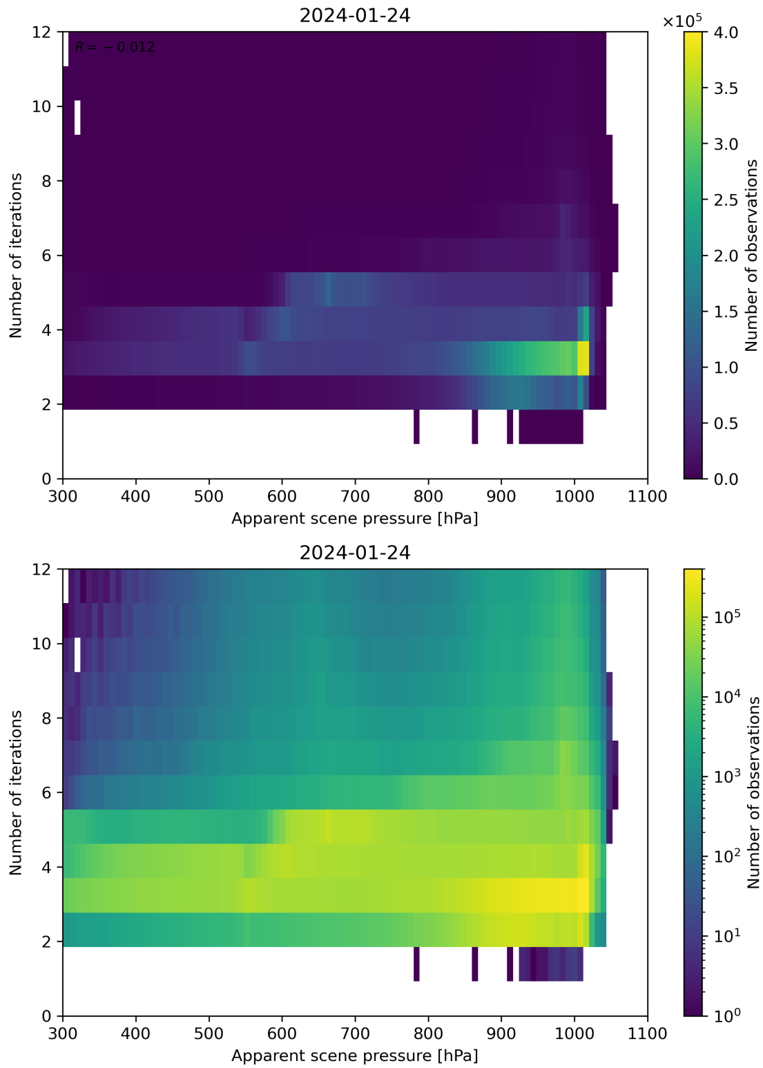
Figure 65: Scatter density plot of “Apparent scene pressure” against “Number of iterations” for 2024-01-23 to 2024-01-25.
