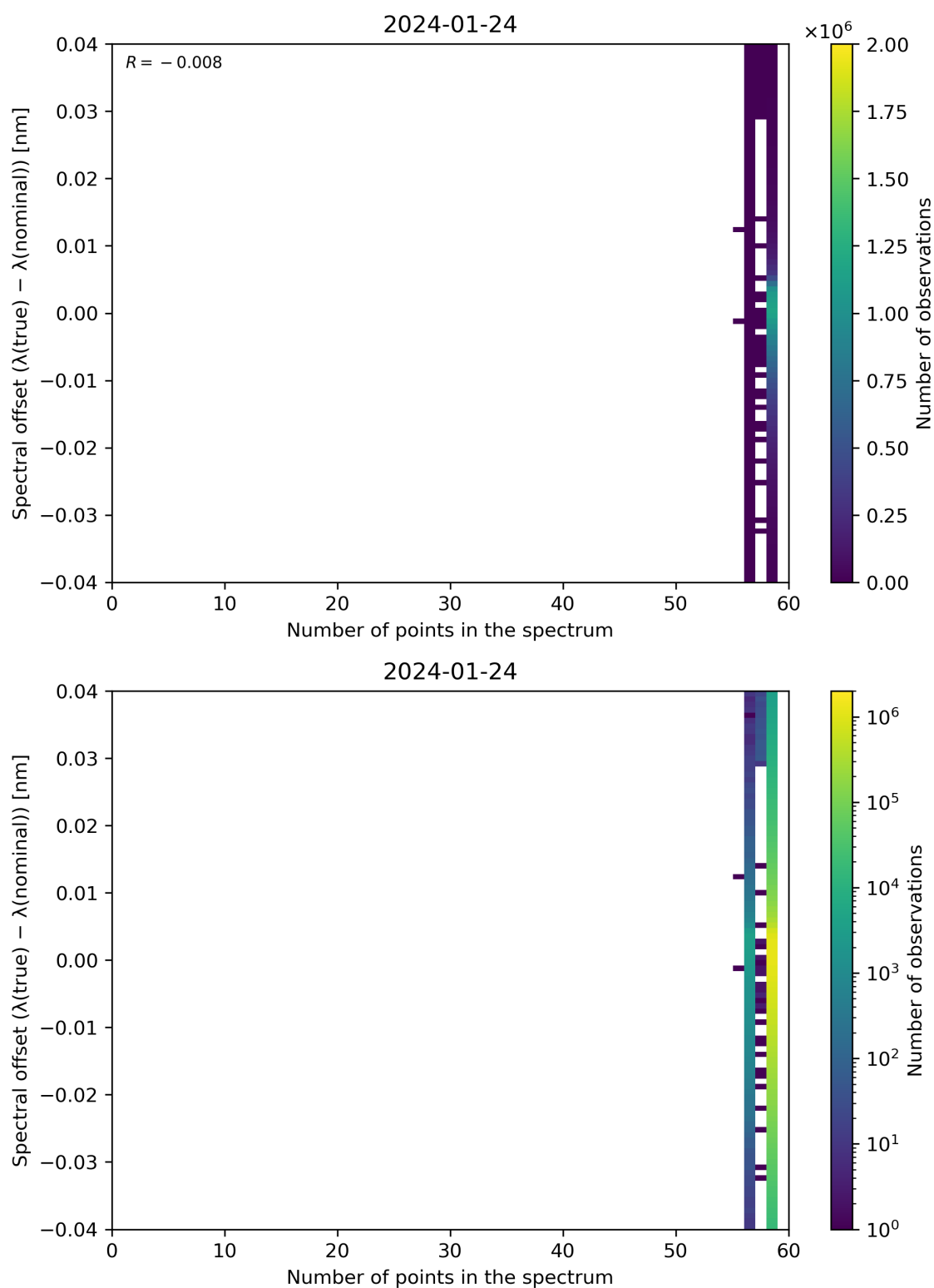
Figure 101: Scatter density plot of “Number of points in the spectrum” against “Spectral offset ( \lambda(\text{true}) - \lambda(\text{nominal}) )” for 2024-01-23 to 2024-01-25.
