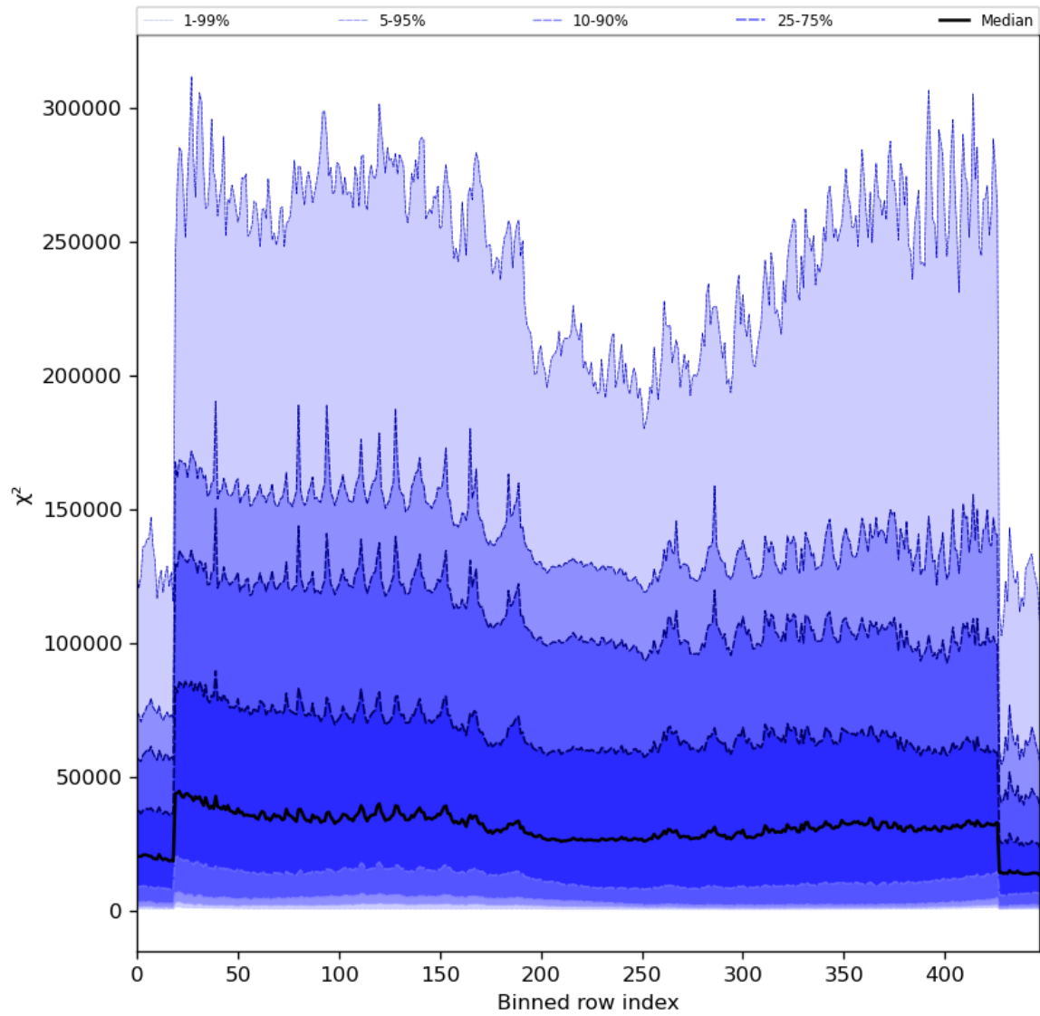
Figure 55: Along track statistics of “ \chi^2 ” for 2024-01-23 to 2024-01-25
