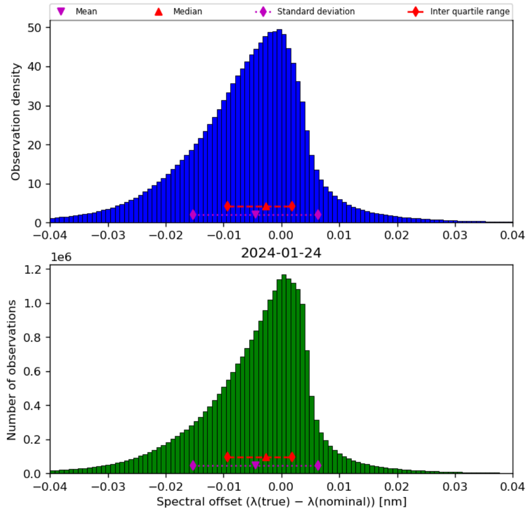
Figure 45: Histogram of “Spectral offset ( \lambda(\text{true}) - \lambda(\text{nominal}) )” for 2024-01-23 to 2024-01-25
