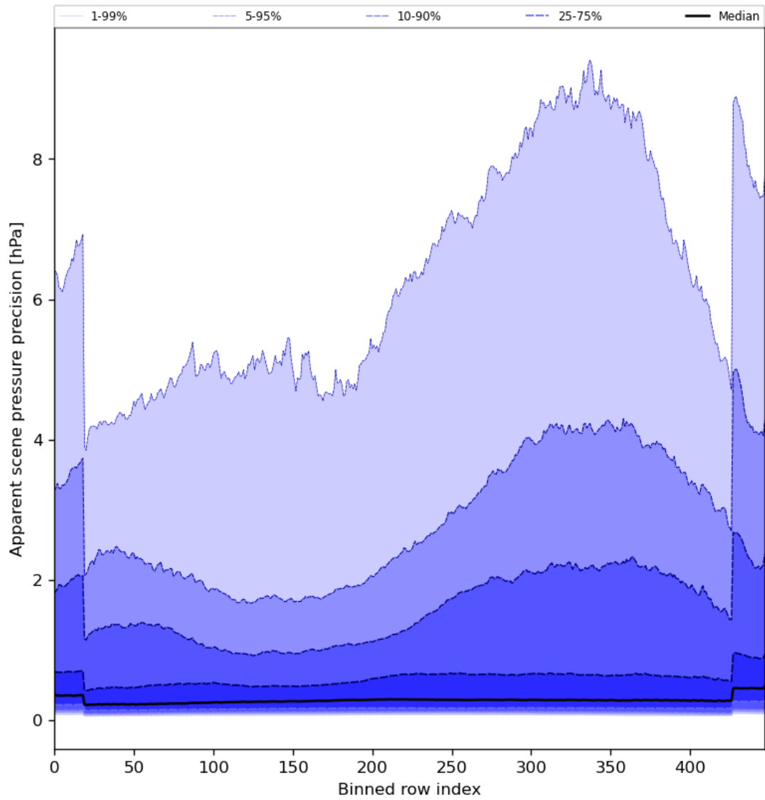
Figure 54: Along track statistics of “Apparent scene pressure precision” for 2024-01-23 to 2024-01-25
