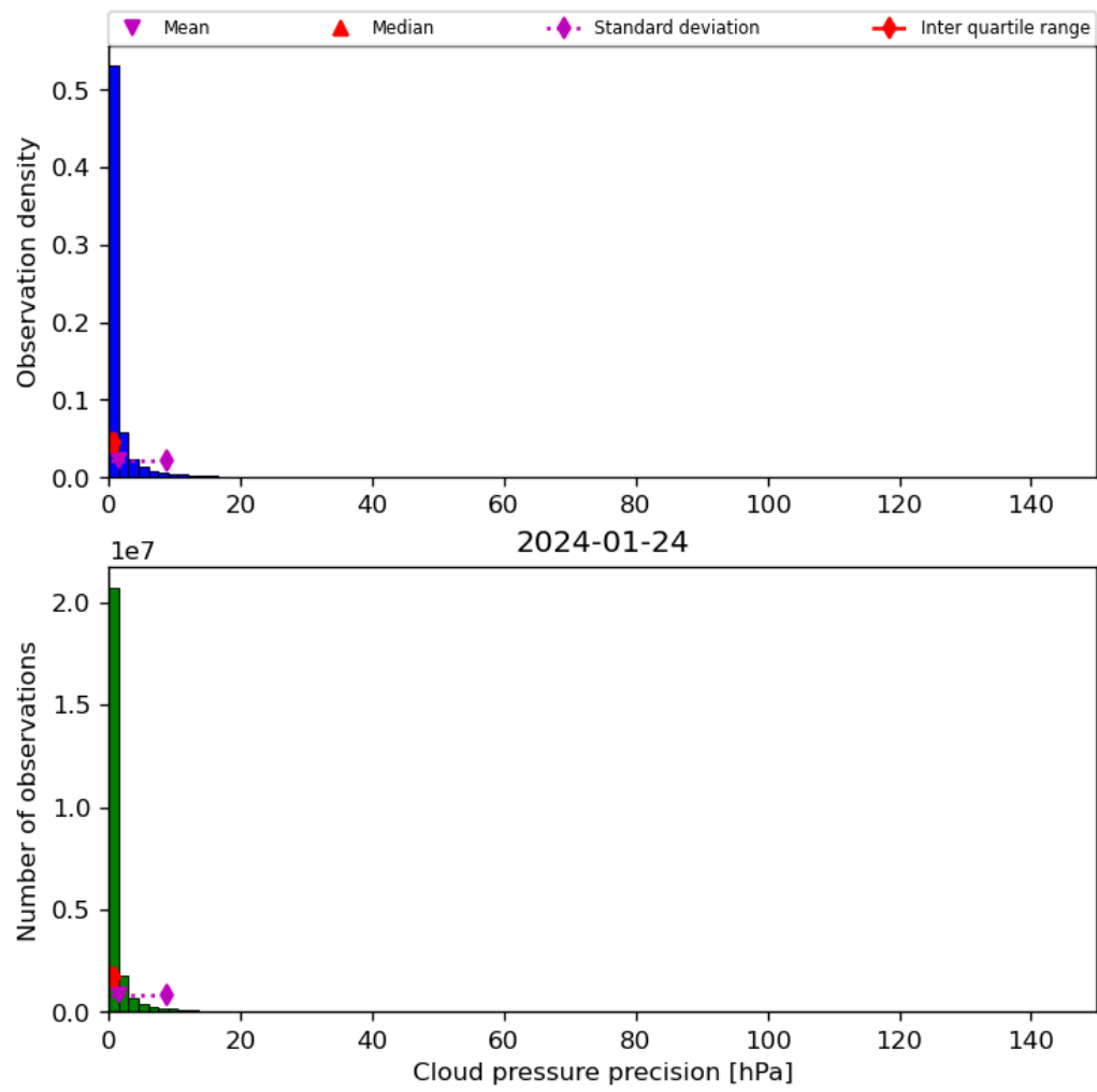
Figure 31: Histogram of “Cloud pressure precision” for 2024-01-23 to 2024-01-25
