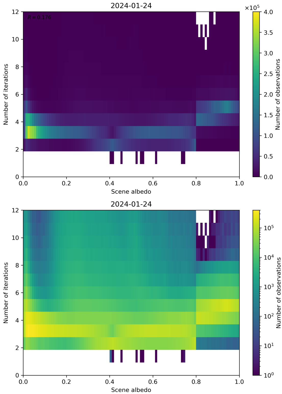
Figure 105: Scatter density plot of “Scene albedo” against “Number of iterations” for 2024-01-23 to 2024-01-25.
