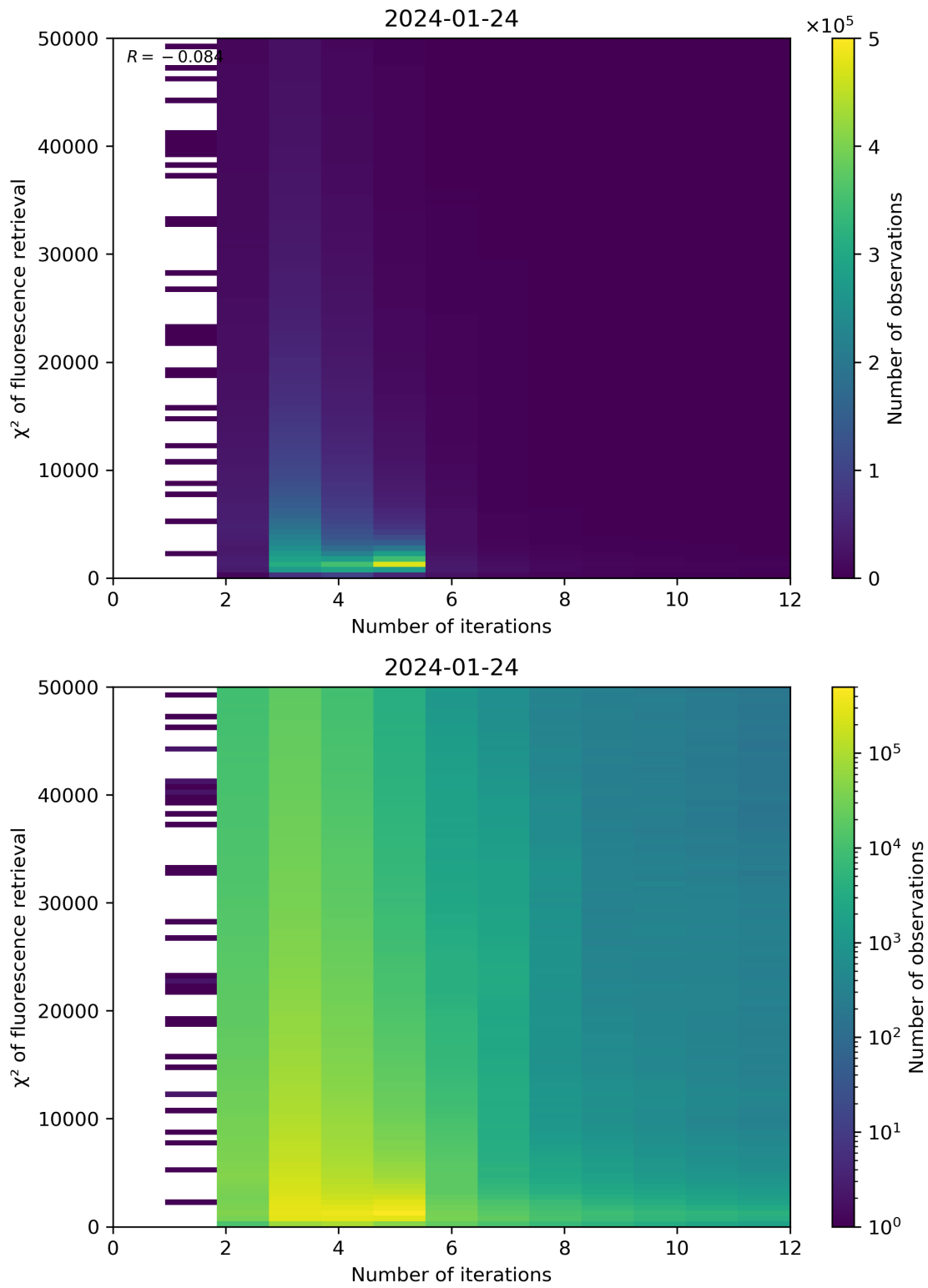
Figure 97: Scatter density plot of “Number of iterations” against “ \chi^2 of fluorescence retrieval” for 2024-01-23 to 2024-01-25.
