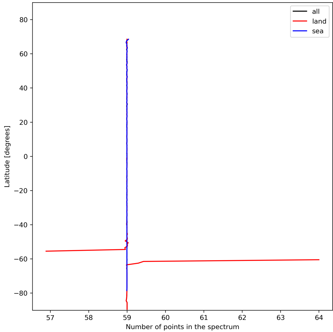
Figure 27: Zonal average of “Number of points in the spectrum” for 2024-01-23 to 2024-01-25.
