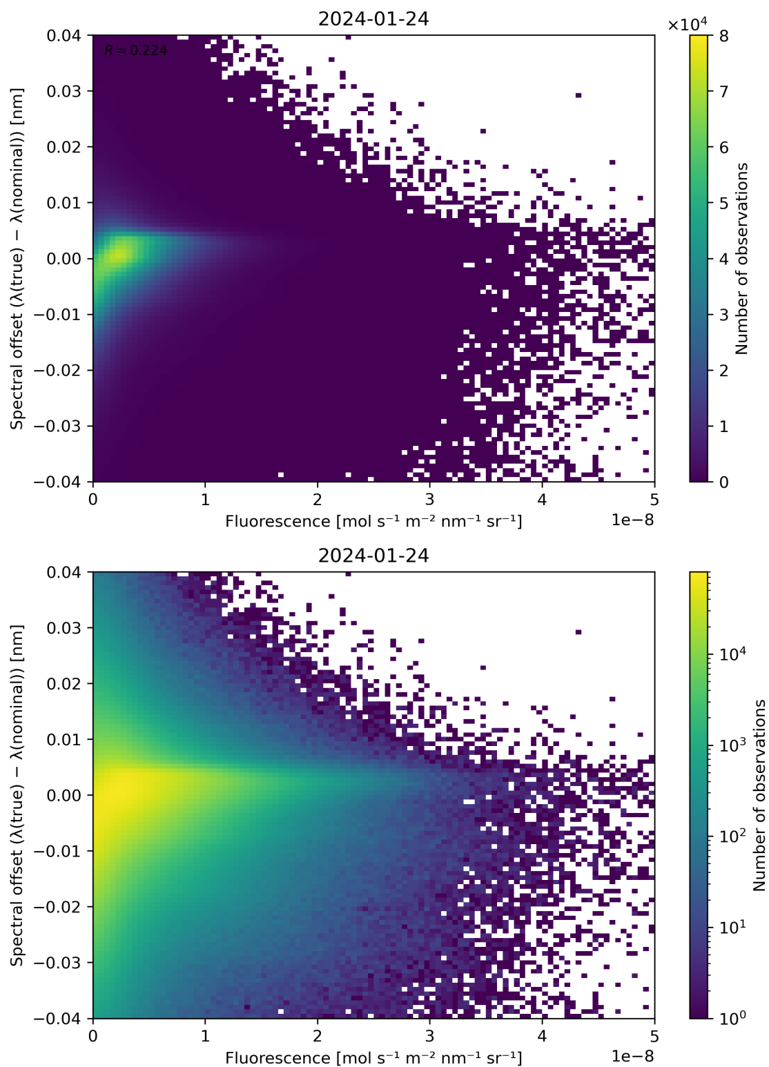
Figure 87: Scatter density plot of “Fluorescence” against “Spectral offset ( \lambda(\text{true}) - \lambda(\text{nominal}) )” for 2024-01-23 to 2024-01-25.
