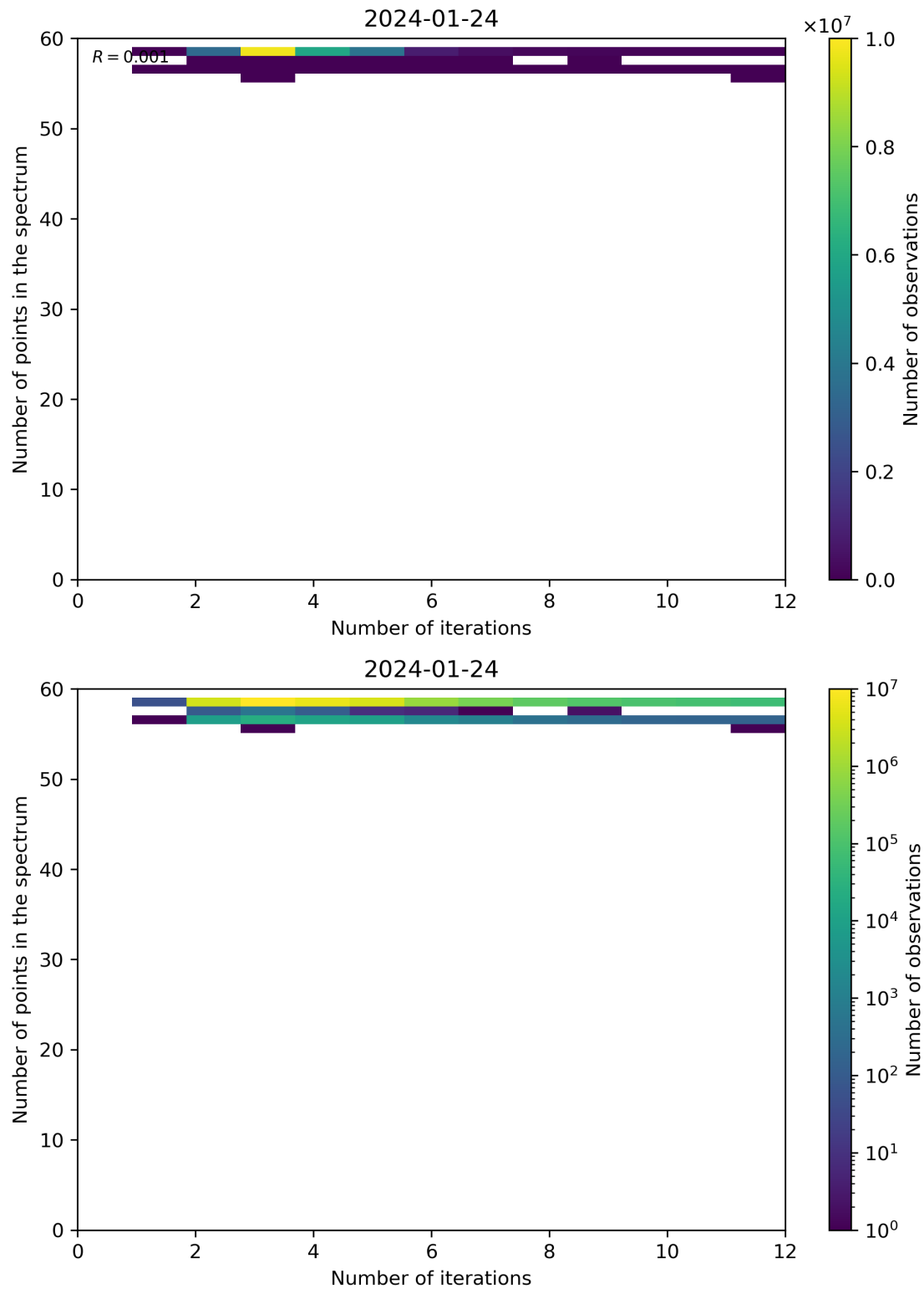
Figure 99: Scatter density plot of “Number of iterations” against “Number of points in the spectrum” for 2024-01-23 to 2024-01-25.
