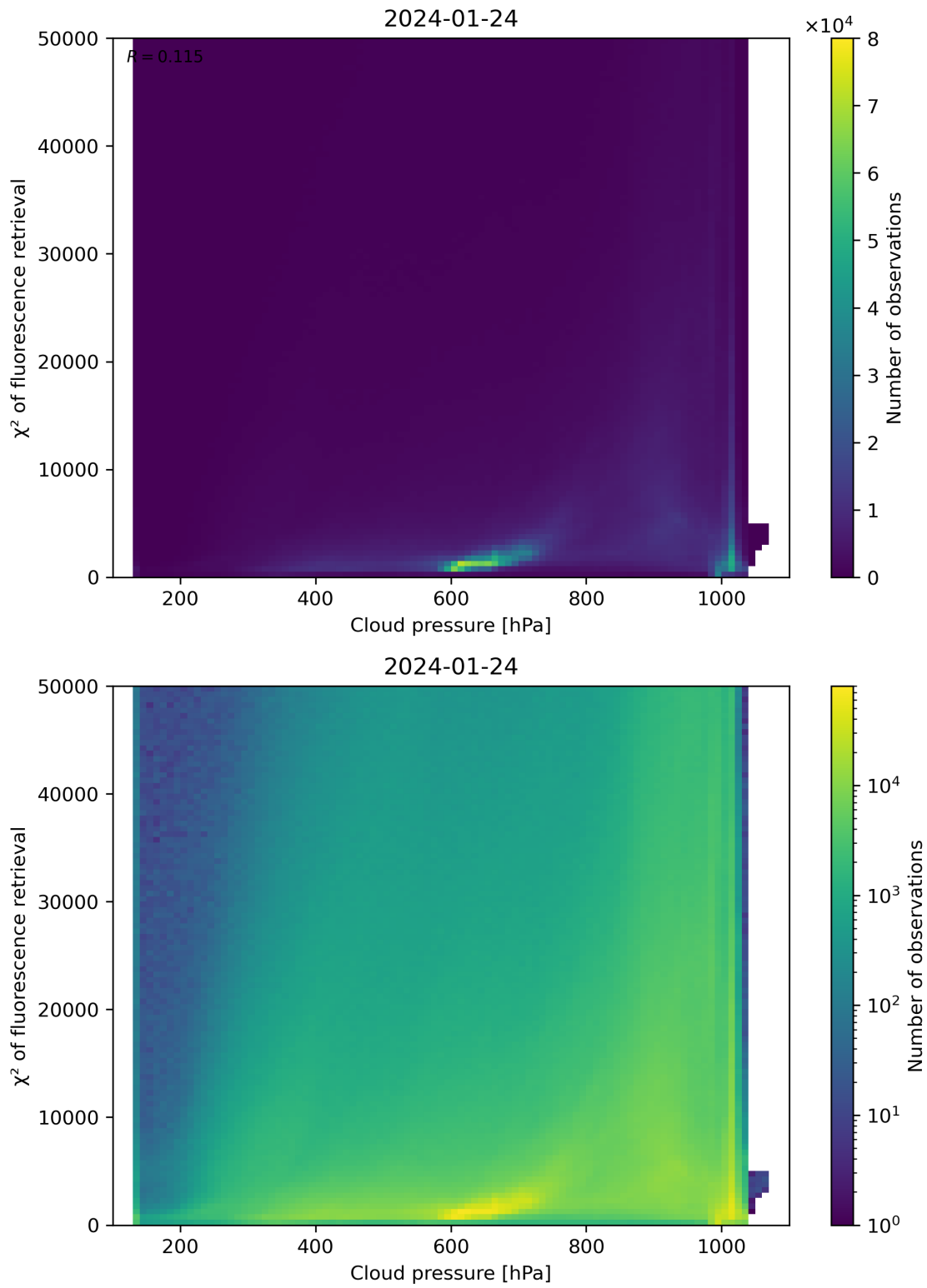
Figure 78: Scatter density plot of “Cloud pressure” against “ \chi^2 of fluorescence retrieval” for 2024-01-23 to 2024-01-25.
