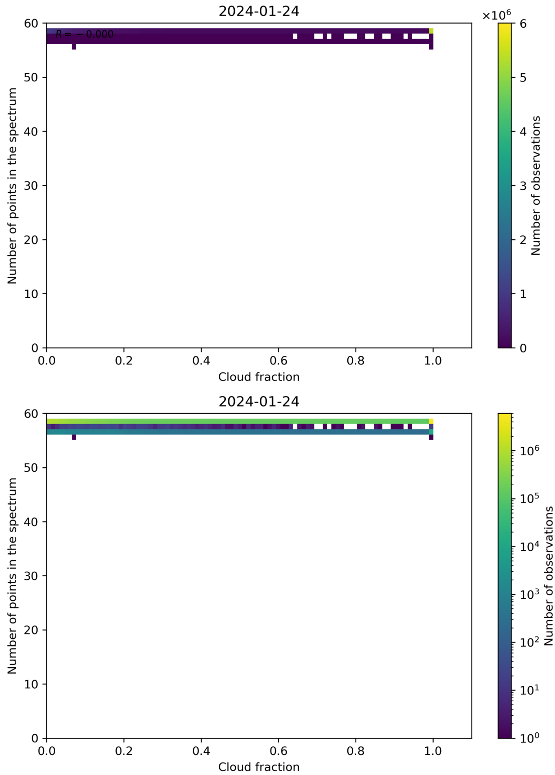
Figure 74: Scatter density plot of “Cloud fraction” against “Number of points in the spectrum” for 2024-01-23 to 2024-01-25.
