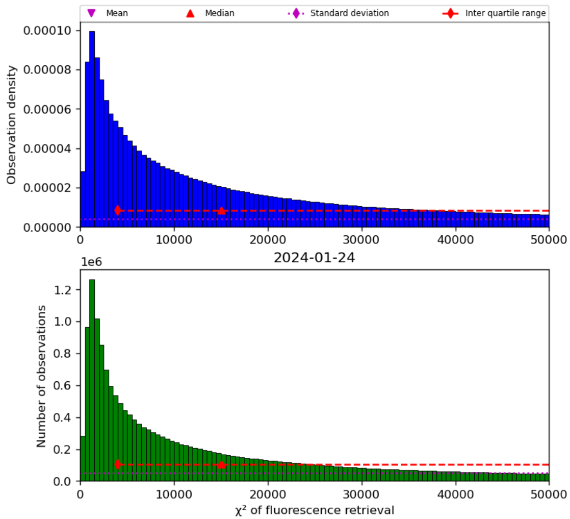
Figure 42: Histogram of “ \chi^2 of fluorescence retrieval” for 2024-01-23 to 2024-01-25
