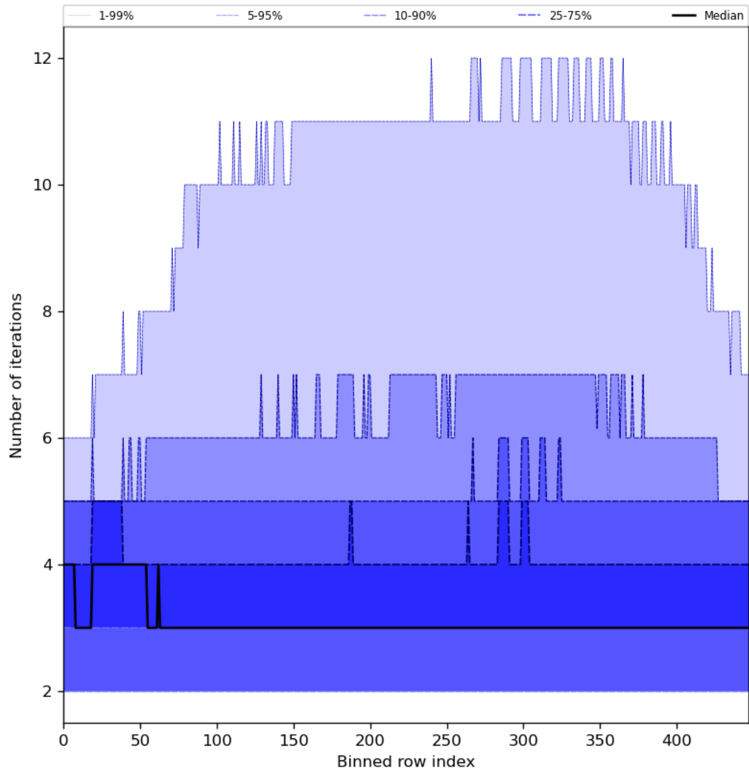
Figure 56: Along track statistics of “Number of iterations” for 2024-01-23 to 2024-01-25
