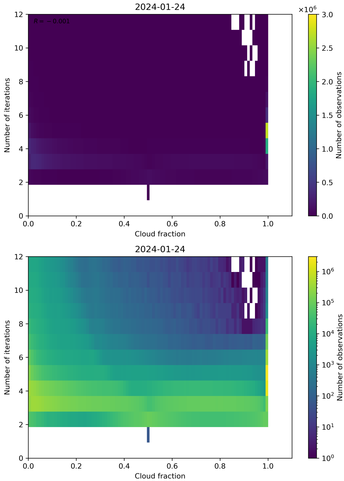
Figure 73: Scatter density plot of “Cloud fraction” against “Number of iterations” for 2024-01-23 to 2024-01-25.
