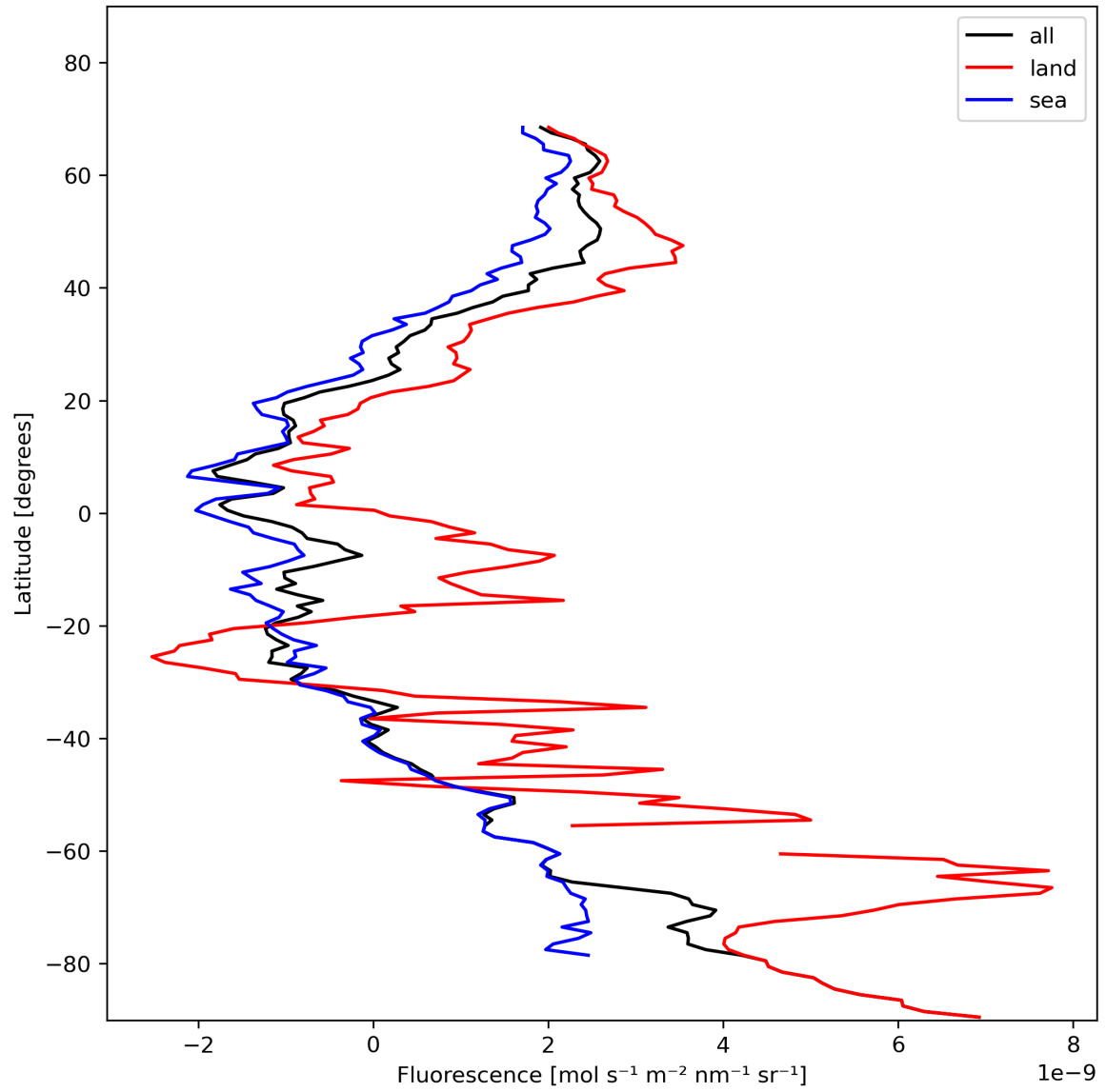
Figure 23: Zonal average of “Fluorescence” for 2024-01-23 to 2024-01-25.
