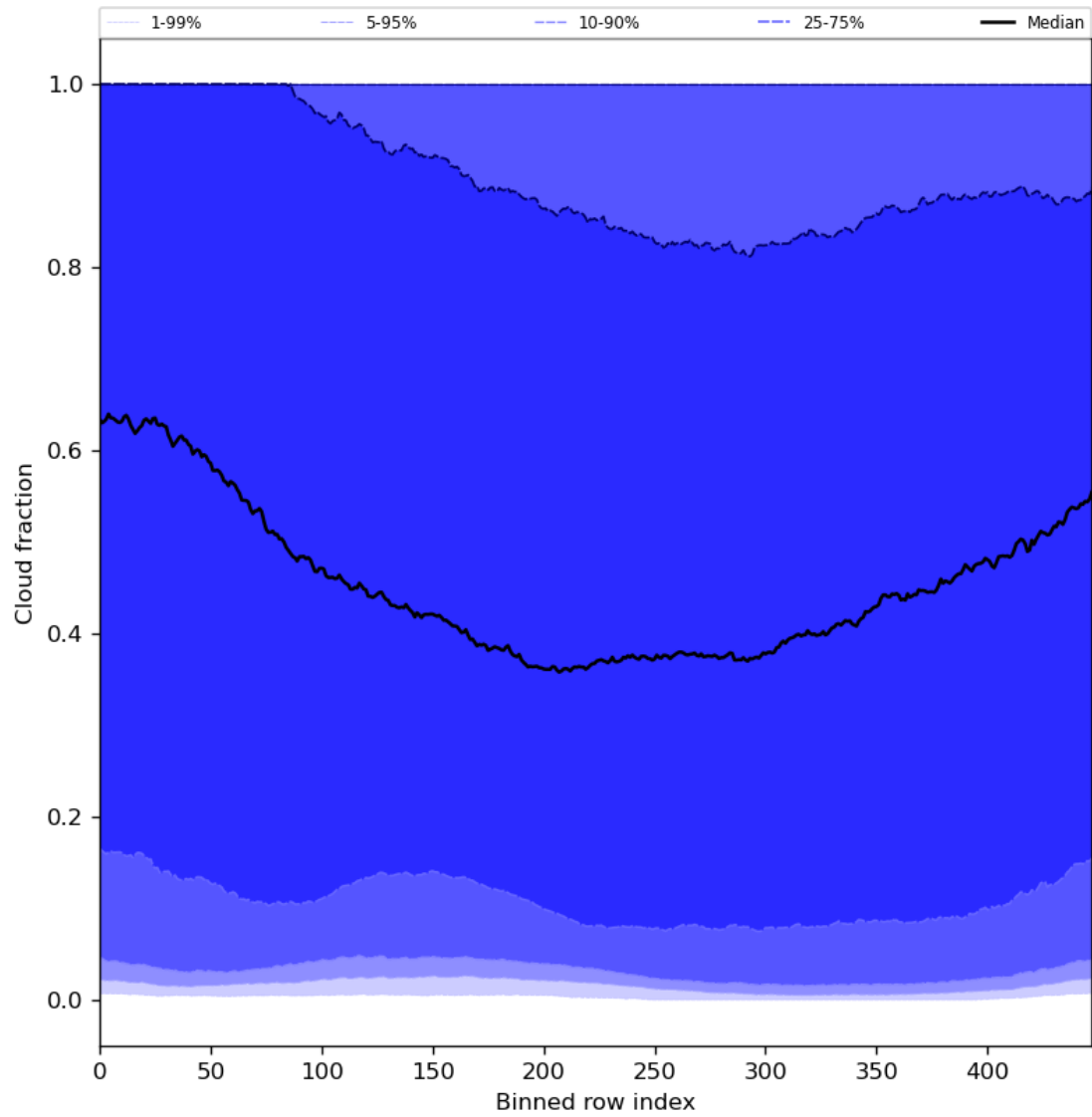
Figure 49: Along track statistics of “Cloud fraction” for 2024-01-23 to 2024-01-25
