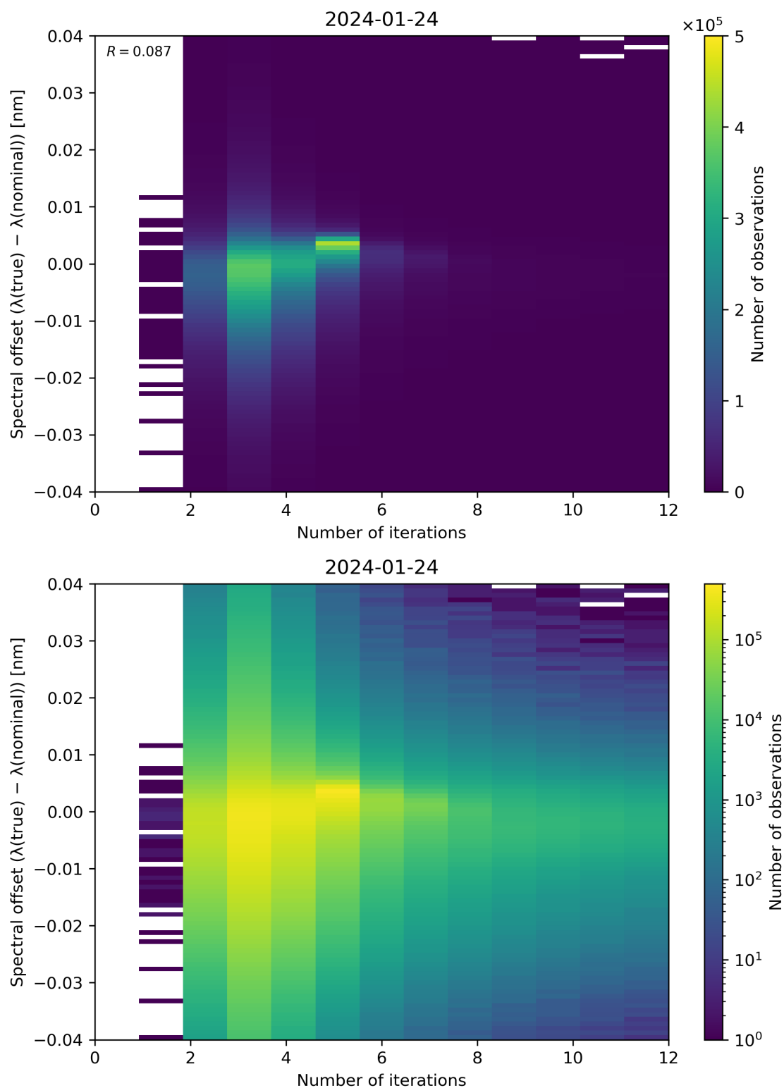
Figure 100: Scatter density plot of “Number of iterations” against “Spectral offset ( \lambda(\text{true}) - \lambda(\text{nominal}) )” for 2024-01-23 to 2024-01-25.
