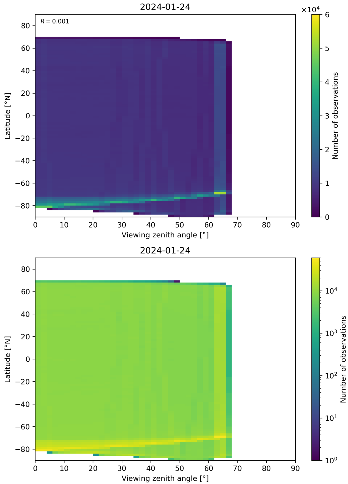
Figure 123: Scatter density plot of “Viewing zenith angle” against “Latitude” for 2024-01-23 to 2024-01-25.
