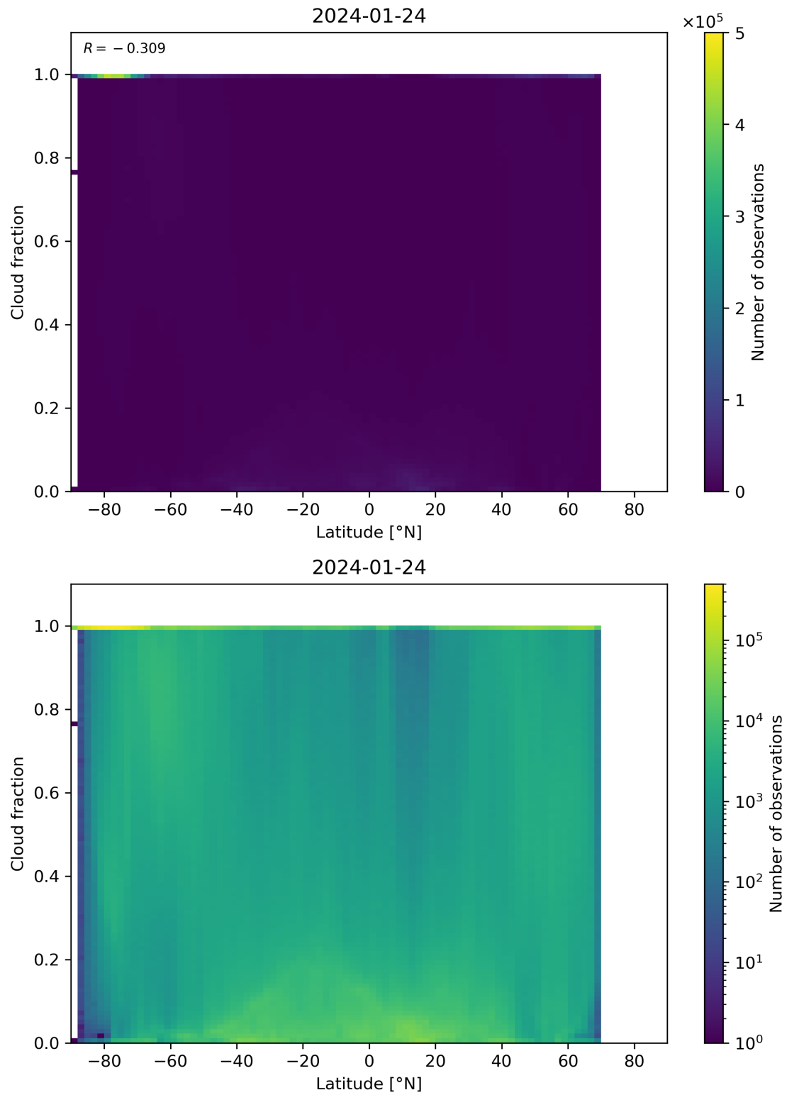
Figure 90: Scatter density plot of “Latitude” against “Cloud fraction” for 2024-01-23 to 2024-01-25.
