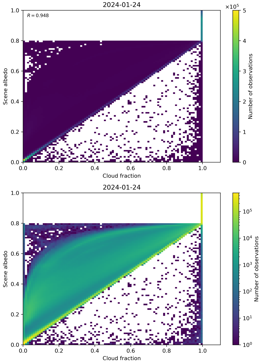
Figure 75: Scatter density plot of “Cloud fraction” against “Scene albedo” for 2024-01-23 to 2024-01-25.
