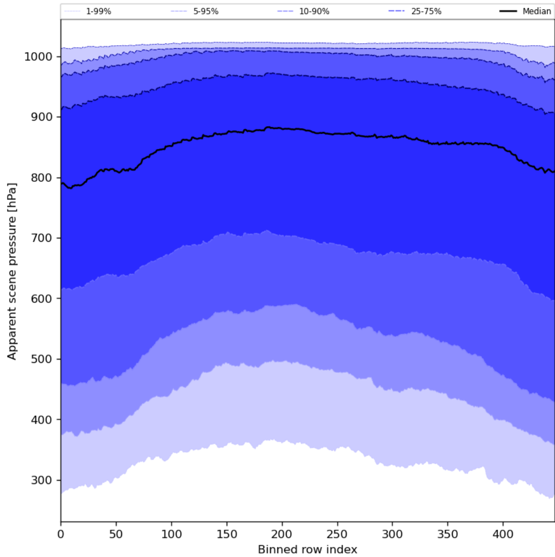
Figure 53: Along track statistics of “Apparent scene pressure” for 2024-01-23 to 2024-01-25
