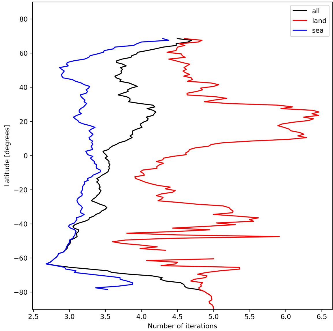
Figure 22: Zonal average of “Number of iterations” for 2024-01-23 to 2024-01-25.
