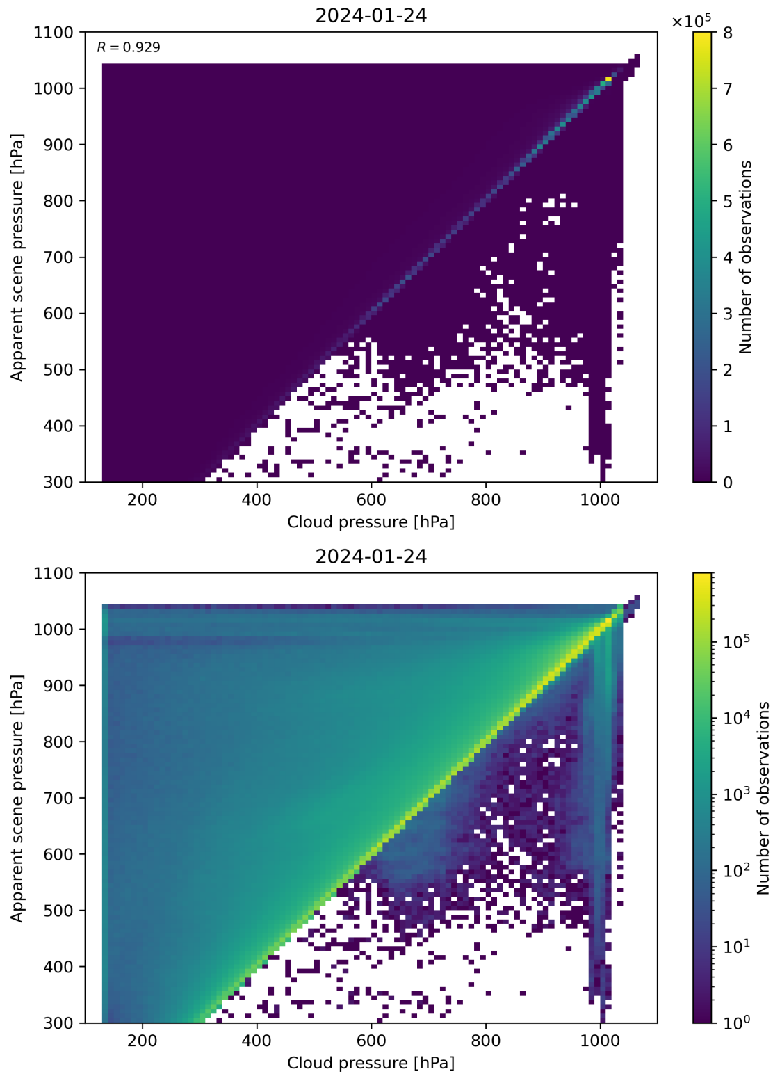
Figure 77: Scatter density plot of “Cloud pressure” against “Apparent scene pressure” for 2024-01-23 to 2024-01-25.
