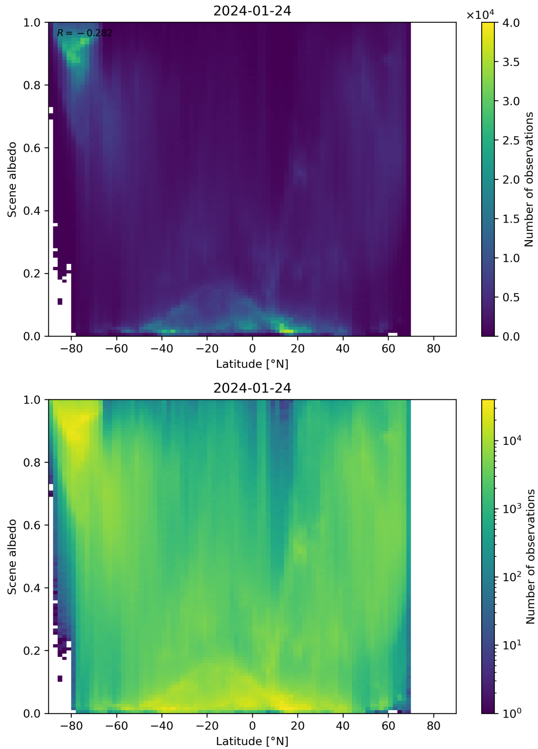
Figure 95: Scatter density plot of “Latitude” against “Scene albedo” for 2024-01-23 to 2024-01-25.
