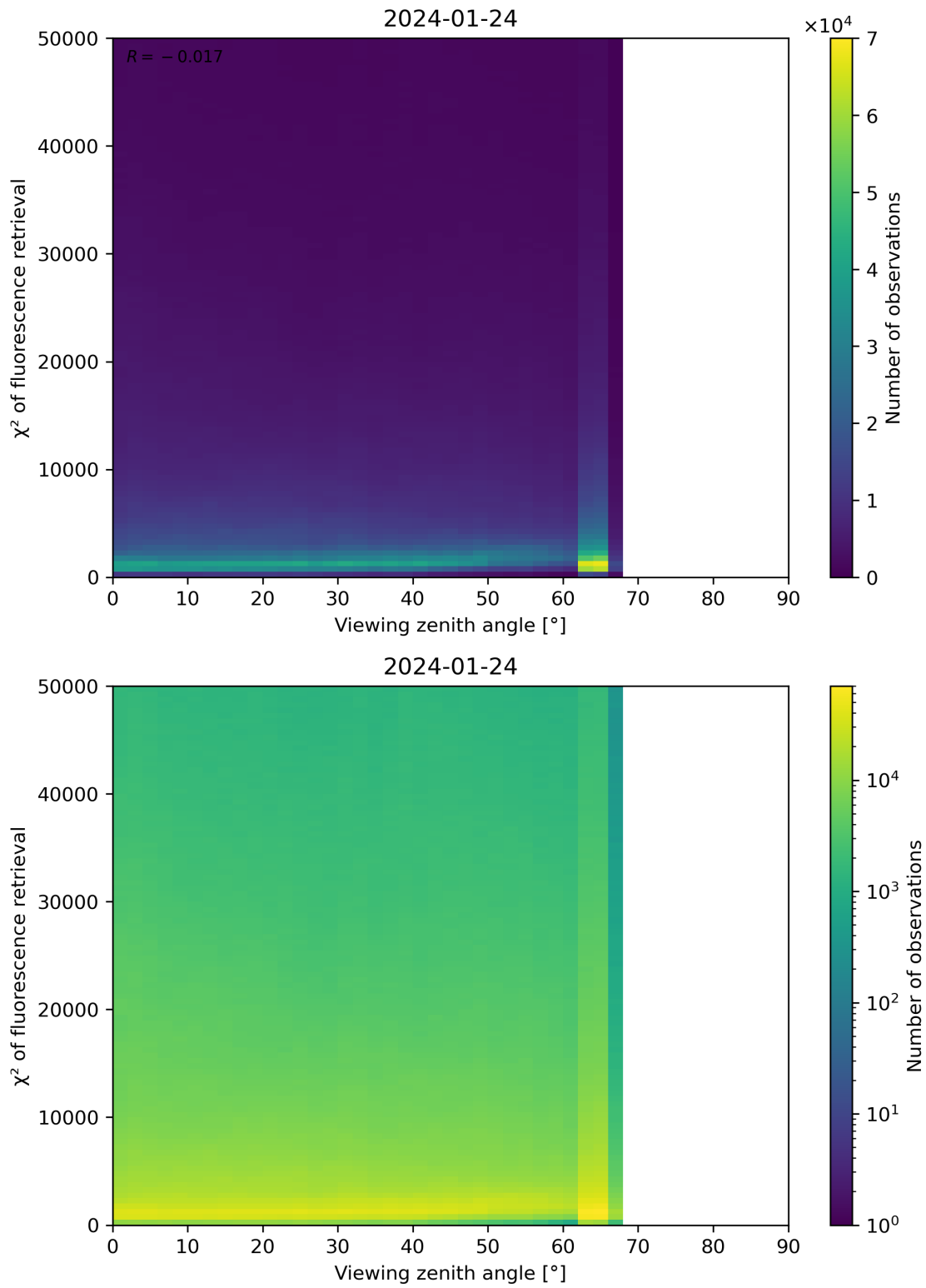
Figure 119: Scatter density plot of “Viewing zenith angle” against “ \chi^2 of fluorescence retrieval” for 2024-01-23 to 2024-01-25.
