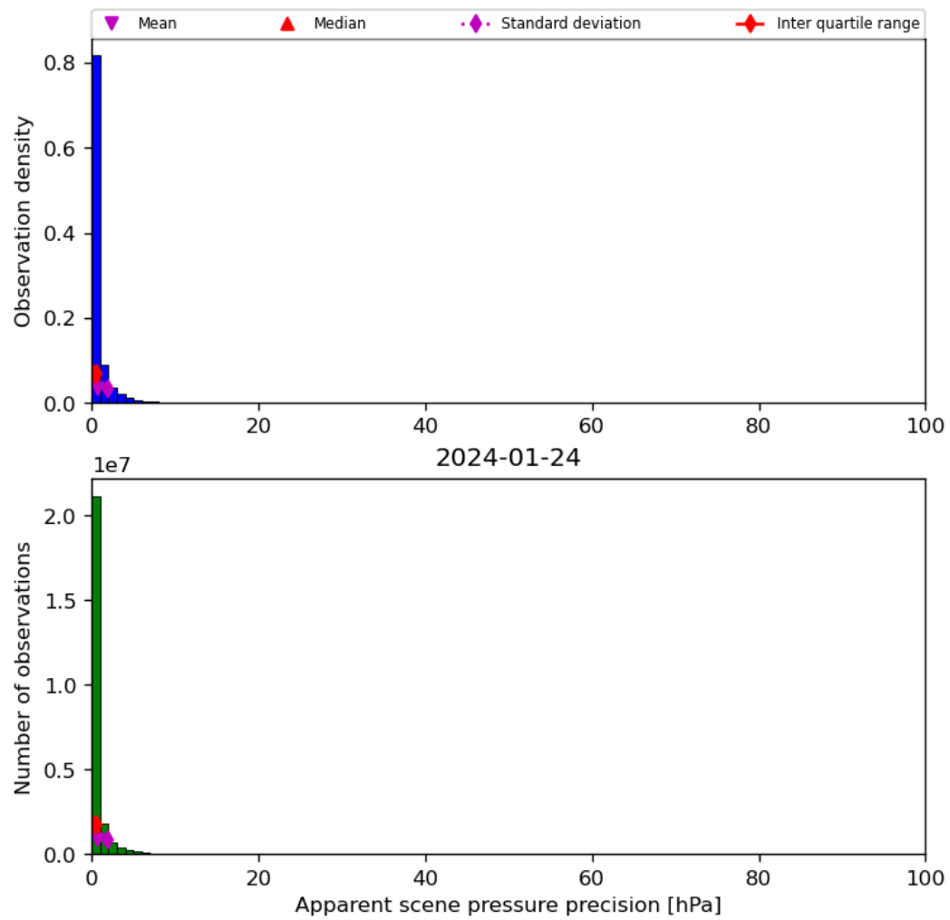
Figure 37: Histogram of “Apparent scene pressure precision” for 2024-01-23 to 2024-01-25
