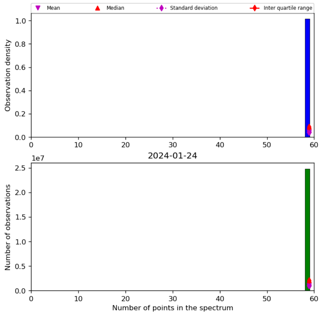
Figure 44: Histogram of “Number of points in the spectrum” for 2024-01-23 to 2024-01-25
