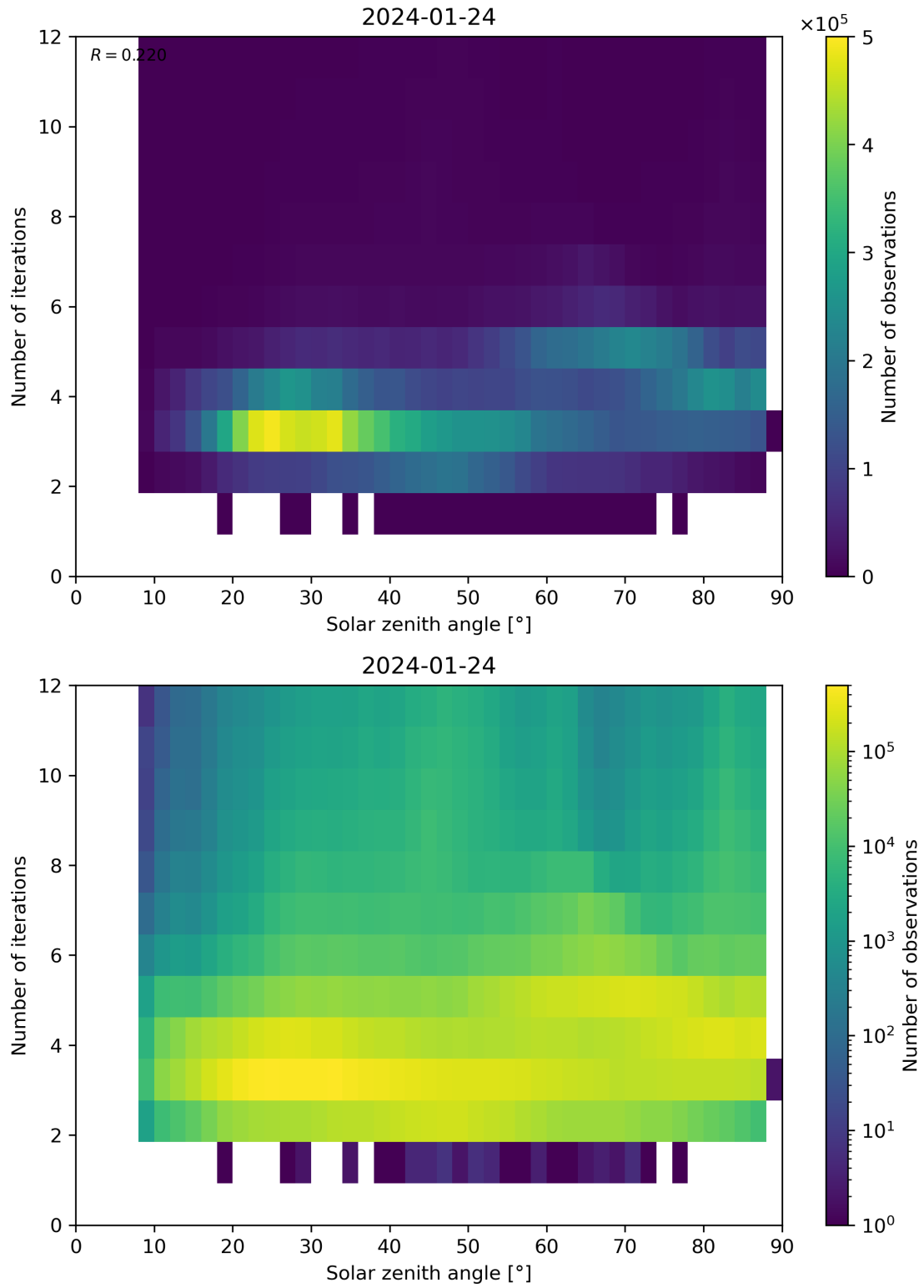
Figure 114: Scatter density plot of “Solar zenith angle” against “Number of iterations” for 2024-01-23 to 2024-01-25.
