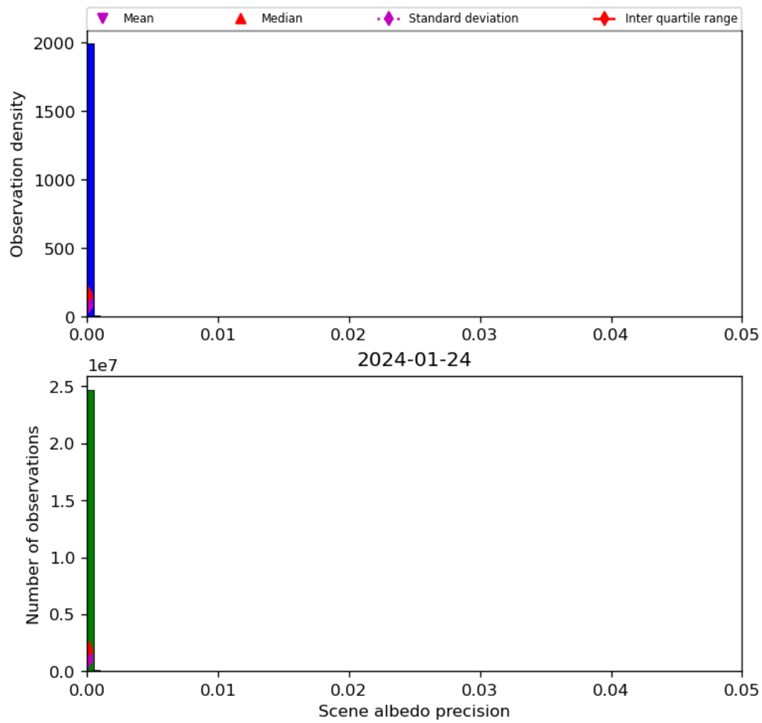
Figure 35: Histogram of “Scene albedo precision” for 2024-01-23 to 2024-01-25
