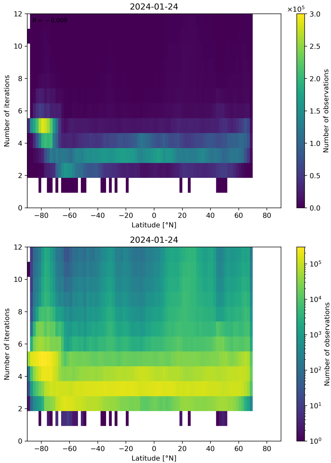
Figure 93: Scatter density plot of “Latitude” against “Number of iterations” for 2024-01-23 to 2024-01-25.
