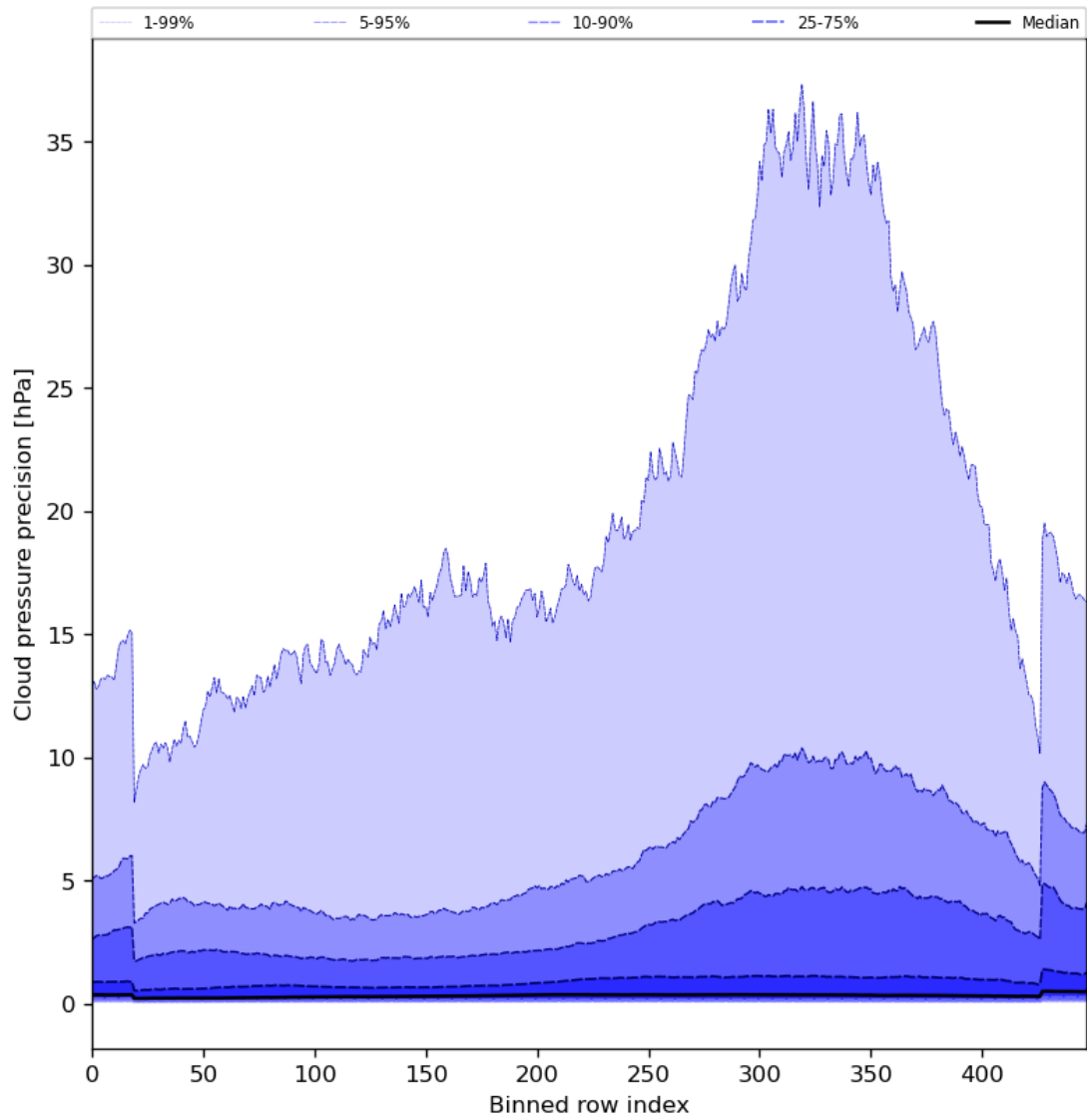
Figure 48: Along track statistics of “Cloud pressure precision” for 2024-01-23 to 2024-01-25
