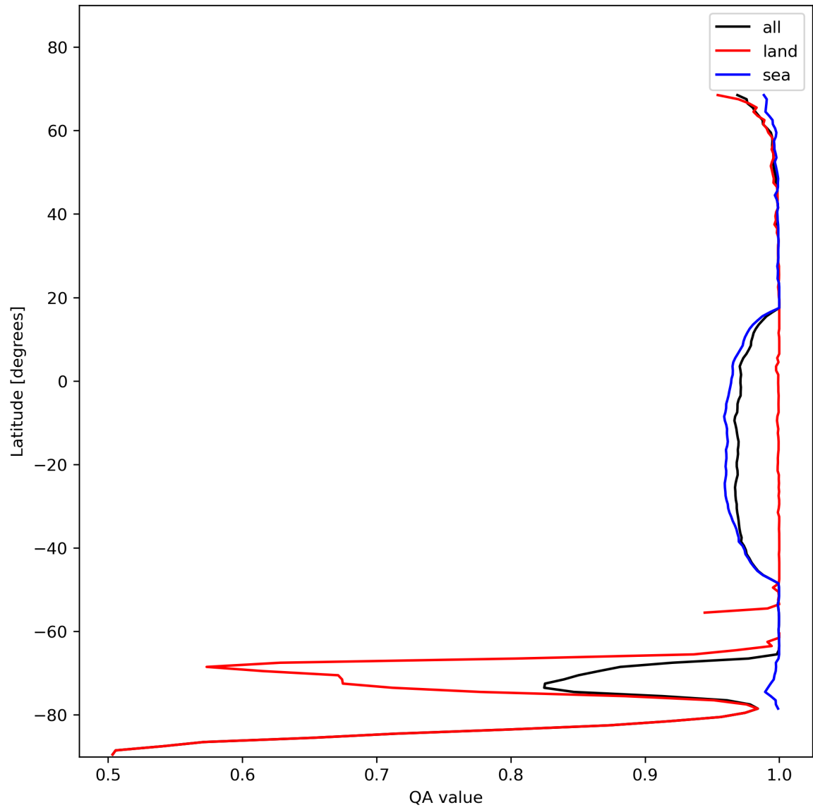
Figure 12: Zonal average of “QA value” for 2024-01-23 to 2024-01-25.
