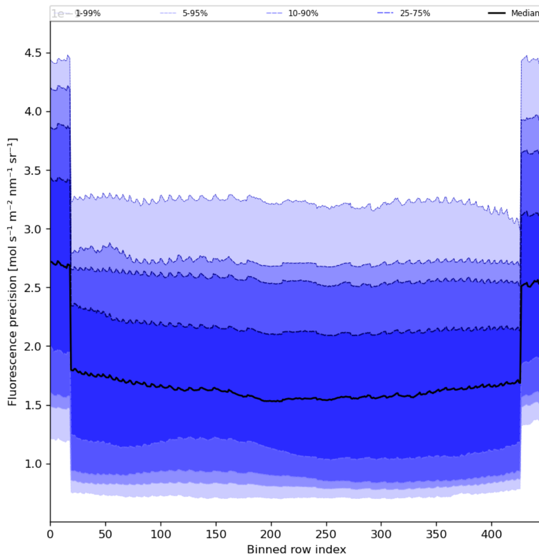
Figure 58: Along track statistics of “Fluorescence precision” for 2024-01-23 to 2024-01-25
