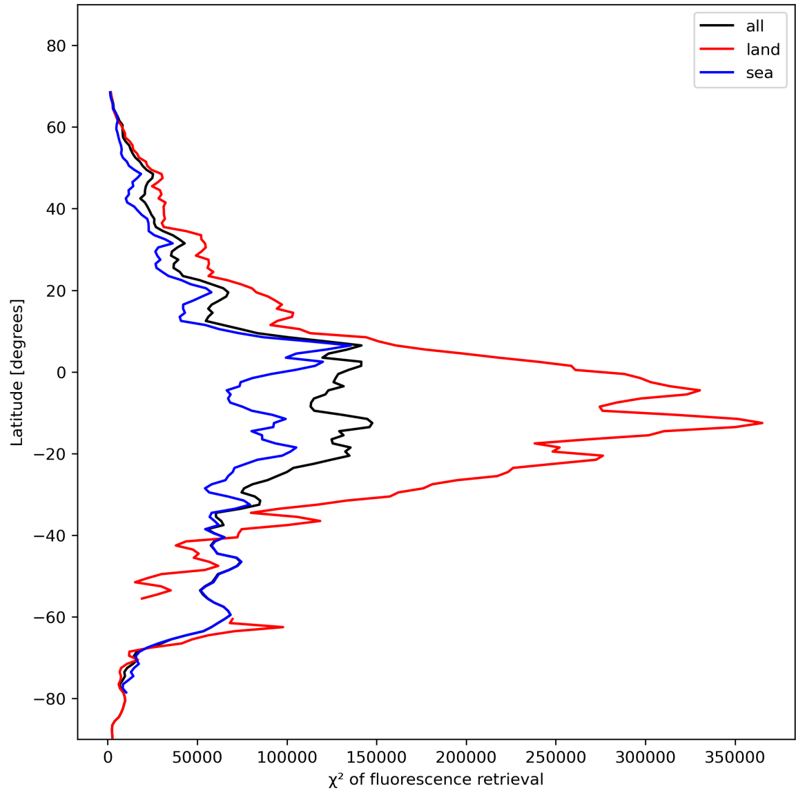
Figure 25: Zonal average of “ \chi^2 of fluorescence retrieval” for 2024-01-23 to 2024-01-25.
