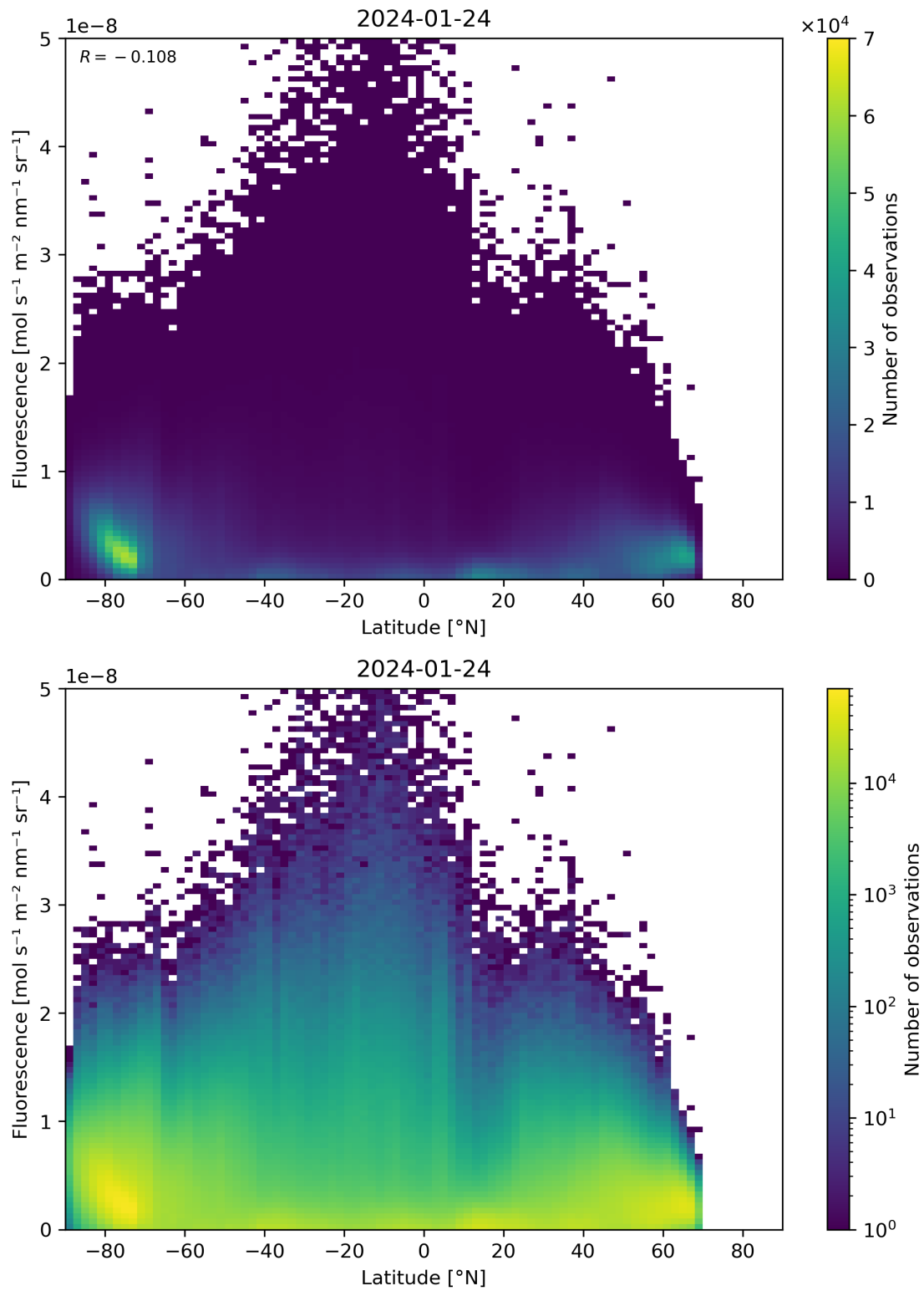
Figure 92: Scatter density plot of “Latitude” against “Fluorescence” for 2024-01-23 to 2024-01-25.
