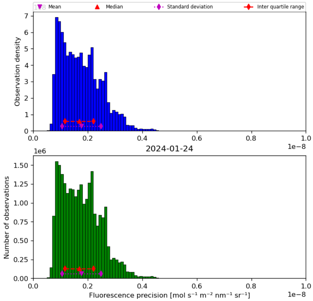
Figure 41: Histogram of “Fluorescence precision” for 2024-01-23 to 2024-01-25
