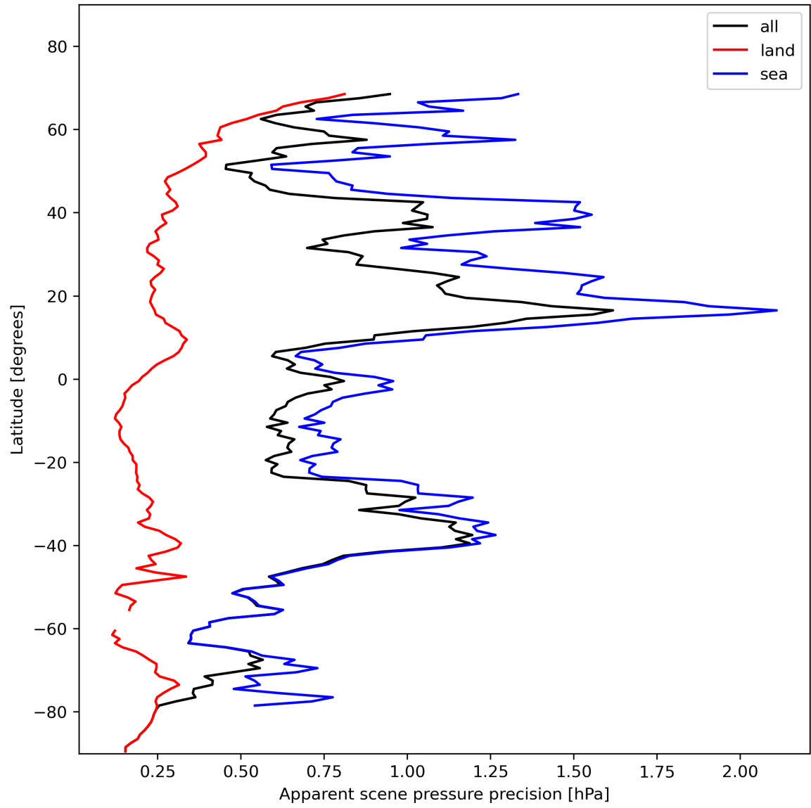
Figure 20: Zonal average of “Apparent scene pressure precision” for 2024-01-23 to 2024-01-25.
