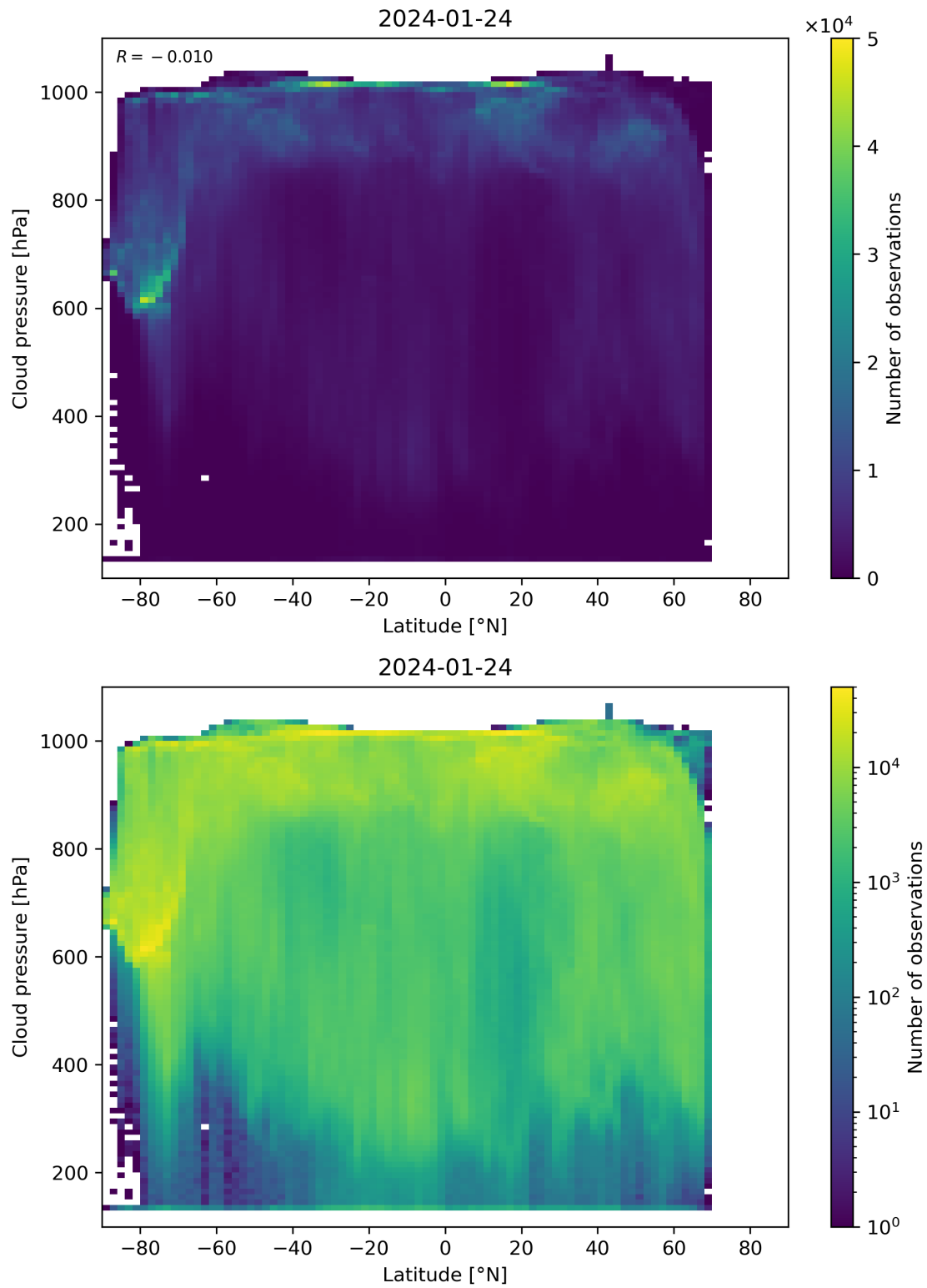
Figure 91: Scatter density plot of “Latitude” against “Cloud pressure” for 2024-01-23 to 2024-01-25.
