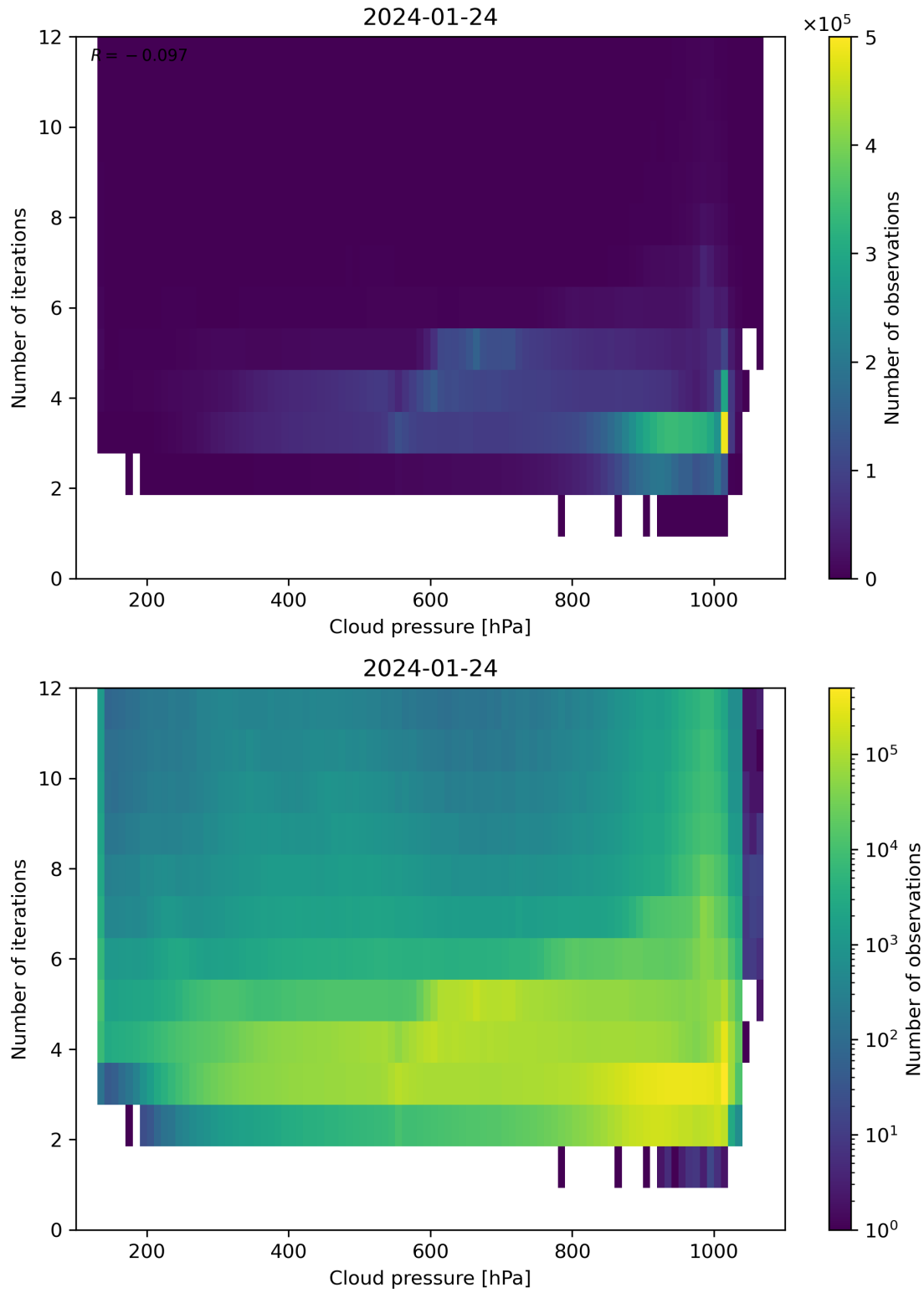
Figure 81: Scatter density plot of “Cloud pressure” against “Number of iterations” for 2024-01-23 to 2024-01-25.
