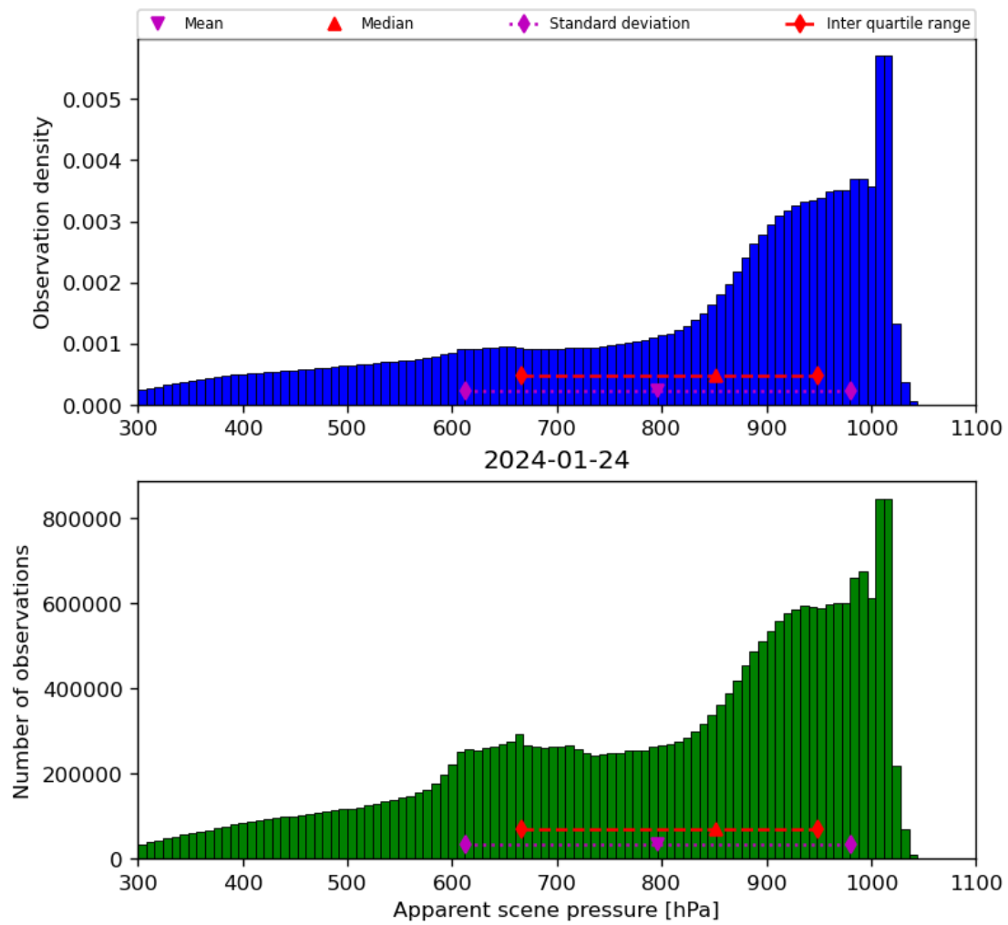
Figure 36: Histogram of “Apparent scene pressure” for 2024-01-23 to 2024-01-25
