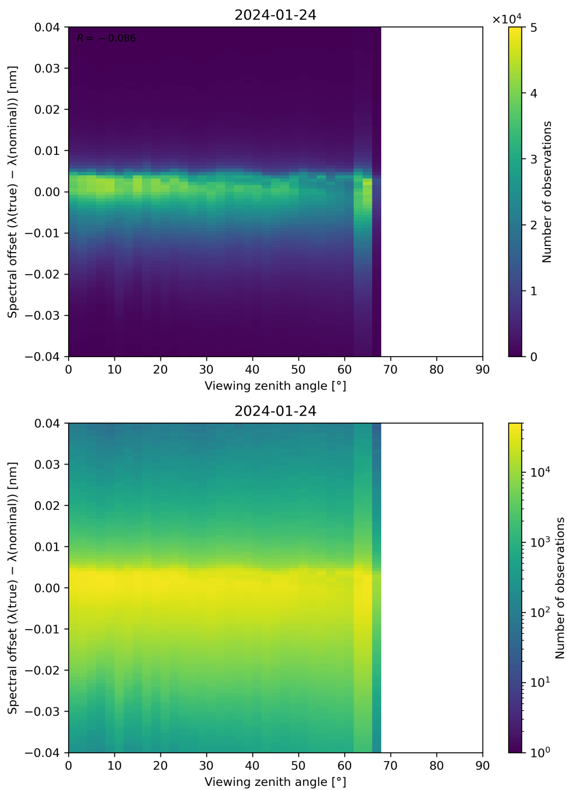
Figure 128: Scatter density plot of “Viewing zenith angle” against “Spectral offset ( \lambda(\text{true}) - \lambda(\text{nominal}) )” for 2024-01-23 to 2024-01-25.
