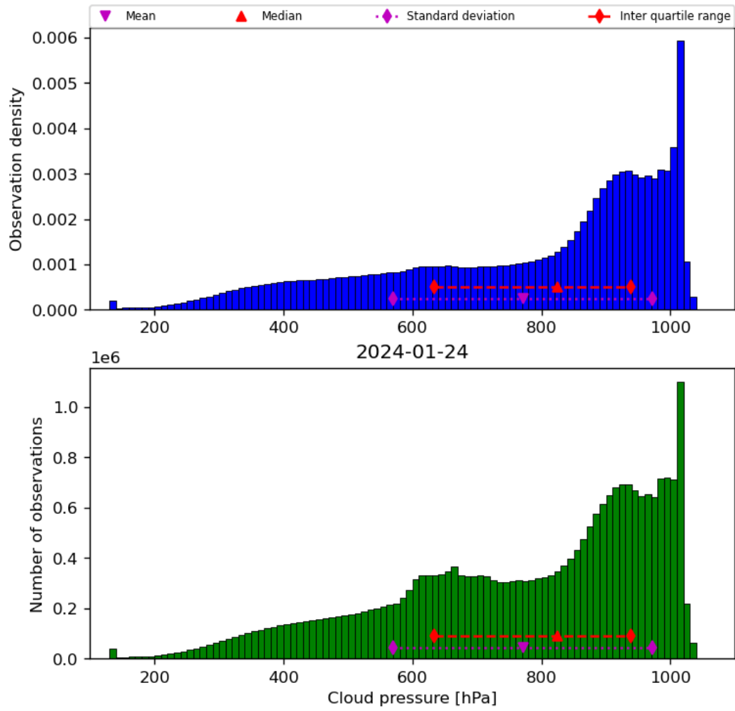
Figure 30: Histogram of “Cloud pressure” for 2024-01-23 to 2024-01-25
