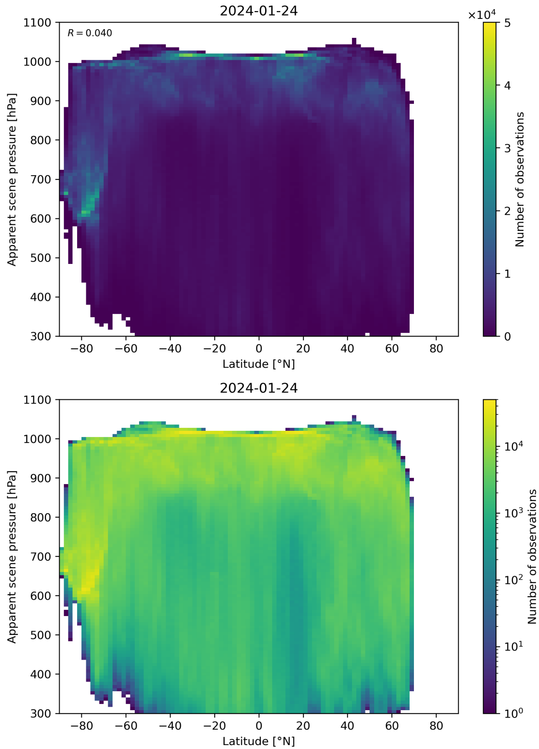
Figure 88: Scatter density plot of “Latitude” against “Apparent scene pressure” for 2024-01-23 to 2024-01-25.
