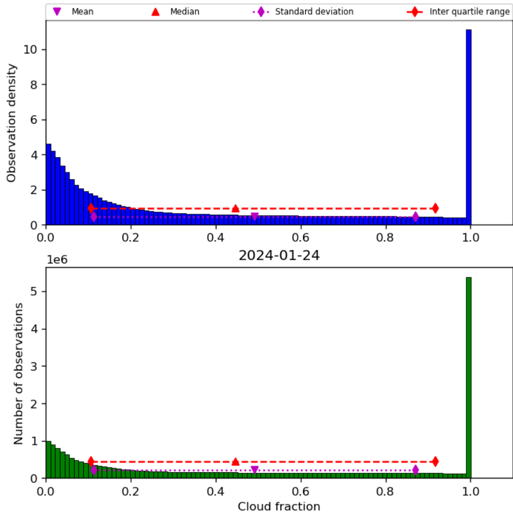
Figure 32: Histogram of “Cloud fraction” for 2024-01-23 to 2024-01-25
