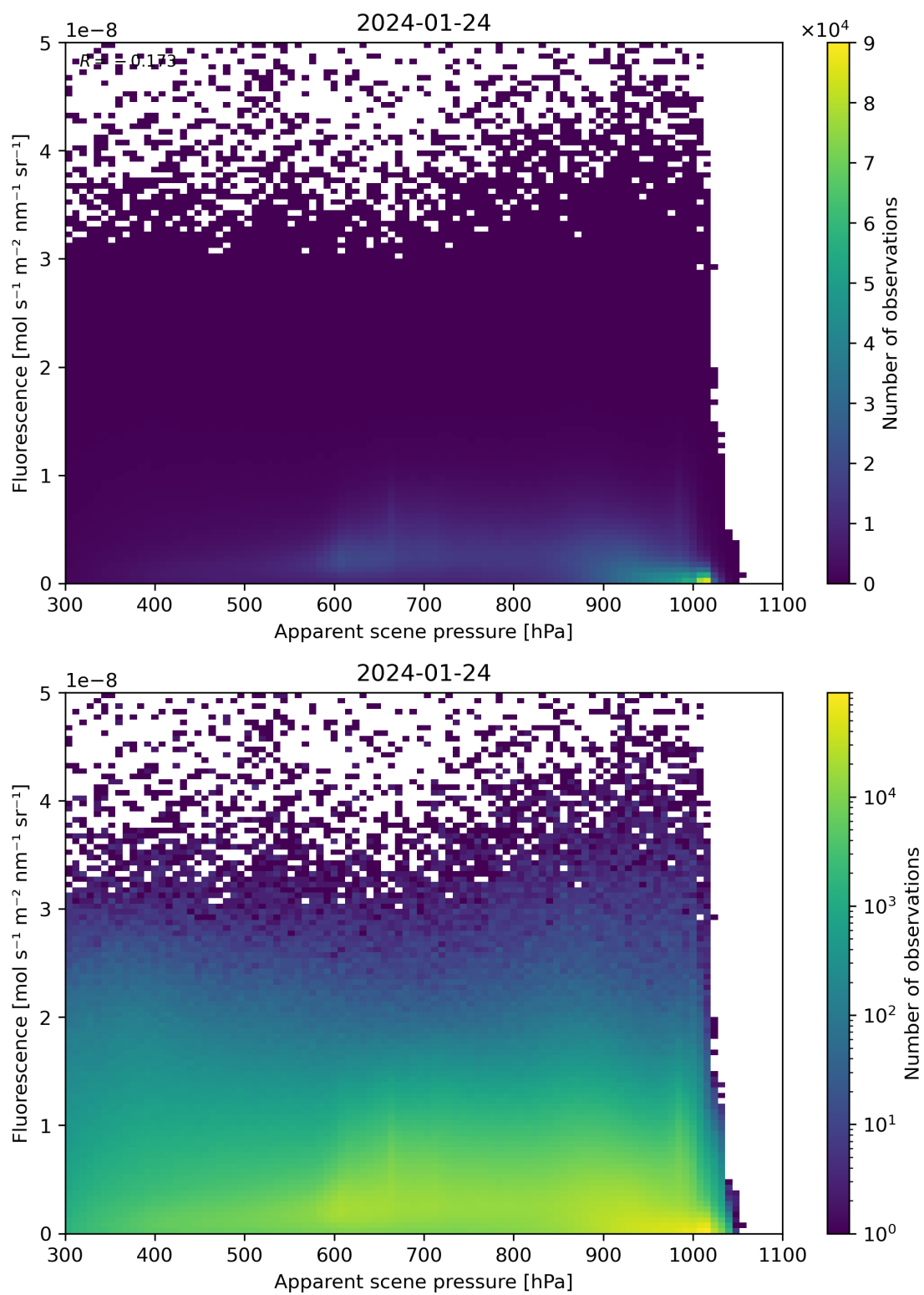
Figure 64: Scatter density plot of “Apparent scene pressure” against “Fluorescence” for 2024-01-23 to 2024-01-25.
