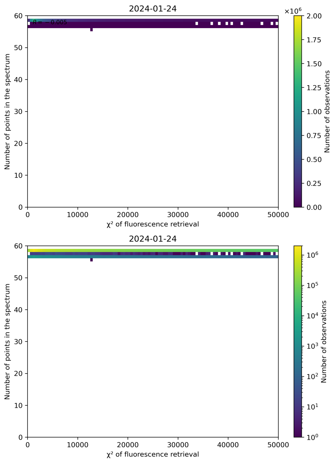
Figure 68: Scatter density plot of " \chi^2 of fluorescence retrieval" against "Number of points in the spectrum" for 2024-01-23 to 2024-01-25.
