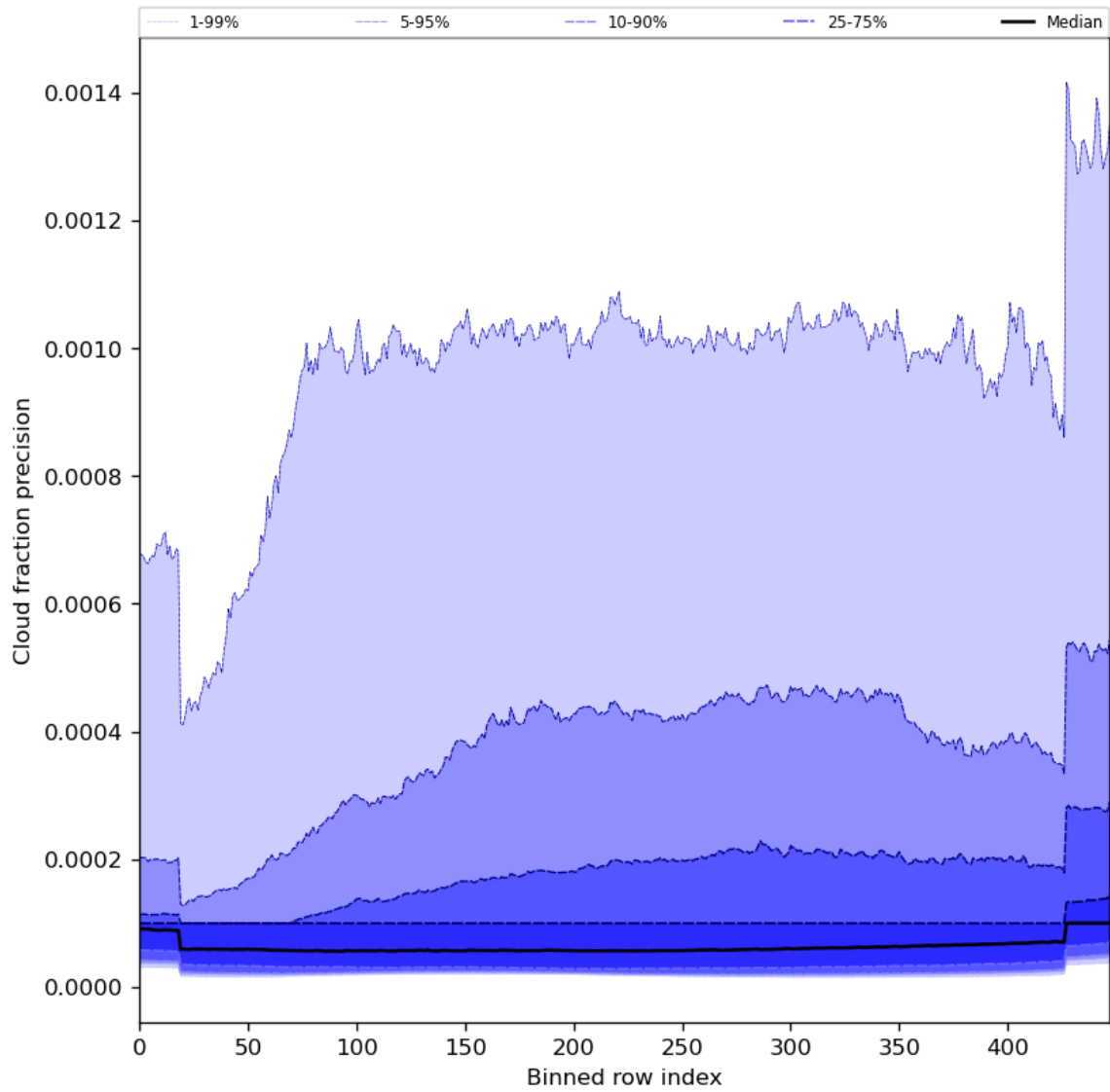
Figure 50: Along track statistics of “Cloud fraction precision” for 2024-01-23 to 2024-01-25
