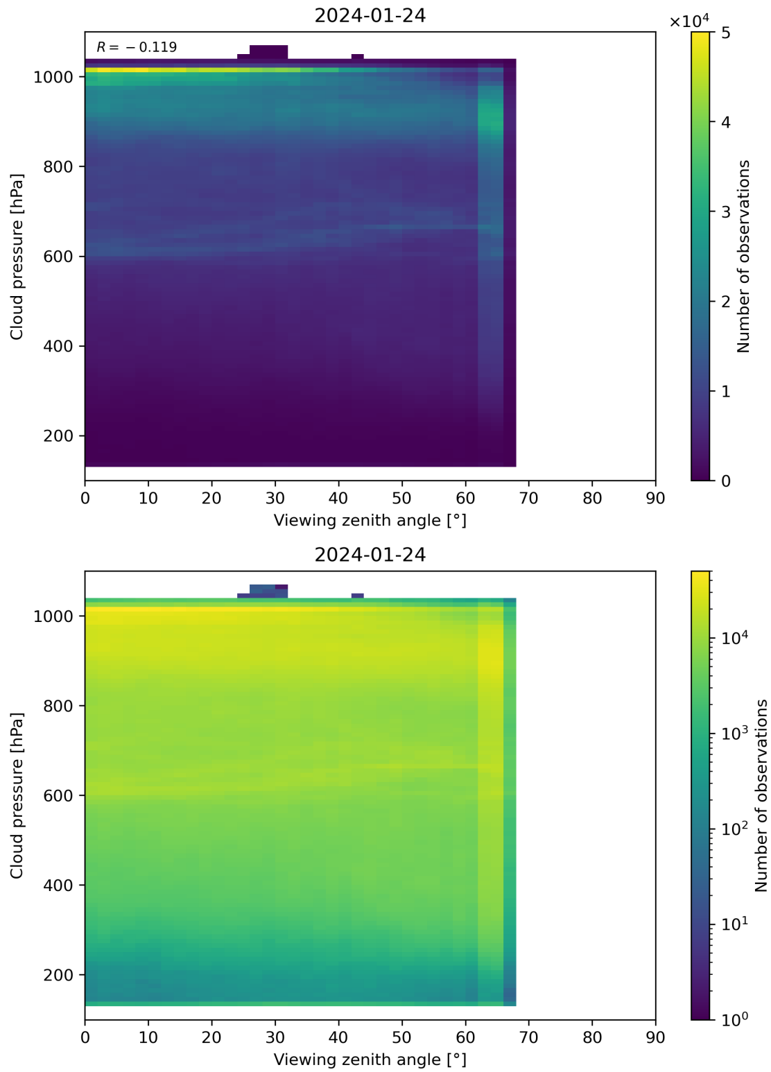
Figure 121: Scatter density plot of “Viewing zenith angle” against “Cloud pressure” for 2024-01-23 to 2024-01-25.
