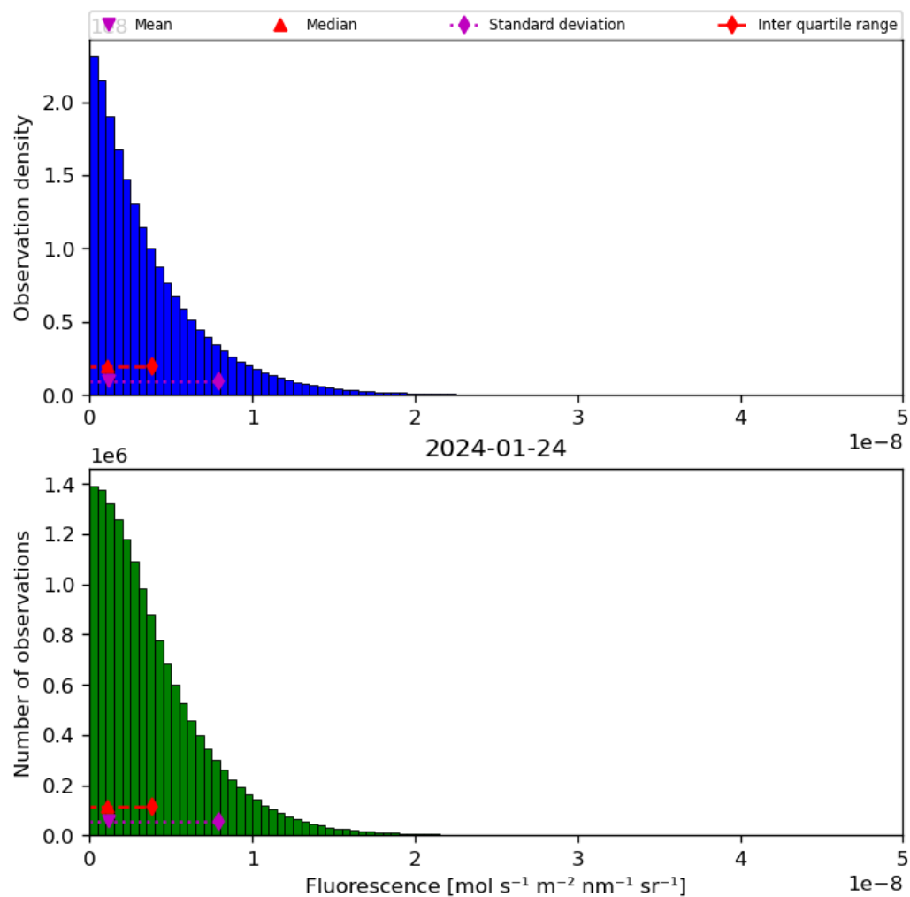
Figure 40: Histogram of “Fluorescence” for 2024-01-23 to 2024-01-25
