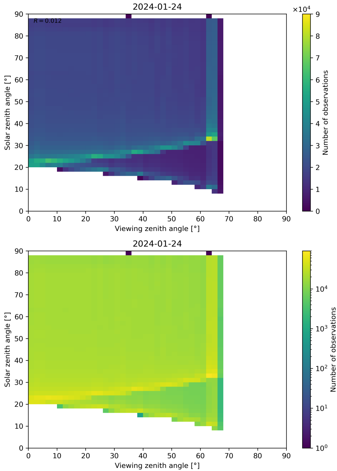
Figure 127: Scatter density plot of “Viewing zenith angle” against “Solar zenith angle” for 2024-01-23 to 2024-01-25.
