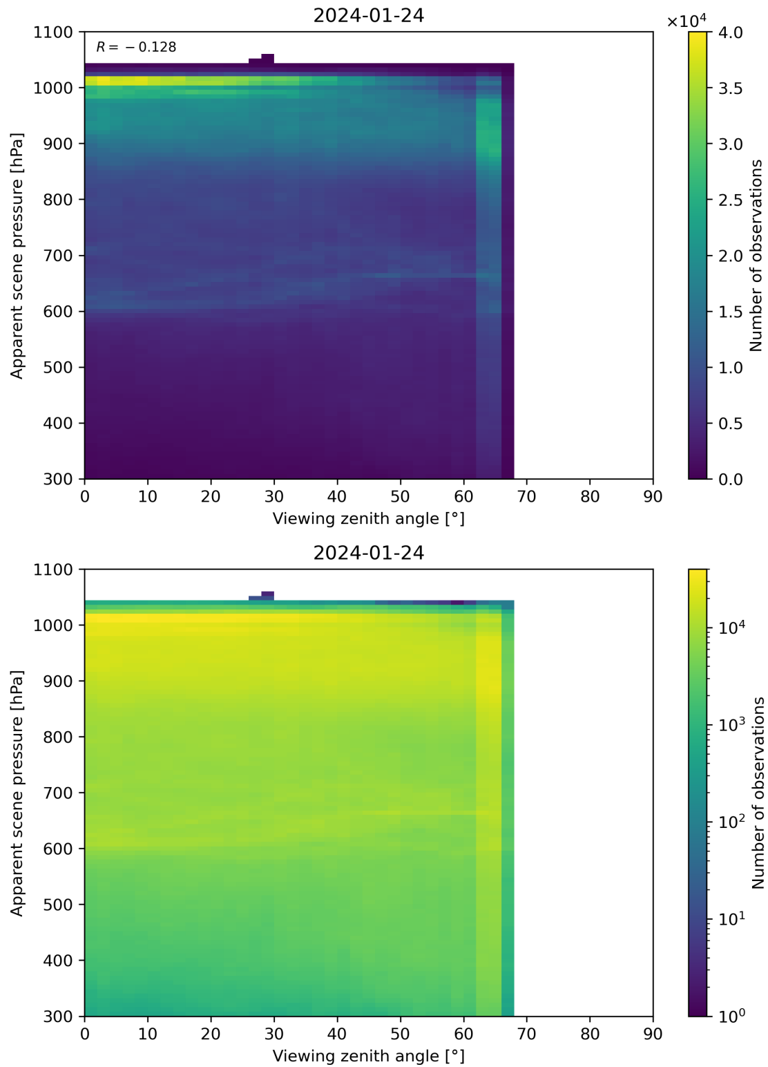
Figure 118: Scatter density plot of “Viewing zenith angle” against “Apparent scene pressure” for 2024-01-23 to 2024-01-25.
