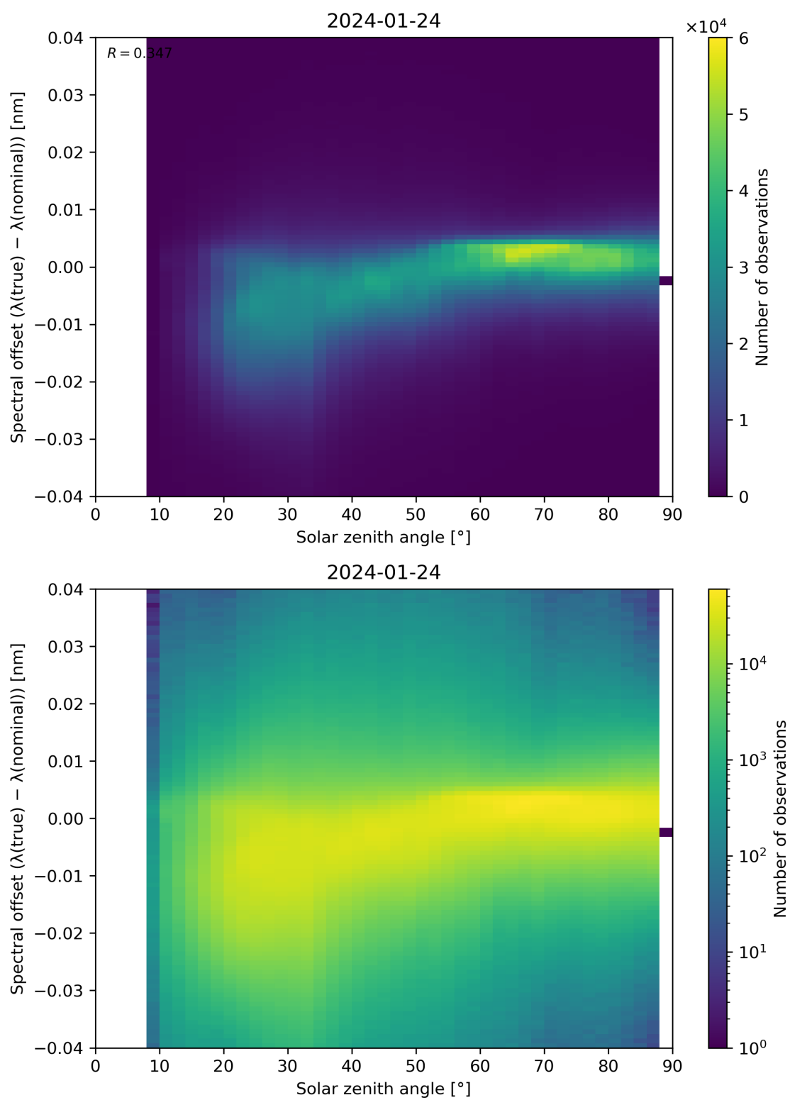
Figure 117: Scatter density plot of “Solar zenith angle” against “Spectral offset ( \lambda(\text{true}) - \lambda(\text{nominal}) )” for 2024-01-23 to 2024-01-25.
