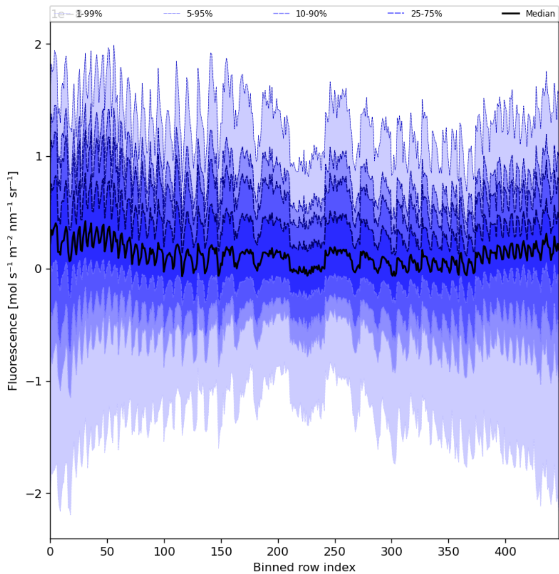
Figure 57: Along track statistics of “Fluorescence” for 2024-01-23 to 2024-01-25
