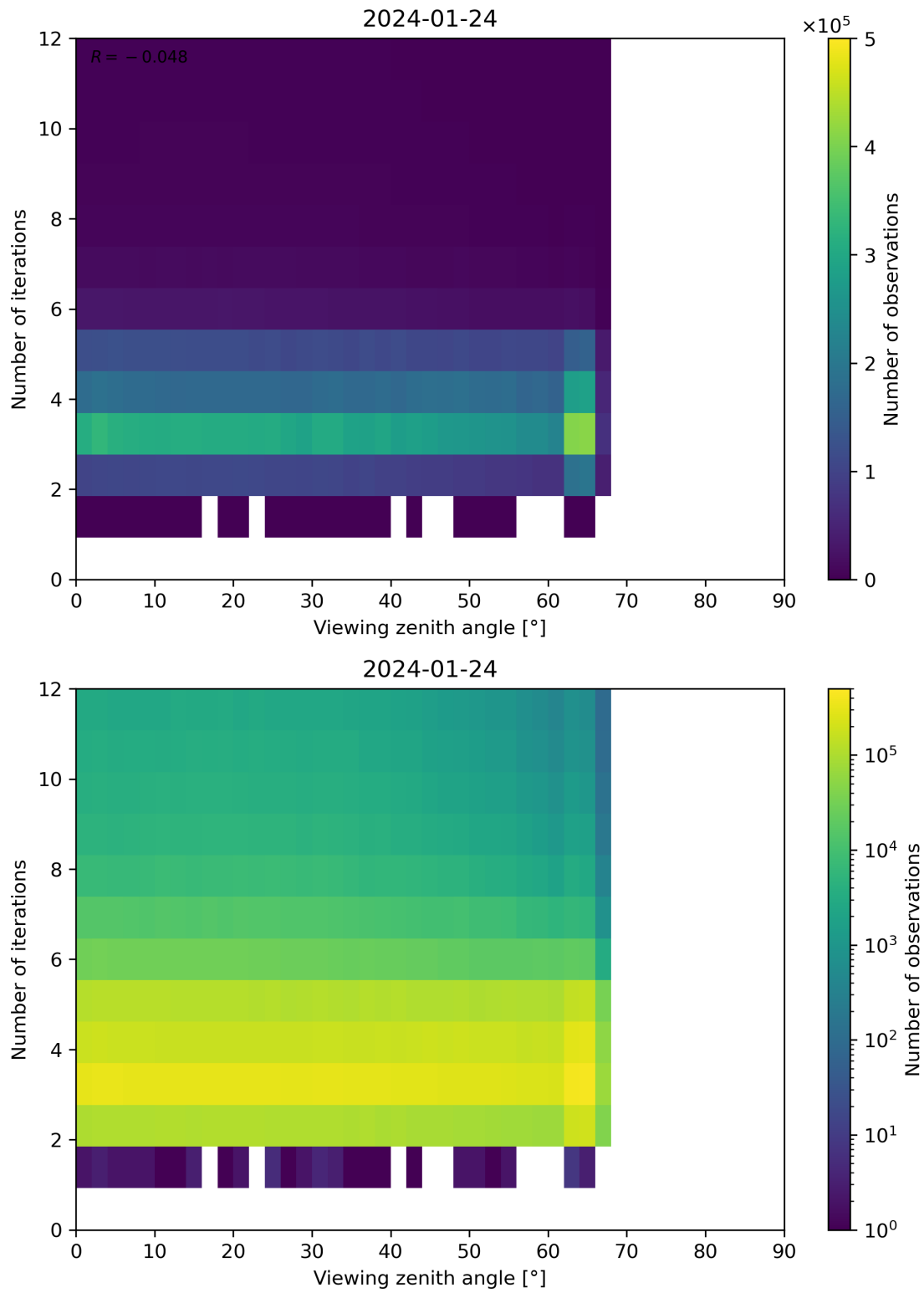
Figure 124: Scatter density plot of “Viewing zenith angle” against “Number of iterations” for 2024-01-23 to 2024-01-25.
