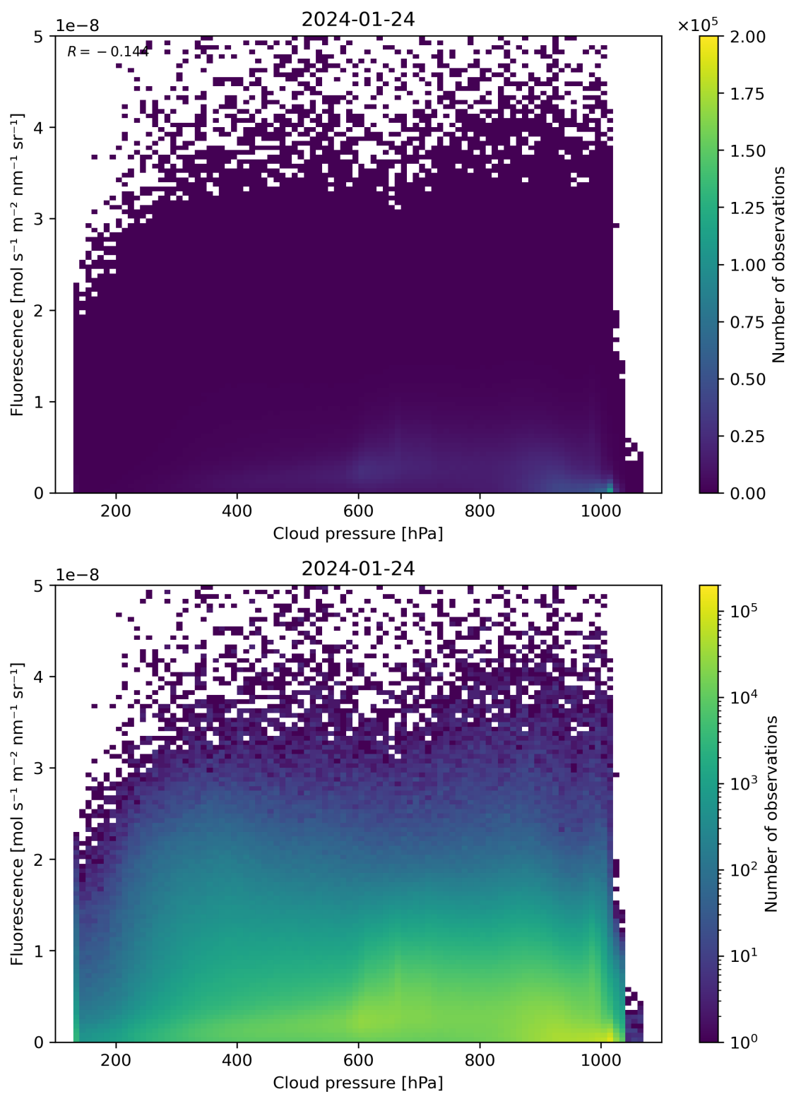
Figure 80: Scatter density plot of “Cloud pressure” against “Fluorescence” for 2024-01-23 to 2024-01-25.
