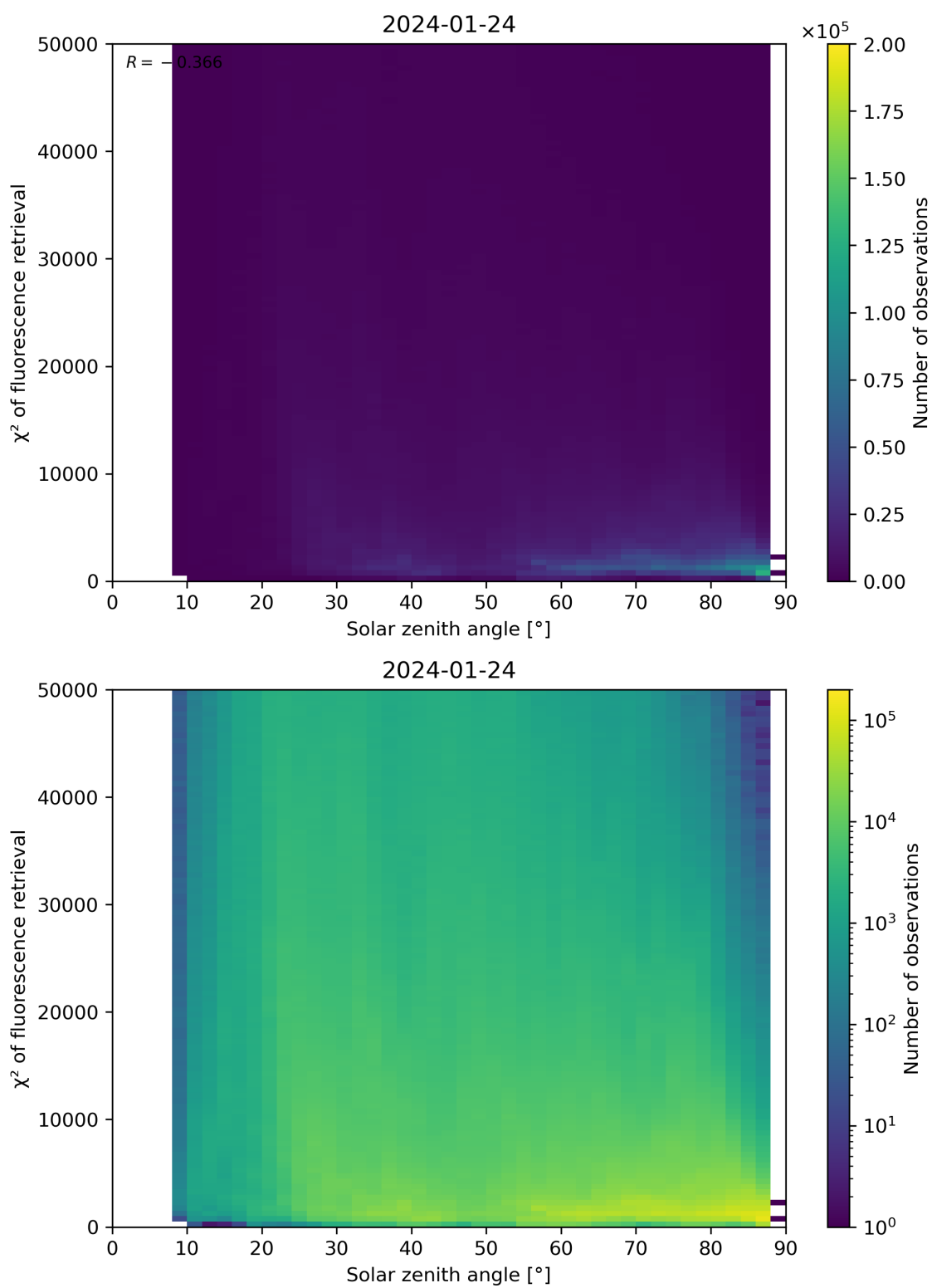
Figure 109: Scatter density plot of “Solar zenith angle” against “ \chi^2 of fluorescence retrieval” for 2024-01-23 to 2024-01-25.
