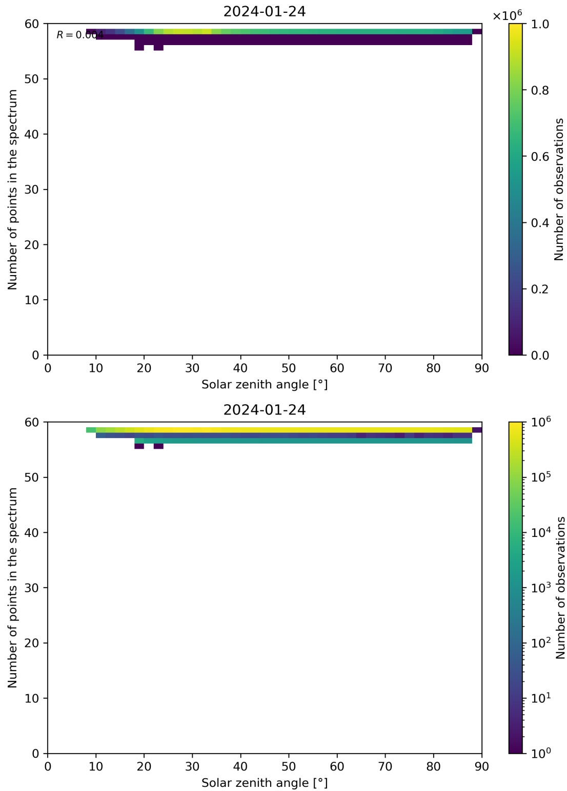
Figure 115: Scatter density plot of “Solar zenith angle” against “Number of points in the spectrum” for 2024-01-23 to 2024-01-25.
