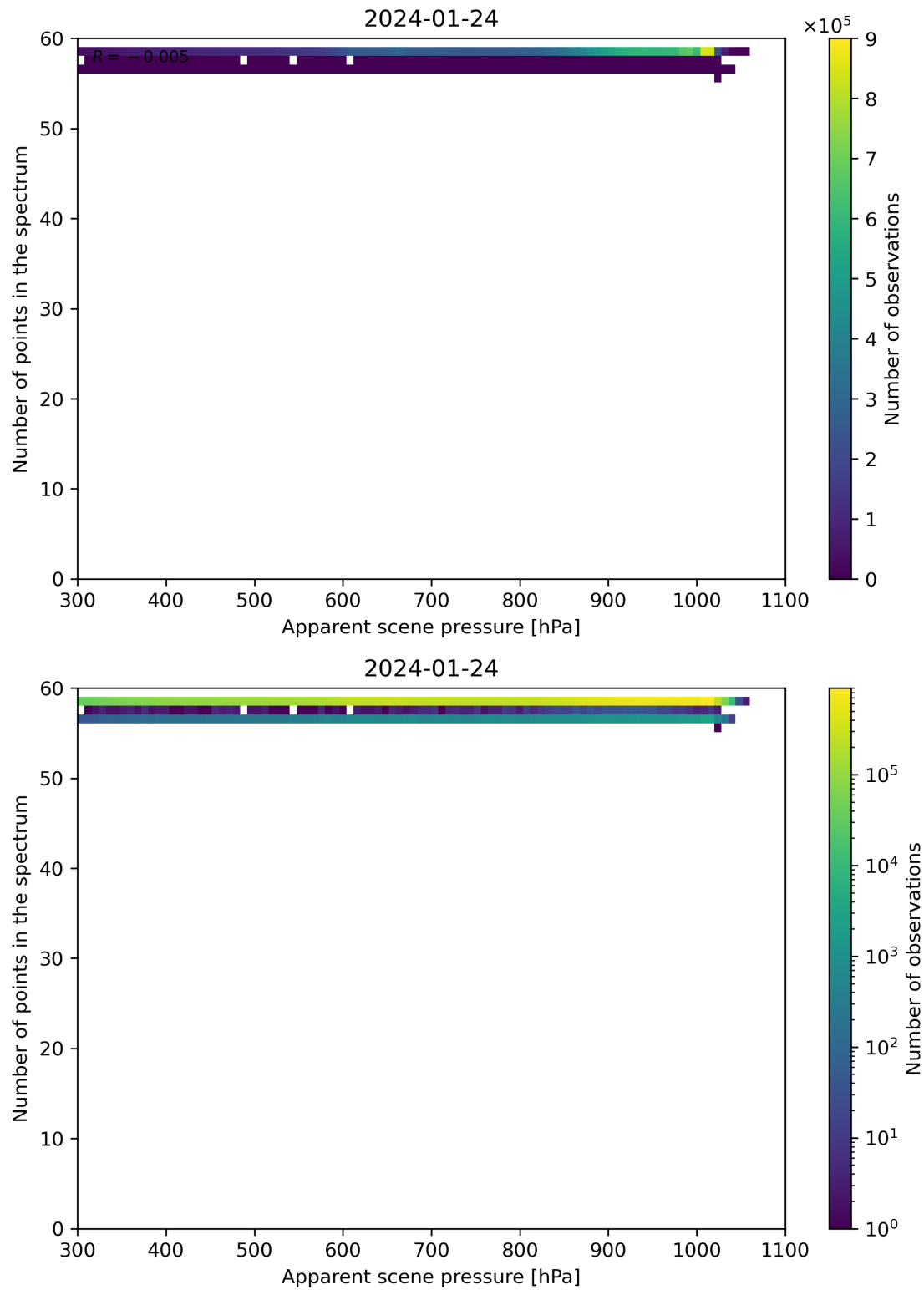
Figure 66: Scatter density plot of “Apparent scene pressure” against “Number of points in the spectrum” for 2024-01-23 to 2024-01-25.
