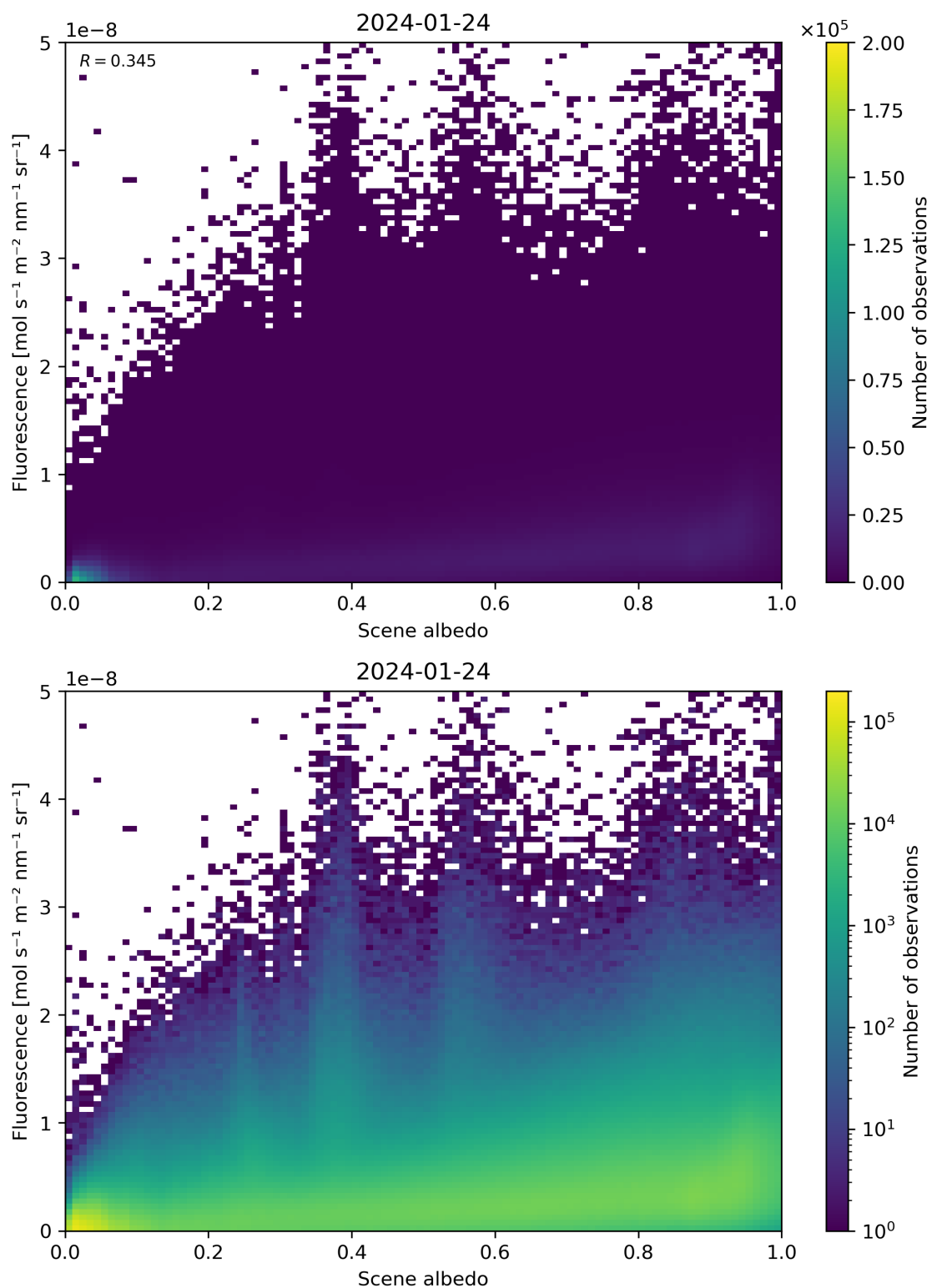
Figure 104: Scatter density plot of “Scene albedo” against “Fluorescence” for 2024-01-23 to 2024-01-25.
