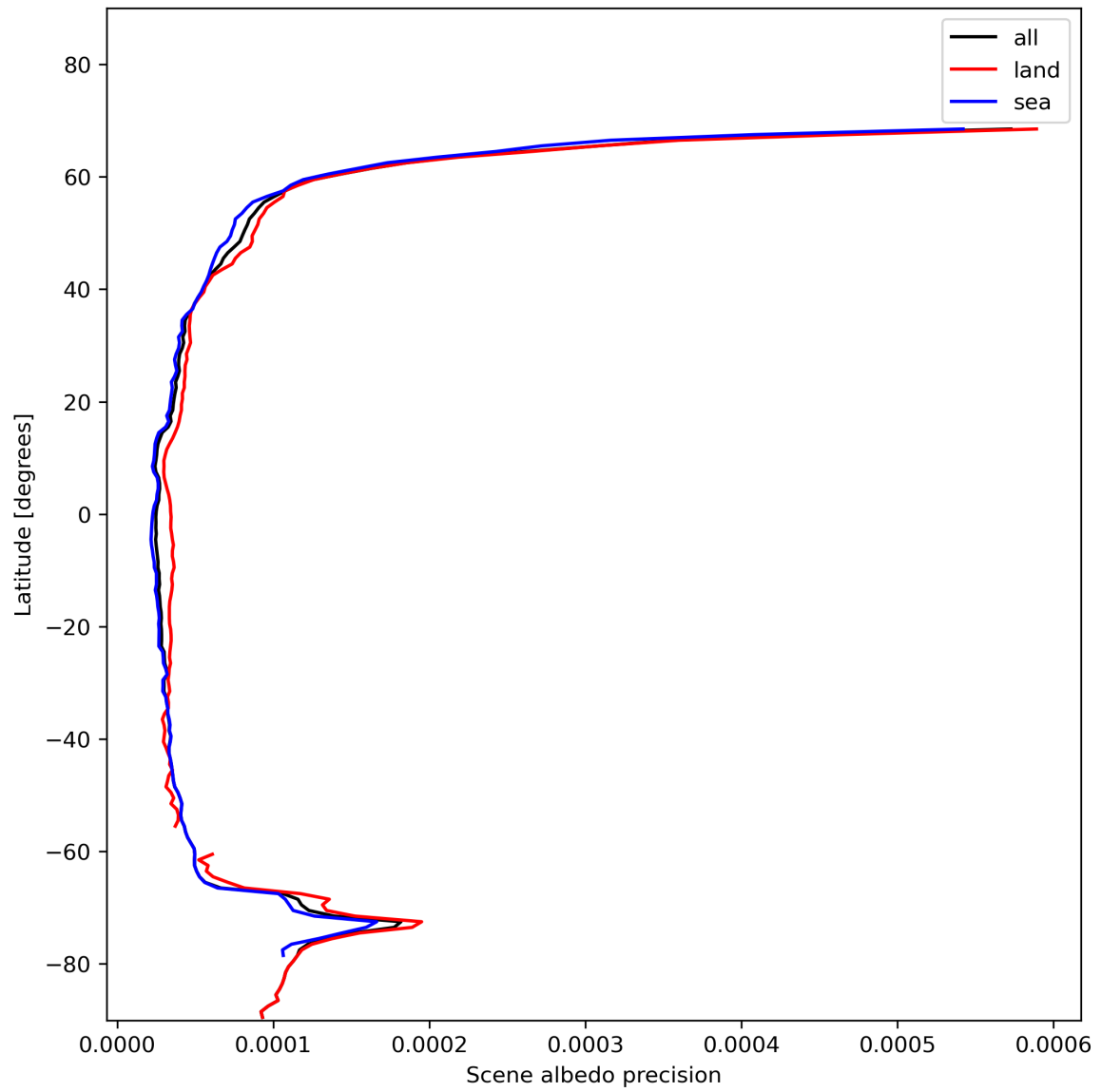
Figure 18: Zonal average of “Scene albedo precision” for 2024-01-23 to 2024-01-25.
