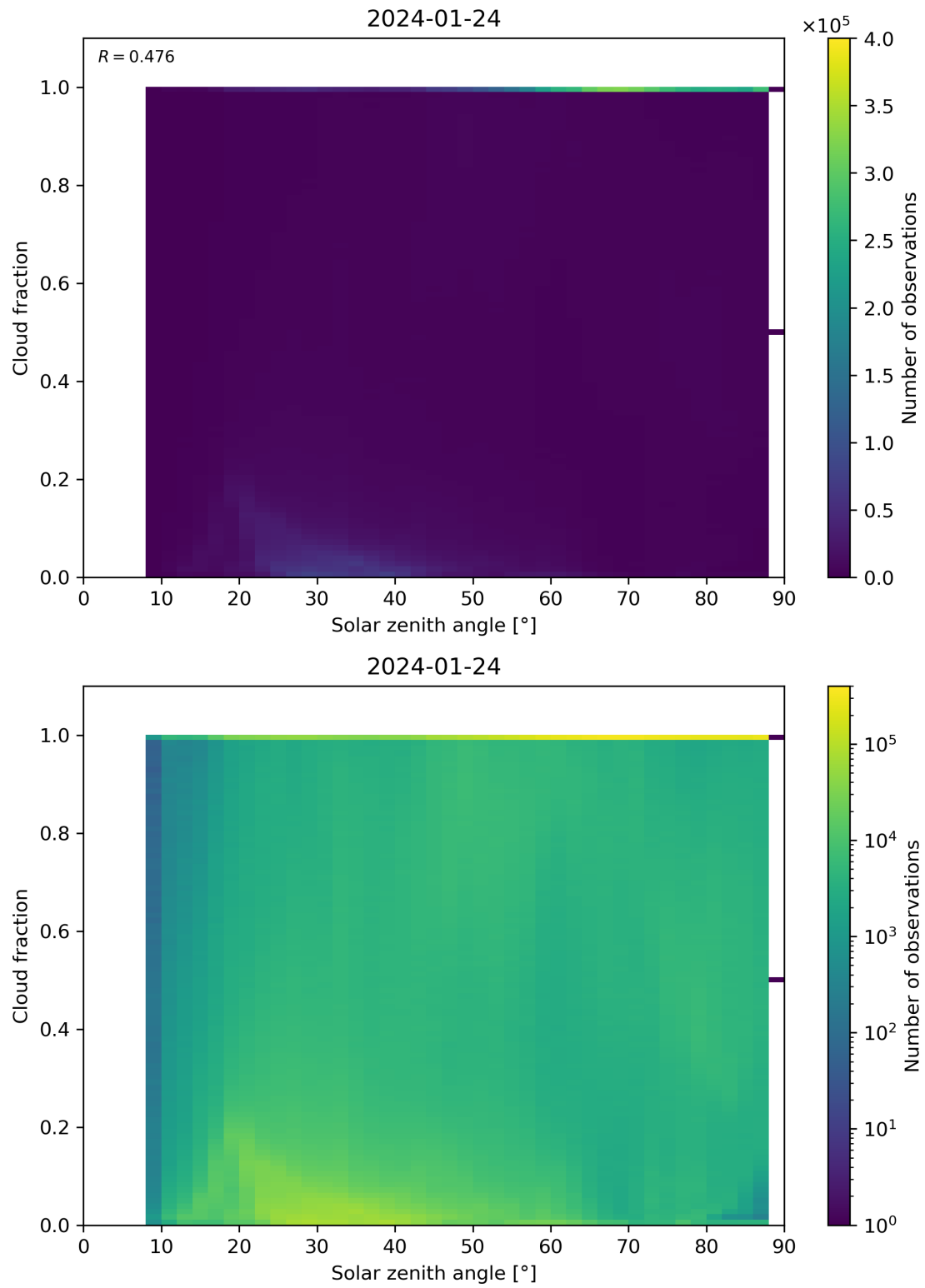
Figure 110: Scatter density plot of “Solar zenith angle” against “Cloud fraction” for 2024-01-23 to 2024-01-25.
