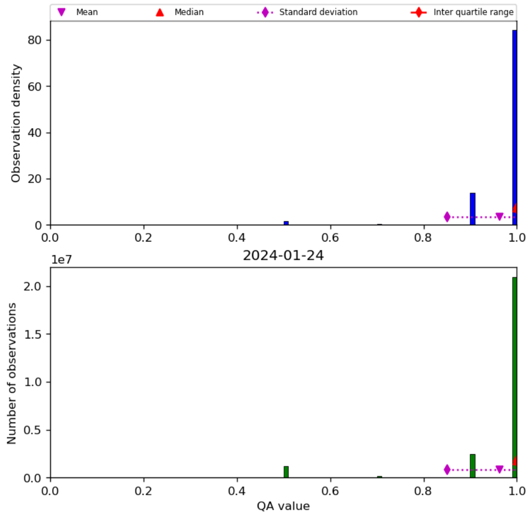
Figure 29: Histogram of “QA value” for 2024-01-23 to 2024-01-25
