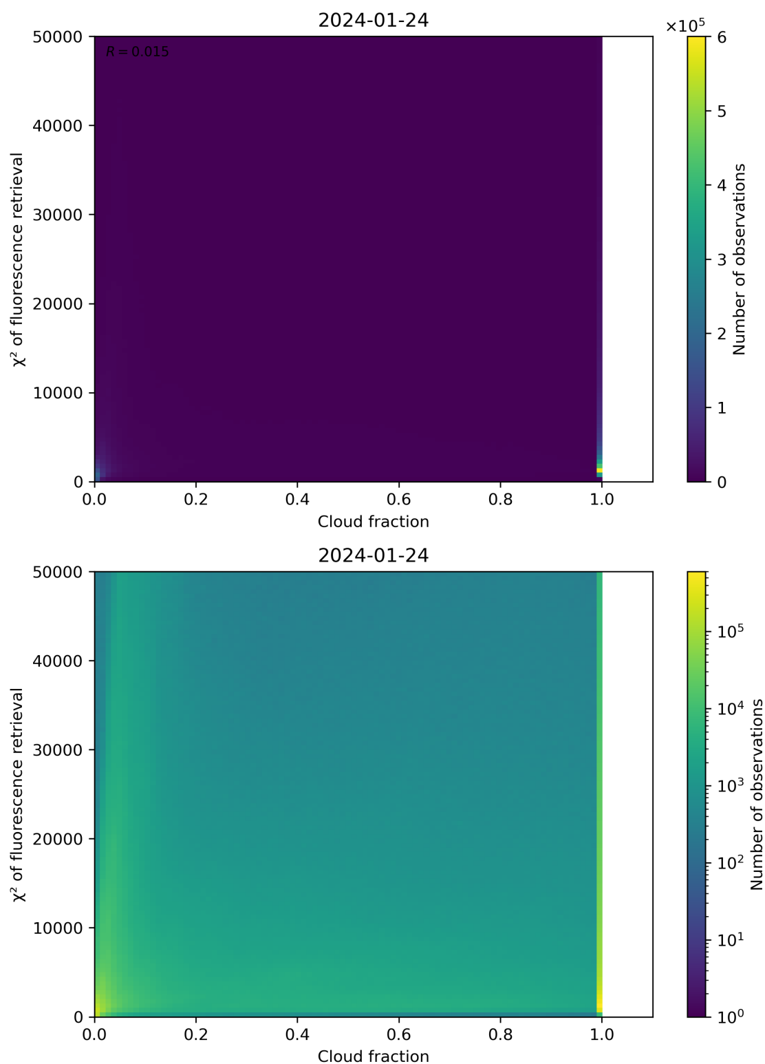
Figure 71: Scatter density plot of “Cloud fraction” against “ \chi^2 of fluorescence retrieval” for 2024-01-23 to 2024-01-25.
