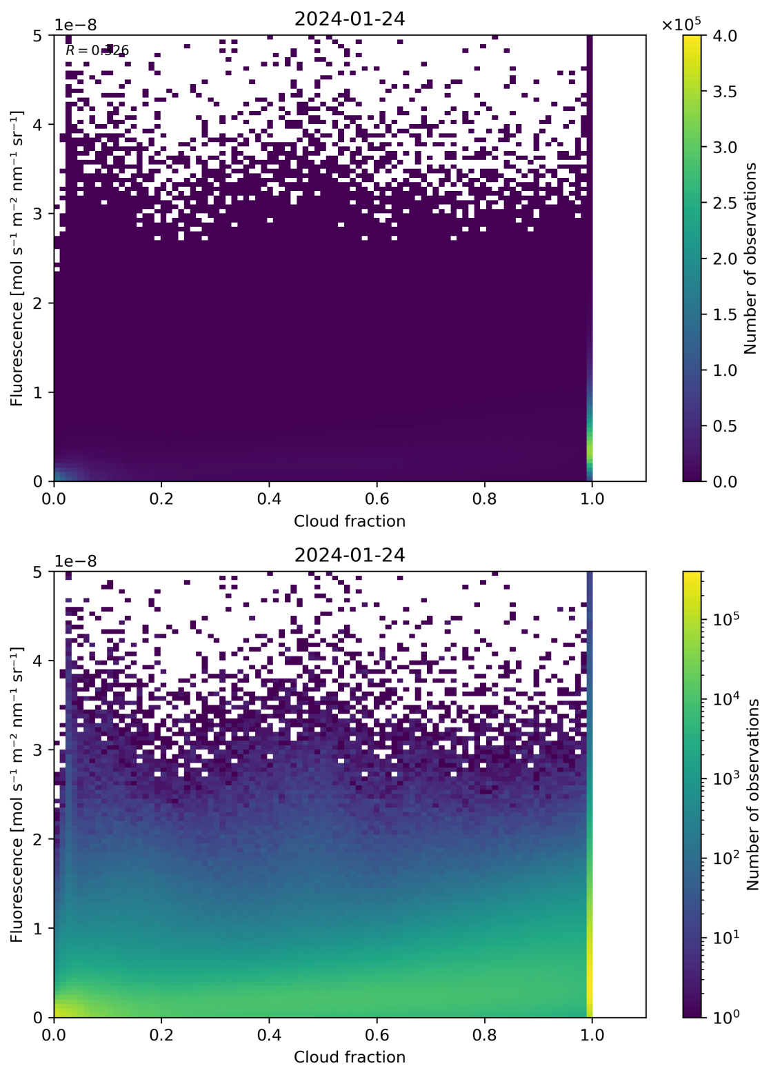
Figure 72: Scatter density plot of “Cloud fraction” against “Fluorescence” for 2024-01-23 to 2024-01-25.
