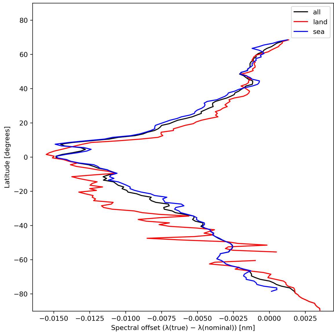
Figure 28: Zonal average of “Spectral offset ( \lambda(\text{true}) - \lambda(\text{nominal}) )” for 2024-01-23 to 2024-01-25.
