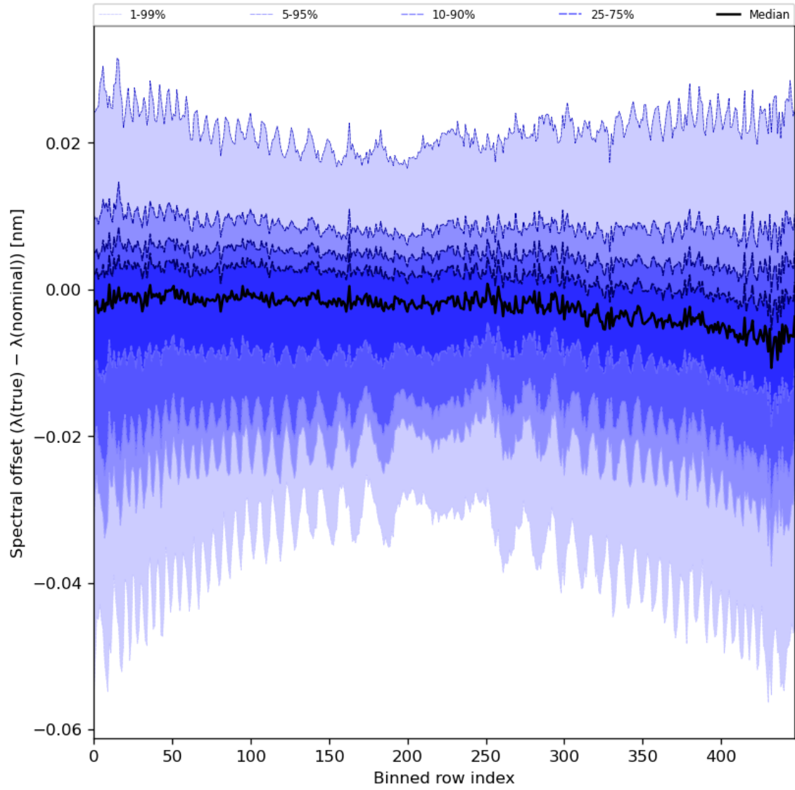
Figure 62: Along track statistics of “Spectral offset ( \lambda(\text{true}) - \lambda(\text{nominal}) )” for 2024-01-23 to 2024-01-25
