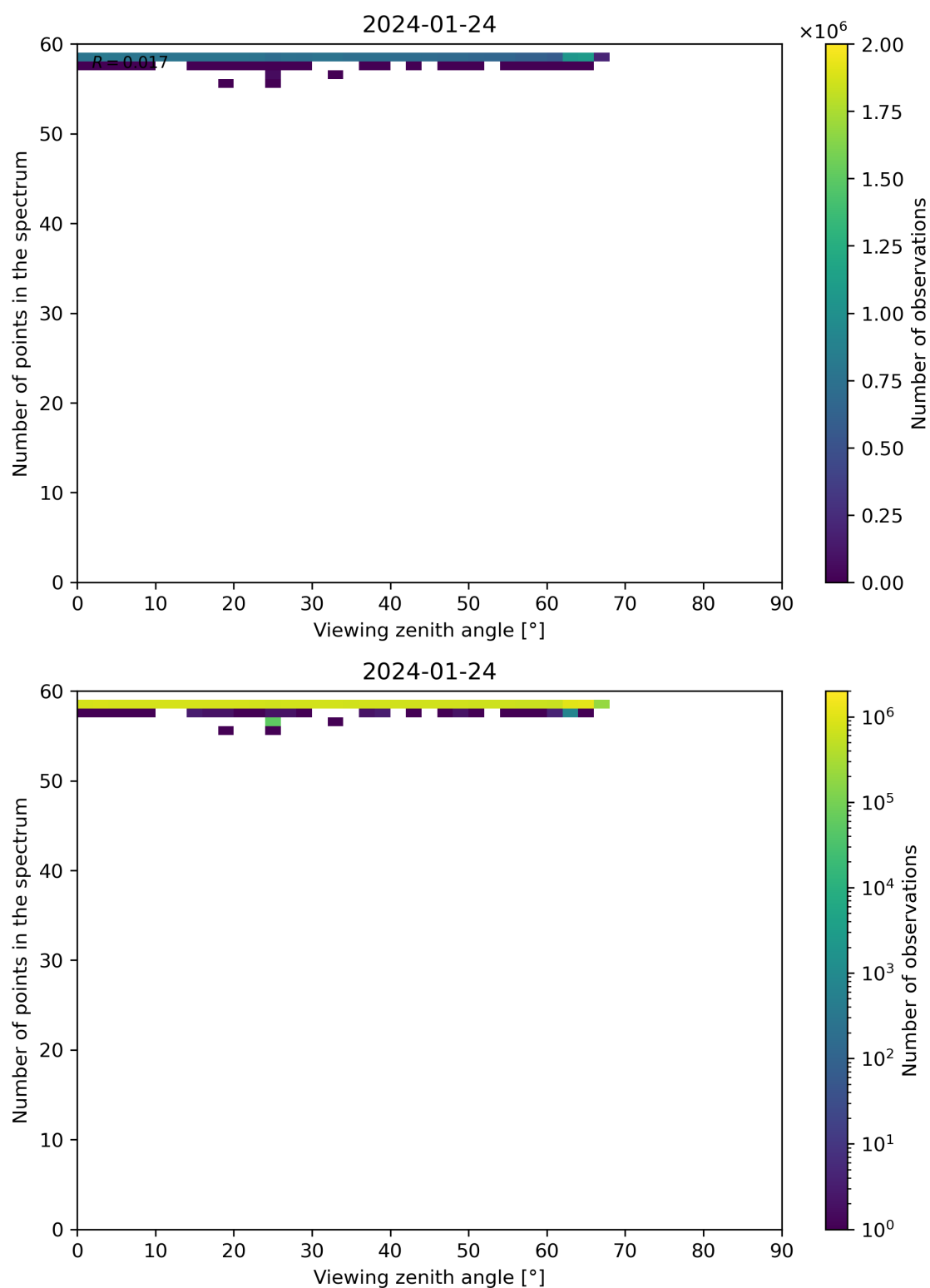
Figure 125: Scatter density plot of “Viewing zenith angle” against “Number of points in the spectrum” for 2024-01-23 to 2024-01-25.
