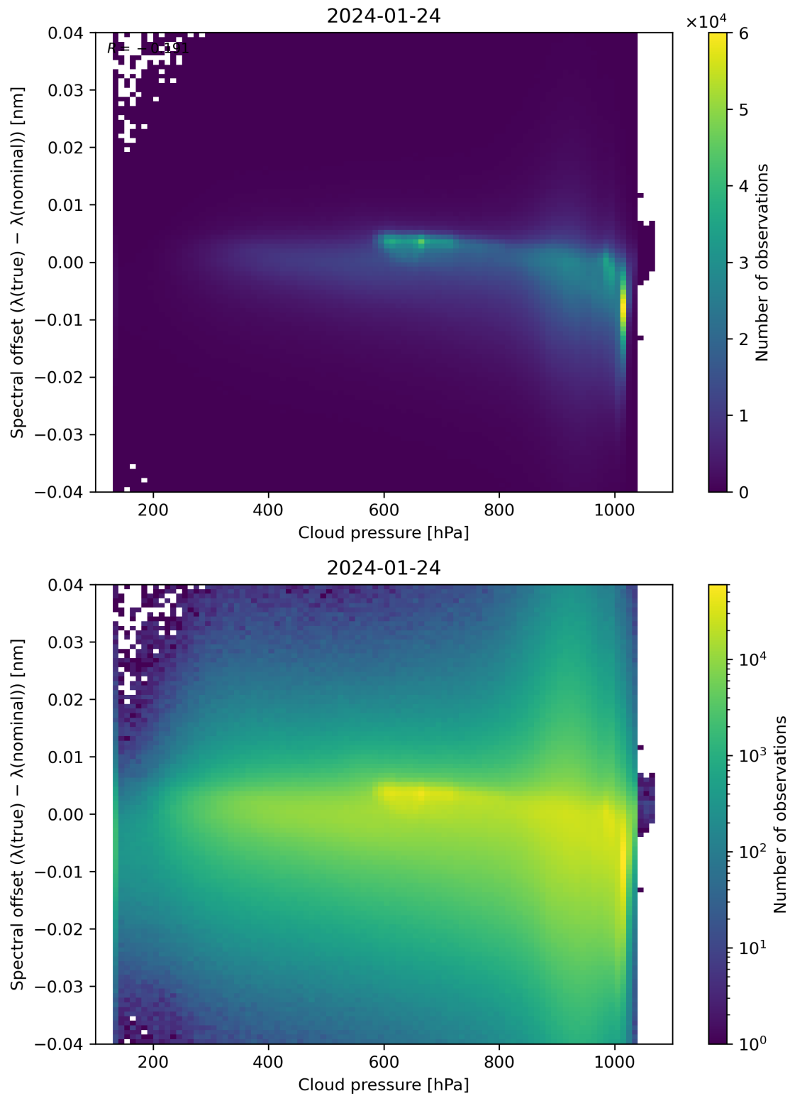
Figure 84: Scatter density plot of “Cloud pressure” against “Spectral offset ( \lambda(\text{true}) - \lambda(\text{nominal}) )” for 2024-01-23 to 2024-01-25.
