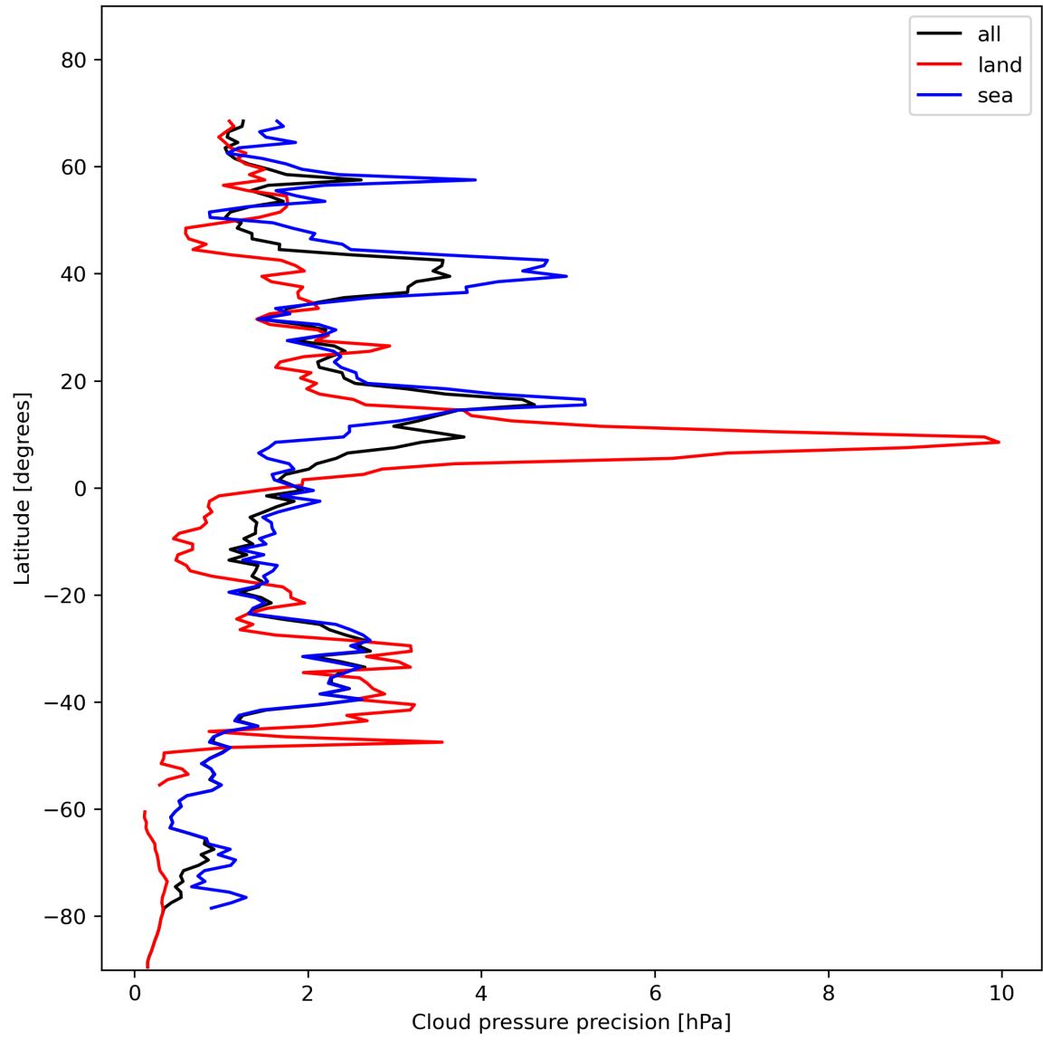
Figure 14: Zonal average of “Cloud pressure precision” for 2024-01-23 to 2024-01-25.
