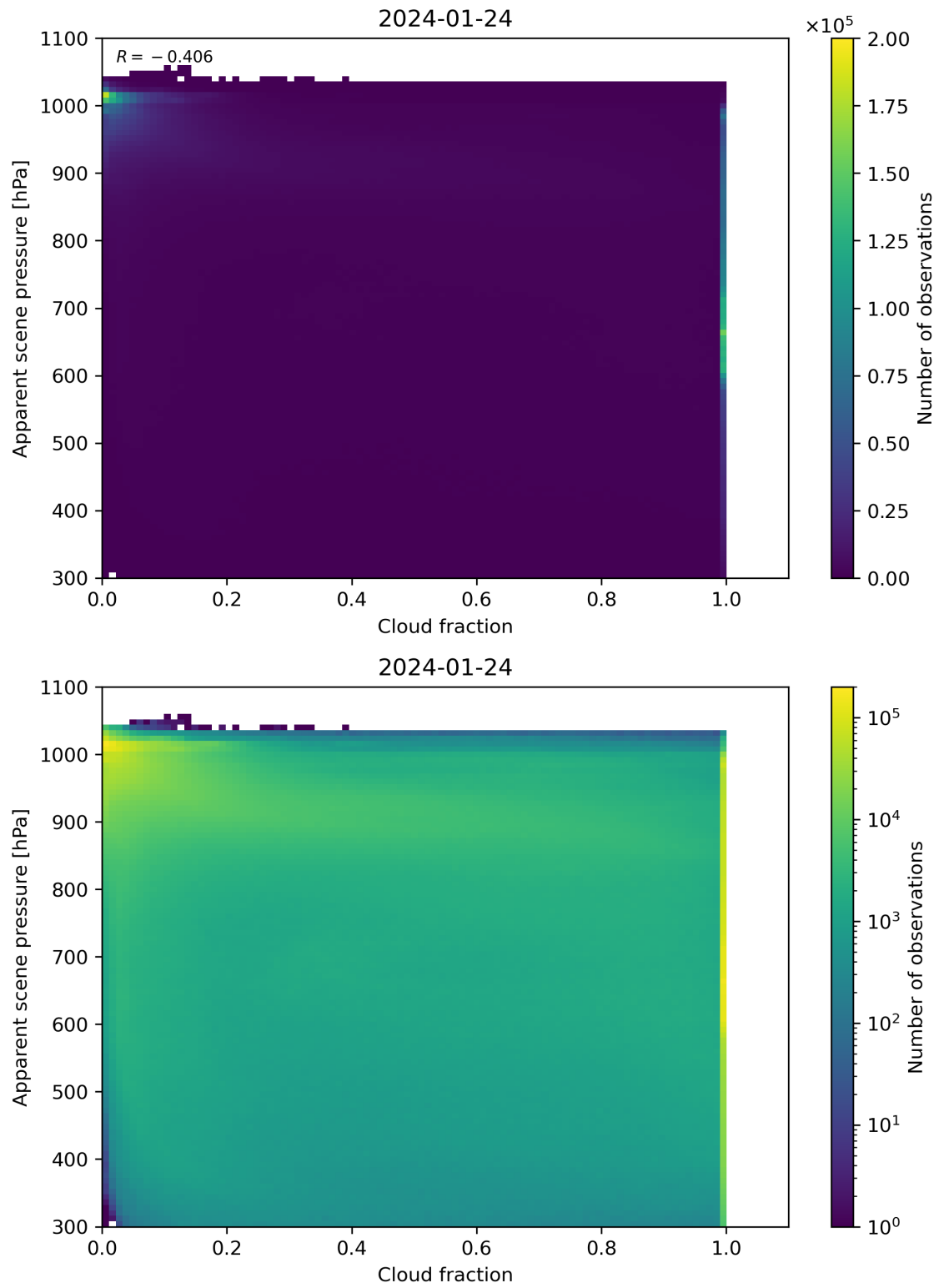
Figure 70: Scatter density plot of “Cloud fraction” against “Apparent scene pressure” for 2024-01-23 to 2024-01-25.
