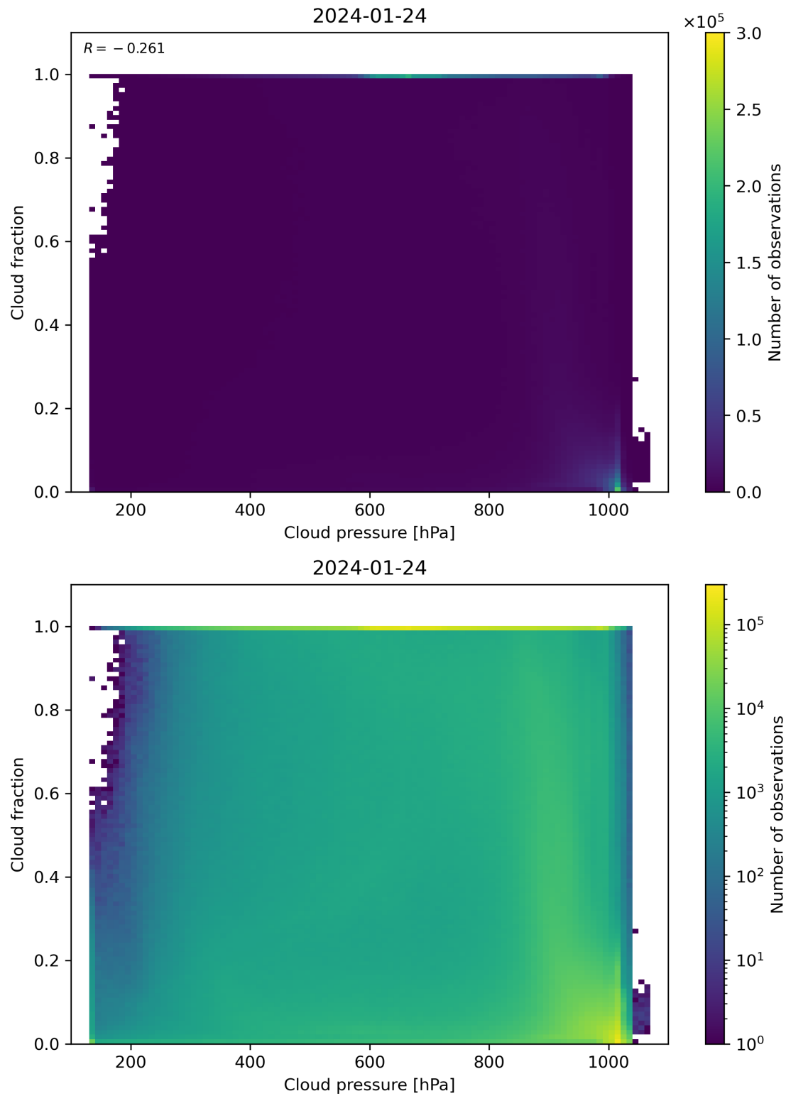
Figure 79: Scatter density plot of “Cloud pressure” against “Cloud fraction” for 2024-01-23 to 2024-01-25.
