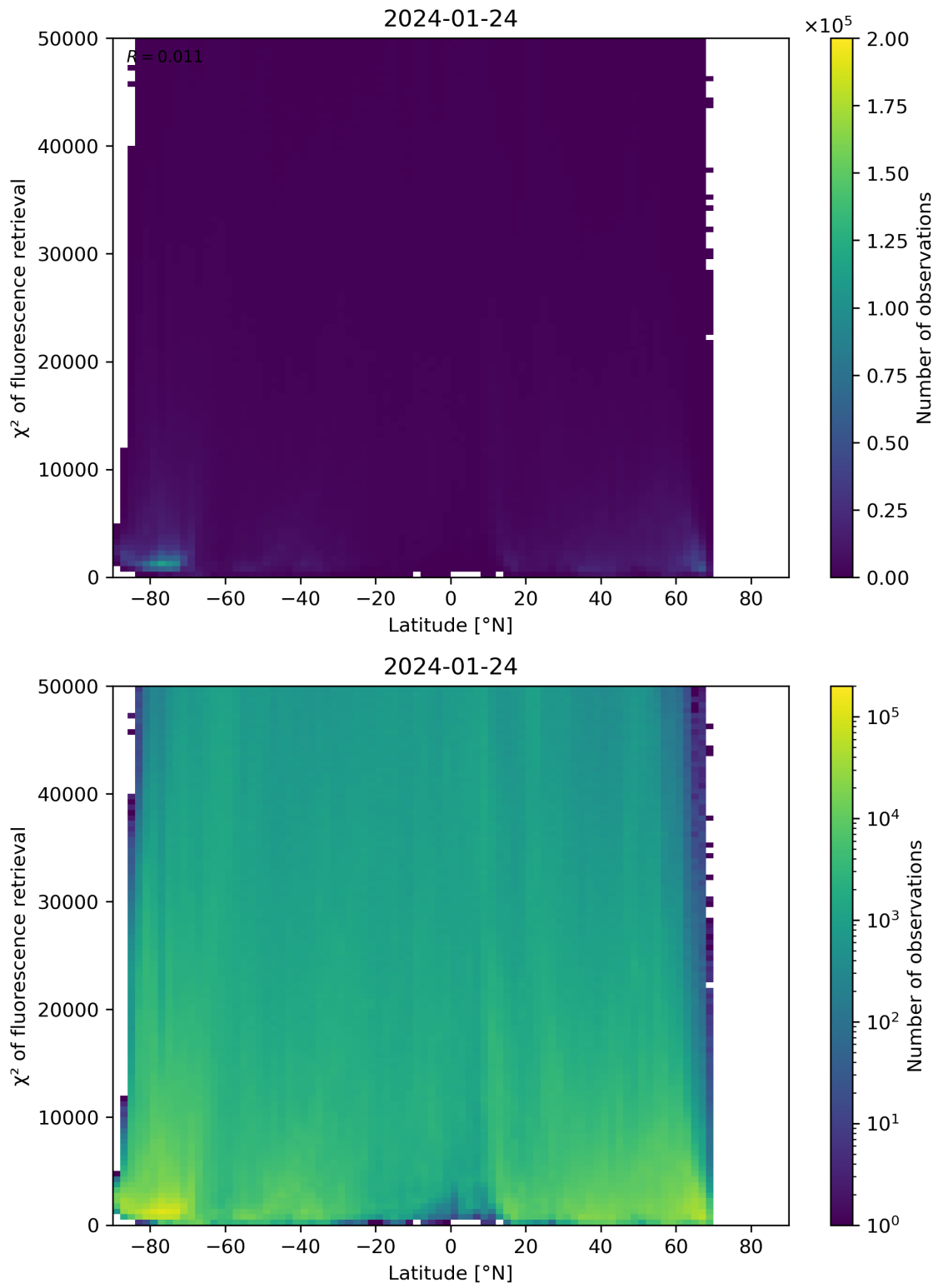
Figure 89: Scatter density plot of “Latitude” against “ \chi^2 of fluorescence retrieval” for 2024-01-23 to 2024-01-25.
