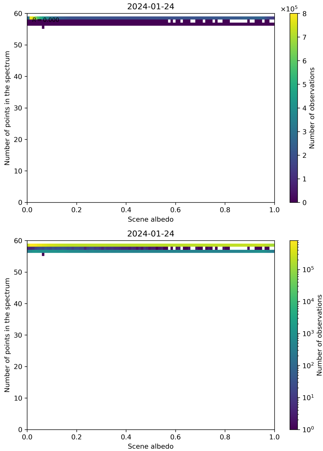
Figure 106: Scatter density plot of “Scene albedo” against “Number of points in the spectrum” for 2024-01-23 to 2024-01-25.
