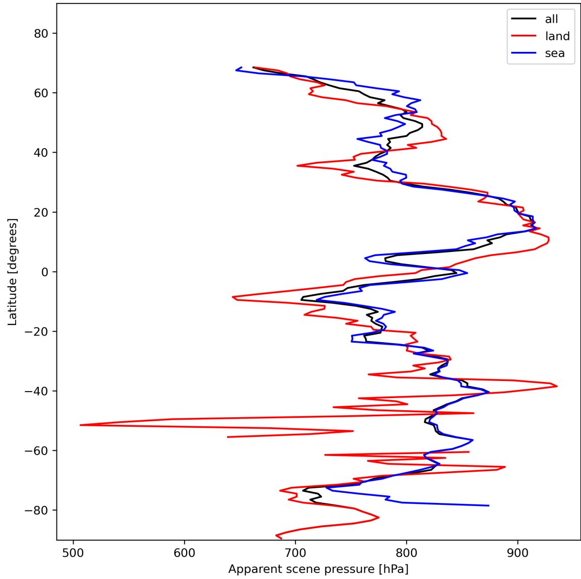
Figure 19: Zonal average of “Apparent scene pressure” for 2024-01-23 to 2024-01-25.
