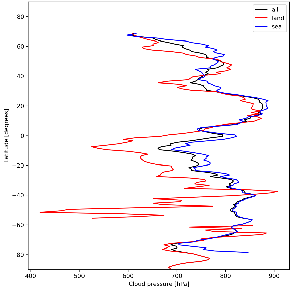
Figure 13: Zonal average of “Cloud pressure” for 2024-01-23 to 2024-01-25.
