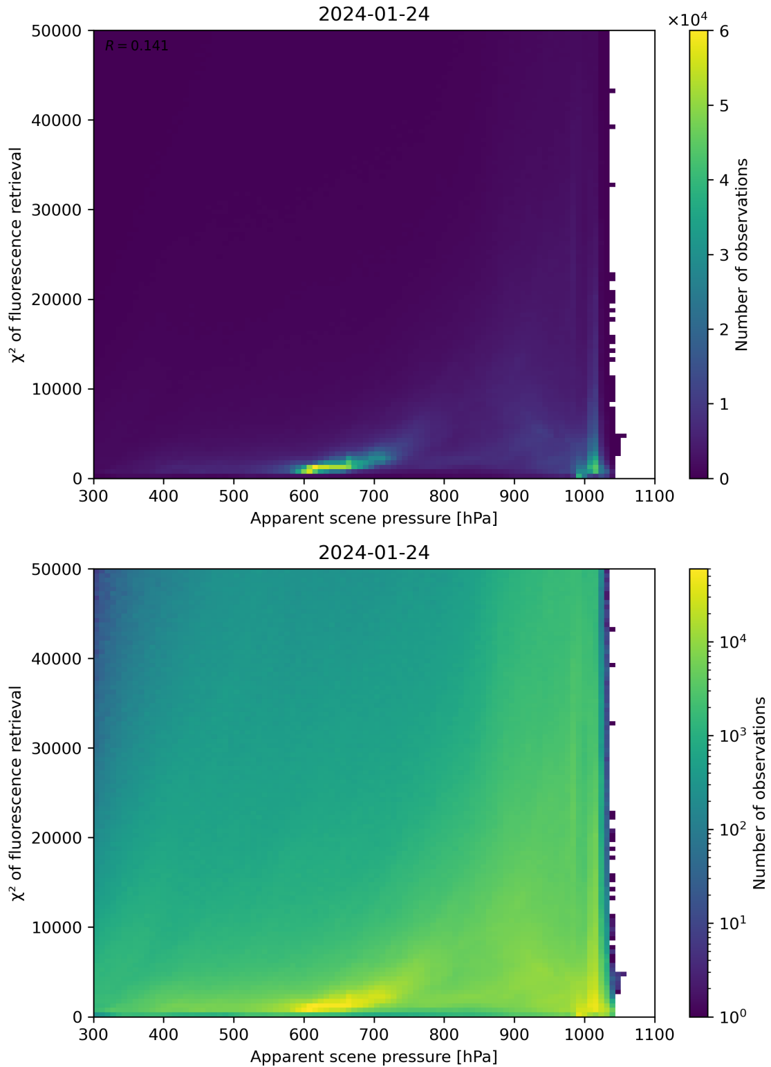
Figure 63: Scatter density plot of “Apparent scene pressure” against “ \chi^2 of fluorescence retrieval” for 2024-01-23 to 2024-01-25.
