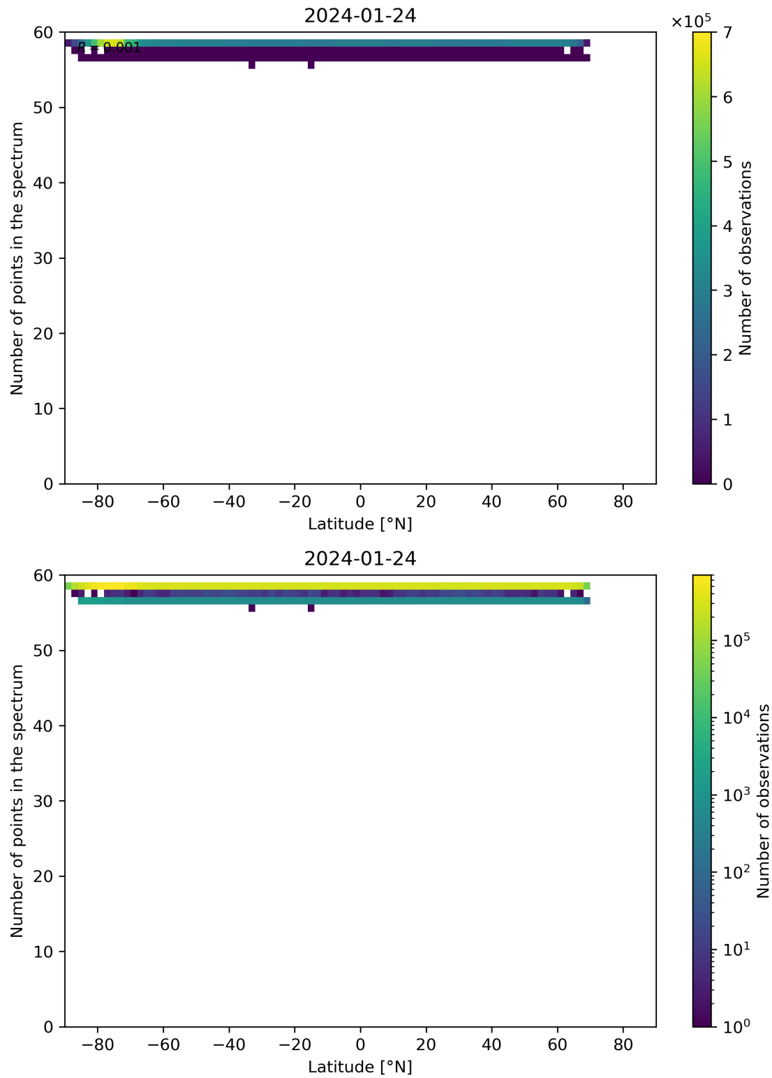
Figure 94: Scatter density plot of “Latitude” against “Number of points in the spectrum” for 2024-01-23 to 2024-01-25.
