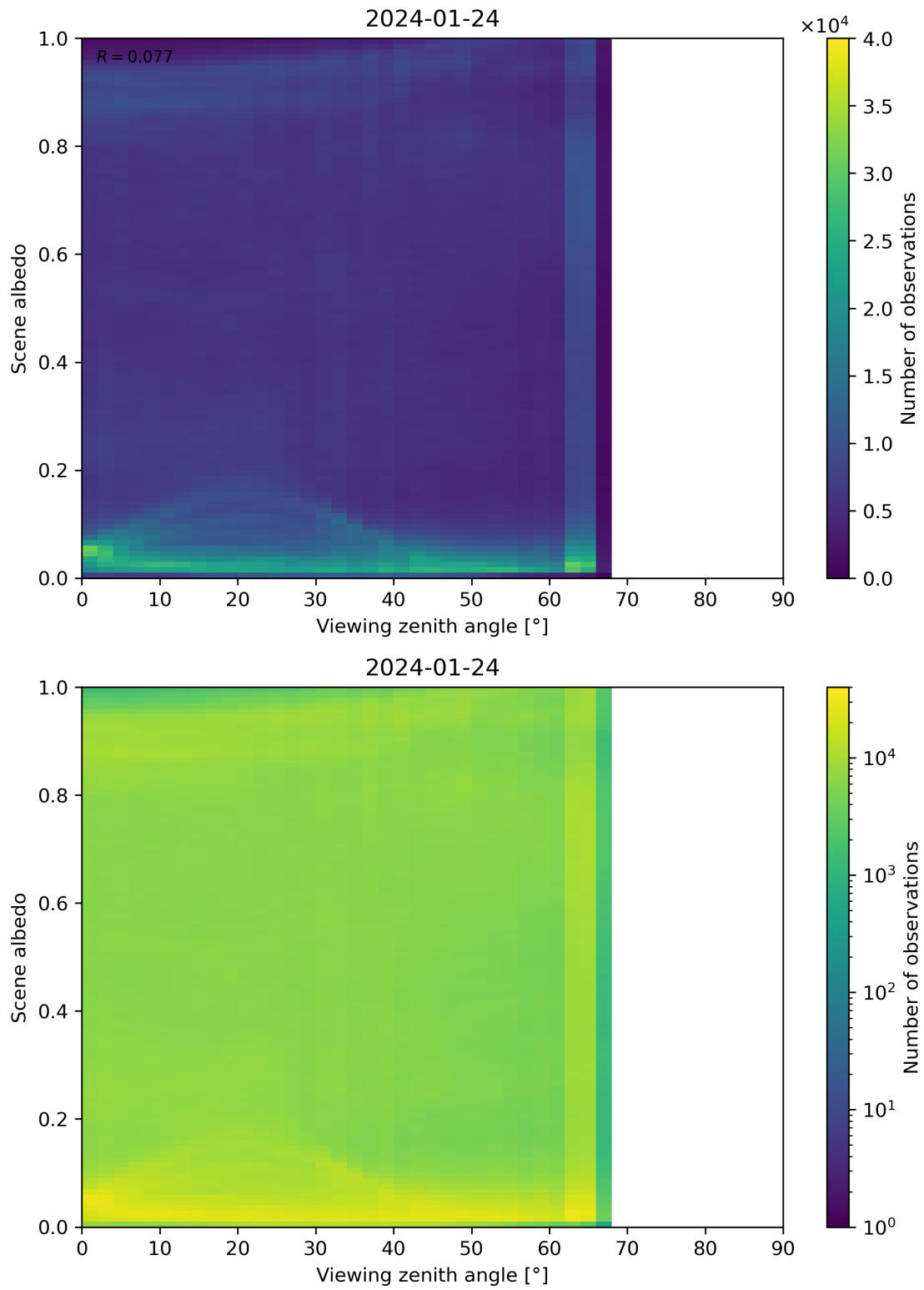
Figure 126: Scatter density plot of “Viewing zenith angle” against “Scene albedo” for 2024-01-23 to 2024-01-25.
