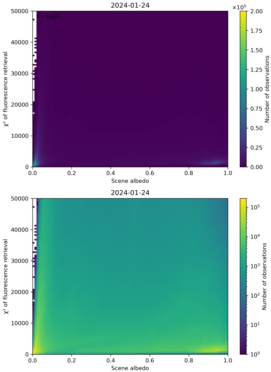
Figure 103: Scatter density plot of “Scene albedo” against “ \chi^2 of fluorescence retrieval” for 2024-01-23 to 2024-01-25.
