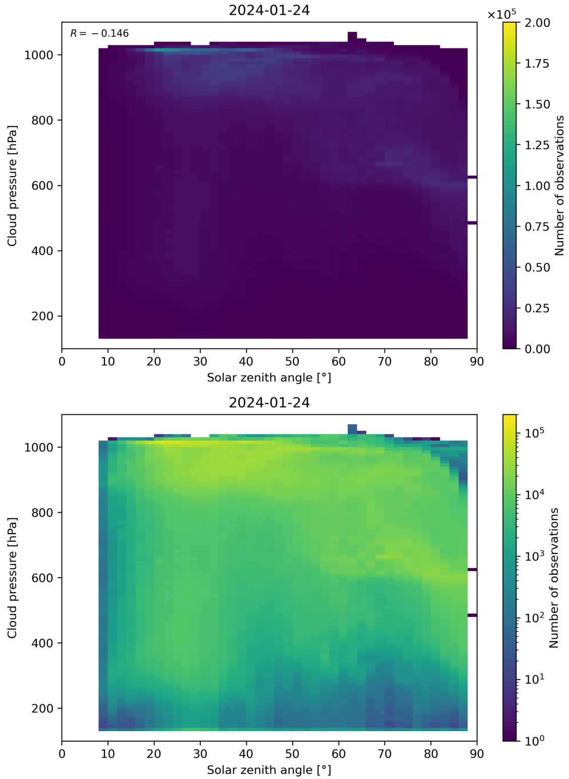
Figure 111: Scatter density plot of “Solar zenith angle” against “Cloud pressure” for 2024-01-23 to 2024-01-25.
