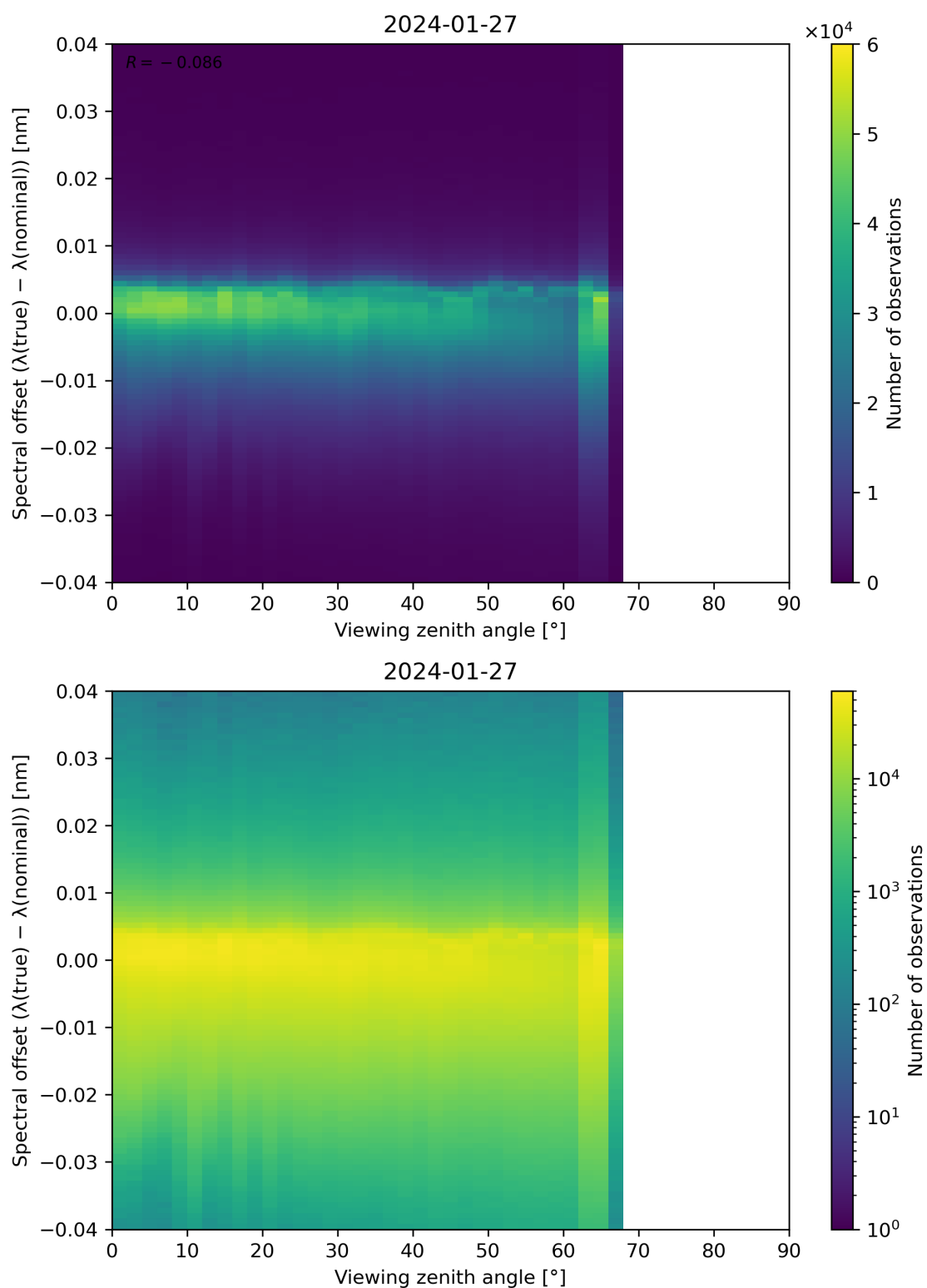
Figure 128: Scatter density plot of “Viewing zenith angle” against “Spectral offset ( \lambda(\text{true}) - \lambda(\text{nominal}) )” for 2024-01-26 to 2024-01-28.
