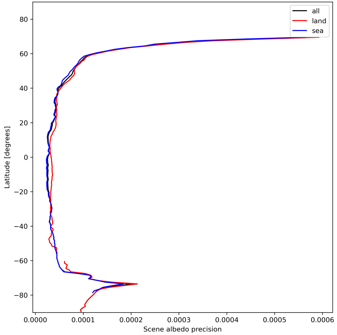
Figure 18: Zonal average of “Scene albedo precision” for 2024-01-26 to 2024-01-28.
