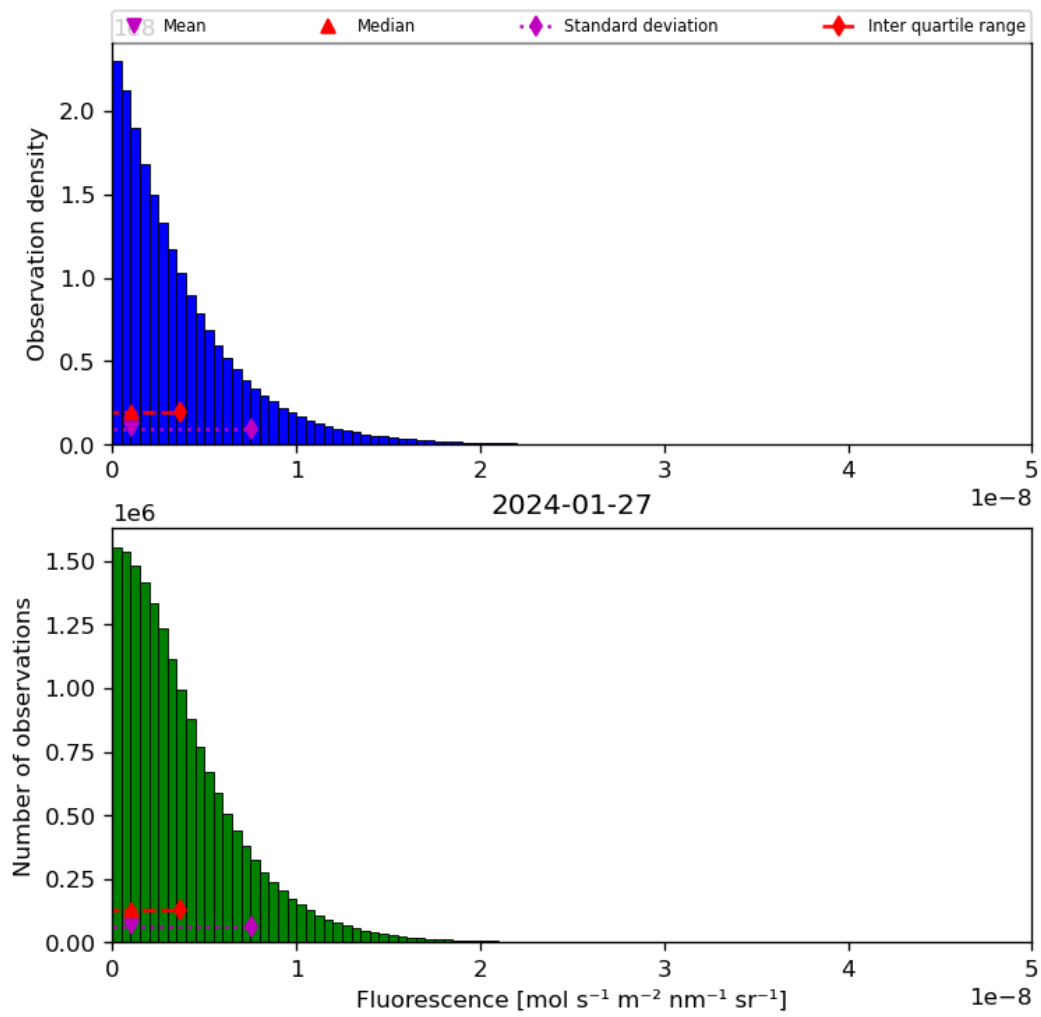
Figure 40: Histogram of “Fluorescence” for 2024-01-26 to 2024-01-28
