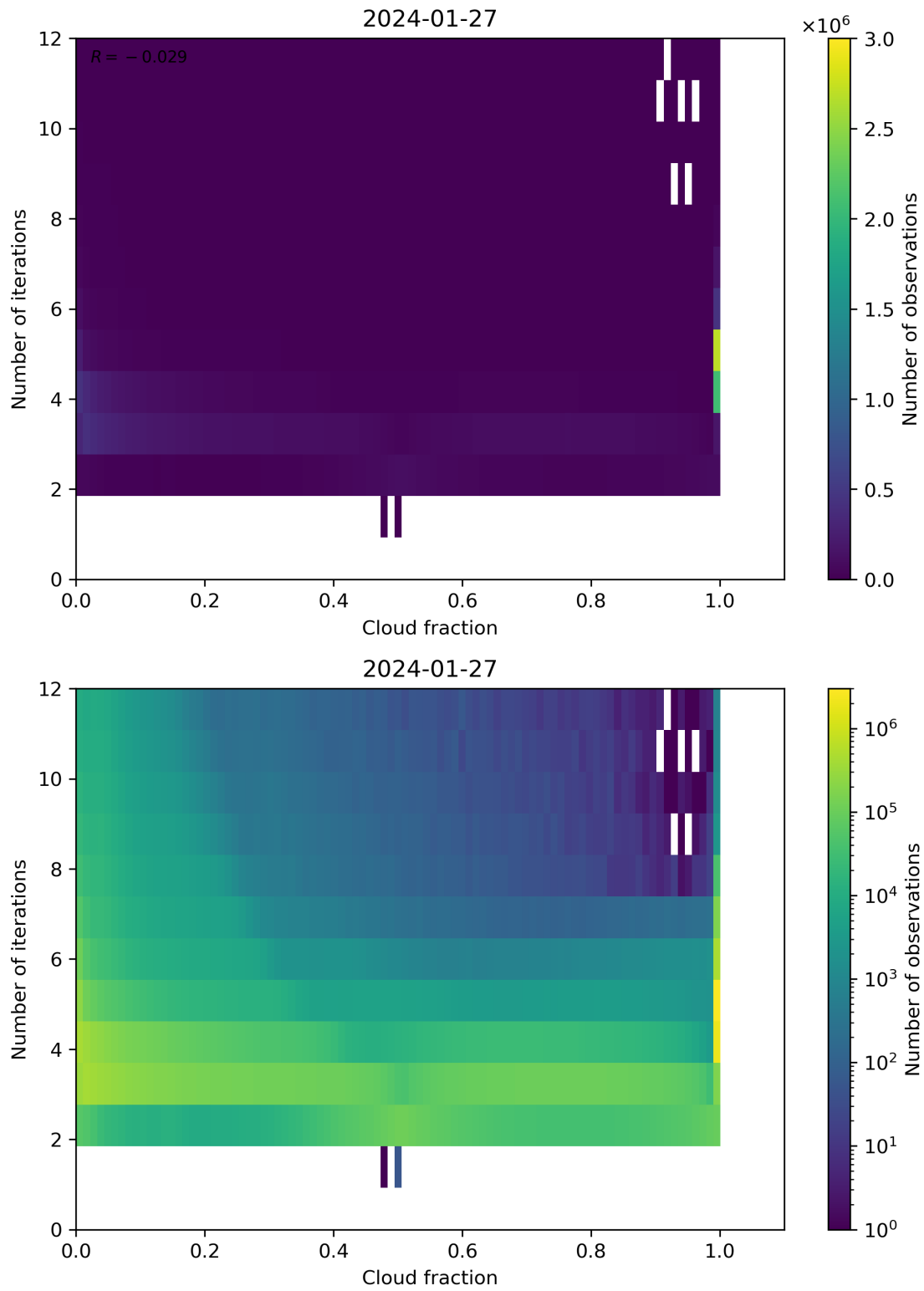
Figure 73: Scatter density plot of “Cloud fraction” against “Number of iterations” for 2024-01-26 to 2024-01-28.
