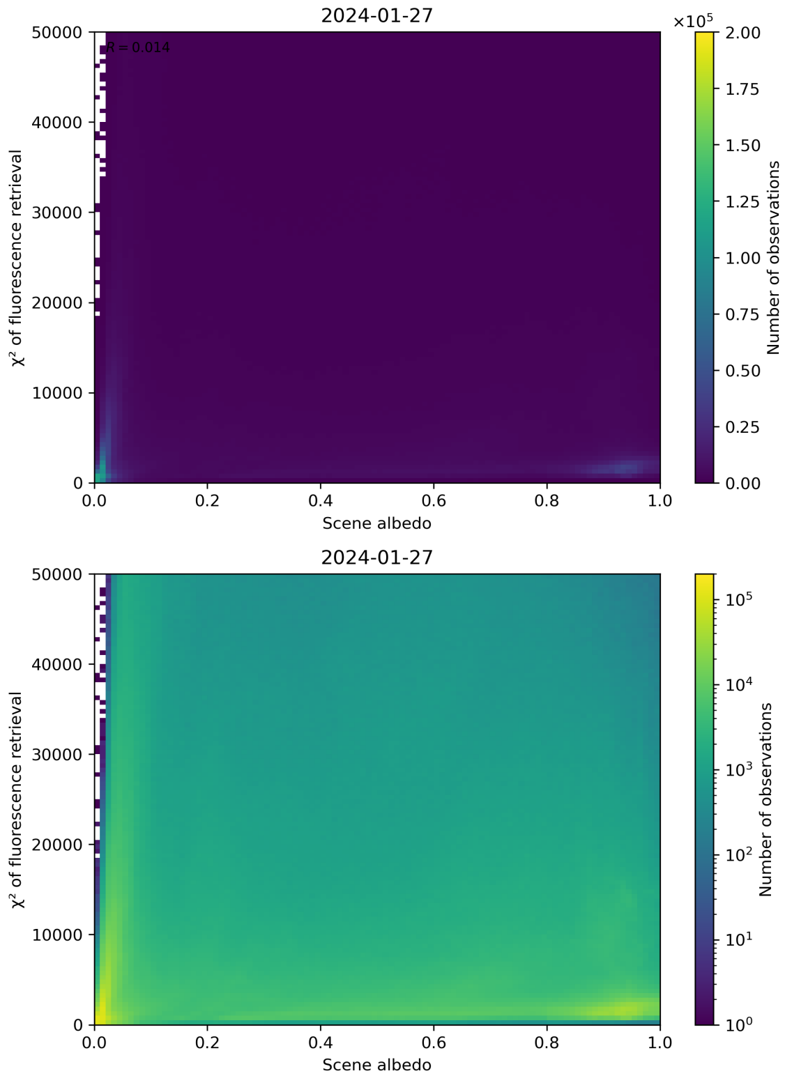
Figure 103: Scatter density plot of “Scene albedo” against “ \chi^2 of fluorescence retrieval” for 2024-01-26 to 2024-01-28.
