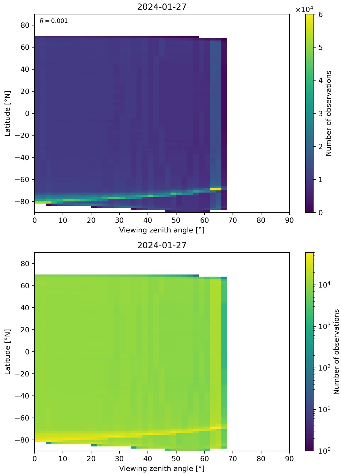
Figure 123: Scatter density plot of “Viewing zenith angle” against “Latitude” for 2024-01-26 to 2024-01-28.
