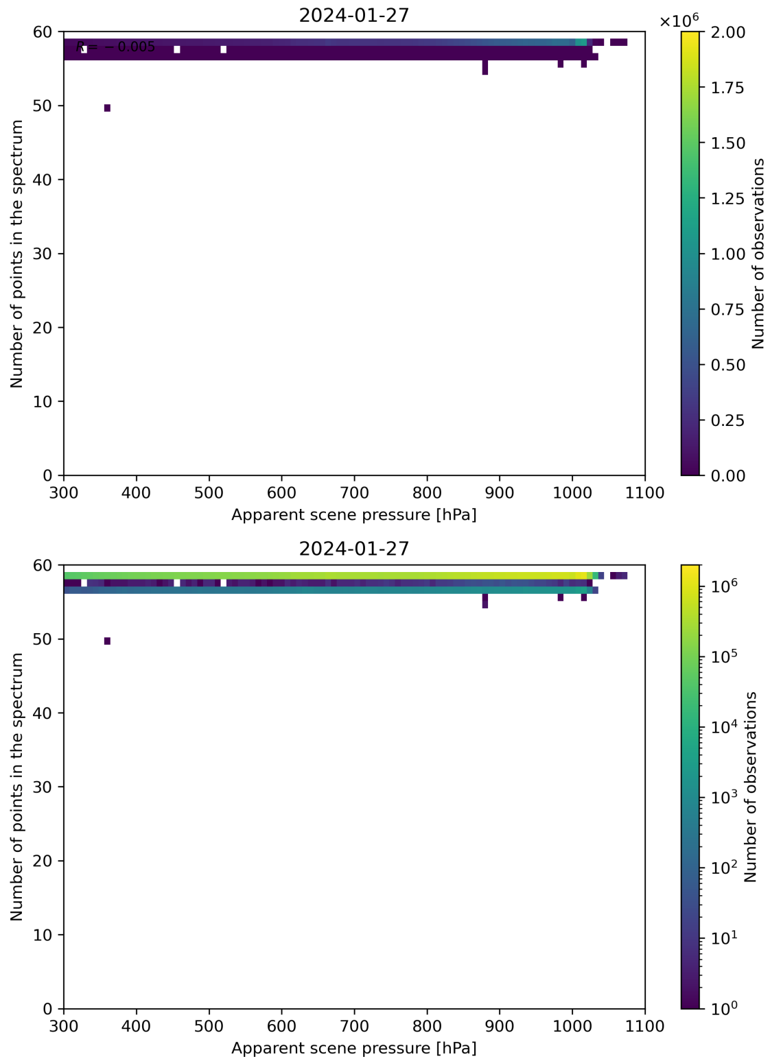
Figure 66: Scatter density plot of “Apparent scene pressure” against “Number of points in the spectrum” for 2024-01-26 to 2024-01-28.
