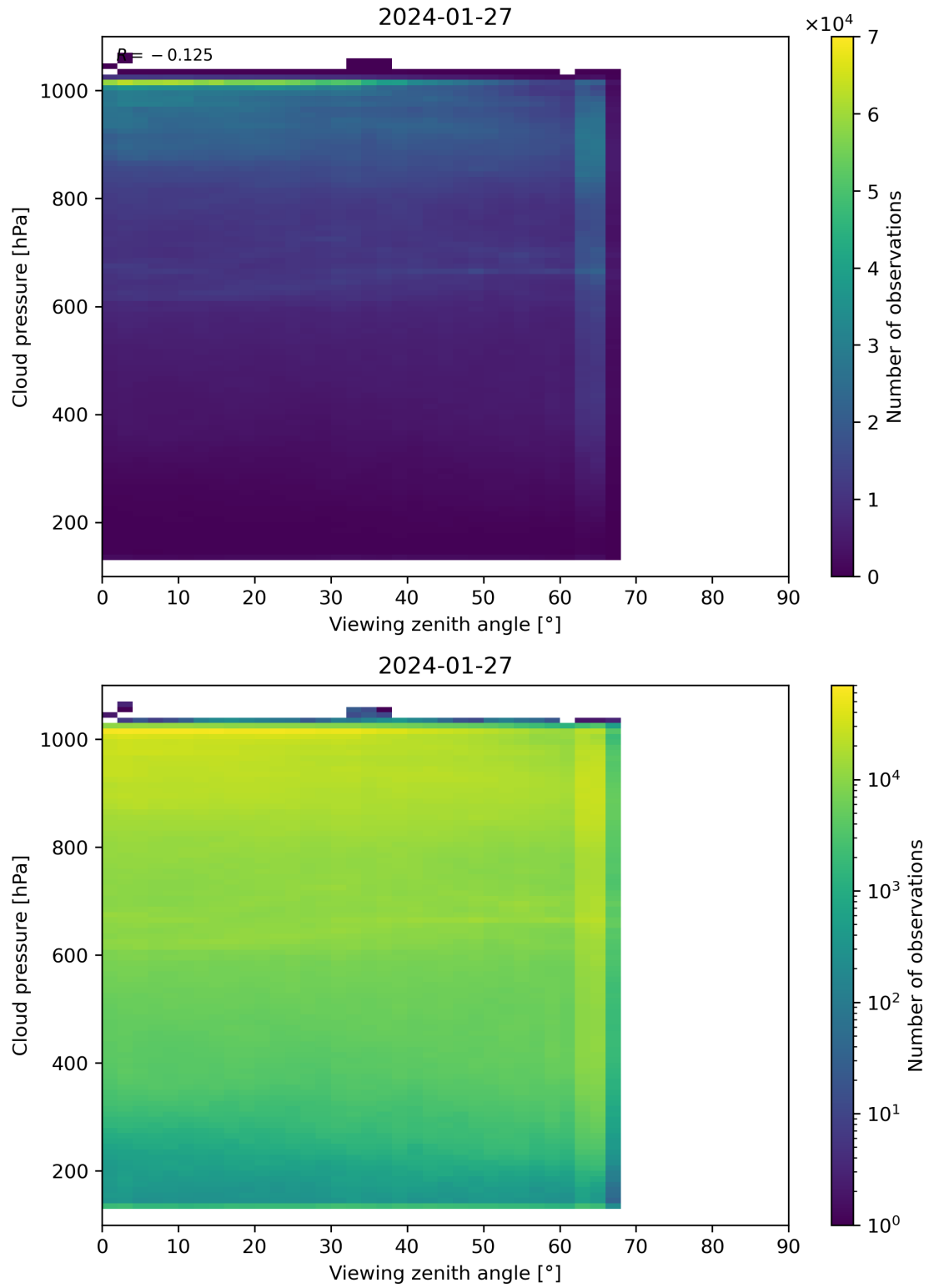
Figure 121: Scatter density plot of “Viewing zenith angle” against “Cloud pressure” for 2024-01-26 to 2024-01-28.
