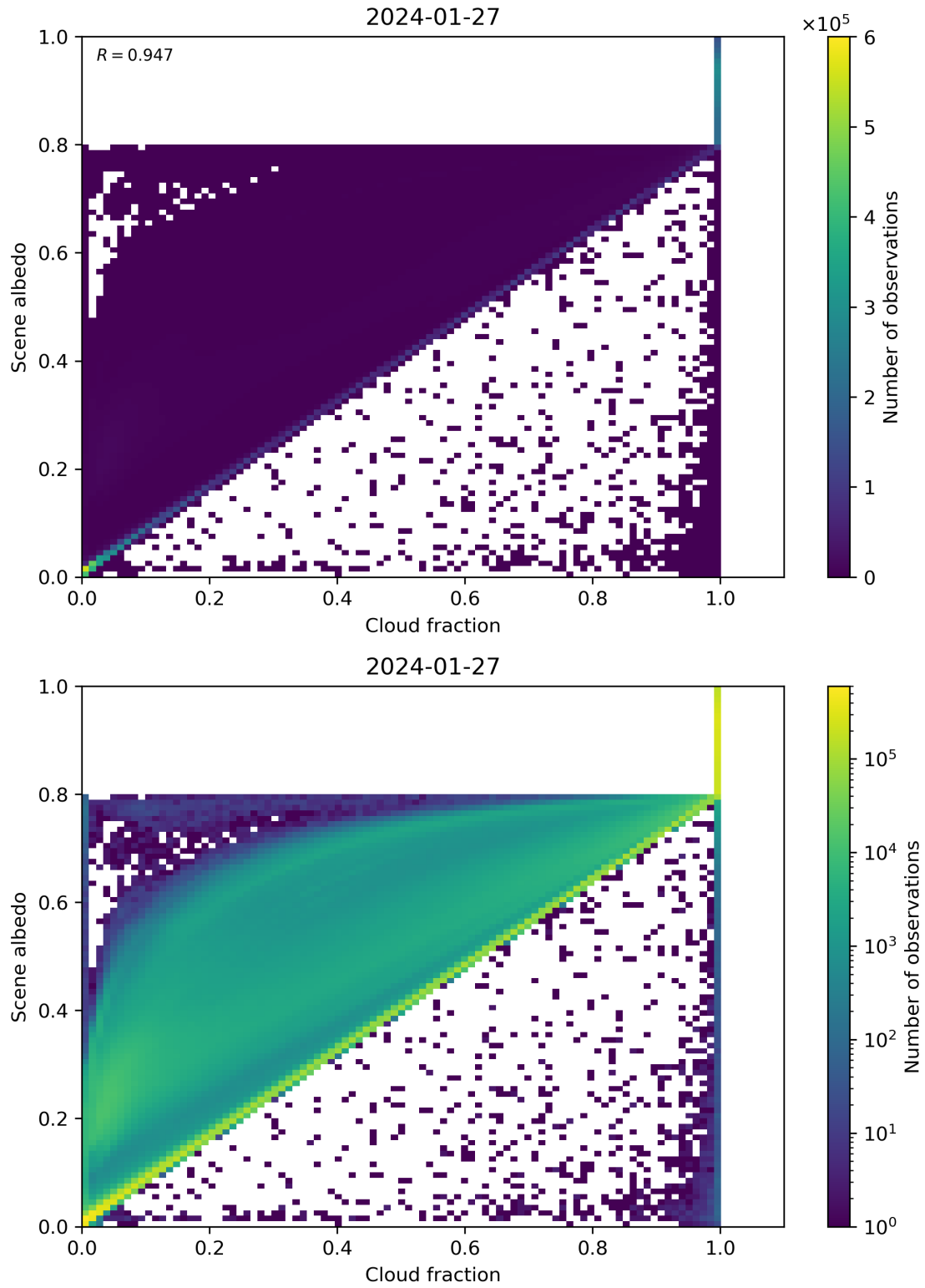
Figure 75: Scatter density plot of “Cloud fraction” against “Scene albedo” for 2024-01-26 to 2024-01-28.
