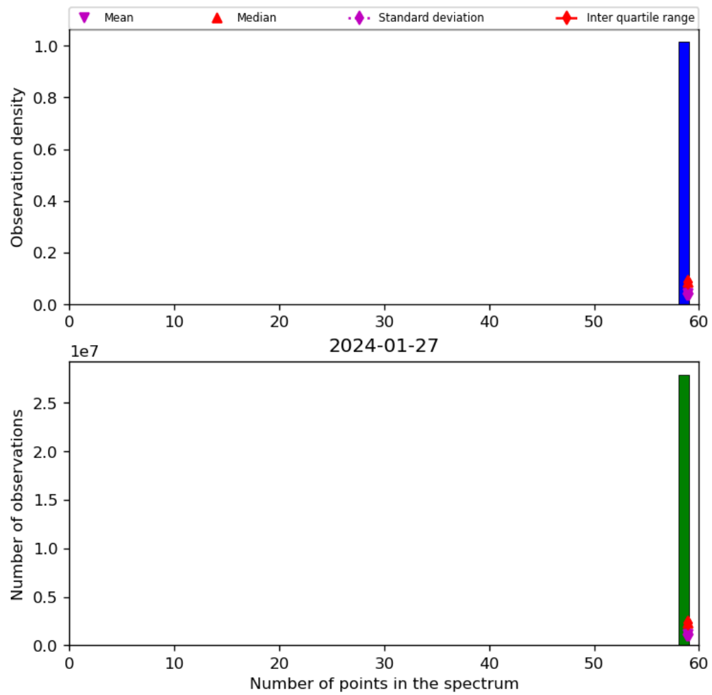
Figure 44: Histogram of “Number of points in the spectrum” for 2024-01-26 to 2024-01-28
