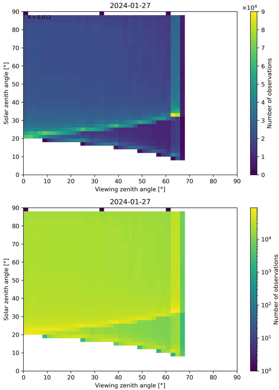
Figure 127: Scatter density plot of “Viewing zenith angle” against “Solar zenith angle” for 2024-01-26 to 2024-01-28.
