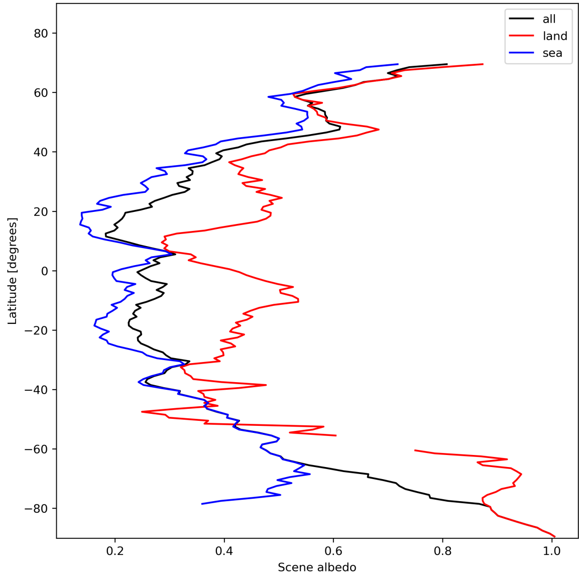
Figure 17: Zonal average of “Scene albedo” for 2024-01-26 to 2024-01-28.
