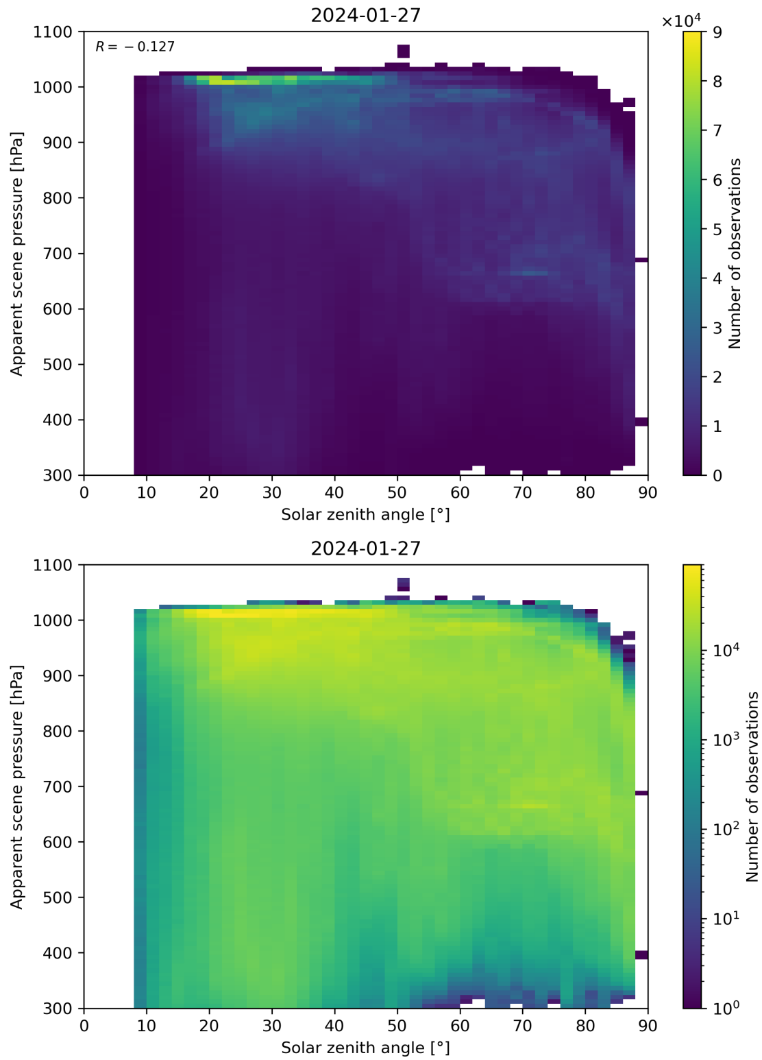
Figure 108: Scatter density plot of “Solar zenith angle” against “Apparent scene pressure” for 2024-01-26 to 2024-01-28.
