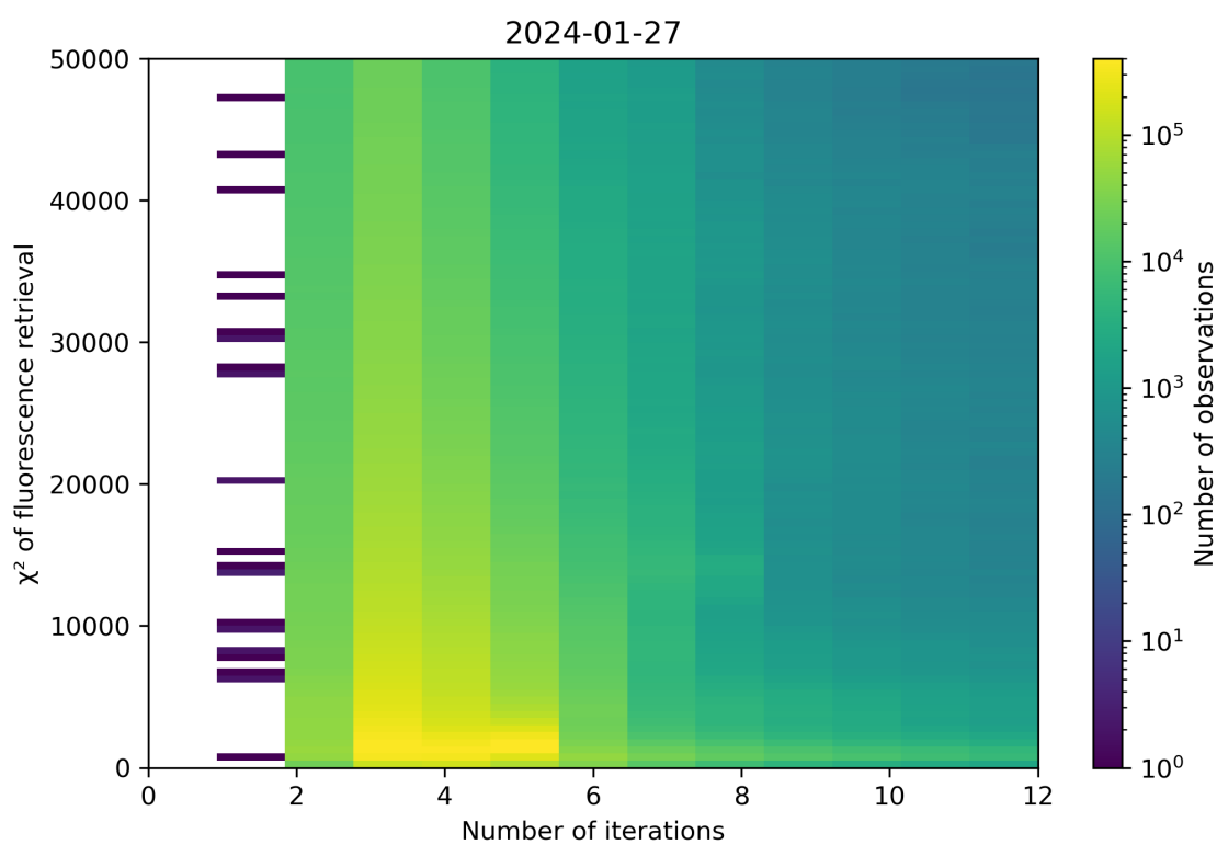
Figure 97: Scatter density plot of “Number of iterations” against “ \chi^2 of fluorescence retrieval” for 2024-01-26 to 2024-01-28.
