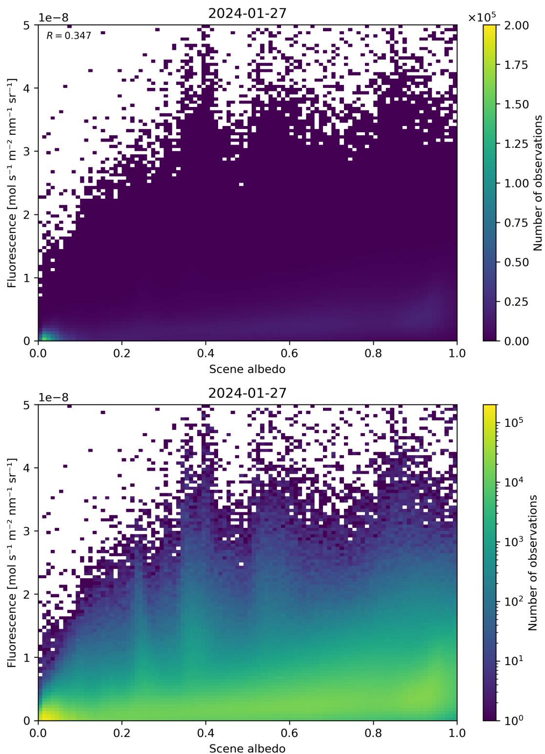
Figure 104: Scatter density plot of “Scene albedo” against “Fluorescence” for 2024-01-26 to 2024-01-28.
