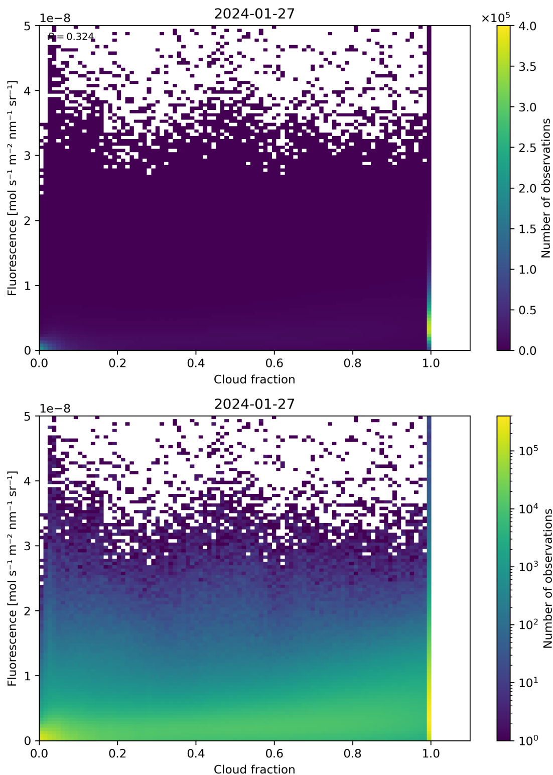
Figure 72: Scatter density plot of “Cloud fraction” against “Fluorescence” for 2024-01-26 to 2024-01-28.
