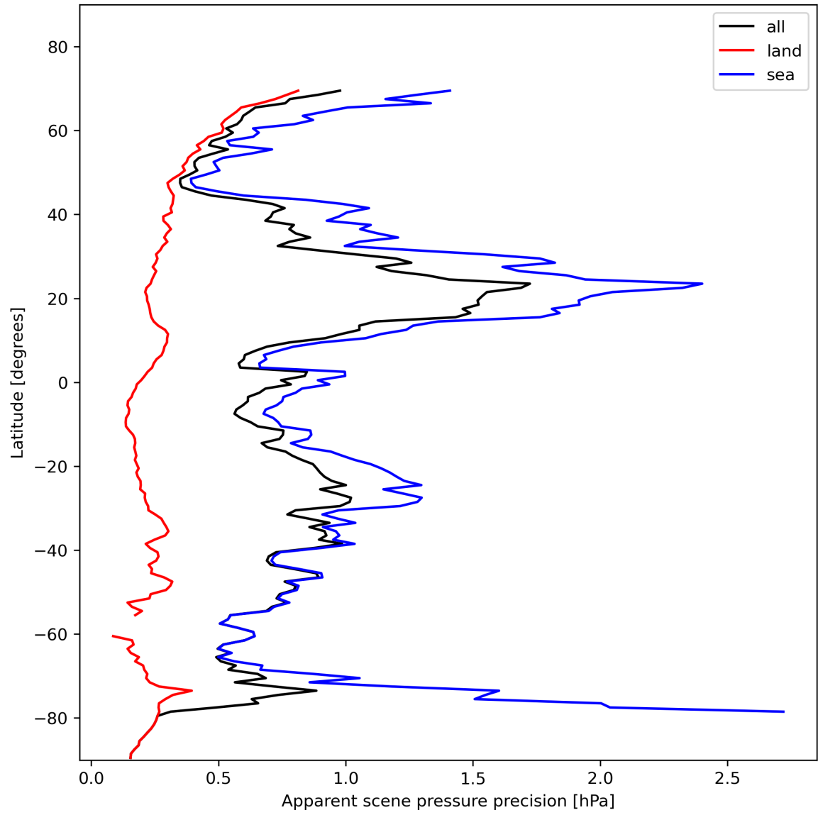
Figure 20: Zonal average of “Apparent scene pressure precision” for 2024-01-26 to 2024-01-28.
