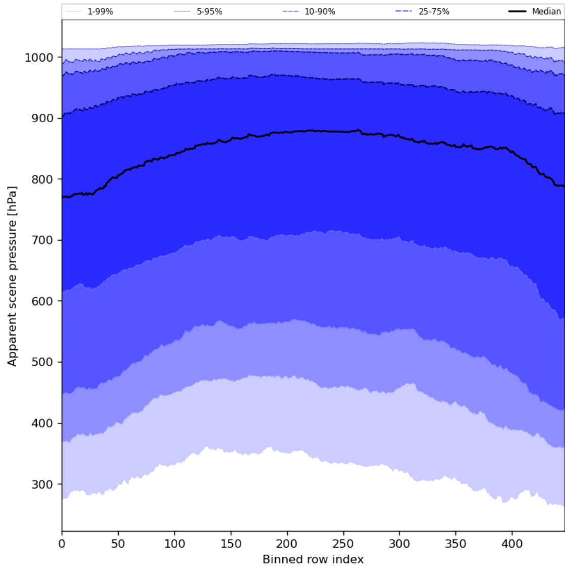
Figure 53: Along track statistics of “Apparent scene pressure” for 2024-01-26 to 2024-01-28
