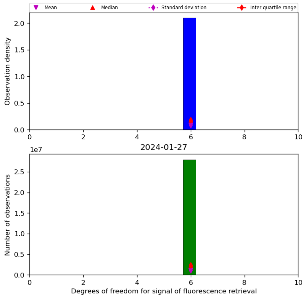
Figure 43: Histogram of “Degrees of freedom for signal of fluorescence retrieval” for 2024-01-26 to 2024-01-28
