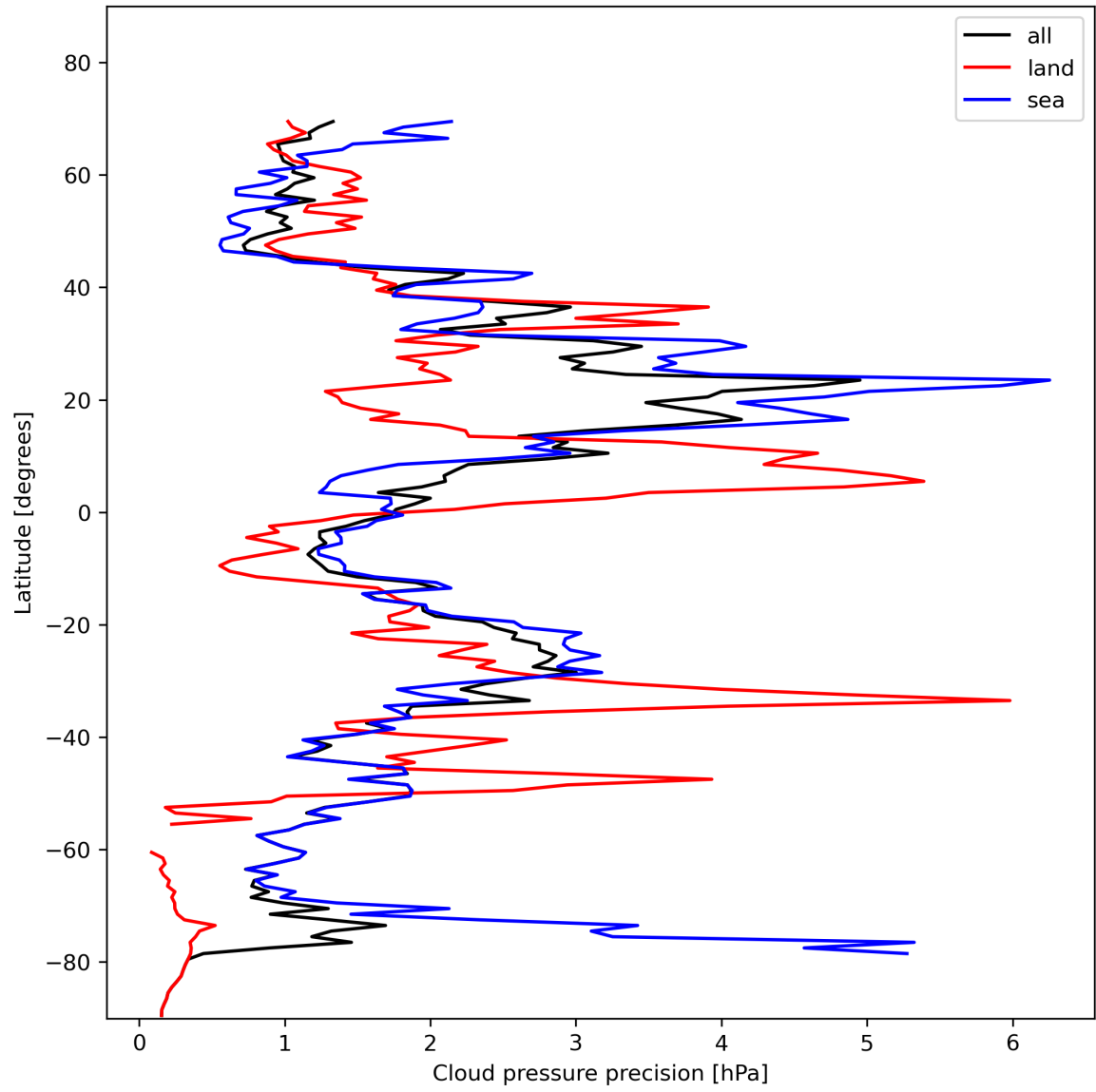
Figure 14: Zonal average of “Cloud pressure precision” for 2024-01-26 to 2024-01-28.
