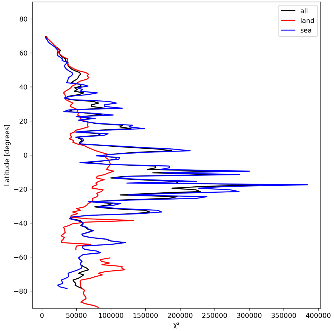
Figure 21: Zonal average of “ \chi^2 ” for 2024-01-26 to 2024-01-28.
