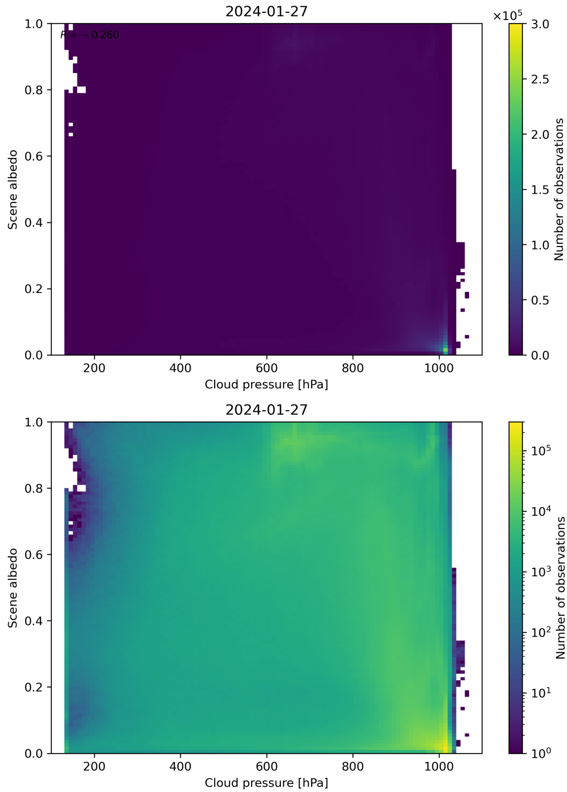
Figure 83: Scatter density plot of “Cloud pressure” against “Scene albedo” for 2024-01-26 to 2024-01-28.
