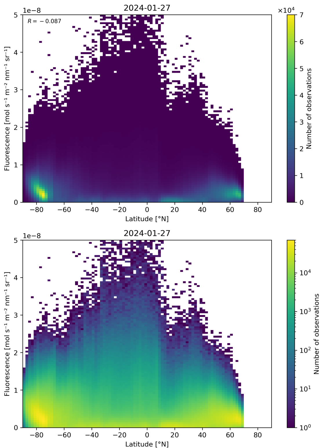
Figure 92: Scatter density plot of “Latitude” against “Fluorescence” for 2024-01-26 to 2024-01-28.
