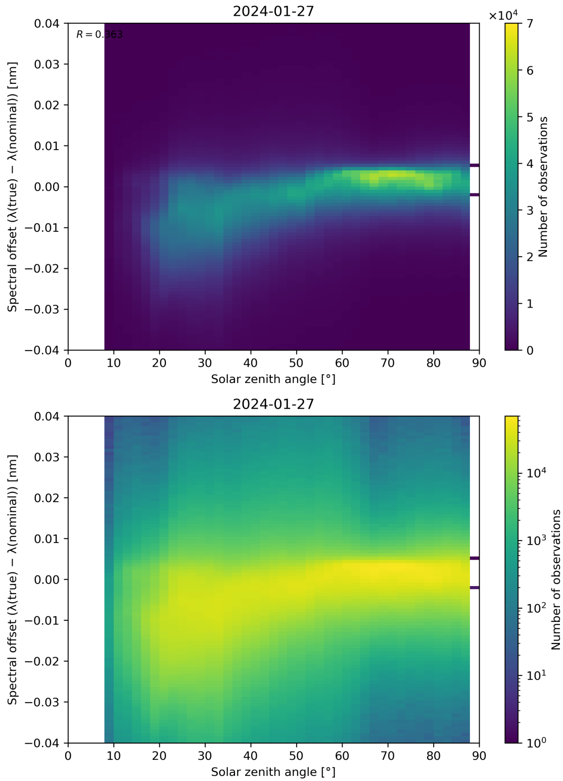
Figure 117: Scatter density plot of “Solar zenith angle” against “Spectral offset ( \lambda(\text{true}) - \lambda(\text{nominal}) )” for 2024-01-26 to 2024-01-28.
