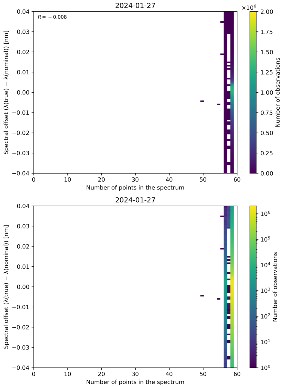
Figure 101: Scatter density plot of “Number of points in the spectrum” against “Spectral offset ( \lambda(\text{true}) - \lambda(\text{nominal}) )” for 2024-01-26 to 2024-01-28.
