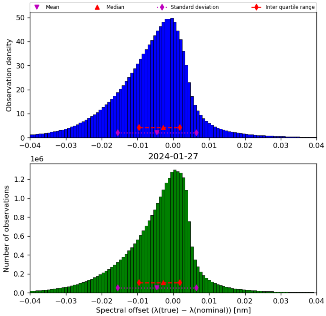
Figure 45: Histogram of “Spectral offset ( \lambda(\text{true}) - \lambda(\text{nominal}) )” for 2024-01-26 to 2024-01-28
