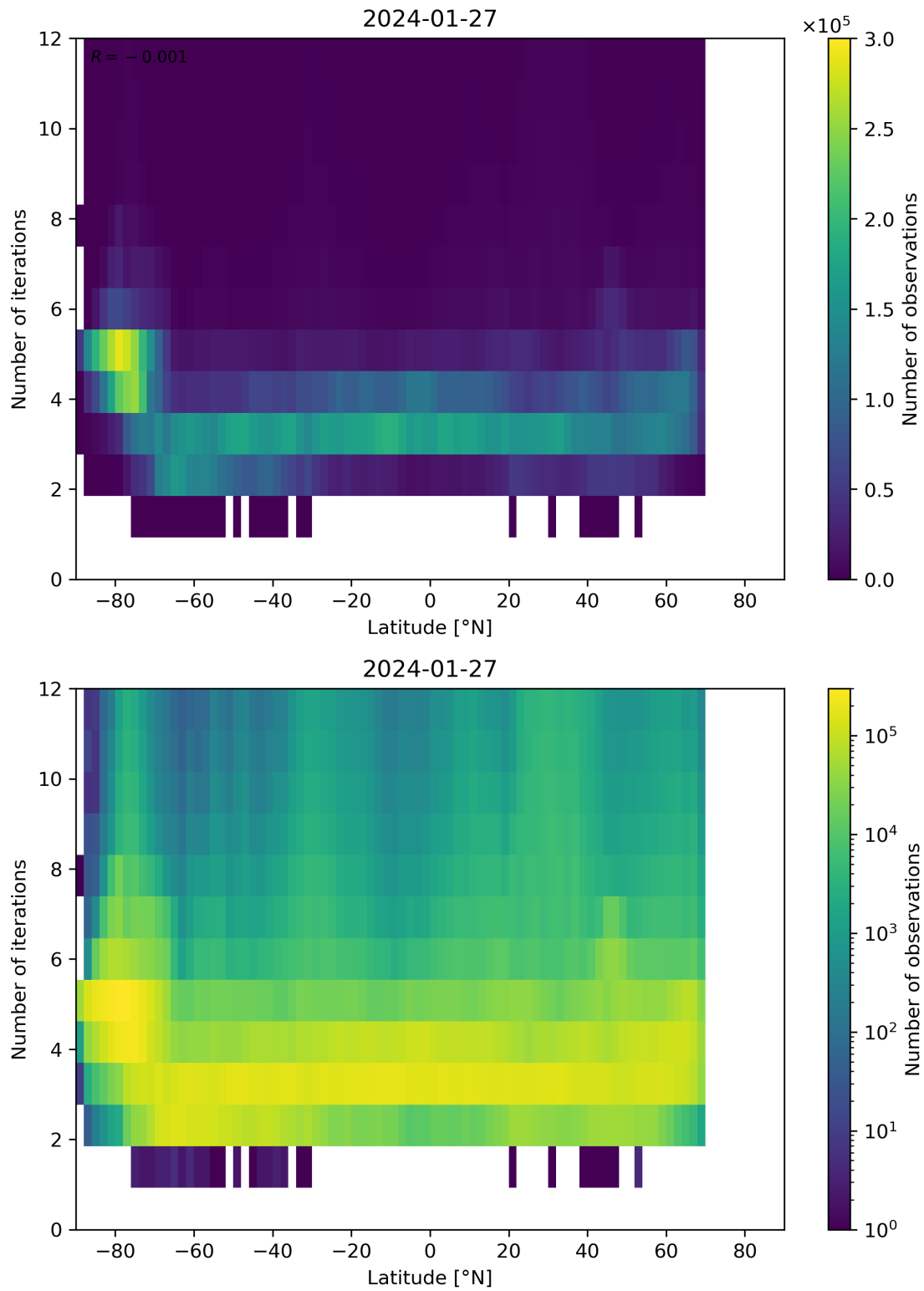
Figure 93: Scatter density plot of “Latitude” against “Number of iterations” for 2024-01-26 to 2024-01-28.
