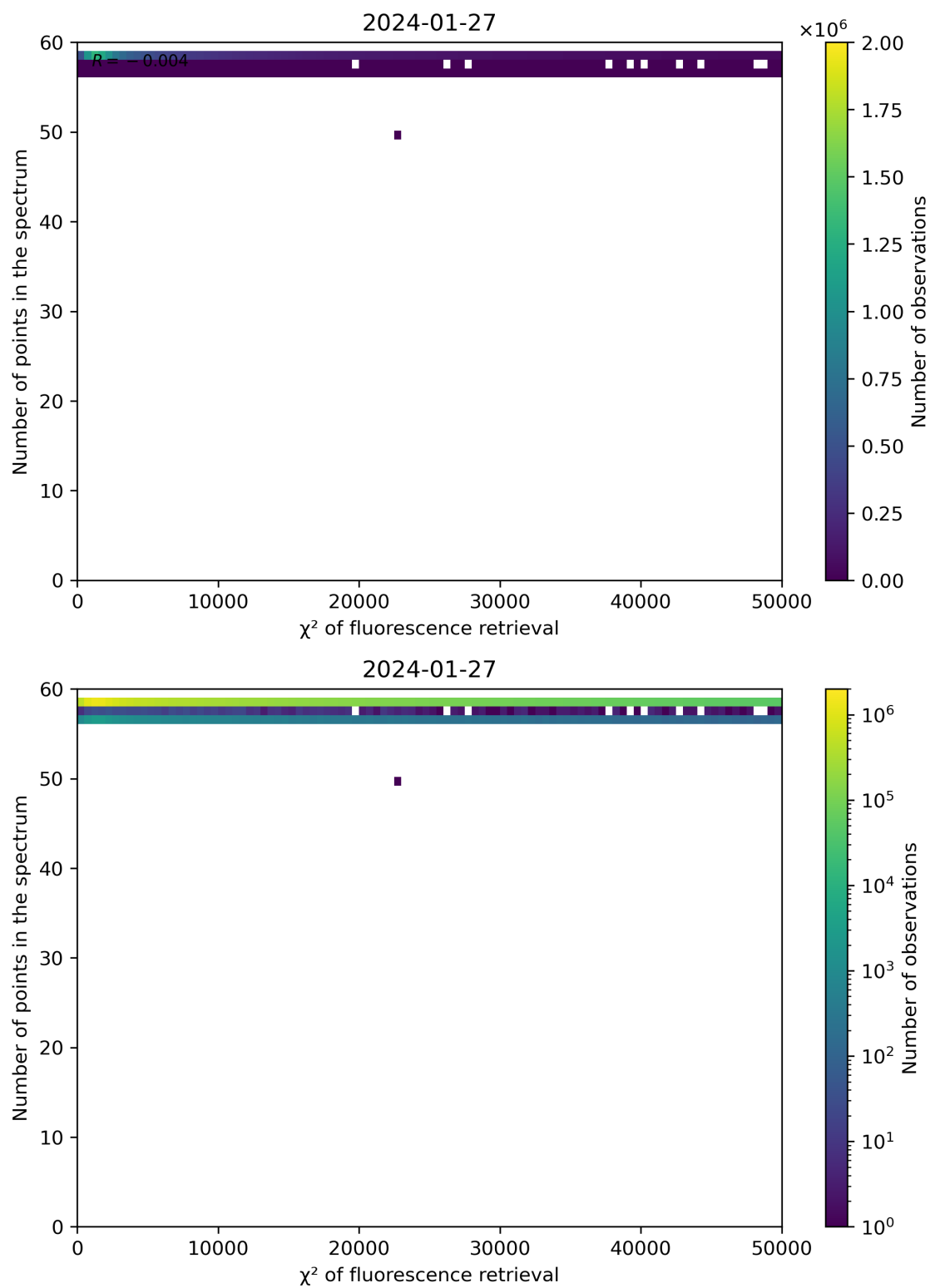
Figure 68: Scatter density plot of " \chi^2 of fluorescence retrieval" against "Number of points in the spectrum" for 2024-01-26 to 2024-01-28.
