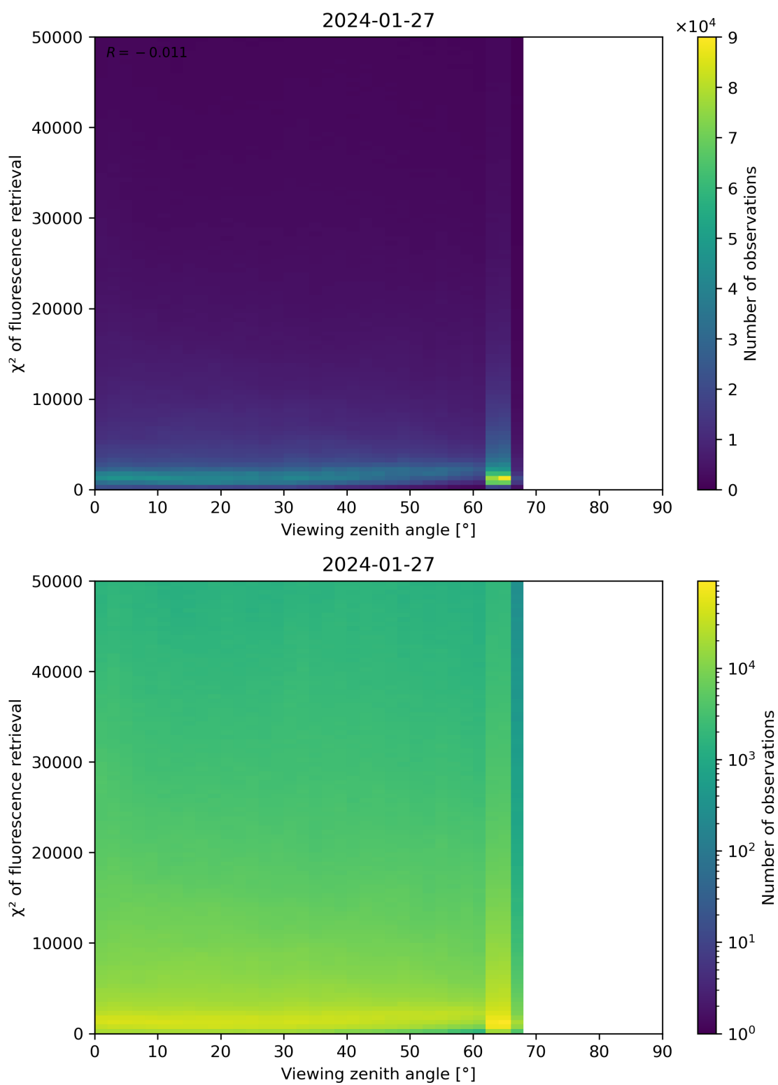
Figure 119: Scatter density plot of “Viewing zenith angle” against “ \chi^2 of fluorescence retrieval” for 2024-01-26 to 2024-01-28.
