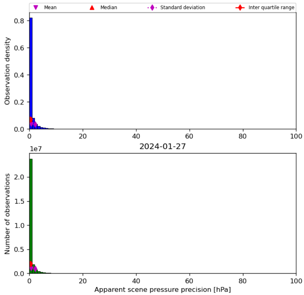
Figure 37: Histogram of “Apparent scene pressure precision” for 2024-01-26 to 2024-01-28
