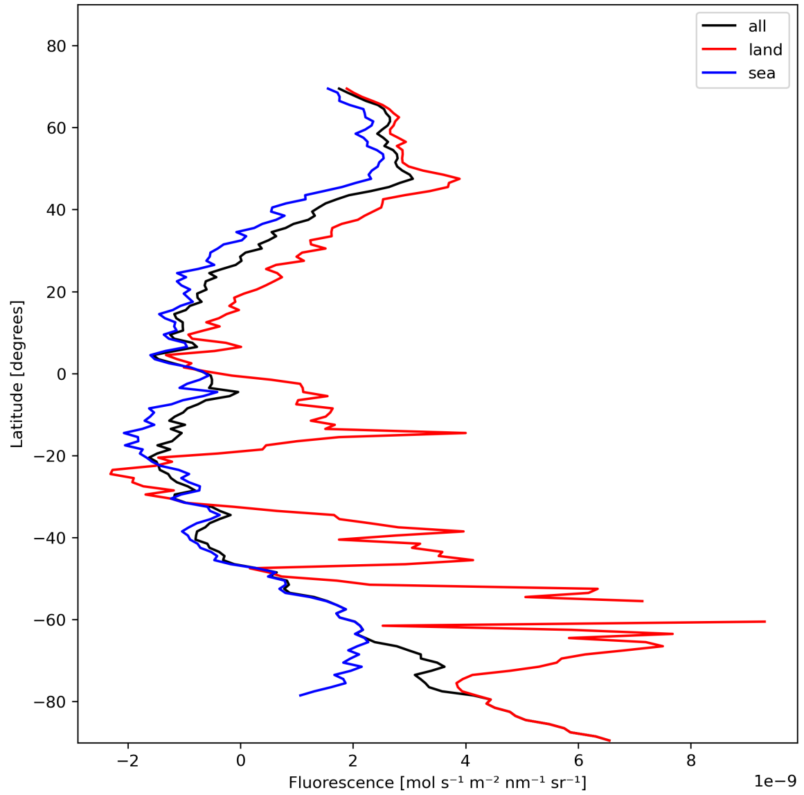
Figure 23: Zonal average of “Fluorescence” for 2024-01-26 to 2024-01-28.
