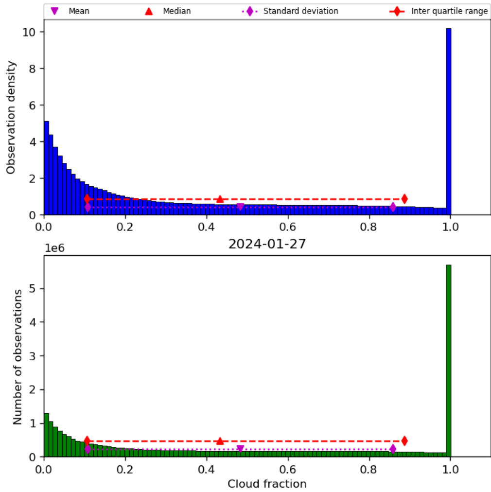
Figure 32: Histogram of “Cloud fraction” for 2024-01-26 to 2024-01-28
