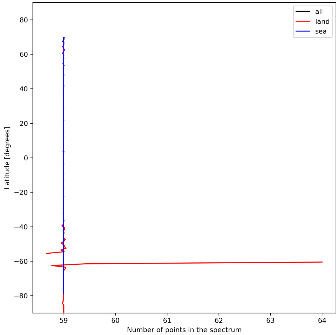
Figure 27: Zonal average of “Number of points in the spectrum” for 2024-01-26 to 2024-01-28.
