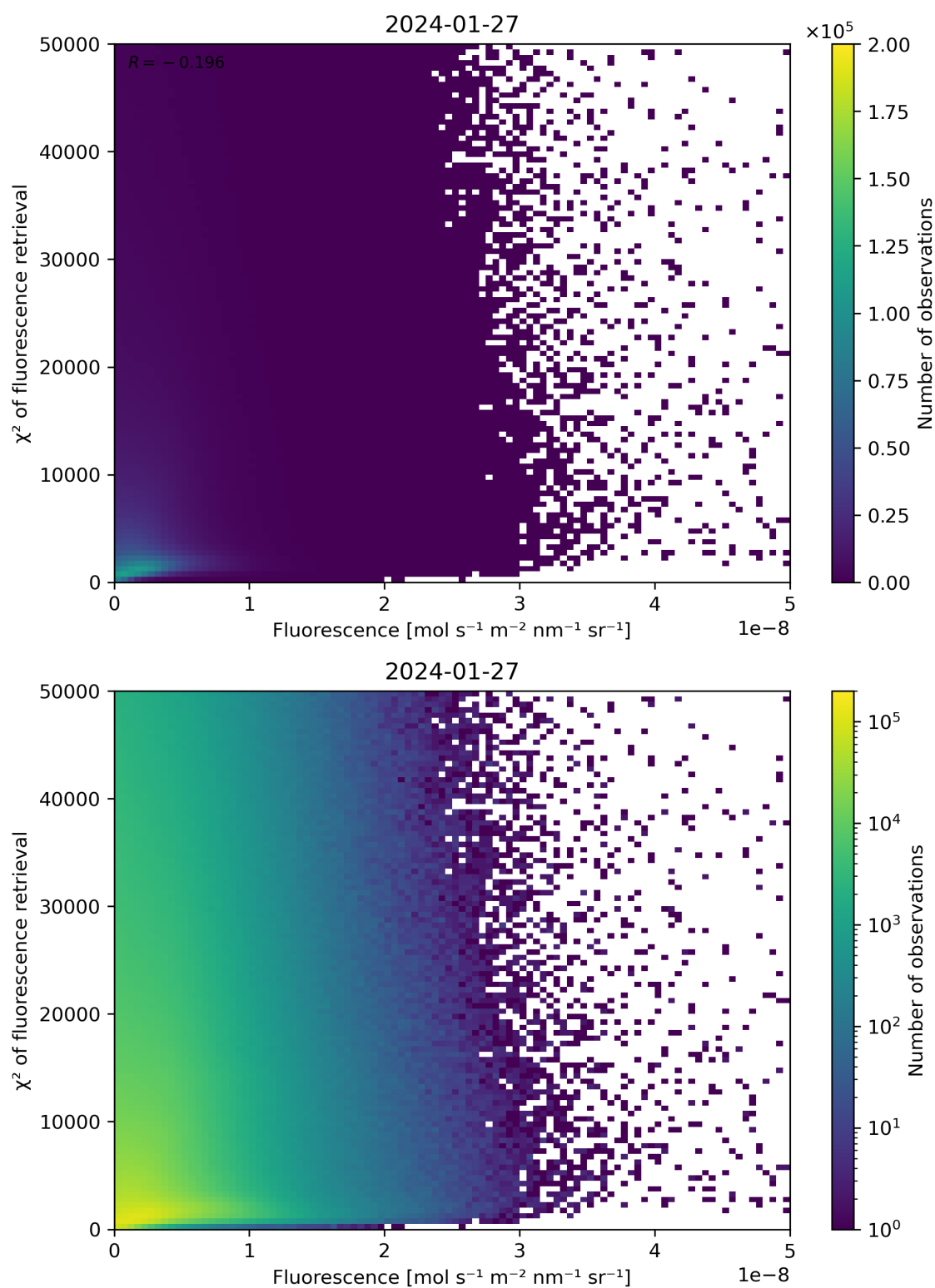
Figure 85: Scatter density plot of “Fluorescence” against “ \chi^2 of fluorescence retrieval” for 2024-01-26 to 2024-01-28.
