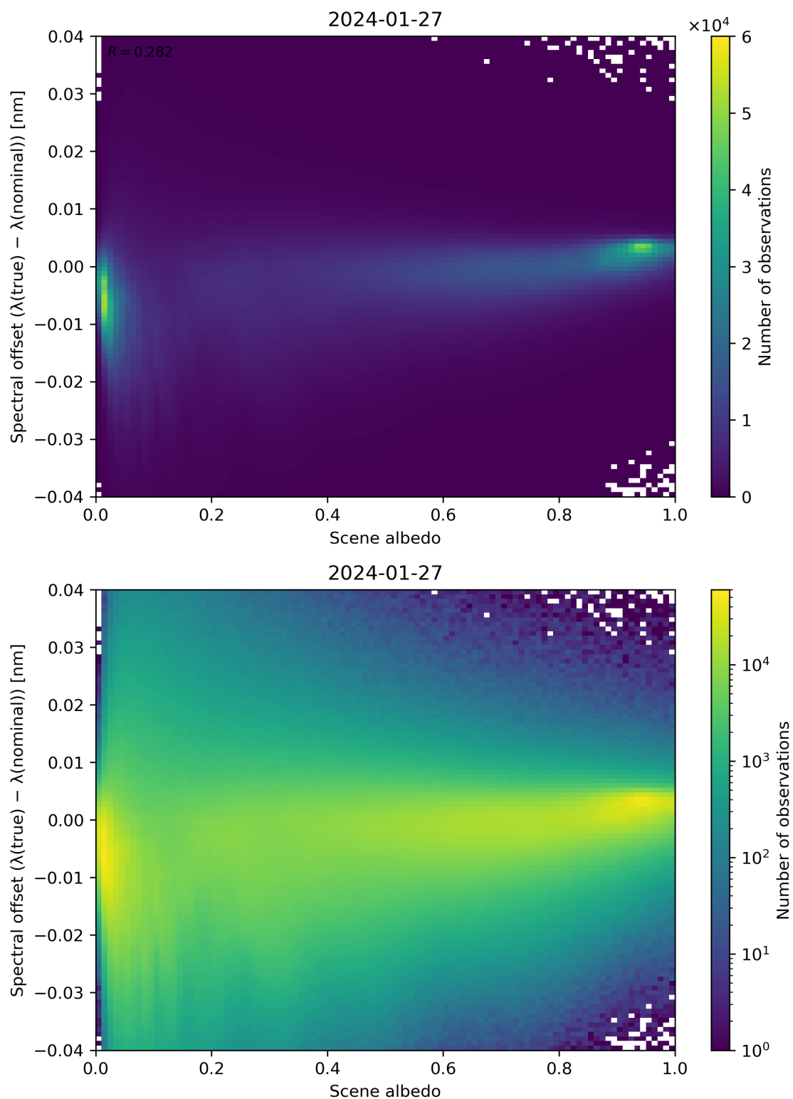
Figure 107: Scatter density plot of “Scene albedo” against “Spectral offset ( \lambda(\text{true}) - \lambda(\text{nominal}) )” for 2024-01-26 to 2024-01-28.
