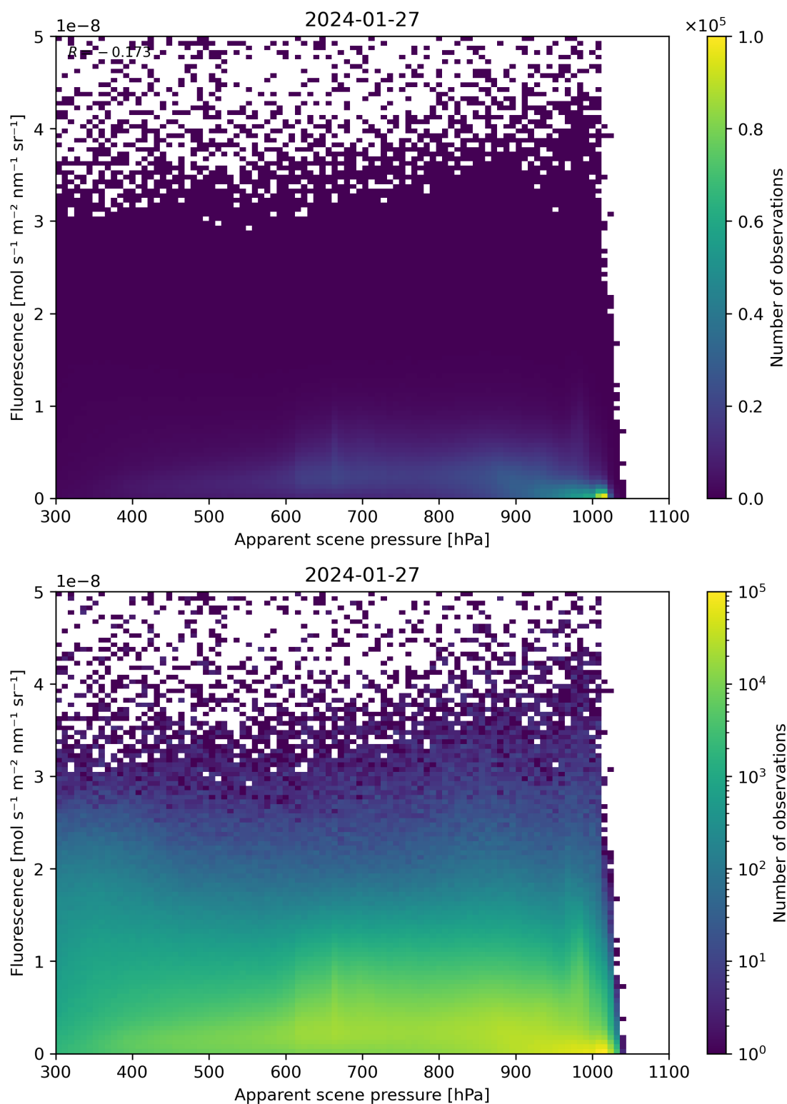
Figure 64: Scatter density plot of “Apparent scene pressure” against “Fluorescence” for 2024-01-26 to 2024-01-28.
