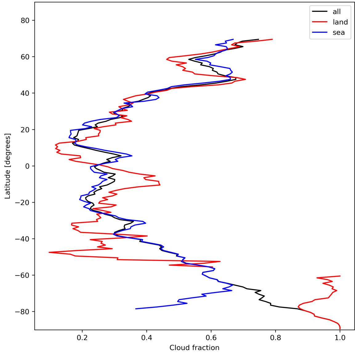
Figure 15: Zonal average of “Cloud fraction” for 2024-01-26 to 2024-01-28.
