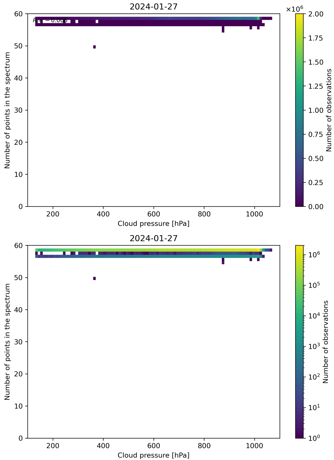
Figure 82: Scatter density plot of “Cloud pressure” against “Number of points in the spectrum” for 2024-01-26 to 2024-01-28.
