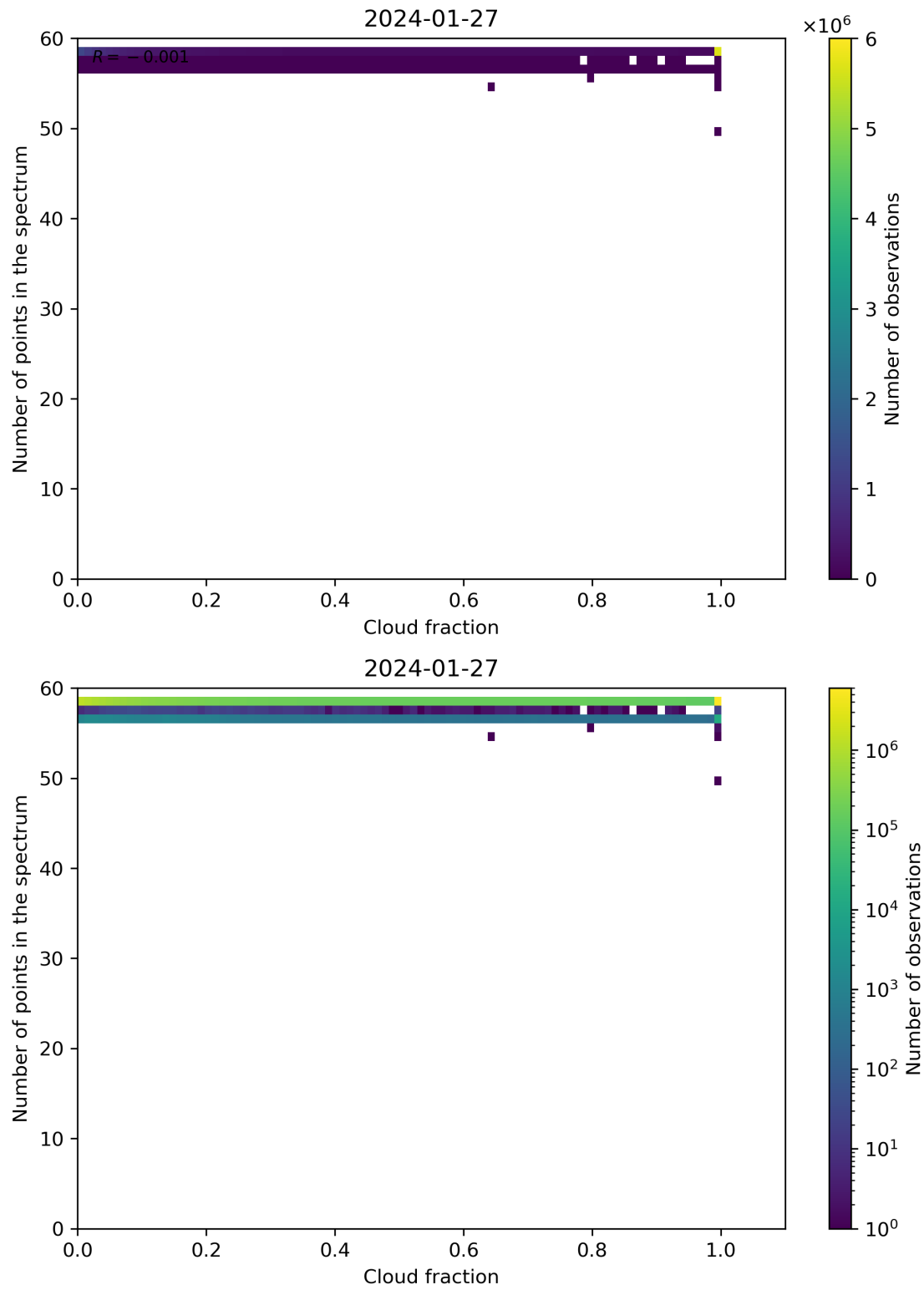
Figure 74: Scatter density plot of “Cloud fraction” against “Number of points in the spectrum” for 2024-01-26 to 2024-01-28.
