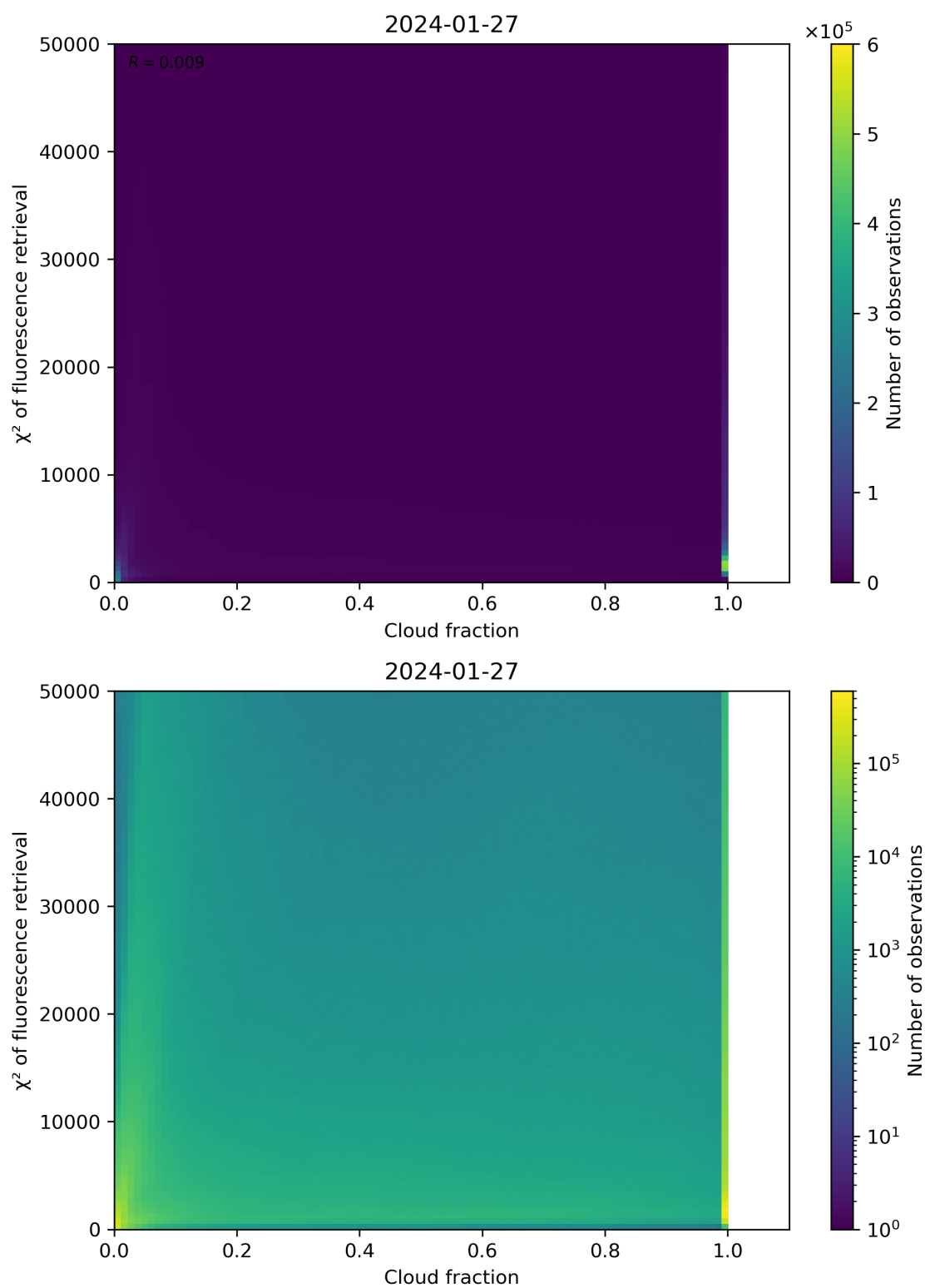
Figure 71: Scatter density plot of “Cloud fraction” against “ \chi^2 of fluorescence retrieval” for 2024-01-26 to 2024-01-28.
