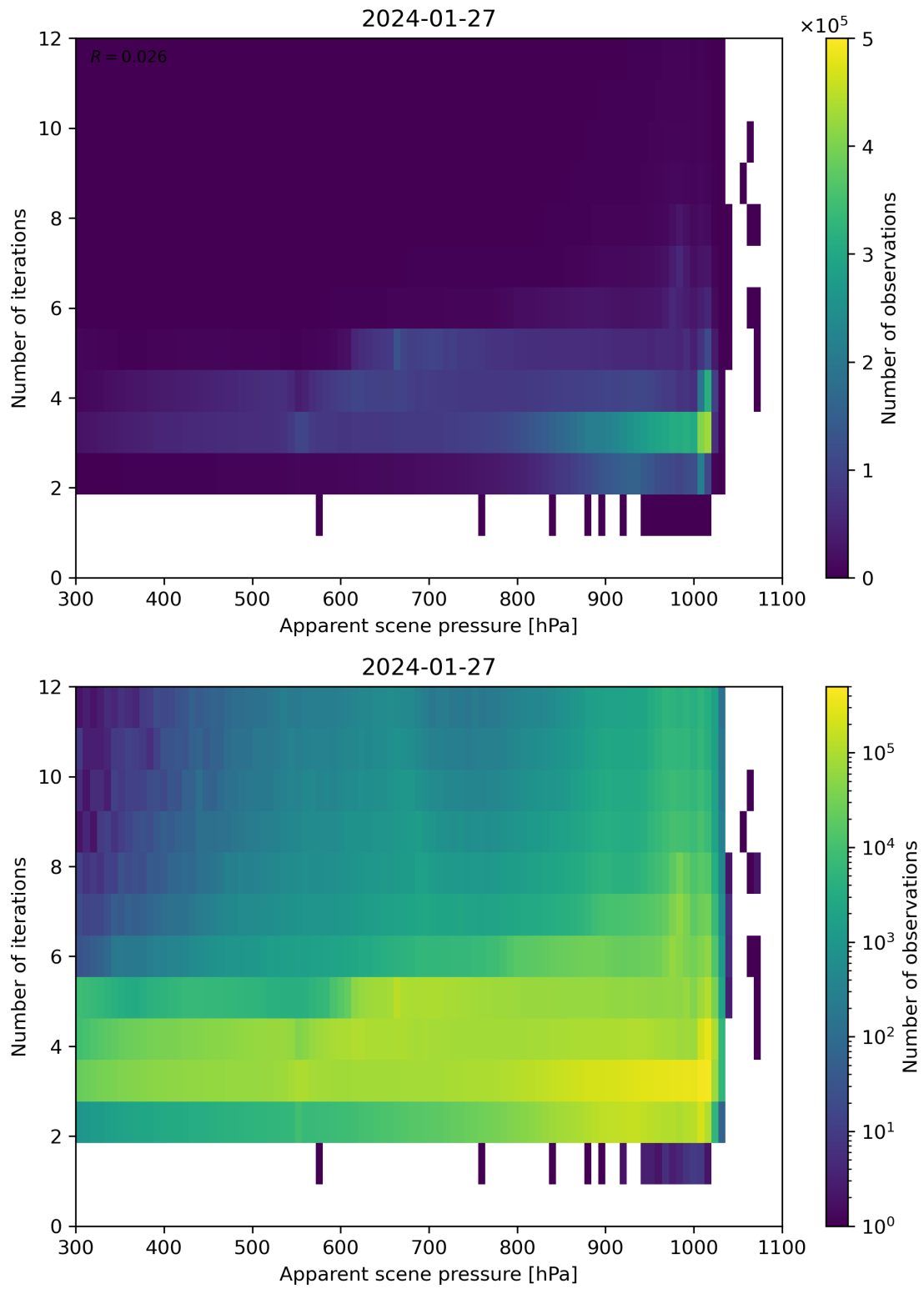
Figure 65: Scatter density plot of “Apparent scene pressure” against “Number of iterations” for 2024-01-26 to 2024-01-28.
