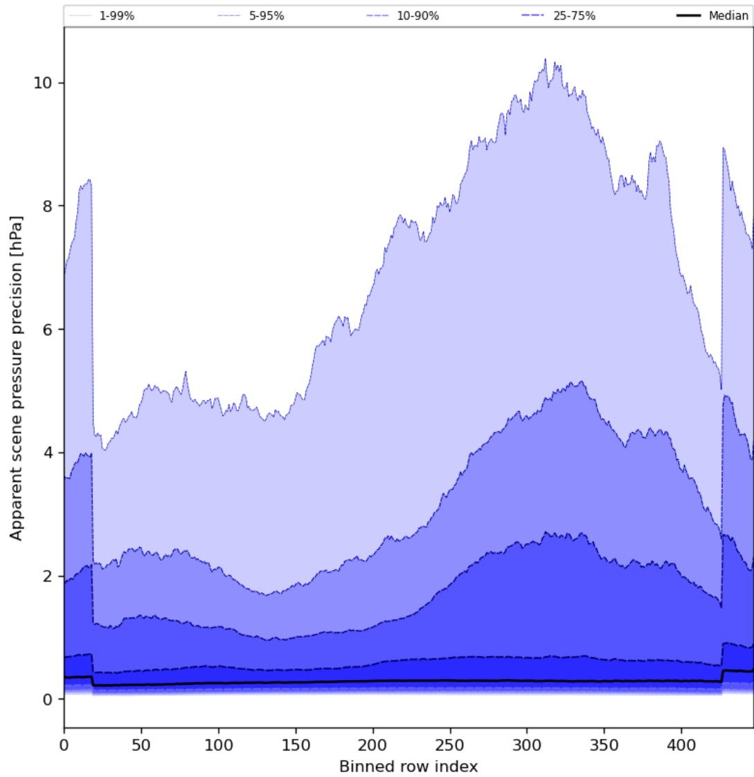
Figure 54: Along track statistics of “Apparent scene pressure precision” for 2024-01-26 to 2024-01-28
