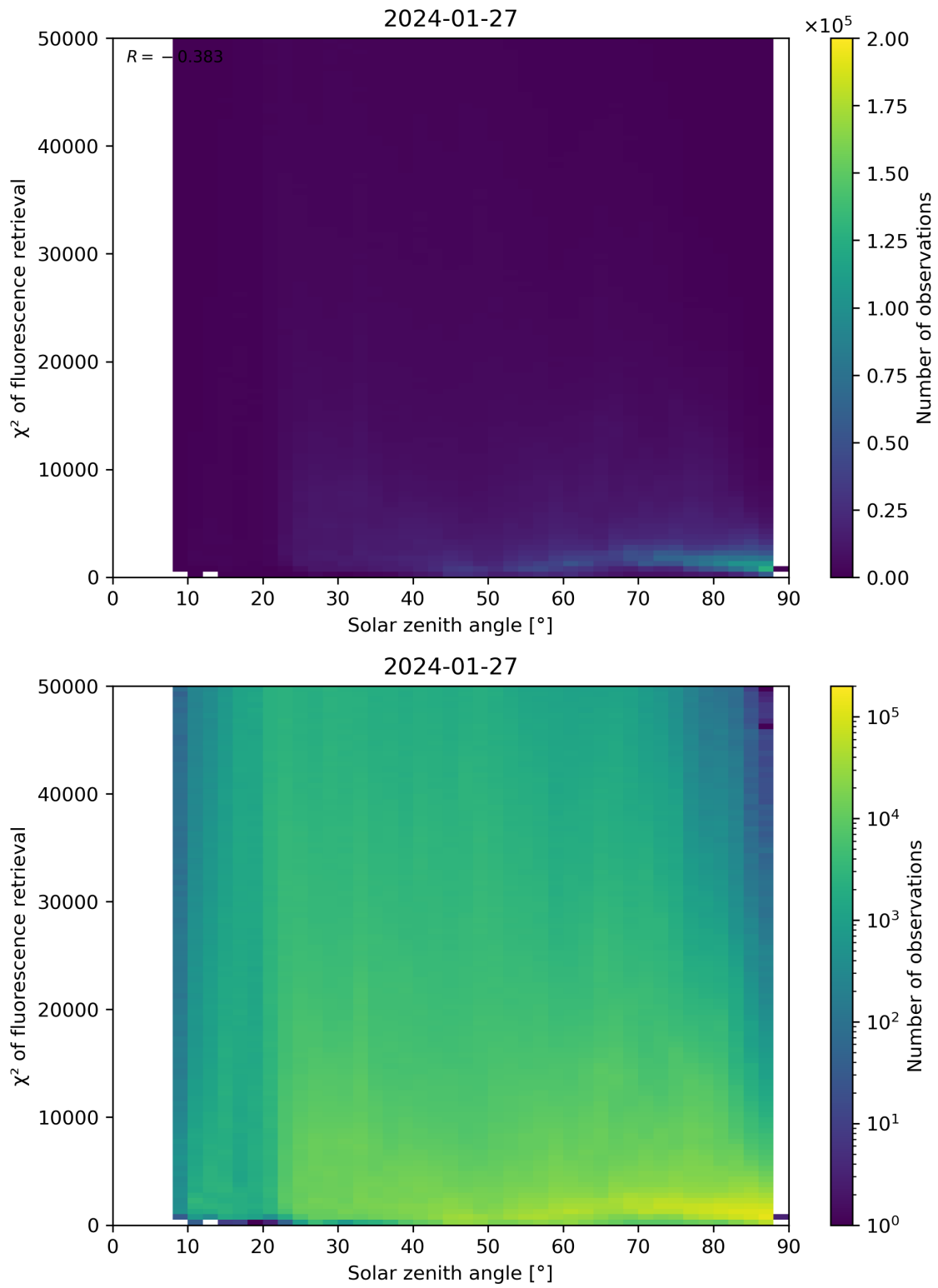
Figure 109: Scatter density plot of “Solar zenith angle” against “ \chi^2 of fluorescence retrieval” for 2024-01-26 to 2024-01-28.
