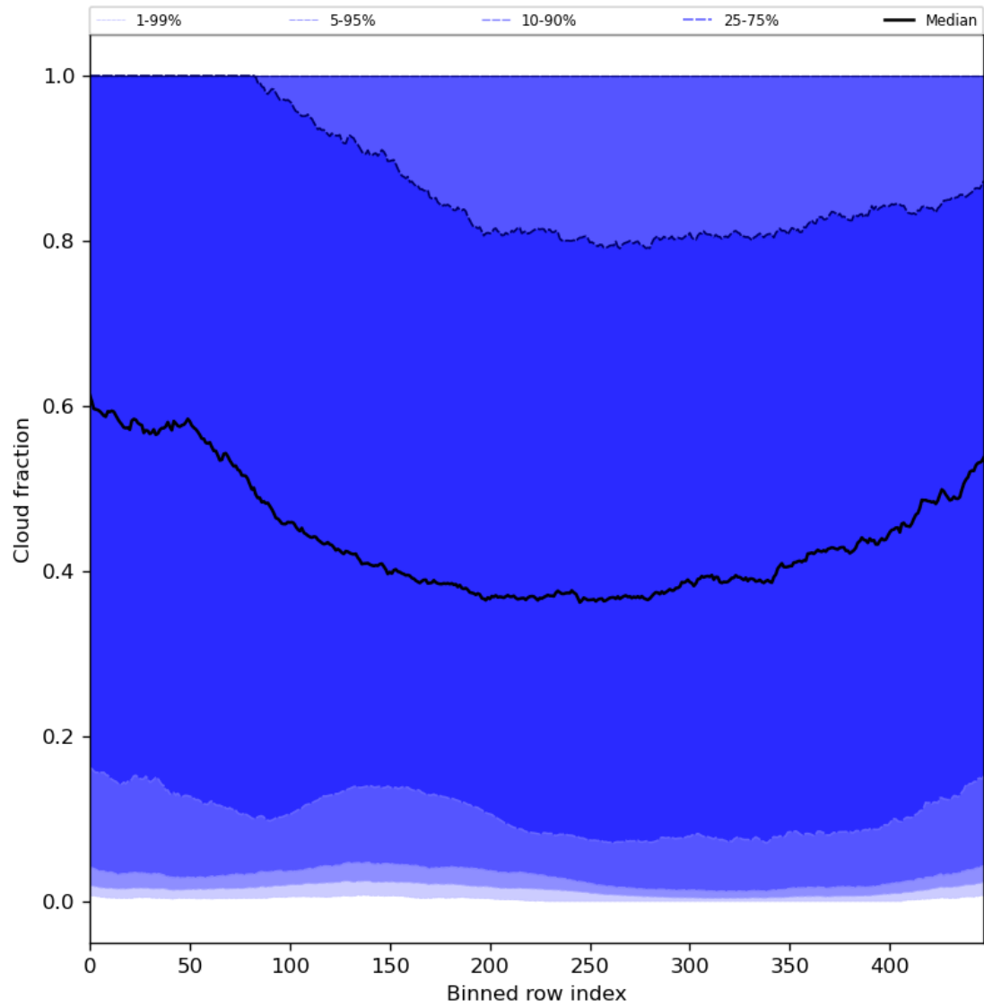
Figure 49: Along track statistics of “Cloud fraction” for 2024-01-26 to 2024-01-28
