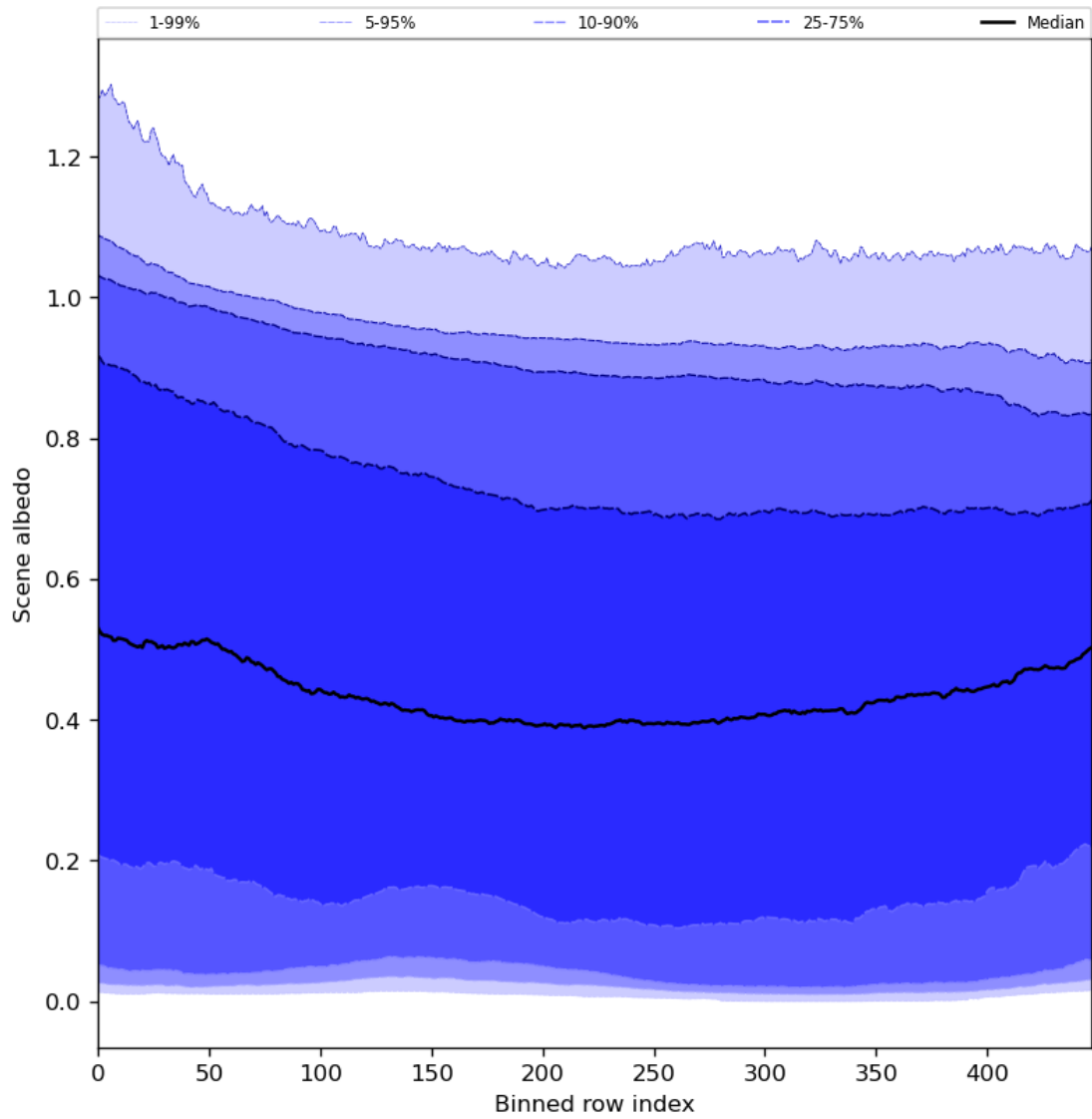
Figure 51: Along track statistics of “Scene albedo” for 2024-01-26 to 2024-01-28
