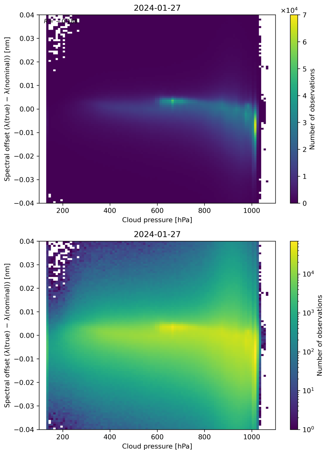
Figure 84: Scatter density plot of “Cloud pressure” against “Spectral offset ( \lambda(\text{true}) - \lambda(\text{nominal}) )” for 2024-01-26 to 2024-01-28.
