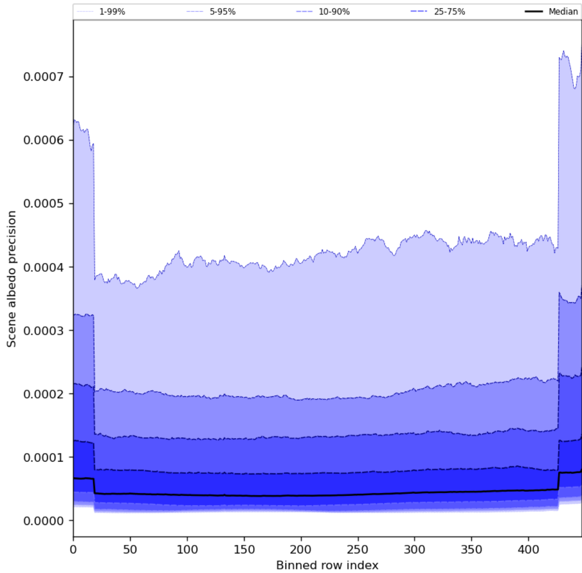
Figure 52: Along track statistics of “Scene albedo precision” for 2024-01-26 to 2024-01-28
