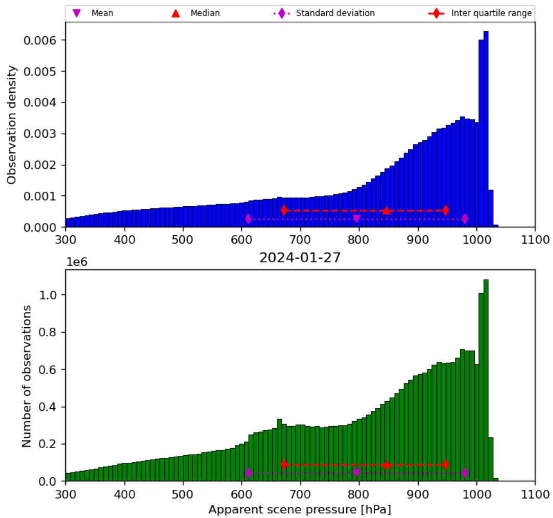
Figure 36: Histogram of “Apparent scene pressure” for 2024-01-26 to 2024-01-28
