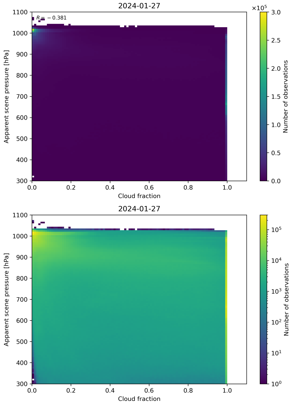
Figure 70: Scatter density plot of “Cloud fraction” against “Apparent scene pressure” for 2024-01-26 to 2024-01-28.
