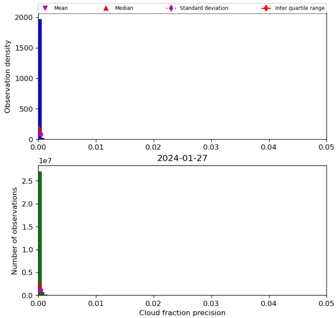
Figure 33: Histogram of “Cloud fraction precision” for 2024-01-26 to 2024-01-28
