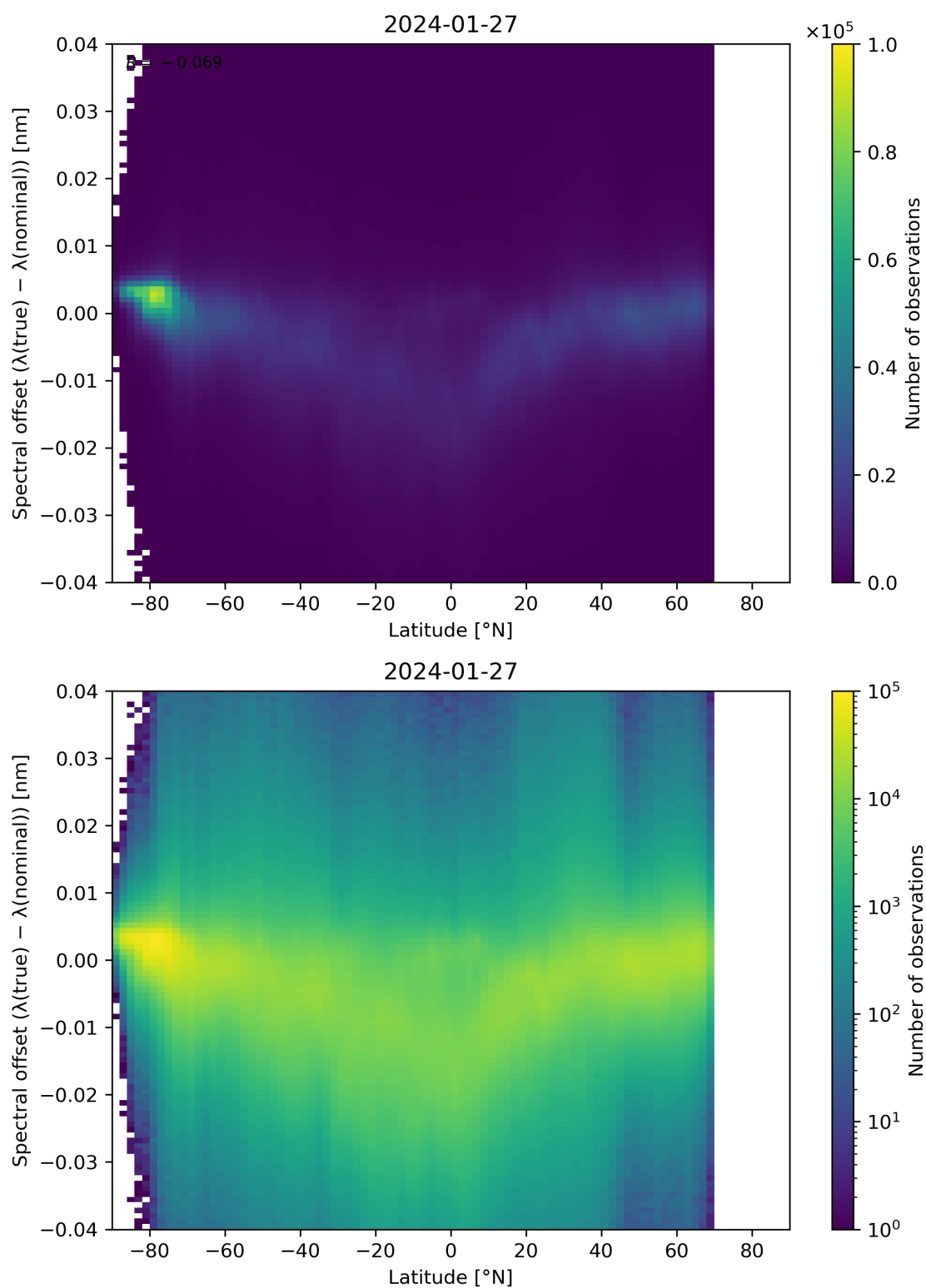
Figure 96: Scatter density plot of “Latitude” against “Spectral offset ( \lambda(\text{true}) - \lambda(\text{nominal}) )” for 2024-01-26 to 2024-01-28.
