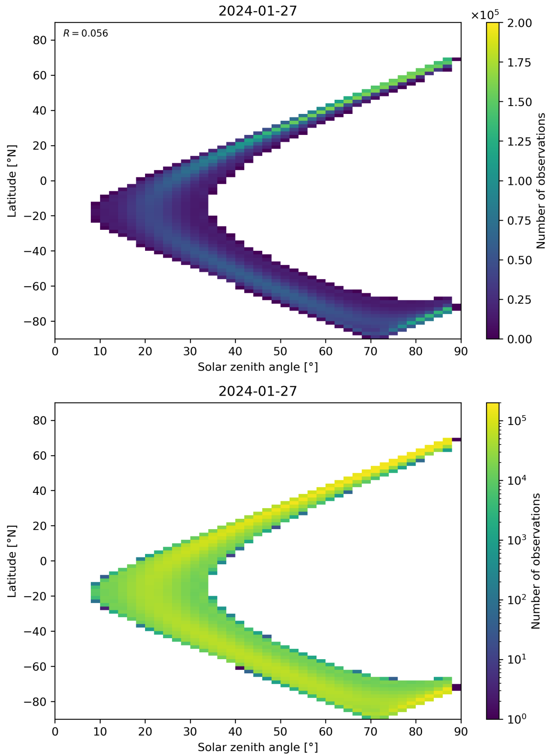
Figure 113: Scatter density plot of “Solar zenith angle” against “Latitude” for 2024-01-26 to 2024-01-28.
