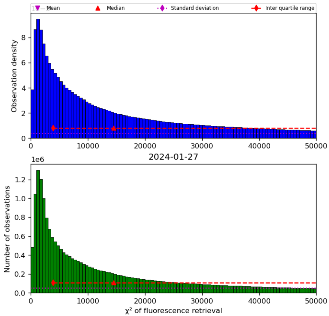
Figure 42: Histogram of “ \chi^2 of fluorescence retrieval” for 2024-01-26 to 2024-01-28
