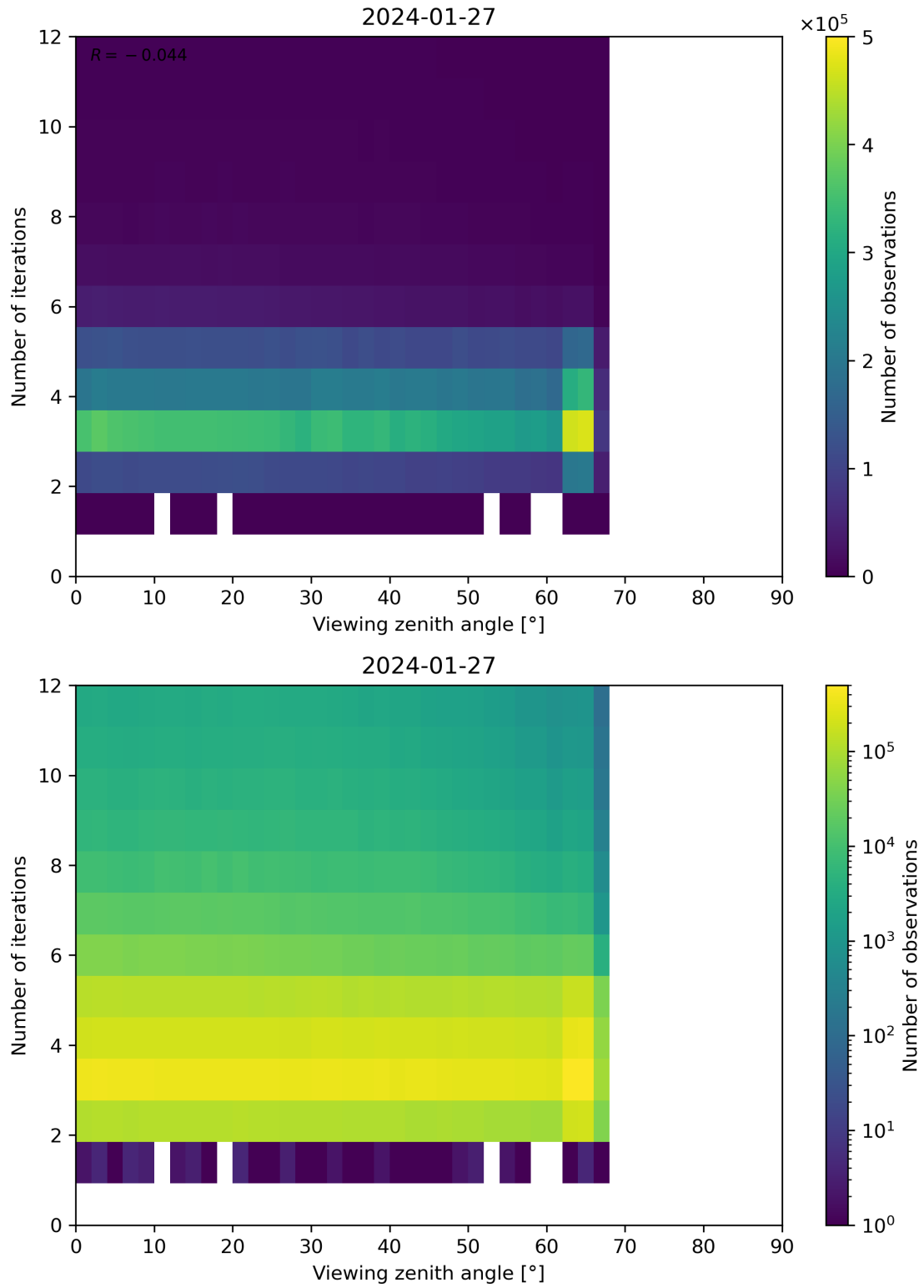
Figure 124: Scatter density plot of “Viewing zenith angle” against “Number of iterations” for 2024-01-26 to 2024-01-28.
