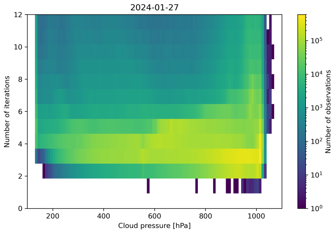
Figure 81: Scatter density plot of “Cloud pressure” against “Number of iterations” for 2024-01-26 to 2024-01-28.
