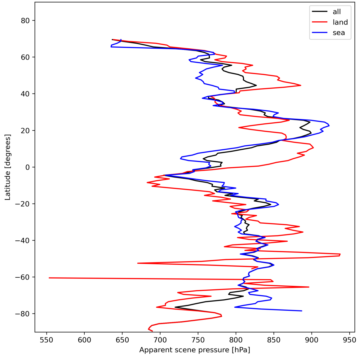
Figure 19: Zonal average of “Apparent scene pressure” for 2024-01-26 to 2024-01-28.
