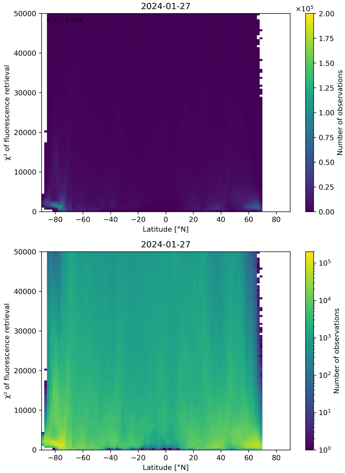
Figure 89: Scatter density plot of “Latitude” against “ \chi^2 of fluorescence retrieval” for 2024-01-26 to 2024-01-28.
