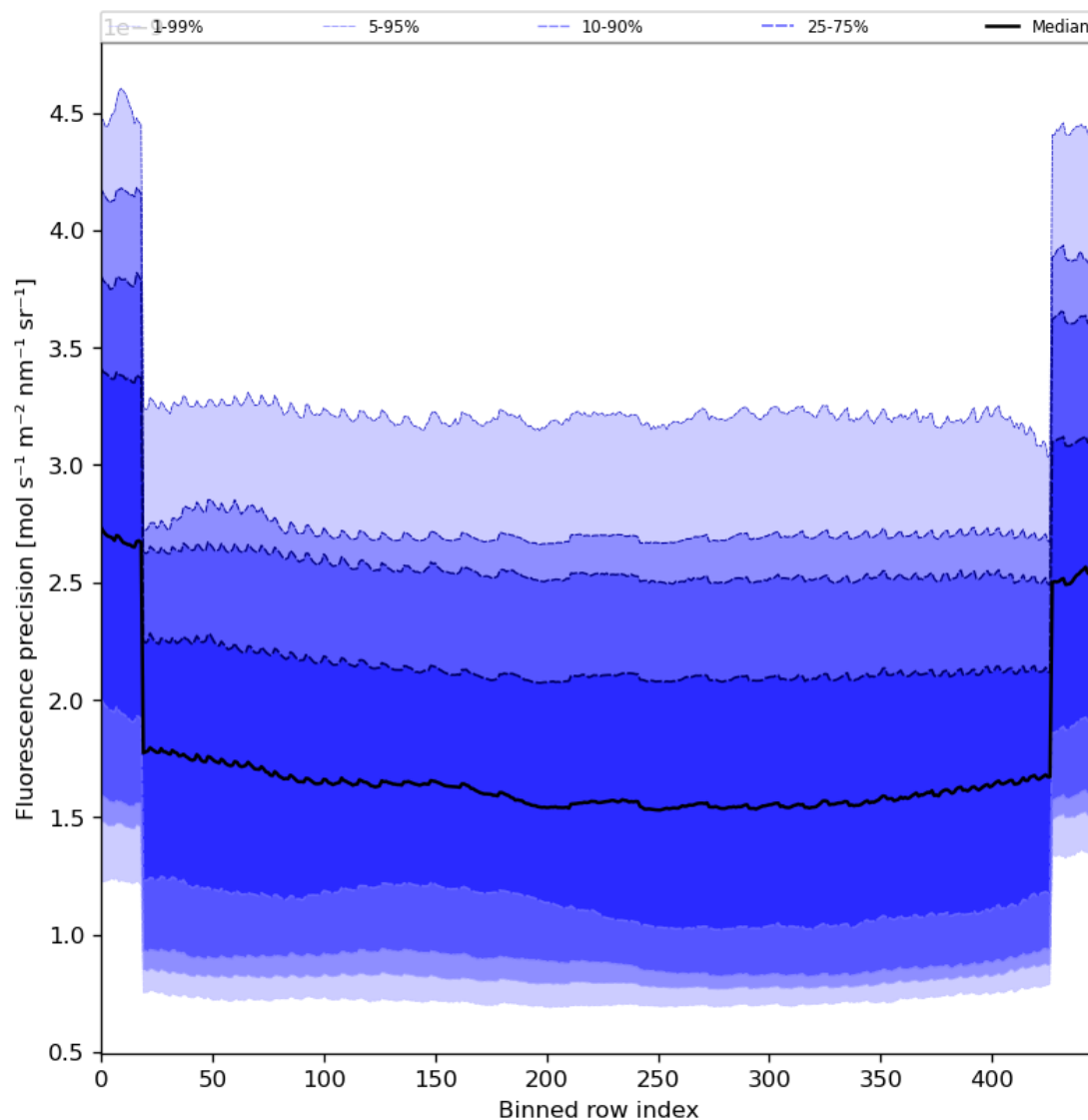
Figure 58: Along track statistics of “Fluorescence precision” for 2024-01-26 to 2024-01-28
