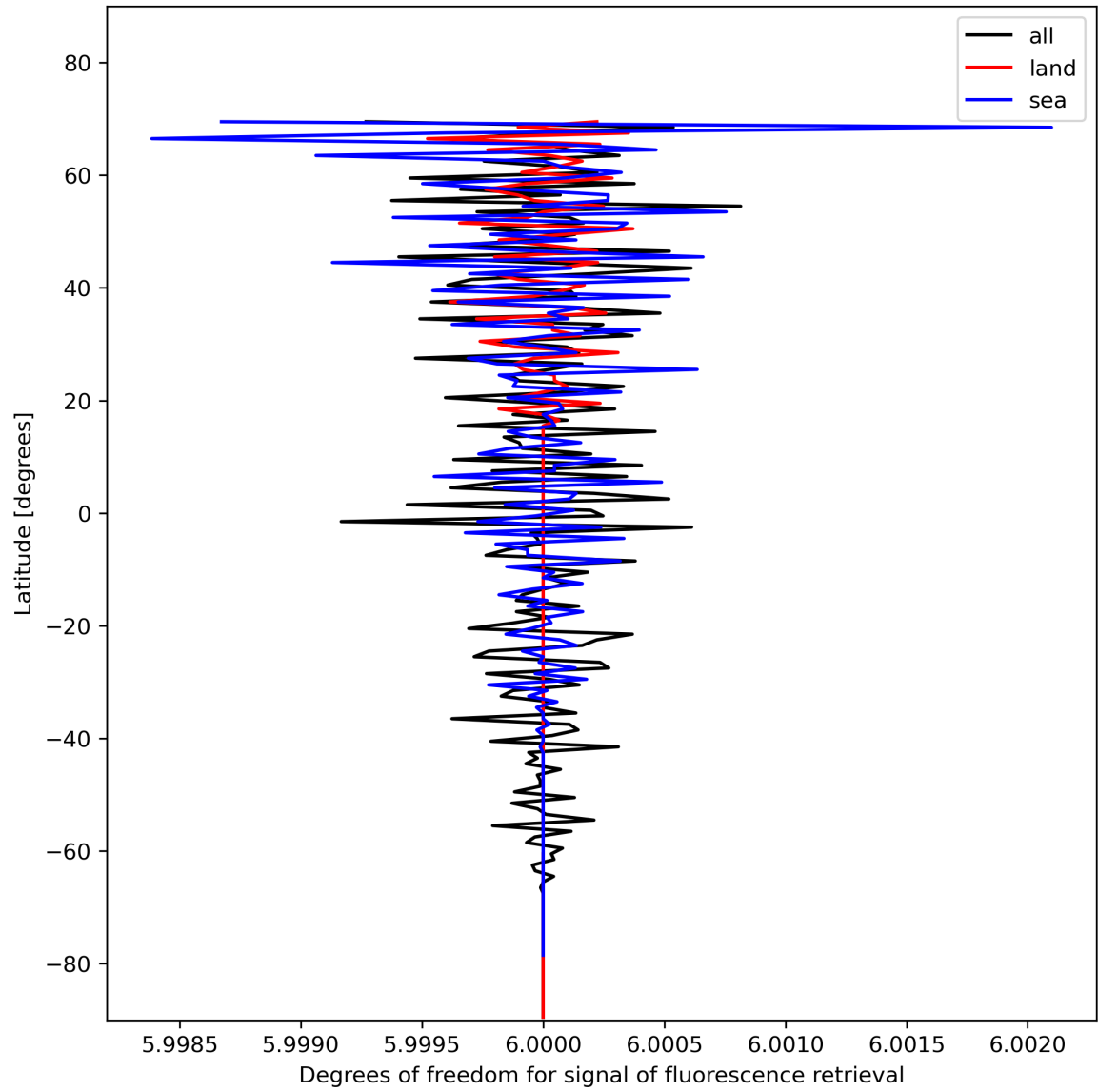
Figure 26: Zonal average of “Degrees of freedom for signal of fluorescence retrieval” for 2024-01-26 to 2024-01-28.
