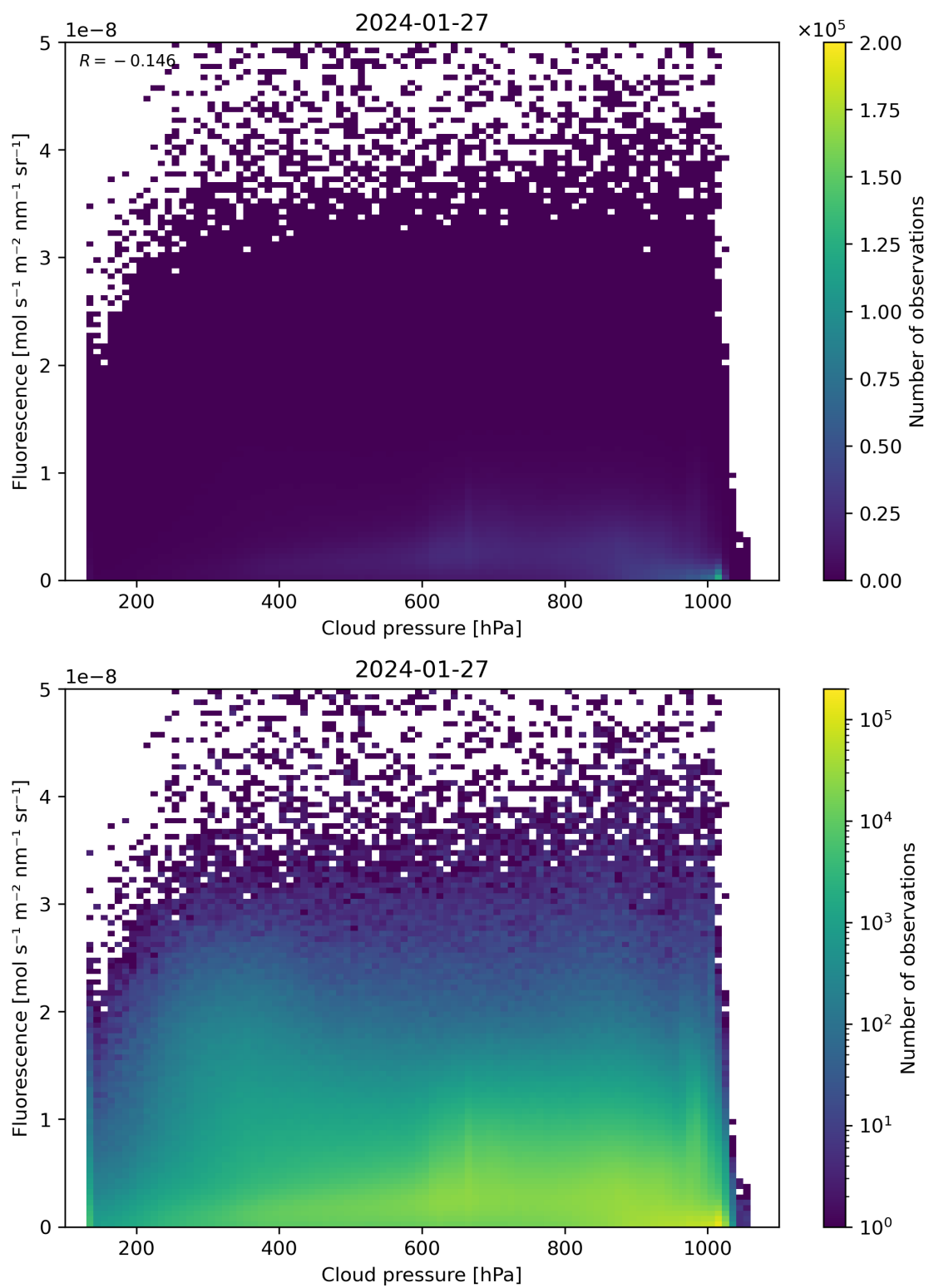
Figure 80: Scatter density plot of “Cloud pressure” against “Fluorescence” for 2024-01-26 to 2024-01-28.
