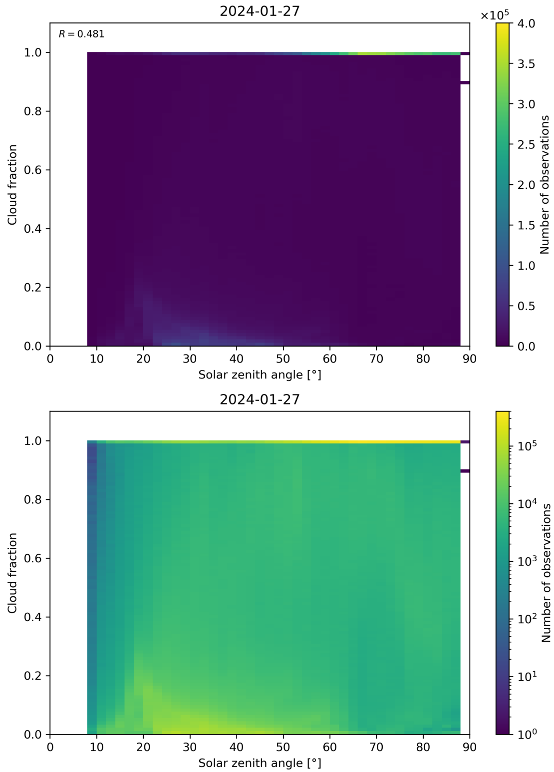
Figure 110: Scatter density plot of “Solar zenith angle” against “Cloud fraction” for 2024-01-26 to 2024-01-28.
