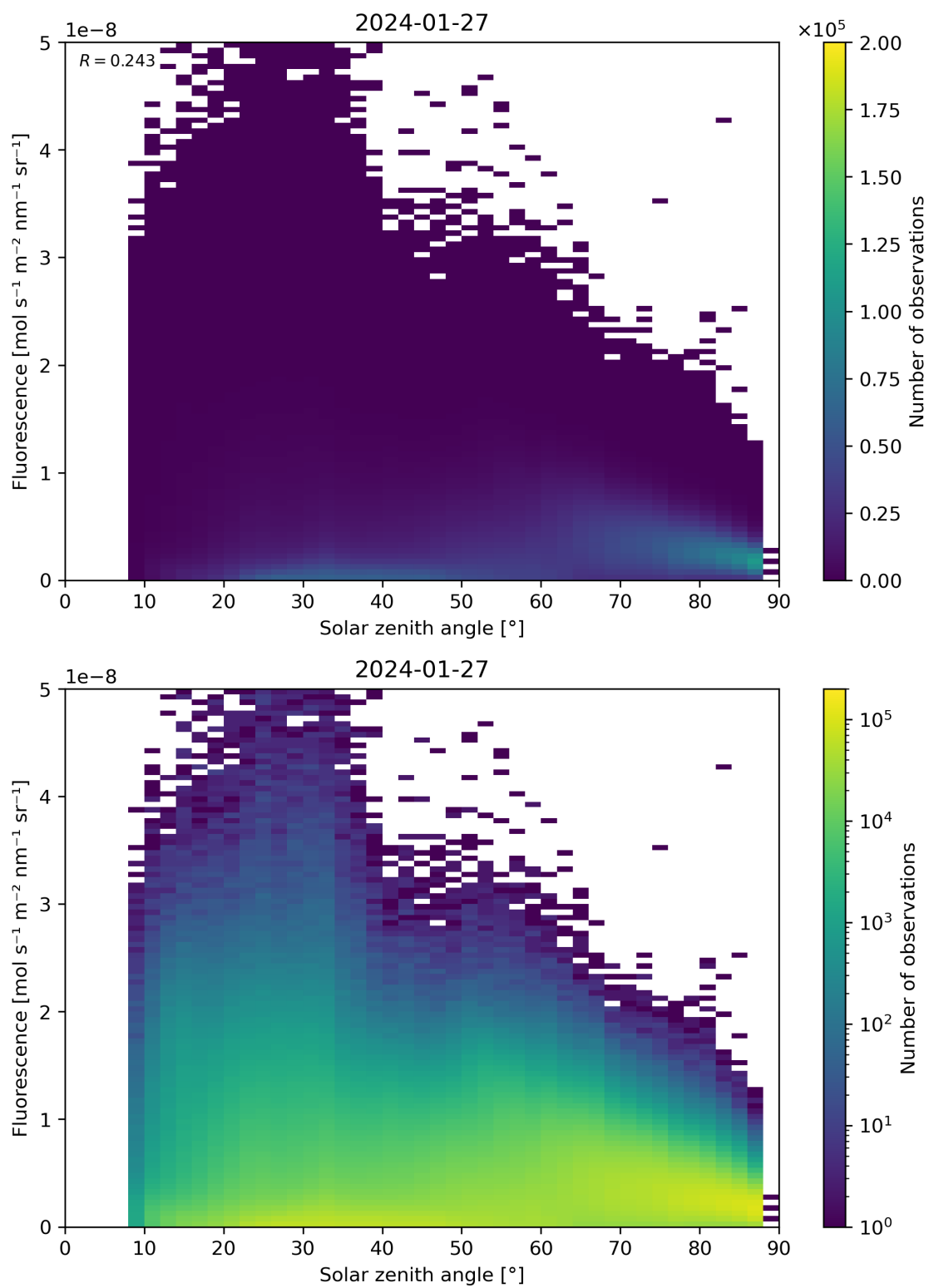
Figure 112: Scatter density plot of “Solar zenith angle” against “Fluorescence” for 2024-01-26 to 2024-01-28.
