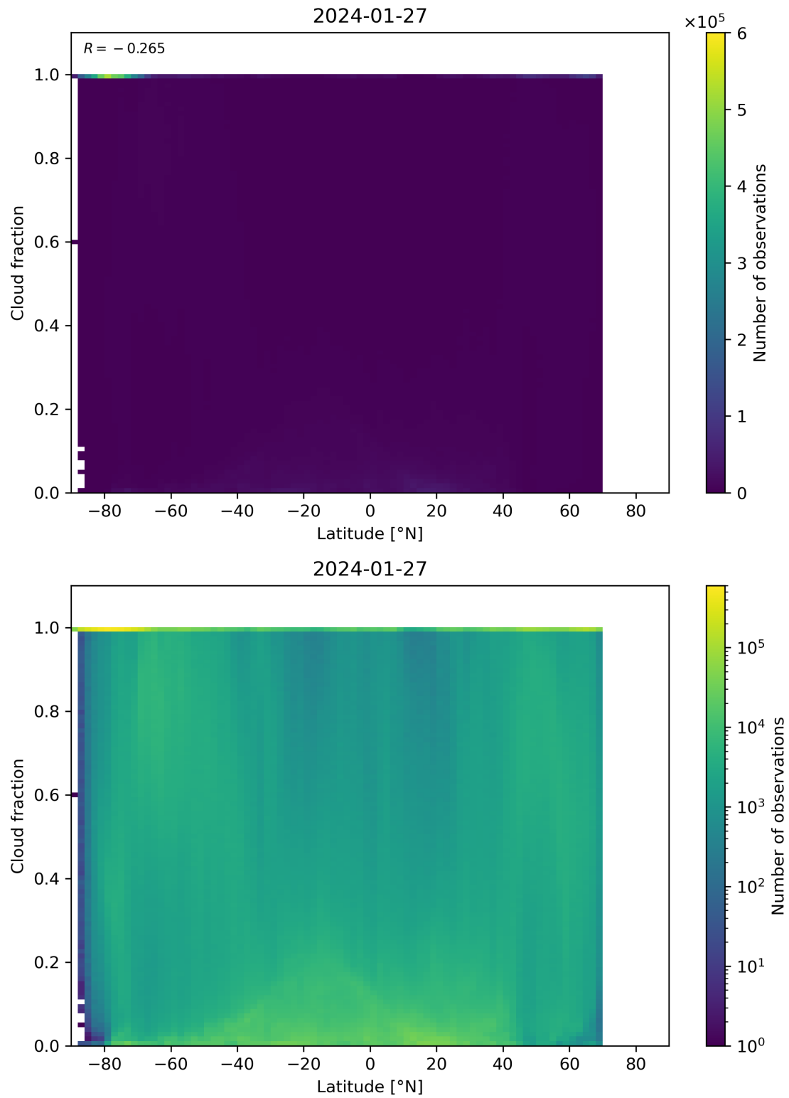
Figure 90: Scatter density plot of “Latitude” against “Cloud fraction” for 2024-01-26 to 2024-01-28.
