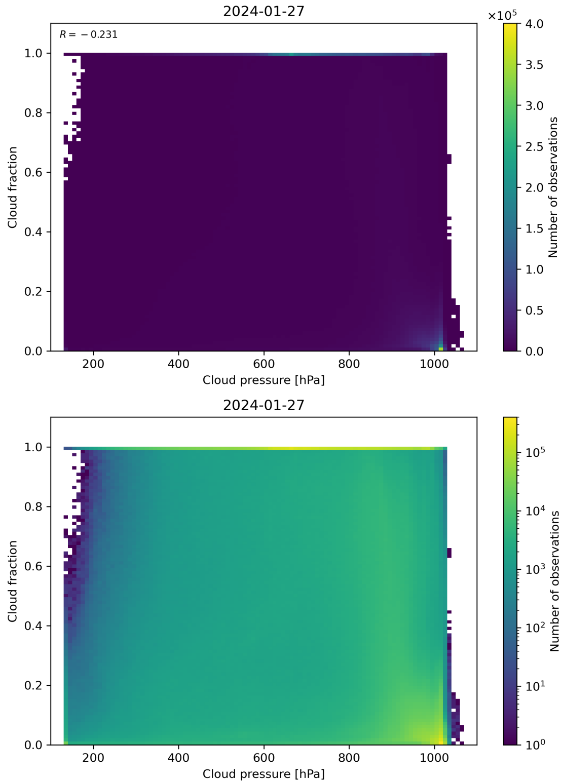
Figure 79: Scatter density plot of “Cloud pressure” against “Cloud fraction” for 2024-01-26 to 2024-01-28.
