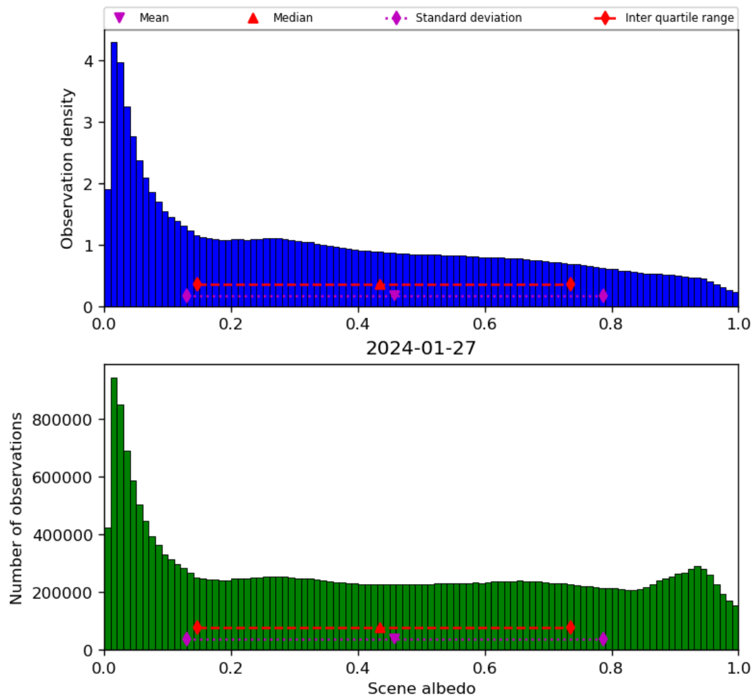
Figure 34: Histogram of “Scene albedo” for 2024-01-26 to 2024-01-28
