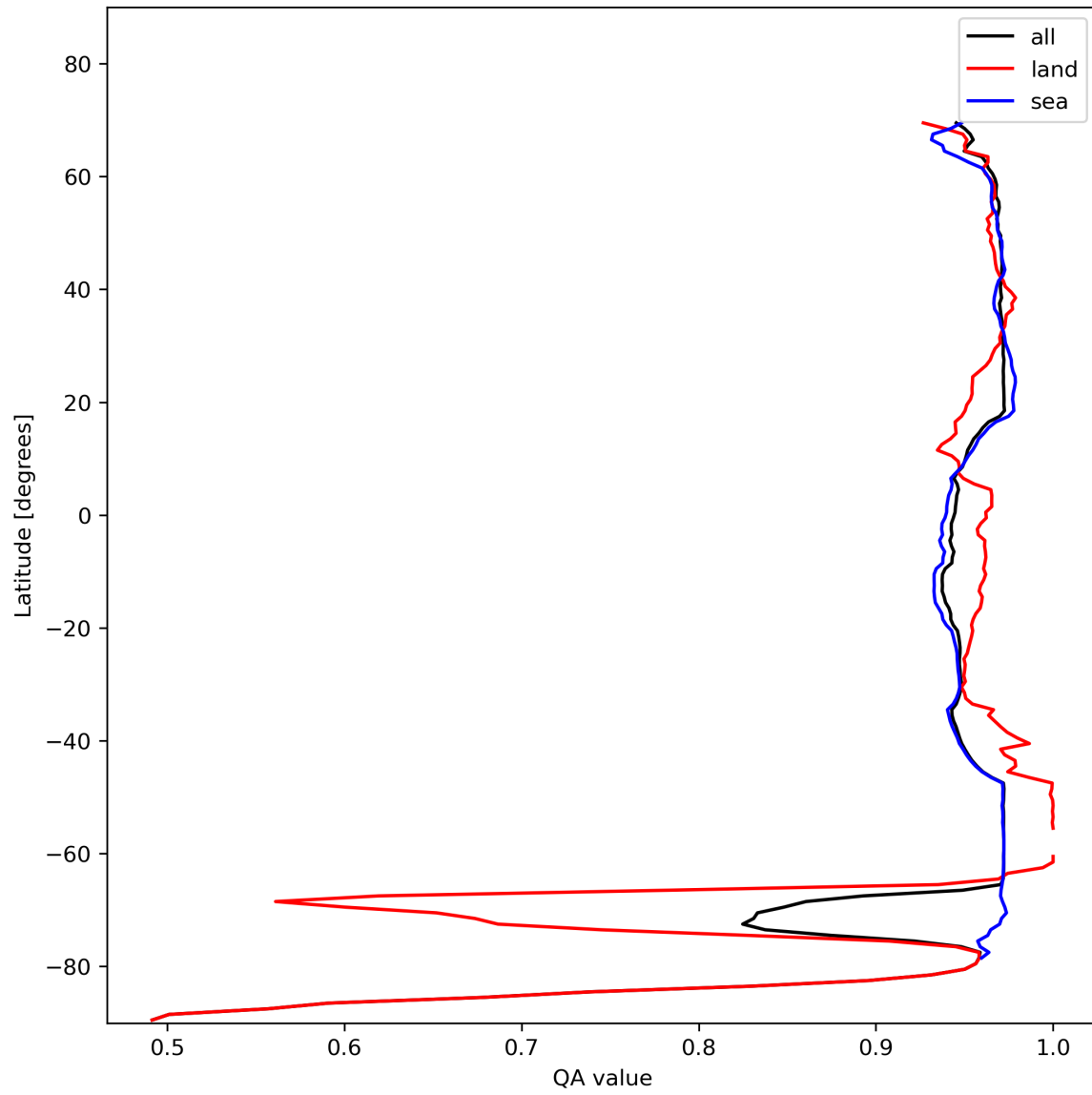
Figure 12: Zonal average of “QA value” for 2024-01-26 to 2024-01-28.
