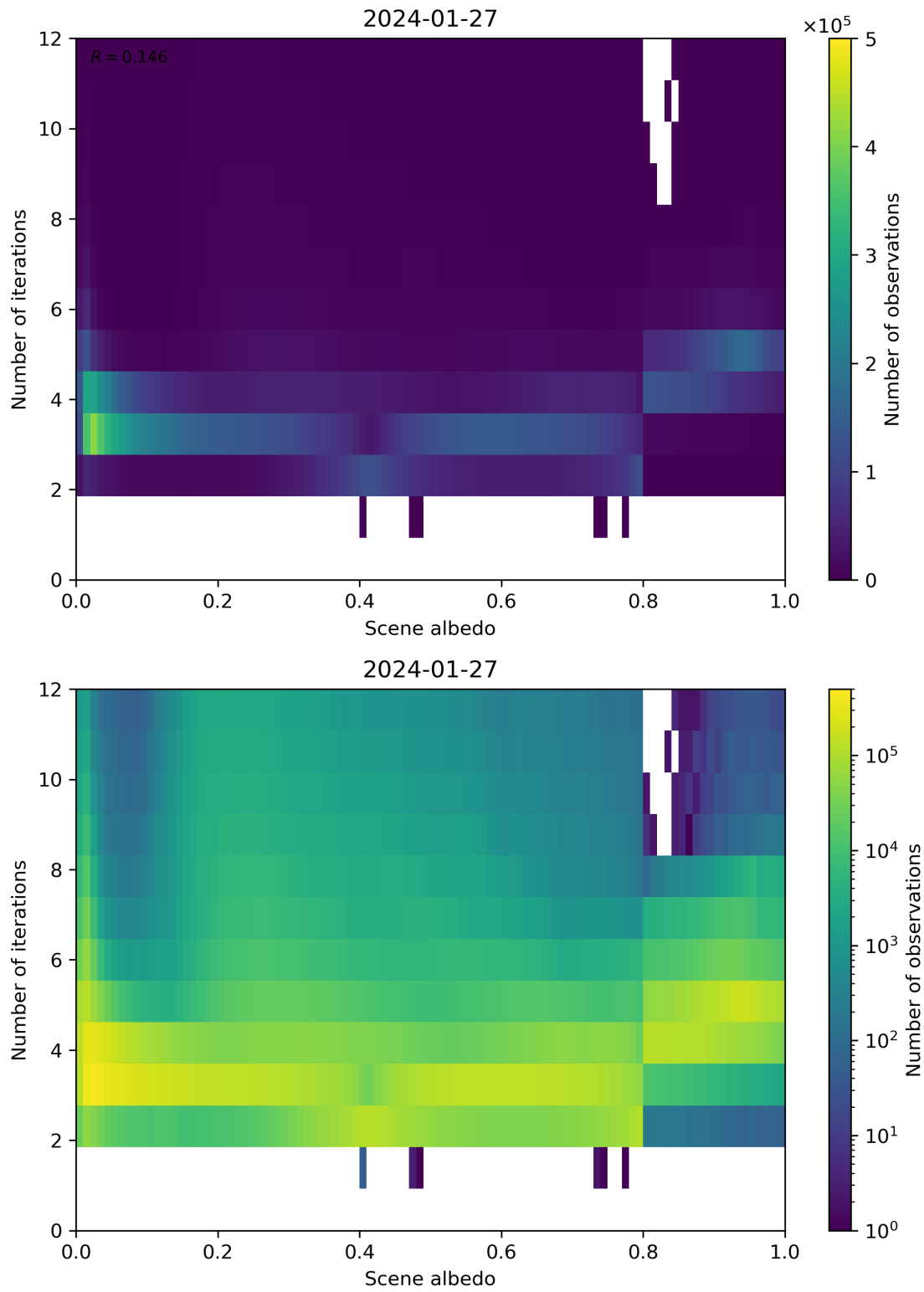
Figure 105: Scatter density plot of “Scene albedo” against “Number of iterations” for 2024-01-26 to 2024-01-28.
