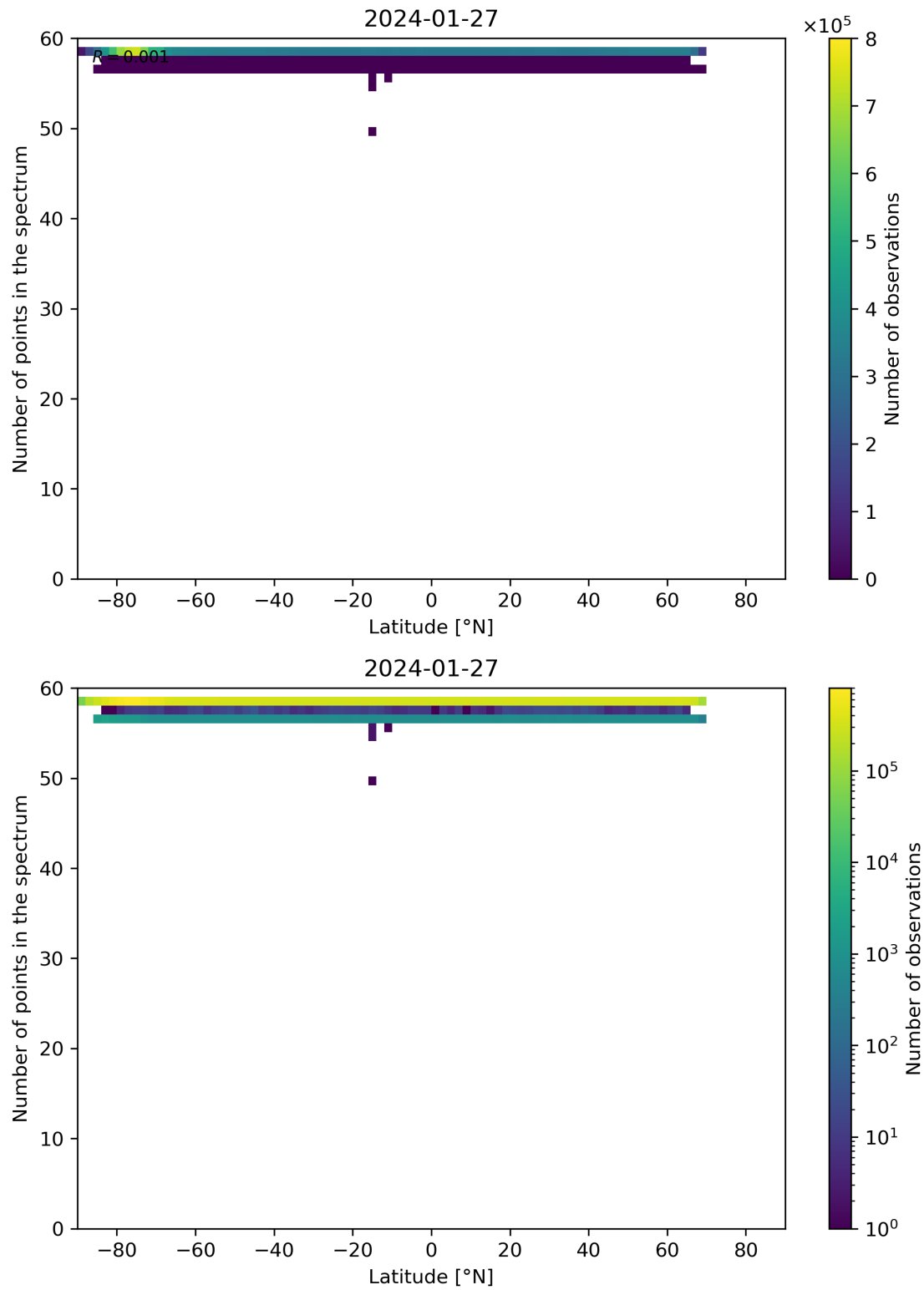
Figure 94: Scatter density plot of “Latitude” against “Number of points in the spectrum” for 2024-01-26 to 2024-01-28.
