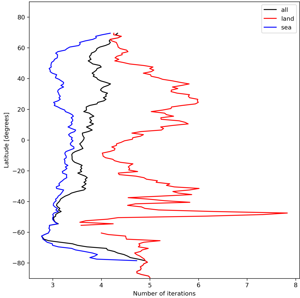
Figure 22: Zonal average of “Number of iterations” for 2024-01-26 to 2024-01-28.
