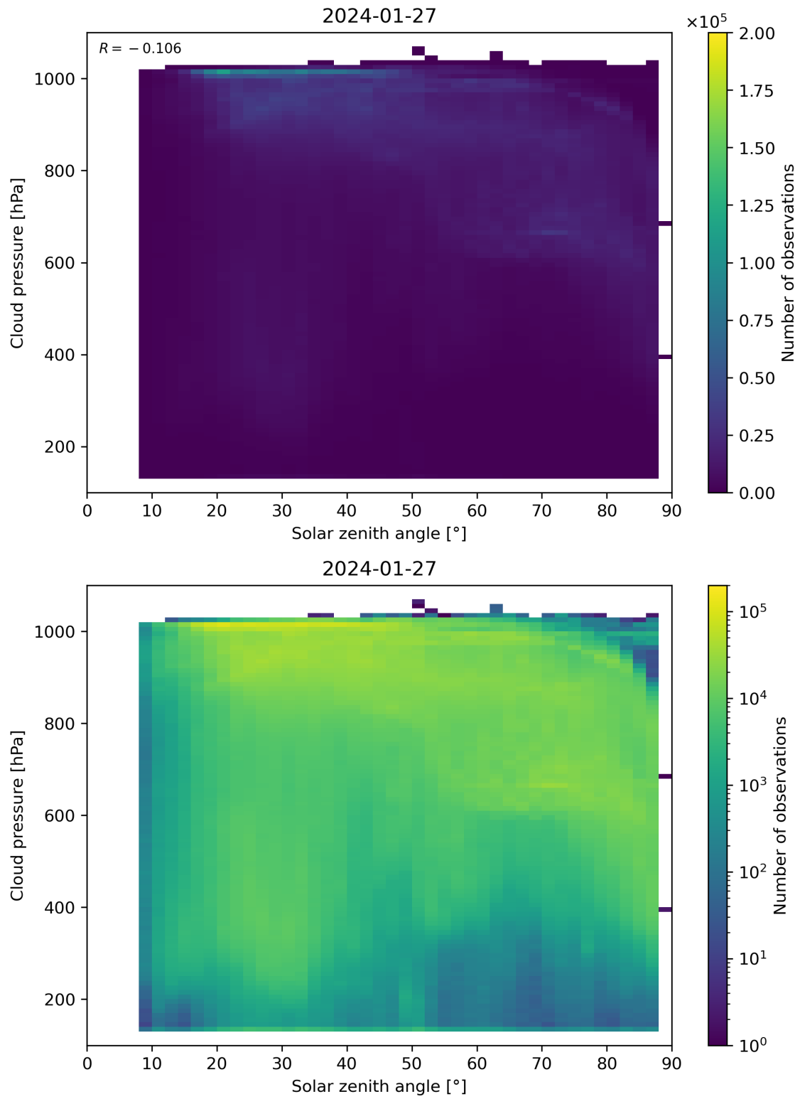
Figure 111: Scatter density plot of “Solar zenith angle” against “Cloud pressure” for 2024-01-26 to 2024-01-28.
