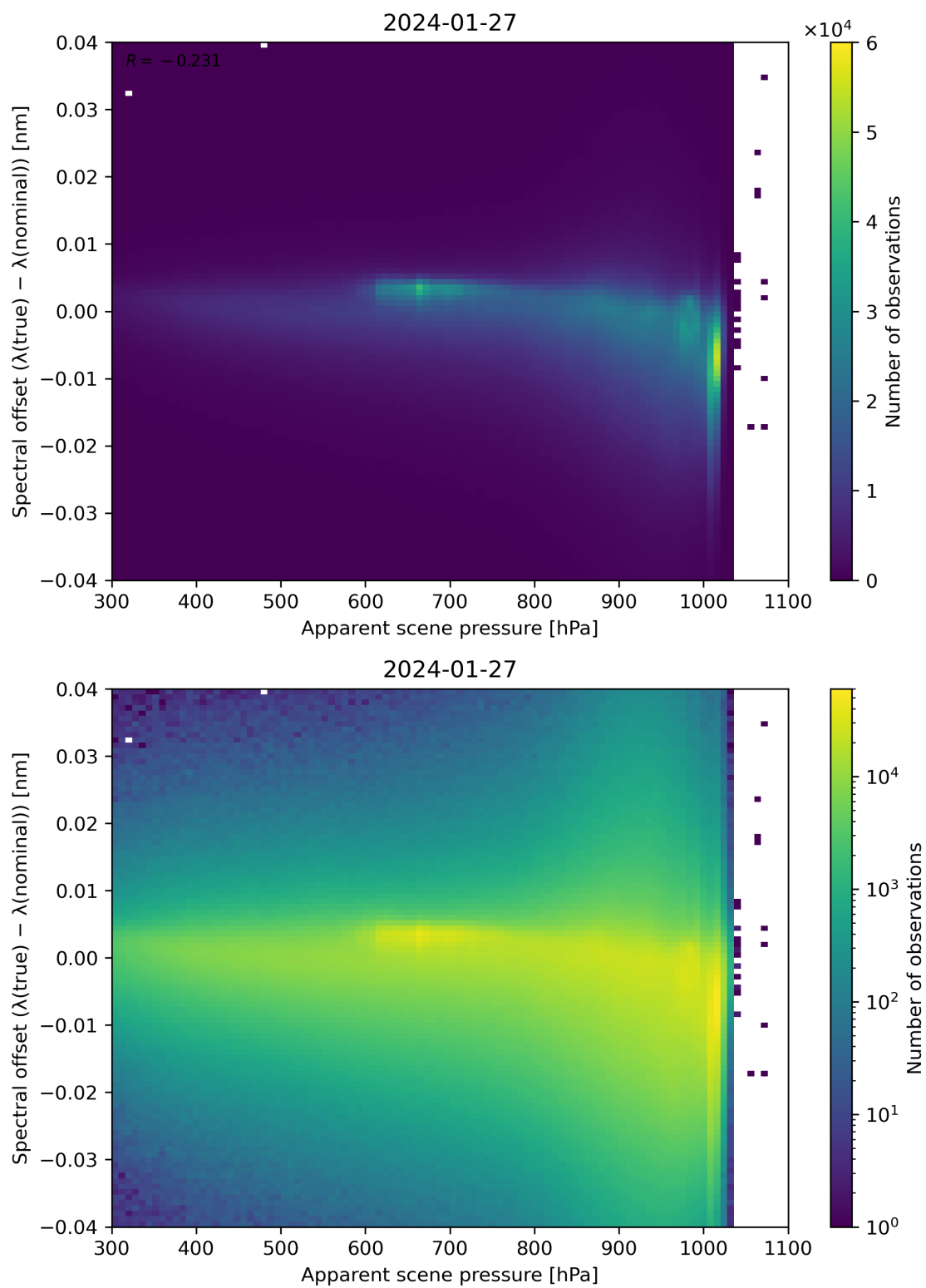
Figure 67: Scatter density plot of “Apparent scene pressure” against “Spectral offset ( \lambda(\text{true}) - \lambda(\text{nominal}) )” for 2024-01-26 to 2024-01-28.
