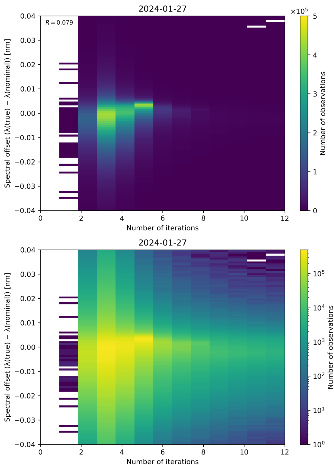
Figure 100: Scatter density plot of “Number of iterations” against “Spectral offset ( \lambda(\text{true}) - \lambda(\text{nominal}) )” for 2024-01-26 to 2024-01-28.
