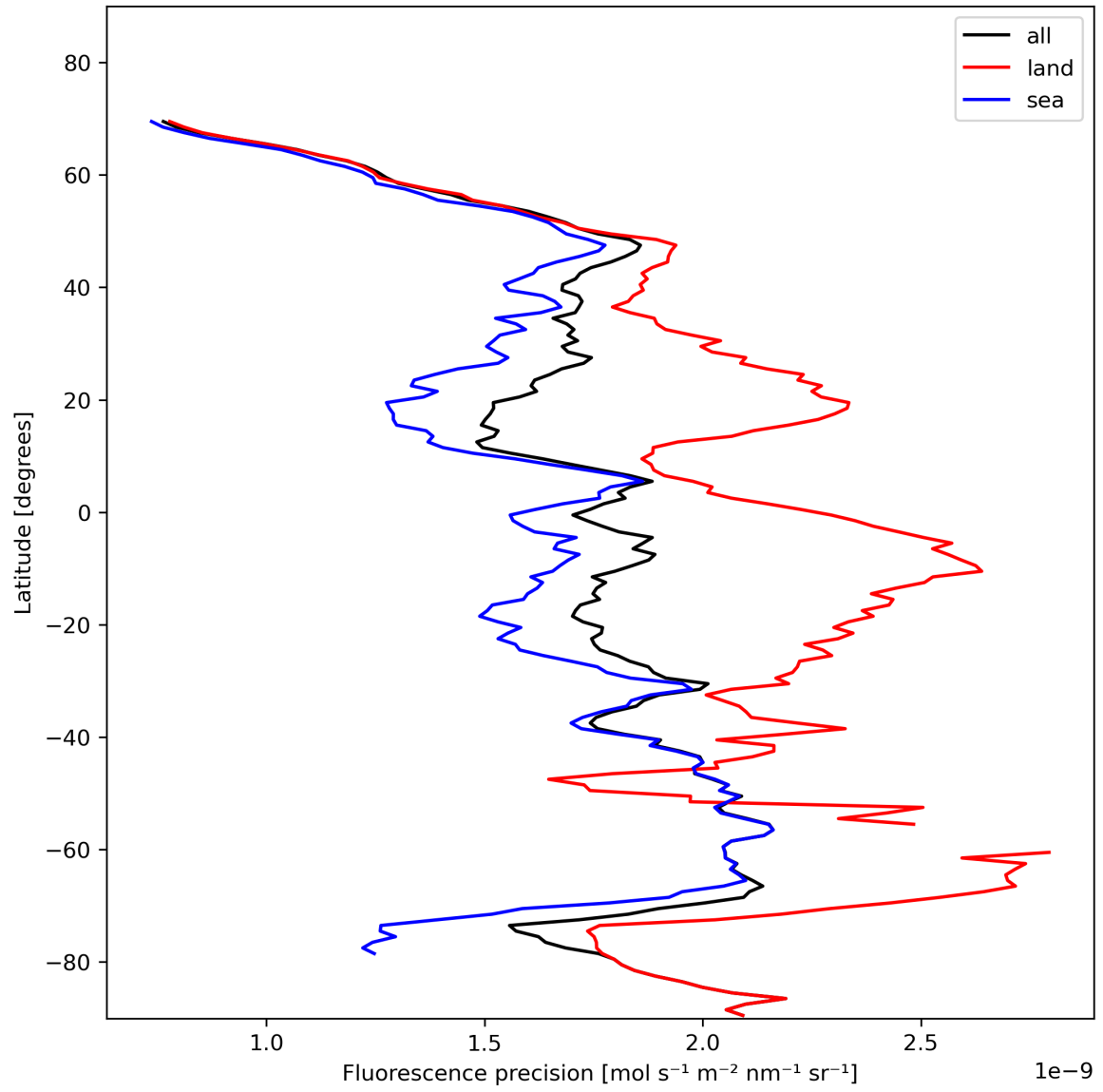
Figure 24: Zonal average of “Fluorescence precision” for 2024-01-26 to 2024-01-28.
