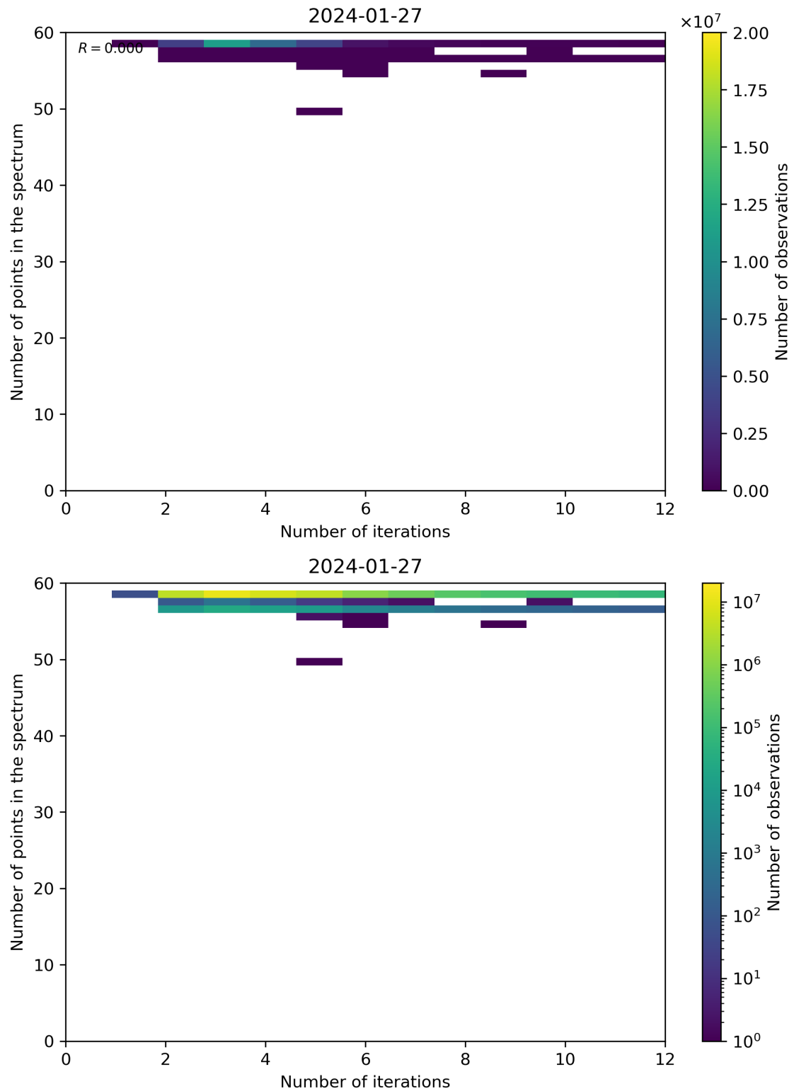
Figure 99: Scatter density plot of “Number of iterations” against “Number of points in the spectrum” for 2024-01-26 to 2024-01-28.
