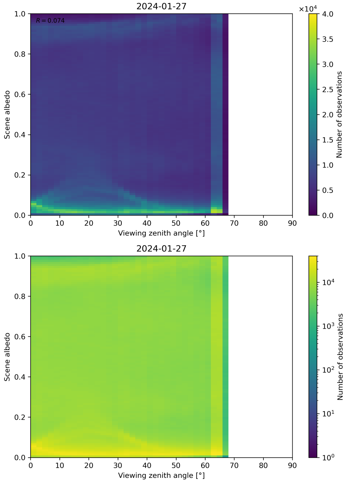
Figure 126: Scatter density plot of “Viewing zenith angle” against “Scene albedo” for 2024-01-26 to 2024-01-28.
