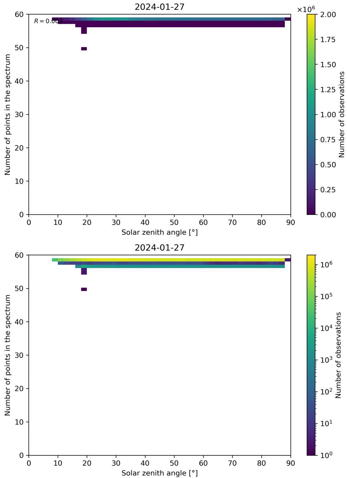
Figure 115: Scatter density plot of “Solar zenith angle” against “Number of points in the spectrum” for 2024-01-26 to 2024-01-28.
