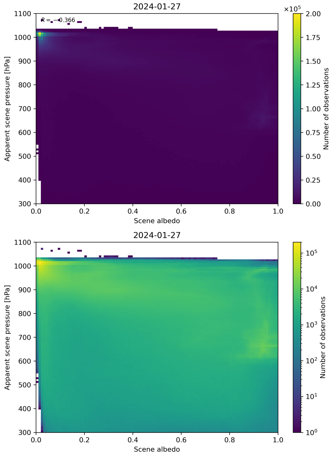
Figure 102: Scatter density plot of “Scene albedo” against “Apparent scene pressure” for 2024-01-26 to 2024-01-28.
