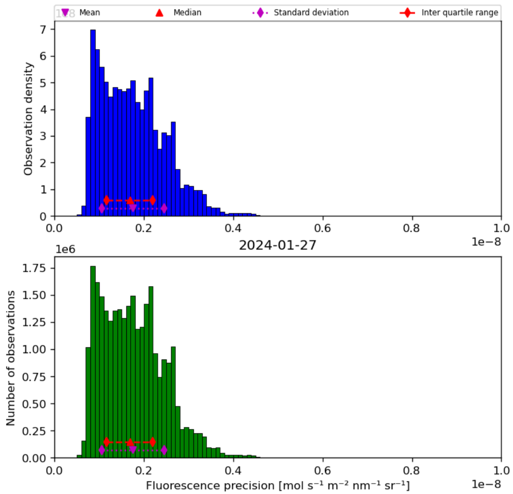
Figure 41: Histogram of “Fluorescence precision” for 2024-01-26 to 2024-01-28
