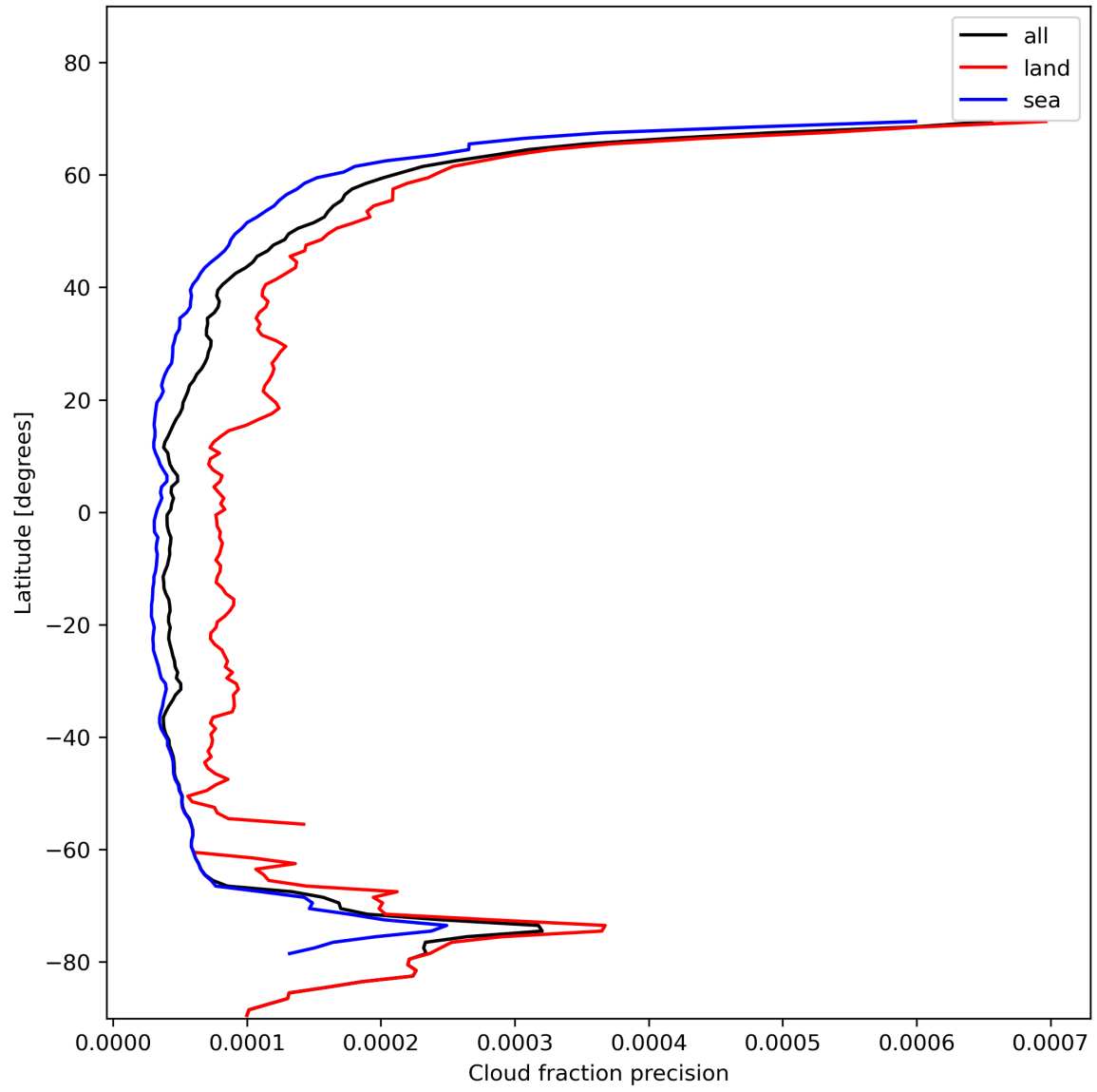
Figure 16: Zonal average of “Cloud fraction precision” for 2024-01-26 to 2024-01-28.
