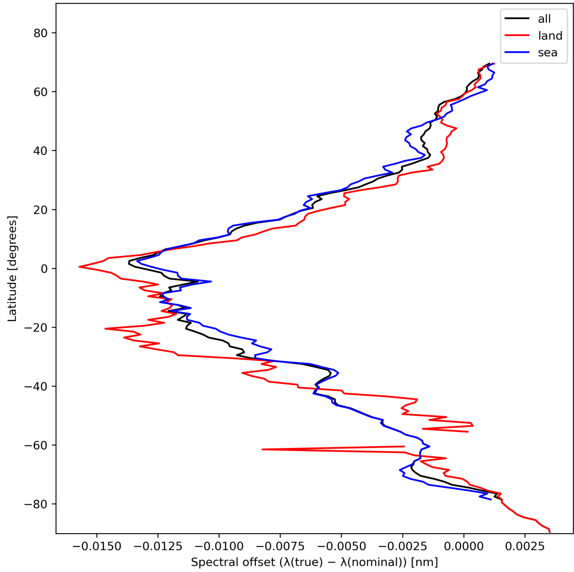
Figure 28: Zonal average of “Spectral offset ( \lambda(\text{true}) - \lambda(\text{nominal}) )” for 2024-01-26 to 2024-01-28.
