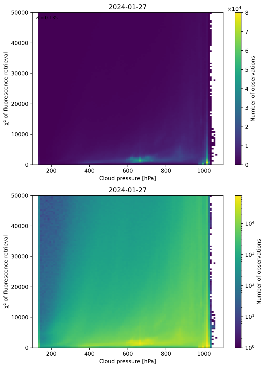
Figure 78: Scatter density plot of “Cloud pressure” against “ \chi^2 of fluorescence retrieval” for 2024-01-26 to 2024-01-28.
