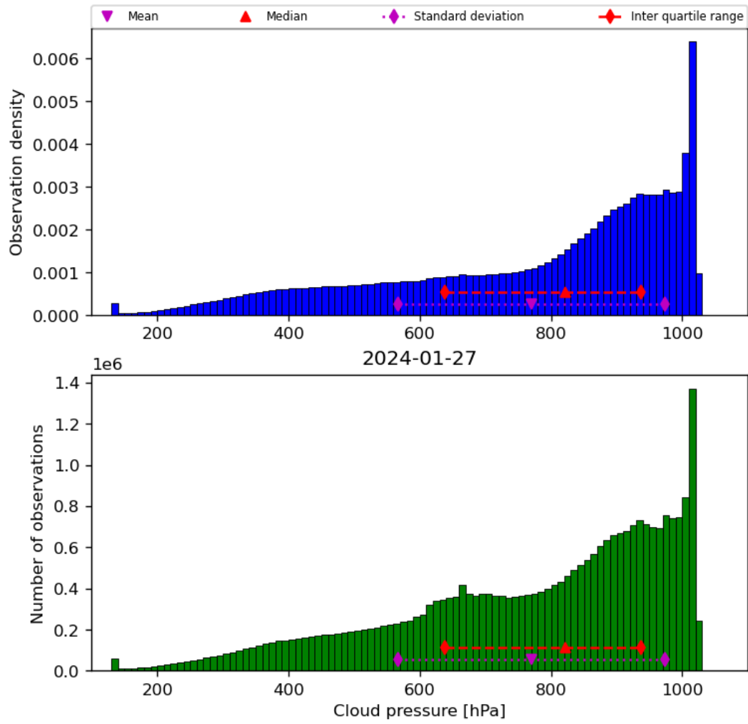
Figure 30: Histogram of “Cloud pressure” for 2024-01-26 to 2024-01-28
