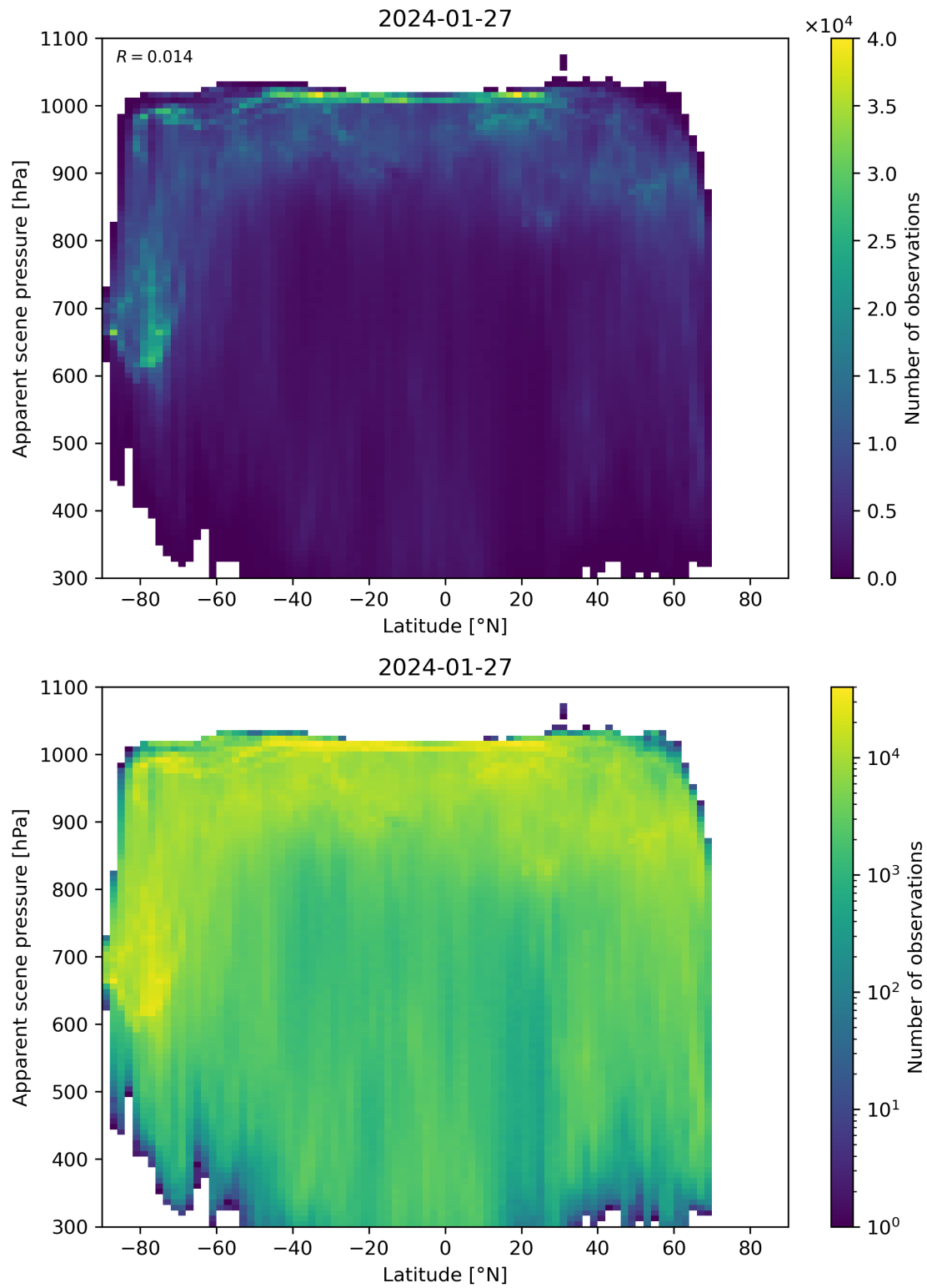
Figure 88: Scatter density plot of “Latitude” against “Apparent scene pressure” for 2024-01-26 to 2024-01-28.
