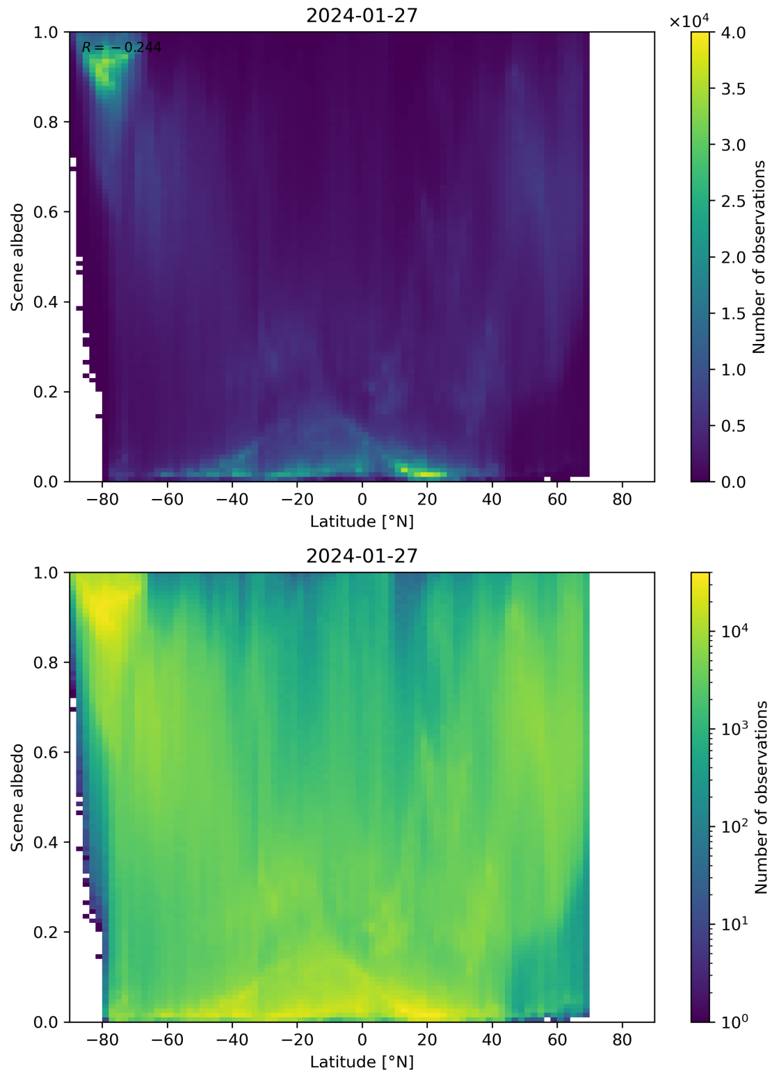
Figure 95: Scatter density plot of “Latitude” against “Scene albedo” for 2024-01-26 to 2024-01-28.
