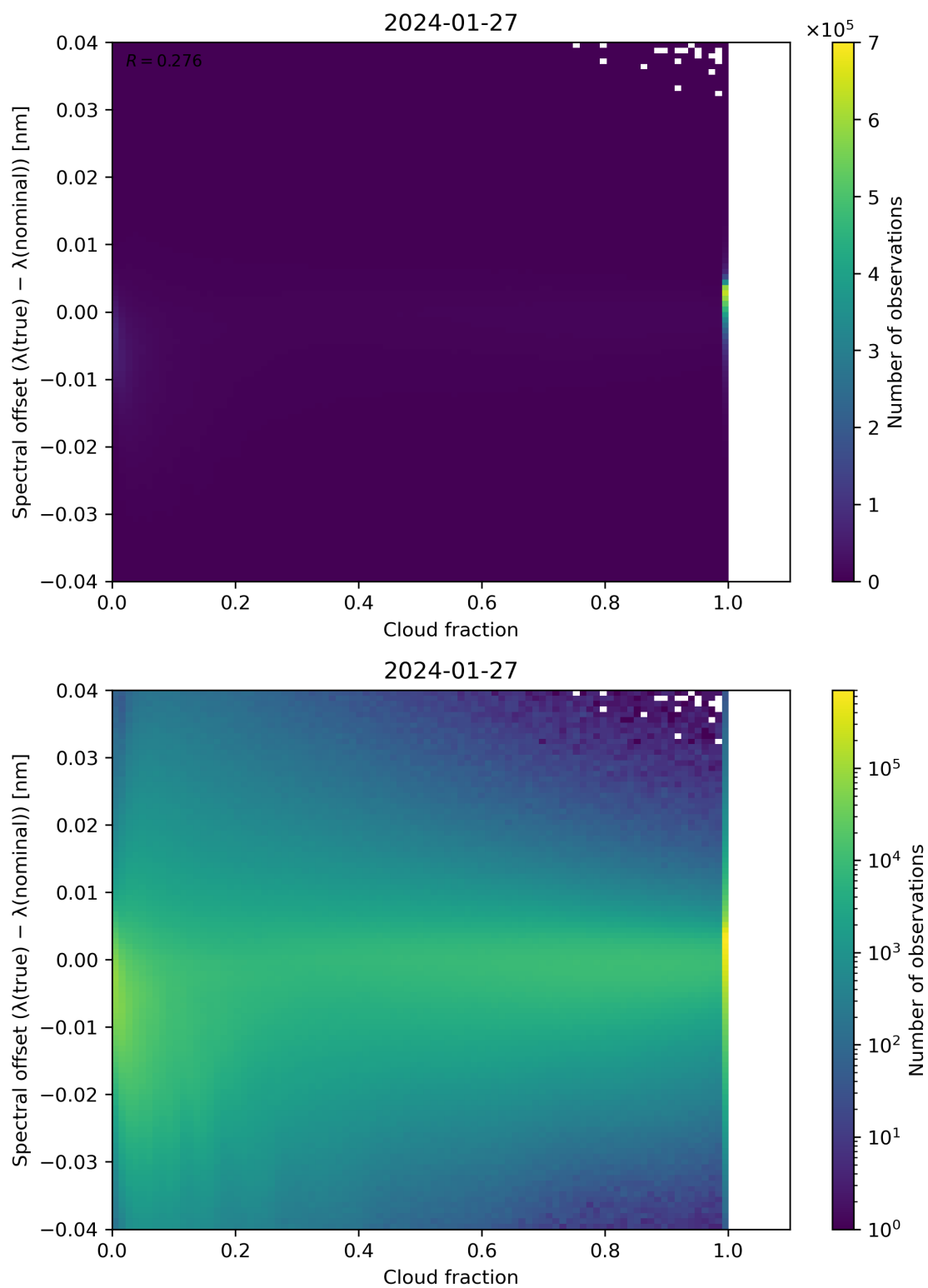
Figure 76: Scatter density plot of “Cloud fraction” against “Spectral offset ( \lambda(\text{true}) - \lambda(\text{nominal}) )” for 2024-01-26 to 2024-01-28.
