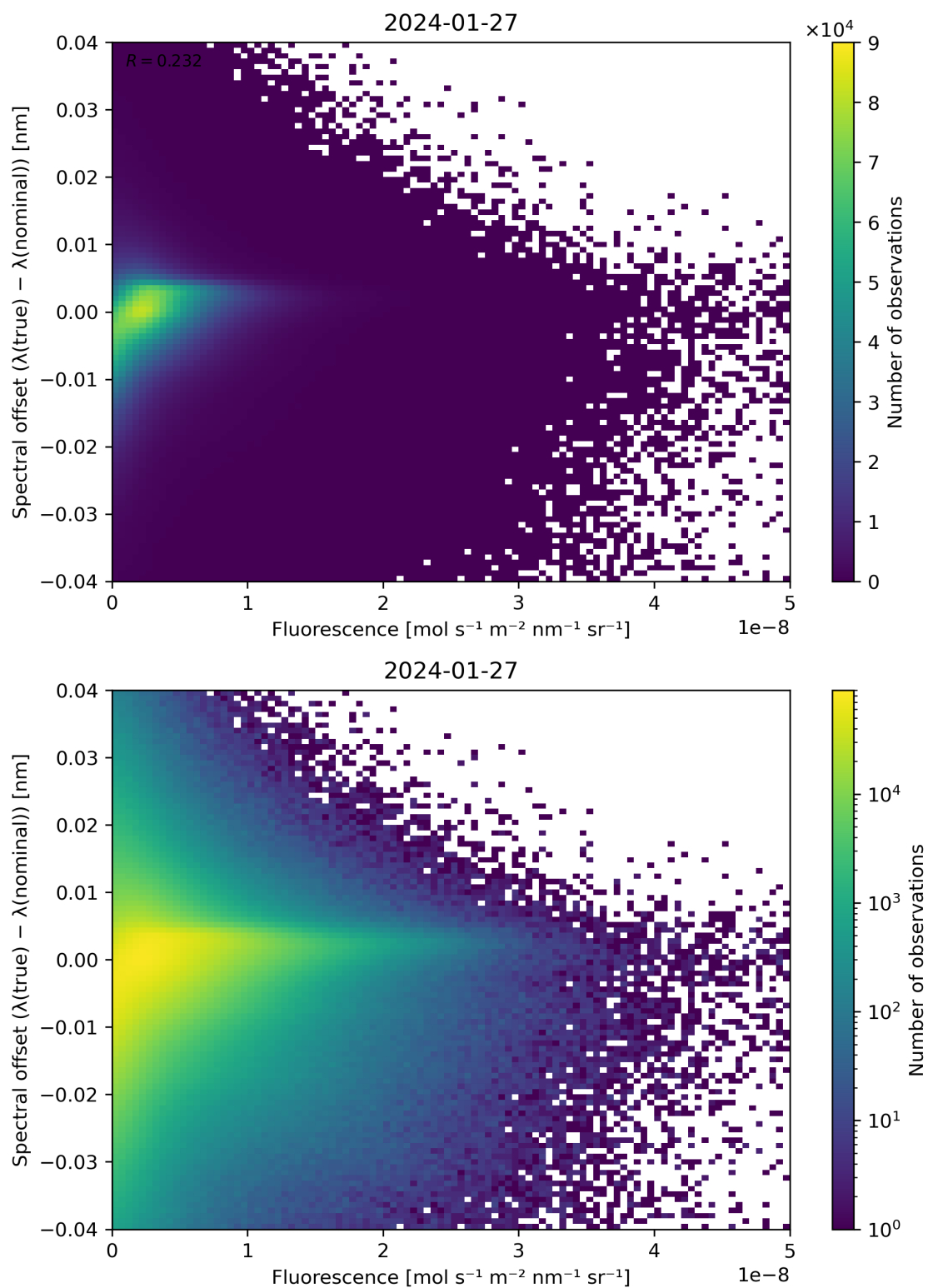
Figure 87: Scatter density plot of “Fluorescence” against “Spectral offset ( \lambda(\text{true}) - \lambda(\text{nominal}) )” for 2024-01-26 to 2024-01-28.
