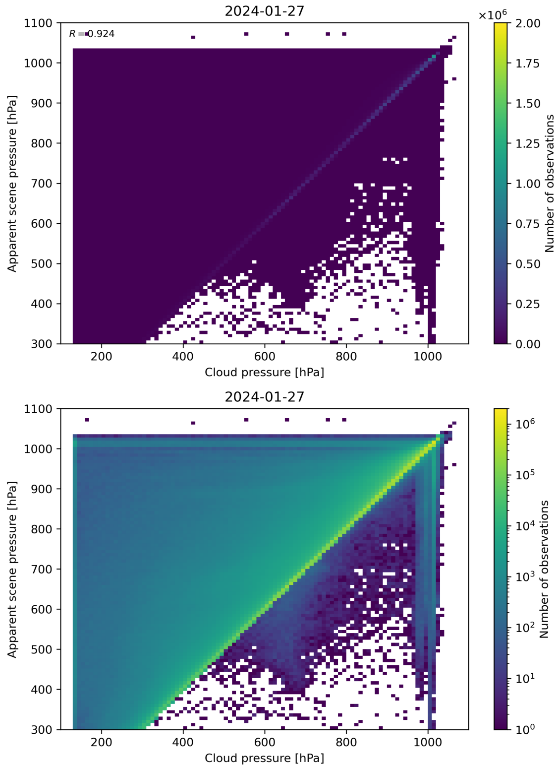
Figure 77: Scatter density plot of “Cloud pressure” against “Apparent scene pressure” for 2024-01-26 to 2024-01-28.
