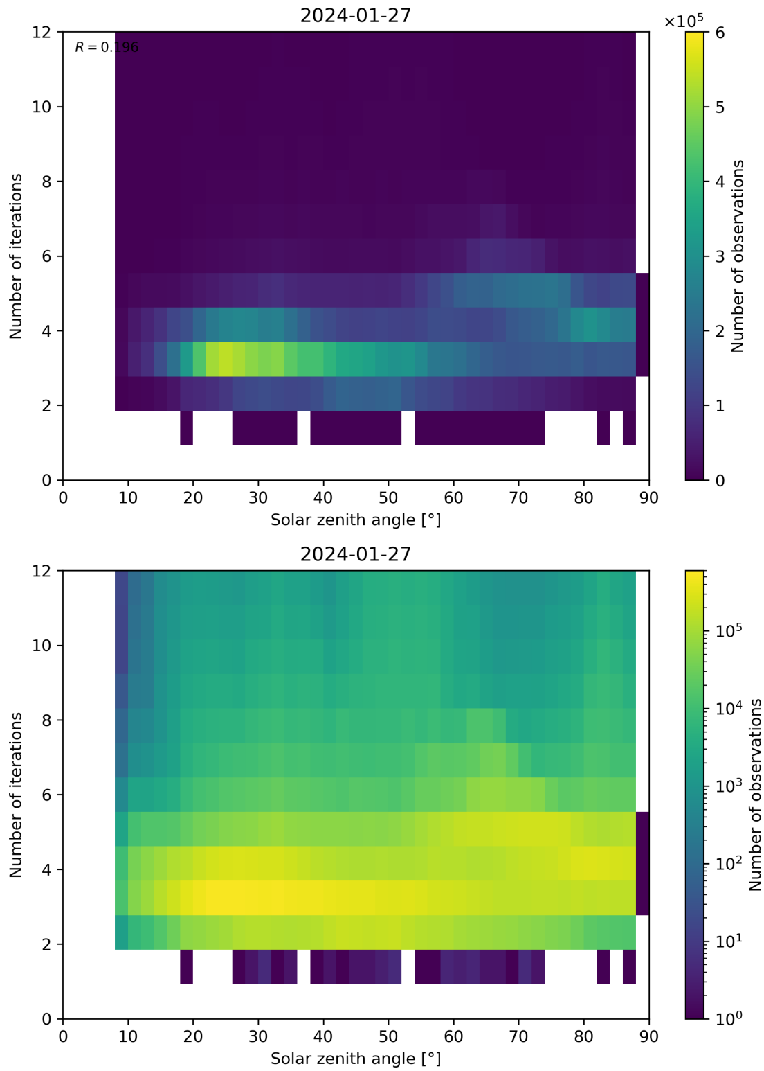
Figure 114: Scatter density plot of “Solar zenith angle” against “Number of iterations” for 2024-01-26 to 2024-01-28.
