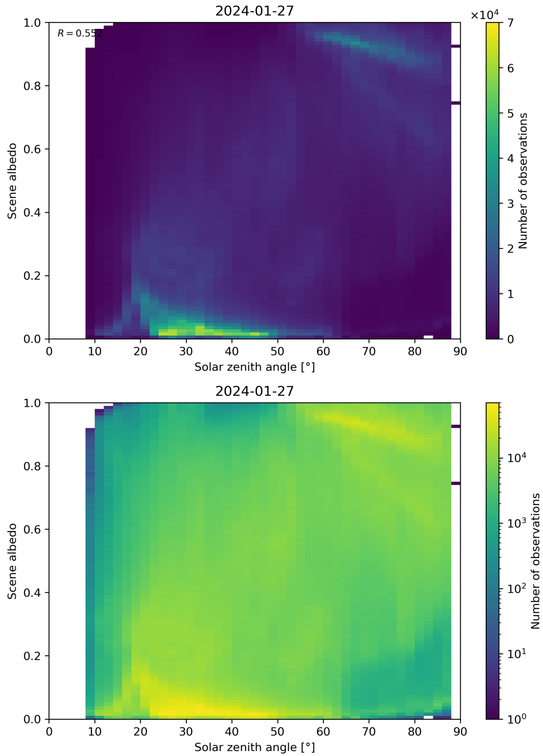
Figure 116: Scatter density plot of “Solar zenith angle” against “Scene albedo” for 2024-01-26 to 2024-01-28.
