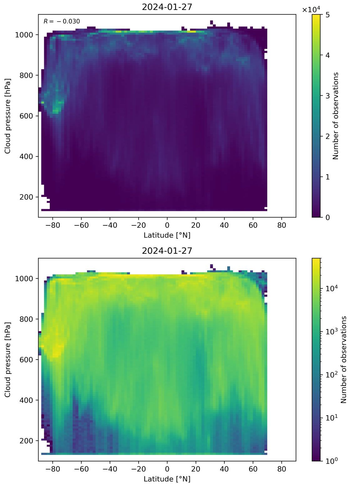
Figure 91: Scatter density plot of “Latitude” against “Cloud pressure” for 2024-01-26 to 2024-01-28.
