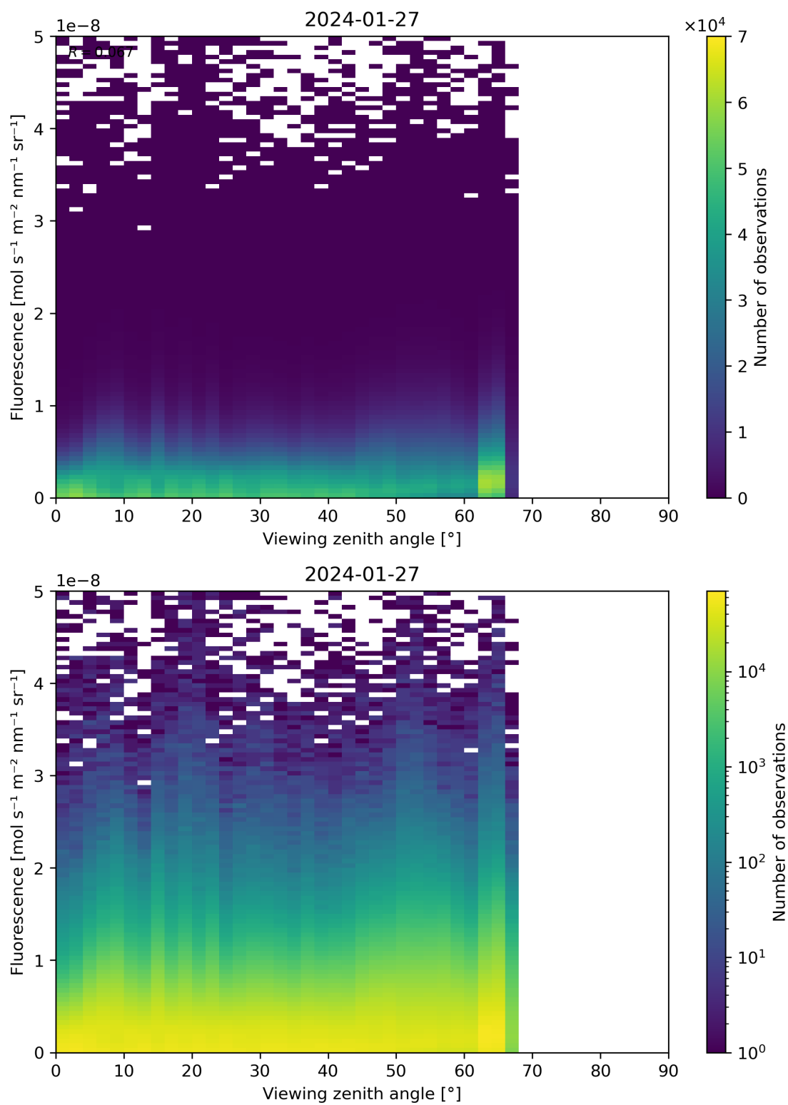
Figure 122: Scatter density plot of “Viewing zenith angle” against “Fluorescence” for 2024-01-26 to 2024-01-28.
