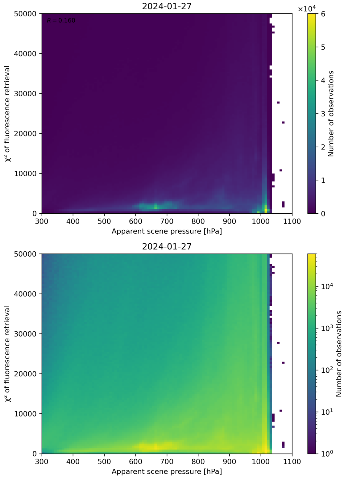
Figure 63: Scatter density plot of “Apparent scene pressure” against “ \chi^2 of fluorescence retrieval” for 2024-01-26 to 2024-01-28.
