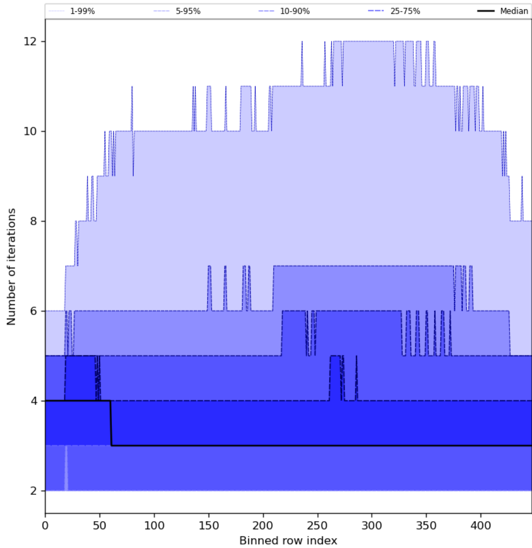
Figure 56: Along track statistics of “Number of iterations” for 2024-01-26 to 2024-01-28
