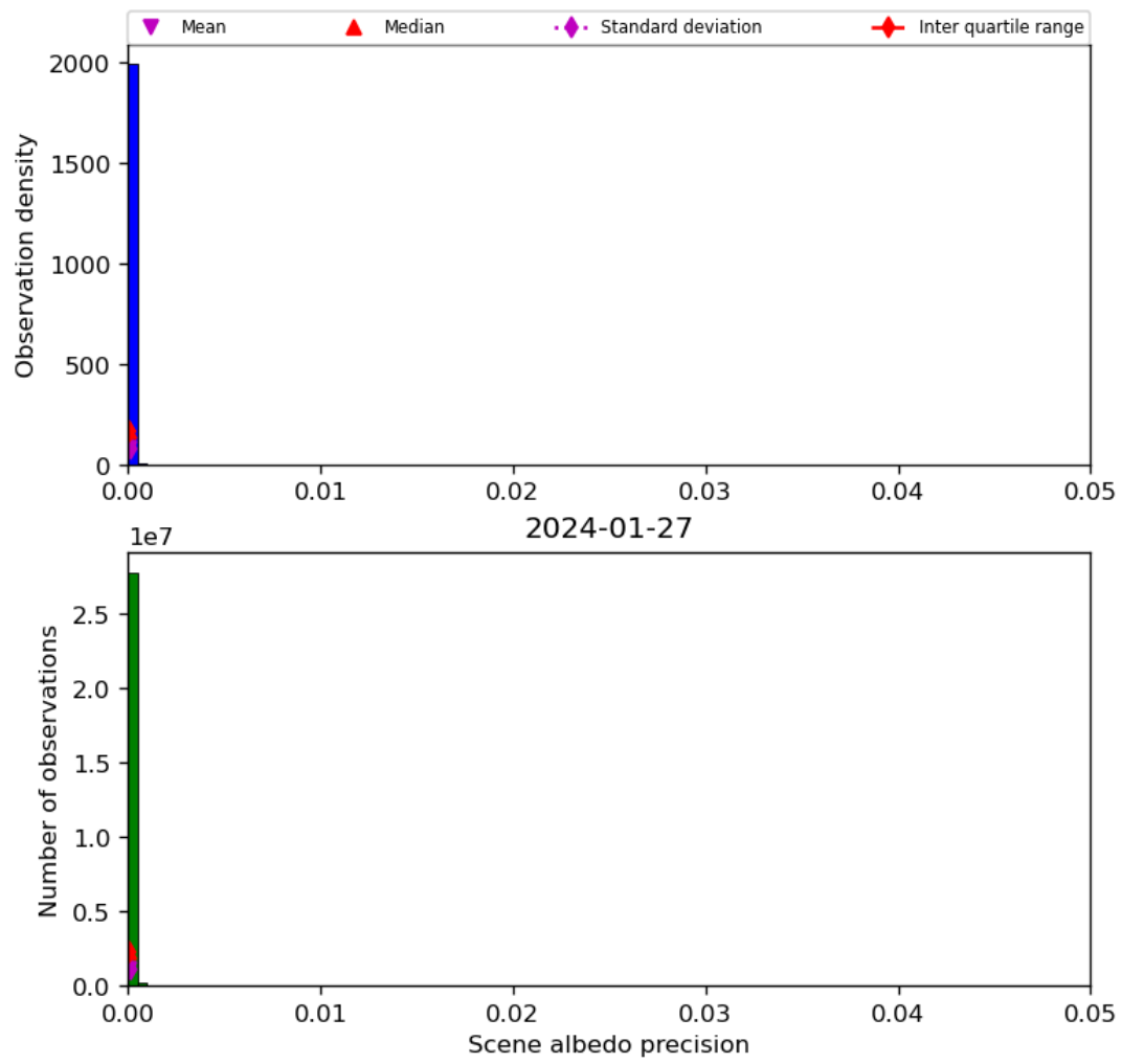
Figure 35: Histogram of “Scene albedo precision” for 2024-01-26 to 2024-01-28
