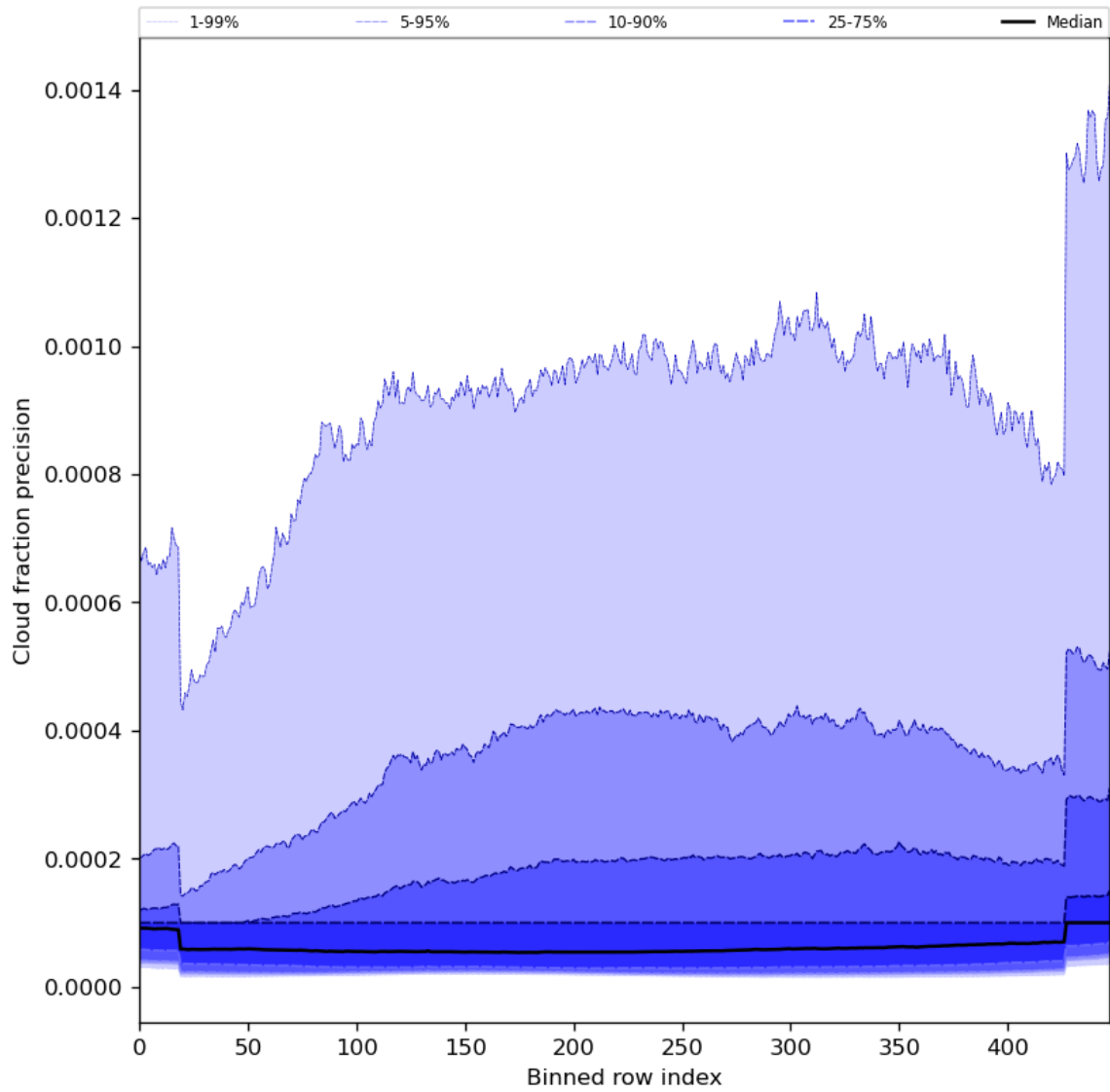
Figure 50: Along track statistics of “Cloud fraction precision” for 2024-01-26 to 2024-01-28
