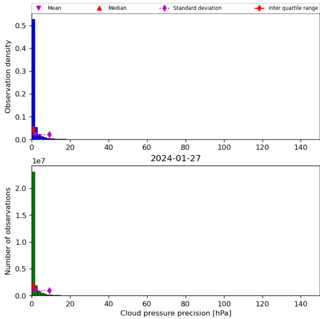
Figure 31: Histogram of “Cloud pressure precision” for 2024-01-26 to 2024-01-28
