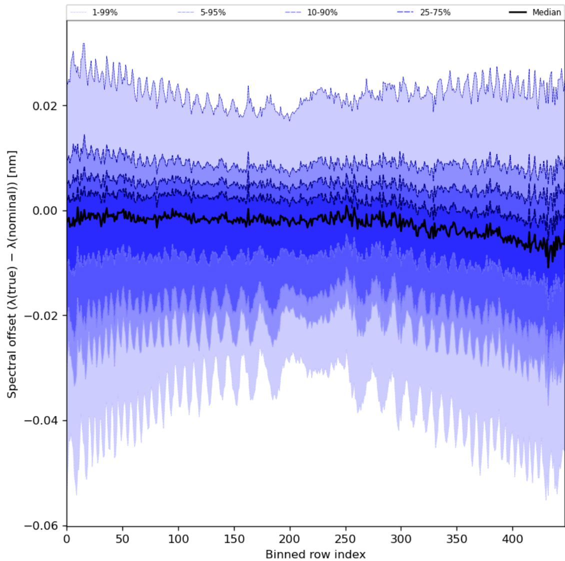
Figure 62: Along track statistics of “Spectral offset ( \lambda(\text{true}) - \lambda(\text{nominal}) )” for 2024-01-26 to 2024-01-28
