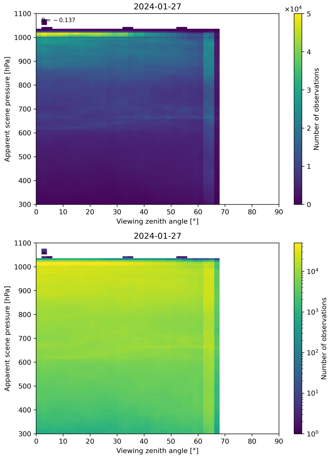
Figure 118: Scatter density plot of “Viewing zenith angle” against “Apparent scene pressure” for 2024-01-26 to 2024-01-28.
