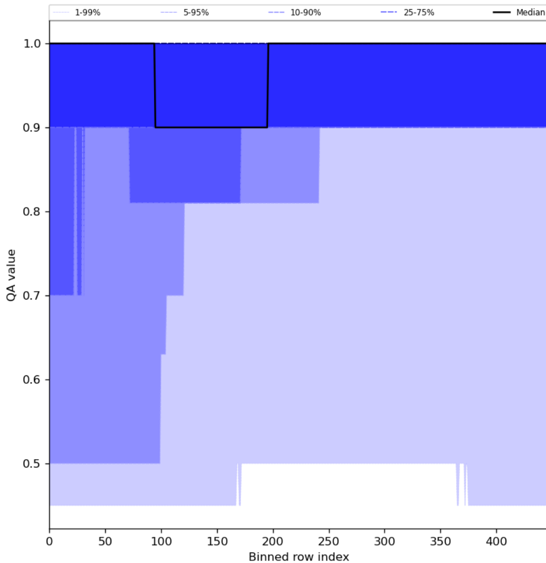
Figure 46: Along track statistics of “QA value” for 2024-01-26 to 2024-01-28
