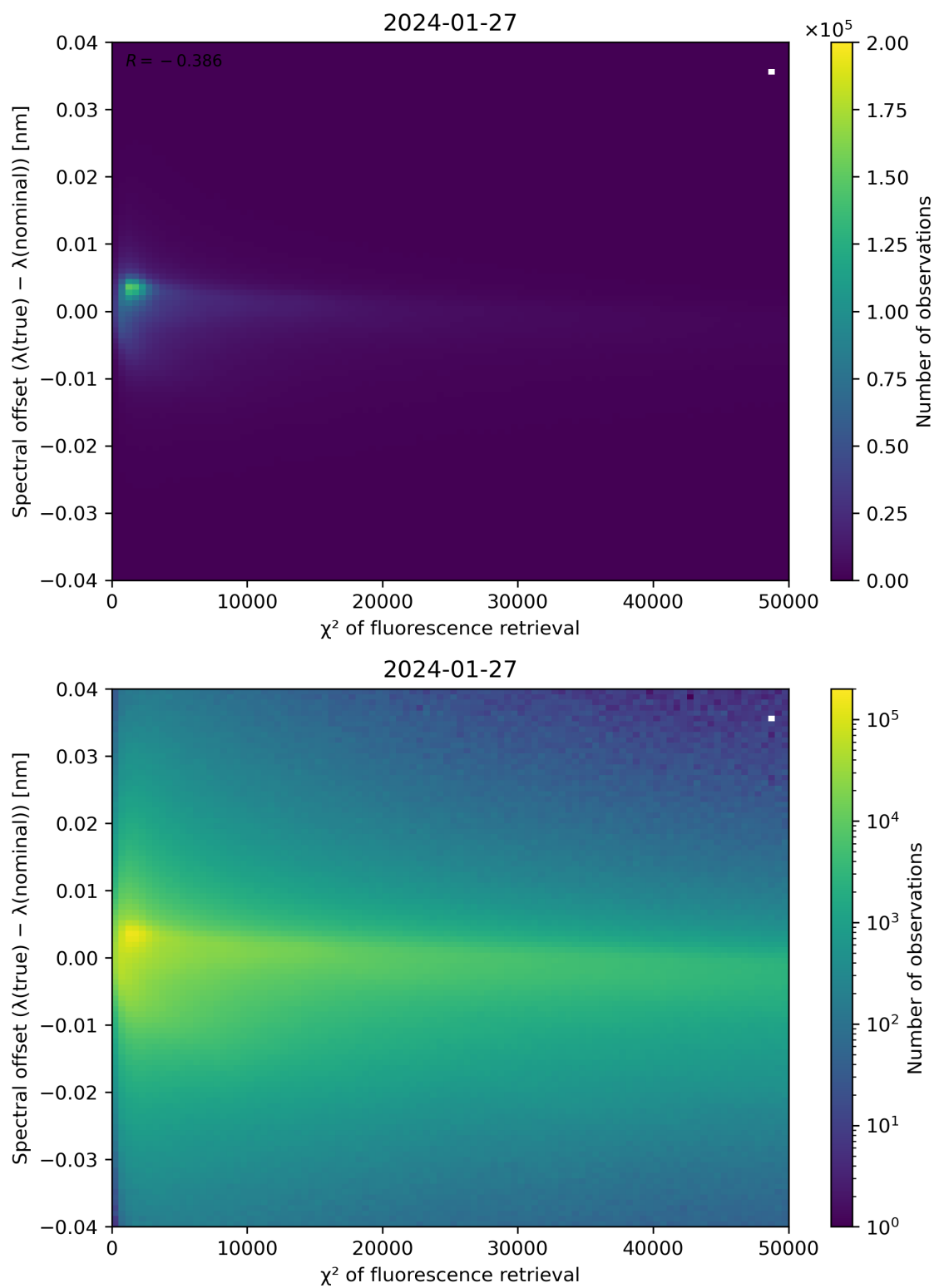
Figure 69: Scatter density plot of “ \chi^2 of fluorescence retrieval” against “Spectral offset ( \lambda(\text{true}) - \lambda(\text{nominal})) ” for 2024-01-26 to 2024-01-28.
