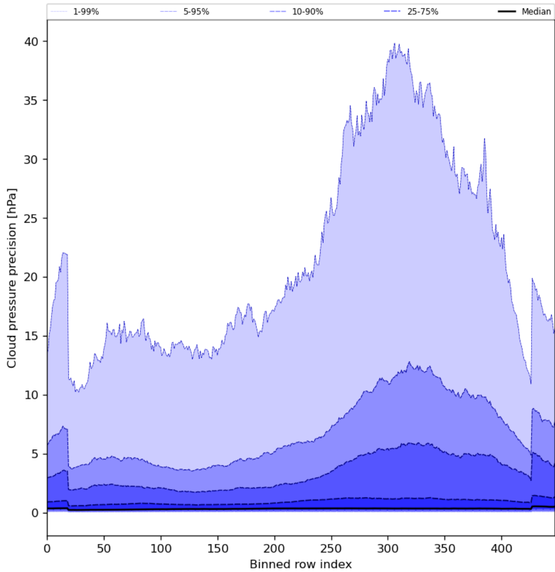
Figure 48: Along track statistics of “Cloud pressure precision” for 2024-01-26 to 2024-01-28
