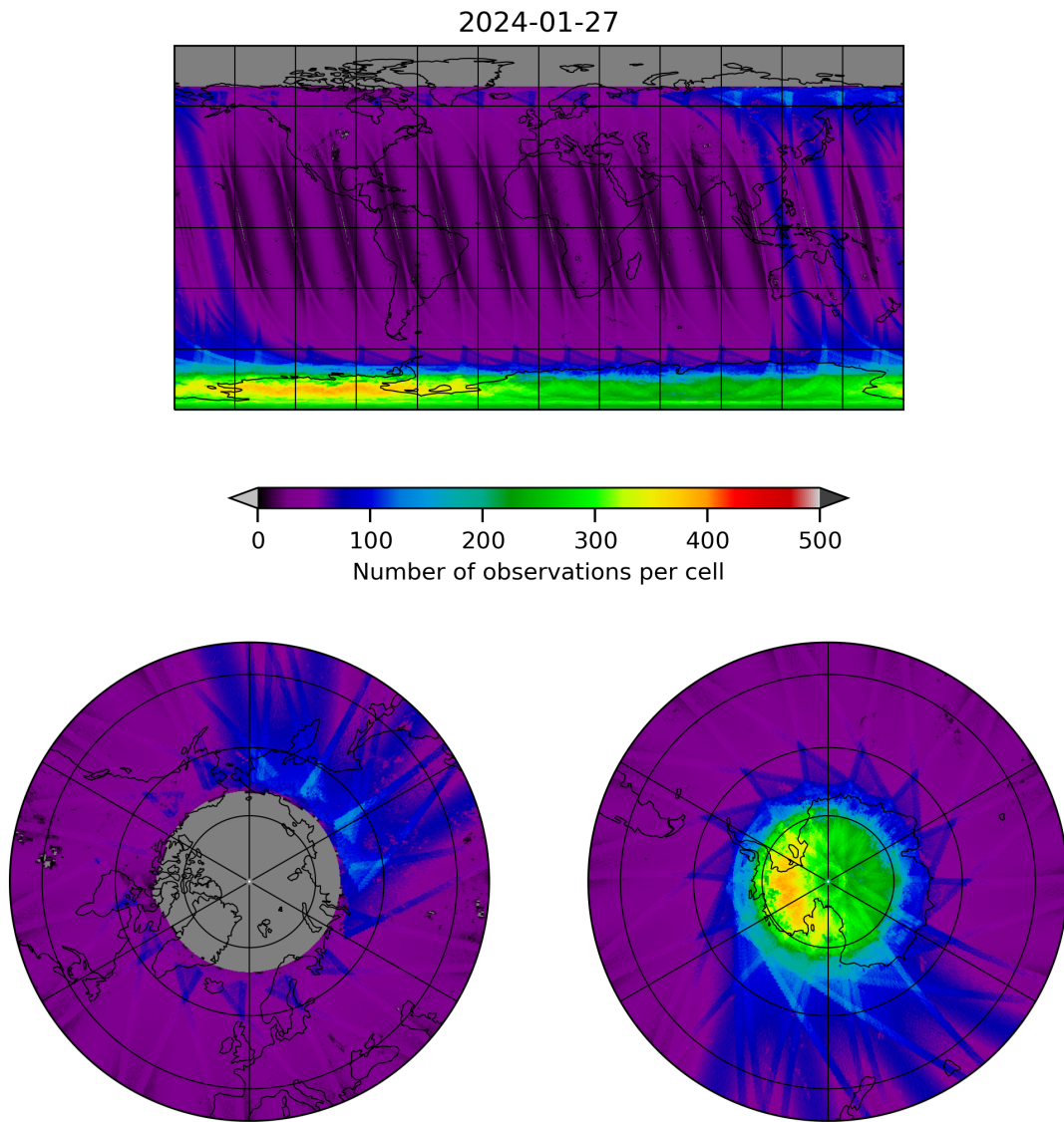
Figure 11: Map of the number of observations for 2024-01-26 to 2024-01-28
