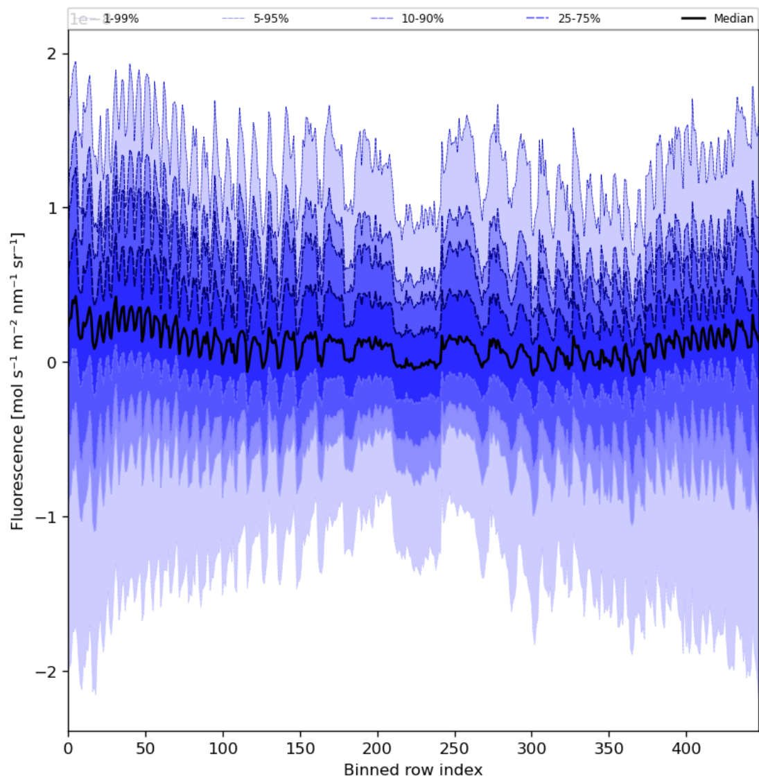
Figure 57: Along track statistics of “Fluorescence” for 2024-01-26 to 2024-01-28
