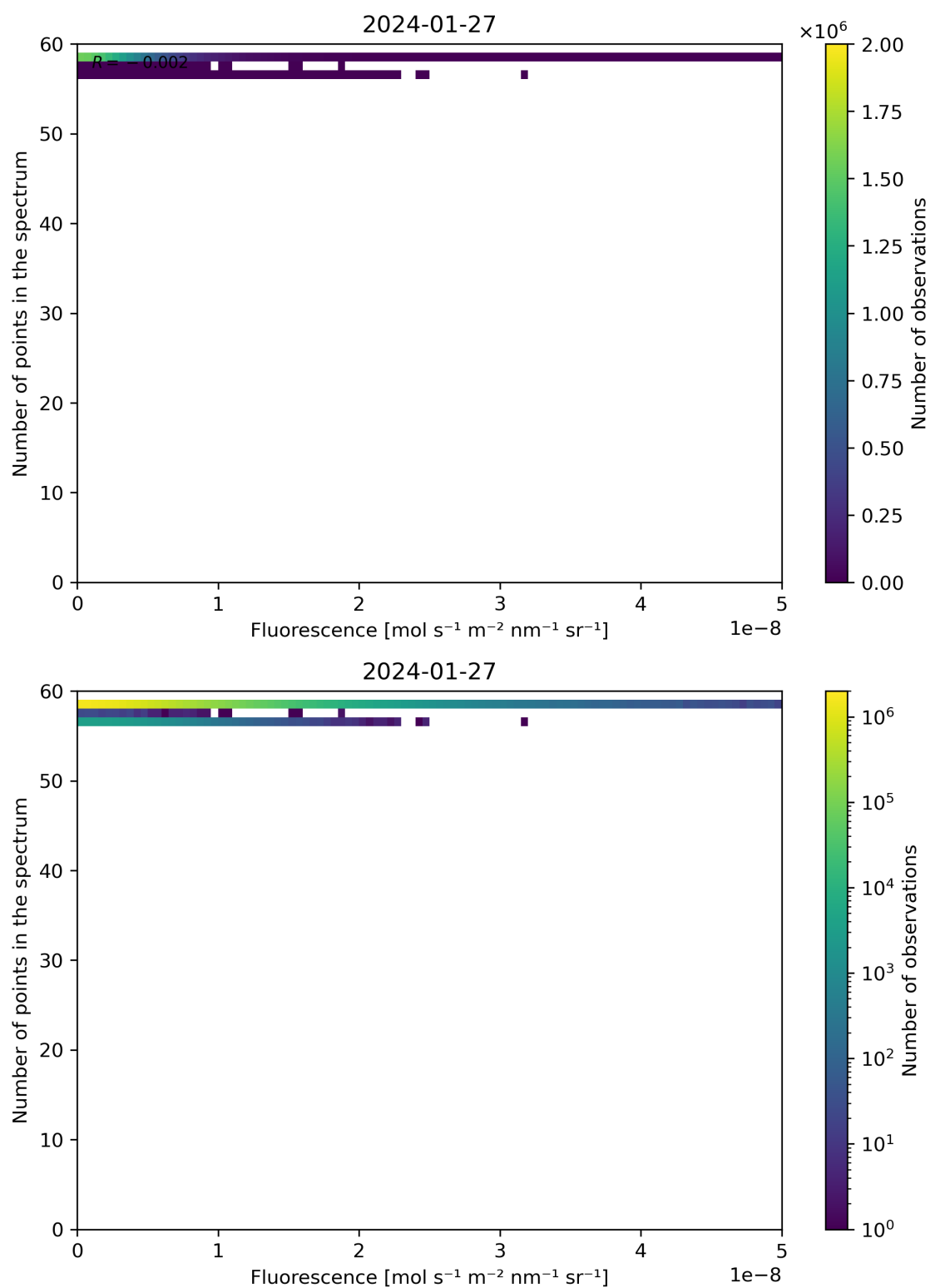
Figure 86: Scatter density plot of “Fluorescence” against “Number of points in the spectrum” for 2024-01-26 to 2024-01-28.
