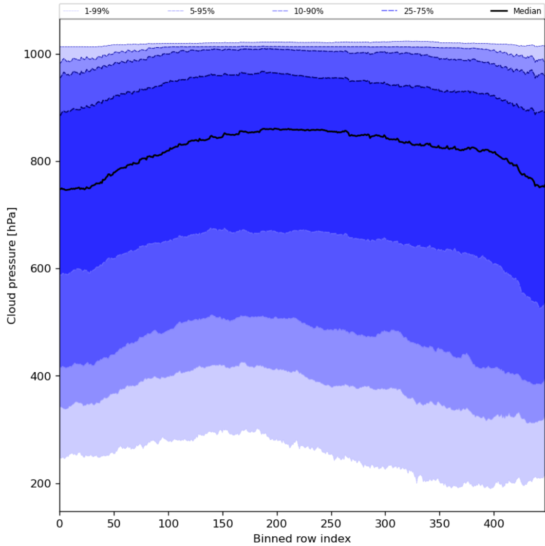
Figure 47: Along track statistics of “Cloud pressure” for 2024-01-26 to 2024-01-28
