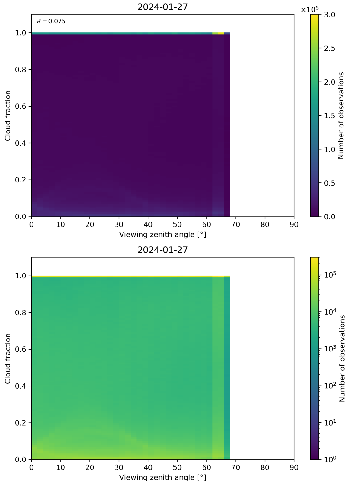
Figure 120: Scatter density plot of “Viewing zenith angle” against “Cloud fraction” for 2024-01-26 to 2024-01-28.
