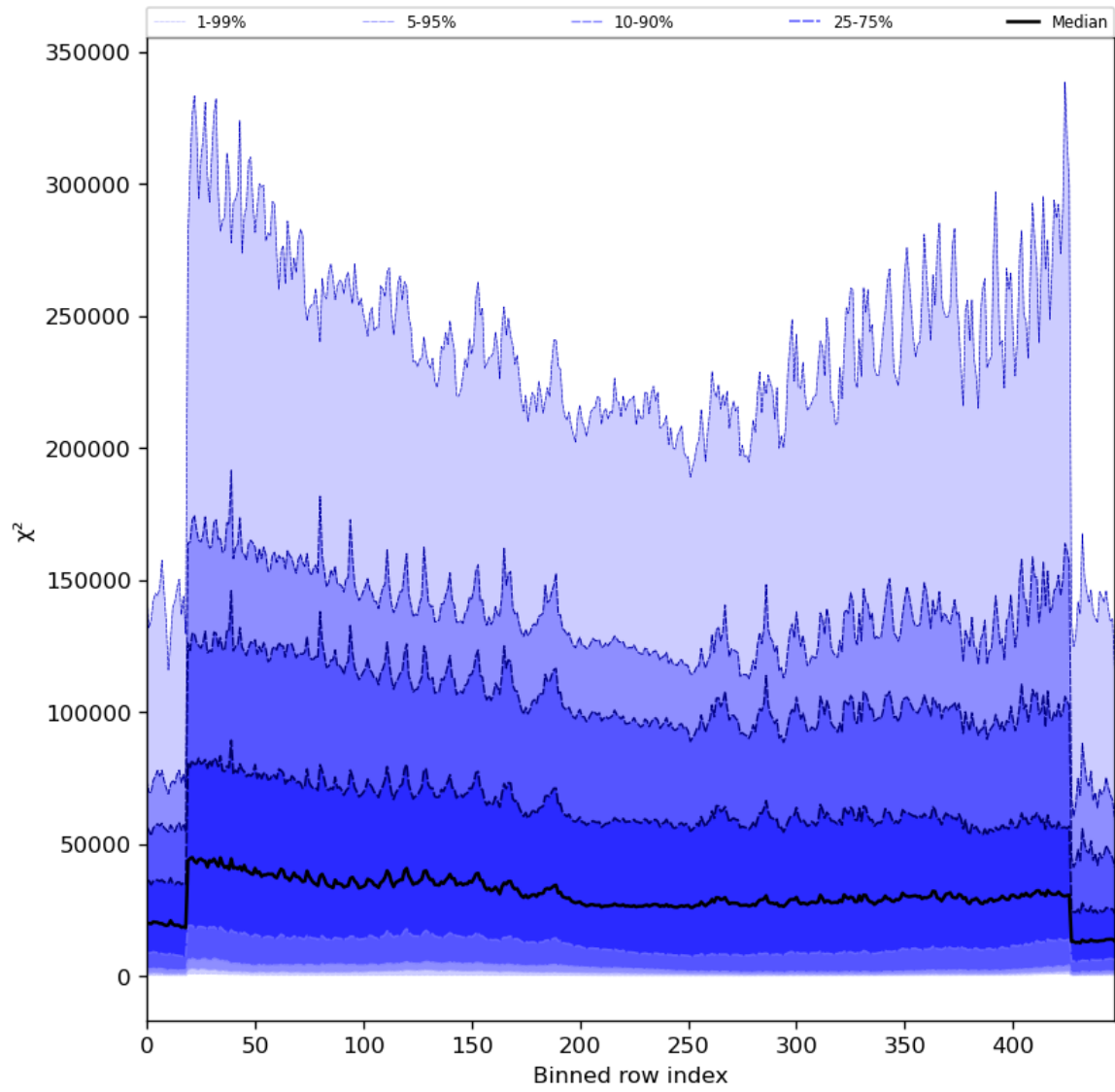
Figure 55: Along track statistics of “ \chi^2 ” for 2024-01-26 to 2024-01-28
