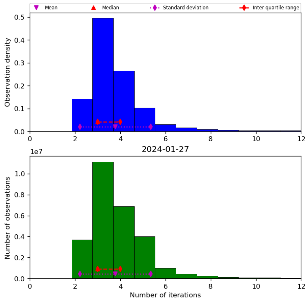
Figure 39: Histogram of “Number of iterations” for 2024-01-26 to 2024-01-28
