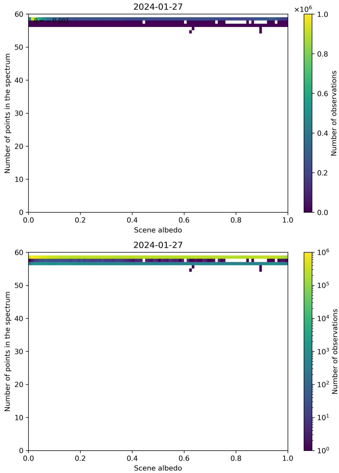
Figure 106: Scatter density plot of “Scene albedo” against “Number of points in the spectrum” for 2024-01-26 to 2024-01-28.
