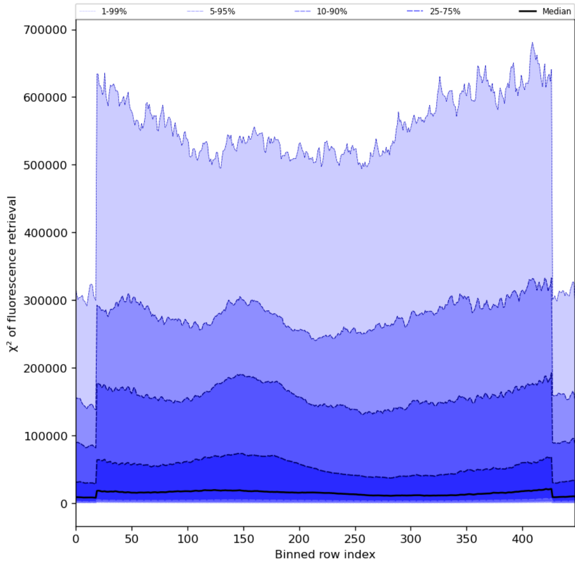
Figure 59: Along track statistics of " \chi^2 of fluorescence retrieval" for 2024-01-26 to 2024-01-28
