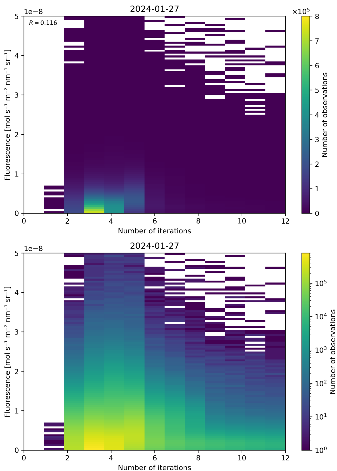
Figure 98: Scatter density plot of “Number of iterations” against “Fluorescence” for 2024-01-26 to 2024-01-28.
