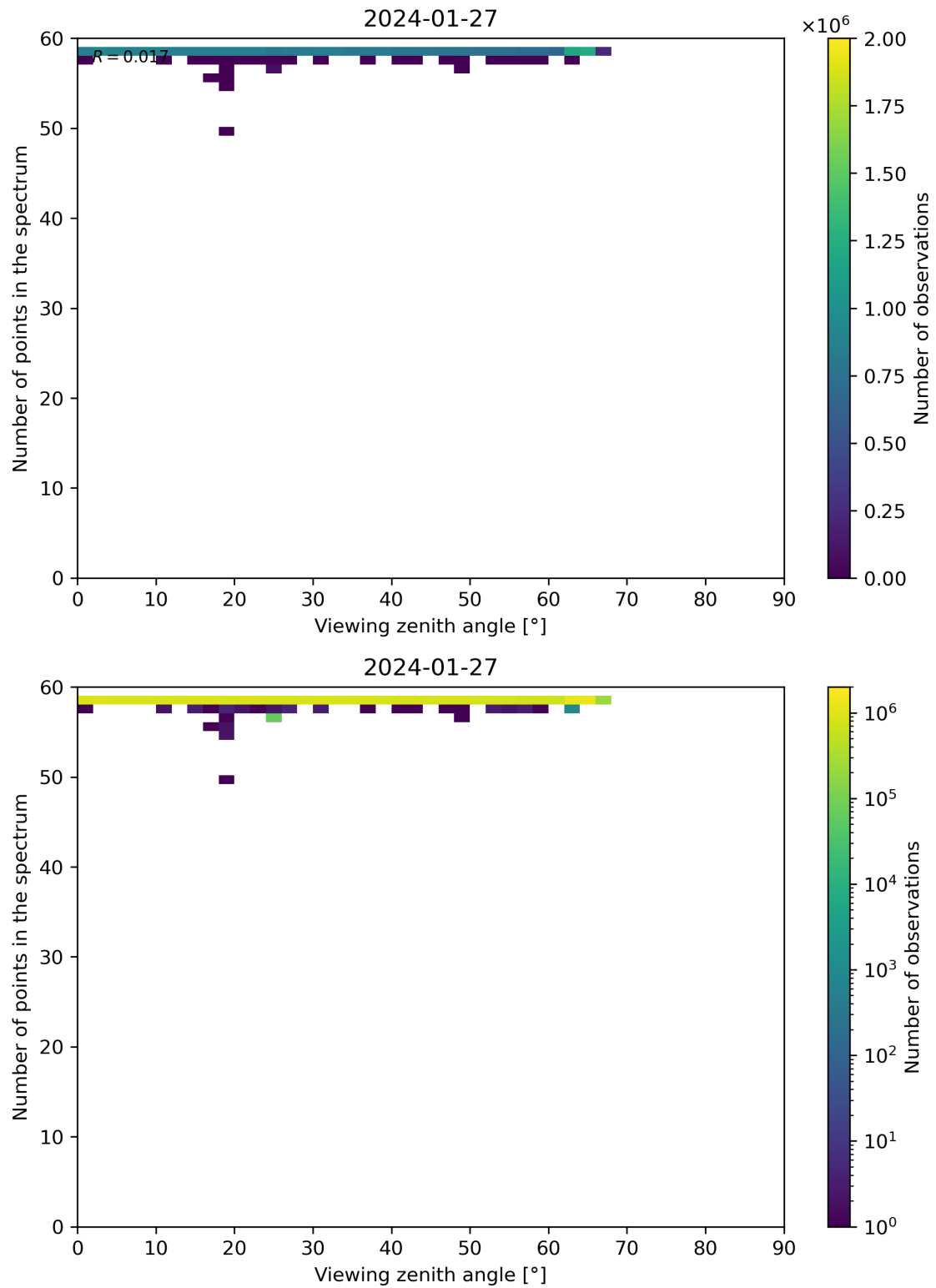
Figure 125: Scatter density plot of “Viewing zenith angle” against “Number of points in the spectrum” for 2024-01-26 to 2024-01-28.
