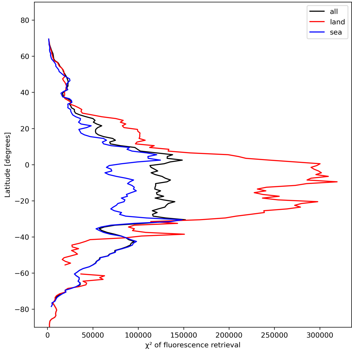
Figure 25: Zonal average of “ \chi^2 of fluorescence retrieval” for 2024-01-26 to 2024-01-28.
