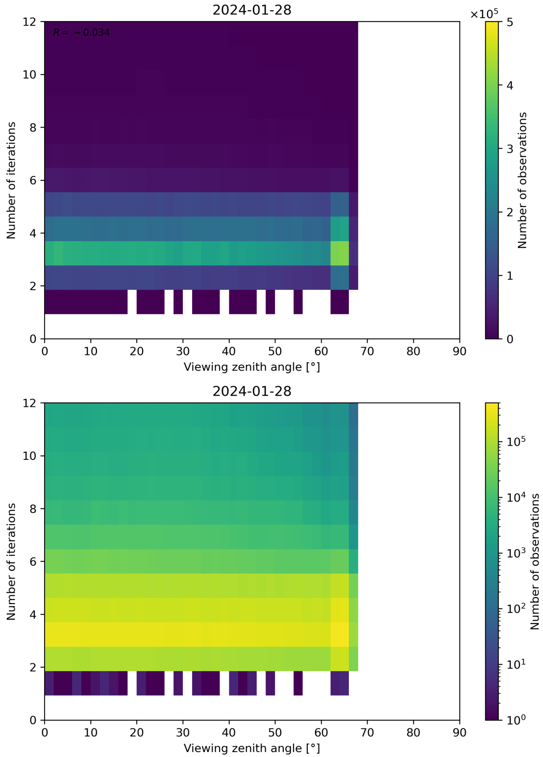
Figure 124: Scatter density plot of “Viewing zenith angle” against “Number of iterations” for 2024-01-27 to 2024-01-29.
