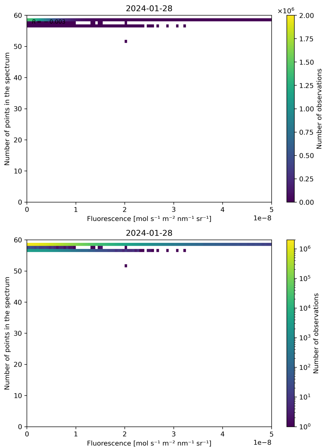
Figure 86: Scatter density plot of “Fluorescence” against “Number of points in the spectrum” for 2024-01-27 to 2024-01-29.
