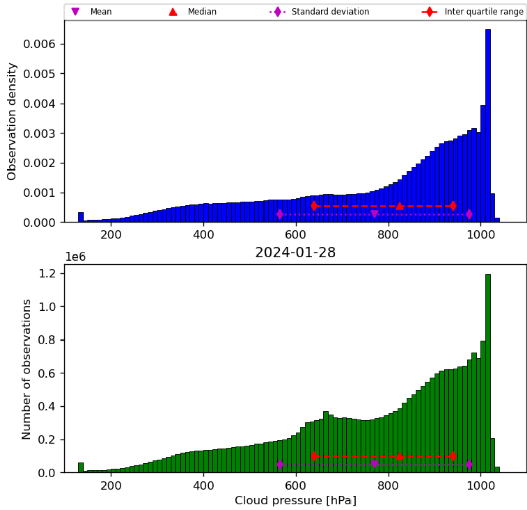
Figure 30: Histogram of “Cloud pressure” for 2024-01-27 to 2024-01-29
