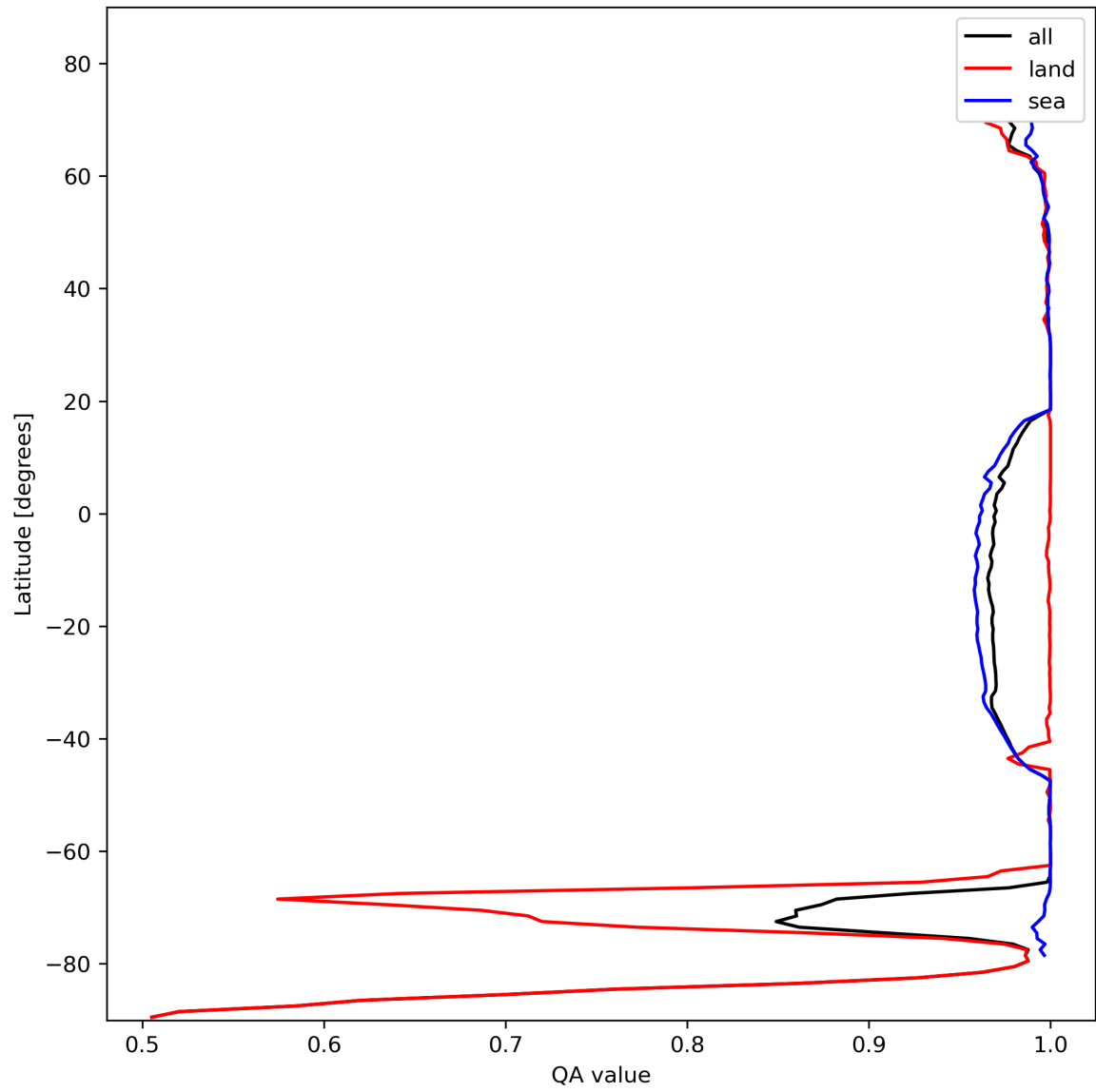
Figure 12: Zonal average of “QA value” for 2024-01-27 to 2024-01-29.
