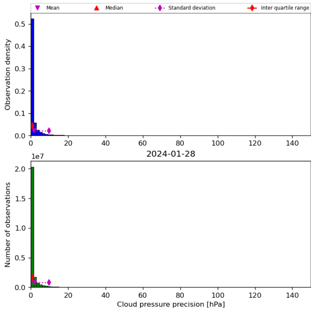
Figure 31: Histogram of “Cloud pressure precision” for 2024-01-27 to 2024-01-29
