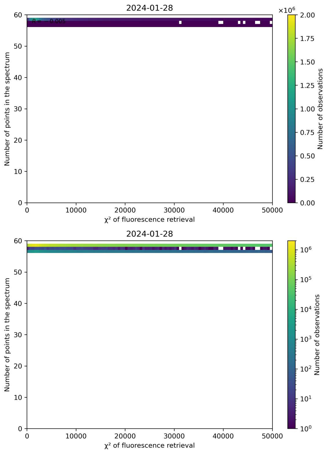
Figure 68: Scatter density plot of " \chi^2 of fluorescence retrieval" against "Number of points in the spectrum" for 2024-01-27 to 2024-01-29.
