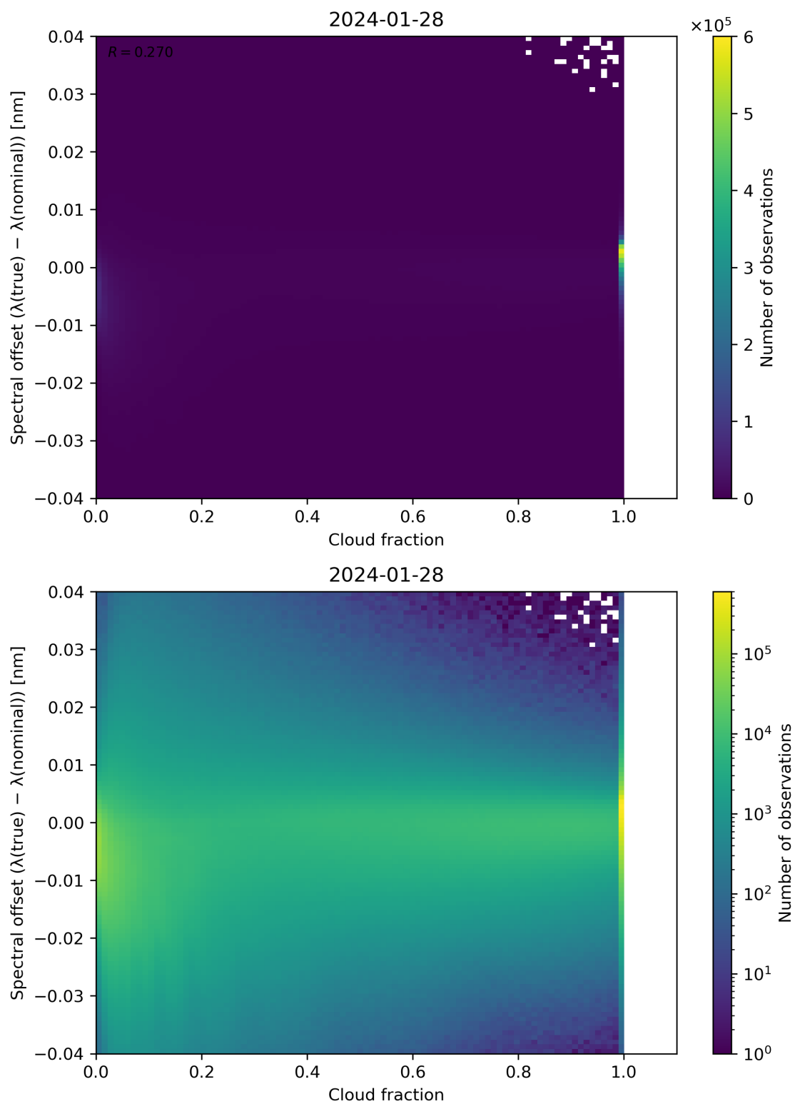
Figure 76: Scatter density plot of “Cloud fraction” against “Spectral offset ( \lambda(\text{true}) - \lambda(\text{nominal}) )” for 2024-01-27 to 2024-01-29.
