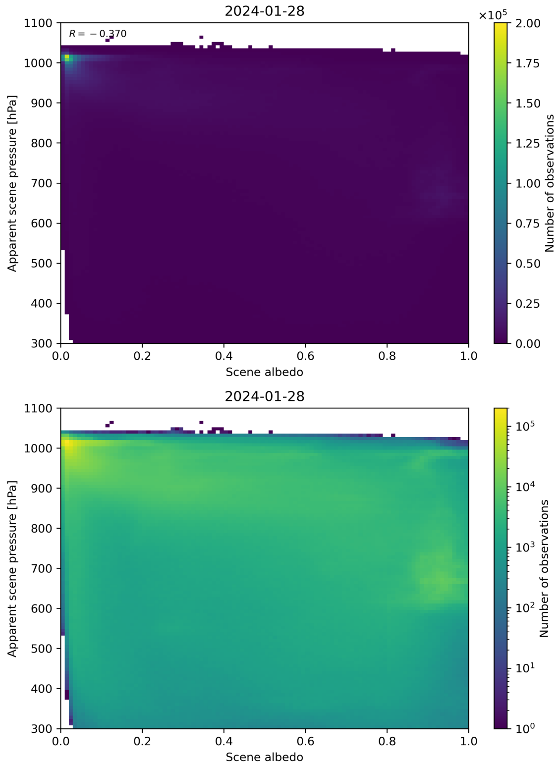
Figure 102: Scatter density plot of “Scene albedo” against “Apparent scene pressure” for 2024-01-27 to 2024-01-29.
