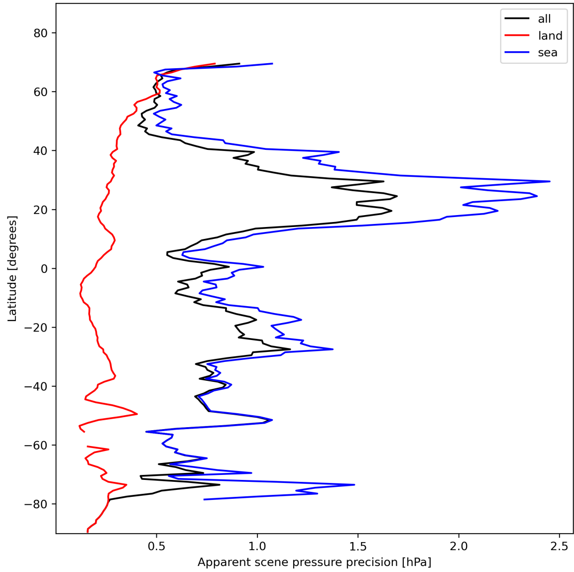
Figure 20: Zonal average of “Apparent scene pressure precision” for 2024-01-27 to 2024-01-29.
