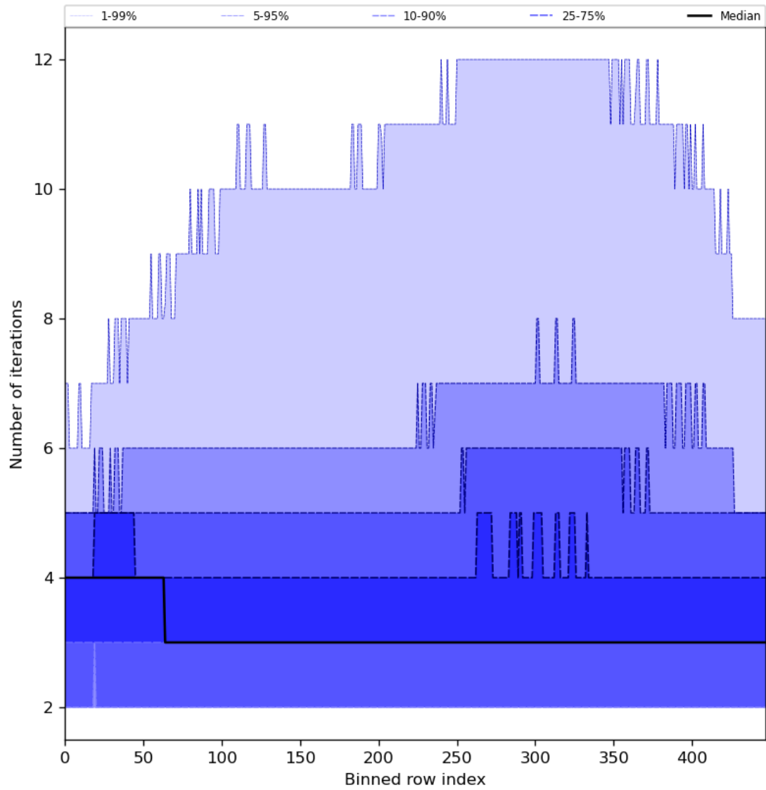
Figure 56: Along track statistics of “Number of iterations” for 2024-01-27 to 2024-01-29
