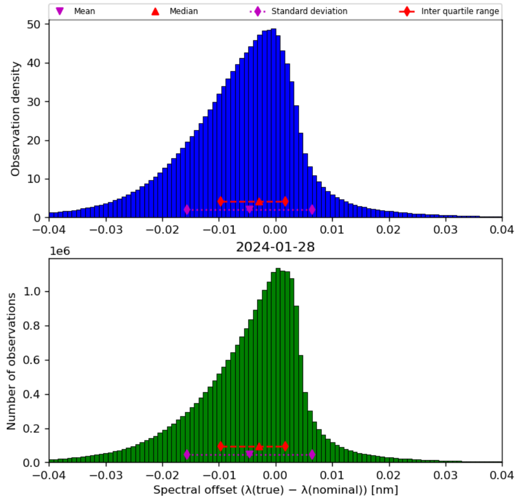
Figure 45: Histogram of “Spectral offset ( \lambda(\text{true}) - \lambda(\text{nominal}) )” for 2024-01-27 to 2024-01-29
