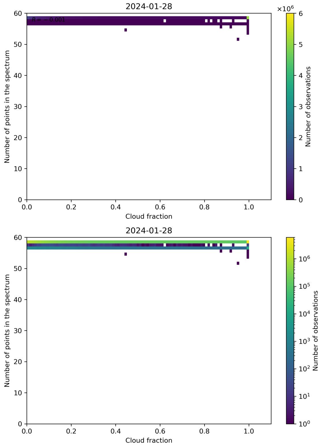
Figure 74: Scatter density plot of “Cloud fraction” against “Number of points in the spectrum” for 2024-01-27 to 2024-01-29.
