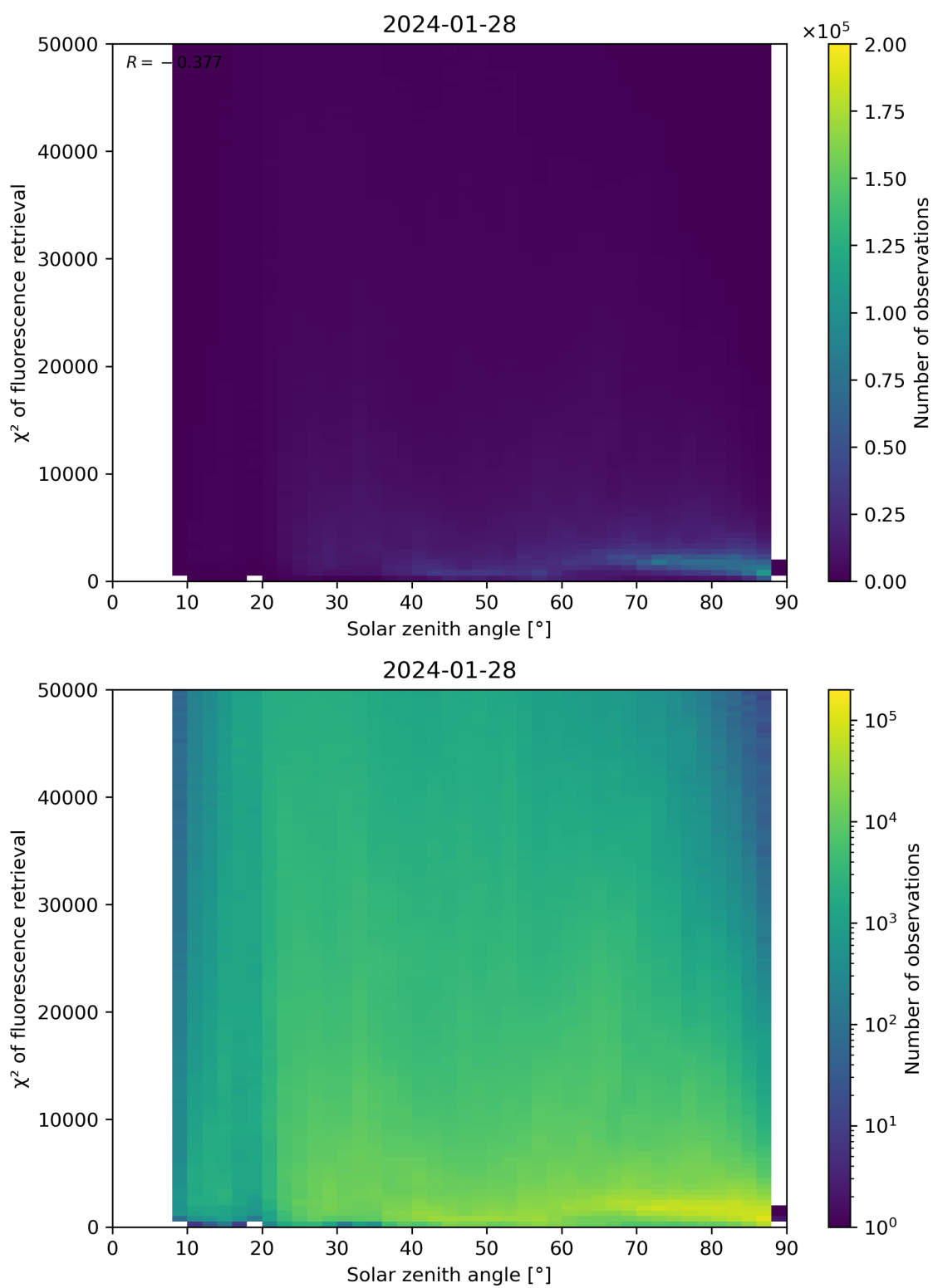
Figure 109: Scatter density plot of “Solar zenith angle” against “ \chi^2 of fluorescence retrieval” for 2024-01-27 to 2024-01-29.
