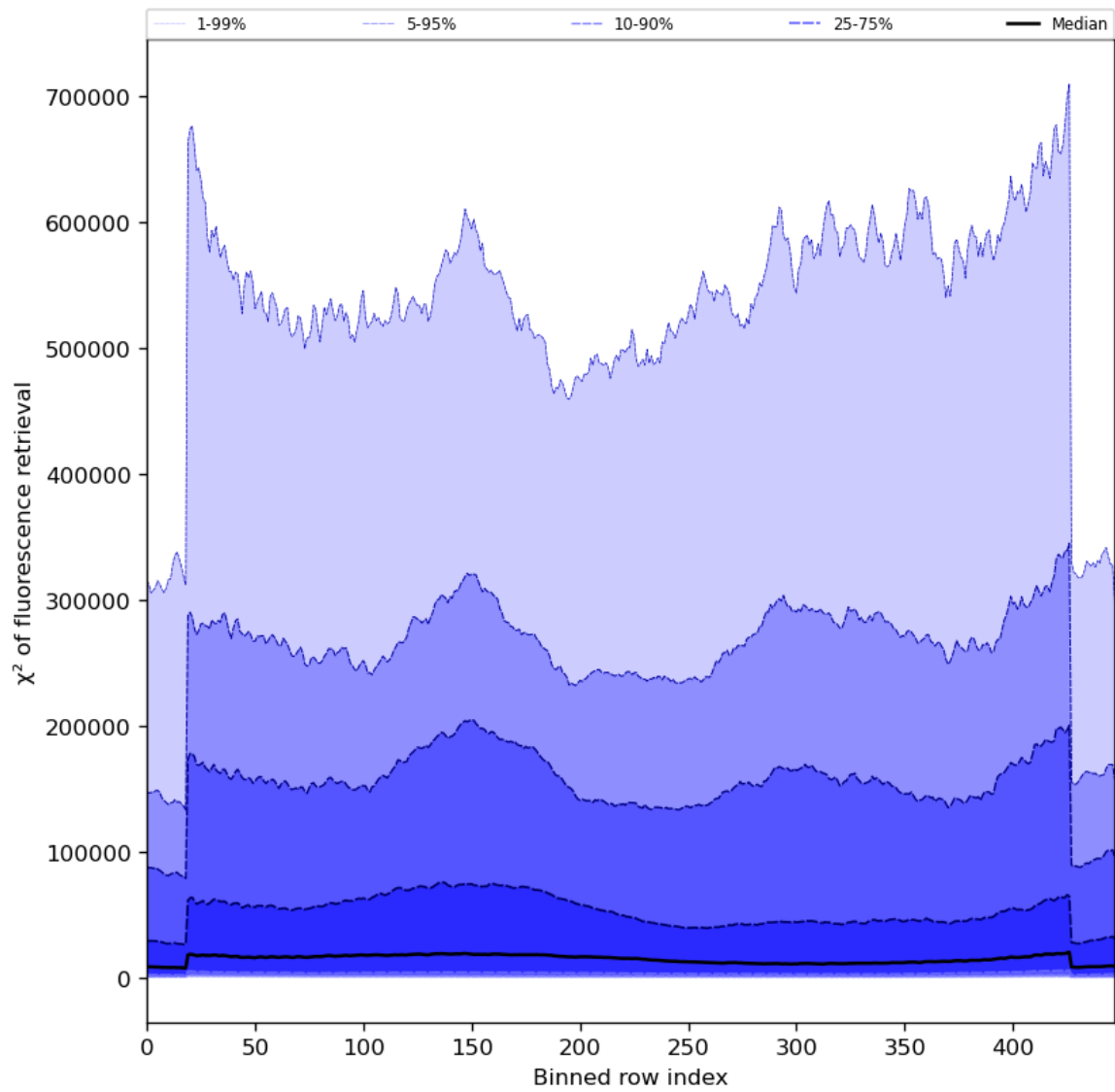
Figure 59: Along track statistics of “ \chi^2 of fluorescence retrieval” for 2024-01-27 to 2024-01-29
