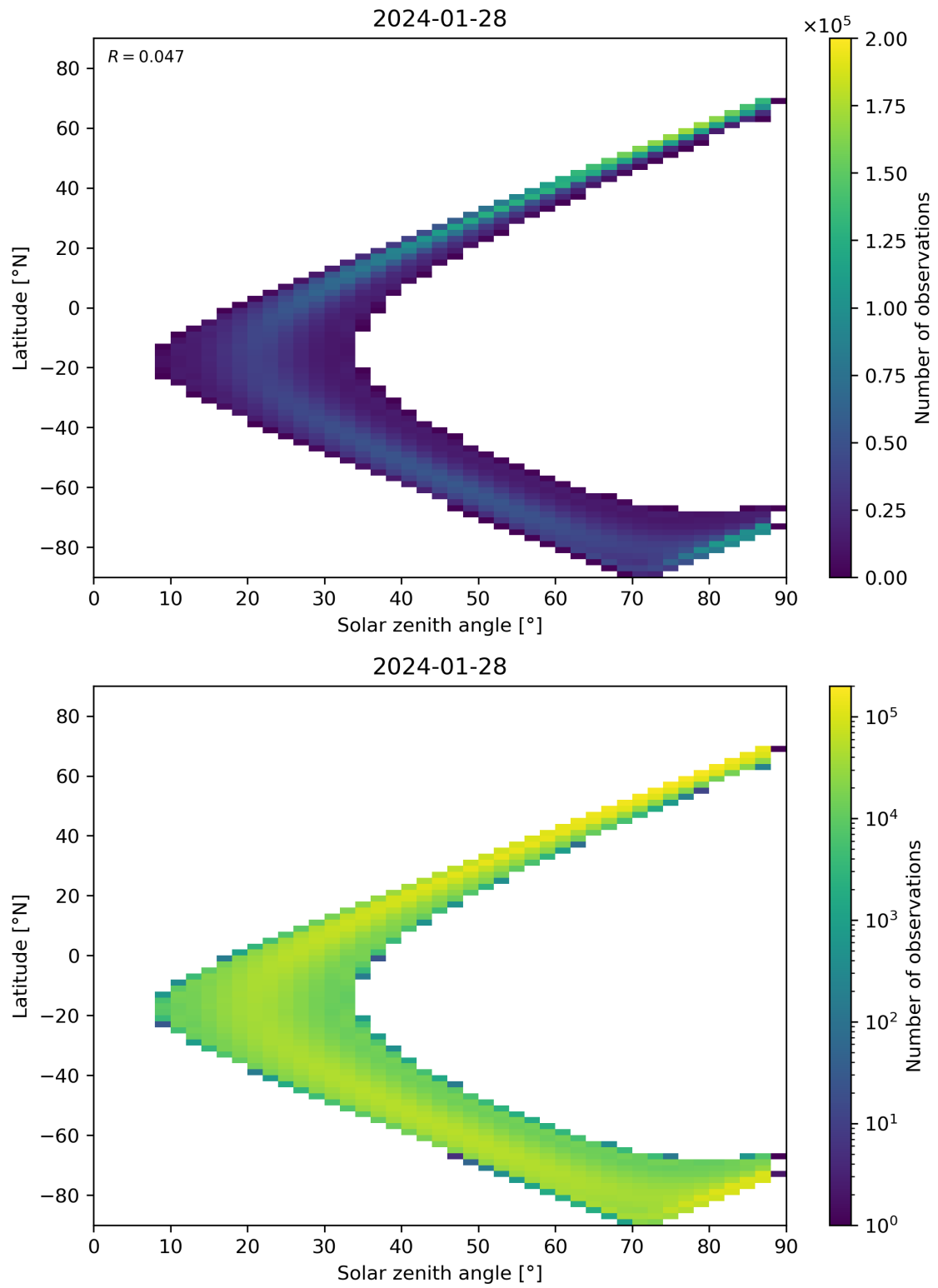
Figure 113: Scatter density plot of “Solar zenith angle” against “Latitude” for 2024-01-27 to 2024-01-29.
