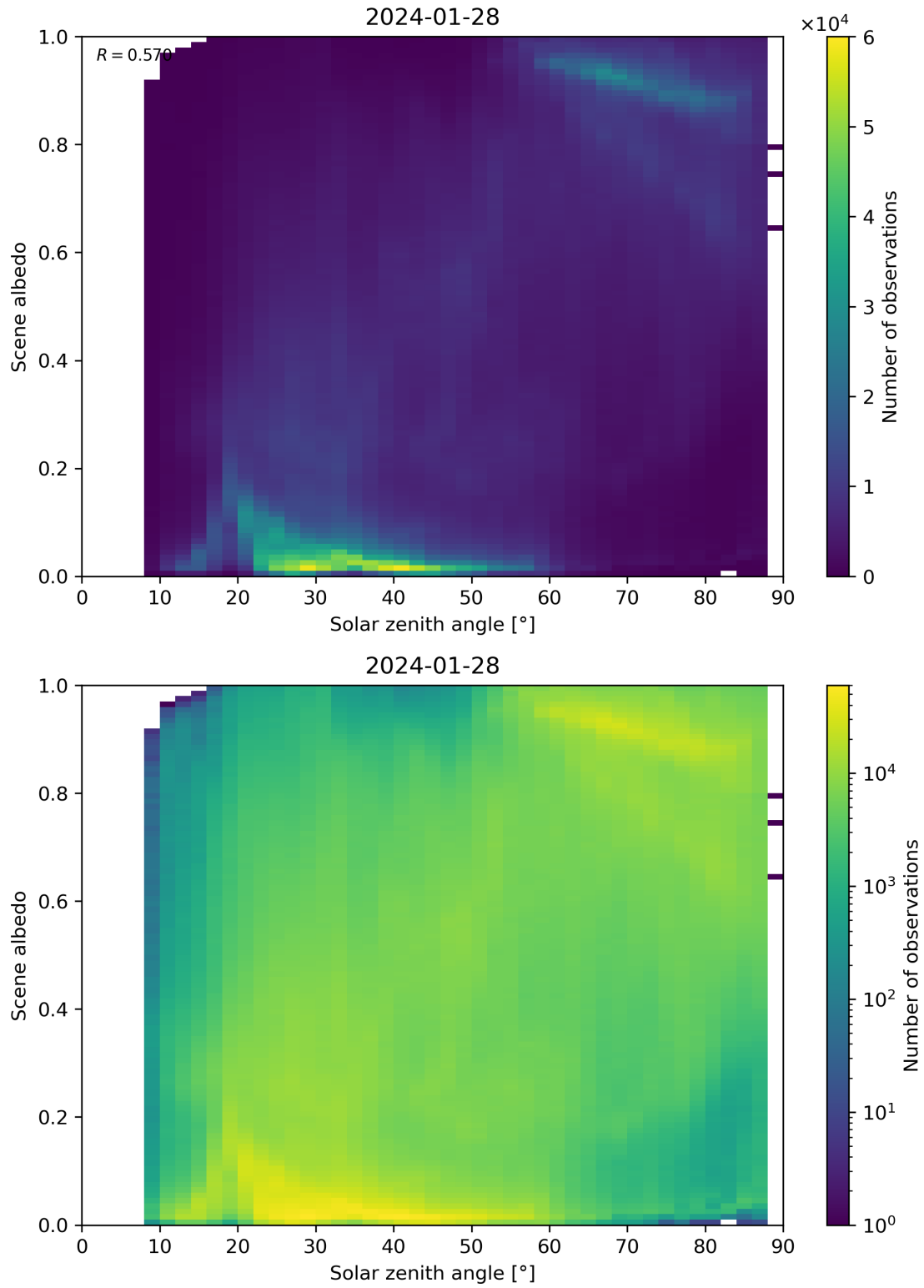
Figure 116: Scatter density plot of “Solar zenith angle” against “Scene albedo” for 2024-01-27 to 2024-01-29.
