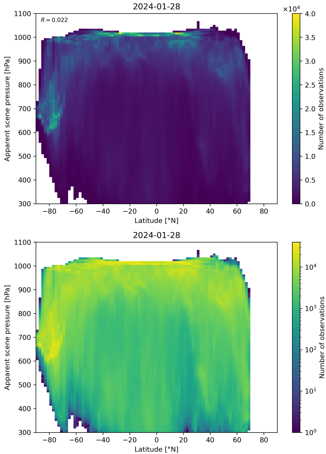
Figure 88: Scatter density plot of “Latitude” against “Apparent scene pressure” for 2024-01-27 to 2024-01-29.
