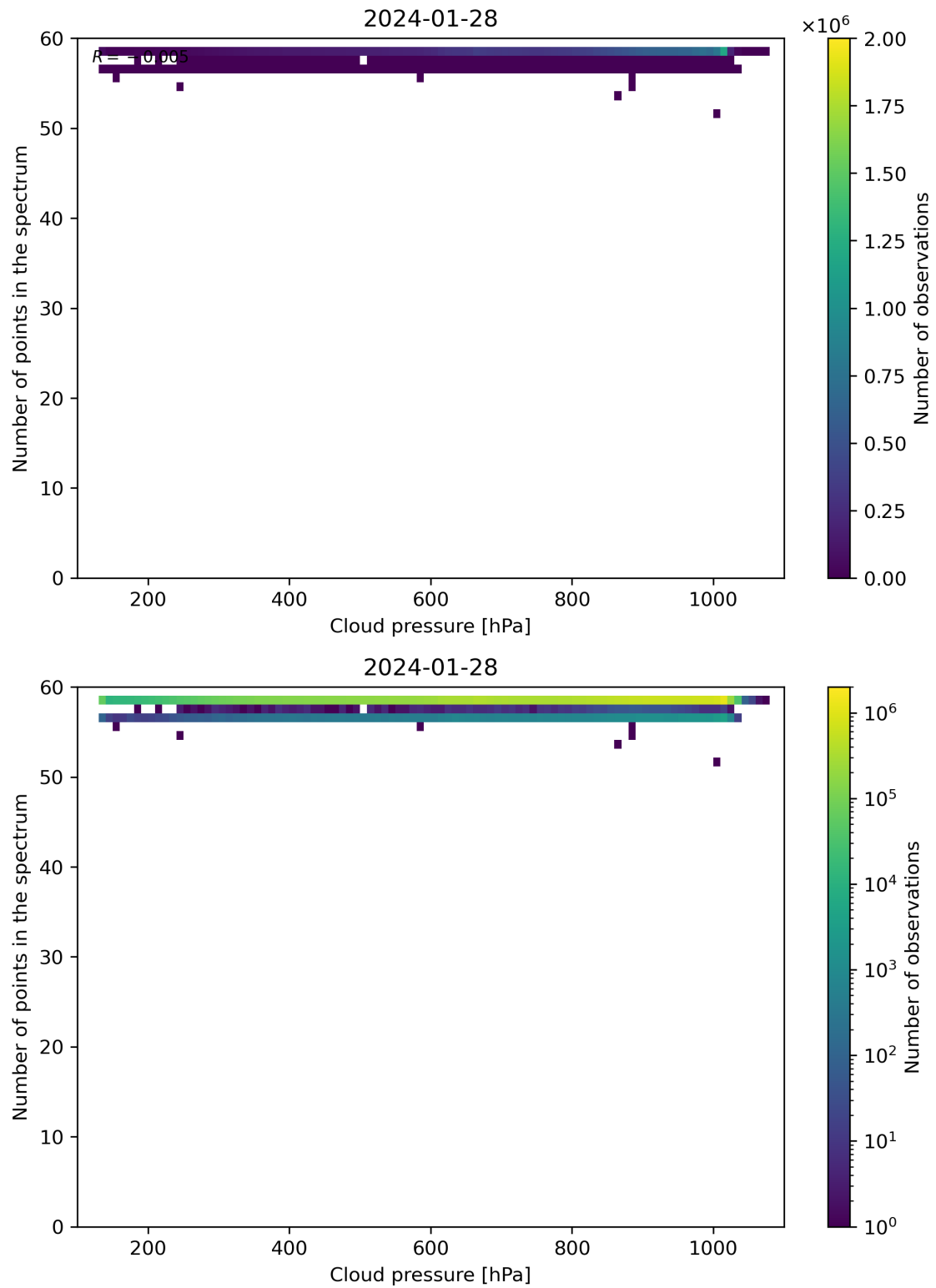
Figure 82: Scatter density plot of “Cloud pressure” against “Number of points in the spectrum” for 2024-01-27 to 2024-01-29.
