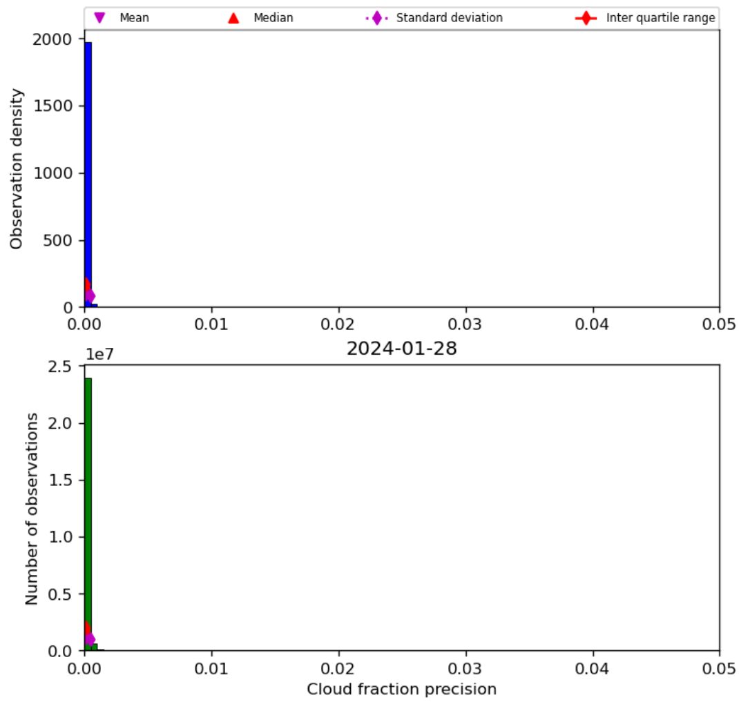
Figure 33: Histogram of “Cloud fraction precision” for 2024-01-27 to 2024-01-29
