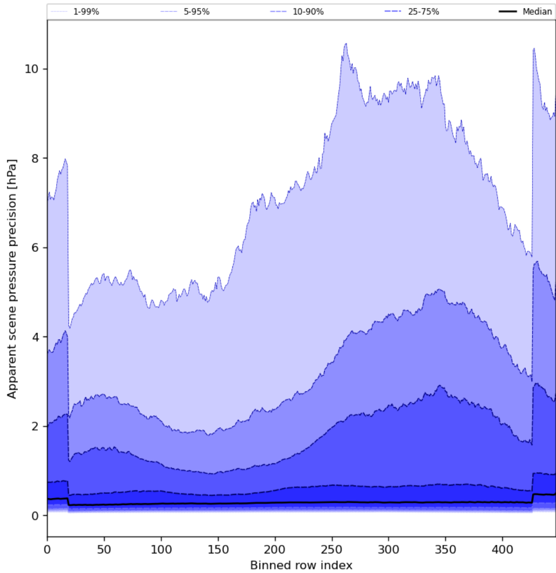
Figure 54: Along track statistics of “Apparent scene pressure precision” for 2024-01-27 to 2024-01-29
