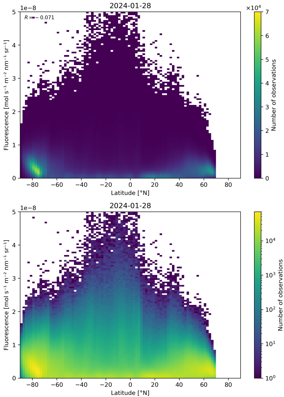
Figure 92: Scatter density plot of “Latitude” against “Fluorescence” for 2024-01-27 to 2024-01-29.
