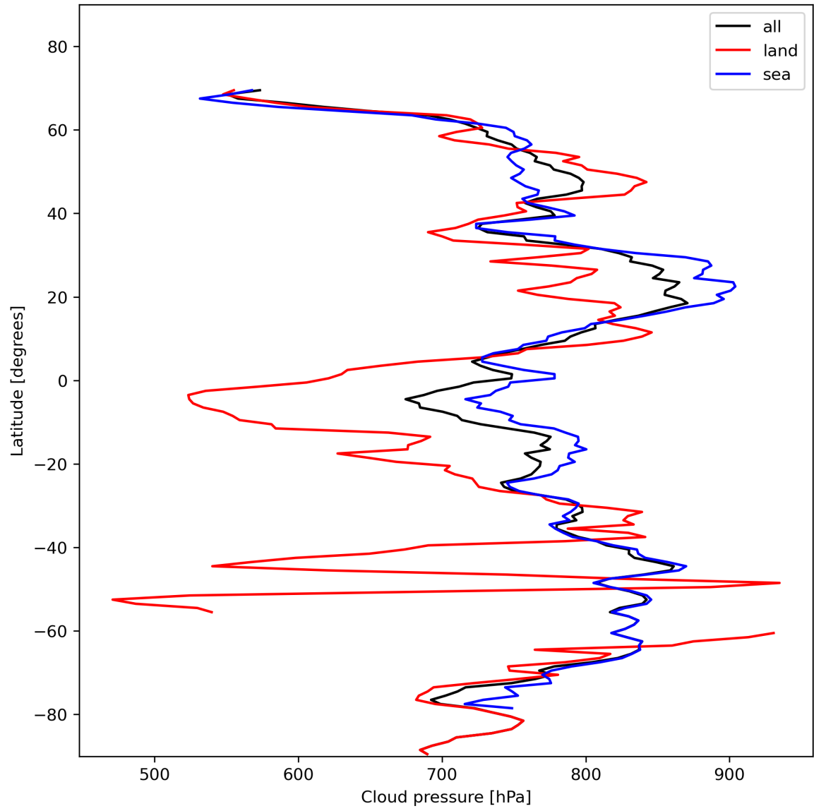
Figure 13: Zonal average of “Cloud pressure” for 2024-01-27 to 2024-01-29.
