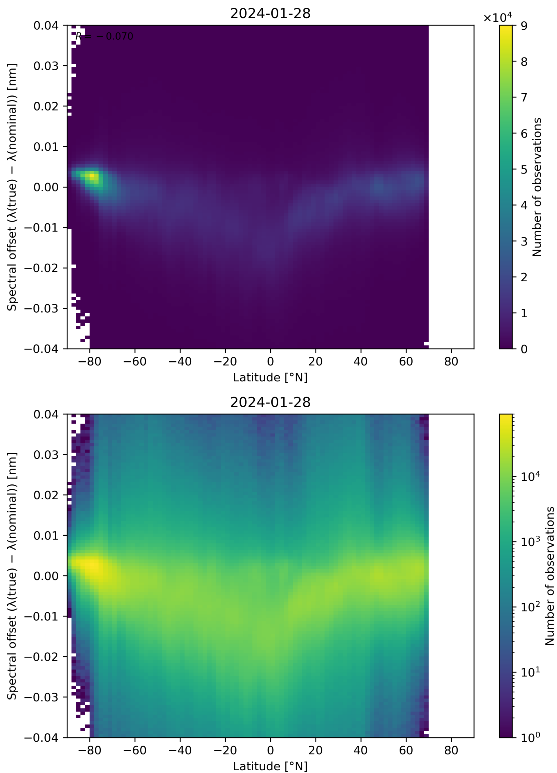
Figure 96: Scatter density plot of “Latitude” against “Spectral offset ( \lambda(\text{true}) - \lambda(\text{nominal}) )” for 2024-01-27 to 2024-01-29.
