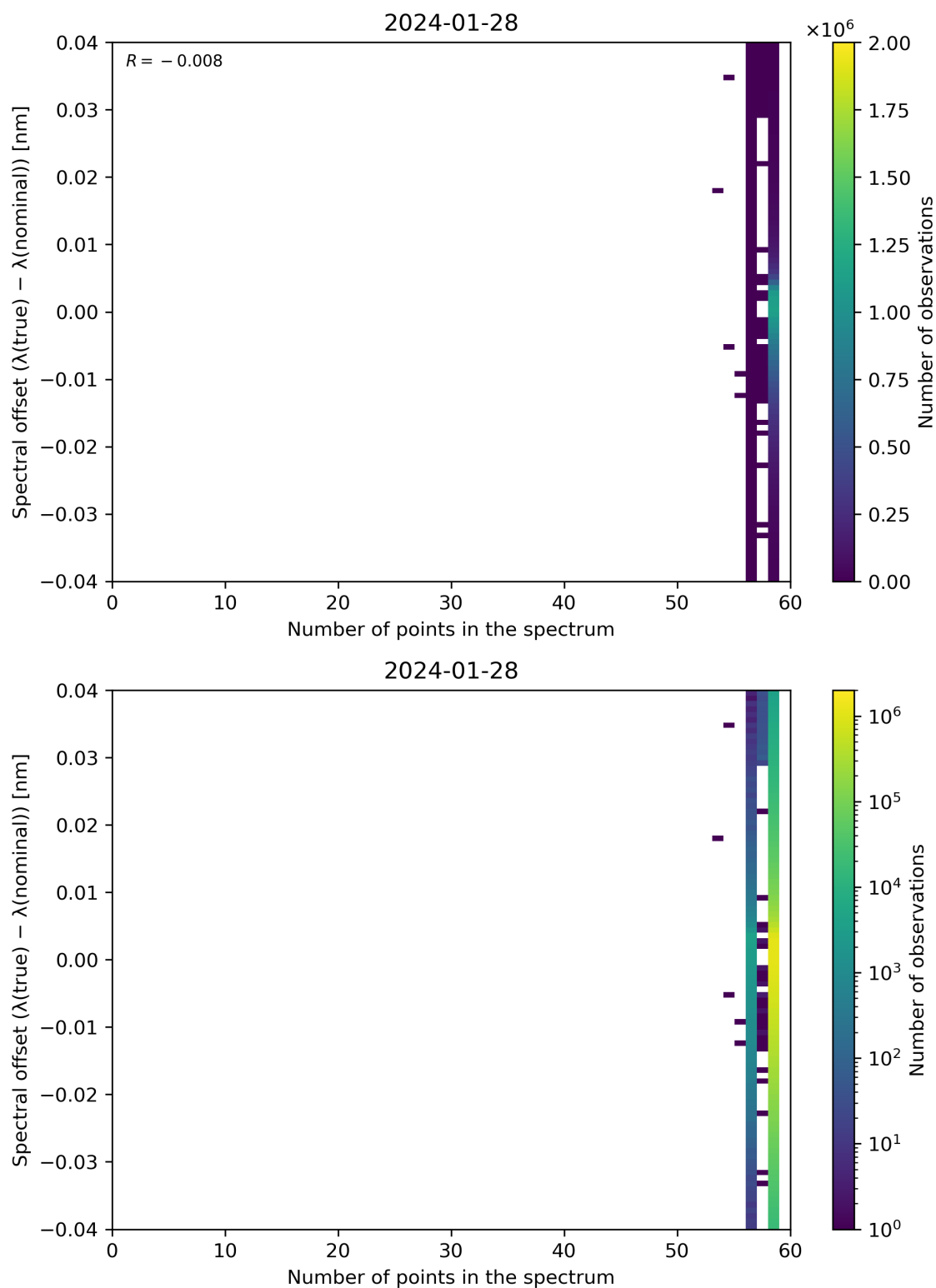
Figure 101: Scatter density plot of “Number of points in the spectrum” against “Spectral offset ( \lambda(\text{true}) - \lambda(\text{nominal}) )” for 2024-01-27 to 2024-01-29.
