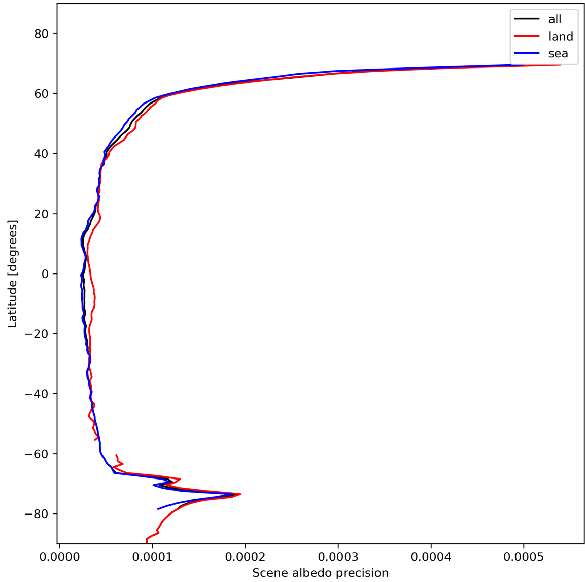
Figure 18: Zonal average of “Scene albedo precision” for 2024-01-27 to 2024-01-29.
