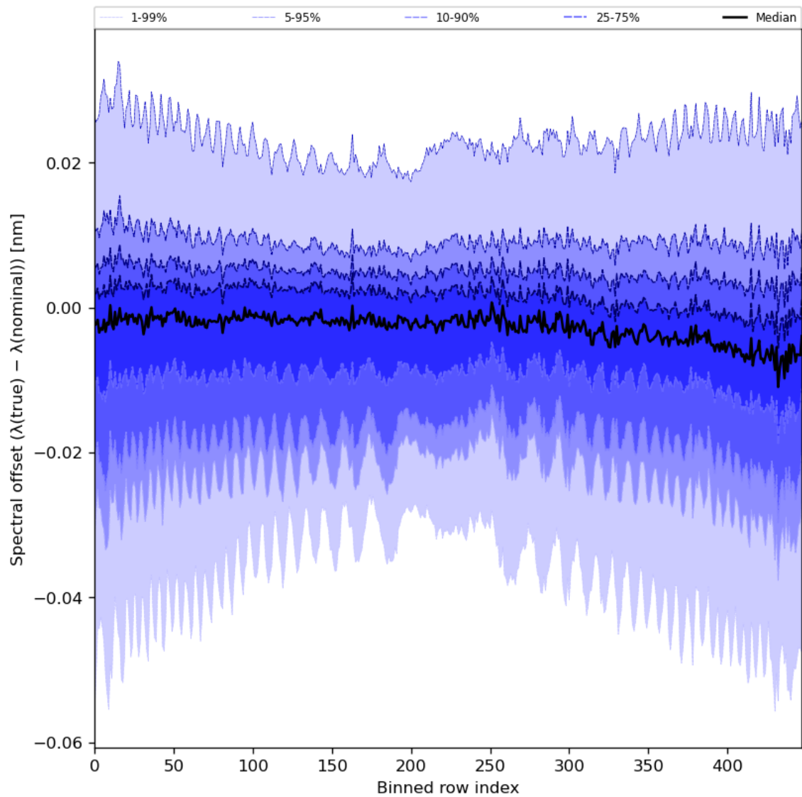
Figure 62: Along track statistics of “Spectral offset ( \lambda(\text{true}) - \lambda(\text{nominal}) )” for 2024-01-27 to 2024-01-29
