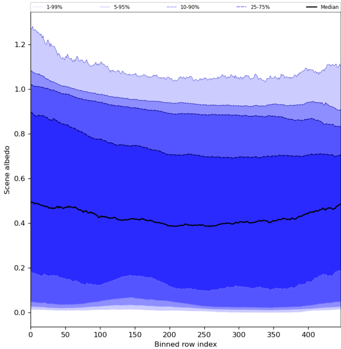
Figure 51: Along track statistics of “Scene albedo” for 2024-01-27 to 2024-01-29
