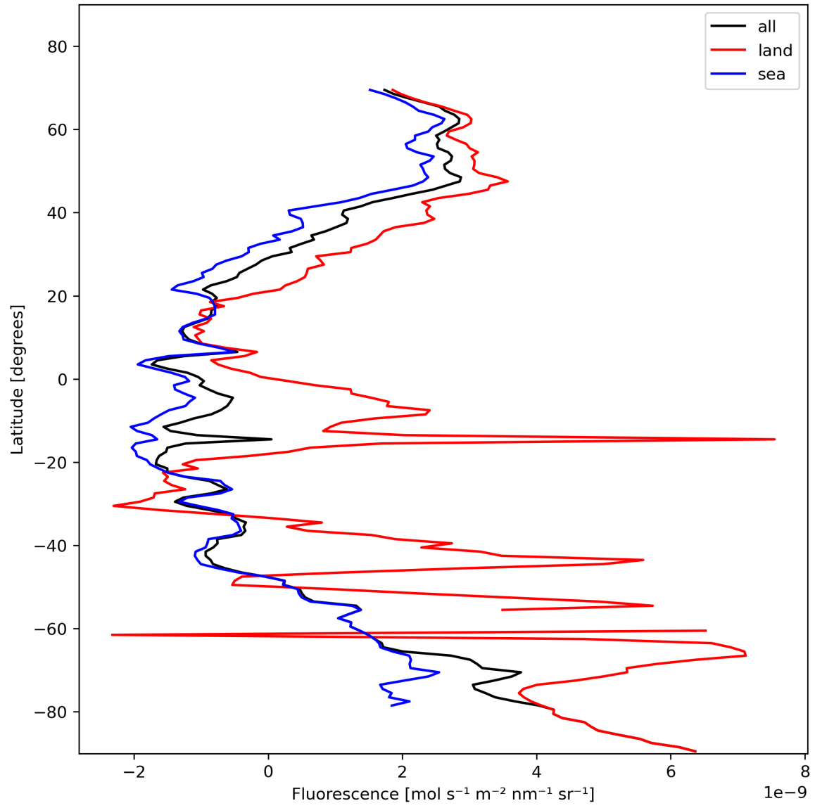
Figure 23: Zonal average of “Fluorescence” for 2024-01-27 to 2024-01-29.
