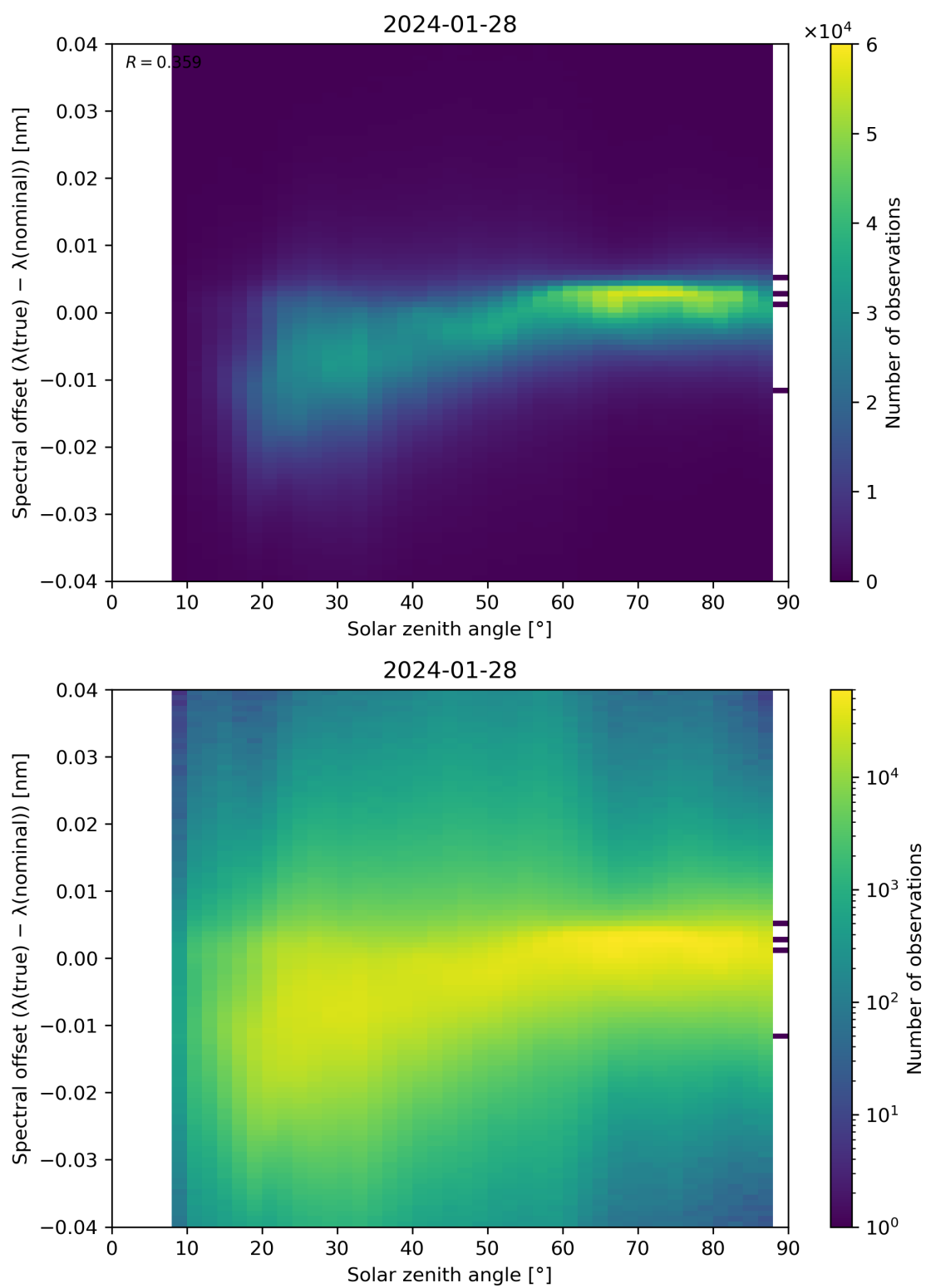
Figure 117: Scatter density plot of “Solar zenith angle” against “Spectral offset ( \lambda(\text{true}) - \lambda(\text{nominal}) )” for 2024-01-27 to 2024-01-29.
