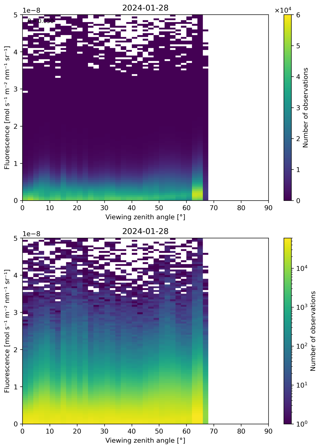
Figure 122: Scatter density plot of “Viewing zenith angle” against “Fluorescence” for 2024-01-27 to 2024-01-29.
