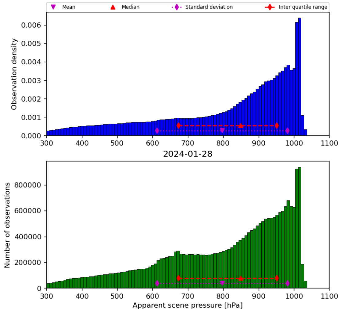
Figure 36: Histogram of “Apparent scene pressure” for 2024-01-27 to 2024-01-29
