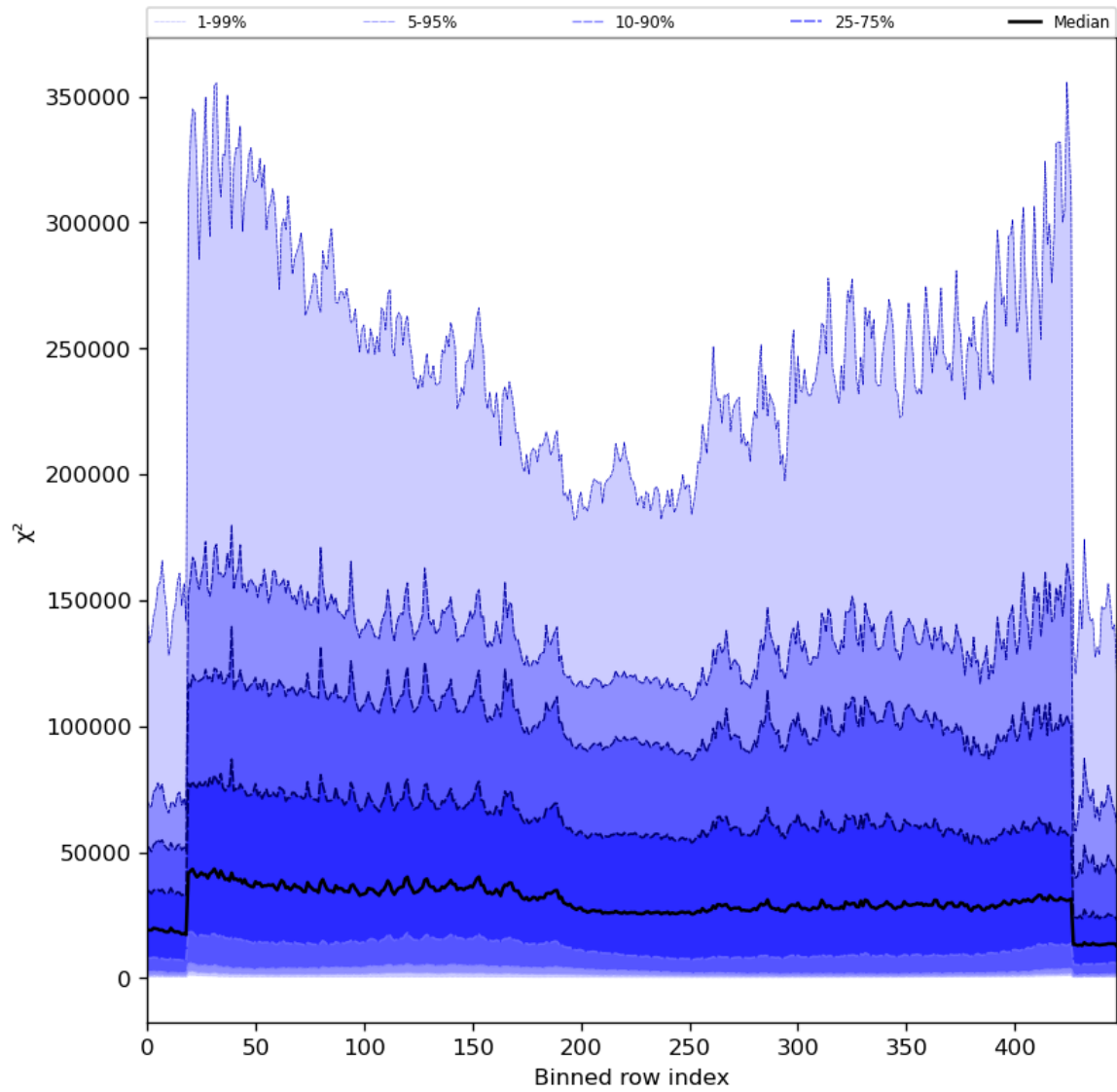
Figure 55: Along track statistics of “ \chi^2 ” for 2024-01-27 to 2024-01-29
