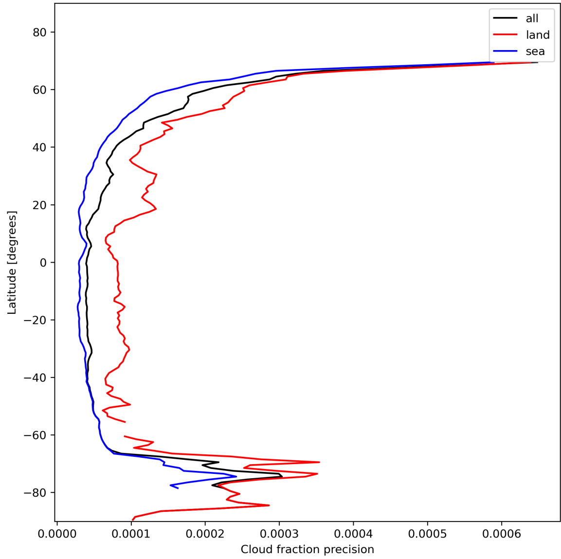
Figure 16: Zonal average of “Cloud fraction precision” for 2024-01-27 to 2024-01-29.
