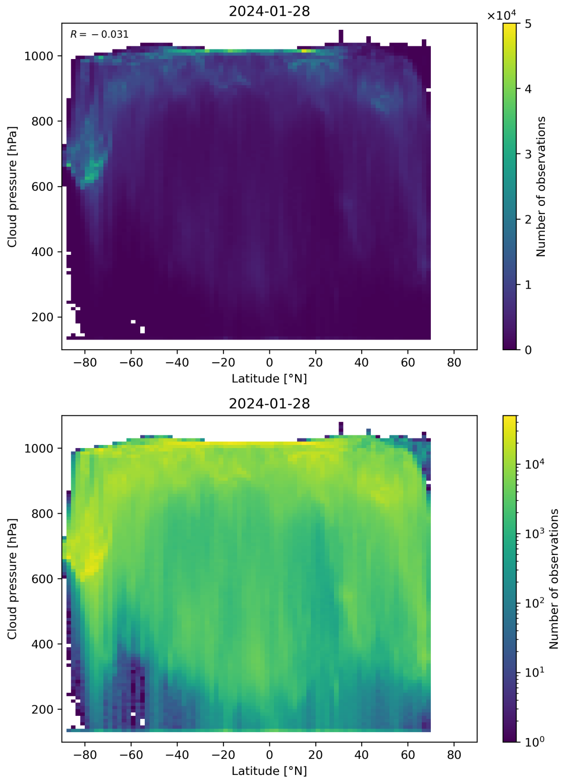
Figure 91: Scatter density plot of “Latitude” against “Cloud pressure” for 2024-01-27 to 2024-01-29.
