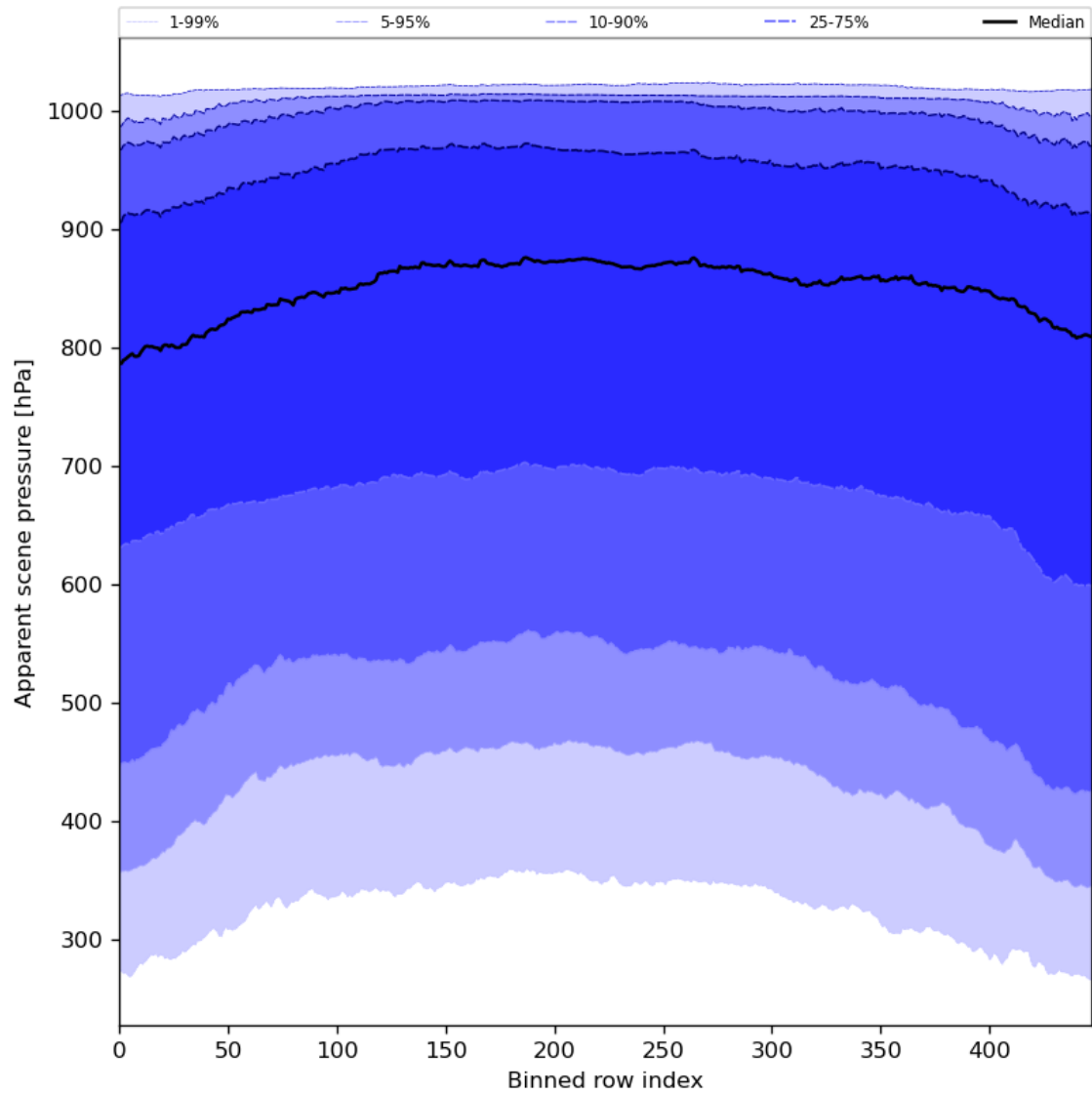
Figure 53: Along track statistics of “Apparent scene pressure” for 2024-01-27 to 2024-01-29
