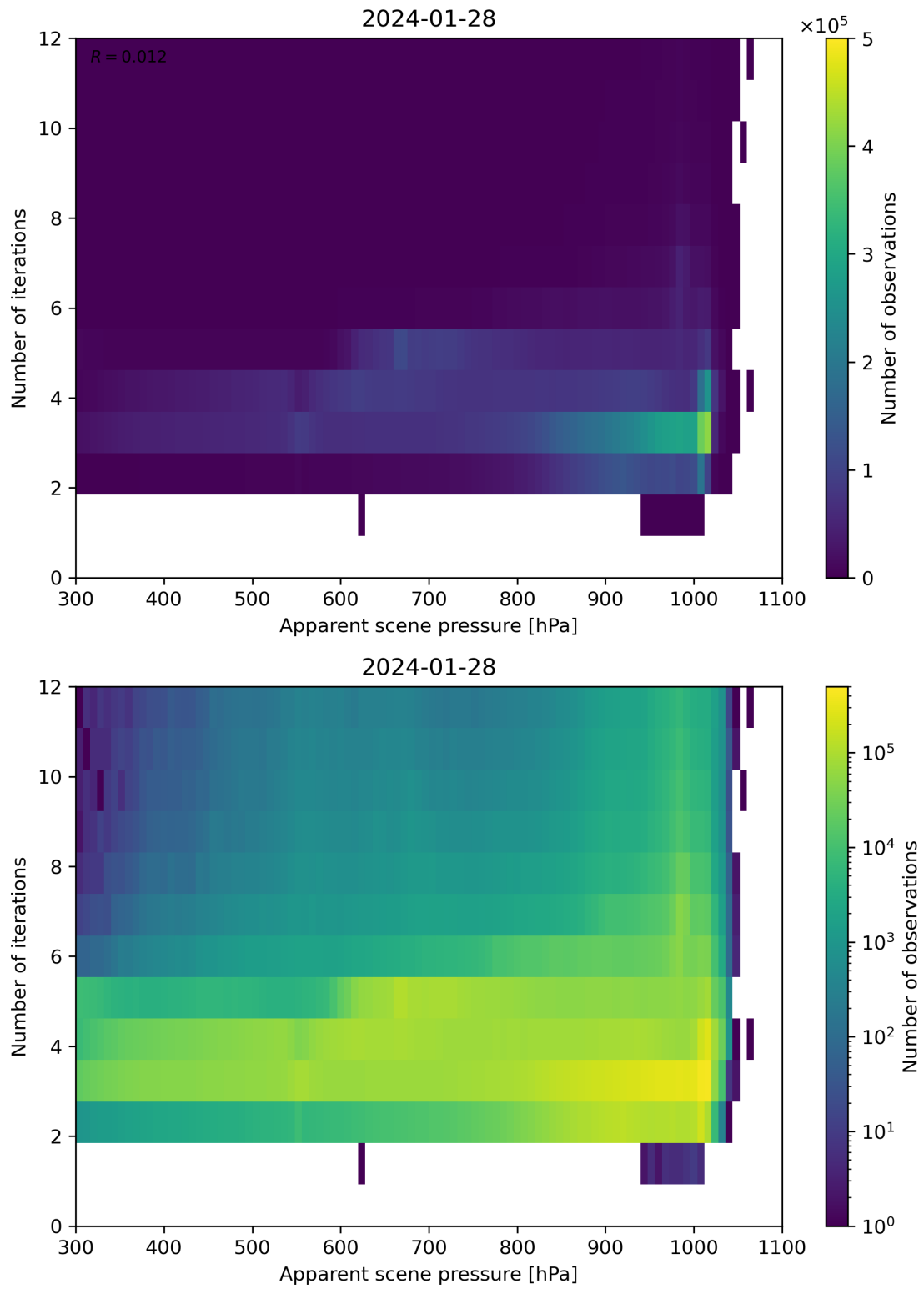
Figure 65: Scatter density plot of “Apparent scene pressure” against “Number of iterations” for 2024-01-27 to 2024-01-29.
