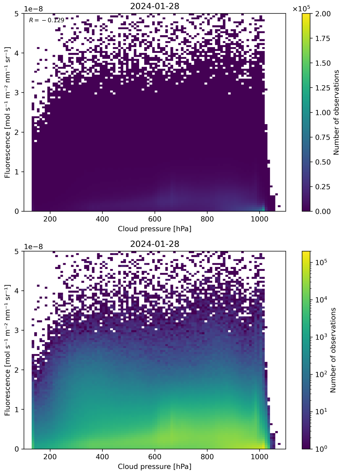
Figure 80: Scatter density plot of “Cloud pressure” against “Fluorescence” for 2024-01-27 to 2024-01-29.
