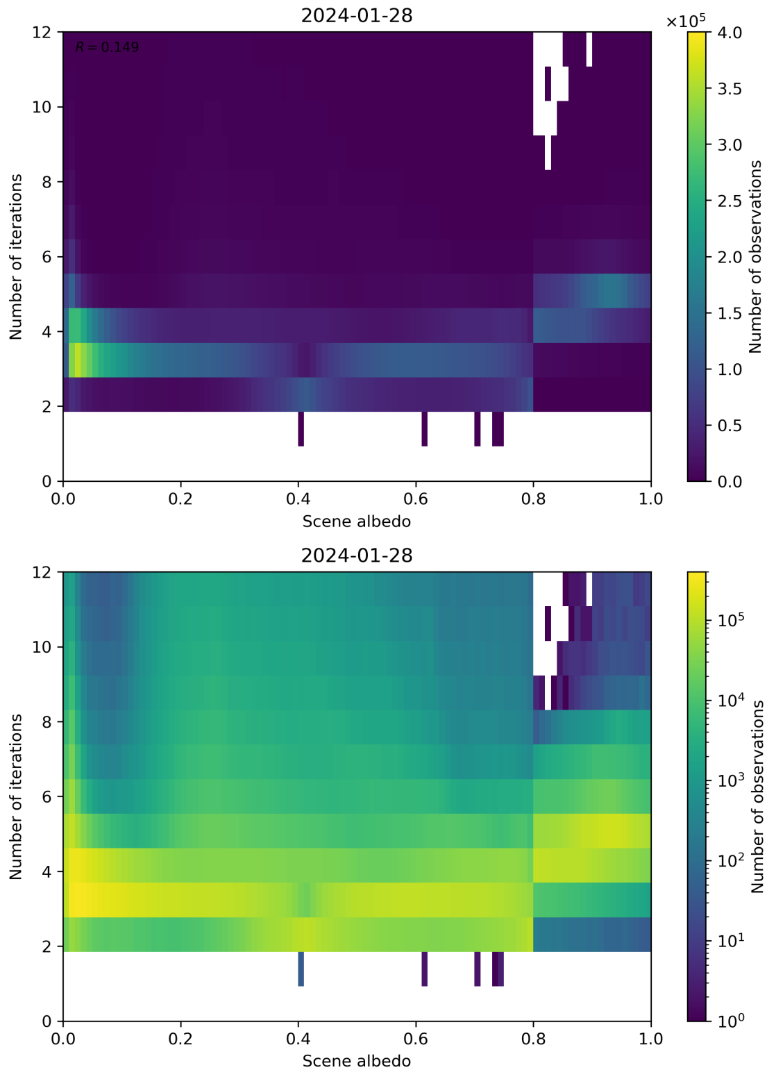
Figure 105: Scatter density plot of “Scene albedo” against “Number of iterations” for 2024-01-27 to 2024-01-29.
