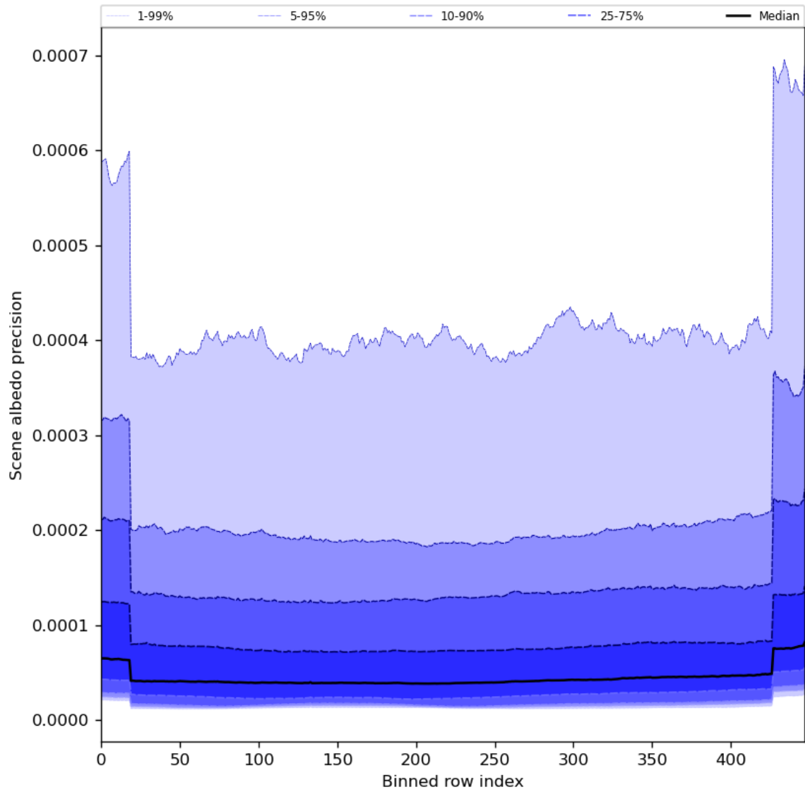
Figure 52: Along track statistics of “Scene albedo precision” for 2024-01-27 to 2024-01-29
