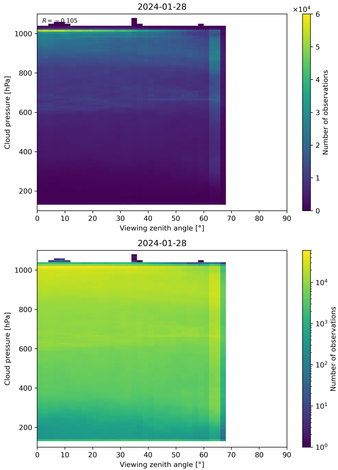
Figure 121: Scatter density plot of “Viewing zenith angle” against “Cloud pressure” for 2024-01-27 to 2024-01-29.
