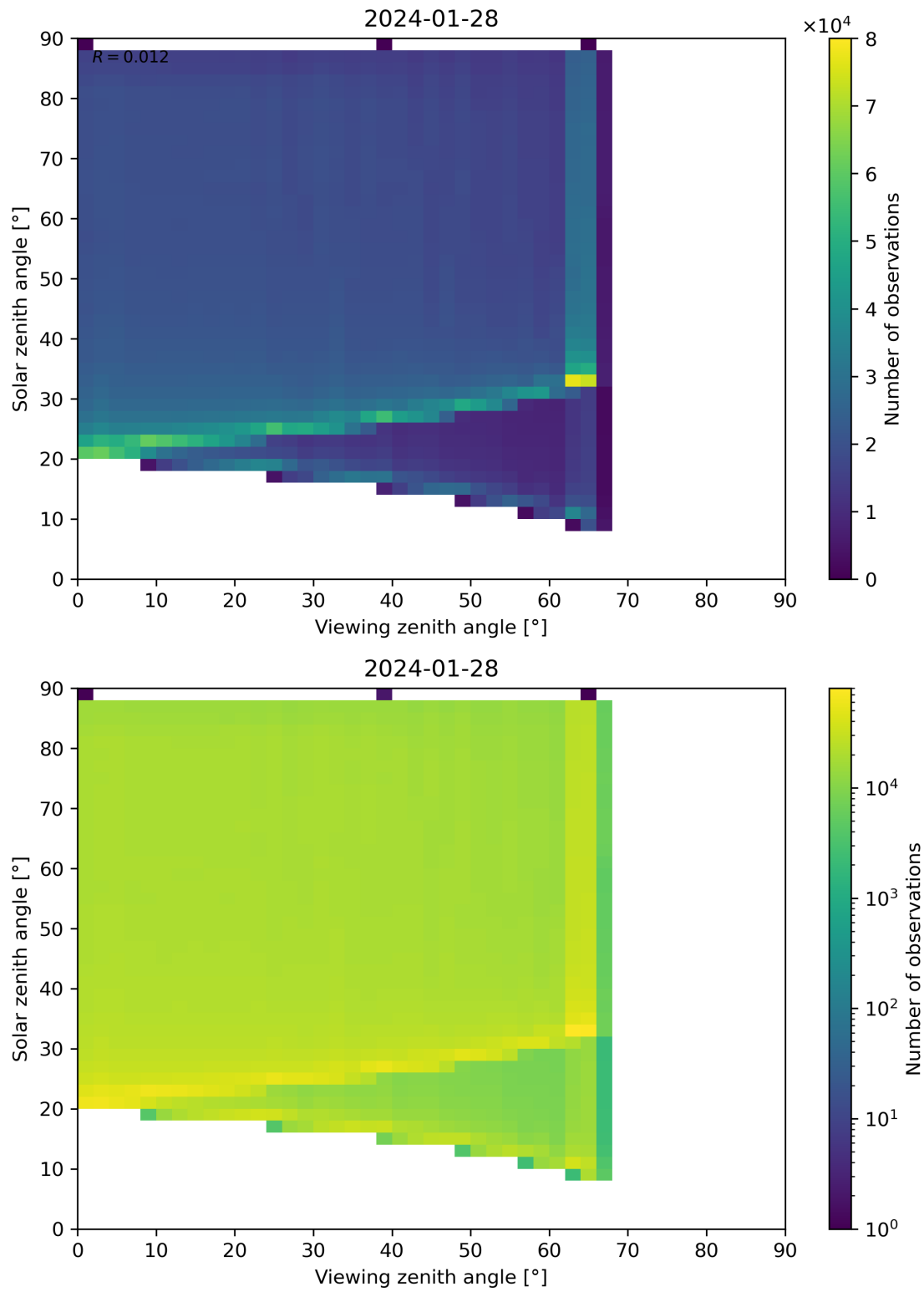
Figure 127: Scatter density plot of “Viewing zenith angle” against “Solar zenith angle” for 2024-01-27 to 2024-01-29.
