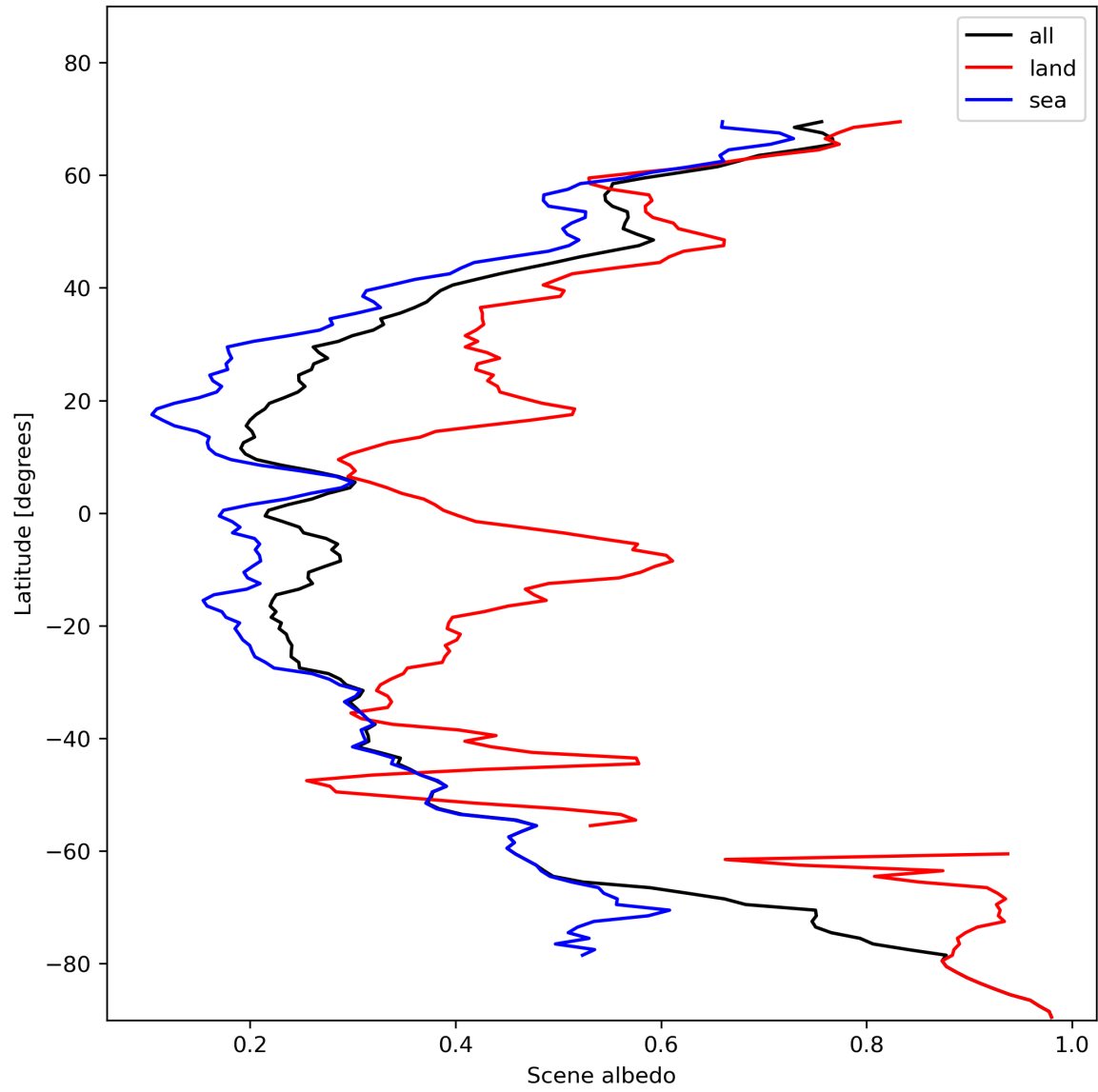
Figure 17: Zonal average of “Scene albedo” for 2024-01-27 to 2024-01-29.
