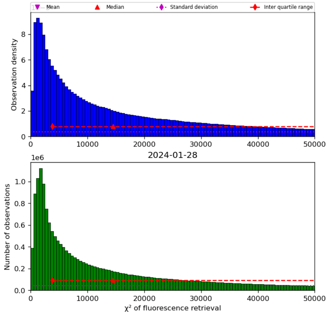
Figure 42: Histogram of “ \chi^2 of fluorescence retrieval” for 2024-01-27 to 2024-01-29
