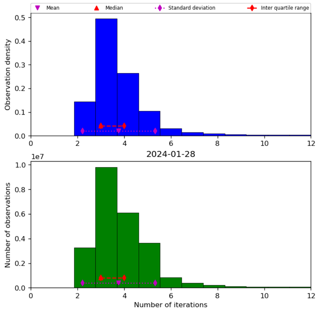
Figure 39: Histogram of “Number of iterations” for 2024-01-27 to 2024-01-29
