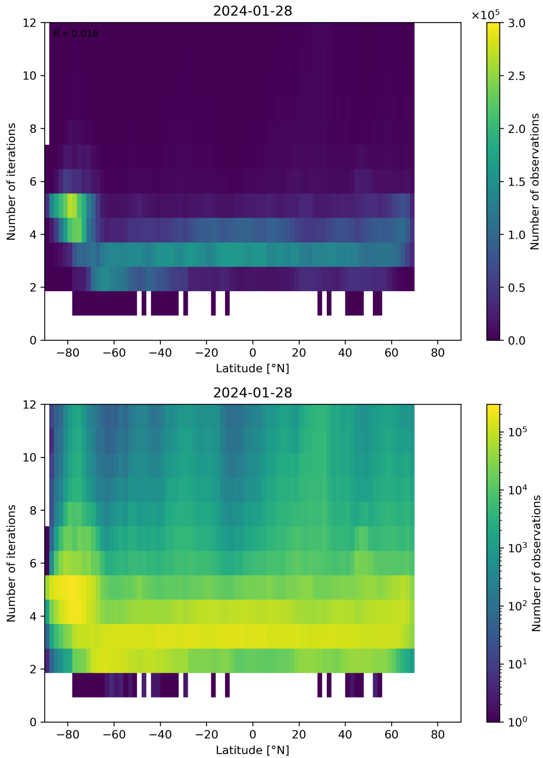
Figure 93: Scatter density plot of “Latitude” against “Number of iterations” for 2024-01-27 to 2024-01-29.
