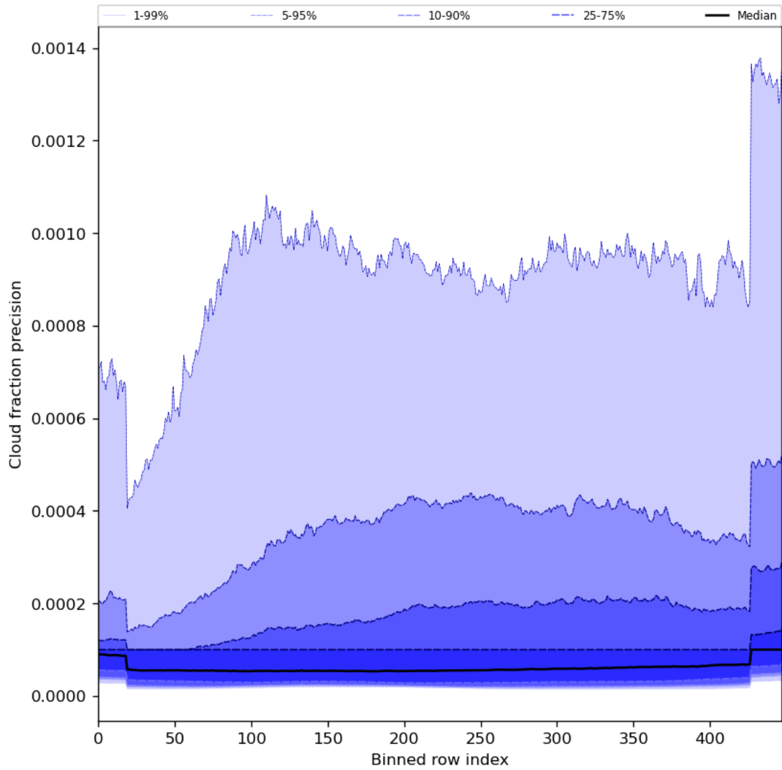
Figure 50: Along track statistics of “Cloud fraction precision” for 2024-01-27 to 2024-01-29
