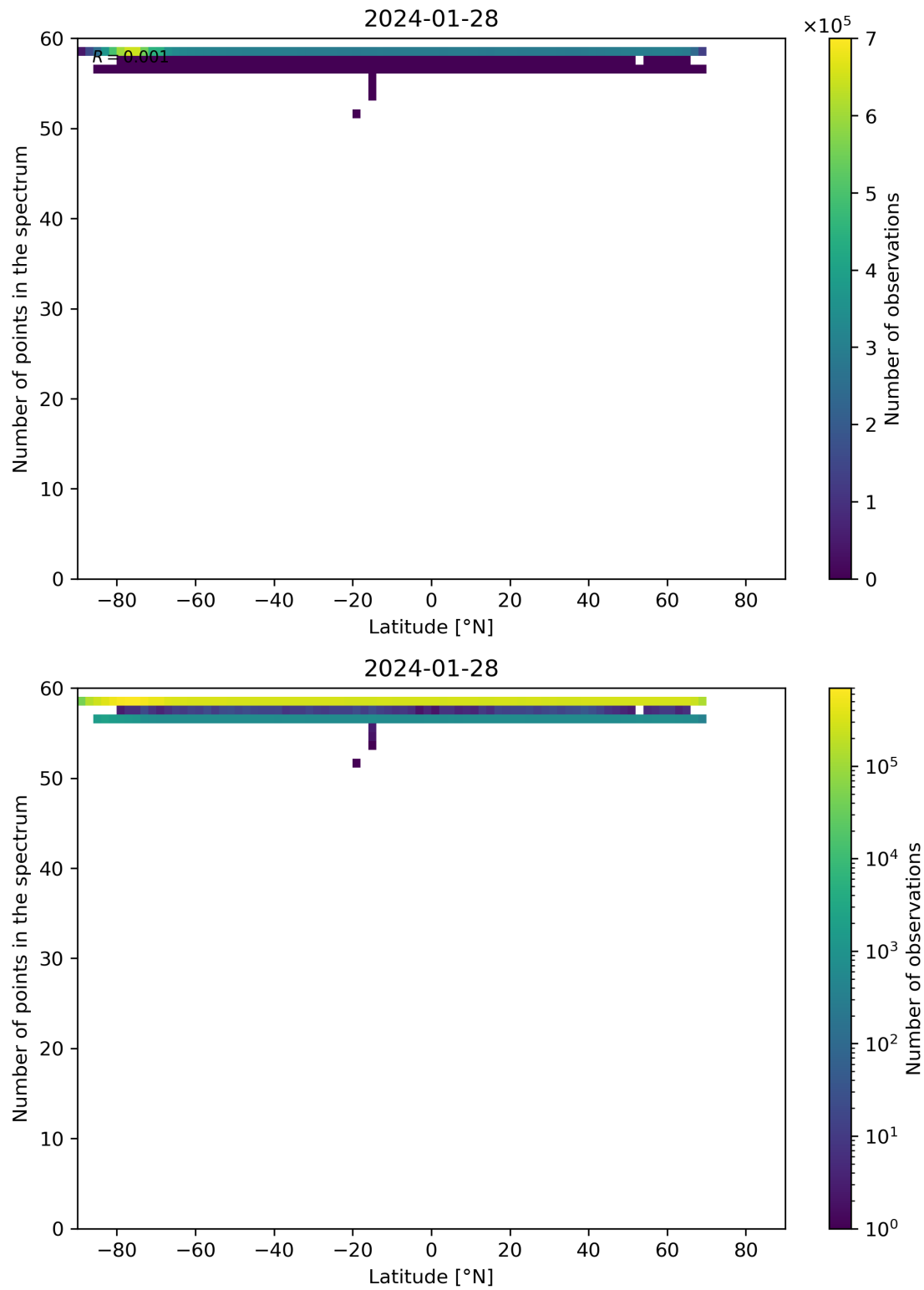
Figure 94: Scatter density plot of “Latitude” against “Number of points in the spectrum” for 2024-01-27 to 2024-01-29.
