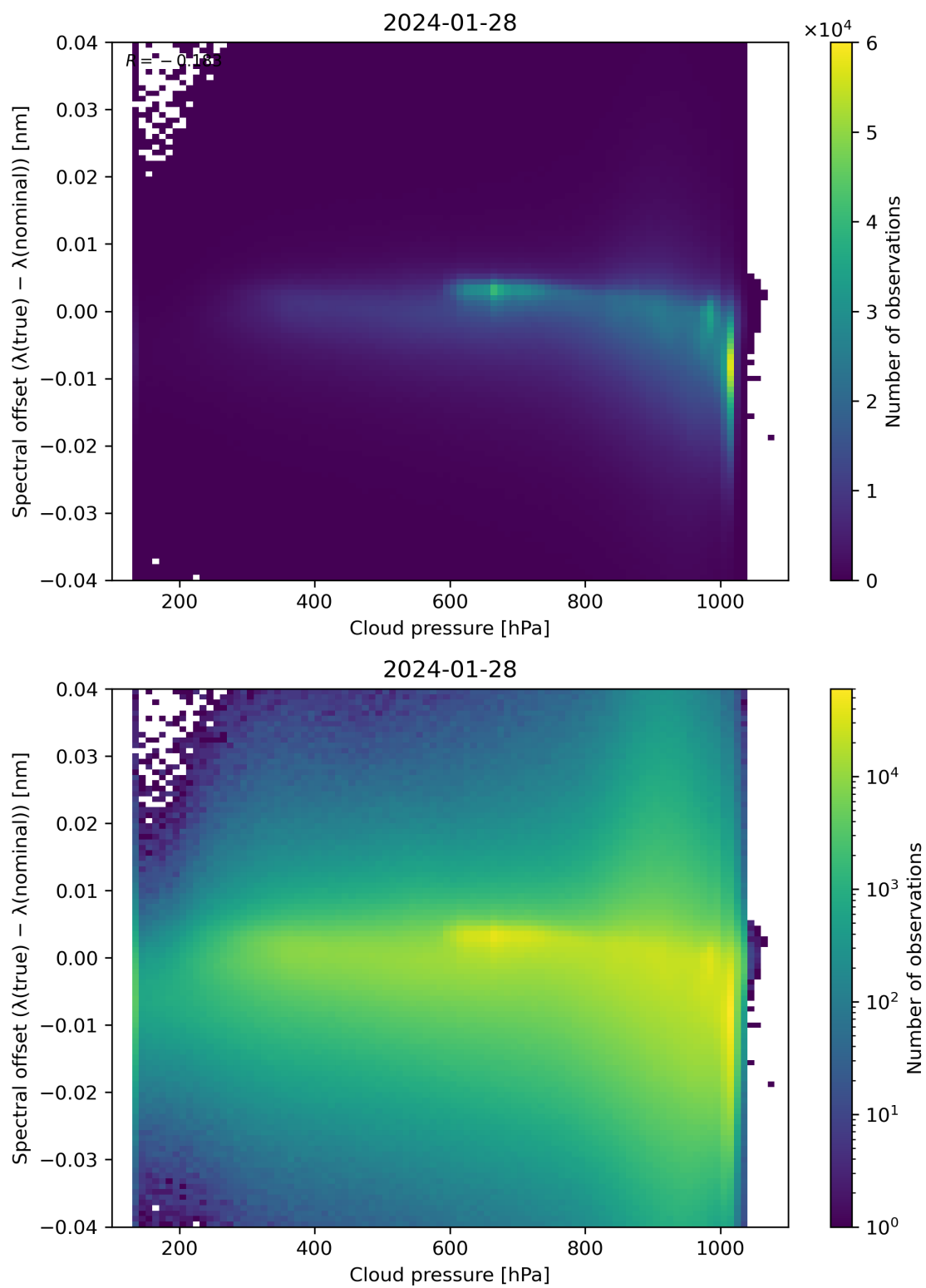
Figure 84: Scatter density plot of “Cloud pressure” against “Spectral offset ( \lambda(\text{true}) - \lambda(\text{nominal}) )” for 2024-01-27 to 2024-01-29.
