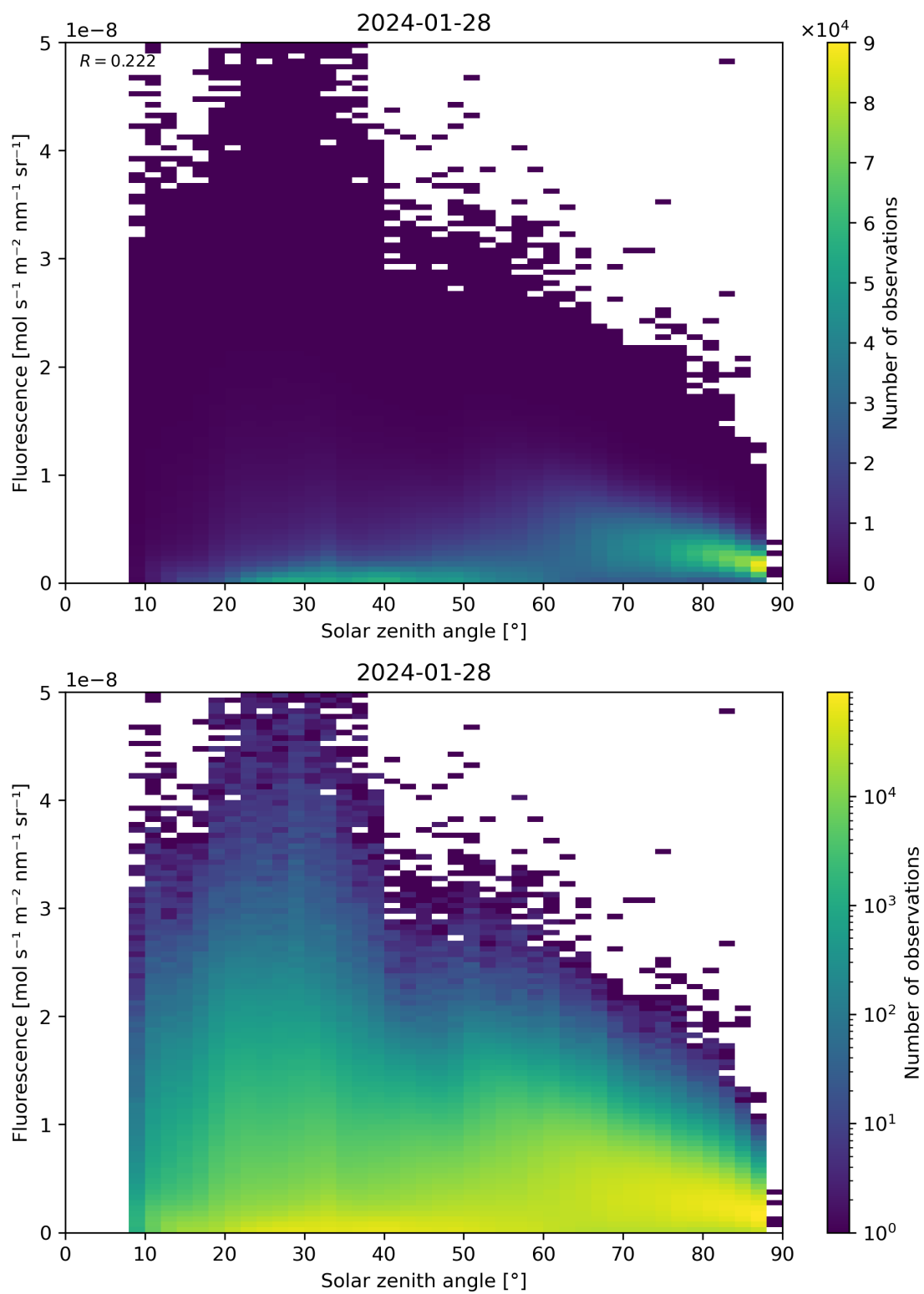
Figure 112: Scatter density plot of “Solar zenith angle” against “Fluorescence” for 2024-01-27 to 2024-01-29.
