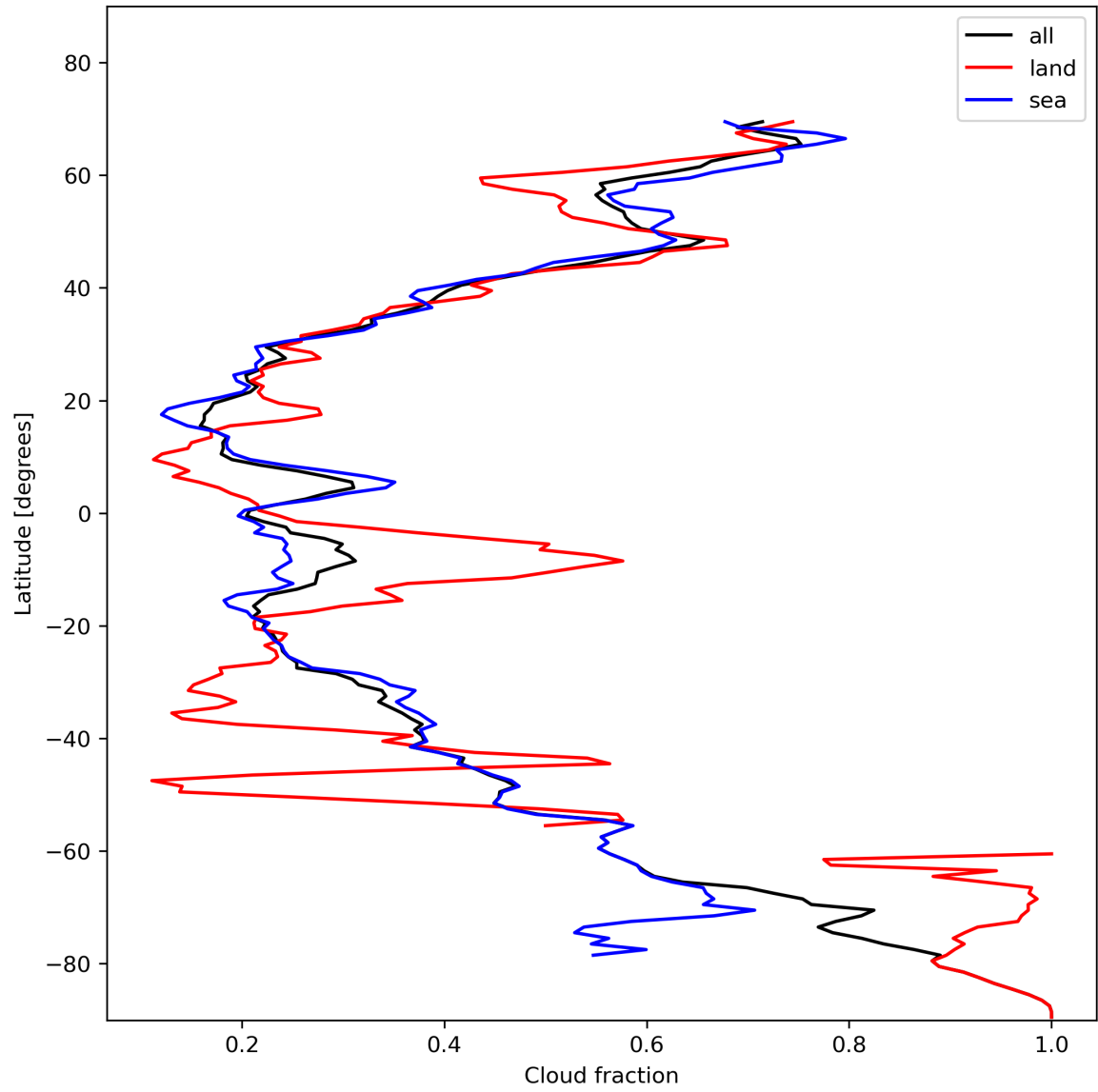
Figure 15: Zonal average of “Cloud fraction” for 2024-01-27 to 2024-01-29.
