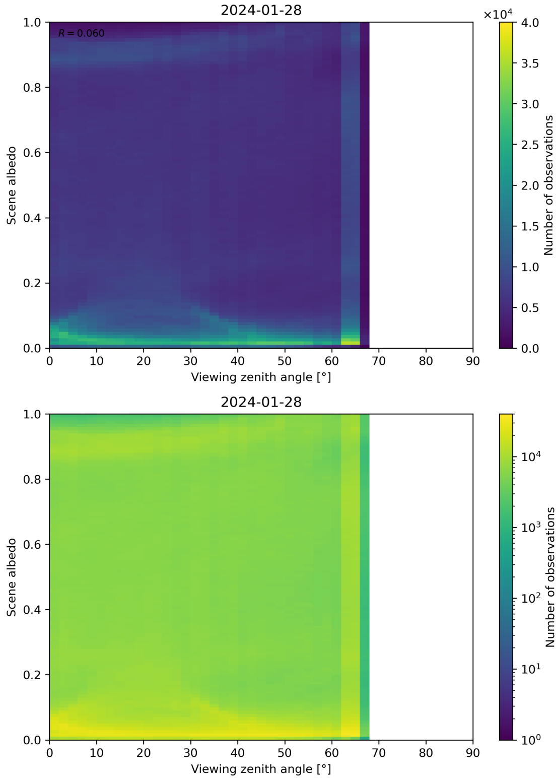
Figure 126: Scatter density plot of “Viewing zenith angle” against “Scene albedo” for 2024-01-27 to 2024-01-29.
