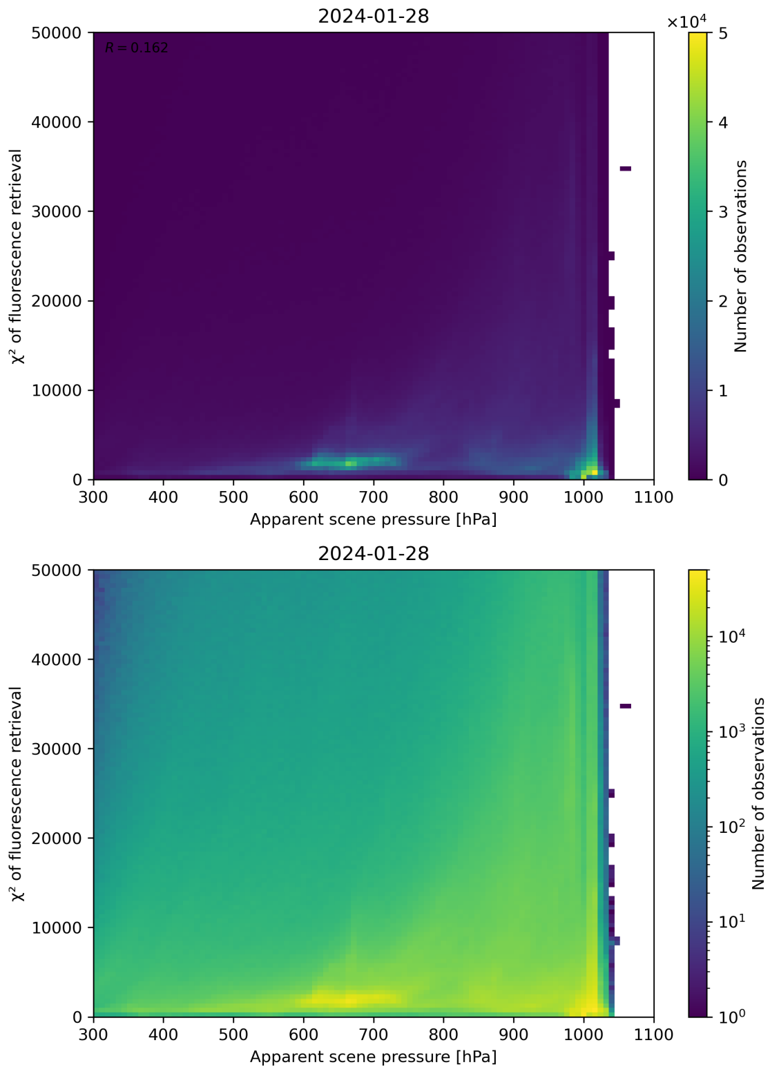
Figure 63: Scatter density plot of “Apparent scene pressure” against “ \chi^2 of fluorescence retrieval” for 2024-01-27 to 2024-01-29.
