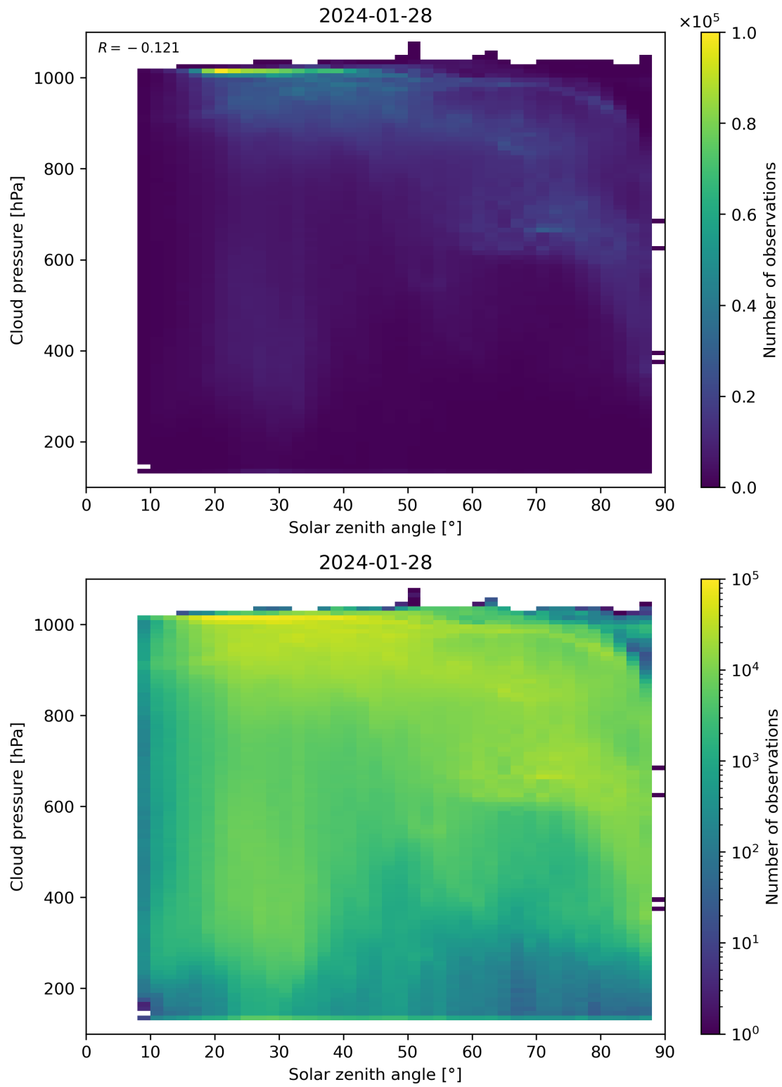
Figure 111: Scatter density plot of “Solar zenith angle” against “Cloud pressure” for 2024-01-27 to 2024-01-29.
