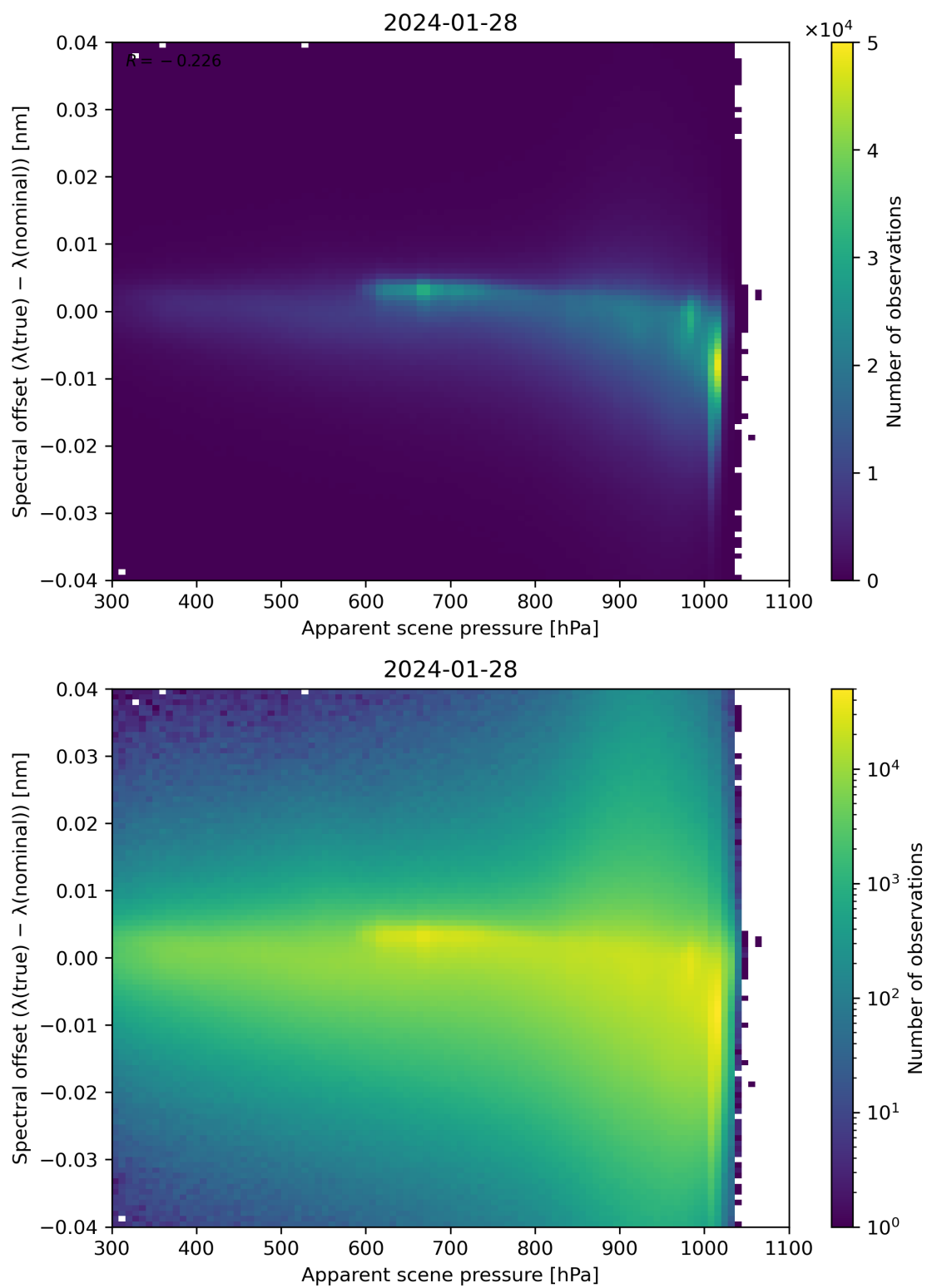
Figure 67: Scatter density plot of “Apparent scene pressure” against “Spectral offset ( \lambda(\text{true}) - \lambda(\text{nominal}) )” for 2024-01-27 to 2024-01-29.
