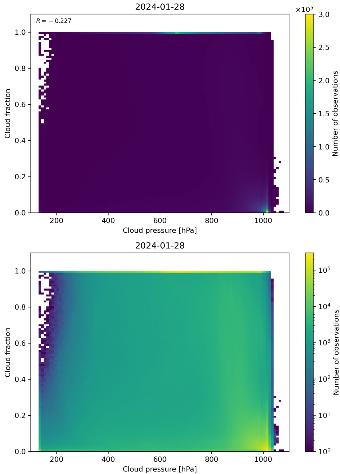
Figure 79: Scatter density plot of “Cloud pressure” against “Cloud fraction” for 2024-01-27 to 2024-01-29.
