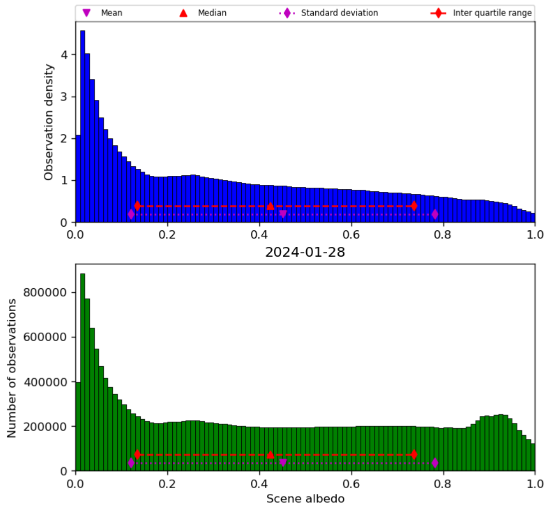
Figure 34: Histogram of “Scene albedo” for 2024-01-27 to 2024-01-29
