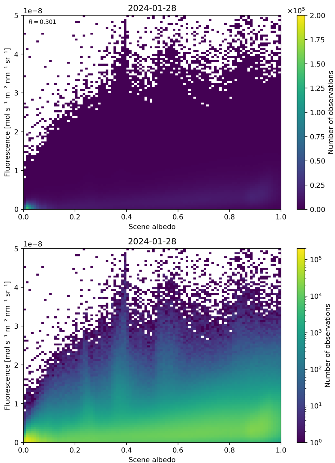
Figure 104: Scatter density plot of “Scene albedo” against “Fluorescence” for 2024-01-27 to 2024-01-29.
