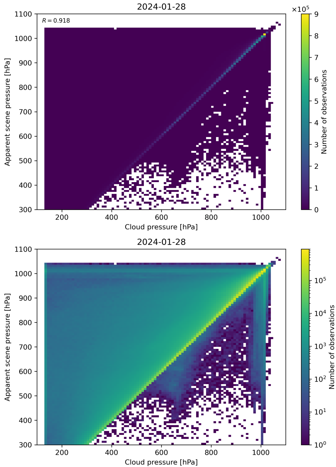
Figure 77: Scatter density plot of “Cloud pressure” against “Apparent scene pressure” for 2024-01-27 to 2024-01-29.
