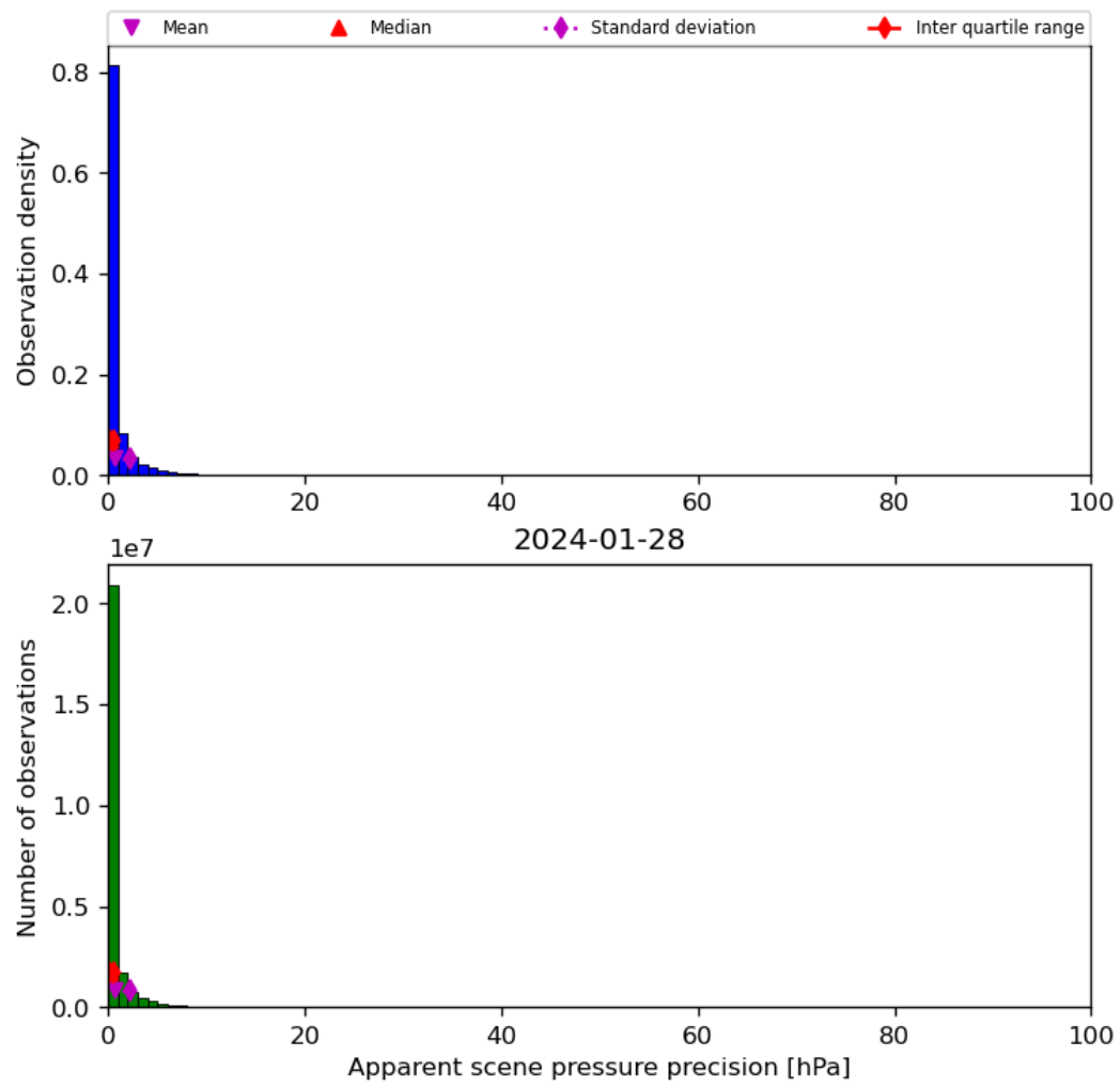
Figure 37: Histogram of “Apparent scene pressure precision” for 2024-01-27 to 2024-01-29
