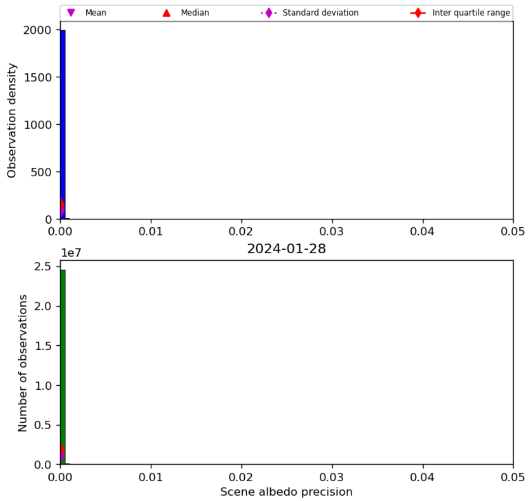
Figure 35: Histogram of “Scene albedo precision” for 2024-01-27 to 2024-01-29
