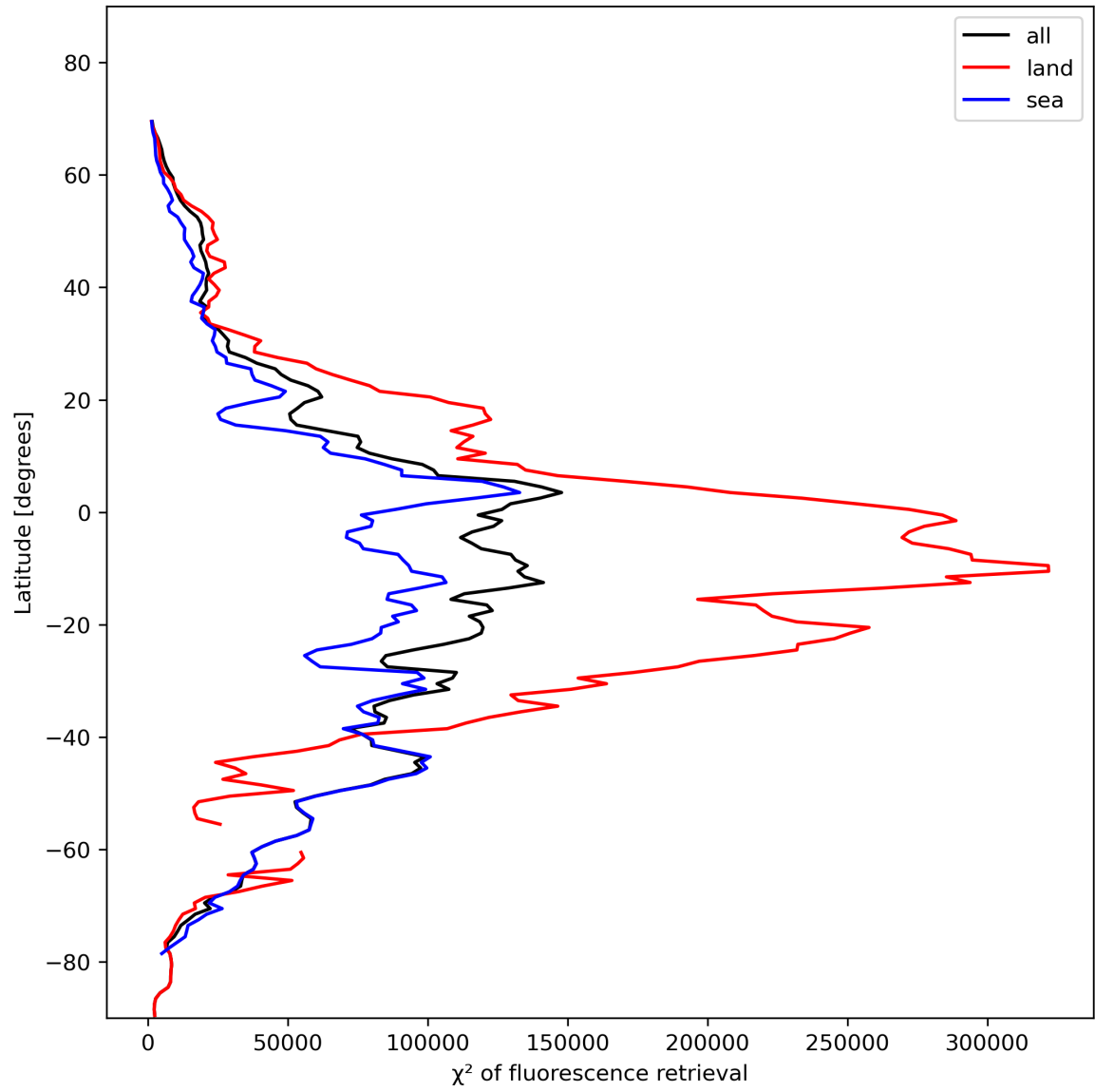
Figure 25: Zonal average of “ \chi^2 of fluorescence retrieval” for 2024-01-27 to 2024-01-29.
