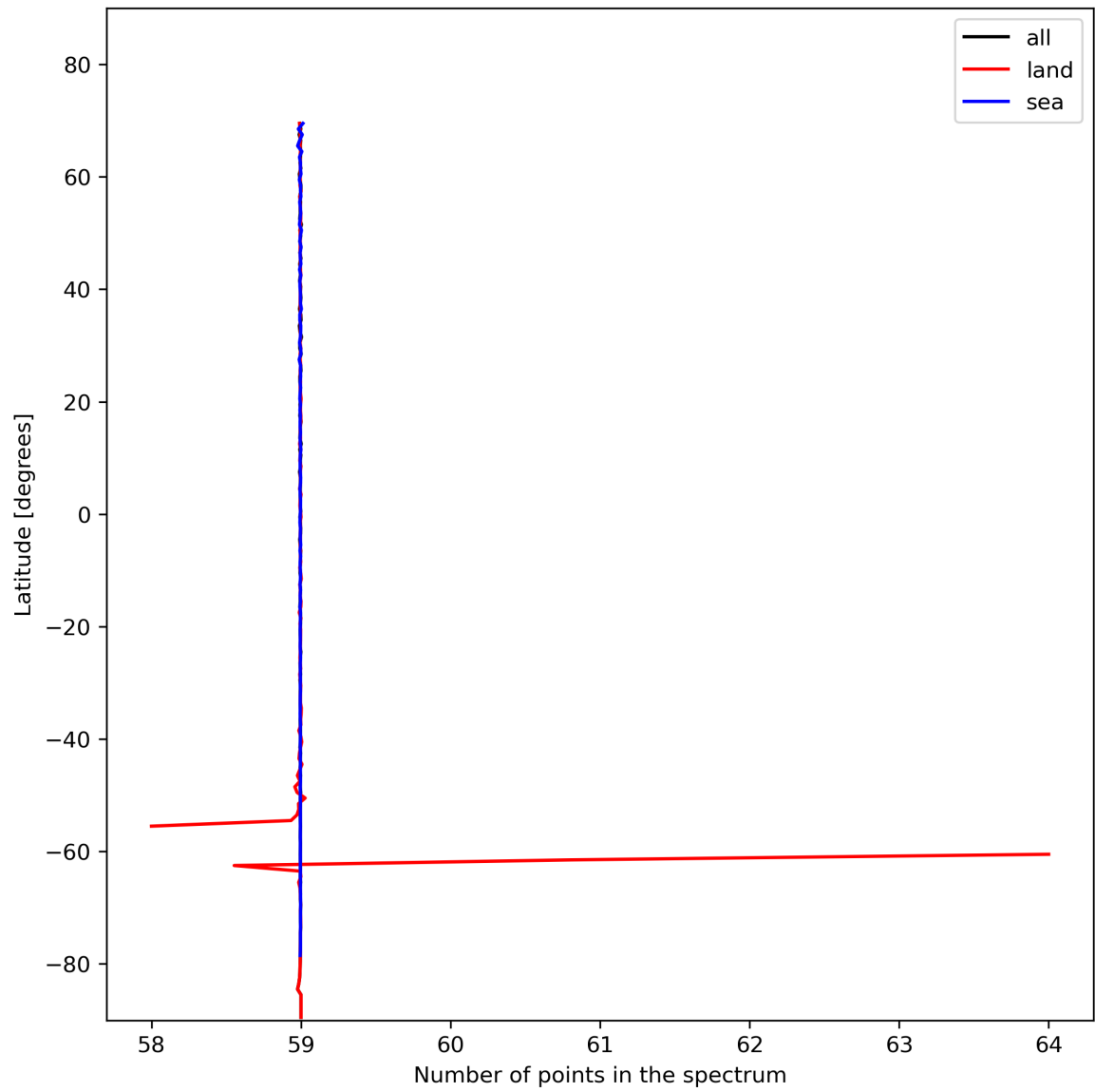
Figure 27: Zonal average of “Number of points in the spectrum” for 2024-01-27 to 2024-01-29.
