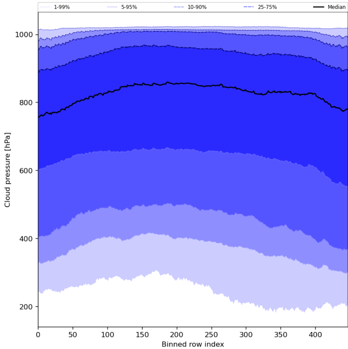
Figure 47: Along track statistics of “Cloud pressure” for 2024-01-27 to 2024-01-29
