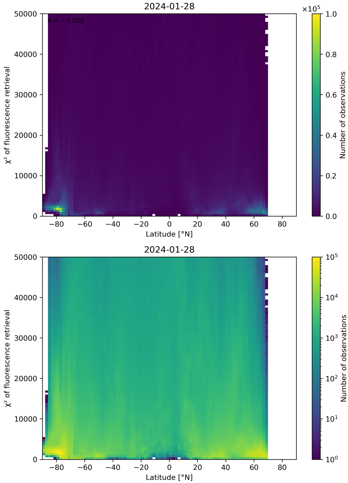
Figure 89: Scatter density plot of “Latitude” against “ \chi^2 of fluorescence retrieval” for 2024-01-27 to 2024-01-29.
