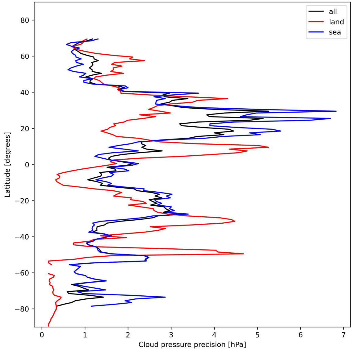
Figure 14: Zonal average of “Cloud pressure precision” for 2024-01-27 to 2024-01-29.
