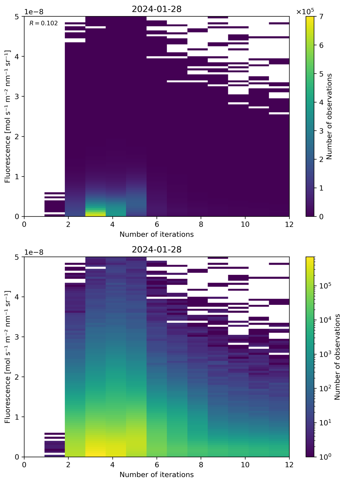
Figure 98: Scatter density plot of “Number of iterations” against “Fluorescence” for 2024-01-27 to 2024-01-29.
