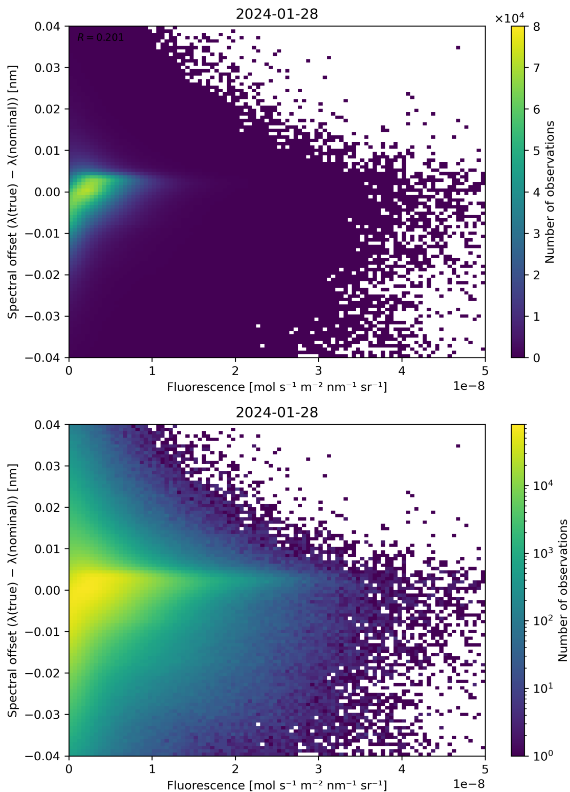
Figure 87: Scatter density plot of “Fluorescence” against “Spectral offset ( \lambda(\text{true}) - \lambda(\text{nominal}) )” for 2024-01-27 to 2024-01-29.
