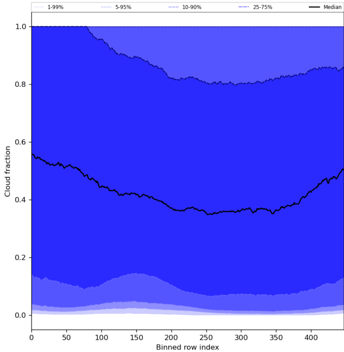
Figure 49: Along track statistics of “Cloud fraction” for 2024-01-27 to 2024-01-29
