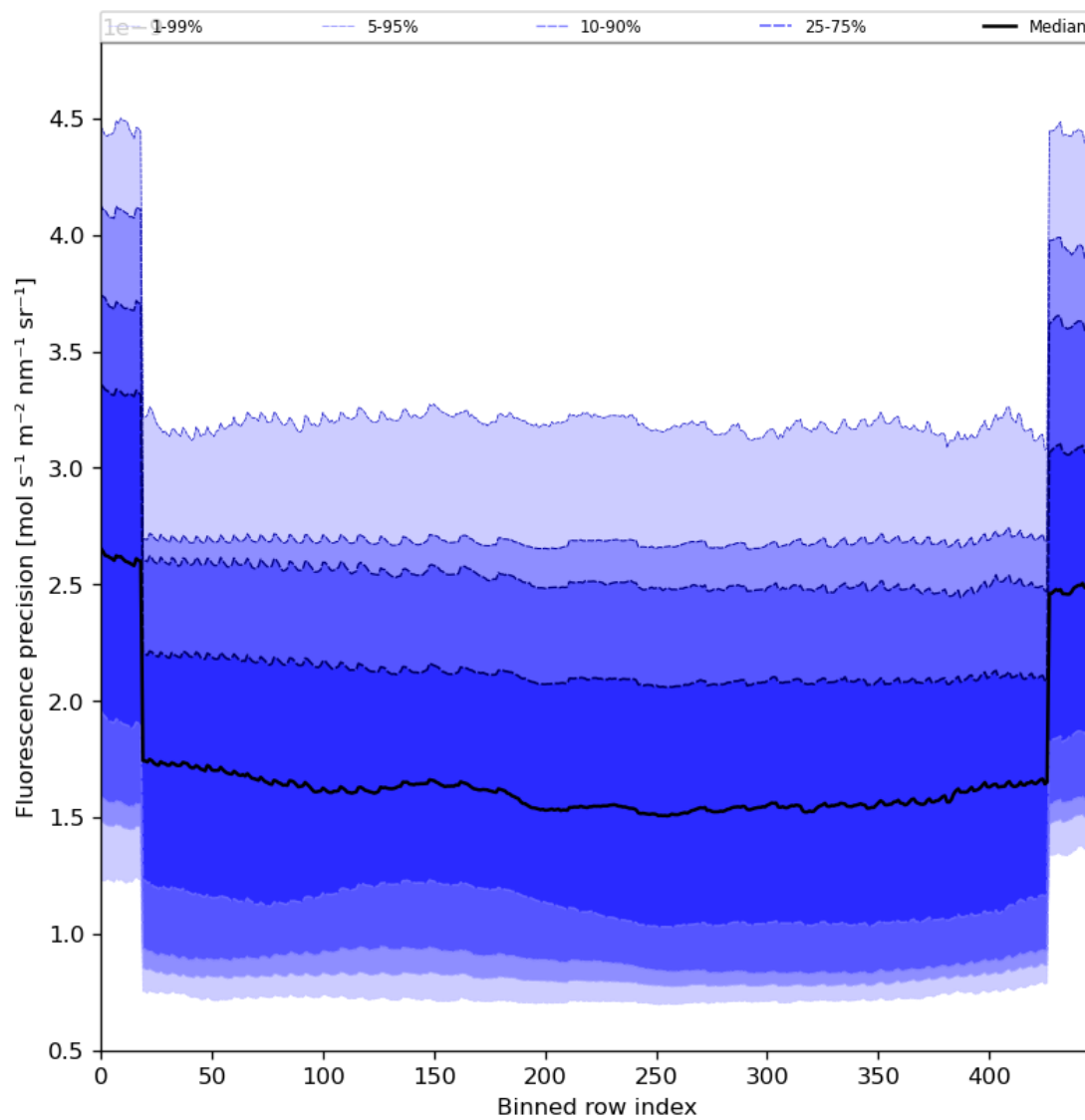
Figure 58: Along track statistics of “Fluorescence precision” for 2024-01-27 to 2024-01-29
