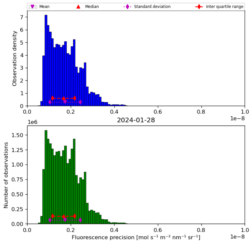
Figure 41: Histogram of “Fluorescence precision” for 2024-01-27 to 2024-01-29
