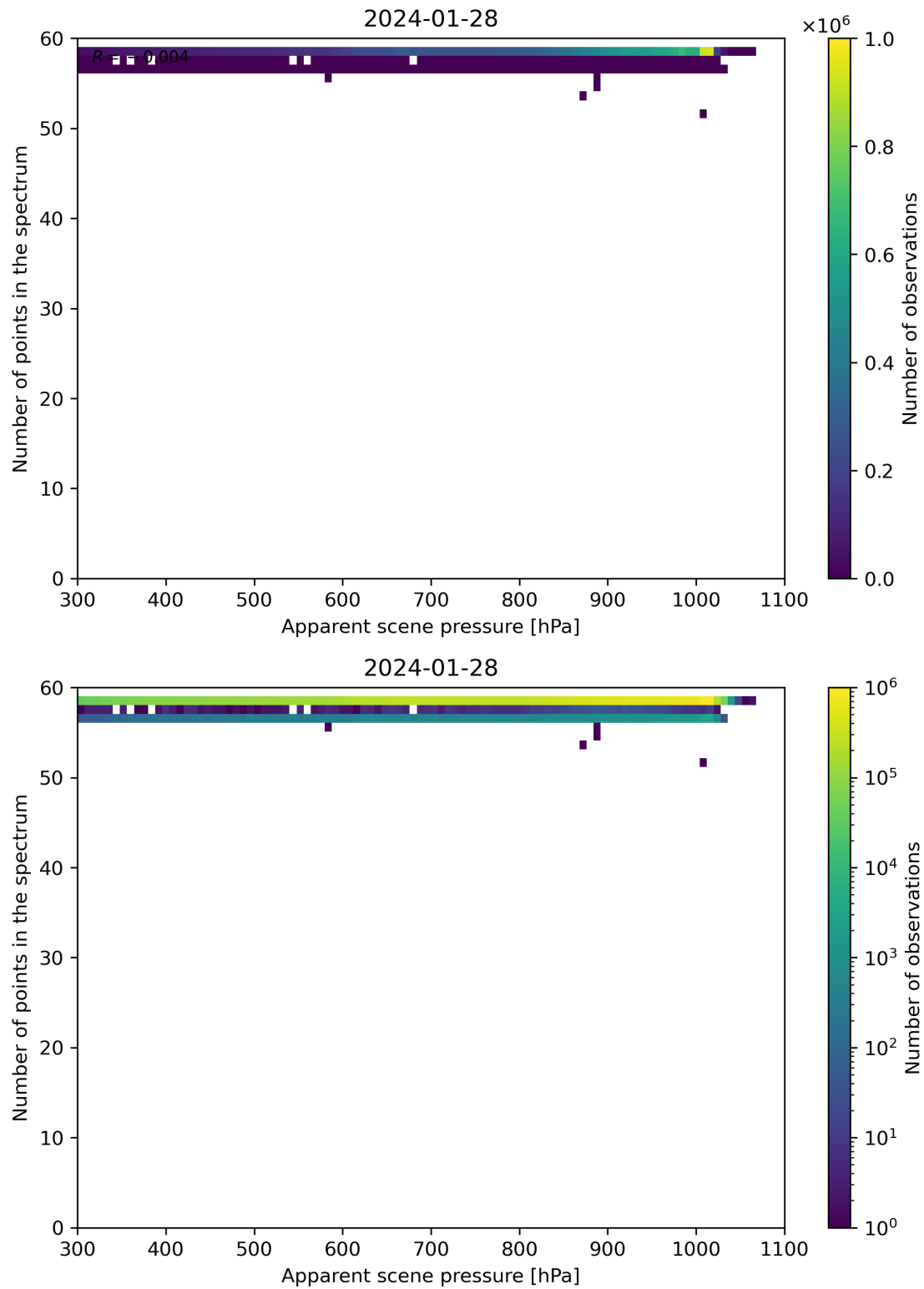
Figure 66: Scatter density plot of “Apparent scene pressure” against “Number of points in the spectrum” for 2024-01-27 to 2024-01-29.
