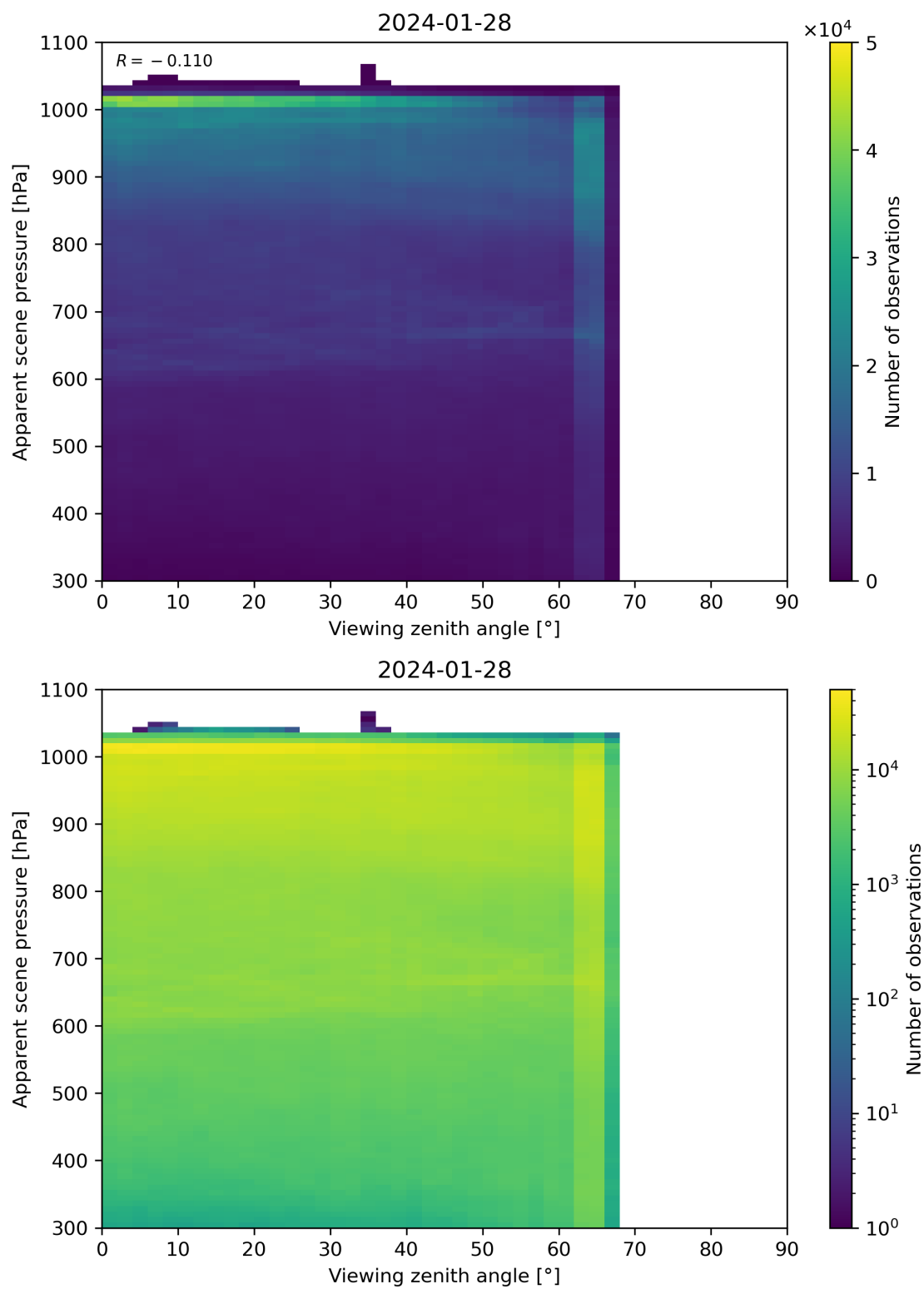
Figure 118: Scatter density plot of “Viewing zenith angle” against “Apparent scene pressure” for 2024-01-27 to 2024-01-29.
