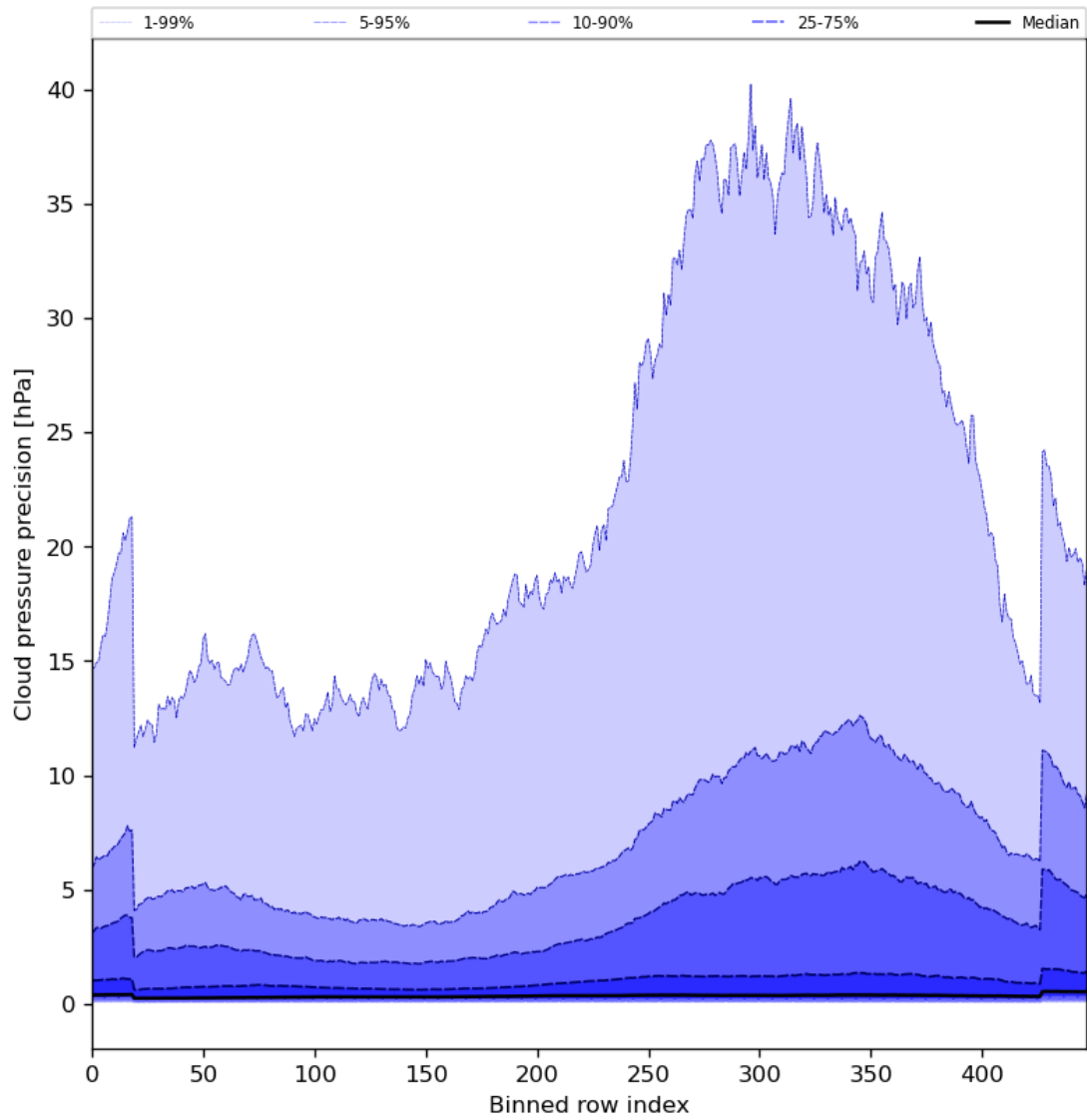
Figure 48: Along track statistics of “Cloud pressure precision” for 2024-01-27 to 2024-01-29
