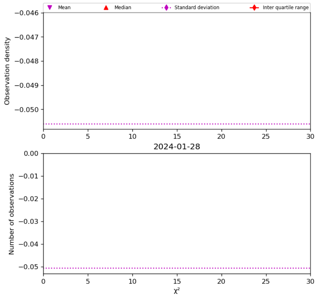
Figure 38: Histogram of “ \chi^2 ” for 2024-01-27 to 2024-01-29
