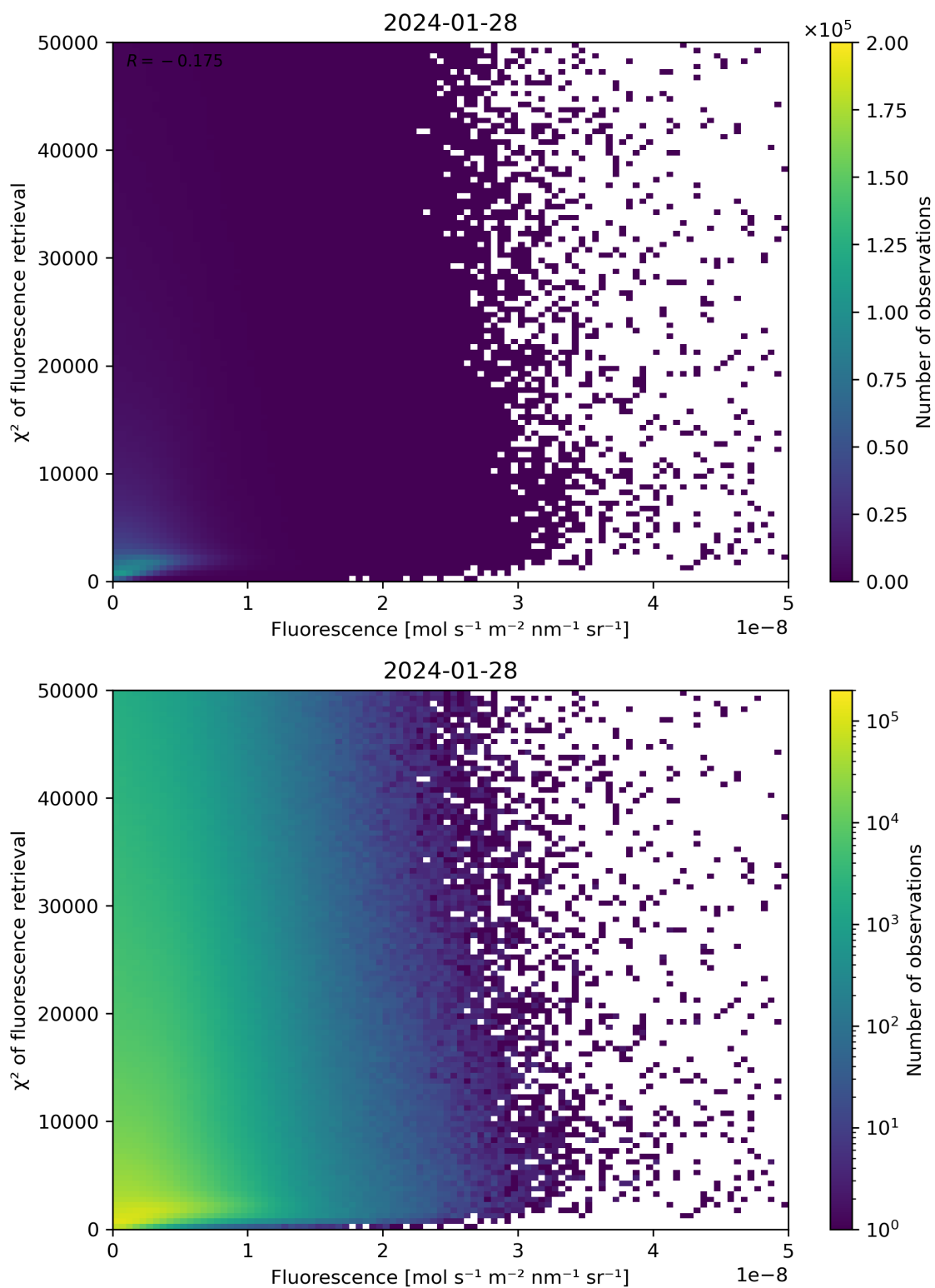
Figure 85: Scatter density plot of “Fluorescence” against “ \chi^2 of fluorescence retrieval” for 2024-01-27 to 2024-01-29.
