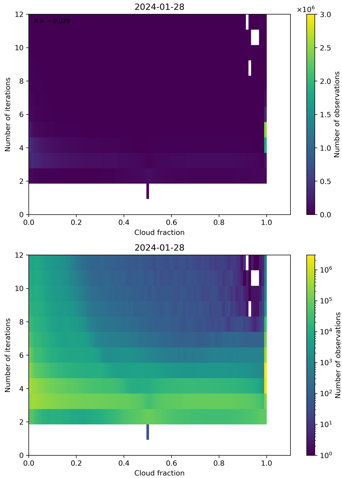
Figure 73: Scatter density plot of “Cloud fraction” against “Number of iterations” for 2024-01-27 to 2024-01-29.
