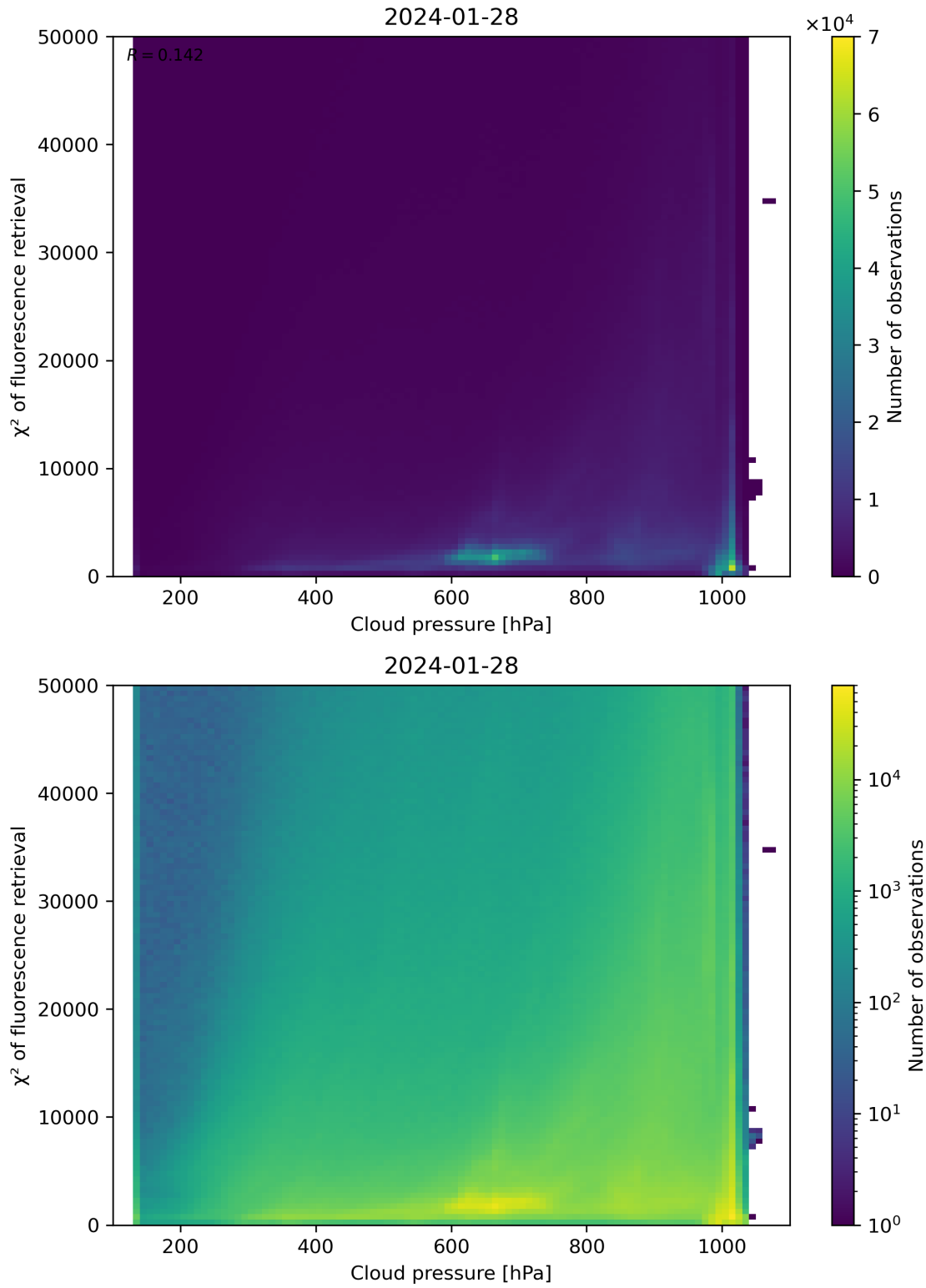
Figure 78: Scatter density plot of “Cloud pressure” against “ \chi^2 of fluorescence retrieval” for 2024-01-27 to 2024-01-29.
