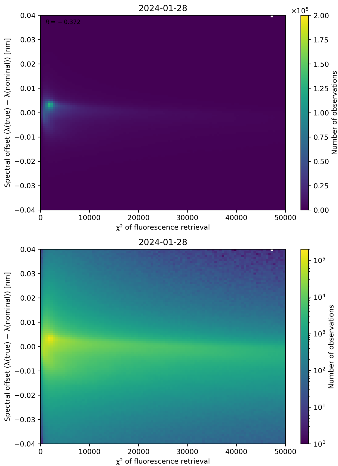
Figure 69: Scatter density plot of " \chi^2 of fluorescence retrieval" against "Spectral offset ( \lambda(\text{true}) - \lambda(\text{nominal}) )" for 2024-01-27 to 2024-01-29.
