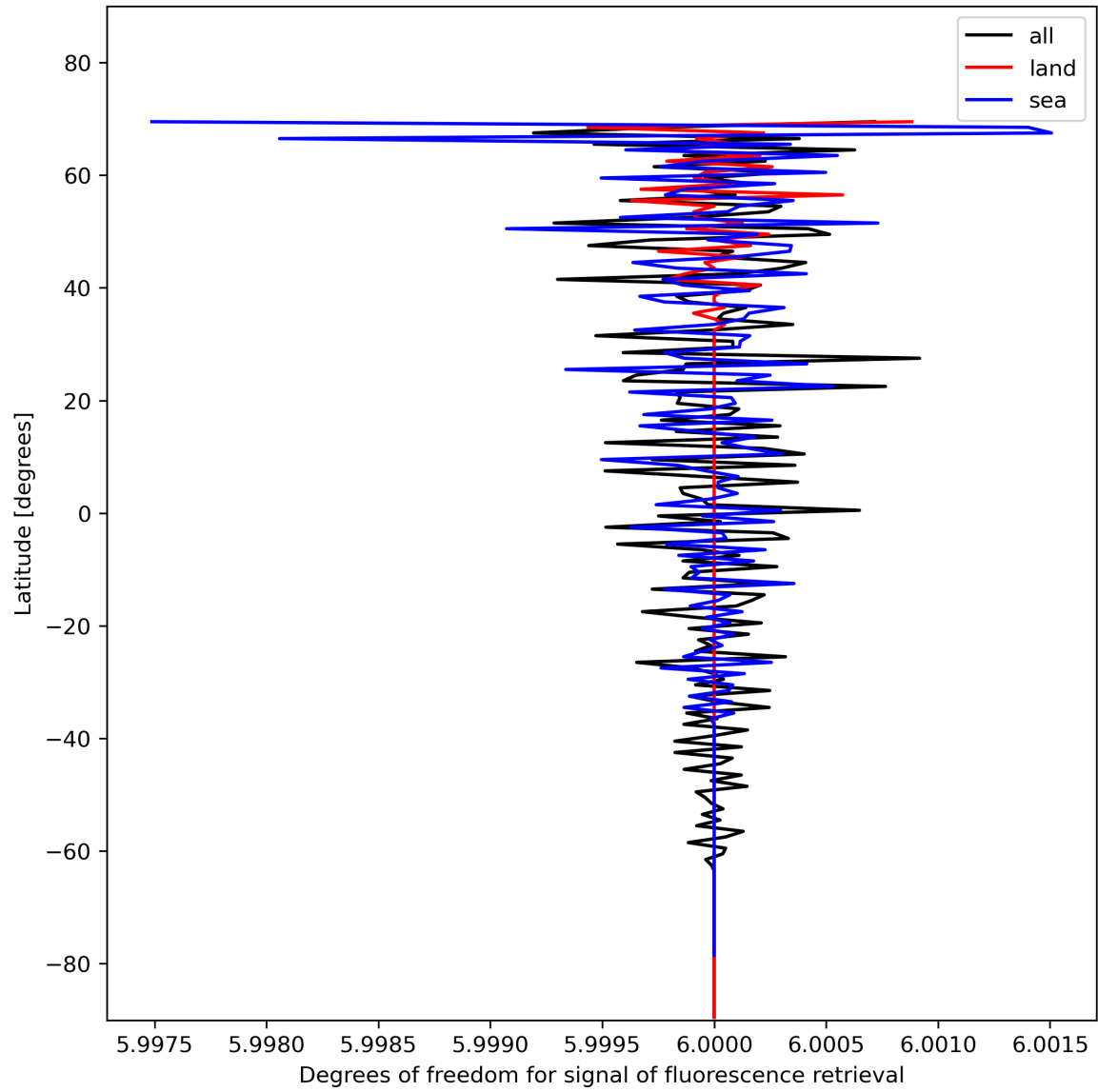
Figure 26: Zonal average of “Degrees of freedom for signal of fluorescence retrieval” for 2024-01-27 to 2024-01-29.
