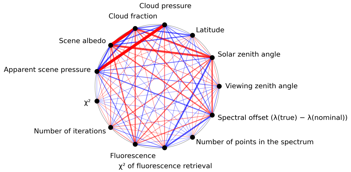
Figure 1: Map of correlation graph for 2024-01-27 to 2024-01-29.
