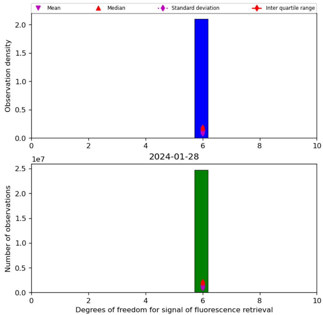
Figure 43: Histogram of “Degrees of freedom for signal of fluorescence retrieval” for 2024-01-27 to 2024-01-29
