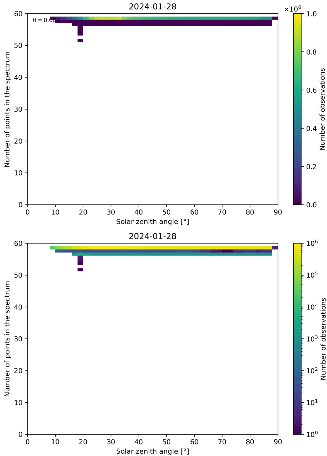
Figure 115: Scatter density plot of “Solar zenith angle” against “Number of points in the spectrum” for 2024-01-27 to 2024-01-29.
