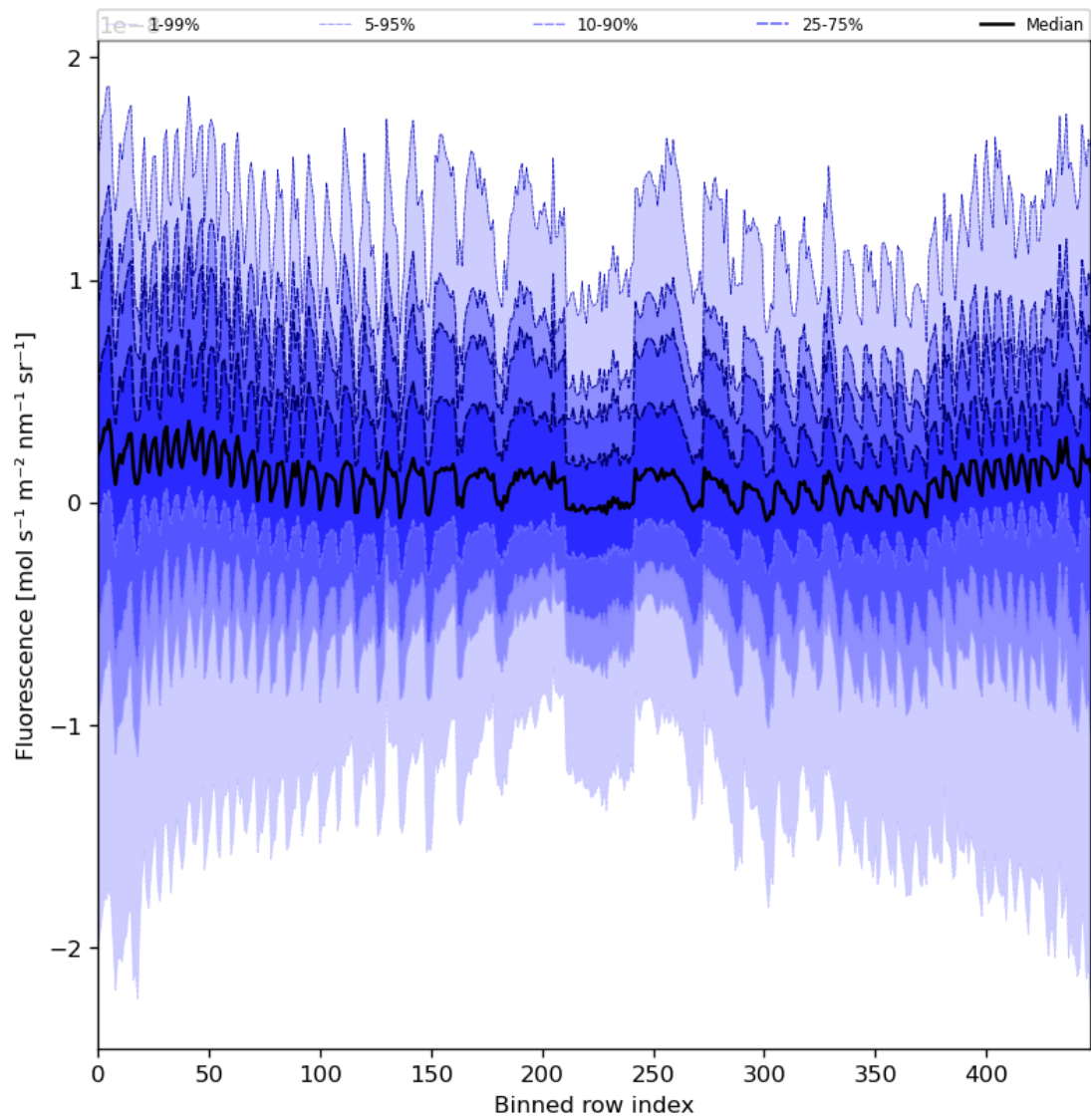
Figure 57: Along track statistics of “Fluorescence” for 2024-01-27 to 2024-01-29
