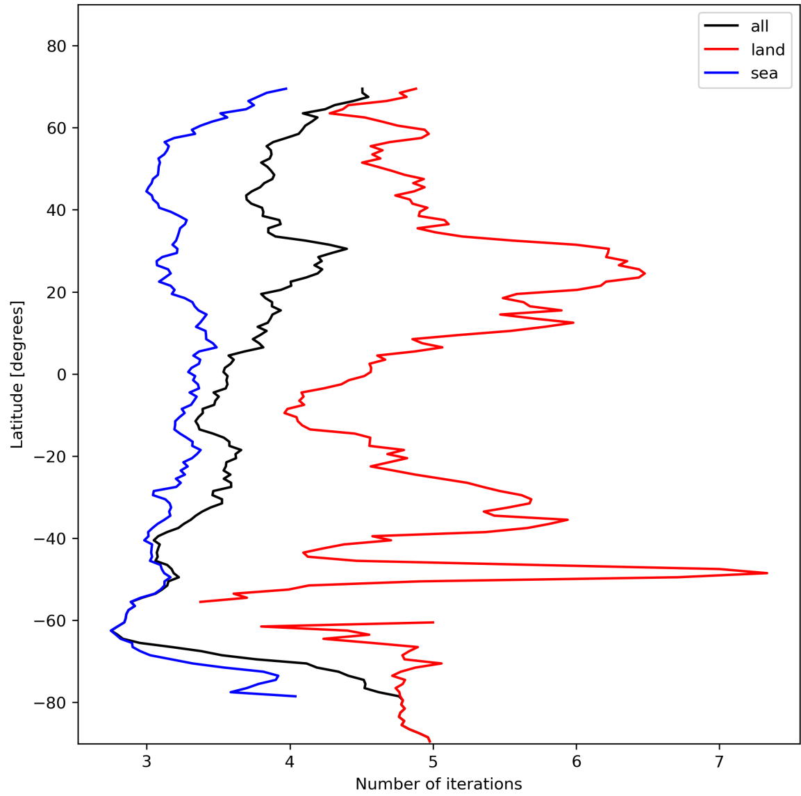
Figure 22: Zonal average of “Number of iterations” for 2024-01-27 to 2024-01-29.
