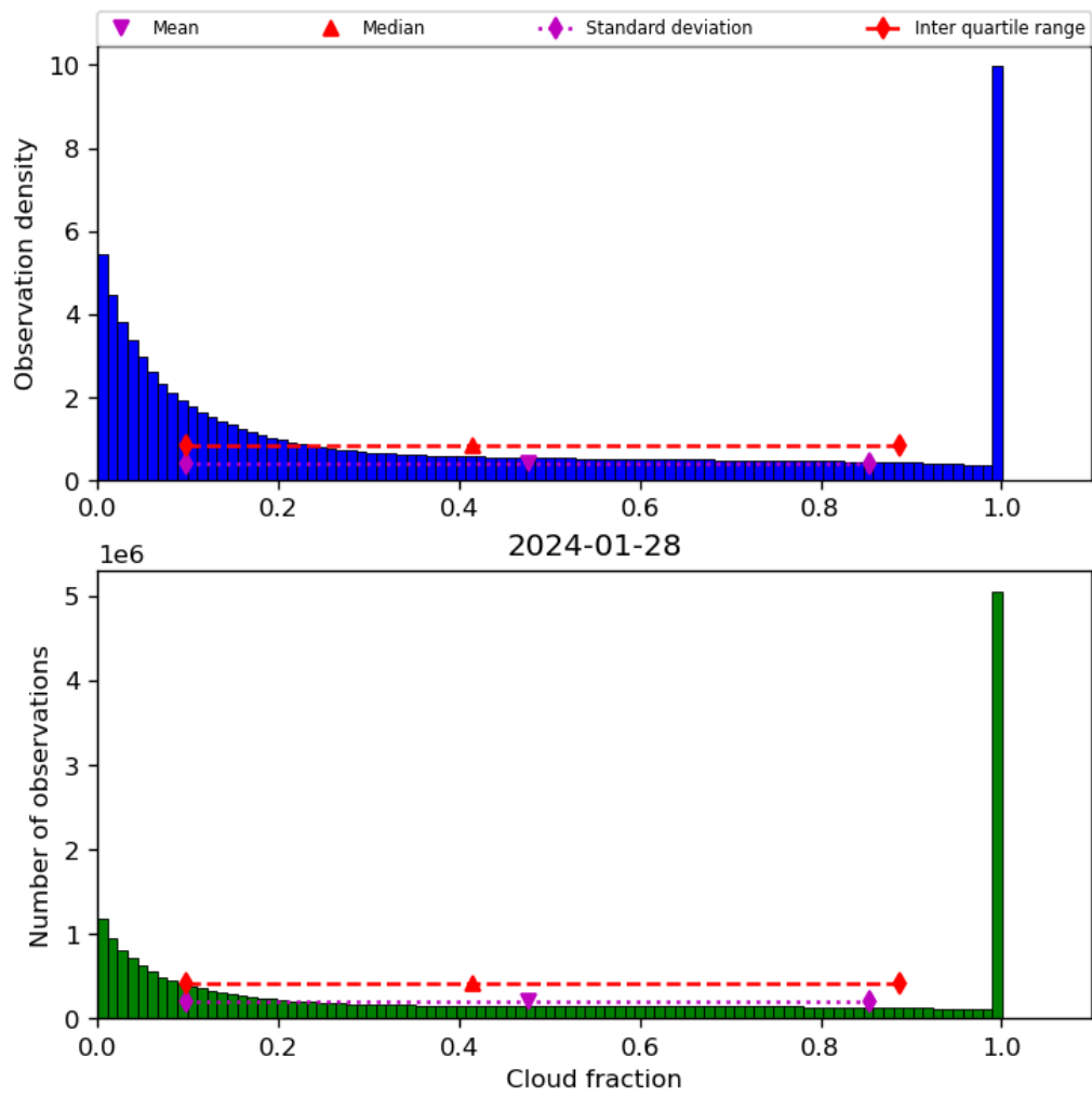
Figure 32: Histogram of “Cloud fraction” for 2024-01-27 to 2024-01-29
