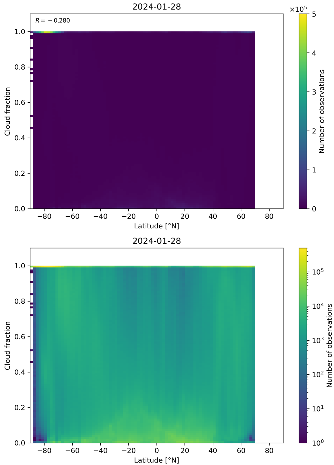
Figure 90: Scatter density plot of “Latitude” against “Cloud fraction” for 2024-01-27 to 2024-01-29.
