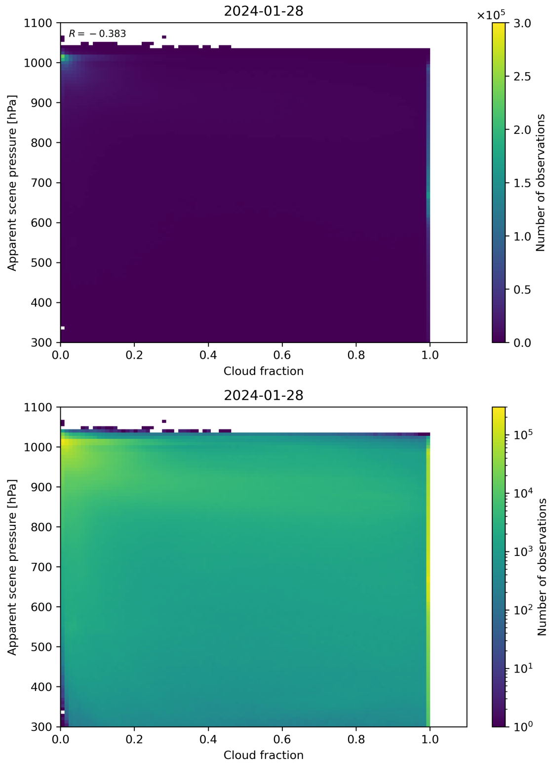
Figure 70: Scatter density plot of “Cloud fraction” against “Apparent scene pressure” for 2024-01-27 to 2024-01-29.
