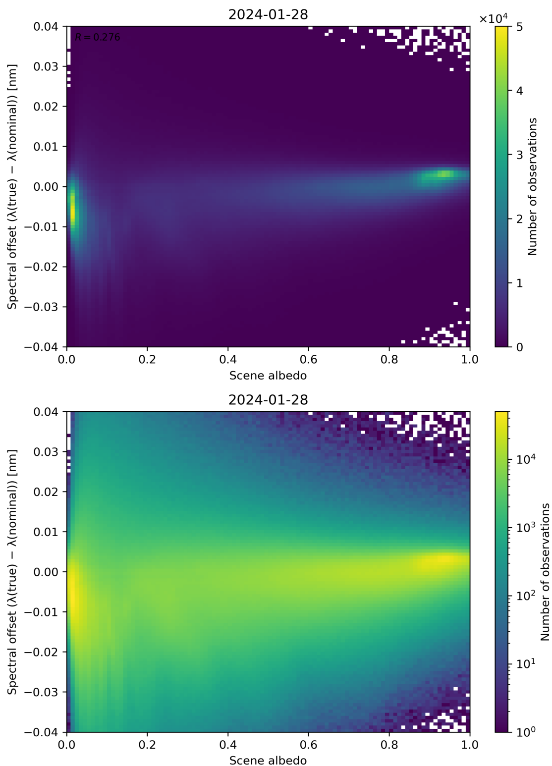
Figure 107: Scatter density plot of “Scene albedo” against “Spectral offset ( \lambda(\text{true}) - \lambda(\text{nominal}) )” for 2024-01-27 to 2024-01-29.
