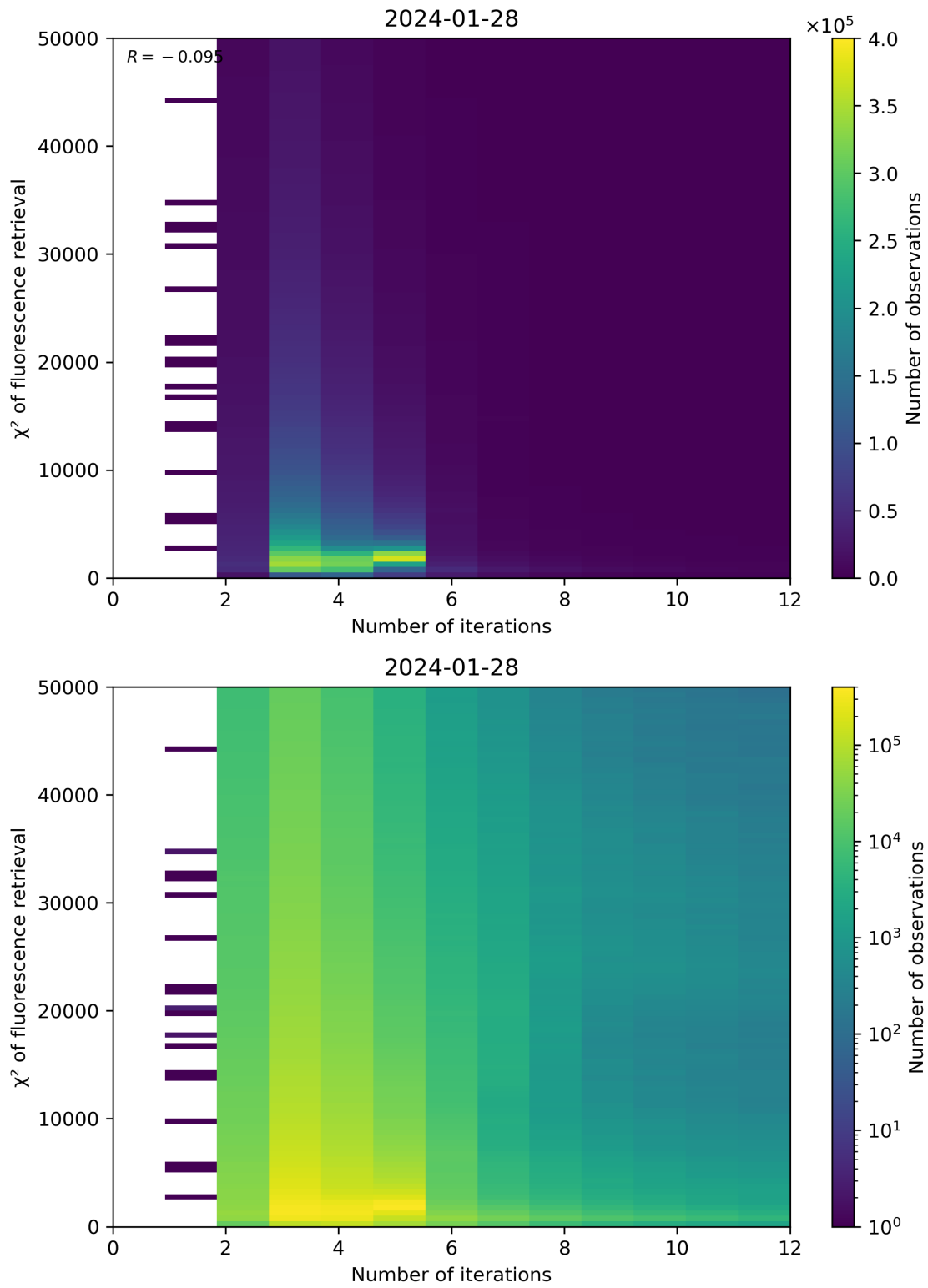
Figure 97: Scatter density plot of “Number of iterations” against “ \chi^2 of fluorescence retrieval” for 2024-01-27 to 2024-01-29.
