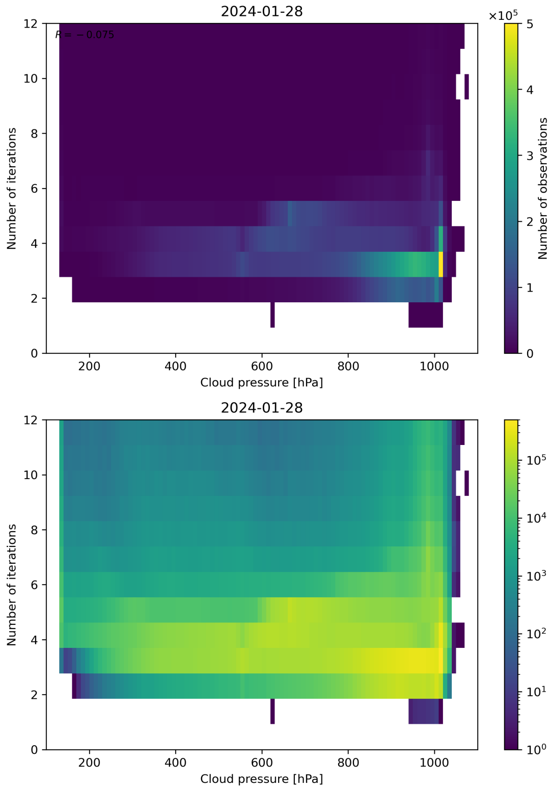
Figure 81: Scatter density plot of “Cloud pressure” against “Number of iterations” for 2024-01-27 to 2024-01-29.
