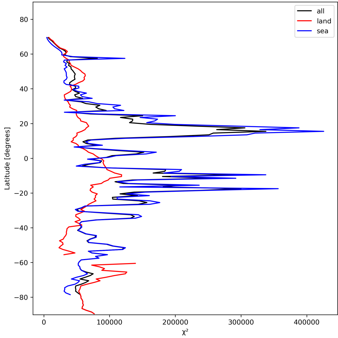
Figure 21: Zonal average of “ \chi^2 ” for 2024-01-27 to 2024-01-29.
