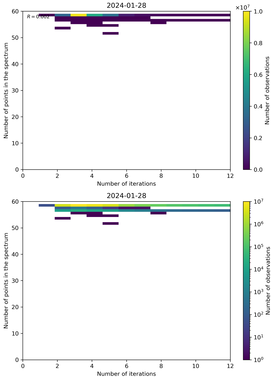
Figure 99: Scatter density plot of “Number of iterations” against “Number of points in the spectrum” for 2024-01-27 to 2024-01-29.
