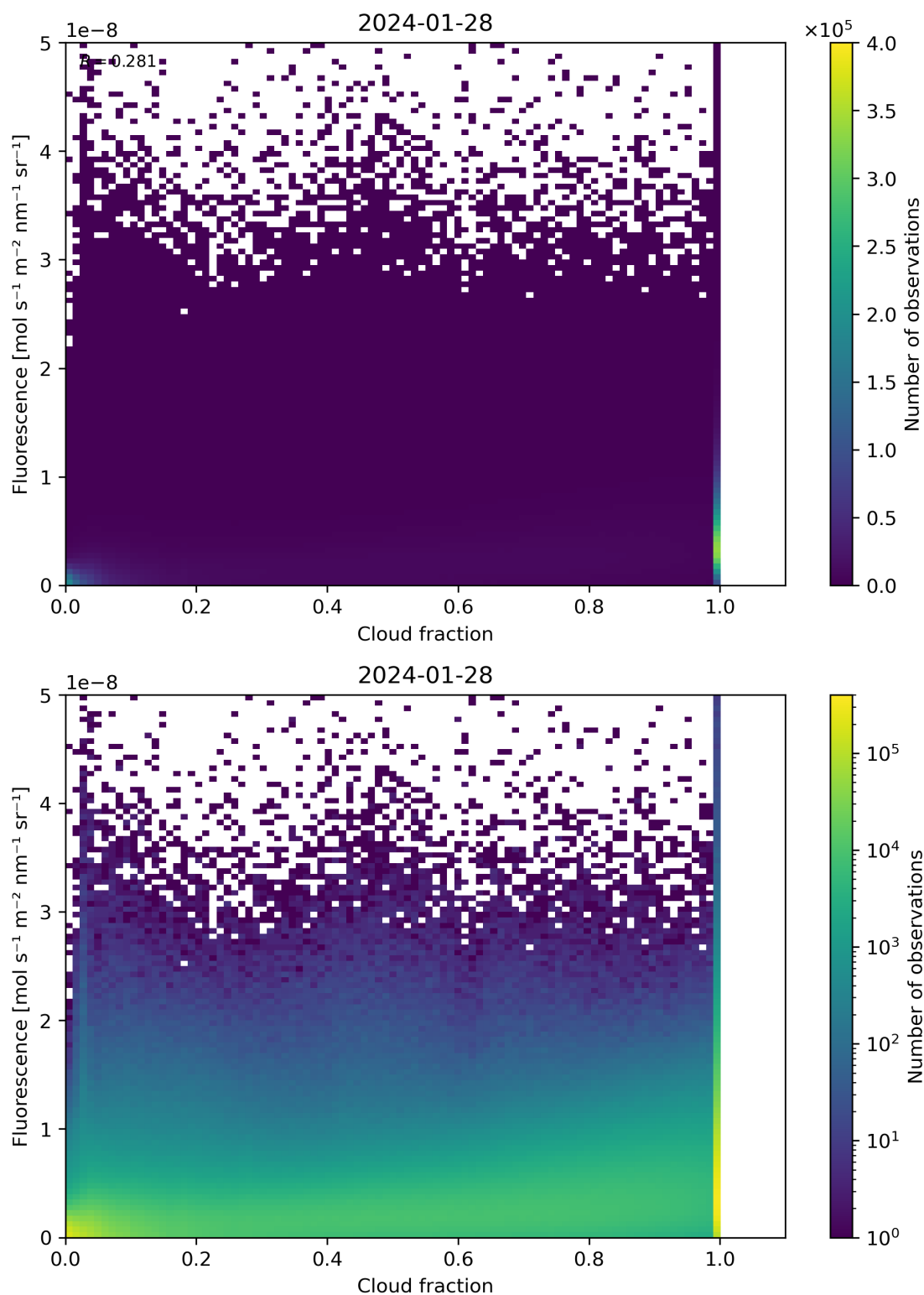
Figure 72: Scatter density plot of “Cloud fraction” against “Fluorescence” for 2024-01-27 to 2024-01-29.
