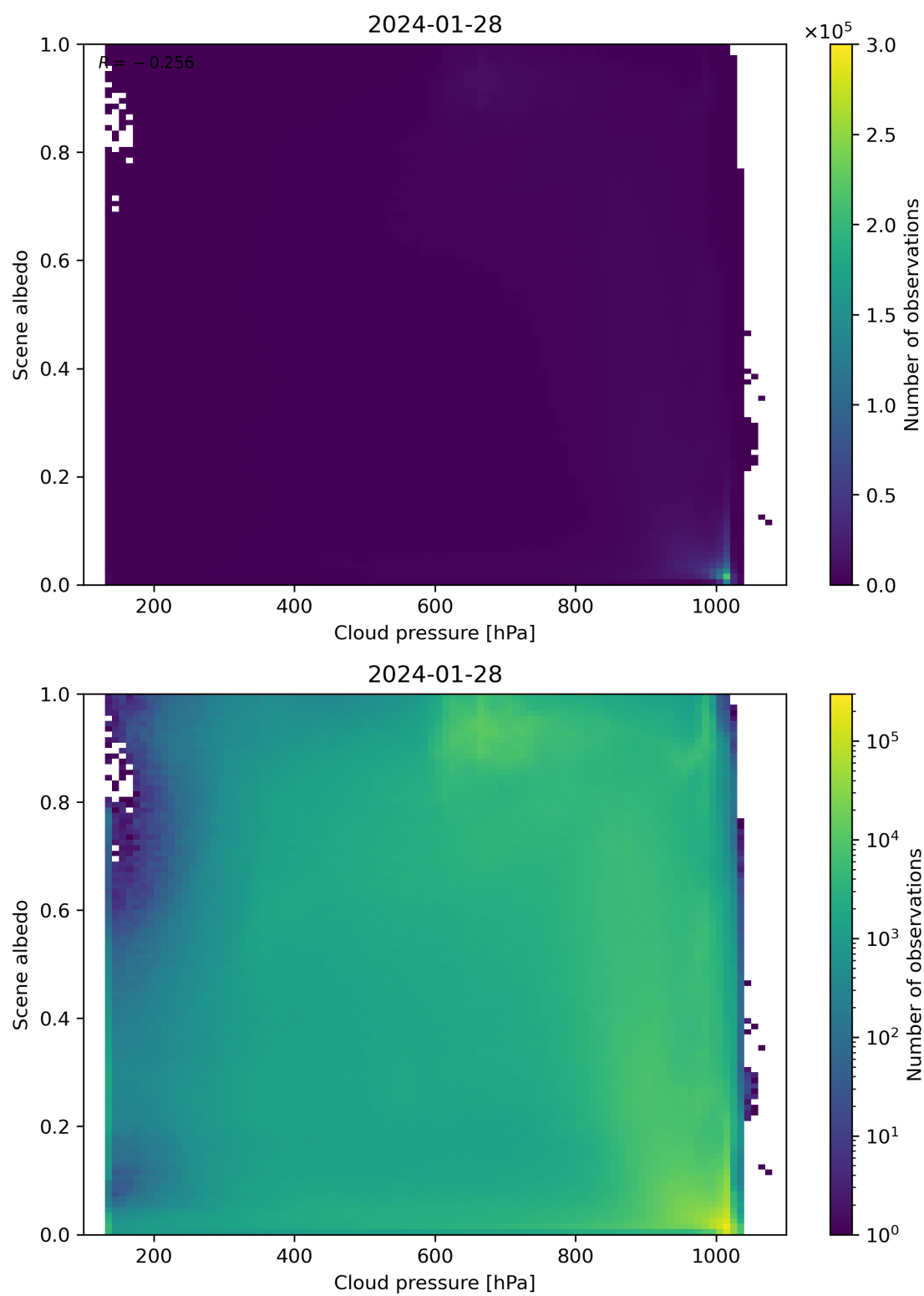
Figure 83: Scatter density plot of “Cloud pressure” against “Scene albedo” for 2024-01-27 to 2024-01-29.
