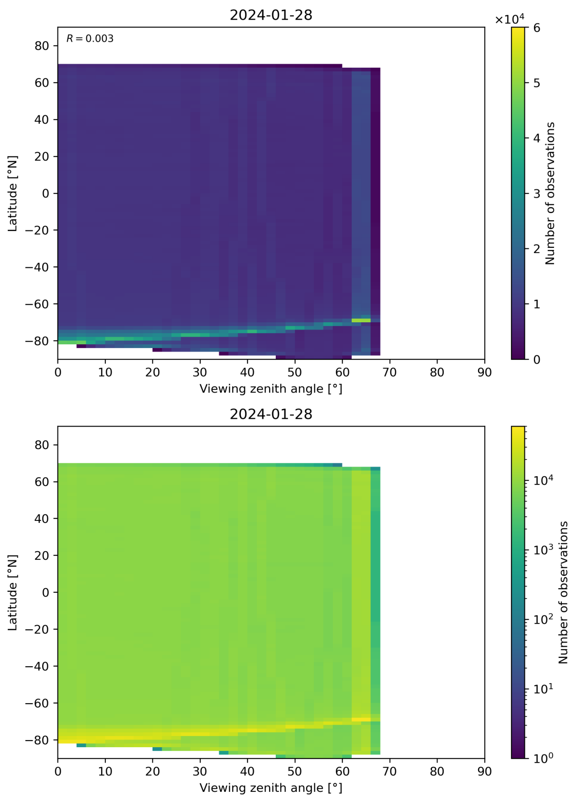
Figure 123: Scatter density plot of “Viewing zenith angle” against “Latitude” for 2024-01-27 to 2024-01-29.
