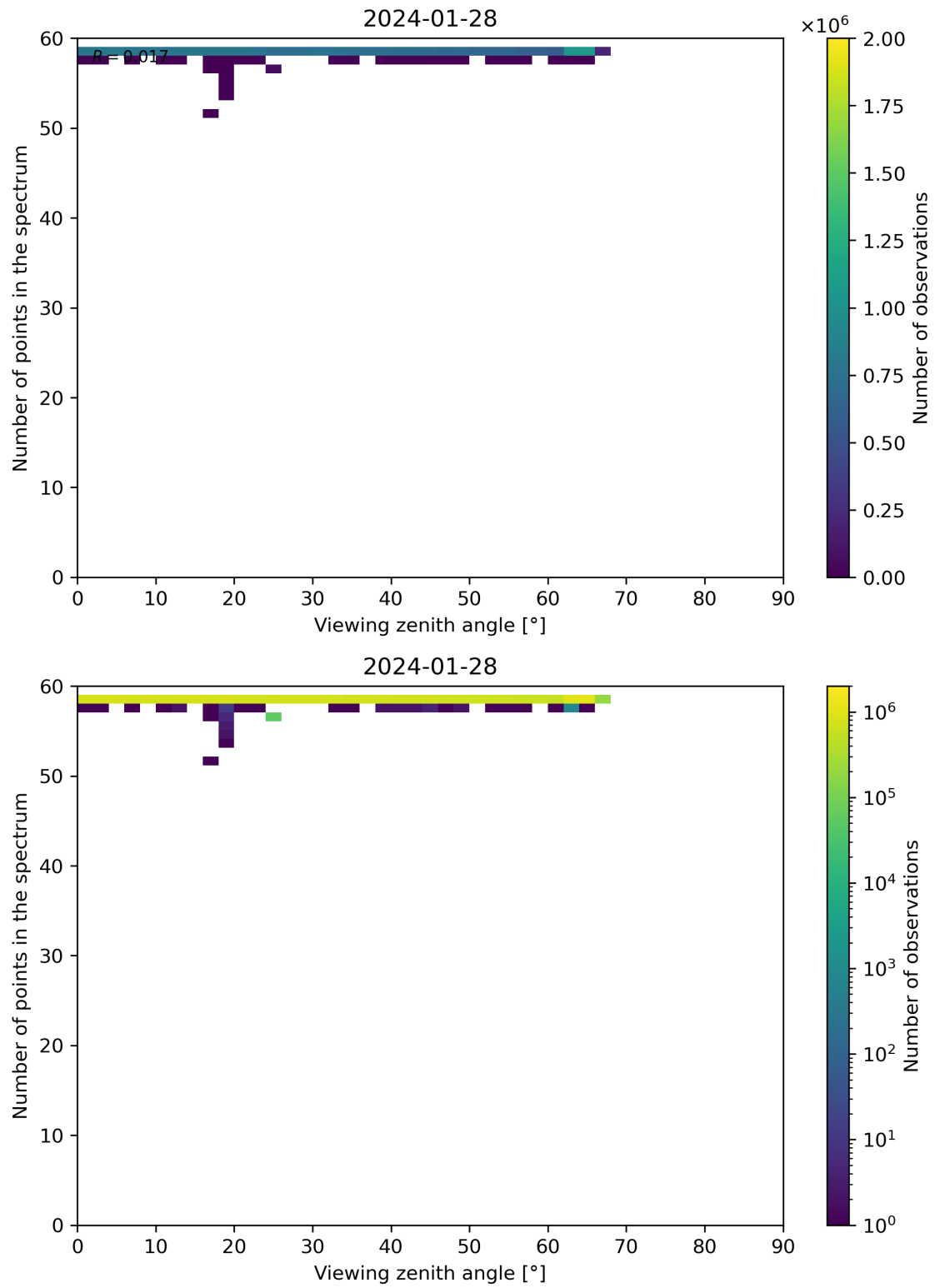
Figure 125: Scatter density plot of “Viewing zenith angle” against “Number of points in the spectrum” for 2024-01-27 to 2024-01-29.
