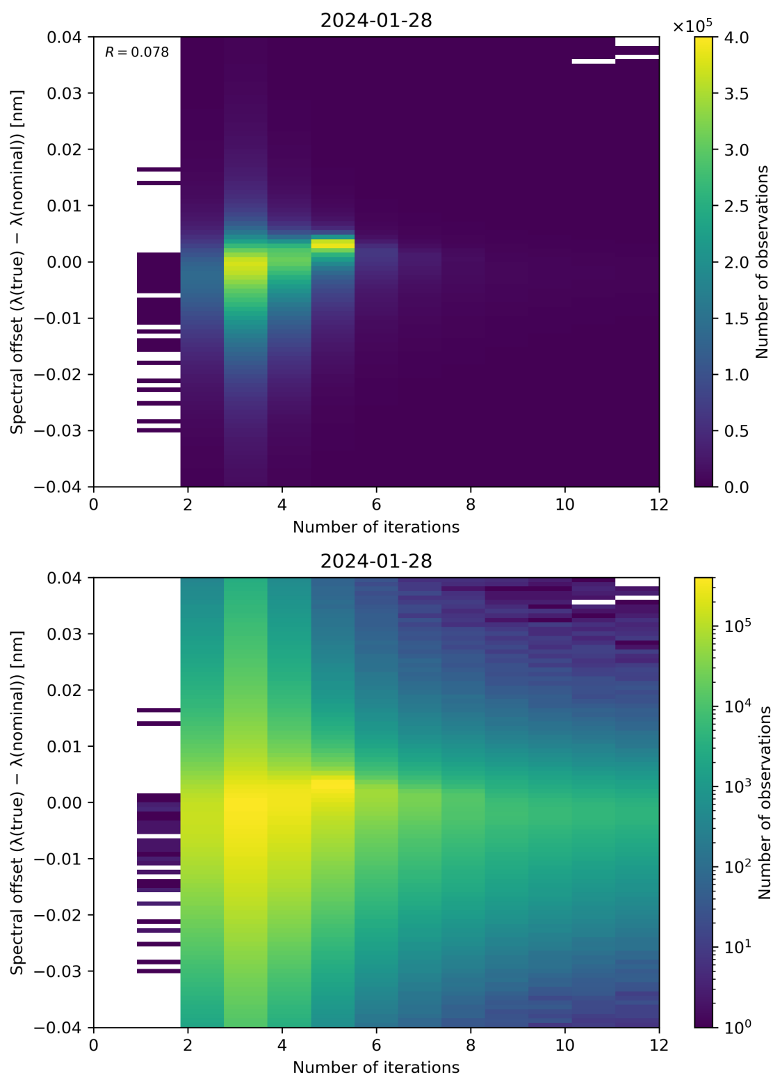
Figure 100: Scatter density plot of “Number of iterations” against “Spectral offset ( \lambda(\text{true}) - \lambda(\text{nominal}) )” for 2024-01-27 to 2024-01-29.
