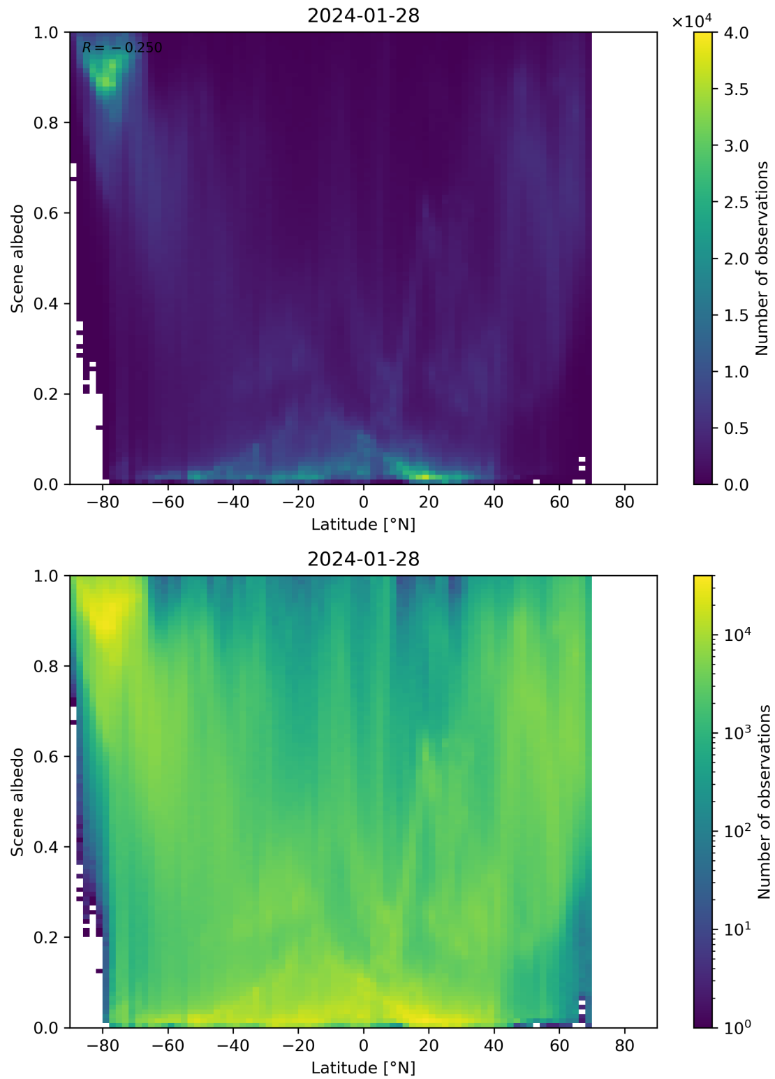
Figure 95: Scatter density plot of “Latitude” against “Scene albedo” for 2024-01-27 to 2024-01-29.
