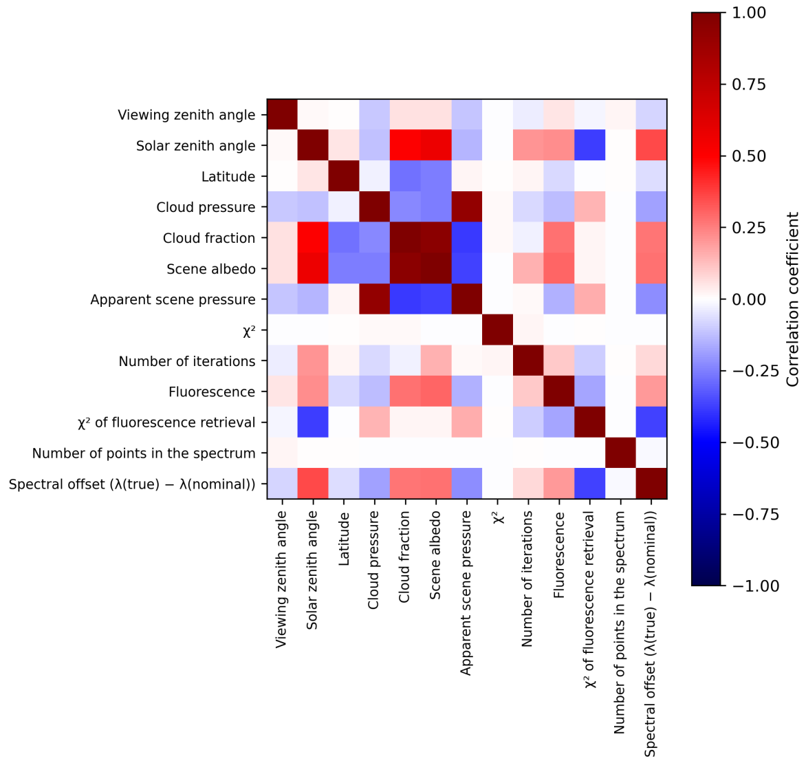
Figure 2: Map of correlation matrix for 2024-01-27 to 2024-01-29.
