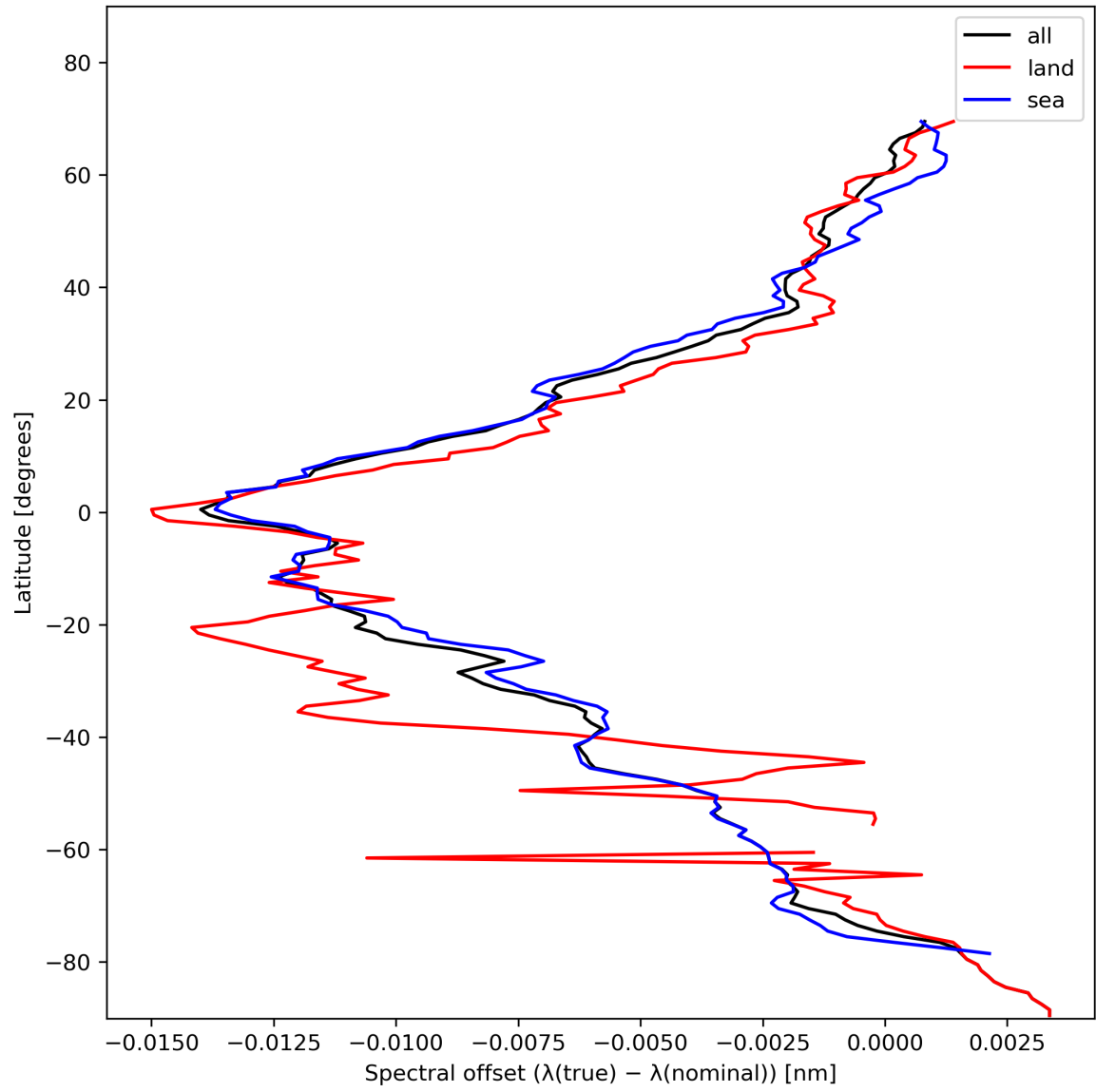
Figure 28: Zonal average of “Spectral offset ( \lambda(\text{true}) - \lambda(\text{nominal}) )” for 2024-01-27 to 2024-01-29.
