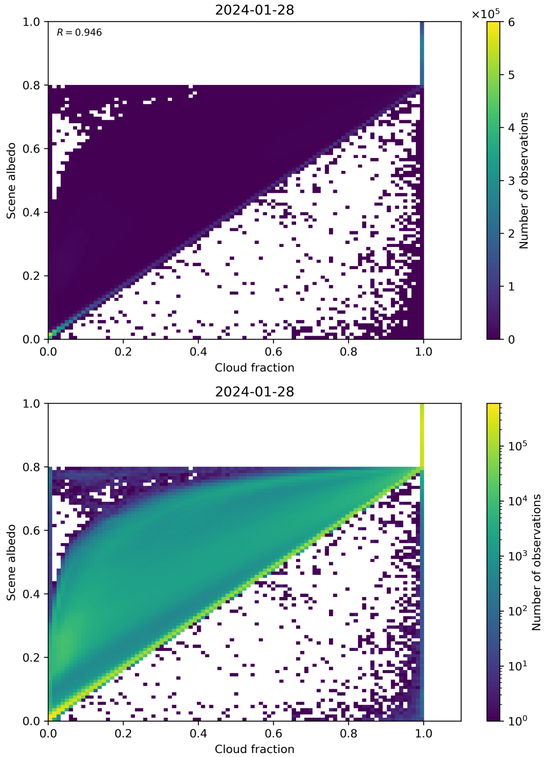
Figure 75: Scatter density plot of “Cloud fraction” against “Scene albedo” for 2024-01-27 to 2024-01-29.
