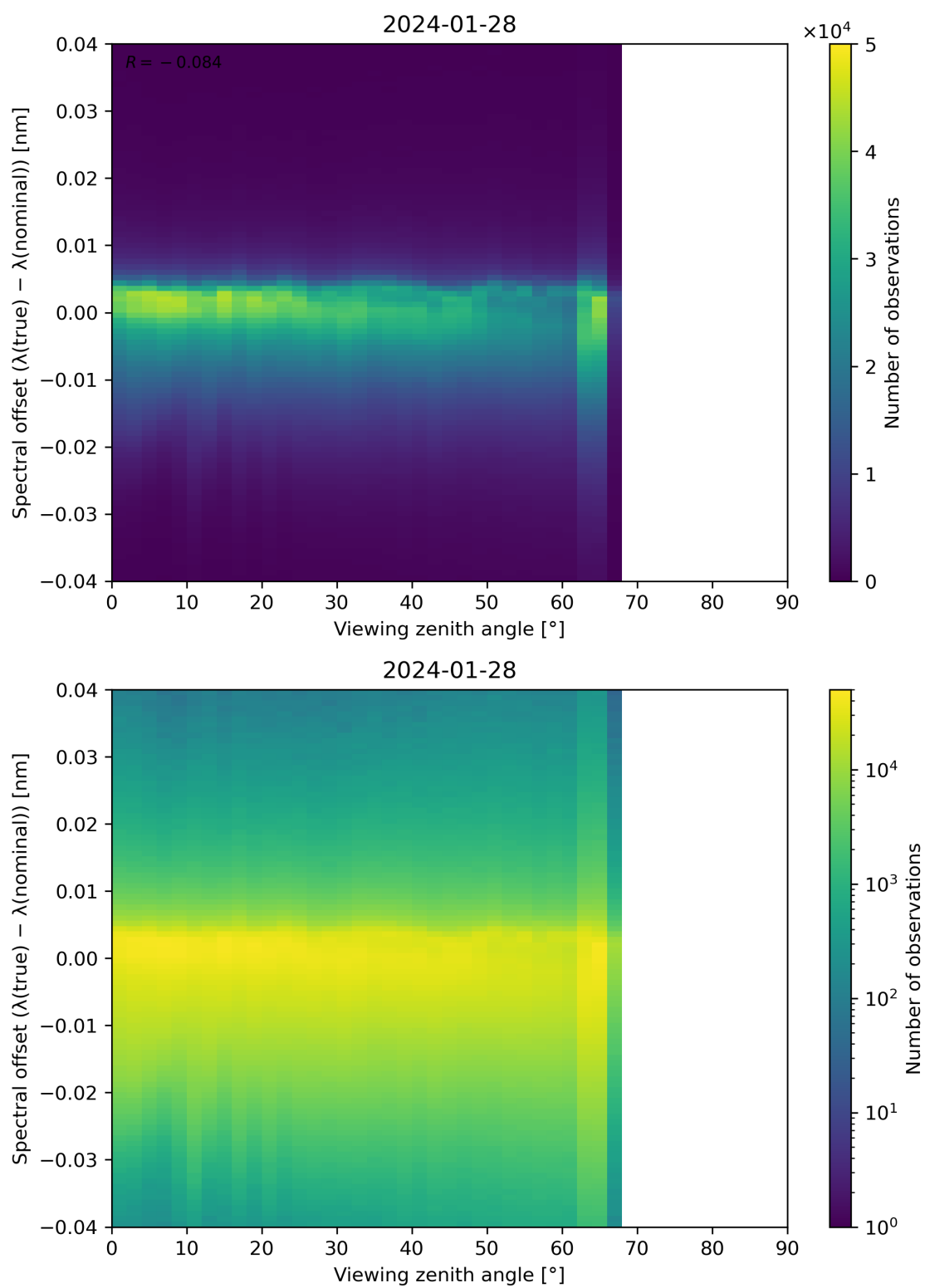
Figure 128: Scatter density plot of “Viewing zenith angle” against “Spectral offset ( \lambda(\text{true}) - \lambda(\text{nominal}) )” for 2024-01-27 to 2024-01-29.
