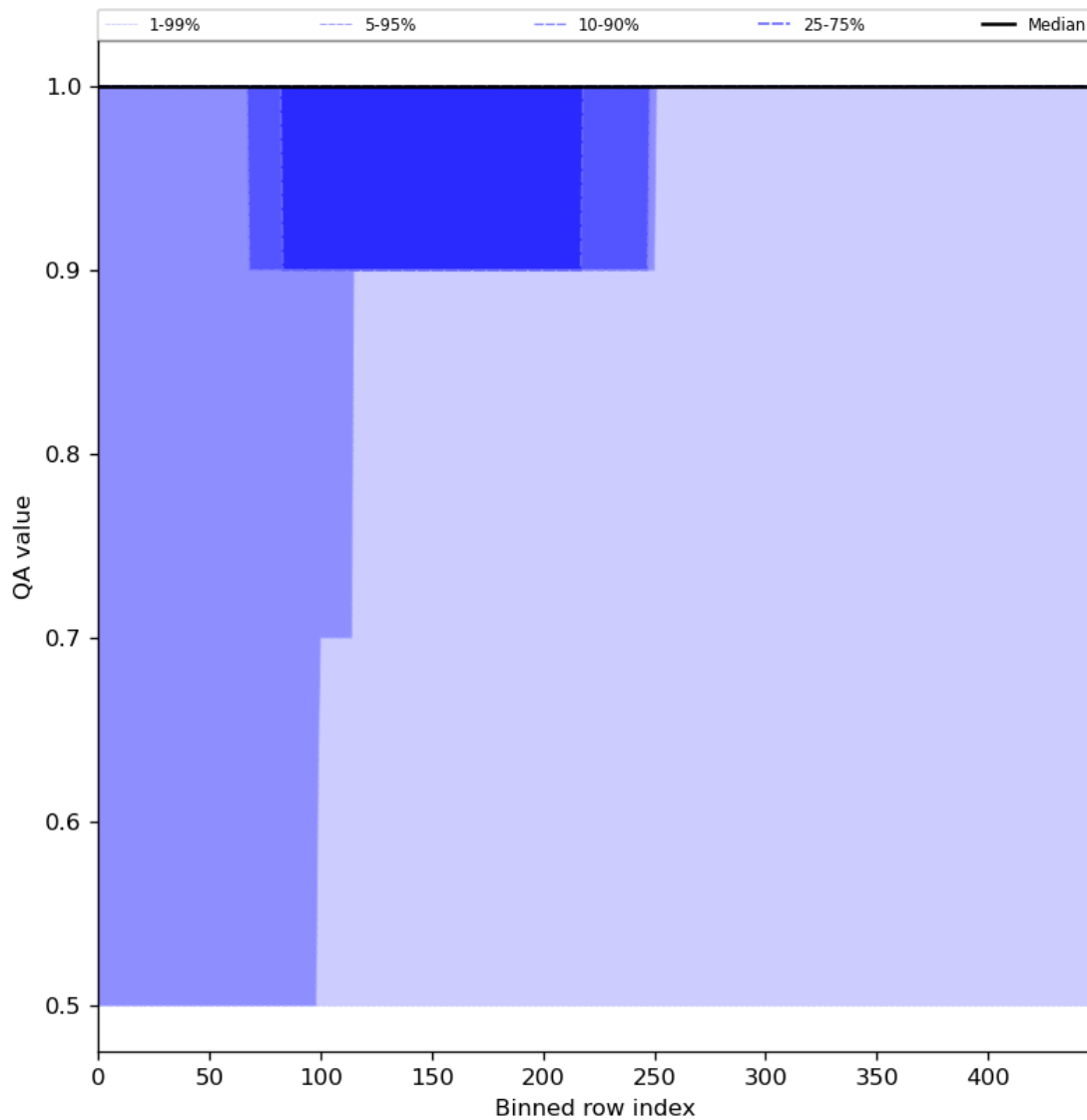
Figure 46: Along track statistics of "QA value" for 2024-01-27 to 2024-01-29
