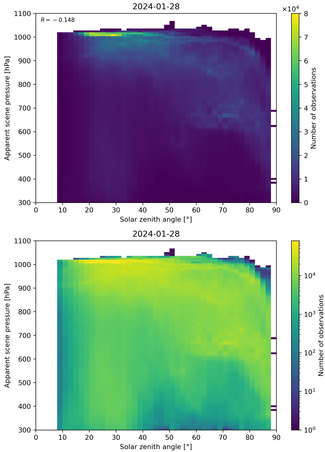
Figure 108: Scatter density plot of “Solar zenith angle” against “Apparent scene pressure” for 2024-01-27 to 2024-01-29.
