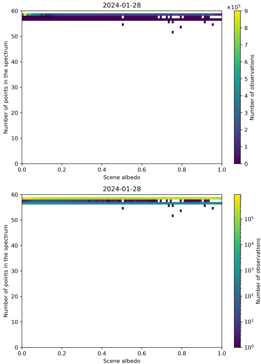
Figure 106: Scatter density plot of “Scene albedo” against “Number of points in the spectrum” for 2024-01-27 to 2024-01-29.
