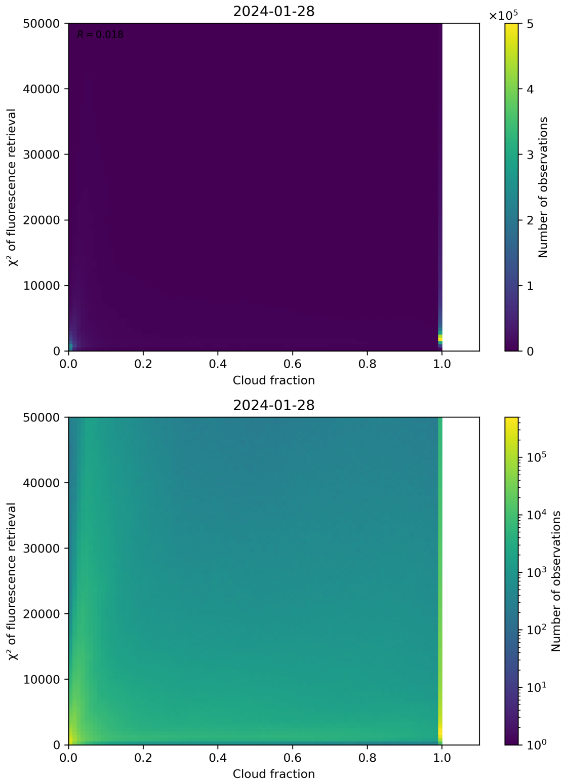
Figure 71: Scatter density plot of “Cloud fraction” against “ \chi^2 of fluorescence retrieval” for 2024-01-27 to 2024-01-29.
