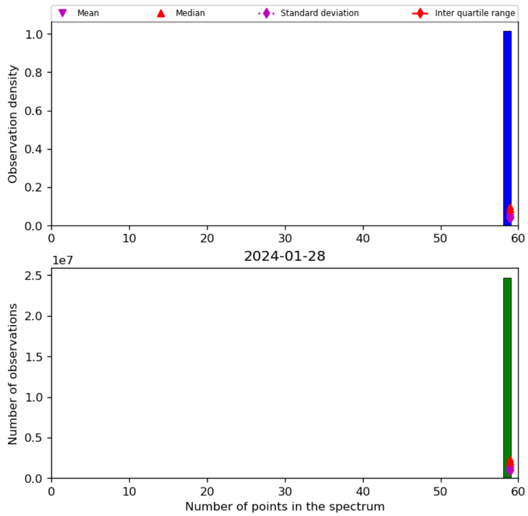
Figure 44: Histogram of “Number of points in the spectrum” for 2024-01-27 to 2024-01-29
