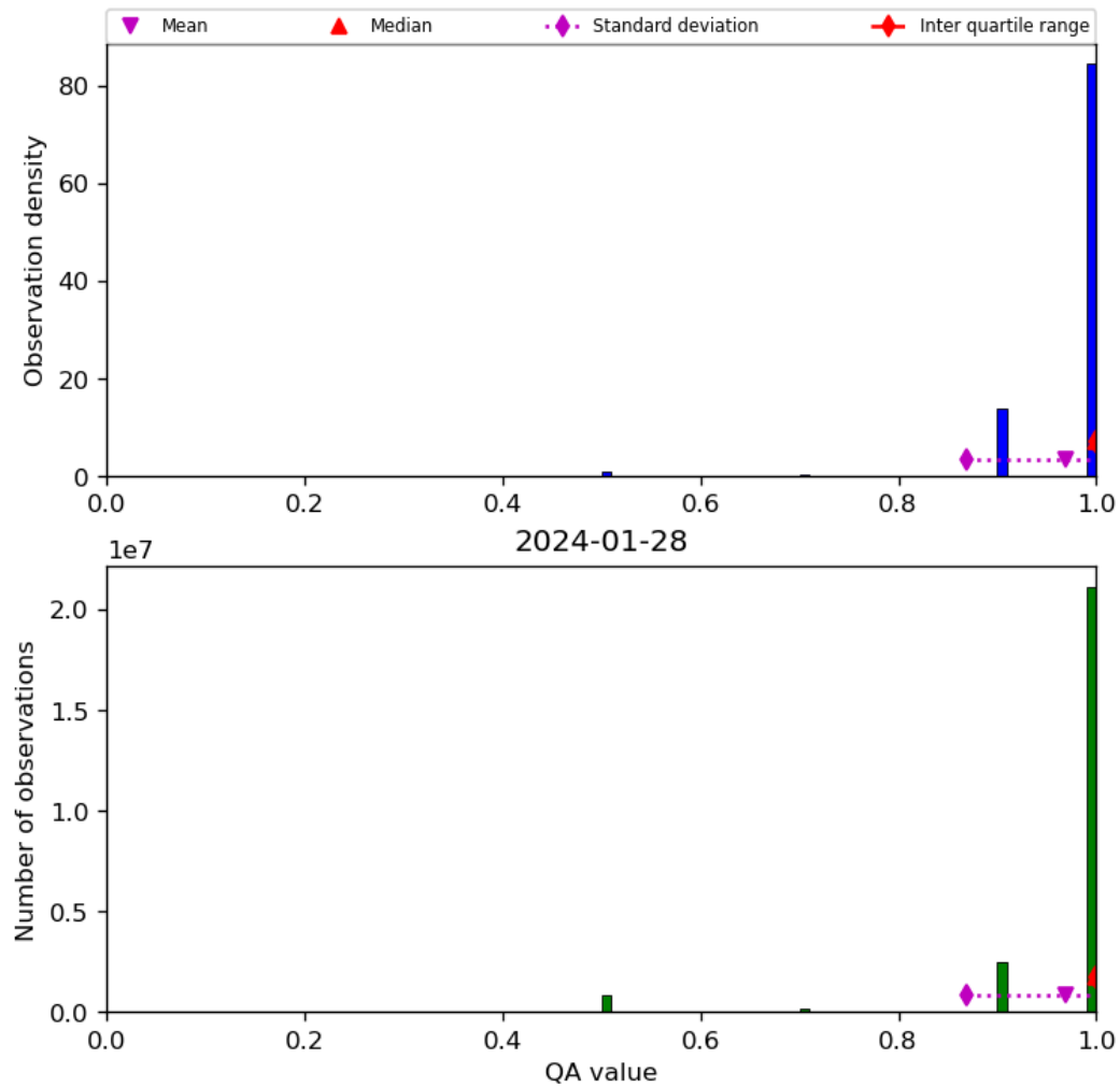
Figure 29: Histogram of “QA value” for 2024-01-27 to 2024-01-29
