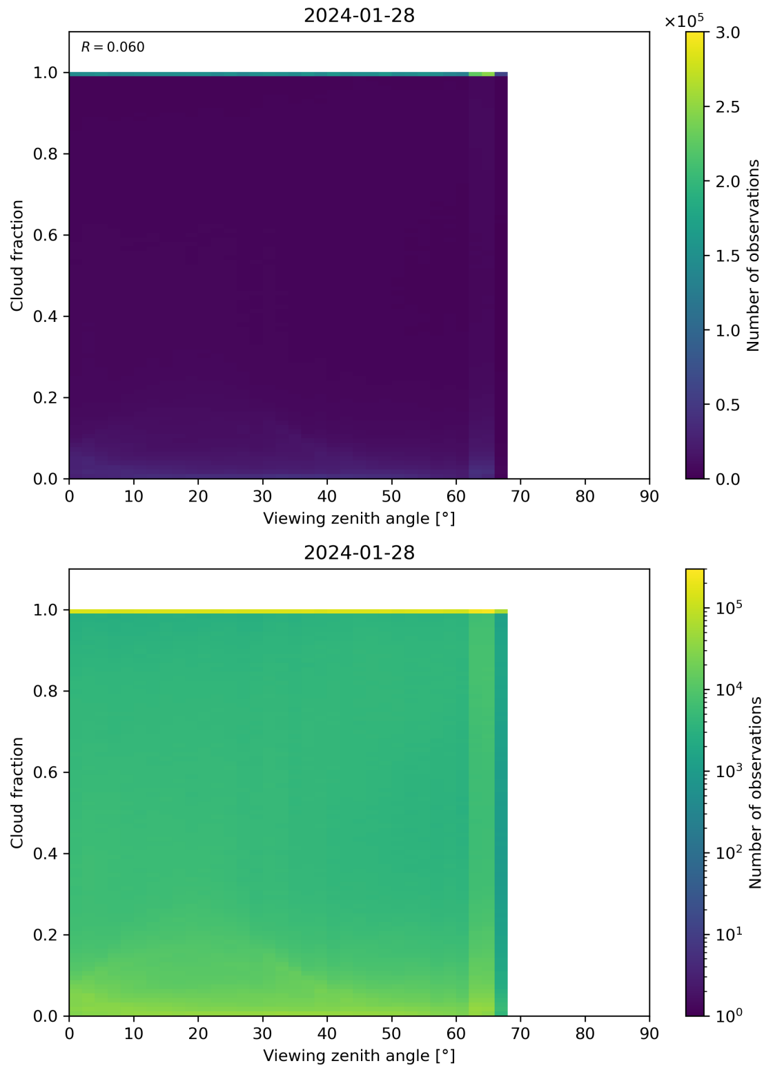
Figure 120: Scatter density plot of “Viewing zenith angle” against “Cloud fraction” for 2024-01-27 to 2024-01-29.
