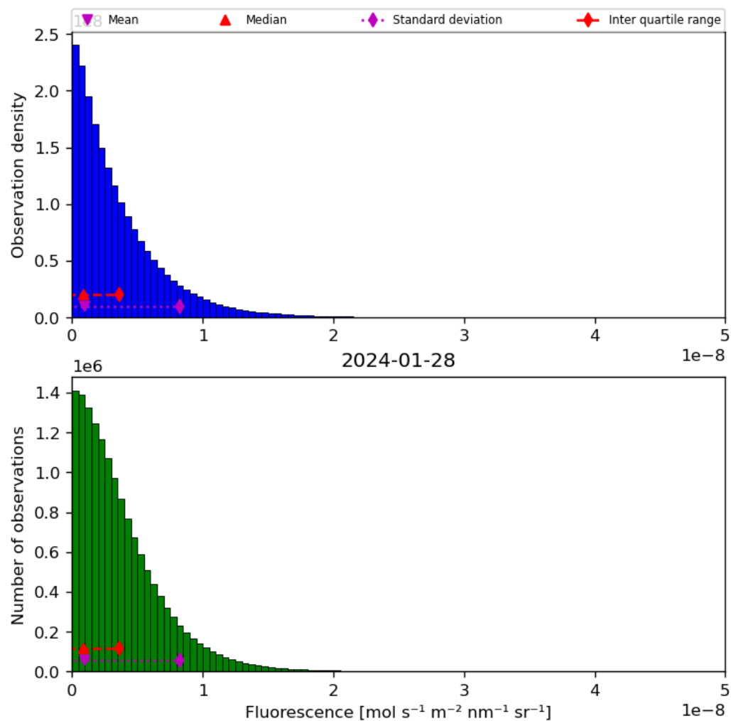
Figure 40: Histogram of “Fluorescence” for 2024-01-27 to 2024-01-29
