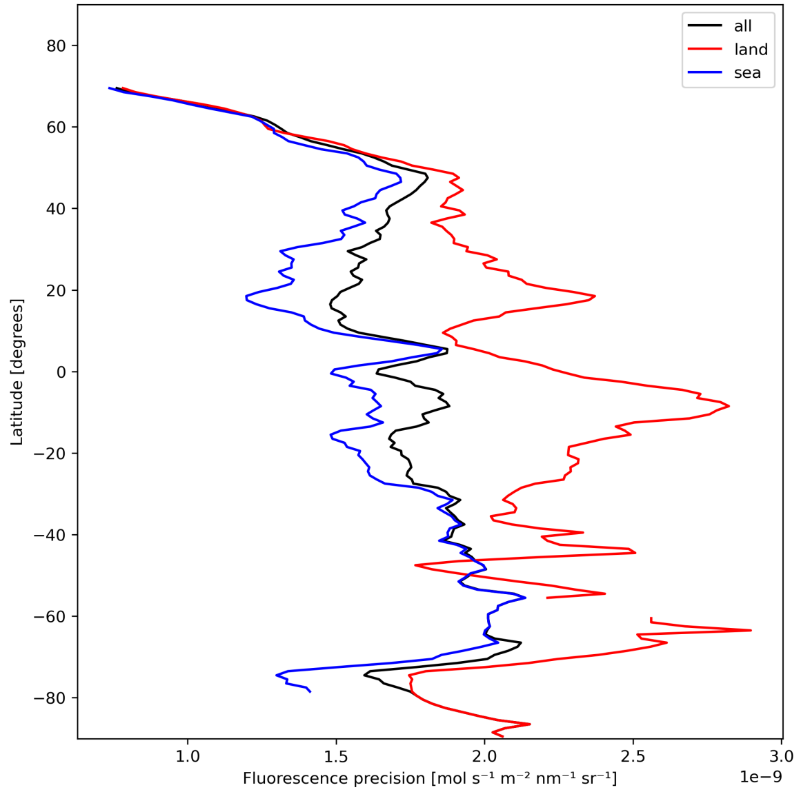
Figure 24: Zonal average of “Fluorescence precision” for 2024-01-27 to 2024-01-29.
