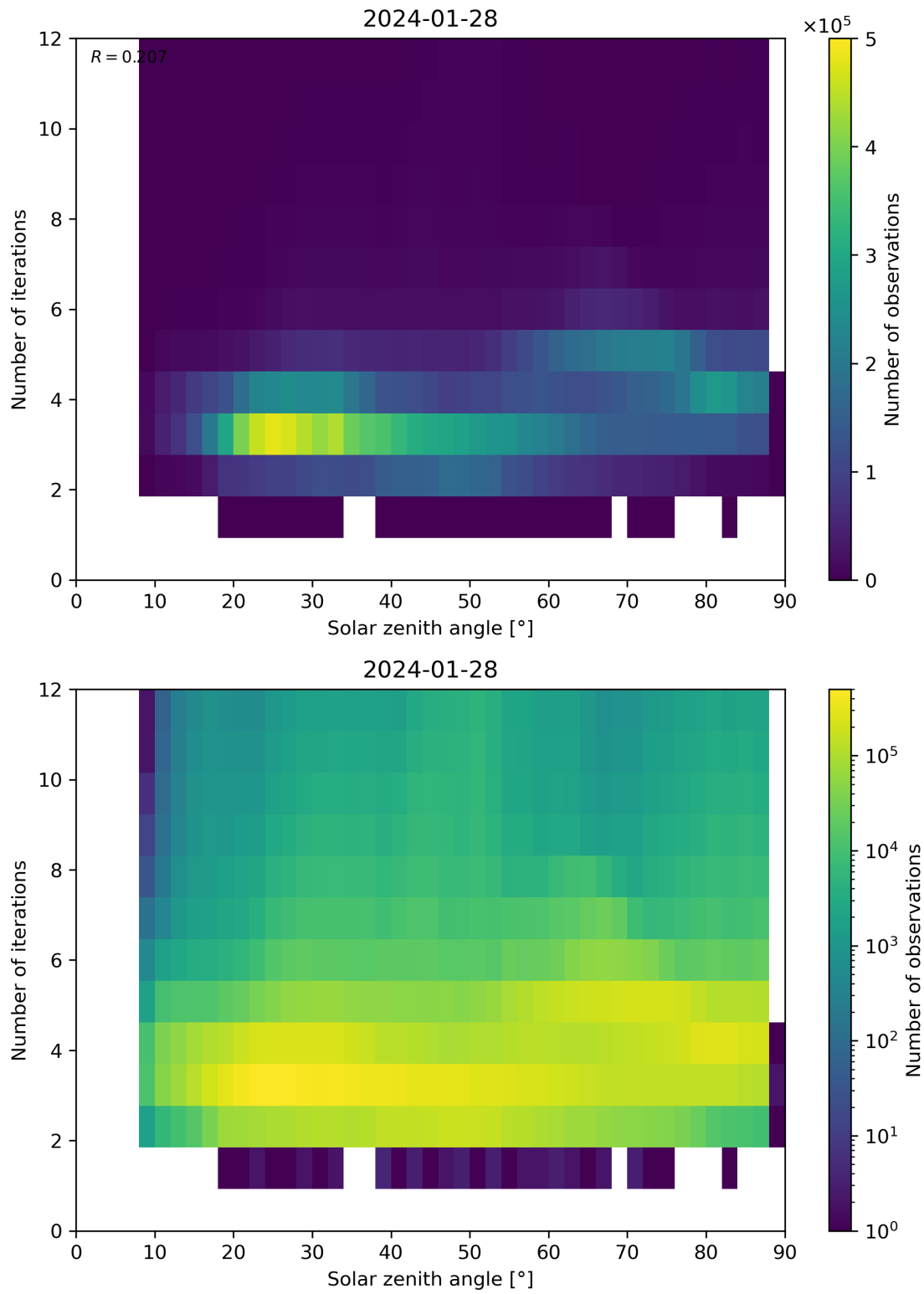
Figure 114: Scatter density plot of “Solar zenith angle” against “Number of iterations” for 2024-01-27 to 2024-01-29.
