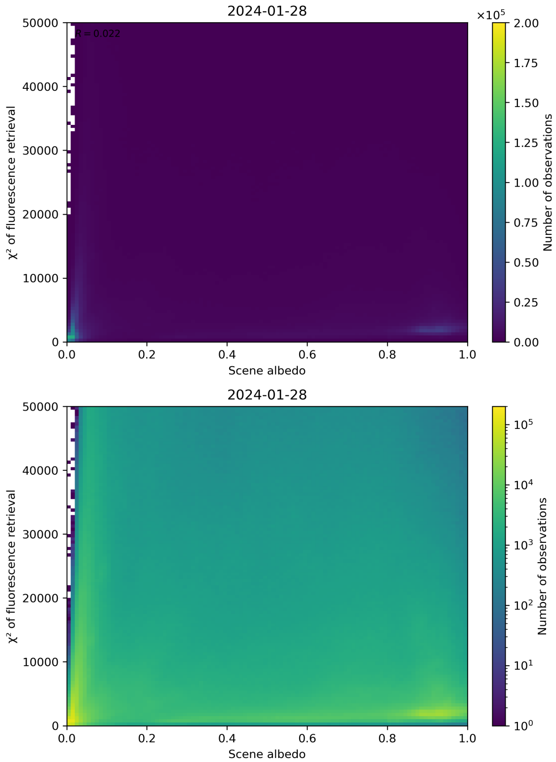
Figure 103: Scatter density plot of “Scene albedo” against “ \chi^2 of fluorescence retrieval” for 2024-01-27 to 2024-01-29.
