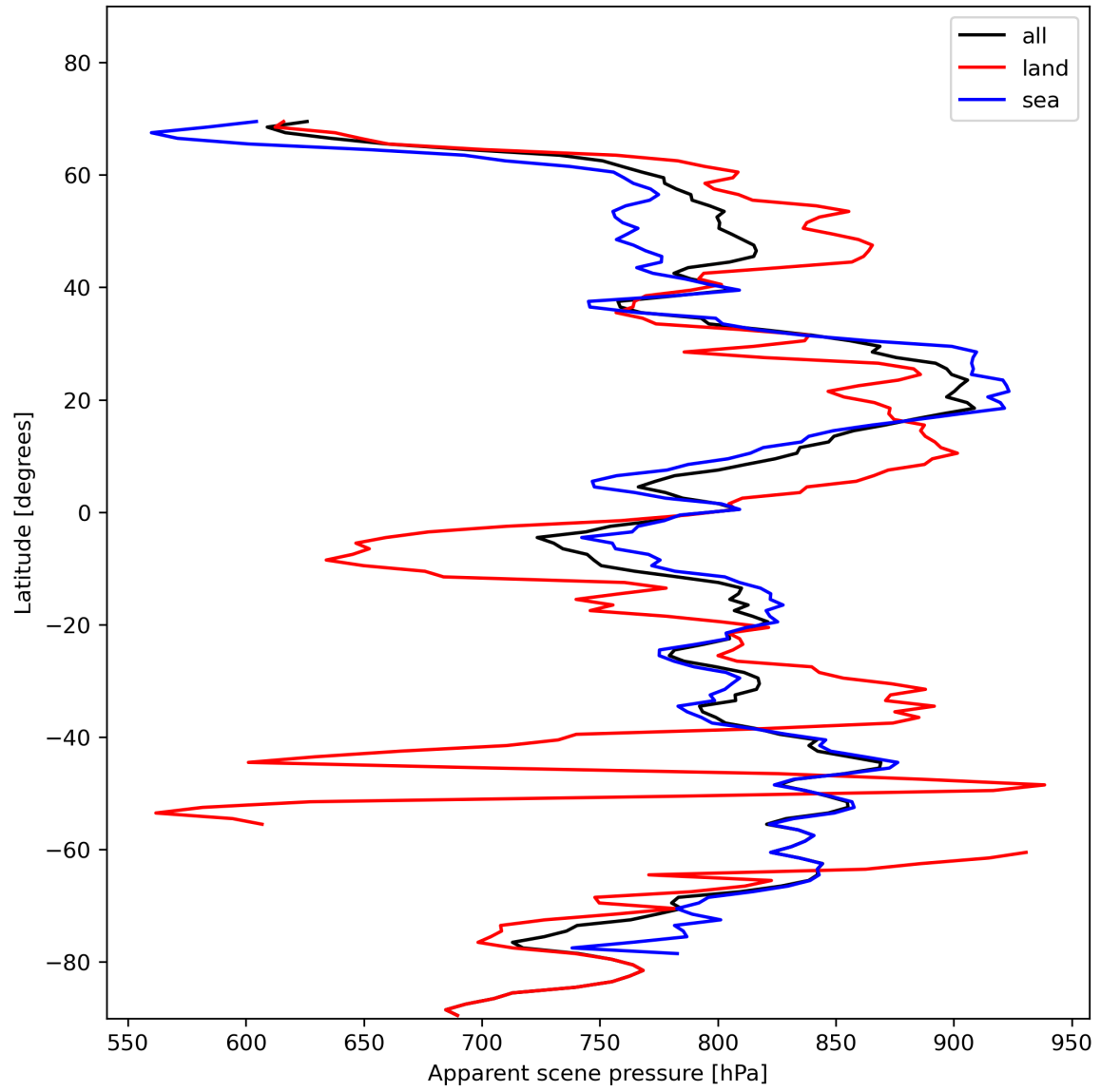
Figure 19: Zonal average of “Apparent scene pressure” for 2024-01-27 to 2024-01-29.
