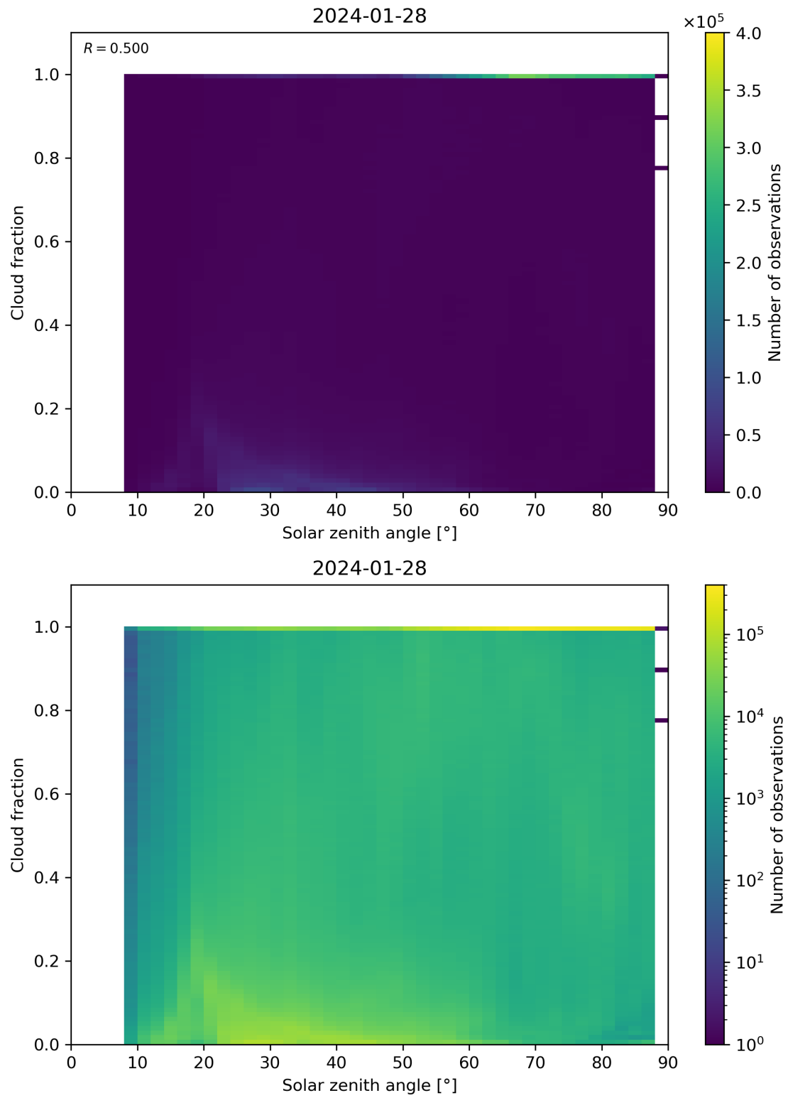
Figure 110: Scatter density plot of “Solar zenith angle” against “Cloud fraction” for 2024-01-27 to 2024-01-29.
