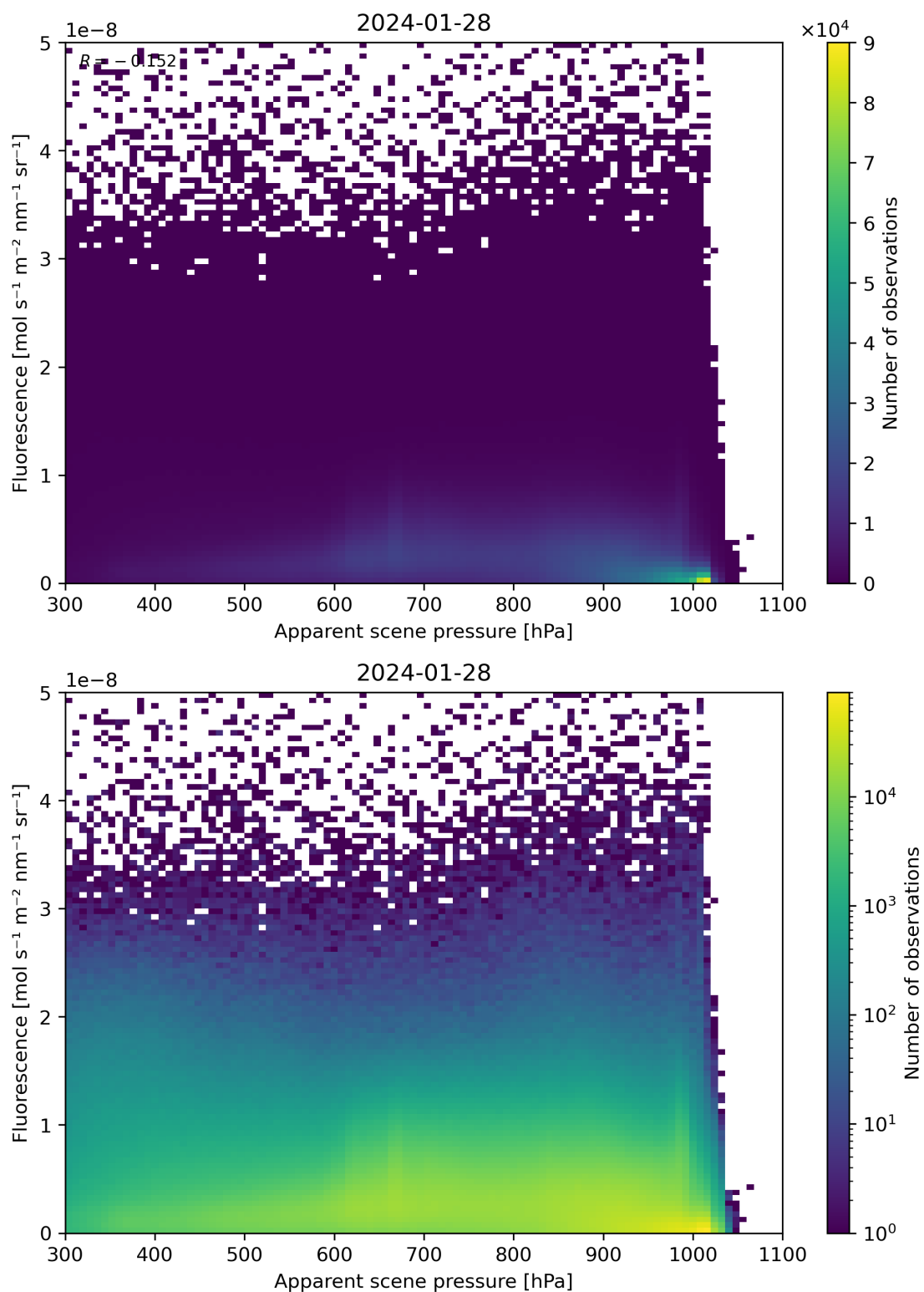
Figure 64: Scatter density plot of “Apparent scene pressure” against “Fluorescence” for 2024-01-27 to 2024-01-29.
