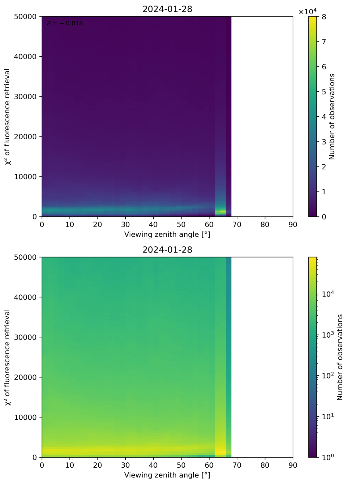
Figure 119: Scatter density plot of “Viewing zenith angle” against “ \chi^2 of fluorescence retrieval” for 2024-01-27 to 2024-01-29.
