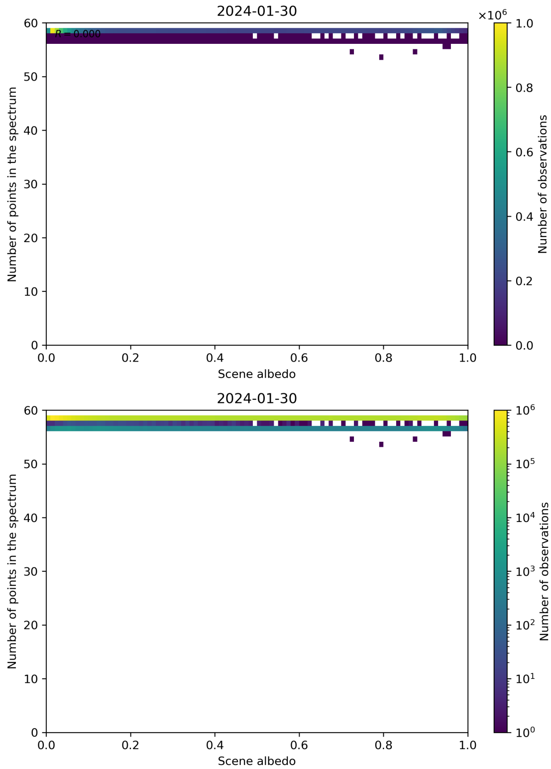
Figure 106: Scatter density plot of “Scene albedo” against “Number of points in the spectrum” for 2024-01-29 to 2024-01-31.
