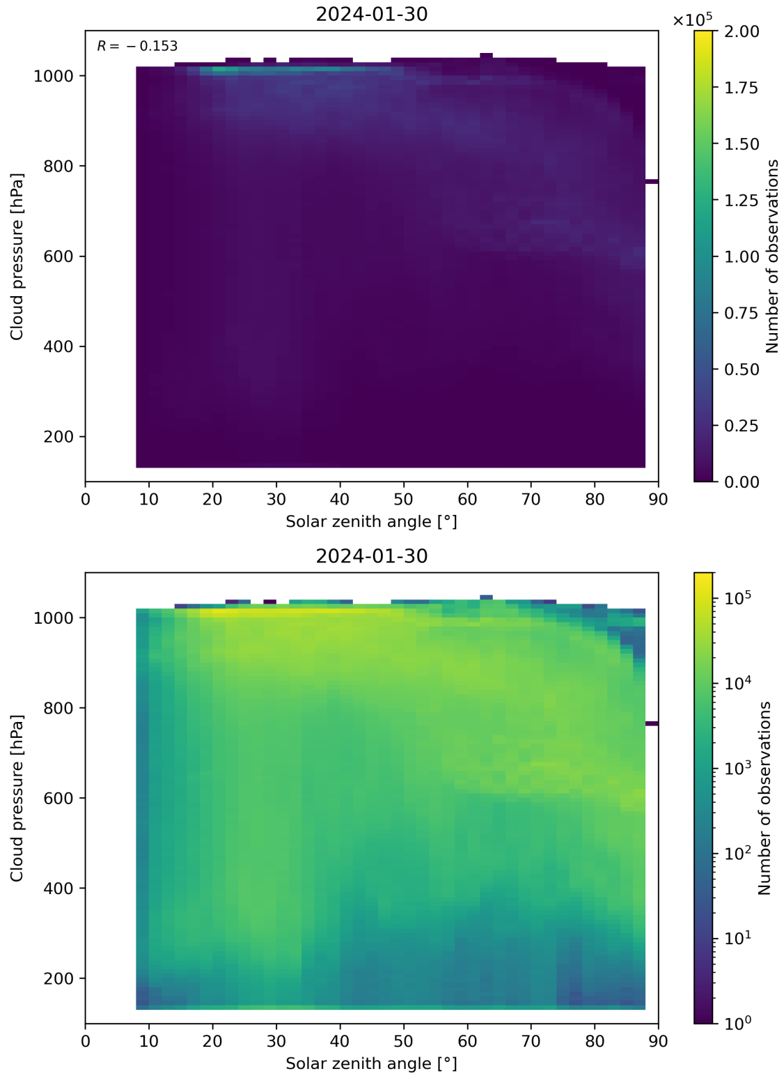
Figure 111: Scatter density plot of “Solar zenith angle” against “Cloud pressure” for 2024-01-29 to 2024-01-31.
