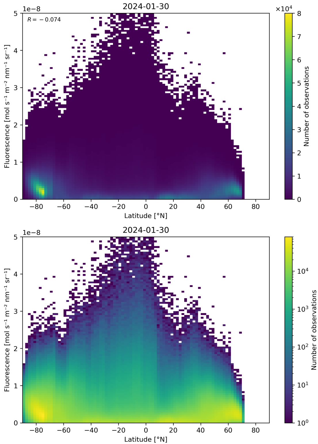
Figure 92: Scatter density plot of “Latitude” against “Fluorescence” for 2024-01-29 to 2024-01-31.
