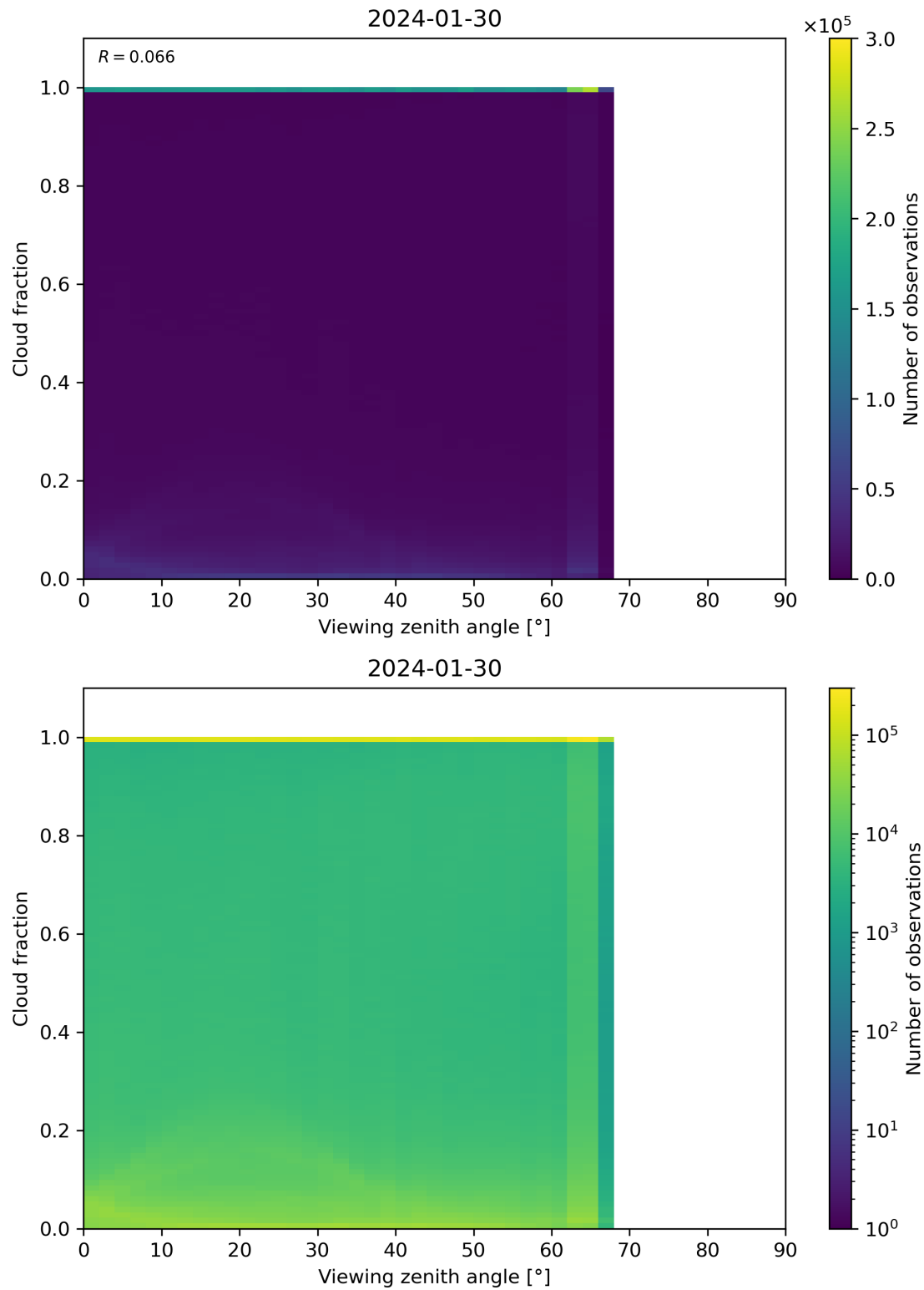
Figure 120: Scatter density plot of “Viewing zenith angle” against “Cloud fraction” for 2024-01-29 to 2024-01-31.
