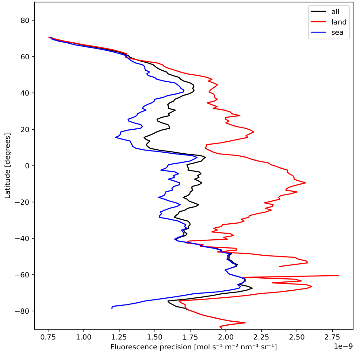
Figure 24: Zonal average of “Fluorescence precision” for 2024-01-29 to 2024-01-31.
