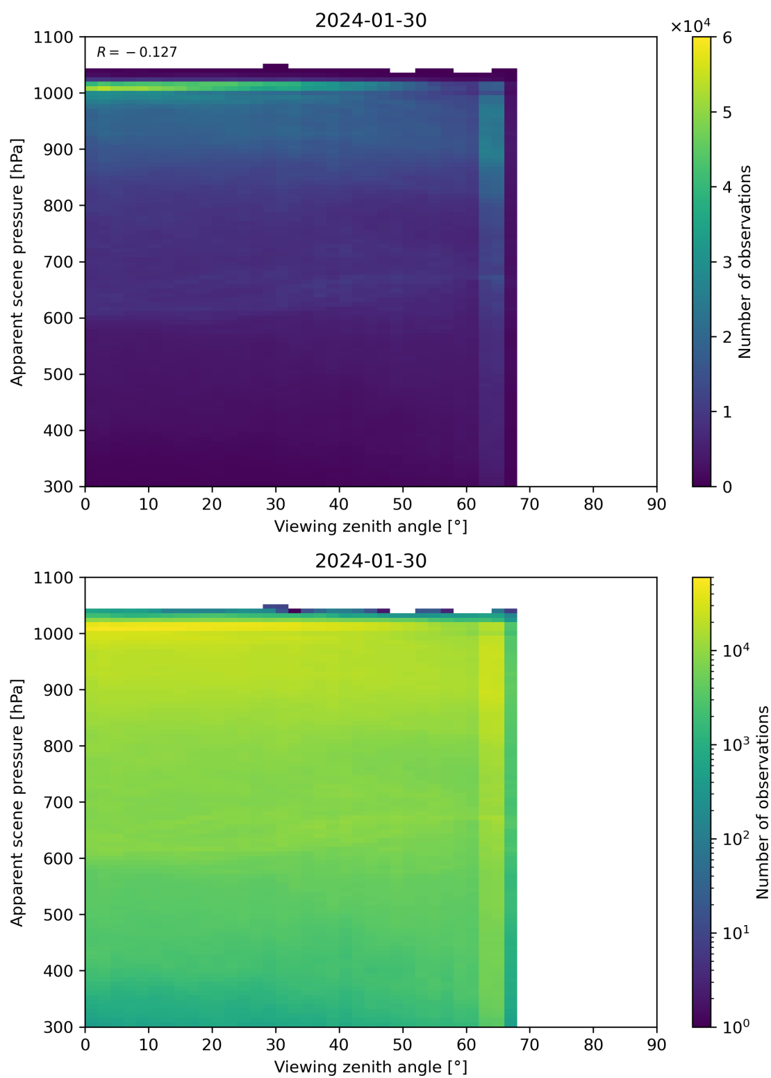
Figure 118: Scatter density plot of “Viewing zenith angle” against “Apparent scene pressure” for 2024-01-29 to 2024-01-31.
