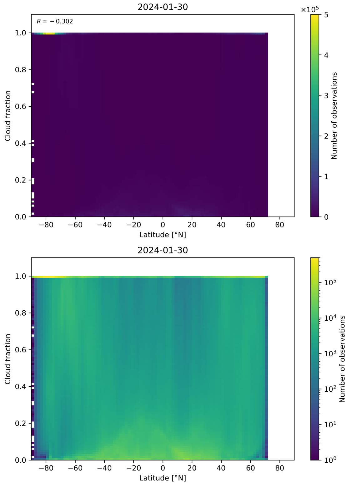
Figure 90: Scatter density plot of “Latitude” against “Cloud fraction” for 2024-01-29 to 2024-01-31.
