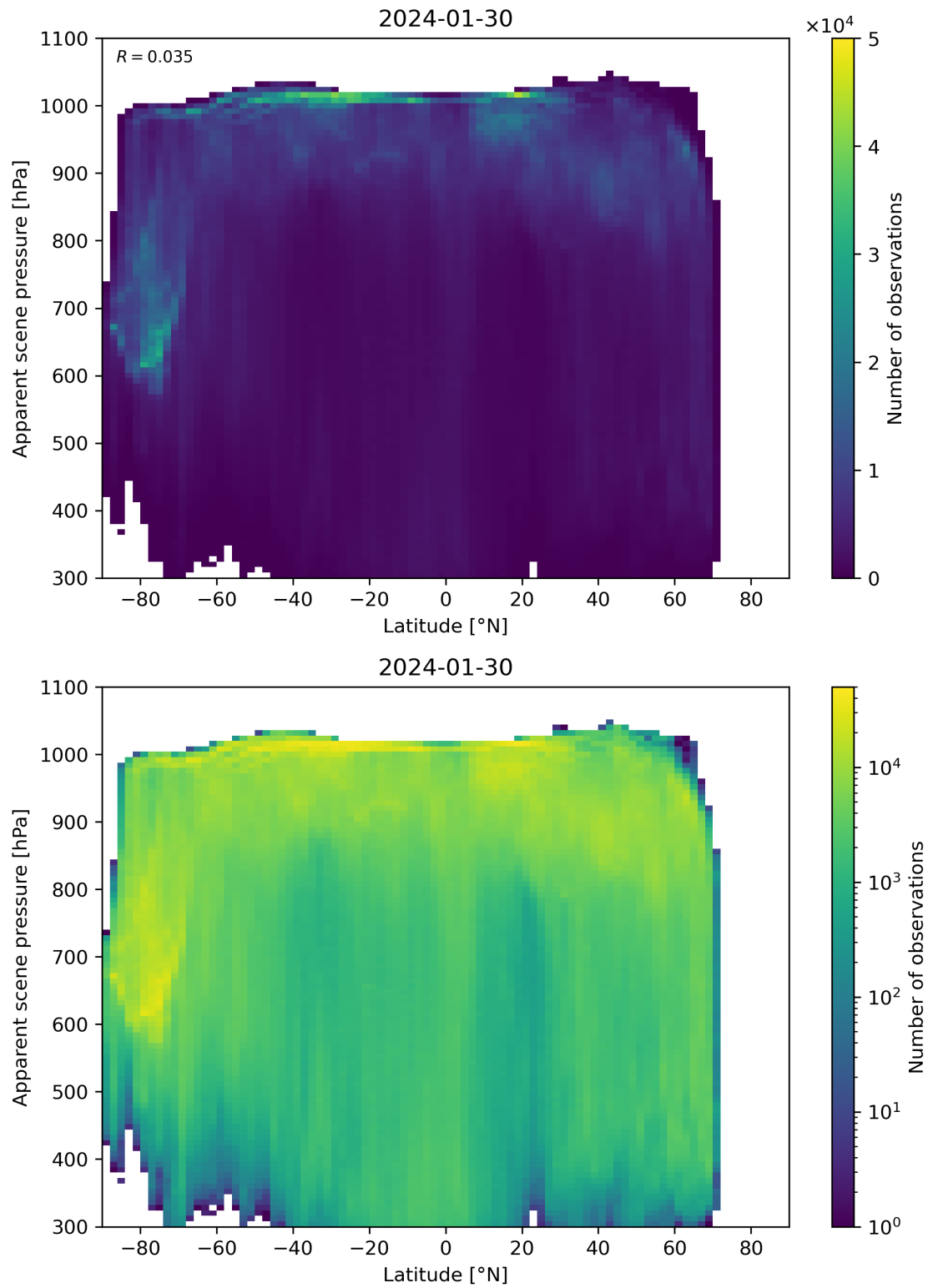
Figure 88: Scatter density plot of “Latitude” against “Apparent scene pressure” for 2024-01-29 to 2024-01-31.
