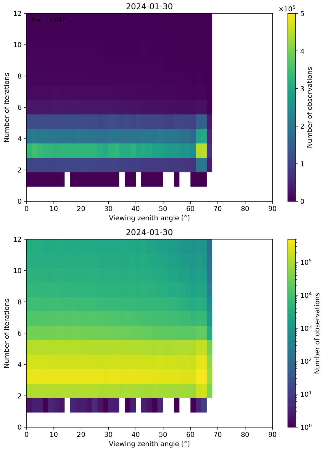
Figure 124: Scatter density plot of “Viewing zenith angle” against “Number of iterations” for 2024-01-29 to 2024-01-31.
