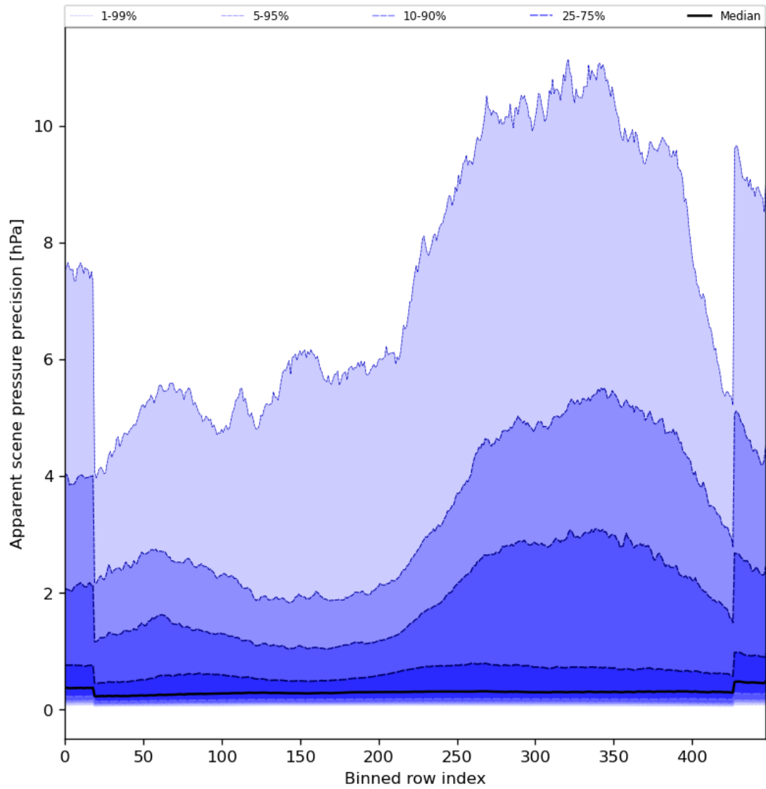
Figure 54: Along track statistics of “Apparent scene pressure precision” for 2024-01-29 to 2024-01-31
