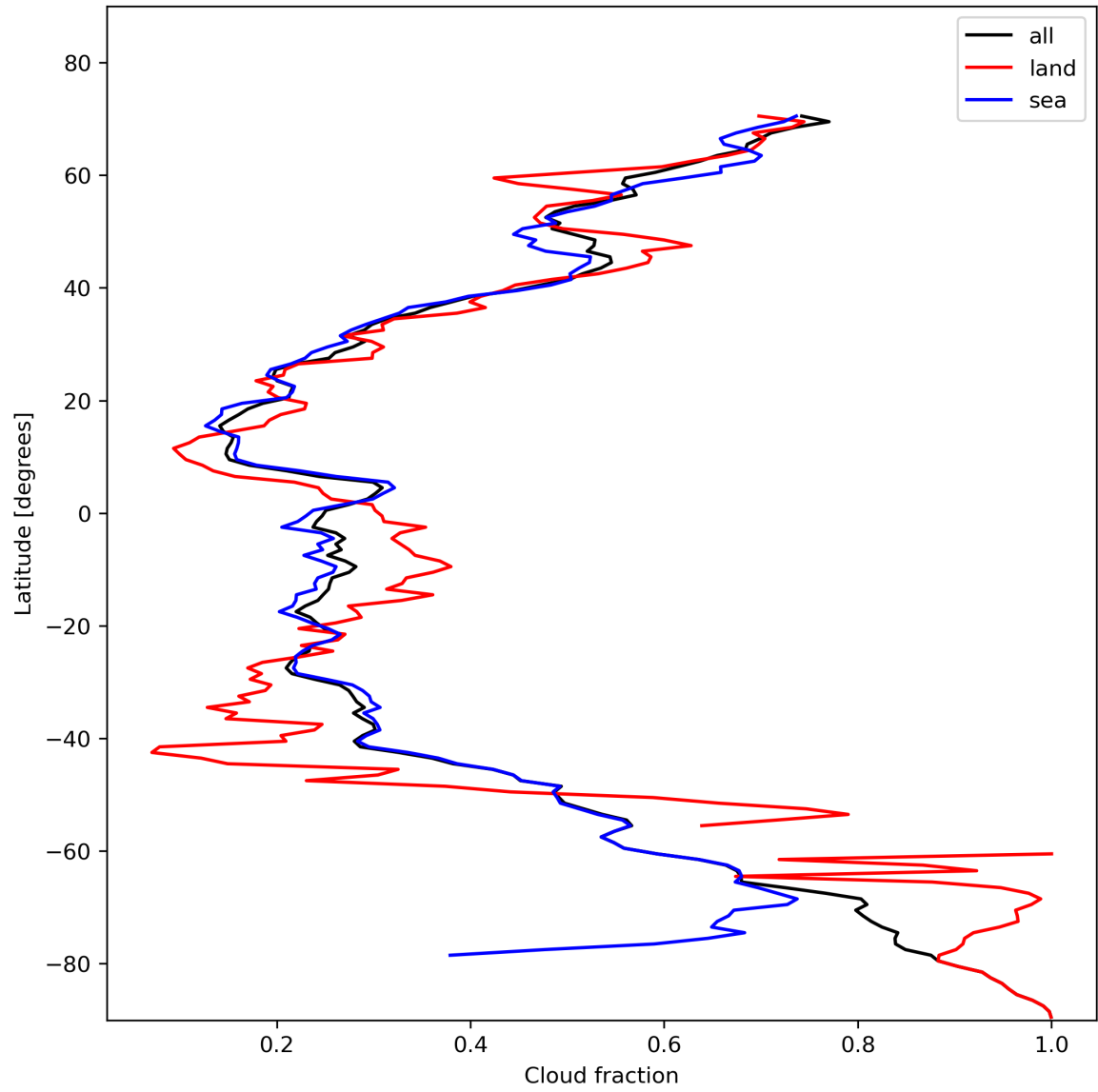
Figure 15: Zonal average of “Cloud fraction” for 2024-01-29 to 2024-01-31.
