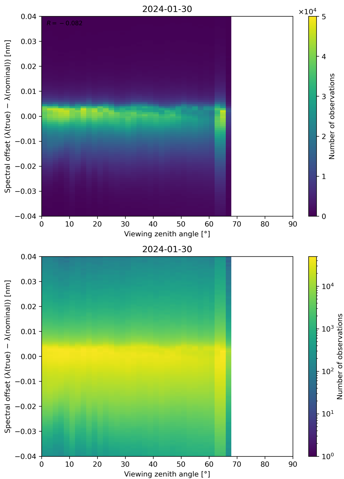
Figure 128: Scatter density plot of “Viewing zenith angle” against “Spectral offset ( \lambda(\text{true}) - \lambda(\text{nominal}) )” for 2024-01-29 to 2024-01-31.
