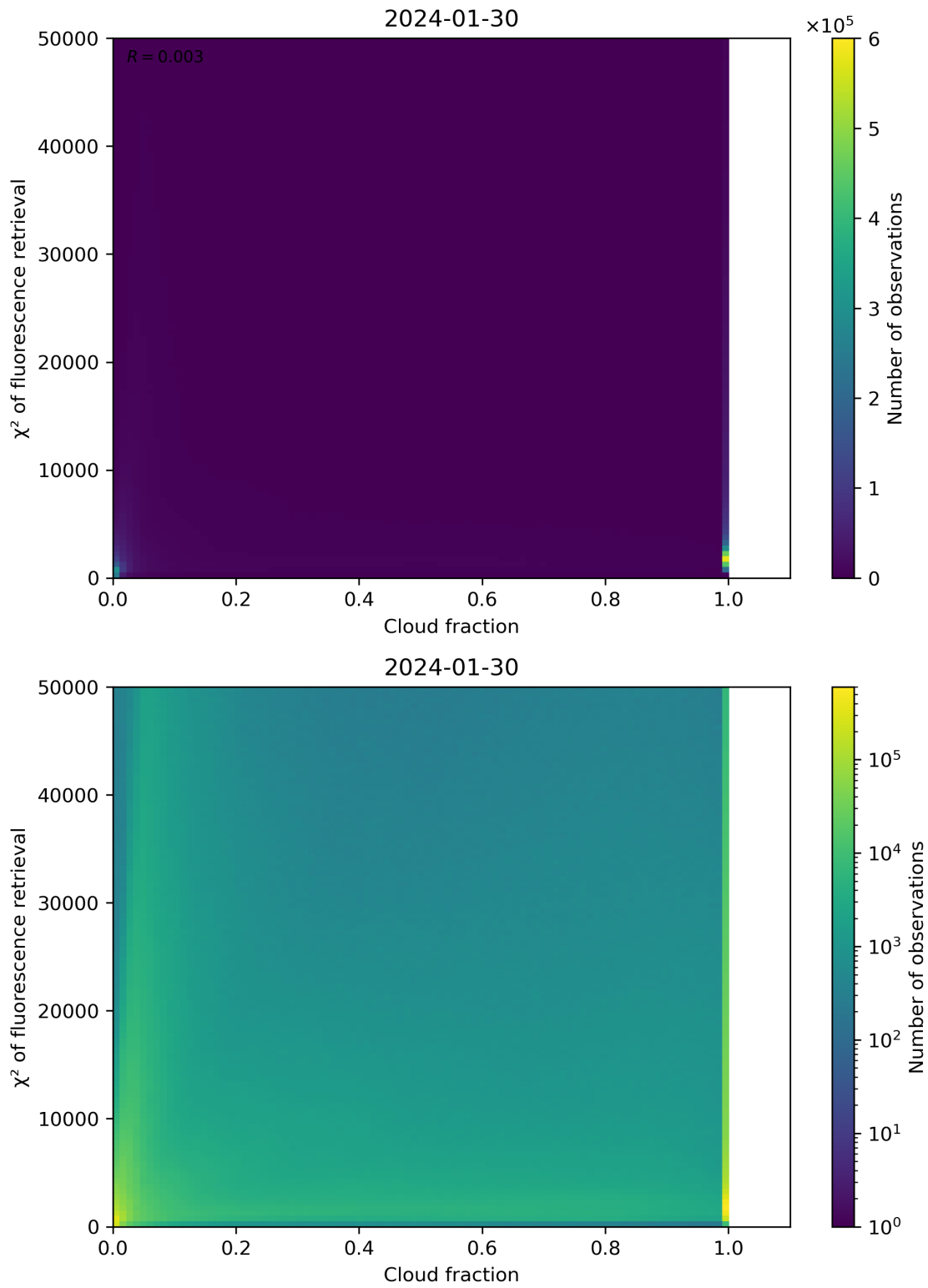
Figure 71: Scatter density plot of “Cloud fraction” against “ \chi^2 of fluorescence retrieval” for 2024-01-29 to 2024-01-31.
