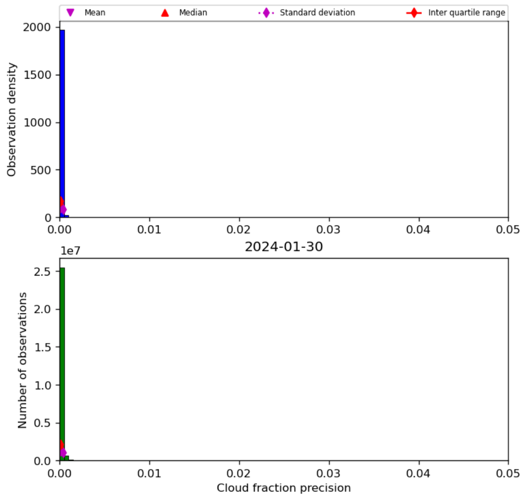
Figure 33: Histogram of “Cloud fraction precision” for 2024-01-29 to 2024-01-31
