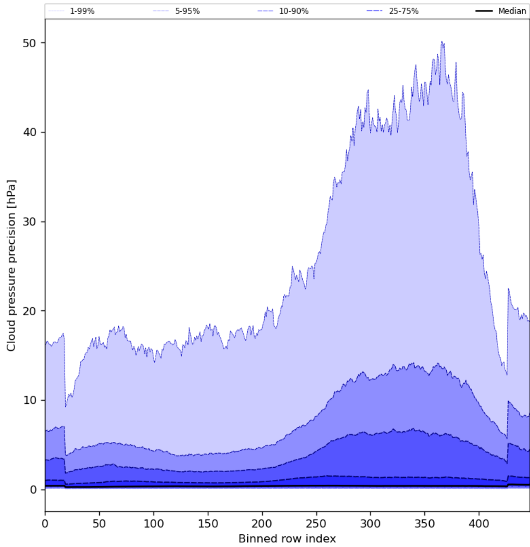
Figure 48: Along track statistics of “Cloud pressure precision” for 2024-01-29 to 2024-01-31
