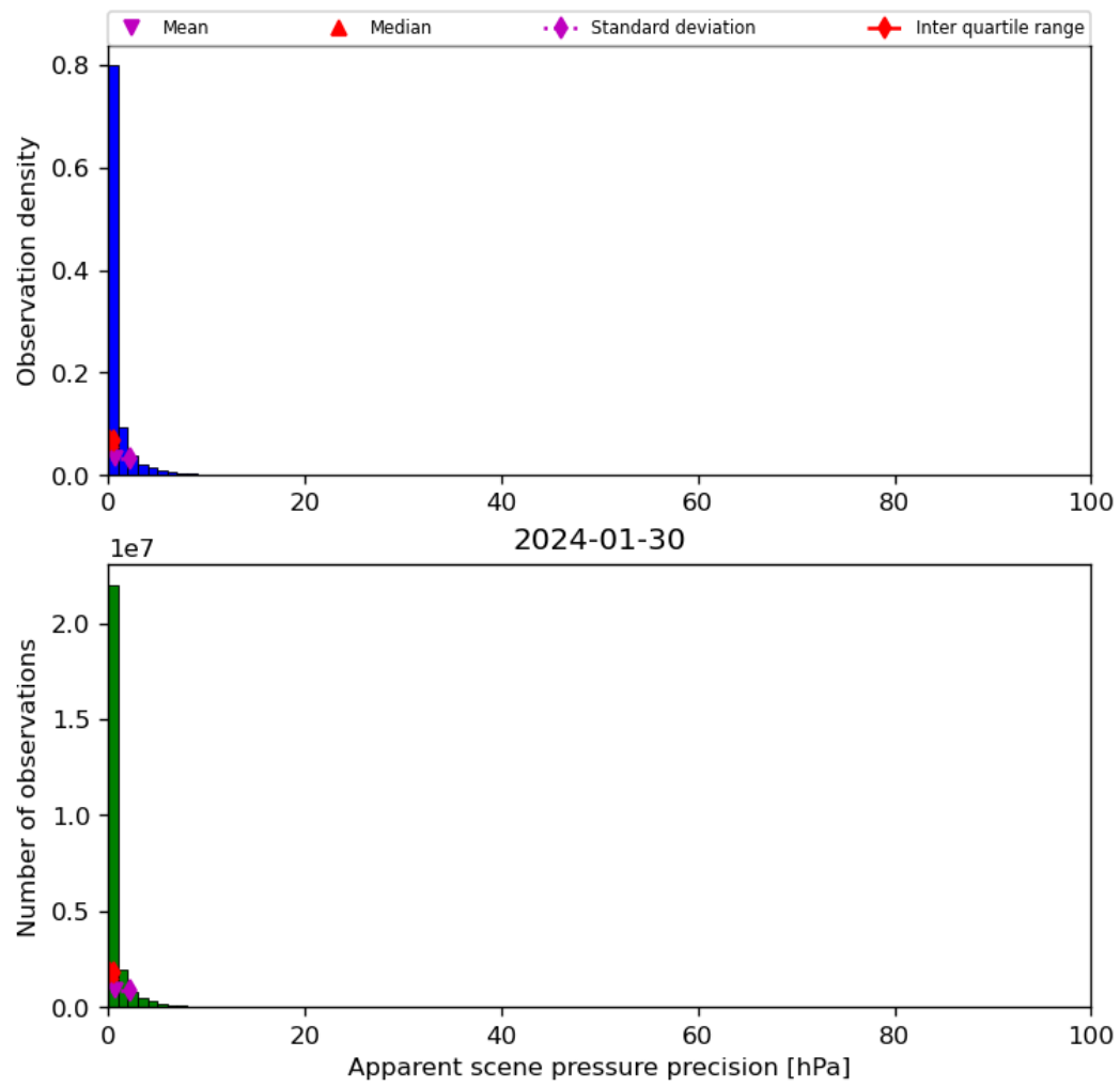
Figure 37: Histogram of “Apparent scene pressure precision” for 2024-01-29 to 2024-01-31
