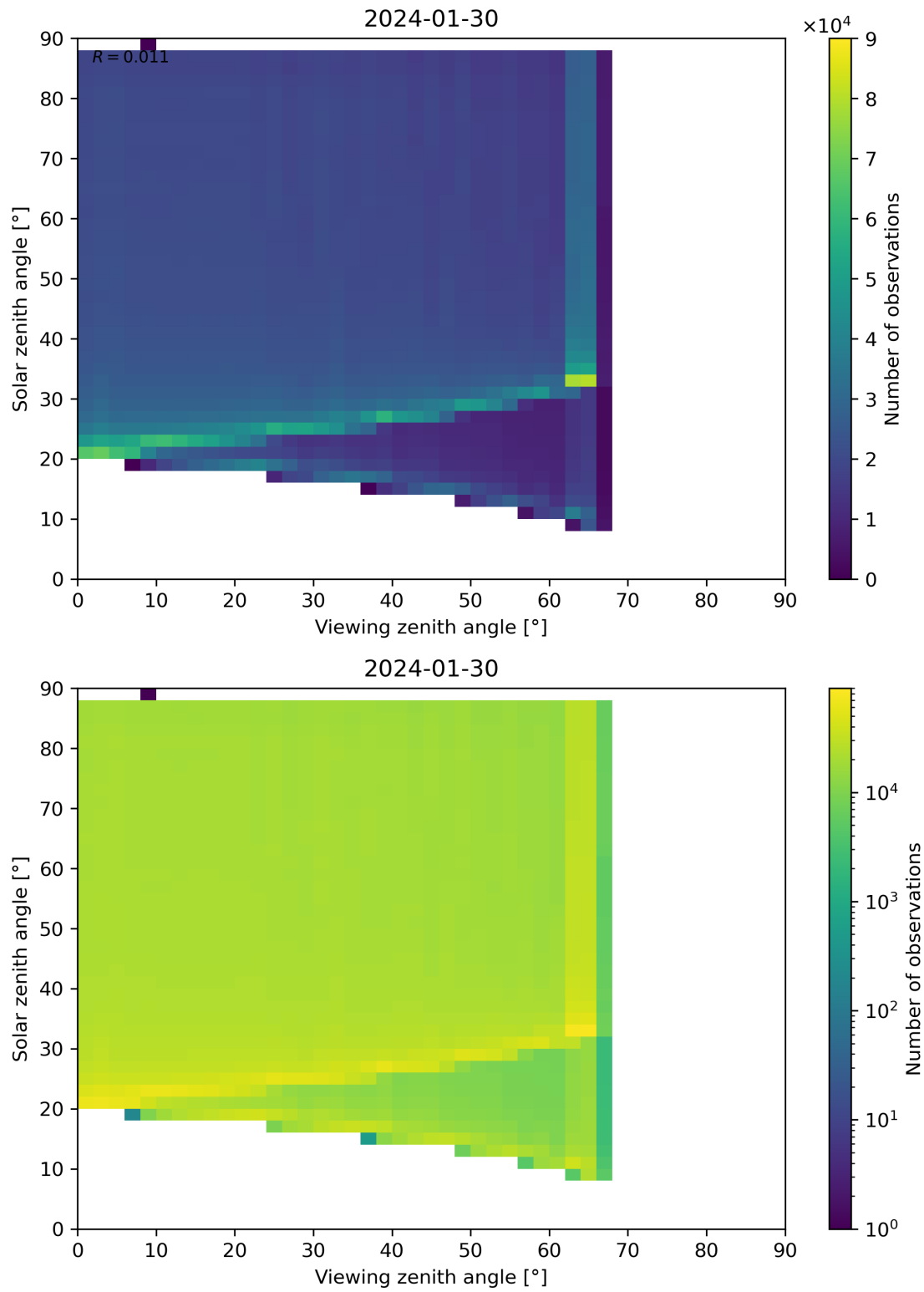
Figure 127: Scatter density plot of “Viewing zenith angle” against “Solar zenith angle” for 2024-01-29 to 2024-01-31.
