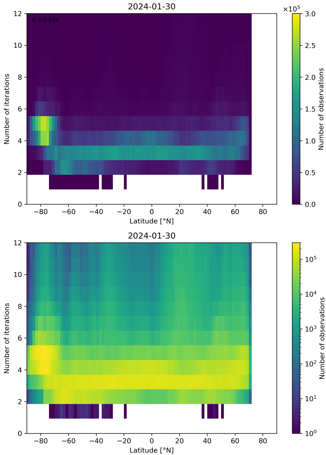
Figure 93: Scatter density plot of “Latitude” against “Number of iterations” for 2024-01-29 to 2024-01-31.
