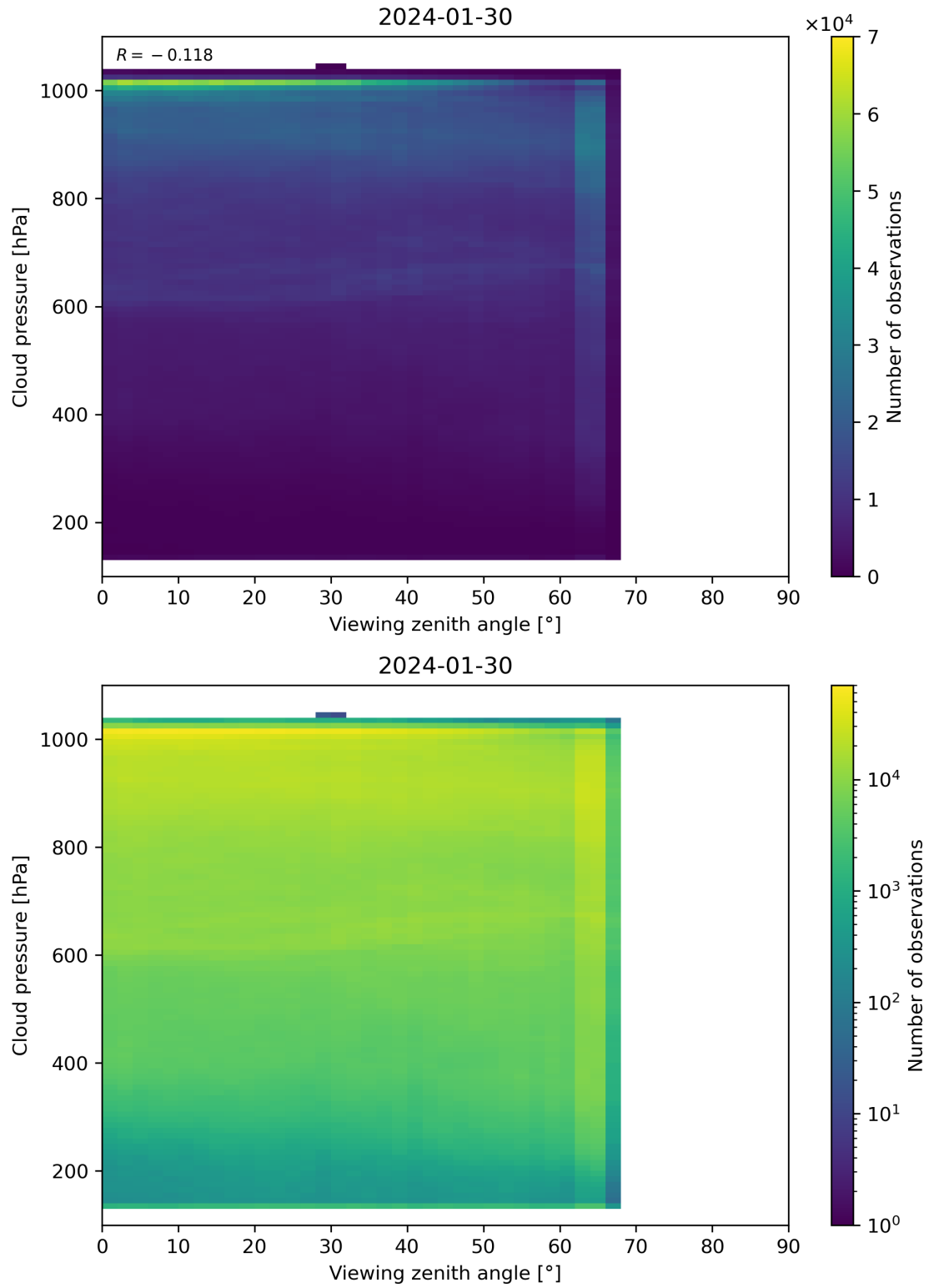
Figure 121: Scatter density plot of “Viewing zenith angle” against “Cloud pressure” for 2024-01-29 to 2024-01-31.
