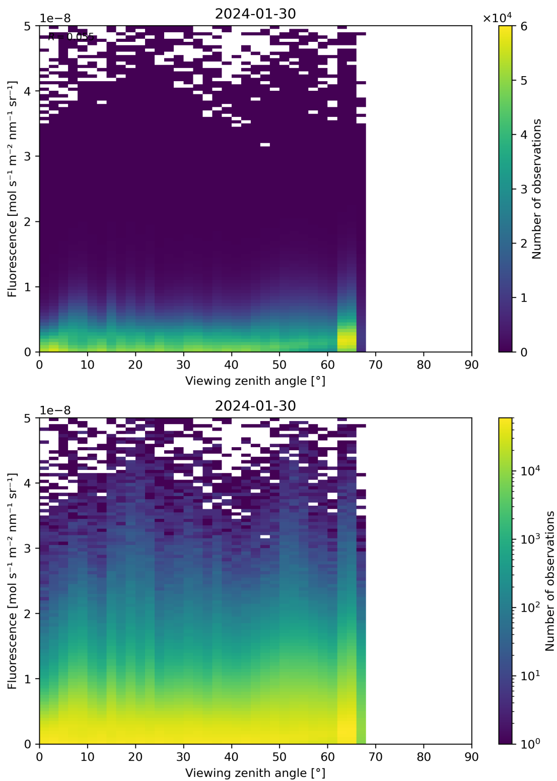
Figure 122: Scatter density plot of “Viewing zenith angle” against “Fluorescence” for 2024-01-29 to 2024-01-31.
