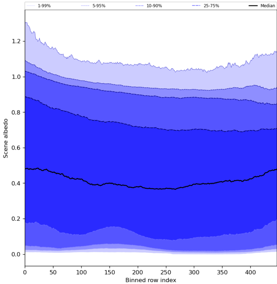
Figure 51: Along track statistics of “Scene albedo” for 2024-01-29 to 2024-01-31
