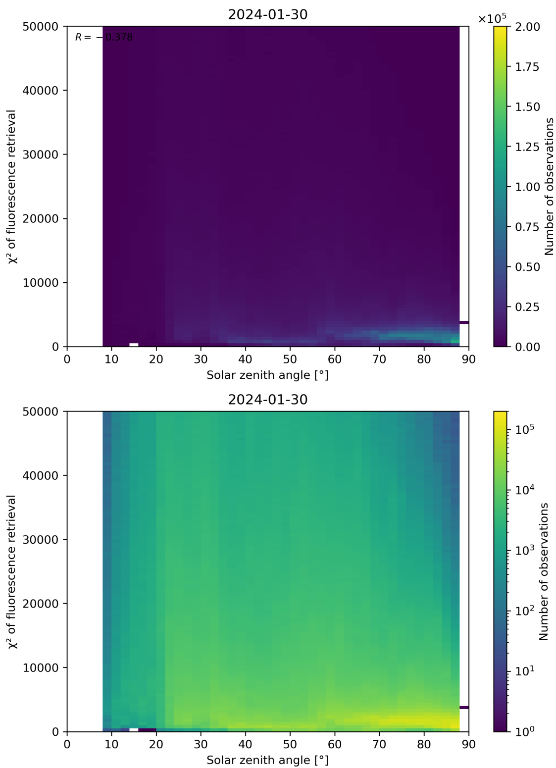
Figure 109: Scatter density plot of “Solar zenith angle” against “ \chi^2 of fluorescence retrieval” for 2024-01-29 to 2024-01-31.
