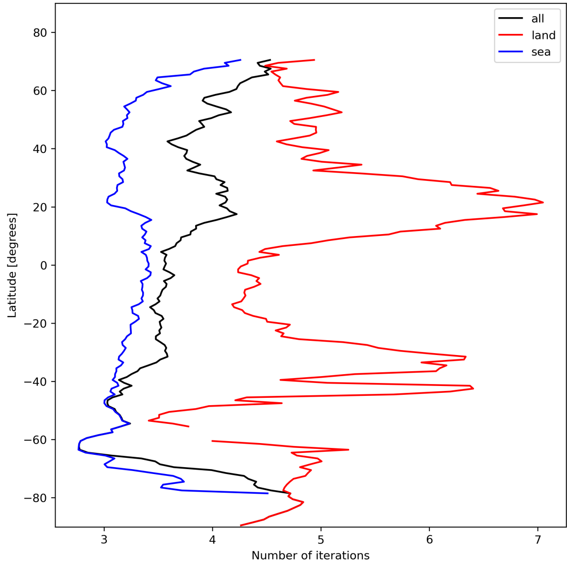
Figure 22: Zonal average of “Number of iterations” for 2024-01-29 to 2024-01-31.
