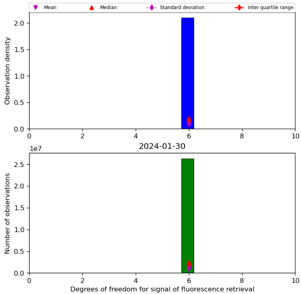
Figure 43: Histogram of “Degrees of freedom for signal of fluorescence retrieval” for 2024-01-29 to 2024-01-31
