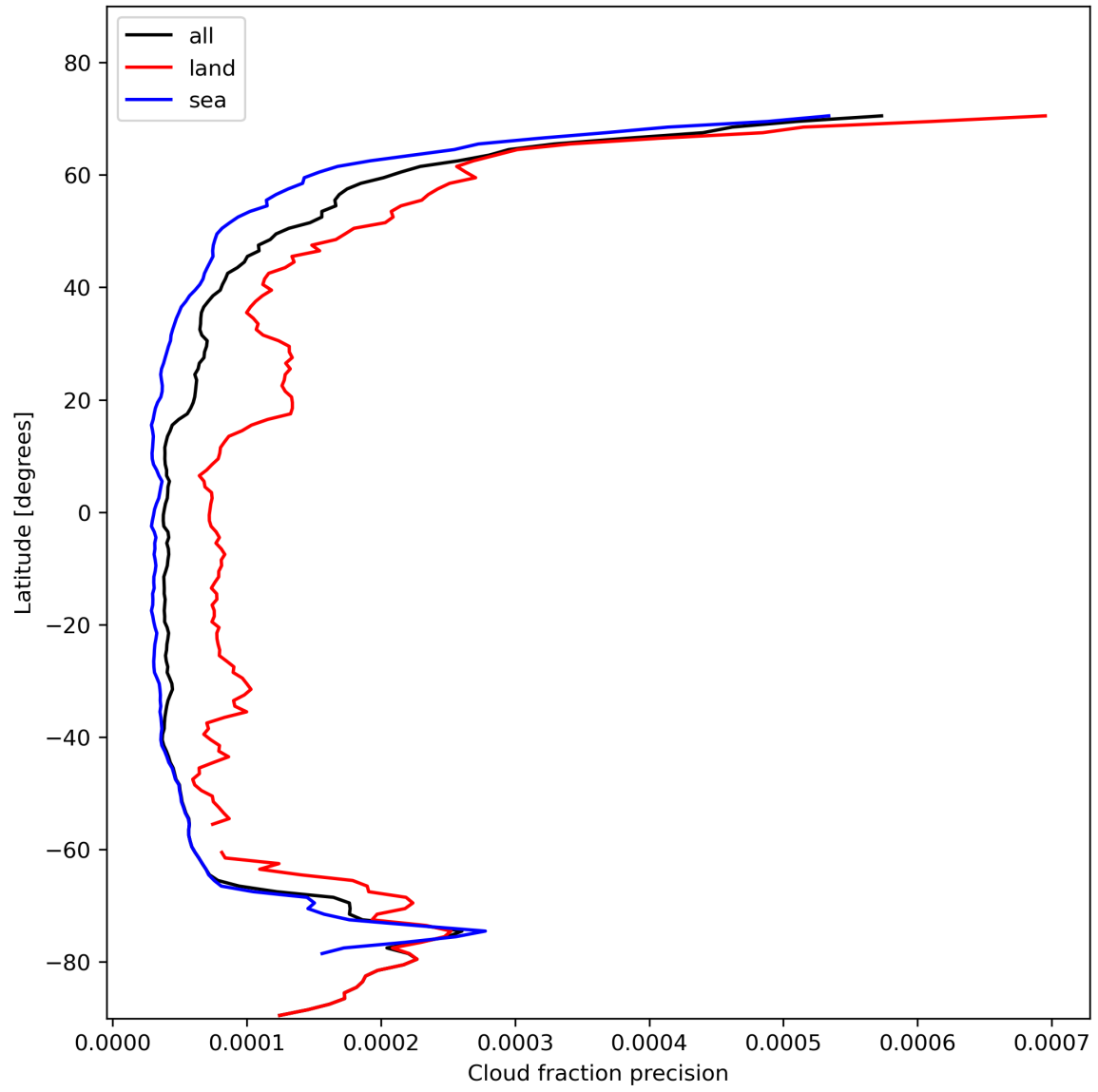
Figure 16: Zonal average of “Cloud fraction precision” for 2024-01-29 to 2024-01-31.
