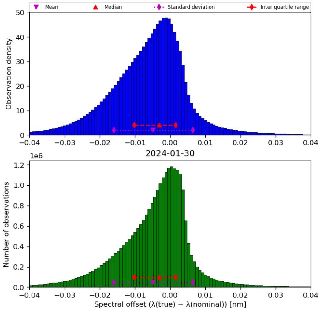
Figure 45: Histogram of “Spectral offset ( \lambda(\text{true}) - \lambda(\text{nominal}) )” for 2024-01-29 to 2024-01-31
