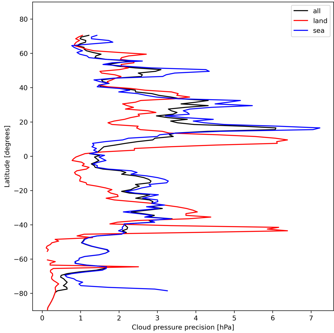
Figure 14: Zonal average of “Cloud pressure precision” for 2024-01-29 to 2024-01-31.
