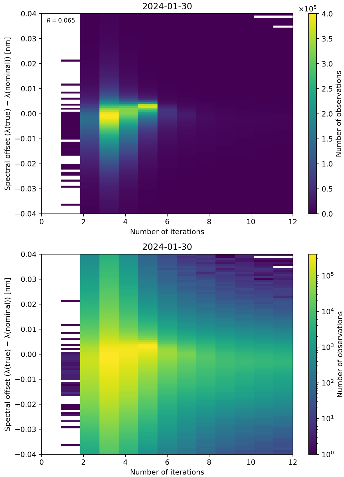
Figure 100: Scatter density plot of “Number of iterations” against “Spectral offset ( \lambda(\text{true}) - \lambda(\text{nominal}) )” for 2024-01-29 to 2024-01-31.
