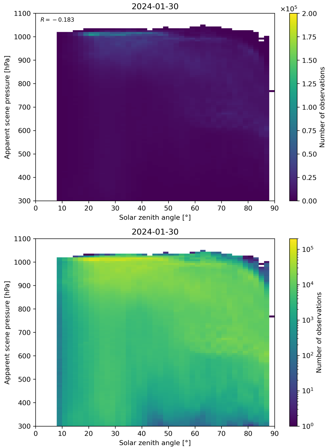
Figure 108: Scatter density plot of “Solar zenith angle” against “Apparent scene pressure” for 2024-01-29 to 2024-01-31.
