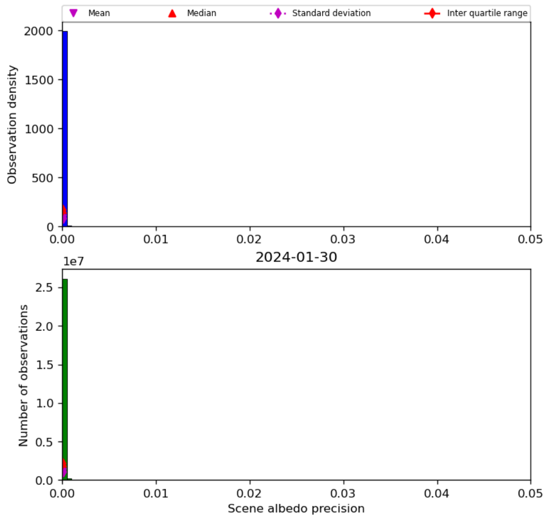
Figure 35: Histogram of “Scene albedo precision” for 2024-01-29 to 2024-01-31
