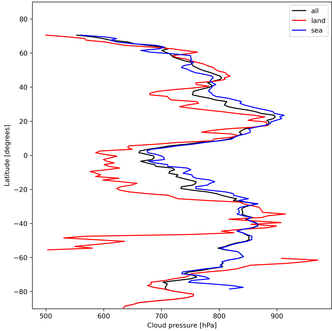
Figure 13: Zonal average of “Cloud pressure” for 2024-01-29 to 2024-01-31.
