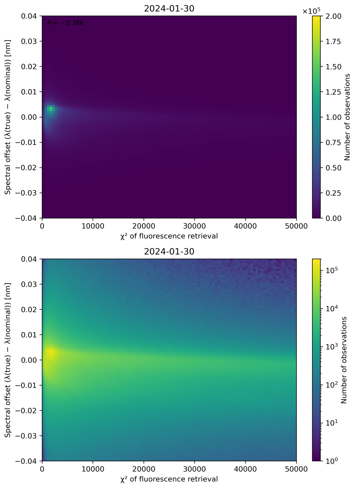
Figure 69: Scatter density plot of " \chi^2 of fluorescence retrieval" against "Spectral offset ( \lambda(\text{true}) - \lambda(\text{nominal}) )" for 2024-01-29 to 2024-01-31.
