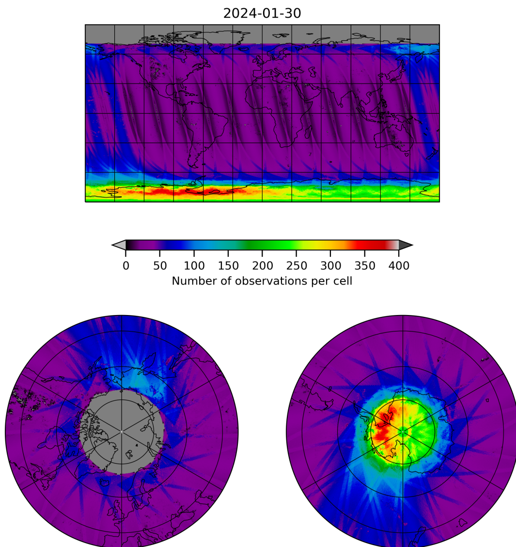
Figure 11: Map of the number of observations for 2024-01-29 to 2024-01-31
