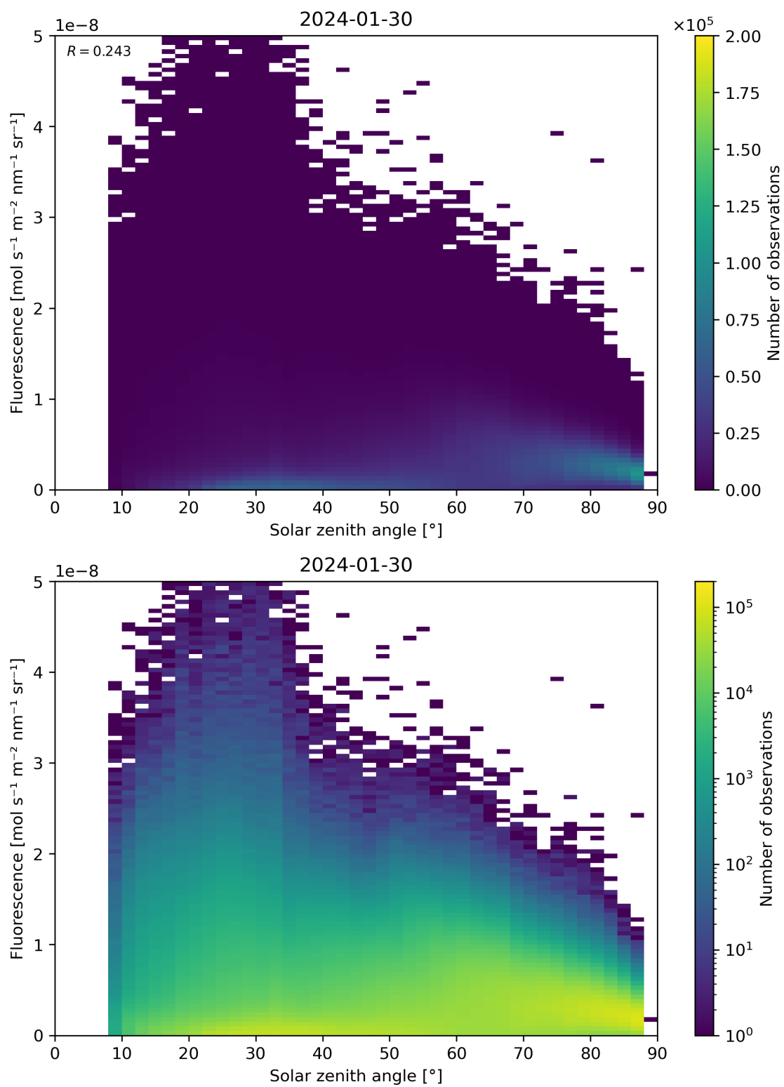
Figure 112: Scatter density plot of “Solar zenith angle” against “Fluorescence” for 2024-01-29 to 2024-01-31.
