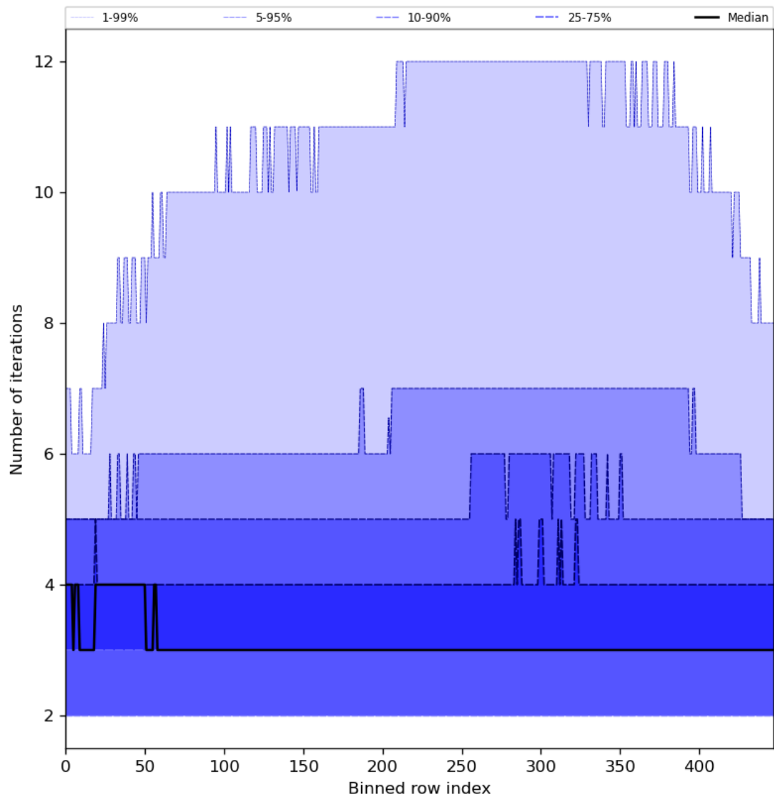
Figure 56: Along track statistics of “Number of iterations” for 2024-01-29 to 2024-01-31
