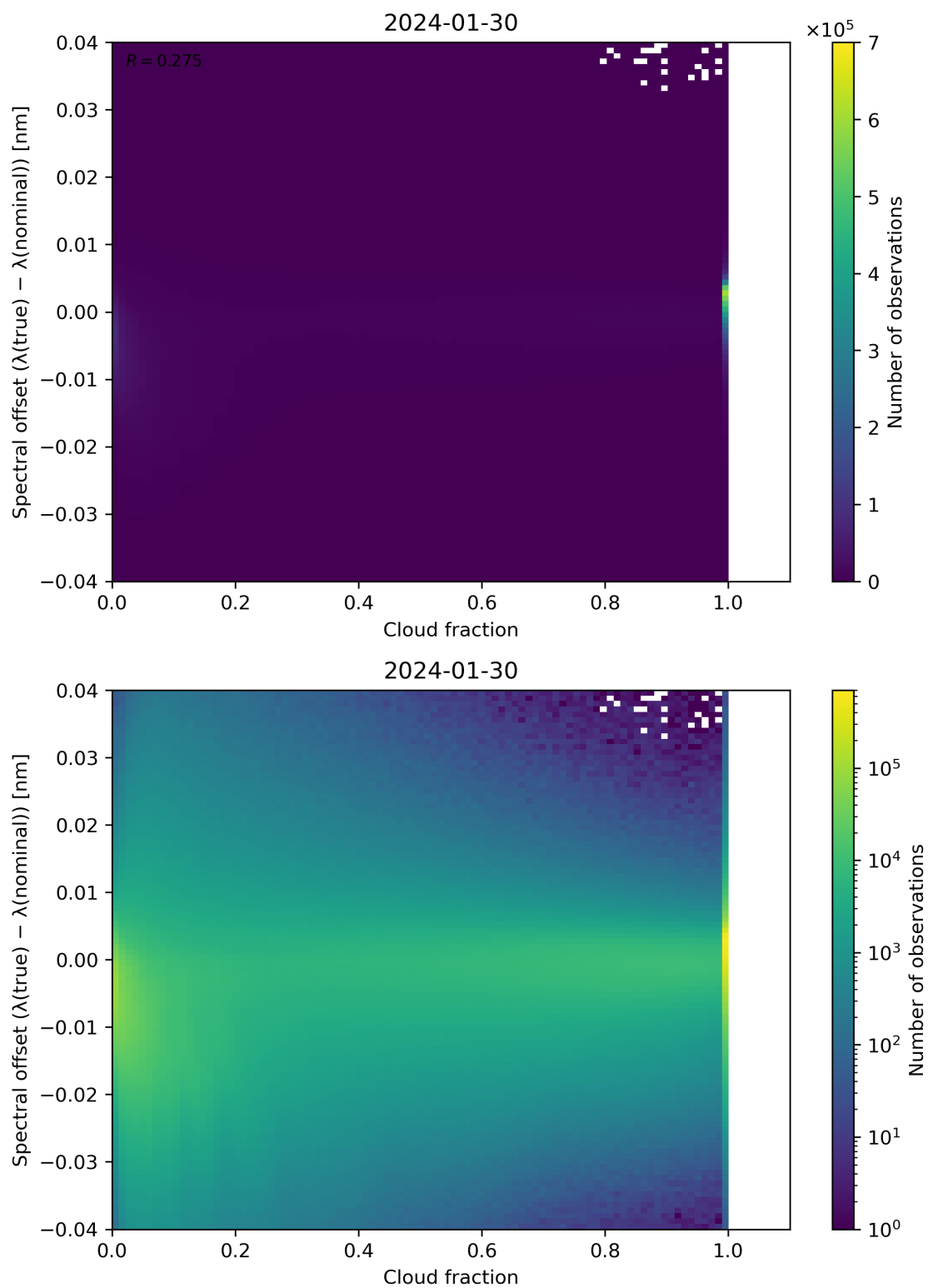
Figure 76: Scatter density plot of “Cloud fraction” against “Spectral offset ( \lambda(\text{true}) - \lambda(\text{nominal}) )” for 2024-01-29 to 2024-01-31.
