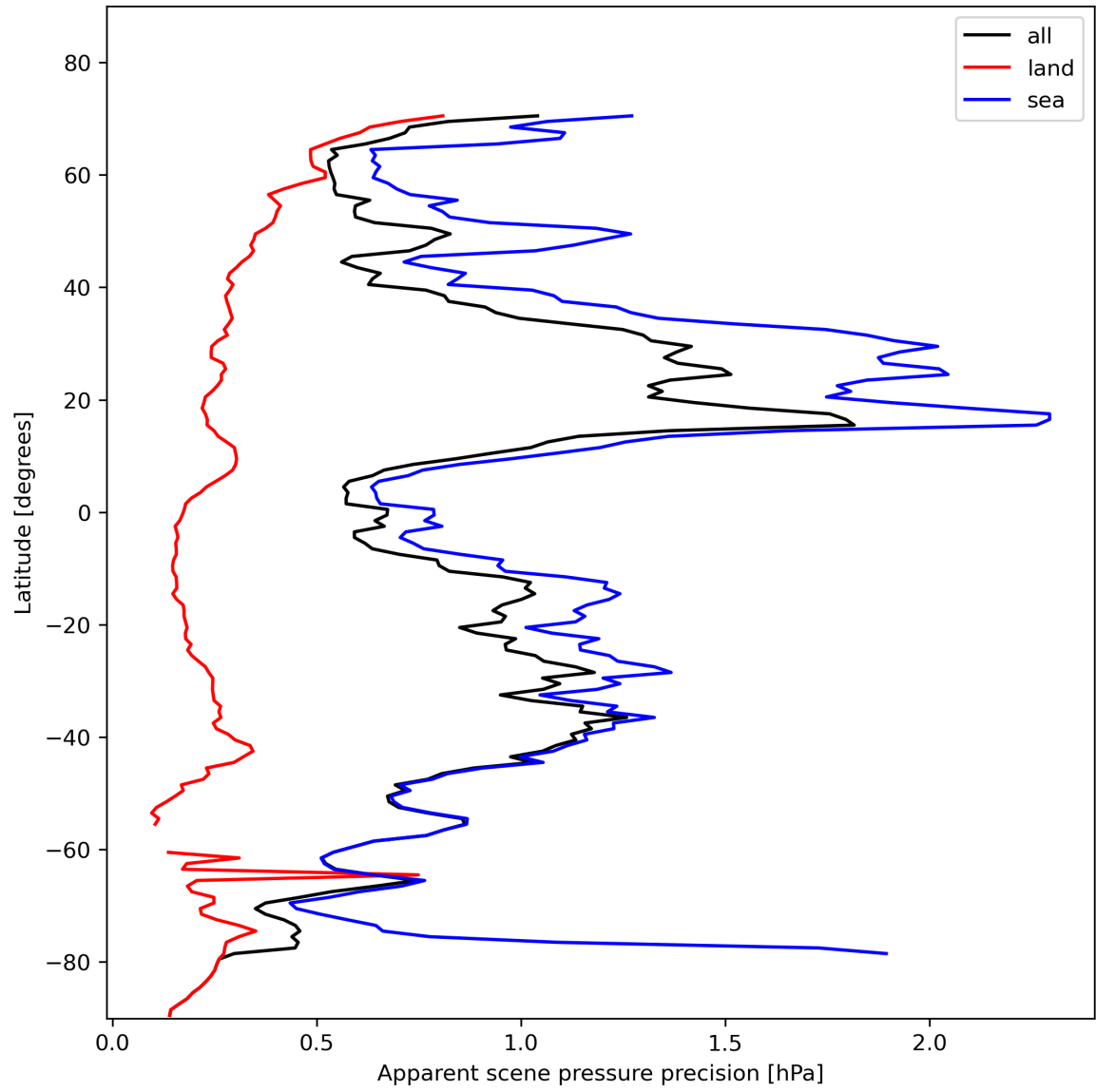
Figure 20: Zonal average of “Apparent scene pressure precision” for 2024-01-29 to 2024-01-31.
