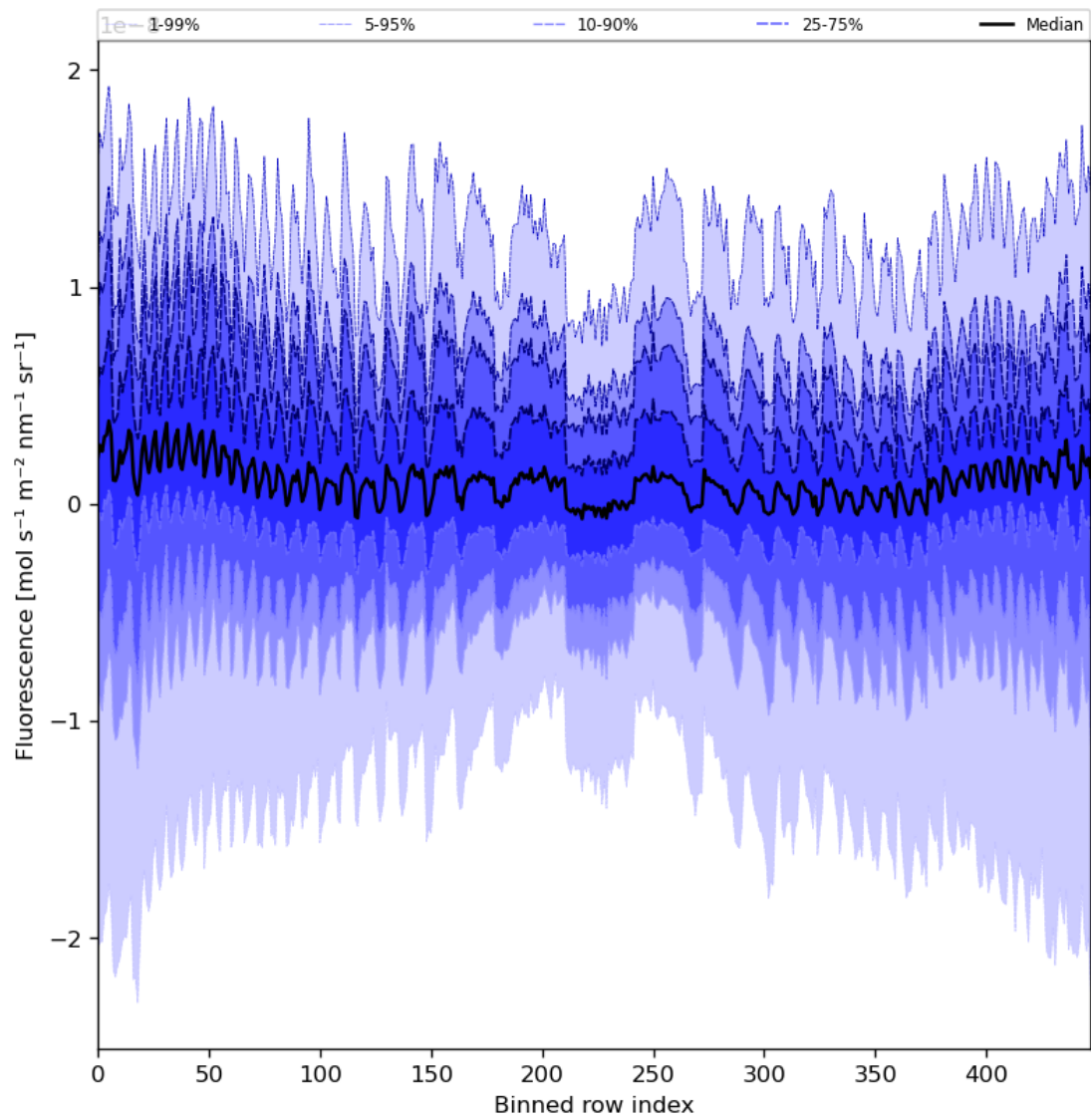
Figure 57: Along track statistics of “Fluorescence” for 2024-01-29 to 2024-01-31
