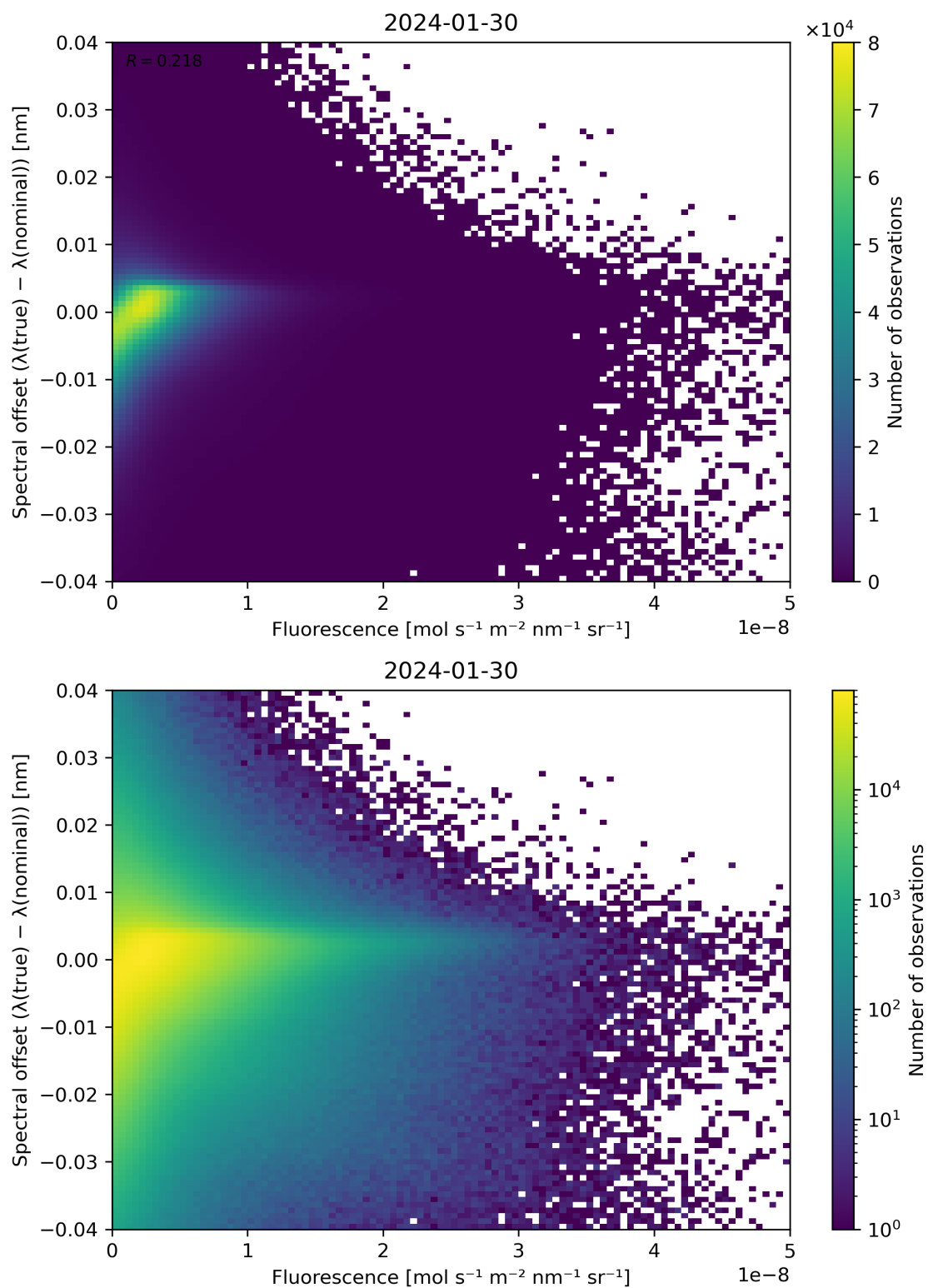
Figure 87: Scatter density plot of “Fluorescence” against “Spectral offset ( \lambda(\text{true}) - \lambda(\text{nominal}) )” for 2024-01-29 to 2024-01-31.
