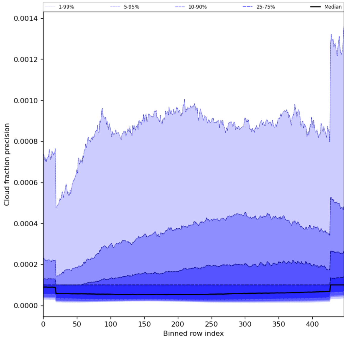
Figure 50: Along track statistics of “Cloud fraction precision” for 2024-01-29 to 2024-01-31
