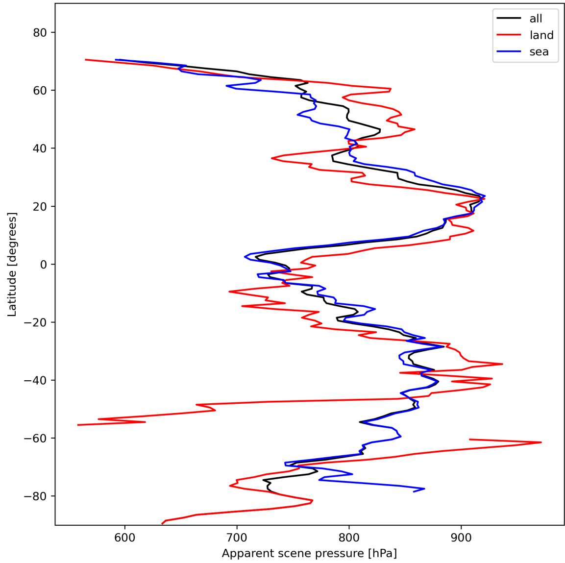
Figure 19: Zonal average of “Apparent scene pressure” for 2024-01-29 to 2024-01-31.
