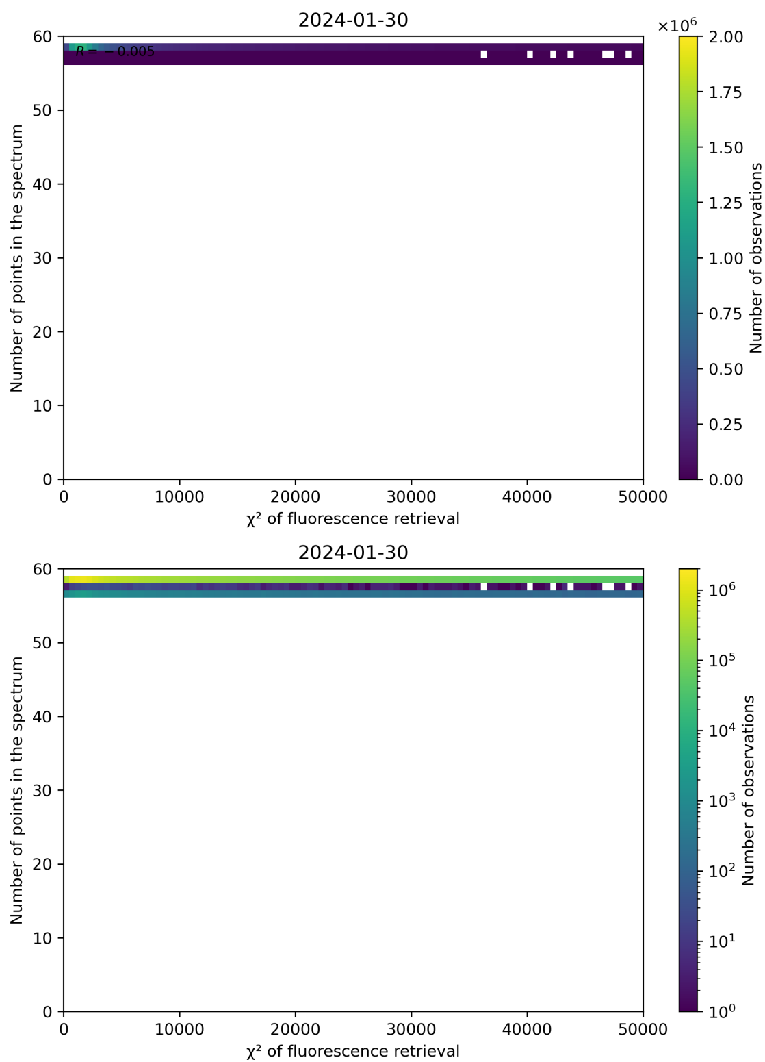
Figure 68: Scatter density plot of " \chi^2 of fluorescence retrieval" against "Number of points in the spectrum" for 2024-01-29 to 2024-01-31.
