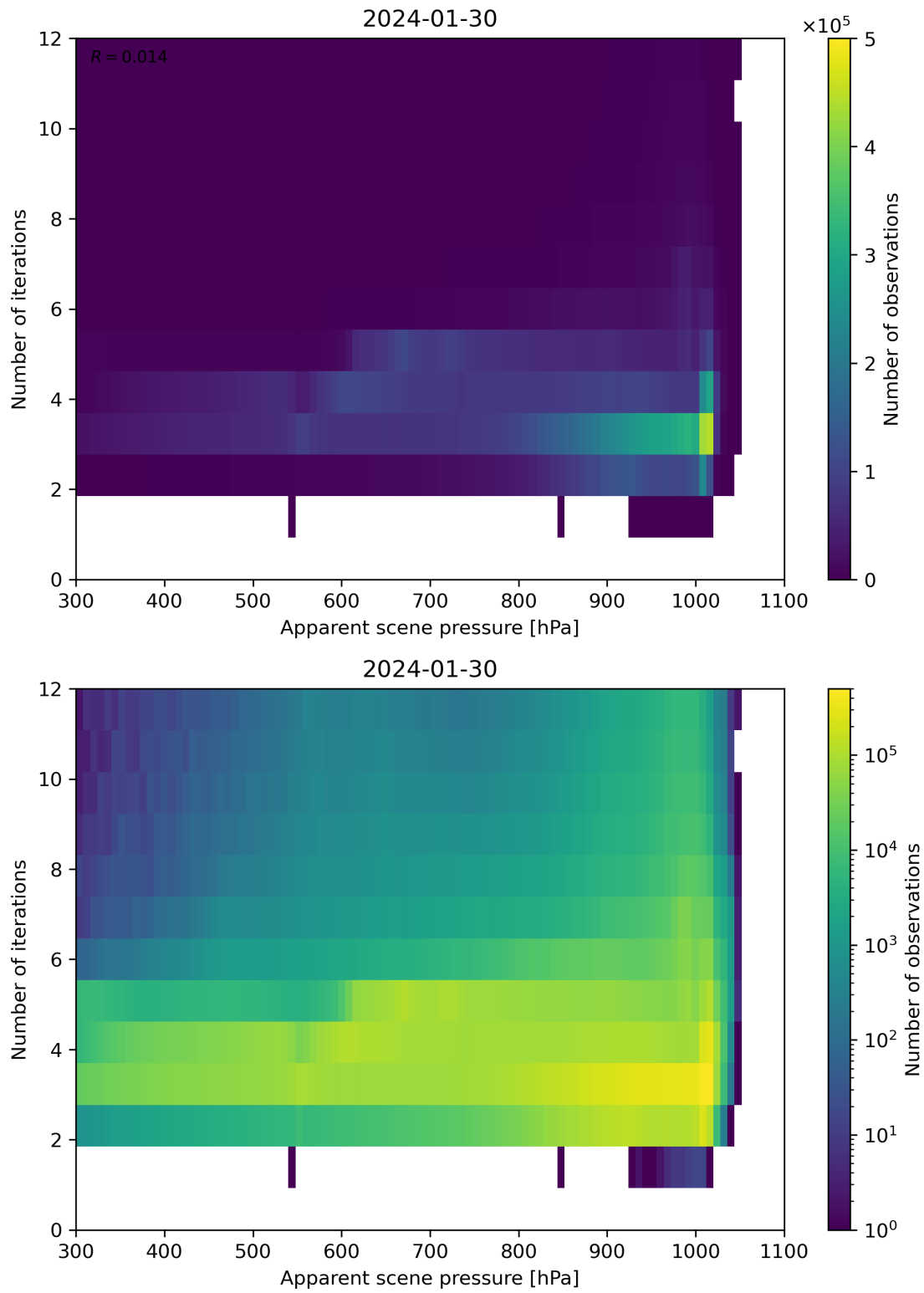
Figure 65: Scatter density plot of “Apparent scene pressure” against “Number of iterations” for 2024-01-29 to 2024-01-31.
