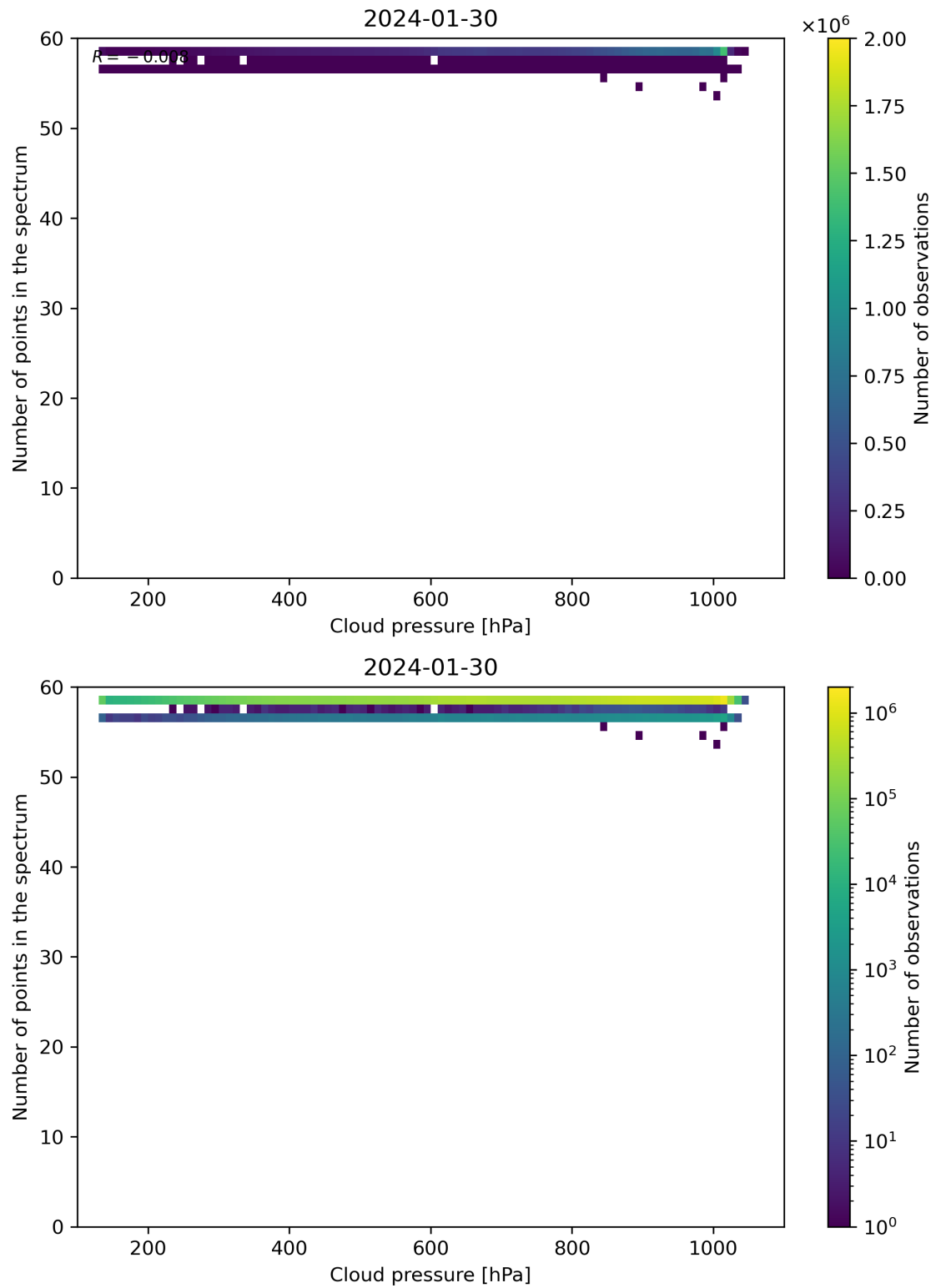
Figure 82: Scatter density plot of “Cloud pressure” against “Number of points in the spectrum” for 2024-01-29 to 2024-01-31.
