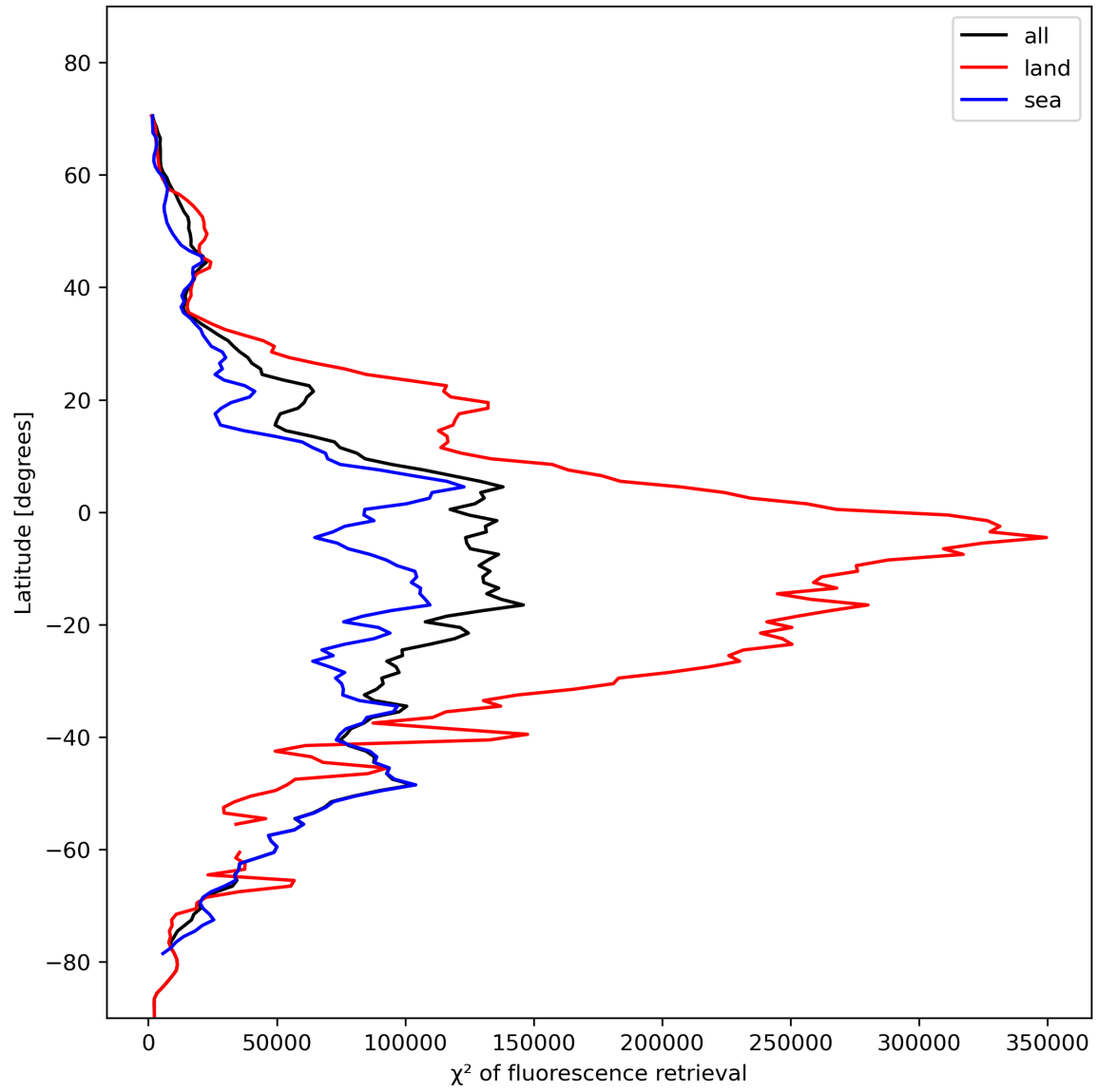
Figure 25: Zonal average of “ \chi^2 of fluorescence retrieval” for 2024-01-29 to 2024-01-31.
