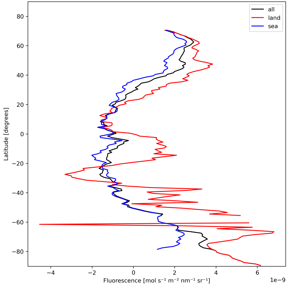
Figure 23: Zonal average of “Fluorescence” for 2024-01-29 to 2024-01-31.
