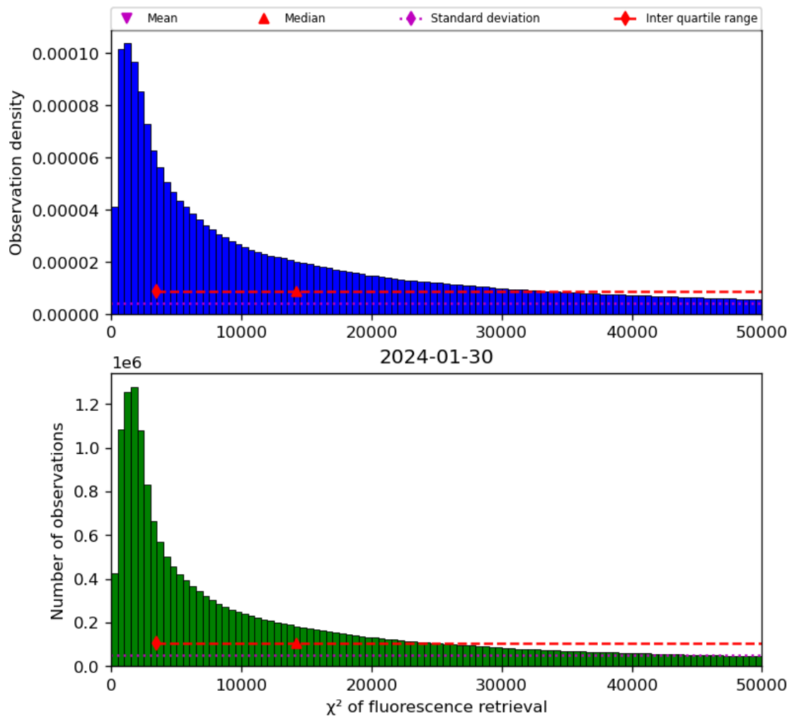
Figure 42: Histogram of “ \chi^2 of fluorescence retrieval” for 2024-01-29 to 2024-01-31
