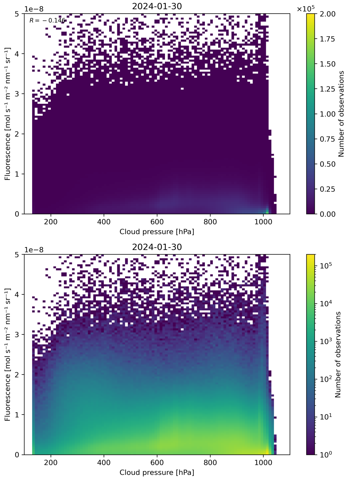
Figure 80: Scatter density plot of “Cloud pressure” against “Fluorescence” for 2024-01-29 to 2024-01-31.
