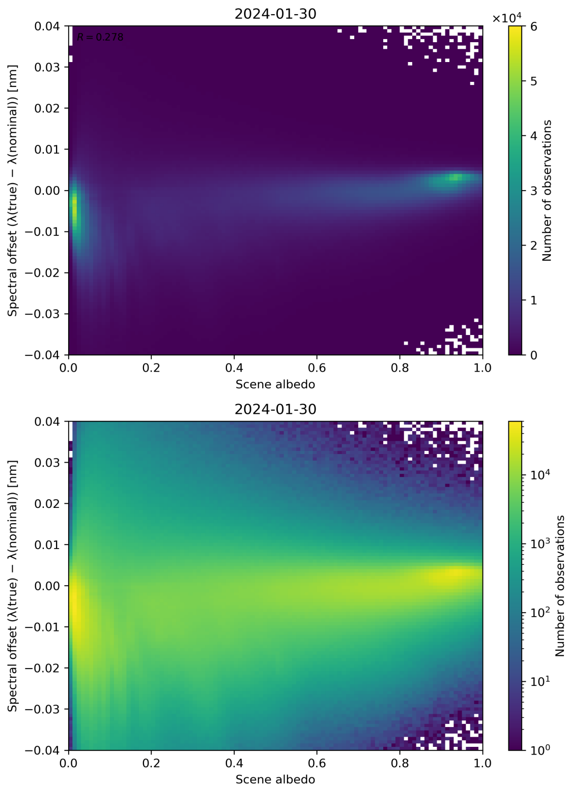
Figure 107: Scatter density plot of “Scene albedo” against “Spectral offset ( \lambda(\text{true}) - \lambda(\text{nominal}) )” for 2024-01-29 to 2024-01-31.
