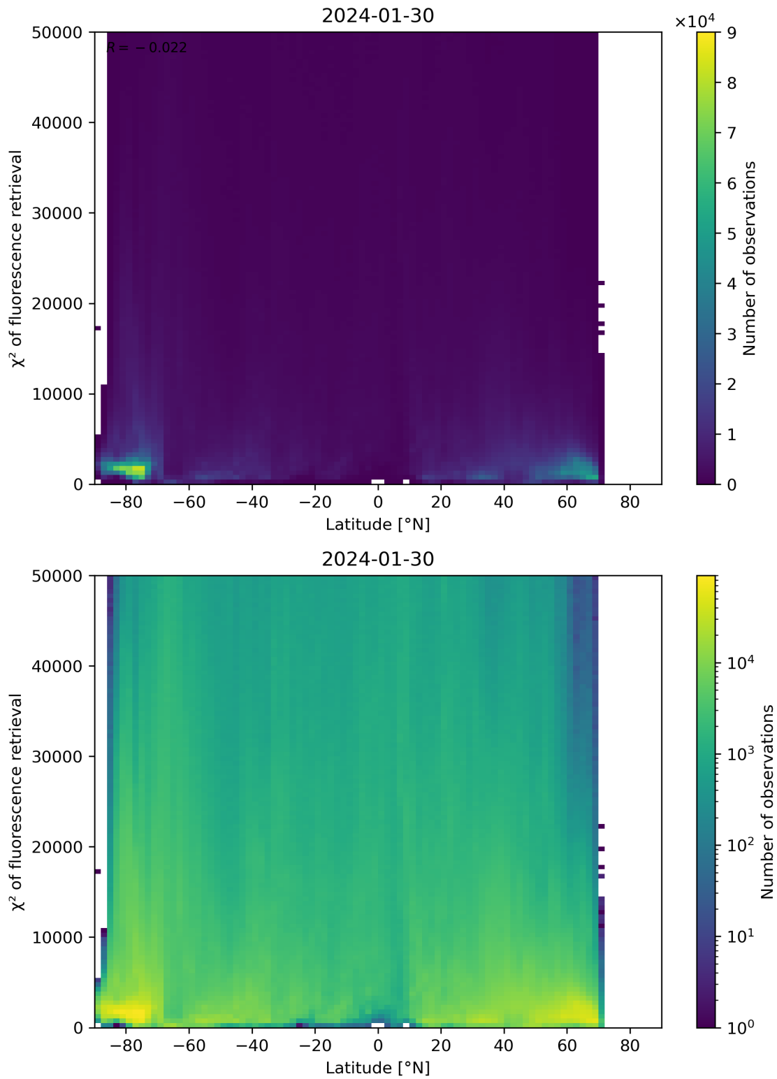
Figure 89: Scatter density plot of “Latitude” against “ \chi^2 of fluorescence retrieval” for 2024-01-29 to 2024-01-31.
