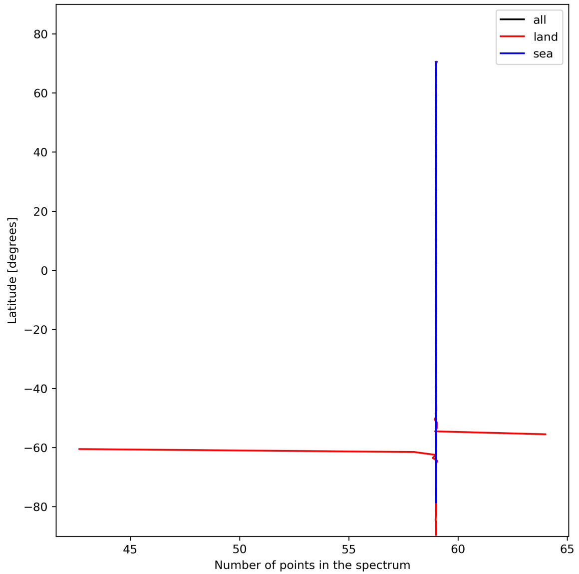
Figure 27: Zonal average of “Number of points in the spectrum” for 2024-01-29 to 2024-01-31.
