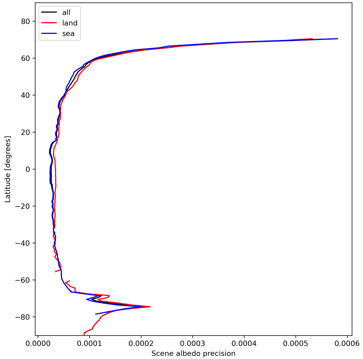
Figure 18: Zonal average of “Scene albedo precision” for 2024-01-29 to 2024-01-31.
