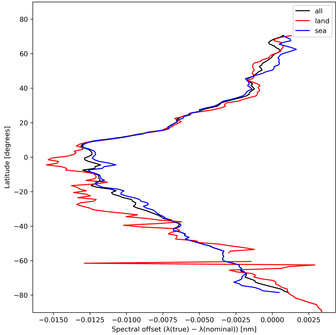
Figure 28: Zonal average of “Spectral offset ( \lambda(\text{true}) - \lambda(\text{nominal}) )” for 2024-01-29 to 2024-01-31.
