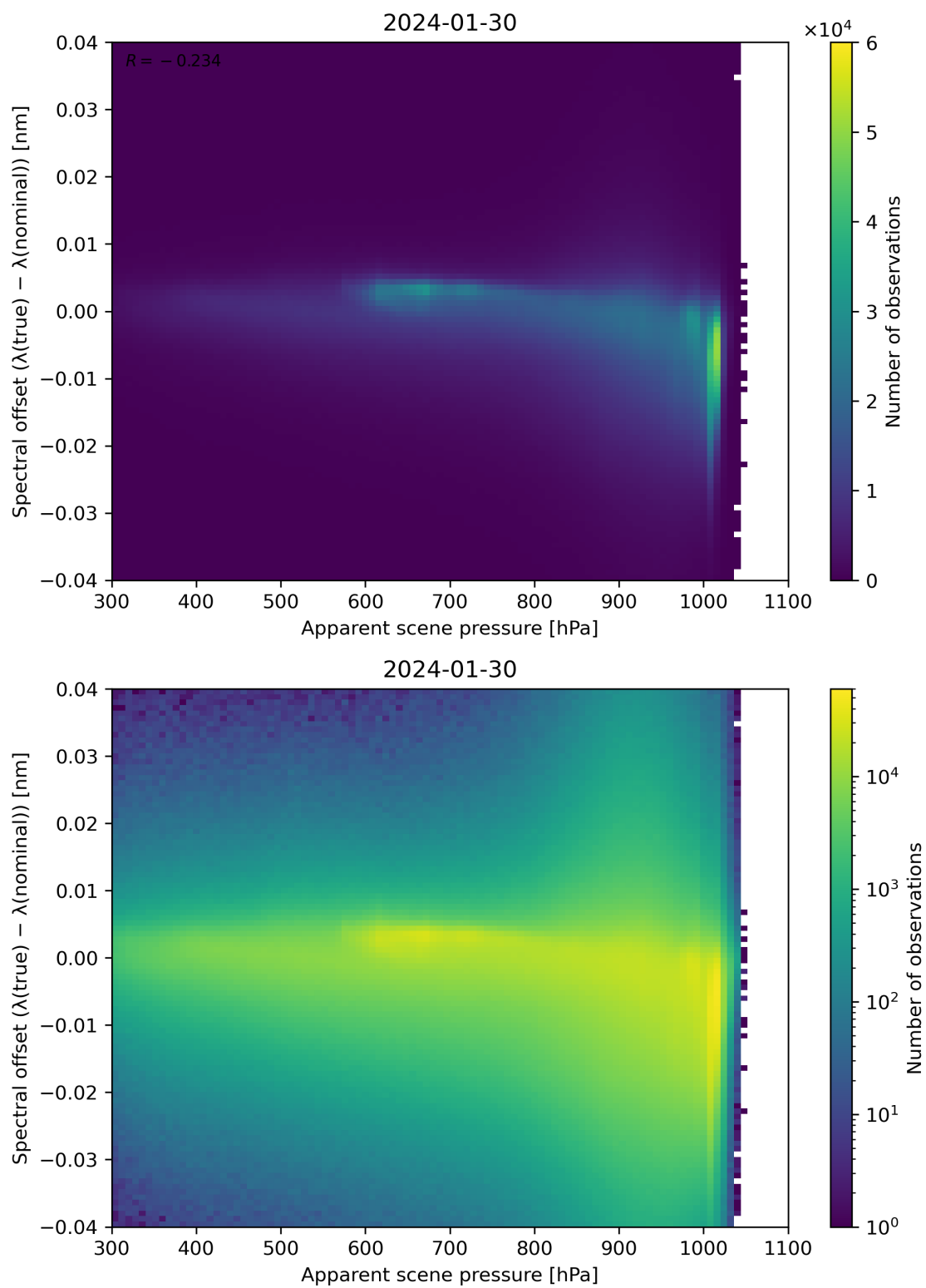
Figure 67: Scatter density plot of “Apparent scene pressure” against “Spectral offset ( \lambda(\text{true}) - \lambda(\text{nominal}) )” for 2024-01-29 to 2024-01-31.
