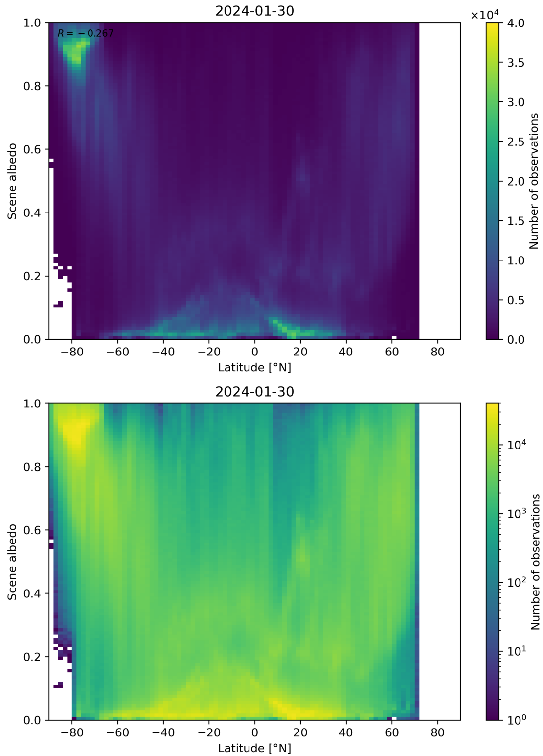
Figure 95: Scatter density plot of “Latitude” against “Scene albedo” for 2024-01-29 to 2024-01-31.
