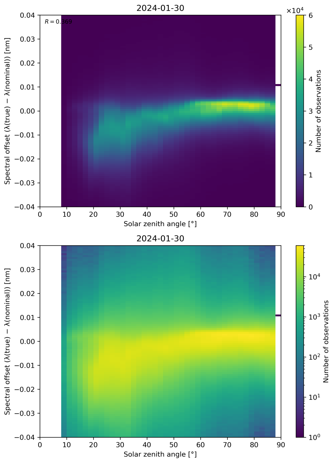
Figure 117: Scatter density plot of “Solar zenith angle” against “Spectral offset ( \lambda(\text{true}) - \lambda(\text{nominal}) )” for 2024-01-29 to 2024-01-31.
