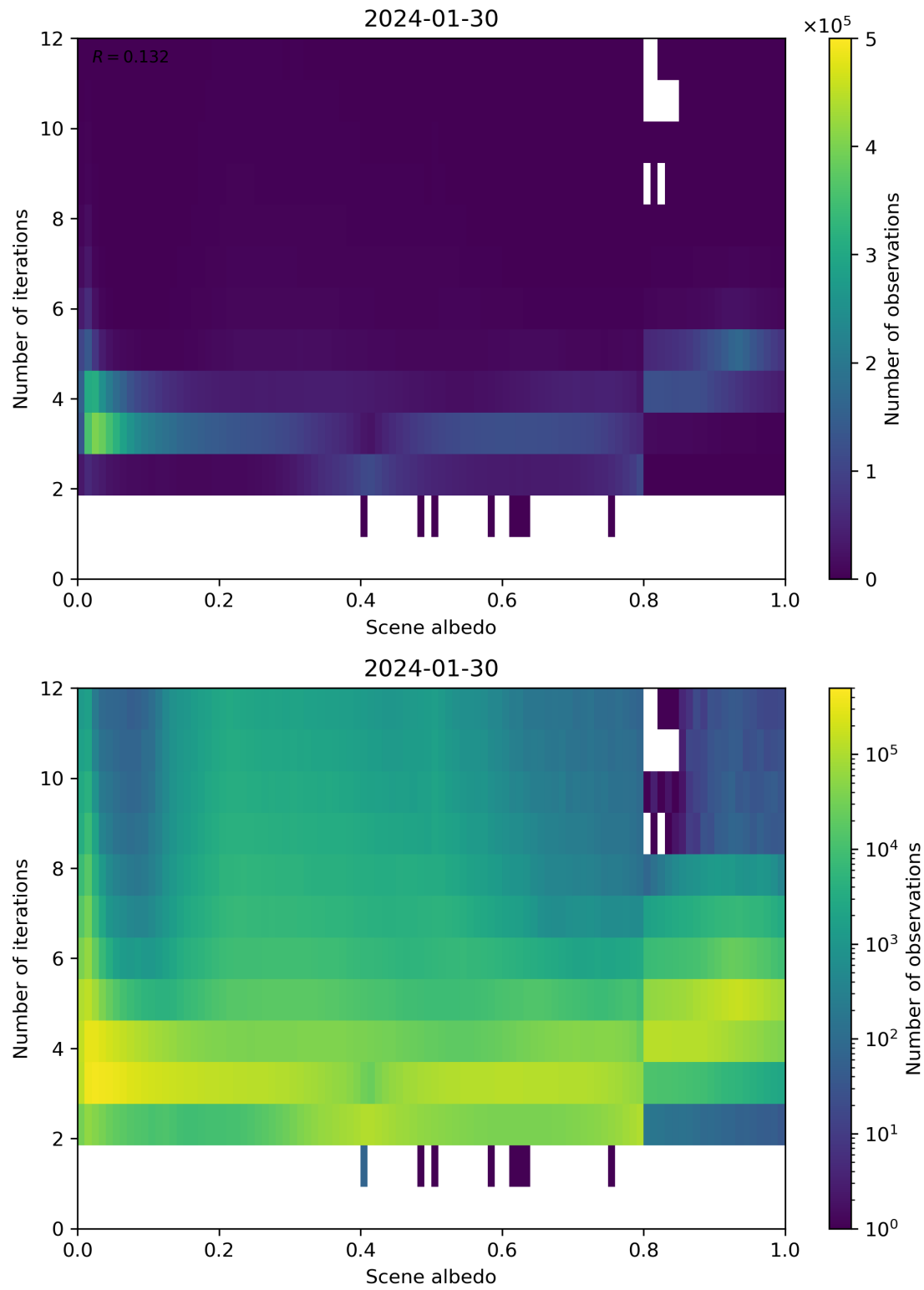
Figure 105: Scatter density plot of “Scene albedo” against “Number of iterations” for 2024-01-29 to 2024-01-31.
