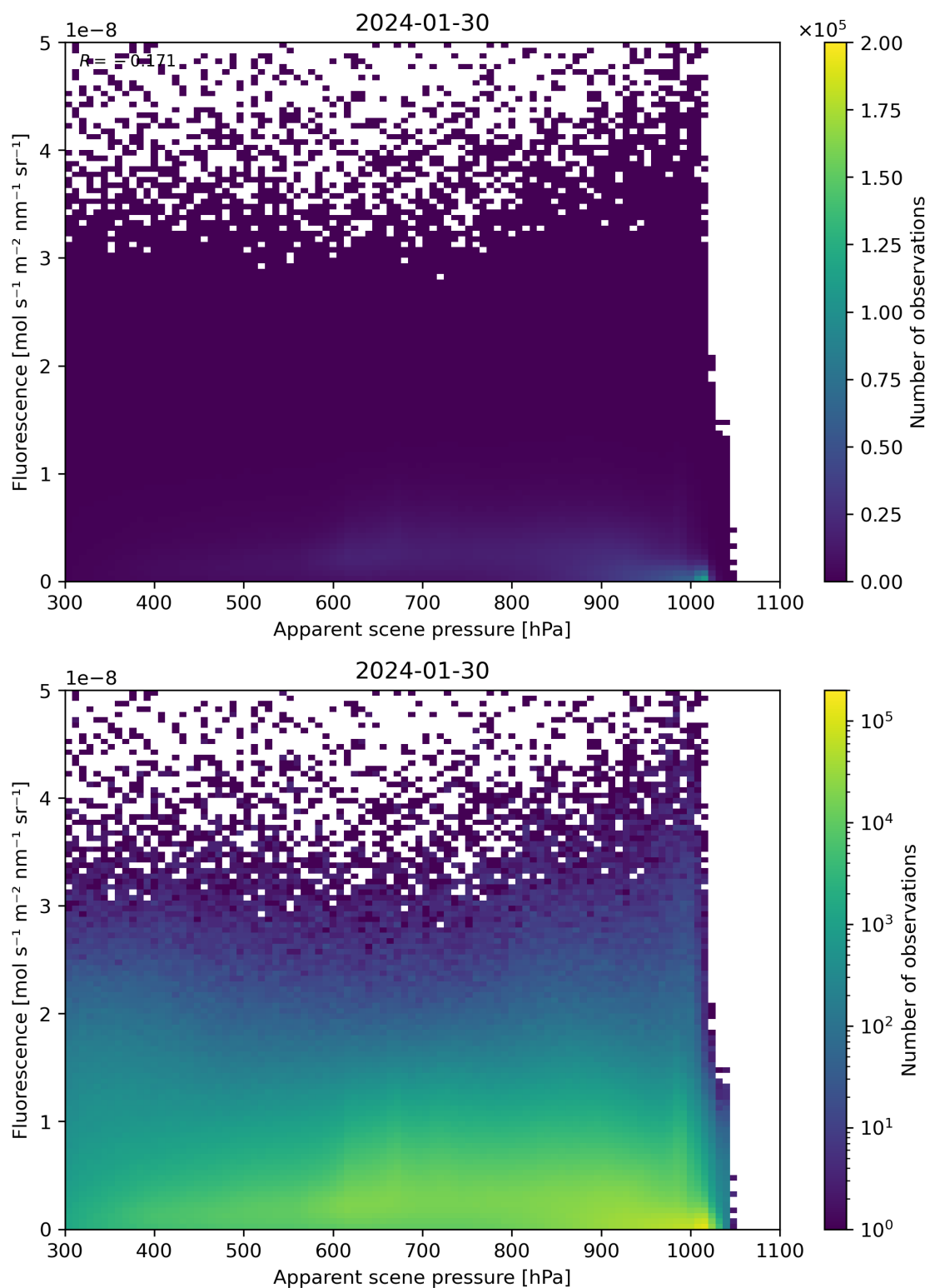
Figure 64: Scatter density plot of “Apparent scene pressure” against “Fluorescence” for 2024-01-29 to 2024-01-31.
