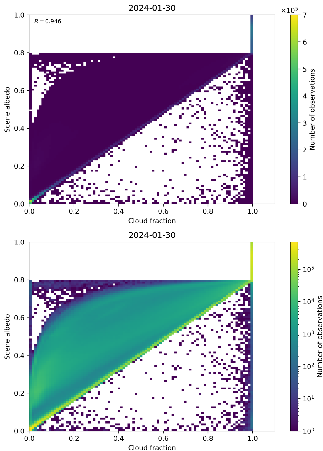
Figure 75: Scatter density plot of “Cloud fraction” against “Scene albedo” for 2024-01-29 to 2024-01-31.
