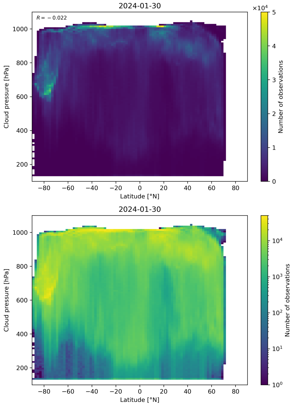
Figure 91: Scatter density plot of “Latitude” against “Cloud pressure” for 2024-01-29 to 2024-01-31.
