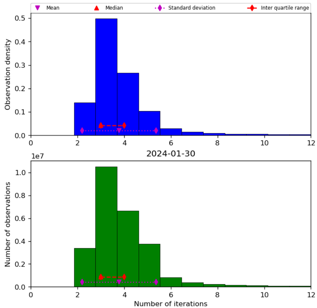
Figure 39: Histogram of “Number of iterations” for 2024-01-29 to 2024-01-31
