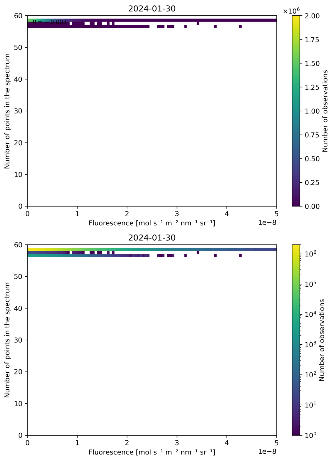
Figure 86: Scatter density plot of “Fluorescence” against “Number of points in the spectrum” for 2024-01-29 to 2024-01-31.
