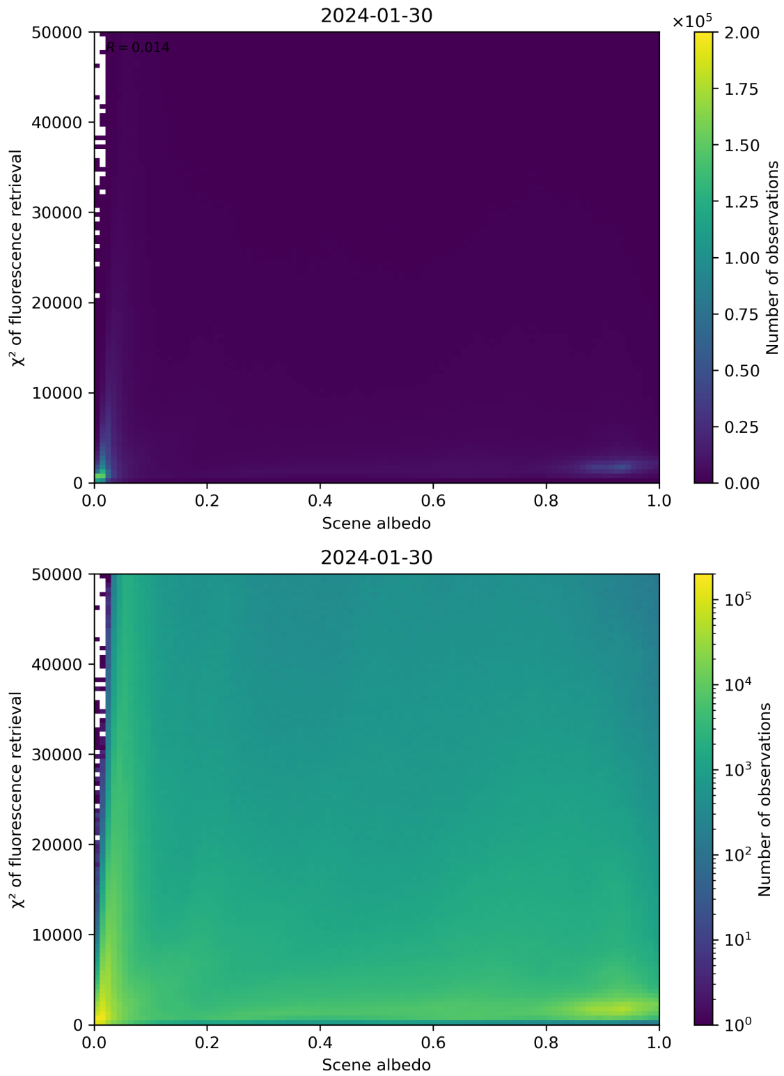
Figure 103: Scatter density plot of “Scene albedo” against “ \chi^2 of fluorescence retrieval” for 2024-01-29 to 2024-01-31.
