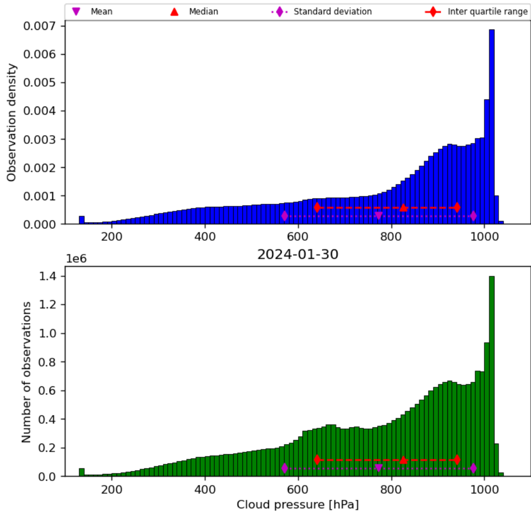
Figure 30: Histogram of “Cloud pressure” for 2024-01-29 to 2024-01-31
