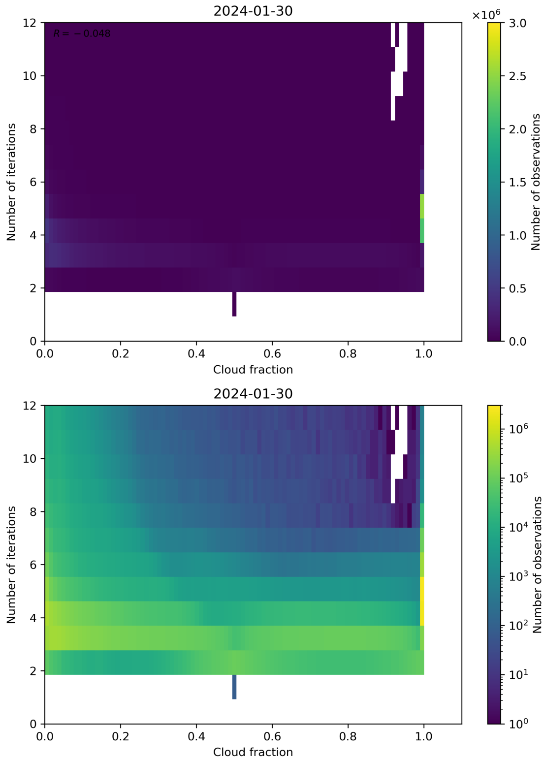
Figure 73: Scatter density plot of “Cloud fraction” against “Number of iterations” for 2024-01-29 to 2024-01-31.
