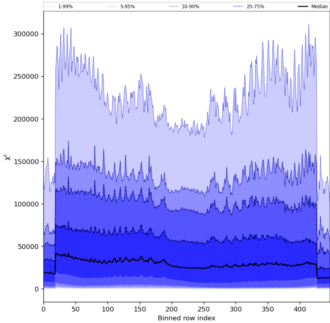
Figure 55: Along track statistics of “ \chi^2 ” for 2024-01-29 to 2024-01-31
