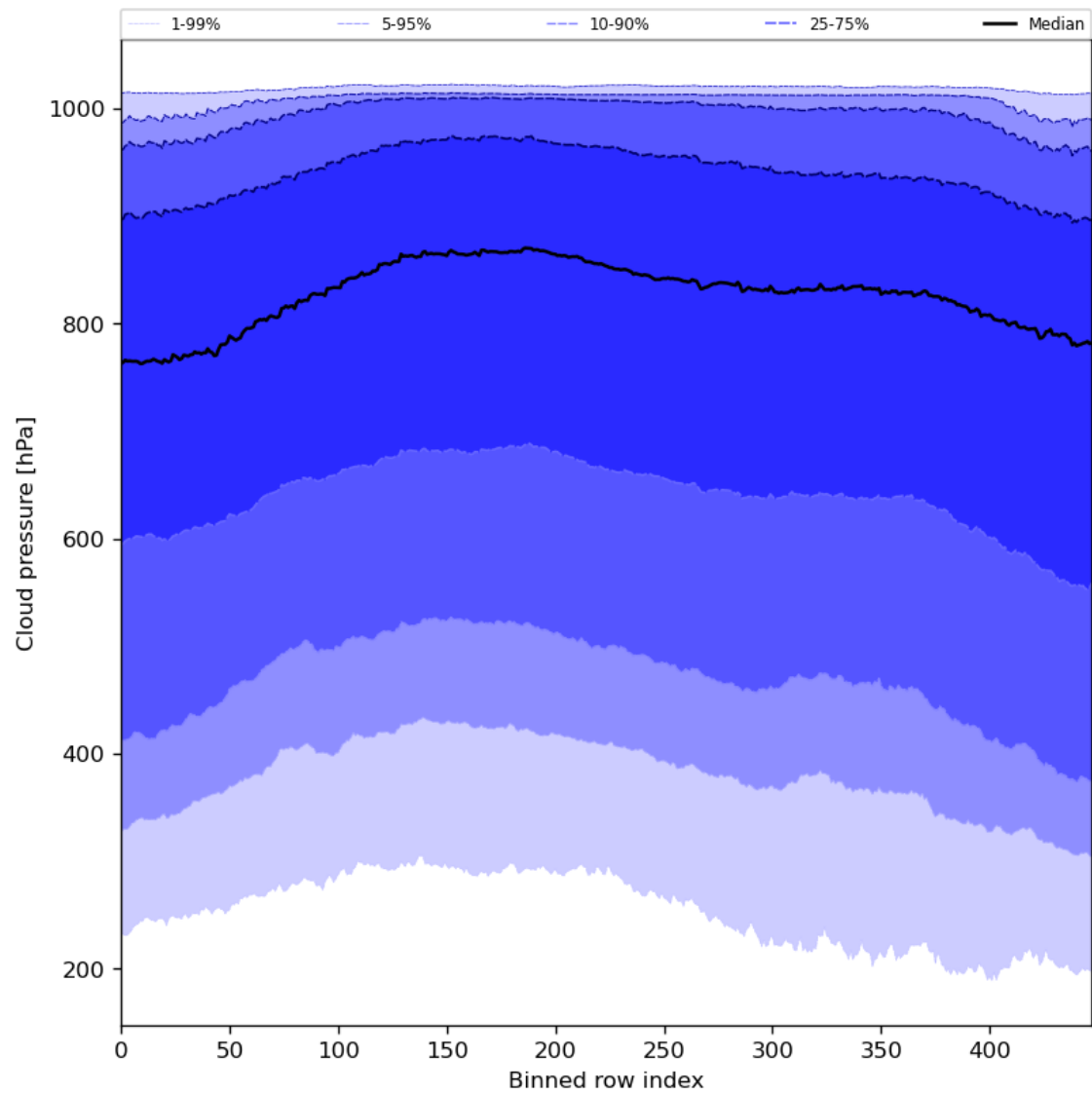
Figure 47: Along track statistics of “Cloud pressure” for 2024-01-29 to 2024-01-31
