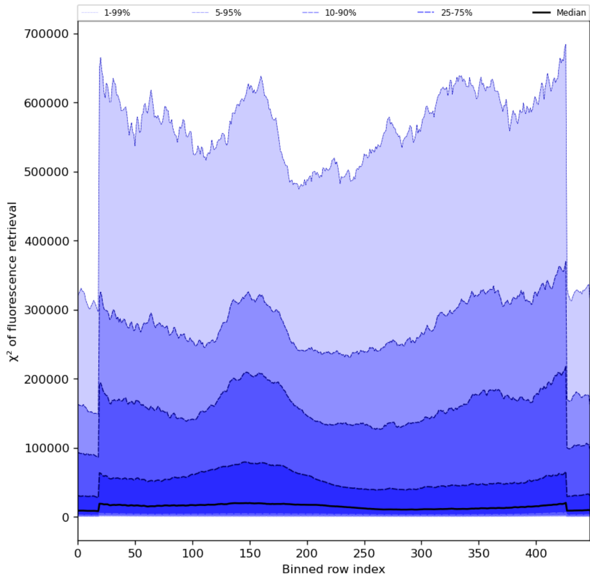
Figure 59: Along track statistics of “ \chi^2 of fluorescence retrieval” for 2024-01-29 to 2024-01-31
