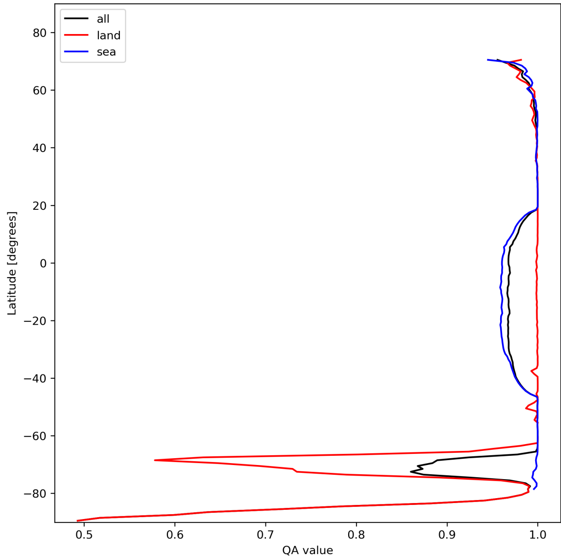
Figure 12: Zonal average of “QA value” for 2024-01-29 to 2024-01-31.
