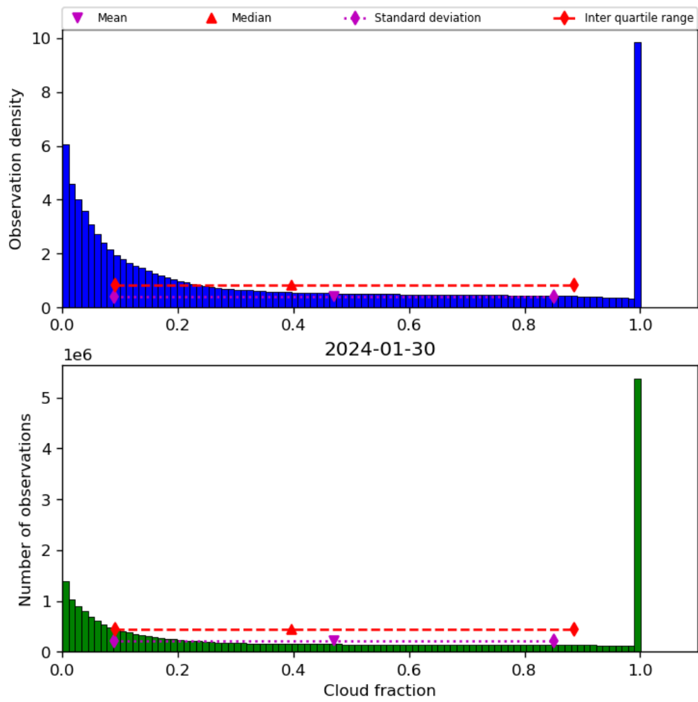
Figure 32: Histogram of “Cloud fraction” for 2024-01-29 to 2024-01-31
