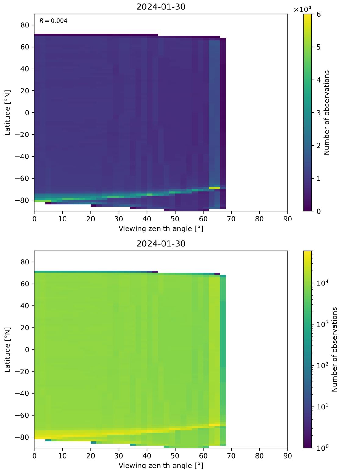
Figure 123: Scatter density plot of “Viewing zenith angle” against “Latitude” for 2024-01-29 to 2024-01-31.
