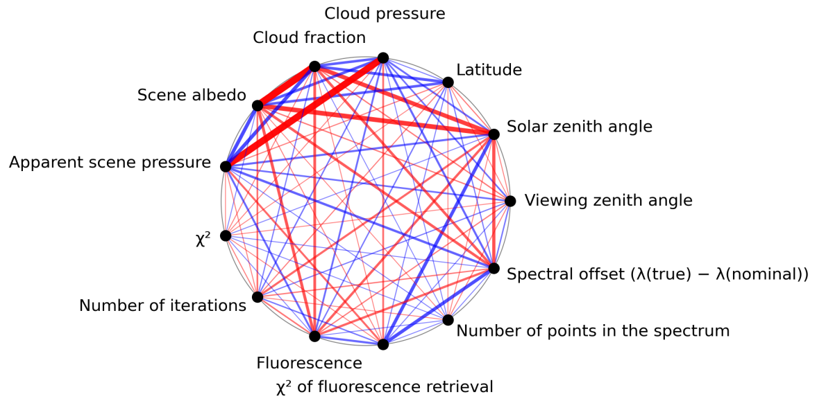
Figure 1: Map of correlation graph for 2024-01-29 to 2024-01-31.
