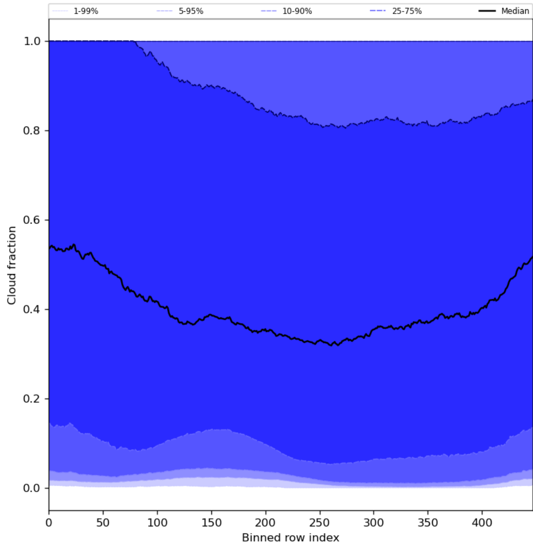
Figure 49: Along track statistics of “Cloud fraction” for 2024-01-29 to 2024-01-31
