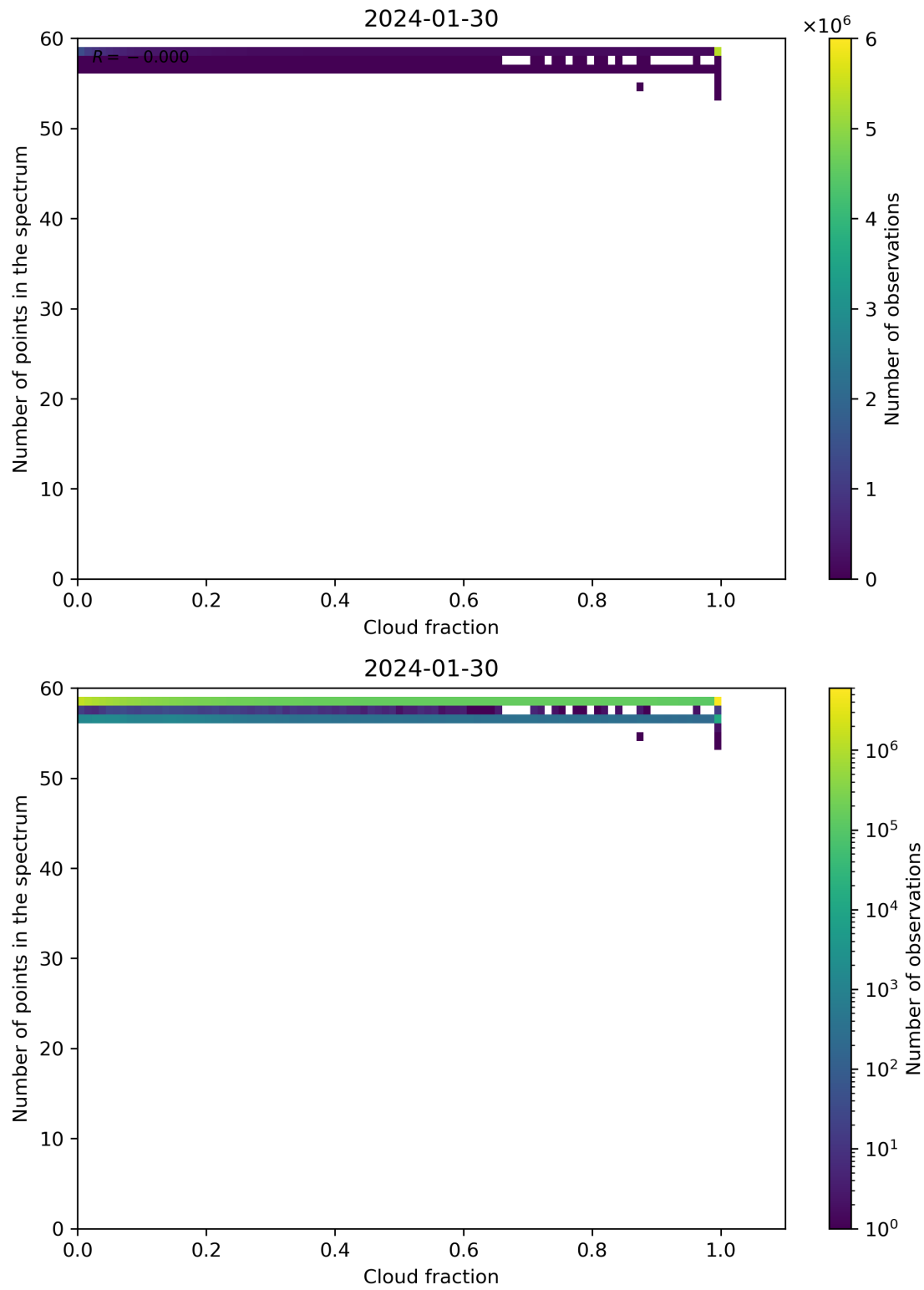
Figure 74: Scatter density plot of “Cloud fraction” against “Number of points in the spectrum” for 2024-01-29 to 2024-01-31.
