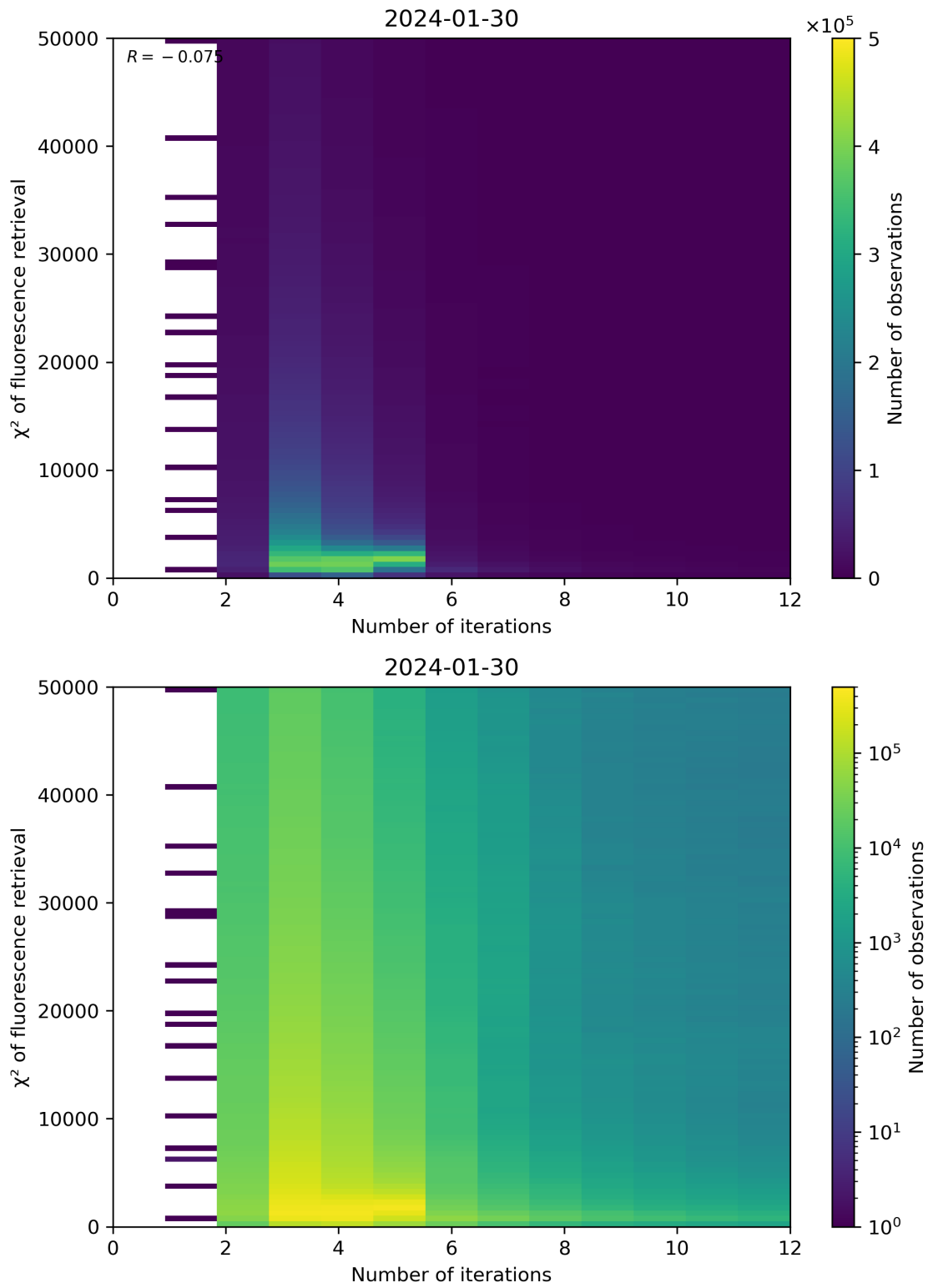
Figure 97: Scatter density plot of “Number of iterations” against “ \chi^2 of fluorescence retrieval” for 2024-01-29 to 2024-01-31.
