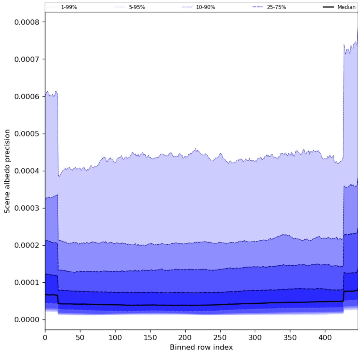
Figure 52: Along track statistics of “Scene albedo precision” for 2024-01-29 to 2024-01-31
