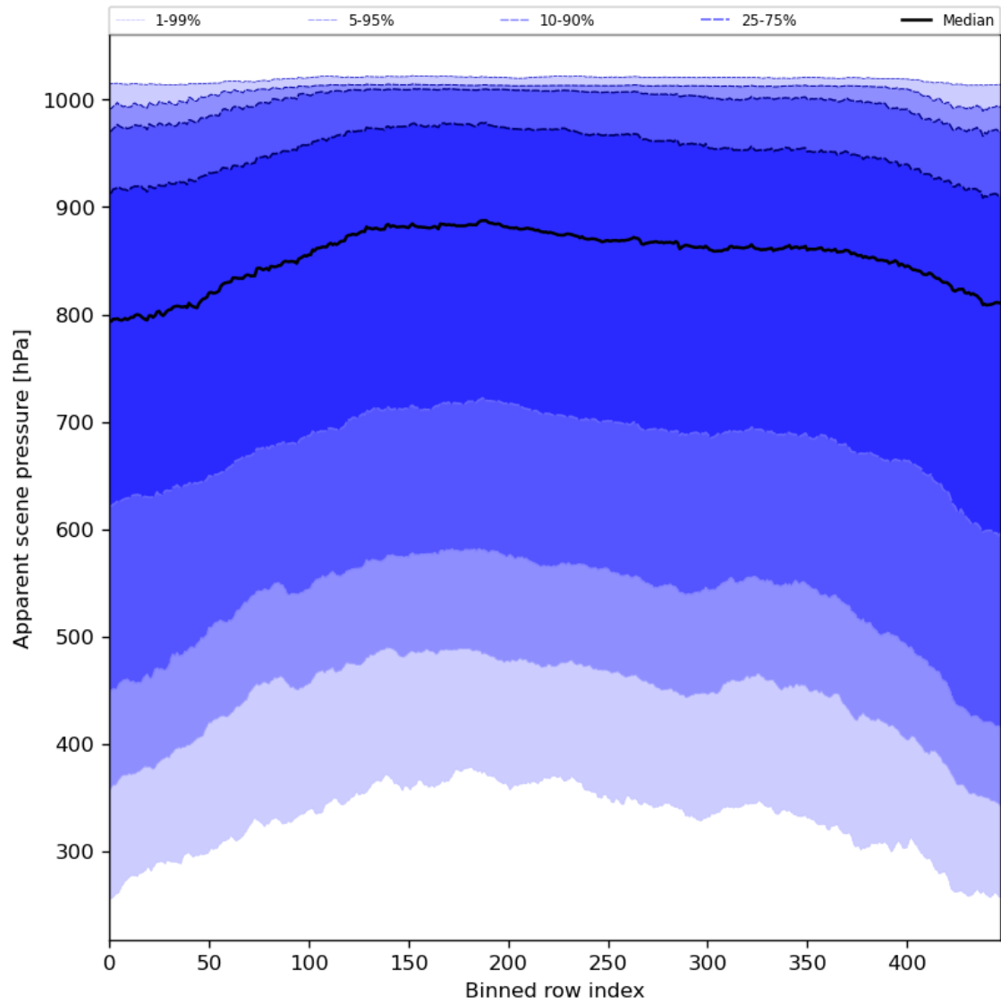
Figure 53: Along track statistics of “Apparent scene pressure” for 2024-01-29 to 2024-01-31
