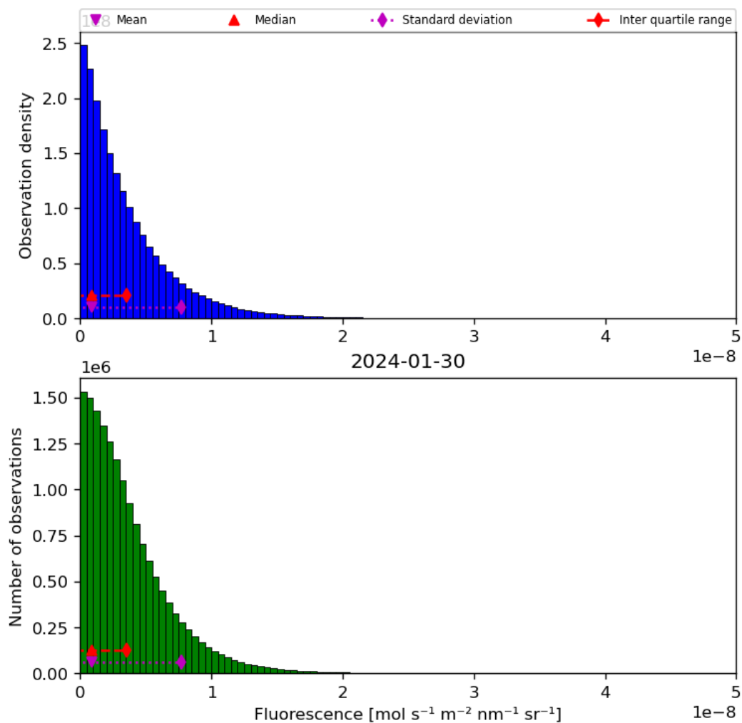
Figure 40: Histogram of “Fluorescence” for 2024-01-29 to 2024-01-31
