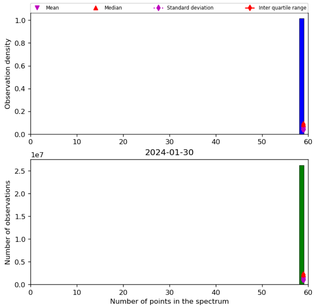
Figure 44: Histogram of “Number of points in the spectrum” for 2024-01-29 to 2024-01-31
