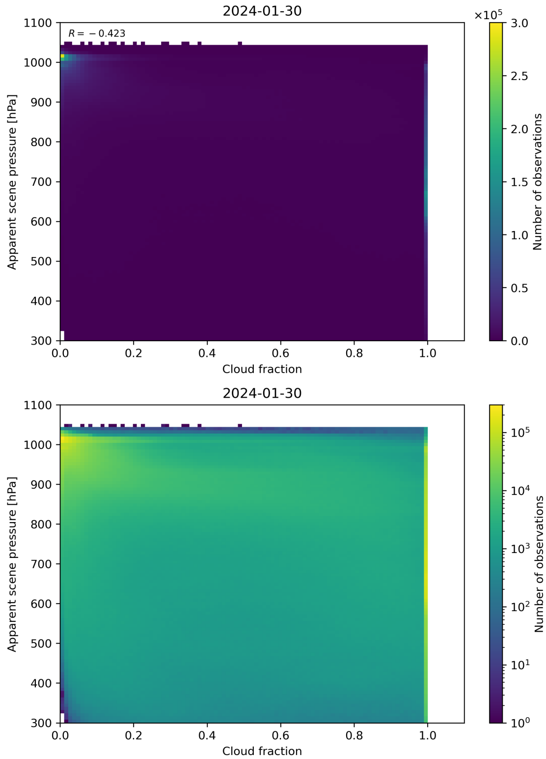
Figure 70: Scatter density plot of “Cloud fraction” against “Apparent scene pressure” for 2024-01-29 to 2024-01-31.
