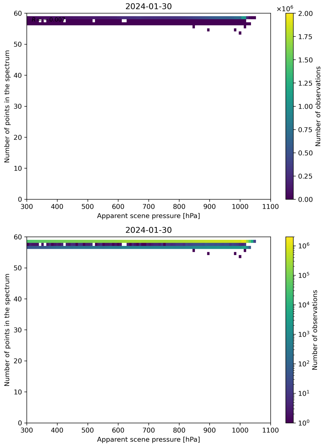
Figure 66: Scatter density plot of “Apparent scene pressure” against “Number of points in the spectrum” for 2024-01-29 to 2024-01-31.
