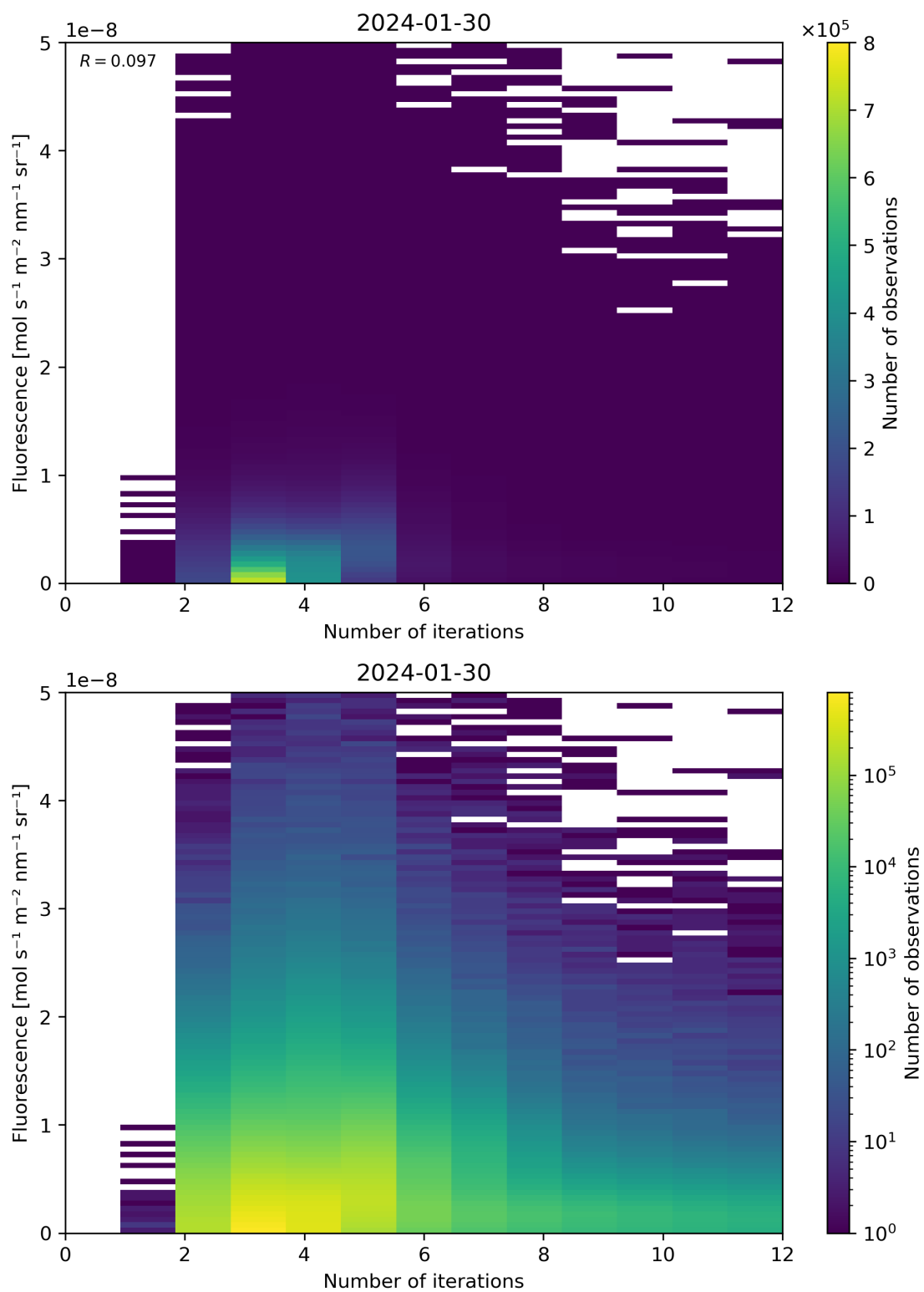
Figure 98: Scatter density plot of “Number of iterations” against “Fluorescence” for 2024-01-29 to 2024-01-31.
