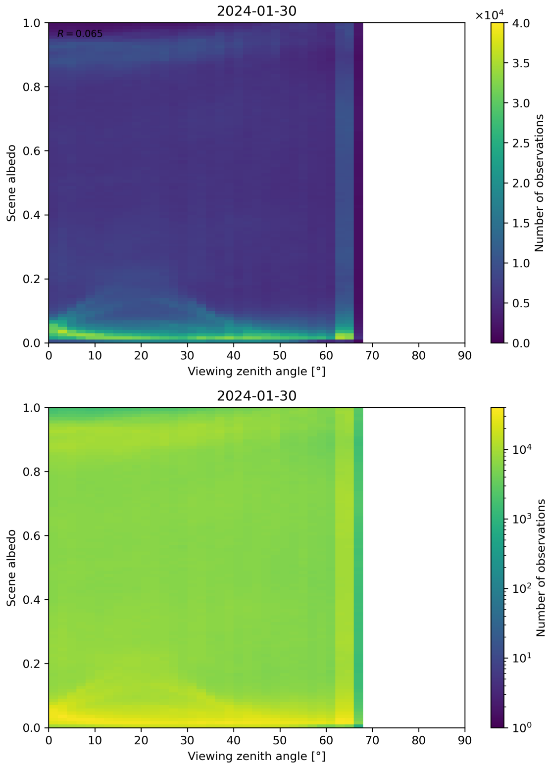
Figure 126: Scatter density plot of “Viewing zenith angle” against “Scene albedo” for 2024-01-29 to 2024-01-31.
