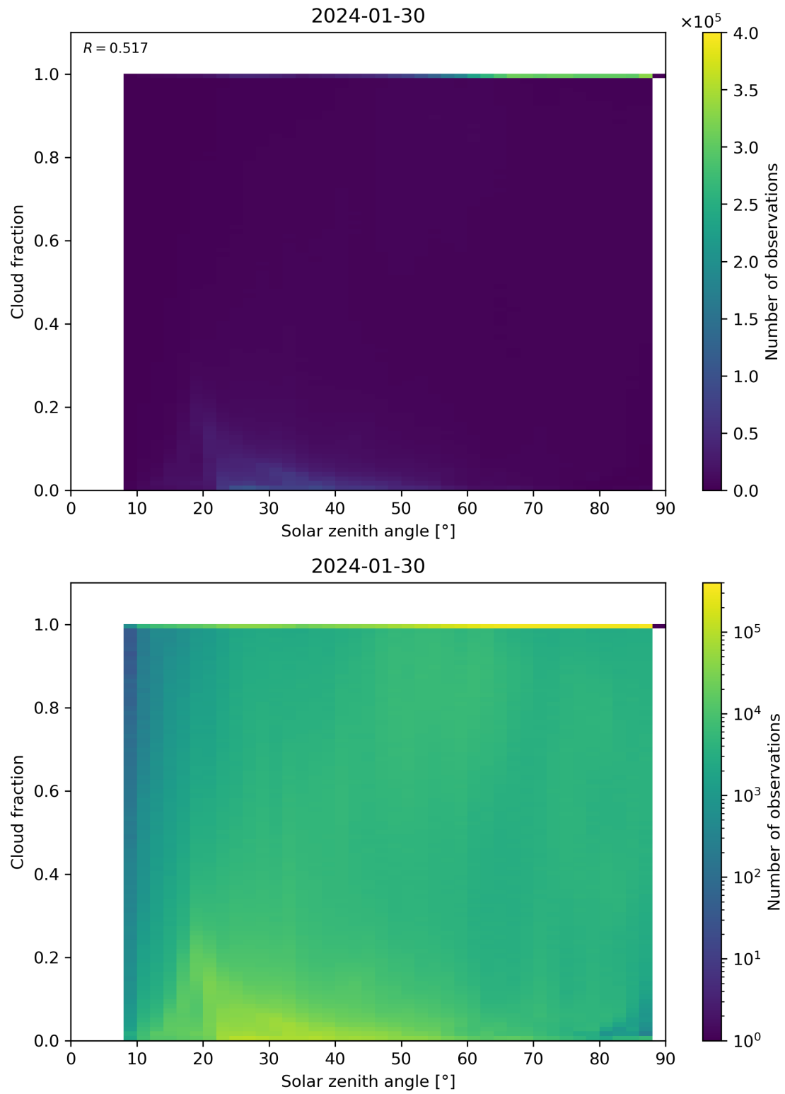
Figure 110: Scatter density plot of “Solar zenith angle” against “Cloud fraction” for 2024-01-29 to 2024-01-31.
