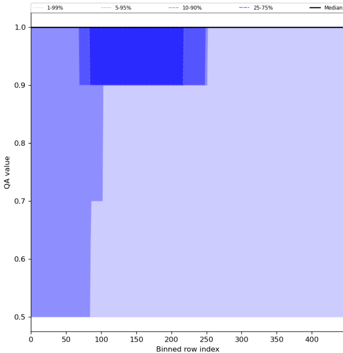
Figure 46: Along track statistics of “QA value” for 2024-01-29 to 2024-01-31
