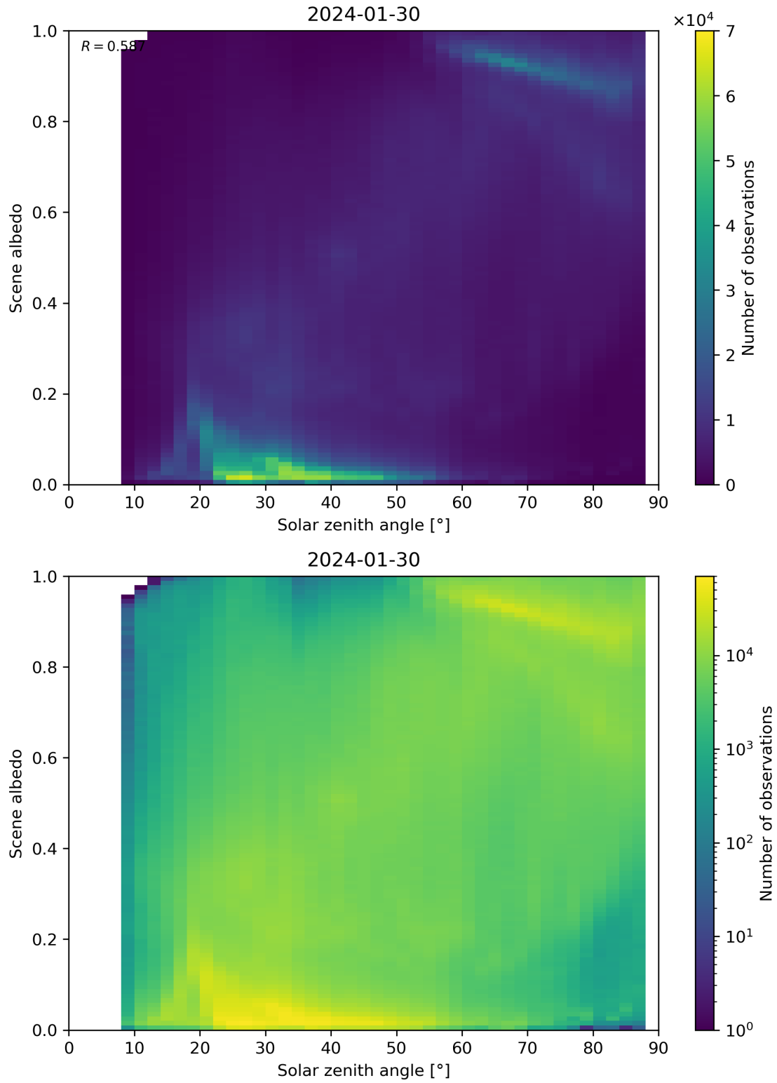
Figure 116: Scatter density plot of “Solar zenith angle” against “Scene albedo” for 2024-01-29 to 2024-01-31.
