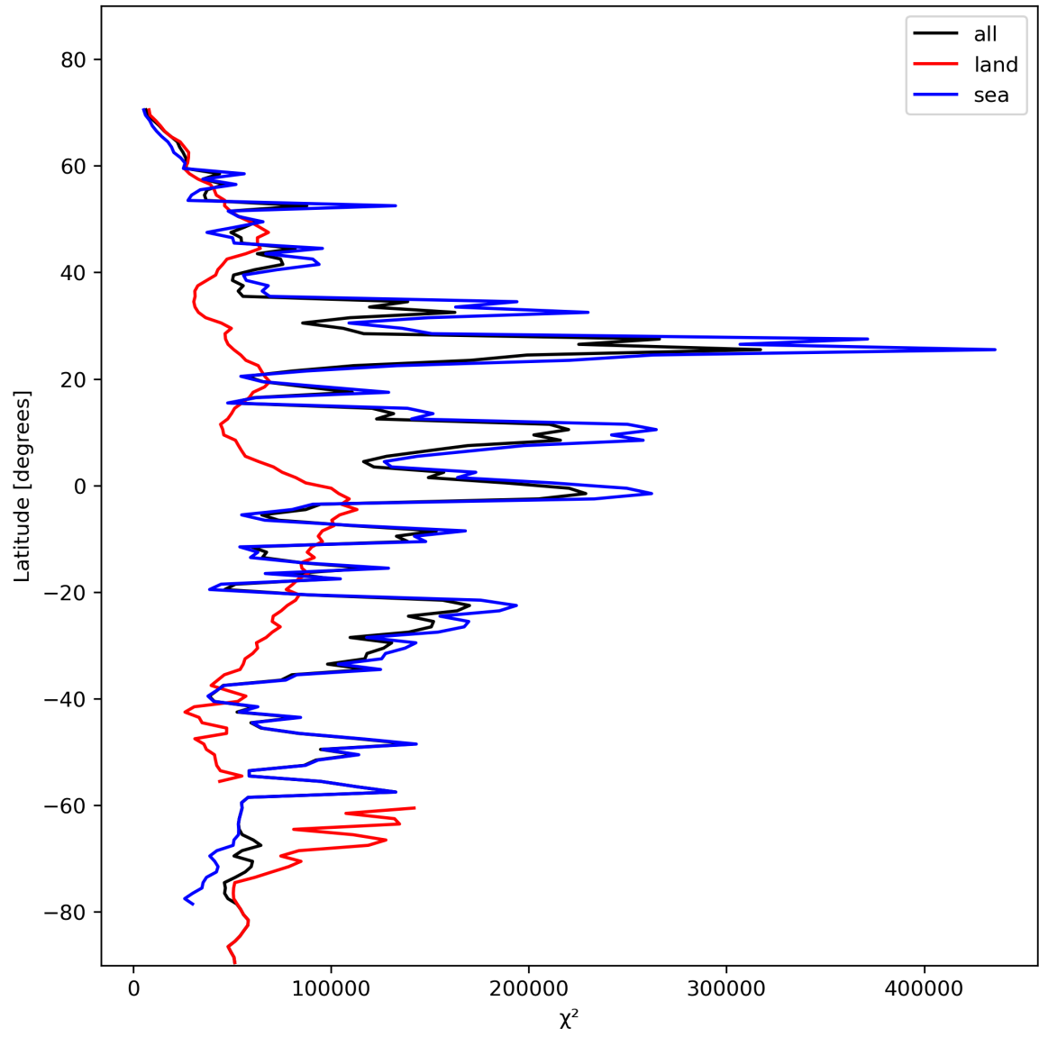
Figure 21: Zonal average of “ \chi^2 ” for 2024-01-29 to 2024-01-31.
