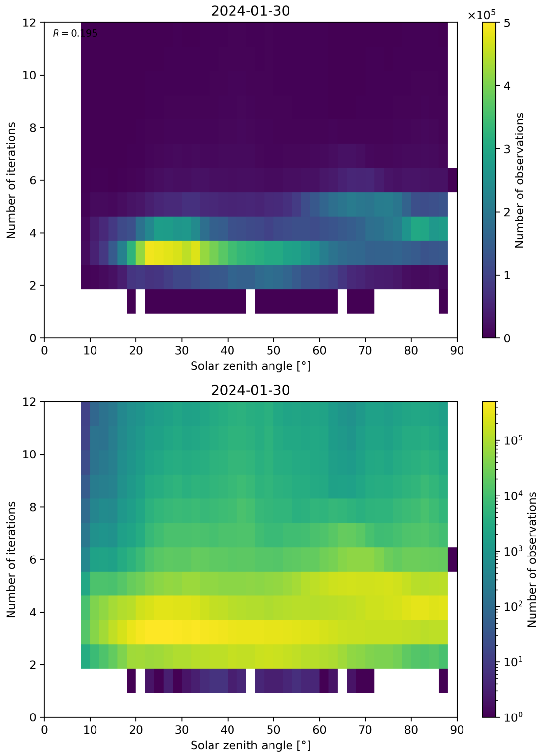
Figure 114: Scatter density plot of “Solar zenith angle” against “Number of iterations” for 2024-01-29 to 2024-01-31.
