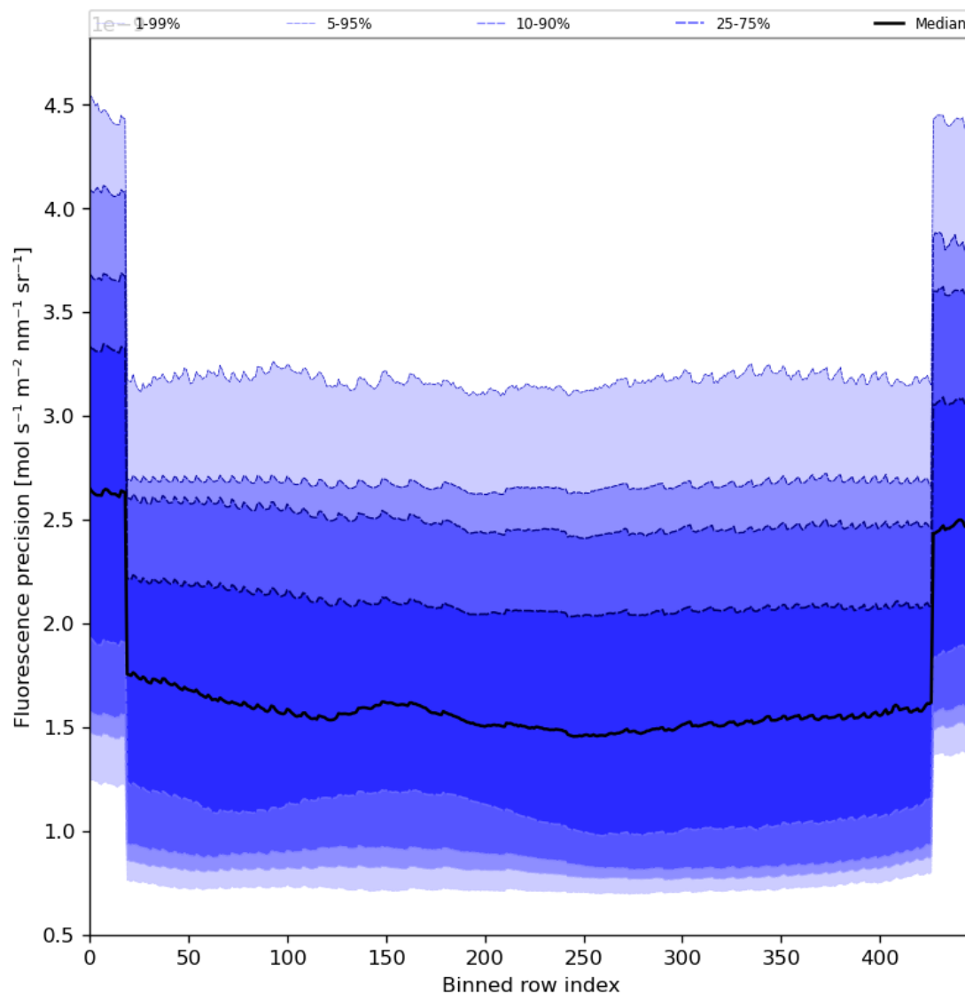
Figure 58: Along track statistics of “Fluorescence precision” for 2024-01-29 to 2024-01-31
