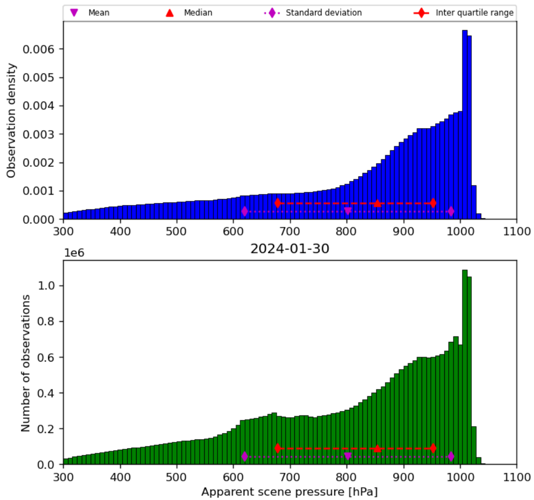
Figure 36: Histogram of “Apparent scene pressure” for 2024-01-29 to 2024-01-31
