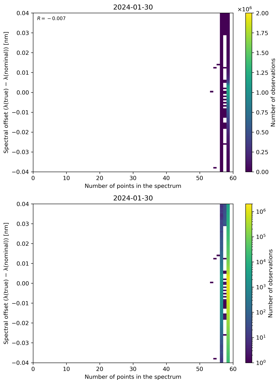
Figure 101: Scatter density plot of “Number of points in the spectrum” against “Spectral offset ( \lambda(\text{true}) - \lambda(\text{nominal}) )” for 2024-01-29 to 2024-01-31.
