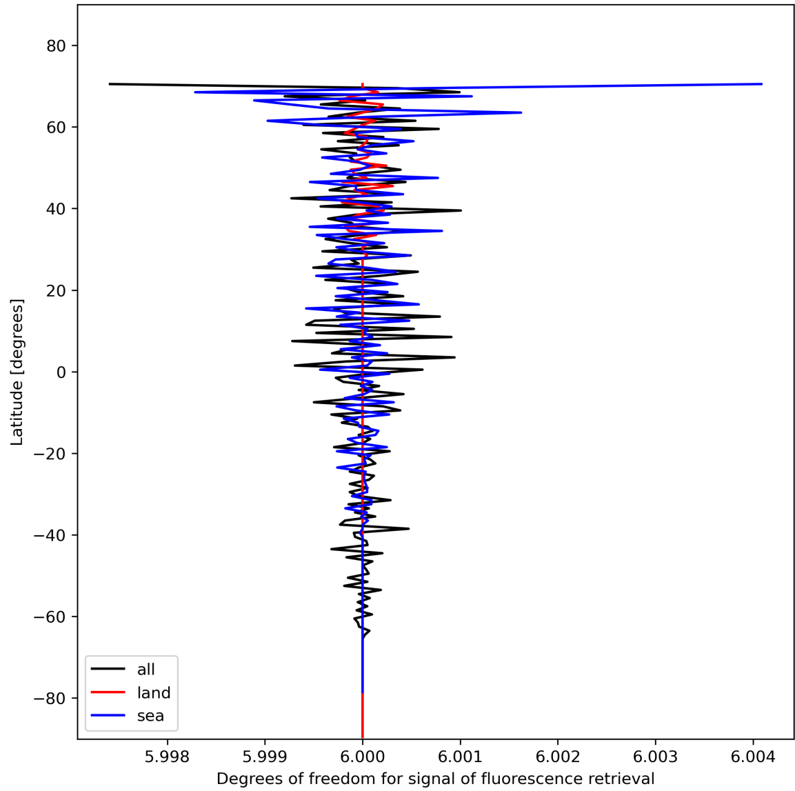
Figure 26: Zonal average of “Degrees of freedom for signal of fluorescence retrieval” for 2024-01-29 to 2024-01-31.
