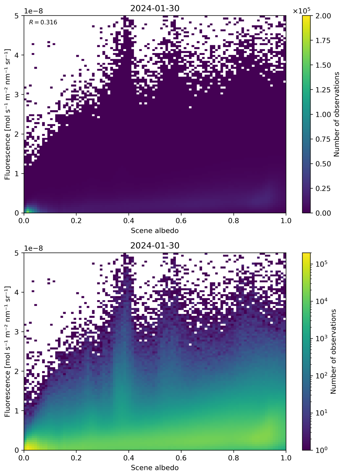
Figure 104: Scatter density plot of “Scene albedo” against “Fluorescence” for 2024-01-29 to 2024-01-31.
