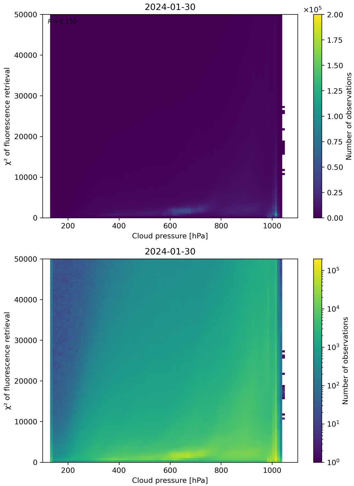
Figure 78: Scatter density plot of “Cloud pressure” against “ \chi^2 of fluorescence retrieval” for 2024-01-29 to 2024-01-31.
