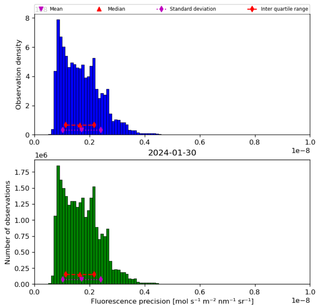
Figure 41: Histogram of “Fluorescence precision” for 2024-01-29 to 2024-01-31
