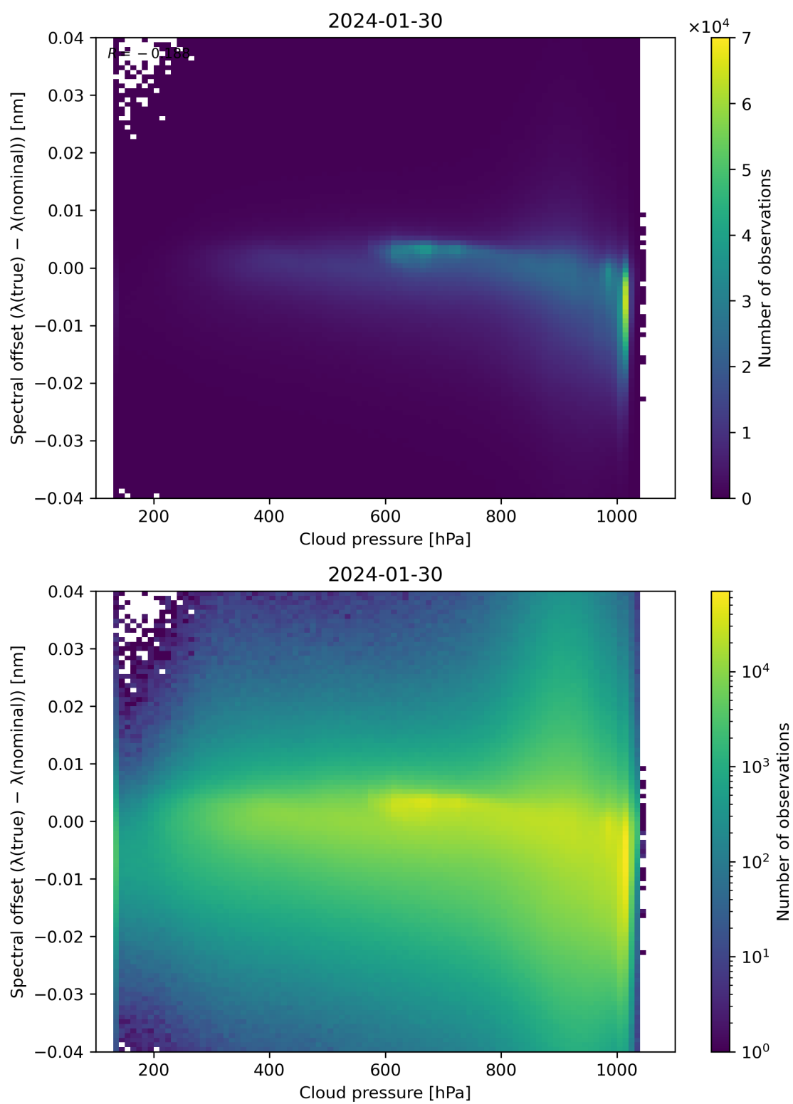
Figure 84: Scatter density plot of “Cloud pressure” against “Spectral offset ( \lambda(\text{true}) - \lambda(\text{nominal}) )” for 2024-01-29 to 2024-01-31.
