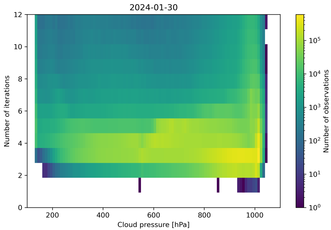
Figure 81: Scatter density plot of “Cloud pressure” against “Number of iterations” for 2024-01-29 to 2024-01-31.
