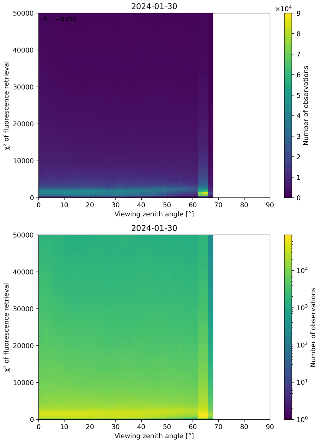
Figure 119: Scatter density plot of “Viewing zenith angle” against “ \chi^2 of fluorescence retrieval” for 2024-01-29 to 2024-01-31.
