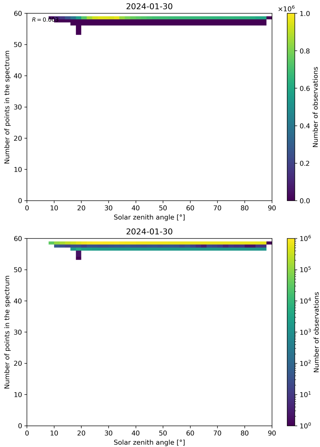
Figure 115: Scatter density plot of “Solar zenith angle” against “Number of points in the spectrum” for 2024-01-29 to 2024-01-31.
