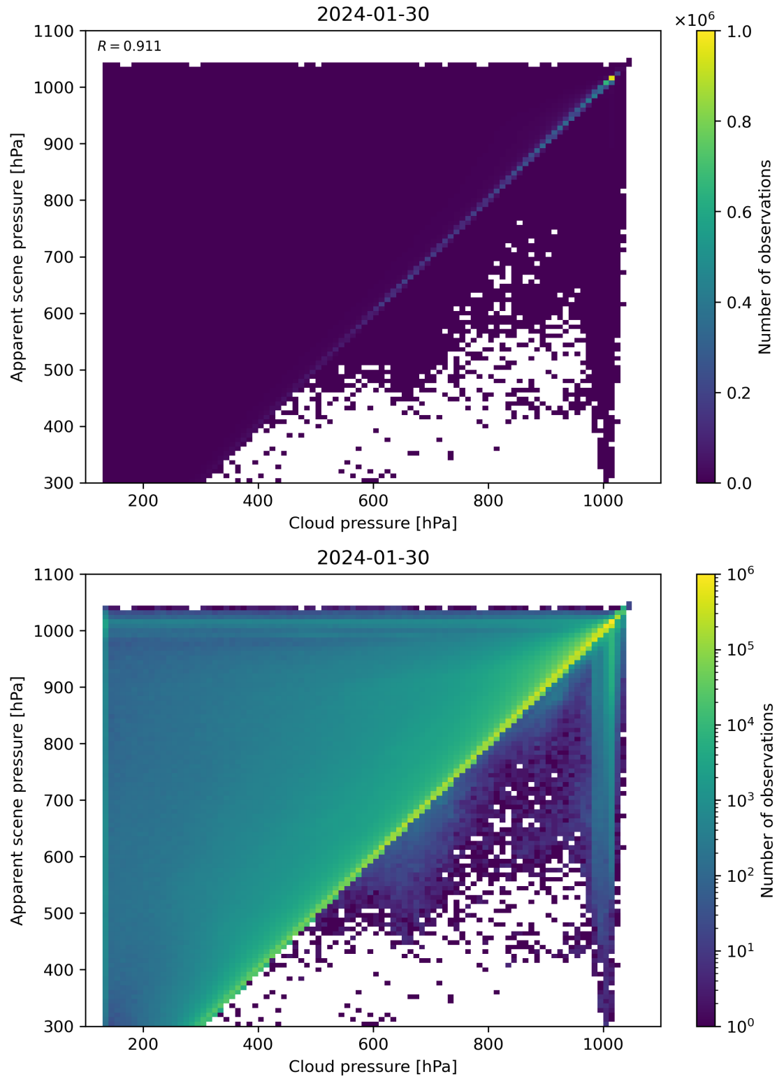
Figure 77: Scatter density plot of “Cloud pressure” against “Apparent scene pressure” for 2024-01-29 to 2024-01-31.
