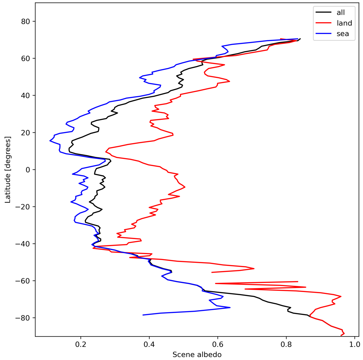
Figure 17: Zonal average of “Scene albedo” for 2024-01-29 to 2024-01-31.
