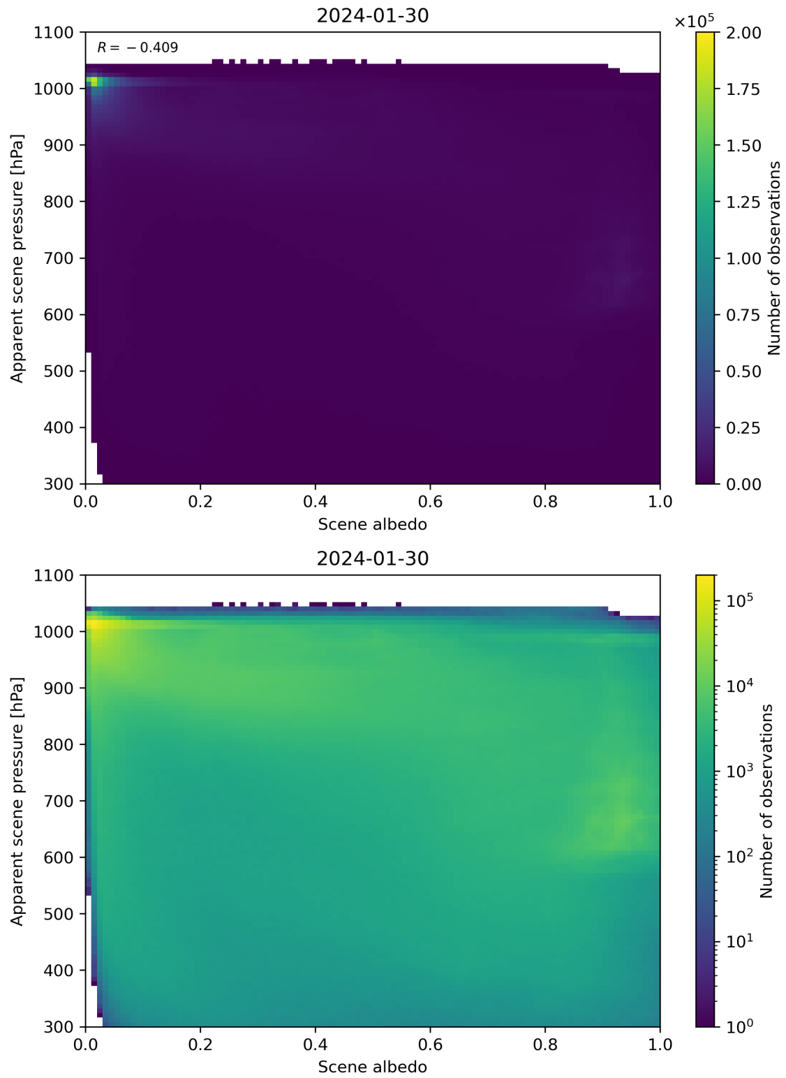
Figure 102: Scatter density plot of “Scene albedo” against “Apparent scene pressure” for 2024-01-29 to 2024-01-31.
