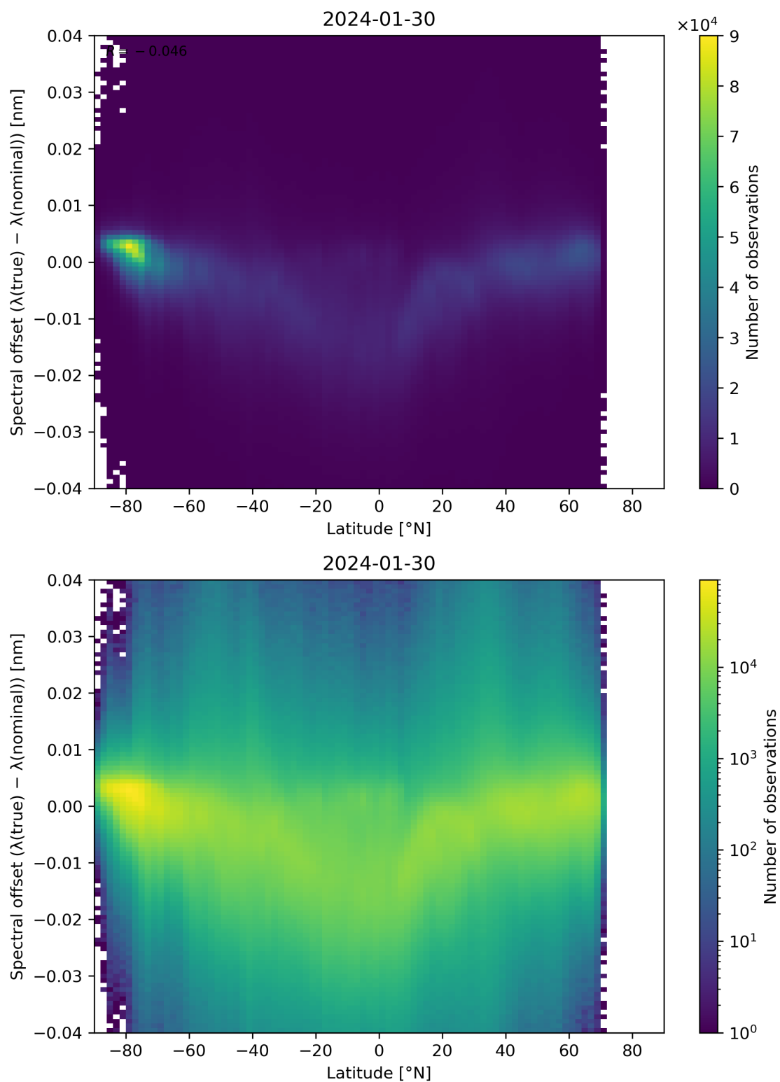
Figure 96: Scatter density plot of “Latitude” against “Spectral offset ( \lambda(\text{true}) - \lambda(\text{nominal}) )” for 2024-01-29 to 2024-01-31.
