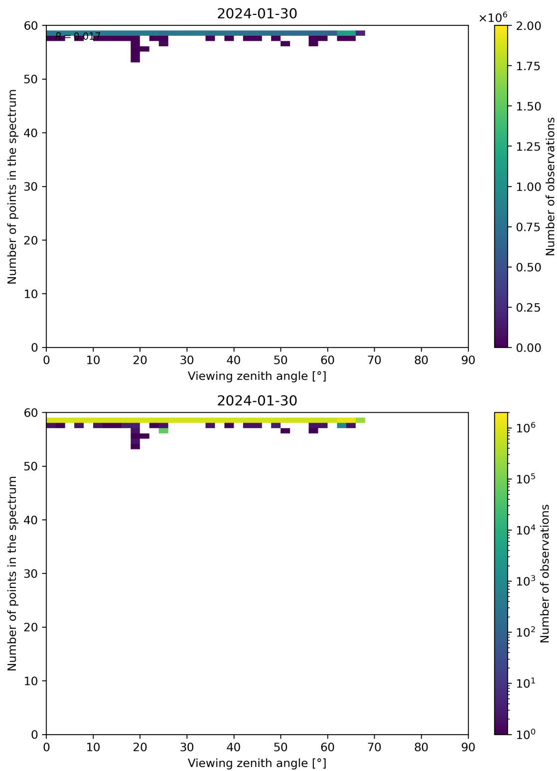
Figure 125: Scatter density plot of “Viewing zenith angle” against “Number of points in the spectrum” for 2024-01-29 to 2024-01-31.
