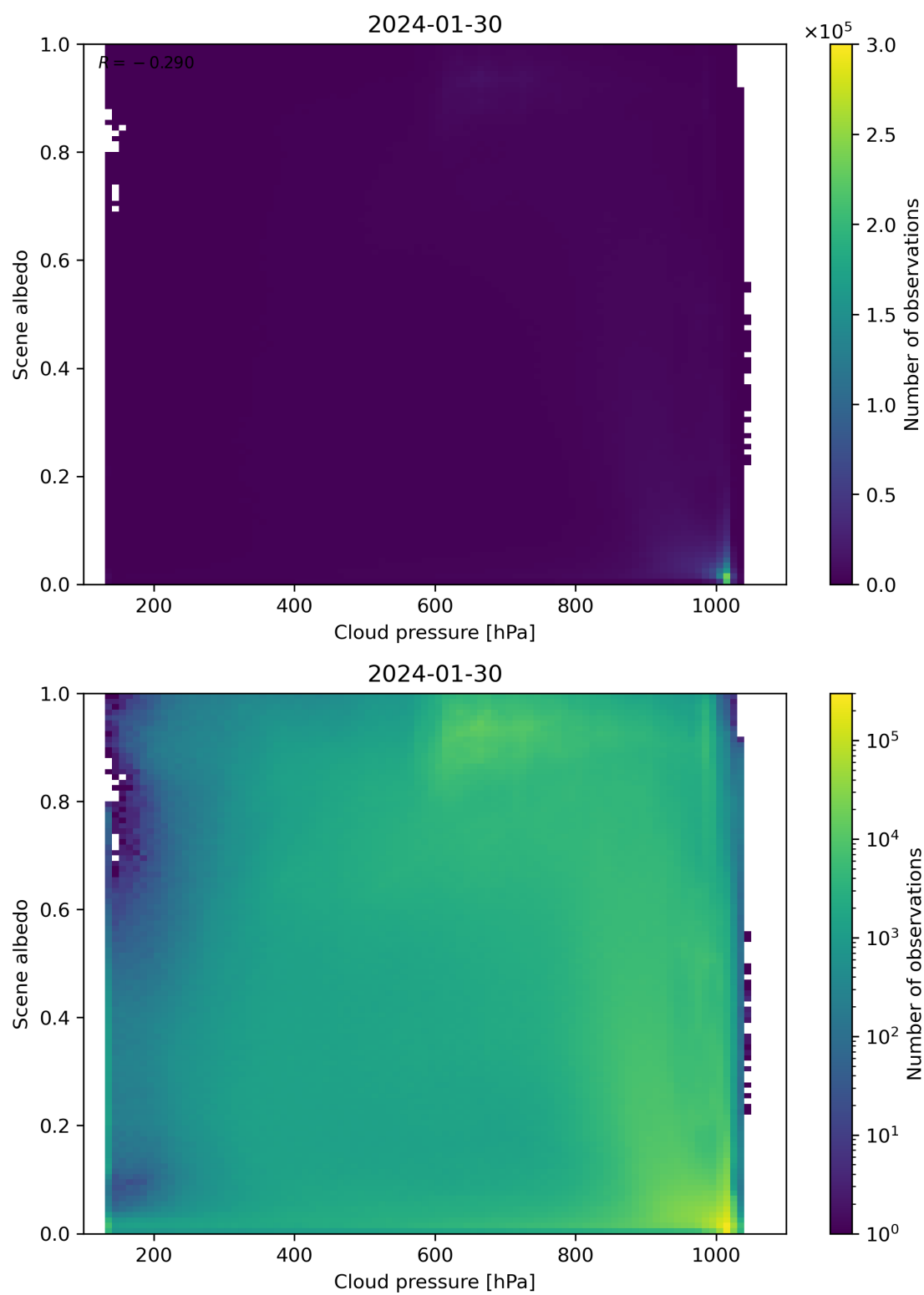
Figure 83: Scatter density plot of “Cloud pressure” against “Scene albedo” for 2024-01-29 to 2024-01-31.
