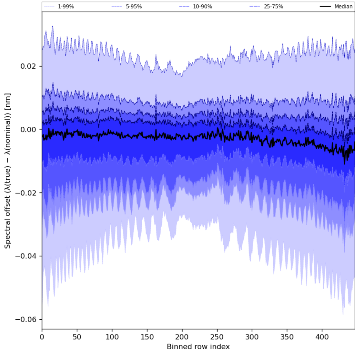
Figure 62: Along track statistics of “Spectral offset ( \lambda(\text{true}) - \lambda(\text{nominal}) )” for 2024-01-29 to 2024-01-31
