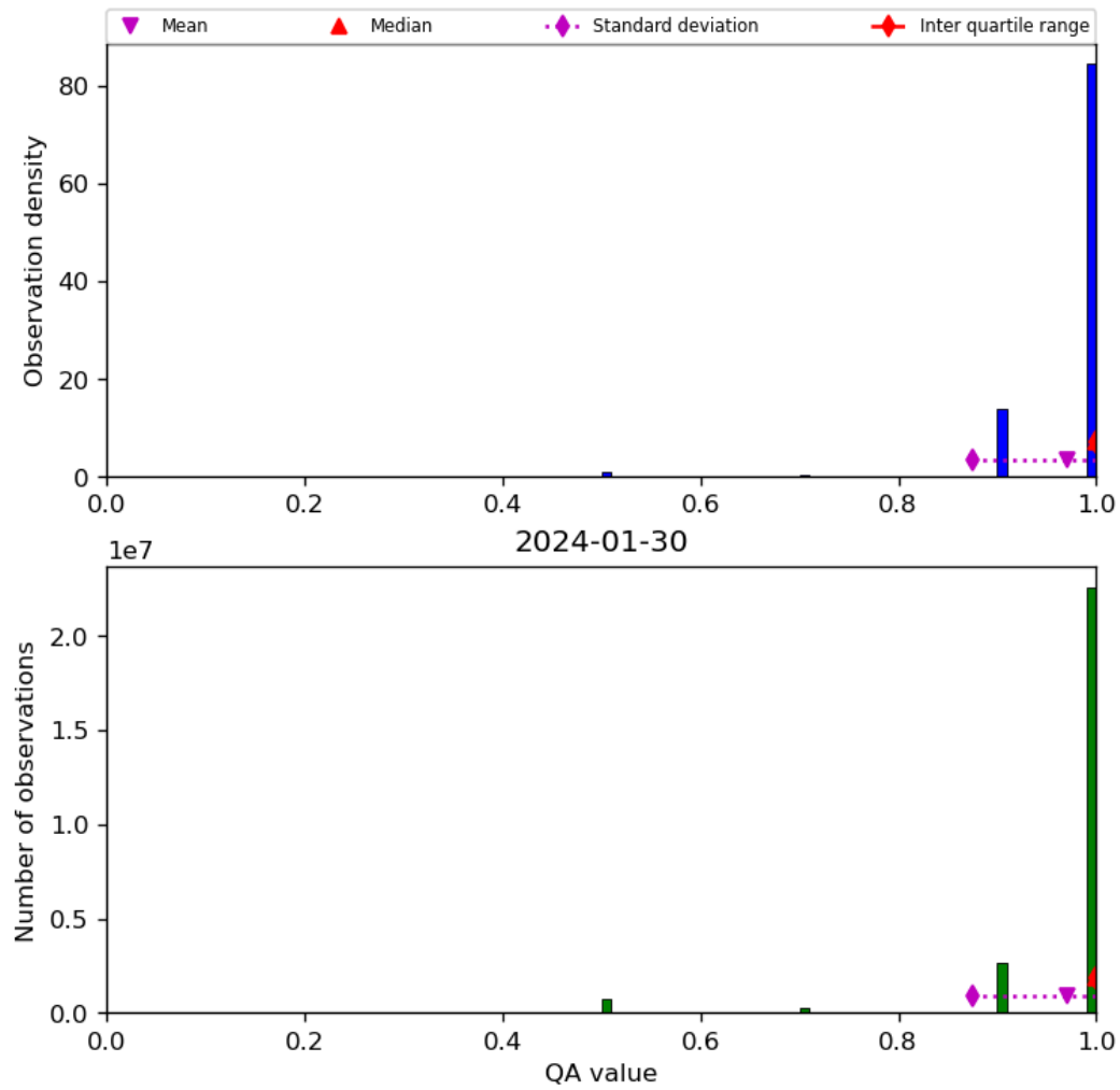
Figure 29: Histogram of “QA value” for 2024-01-29 to 2024-01-31
