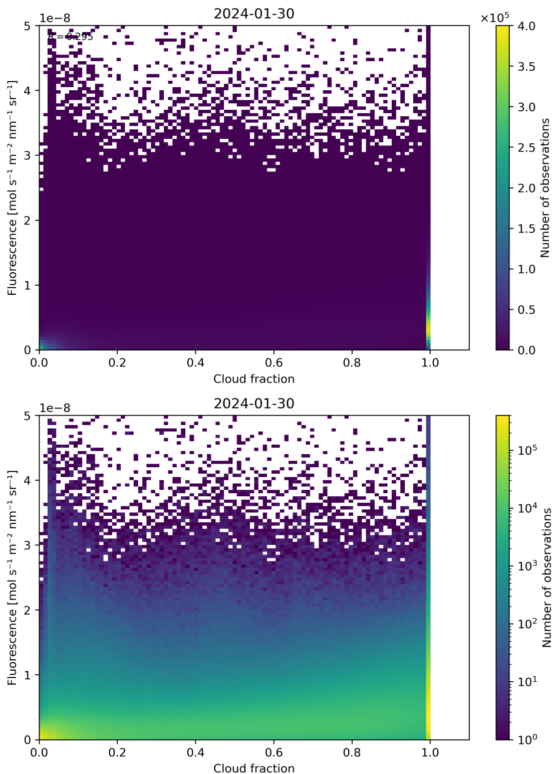
Figure 72: Scatter density plot of “Cloud fraction” against “Fluorescence” for 2024-01-29 to 2024-01-31.
