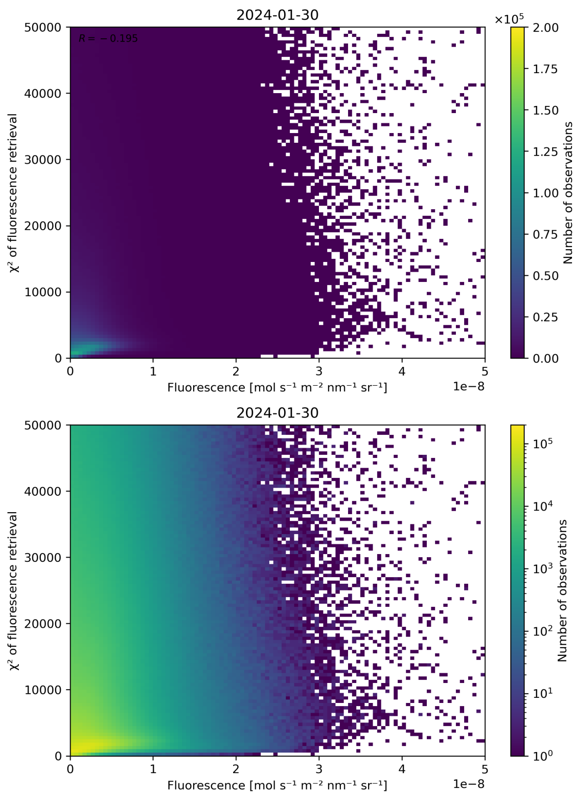
Figure 85: Scatter density plot of “Fluorescence” against “ \chi^2 of fluorescence retrieval” for 2024-01-29 to 2024-01-31.
