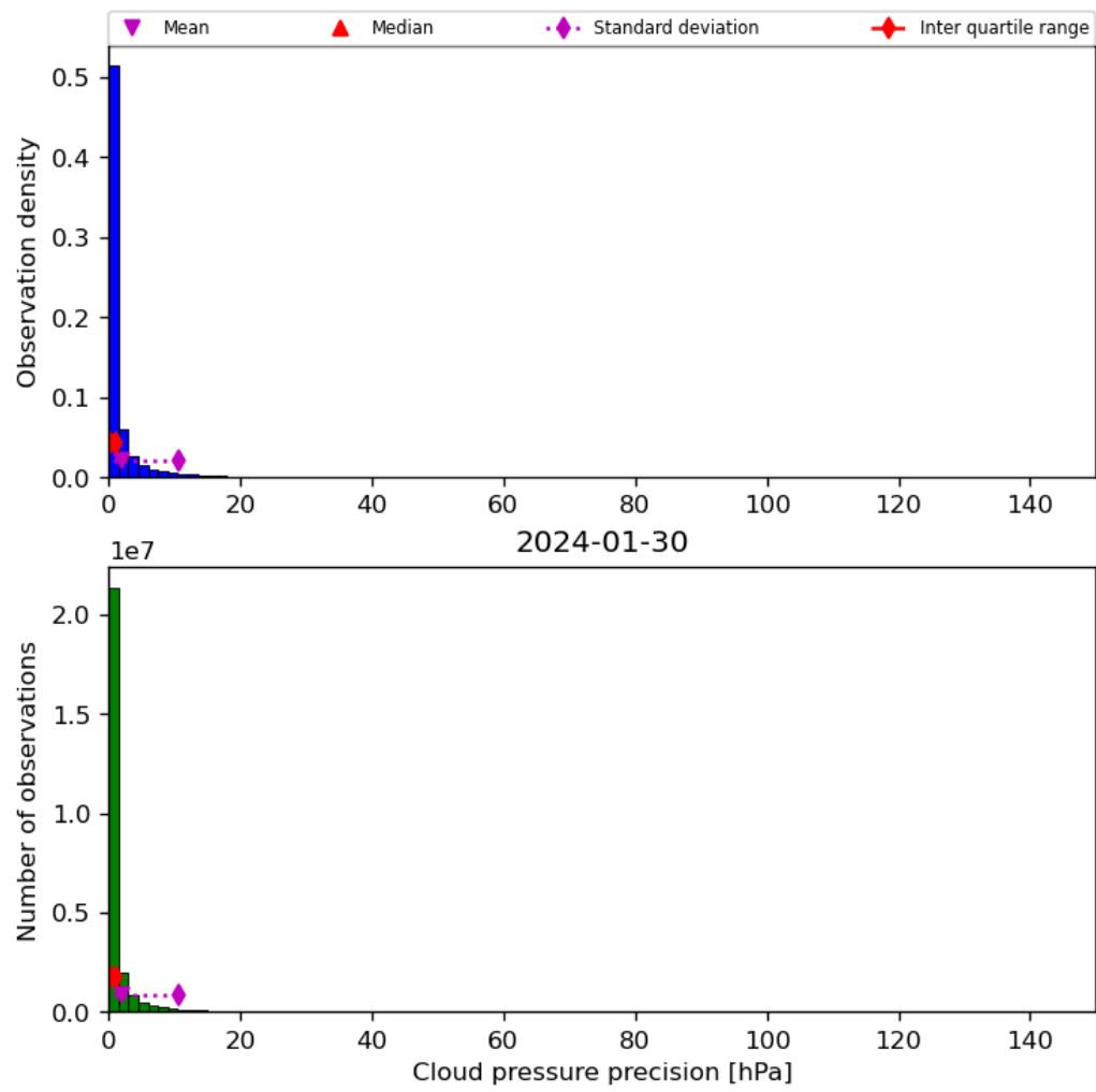
Figure 31: Histogram of “Cloud pressure precision” for 2024-01-29 to 2024-01-31
