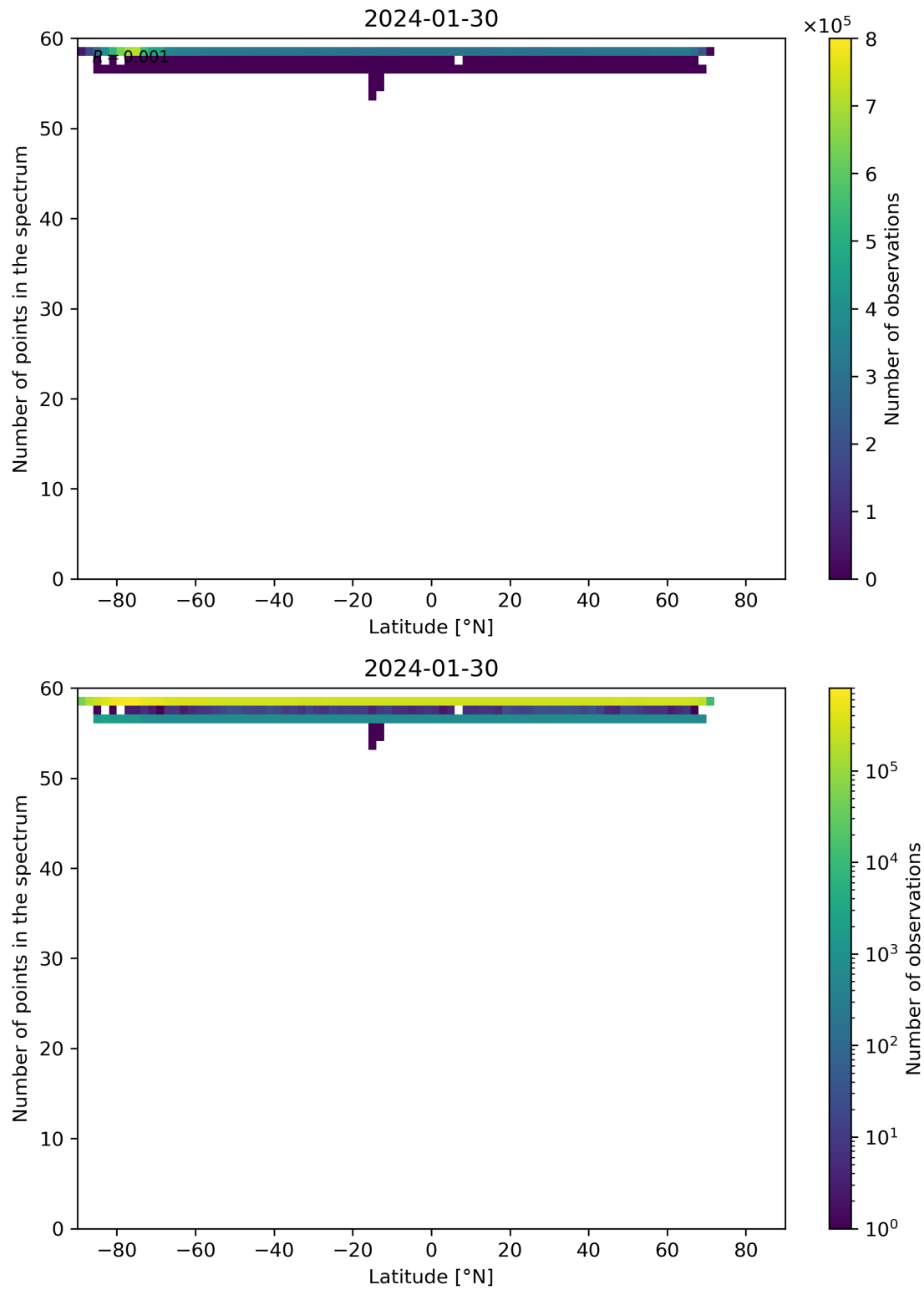
Figure 94: Scatter density plot of “Latitude” against “Number of points in the spectrum” for 2024-01-29 to 2024-01-31.
