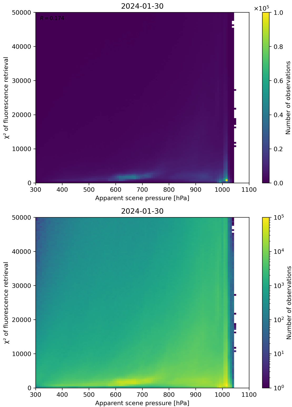
Figure 63: Scatter density plot of “Apparent scene pressure” against “ \chi^2 of fluorescence retrieval” for 2024-01-29 to 2024-01-31.
