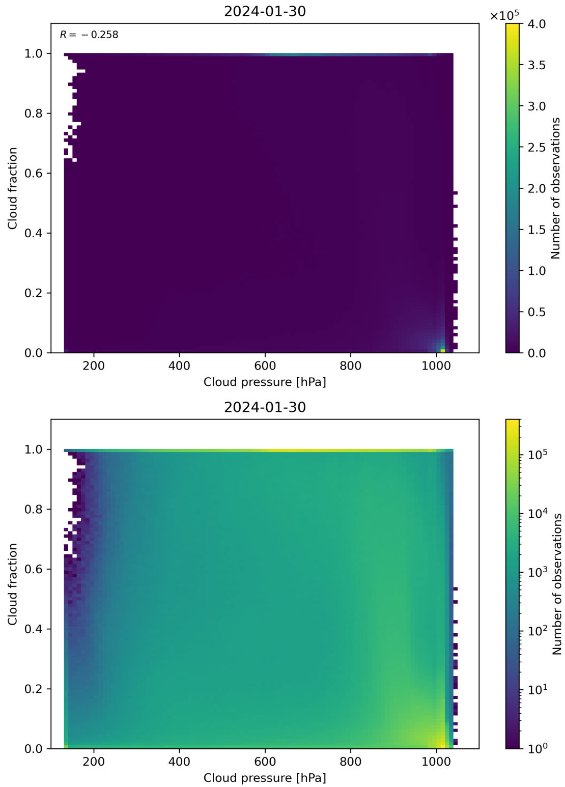
Figure 79: Scatter density plot of “Cloud pressure” against “Cloud fraction” for 2024-01-29 to 2024-01-31.
