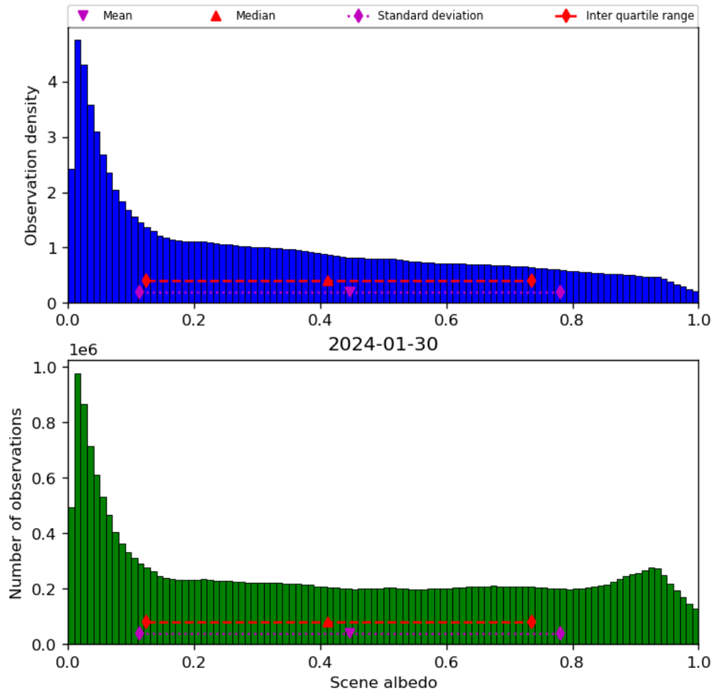
Figure 34: Histogram of “Scene albedo” for 2024-01-29 to 2024-01-31
