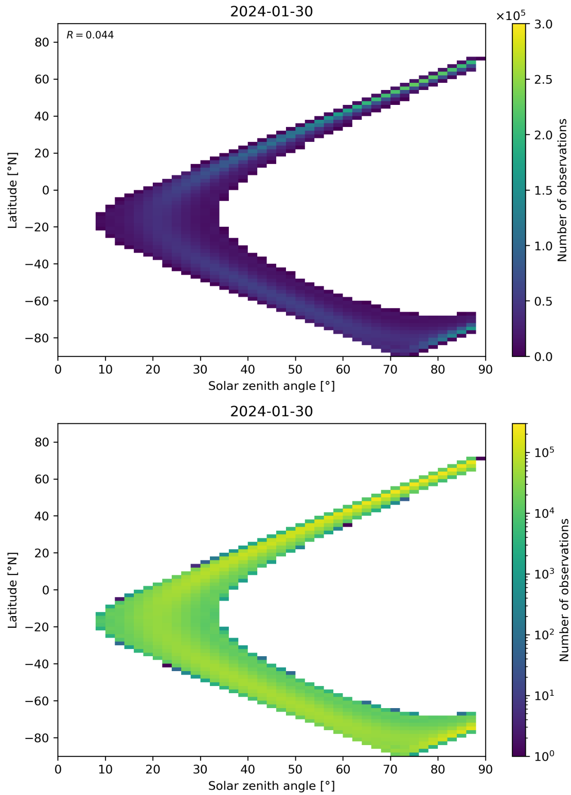
Figure 113: Scatter density plot of “Solar zenith angle” against “Latitude” for 2024-01-29 to 2024-01-31.
