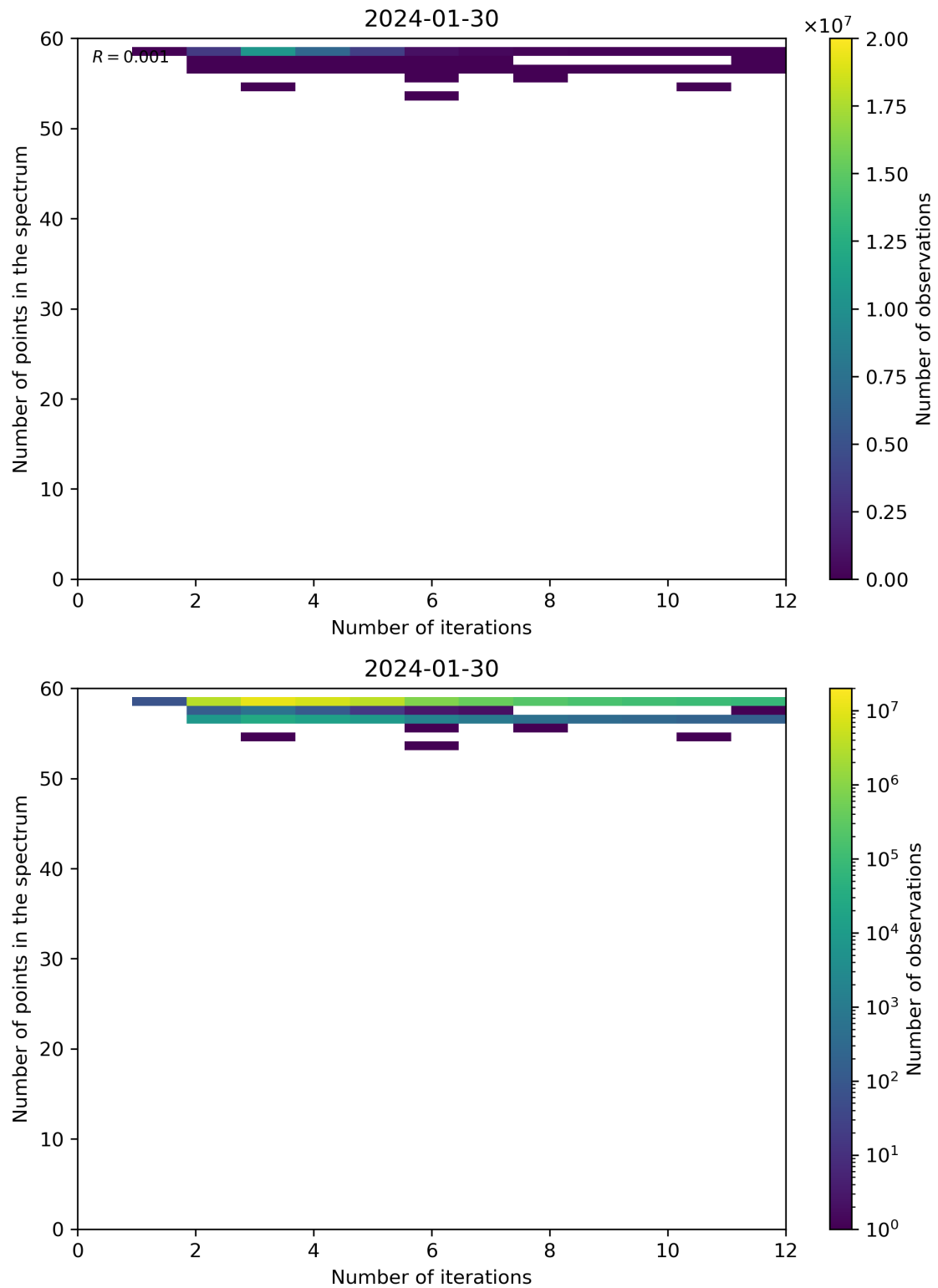
Figure 99: Scatter density plot of “Number of iterations” against “Number of points in the spectrum” for 2024-01-29 to 2024-01-31.
