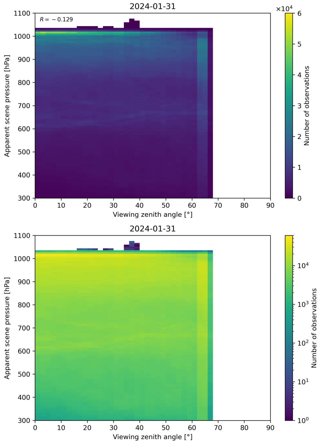
Figure 118: Scatter density plot of “Viewing zenith angle” against “Apparent scene pressure” for 2024-01-31 to 2024-02-01.
