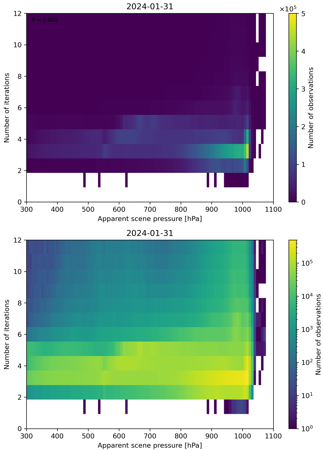
Figure 65: Scatter density plot of “Apparent scene pressure” against “Number of iterations” for 2024-01-31 to 2024-02-01.
