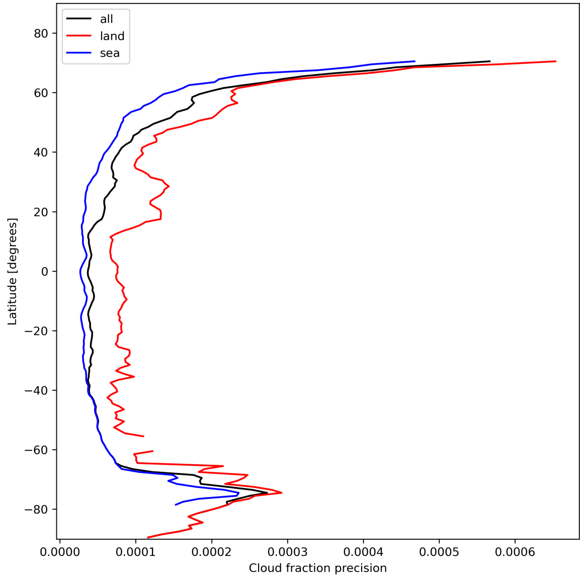
Figure 16: Zonal average of “Cloud fraction precision” for 2024-01-31 to 2024-02-01.
