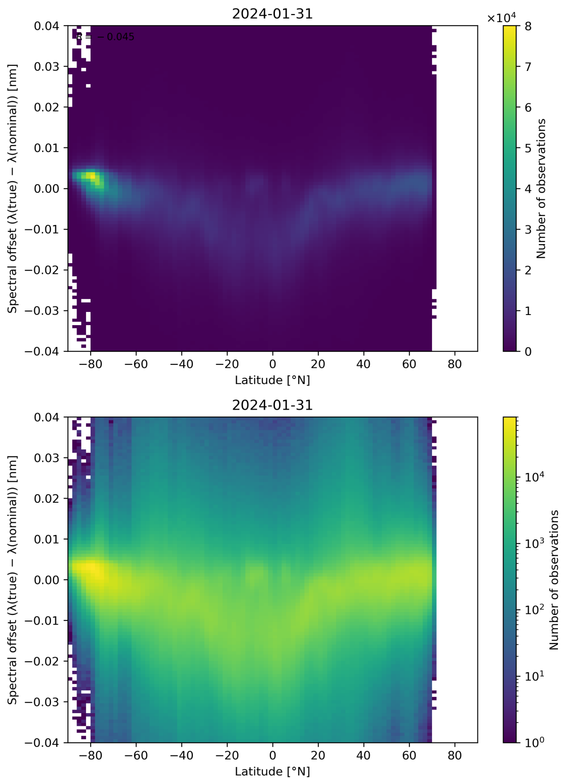
Figure 96: Scatter density plot of “Latitude” against “Spectral offset ( \lambda(\text{true}) - \lambda(\text{nominal}) )” for 2024-01-31 to 2024-02-01.
