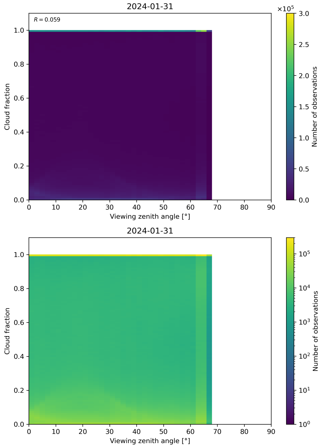
Figure 120: Scatter density plot of “Viewing zenith angle” against “Cloud fraction” for 2024-01-31 to 2024-02-01.
