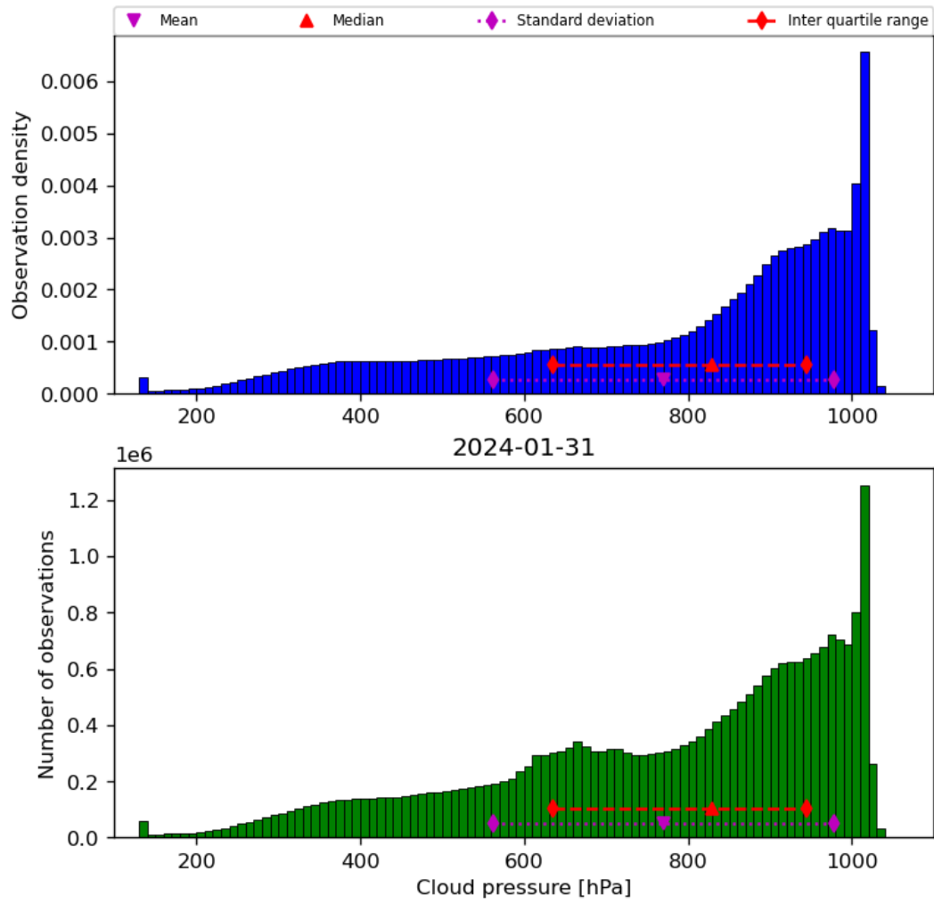
Figure 30: Histogram of “Cloud pressure” for 2024-01-31 to 2024-02-01
