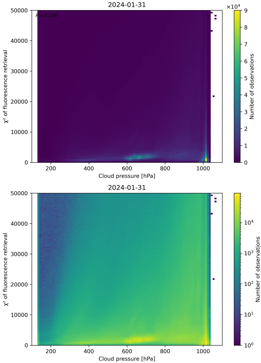
Figure 78: Scatter density plot of “Cloud pressure” against “ \chi^2 of fluorescence retrieval” for 2024-01-31 to 2024-02-01.
