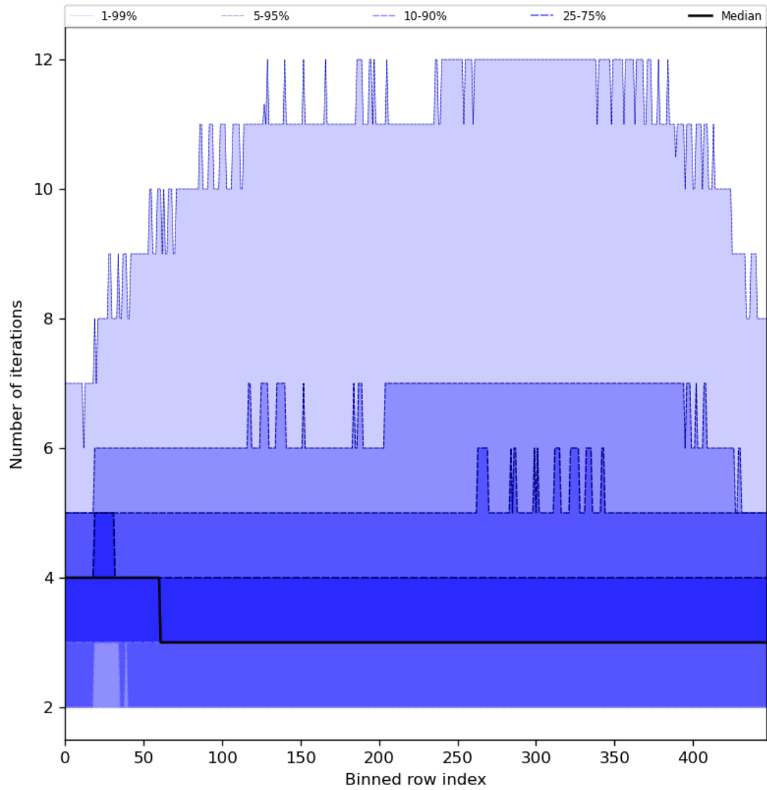
Figure 56: Along track statistics of “Number of iterations” for 2024-01-31 to 2024-02-01
