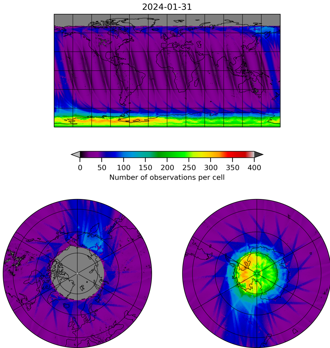
Figure 11: Map of the number of observations for 2024-01-31 to 2024-02-01
