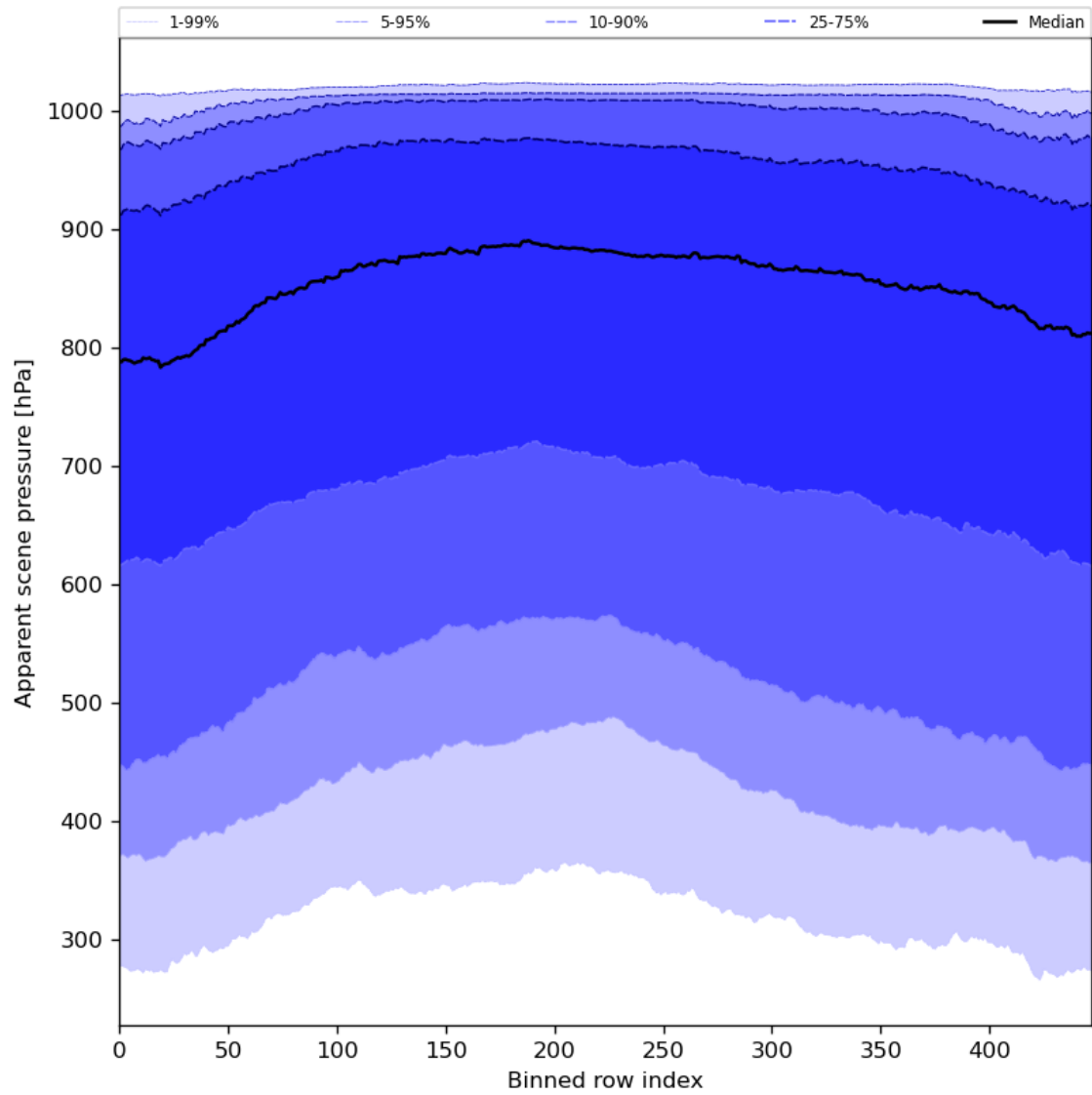
Figure 53: Along track statistics of “Apparent scene pressure” for 2024-01-31 to 2024-02-01
