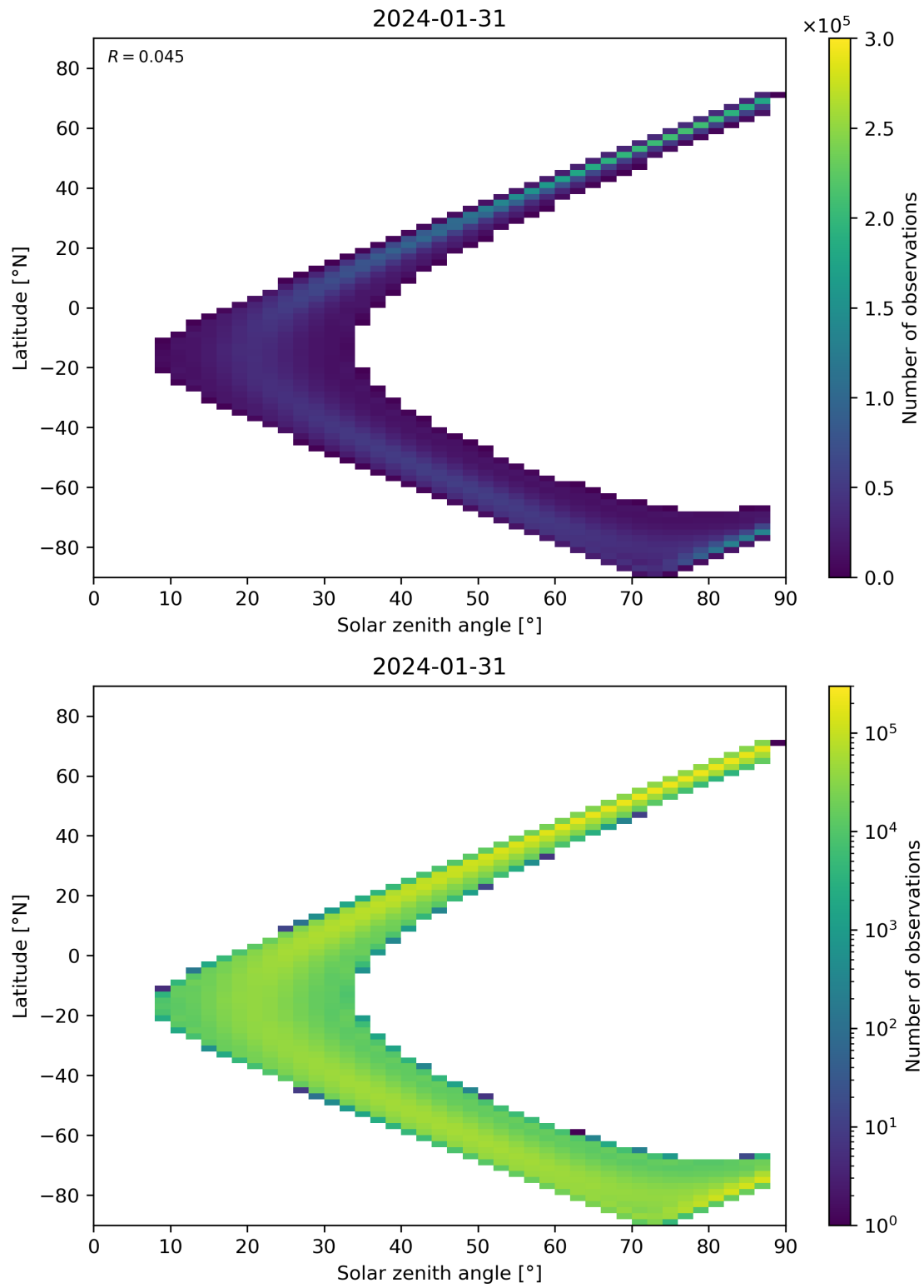
Figure 113: Scatter density plot of “Solar zenith angle” against “Latitude” for 2024-01-31 to 2024-02-01.
