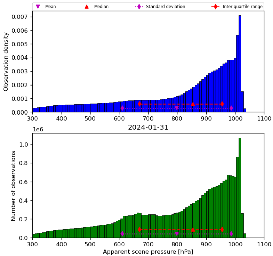
Figure 36: Histogram of “Apparent scene pressure” for 2024-01-31 to 2024-02-01
