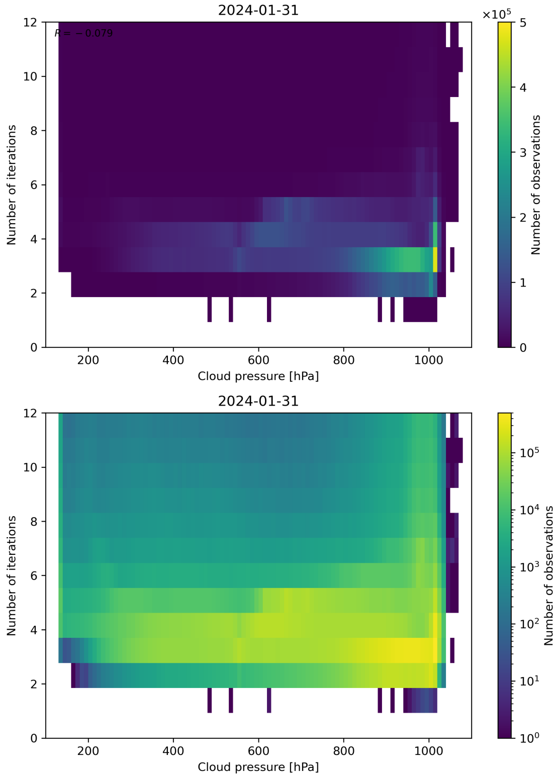
Figure 81: Scatter density plot of “Cloud pressure” against “Number of iterations” for 2024-01-31 to 2024-02-01.
