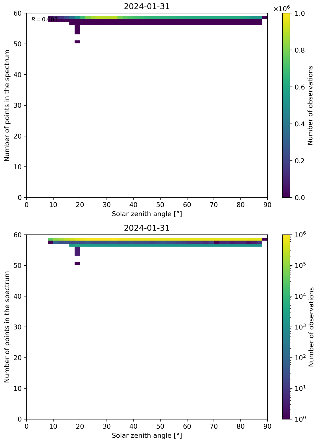
Figure 115: Scatter density plot of “Solar zenith angle” against “Number of points in the spectrum” for 2024-01-31 to 2024-02-01.
