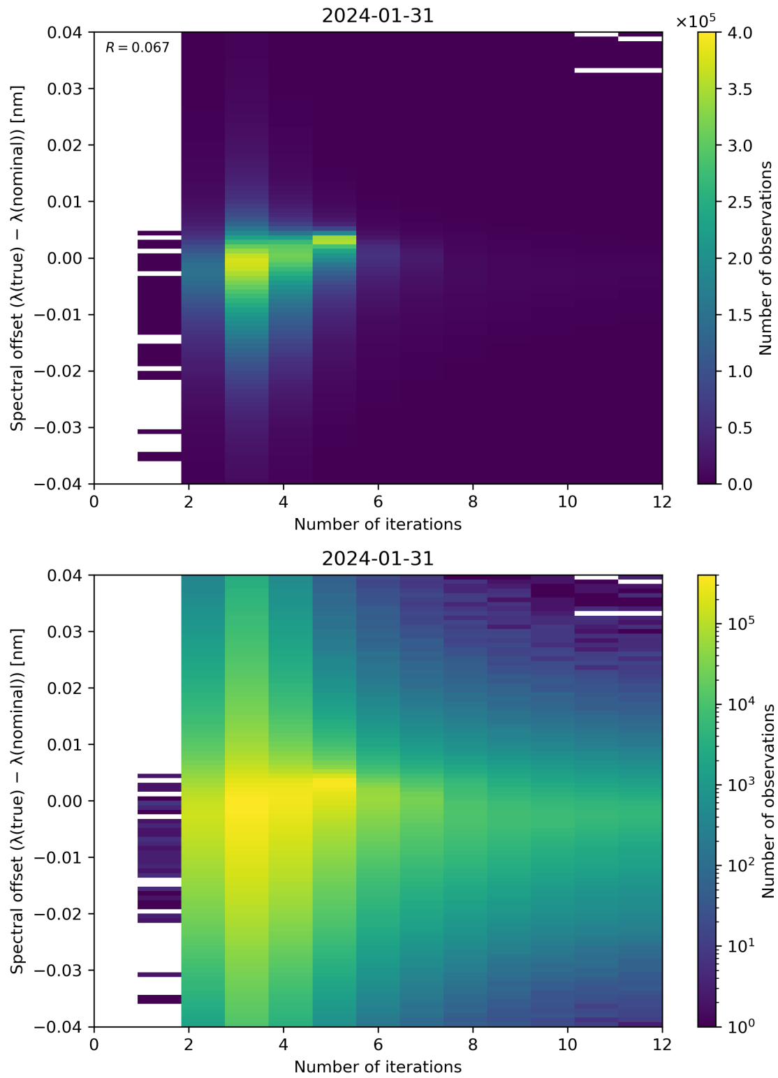
Figure 100: Scatter density plot of “Number of iterations” against “Spectral offset ( \lambda(\text{true}) - \lambda(\text{nominal}) )” for 2024-01-31 to 2024-02-01.
