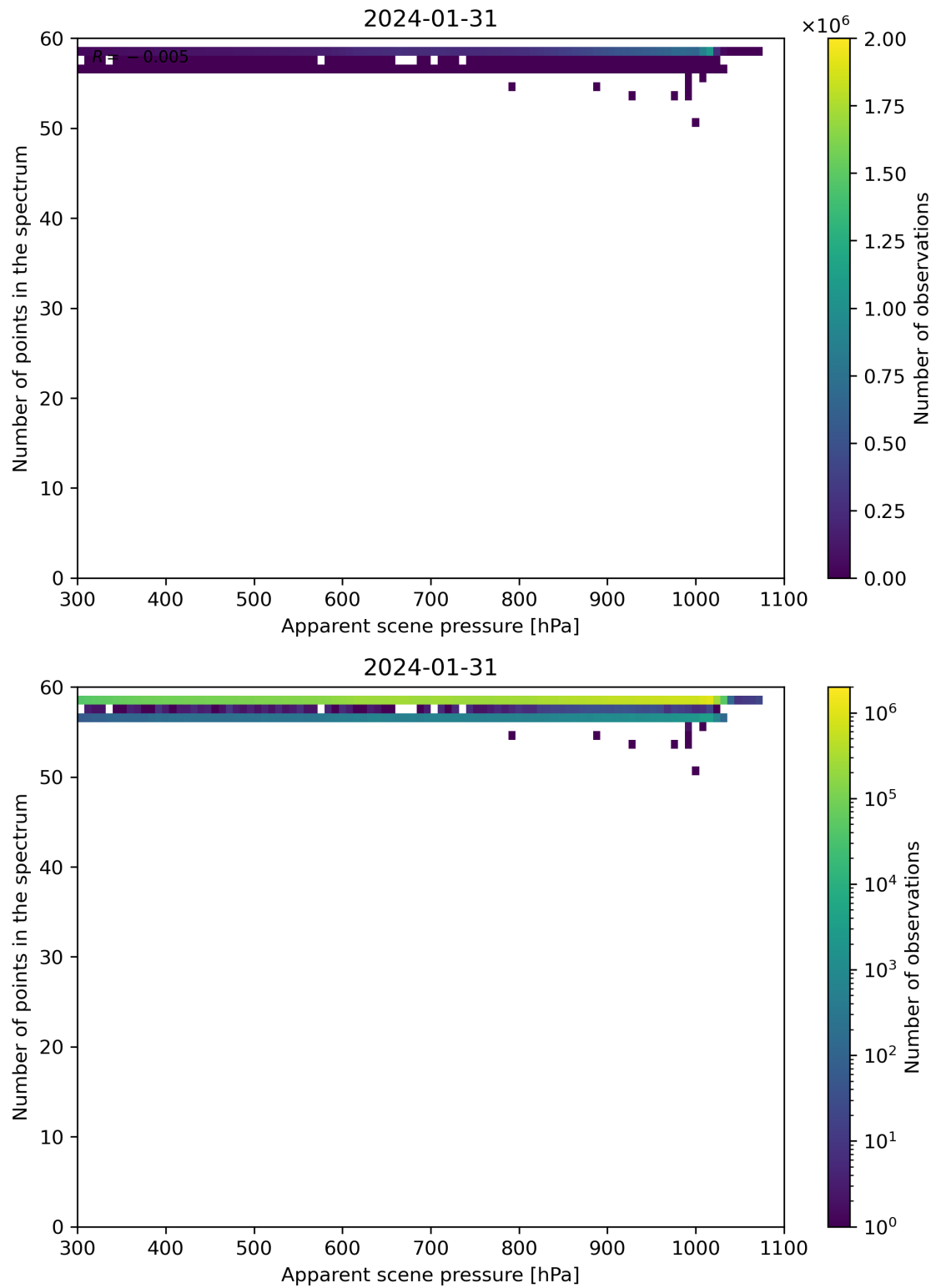
Figure 66: Scatter density plot of “Apparent scene pressure” against “Number of points in the spectrum” for 2024-01-31 to 2024-02-01.
