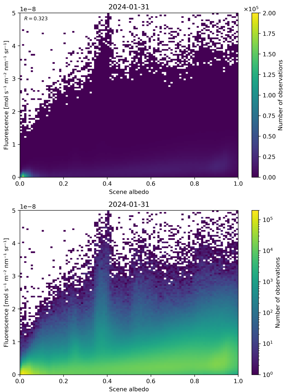
Figure 104: Scatter density plot of “Scene albedo” against “Fluorescence” for 2024-01-31 to 2024-02-01.
