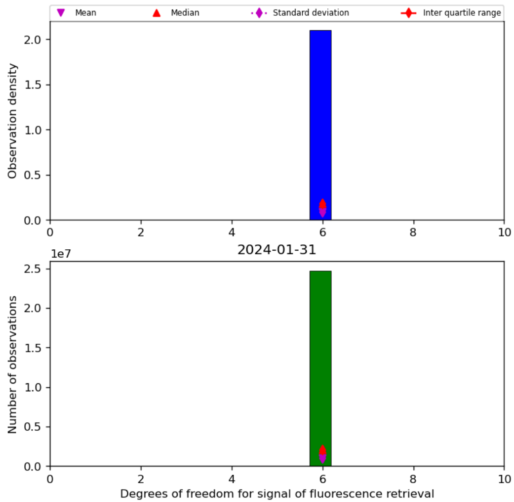
Figure 43: Histogram of “Degrees of freedom for signal of fluorescence retrieval” for 2024-01-31 to 2024-02-01
