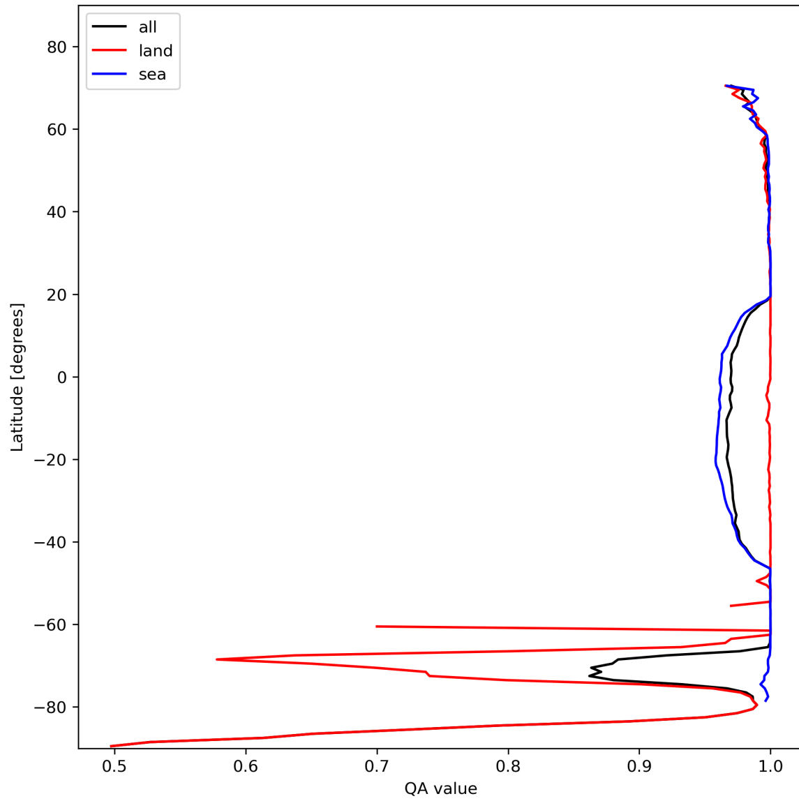
Figure 12: Zonal average of “QA value” for 2024-01-31 to 2024-02-01.
