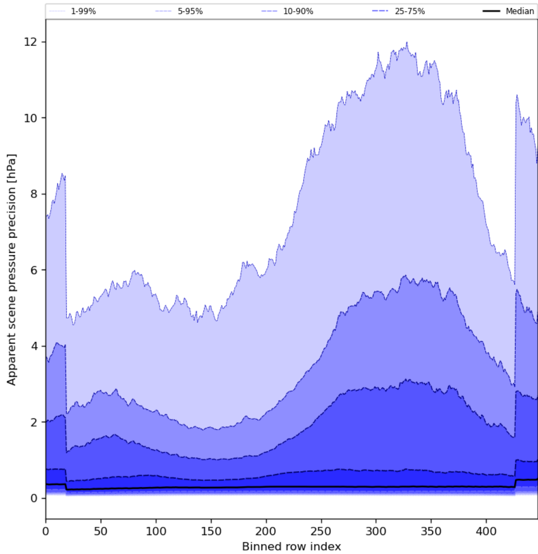
Figure 54: Along track statistics of “Apparent scene pressure precision” for 2024-01-31 to 2024-02-01
