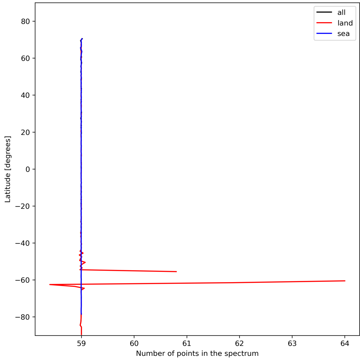
Figure 27: Zonal average of “Number of points in the spectrum” for 2024-01-31 to 2024-02-01.
