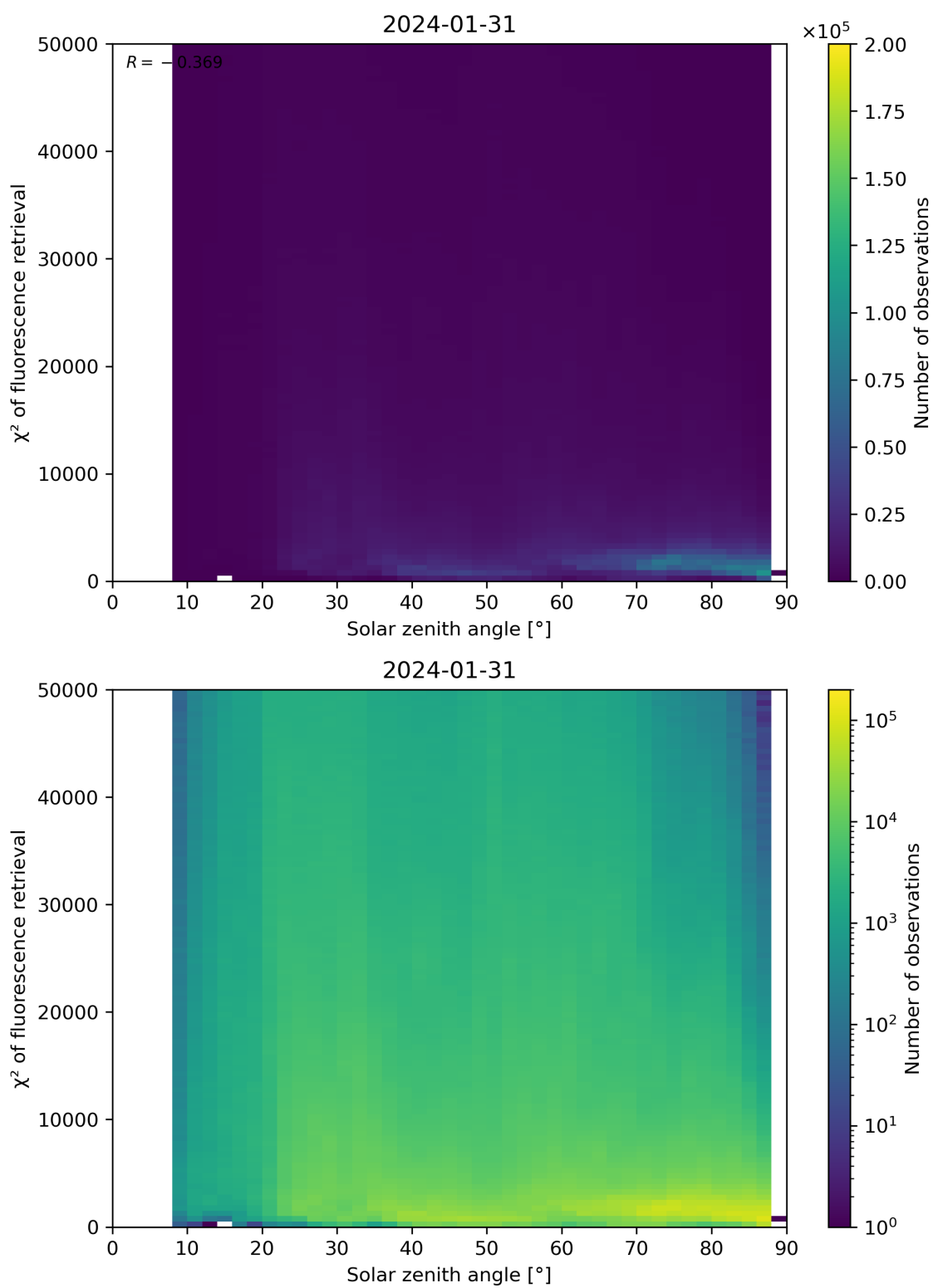
Figure 109: Scatter density plot of “Solar zenith angle” against “ \chi^2 of fluorescence retrieval” for 2024-01-31 to 2024-02-01.
