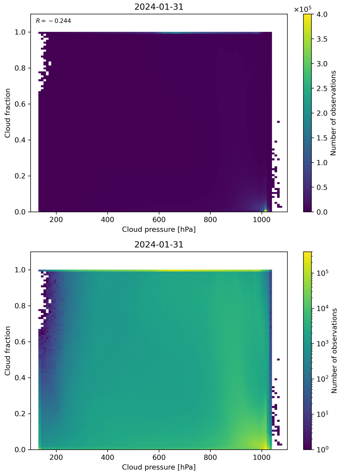
Figure 79: Scatter density plot of “Cloud pressure” against “Cloud fraction” for 2024-01-31 to 2024-02-01.
