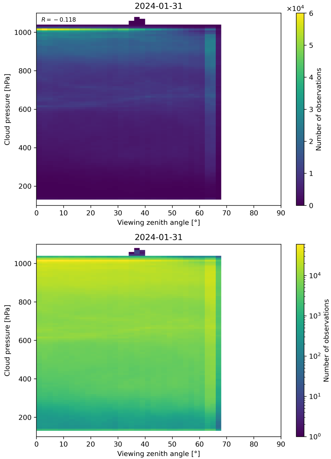
Figure 121: Scatter density plot of “Viewing zenith angle” against “Cloud pressure” for 2024-01-31 to 2024-02-01.
