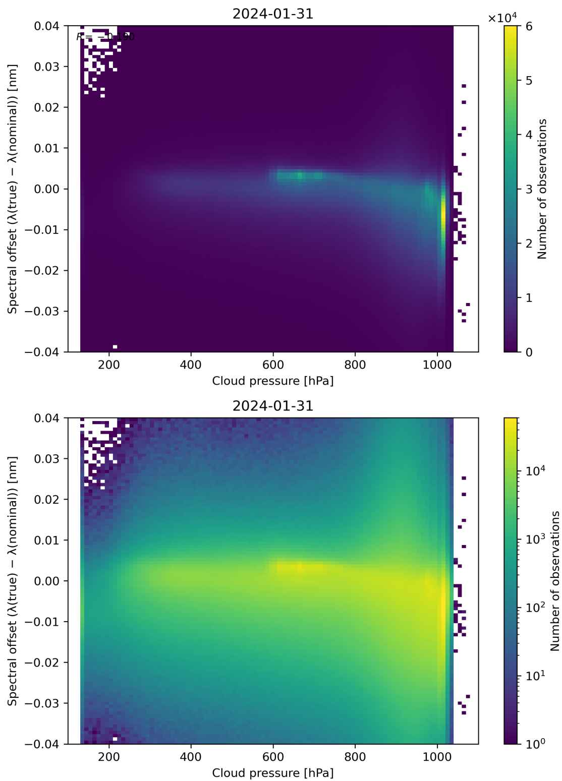
Figure 84: Scatter density plot of “Cloud pressure” against “Spectral offset ( \lambda(\text{true}) - \lambda(\text{nominal}) )” for 2024-01-31 to 2024-02-01.
