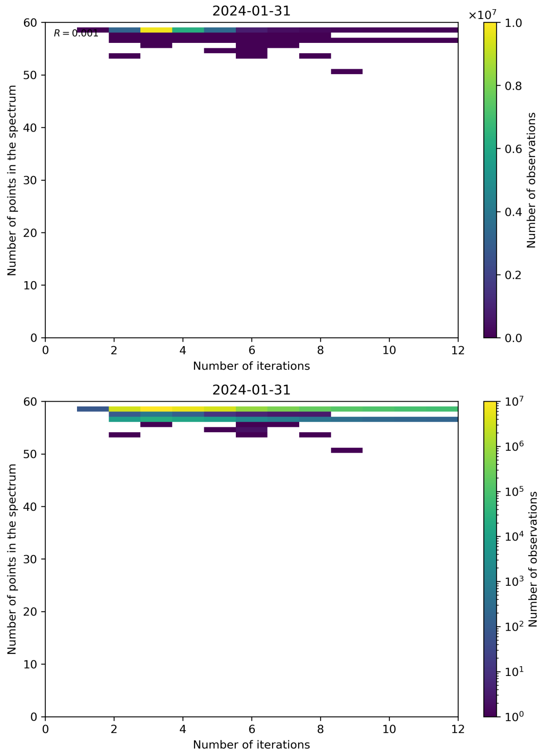
Figure 99: Scatter density plot of “Number of iterations” against “Number of points in the spectrum” for 2024-01-31 to 2024-02-01.
