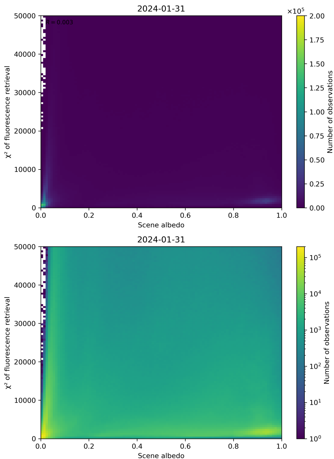
Figure 103: Scatter density plot of “Scene albedo” against “ \chi^2 of fluorescence retrieval” for 2024-01-31 to 2024-02-01.
