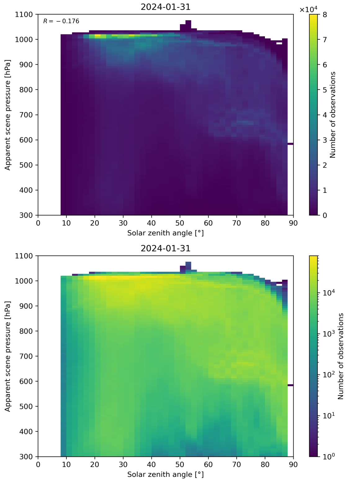
Figure 108: Scatter density plot of “Solar zenith angle” against “Apparent scene pressure” for 2024-01-31 to 2024-02-01.
