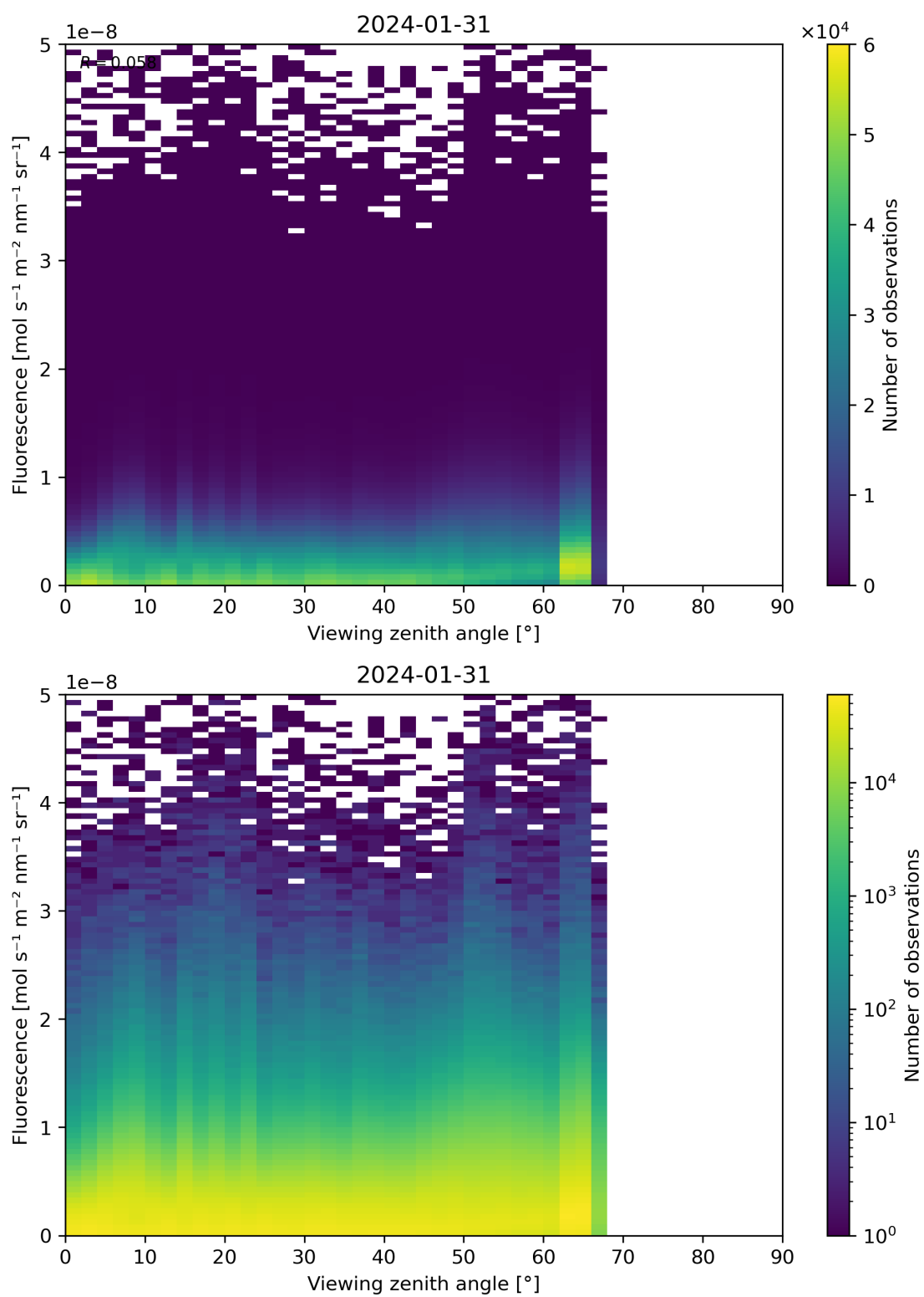
Figure 122: Scatter density plot of “Viewing zenith angle” against “Fluorescence” for 2024-01-31 to 2024-02-01.
