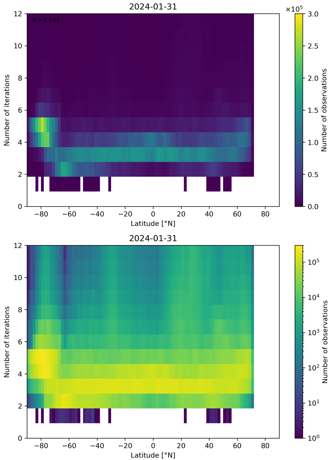
Figure 93: Scatter density plot of “Latitude” against “Number of iterations” for 2024-01-31 to 2024-02-01.
