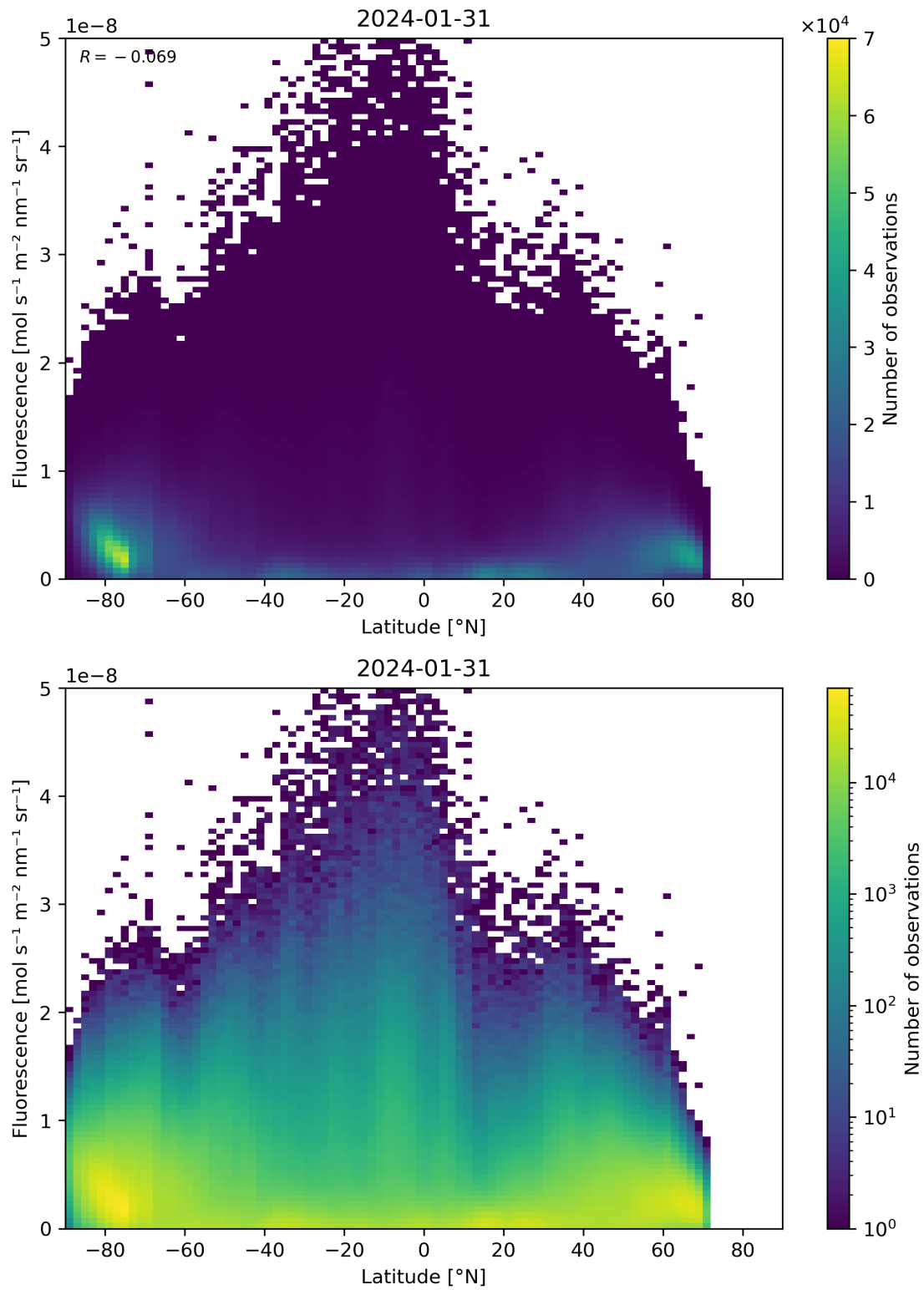
Figure 92: Scatter density plot of “Latitude” against “Fluorescence” for 2024-01-31 to 2024-02-01.
