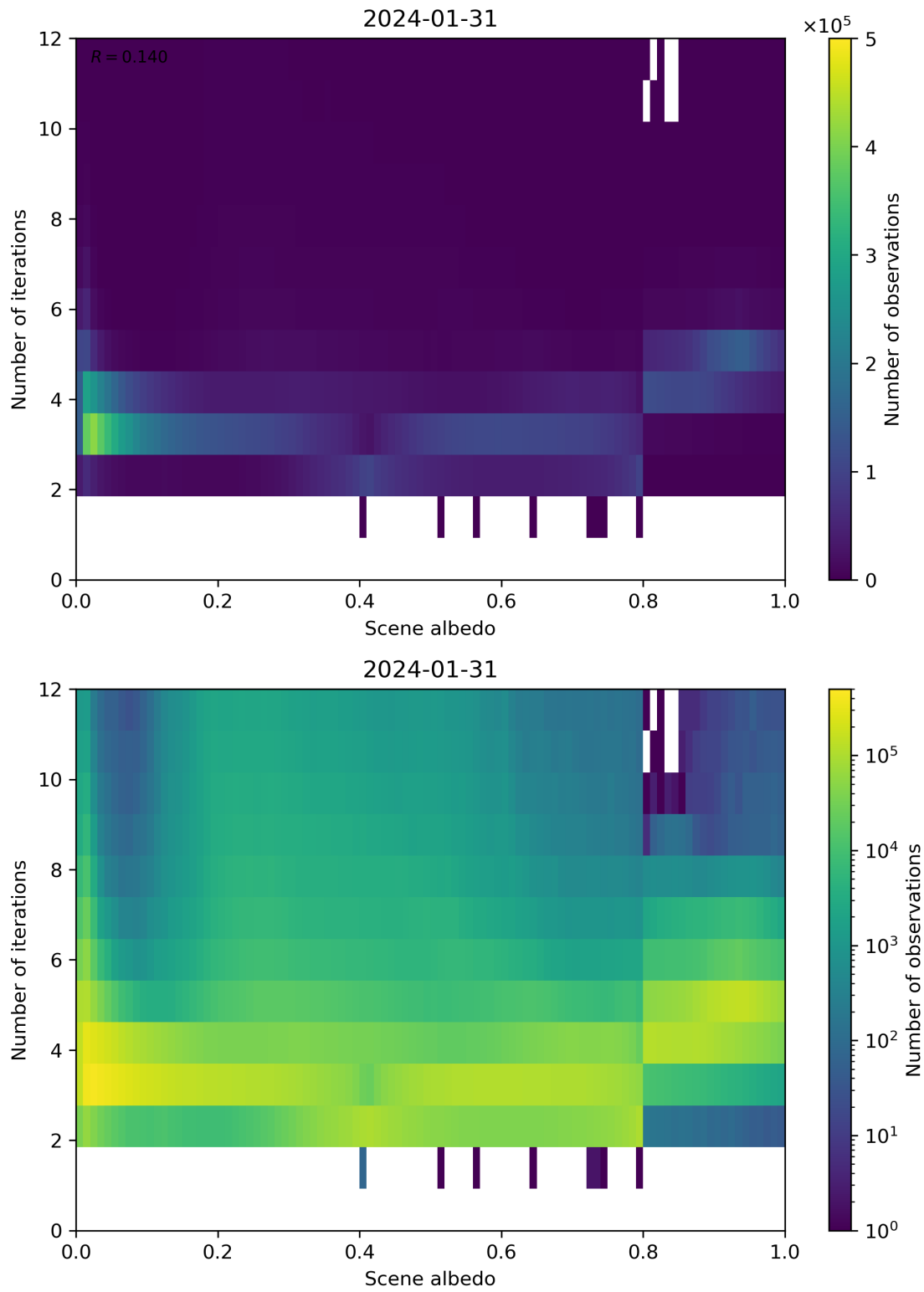
Figure 105: Scatter density plot of “Scene albedo” against “Number of iterations” for 2024-01-31 to 2024-02-01.
