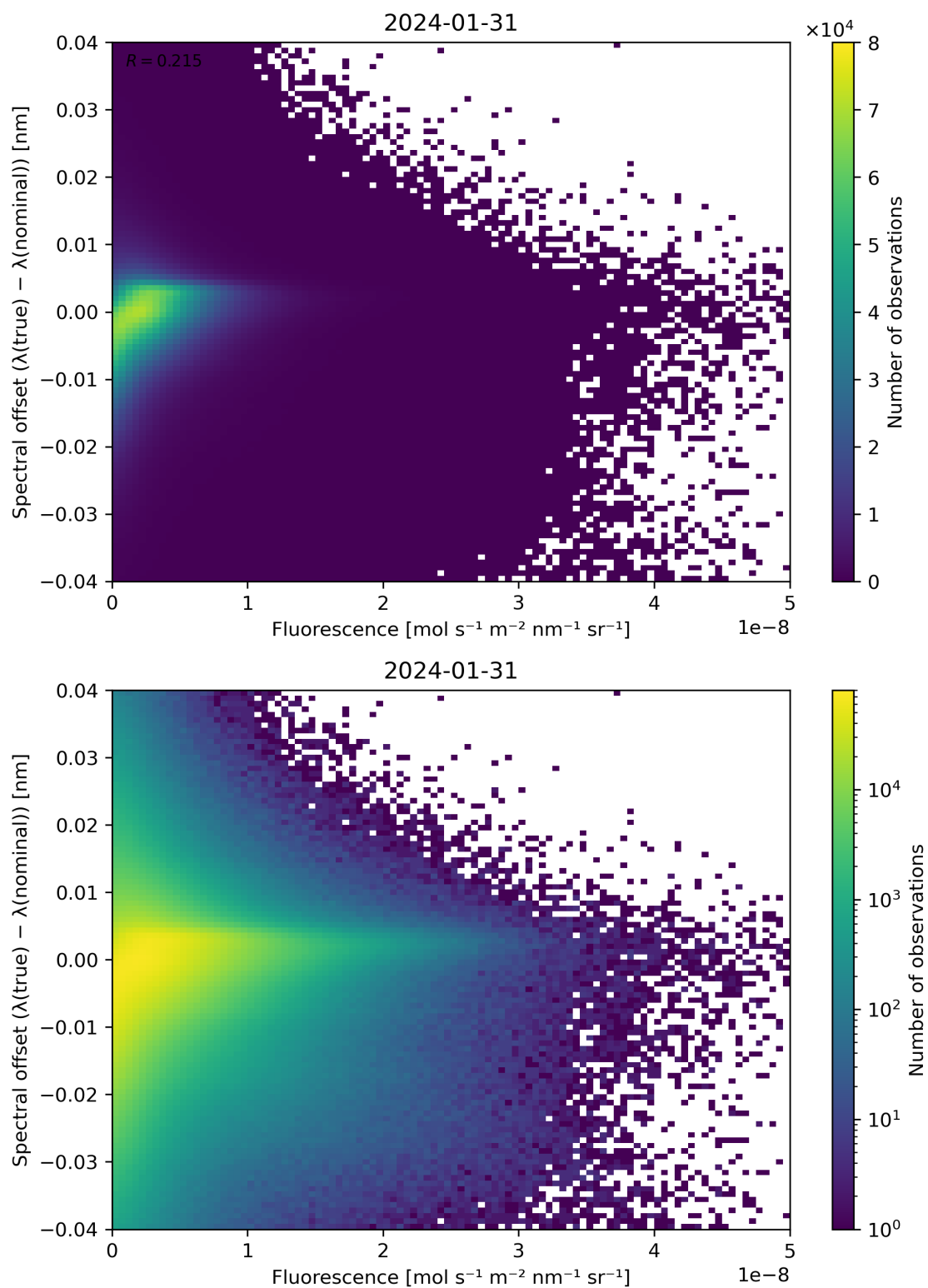
Figure 87: Scatter density plot of “Fluorescence” against “Spectral offset ( \lambda(\text{true}) - \lambda(\text{nominal}) )” for 2024-01-31 to 2024-02-01.
