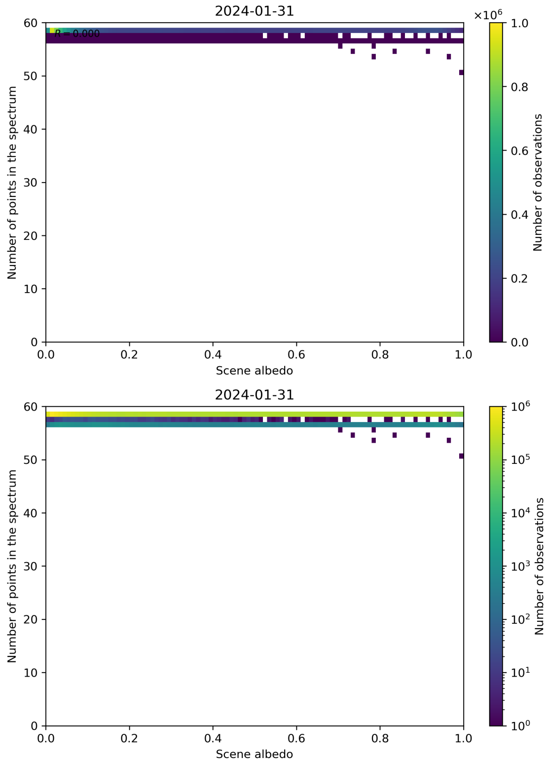
Figure 106: Scatter density plot of “Scene albedo” against “Number of points in the spectrum” for 2024-01-31 to 2024-02-01.
