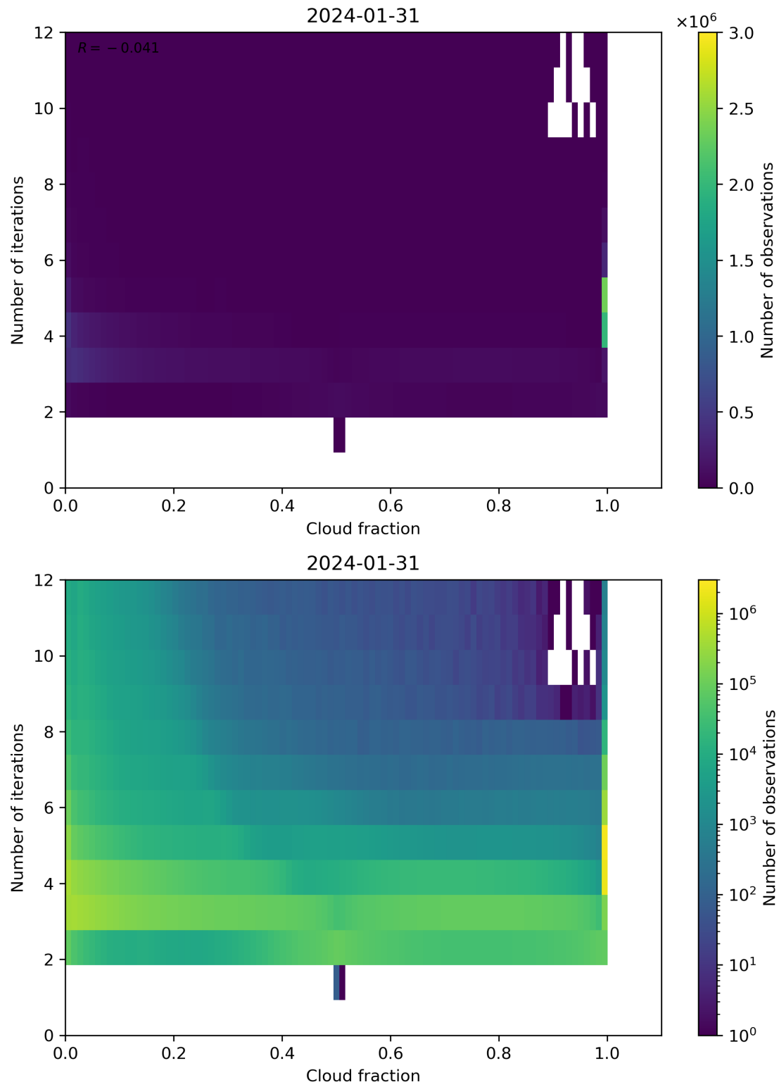
Figure 73: Scatter density plot of “Cloud fraction” against “Number of iterations” for 2024-01-31 to 2024-02-01.
