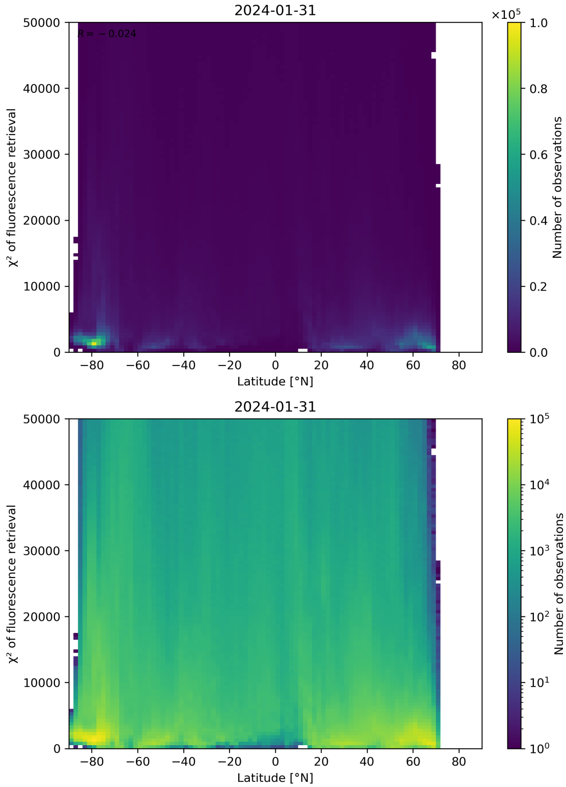
Figure 89: Scatter density plot of “Latitude” against “ \chi^2 of fluorescence retrieval” for 2024-01-31 to 2024-02-01.
