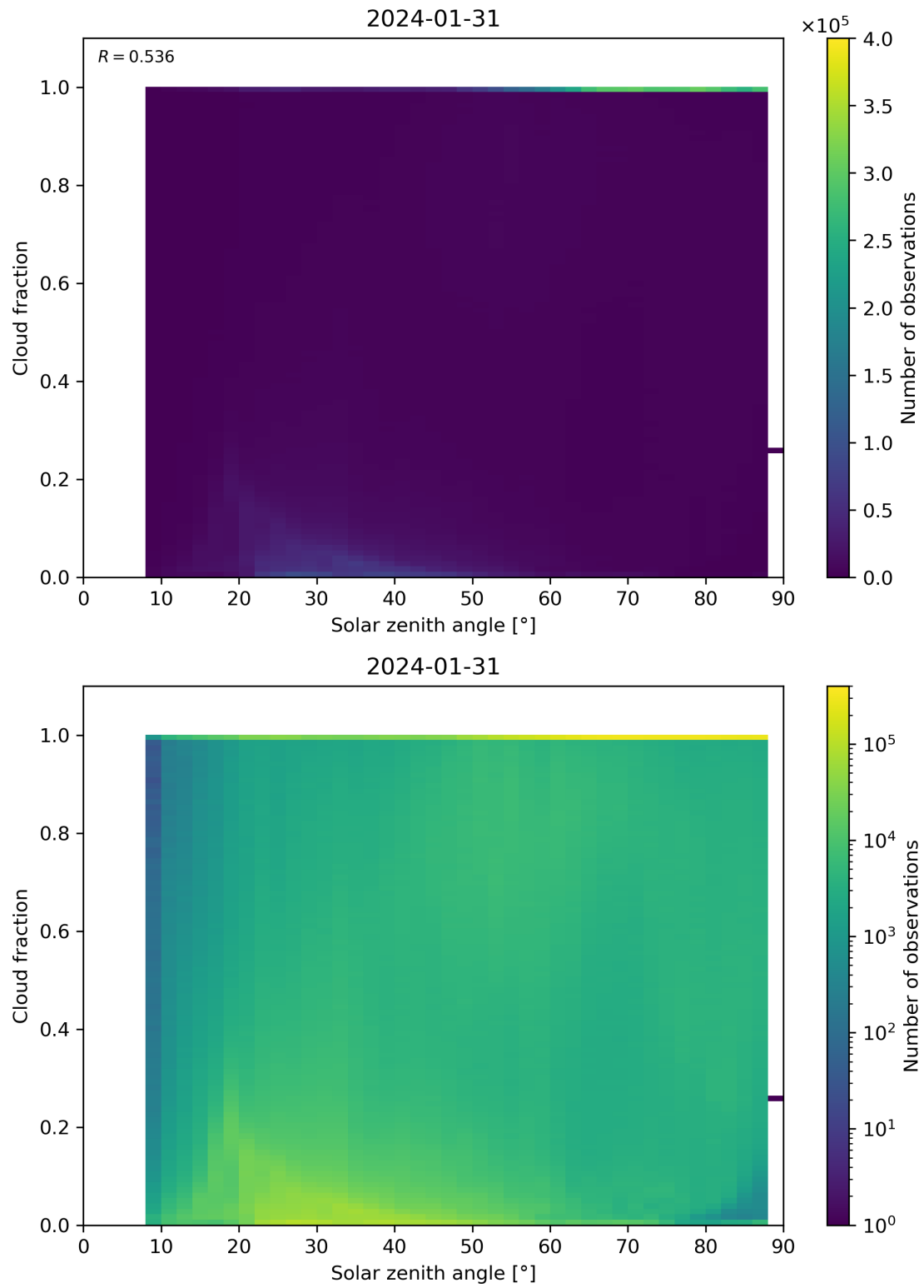
Figure 110: Scatter density plot of “Solar zenith angle” against “Cloud fraction” for 2024-01-31 to 2024-02-01.
