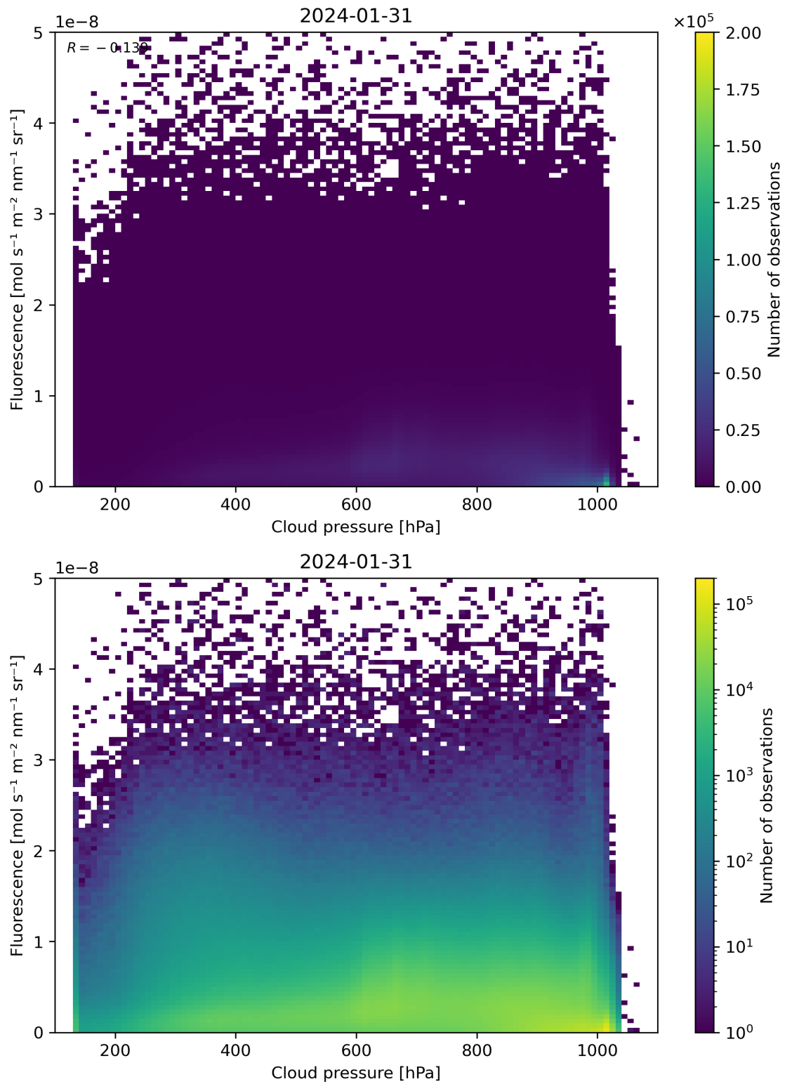
Figure 80: Scatter density plot of “Cloud pressure” against “Fluorescence” for 2024-01-31 to 2024-02-01.
