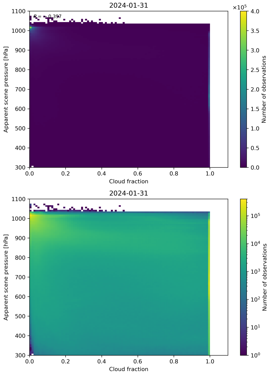
Figure 70: Scatter density plot of “Cloud fraction” against “Apparent scene pressure” for 2024-01-31 to 2024-02-01.
