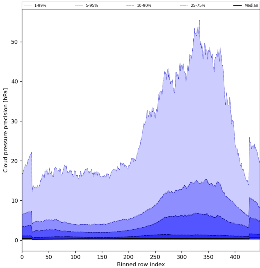
Figure 48: Along track statistics of “Cloud pressure precision” for 2024-01-31 to 2024-02-01
