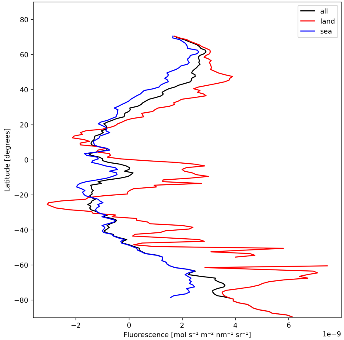
Figure 23: Zonal average of “Fluorescence” for 2024-01-31 to 2024-02-01.
