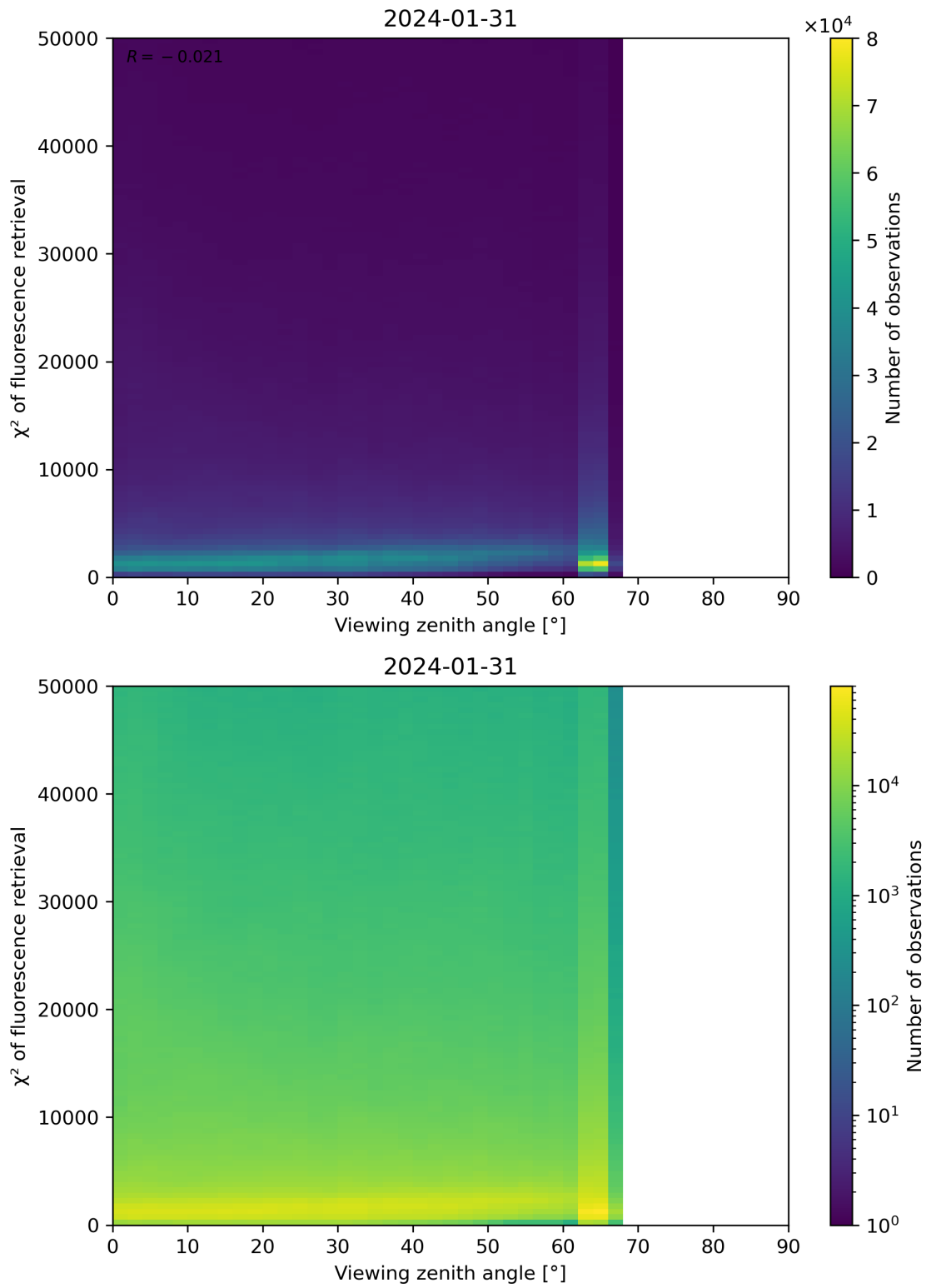
Figure 119: Scatter density plot of “Viewing zenith angle” against “ \chi^2 of fluorescence retrieval” for 2024-01-31 to 2024-02-01.
