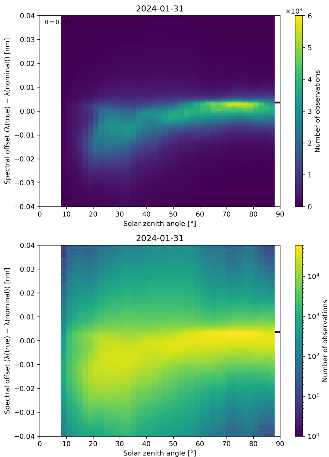
Figure 117: Scatter density plot of “Solar zenith angle” against “Spectral offset ( \lambda(\text{true}) - \lambda(\text{nominal}) )” for 2024-01-31 to 2024-02-01.
