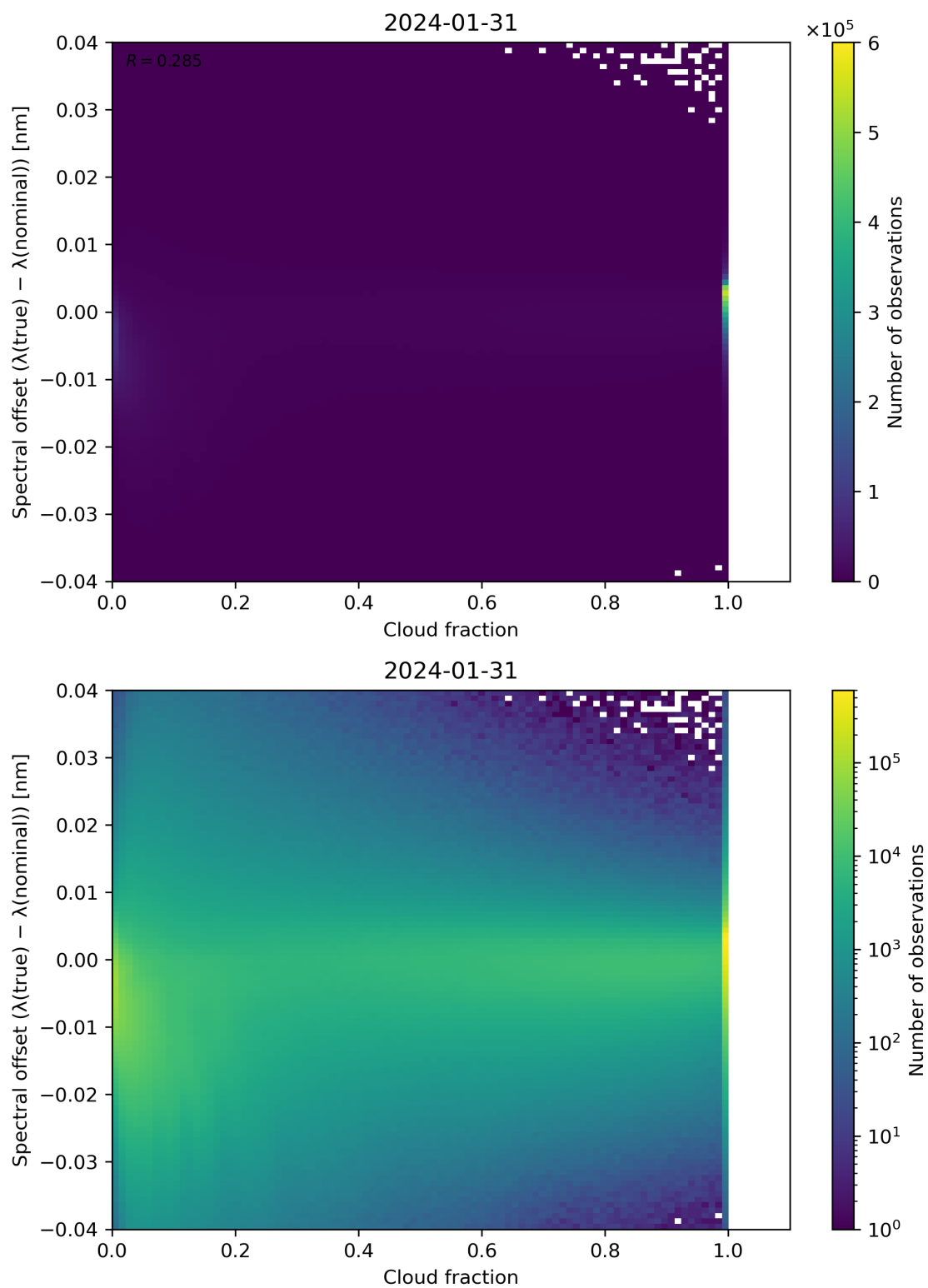
Figure 76: Scatter density plot of “Cloud fraction” against “Spectral offset ( \lambda(\text{true}) - \lambda(\text{nominal}) )” for 2024-01-31 to 2024-02-01.
