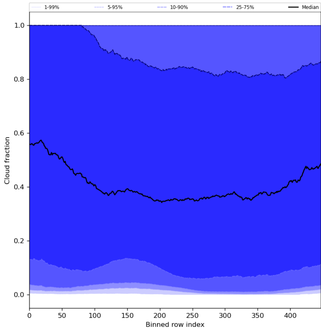
Figure 49: Along track statistics of “Cloud fraction” for 2024-01-31 to 2024-02-01
