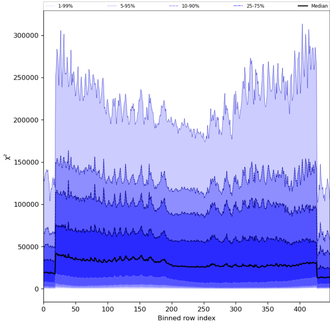
Figure 55: Along track statistics of “ \chi^2 ” for 2024-01-31 to 2024-02-01
