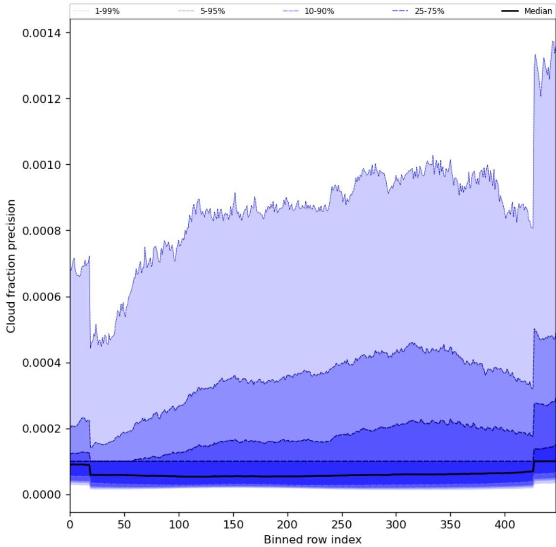
Figure 50: Along track statistics of “Cloud fraction precision” for 2024-01-31 to 2024-02-01
