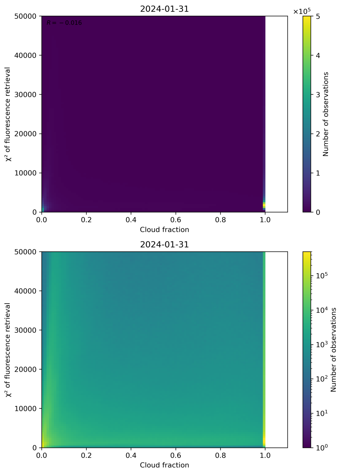
Figure 71: Scatter density plot of “Cloud fraction” against “ \chi^2 of fluorescence retrieval” for 2024-01-31 to 2024-02-01.
