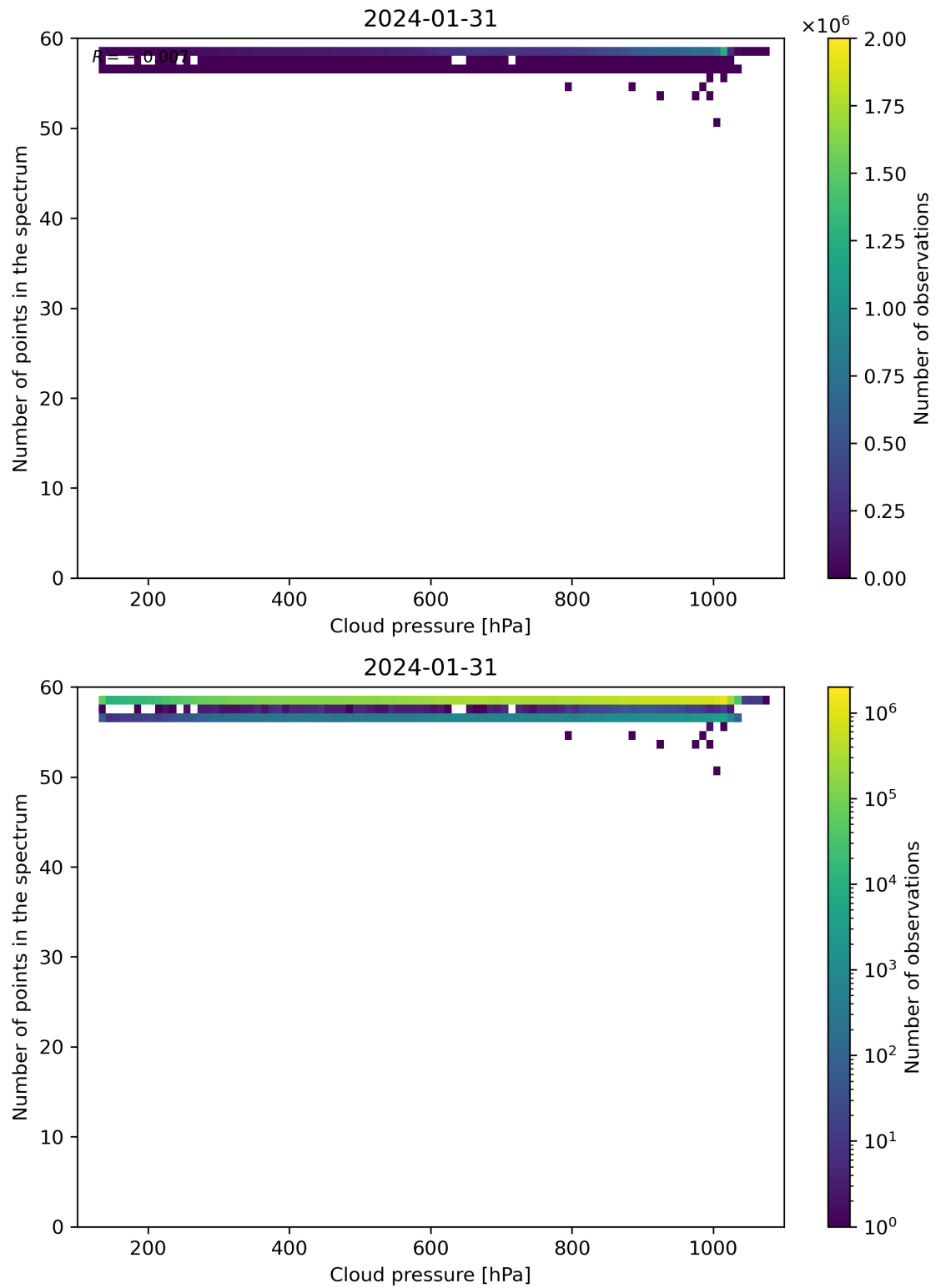
Figure 82: Scatter density plot of “Cloud pressure” against “Number of points in the spectrum” for 2024-01-31 to 2024-02-01.
