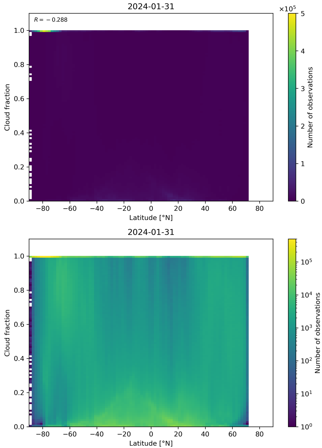
Figure 90: Scatter density plot of “Latitude” against “Cloud fraction” for 2024-01-31 to 2024-02-01.
