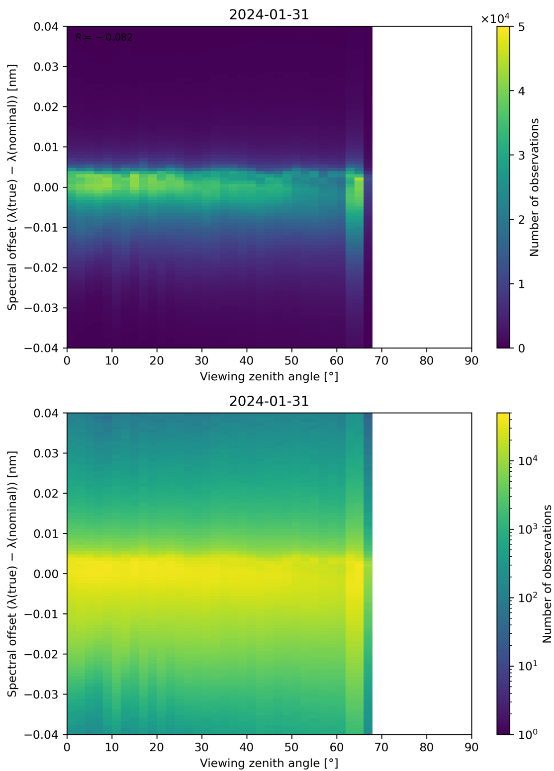
Figure 128: Scatter density plot of “Viewing zenith angle” against “Spectral offset ( \lambda(\text{true}) - \lambda(\text{nominal}) )” for 2024-01-31 to 2024-02-01.
