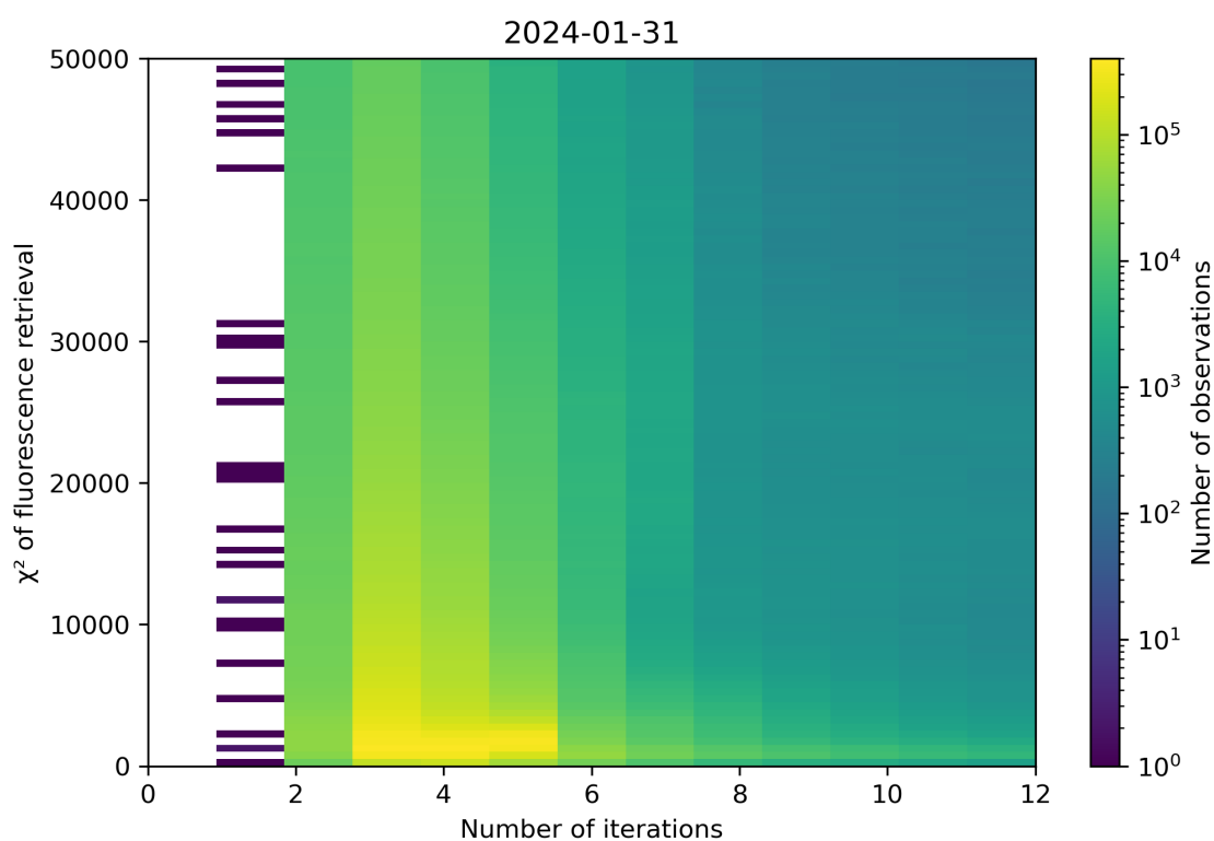
Figure 97: Scatter density plot of “Number of iterations” against “ \chi^2 of fluorescence retrieval” for 2024-01-31 to 2024-02-01.
