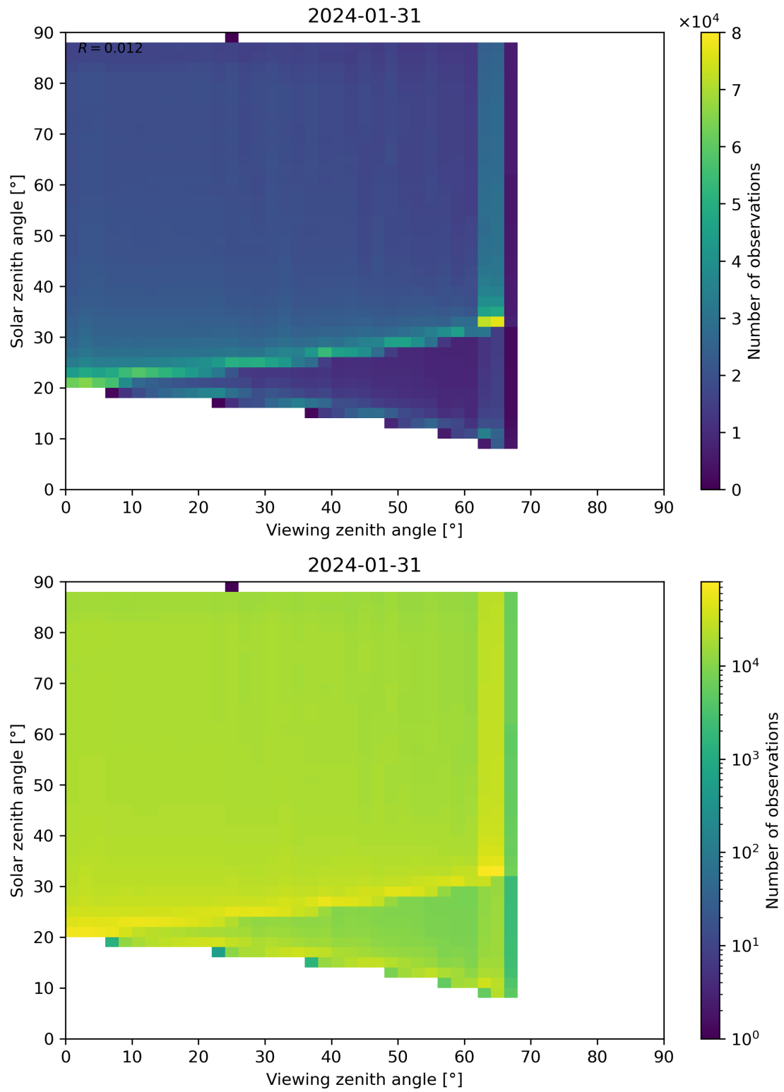
Figure 127: Scatter density plot of “Viewing zenith angle” against “Solar zenith angle” for 2024-01-31 to 2024-02-01.
