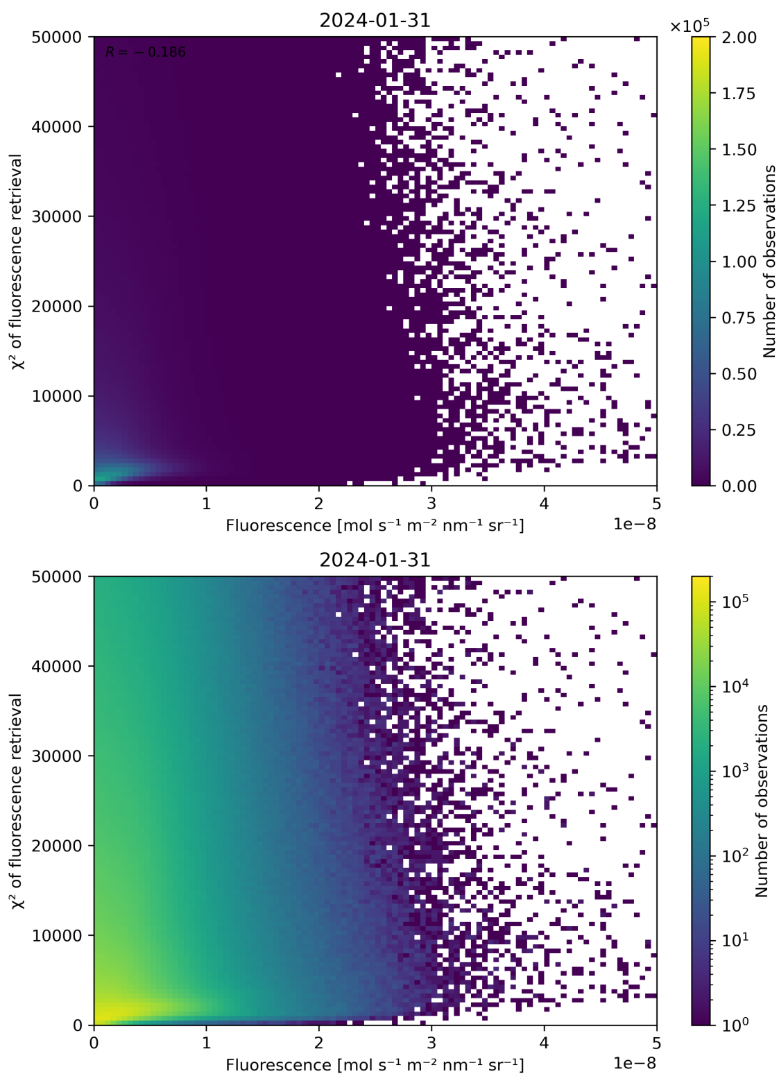
Figure 85: Scatter density plot of “Fluorescence” against “ \chi^2 of fluorescence retrieval” for 2024-01-31 to 2024-02-01.
