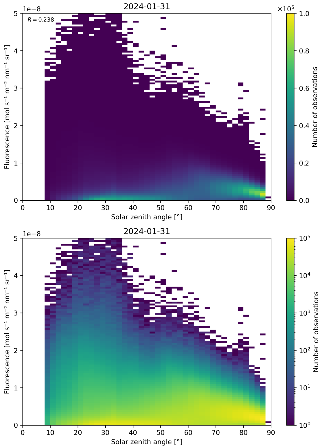
Figure 112: Scatter density plot of “Solar zenith angle” against “Fluorescence” for 2024-01-31 to 2024-02-01.
