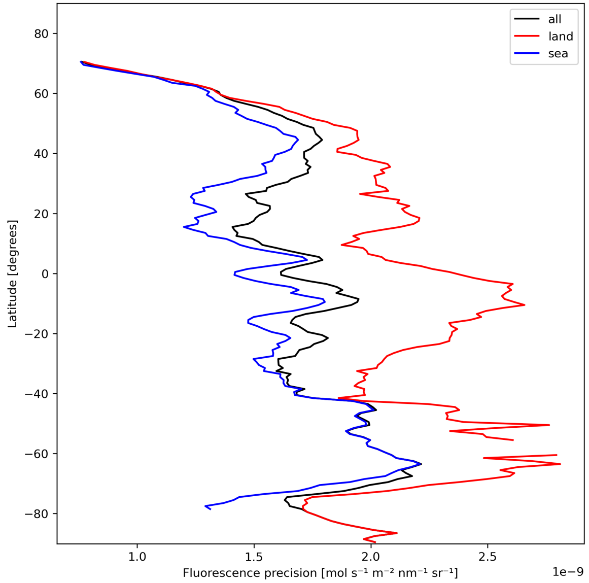
Figure 24: Zonal average of “Fluorescence precision” for 2024-01-31 to 2024-02-01.
