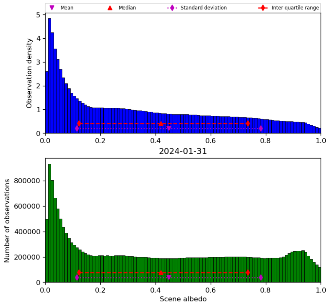
Figure 34: Histogram of “Scene albedo” for 2024-01-31 to 2024-02-01
