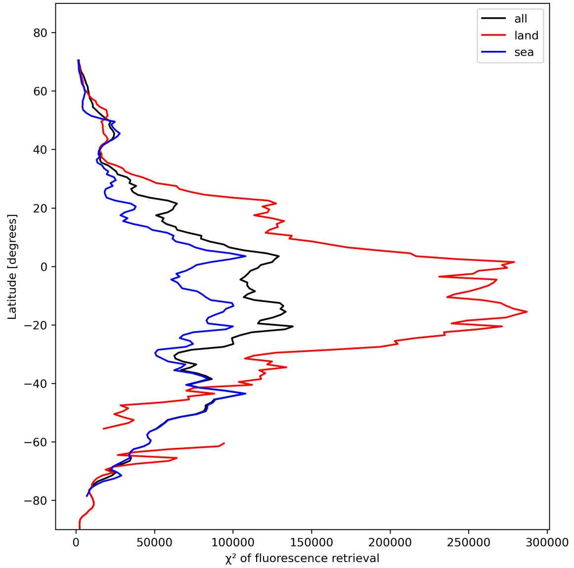
Figure 25: Zonal average of “ \chi^2 of fluorescence retrieval” for 2024-01-31 to 2024-02-01.
