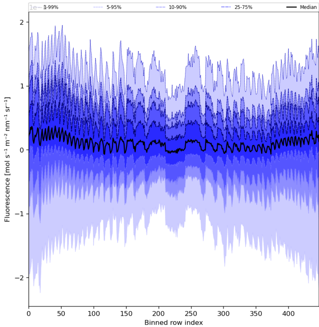
Figure 57: Along track statistics of “Fluorescence” for 2024-01-31 to 2024-02-01
