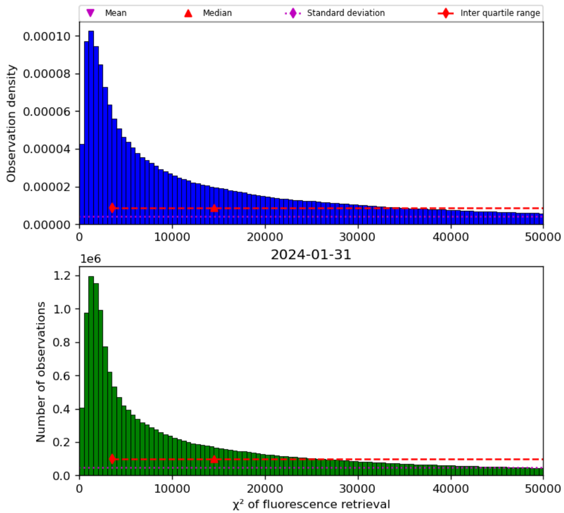
Figure 42: Histogram of “ \chi^2 of fluorescence retrieval” for 2024-01-31 to 2024-02-01
