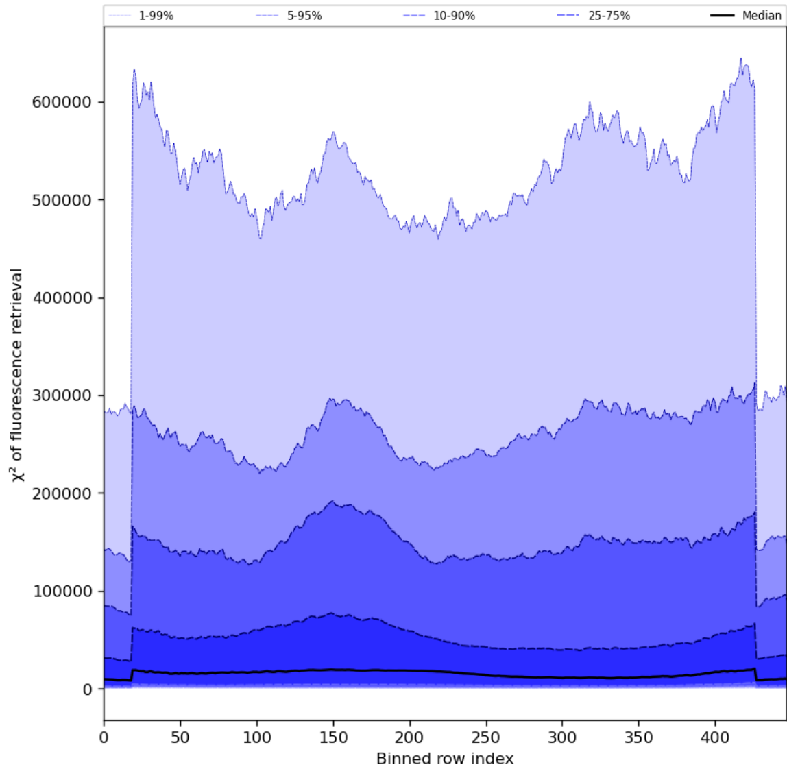
Figure 59: Along track statistics of “ \chi^2 of fluorescence retrieval” for 2024-01-31 to 2024-02-01
