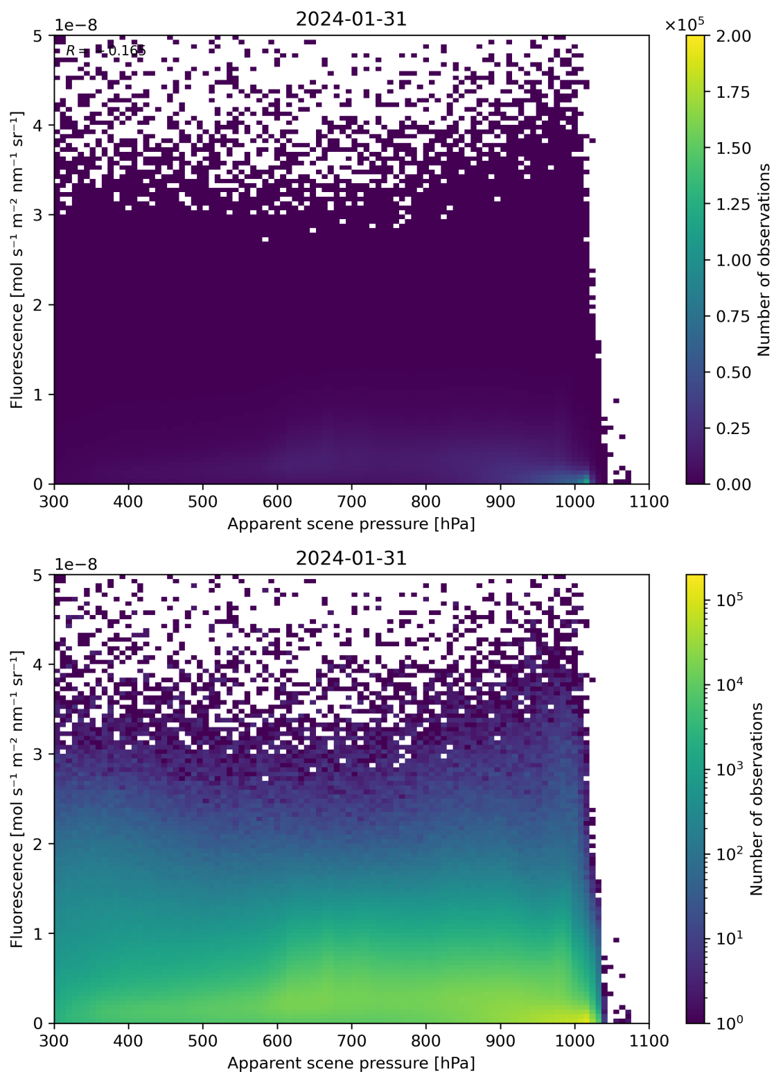
Figure 64: Scatter density plot of “Apparent scene pressure” against “Fluorescence” for 2024-01-31 to 2024-02-01.
