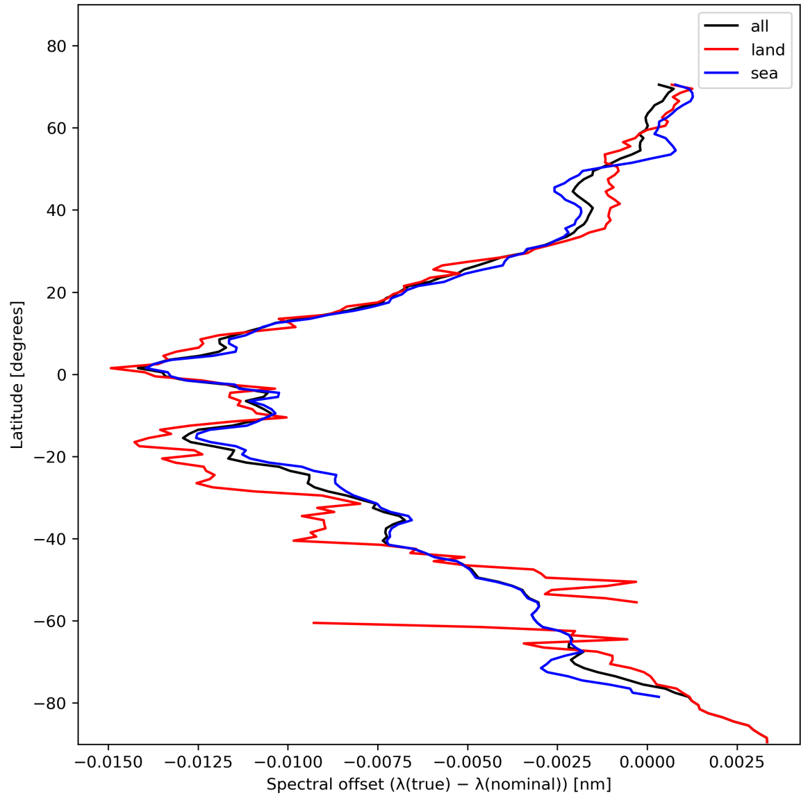
Figure 28: Zonal average of “Spectral offset ( \lambda(\text{true}) - \lambda(\text{nominal}) )” for 2024-01-31 to 2024-02-01.
