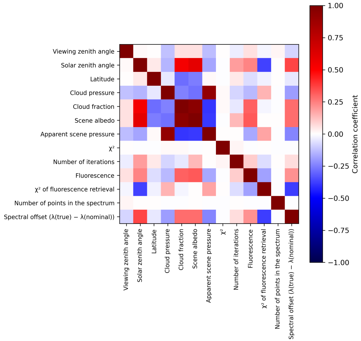
Figure 2: Map of correlation matrix for 2024-01-31 to 2024-02-01.
