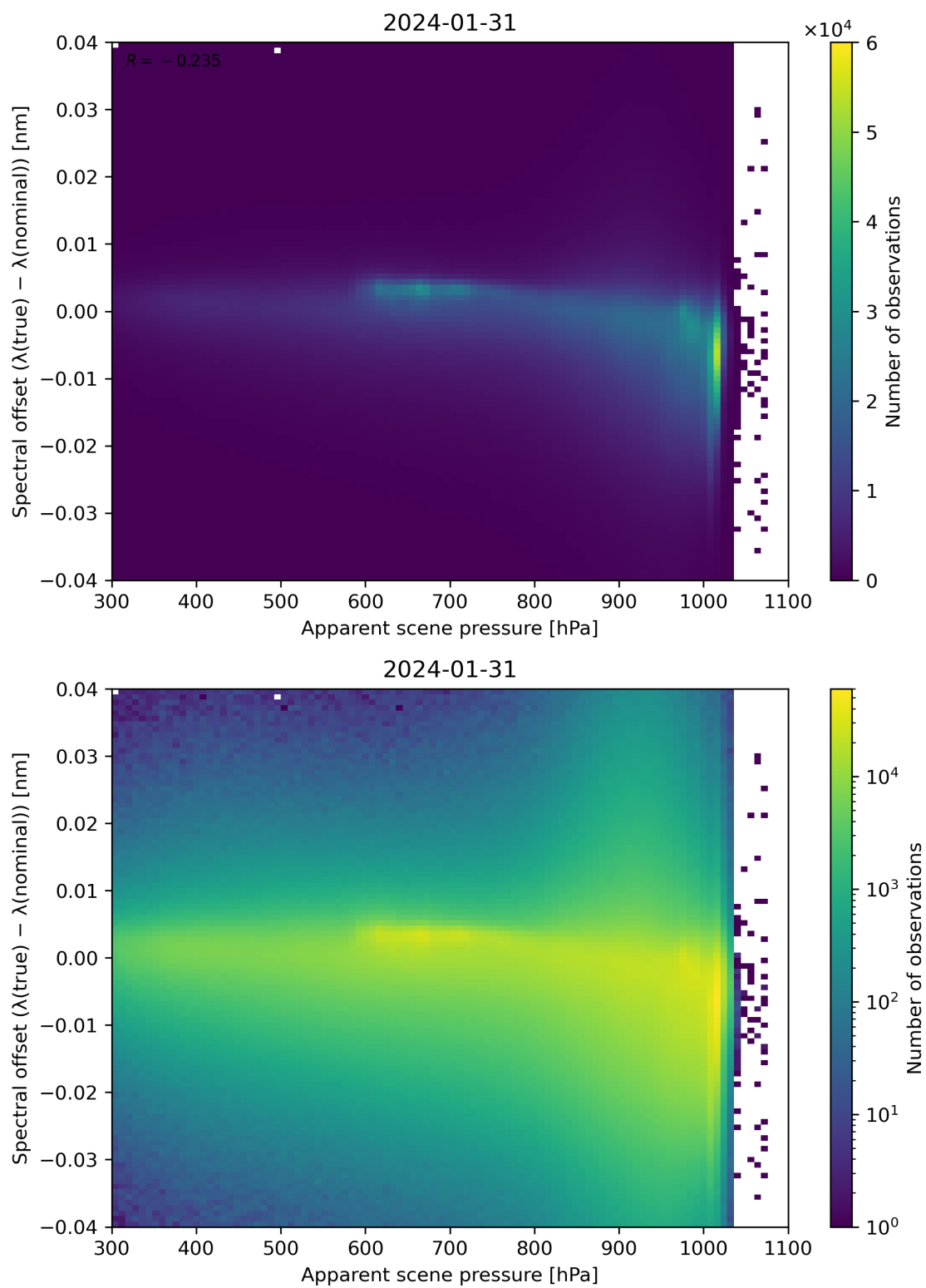
Figure 67: Scatter density plot of “Apparent scene pressure” against “Spectral offset ( \lambda(\text{true}) - \lambda(\text{nominal}) )” for 2024-01-31 to 2024-02-01.
