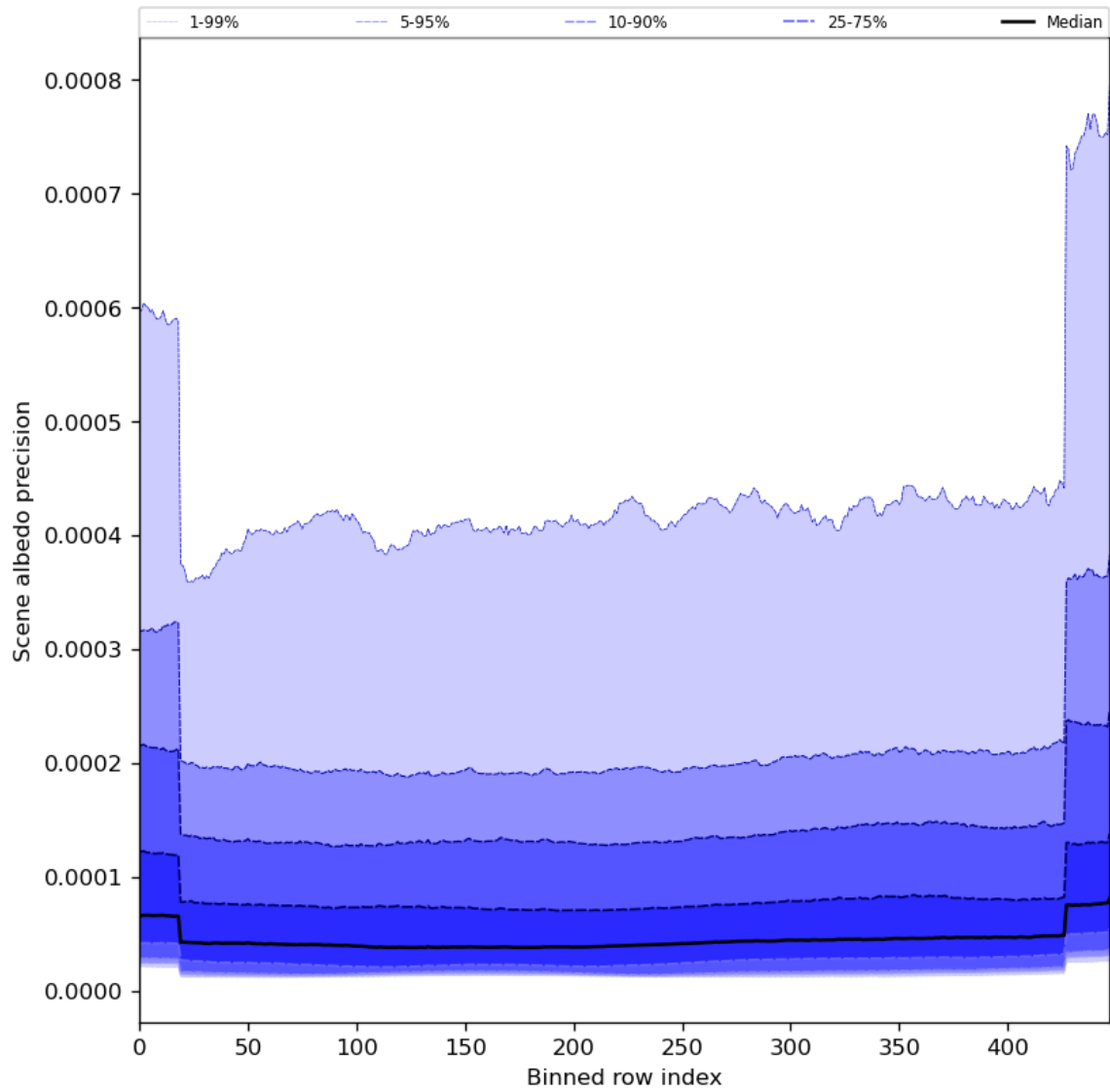
Figure 52: Along track statistics of “Scene albedo precision” for 2024-01-31 to 2024-02-01
