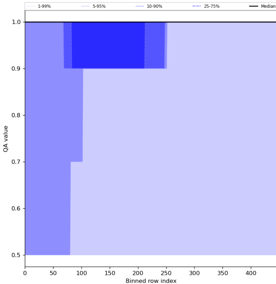
Figure 46: Along track statistics of “QA value” for 2024-01-31 to 2024-02-01
