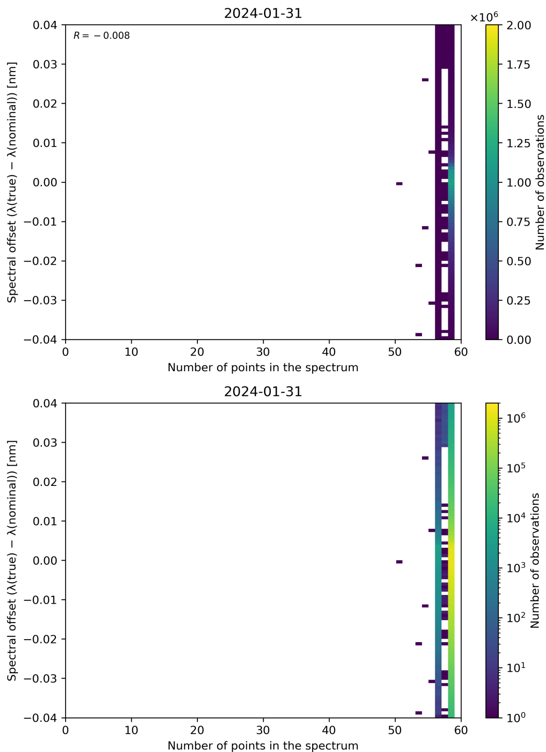
Figure 101: Scatter density plot of “Number of points in the spectrum” against “Spectral offset ( \lambda(\text{true}) - \lambda(\text{nominal}) )” for 2024-01-31 to 2024-02-01.
