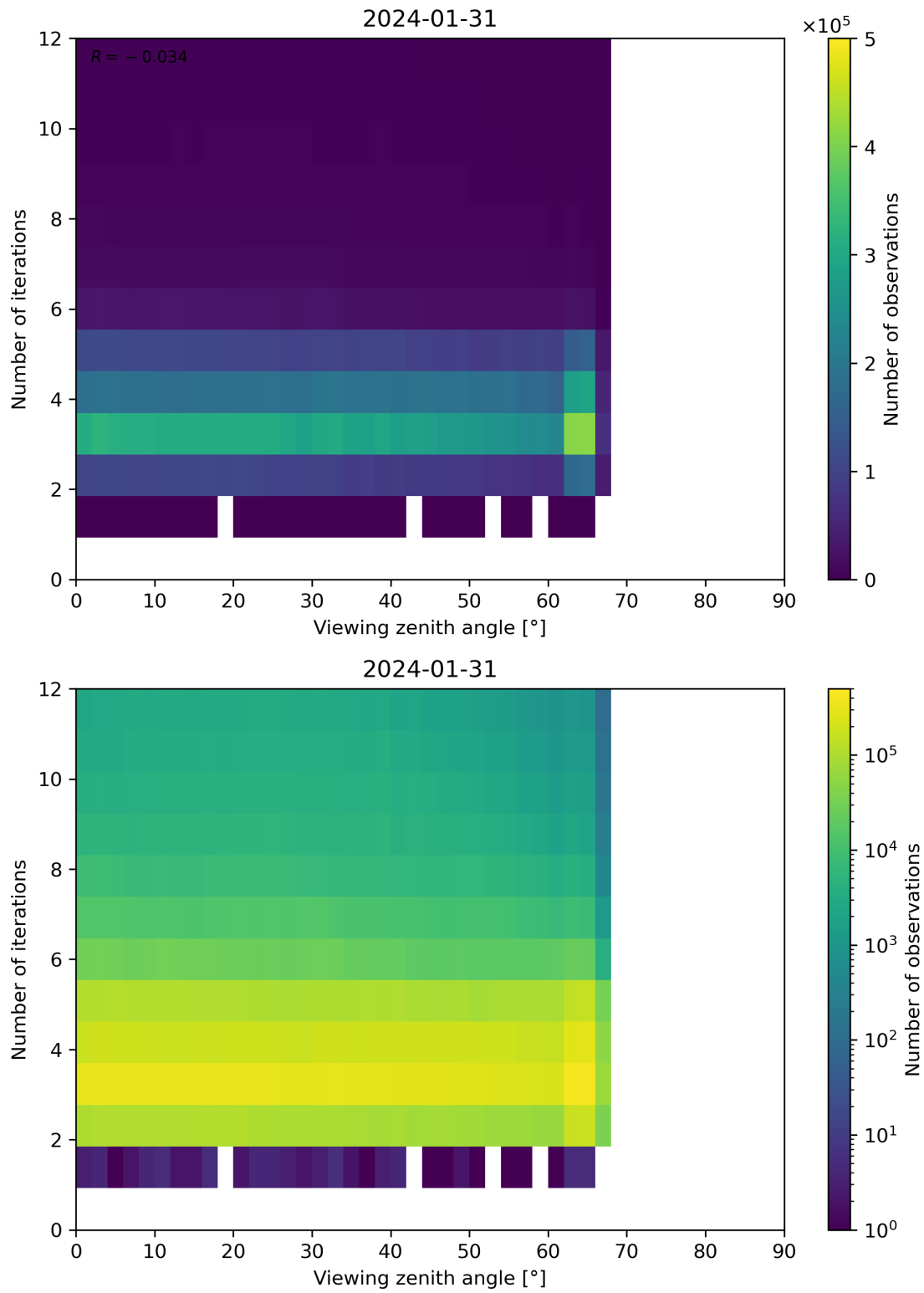
Figure 124: Scatter density plot of “Viewing zenith angle” against “Number of iterations” for 2024-01-31 to 2024-02-01.
