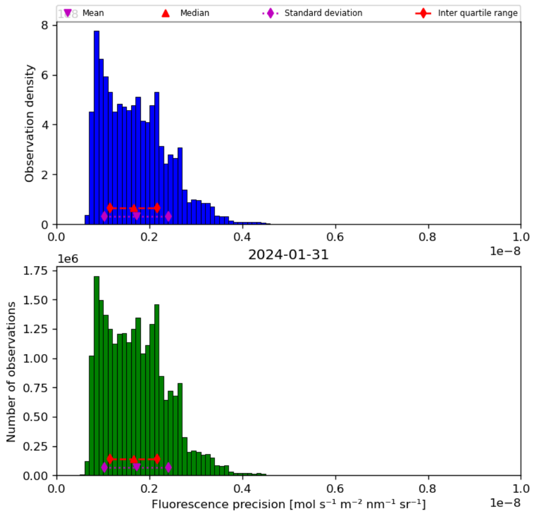
Figure 41: Histogram of “Fluorescence precision” for 2024-01-31 to 2024-02-01
