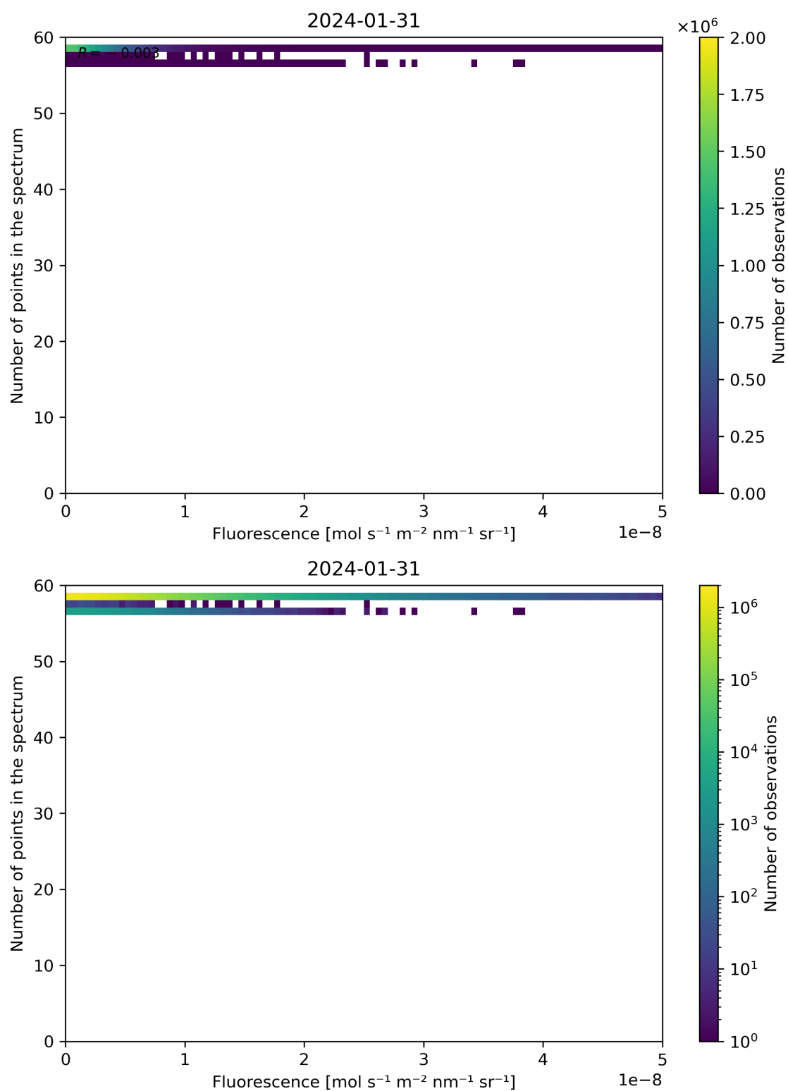
Figure 86: Scatter density plot of “Fluorescence” against “Number of points in the spectrum” for 2024-01-31 to 2024-02-01.
