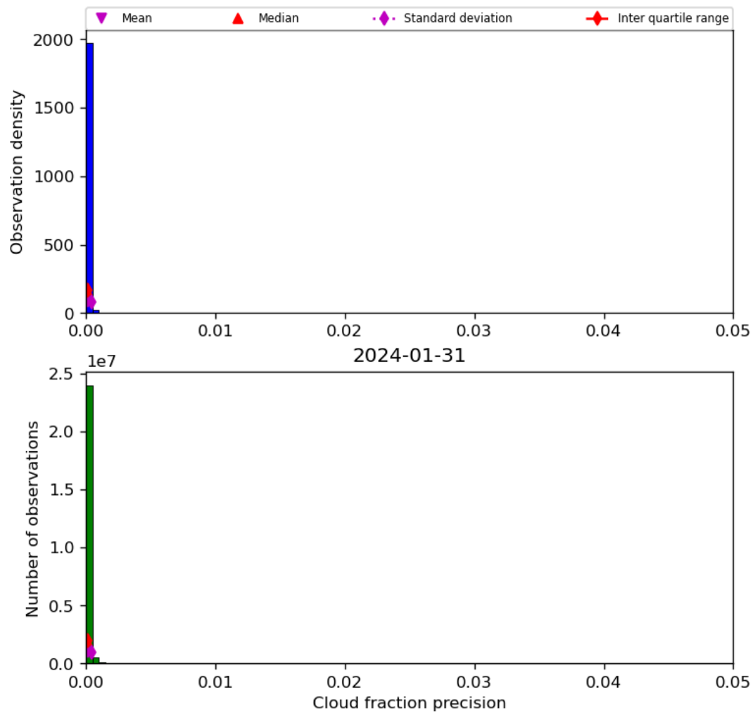
Figure 33: Histogram of “Cloud fraction precision” for 2024-01-31 to 2024-02-01
