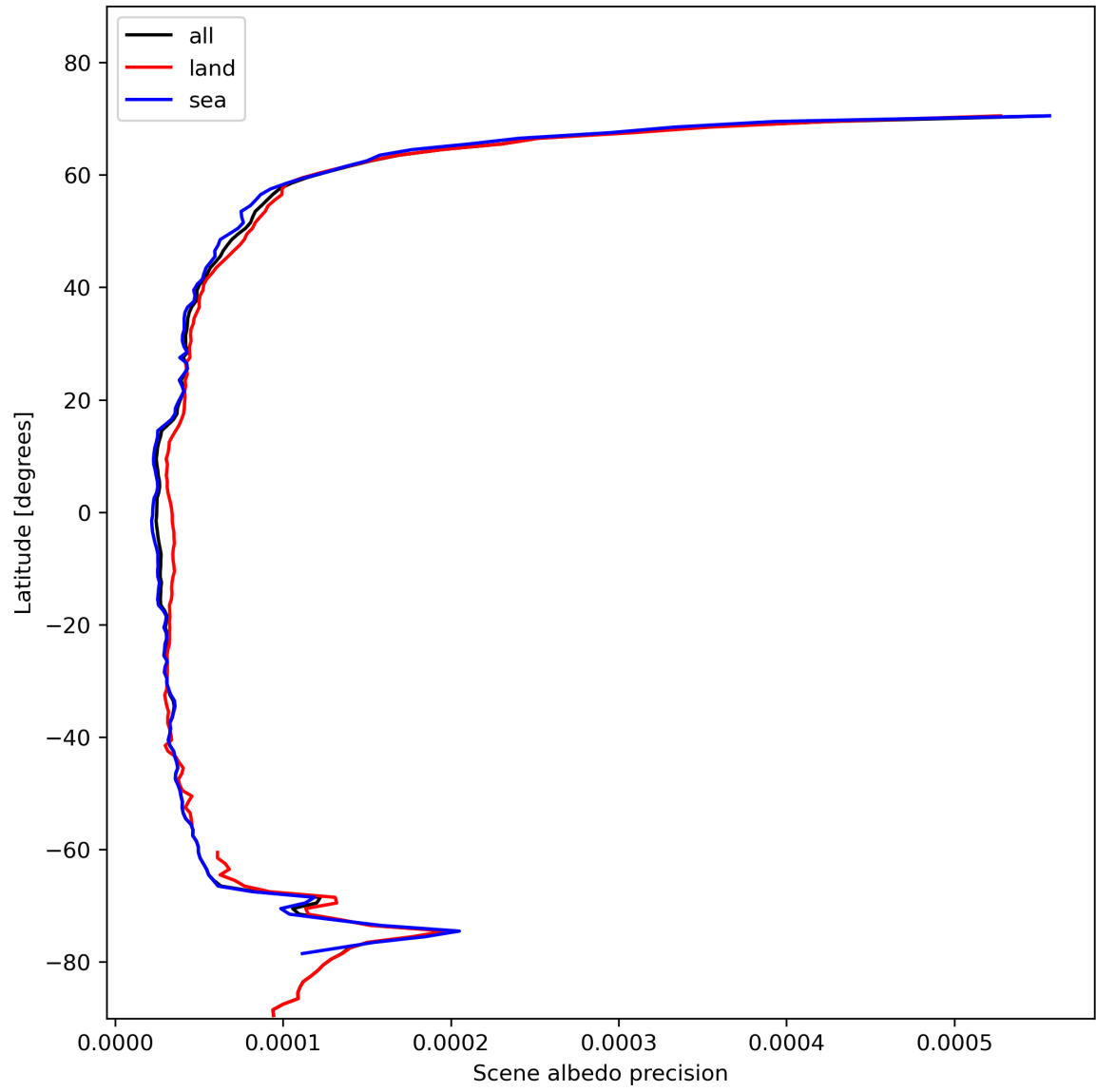
Figure 18: Zonal average of “Scene albedo precision” for 2024-01-31 to 2024-02-01.
