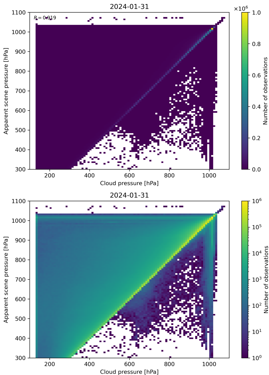
Figure 77: Scatter density plot of “Cloud pressure” against “Apparent scene pressure” for 2024-01-31 to 2024-02-01.
