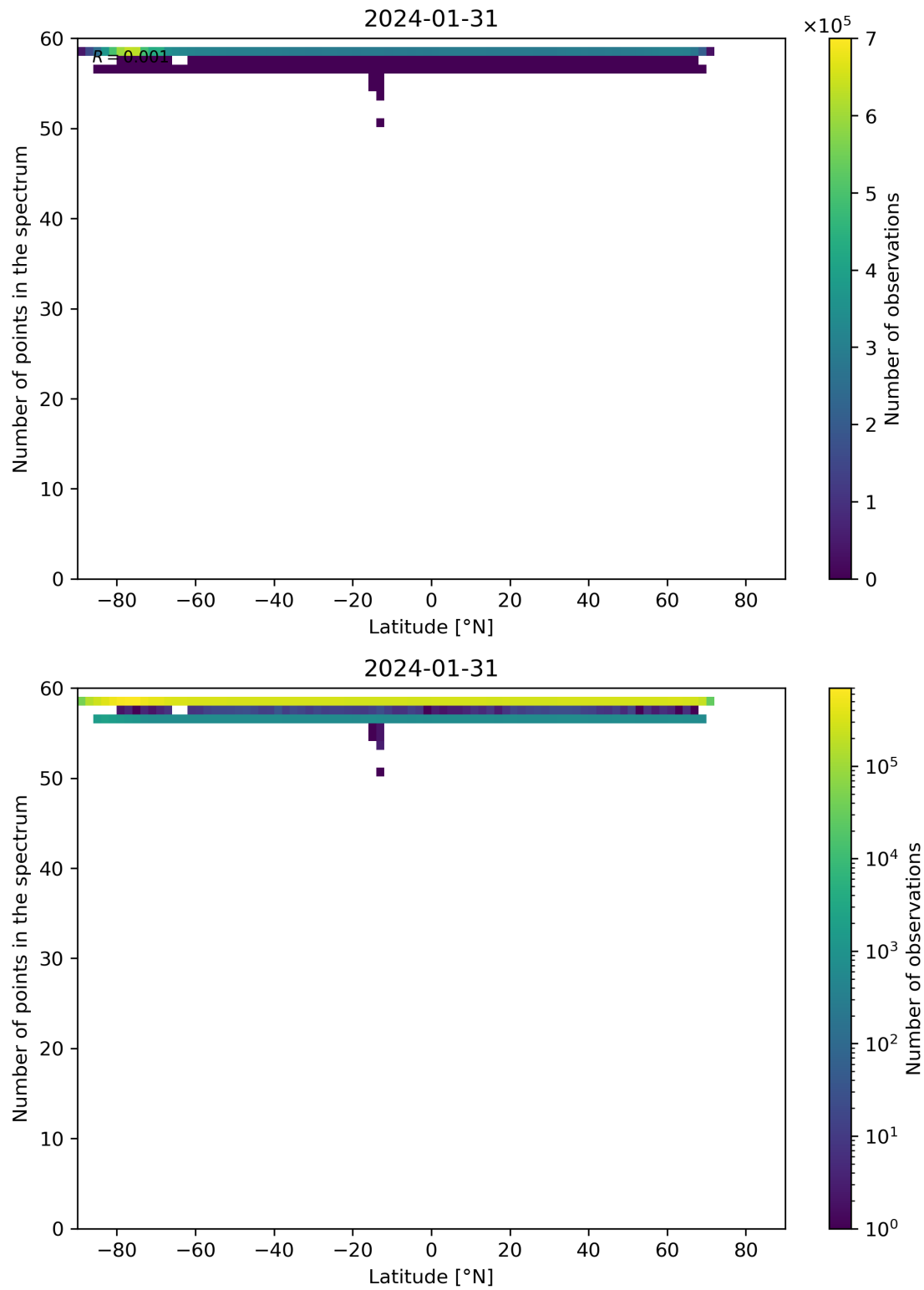
Figure 94: Scatter density plot of “Latitude” against “Number of points in the spectrum” for 2024-01-31 to 2024-02-01.
