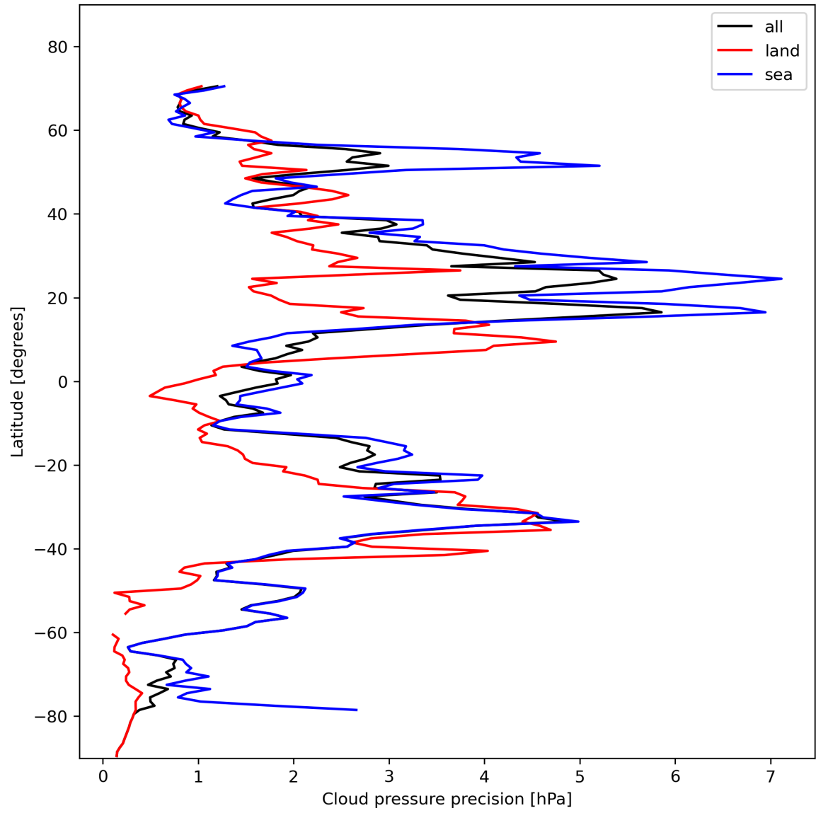
Figure 14: Zonal average of “Cloud pressure precision” for 2024-01-31 to 2024-02-01.
