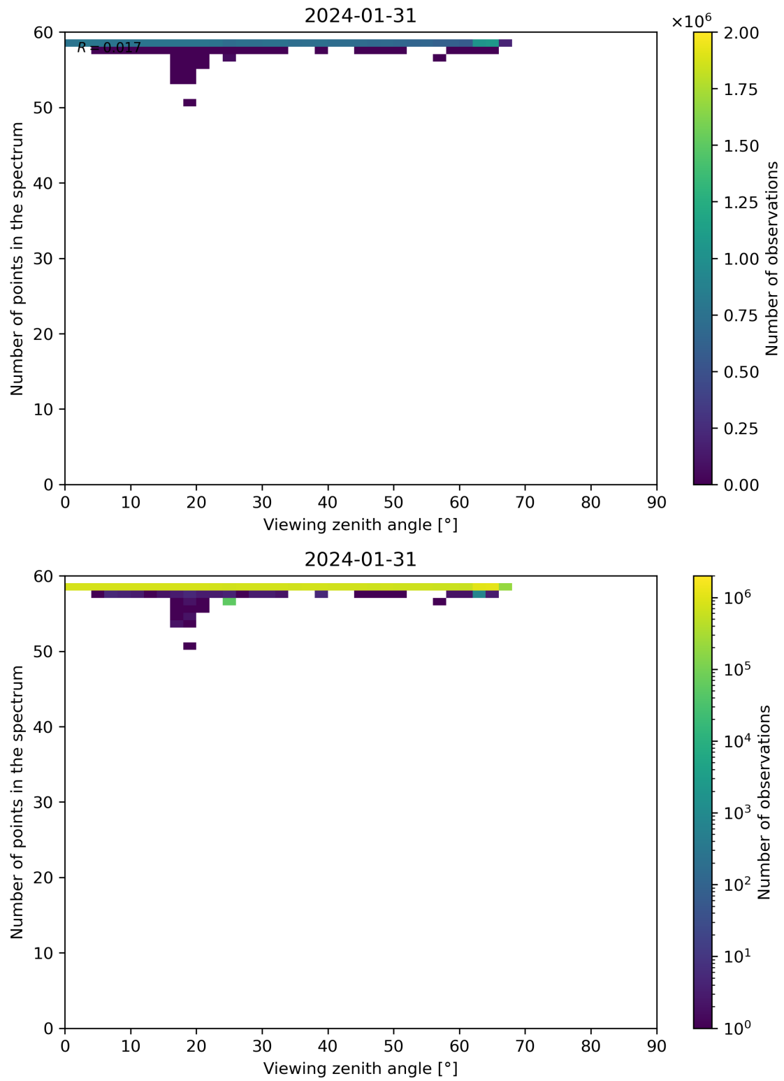
Figure 125: Scatter density plot of “Viewing zenith angle” against “Number of points in the spectrum” for 2024-01-31 to 2024-02-01.
