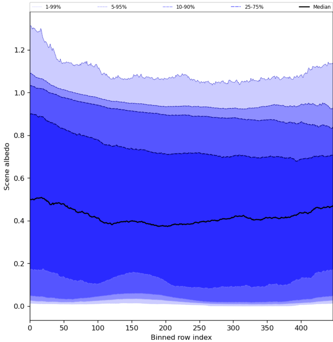
Figure 51: Along track statistics of “Scene albedo” for 2024-01-31 to 2024-02-01
