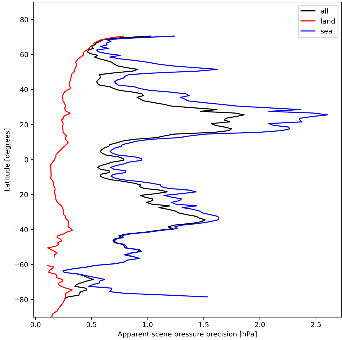
Figure 20: Zonal average of “Apparent scene pressure precision” for 2024-01-31 to 2024-02-01.
