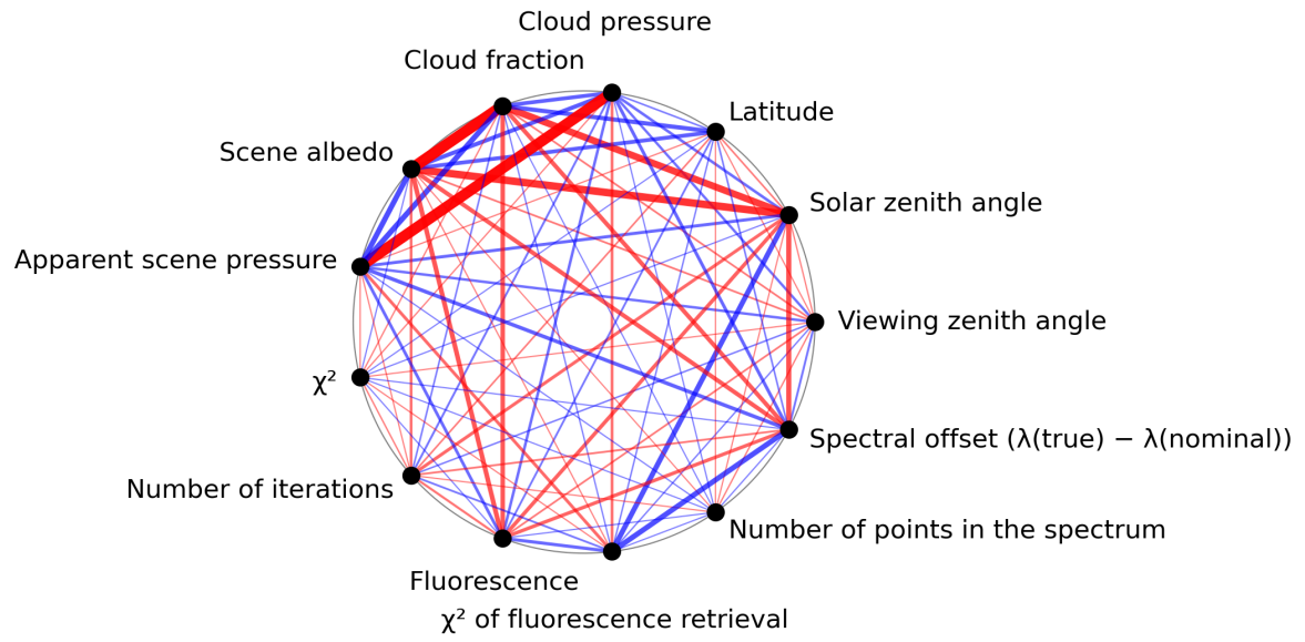
Figure 1: Map of correlation graph for 2024-01-31 to 2024-02-01.
