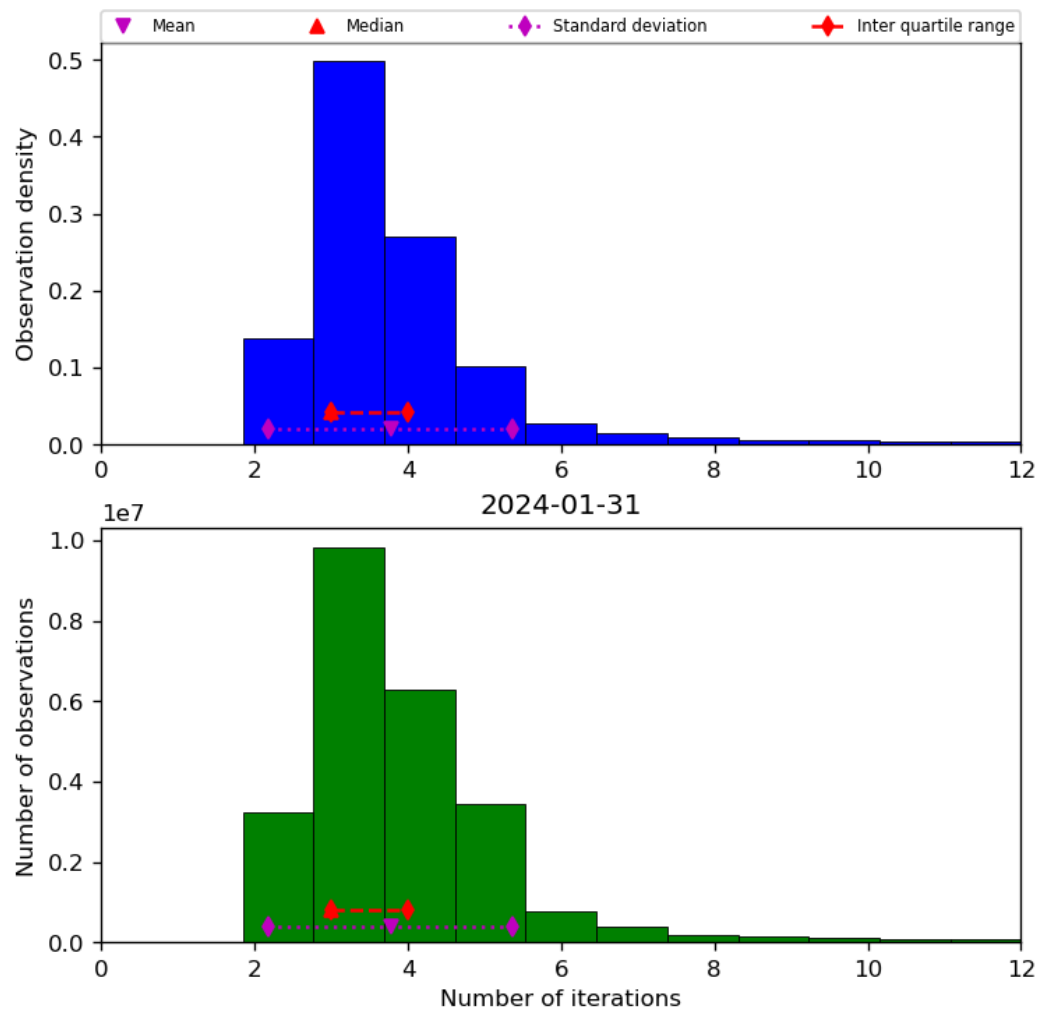
Figure 39: Histogram of “Number of iterations” for 2024-01-31 to 2024-02-01
