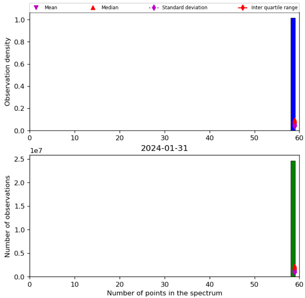
Figure 44: Histogram of “Number of points in the spectrum” for 2024-01-31 to 2024-02-01
