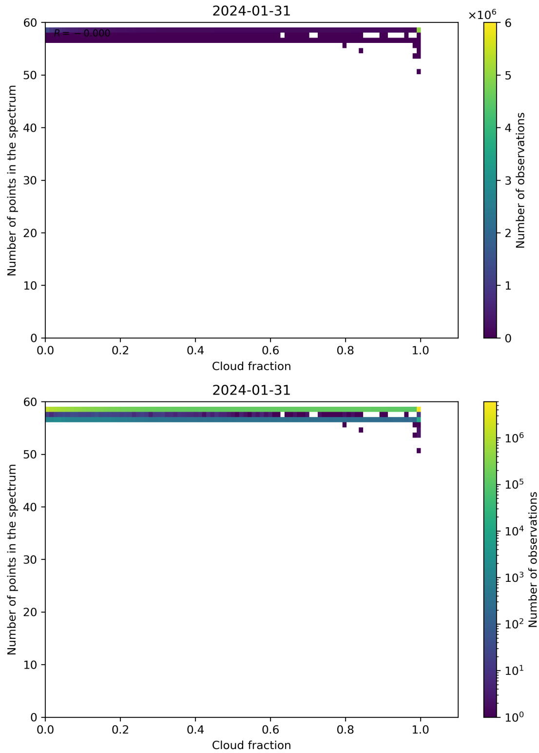
Figure 74: Scatter density plot of “Cloud fraction” against “Number of points in the spectrum” for 2024-01-31 to 2024-02-01.
