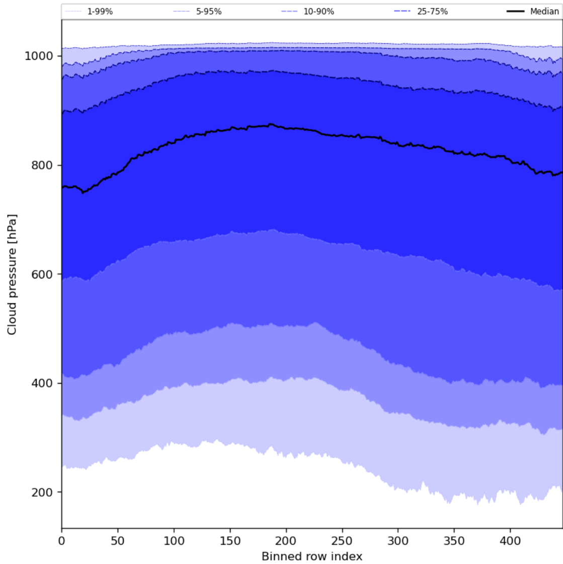
Figure 47: Along track statistics of “Cloud pressure” for 2024-01-31 to 2024-02-01
