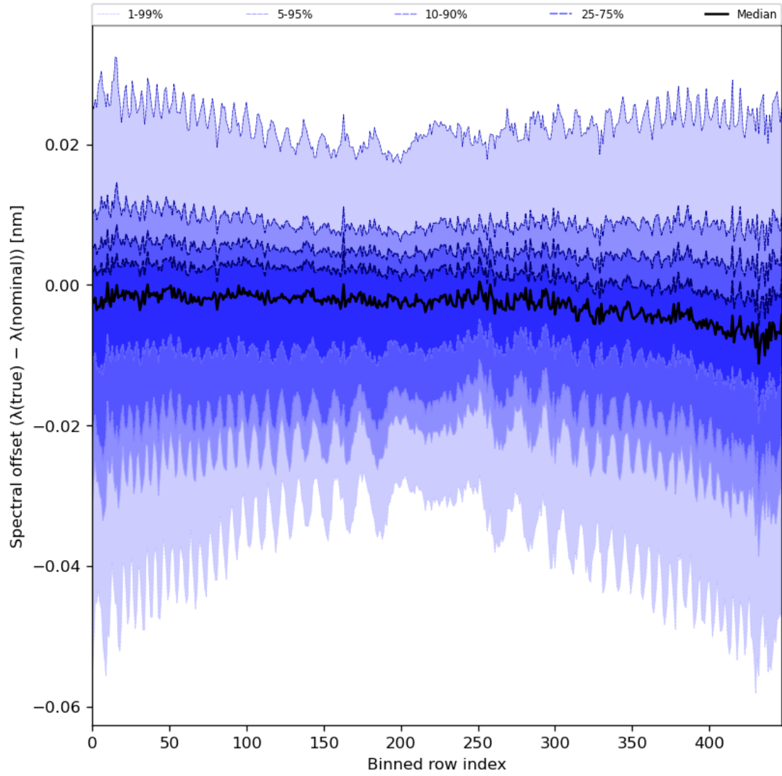
Figure 62: Along track statistics of “Spectral offset ( \lambda(\text{true}) - \lambda(\text{nominal}) )” for 2024-01-31 to 2024-02-01
