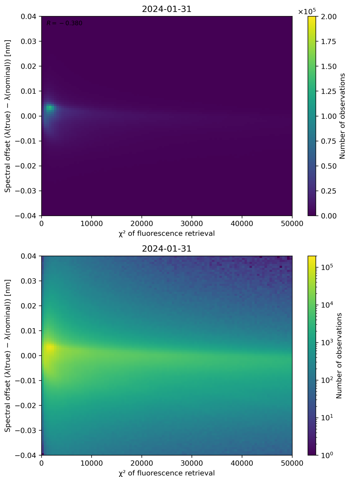
Figure 69: Scatter density plot of " \chi^2 of fluorescence retrieval" against "Spectral offset ( \lambda(\text{true}) - \lambda(\text{nominal}) )" for 2024-01-31 to 2024-02-01.
