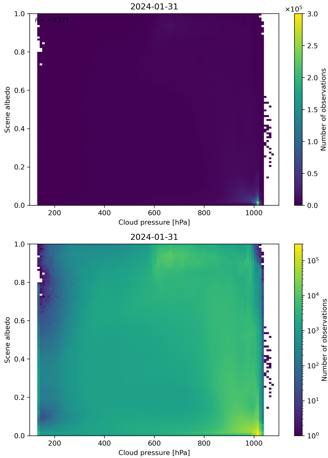
Figure 83: Scatter density plot of “Cloud pressure” against “Scene albedo” for 2024-01-31 to 2024-02-01.
