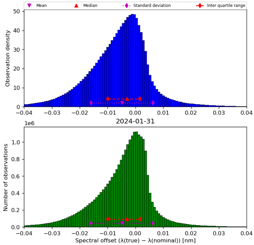
Figure 45: Histogram of “Spectral offset ( \lambda(\text{true}) - \lambda(\text{nominal}) )” for 2024-01-31 to 2024-02-01
