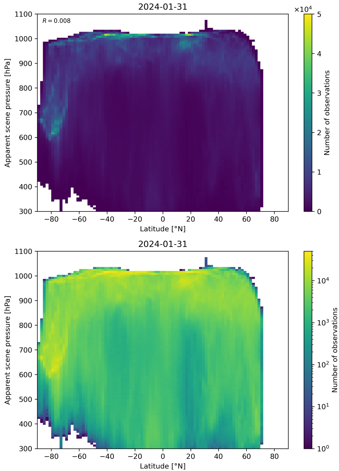
Figure 88: Scatter density plot of “Latitude” against “Apparent scene pressure” for 2024-01-31 to 2024-02-01.
