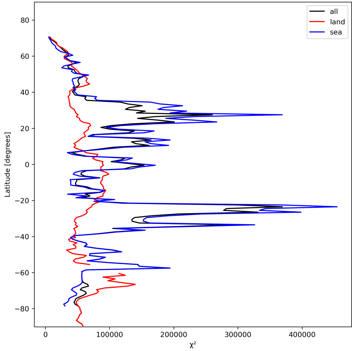
Figure 21: Zonal average of “ \chi^2 ” for 2024-01-31 to 2024-02-01.
