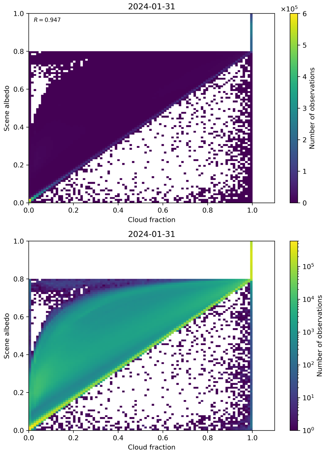
Figure 75: Scatter density plot of “Cloud fraction” against “Scene albedo” for 2024-01-31 to 2024-02-01.
