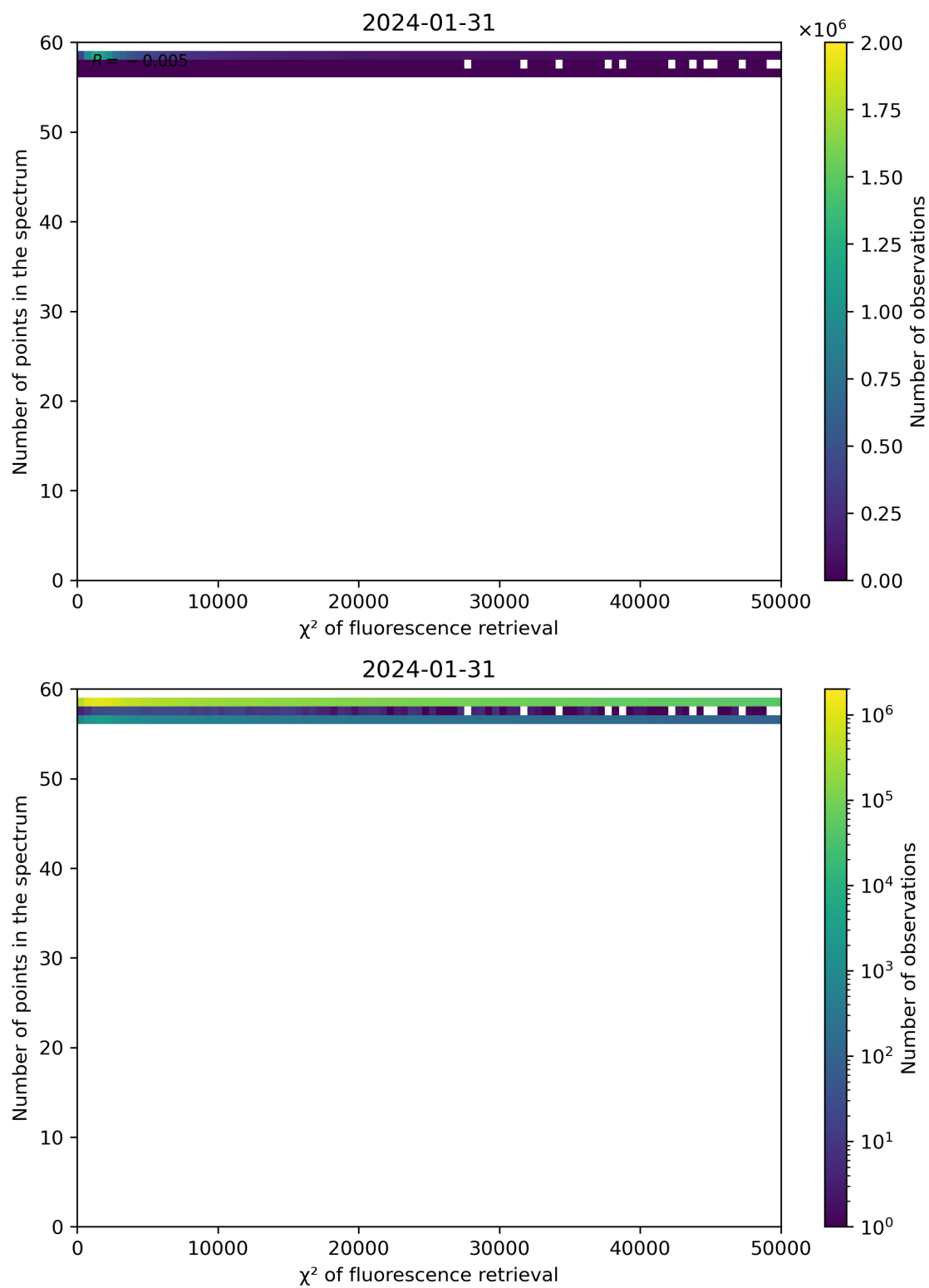
Figure 68: Scatter density plot of “ \chi^2 of fluorescence retrieval” against “Number of points in the spectrum” for 2024-01-31 to 2024-02-01.
