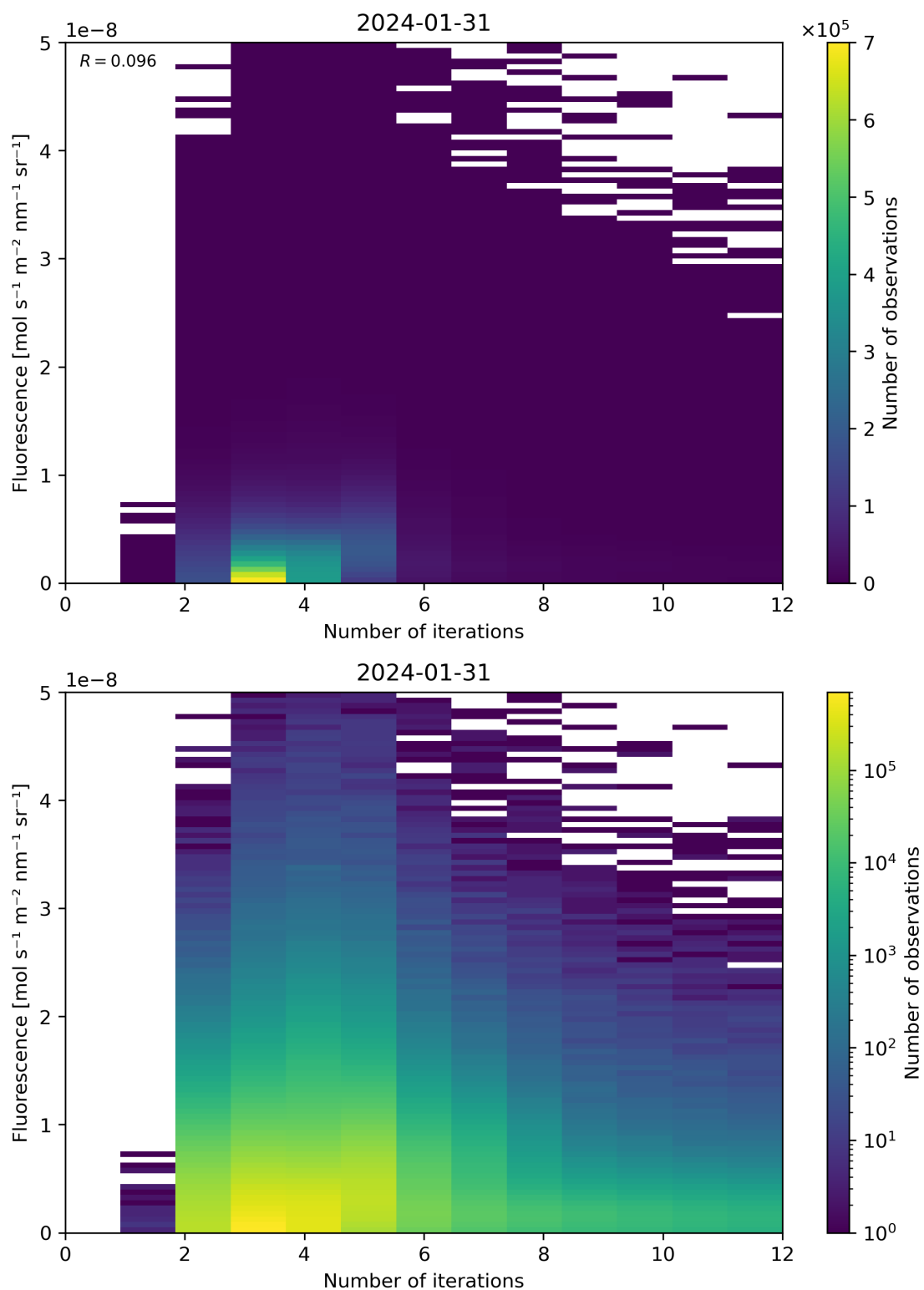
Figure 98: Scatter density plot of “Number of iterations” against “Fluorescence” for 2024-01-31 to 2024-02-01.
