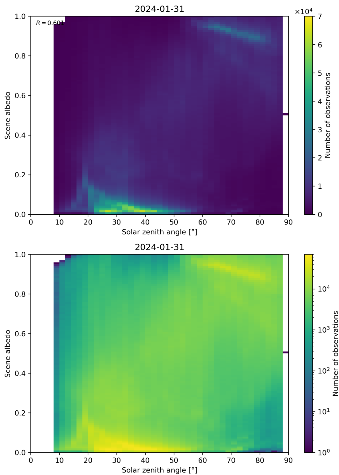
Figure 116: Scatter density plot of “Solar zenith angle” against “Scene albedo” for 2024-01-31 to 2024-02-01.
