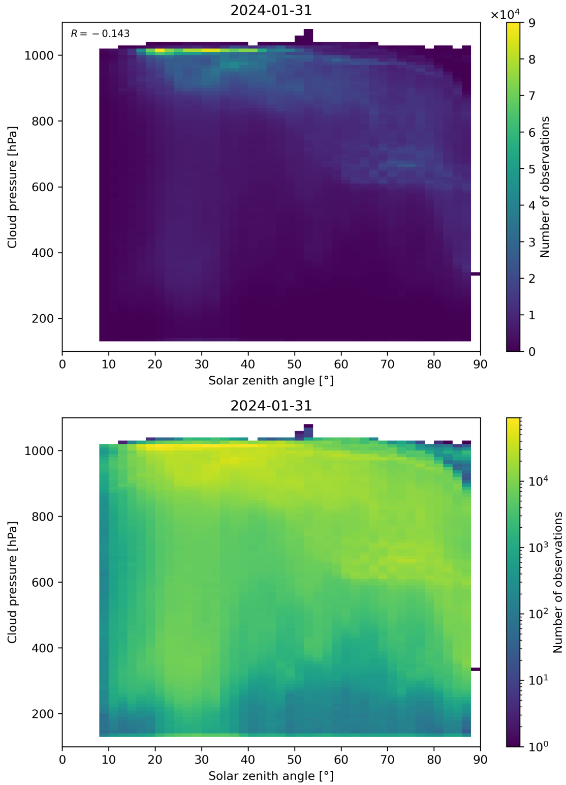
Figure 111: Scatter density plot of “Solar zenith angle” against “Cloud pressure” for 2024-01-31 to 2024-02-01.
