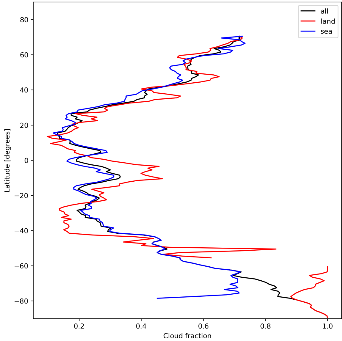
Figure 15: Zonal average of “Cloud fraction” for 2024-01-31 to 2024-02-01.
