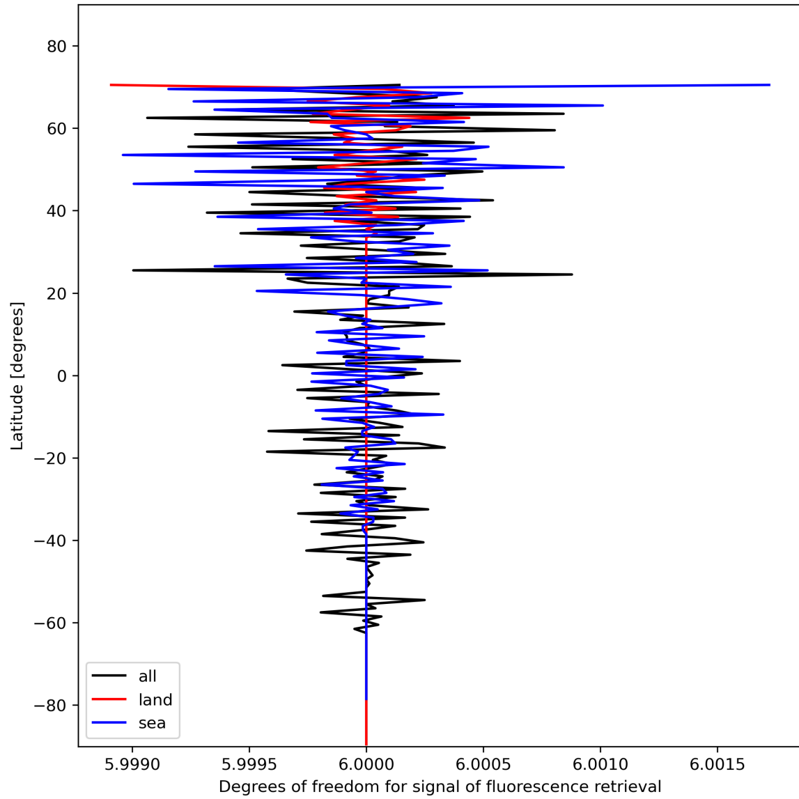
Figure 26: Zonal average of “Degrees of freedom for signal of fluorescence retrieval” for 2024-01-31 to 2024-02-01.
