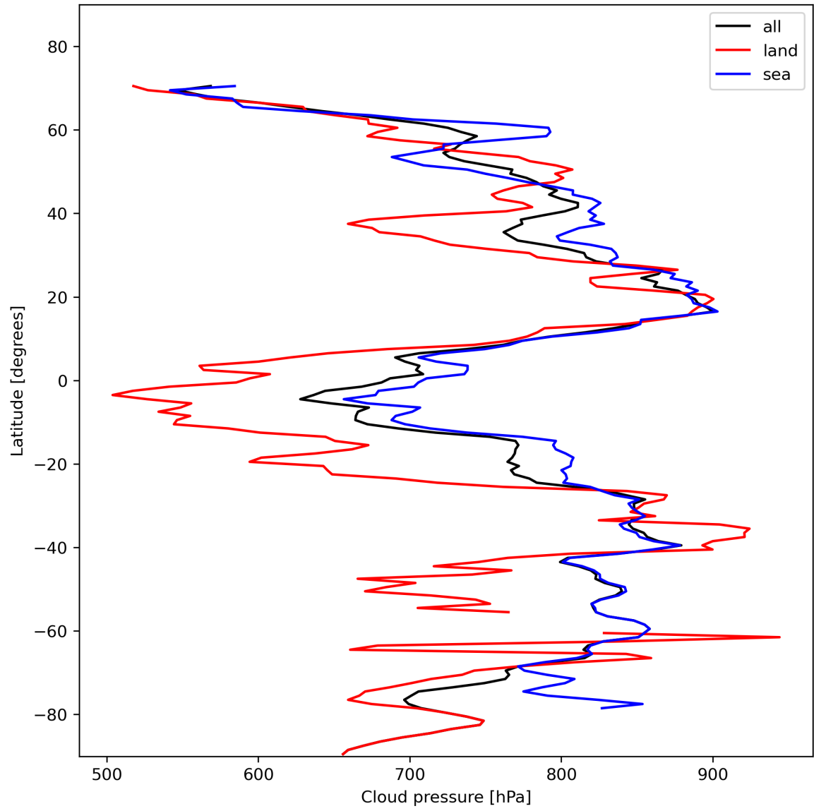
Figure 13: Zonal average of “Cloud pressure” for 2024-01-31 to 2024-02-01.
