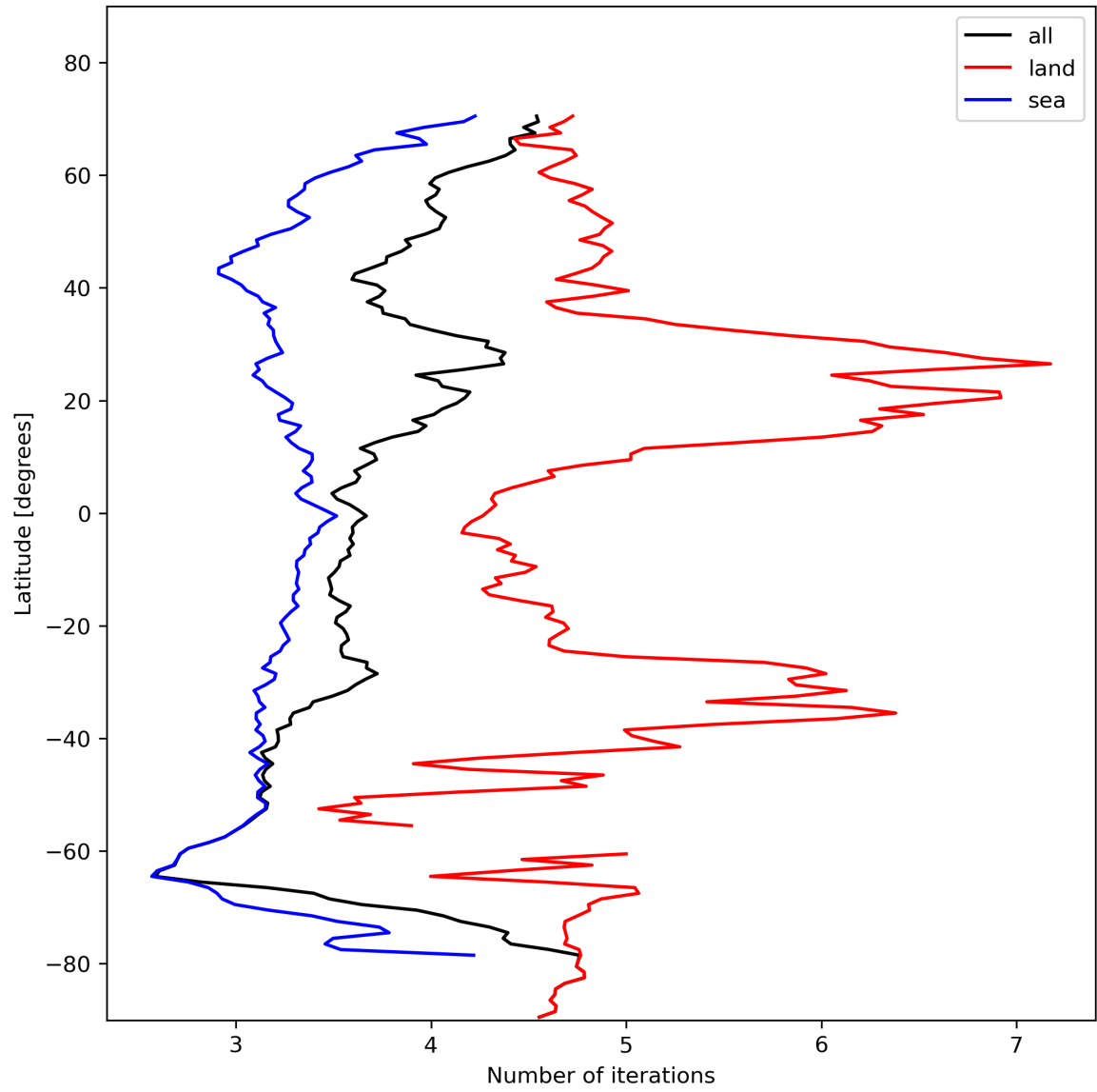
Figure 22: Zonal average of “Number of iterations” for 2024-01-31 to 2024-02-01.
