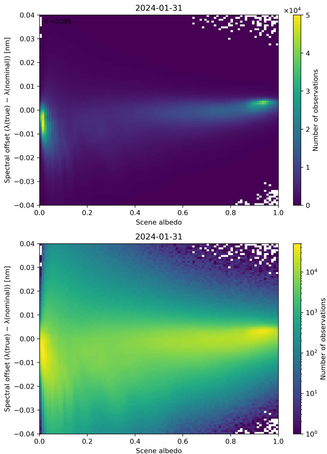
Figure 107: Scatter density plot of “Scene albedo” against “Spectral offset ( \lambda(\text{true}) - \lambda(\text{nominal}) )” for 2024-01-31 to 2024-02-01.
