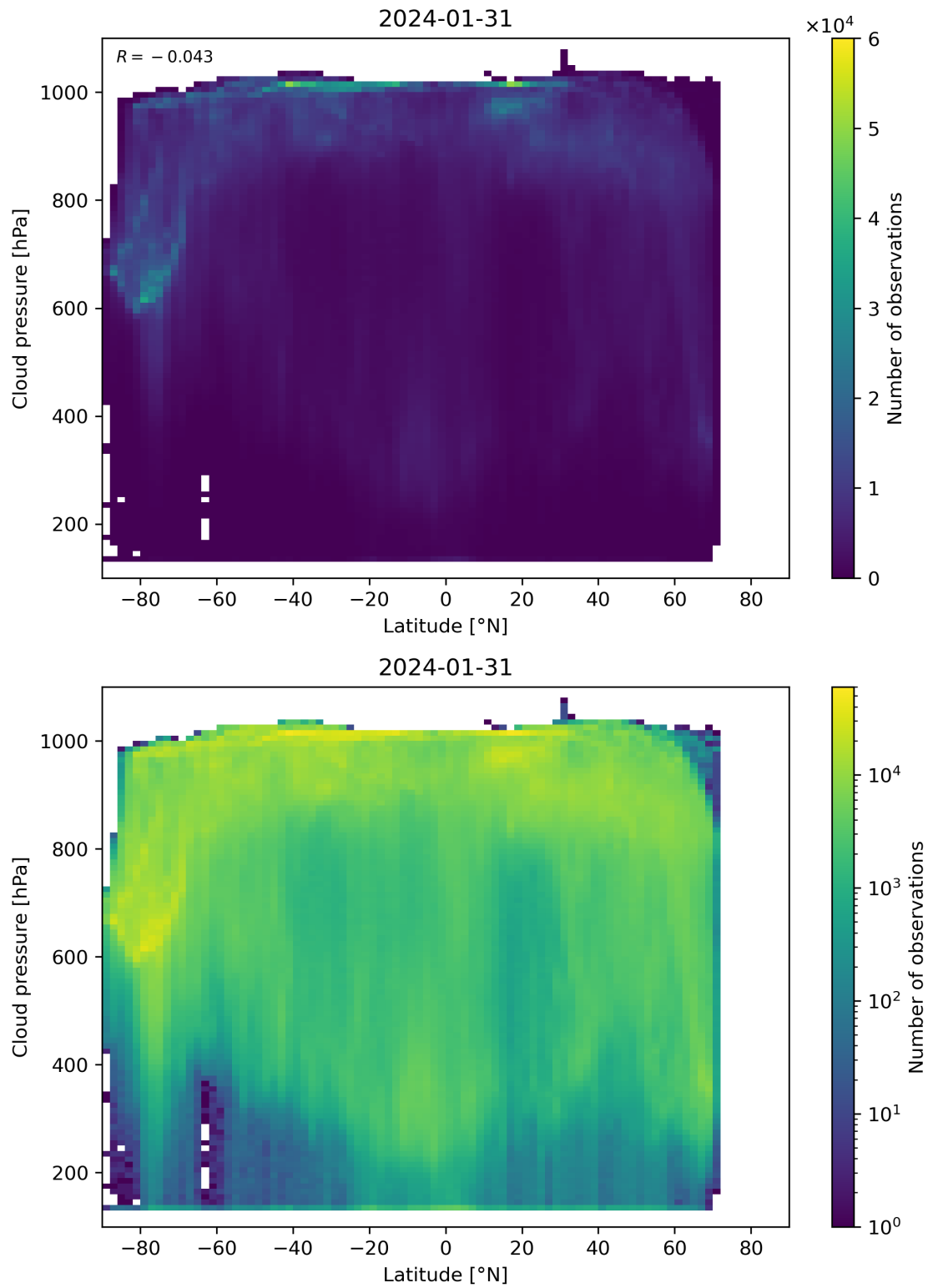
Figure 91: Scatter density plot of “Latitude” against “Cloud pressure” for 2024-01-31 to 2024-02-01.
