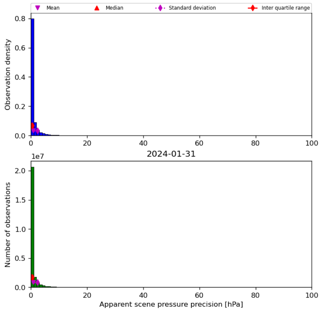
Figure 37: Histogram of “Apparent scene pressure precision” for 2024-01-31 to 2024-02-01
