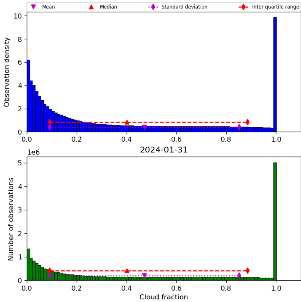
Figure 32: Histogram of “Cloud fraction” for 2024-01-31 to 2024-02-01
