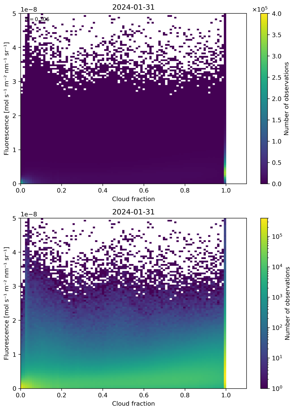
Figure 72: Scatter density plot of “Cloud fraction” against “Fluorescence” for 2024-01-31 to 2024-02-01.
