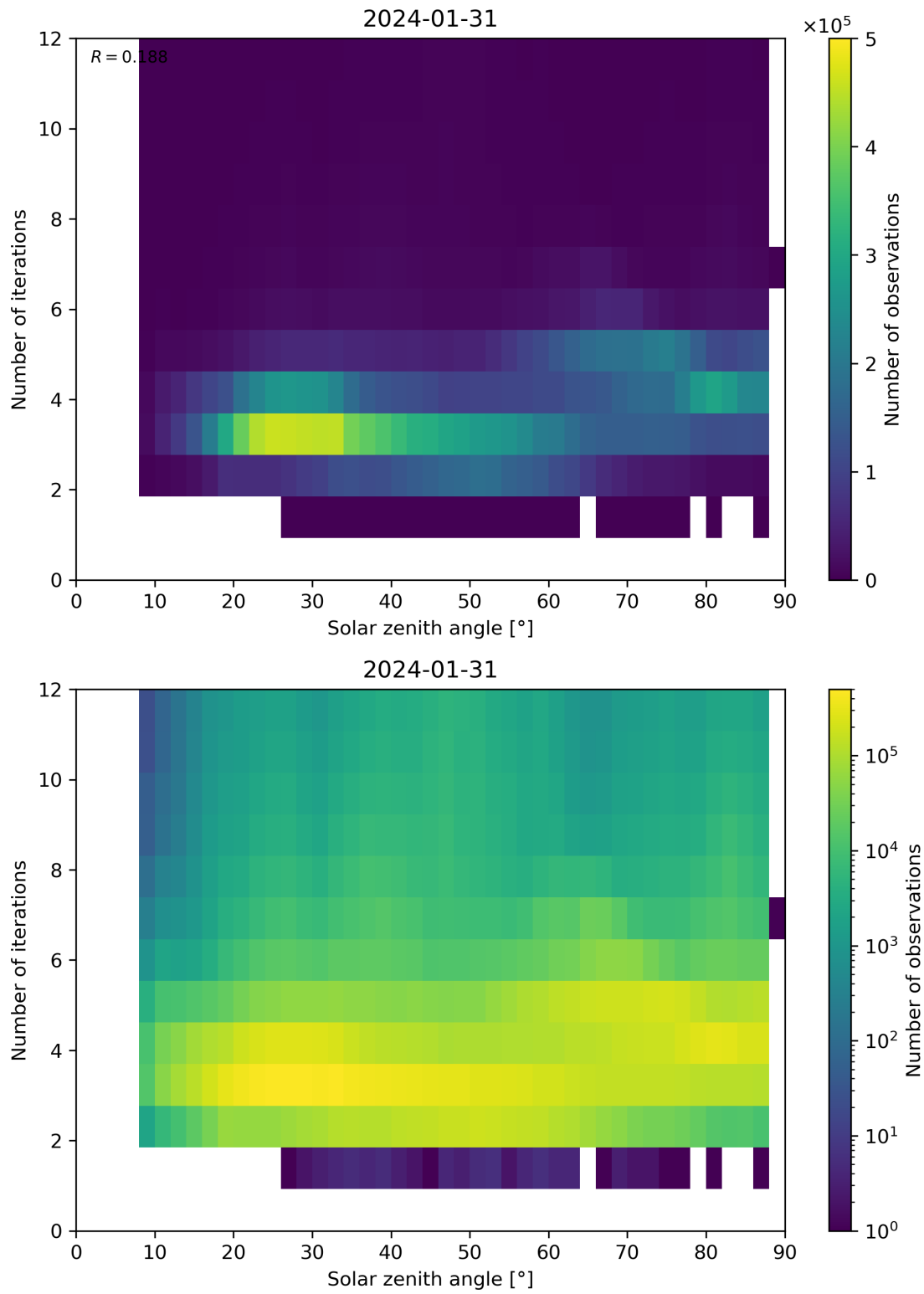
Figure 114: Scatter density plot of “Solar zenith angle” against “Number of iterations” for 2024-01-31 to 2024-02-01.
