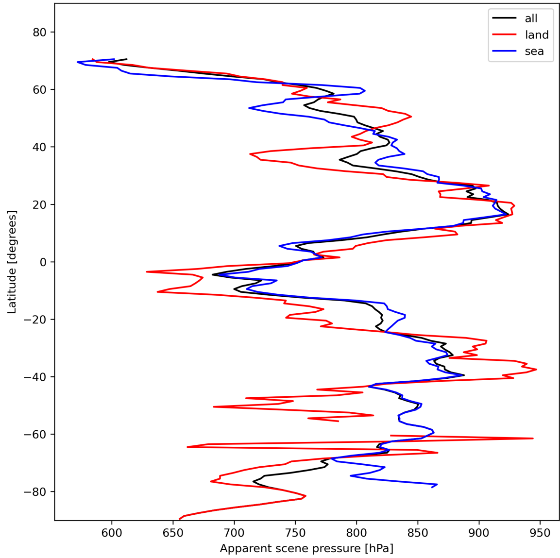
Figure 19: Zonal average of “Apparent scene pressure” for 2024-01-31 to 2024-02-01.
