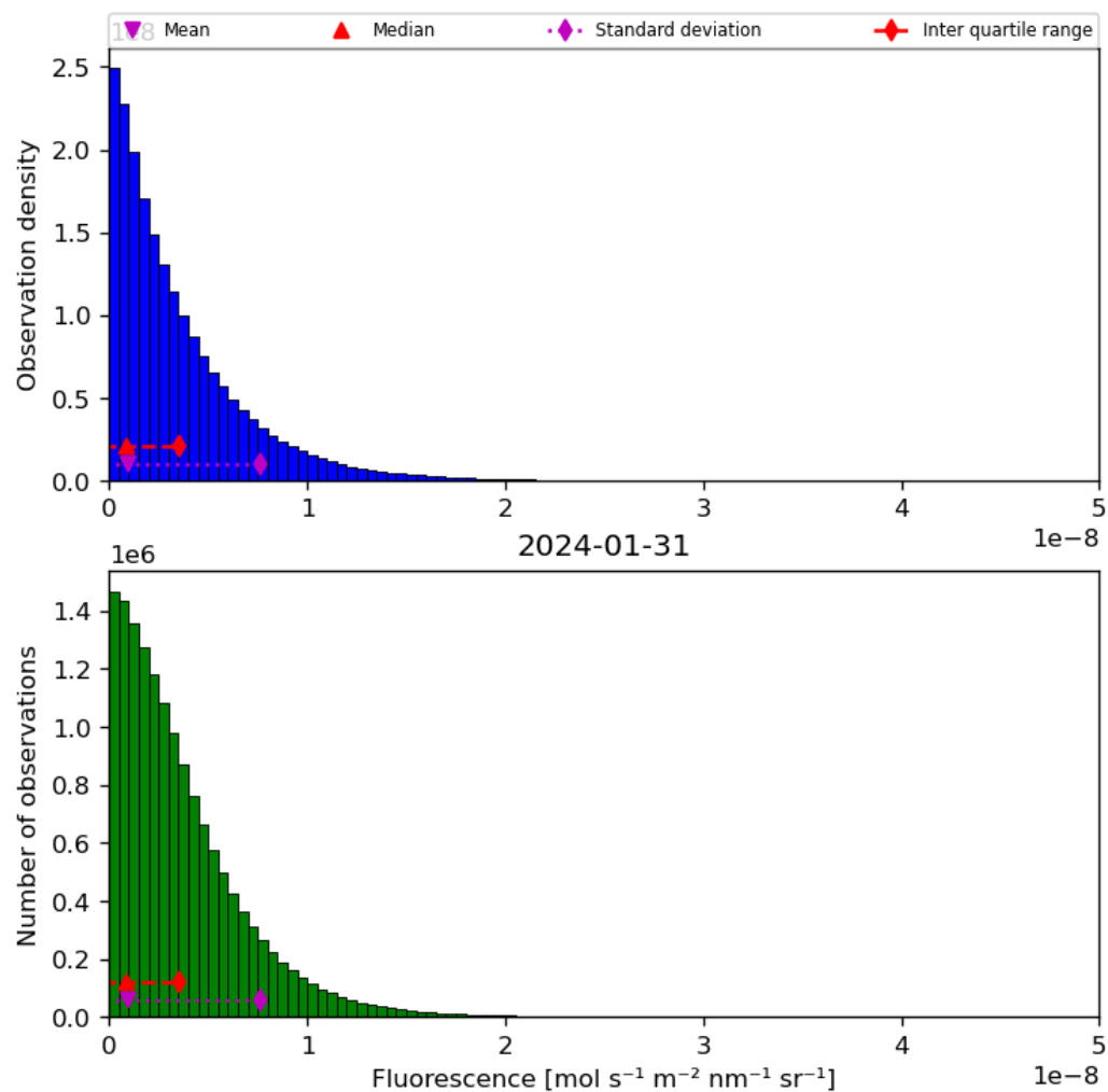
Figure 40: Histogram of “Fluorescence” for 2024-01-31 to 2024-02-01
