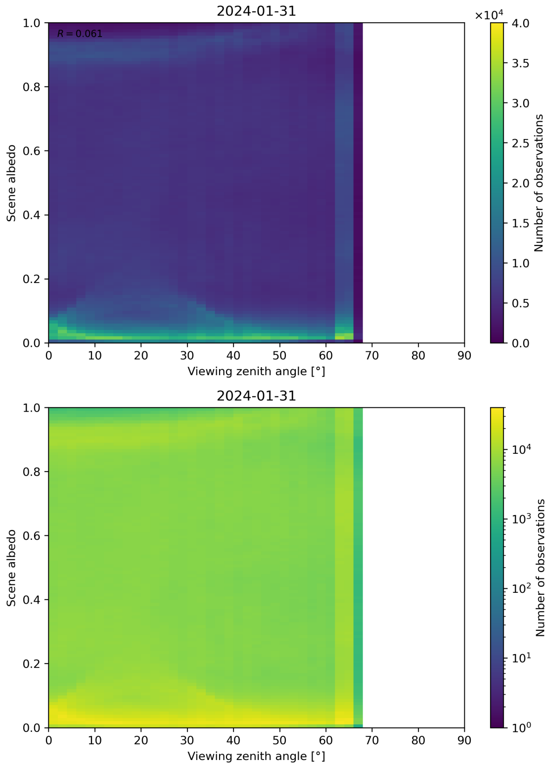
Figure 126: Scatter density plot of “Viewing zenith angle” against “Scene albedo” for 2024-01-31 to 2024-02-01.
