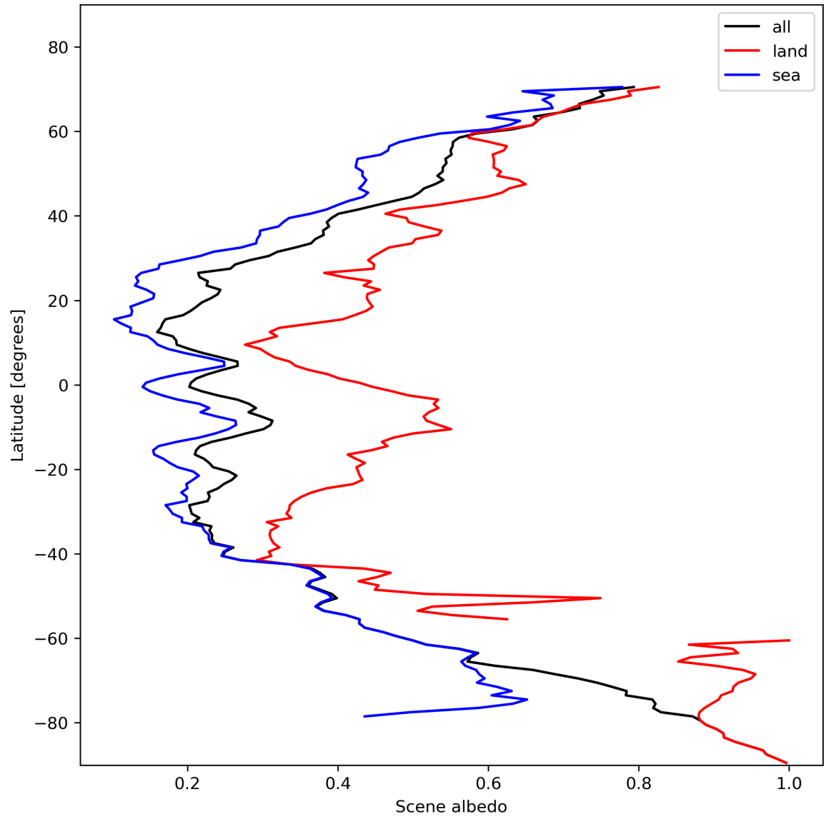
Figure 17: Zonal average of “Scene albedo” for 2024-01-31 to 2024-02-01.
