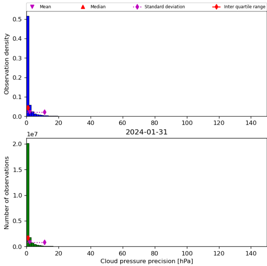
Figure 31: Histogram of “Cloud pressure precision” for 2024-01-31 to 2024-02-01
