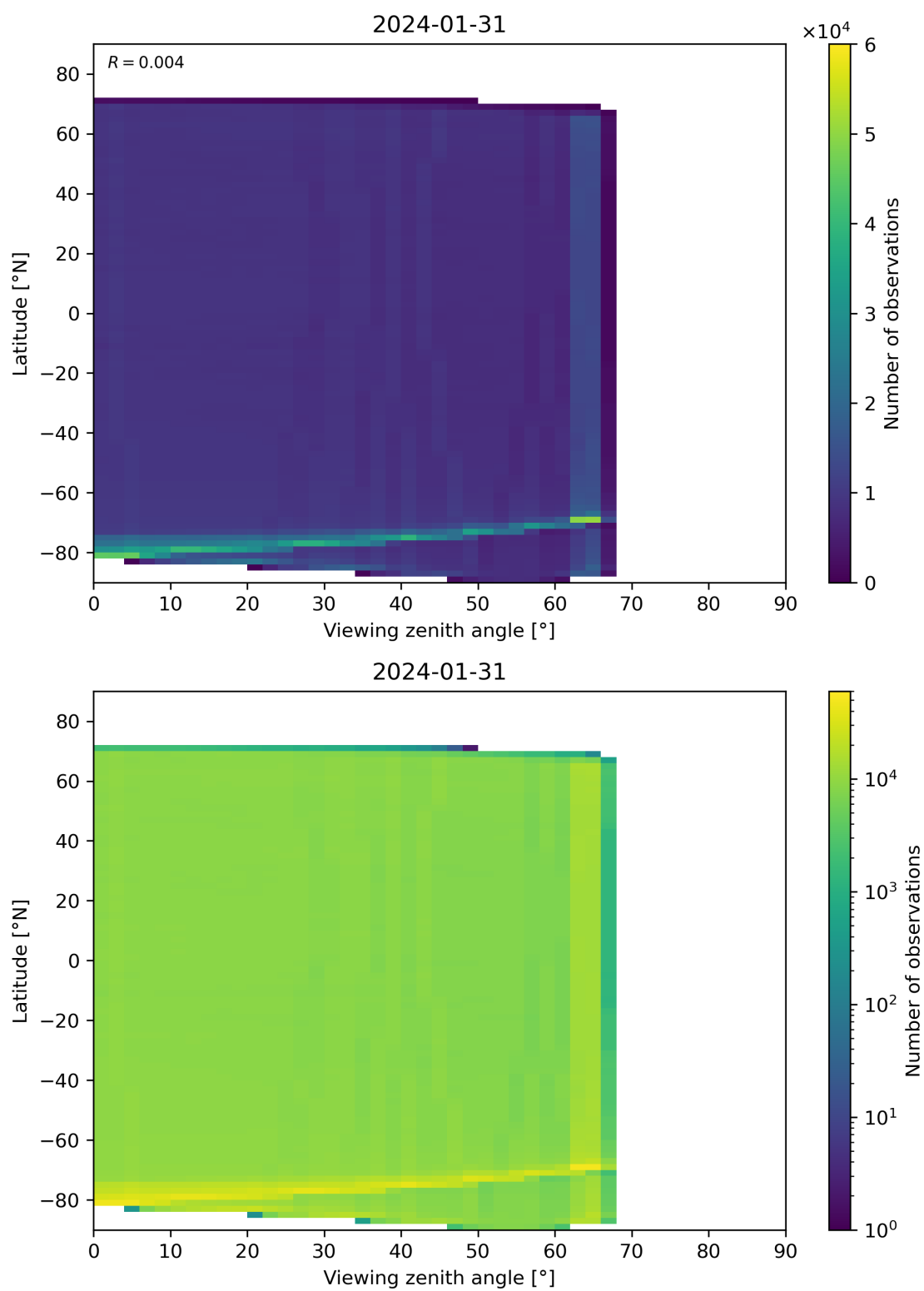
Figure 123: Scatter density plot of “Viewing zenith angle” against “Latitude” for 2024-01-31 to 2024-02-01.
