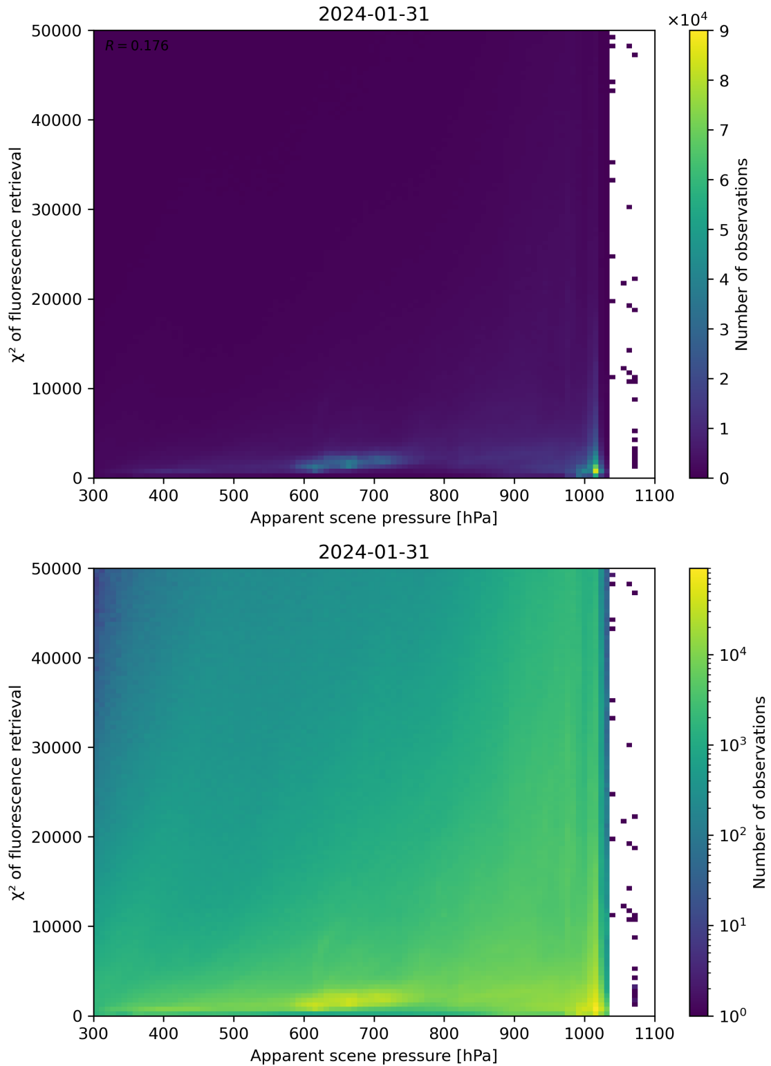
Figure 63: Scatter density plot of “Apparent scene pressure” against “ \chi^2 of fluorescence retrieval” for 2024-01-31 to 2024-02-01.
