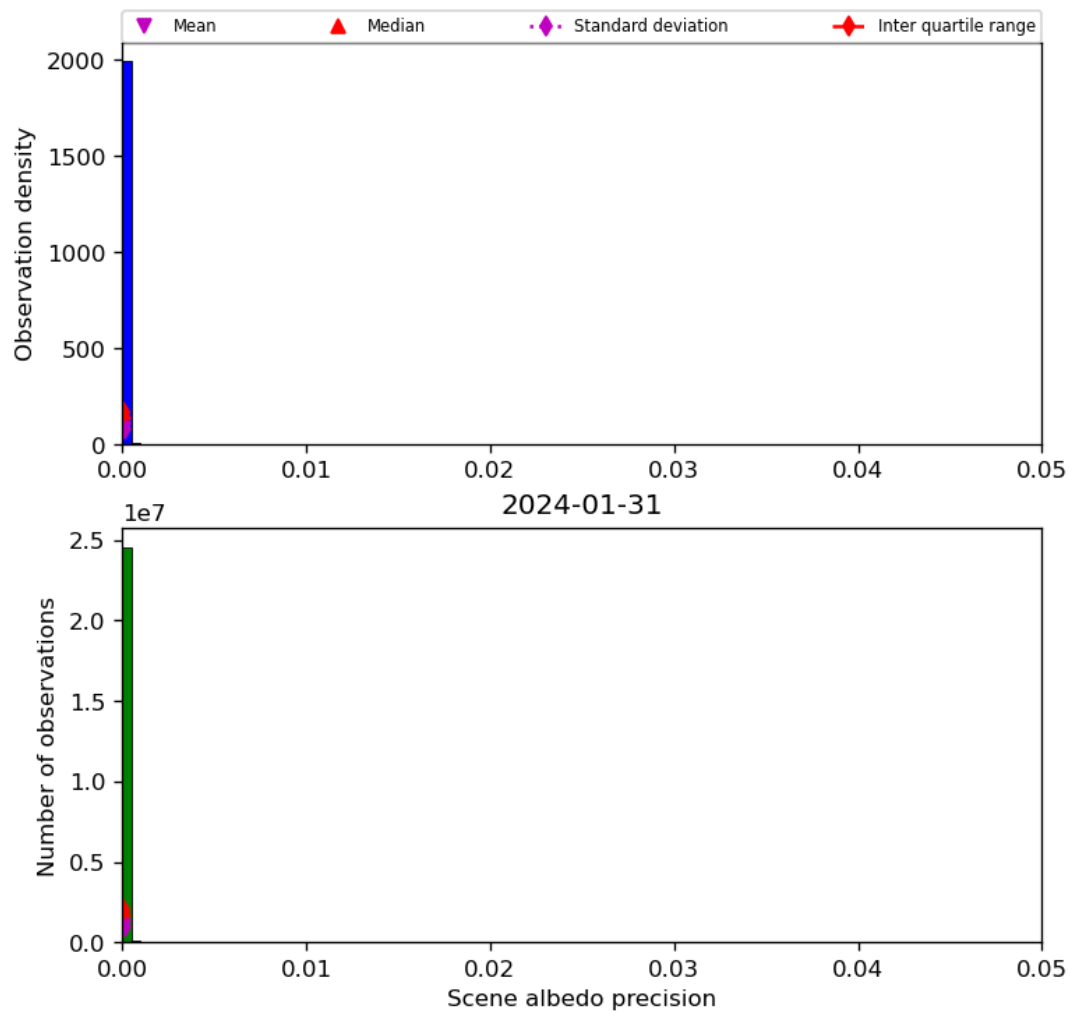
Figure 35: Histogram of “Scene albedo precision” for 2024-01-31 to 2024-02-01
