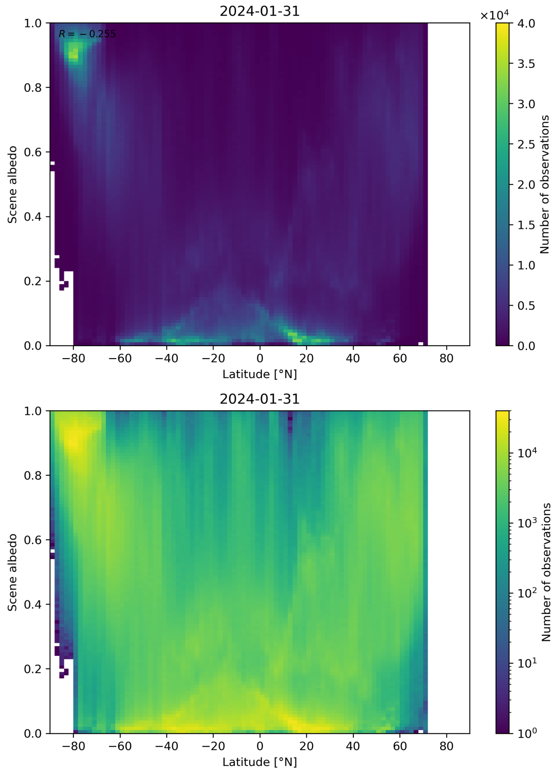
Figure 95: Scatter density plot of “Latitude” against “Scene albedo” for 2024-01-31 to 2024-02-01.
