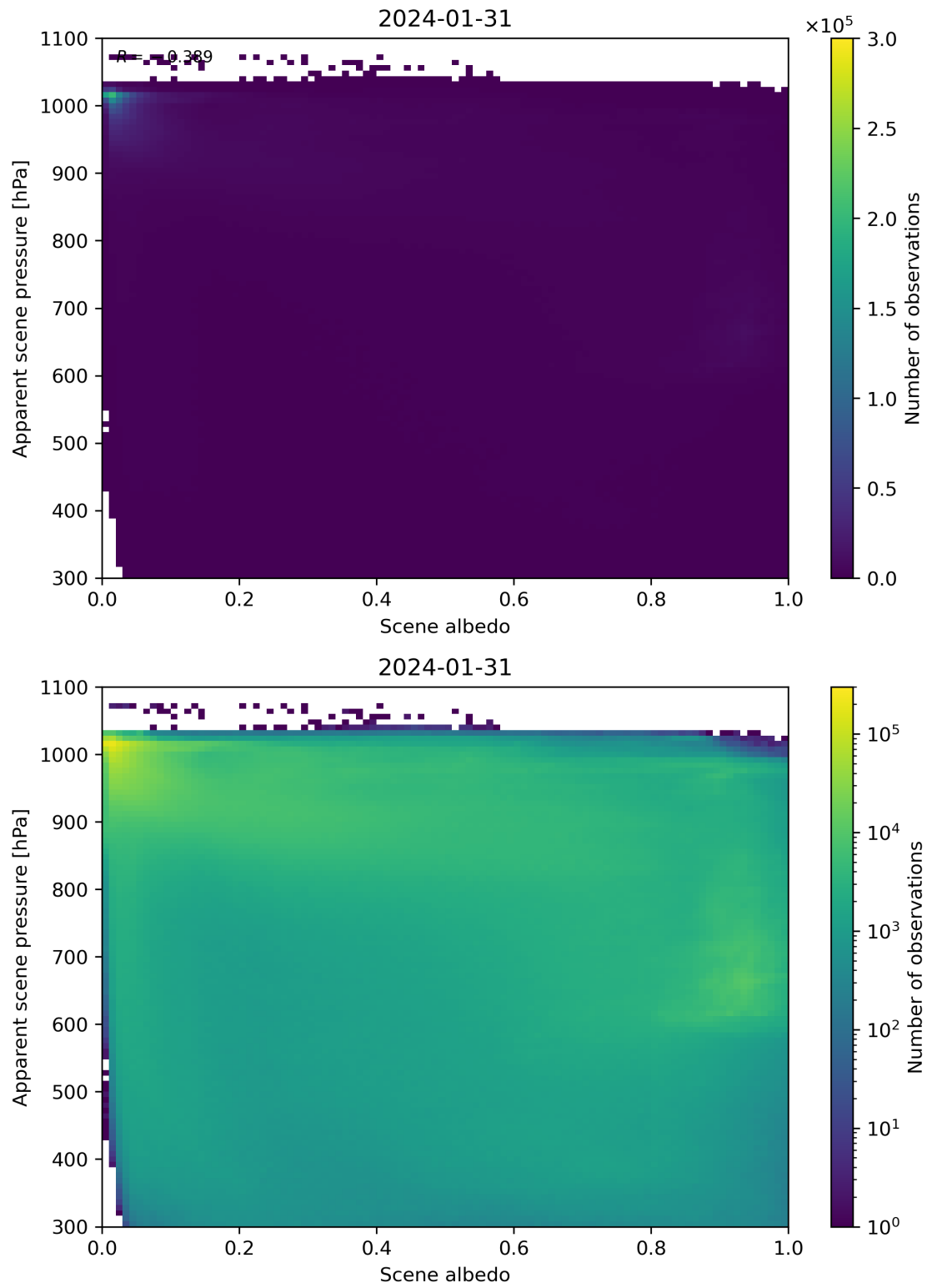
Figure 102: Scatter density plot of “Scene albedo” against “Apparent scene pressure” for 2024-01-31 to 2024-02-01.
