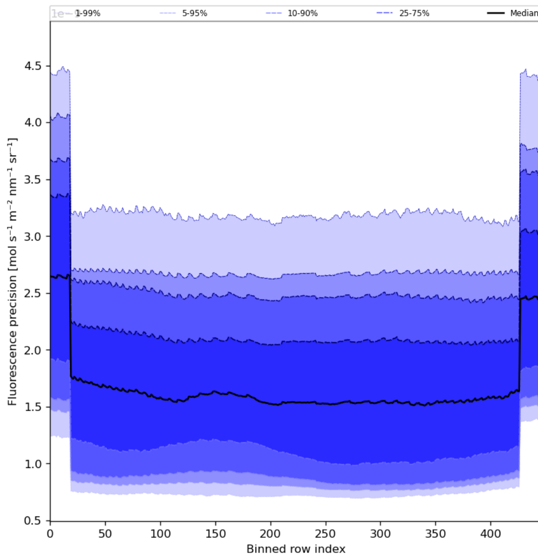
Figure 58: Along track statistics of “Fluorescence precision” for 2024-01-31 to 2024-02-01
