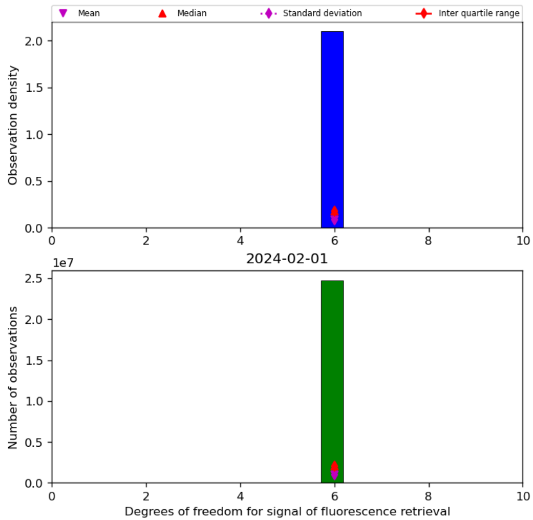
Figure 43: Histogram of “Degrees of freedom for signal of fluorescence retrieval” for 2024-01-31 to 2024-02-02
