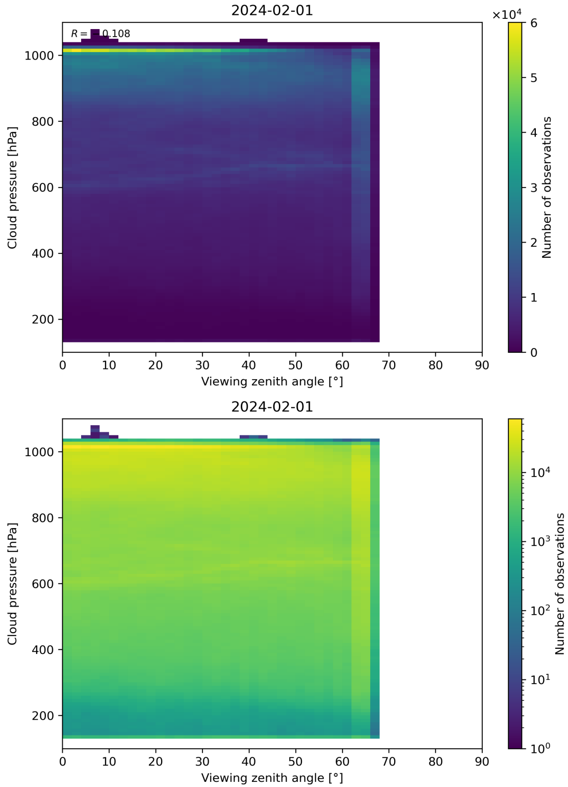
Figure 121: Scatter density plot of “Viewing zenith angle” against “Cloud pressure” for 2024-01-31 to 2024-02-02.
