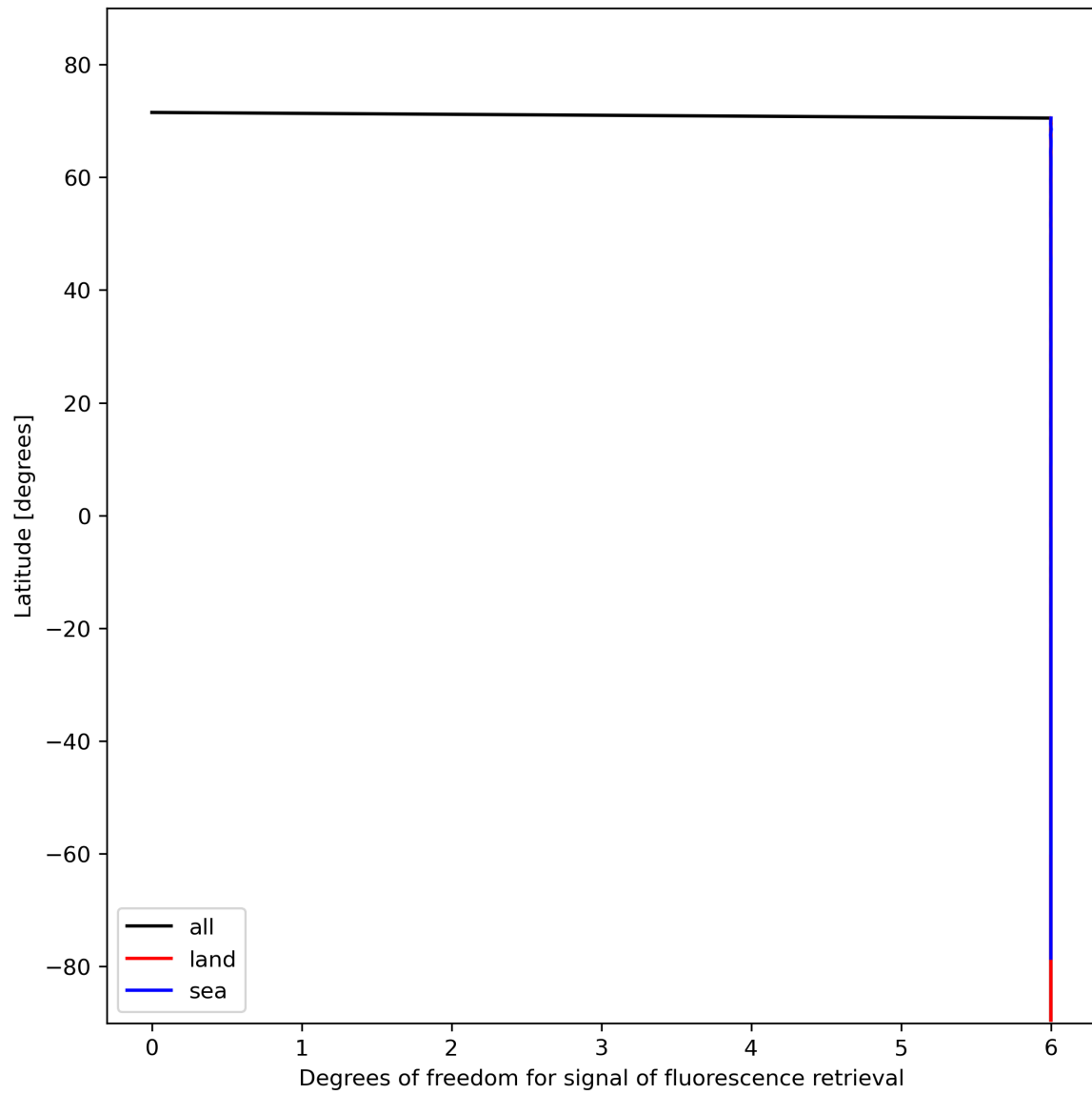
Figure 26: Zonal average of “Degrees of freedom for signal of fluorescence retrieval” for 2024-01-31 to 2024-02-02.
