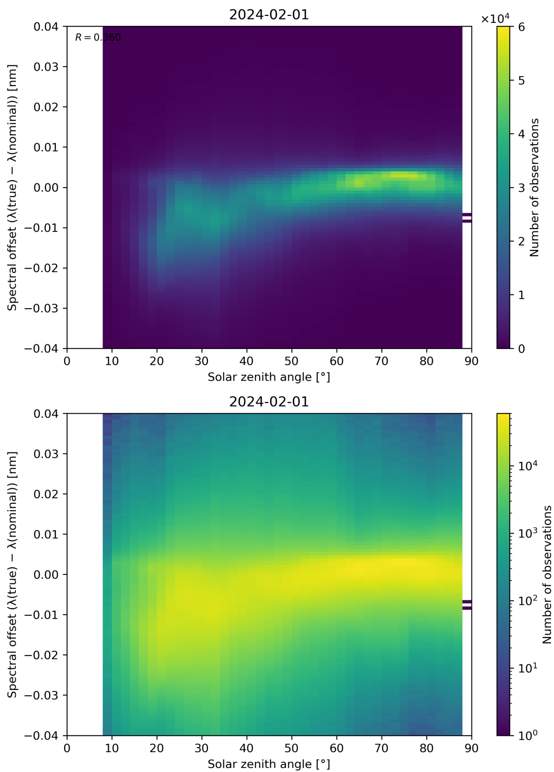
Figure 117: Scatter density plot of “Solar zenith angle” against “Spectral offset ( \lambda(\text{true}) - \lambda(\text{nominal}) )” for 2024-01-31 to 2024-02-02.
