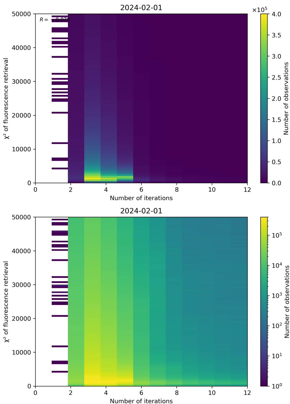
Figure 97: Scatter density plot of “Number of iterations” against “ \chi^2 of fluorescence retrieval” for 2024-01-31 to 2024-02-02.
