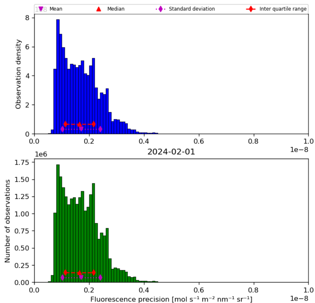
Figure 41: Histogram of “Fluorescence precision” for 2024-01-31 to 2024-02-02
