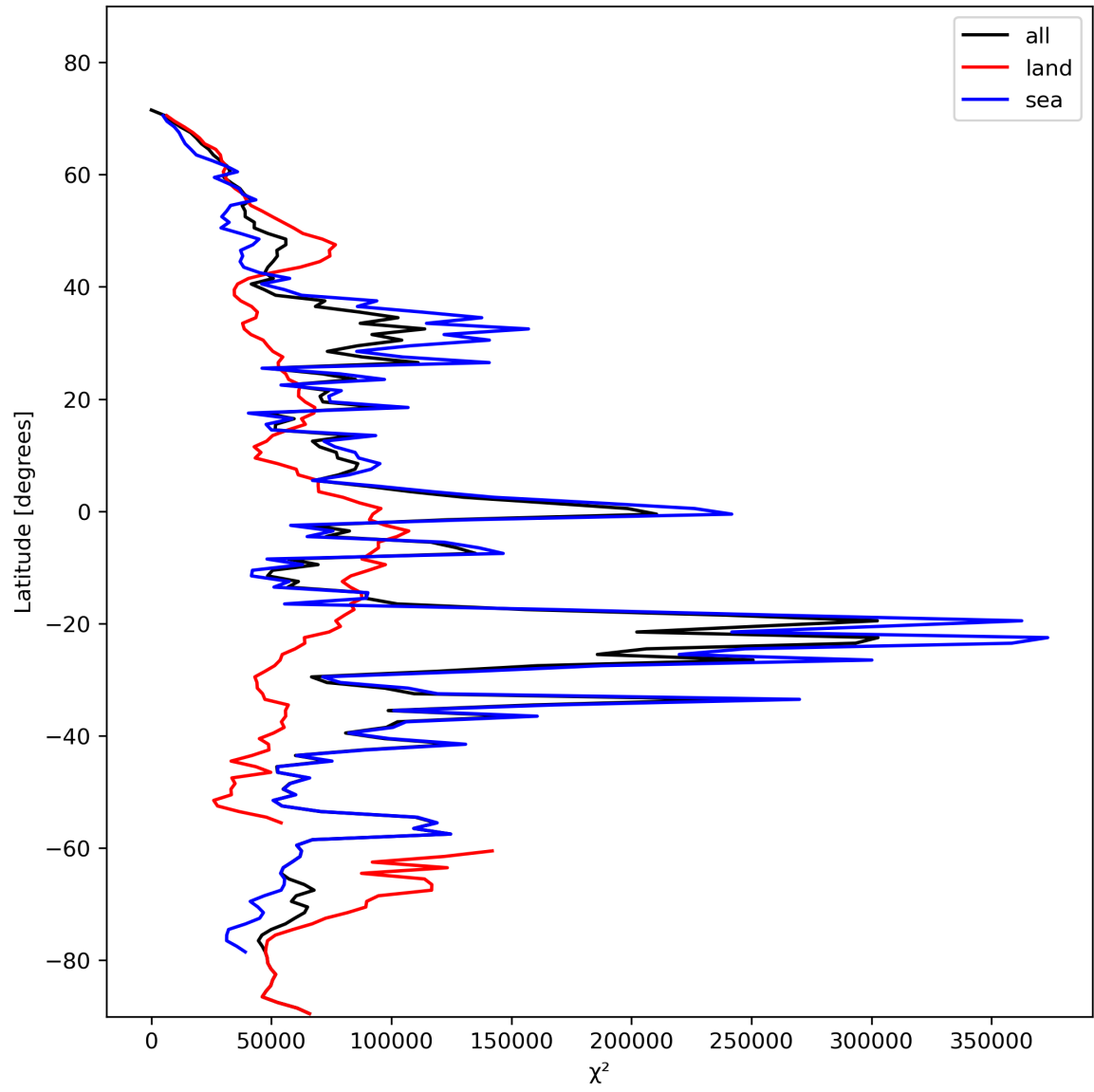
Figure 21: Zonal average of “ \chi^2 ” for 2024-01-31 to 2024-02-02.
