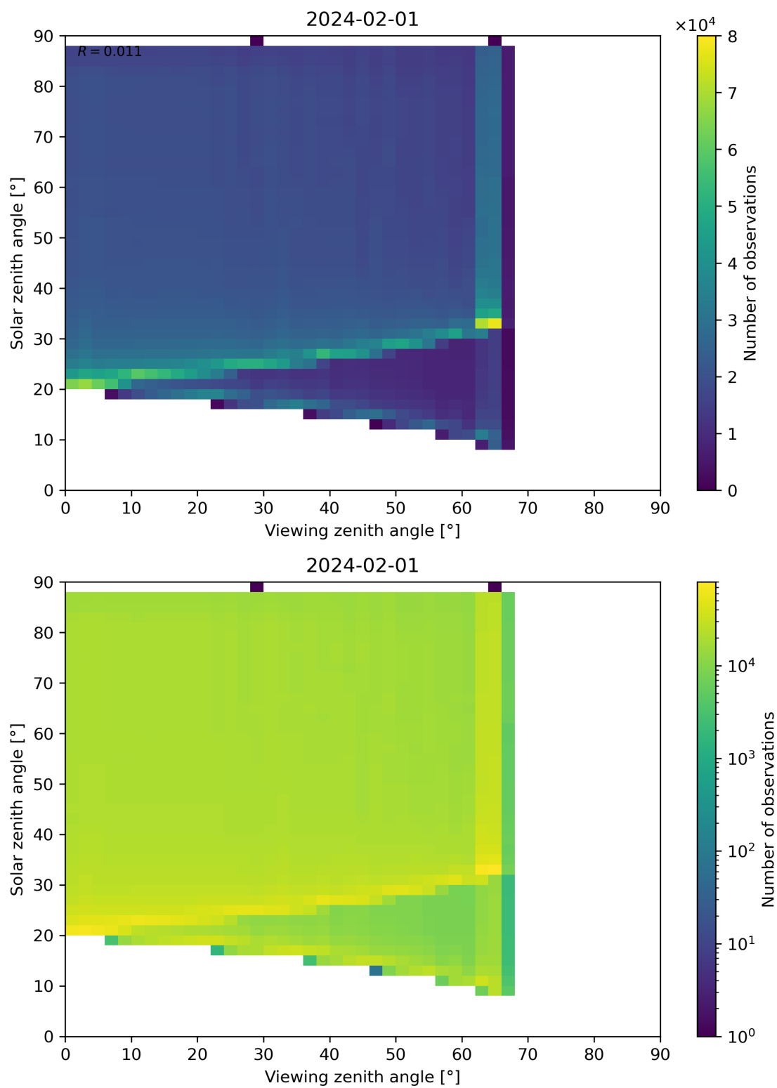
Figure 127: Scatter density plot of “Viewing zenith angle” against “Solar zenith angle” for 2024-01-31 to 2024-02-02.
