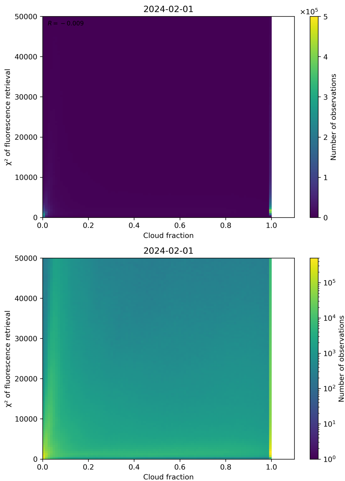
Figure 71: Scatter density plot of “Cloud fraction” against “ \chi^2 of fluorescence retrieval” for 2024-01-31 to 2024-02-02.
