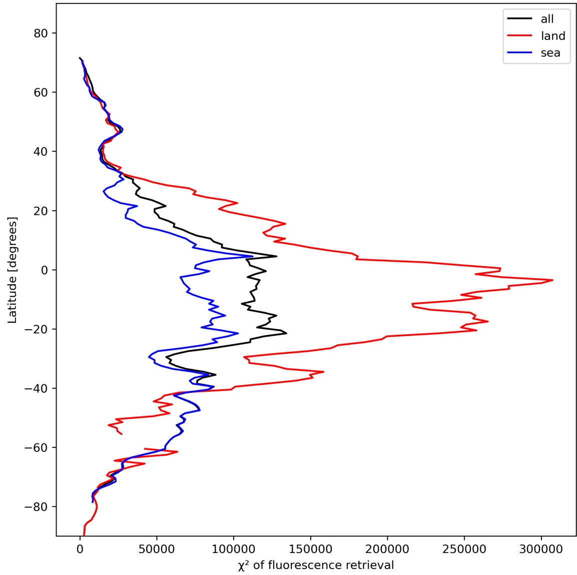
Figure 25: Zonal average of “ \chi^2 of fluorescence retrieval” for 2024-01-31 to 2024-02-02.
