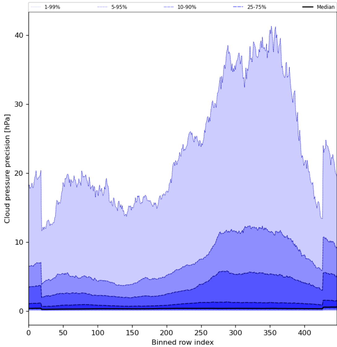
Figure 48: Along track statistics of “Cloud pressure precision” for 2024-01-31 to 2024-02-02
