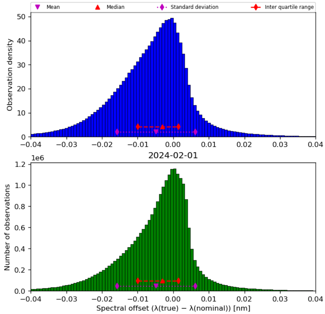
Figure 45: Histogram of “Spectral offset ( \lambda(\text{true}) - \lambda(\text{nominal}) )” for 2024-01-31 to 2024-02-02
