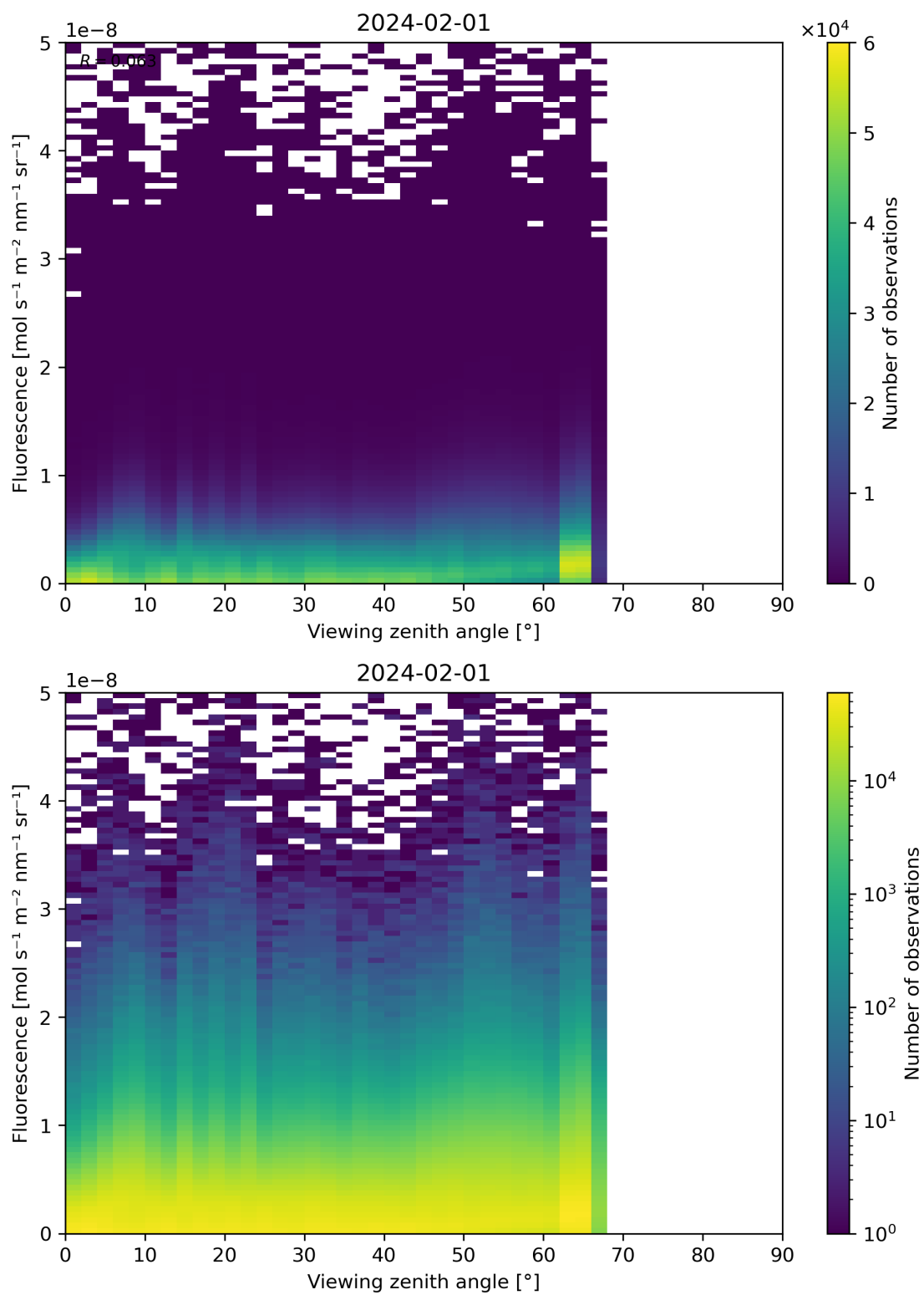
Figure 122: Scatter density plot of “Viewing zenith angle” against “Fluorescence” for 2024-01-31 to 2024-02-02.
