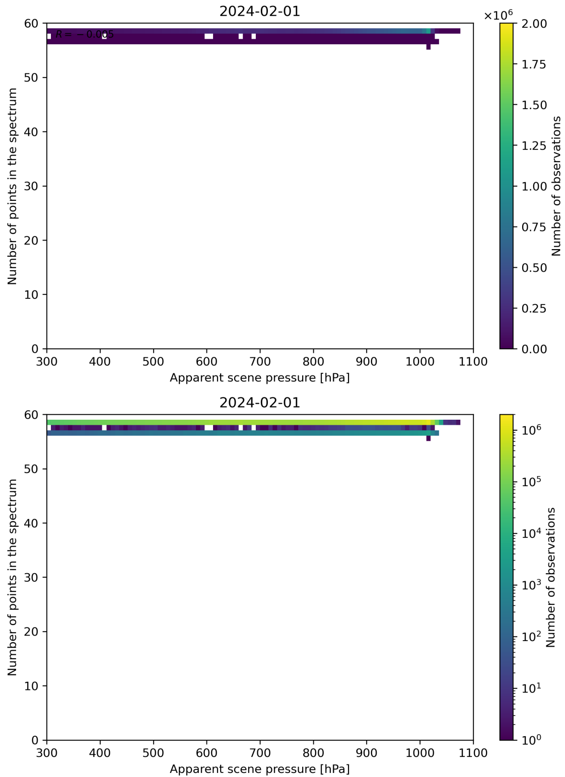
Figure 66: Scatter density plot of “Apparent scene pressure” against “Number of points in the spectrum” for 2024-01-31 to 2024-02-02.
