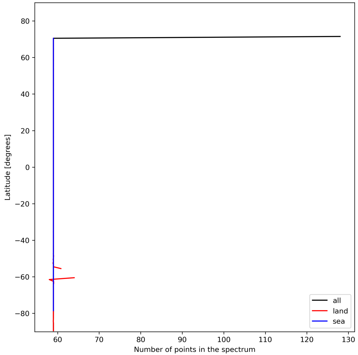
Figure 27: Zonal average of “Number of points in the spectrum” for 2024-01-31 to 2024-02-02.
