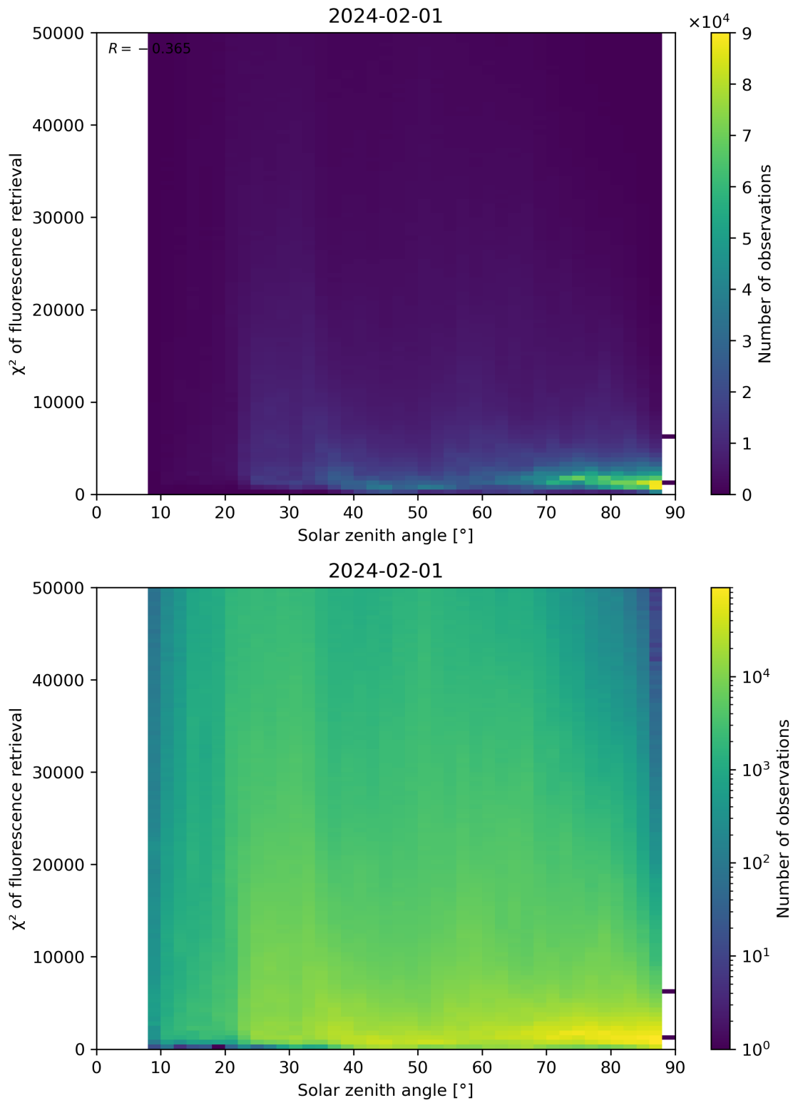
Figure 109: Scatter density plot of “Solar zenith angle” against “ \chi^2 of fluorescence retrieval” for 2024-01-31 to 2024-02-02.
