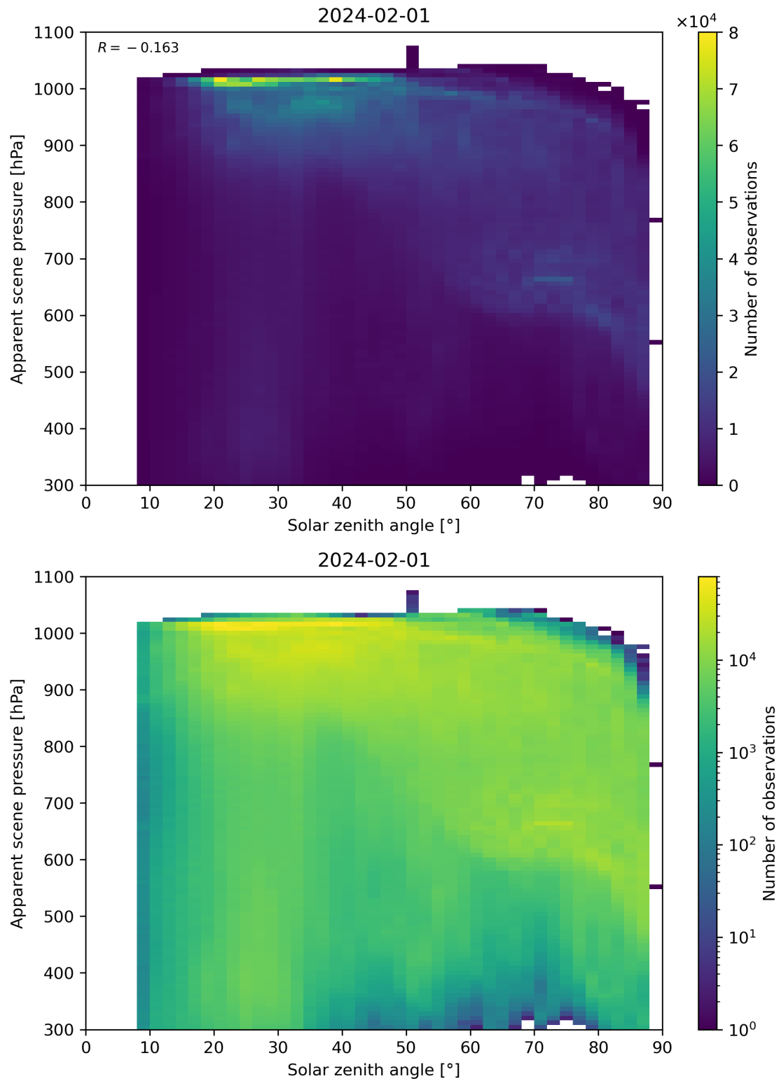
Figure 108: Scatter density plot of “Solar zenith angle” against “Apparent scene pressure” for 2024-01-31 to 2024-02-02.
