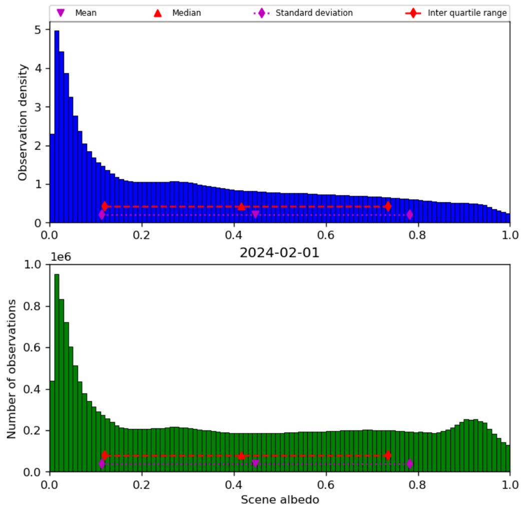
Figure 34: Histogram of “Scene albedo” for 2024-01-31 to 2024-02-02
