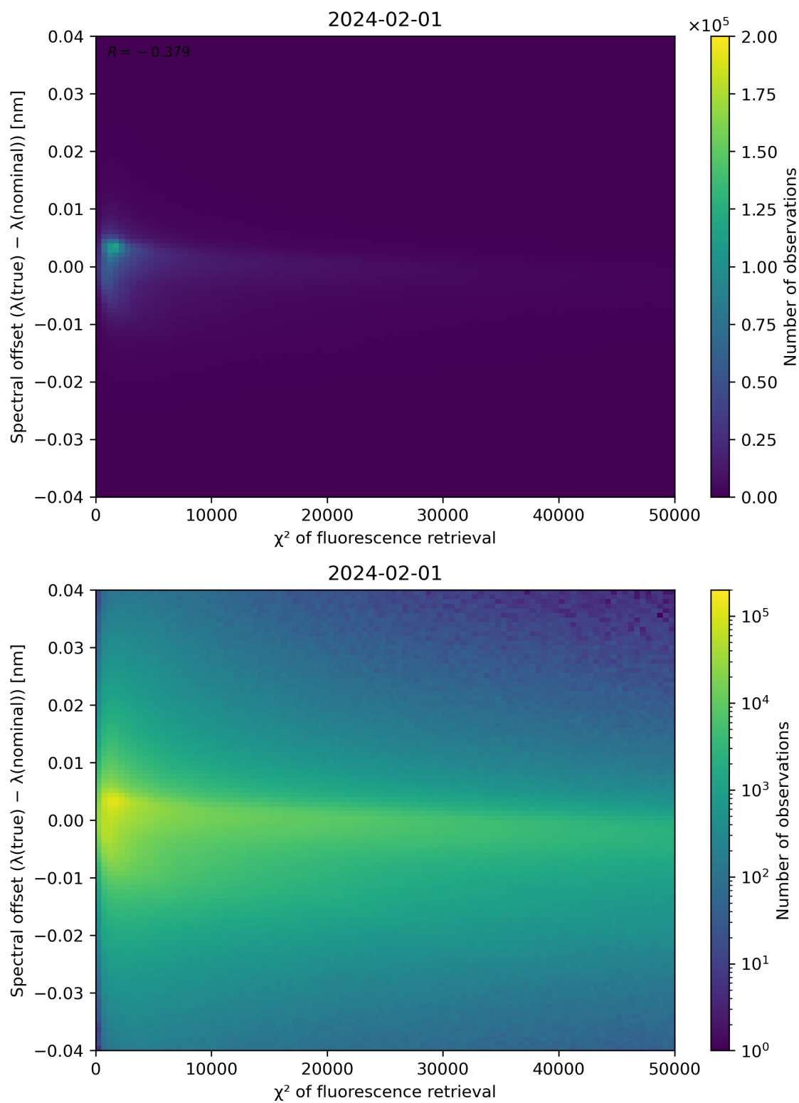
Figure 69: Scatter density plot of " \chi^2 of fluorescence retrieval" against "Spectral offset ( \lambda(\text{true}) - \lambda(\text{nominal})) " for 2024-01-31 to 2024-02-02.
