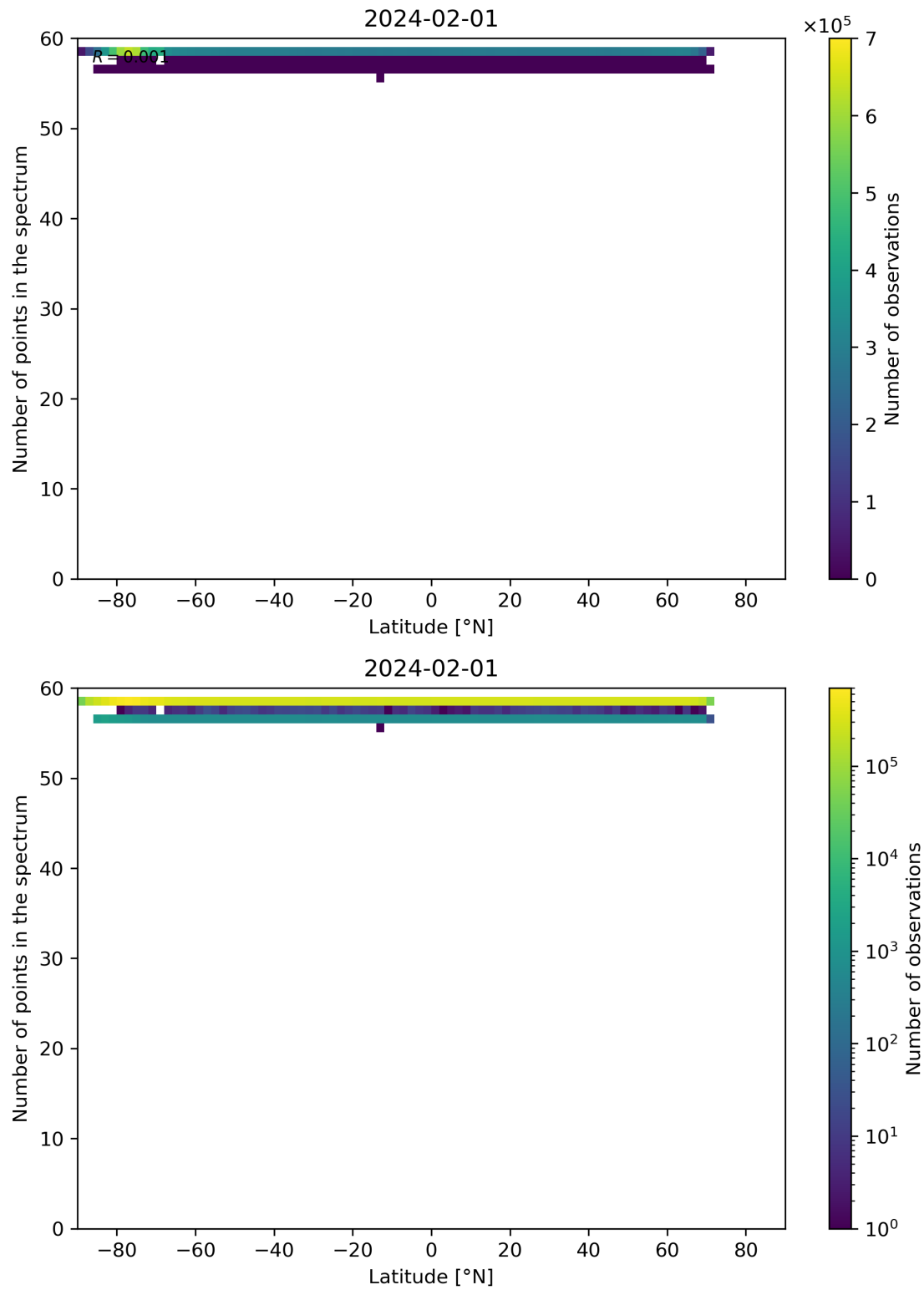
Figure 94: Scatter density plot of “Latitude” against “Number of points in the spectrum” for 2024-01-31 to 2024-02-02.
