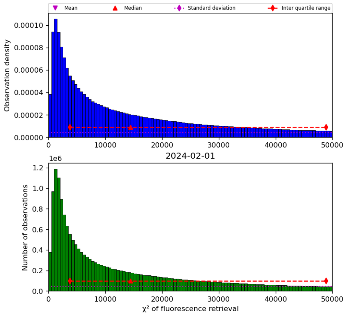
Figure 42: Histogram of “ \chi^2 of fluorescence retrieval” for 2024-01-31 to 2024-02-02
