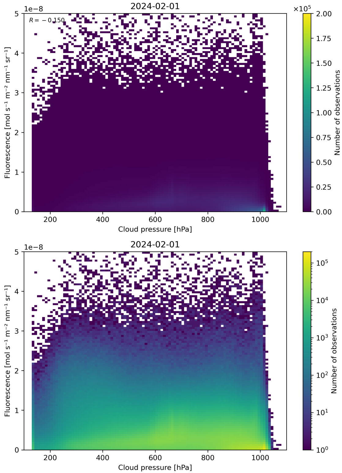
Figure 80: Scatter density plot of “Cloud pressure” against “Fluorescence” for 2024-01-31 to 2024-02-02.
