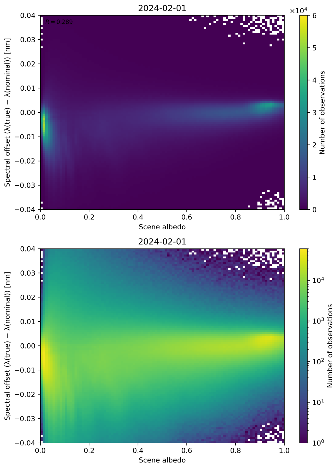
Figure 107: Scatter density plot of “Scene albedo” against “Spectral offset ( \lambda(\text{true}) - \lambda(\text{nominal}) )” for 2024-01-31 to 2024-02-02.
