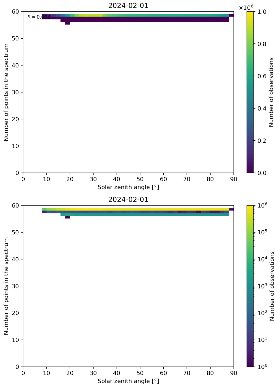
Figure 115: Scatter density plot of “Solar zenith angle” against “Number of points in the spectrum” for 2024-01-31 to 2024-02-02.
