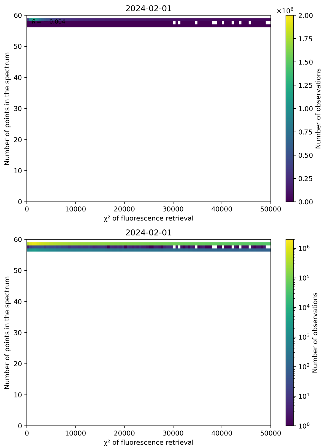
Figure 68: Scatter density plot of " \chi^2 of fluorescence retrieval" against "Number of points in the spectrum" for 2024-01-31 to 2024-02-02.
