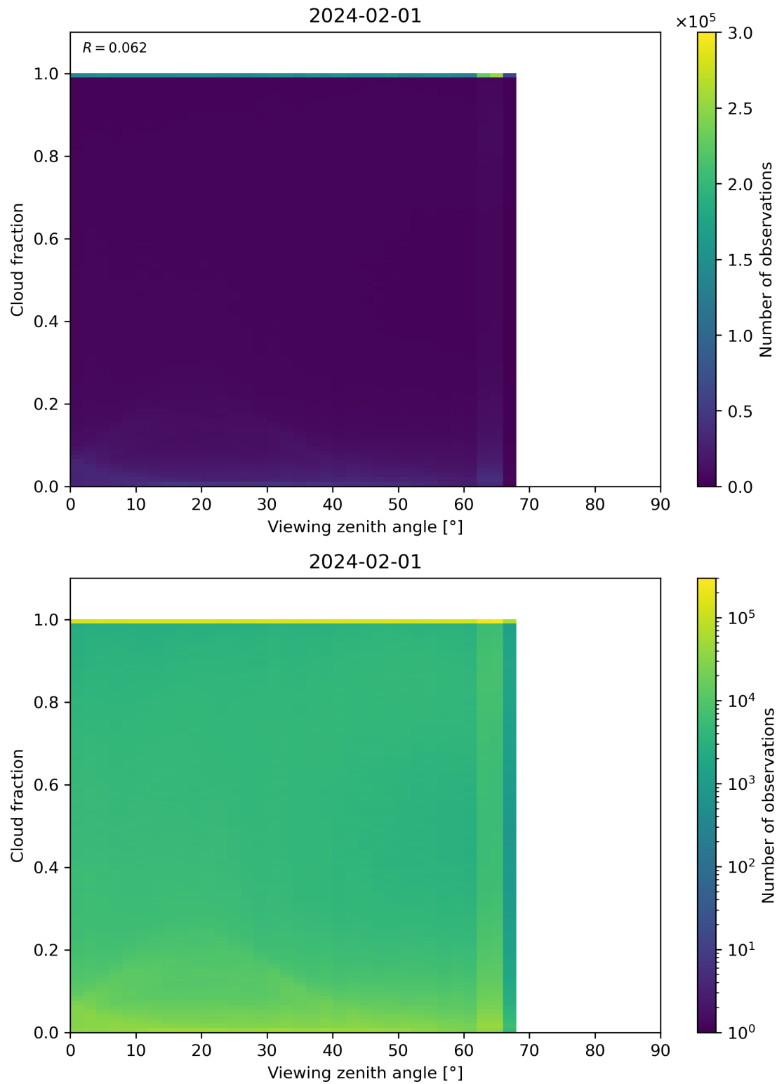
Figure 120: Scatter density plot of “Viewing zenith angle” against “Cloud fraction” for 2024-01-31 to 2024-02-02.
