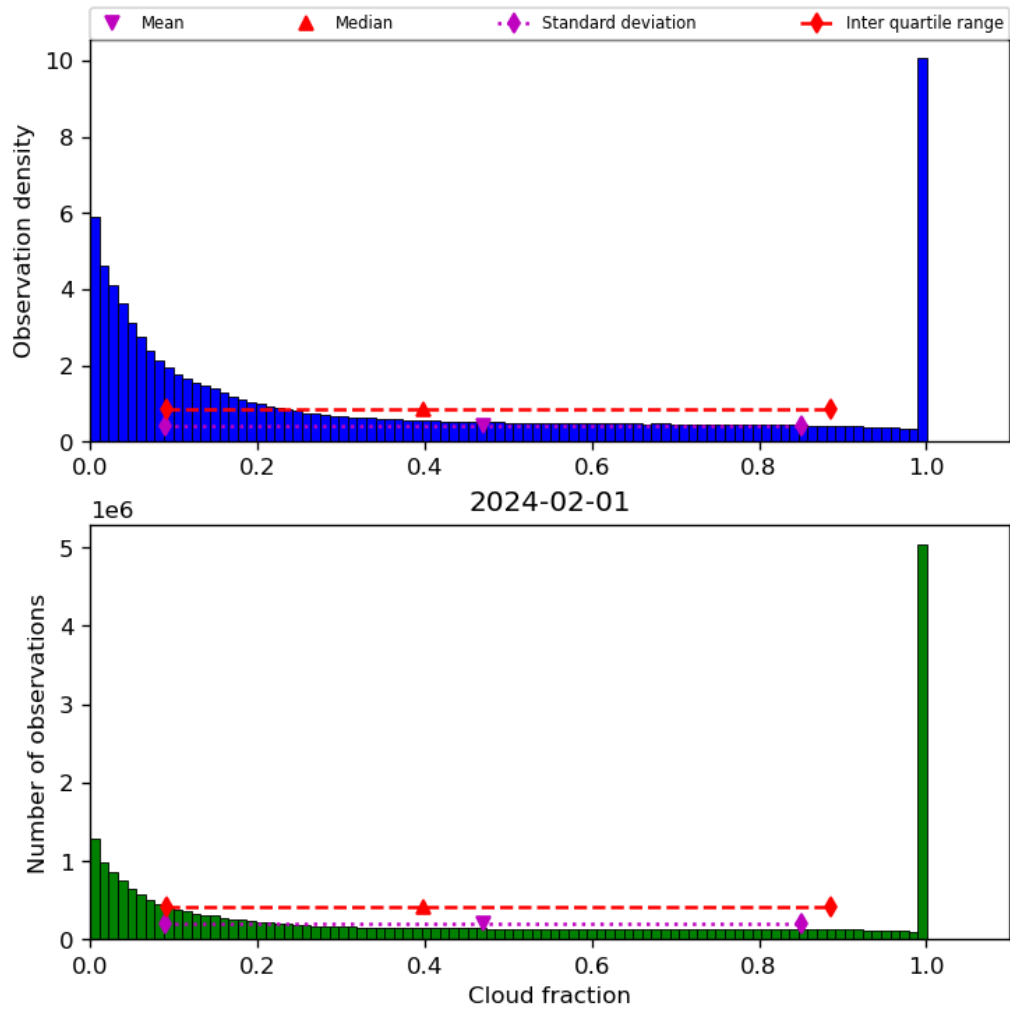
Figure 32: Histogram of “Cloud fraction” for 2024-01-31 to 2024-02-02
