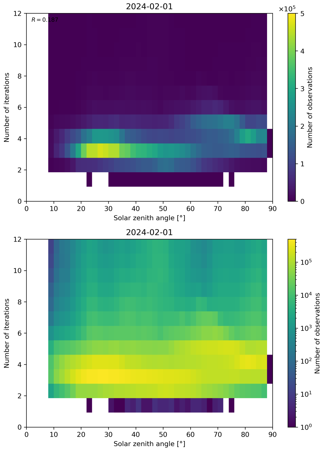
Figure 114: Scatter density plot of “Solar zenith angle” against “Number of iterations” for 2024-01-31 to 2024-02-02.
