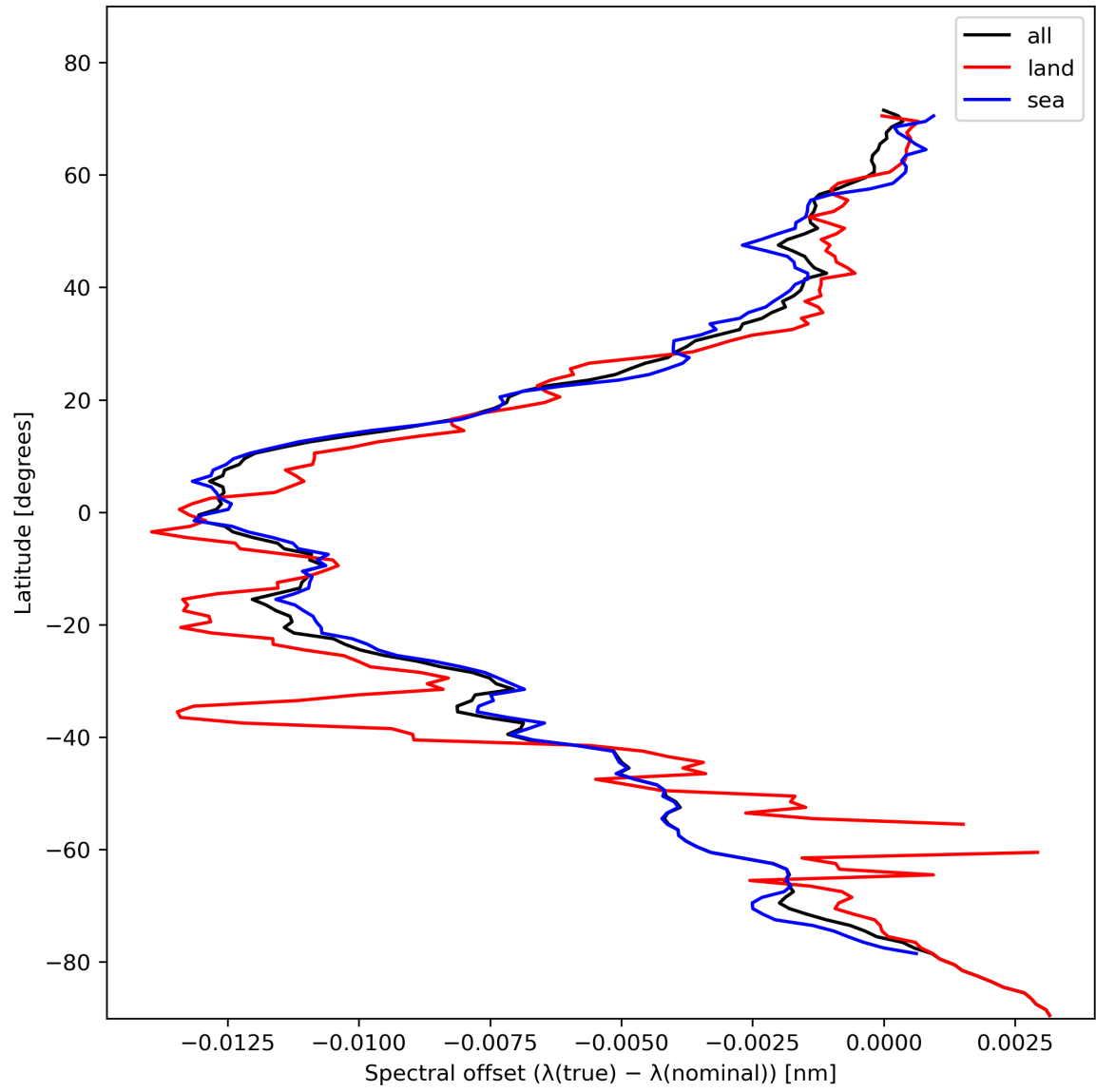
Figure 28: Zonal average of “Spectral offset ( \lambda(\text{true}) - \lambda(\text{nominal}) )” for 2024-01-31 to 2024-02-02.
