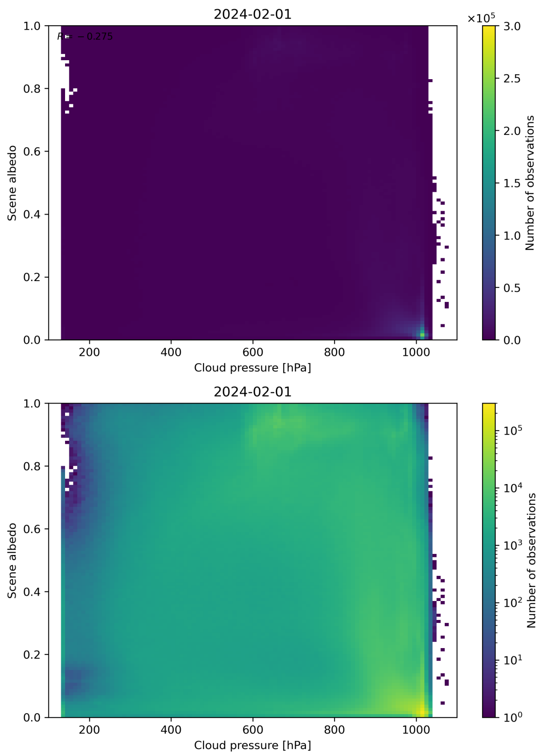
Figure 83: Scatter density plot of “Cloud pressure” against “Scene albedo” for 2024-01-31 to 2024-02-02.
