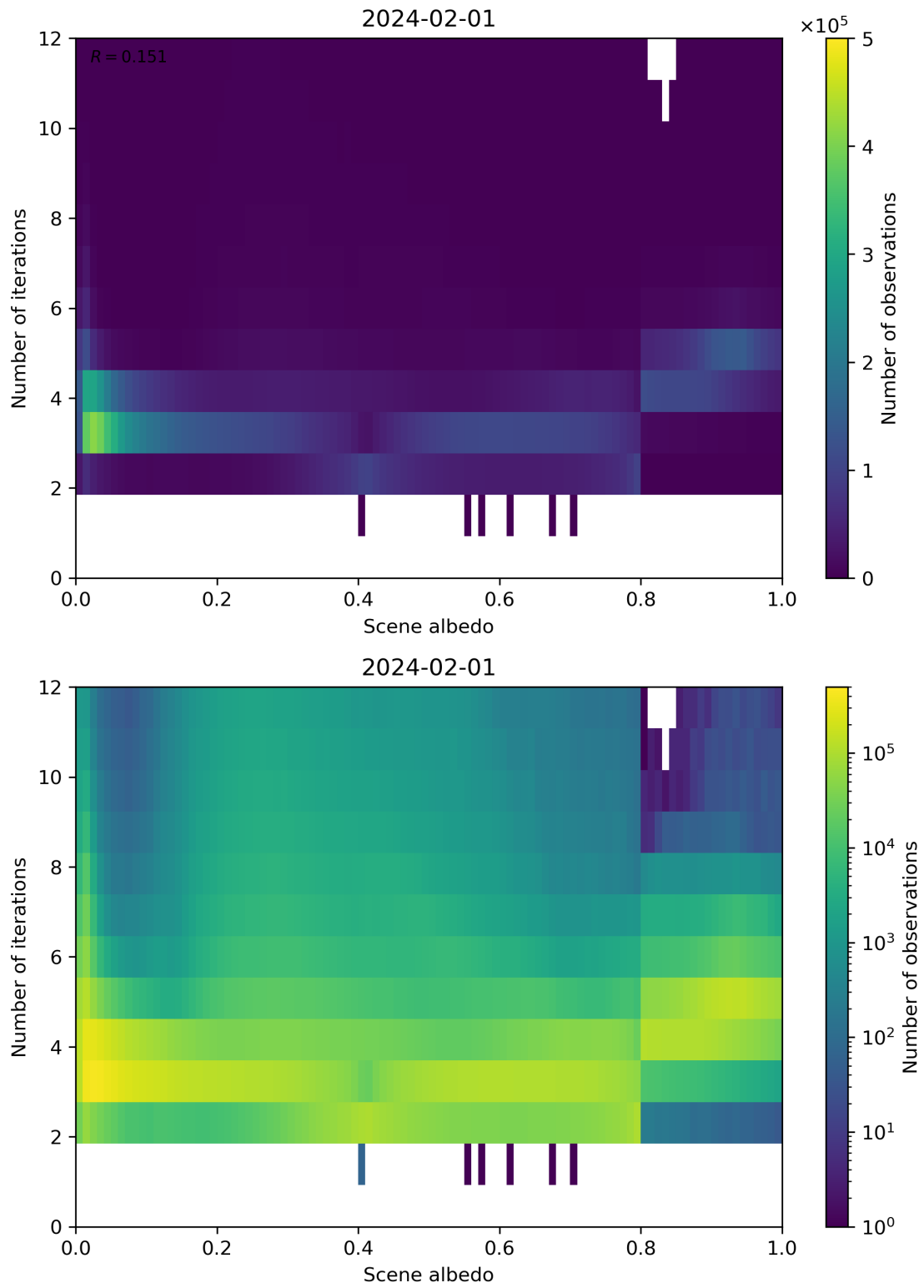
Figure 105: Scatter density plot of “Scene albedo” against “Number of iterations” for 2024-01-31 to 2024-02-02.
