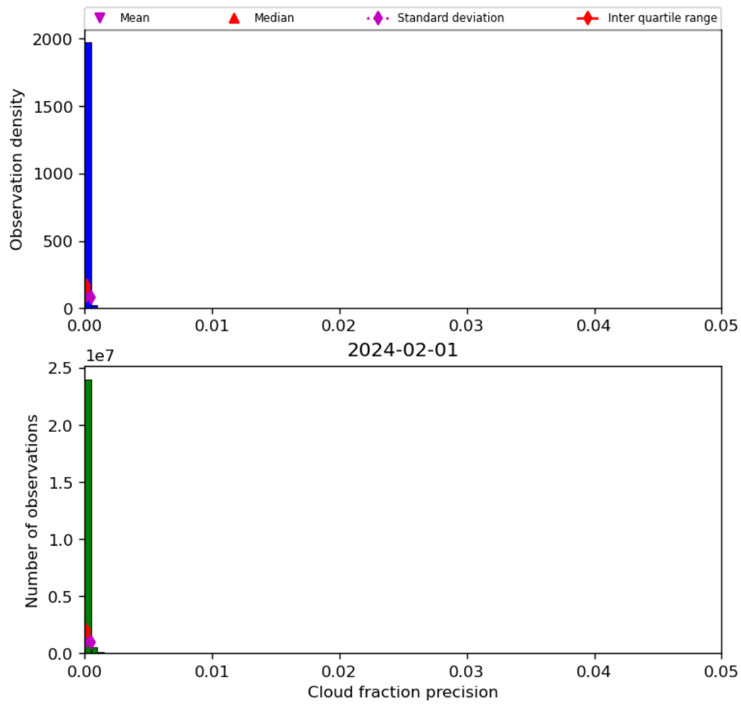
Figure 33: Histogram of “Cloud fraction precision” for 2024-01-31 to 2024-02-02
