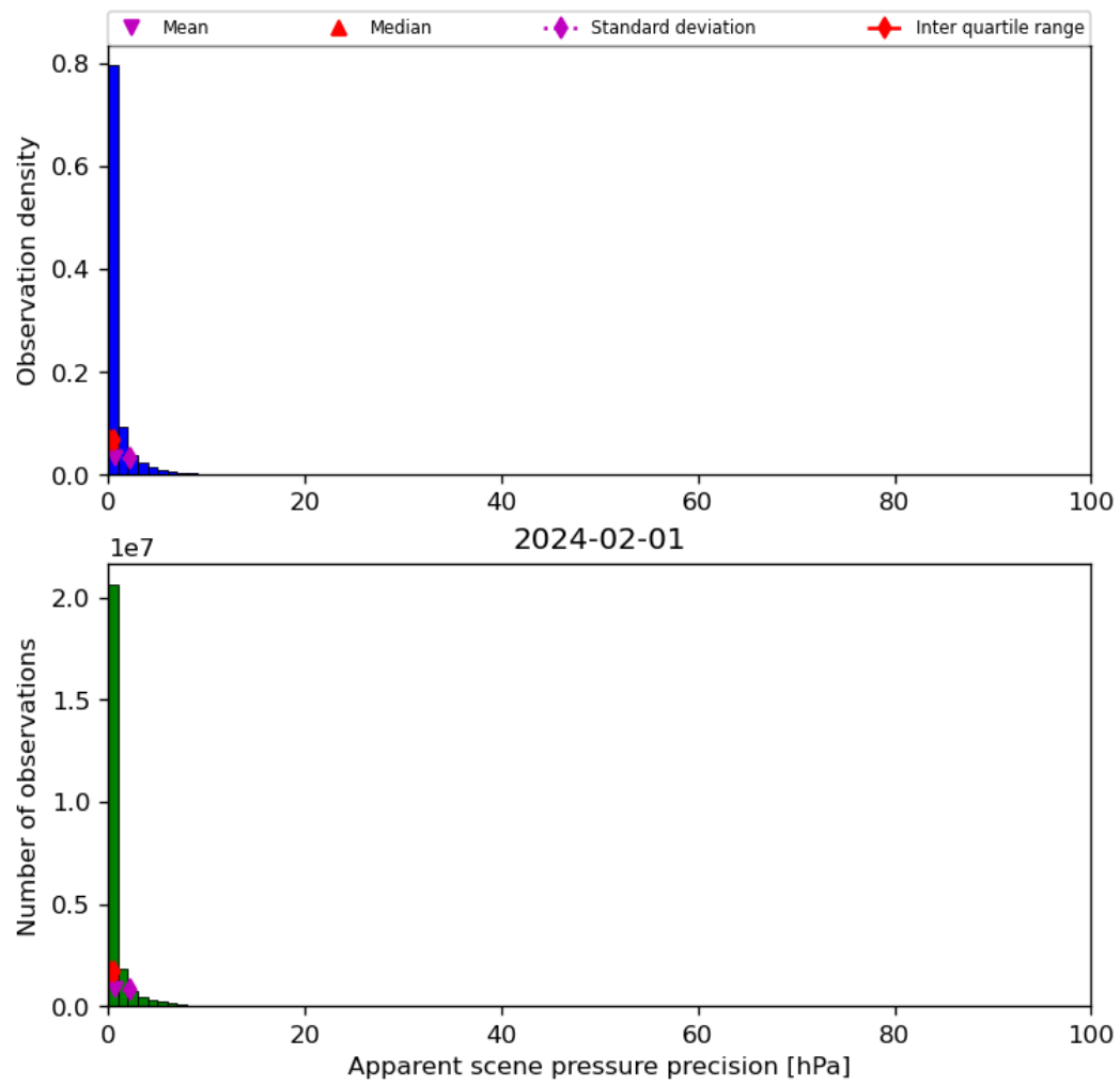
Figure 37: Histogram of “Apparent scene pressure precision” for 2024-01-31 to 2024-02-02
