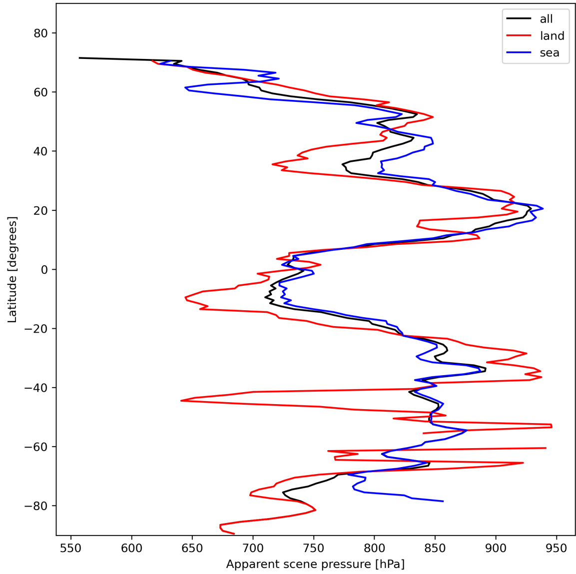
Figure 19: Zonal average of “Apparent scene pressure” for 2024-01-31 to 2024-02-02.
