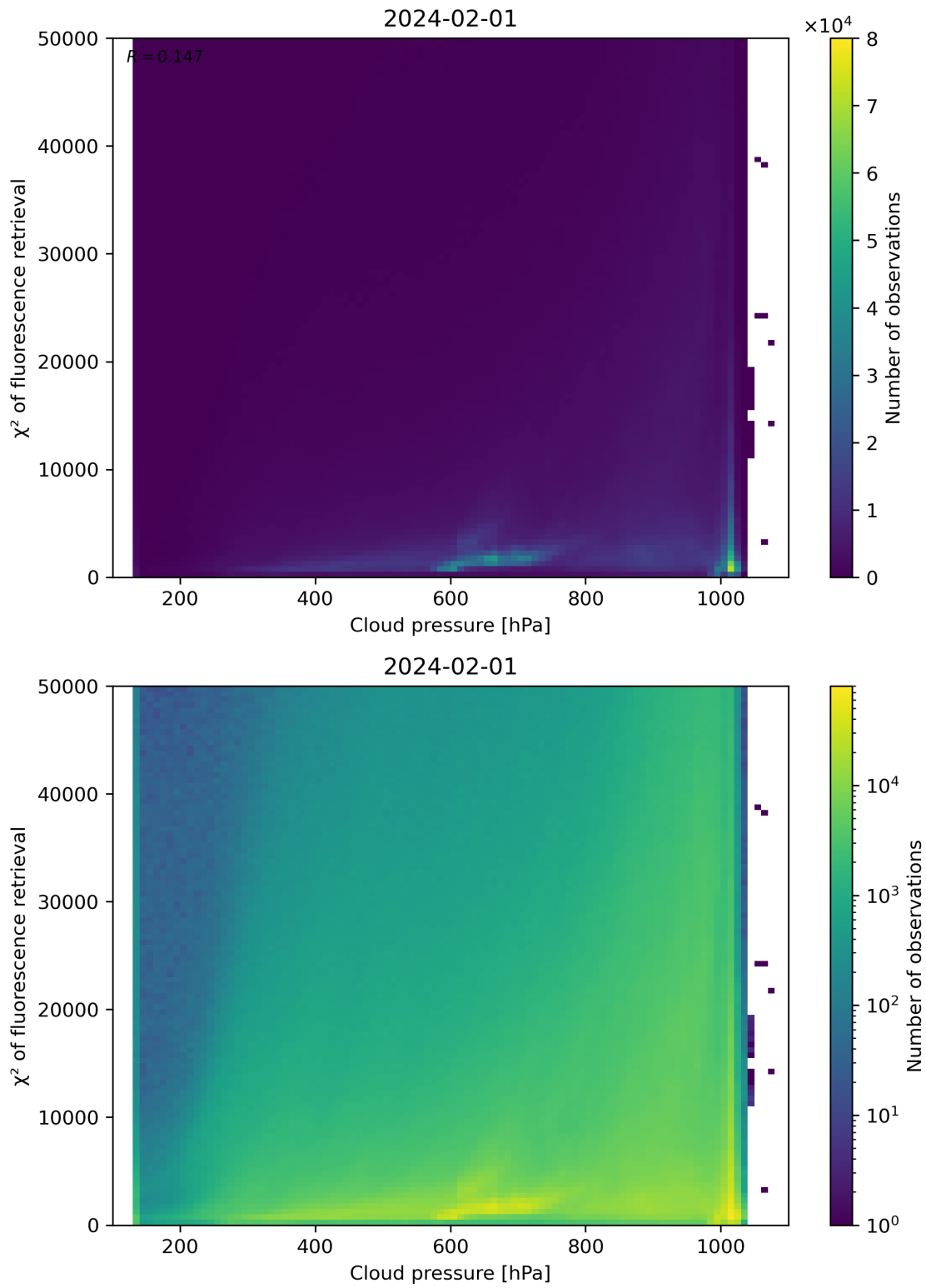
Figure 78: Scatter density plot of “Cloud pressure” against “ \chi^2 of fluorescence retrieval” for 2024-01-31 to 2024-02-02.
