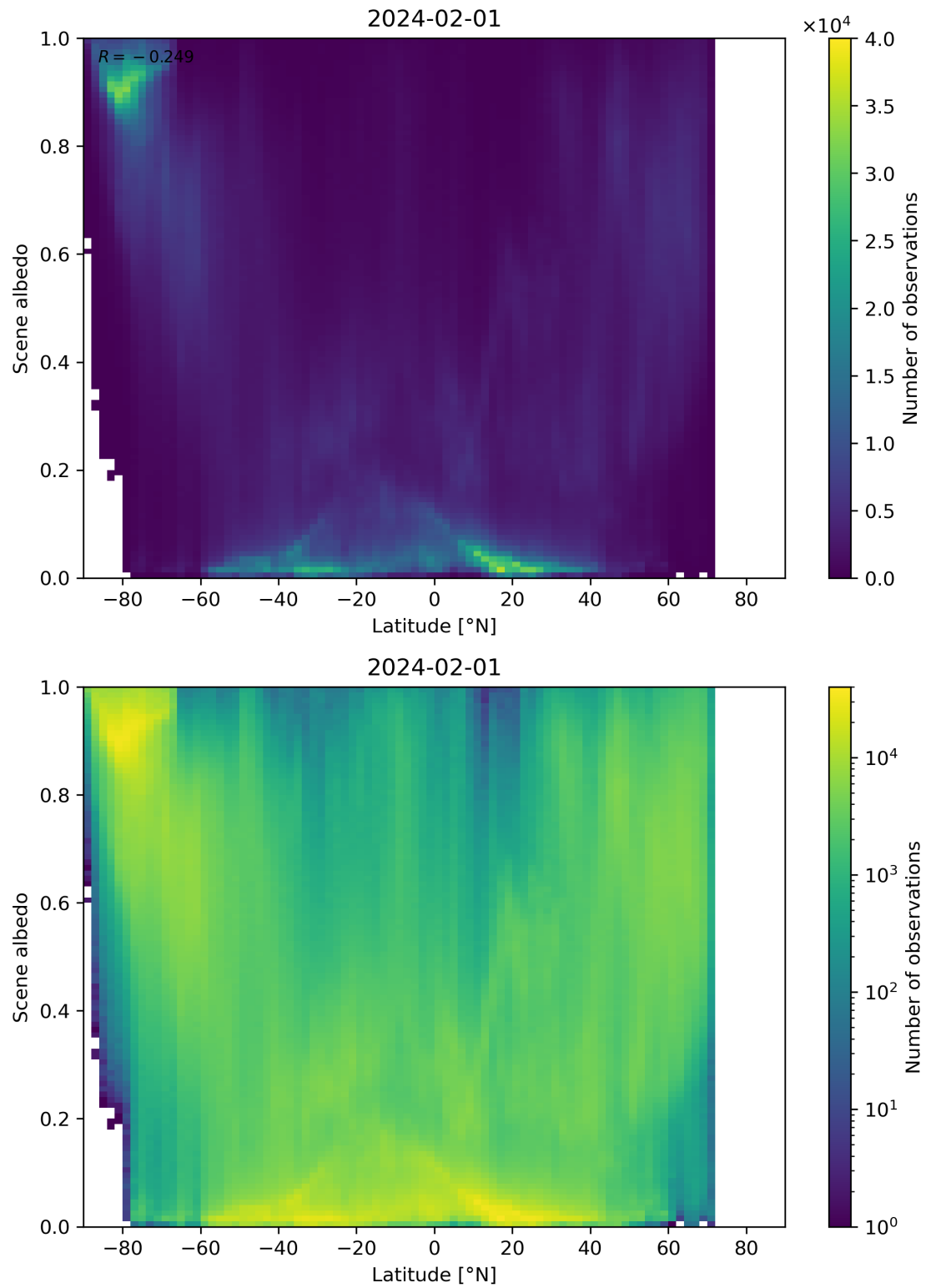
Figure 95: Scatter density plot of “Latitude” against “Scene albedo” for 2024-01-31 to 2024-02-02.
