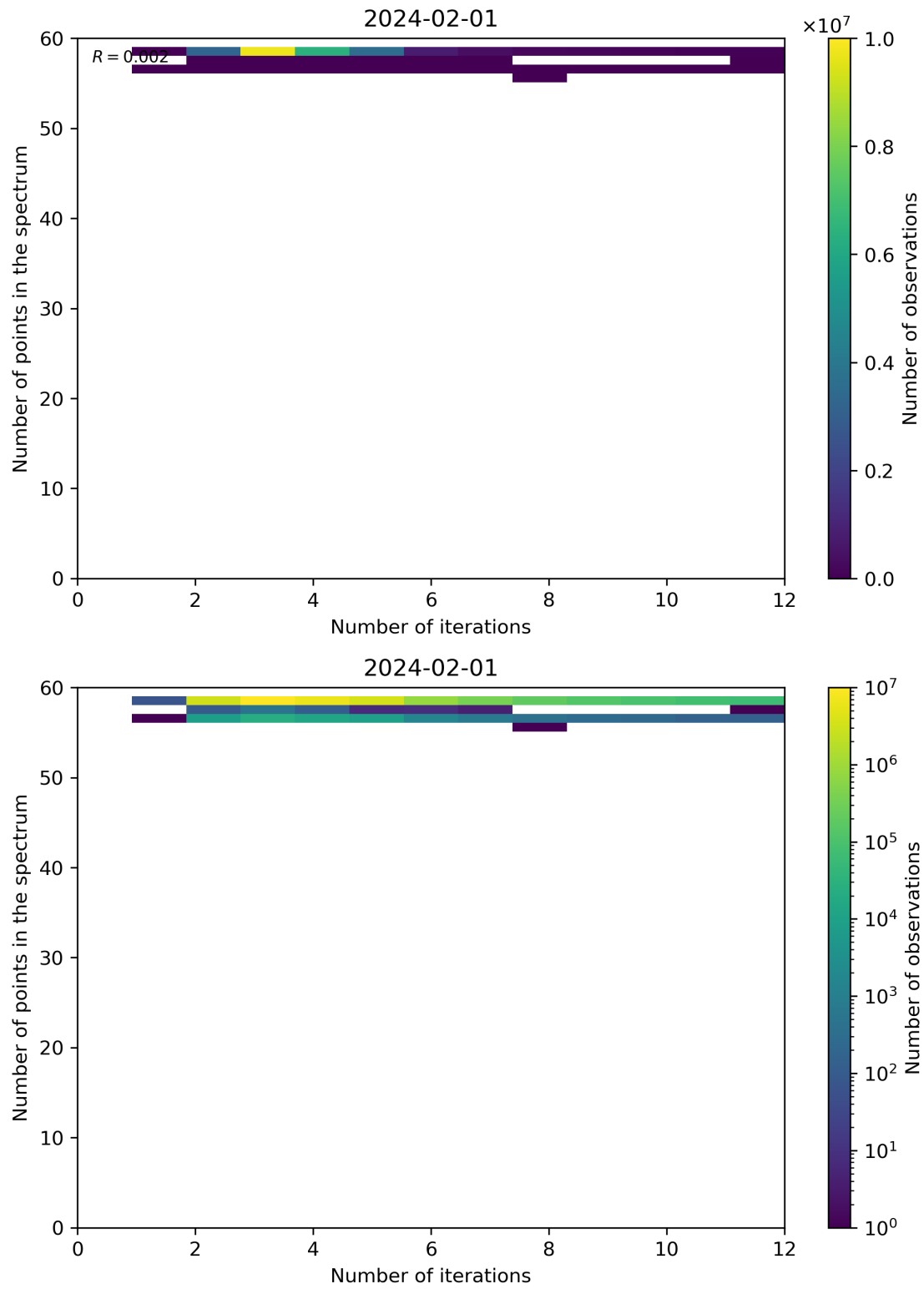
Figure 99: Scatter density plot of “Number of iterations” against “Number of points in the spectrum” for 2024-01-31 to 2024-02-02.
