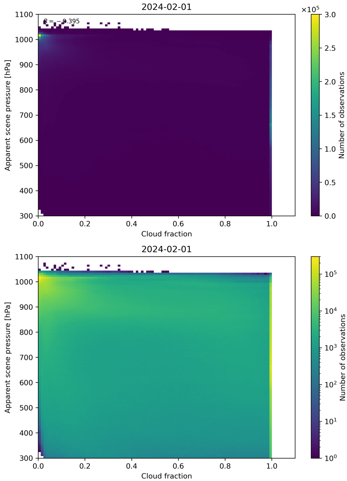
Figure 70: Scatter density plot of “Cloud fraction” against “Apparent scene pressure” for 2024-01-31 to 2024-02-02.
