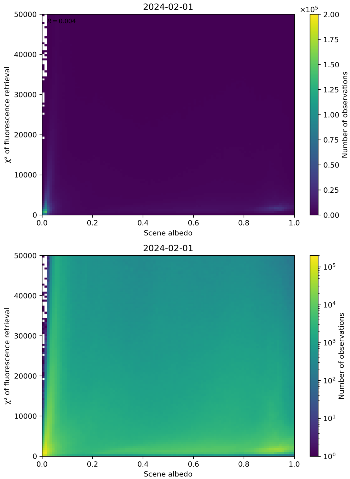
Figure 103: Scatter density plot of “Scene albedo” against “ \chi^2 of fluorescence retrieval” for 2024-01-31 to 2024-02-02.
