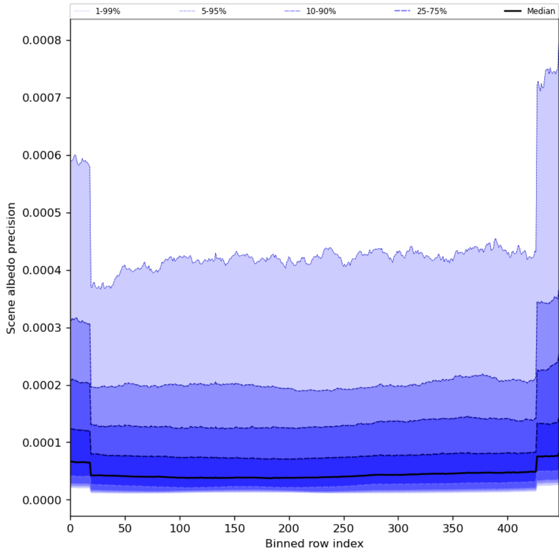
Figure 52: Along track statistics of “Scene albedo precision” for 2024-01-31 to 2024-02-02
