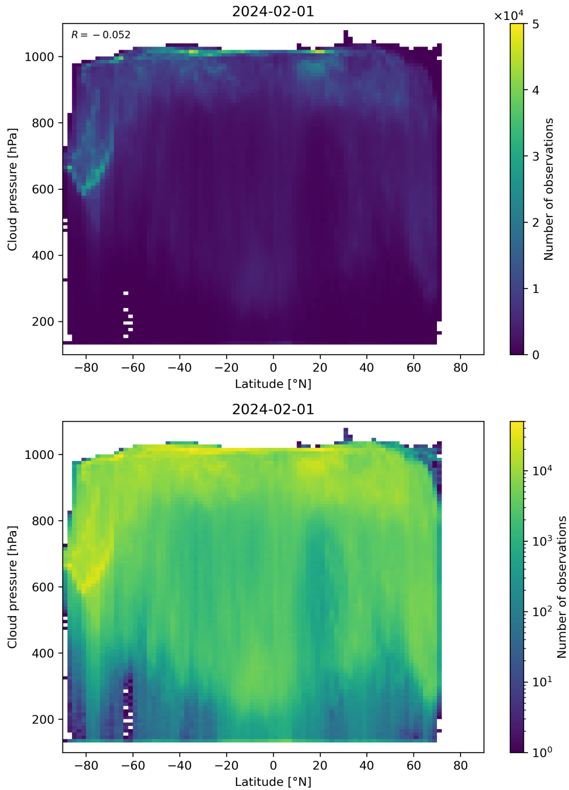
Figure 91: Scatter density plot of “Latitude” against “Cloud pressure” for 2024-01-31 to 2024-02-02.
