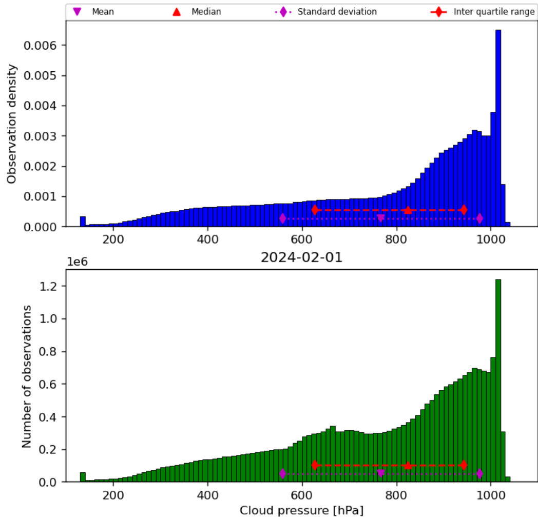
Figure 30: Histogram of “Cloud pressure” for 2024-01-31 to 2024-02-02
