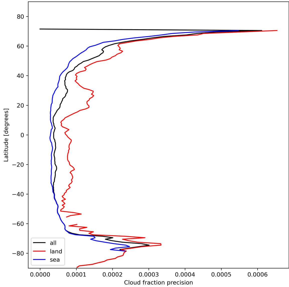
Figure 16: Zonal average of “Cloud fraction precision” for 2024-01-31 to 2024-02-02.
