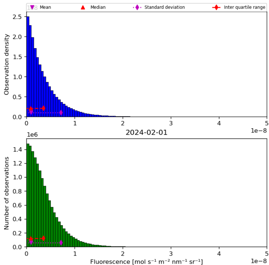
Figure 40: Histogram of “Fluorescence” for 2024-01-31 to 2024-02-02
