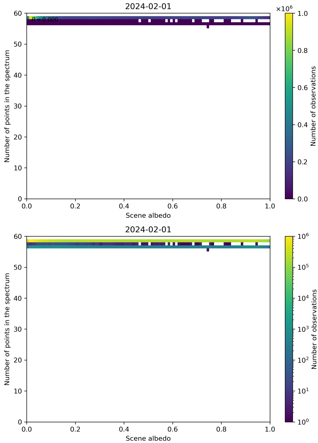
Figure 106: Scatter density plot of “Scene albedo” against “Number of points in the spectrum” for 2024-01-31 to 2024-02-02.
