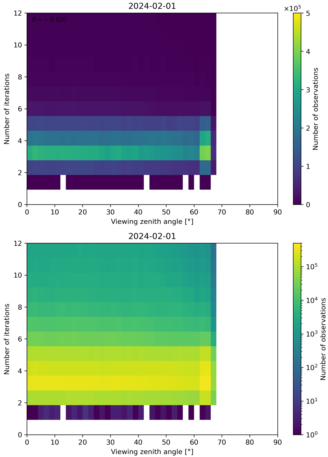
Figure 124: Scatter density plot of “Viewing zenith angle” against “Number of iterations” for 2024-01-31 to 2024-02-02.
