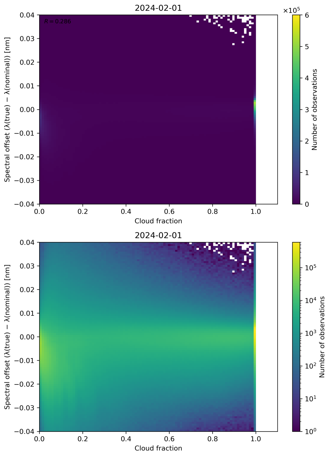
Figure 76: Scatter density plot of “Cloud fraction” against “Spectral offset ( \lambda(\text{true}) - \lambda(\text{nominal}) )” for 2024-01-31 to 2024-02-02.
