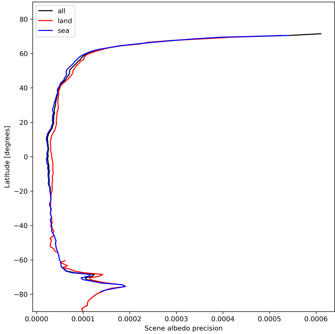
Figure 18: Zonal average of “Scene albedo precision” for 2024-01-31 to 2024-02-02.
