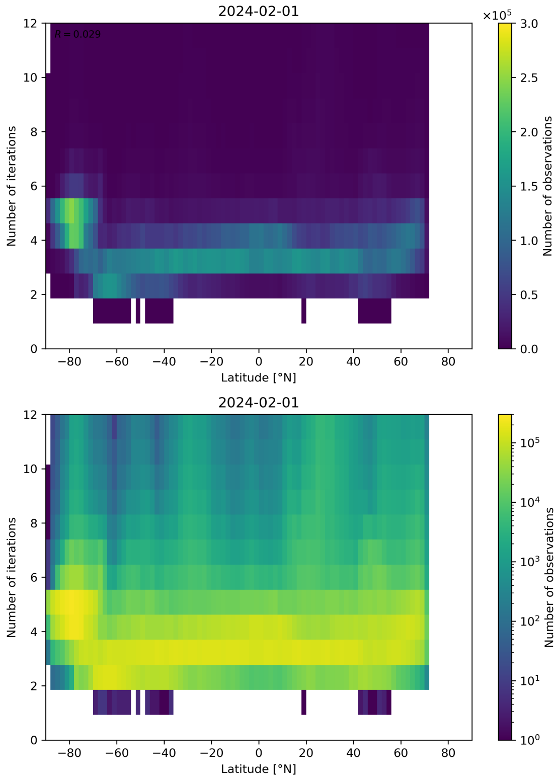
Figure 93: Scatter density plot of “Latitude” against “Number of iterations” for 2024-01-31 to 2024-02-02.
