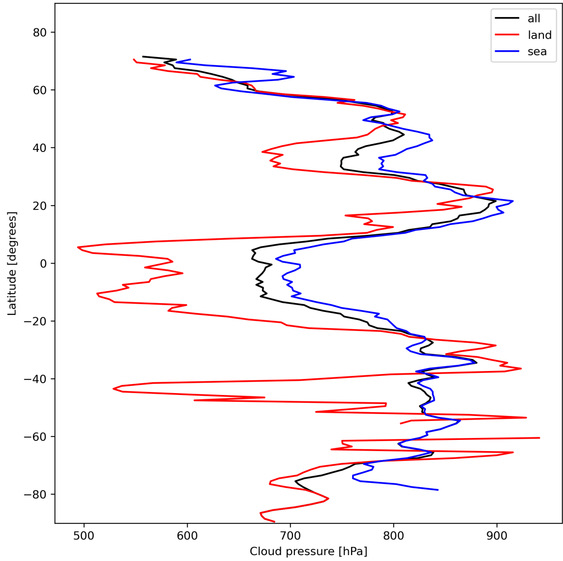
Figure 13: Zonal average of “Cloud pressure” for 2024-01-31 to 2024-02-02.
