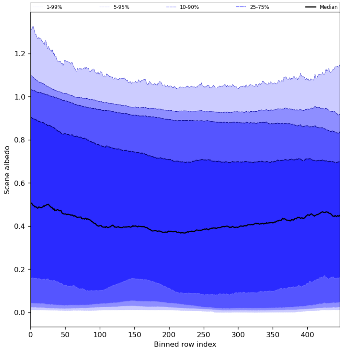
Figure 51: Along track statistics of “Scene albedo” for 2024-01-31 to 2024-02-02
