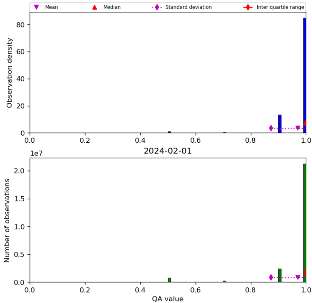
Figure 29: Histogram of “QA value” for 2024-01-31 to 2024-02-02
