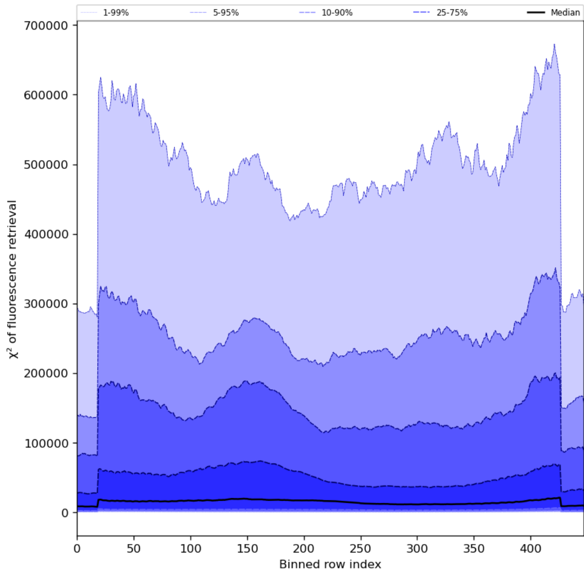
Figure 59: Along track statistics of “ \chi^2 of fluorescence retrieval” for 2024-01-31 to 2024-02-02
