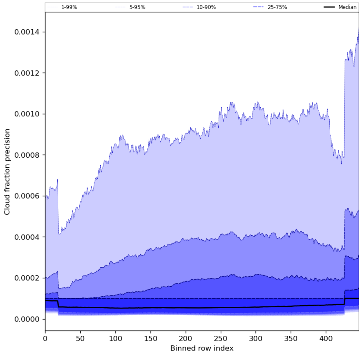
Figure 50: Along track statistics of “Cloud fraction precision” for 2024-01-31 to 2024-02-02
