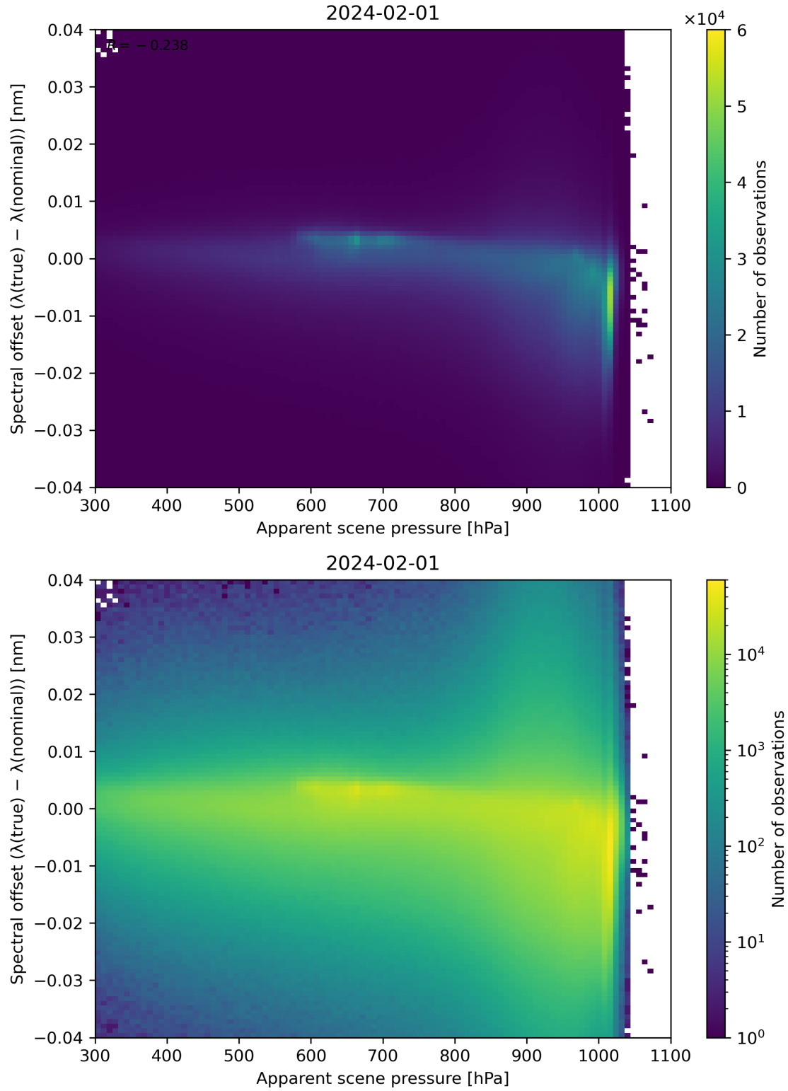
Figure 67: Scatter density plot of “Apparent scene pressure” against “Spectral offset ( \lambda(\text{true}) - \lambda(\text{nominal}) )” for 2024-01-31 to 2024-02-02.
