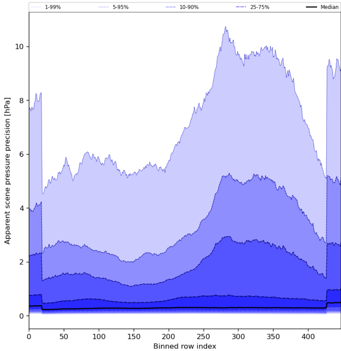
Figure 54: Along track statistics of “Apparent scene pressure precision” for 2024-01-31 to 2024-02-02
