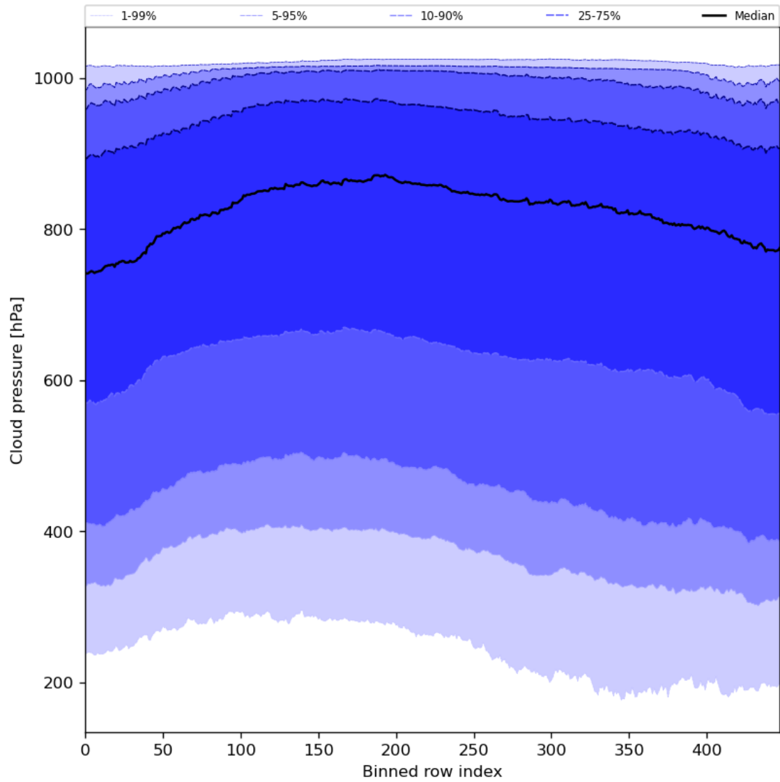
Figure 47: Along track statistics of “Cloud pressure” for 2024-01-31 to 2024-02-02
