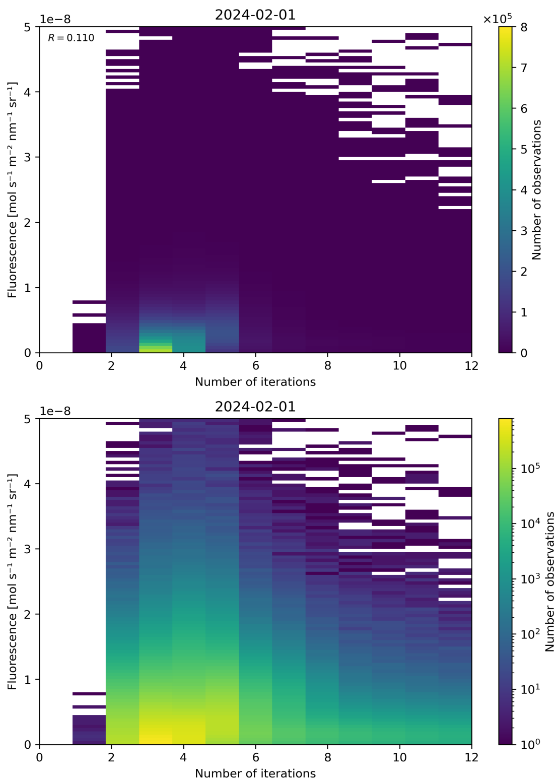
Figure 98: Scatter density plot of “Number of iterations” against “Fluorescence” for 2024-01-31 to 2024-02-02.
