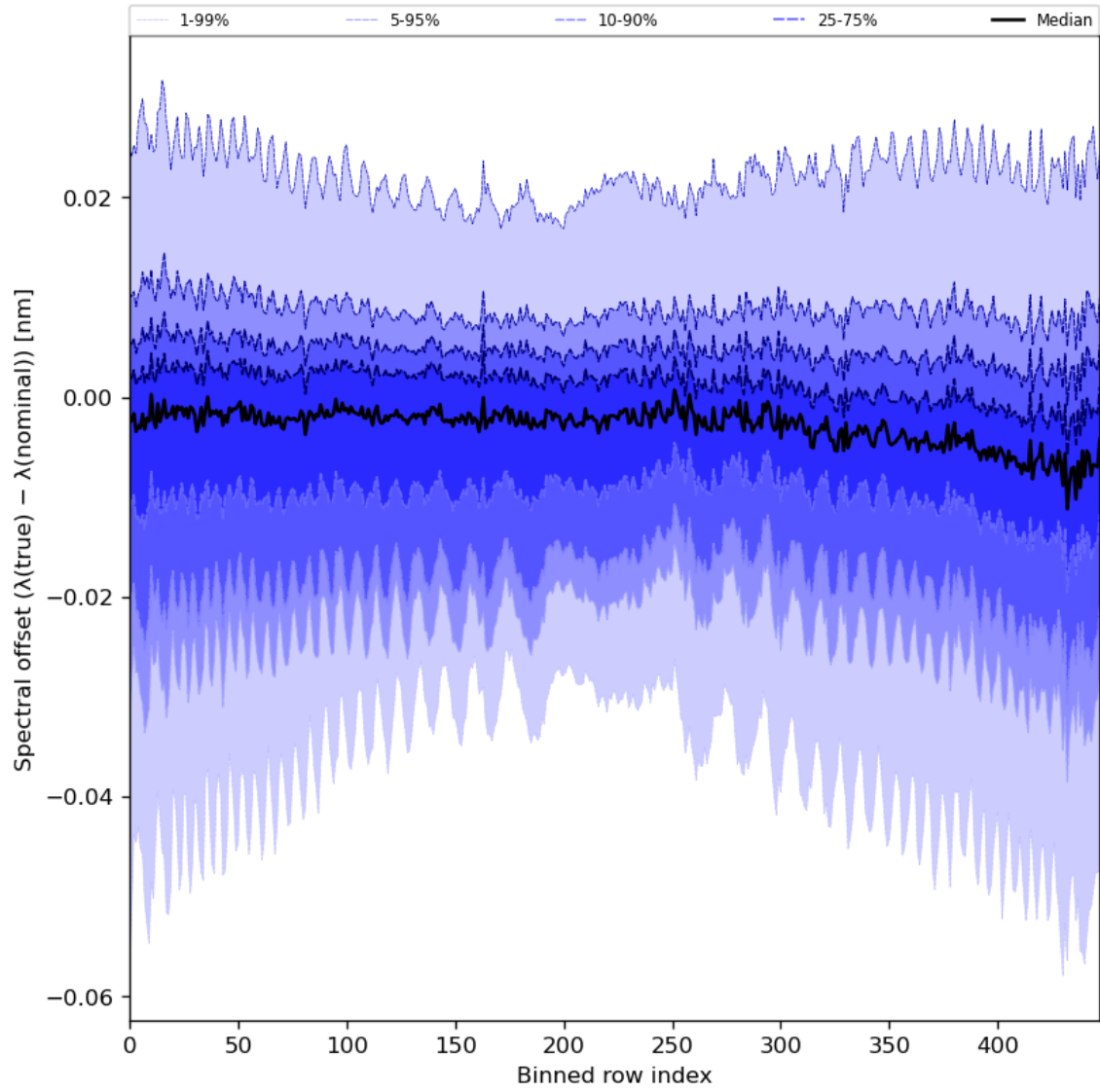
Figure 62: Along track statistics of “Spectral offset ( \lambda(\text{true}) - \lambda(\text{nominal}) )” for 2024-01-31 to 2024-02-02
