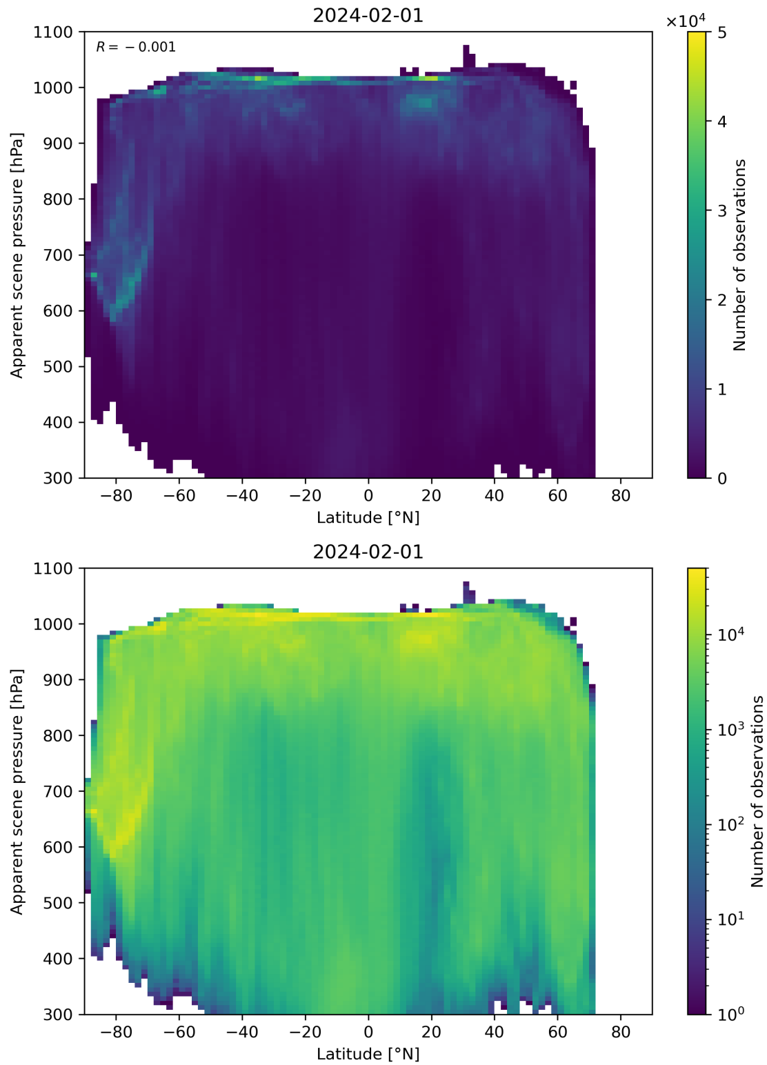
Figure 88: Scatter density plot of “Latitude” against “Apparent scene pressure” for 2024-01-31 to 2024-02-02.
