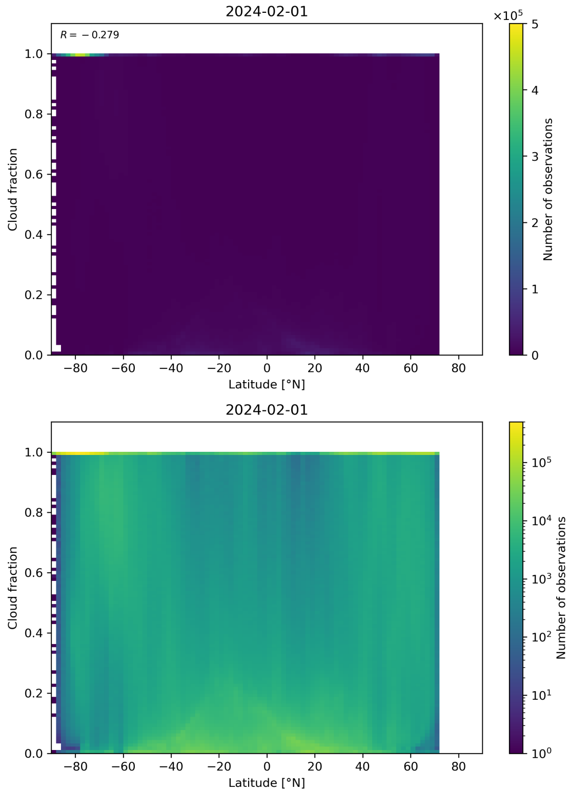
Figure 90: Scatter density plot of “Latitude” against “Cloud fraction” for 2024-01-31 to 2024-02-02.
