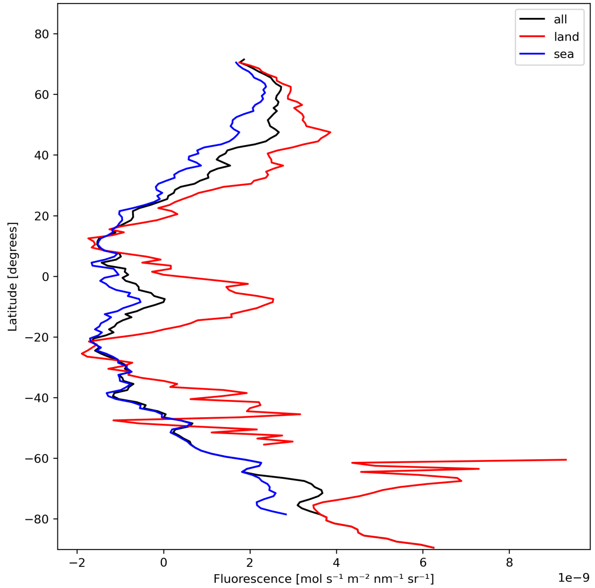
Figure 23: Zonal average of “Fluorescence” for 2024-01-31 to 2024-02-02.
