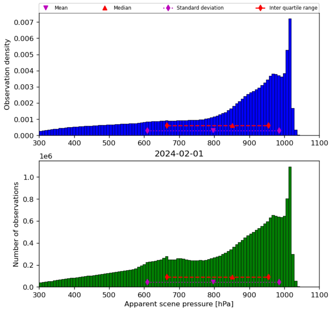
Figure 36: Histogram of “Apparent scene pressure” for 2024-01-31 to 2024-02-02
