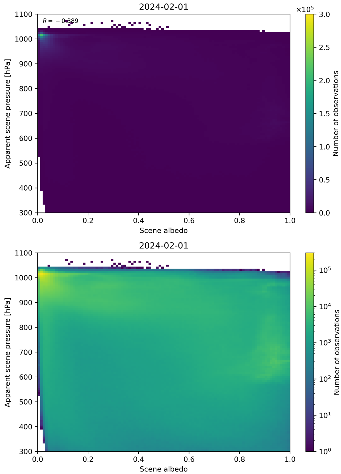
Figure 102: Scatter density plot of “Scene albedo” against “Apparent scene pressure” for 2024-01-31 to 2024-02-02.
