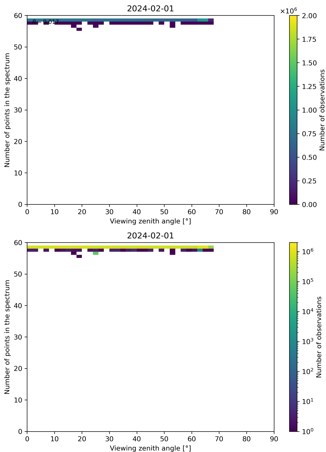
Figure 125: Scatter density plot of “Viewing zenith angle” against “Number of points in the spectrum” for 2024-01-31 to 2024-02-02.
