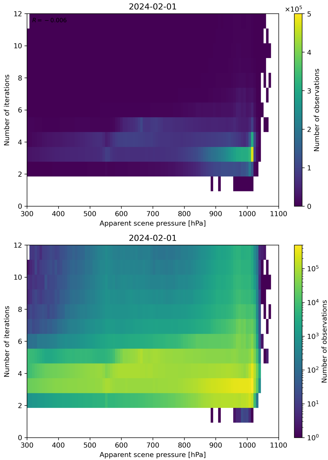
Figure 65: Scatter density plot of “Apparent scene pressure” against “Number of iterations” for 2024-01-31 to 2024-02-02.
