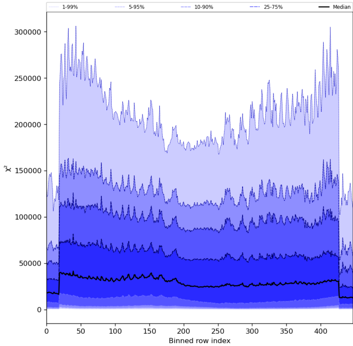
Figure 55: Along track statistics of “ \chi^2 ” for 2024-01-31 to 2024-02-02
