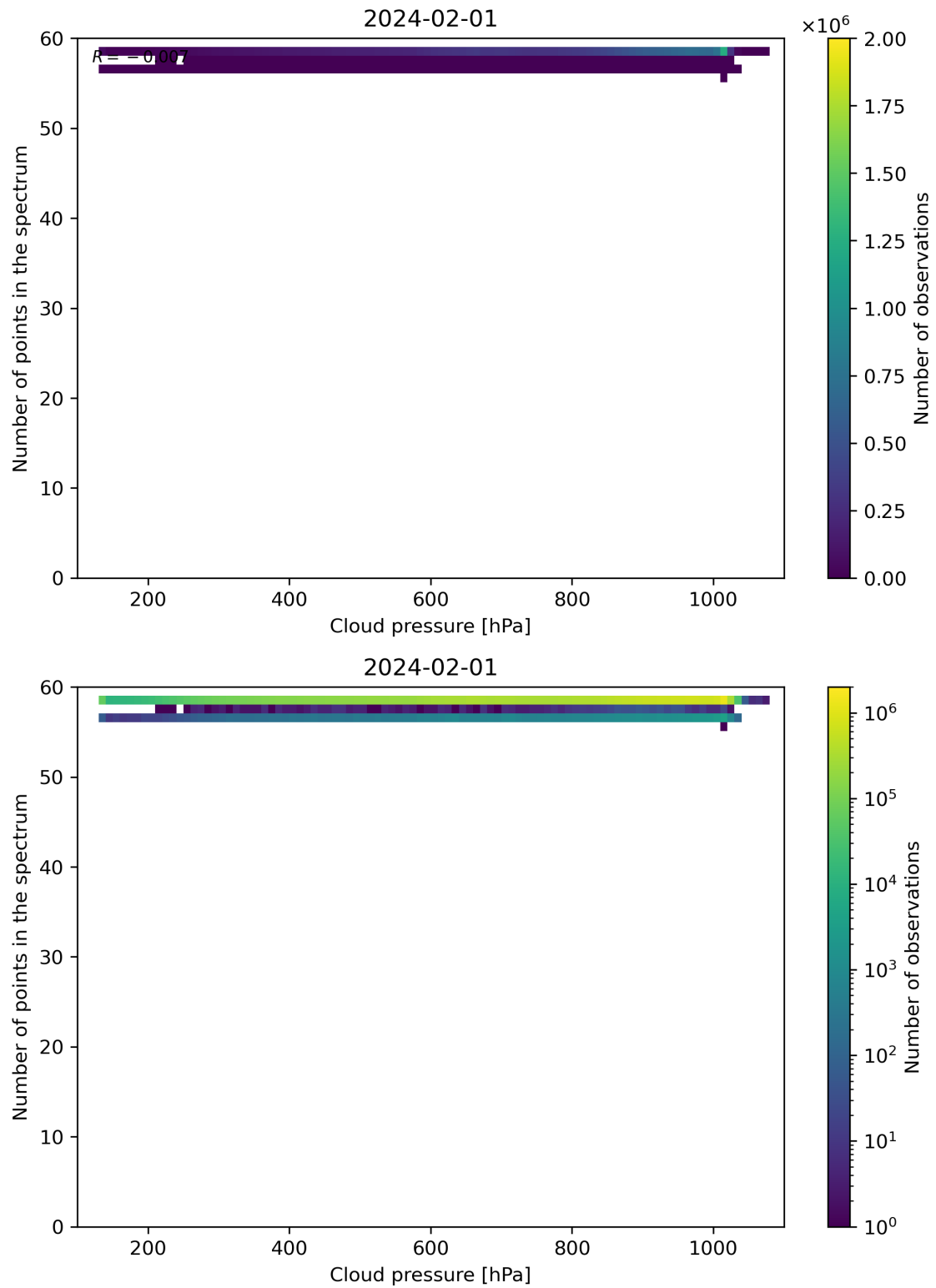
Figure 82: Scatter density plot of “Cloud pressure” against “Number of points in the spectrum” for 2024-01-31 to 2024-02-02.
