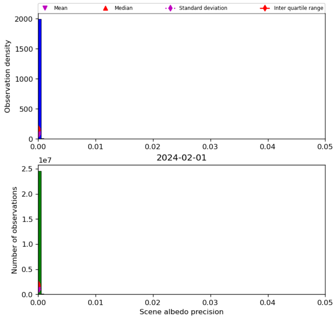
Figure 35: Histogram of “Scene albedo precision” for 2024-01-31 to 2024-02-02
