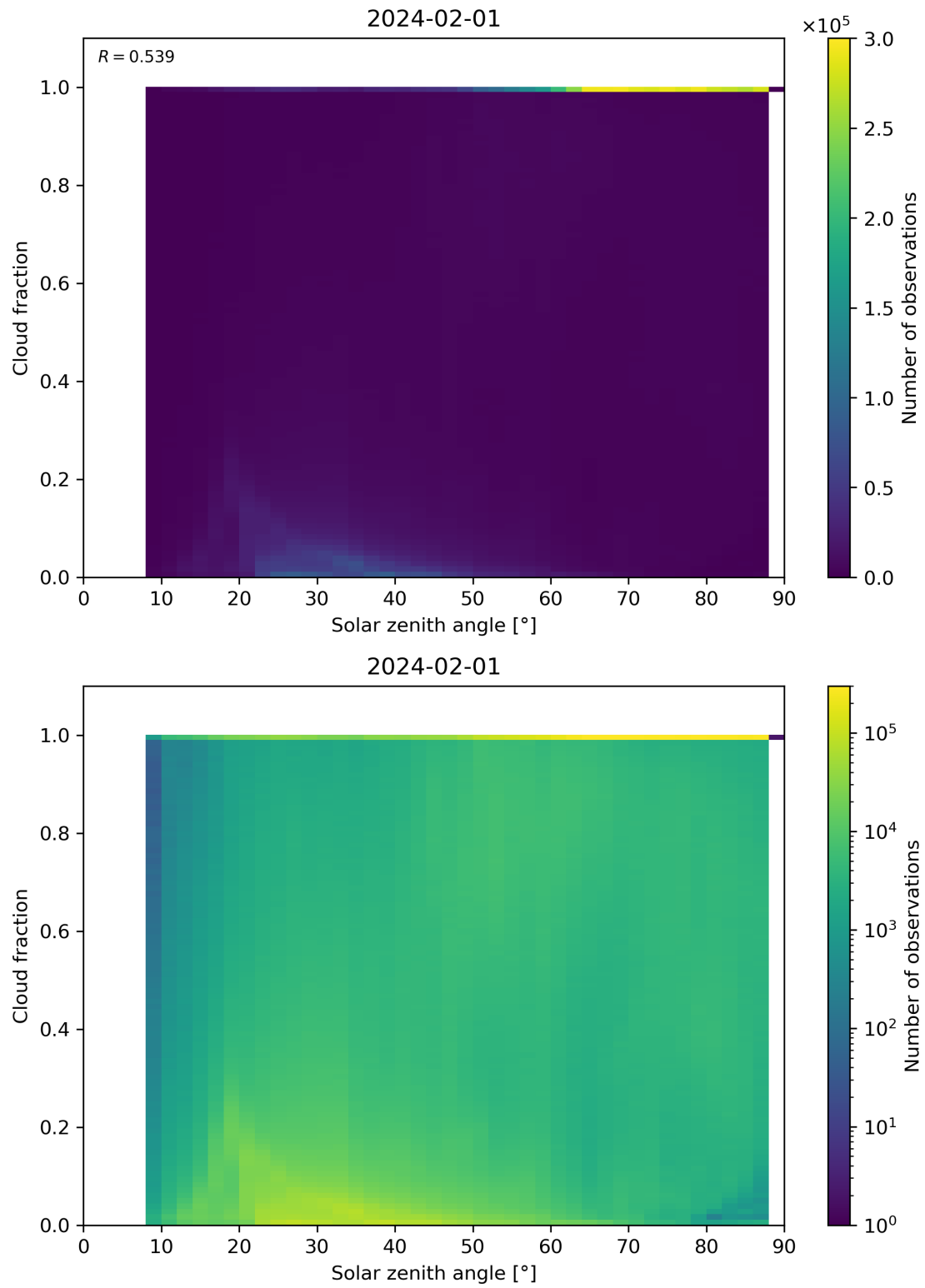
Figure 110: Scatter density plot of “Solar zenith angle” against “Cloud fraction” for 2024-01-31 to 2024-02-02.
