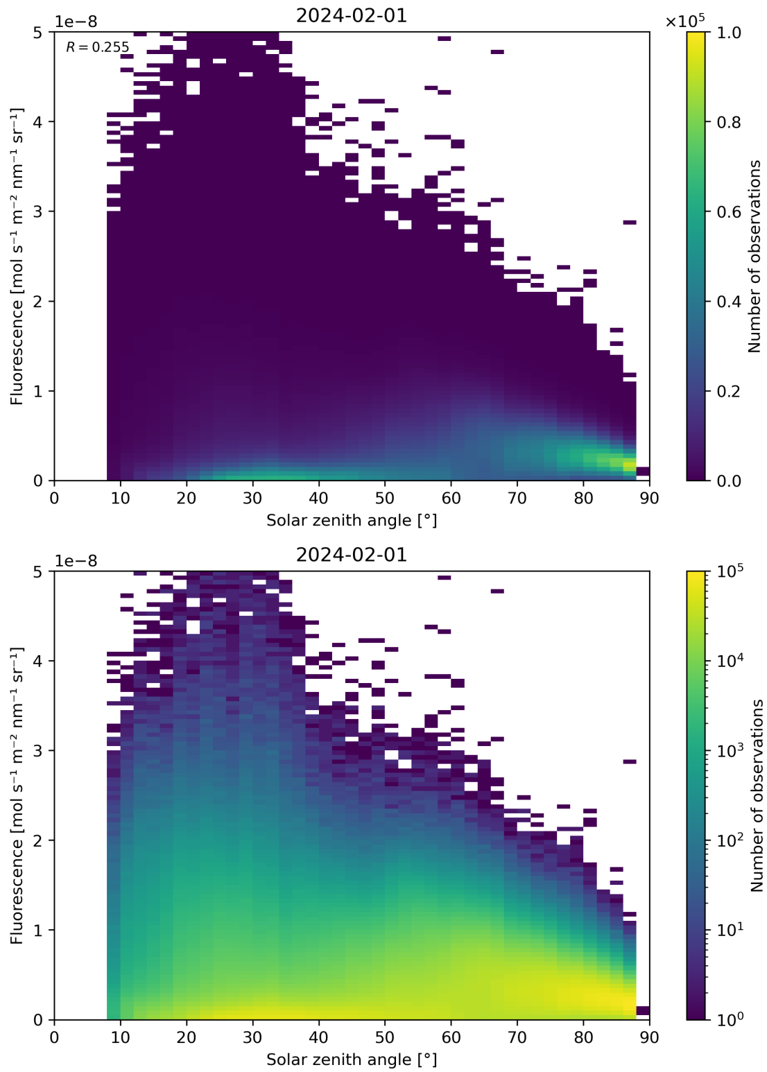
Figure 112: Scatter density plot of “Solar zenith angle” against “Fluorescence” for 2024-01-31 to 2024-02-02.
