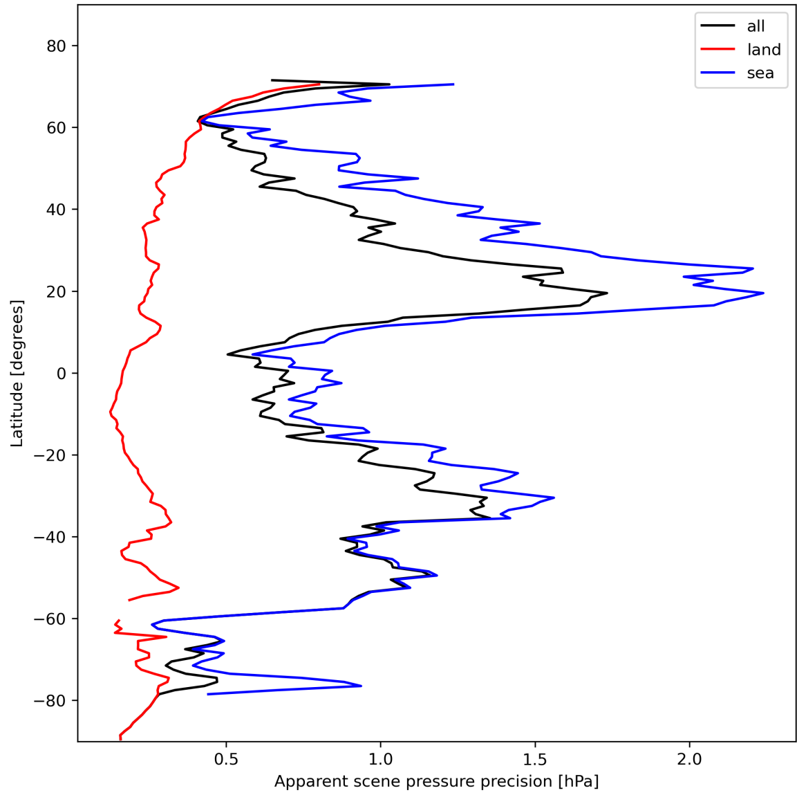
Figure 20: Zonal average of “Apparent scene pressure precision” for 2024-01-31 to 2024-02-02.
