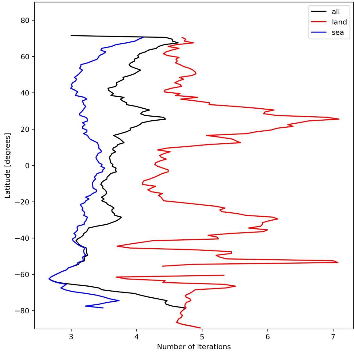
Figure 22: Zonal average of “Number of iterations” for 2024-01-31 to 2024-02-02.
