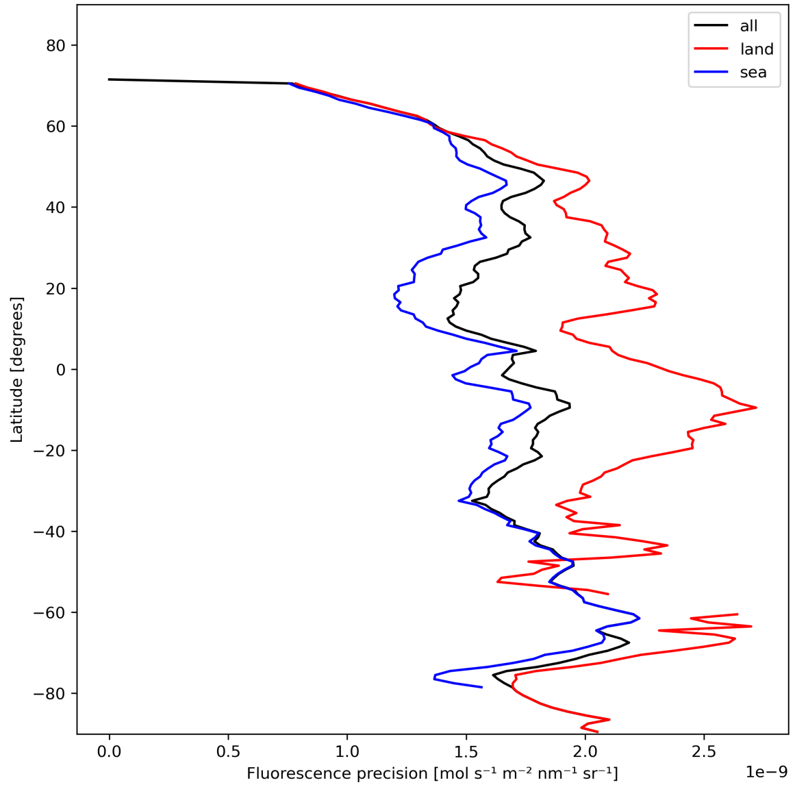
Figure 24: Zonal average of “Fluorescence precision” for 2024-01-31 to 2024-02-02.
