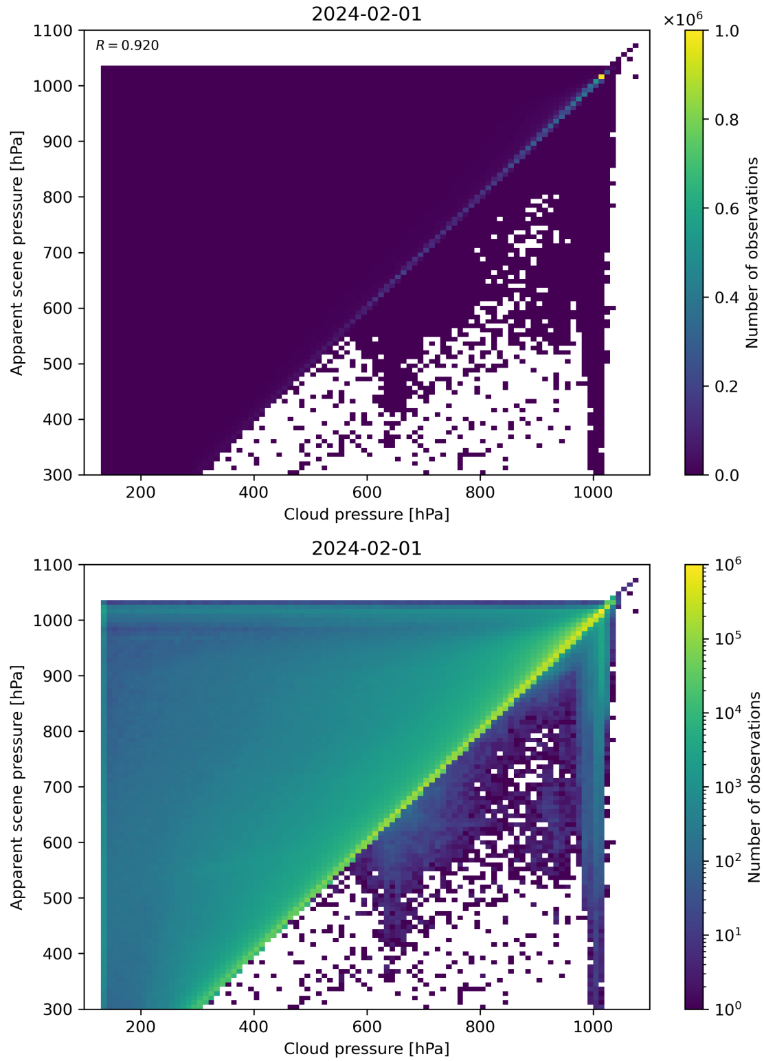
Figure 77: Scatter density plot of “Cloud pressure” against “Apparent scene pressure” for 2024-01-31 to 2024-02-02.
