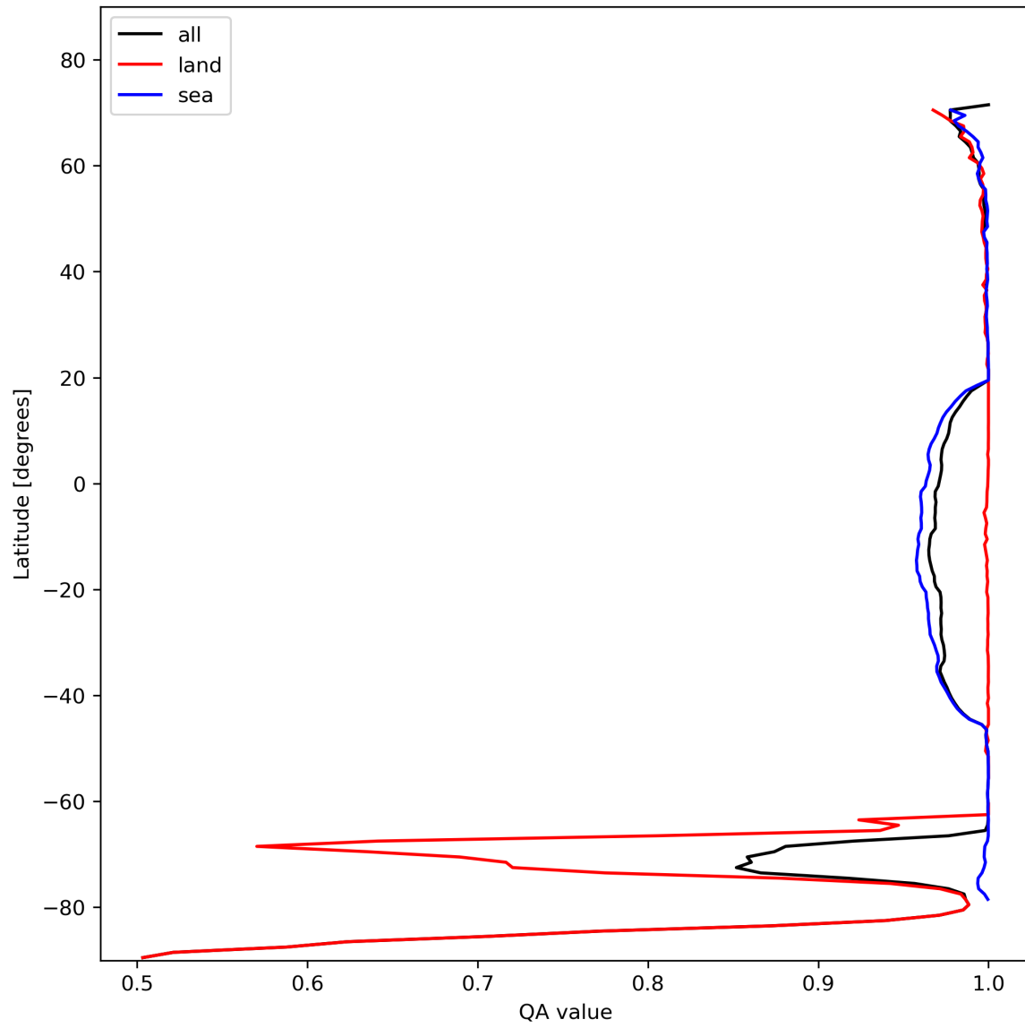
Figure 12: Zonal average of “QA value” for 2024-01-31 to 2024-02-02.
