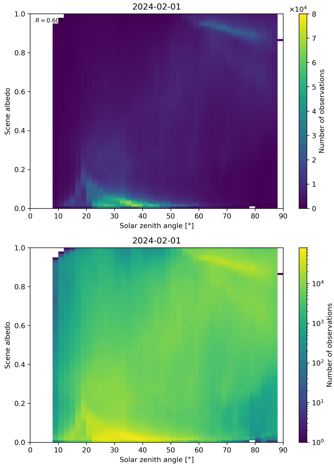
Figure 116: Scatter density plot of “Solar zenith angle” against “Scene albedo” for 2024-01-31 to 2024-02-02.
