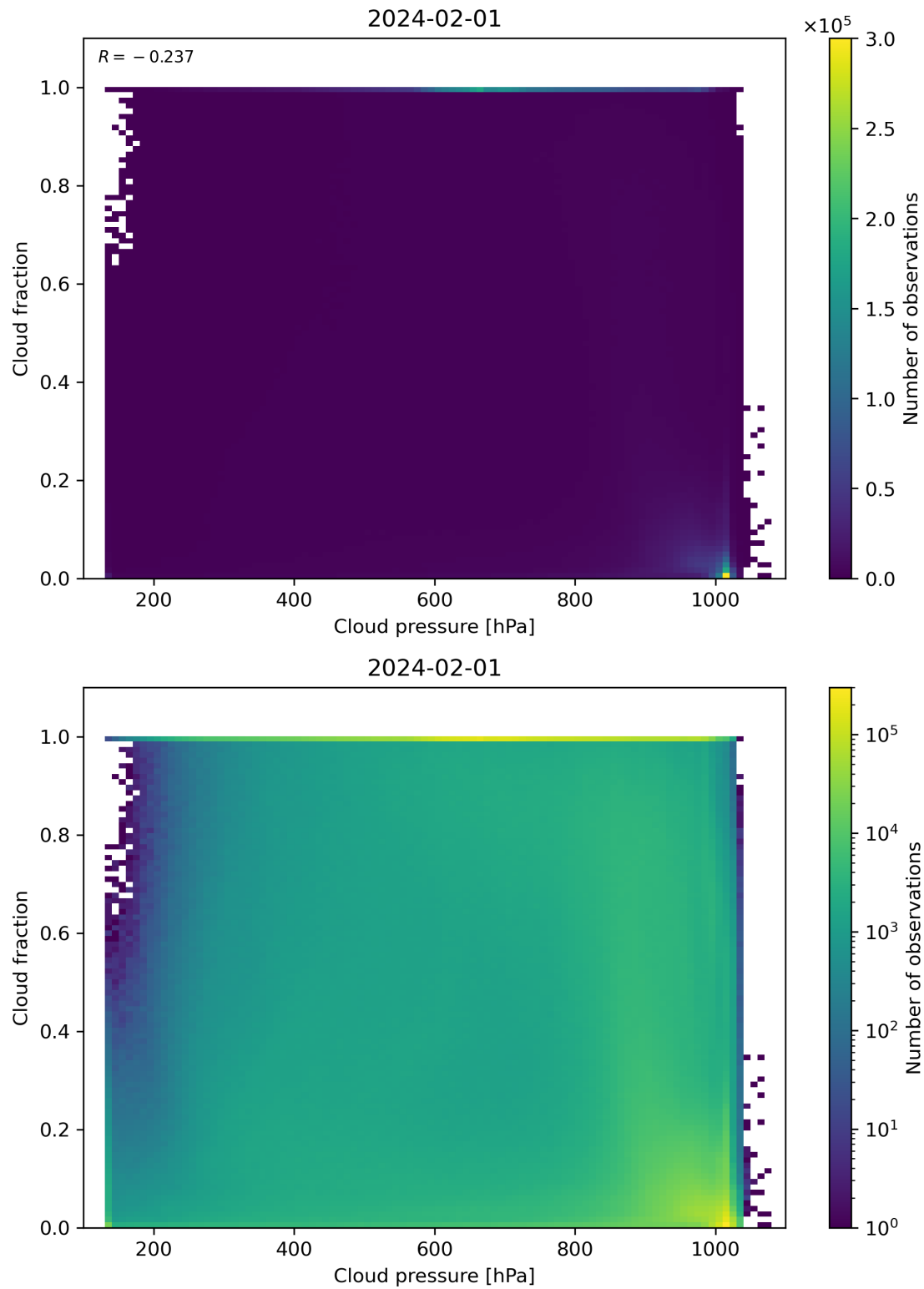
Figure 79: Scatter density plot of “Cloud pressure” against “Cloud fraction” for 2024-01-31 to 2024-02-02.
