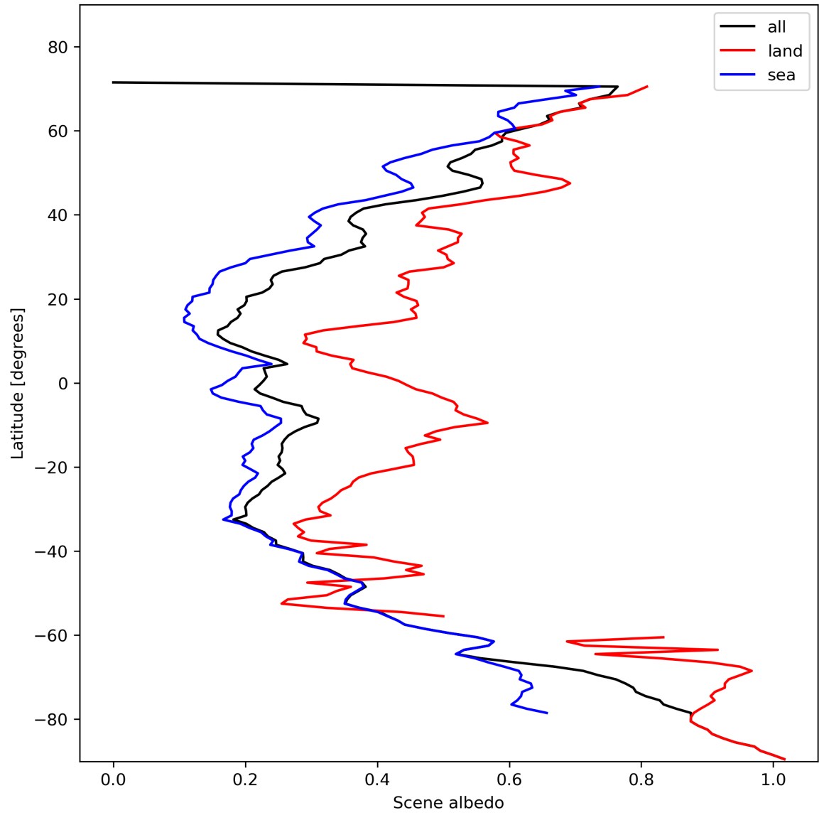
Figure 17: Zonal average of “Scene albedo” for 2024-01-31 to 2024-02-02.
