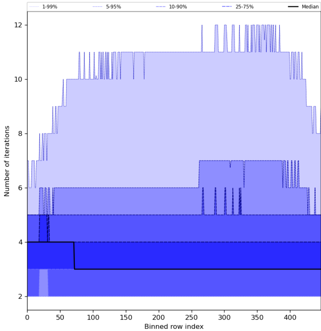
Figure 56: Along track statistics of “Number of iterations” for 2024-01-31 to 2024-02-02
