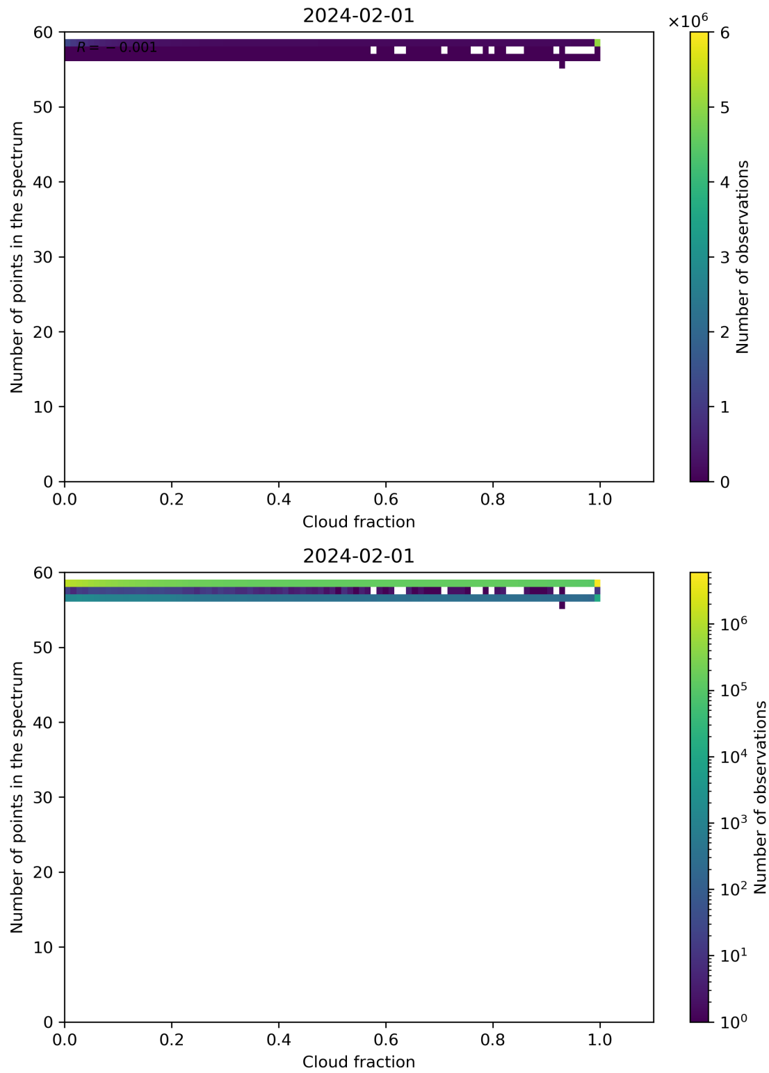
Figure 74: Scatter density plot of “Cloud fraction” against “Number of points in the spectrum” for 2024-01-31 to 2024-02-02.
