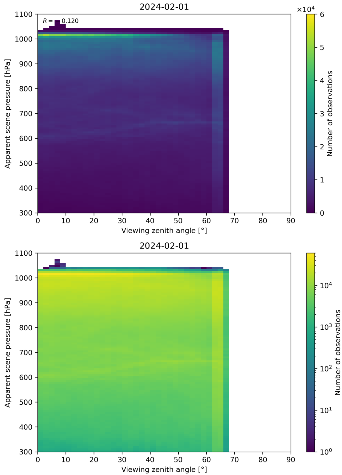
Figure 118: Scatter density plot of “Viewing zenith angle” against “Apparent scene pressure” for 2024-01-31 to 2024-02-02.
