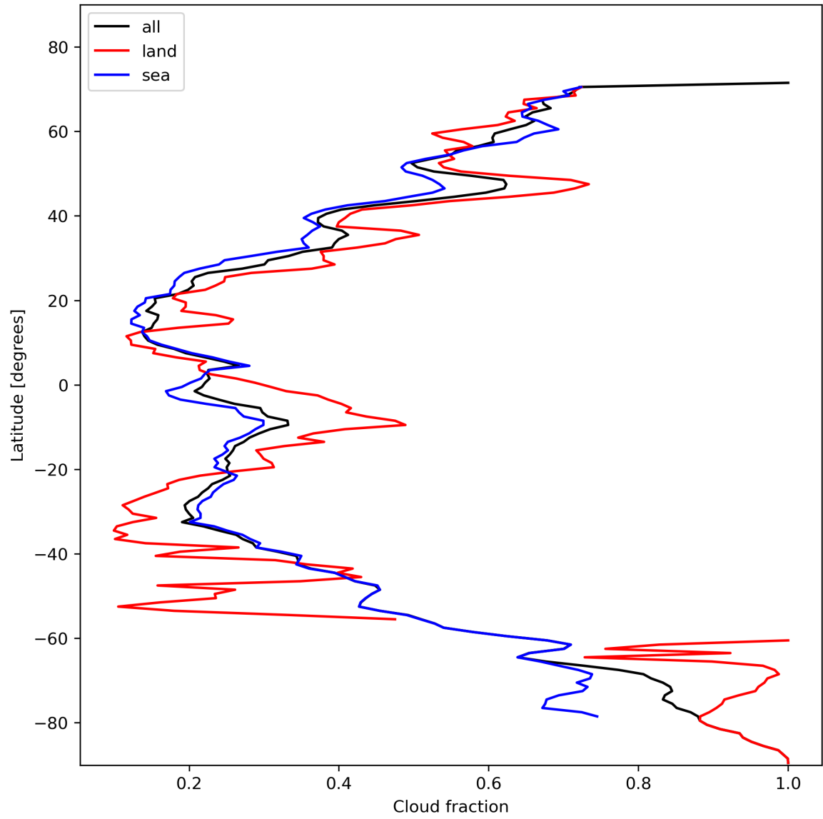
Figure 15: Zonal average of “Cloud fraction” for 2024-01-31 to 2024-02-02.
