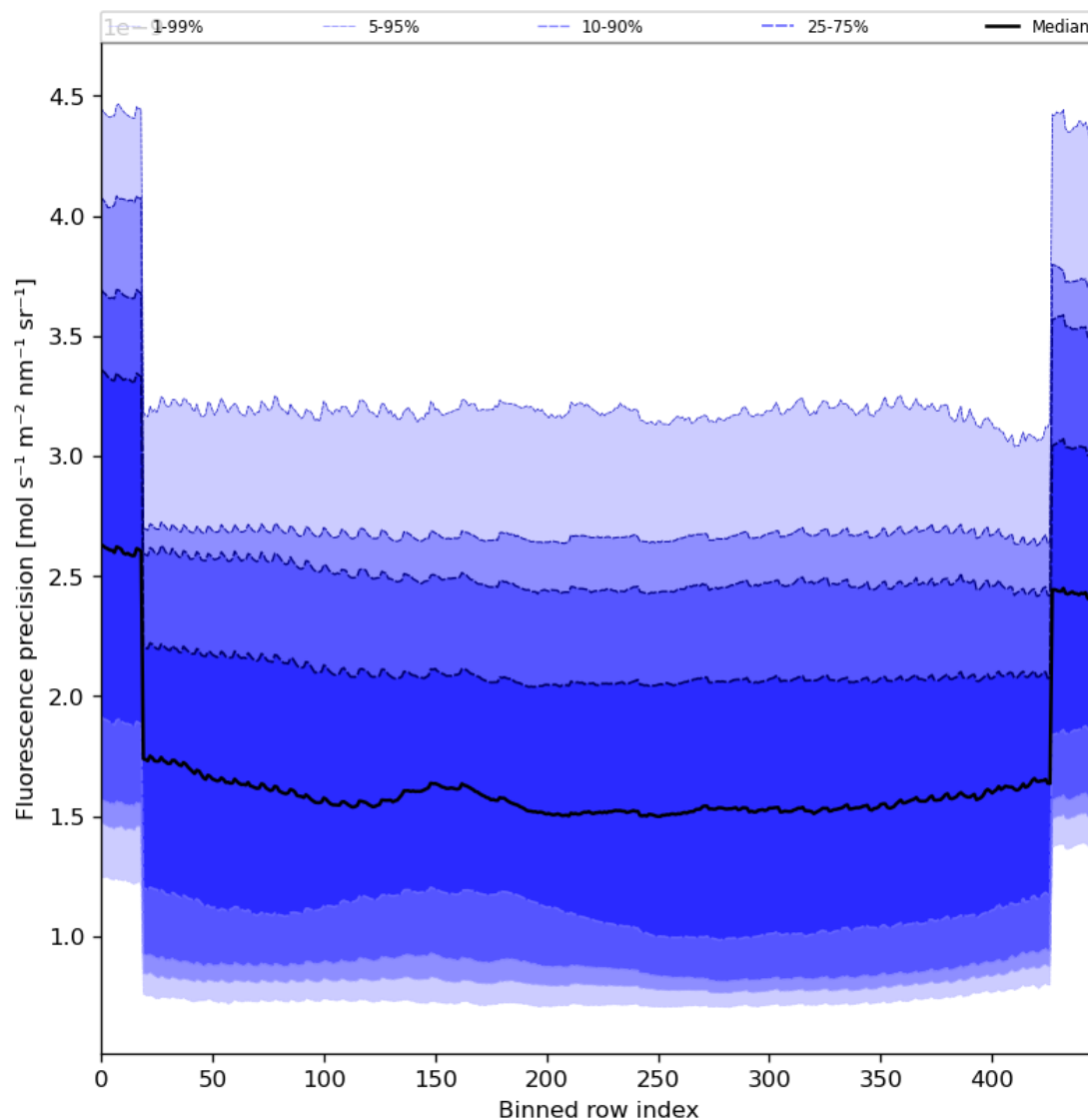
Figure 58: Along track statistics of “Fluorescence precision” for 2024-01-31 to 2024-02-02
