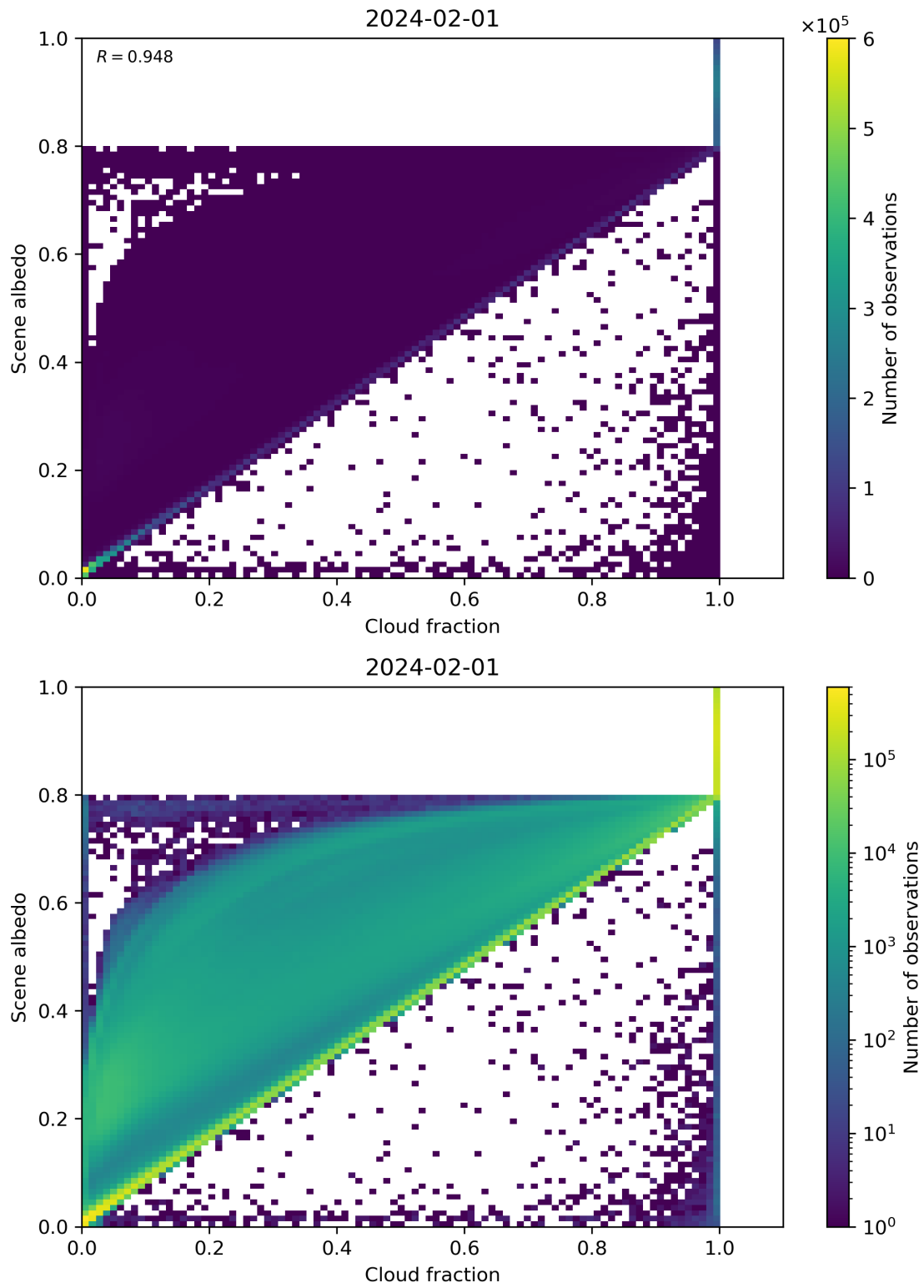
Figure 75: Scatter density plot of “Cloud fraction” against “Scene albedo” for 2024-01-31 to 2024-02-02.
