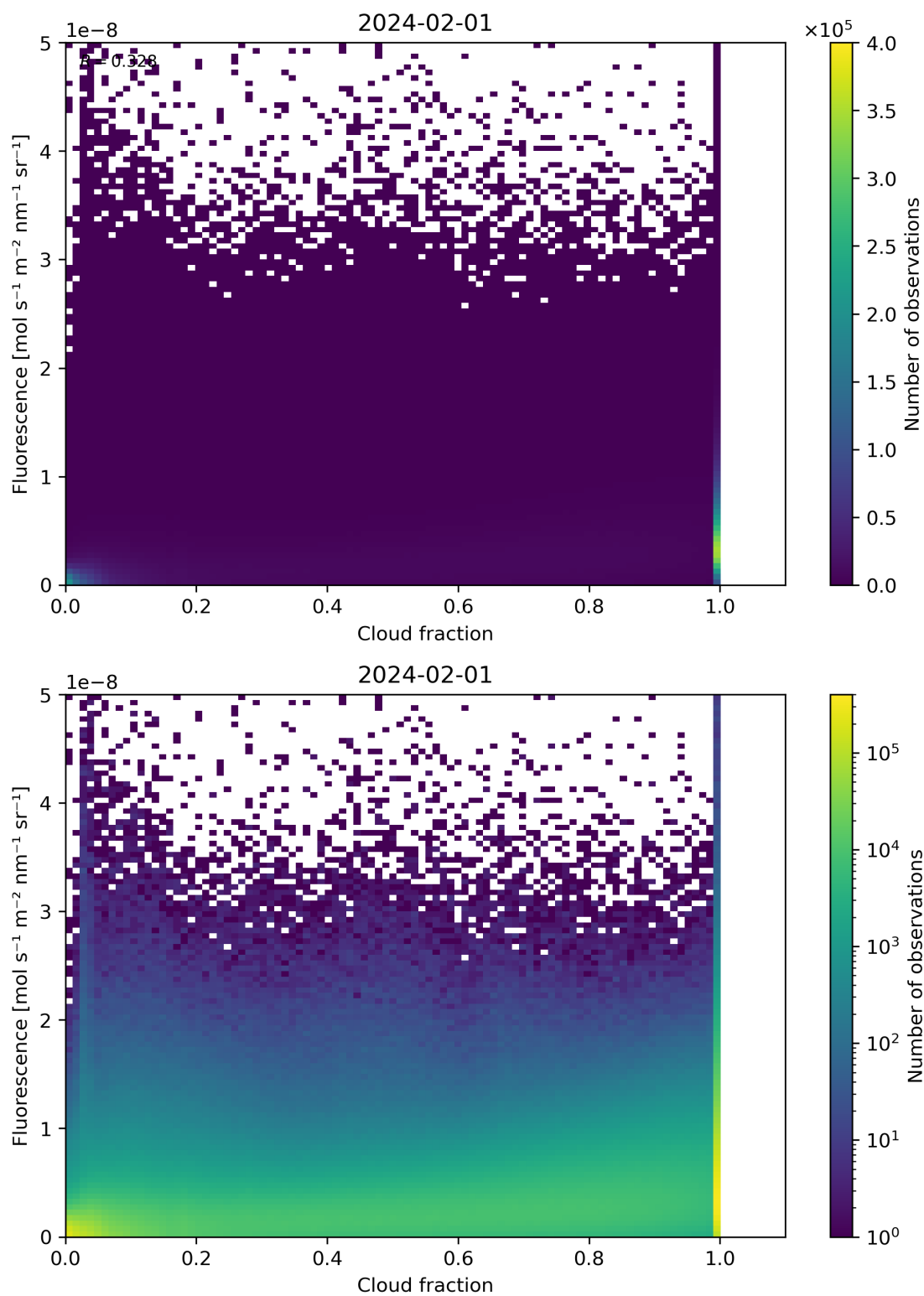
Figure 72: Scatter density plot of “Cloud fraction” against “Fluorescence” for 2024-01-31 to 2024-02-02.
