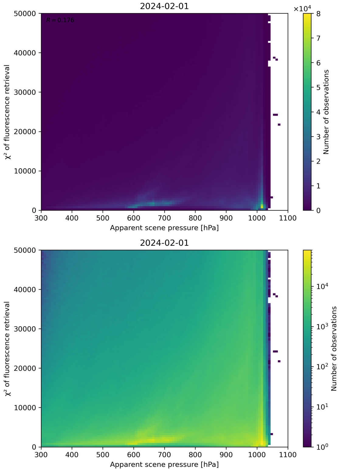
Figure 63: Scatter density plot of “Apparent scene pressure” against “ \chi^2 of fluorescence retrieval” for 2024-01-31 to 2024-02-02.
