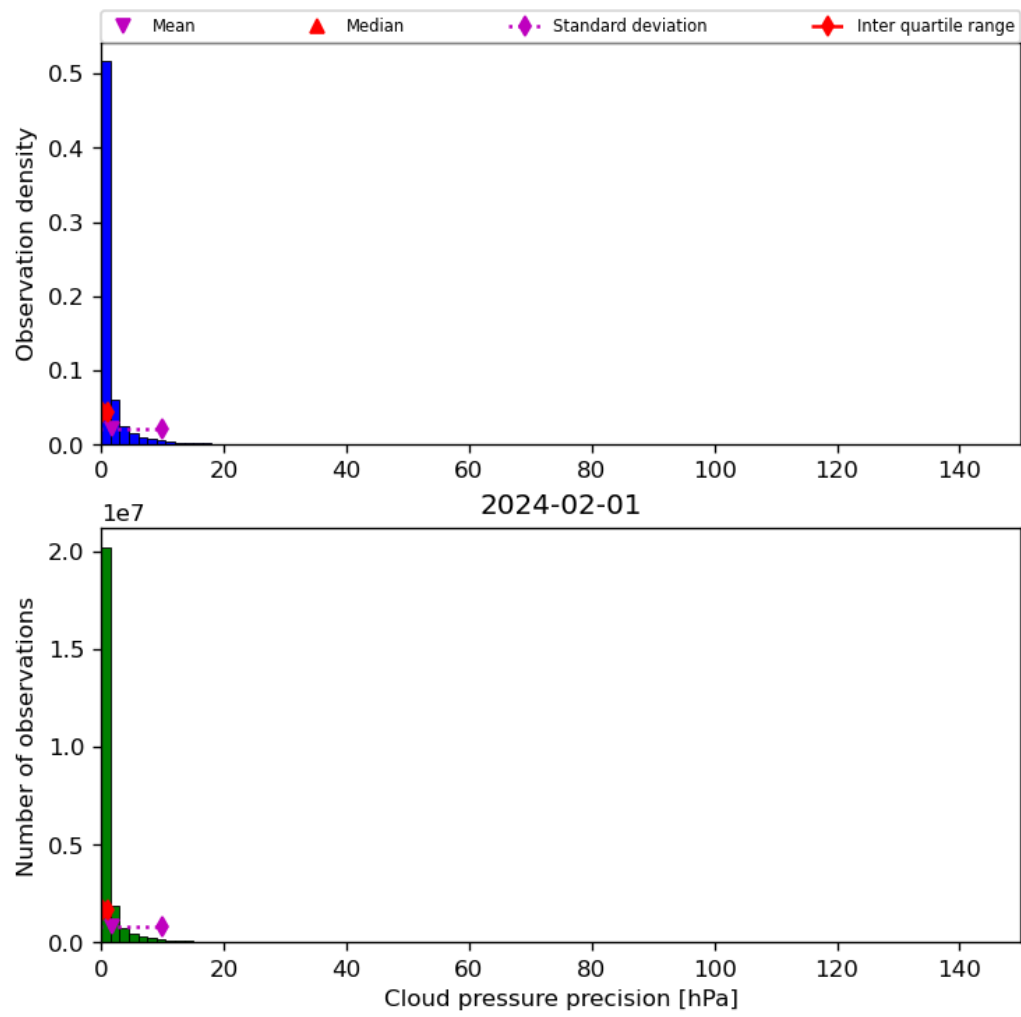
Figure 31: Histogram of “Cloud pressure precision” for 2024-01-31 to 2024-02-02
