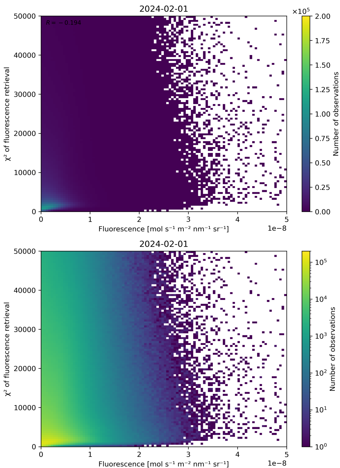
Figure 85: Scatter density plot of “Fluorescence” against “ \chi^2 of fluorescence retrieval” for 2024-01-31 to 2024-02-02.
