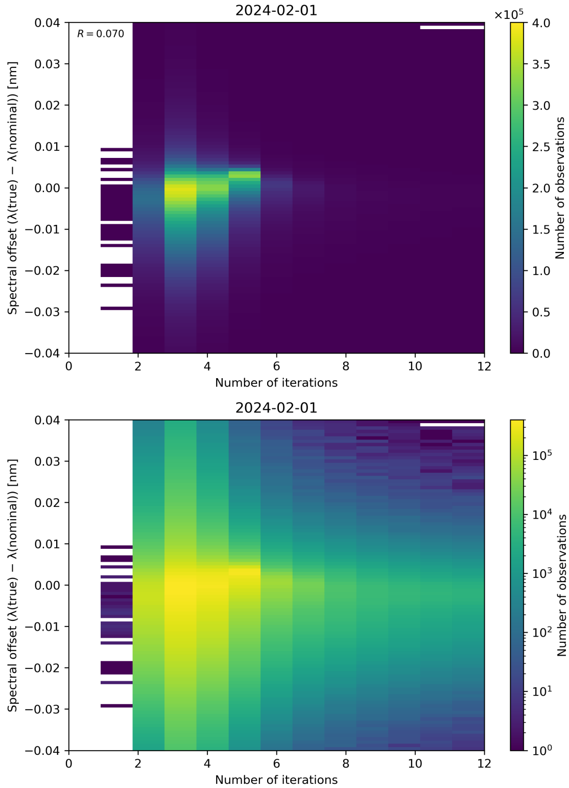
Figure 100: Scatter density plot of “Number of iterations” against “Spectral offset ( \lambda(\text{true}) - \lambda(\text{nominal}) )” for 2024-01-31 to 2024-02-02.
