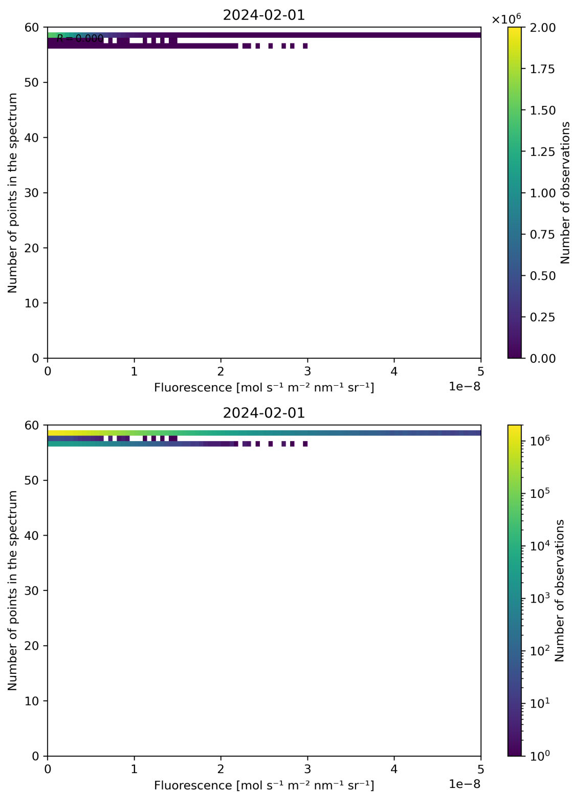
Figure 86: Scatter density plot of “Fluorescence” against “Number of points in the spectrum” for 2024-01-31 to 2024-02-02.
