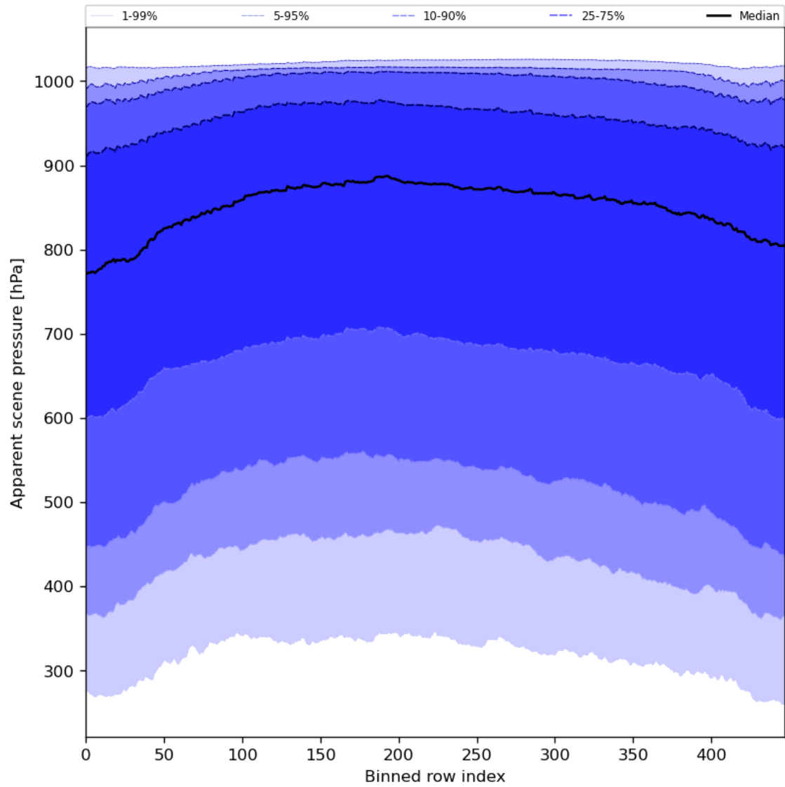
Figure 53: Along track statistics of “Apparent scene pressure” for 2024-01-31 to 2024-02-02
