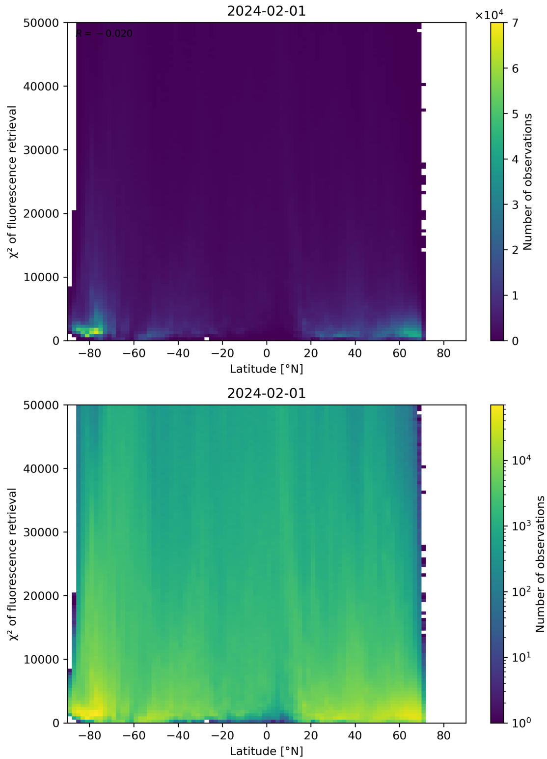
Figure 89: Scatter density plot of “Latitude” against “ \chi^2 of fluorescence retrieval” for 2024-01-31 to 2024-02-02.
