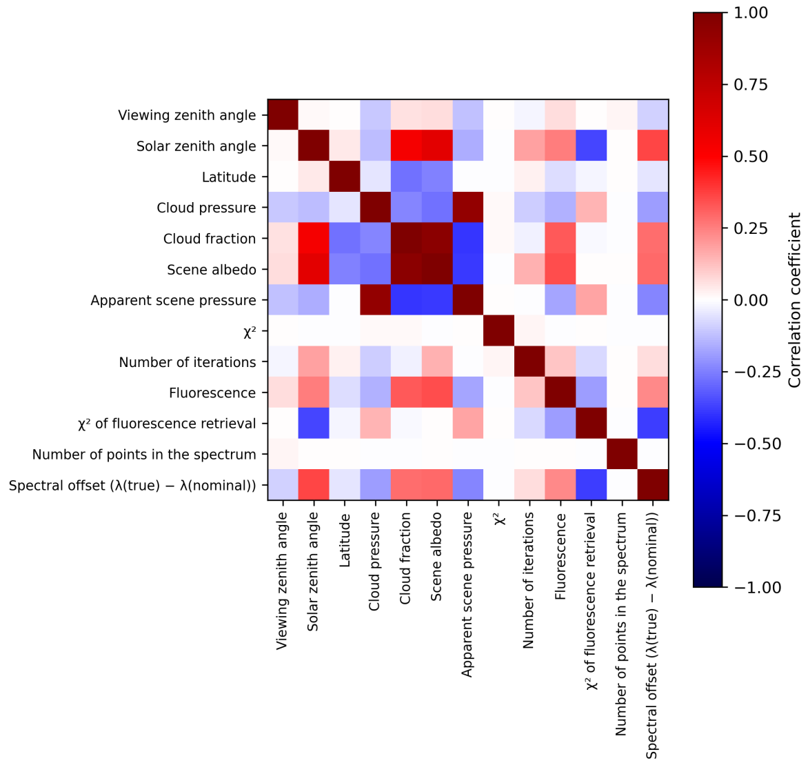
Figure 2: Map of correlation matrix for 2024-01-31 to 2024-02-02.
