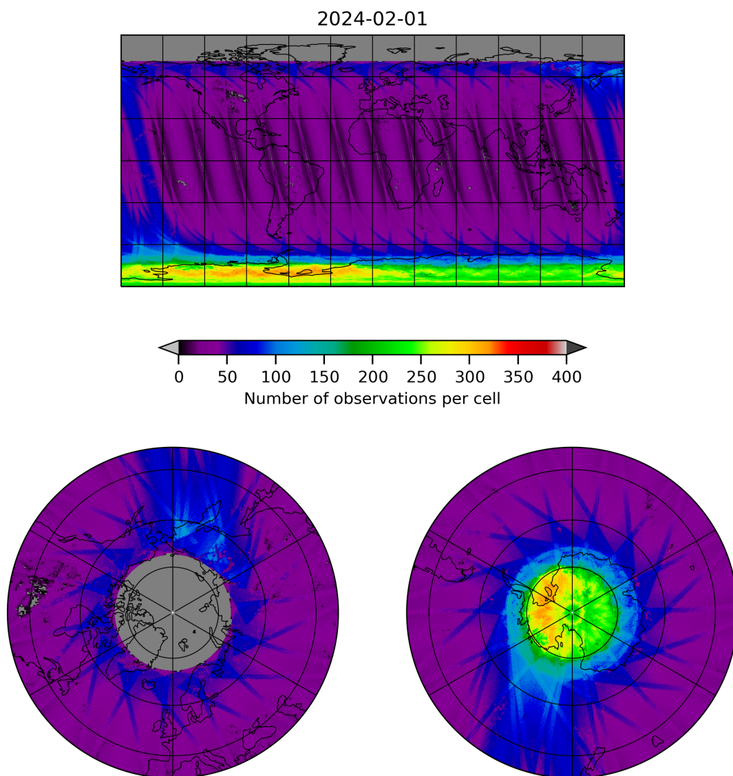
Figure 11: Map of the number of observations for 2024-01-31 to 2024-02-02
