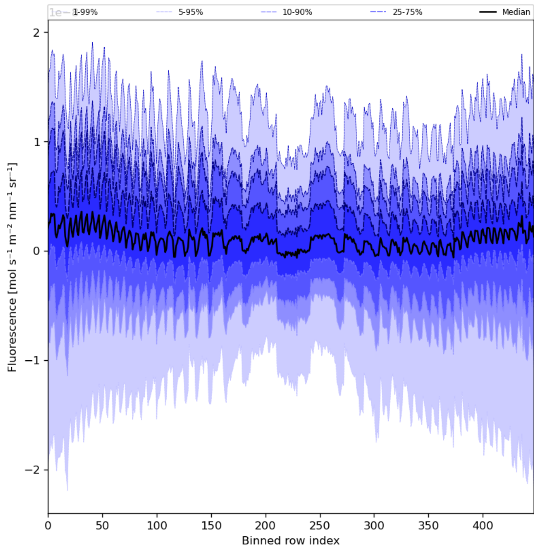
Figure 57: Along track statistics of “Fluorescence” for 2024-01-31 to 2024-02-02
