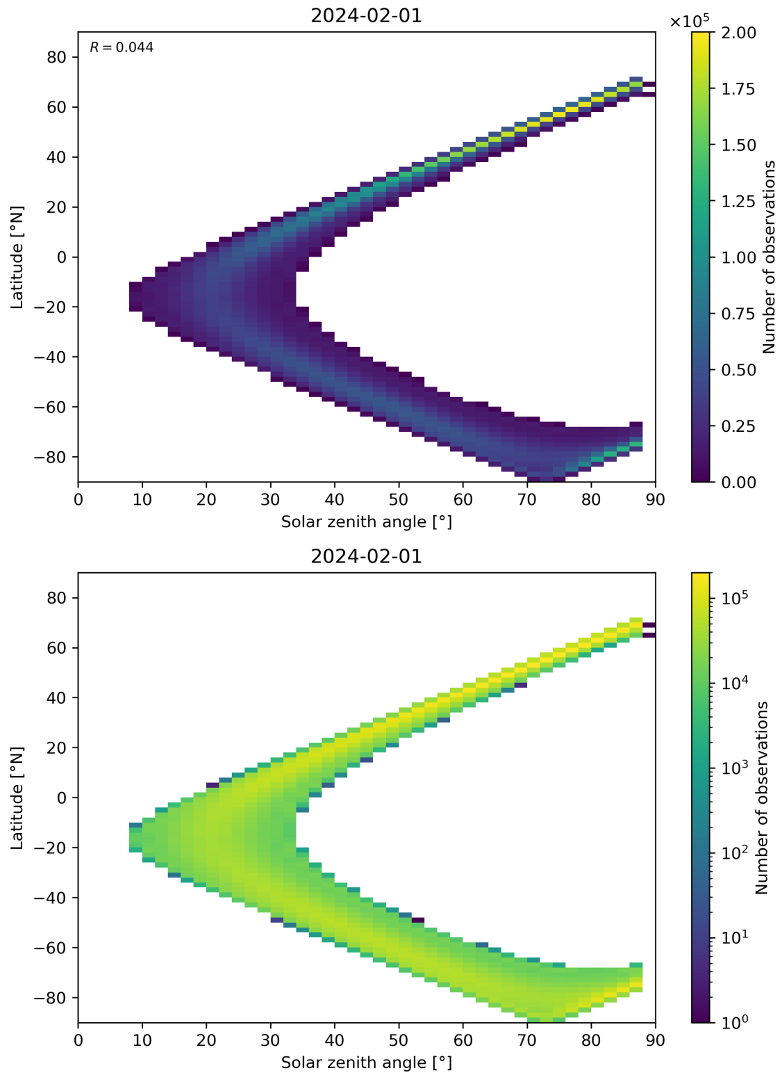
Figure 113: Scatter density plot of “Solar zenith angle” against “Latitude” for 2024-01-31 to 2024-02-02.
