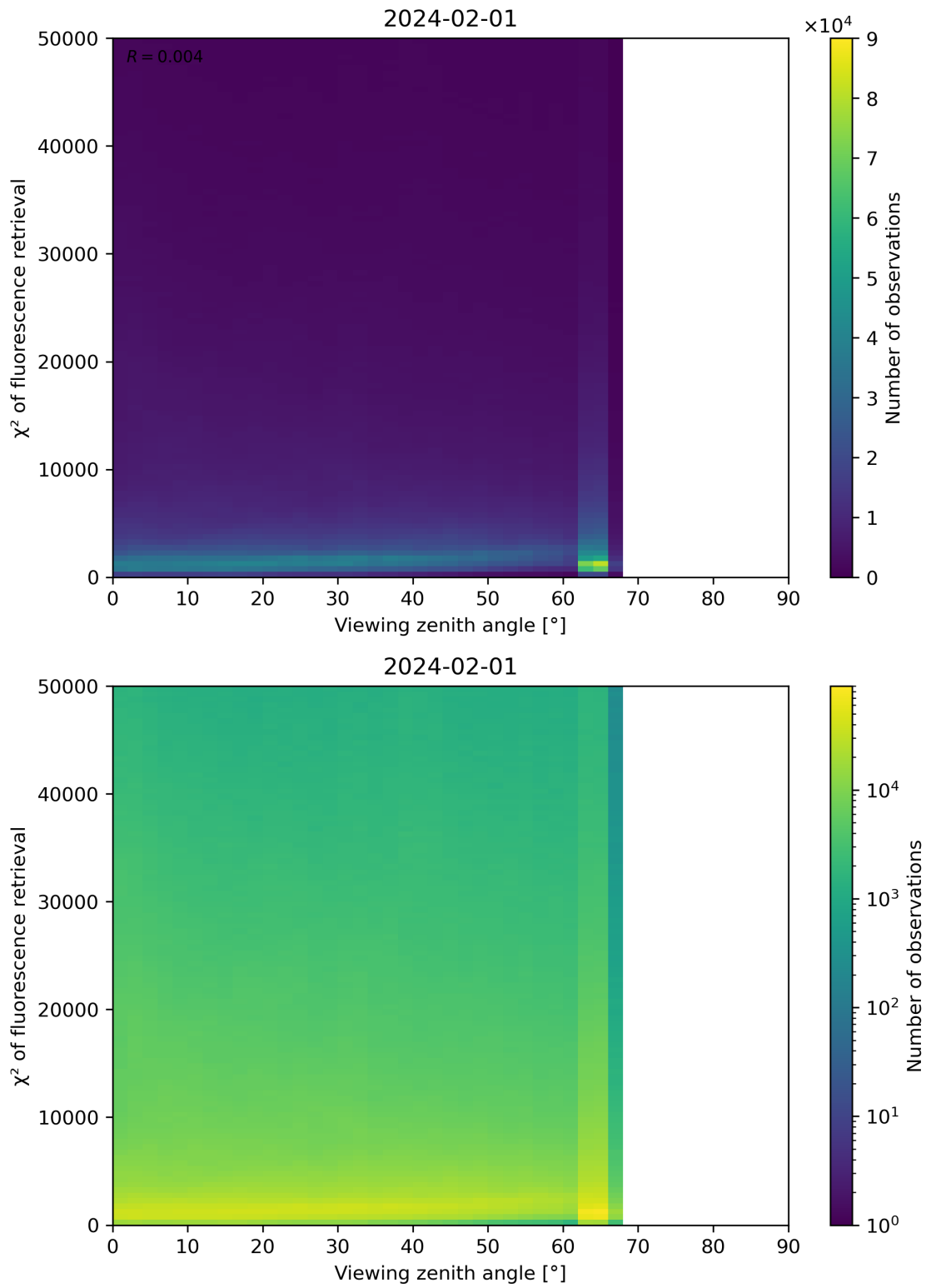
Figure 119: Scatter density plot of “Viewing zenith angle” against “ \chi^2 of fluorescence retrieval” for 2024-01-31 to 2024-02-02.
