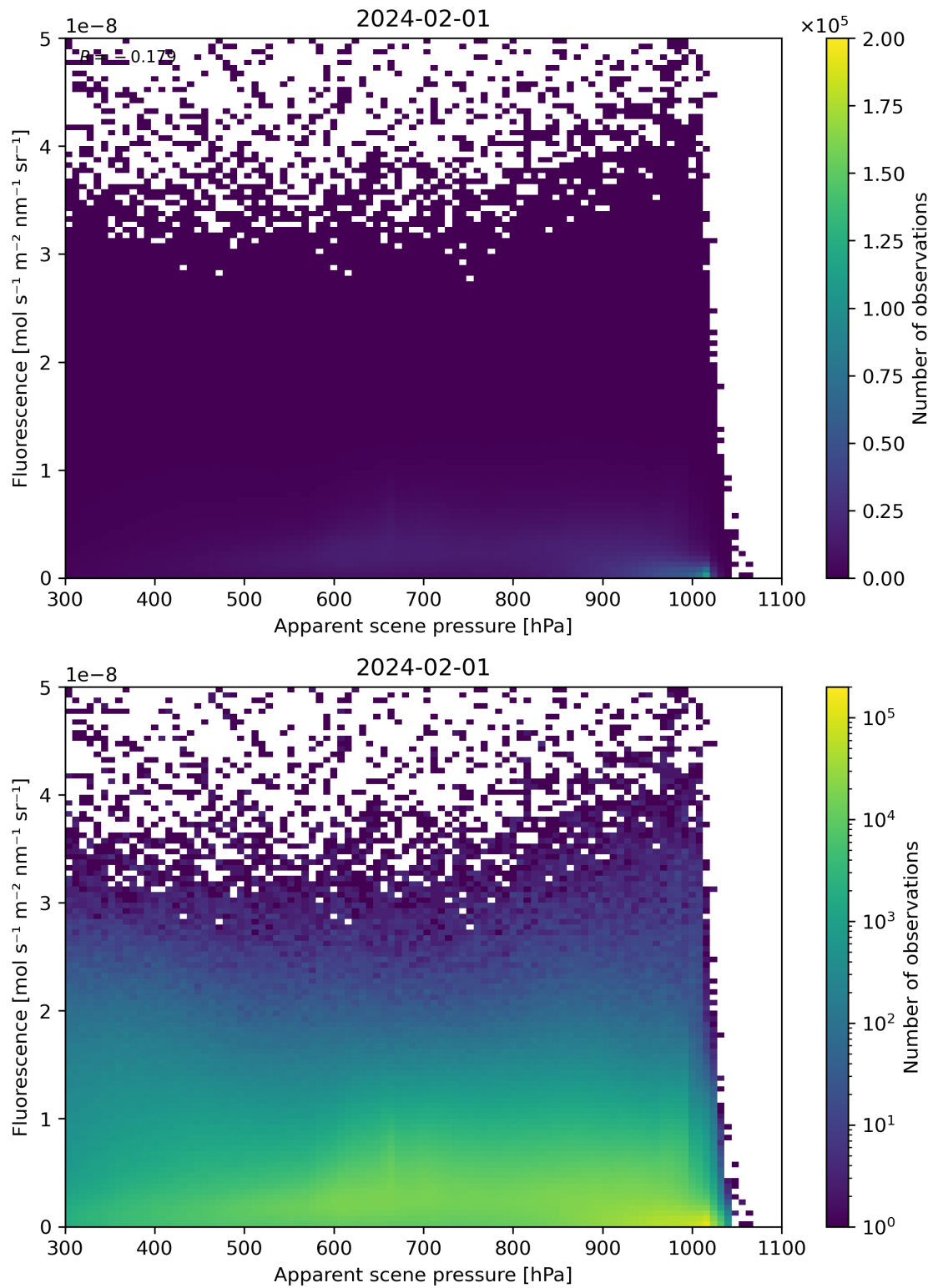
Figure 64: Scatter density plot of “Apparent scene pressure” against “Fluorescence” for 2024-01-31 to 2024-02-02.
