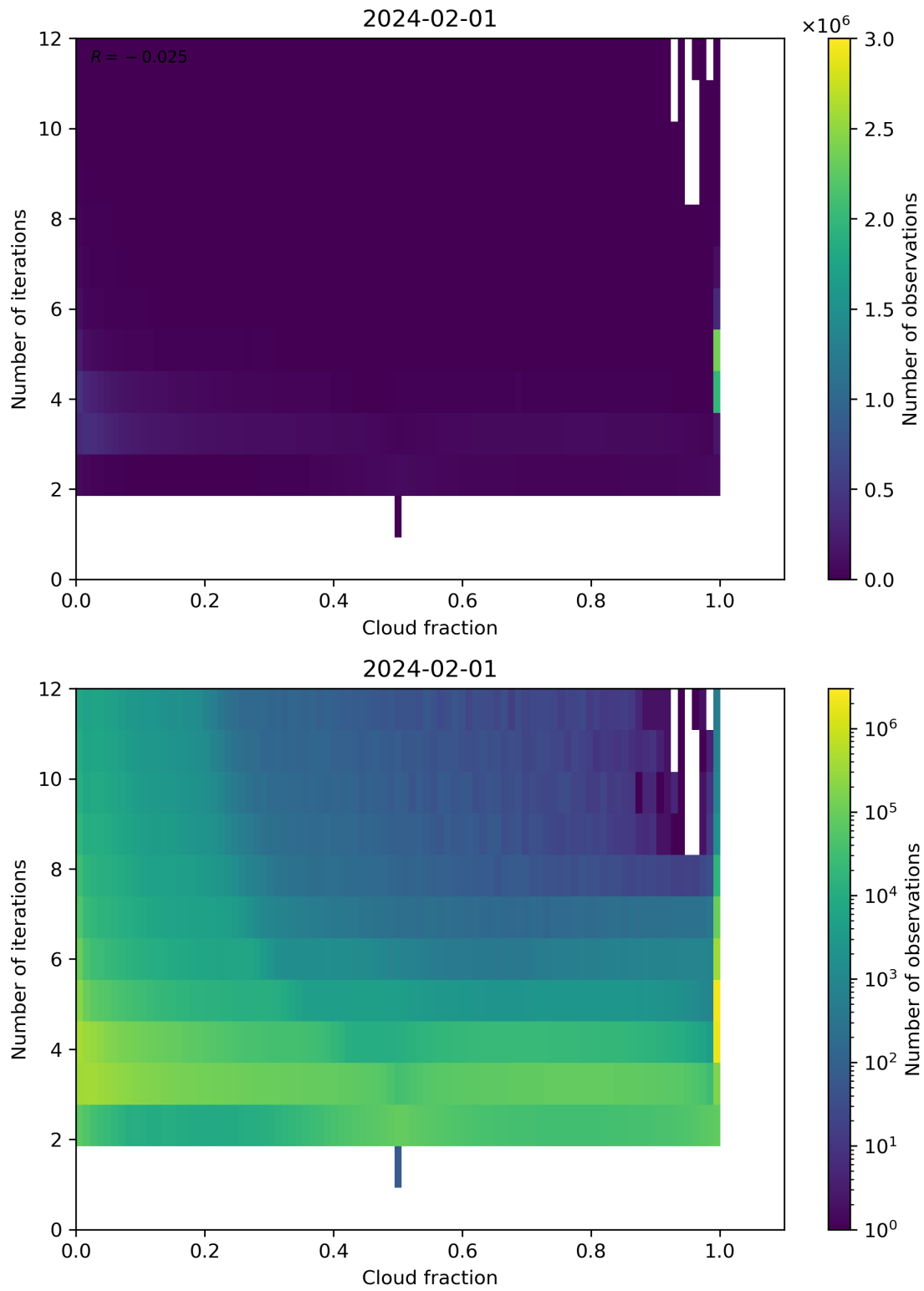
Figure 73: Scatter density plot of “Cloud fraction” against “Number of iterations” for 2024-01-31 to 2024-02-02.
