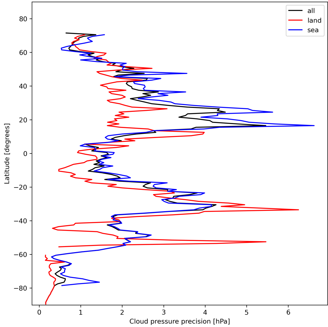
Figure 14: Zonal average of "Cloud pressure precision" for 2024-01-31 to 2024-02-02.
