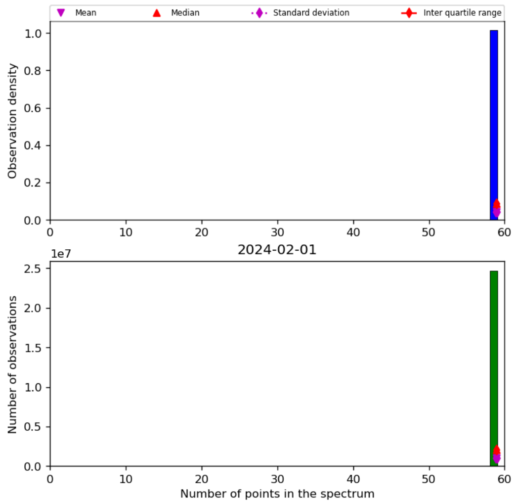
Figure 44: Histogram of “Number of points in the spectrum” for 2024-01-31 to 2024-02-02
