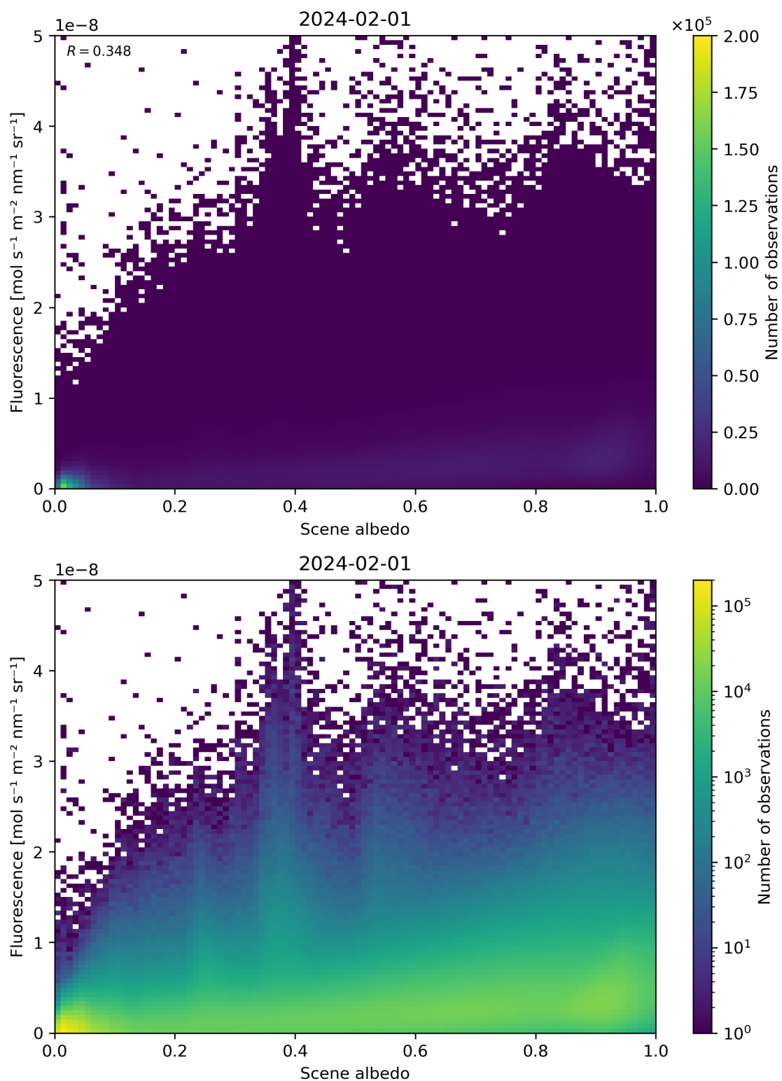
Figure 104: Scatter density plot of “Scene albedo” against “Fluorescence” for 2024-01-31 to 2024-02-02.
