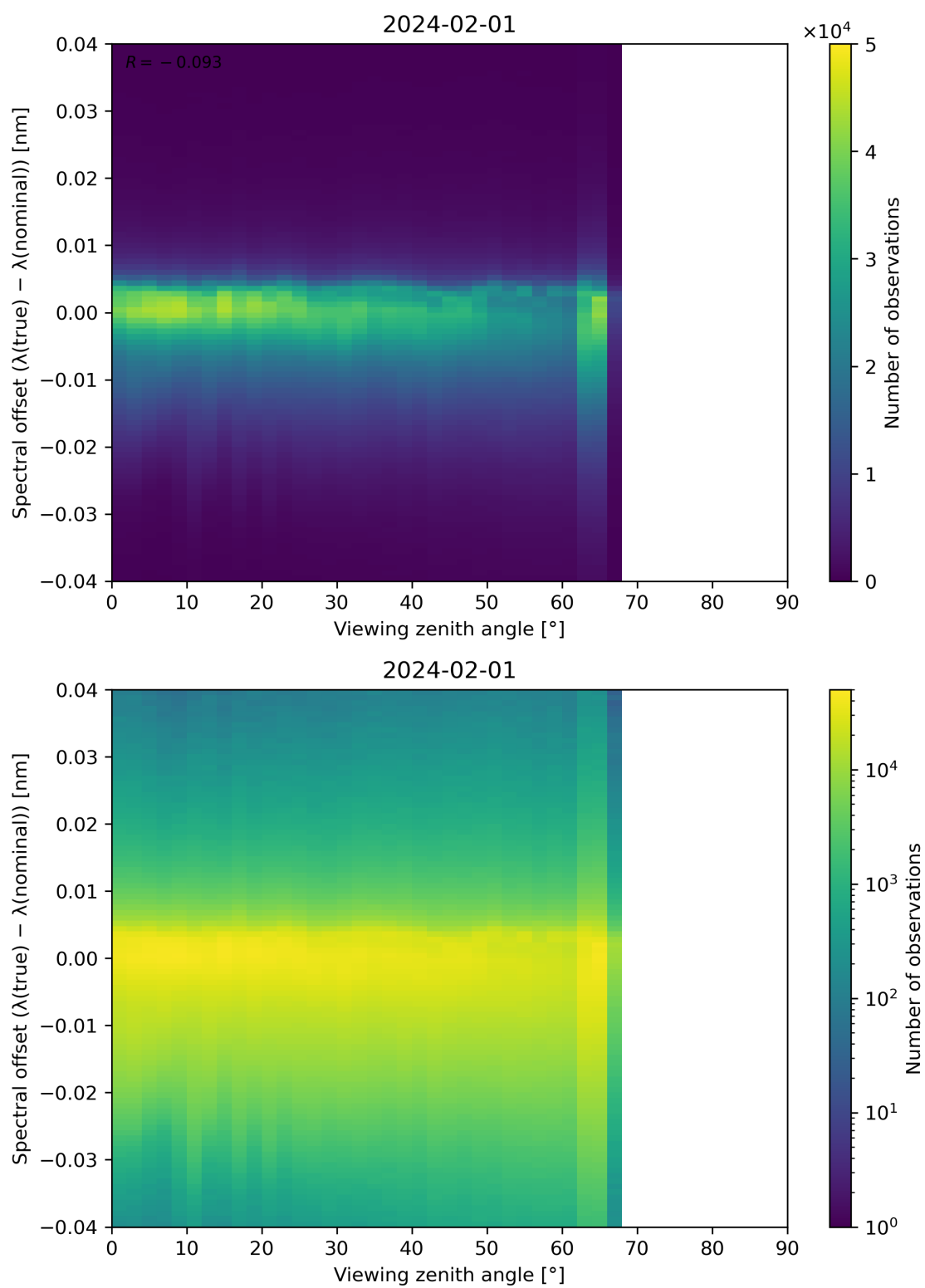
Figure 128: Scatter density plot of “Viewing zenith angle” against “Spectral offset ( \lambda(\text{true}) - \lambda(\text{nominal}) )” for 2024-01-31 to 2024-02-02.
