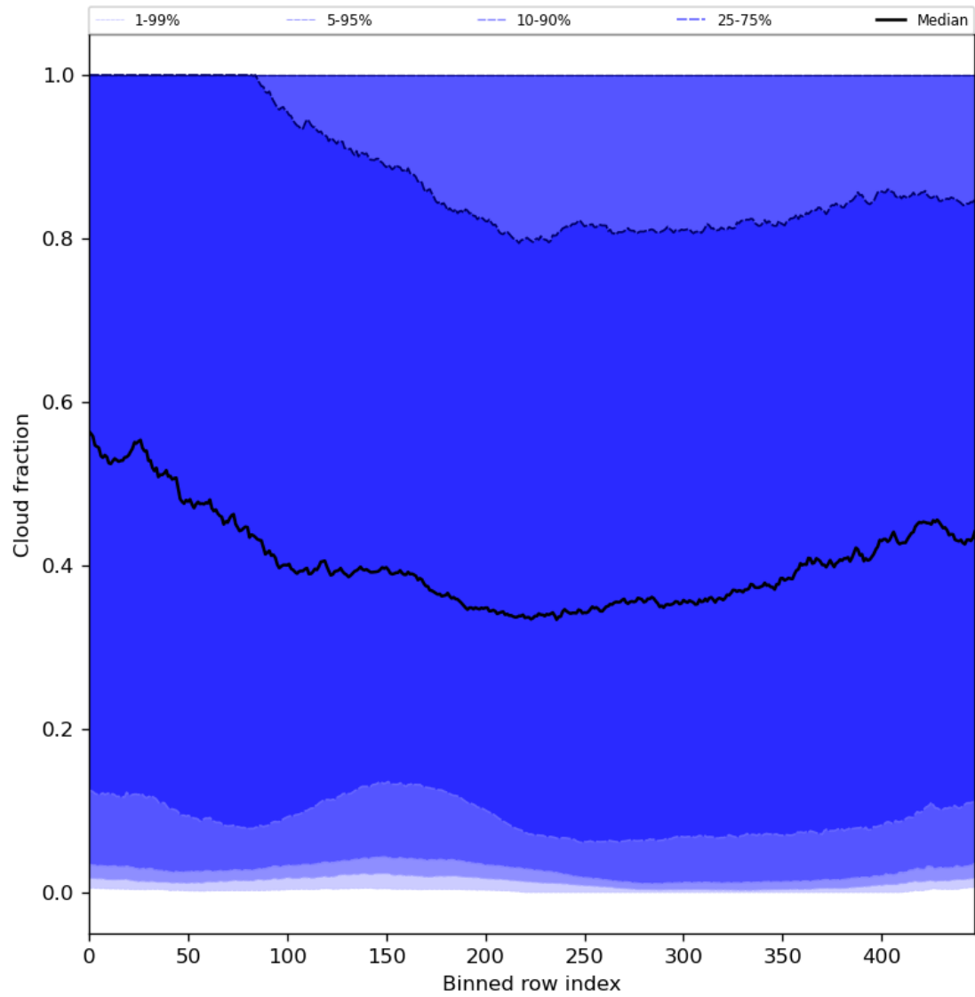
Figure 49: Along track statistics of “Cloud fraction” for 2024-01-31 to 2024-02-02
