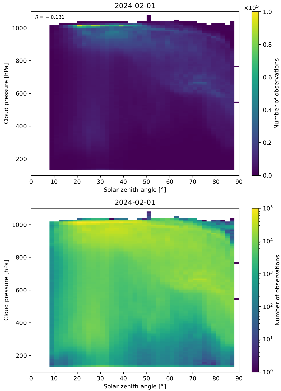
Figure 111: Scatter density plot of “Solar zenith angle” against “Cloud pressure” for 2024-01-31 to 2024-02-02.
