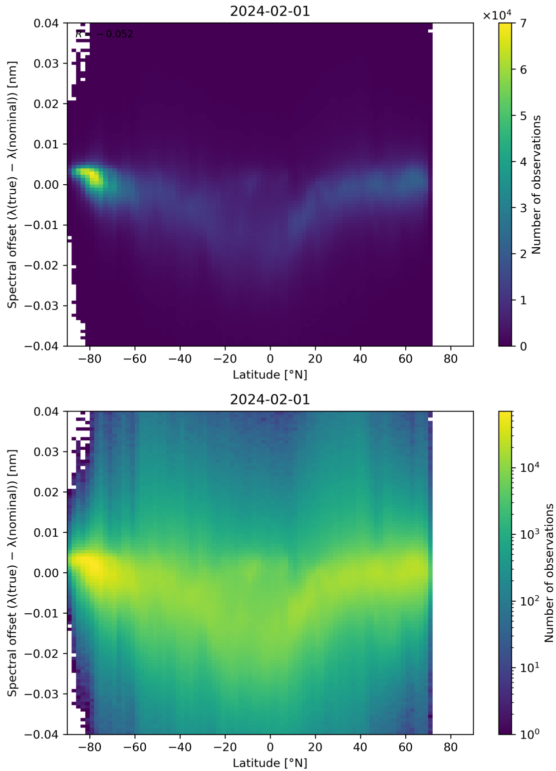
Figure 96: Scatter density plot of “Latitude” against “Spectral offset ( \lambda(\text{true}) - \lambda(\text{nominal}) )” for 2024-01-31 to 2024-02-02.
