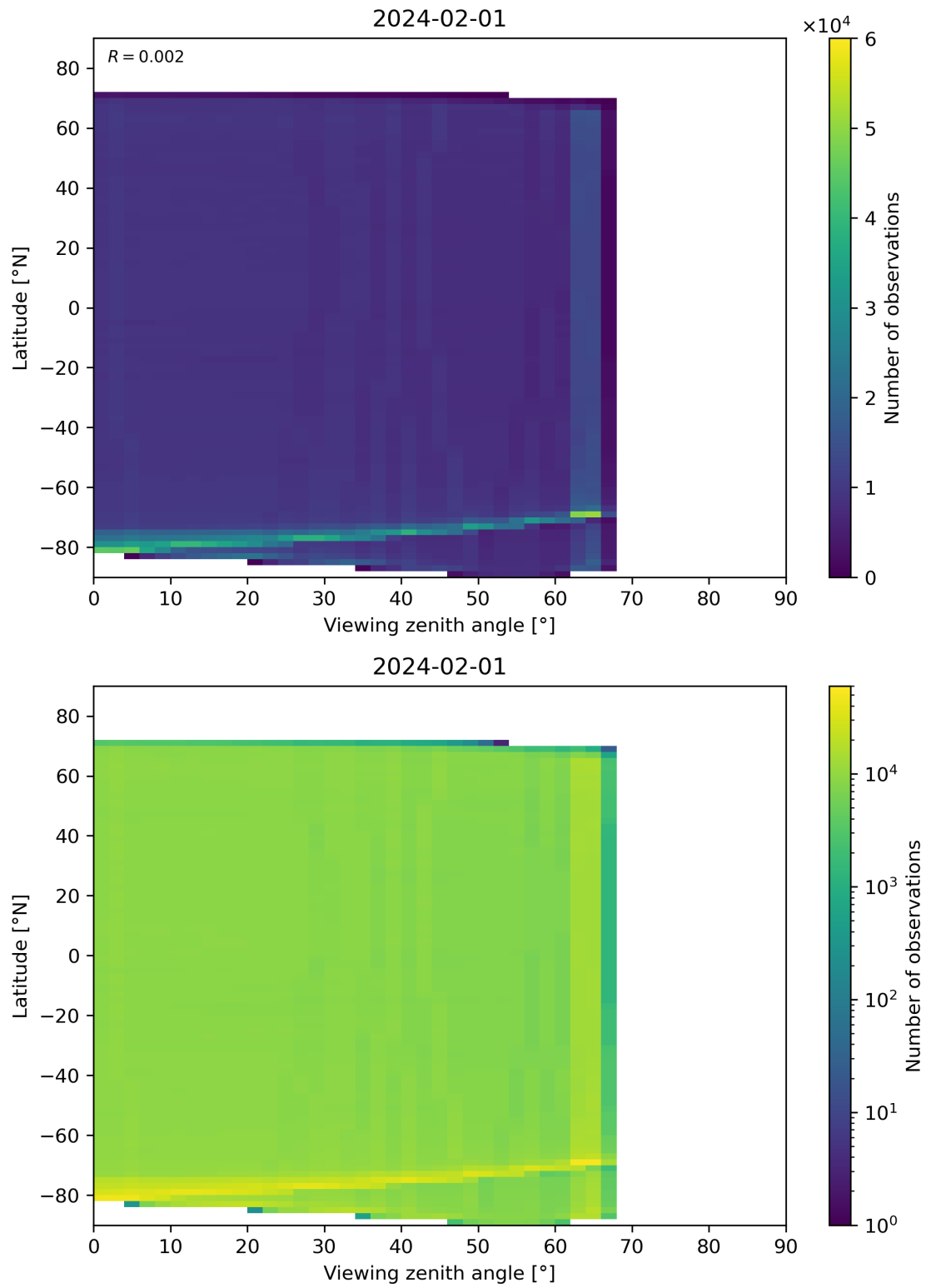
Figure 123: Scatter density plot of “Viewing zenith angle” against “Latitude” for 2024-01-31 to 2024-02-02.
