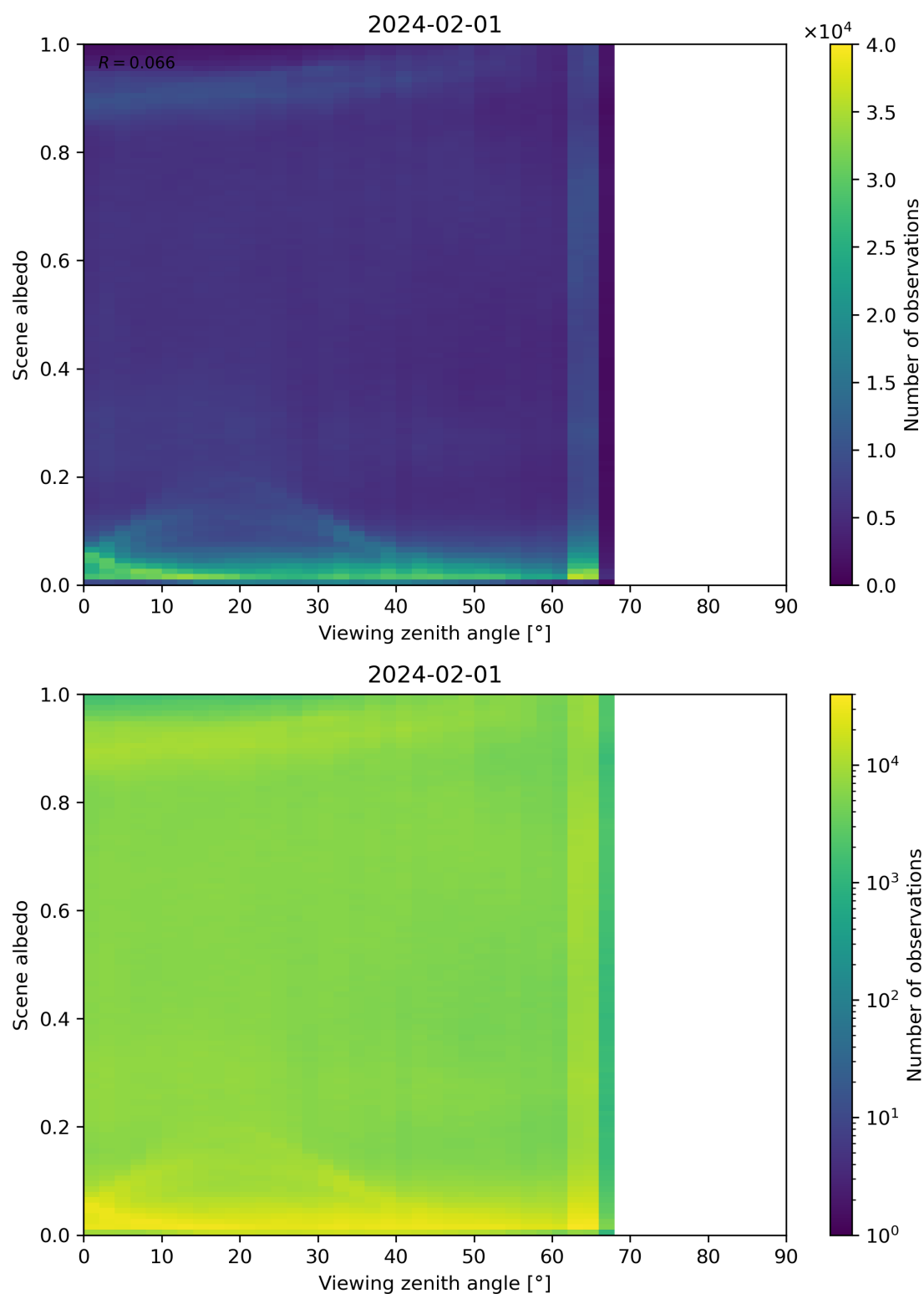
Figure 126: Scatter density plot of “Viewing zenith angle” against “Scene albedo” for 2024-01-31 to 2024-02-02.
