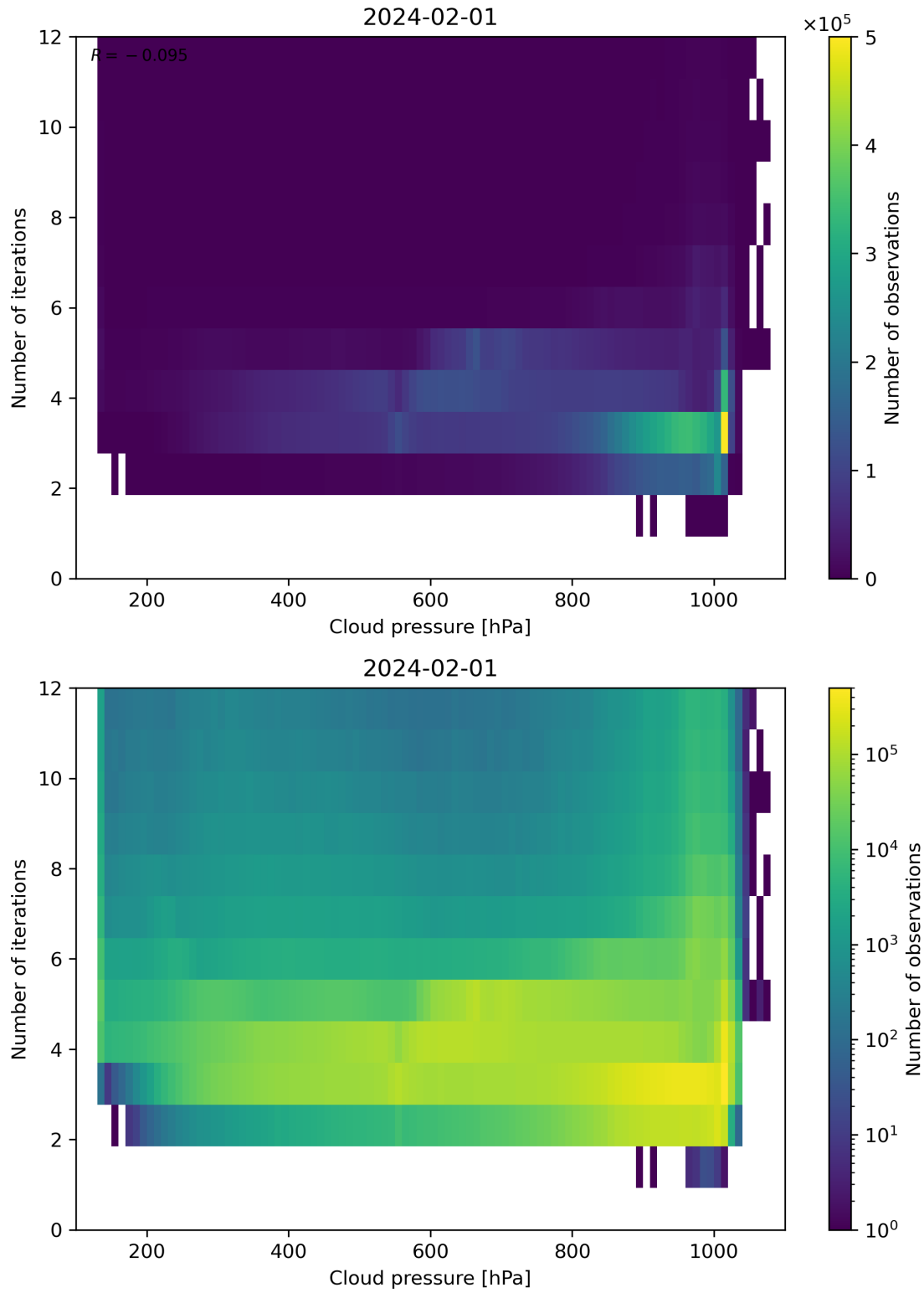
Figure 81: Scatter density plot of “Cloud pressure” against “Number of iterations” for 2024-01-31 to 2024-02-02.
