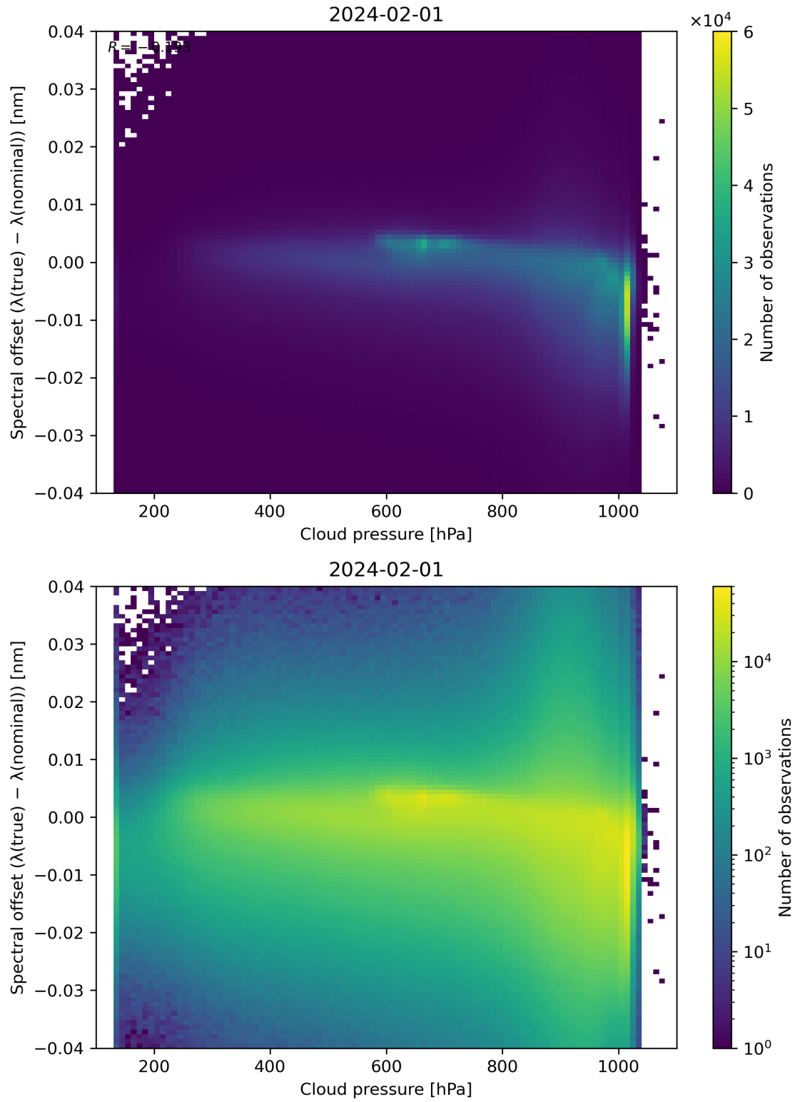
Figure 84: Scatter density plot of “Cloud pressure” against “Spectral offset ( \lambda(\text{true}) - \lambda(\text{nominal}) )” for 2024-01-31 to 2024-02-02.
