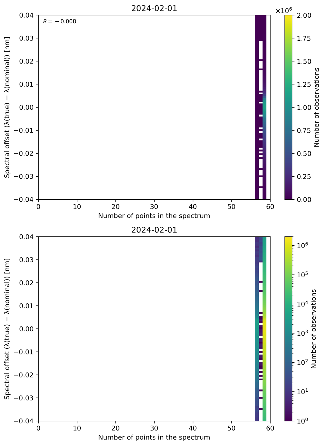
Figure 101: Scatter density plot of “Number of points in the spectrum” against “Spectral offset ( \lambda(\text{true}) - \lambda(\text{nominal}) )” for 2024-01-31 to 2024-02-02.
