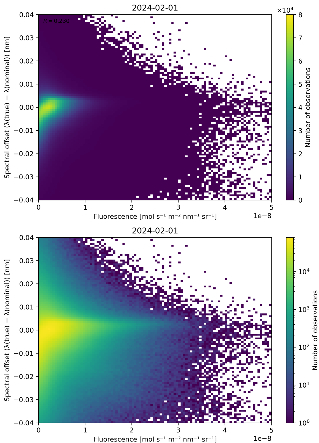
Figure 87: Scatter density plot of “Fluorescence” against “Spectral offset ( \lambda(\text{true}) - \lambda(\text{nominal}) )” for 2024-01-31 to 2024-02-02.
