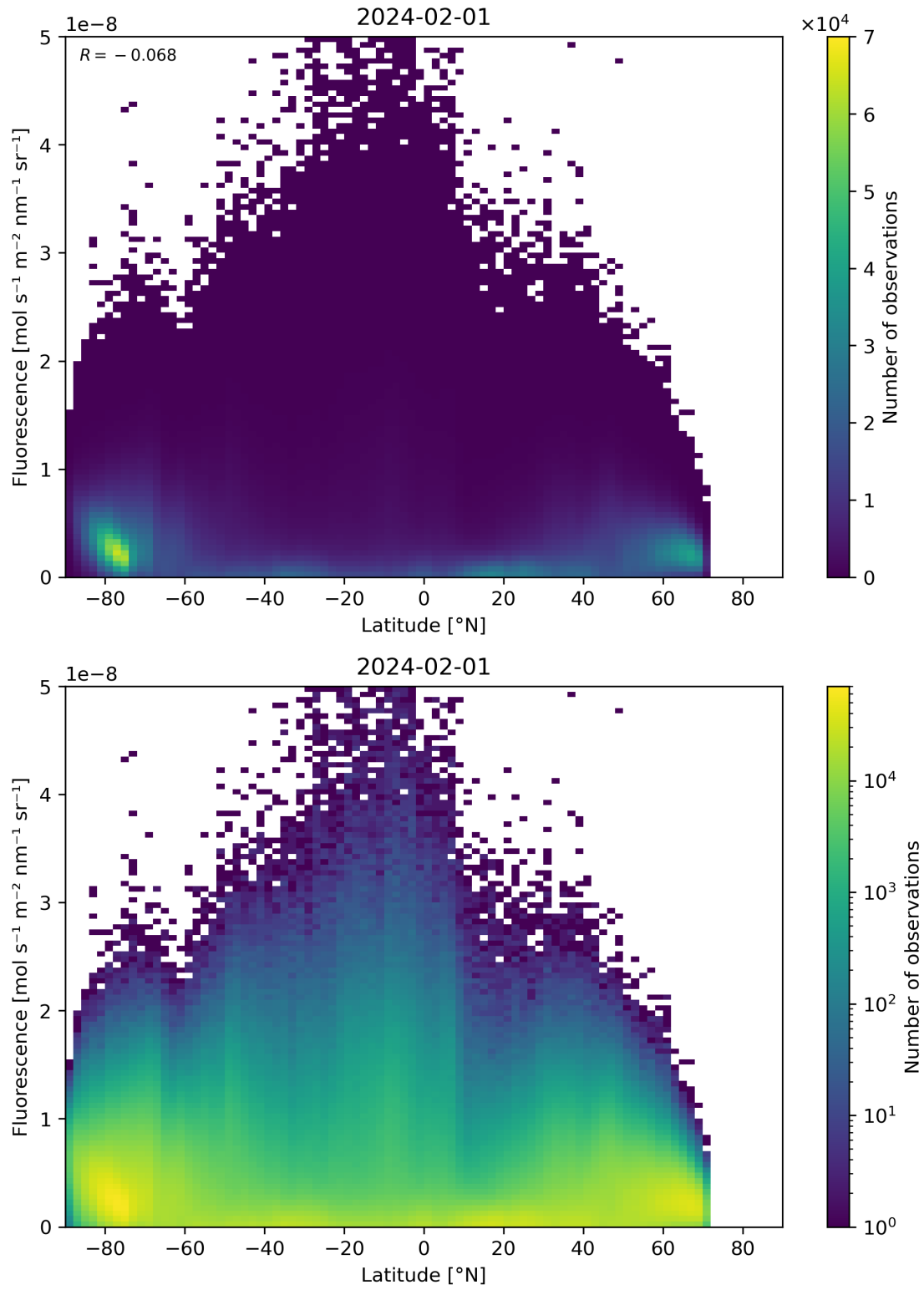
Figure 92: Scatter density plot of “Latitude” against “Fluorescence” for 2024-01-31 to 2024-02-02.
