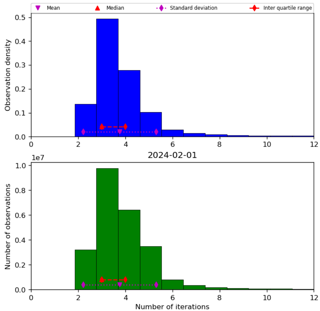
Figure 39: Histogram of “Number of iterations” for 2024-01-31 to 2024-02-02
