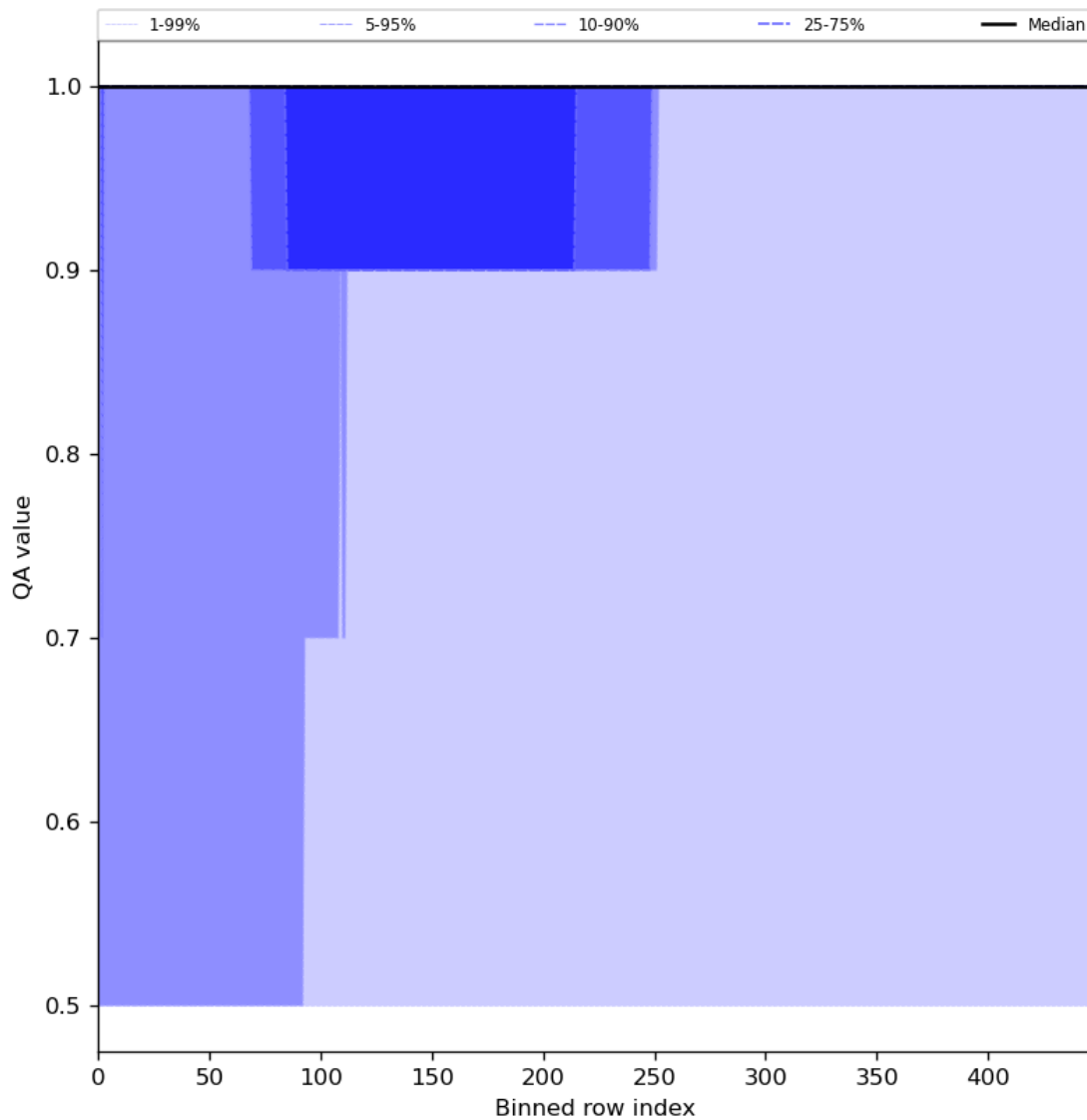
Figure 46: Along track statistics of “QA value” for 2024-01-31 to 2024-02-02
