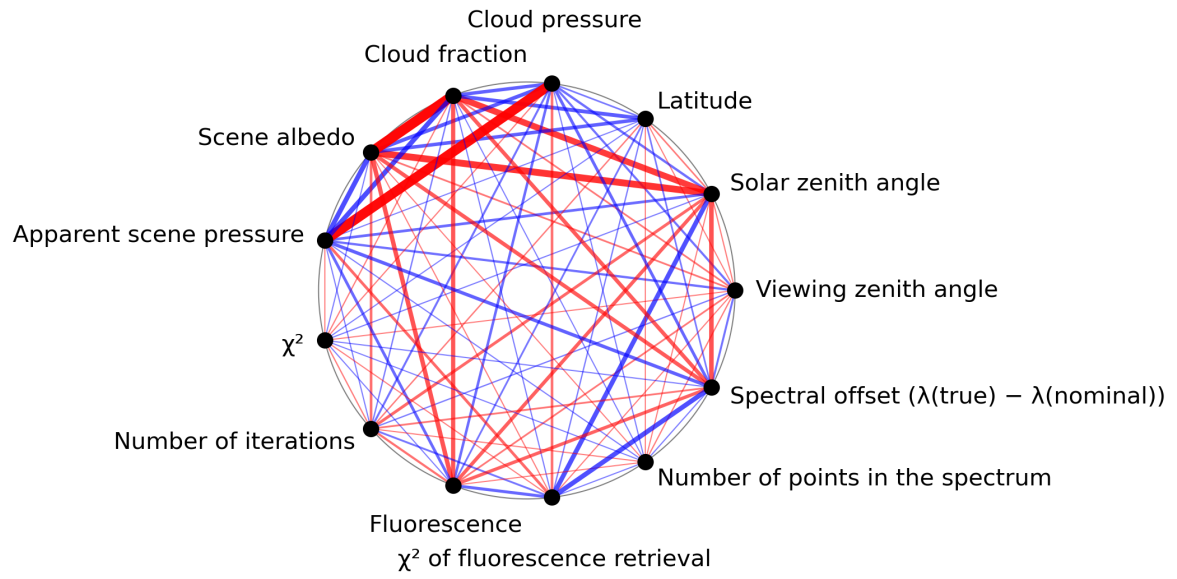
Figure 1: Map of correlation graph for 2024-01-31 to 2024-02-02.
