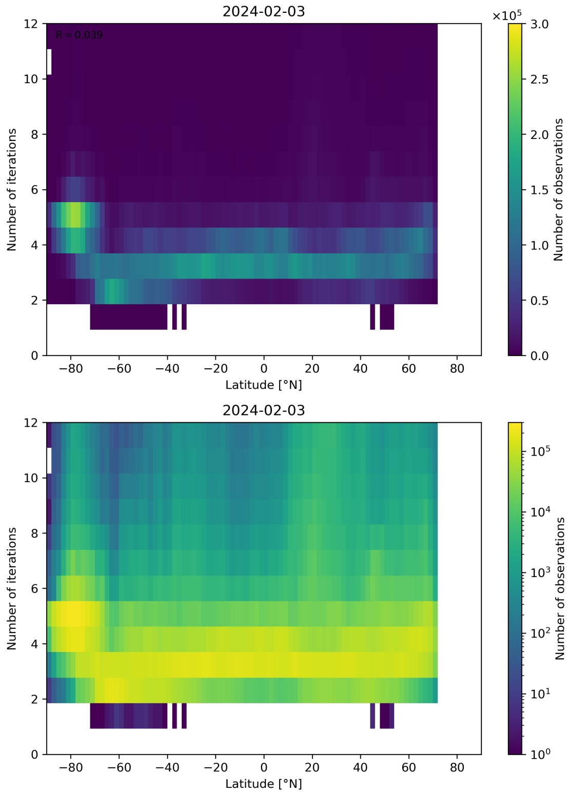
Figure 93: Scatter density plot of “Latitude” against “Number of iterations” for 2024-02-02 to 2024-02-04.
