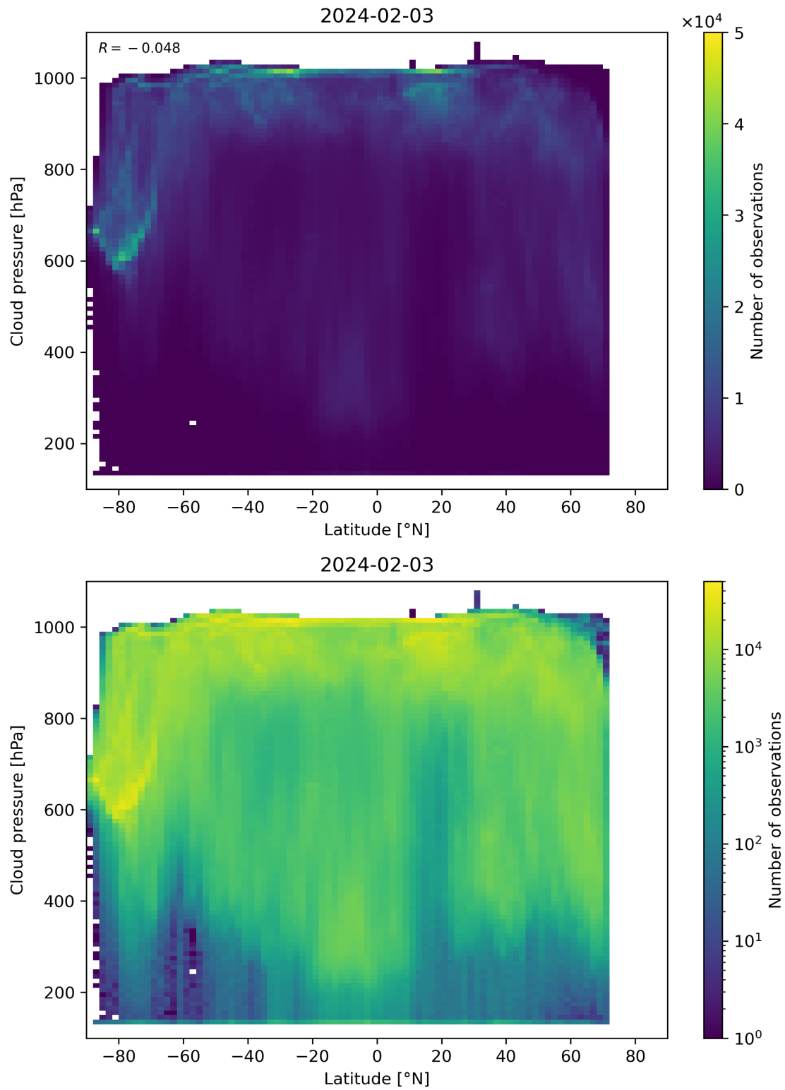
Figure 91: Scatter density plot of “Latitude” against “Cloud pressure” for 2024-02-02 to 2024-02-04.
