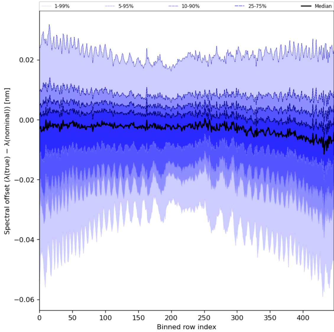
Figure 62: Along track statistics of “Spectral offset ( \lambda(\text{true}) - \lambda(\text{nominal}) )” for 2024-02-02 to 2024-02-04
