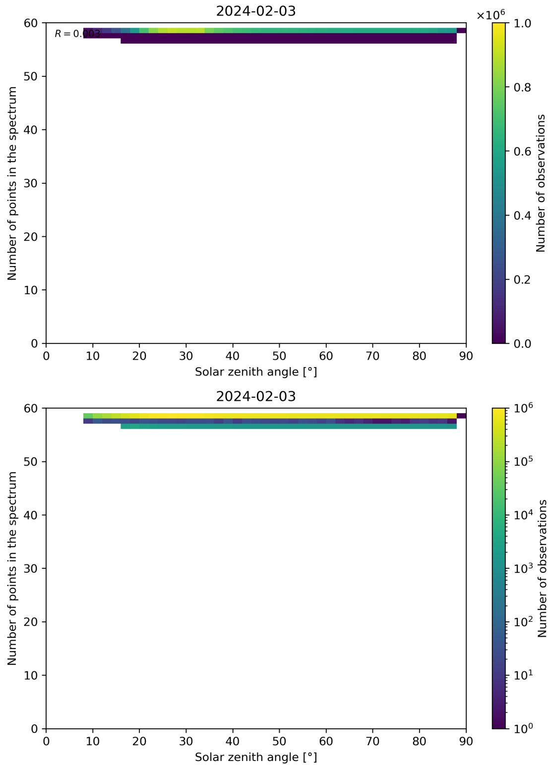
Figure 115: Scatter density plot of “Solar zenith angle” against “Number of points in the spectrum” for 2024-02-02 to 2024-02-04.
