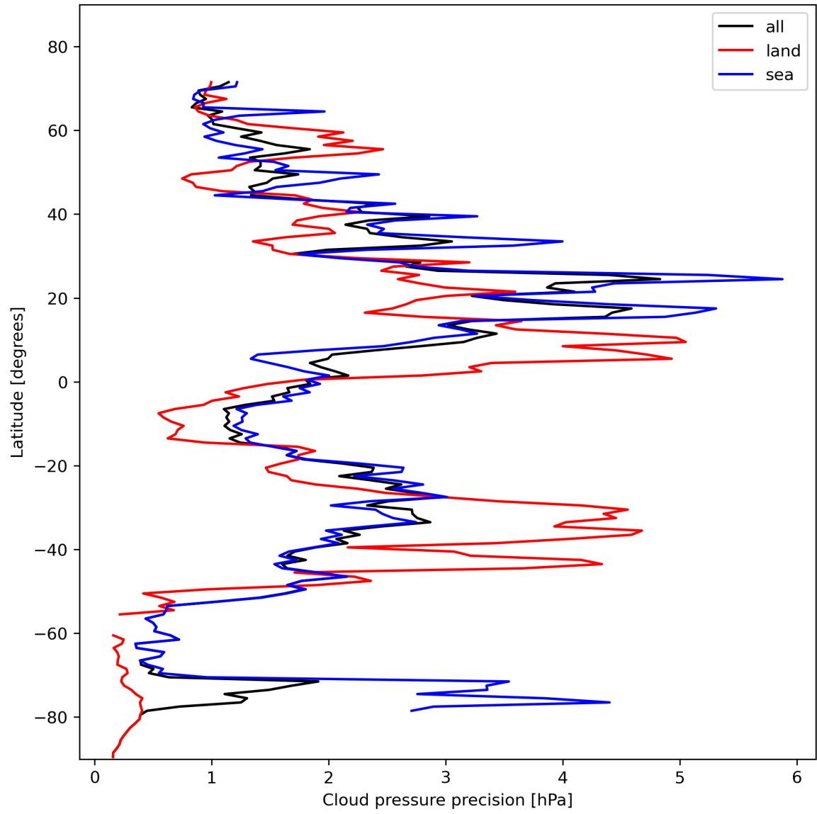
Figure 14: Zonal average of “Cloud pressure precision” for 2024-02-02 to 2024-02-04.
