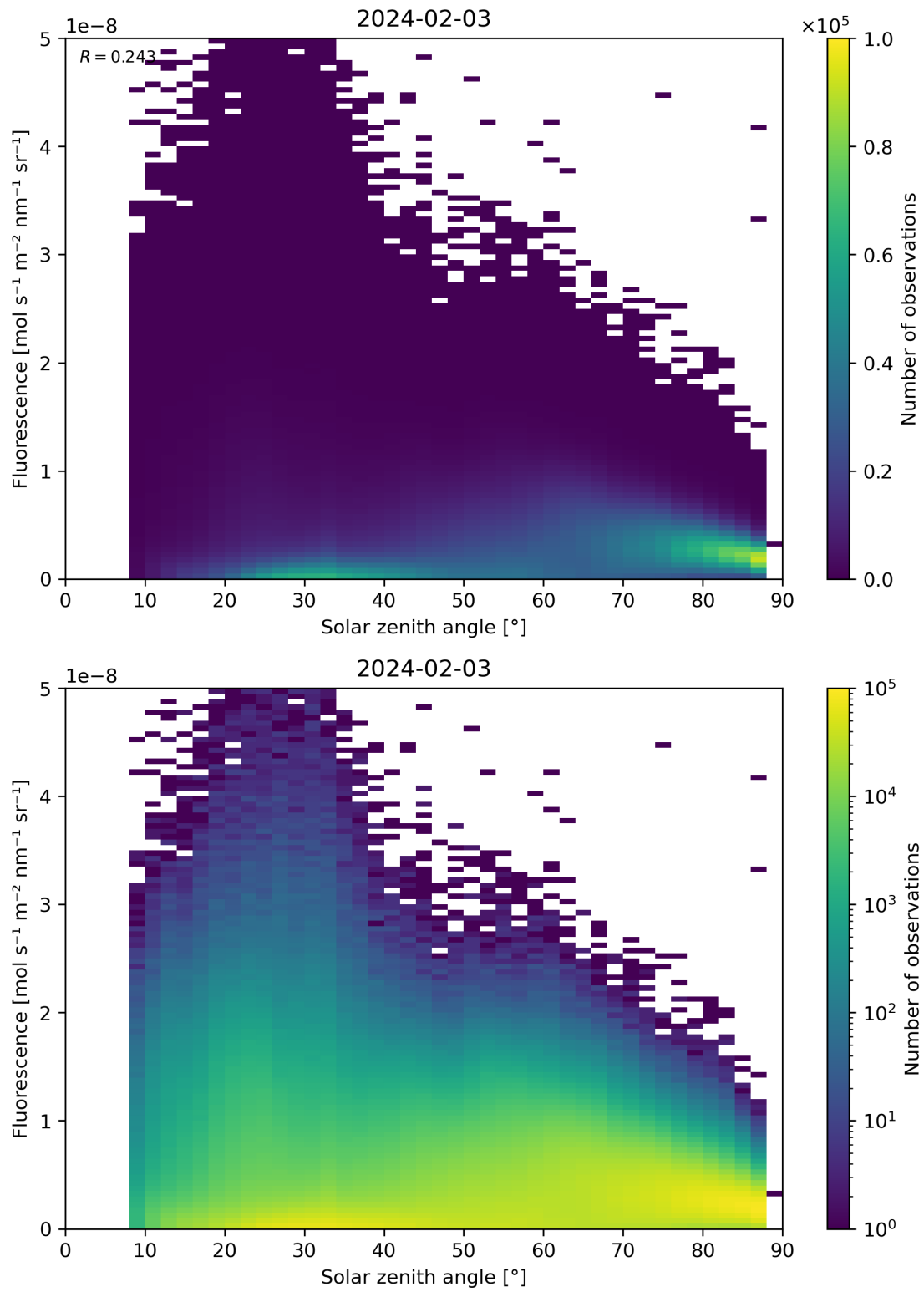
Figure 112: Scatter density plot of “Solar zenith angle” against “Fluorescence” for 2024-02-02 to 2024-02-04.
