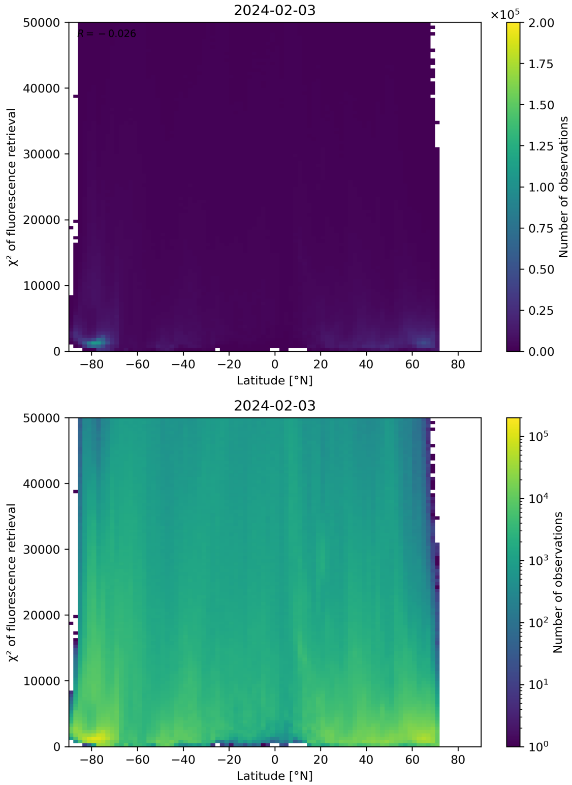
Figure 89: Scatter density plot of “Latitude” against “ \chi^2 of fluorescence retrieval” for 2024-02-02 to 2024-02-04.
