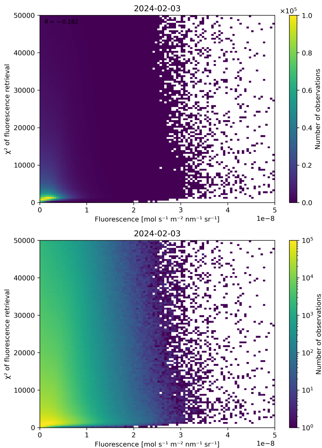
Figure 85: Scatter density plot of “Fluorescence” against “ \chi^2 of fluorescence retrieval” for 2024-02-02 to 2024-02-04.
