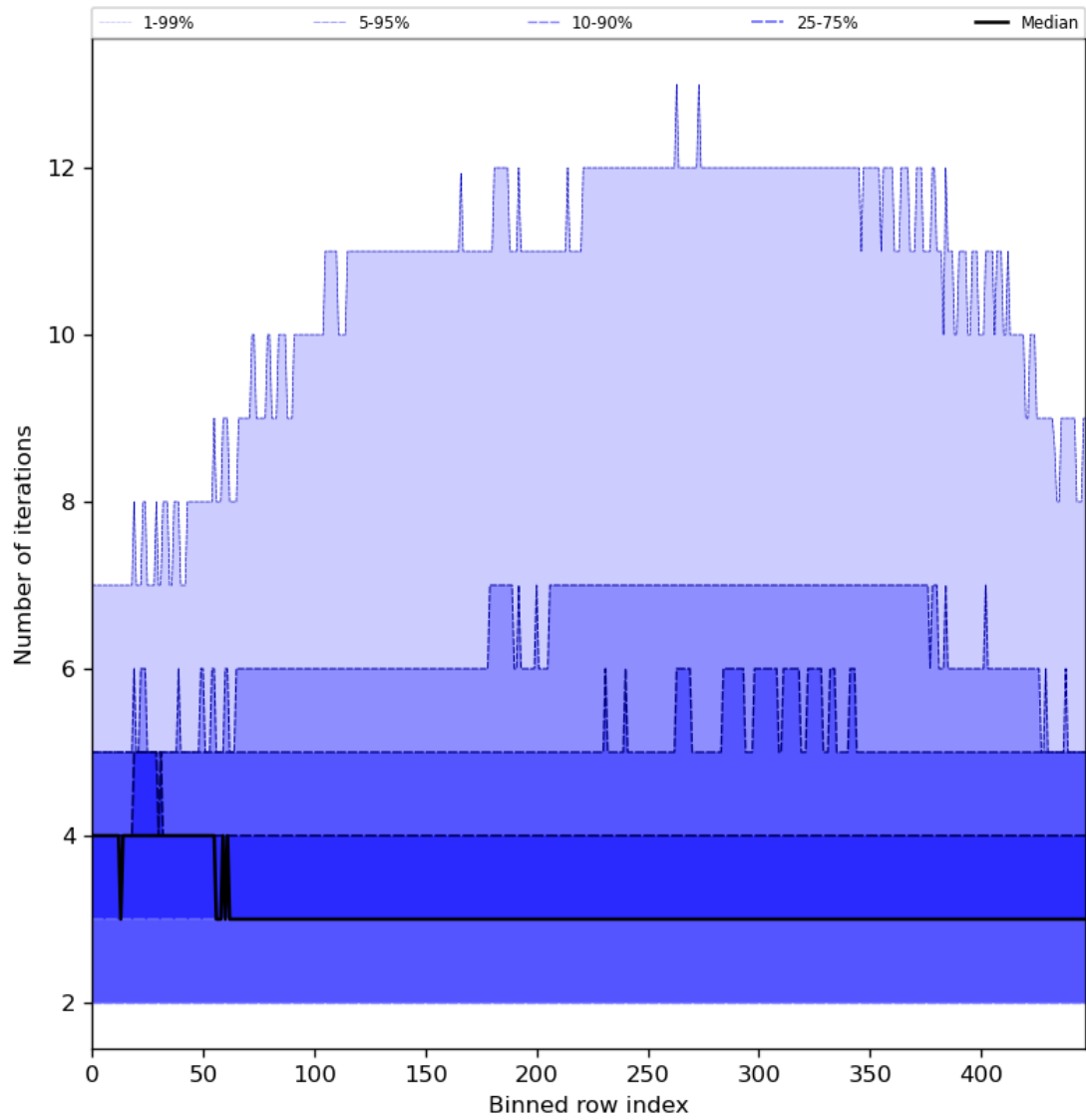
Figure 56: Along track statistics of “Number of iterations” for 2024-02-02 to 2024-02-04
