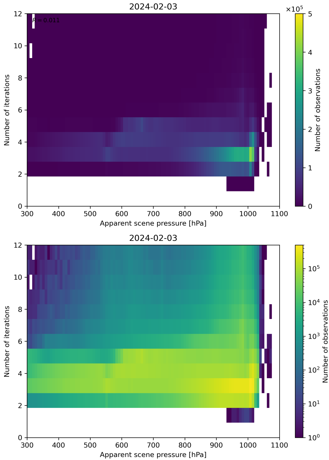
Figure 65: Scatter density plot of “Apparent scene pressure” against “Number of iterations” for 2024-02-02 to 2024-02-04.
