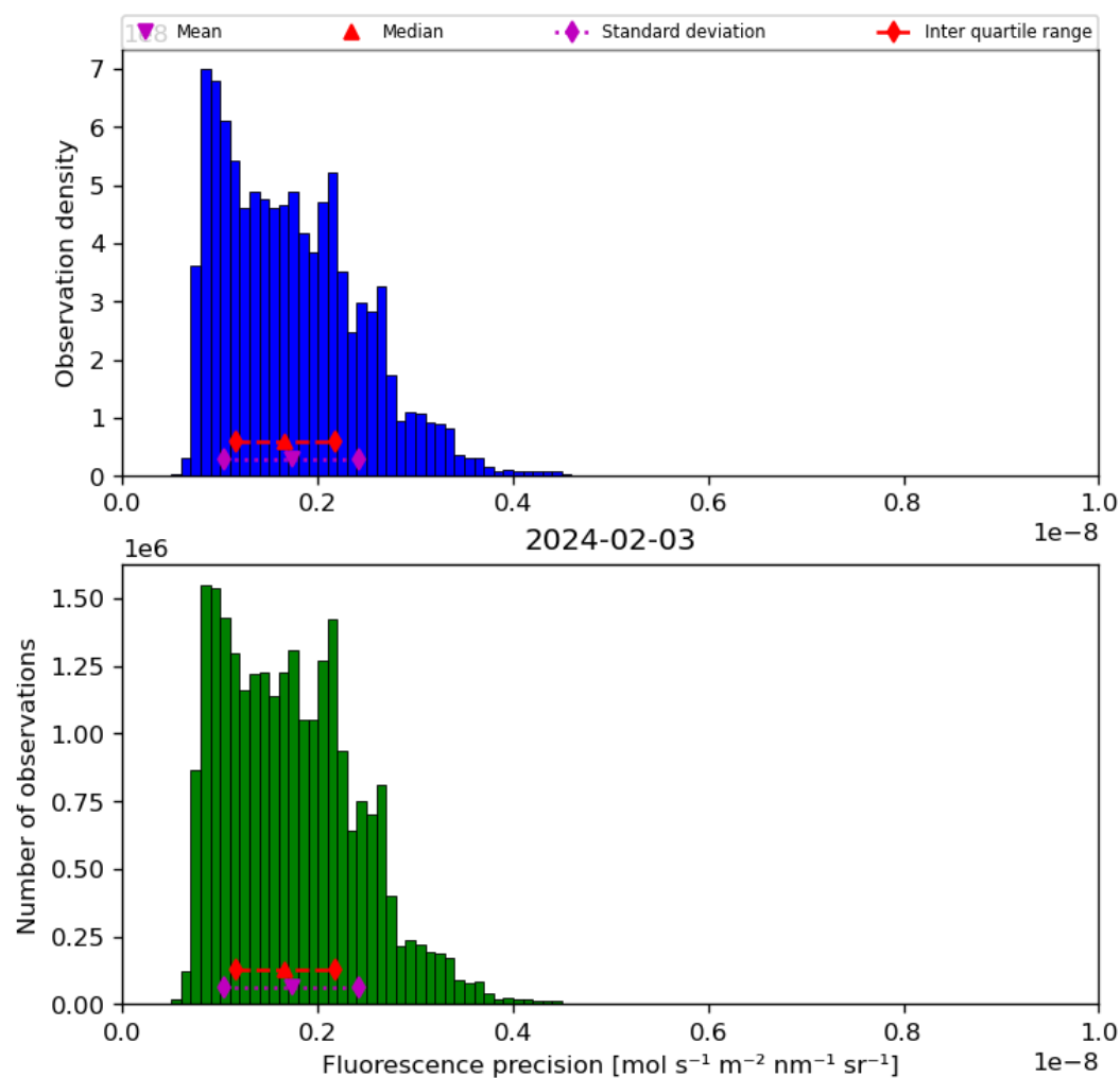
Figure 41: Histogram of “Fluorescence precision” for 2024-02-02 to 2024-02-04
