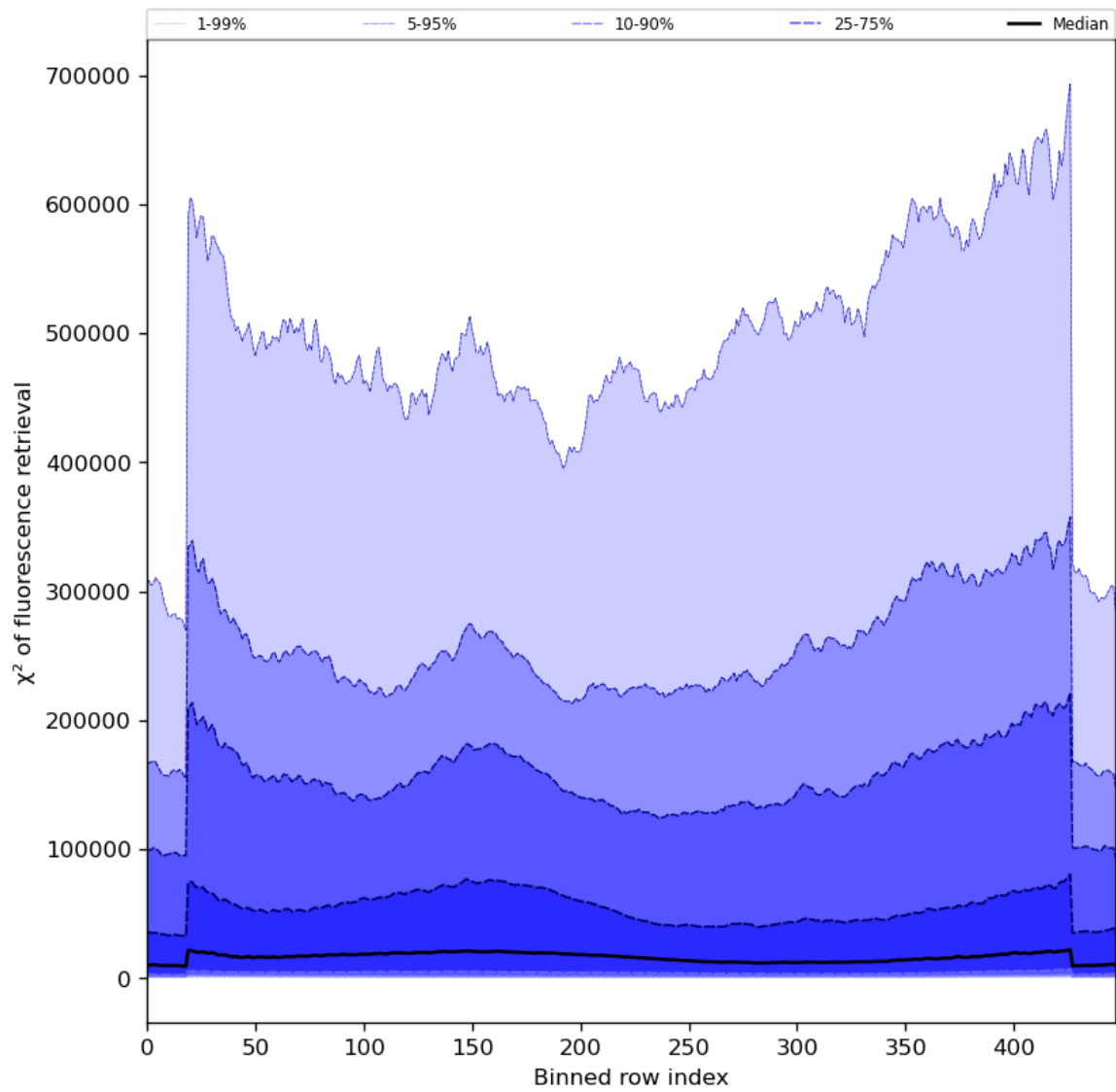
Figure 59: Along track statistics of “ \chi^2 of fluorescence retrieval” for 2024-02-02 to 2024-02-04
