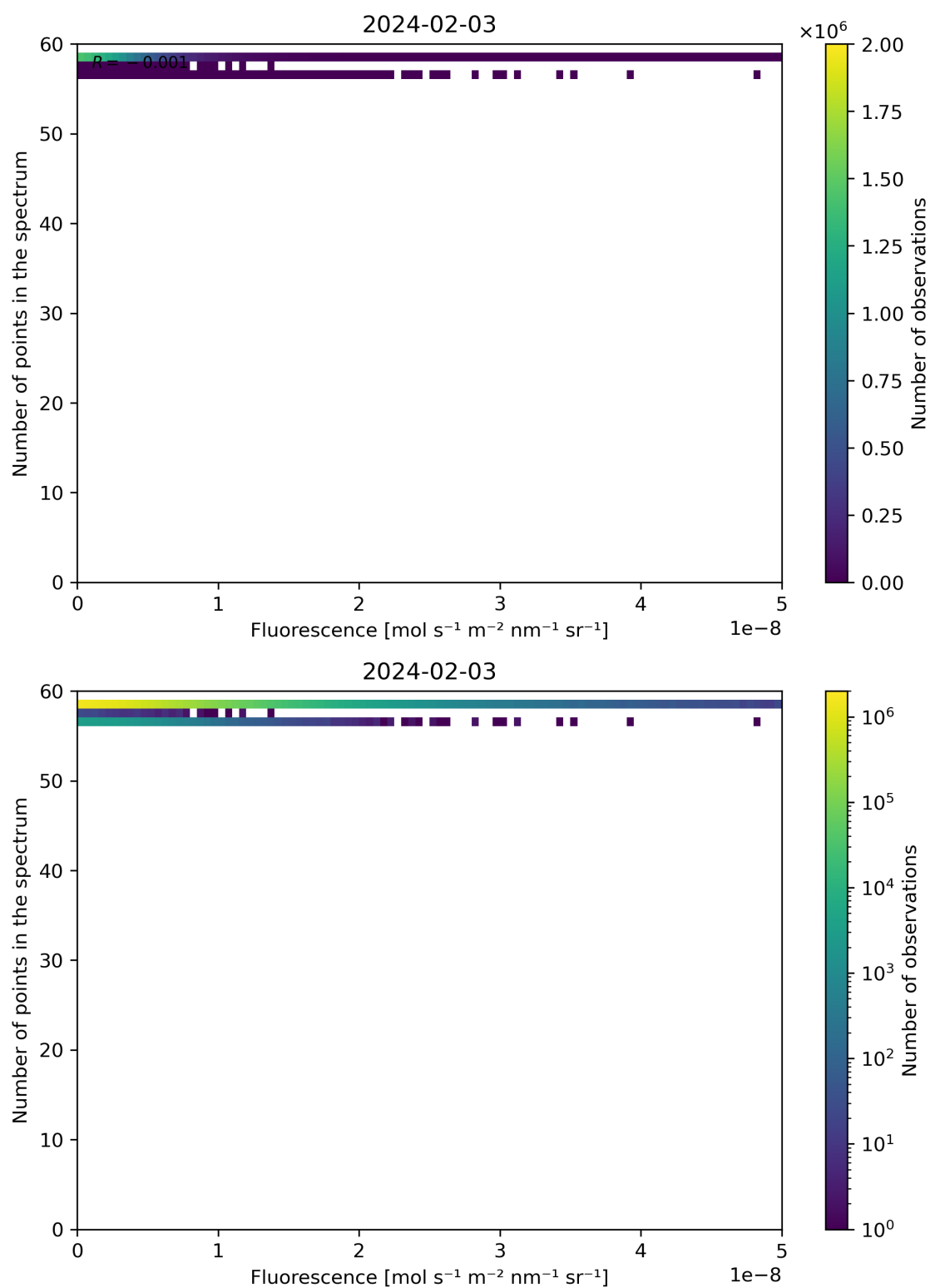
Figure 86: Scatter density plot of “Fluorescence” against “Number of points in the spectrum” for 2024-02-02 to 2024-02-04.
