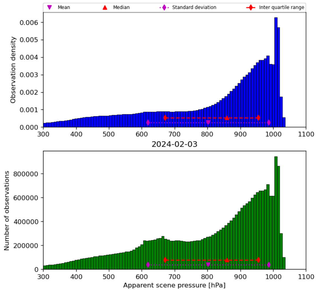
Figure 36: Histogram of “Apparent scene pressure” for 2024-02-02 to 2024-02-04
