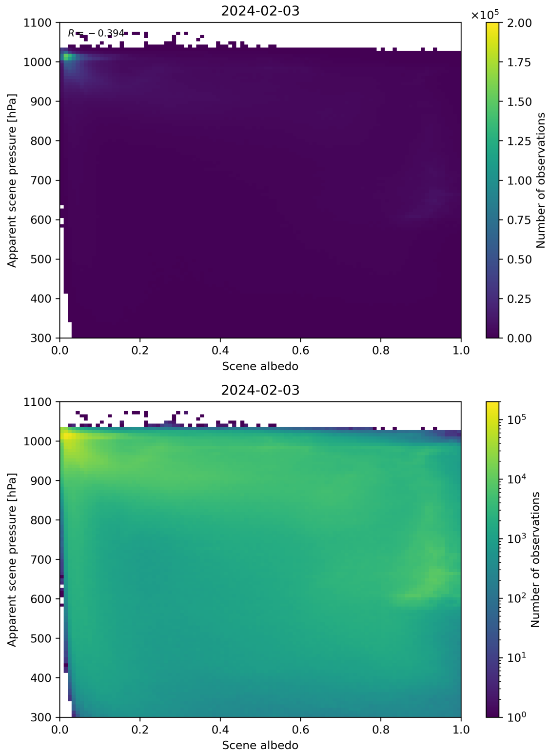
Figure 102: Scatter density plot of “Scene albedo” against “Apparent scene pressure” for 2024-02-02 to 2024-02-04.
