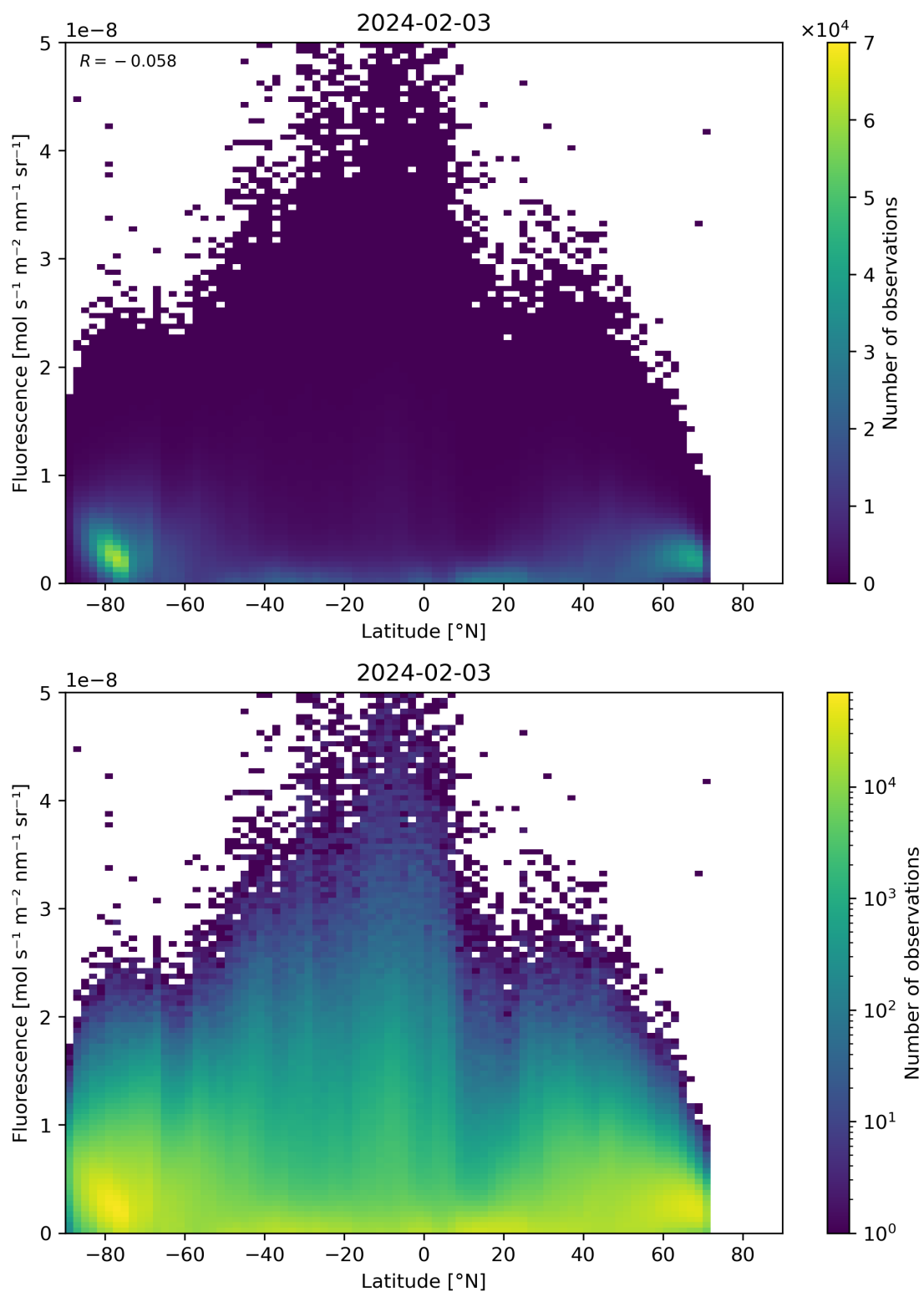
Figure 92: Scatter density plot of “Latitude” against “Fluorescence” for 2024-02-02 to 2024-02-04.
