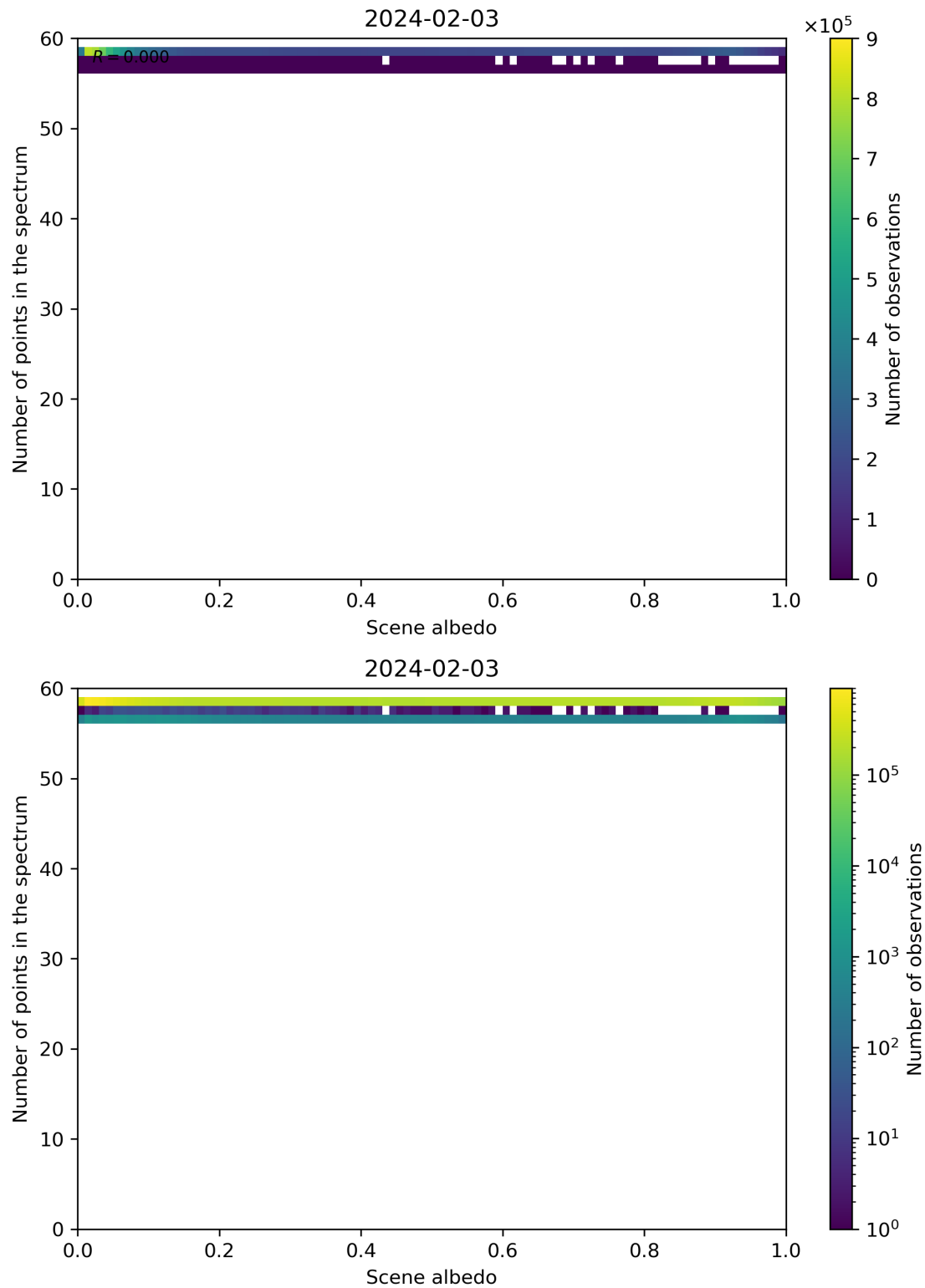
Figure 106: Scatter density plot of “Scene albedo” against “Number of points in the spectrum” for 2024-02-02 to 2024-02-04.
