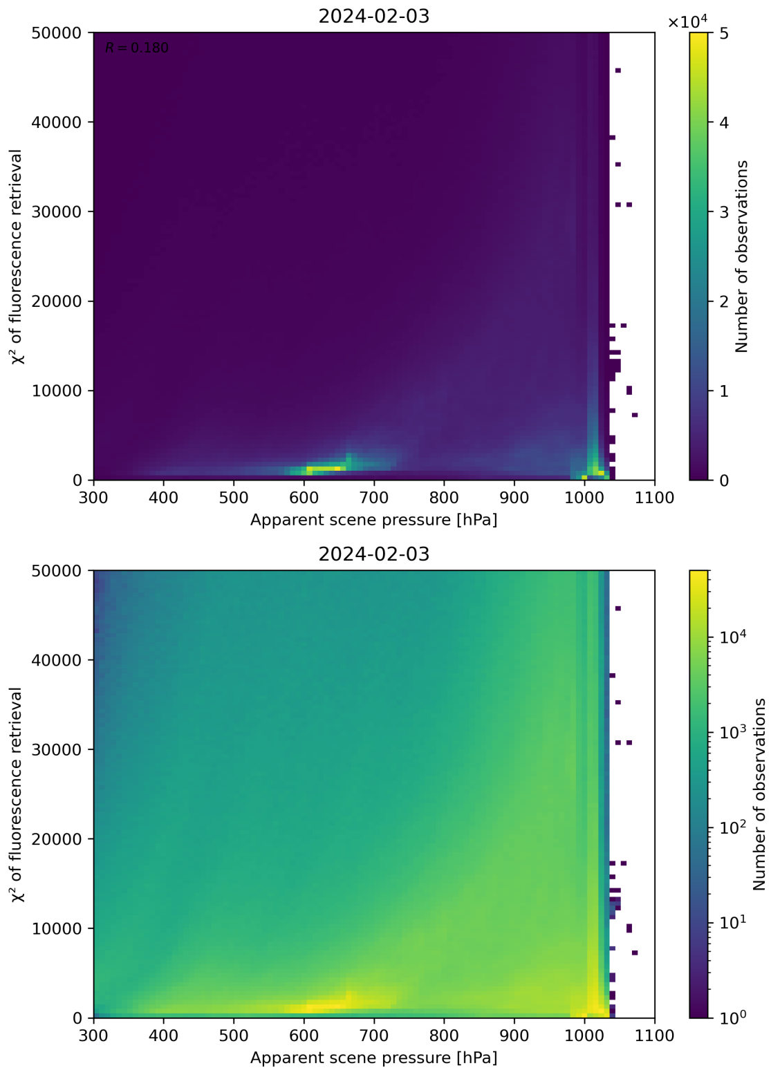
Figure 63: Scatter density plot of “Apparent scene pressure” against “ \chi^2 of fluorescence retrieval” for 2024-02-02 to 2024-02-04.
