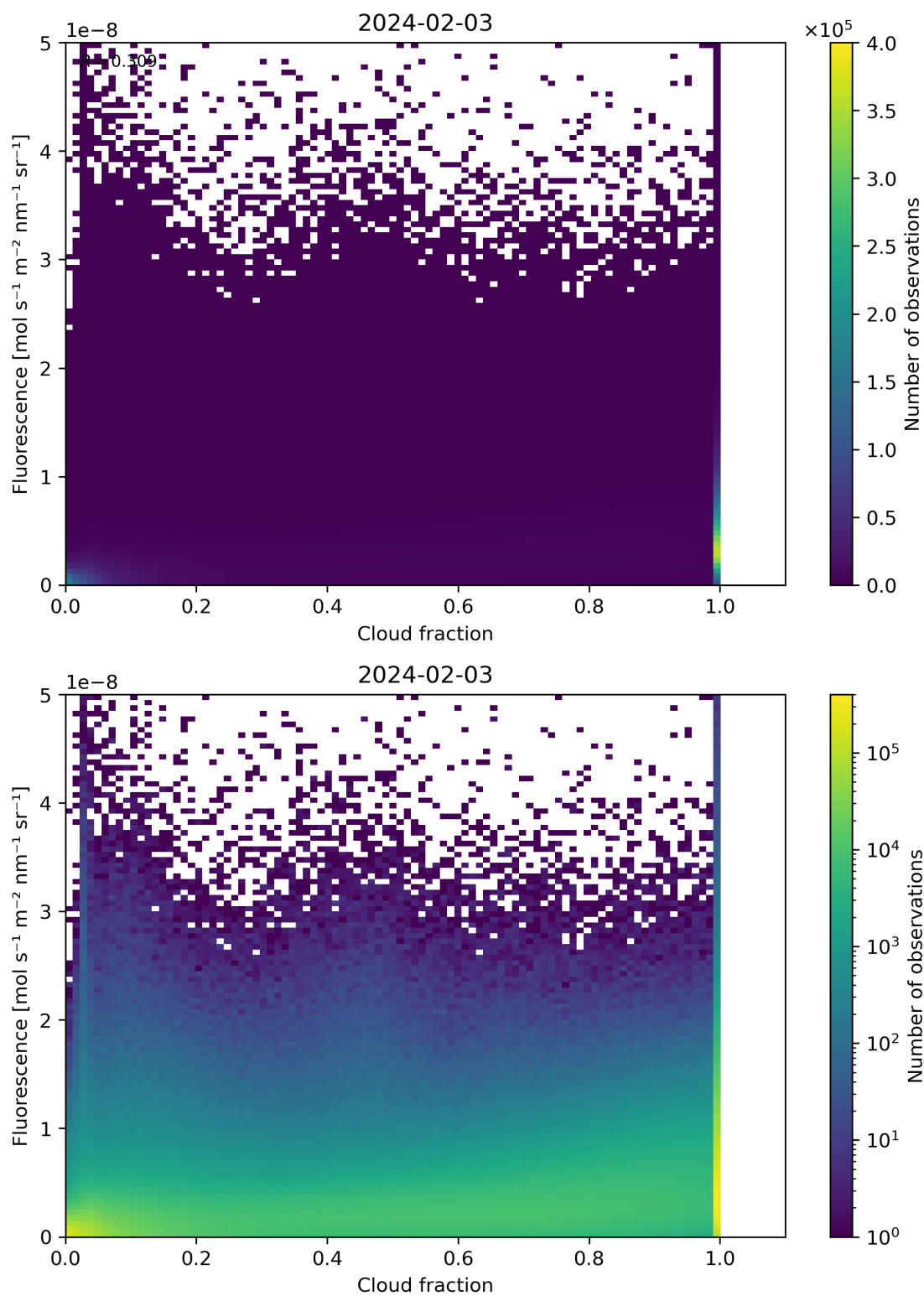
Figure 72: Scatter density plot of “Cloud fraction” against “Fluorescence” for 2024-02-02 to 2024-02-04.
