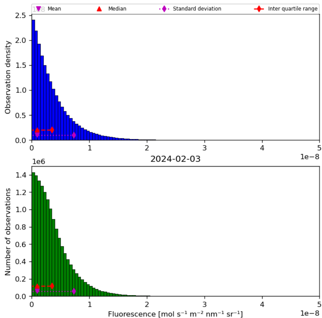
Figure 40: Histogram of “Fluorescence” for 2024-02-02 to 2024-02-04
