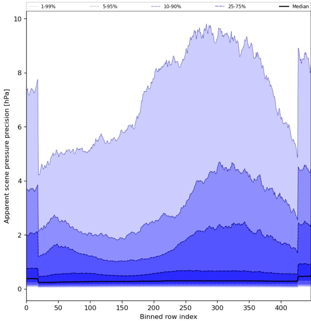
Figure 54: Along track statistics of “Apparent scene pressure precision” for 2024-02-02 to 2024-02-04
