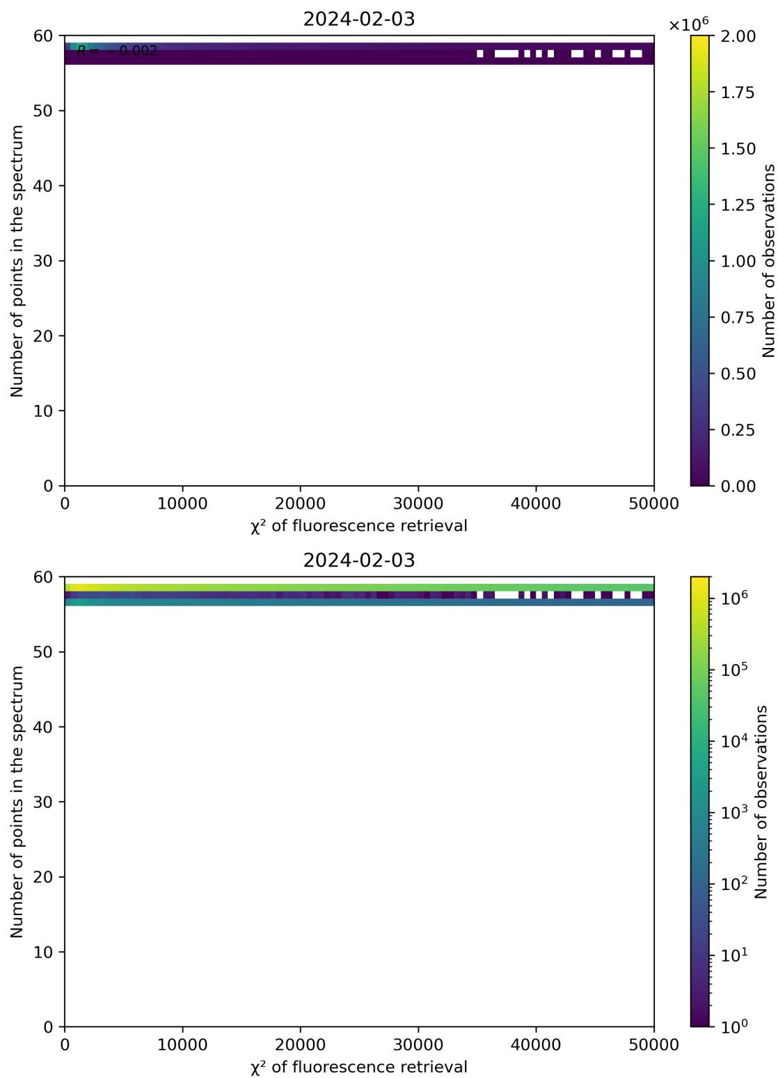
Figure 68: Scatter density plot of " \chi^2 of fluorescence retrieval" against "Number of points in the spectrum" for 2024-02-02 to 2024-02-04.
