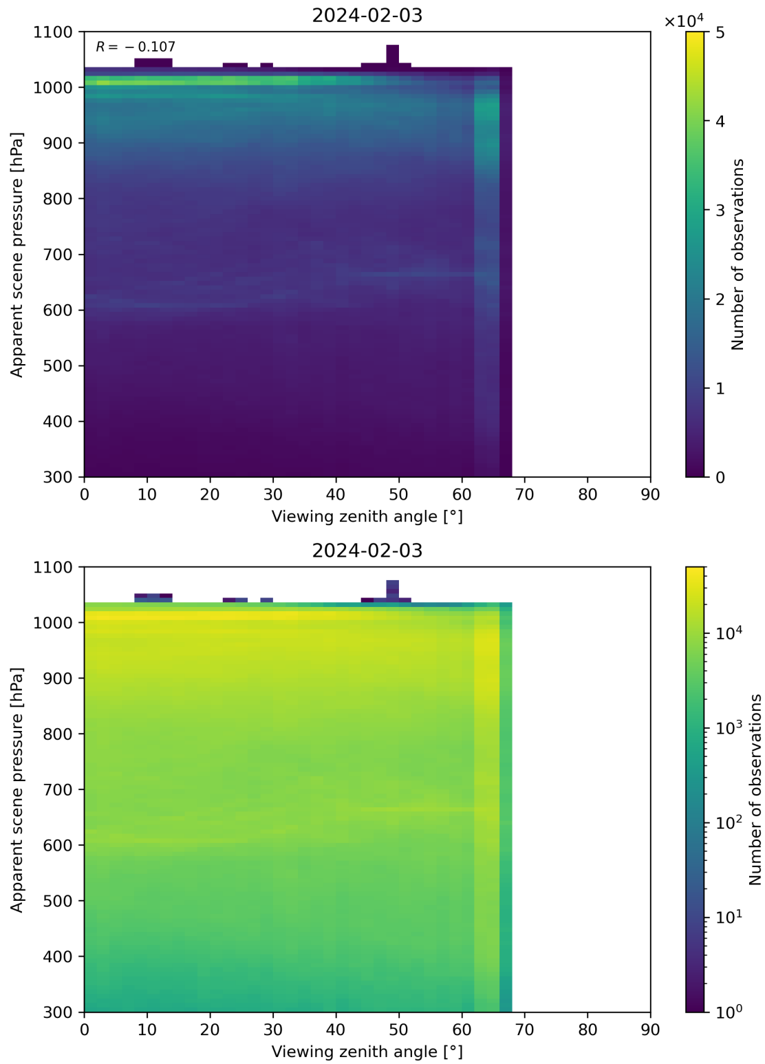
Figure 118: Scatter density plot of “Viewing zenith angle” against “Apparent scene pressure” for 2024-02-02 to 2024-02-04.
