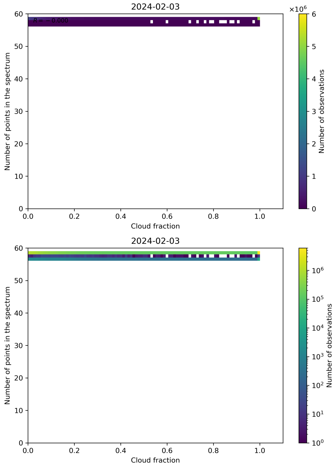
Figure 74: Scatter density plot of “Cloud fraction” against “Number of points in the spectrum” for 2024-02-02 to 2024-02-04.
