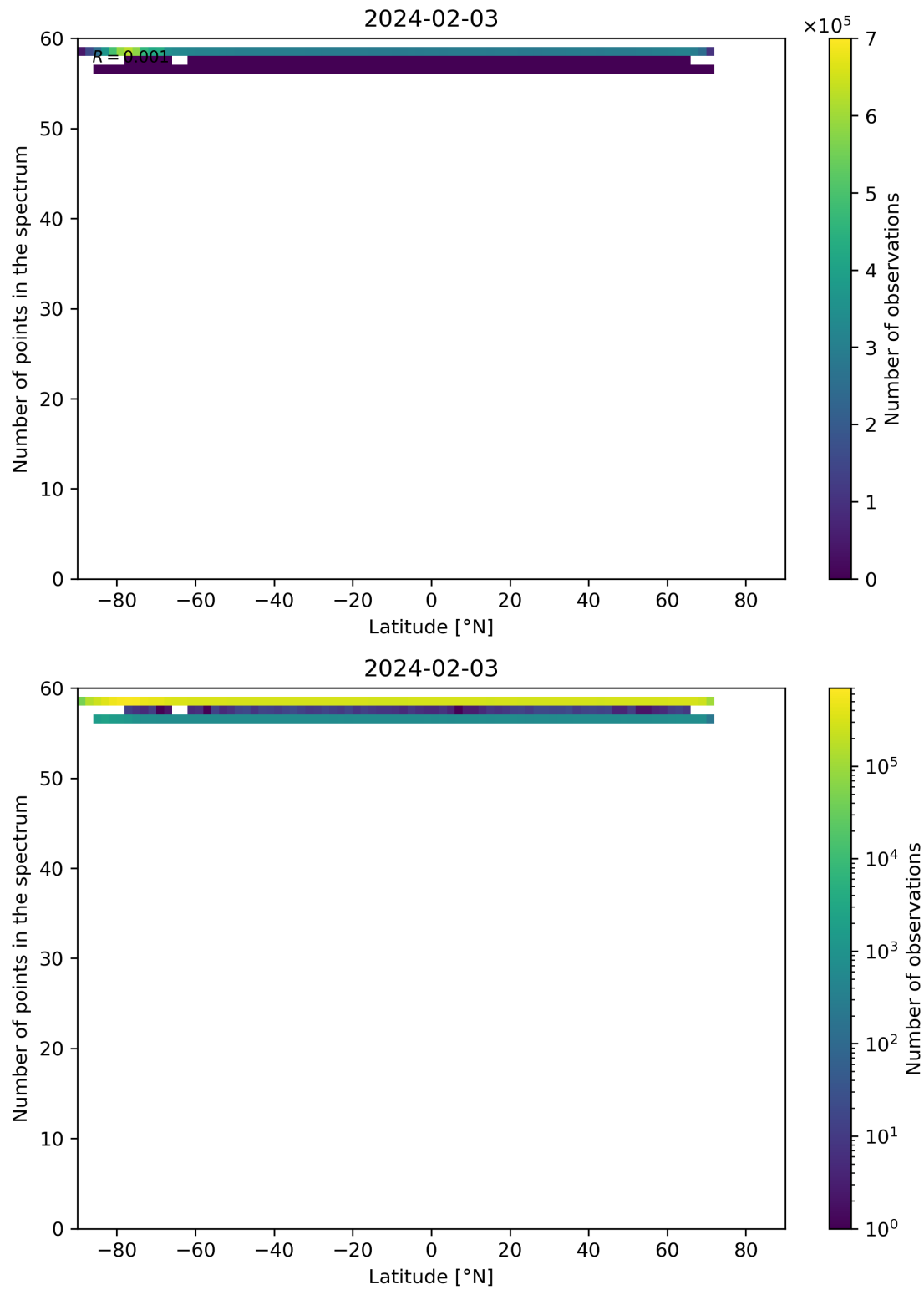
Figure 94: Scatter density plot of “Latitude” against “Number of points in the spectrum” for 2024-02-02 to 2024-02-04.
