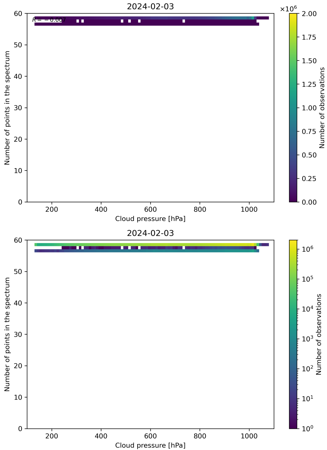
Figure 82: Scatter density plot of “Cloud pressure” against “Number of points in the spectrum” for 2024-02-02 to 2024-02-04.
