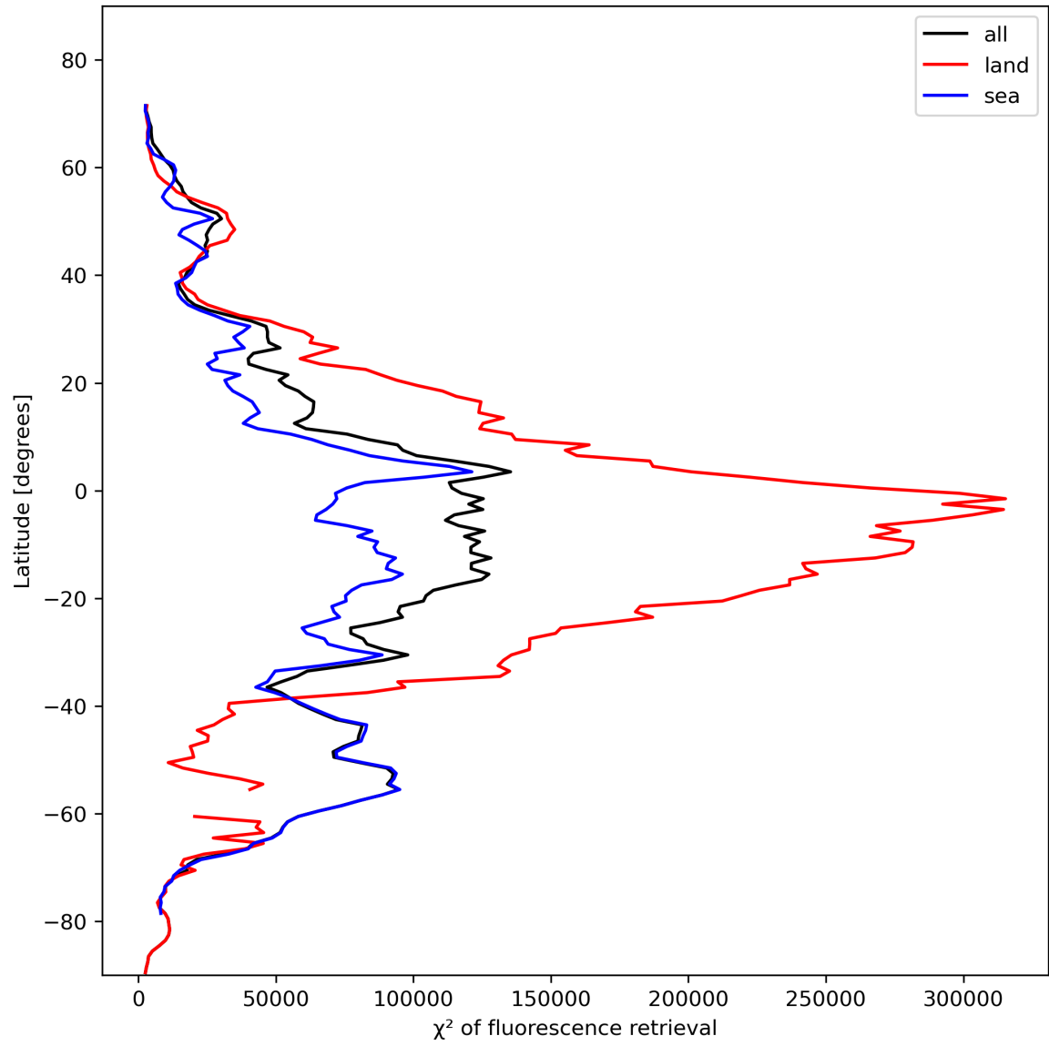
Figure 25: Zonal average of “ \chi^2 of fluorescence retrieval” for 2024-02-02 to 2024-02-04.
