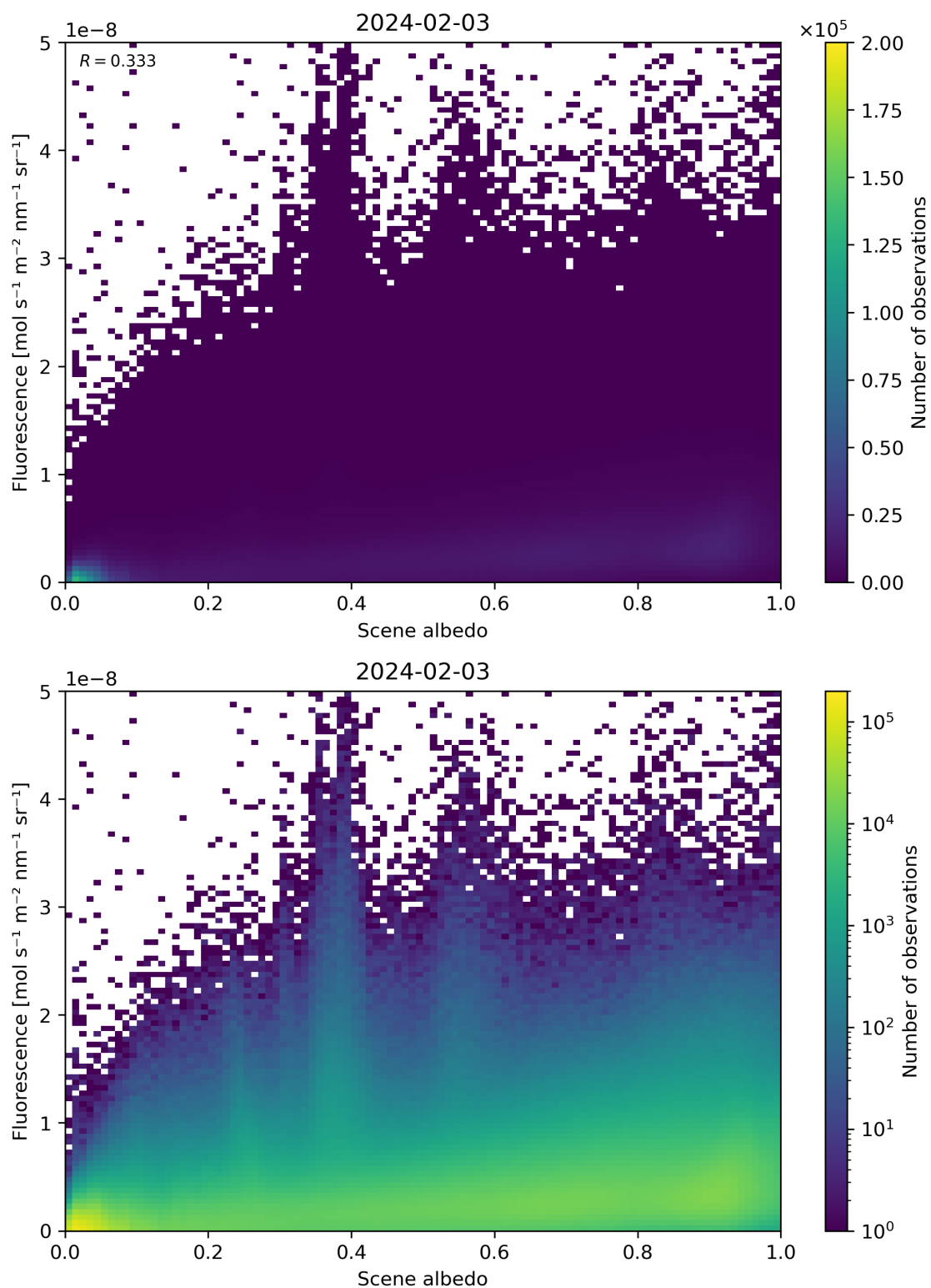
Figure 104: Scatter density plot of “Scene albedo” against “Fluorescence” for 2024-02-02 to 2024-02-04.
