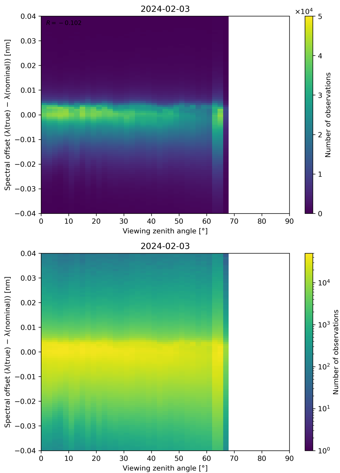
Figure 128: Scatter density plot of “Viewing zenith angle” against “Spectral offset ( \lambda(\text{true}) - \lambda(\text{nominal}) )” for 2024-02-02 to 2024-02-04.
