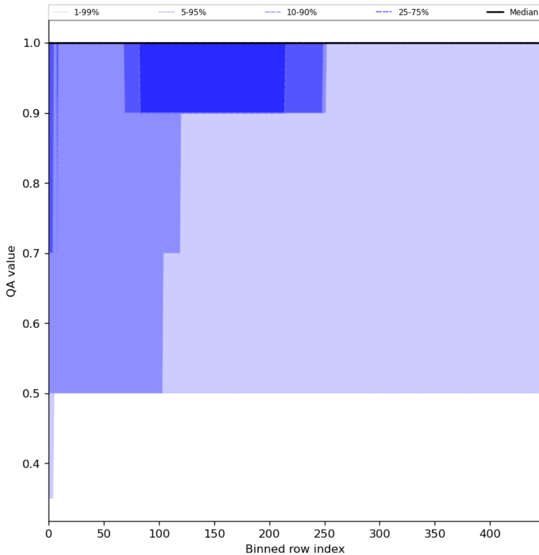
Figure 46: Along track statistics of “QA value” for 2024-02-02 to 2024-02-04
