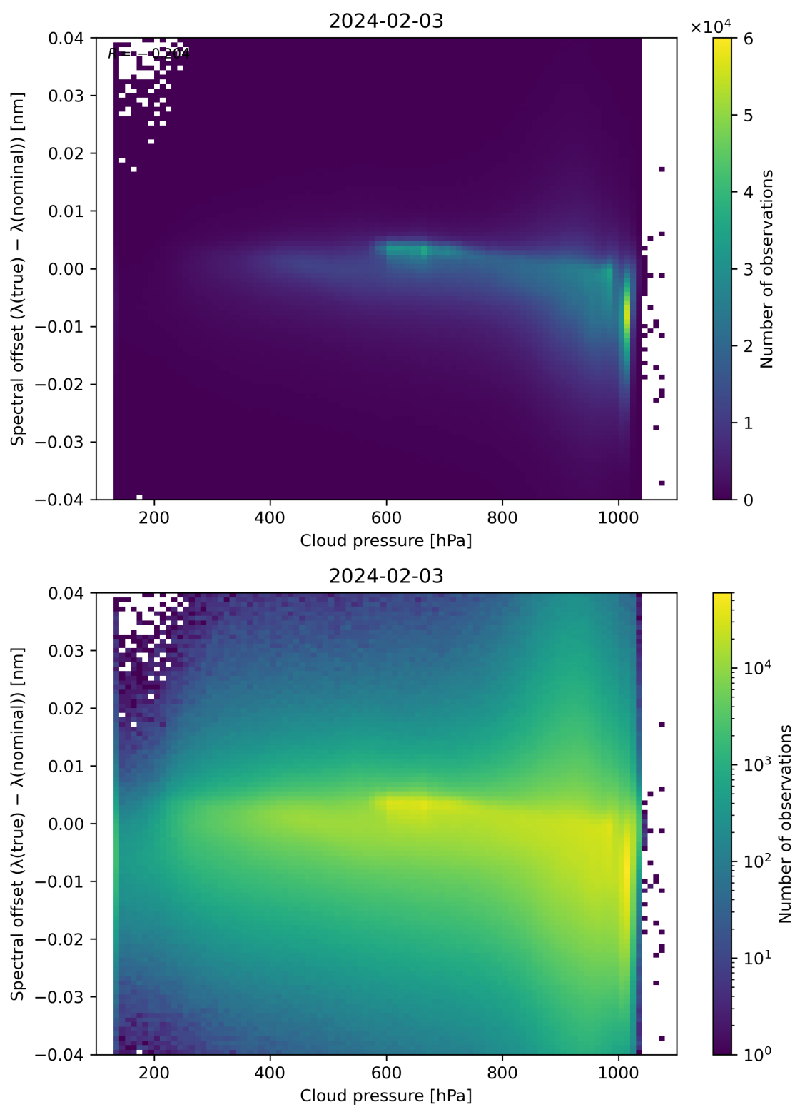
Figure 84: Scatter density plot of “Cloud pressure” against “Spectral offset ( \lambda(\text{true}) - \lambda(\text{nominal}) )” for 2024-02-02 to 2024-02-04.
