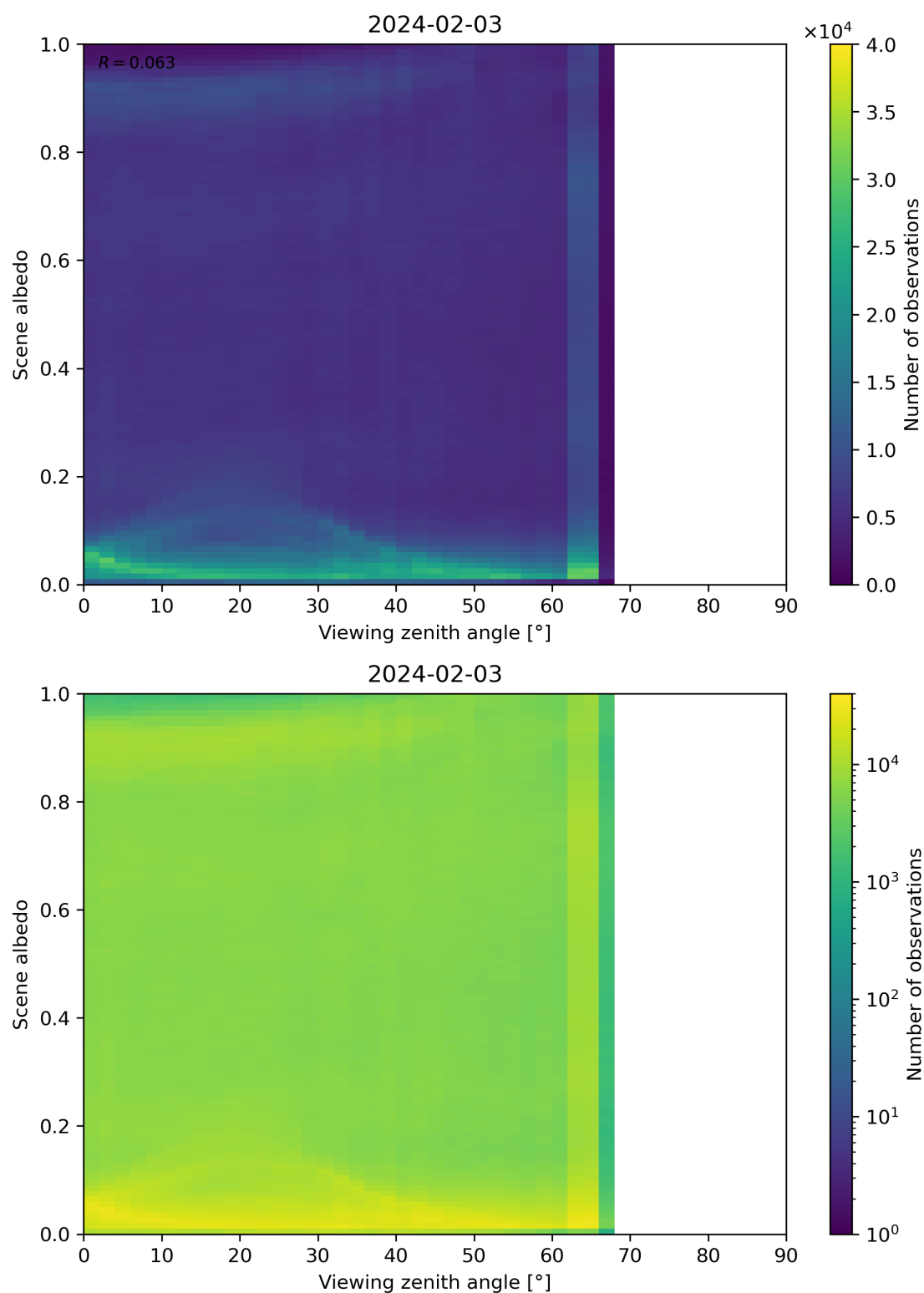
Figure 126: Scatter density plot of “Viewing zenith angle” against “Scene albedo” for 2024-02-02 to 2024-02-04.
