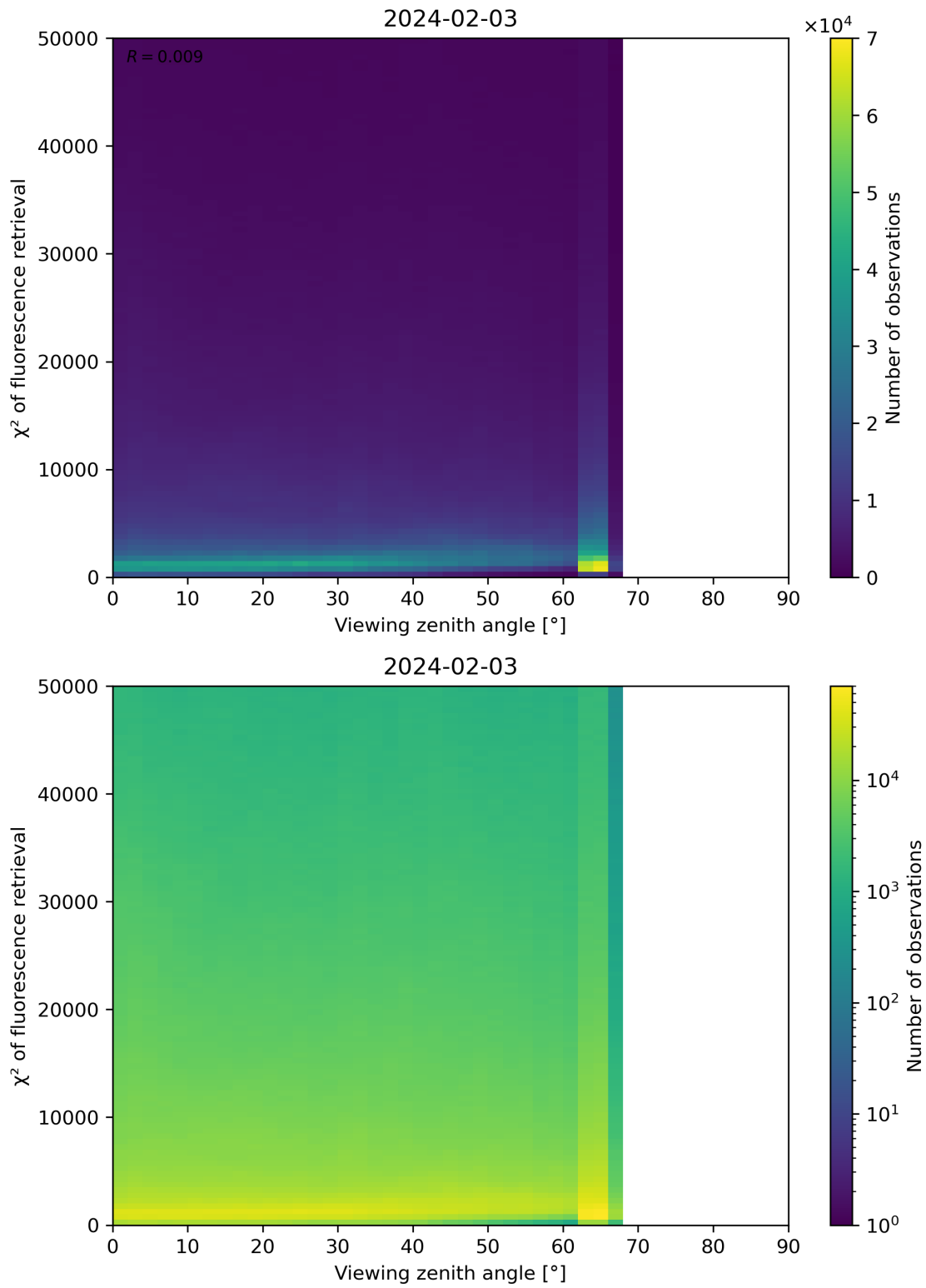
Figure 119: Scatter density plot of “Viewing zenith angle” against “ \chi^2 of fluorescence retrieval” for 2024-02-02 to 2024-02-04.
