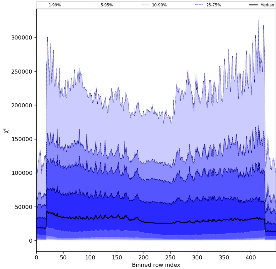
Figure 55: Along track statistics of “ \chi^2 ” for 2024-02-02 to 2024-02-04
