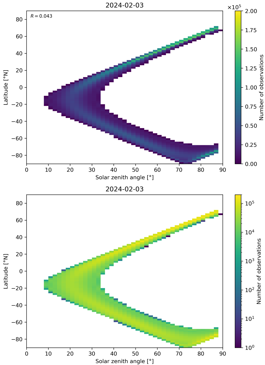
Figure 113: Scatter density plot of “Solar zenith angle” against “Latitude” for 2024-02-02 to 2024-02-04.
