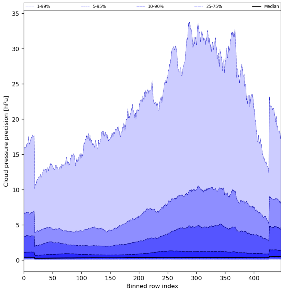
Figure 48: Along track statistics of “Cloud pressure precision” for 2024-02-02 to 2024-02-04
