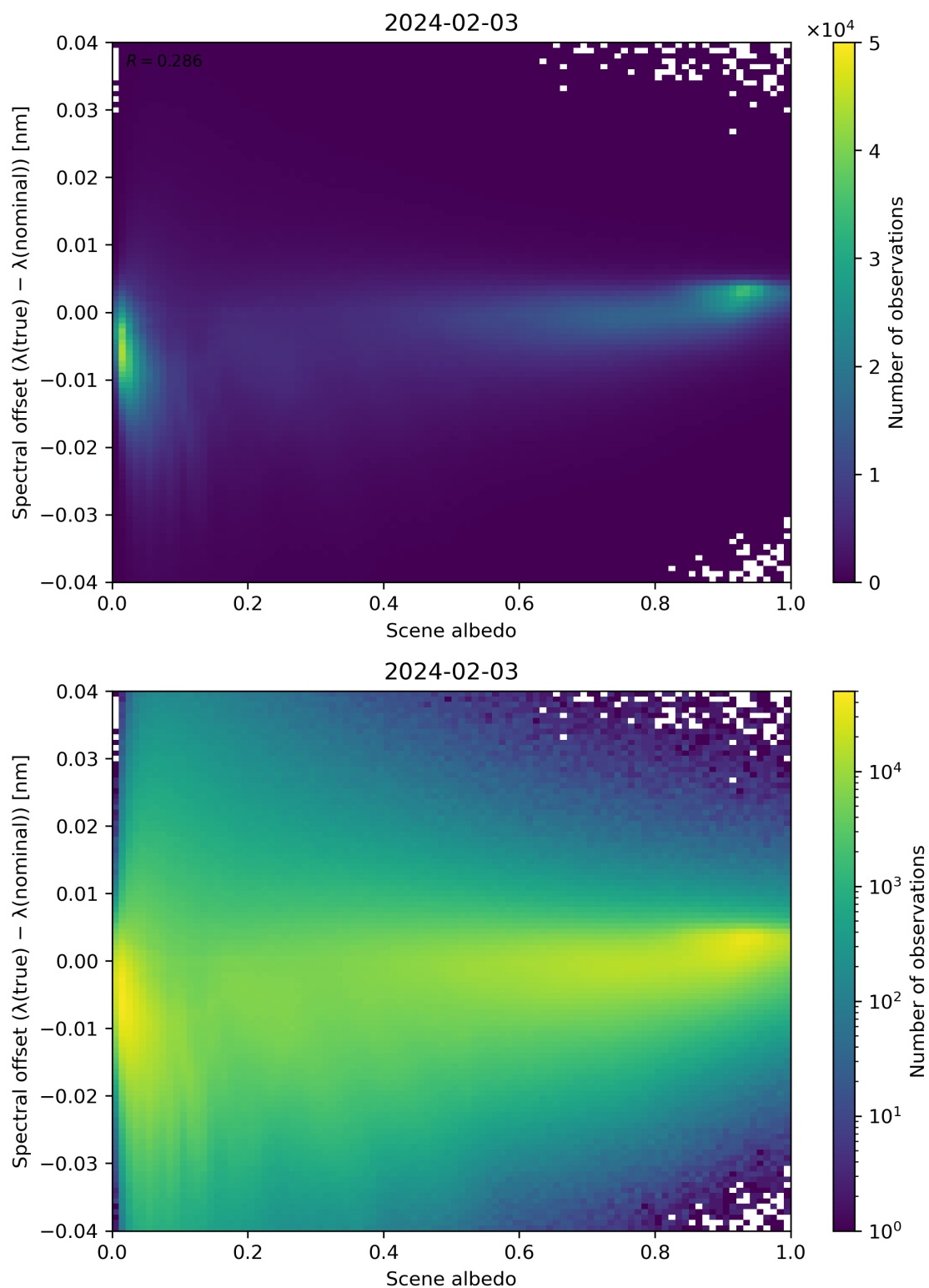
Figure 107: Scatter density plot of “Scene albedo” against “Spectral offset ( \lambda(\text{true}) - \lambda(\text{nominal}) )” for 2024-02-02 to 2024-02-04.
