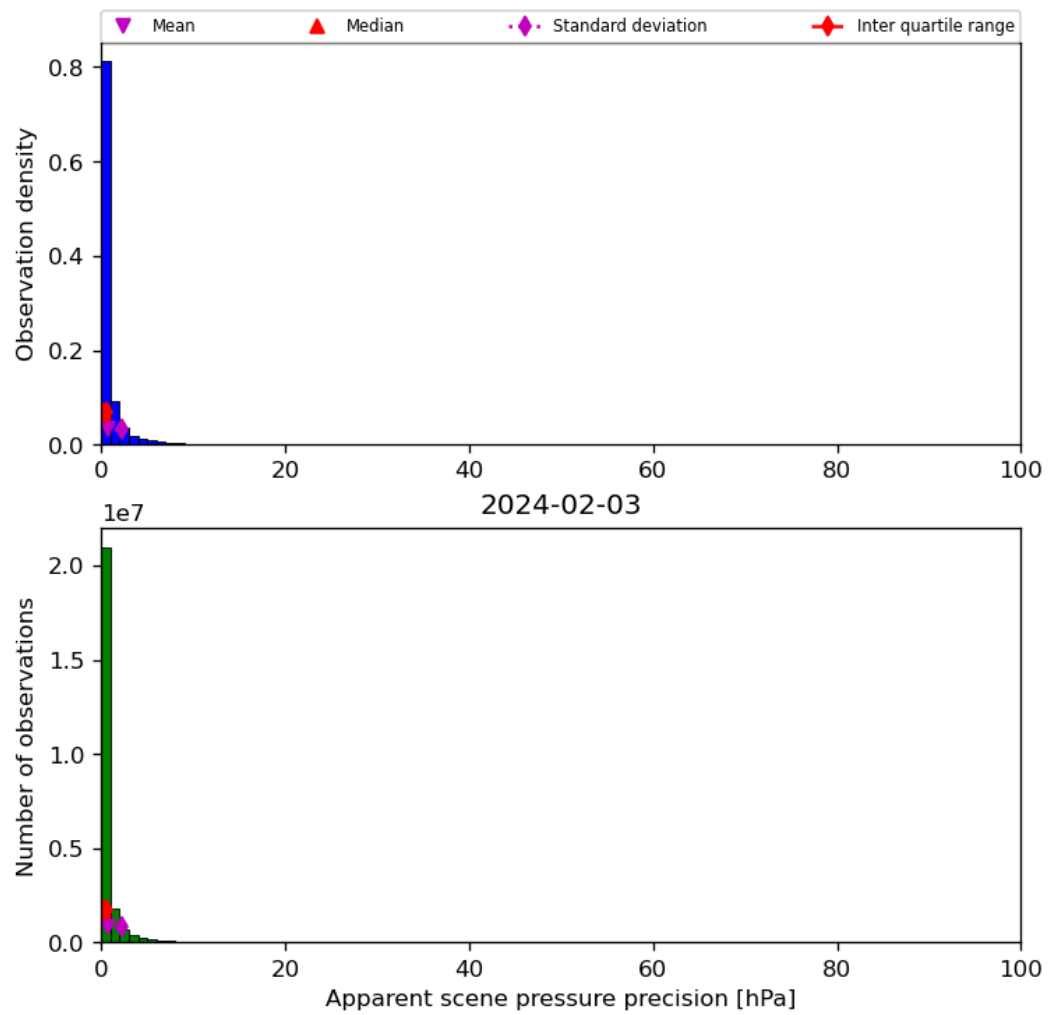
Figure 37: Histogram of “Apparent scene pressure precision” for 2024-02-02 to 2024-02-04
