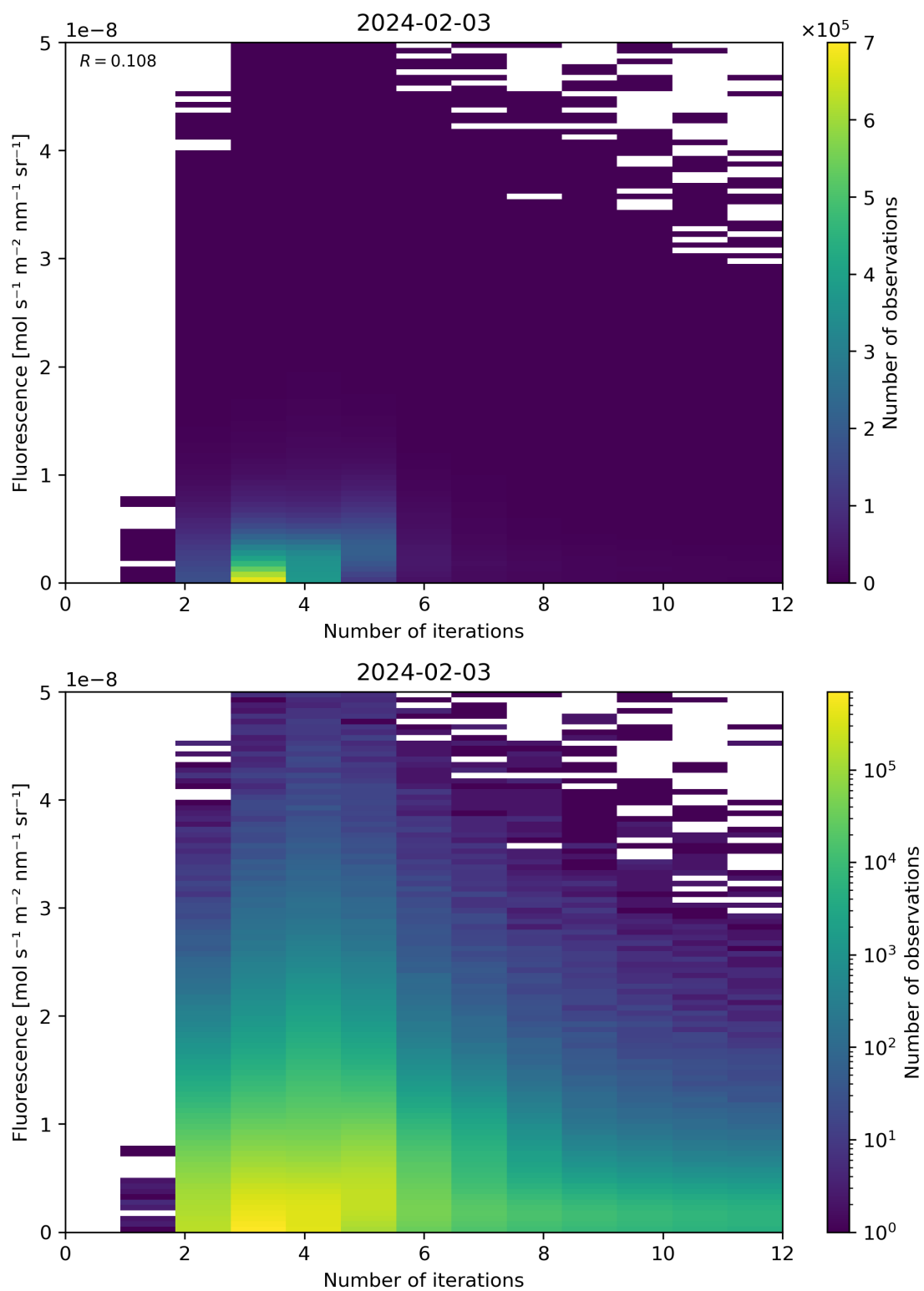
Figure 98: Scatter density plot of “Number of iterations” against “Fluorescence” for 2024-02-02 to 2024-02-04.
