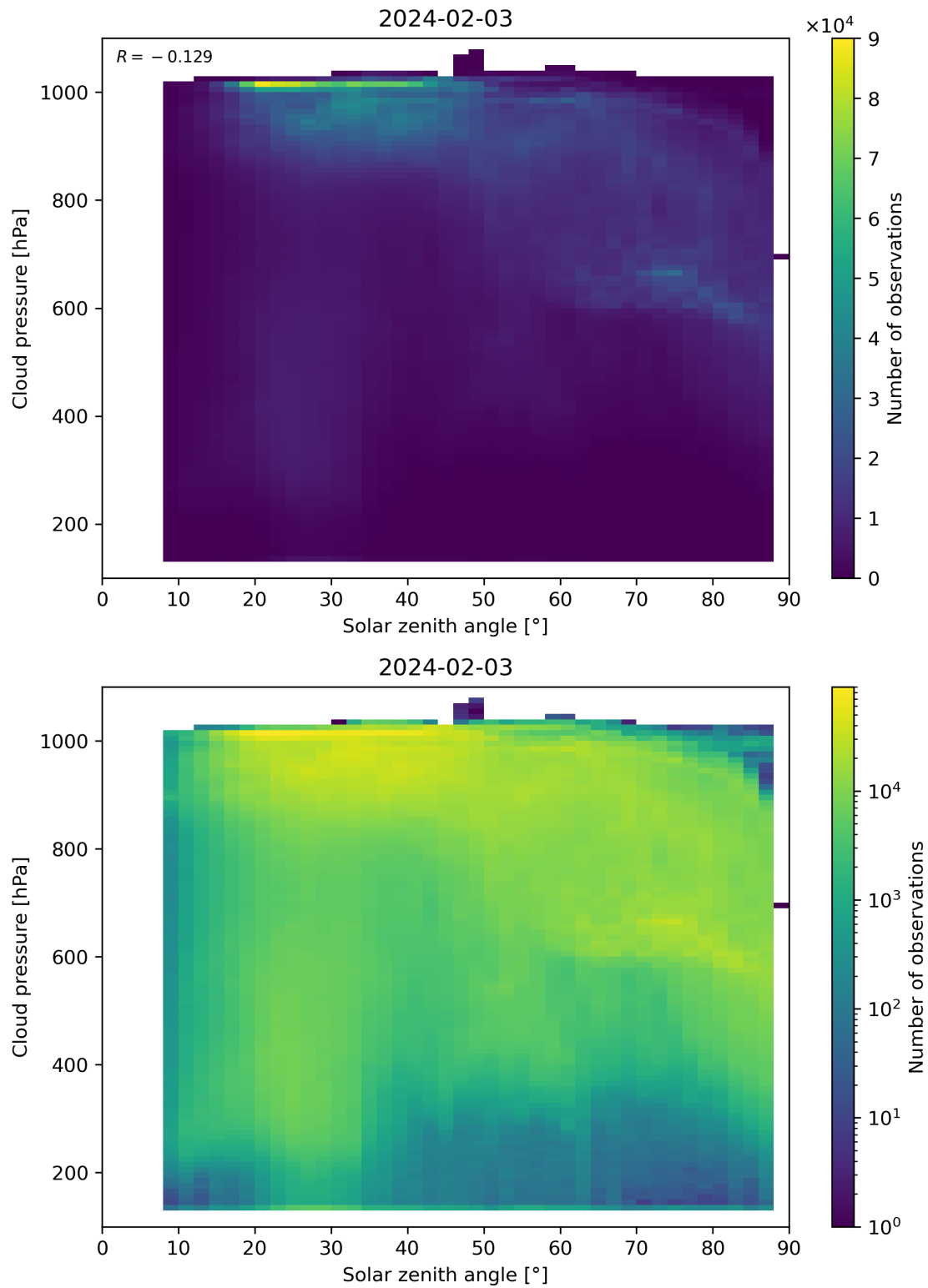
Figure 111: Scatter density plot of “Solar zenith angle” against “Cloud pressure” for 2024-02-02 to 2024-02-04.
