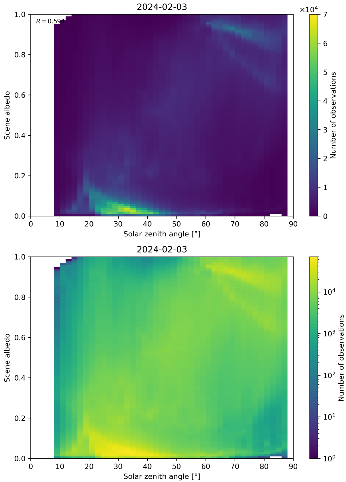
Figure 116: Scatter density plot of “Solar zenith angle” against “Scene albedo” for 2024-02-02 to 2024-02-04.
