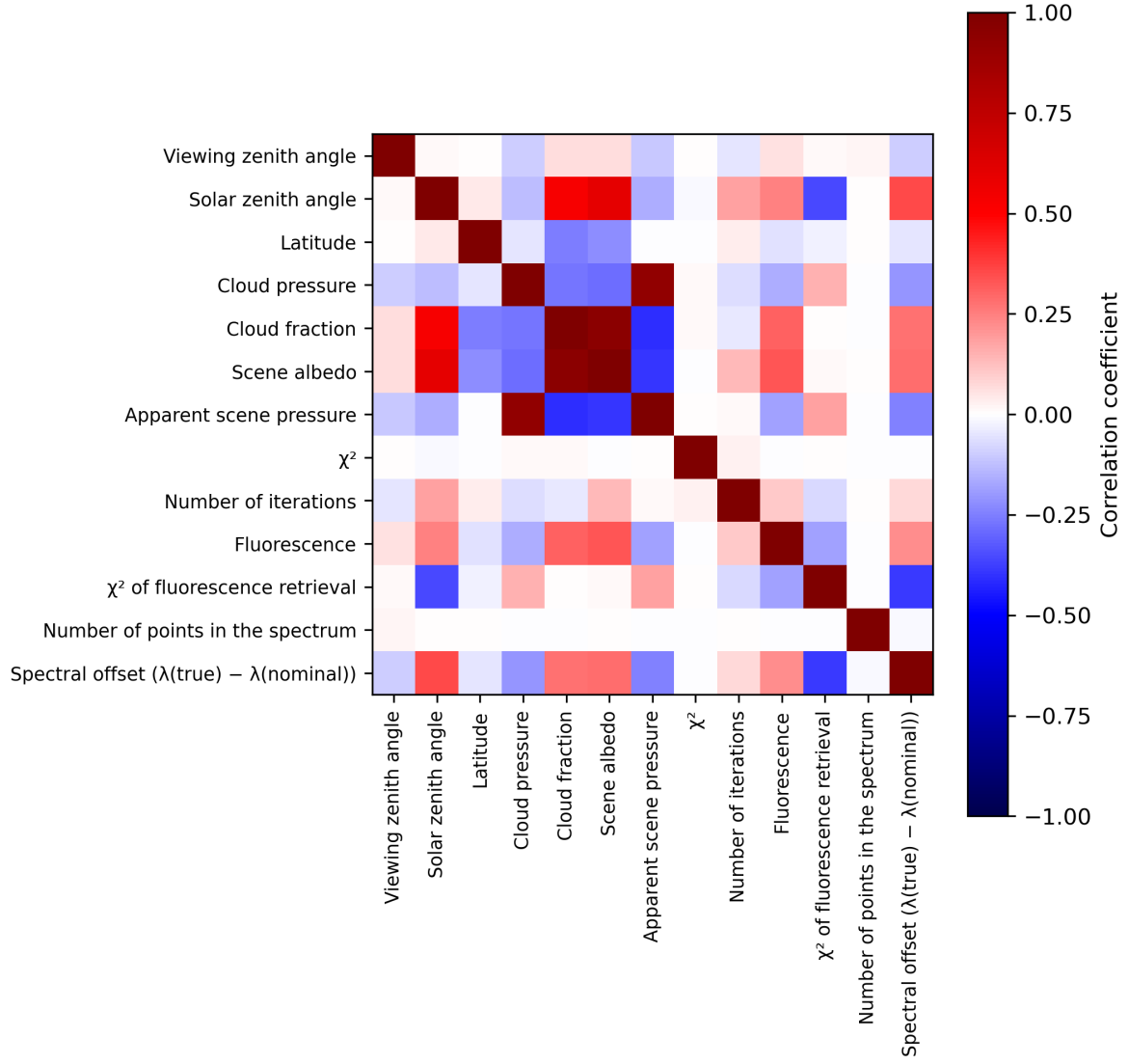
Figure 2: Map of correlation matrix for 2024-02-02 to 2024-02-04.
