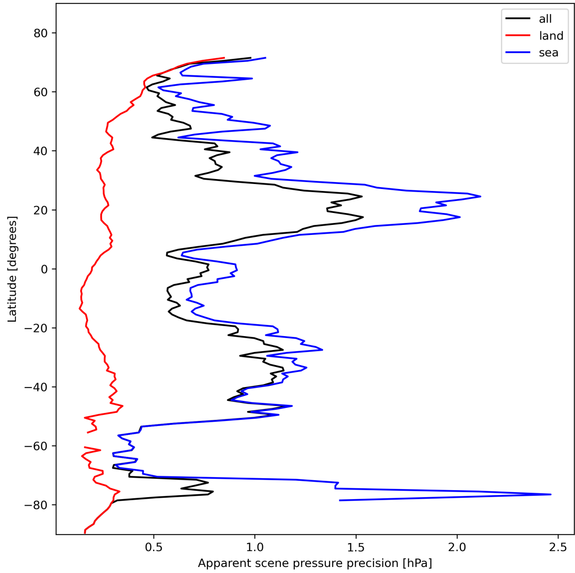
Figure 20: Zonal average of “Apparent scene pressure precision” for 2024-02-02 to 2024-02-04.
