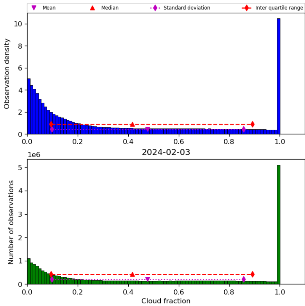
Figure 32: Histogram of “Cloud fraction” for 2024-02-02 to 2024-02-04
