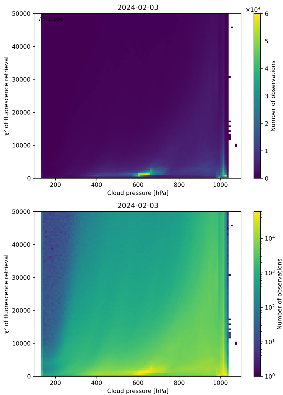
Figure 78: Scatter density plot of “Cloud pressure” against “ \chi^2 of fluorescence retrieval” for 2024-02-02 to 2024-02-04.
