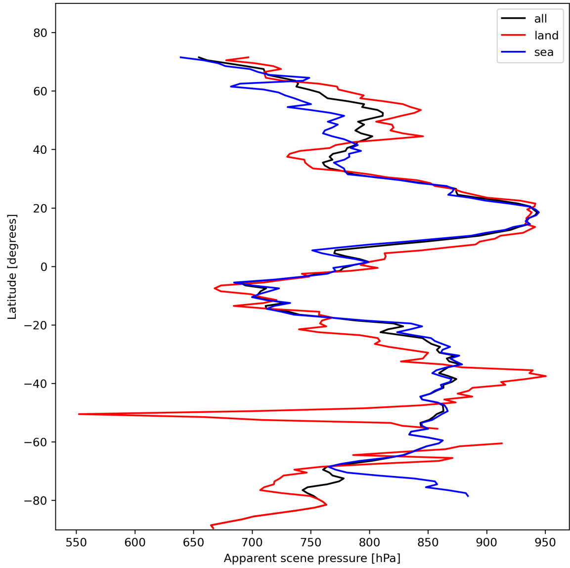
Figure 19: Zonal average of “Apparent scene pressure” for 2024-02-02 to 2024-02-04.
