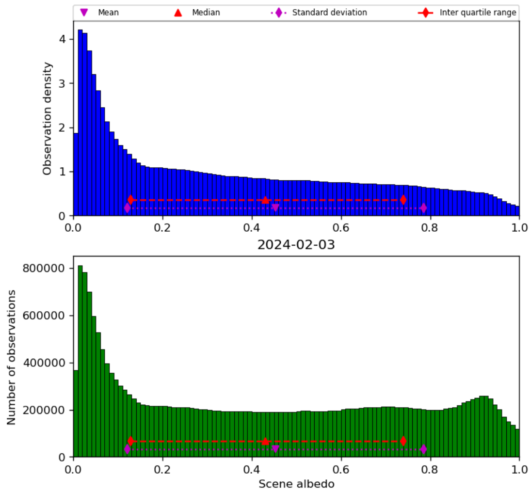
Figure 34: Histogram of “Scene albedo” for 2024-02-02 to 2024-02-04
