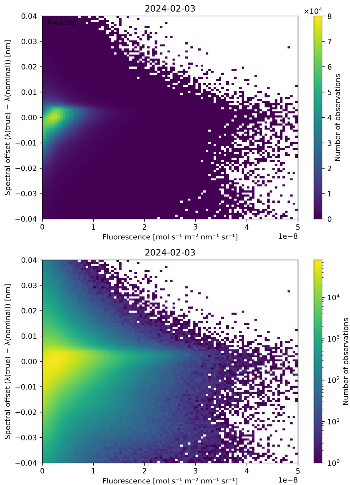
Figure 87: Scatter density plot of “Fluorescence” against “Spectral offset ( \lambda(\text{true}) - \lambda(\text{nominal}) )” for 2024-02-02 to 2024-02-04.
