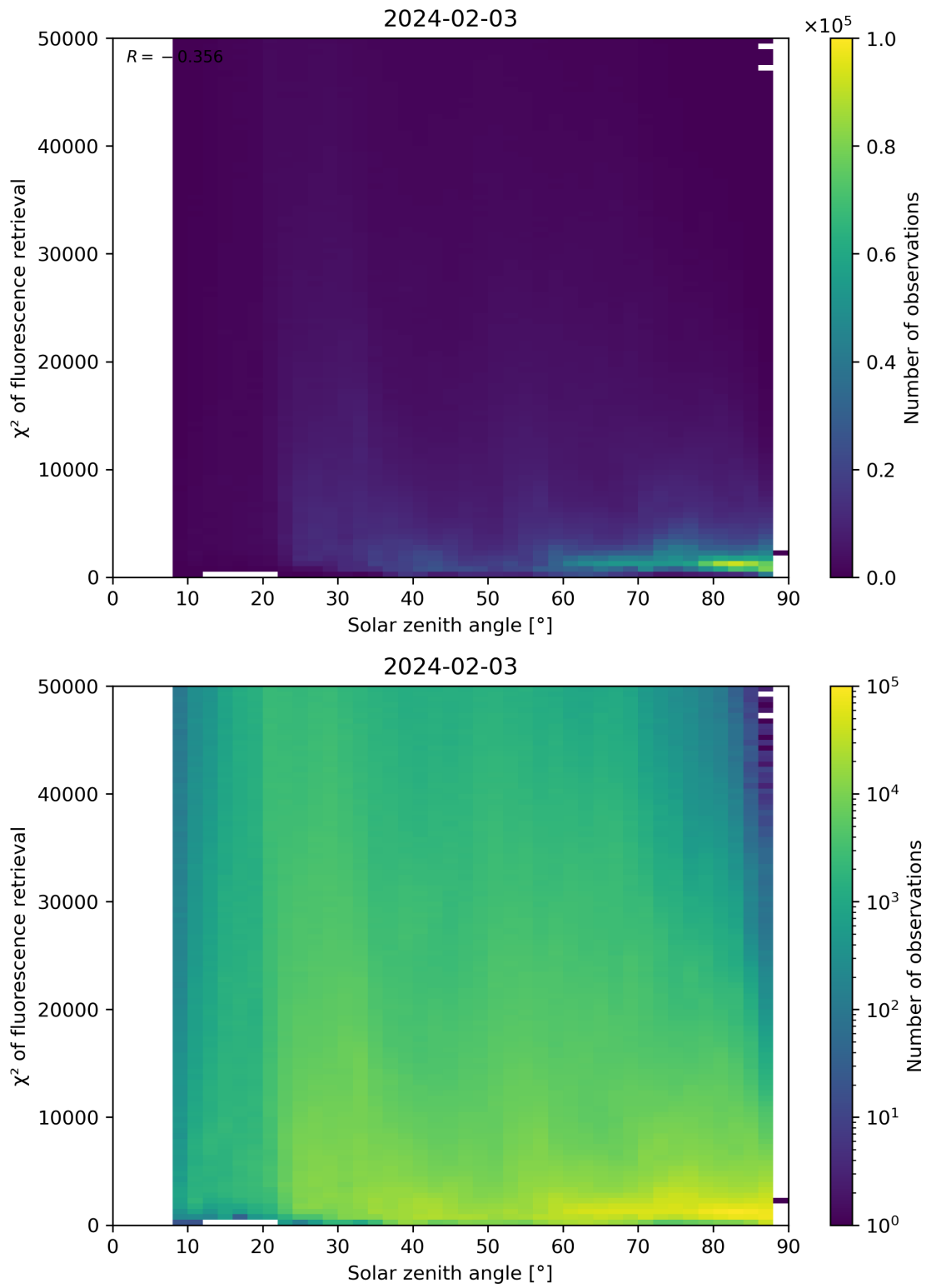
Figure 109: Scatter density plot of “Solar zenith angle” against “ \chi^2 of fluorescence retrieval” for 2024-02-02 to 2024-02-04.
