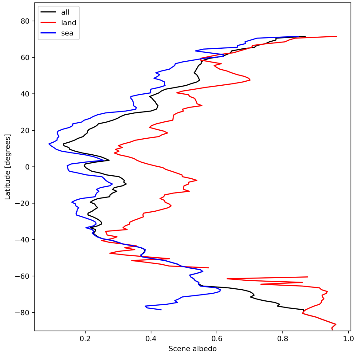
Figure 17: Zonal average of “Scene albedo” for 2024-02-02 to 2024-02-04.
