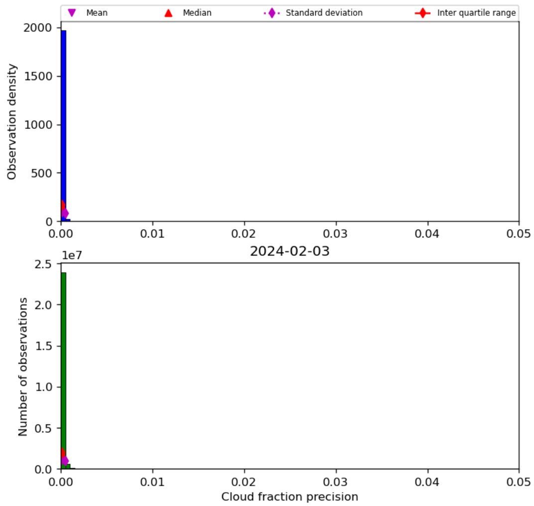
Figure 33: Histogram of “Cloud fraction precision” for 2024-02-02 to 2024-02-04
