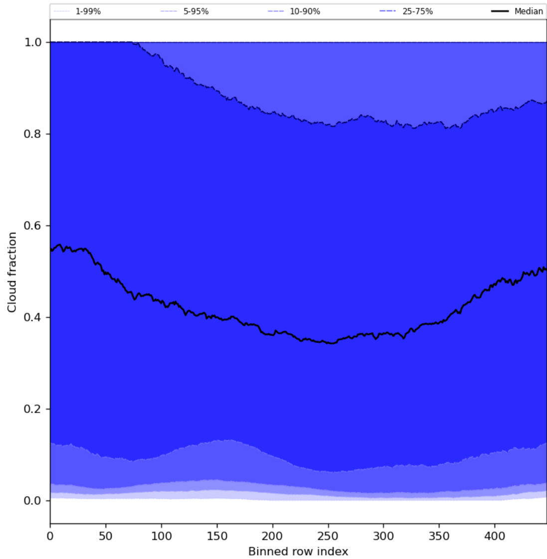
Figure 49: Along track statistics of “Cloud fraction” for 2024-02-02 to 2024-02-04
