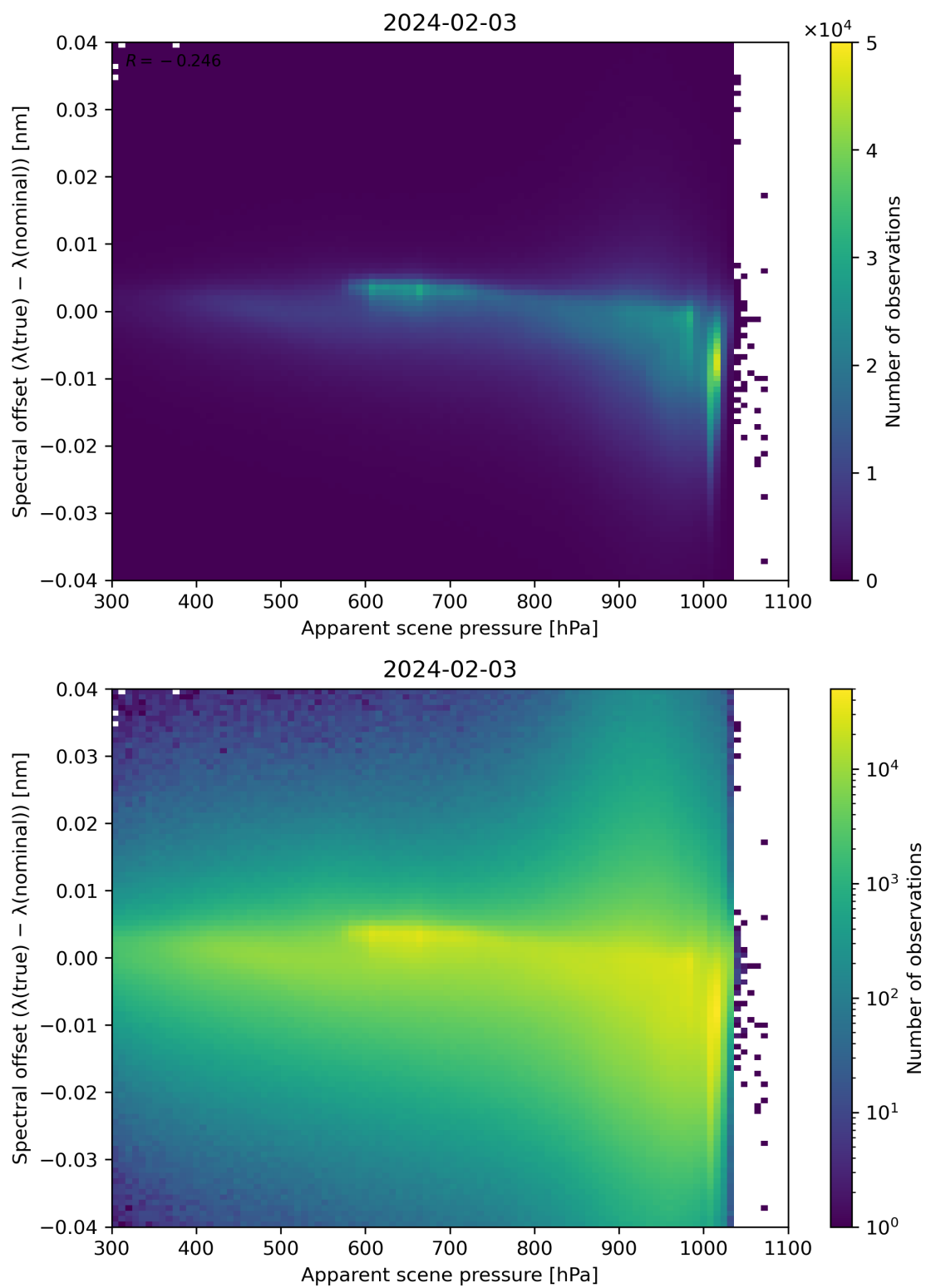
Figure 67: Scatter density plot of “Apparent scene pressure” against “Spectral offset ( \lambda(\text{true}) - \lambda(\text{nominal}) )” for 2024-02-02 to 2024-02-04.
