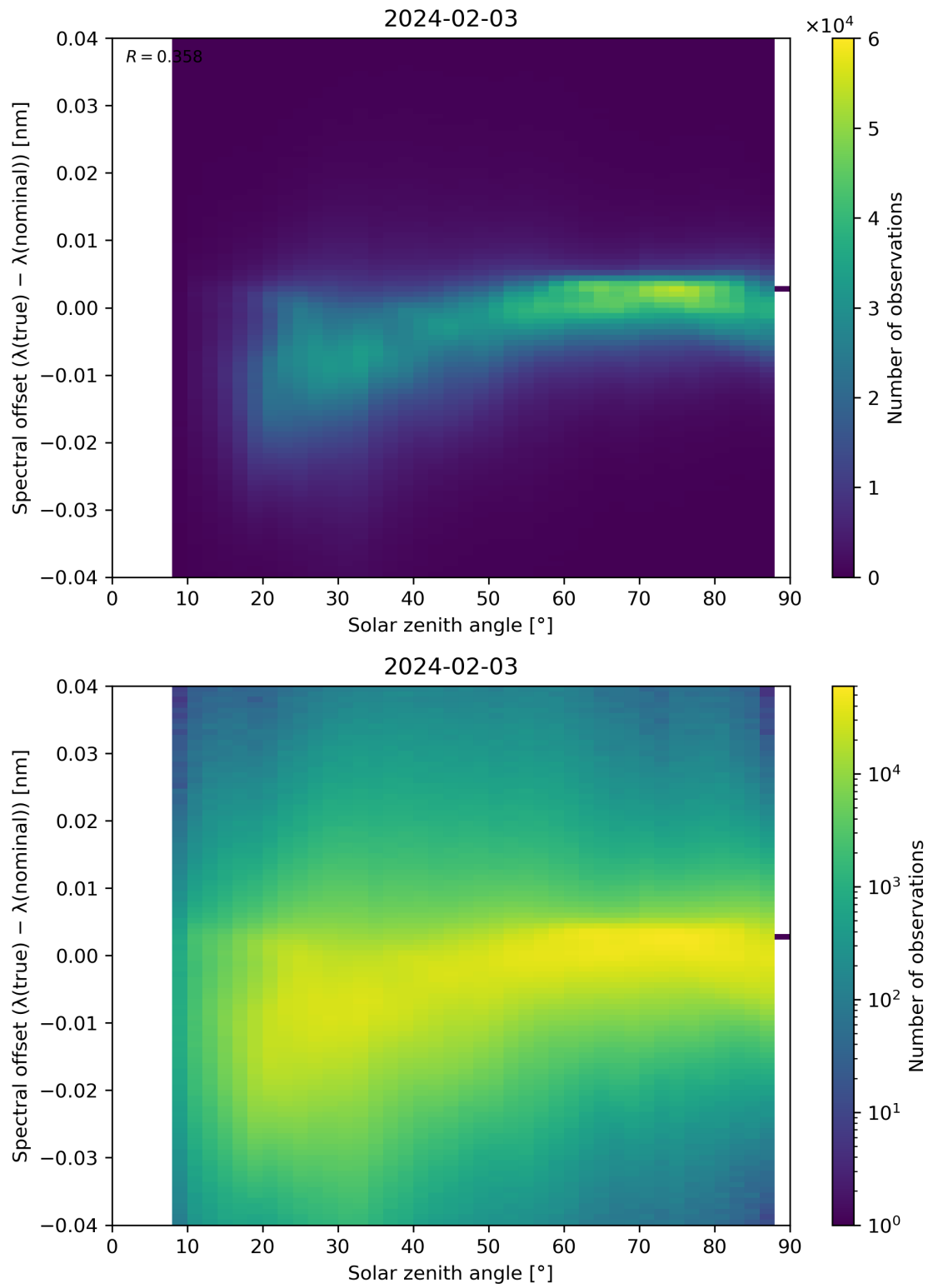
Figure 117: Scatter density plot of “Solar zenith angle” against “Spectral offset ( \lambda(\text{true}) - \lambda(\text{nominal}) )” for 2024-02-02 to 2024-02-04.
