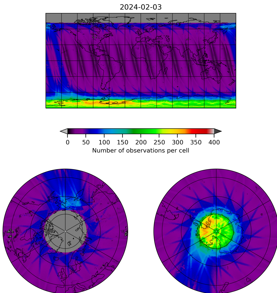
Figure 11: Map of the number of observations for 2024-02-02 to 2024-02-04
