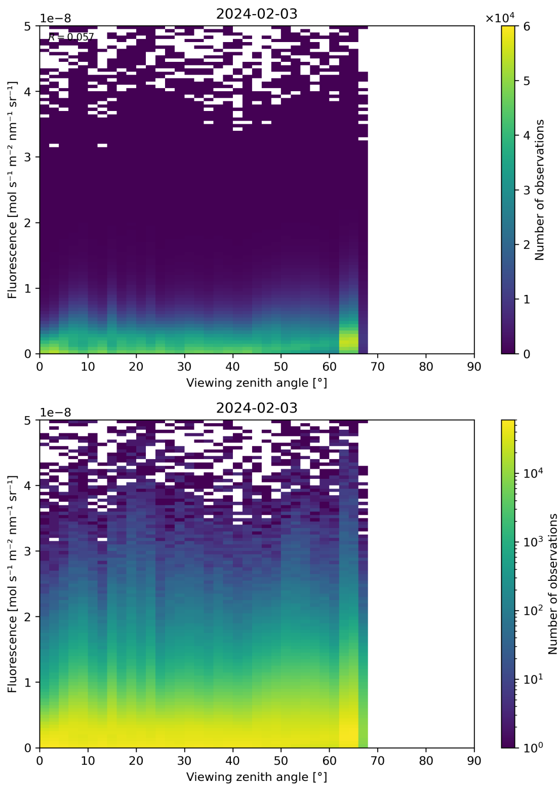
Figure 122: Scatter density plot of “Viewing zenith angle” against “Fluorescence” for 2024-02-02 to 2024-02-04.
