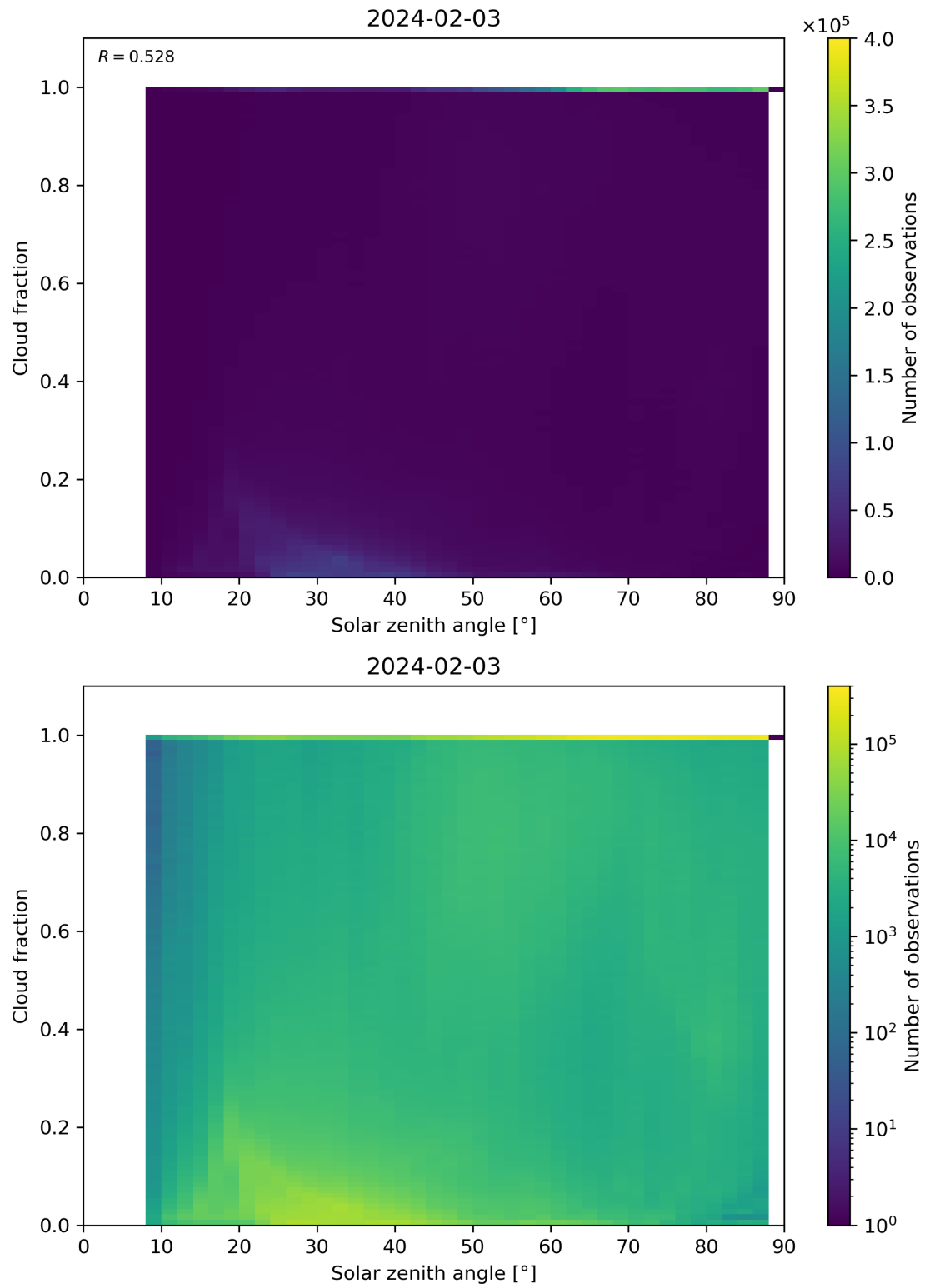
Figure 110: Scatter density plot of “Solar zenith angle” against “Cloud fraction” for 2024-02-02 to 2024-02-04.
