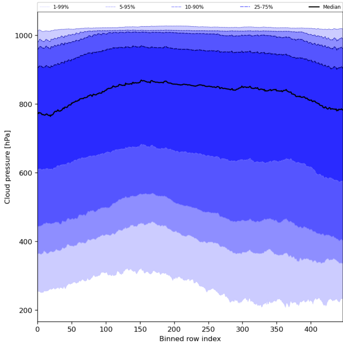
Figure 47: Along track statistics of “Cloud pressure” for 2024-02-02 to 2024-02-04
