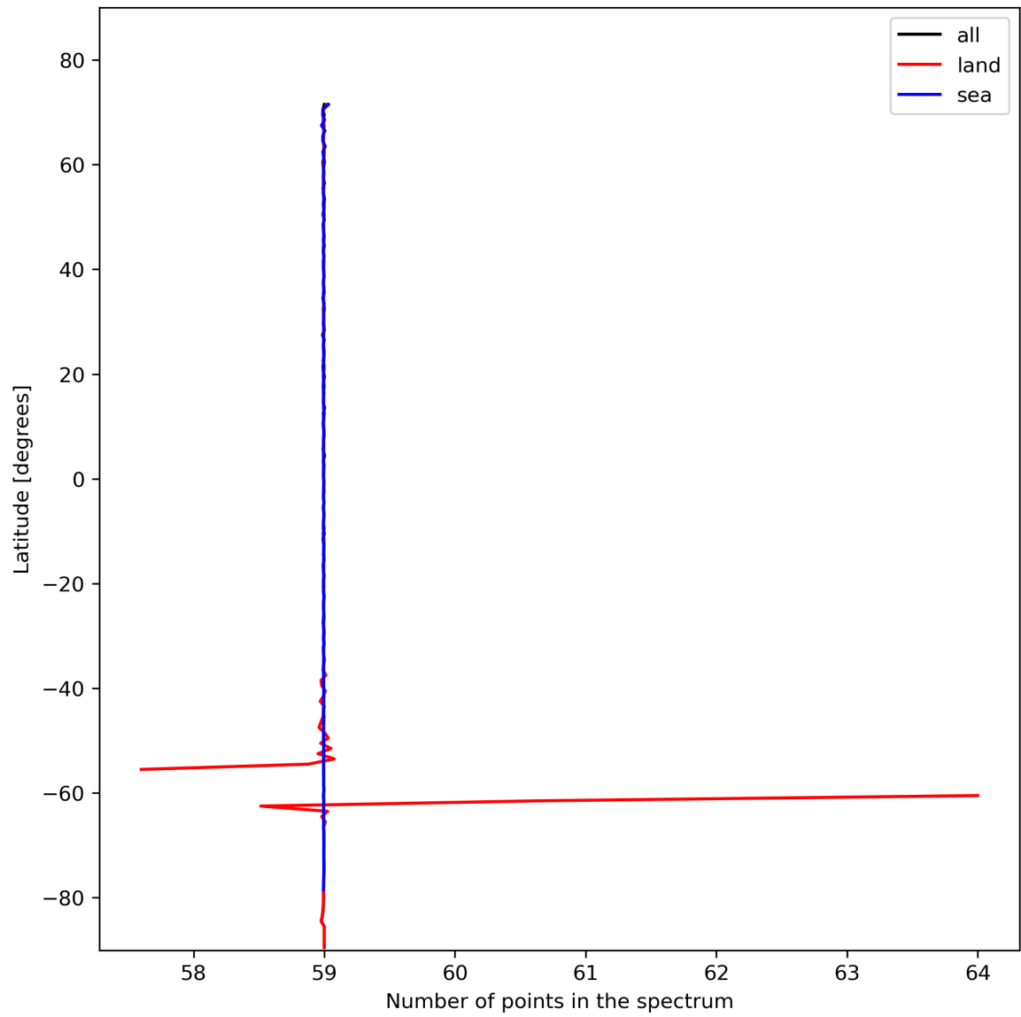
Figure 27: Zonal average of “Number of points in the spectrum” for 2024-02-02 to 2024-02-04.
