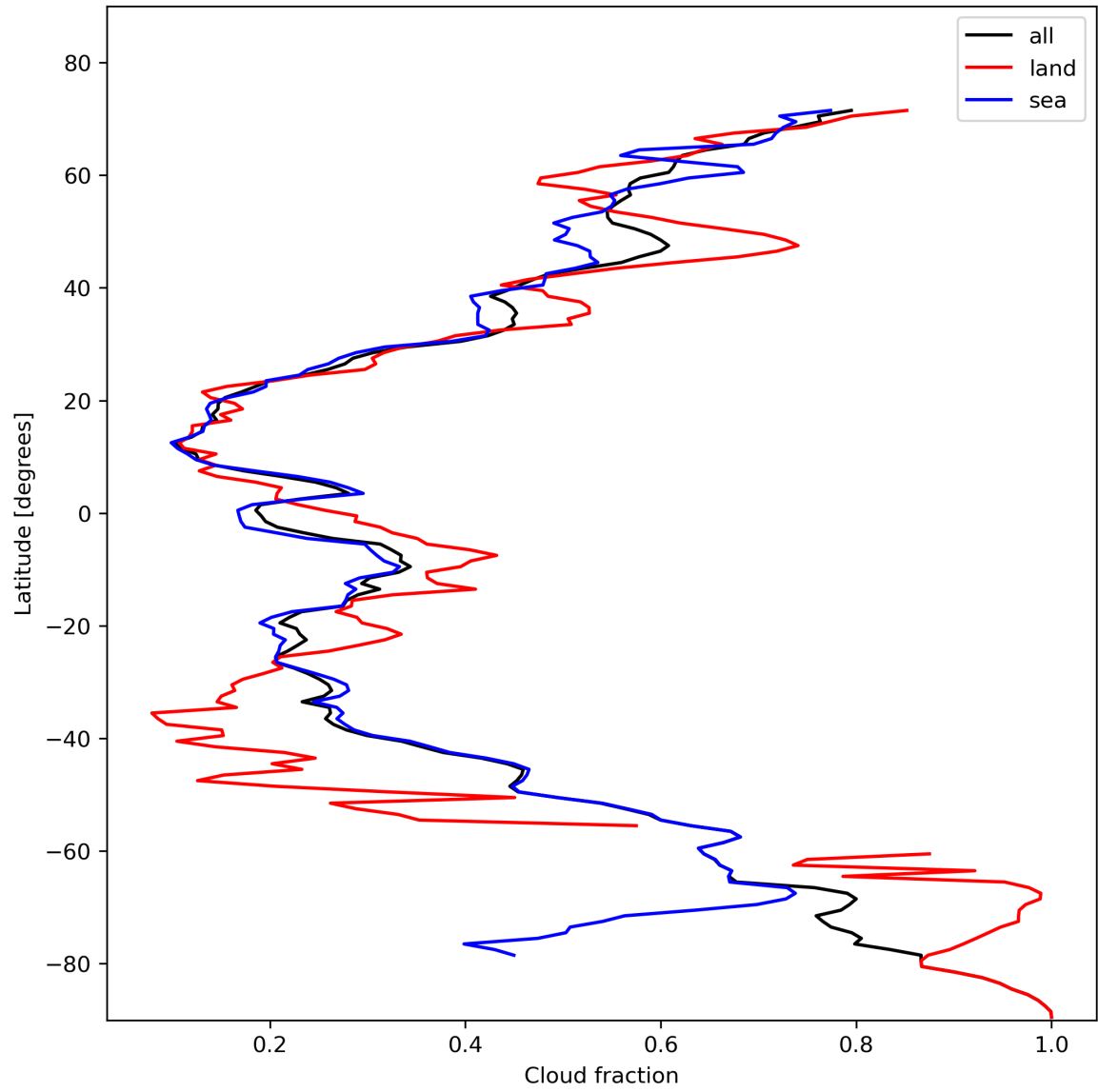
Figure 15: Zonal average of “Cloud fraction” for 2024-02-02 to 2024-02-04.
