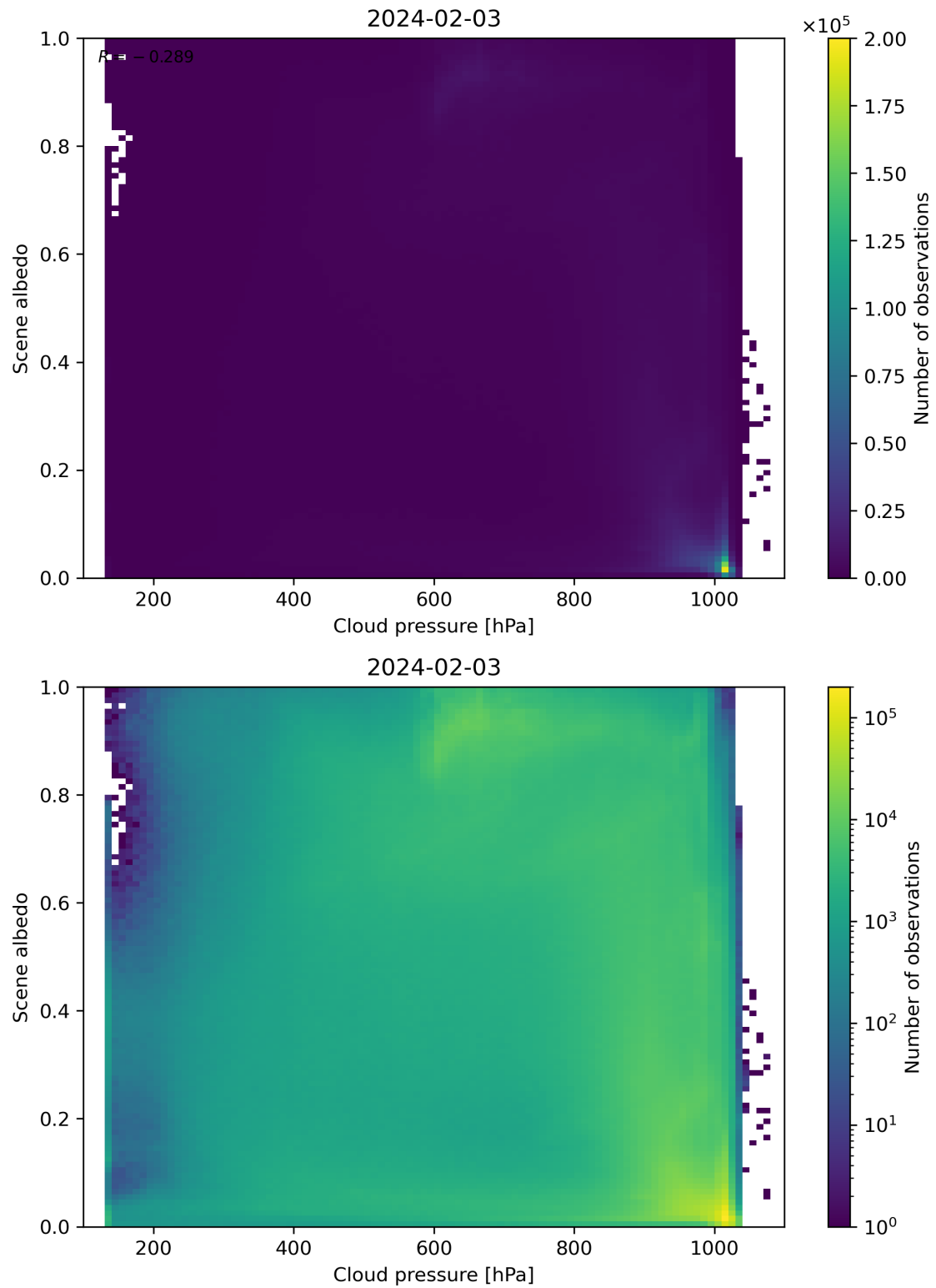
Figure 83: Scatter density plot of “Cloud pressure” against “Scene albedo” for 2024-02-02 to 2024-02-04.
