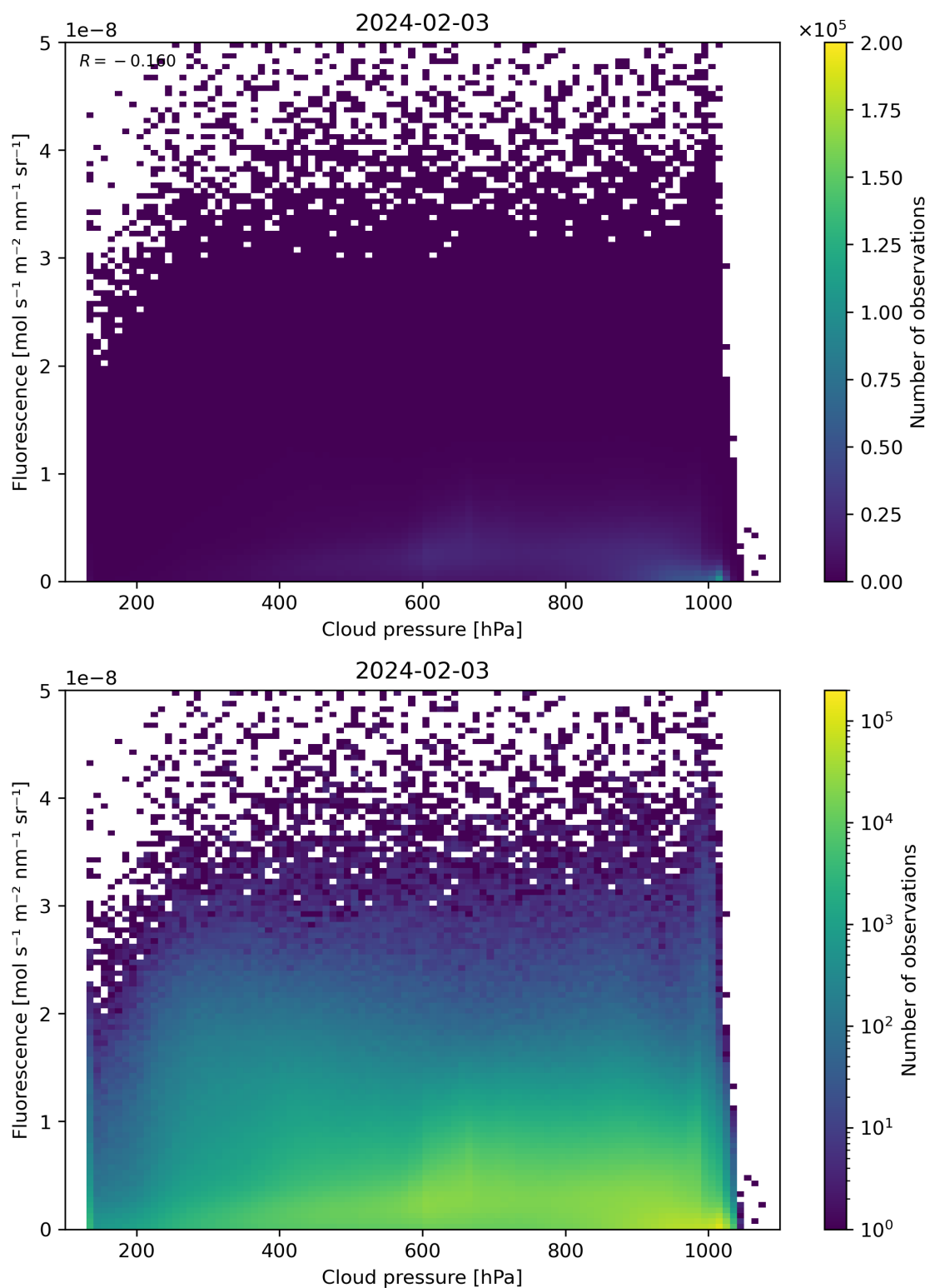
Figure 80: Scatter density plot of “Cloud pressure” against “Fluorescence” for 2024-02-02 to 2024-02-04.
