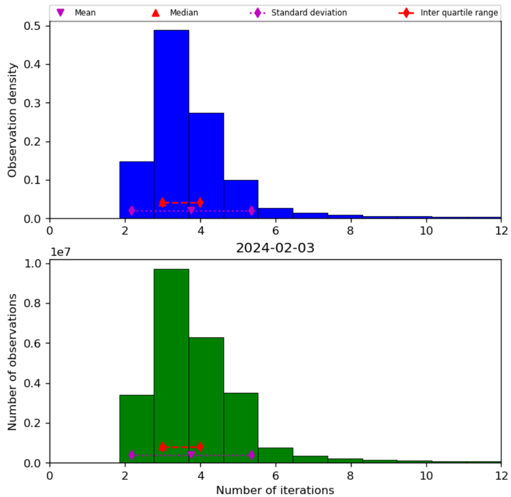
Figure 39: Histogram of “Number of iterations” for 2024-02-02 to 2024-02-04
