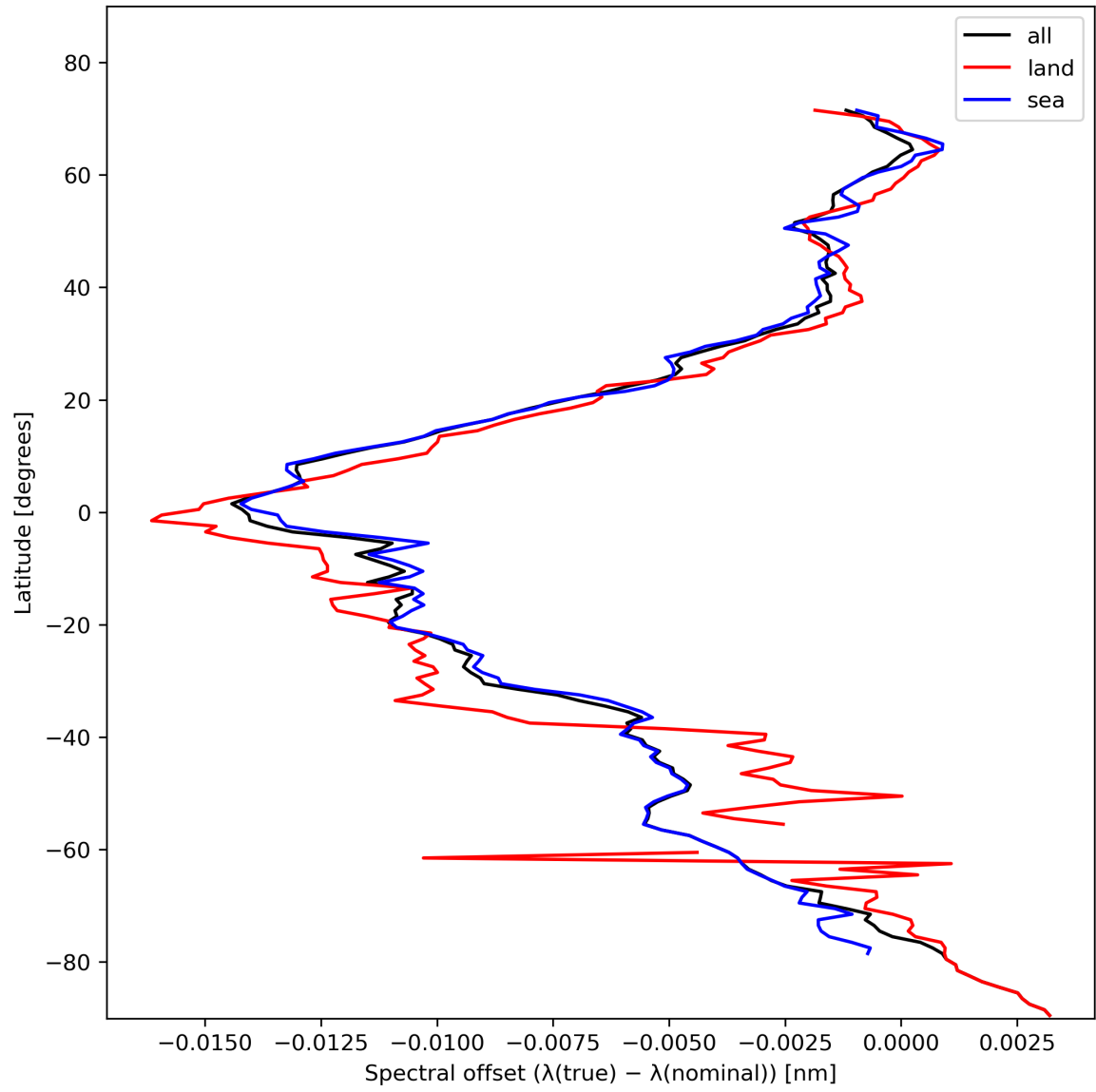
Figure 28: Zonal average of “Spectral offset ( \lambda(\text{true}) - \lambda(\text{nominal}) )” for 2024-02-02 to 2024-02-04.
