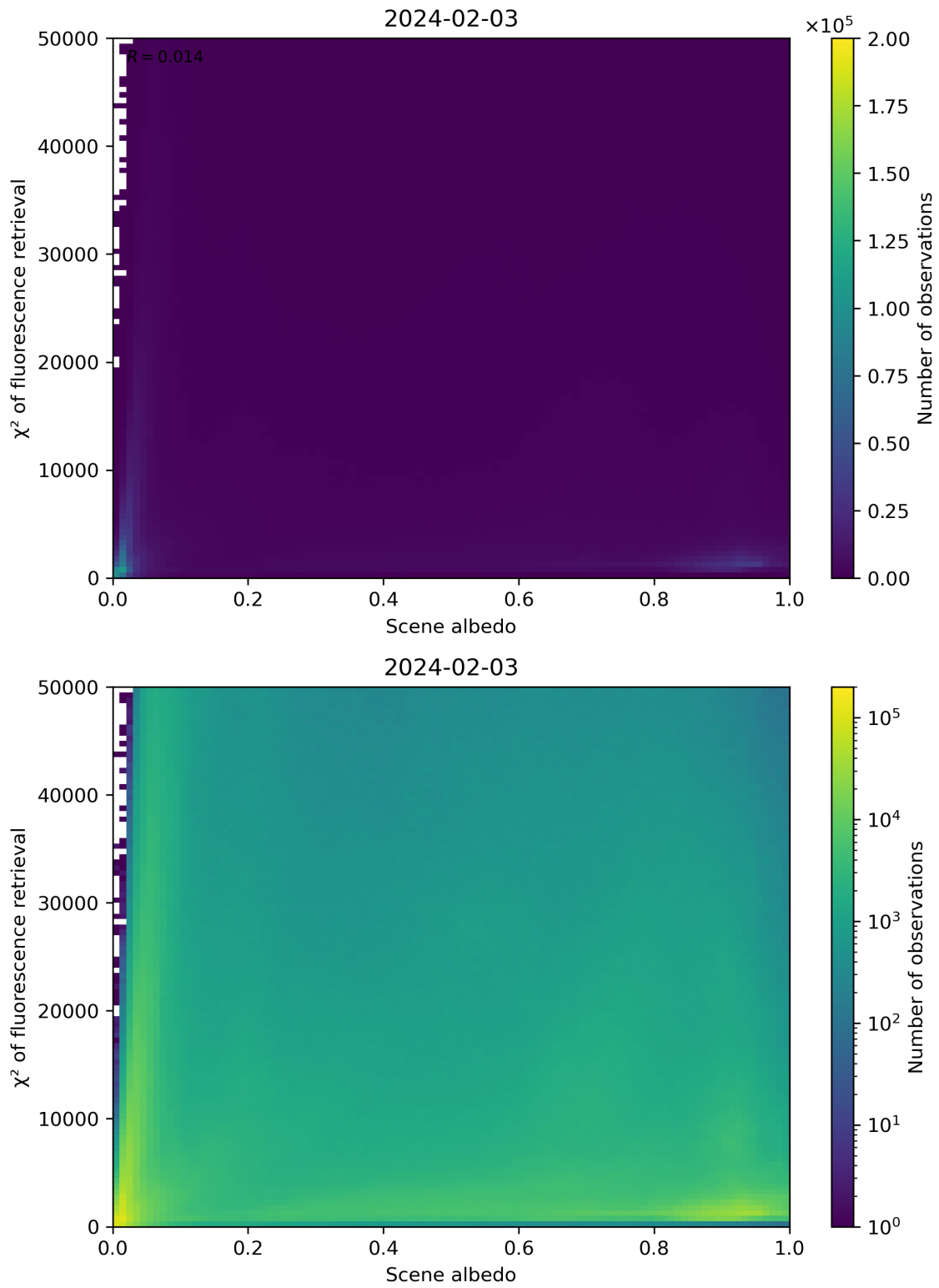
Figure 103: Scatter density plot of “Scene albedo” against “ \chi^2 of fluorescence retrieval” for 2024-02-02 to 2024-02-04.
