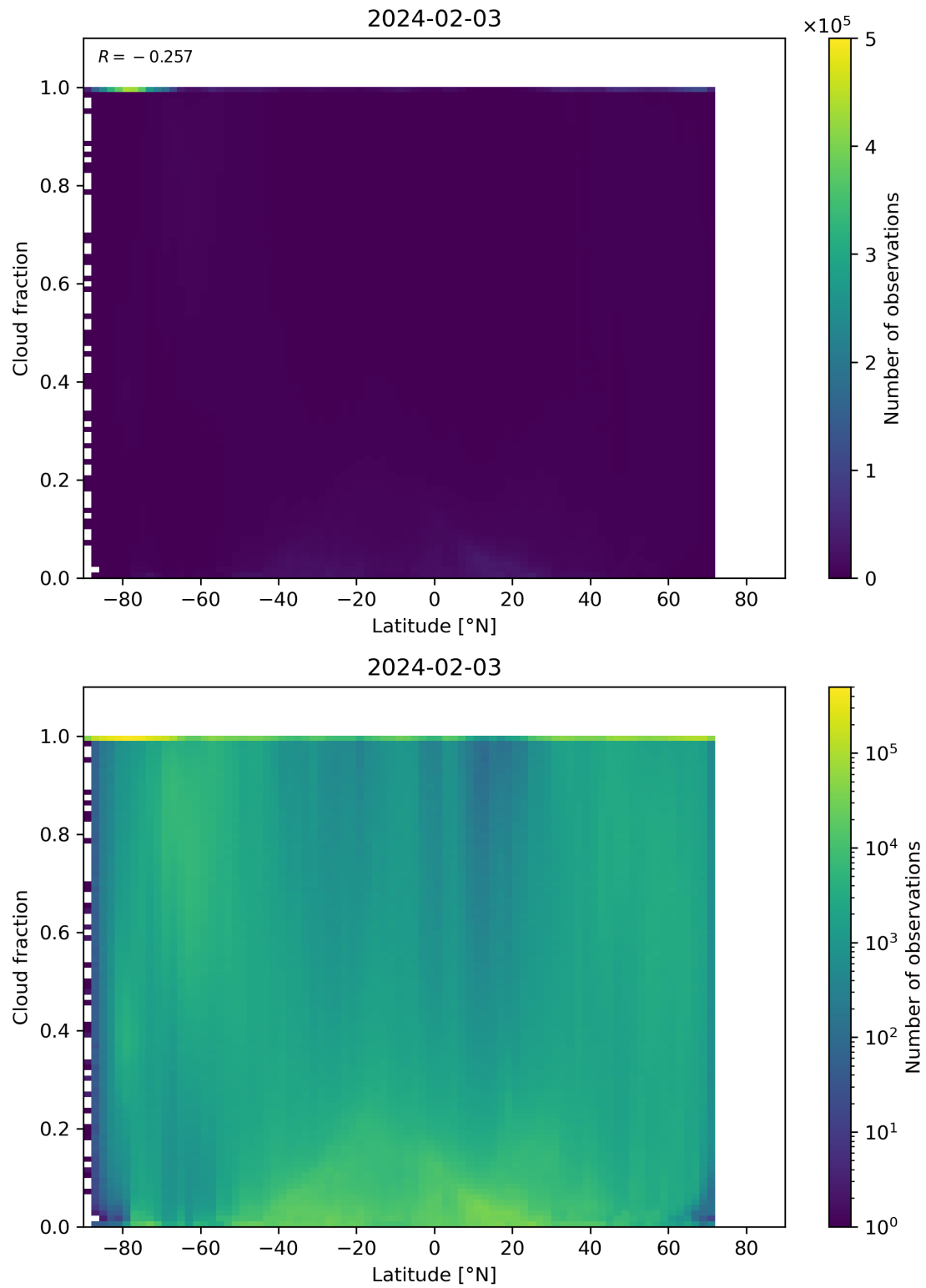
Figure 90: Scatter density plot of “Latitude” against “Cloud fraction” for 2024-02-02 to 2024-02-04.
