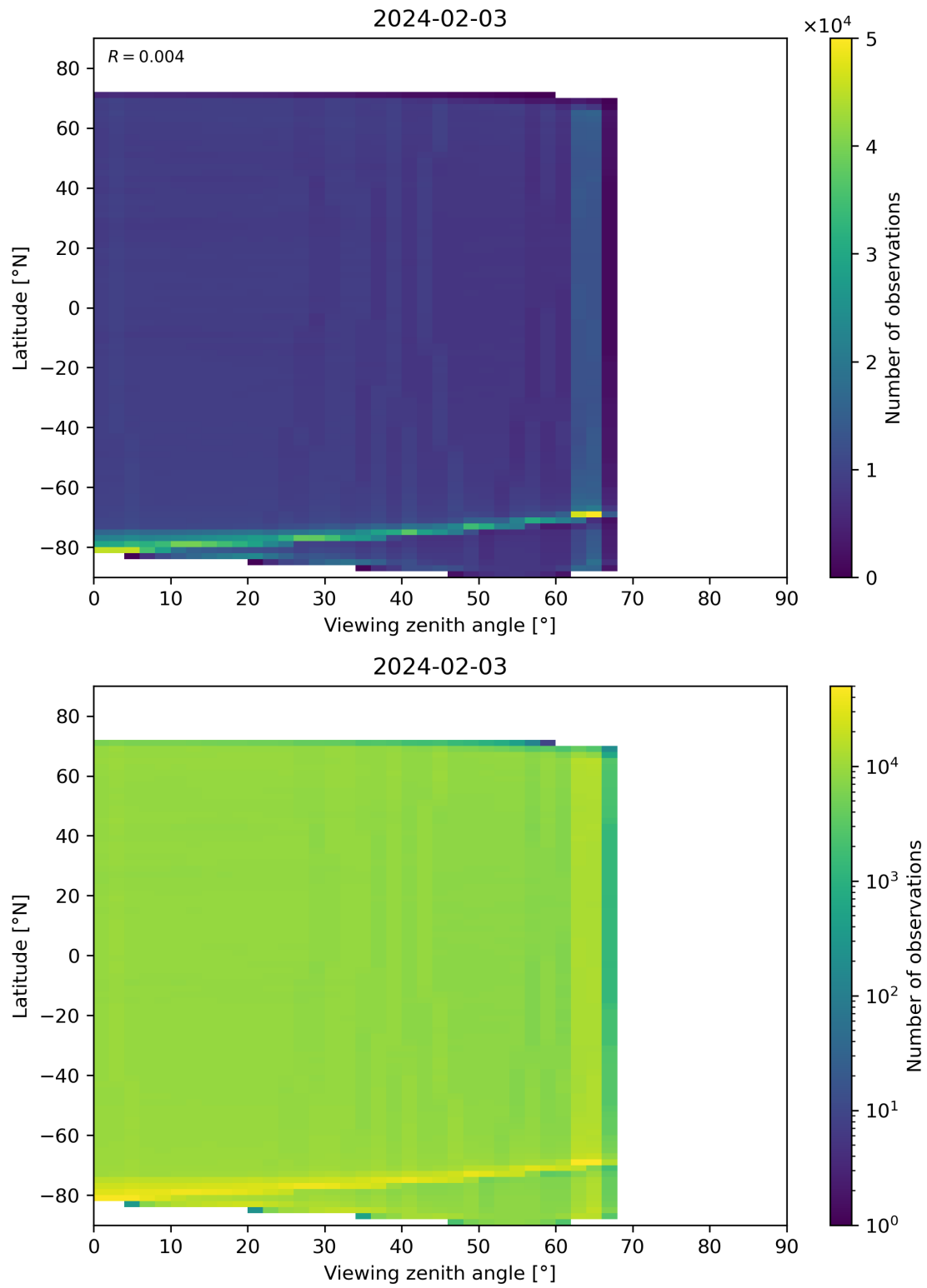
Figure 123: Scatter density plot of “Viewing zenith angle” against “Latitude” for 2024-02-02 to 2024-02-04.
