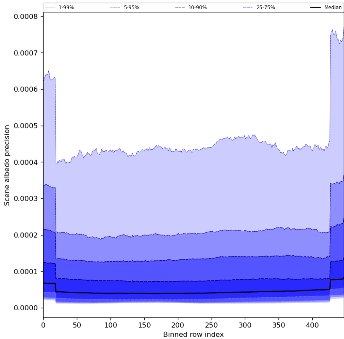
Figure 52: Along track statistics of “Scene albedo precision” for 2024-02-02 to 2024-02-04
