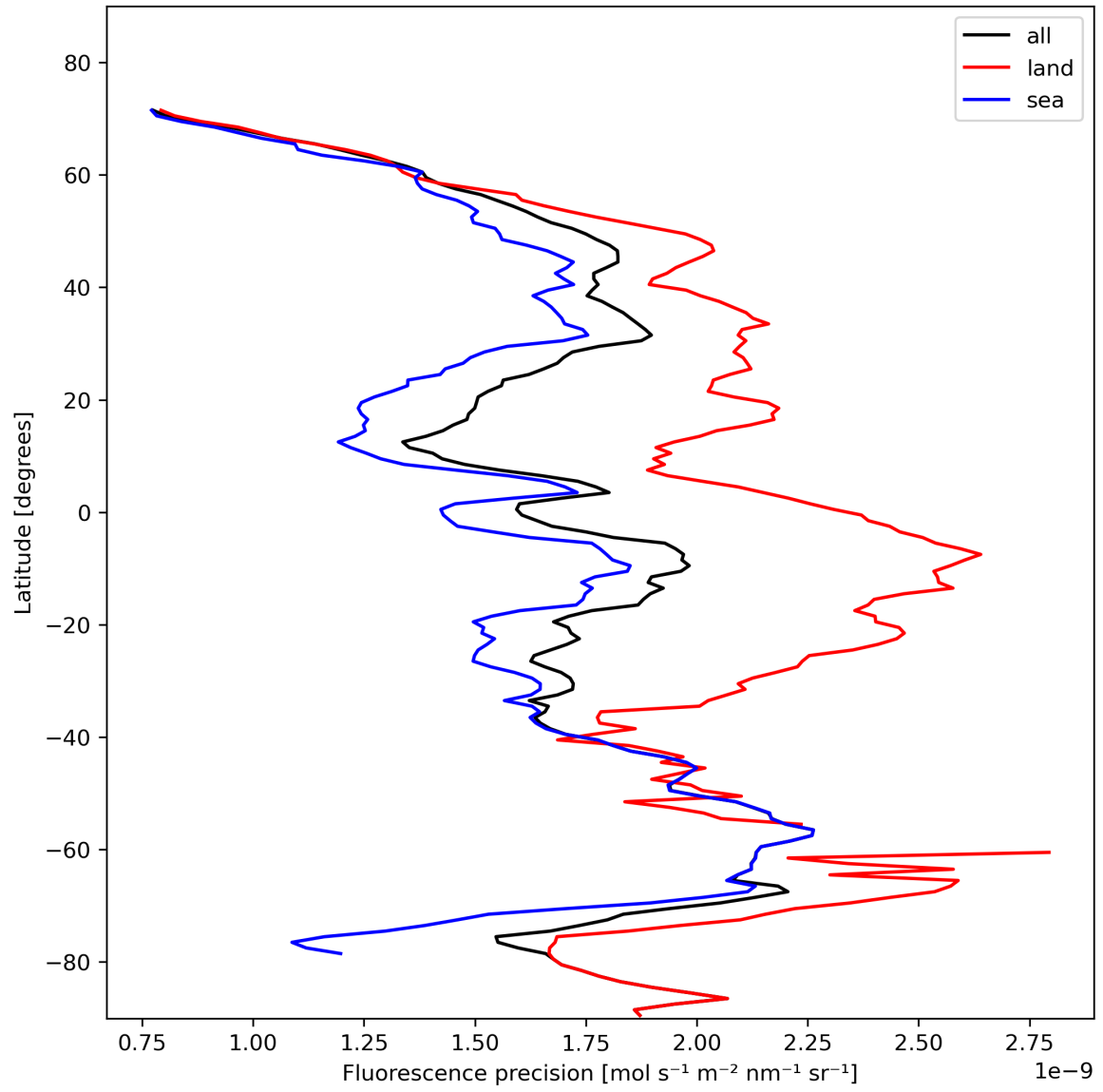
Figure 24: Zonal average of “Fluorescence precision” for 2024-02-02 to 2024-02-04.
