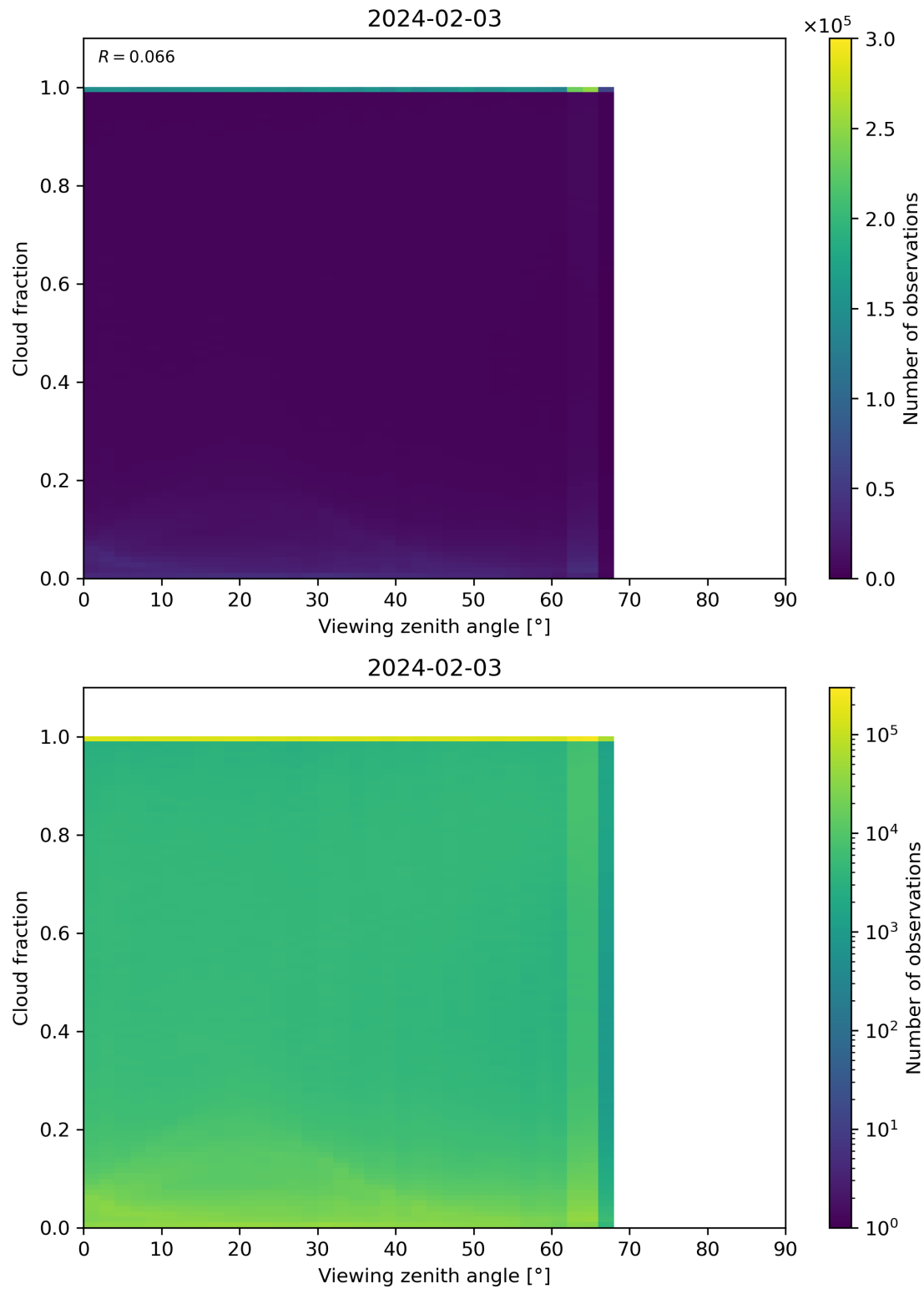
Figure 120: Scatter density plot of “Viewing zenith angle” against “Cloud fraction” for 2024-02-02 to 2024-02-04.
