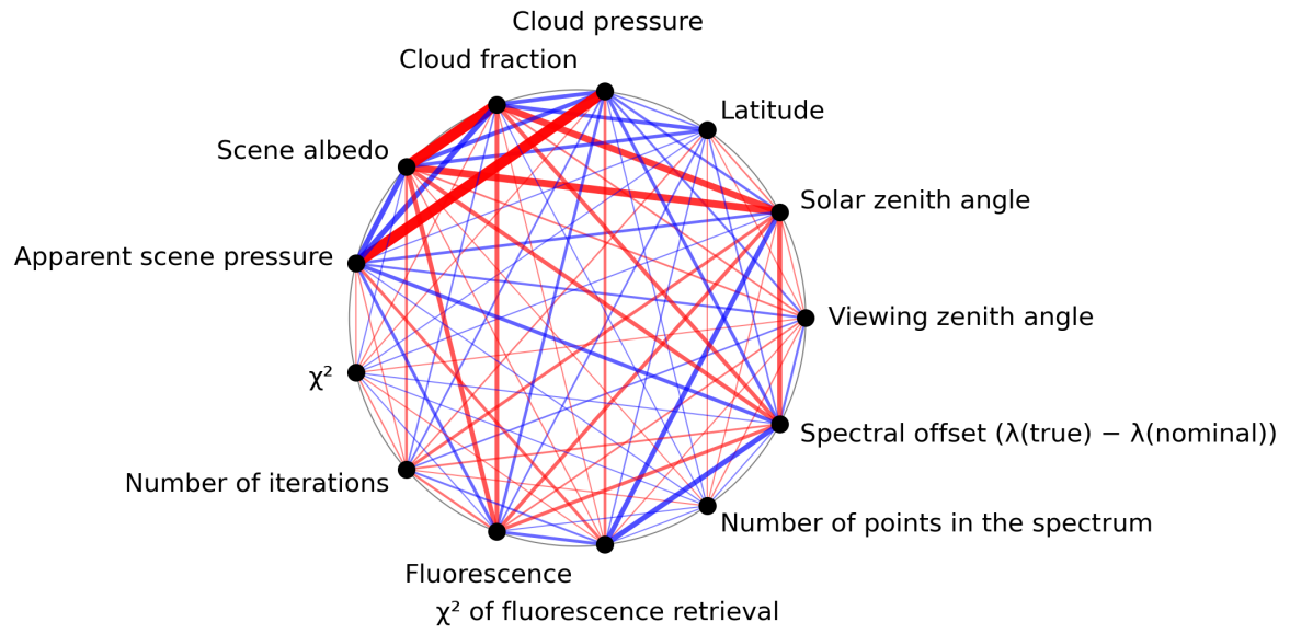
Figure 1: Map of correlation graph for 2024-02-02 to 2024-02-04.
