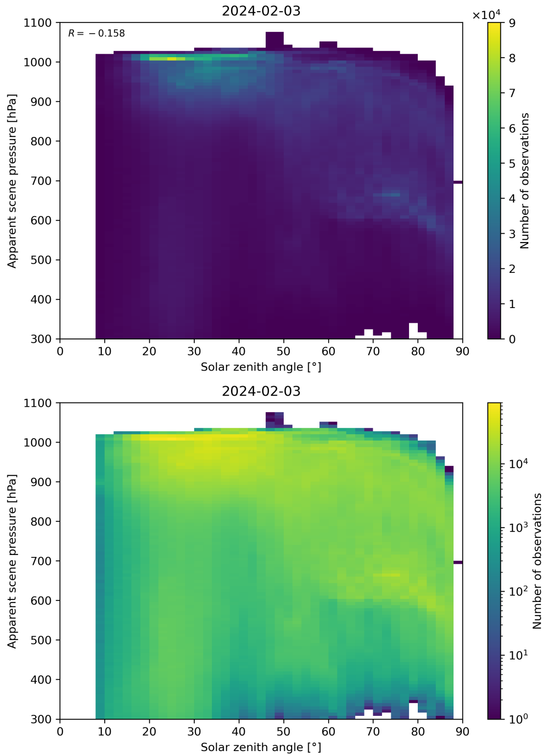
Figure 108: Scatter density plot of “Solar zenith angle” against “Apparent scene pressure” for 2024-02-02 to 2024-02-04.
