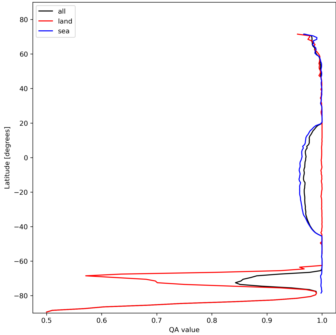
Figure 12: Zonal average of “QA value” for 2024-02-02 to 2024-02-04.
