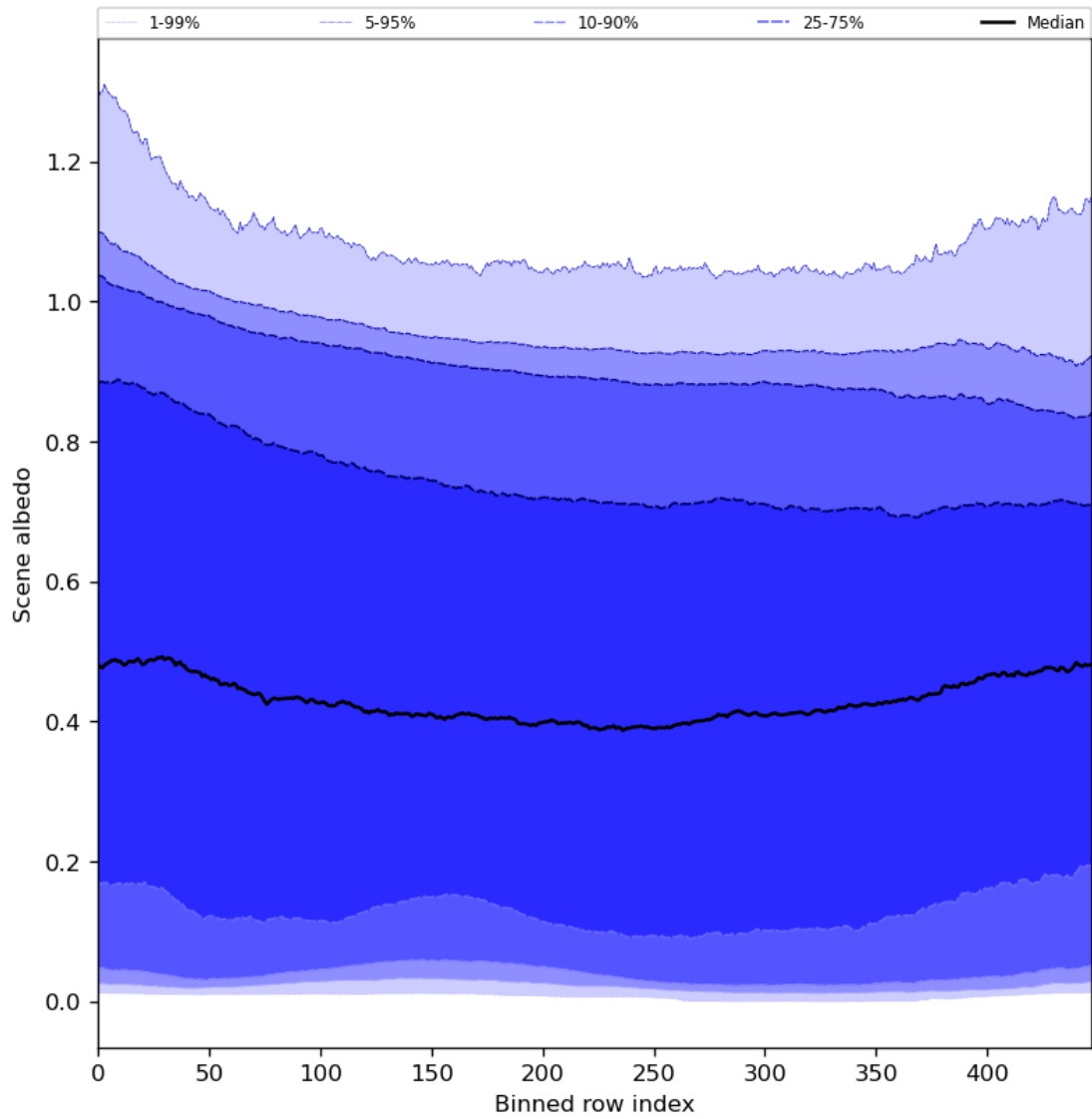
Figure 51: Along track statistics of “Scene albedo” for 2024-02-02 to 2024-02-04
