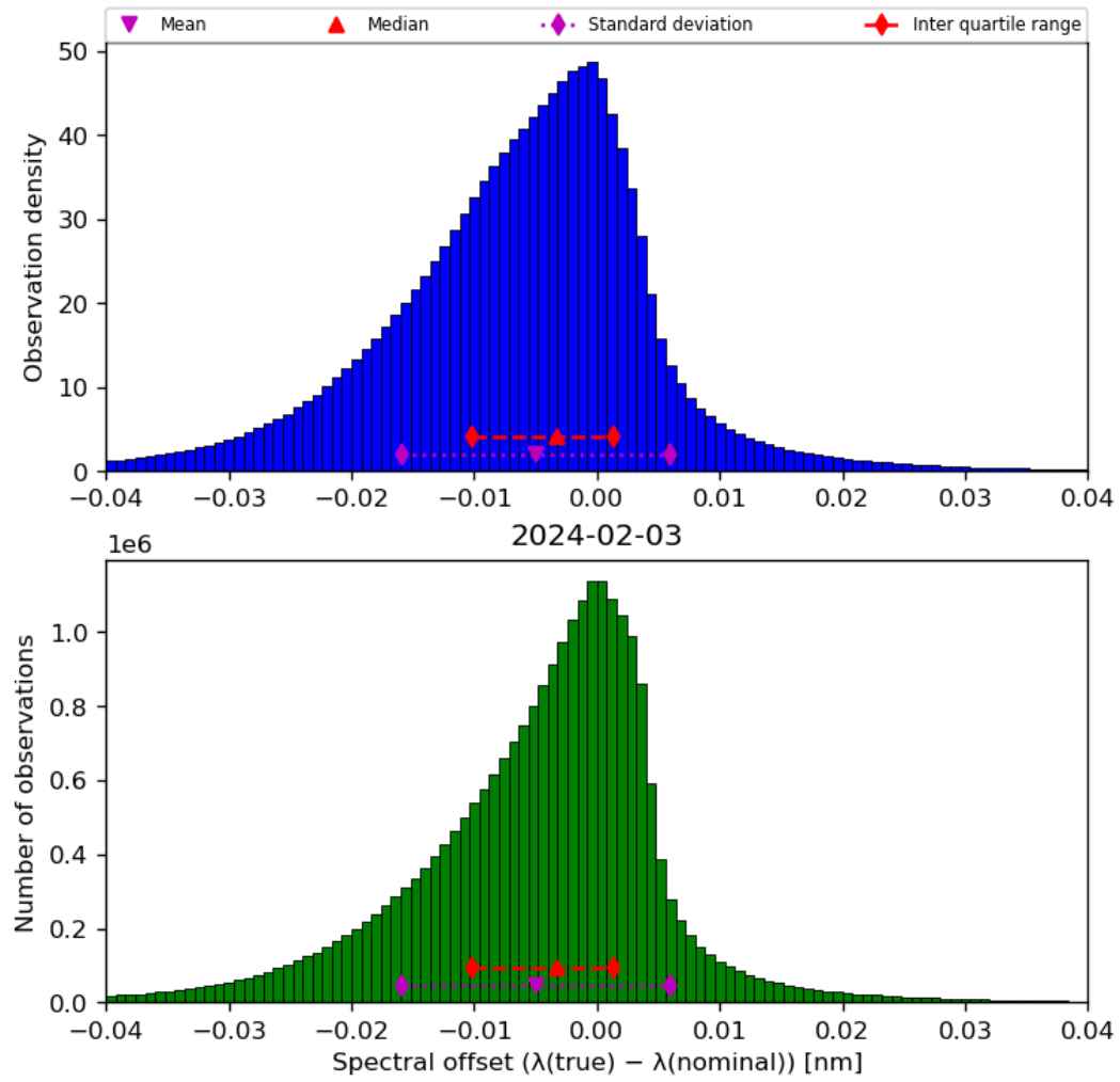
Figure 45: Histogram of “Spectral offset ( \lambda(\text{true}) - \lambda(\text{nominal}) )” for 2024-02-02 to 2024-02-04
