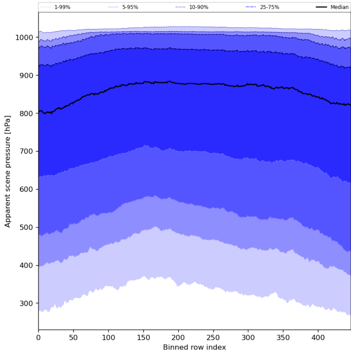
Figure 53: Along track statistics of “Apparent scene pressure” for 2024-02-02 to 2024-02-04
