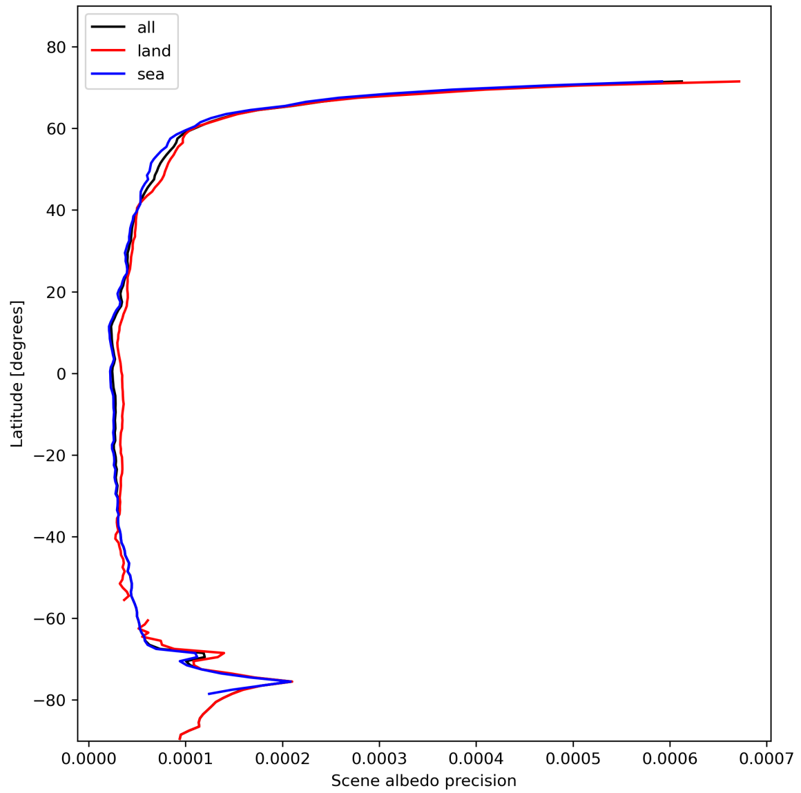
Figure 18: Zonal average of “Scene albedo precision” for 2024-02-02 to 2024-02-04.
