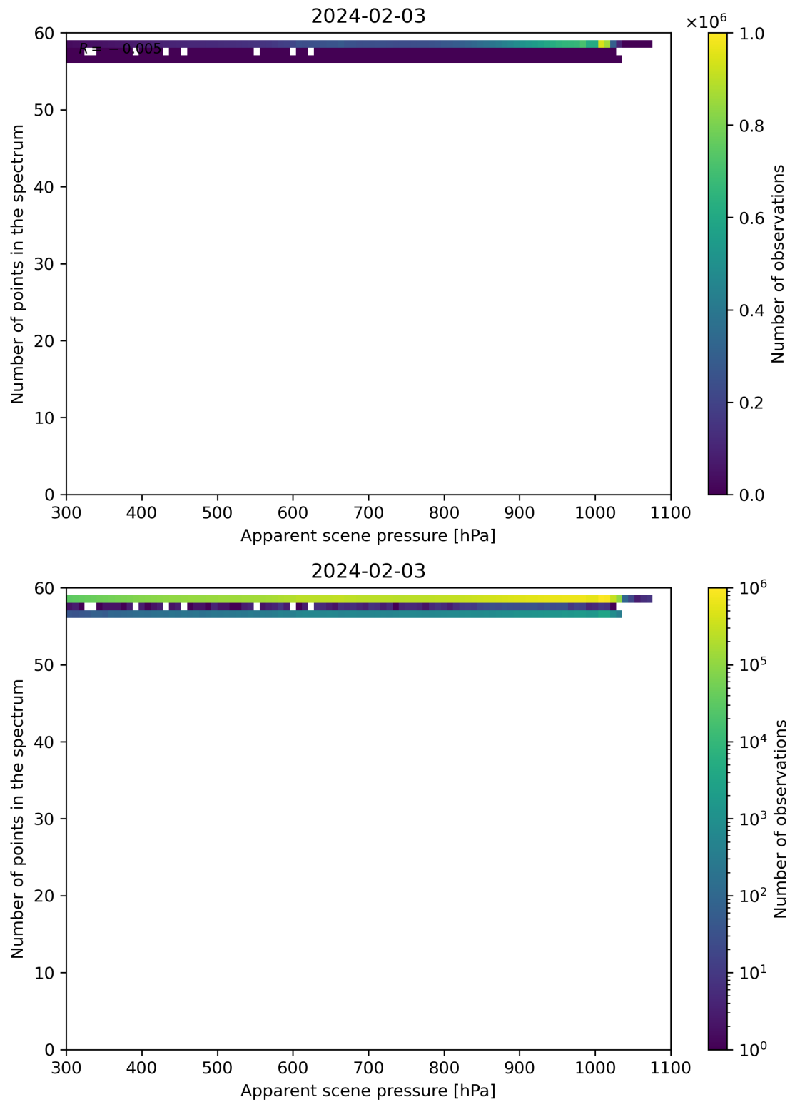
Figure 66: Scatter density plot of “Apparent scene pressure” against “Number of points in the spectrum” for 2024-02-02 to 2024-02-04.
