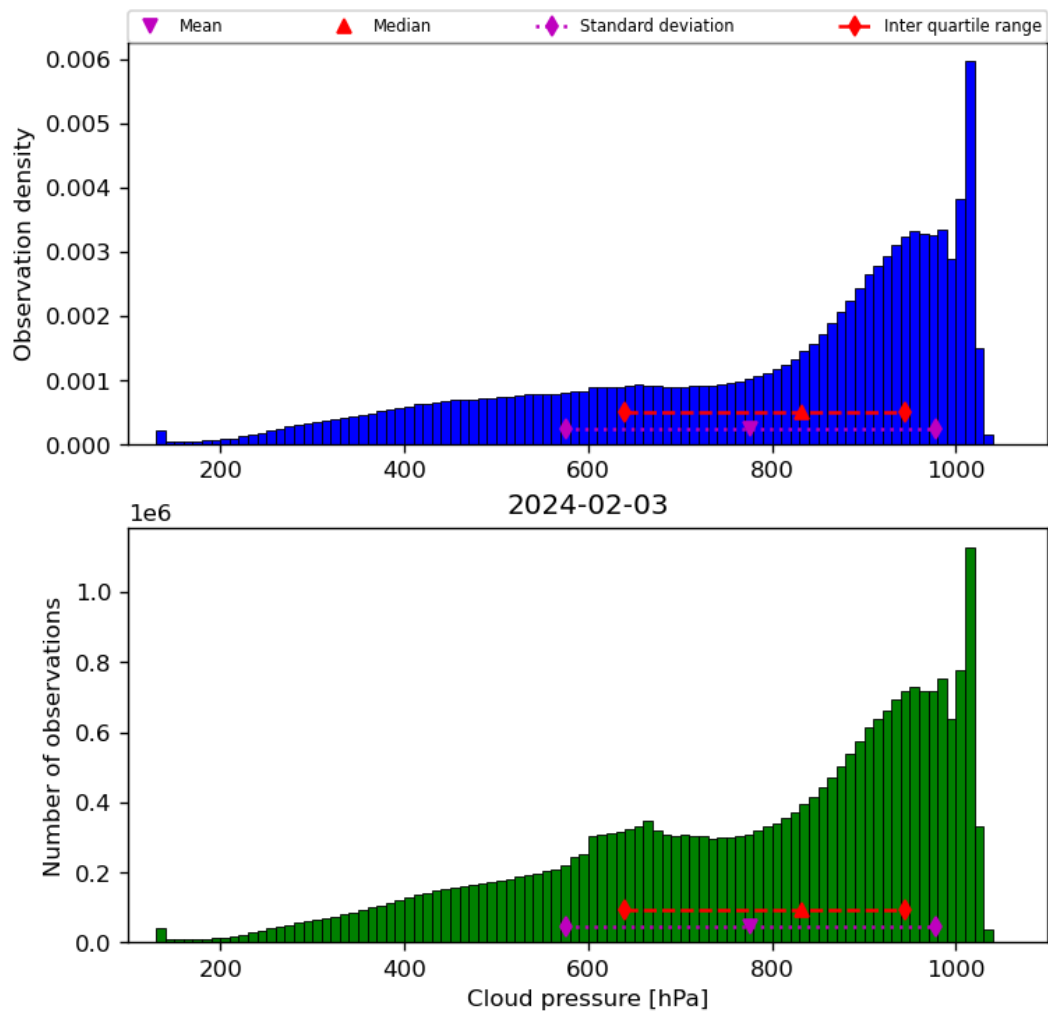
Figure 30: Histogram of “Cloud pressure” for 2024-02-02 to 2024-02-04
