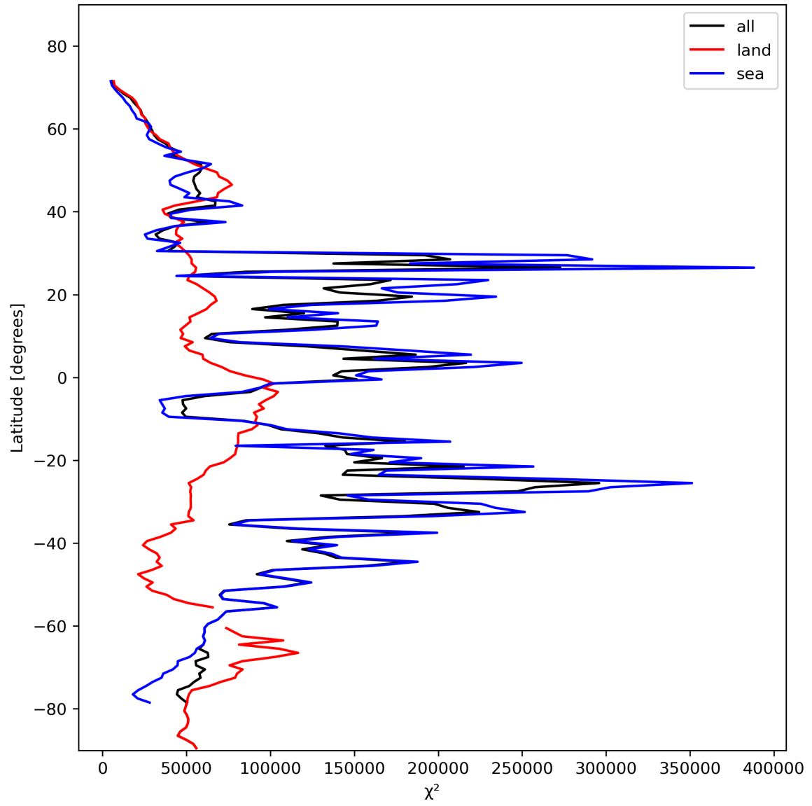
Figure 21: Zonal average of “ \chi^2 ” for 2024-02-02 to 2024-02-04.
