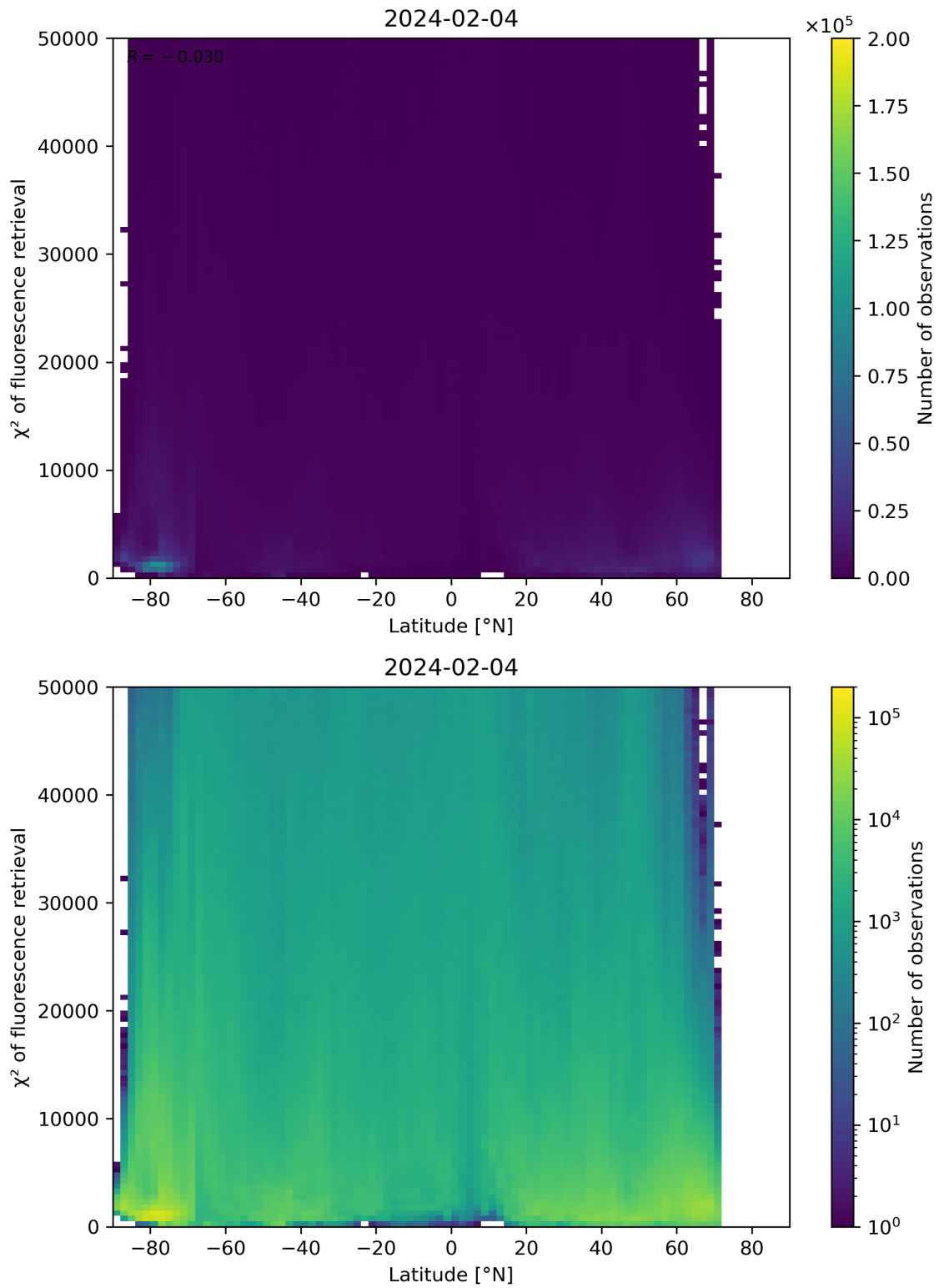
Figure 89: Scatter density plot of “Latitude” against “ \chi^2 of fluorescence retrieval” for 2024-02-03 to 2024-02-05.
