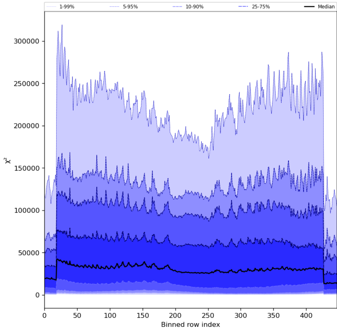
Figure 55: Along track statistics of “ \chi^2 ” for 2024-02-03 to 2024-02-05
