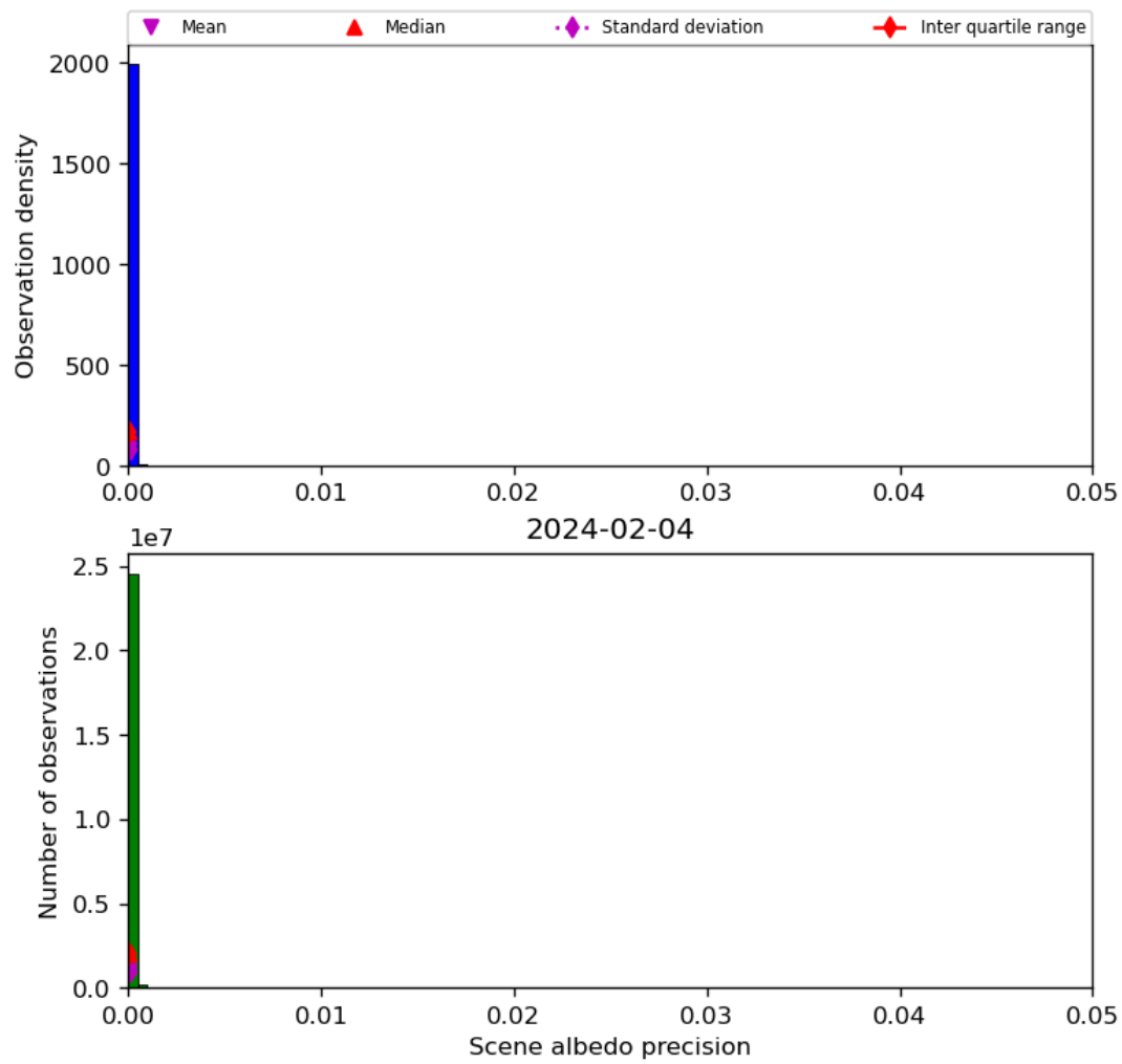
Figure 35: Histogram of “Scene albedo precision” for 2024-02-03 to 2024-02-05
