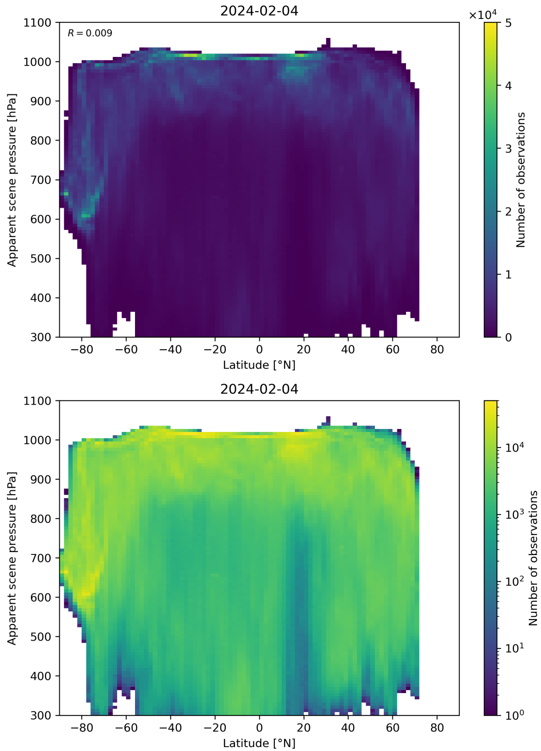
Figure 88: Scatter density plot of “Latitude” against “Apparent scene pressure” for 2024-02-03 to 2024-02-05.
