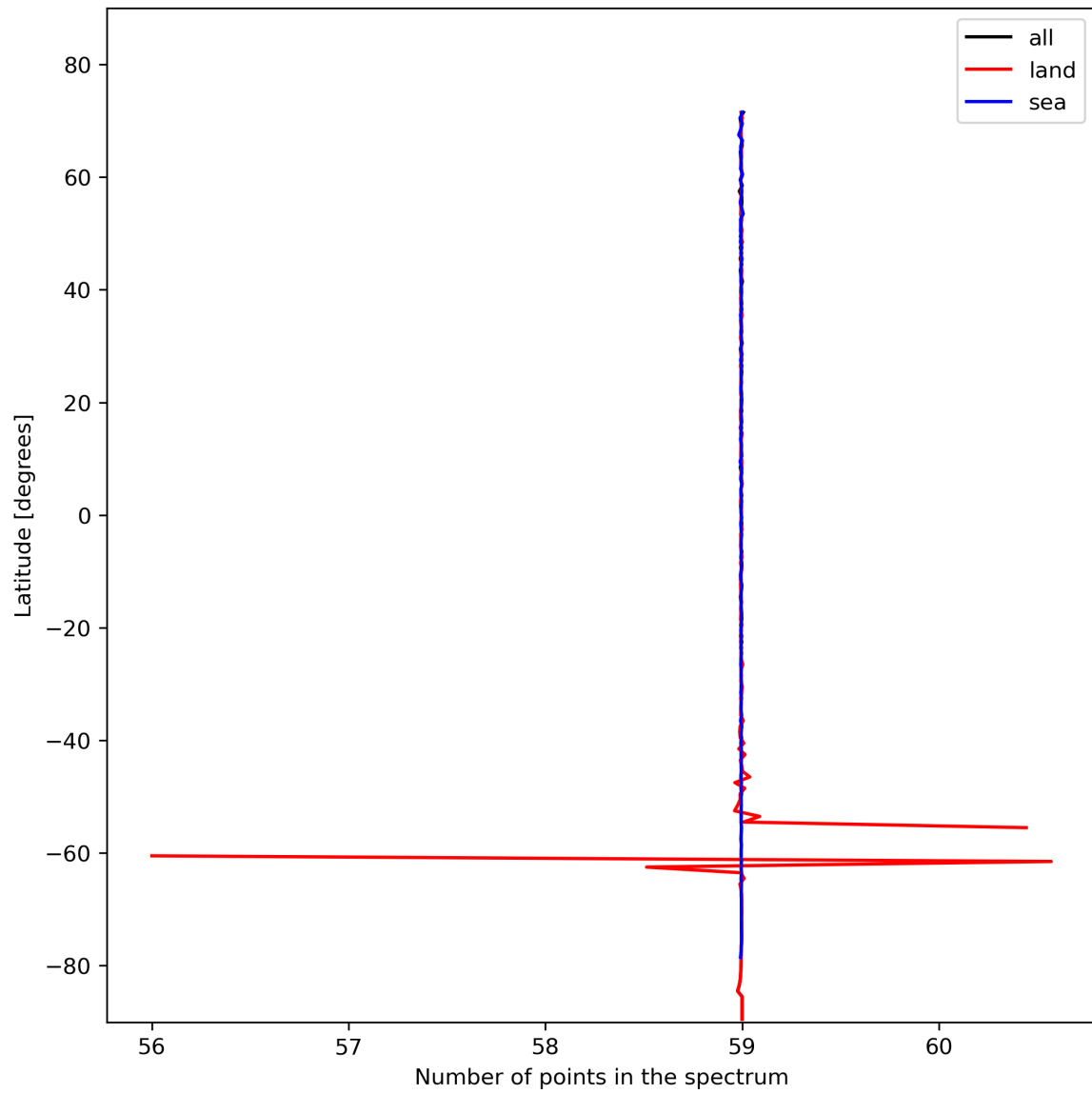
Figure 27: Zonal average of “Number of points in the spectrum” for 2024-02-03 to 2024-02-05.
