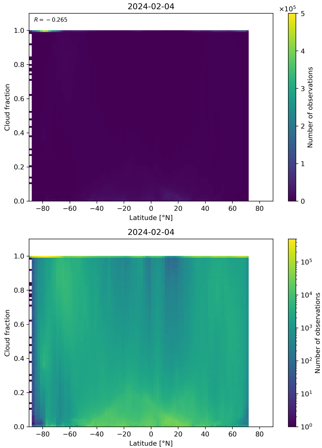
Figure 90: Scatter density plot of “Latitude” against “Cloud fraction” for 2024-02-03 to 2024-02-05.
