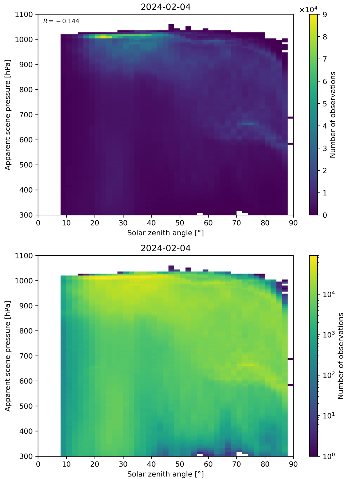
Figure 108: Scatter density plot of “Solar zenith angle” against “Apparent scene pressure” for 2024-02-03 to 2024-02-05.
