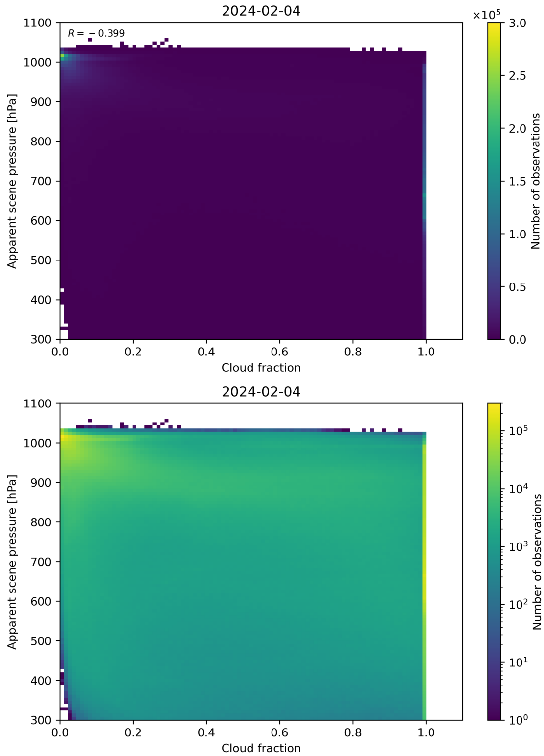
Figure 70: Scatter density plot of “Cloud fraction” against “Apparent scene pressure” for 2024-02-03 to 2024-02-05.
