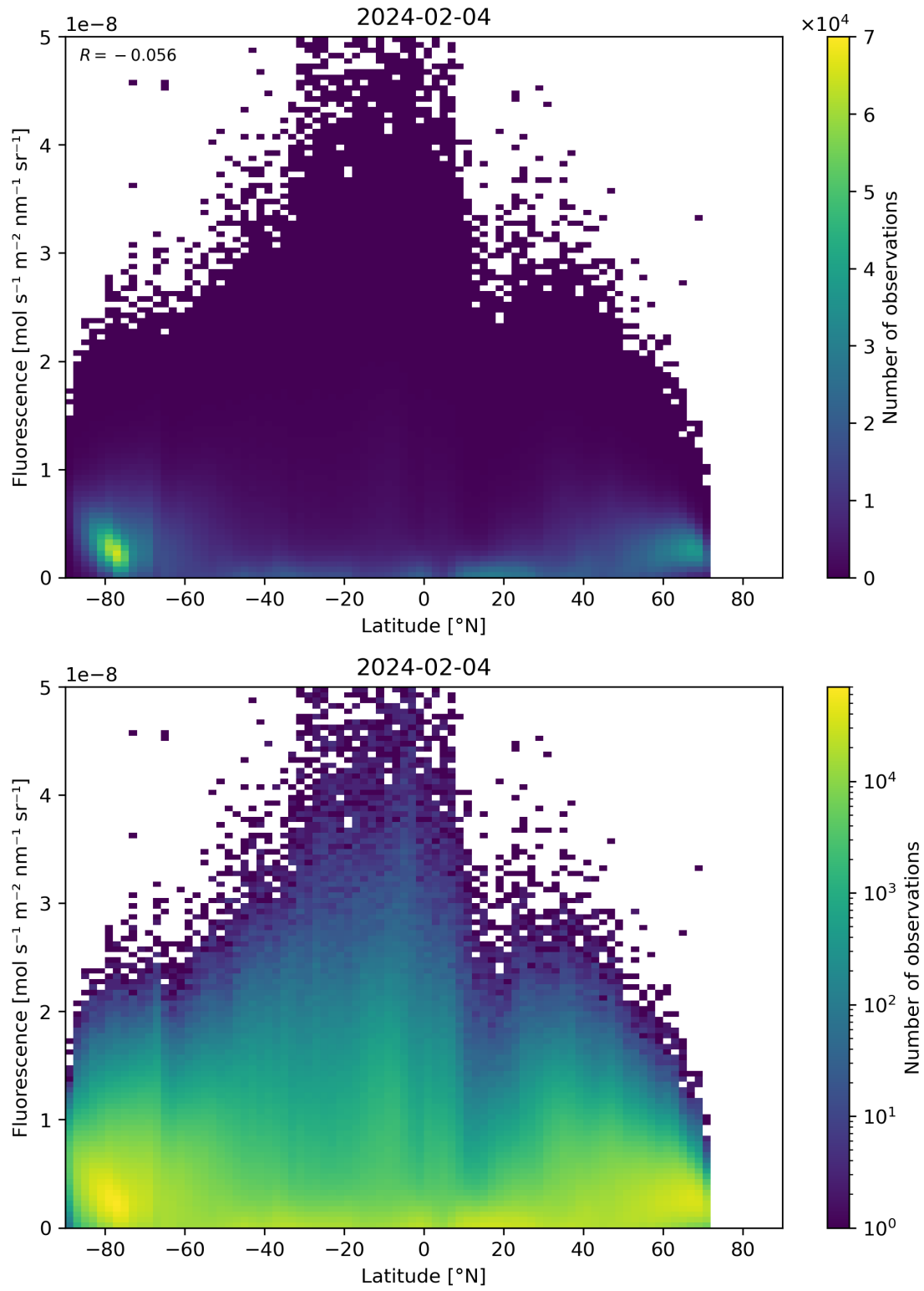
Figure 92: Scatter density plot of “Latitude” against “Fluorescence” for 2024-02-03 to 2024-02-05.
