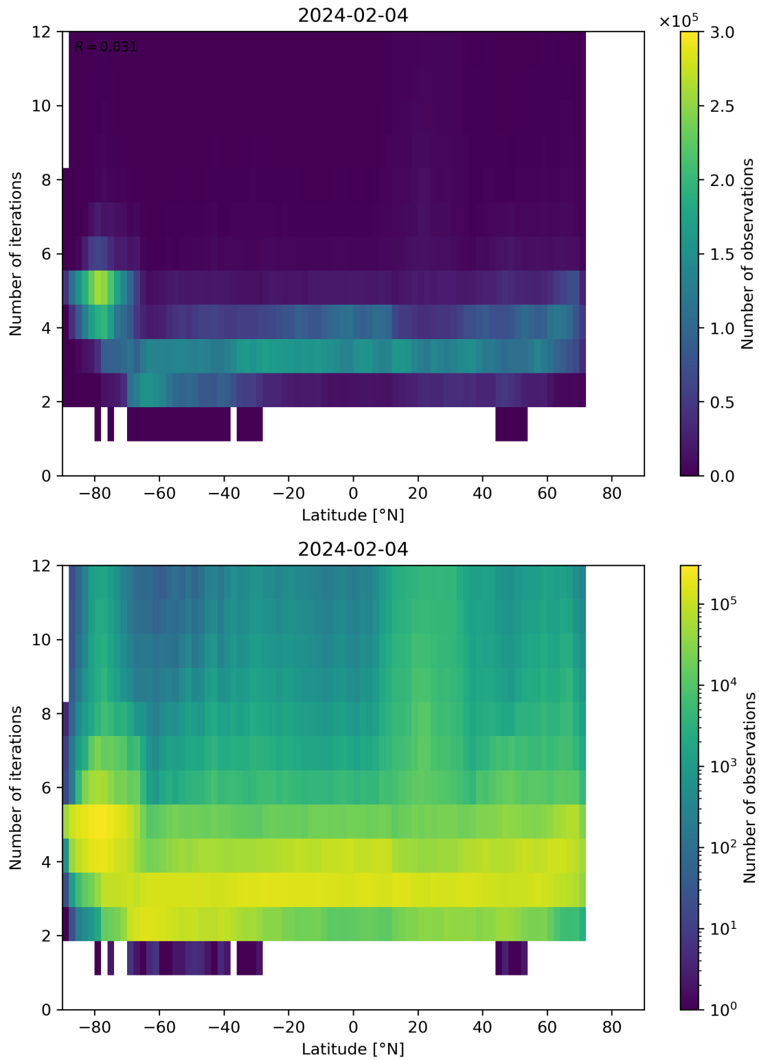
Figure 93: Scatter density plot of “Latitude” against “Number of iterations” for 2024-02-03 to 2024-02-05.
