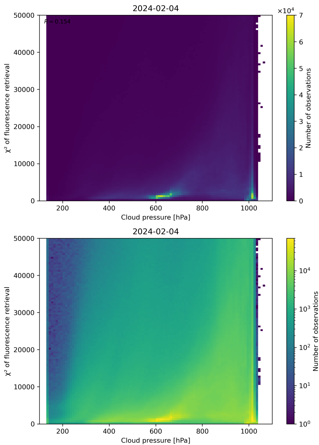
Figure 78: Scatter density plot of “Cloud pressure” against “ \chi^2 of fluorescence retrieval” for 2024-02-03 to 2024-02-05.
