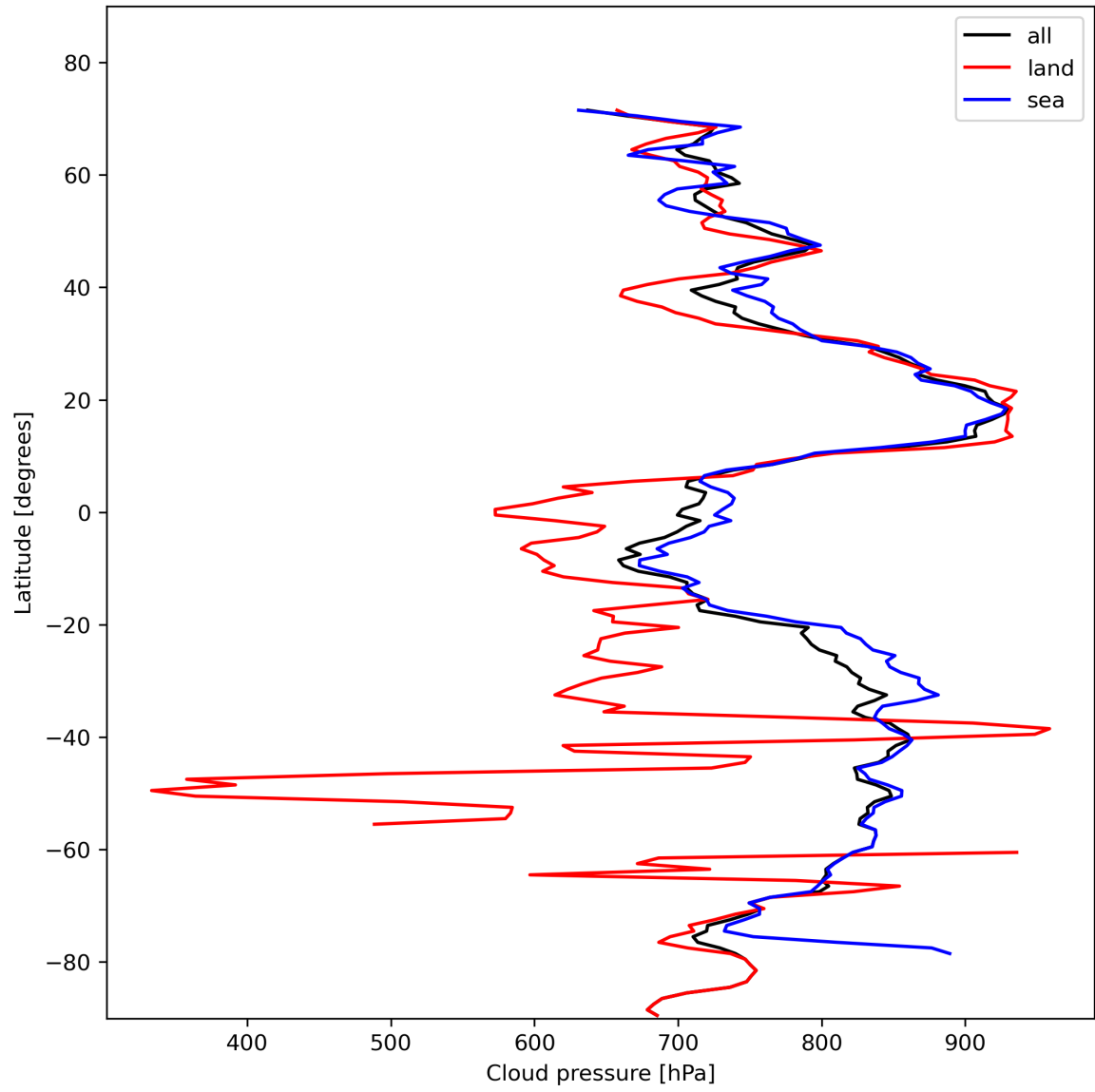
Figure 13: Zonal average of “Cloud pressure” for 2024-02-03 to 2024-02-05.
