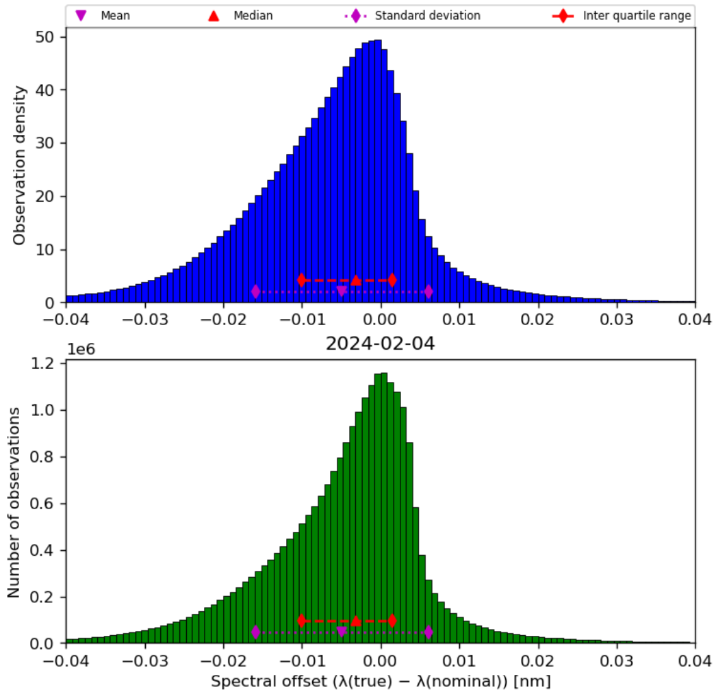
Figure 45: Histogram of “Spectral offset ( \lambda(\text{true}) - \lambda(\text{nominal}) )” for 2024-02-03 to 2024-02-05
