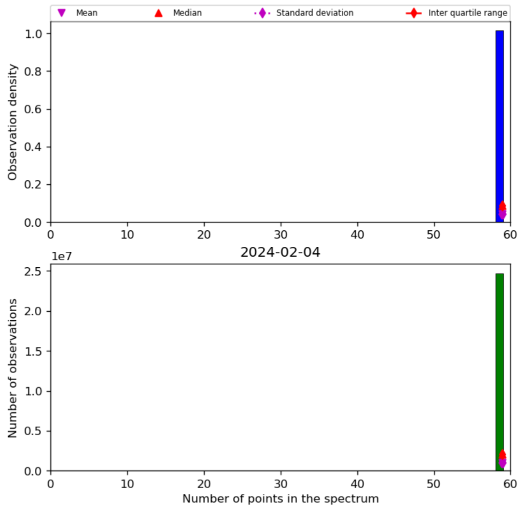
Figure 44: Histogram of “Number of points in the spectrum” for 2024-02-03 to 2024-02-05
