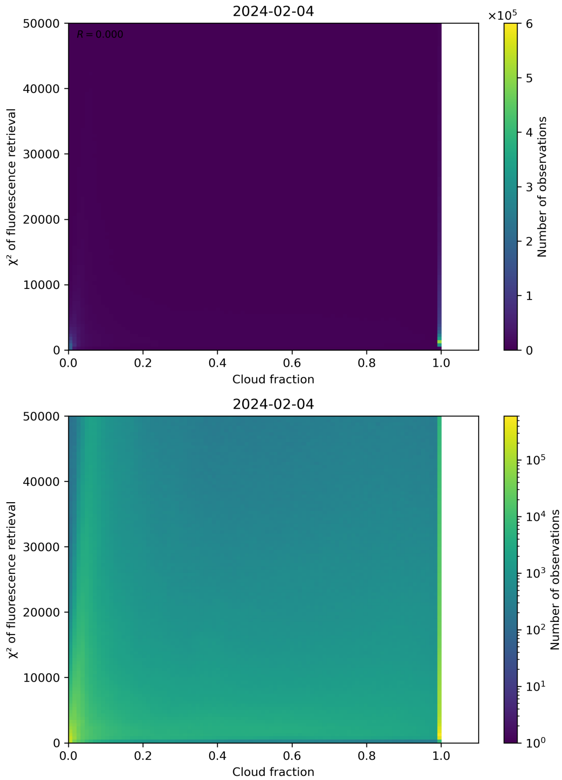
Figure 71: Scatter density plot of “Cloud fraction” against “ \chi^2 of fluorescence retrieval” for 2024-02-03 to 2024-02-05.
