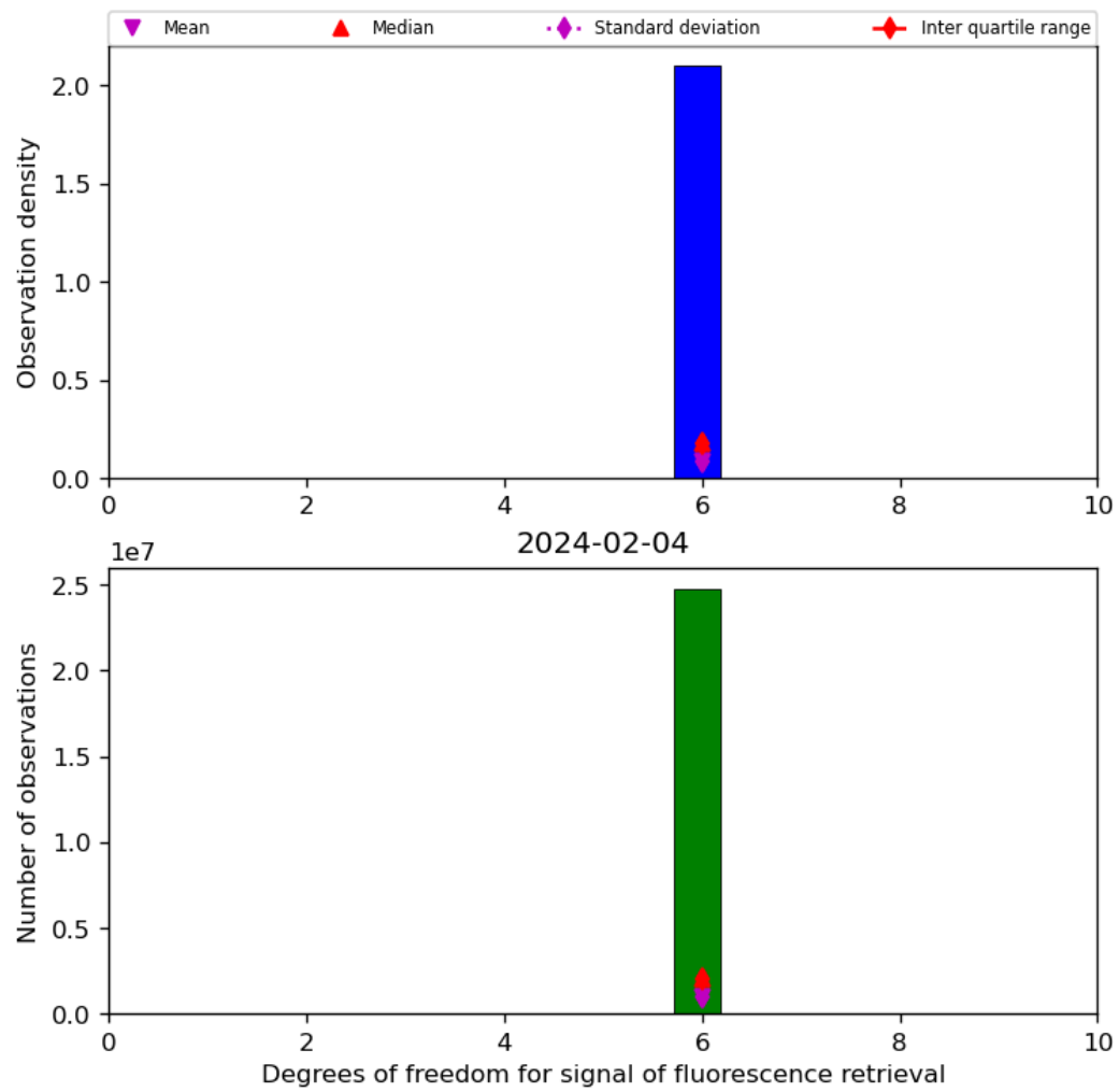
Figure 43: Histogram of “Degrees of freedom for signal of fluorescence retrieval” for 2024-02-03 to 2024-02-05
