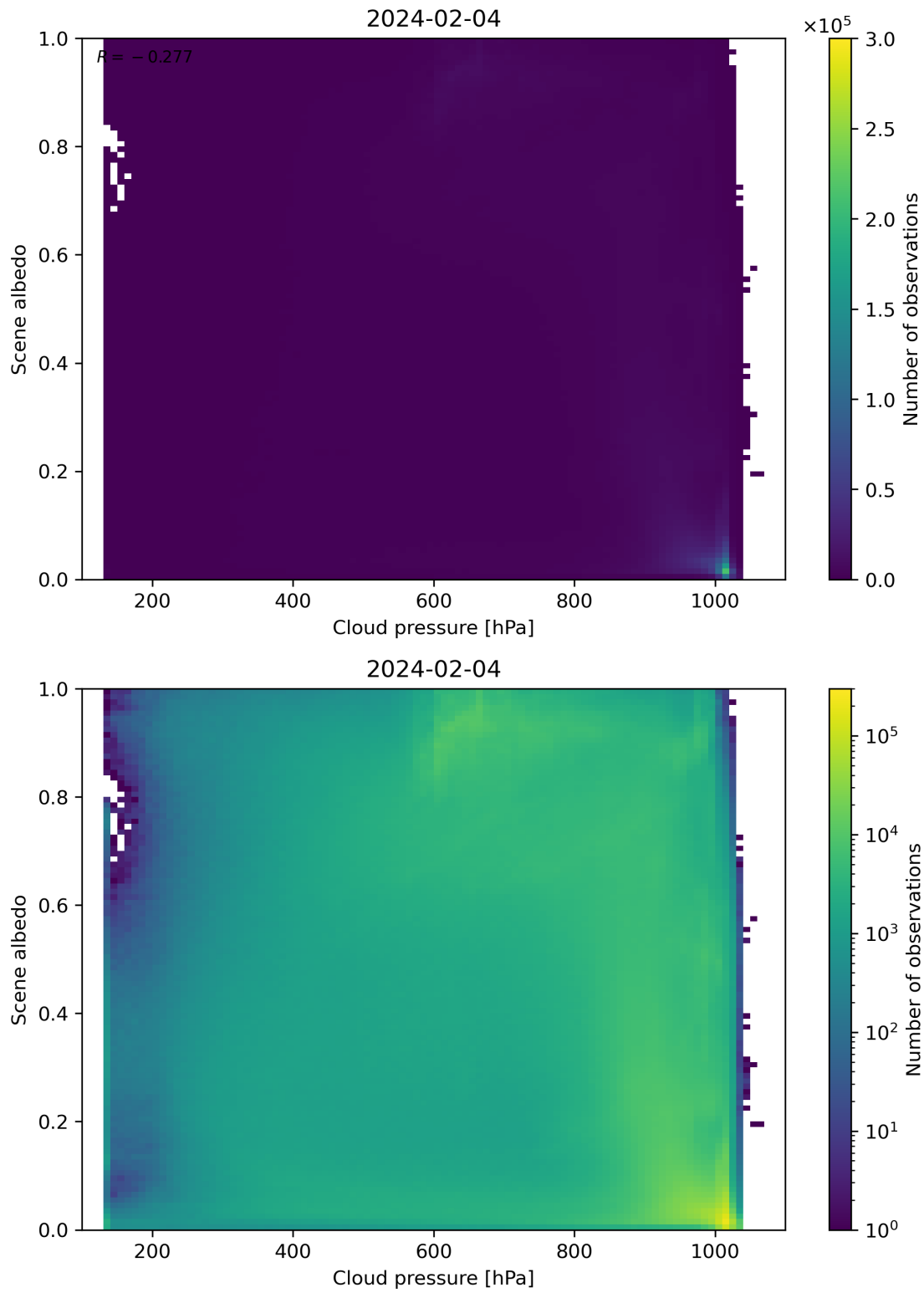
Figure 83: Scatter density plot of “Cloud pressure” against “Scene albedo” for 2024-02-03 to 2024-02-05.
