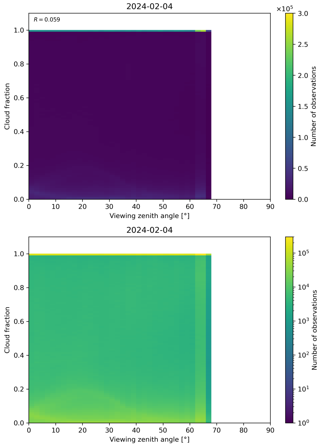
Figure 120: Scatter density plot of “Viewing zenith angle” against “Cloud fraction” for 2024-02-03 to 2024-02-05.
