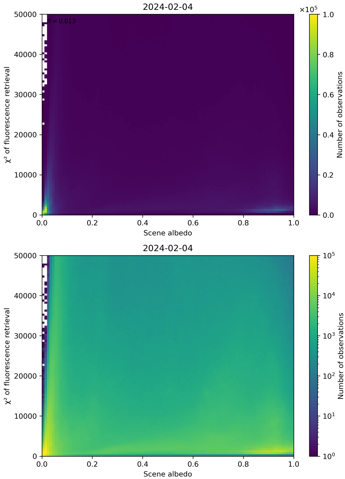
Figure 103: Scatter density plot of “Scene albedo” against “ \chi^2 of fluorescence retrieval” for 2024-02-03 to 2024-02-05.
