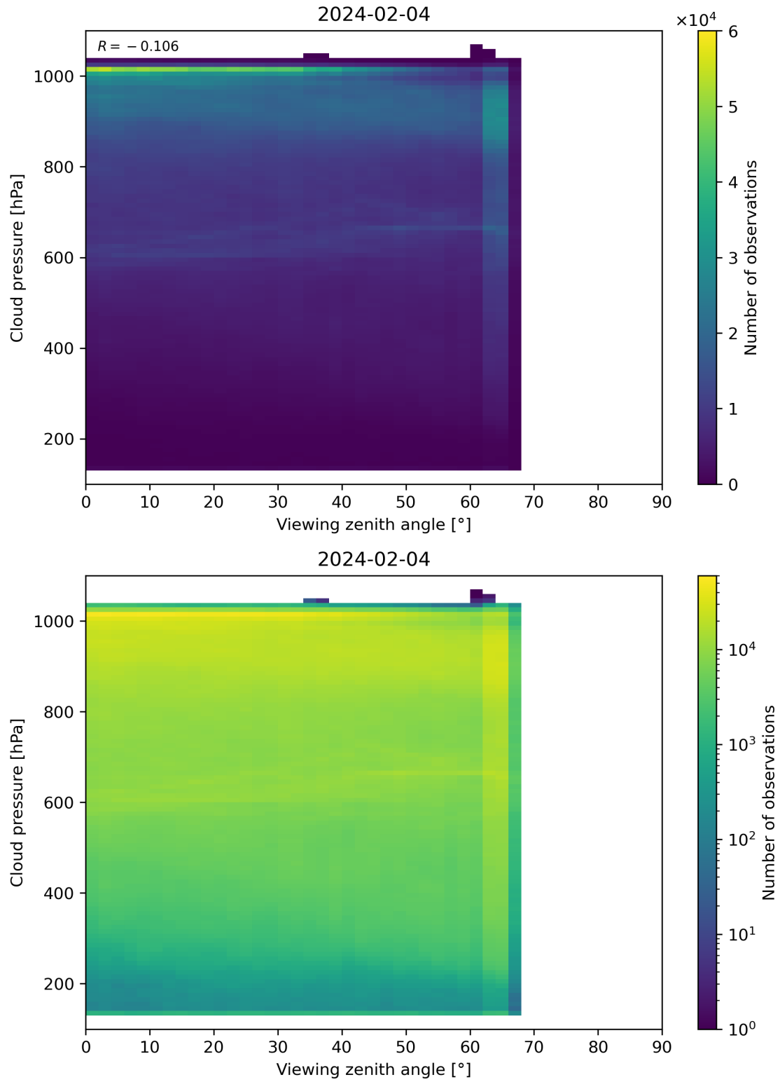
Figure 121: Scatter density plot of “Viewing zenith angle” against “Cloud pressure” for 2024-02-03 to 2024-02-05.
