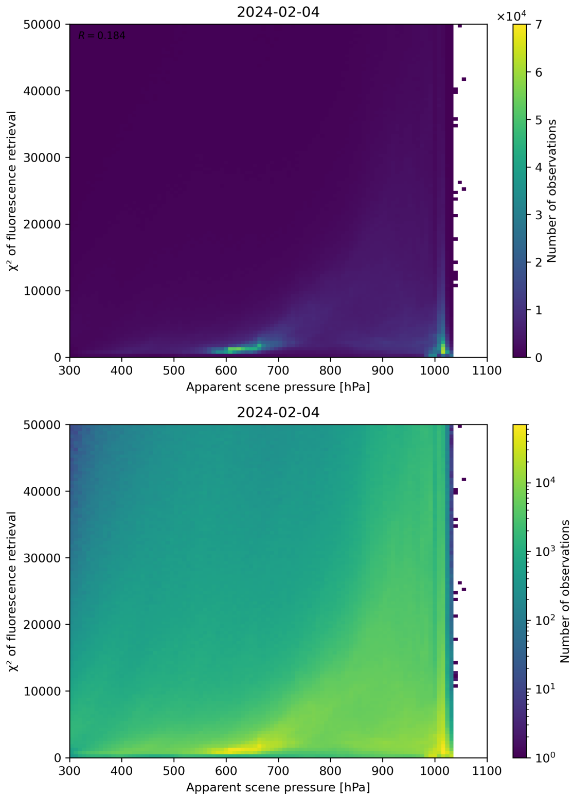
Figure 63: Scatter density plot of “Apparent scene pressure” against “ \chi^2 of fluorescence retrieval” for 2024-02-03 to 2024-02-05.
