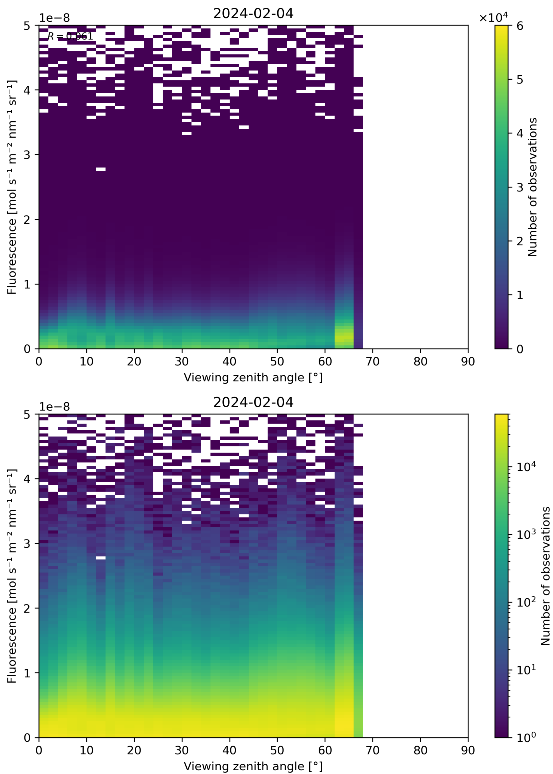
Figure 122: Scatter density plot of “Viewing zenith angle” against “Fluorescence” for 2024-02-03 to 2024-02-05.
