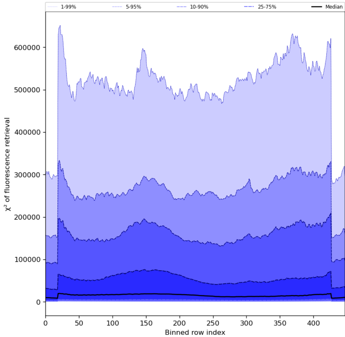
Figure 59: Along track statistics of “ \chi^2 of fluorescence retrieval” for 2024-02-03 to 2024-02-05
