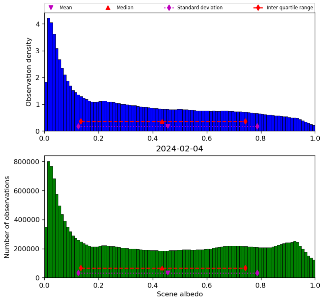
Figure 34: Histogram of “Scene albedo” for 2024-02-03 to 2024-02-05
