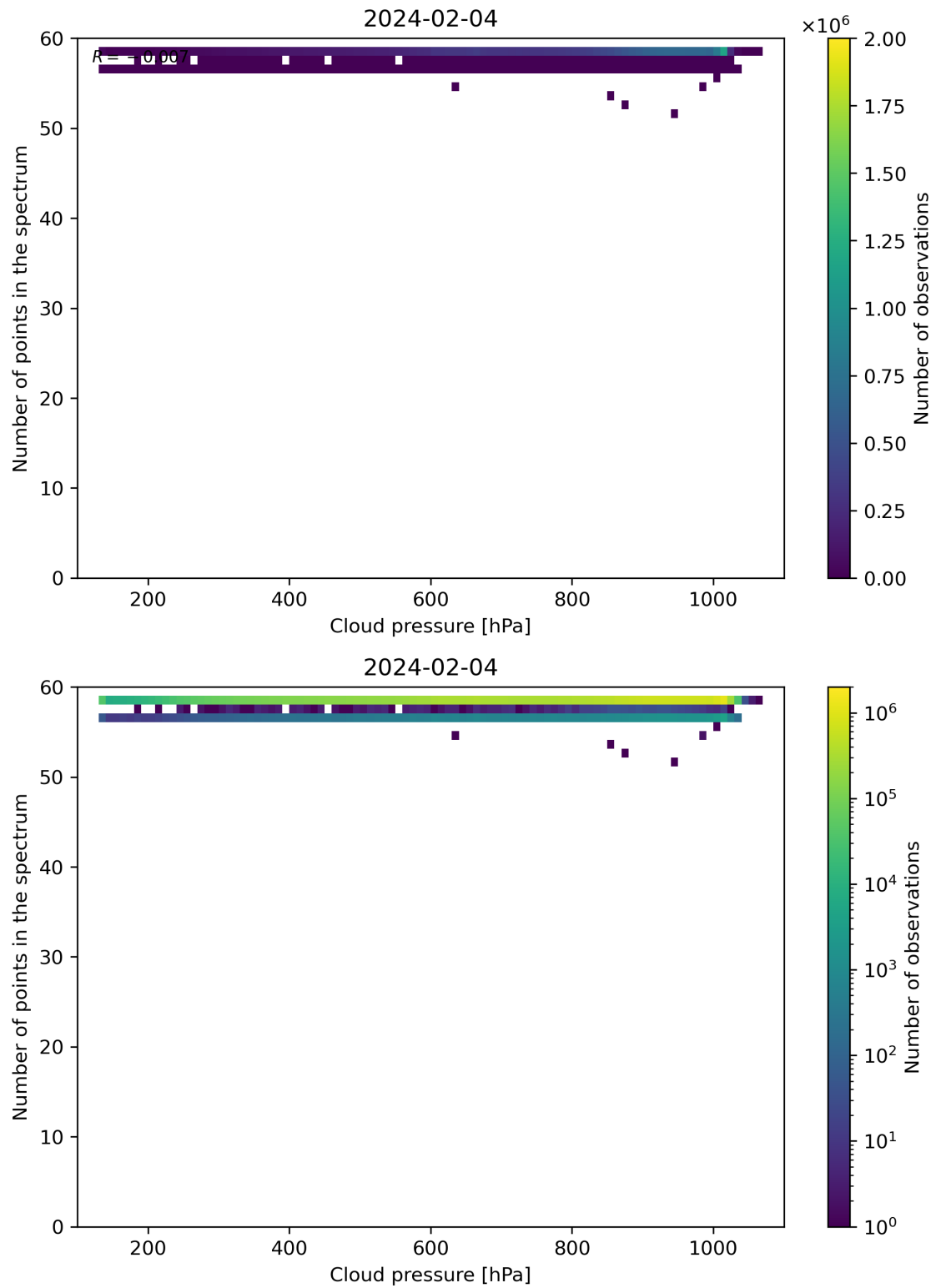
Figure 82: Scatter density plot of “Cloud pressure” against “Number of points in the spectrum” for 2024-02-03 to 2024-02-05.
