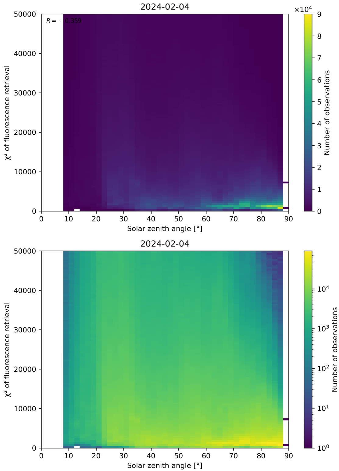
Figure 109: Scatter density plot of “Solar zenith angle” against “ \chi^2 of fluorescence retrieval” for 2024-02-03 to 2024-02-05.
