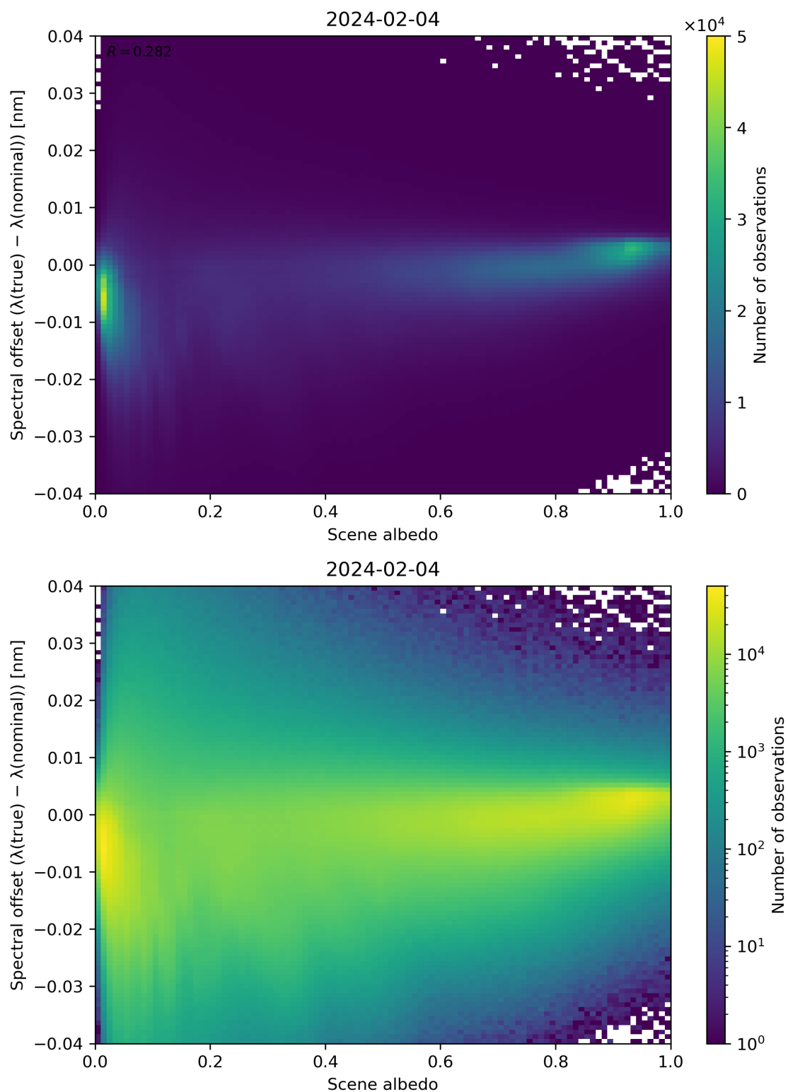
Figure 107: Scatter density plot of “Scene albedo” against “Spectral offset ( \lambda(\text{true}) - \lambda(\text{nominal}) )” for 2024-02-03 to 2024-02-05.
