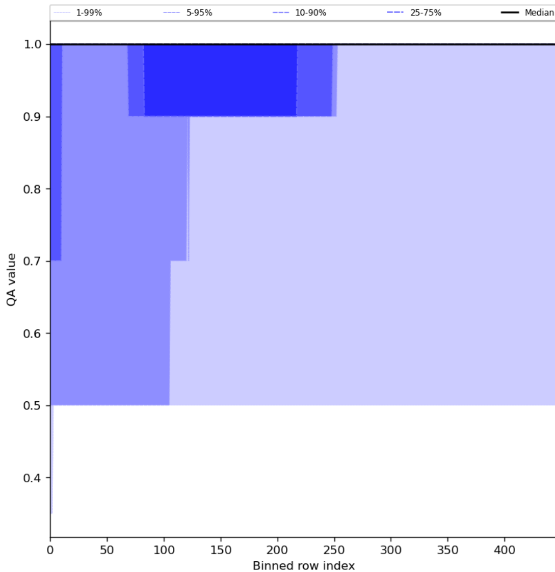
Figure 46: Along track statistics of “QA value” for 2024-02-03 to 2024-02-05
