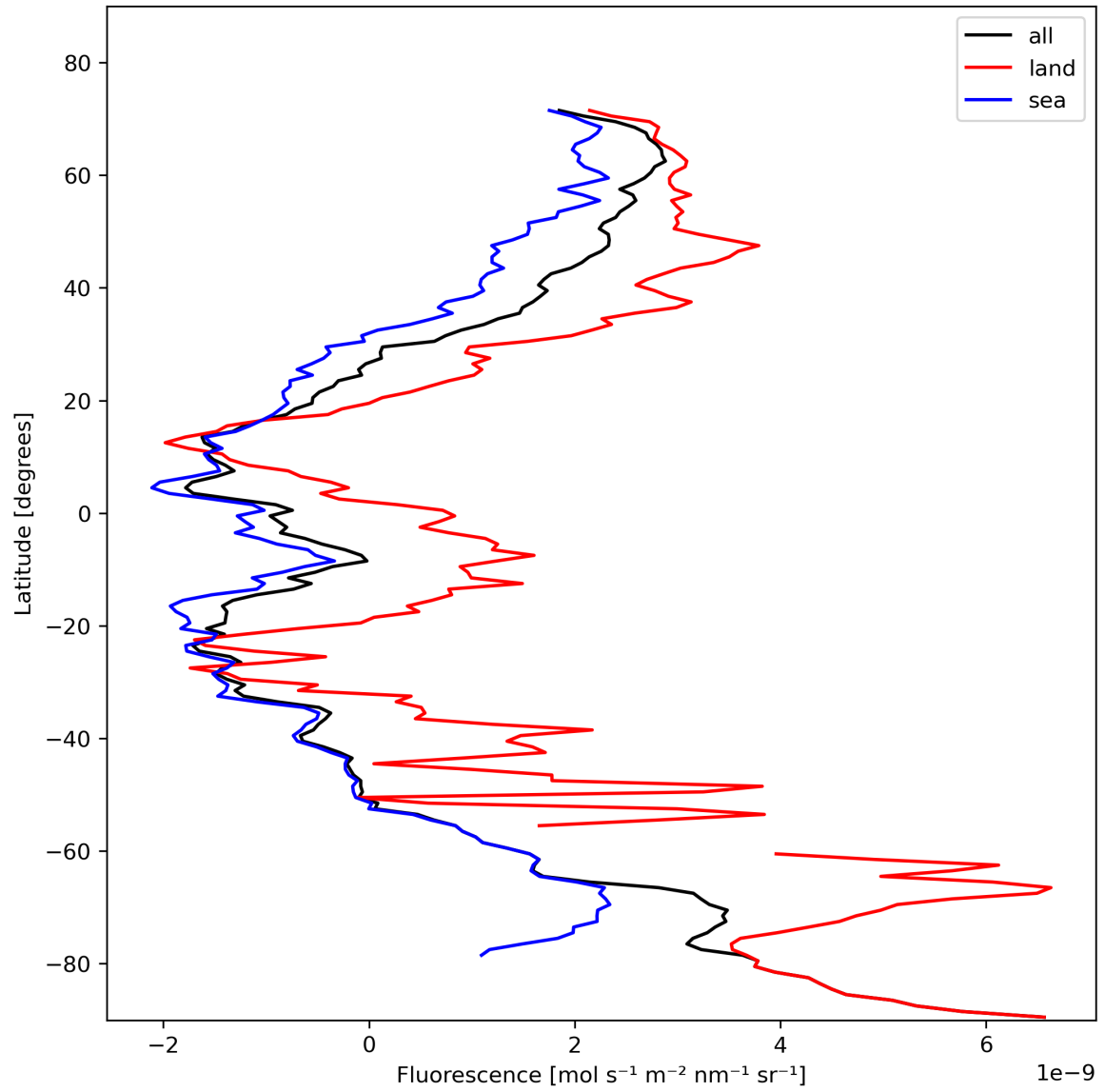
Figure 23: Zonal average of “Fluorescence” for 2024-02-03 to 2024-02-05.
