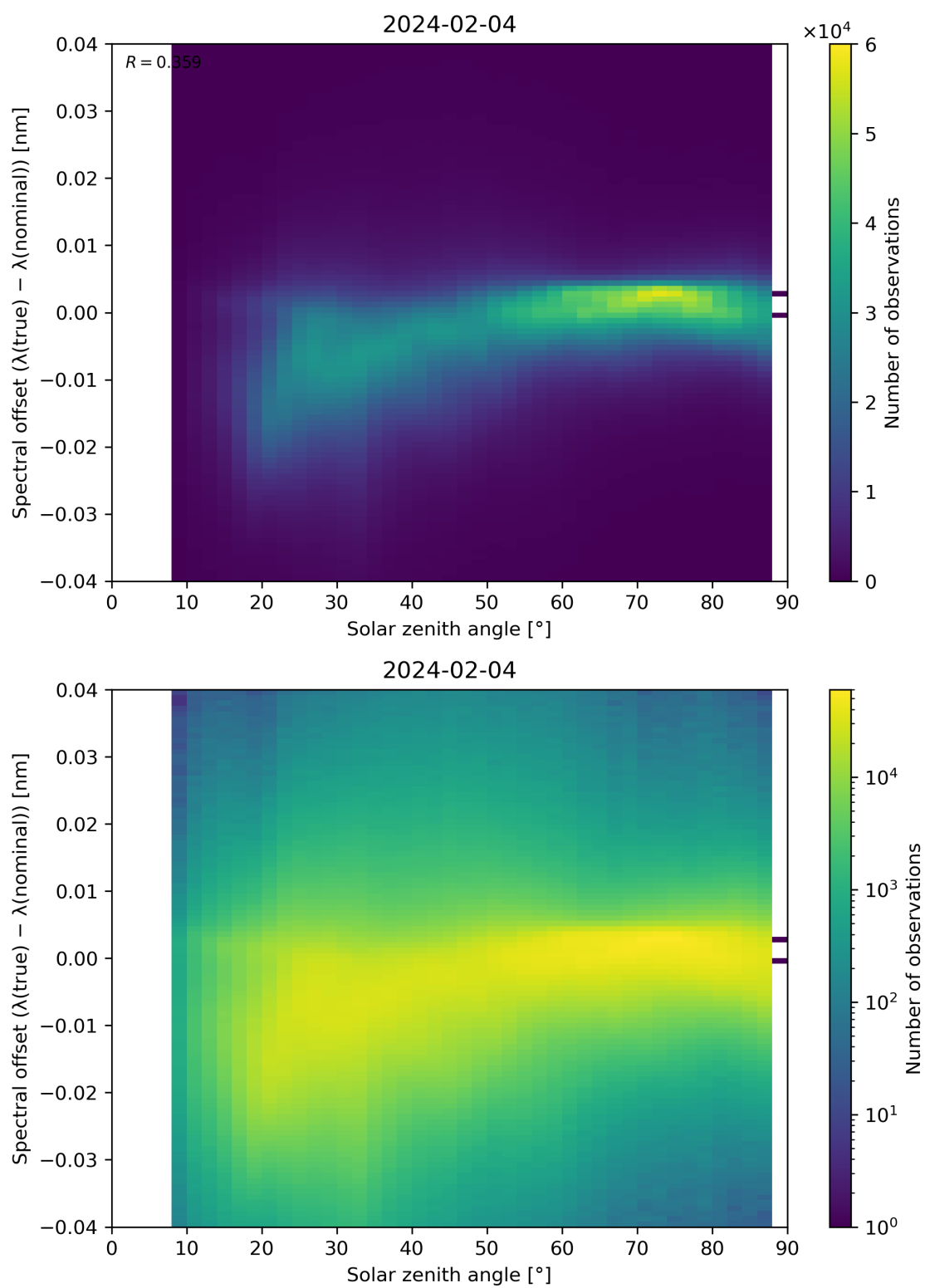
Figure 117: Scatter density plot of “Solar zenith angle” against “Spectral offset ( \lambda(\text{true}) - \lambda(\text{nominal}) )” for 2024-02-03 to 2024-02-05.
