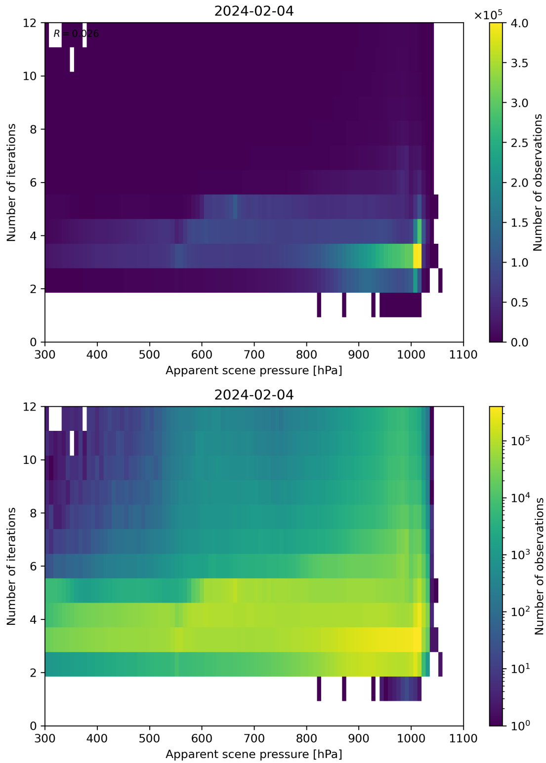
Figure 65: Scatter density plot of “Apparent scene pressure” against “Number of iterations” for 2024-02-03 to 2024-02-05.
