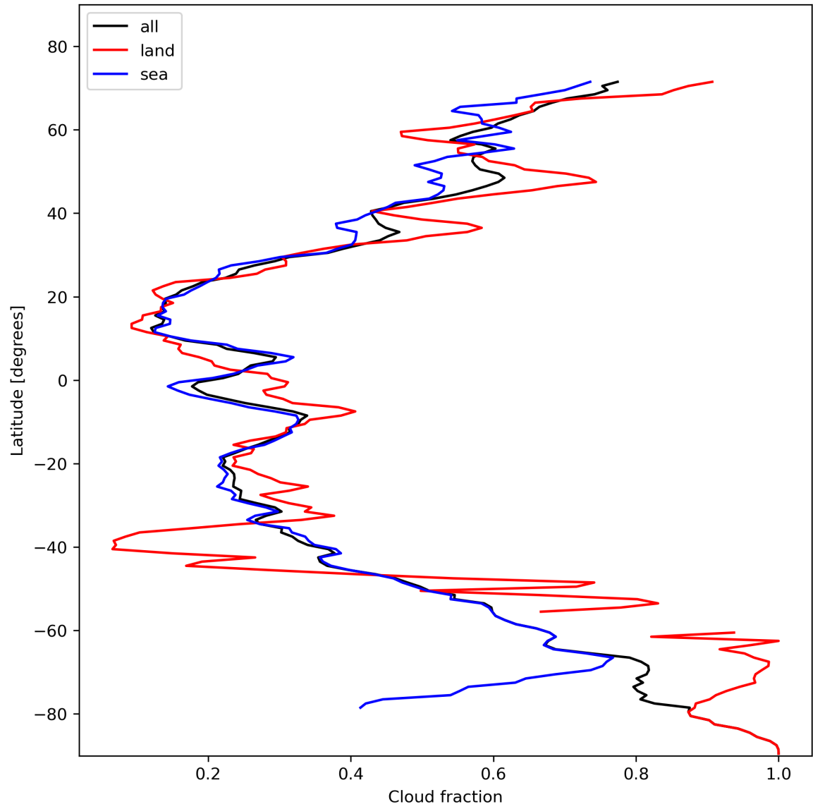
Figure 15: Zonal average of “Cloud fraction” for 2024-02-03 to 2024-02-05.
