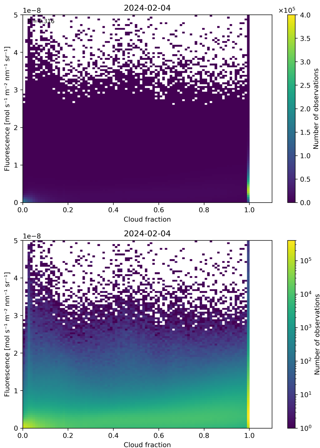
Figure 72: Scatter density plot of “Cloud fraction” against “Fluorescence” for 2024-02-03 to 2024-02-05.
