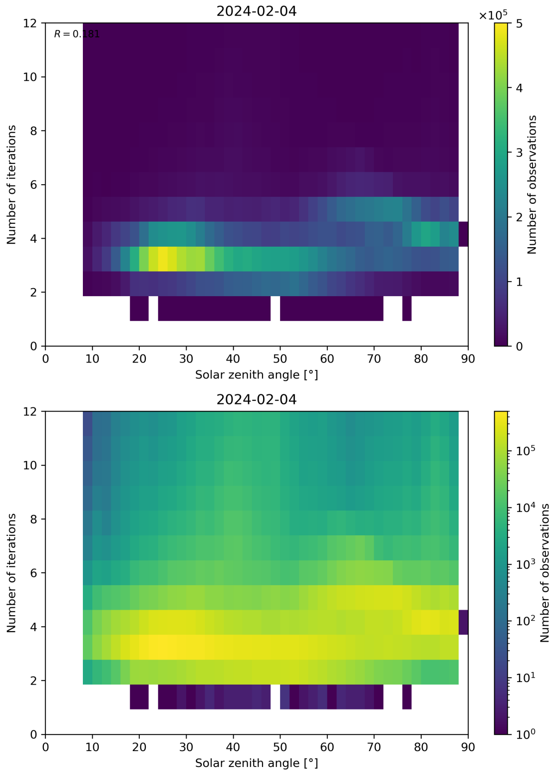
Figure 114: Scatter density plot of “Solar zenith angle” against “Number of iterations” for 2024-02-03 to 2024-02-05.
