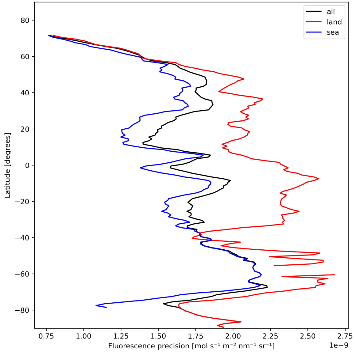
Figure 24: Zonal average of “Fluorescence precision” for 2024-02-03 to 2024-02-05.
