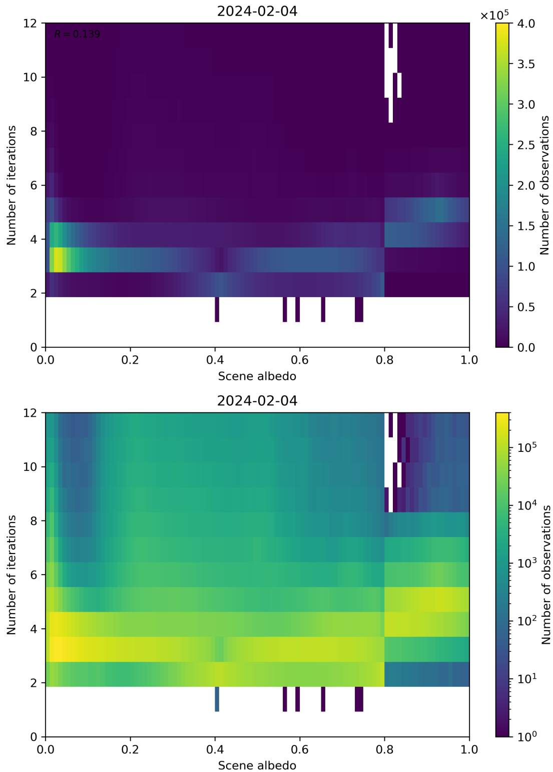
Figure 105: Scatter density plot of “Scene albedo” against “Number of iterations” for 2024-02-03 to 2024-02-05.
