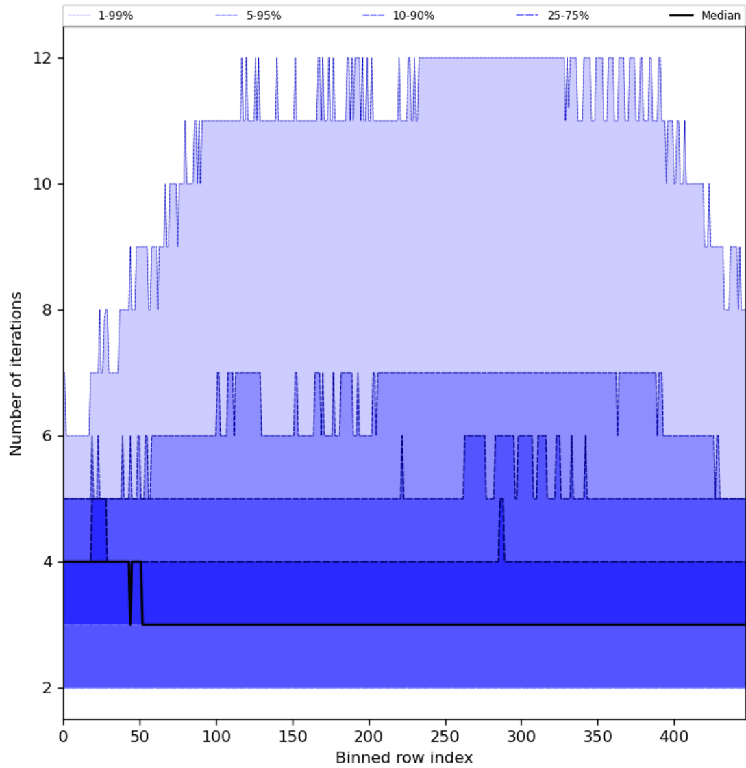
Figure 56: Along track statistics of “Number of iterations” for 2024-02-03 to 2024-02-05
