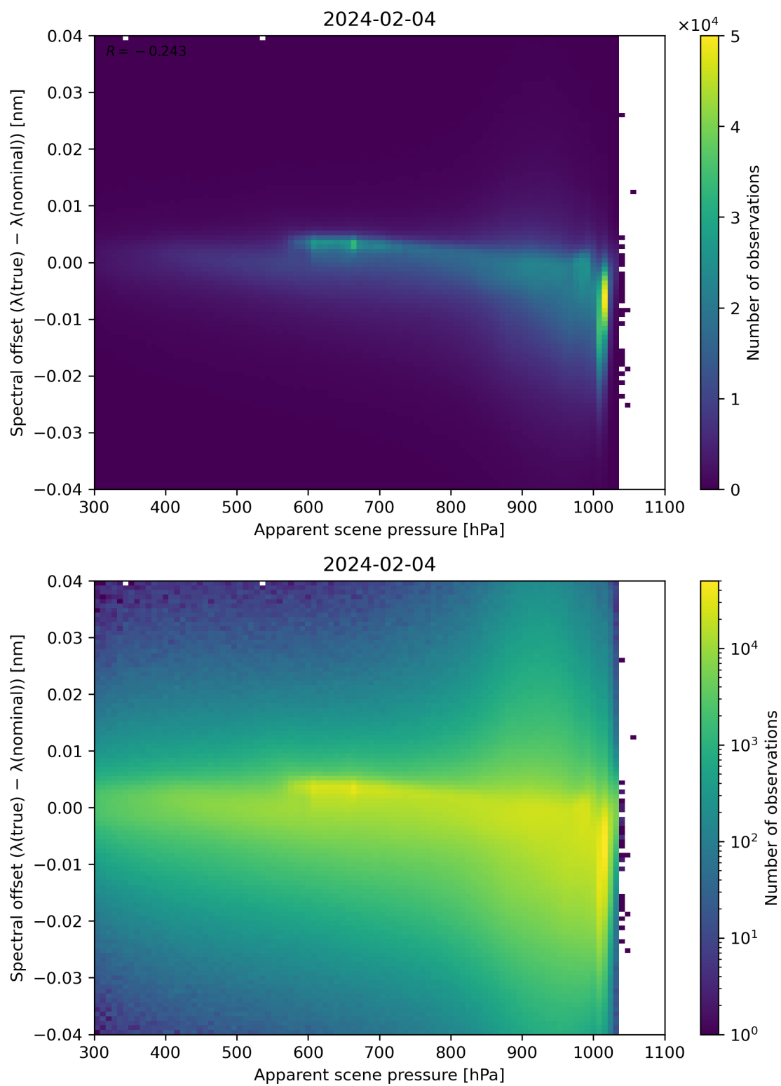
Figure 67: Scatter density plot of “Apparent scene pressure” against “Spectral offset ( \lambda(\text{true}) - \lambda(\text{nominal}) )” for 2024-02-03 to 2024-02-05.
