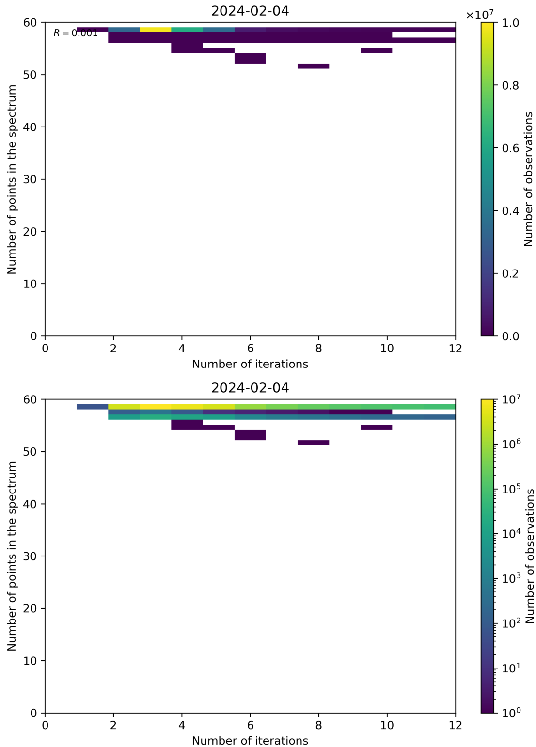
Figure 99: Scatter density plot of “Number of iterations” against “Number of points in the spectrum” for 2024-02-03 to 2024-02-05.
