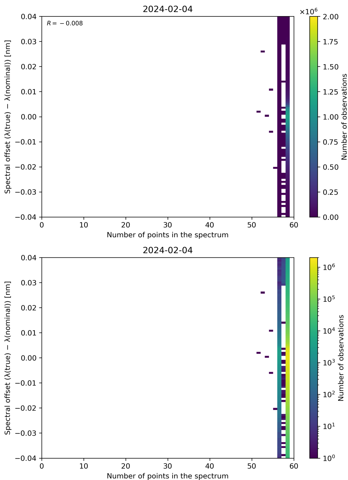
Figure 101: Scatter density plot of “Number of points in the spectrum” against “Spectral offset ( \lambda(\text{true}) - \lambda(\text{nominal}) )” for 2024-02-03 to 2024-02-05.
