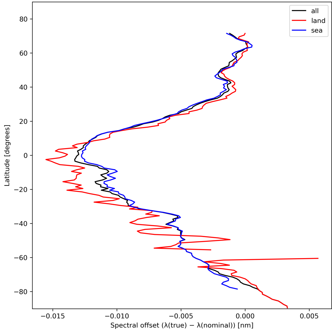
Figure 28: Zonal average of “Spectral offset ( \lambda(\text{true}) - \lambda(\text{nominal}) )” for 2024-02-03 to 2024-02-05.
