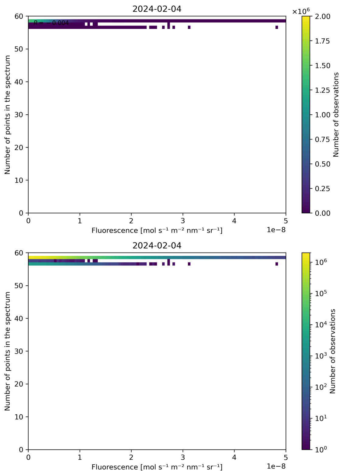
Figure 86: Scatter density plot of “Fluorescence” against “Number of points in the spectrum” for 2024-02-03 to 2024-02-05.
