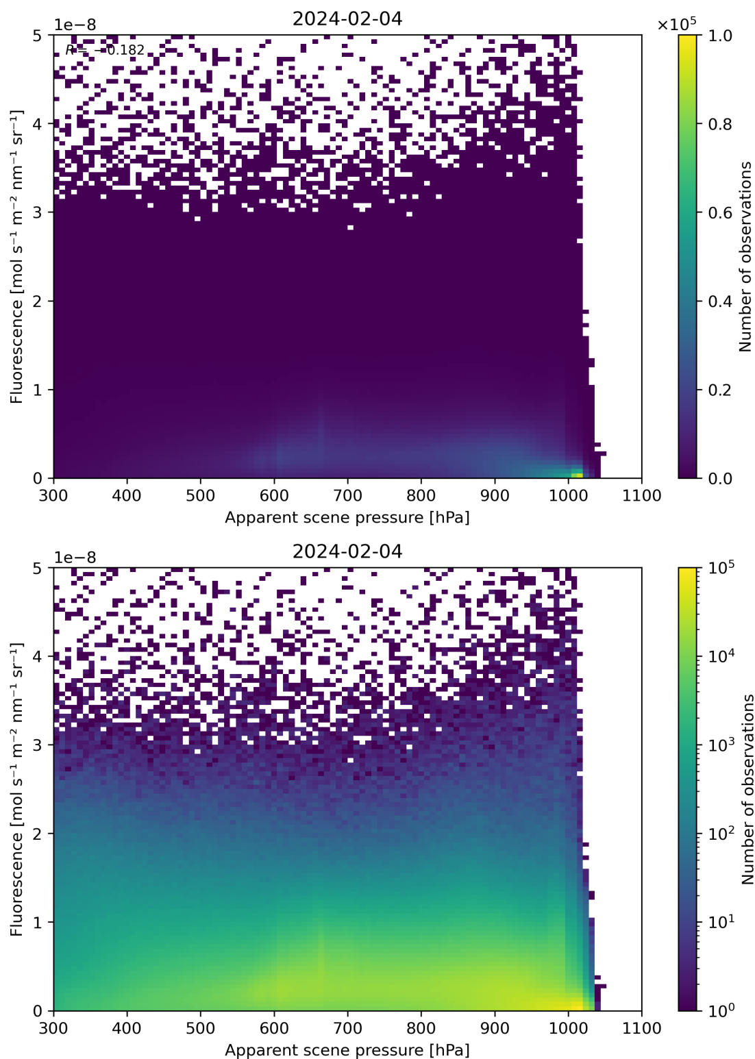
Figure 64: Scatter density plot of “Apparent scene pressure” against “Fluorescence” for 2024-02-03 to 2024-02-05.
