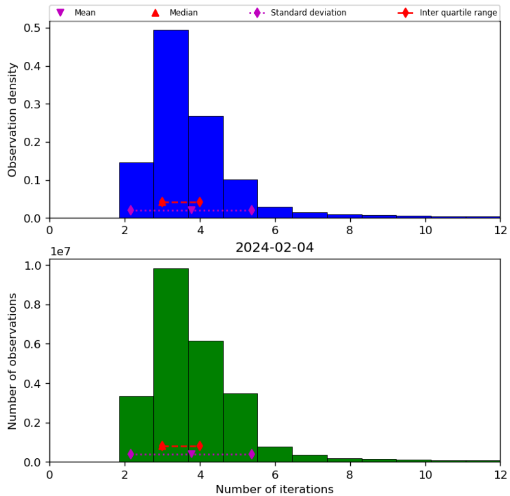
Figure 39: Histogram of “Number of iterations” for 2024-02-03 to 2024-02-05
