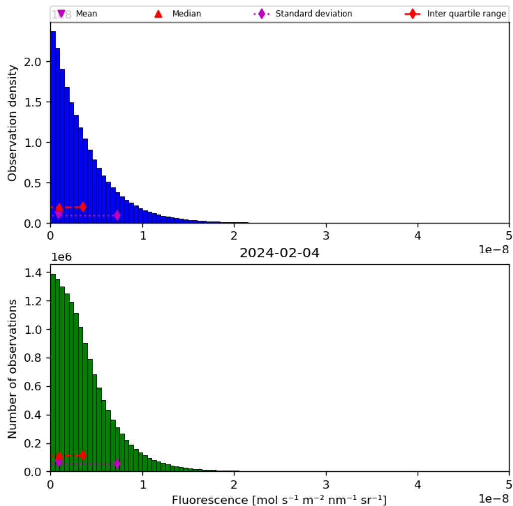
Figure 40: Histogram of “Fluorescence” for 2024-02-03 to 2024-02-05
