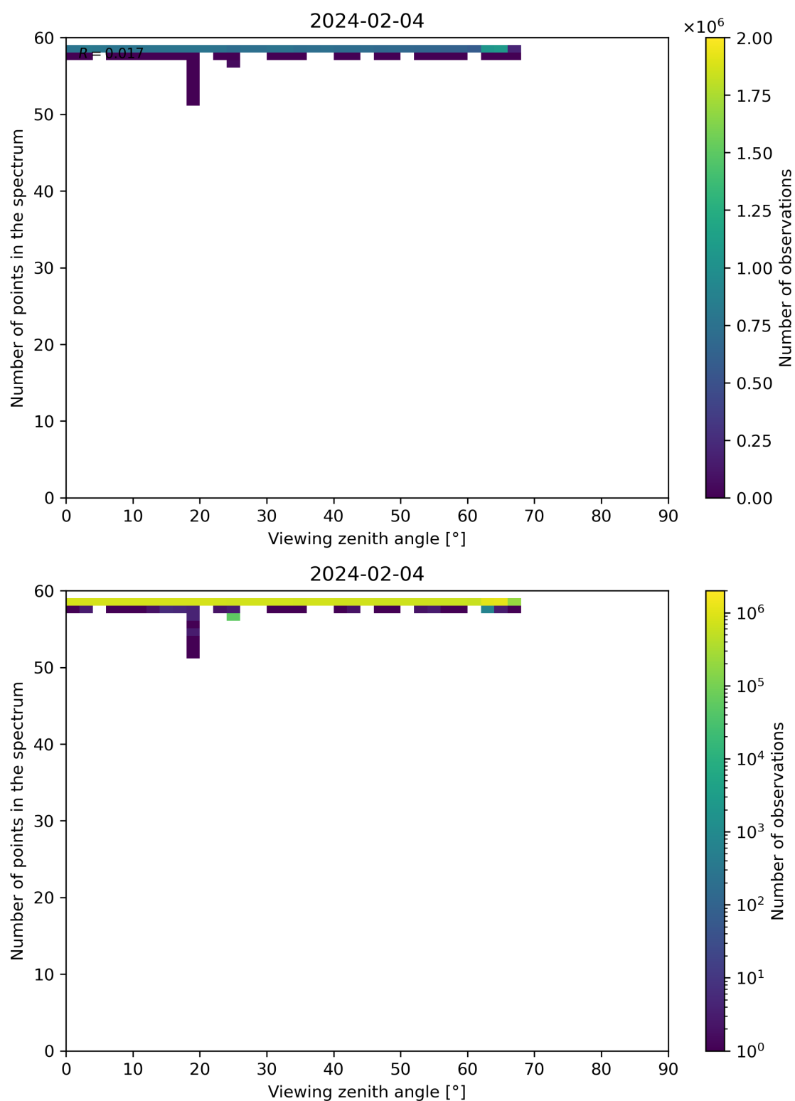
Figure 125: Scatter density plot of “Viewing zenith angle” against “Number of points in the spectrum” for 2024-02-03 to 2024-02-05.
