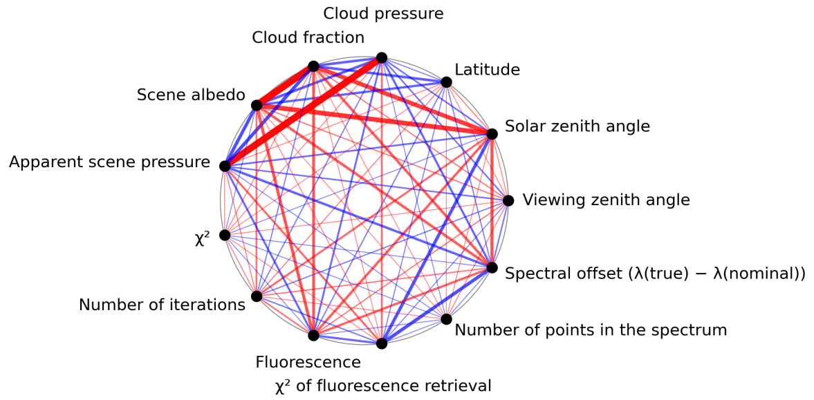
Figure 1: Map of correlation graph for 2024-02-03 to 2024-02-05.
