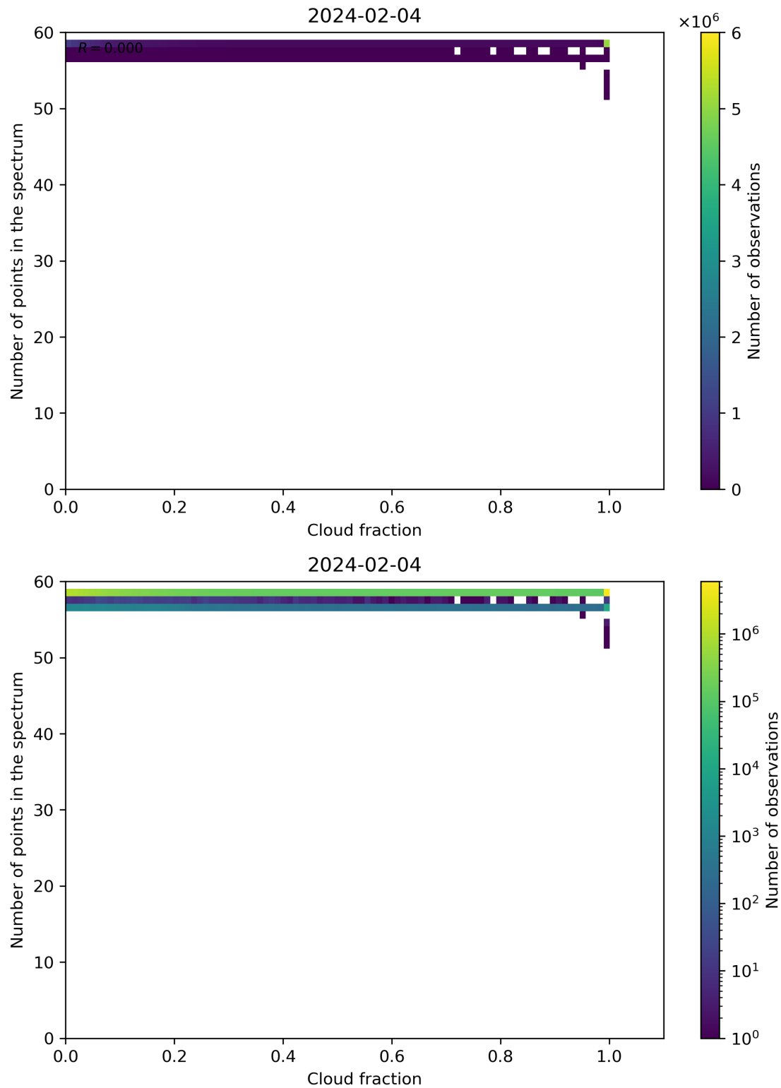
Figure 74: Scatter density plot of “Cloud fraction” against “Number of points in the spectrum” for 2024-02-03 to 2024-02-05.
