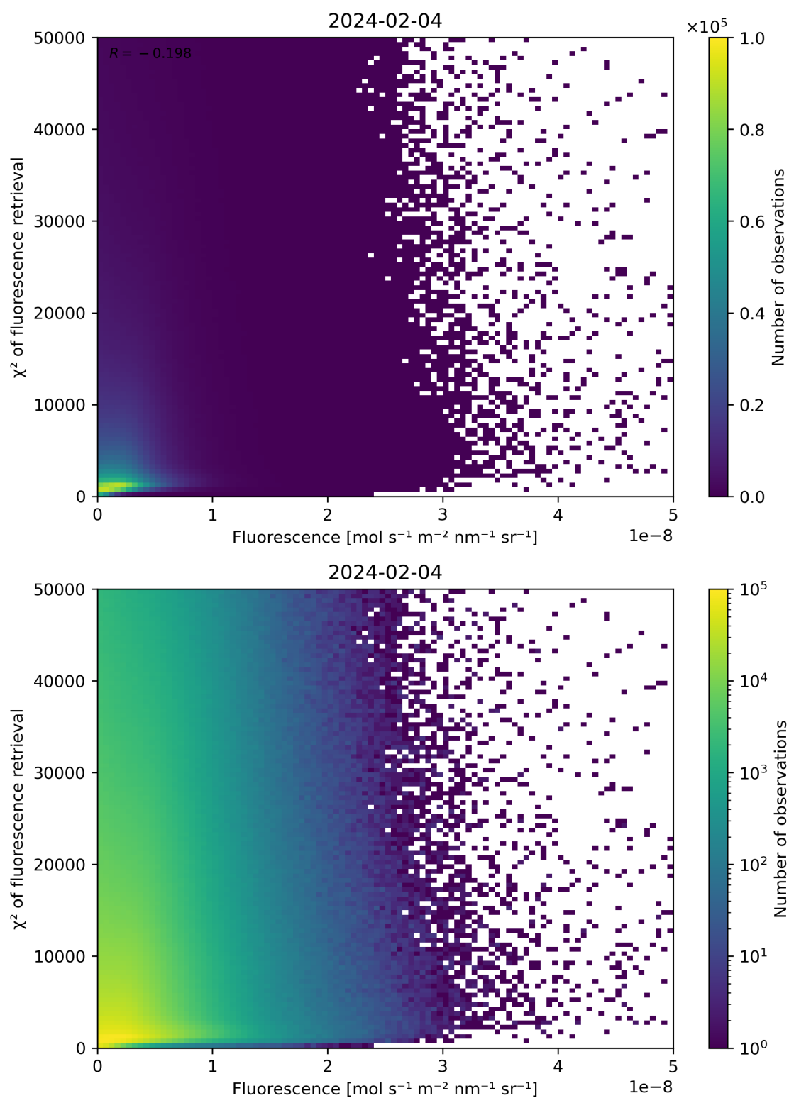
Figure 85: Scatter density plot of “Fluorescence” against “ \chi^2 of fluorescence retrieval” for 2024-02-03 to 2024-02-05.
