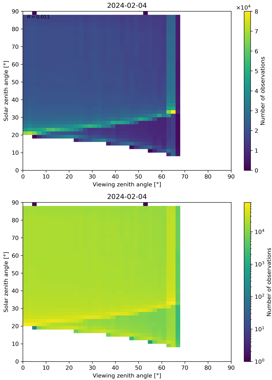
Figure 127: Scatter density plot of “Viewing zenith angle” against “Solar zenith angle” for 2024-02-03 to 2024-02-05.
