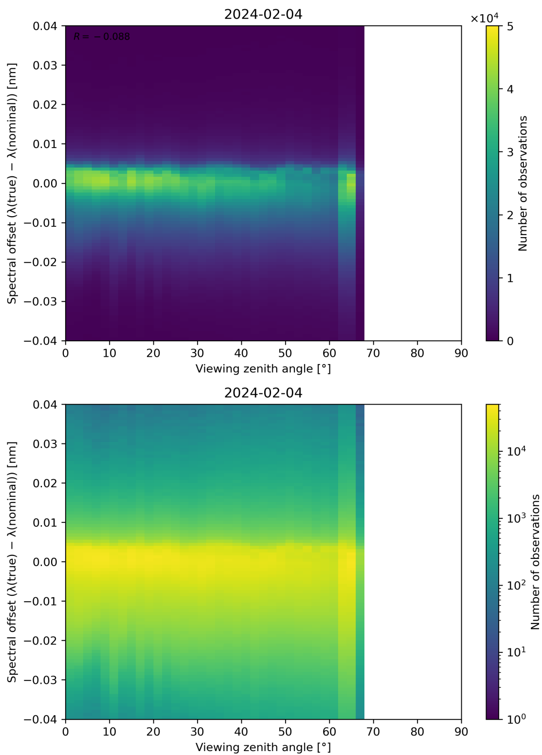
Figure 128: Scatter density plot of “Viewing zenith angle” against “Spectral offset ( \lambda(\text{true}) - \lambda(\text{nominal}) )” for 2024-02-03 to 2024-02-05.
