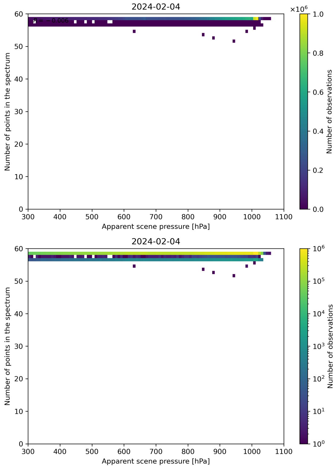
Figure 66: Scatter density plot of “Apparent scene pressure” against “Number of points in the spectrum” for 2024-02-03 to 2024-02-05.
