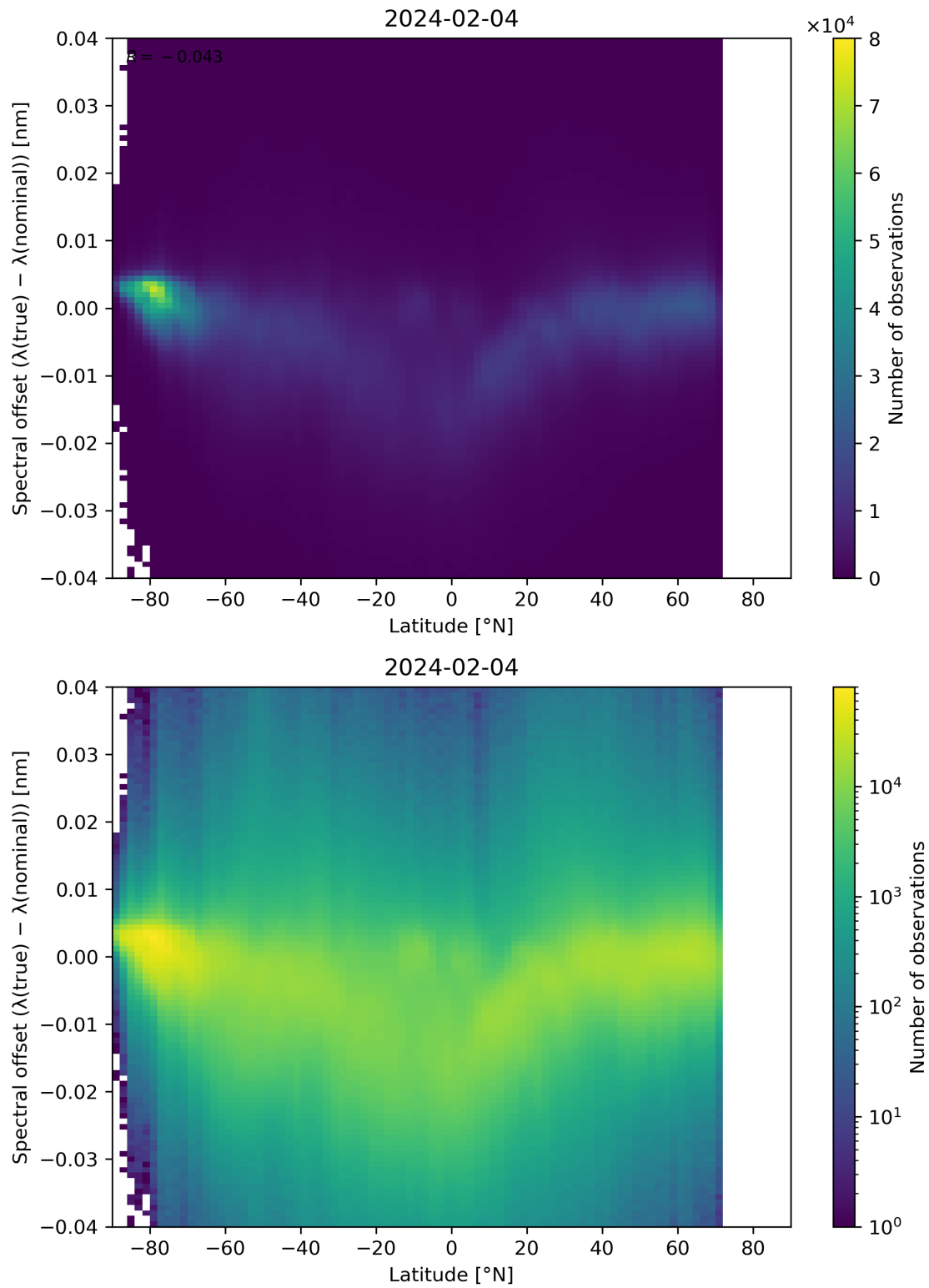
Figure 96: Scatter density plot of “Latitude” against “Spectral offset ( \lambda(\text{true}) - \lambda(\text{nominal}) )” for 2024-02-03 to 2024-02-05.
