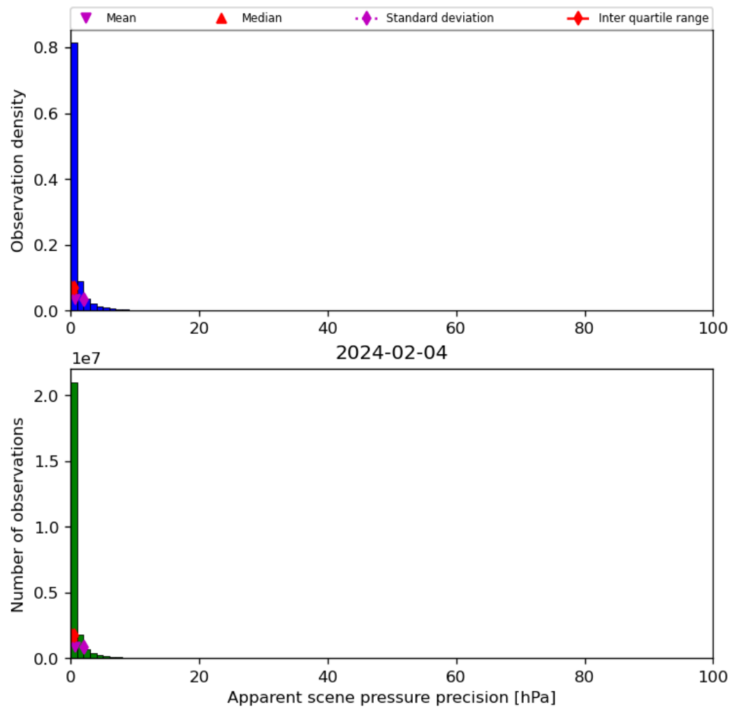
Figure 37: Histogram of “Apparent scene pressure precision” for 2024-02-03 to 2024-02-05
