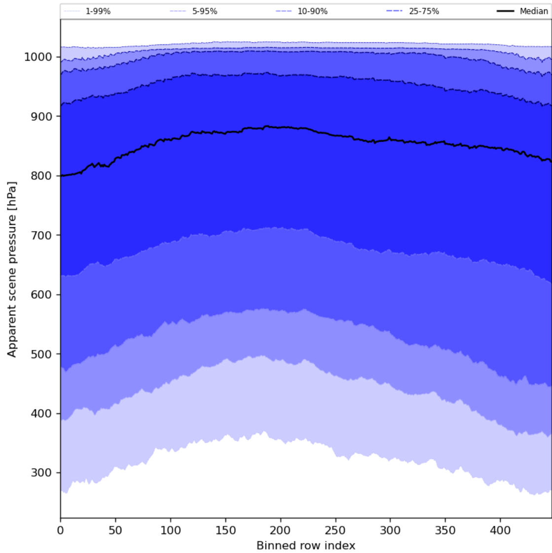
Figure 53: Along track statistics of “Apparent scene pressure” for 2024-02-03 to 2024-02-05
