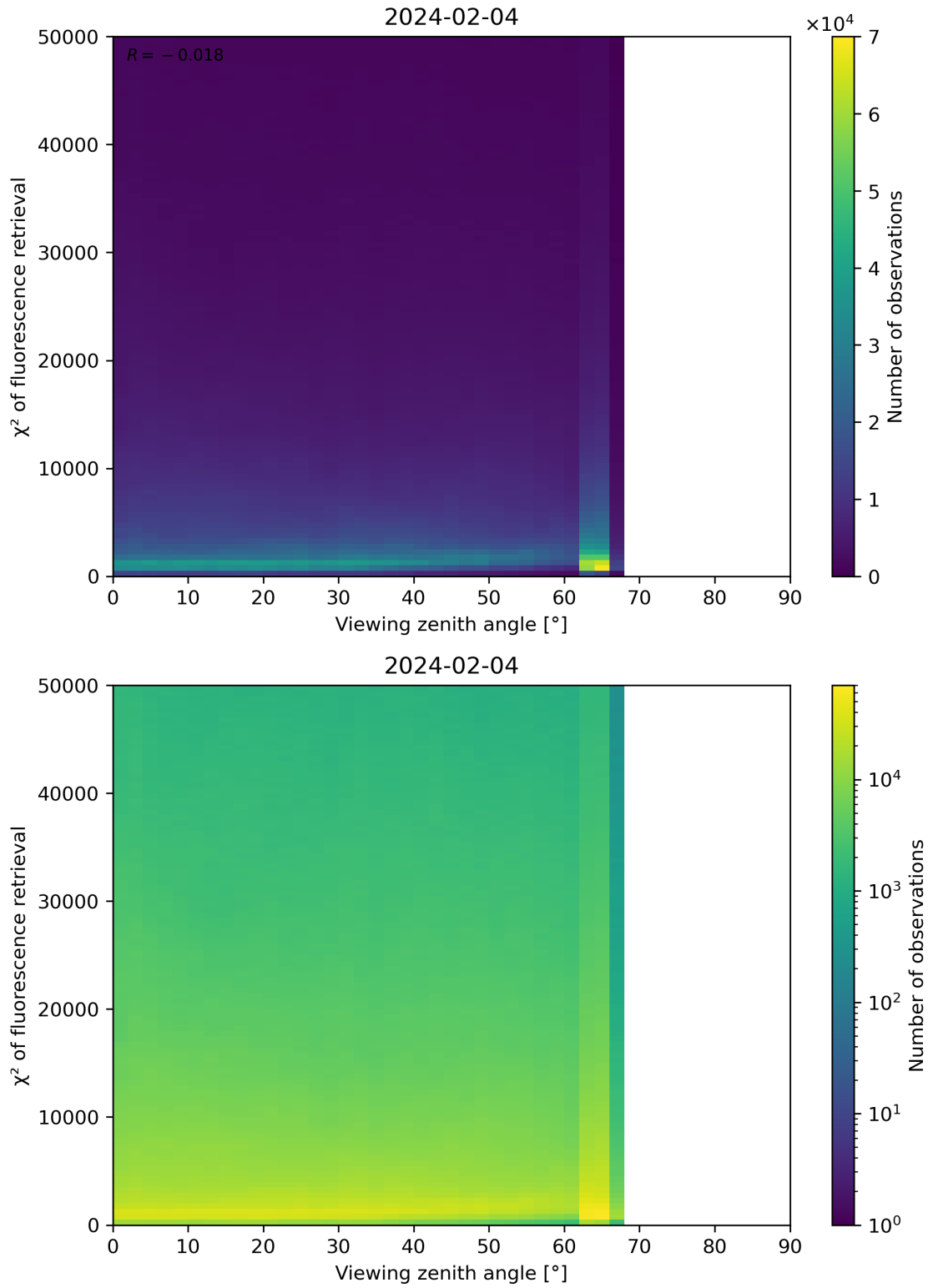
Figure 119: Scatter density plot of “Viewing zenith angle” against “ \chi^2 of fluorescence retrieval” for 2024-02-03 to 2024-02-05.
