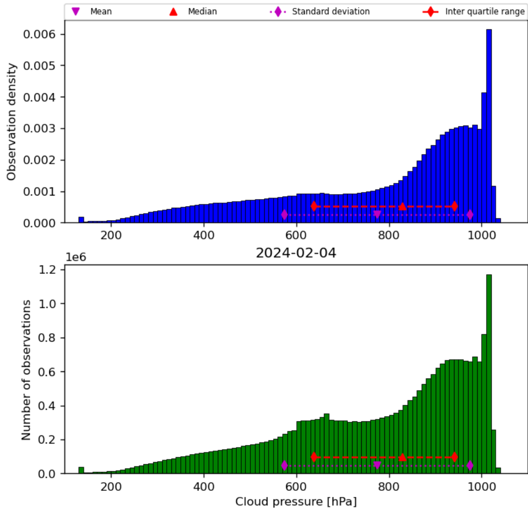
Figure 30: Histogram of “Cloud pressure” for 2024-02-03 to 2024-02-05
