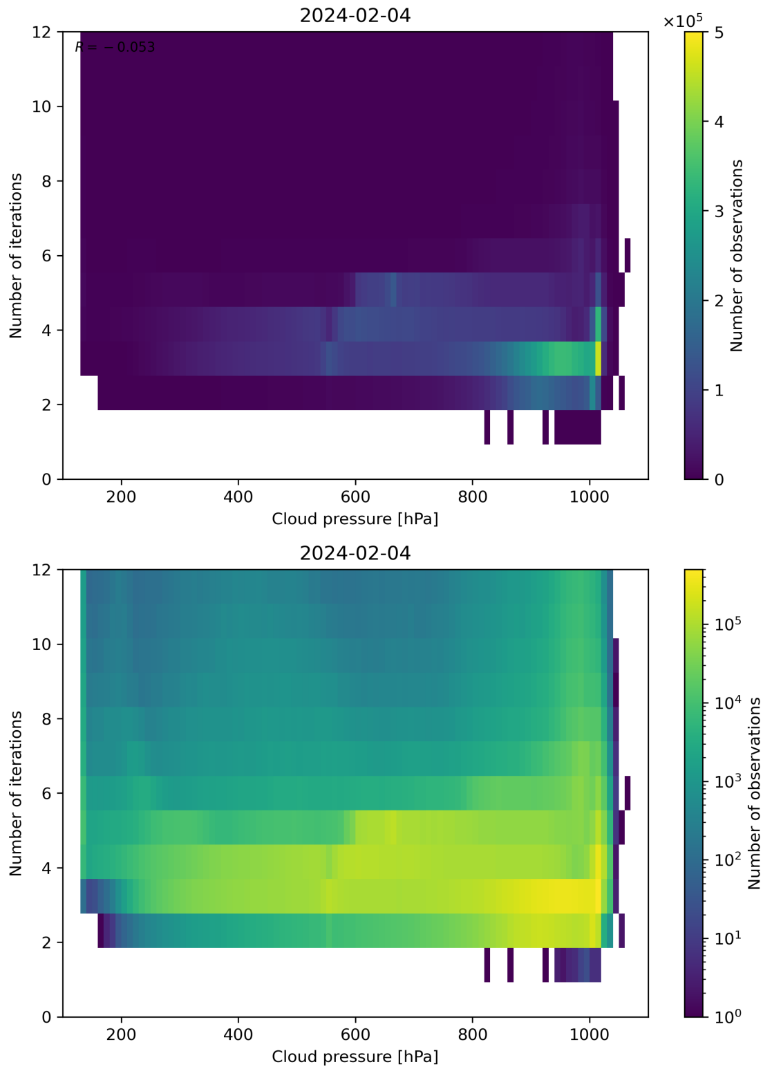
Figure 81: Scatter density plot of “Cloud pressure” against “Number of iterations” for 2024-02-03 to 2024-02-05.
