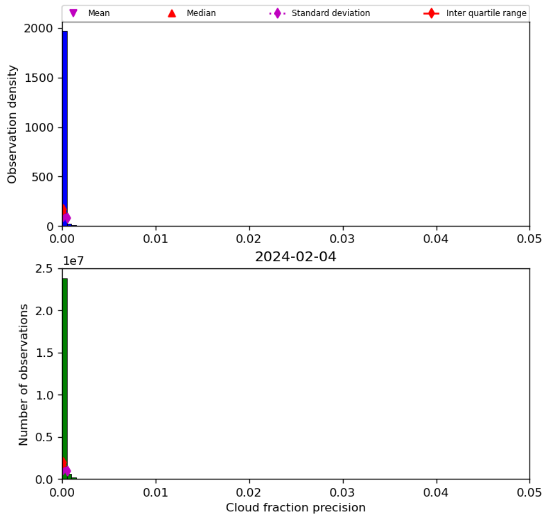
Figure 33: Histogram of “Cloud fraction precision” for 2024-02-03 to 2024-02-05
