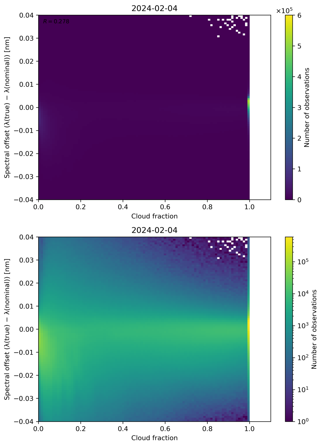
Figure 76: Scatter density plot of “Cloud fraction” against “Spectral offset ( \lambda(\text{true}) - \lambda(\text{nominal}) )” for 2024-02-03 to 2024-02-05.
