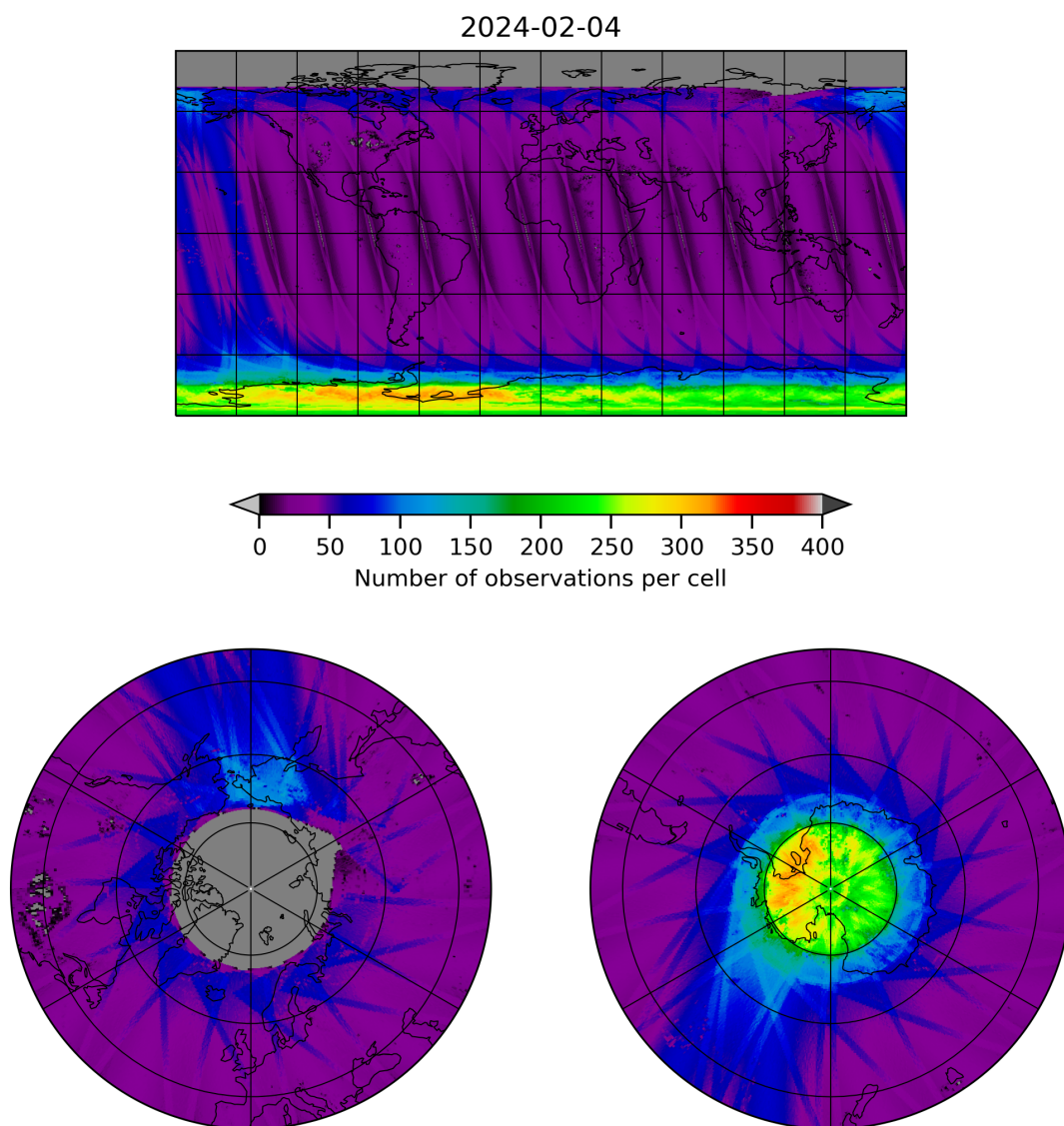
Figure 11: Map of the number of observations for 2024-02-03 to 2024-02-05
