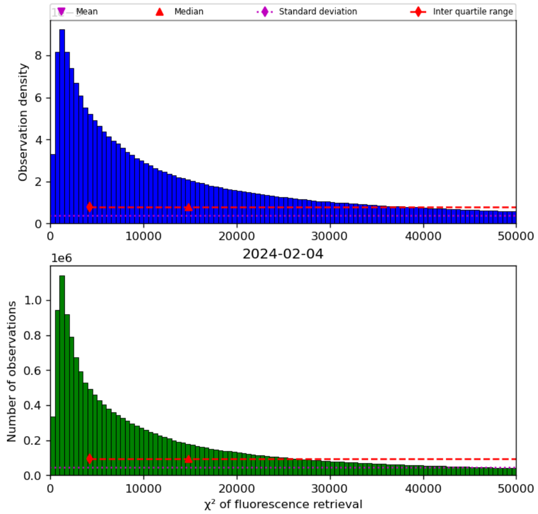
Figure 42: Histogram of “ \chi^2 of fluorescence retrieval” for 2024-02-03 to 2024-02-05
