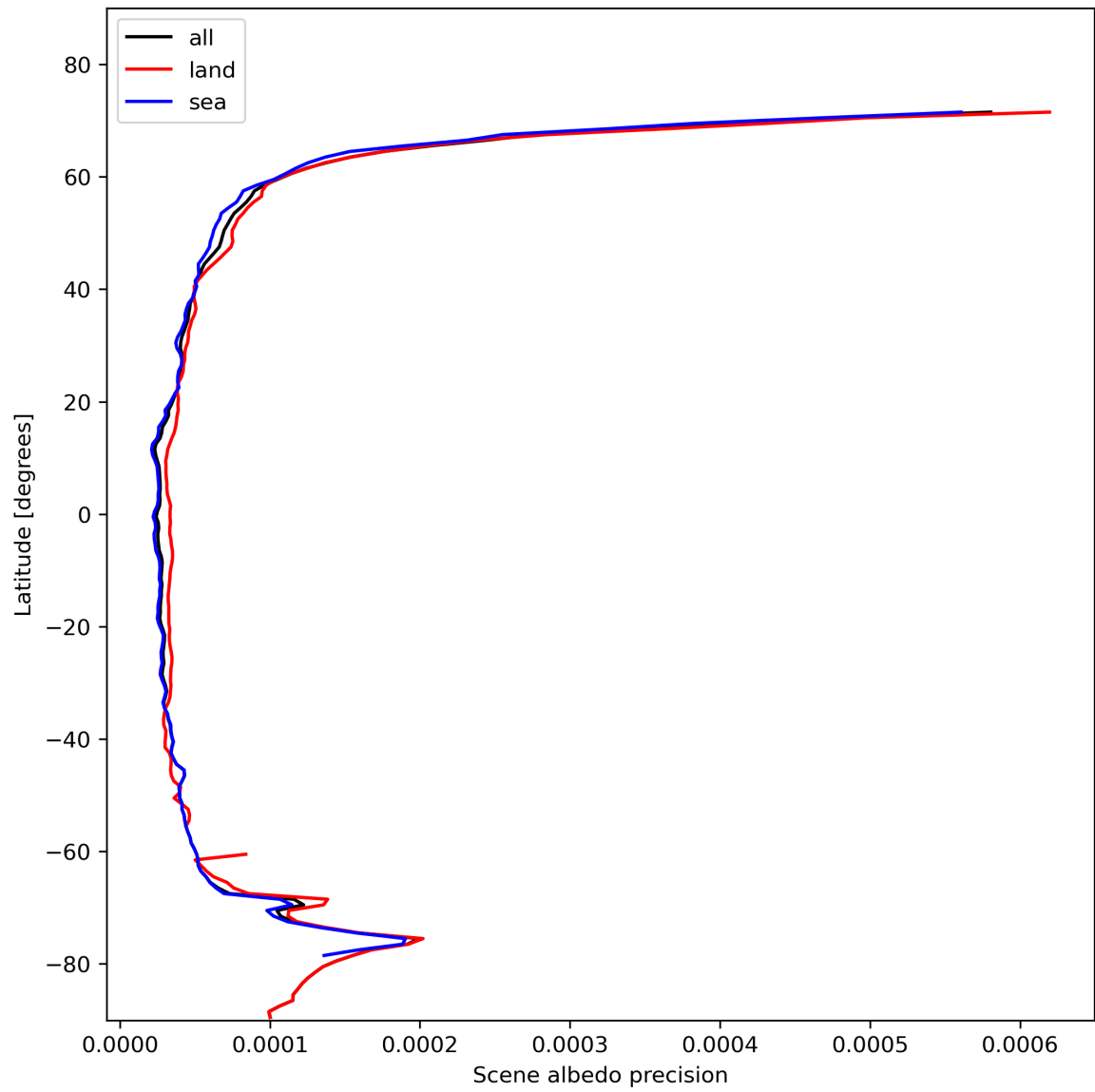
Figure 18: Zonal average of “Scene albedo precision” for 2024-02-03 to 2024-02-05.
