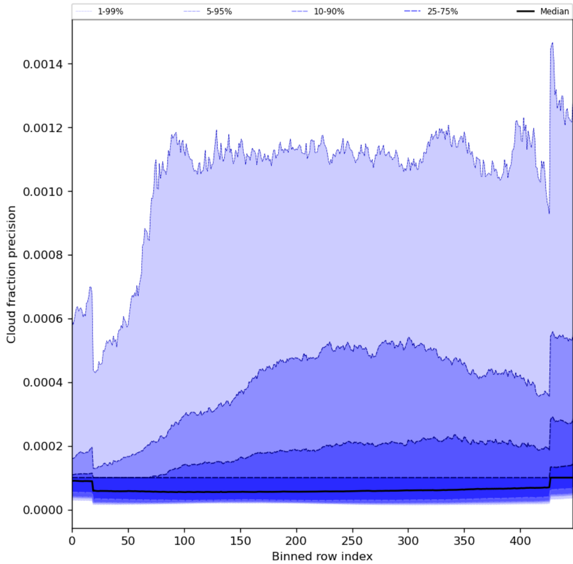
Figure 50: Along track statistics of “Cloud fraction precision” for 2024-02-03 to 2024-02-05
