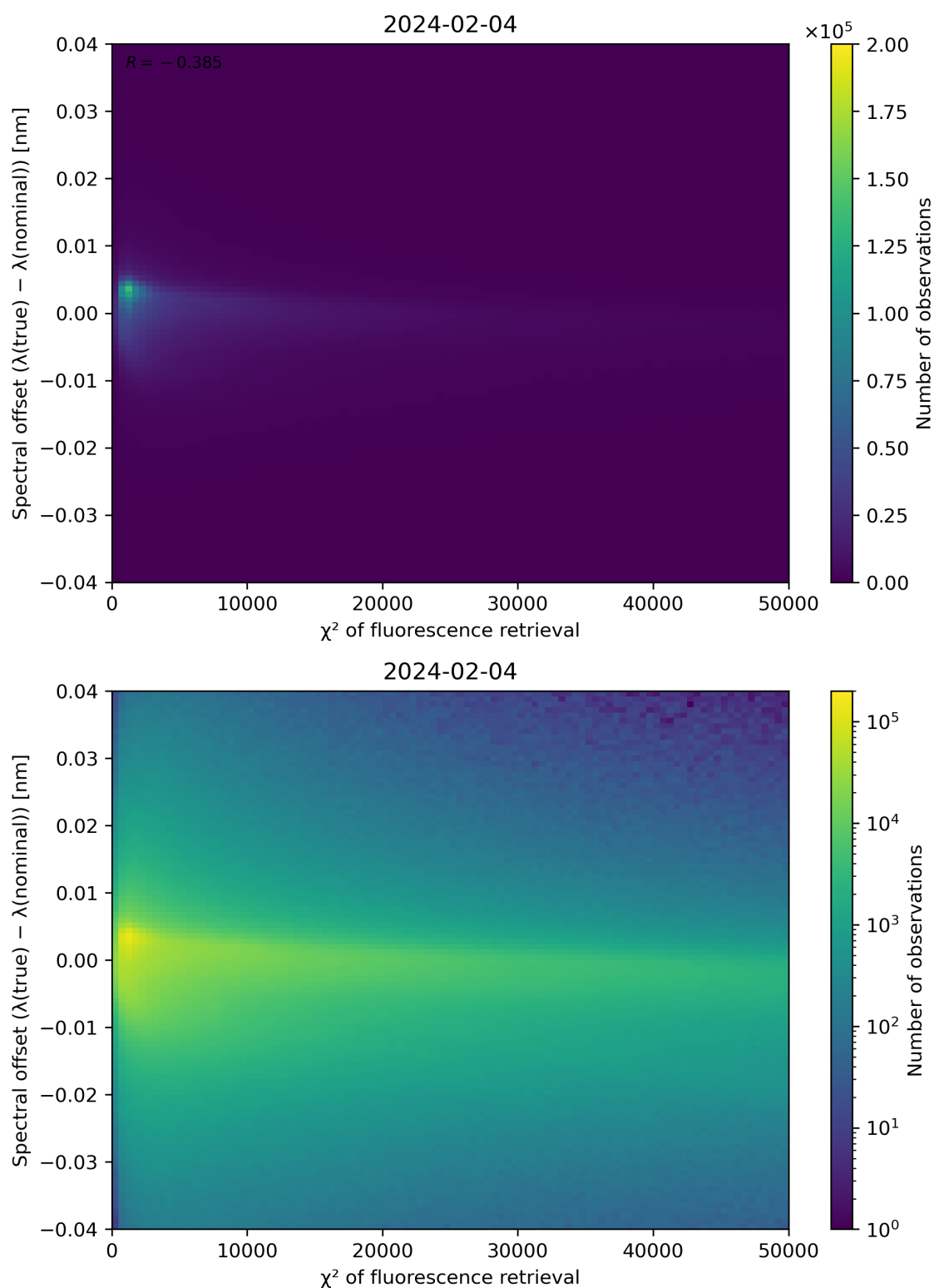
Figure 69: Scatter density plot of " \chi^2 of fluorescence retrieval" against "Spectral offset ( \lambda(\text{true}) - \lambda(\text{nominal}) )" for 2024-02-03 to 2024-02-05.
