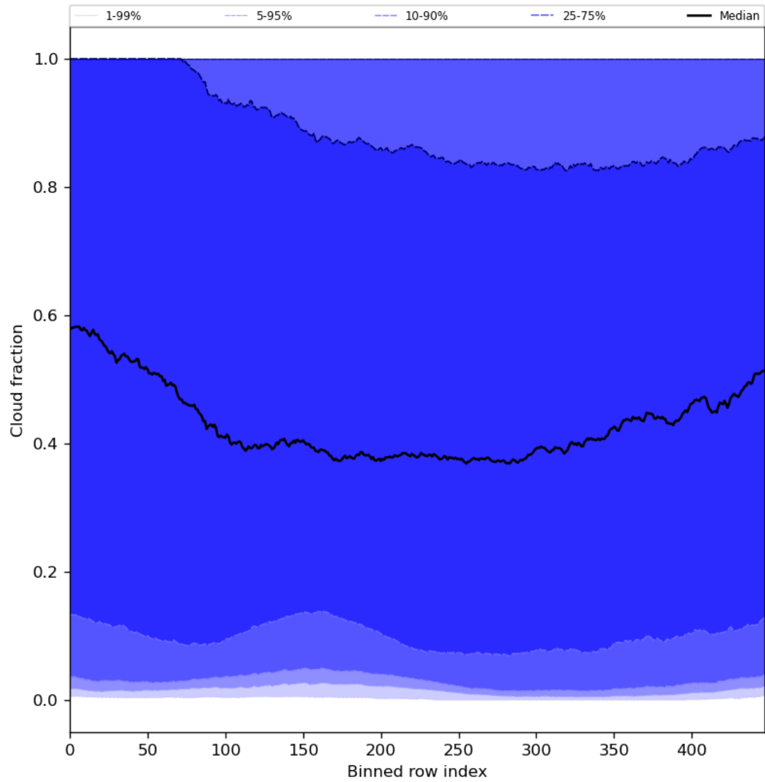
Figure 49: Along track statistics of “Cloud fraction” for 2024-02-03 to 2024-02-05
