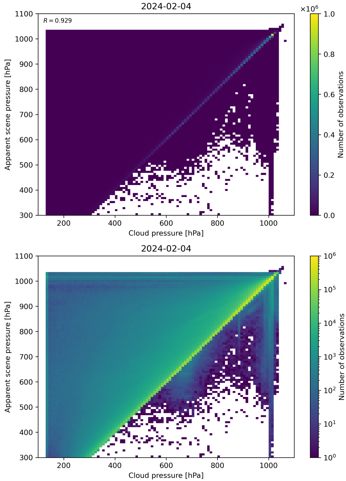
Figure 77: Scatter density plot of “Cloud pressure” against “Apparent scene pressure” for 2024-02-03 to 2024-02-05.
