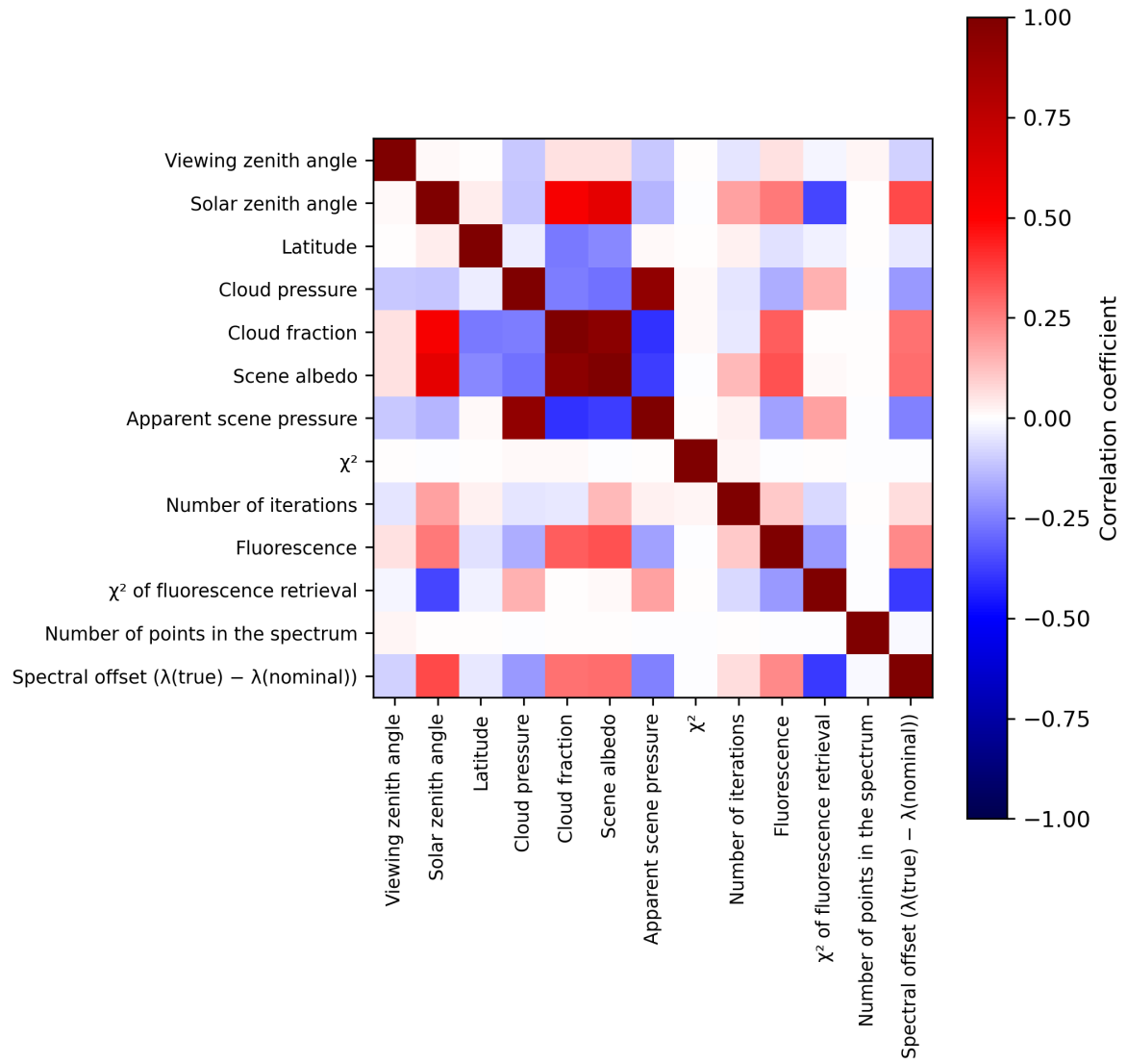
Figure 2: Map of correlation matrix for 2024-02-03 to 2024-02-05.
