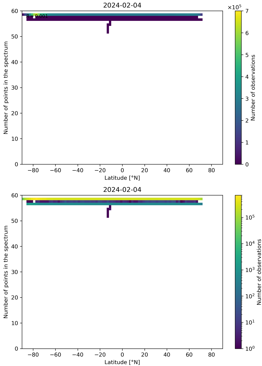
Figure 94: Scatter density plot of “Latitude” against “Number of points in the spectrum” for 2024-02-03 to 2024-02-05.
