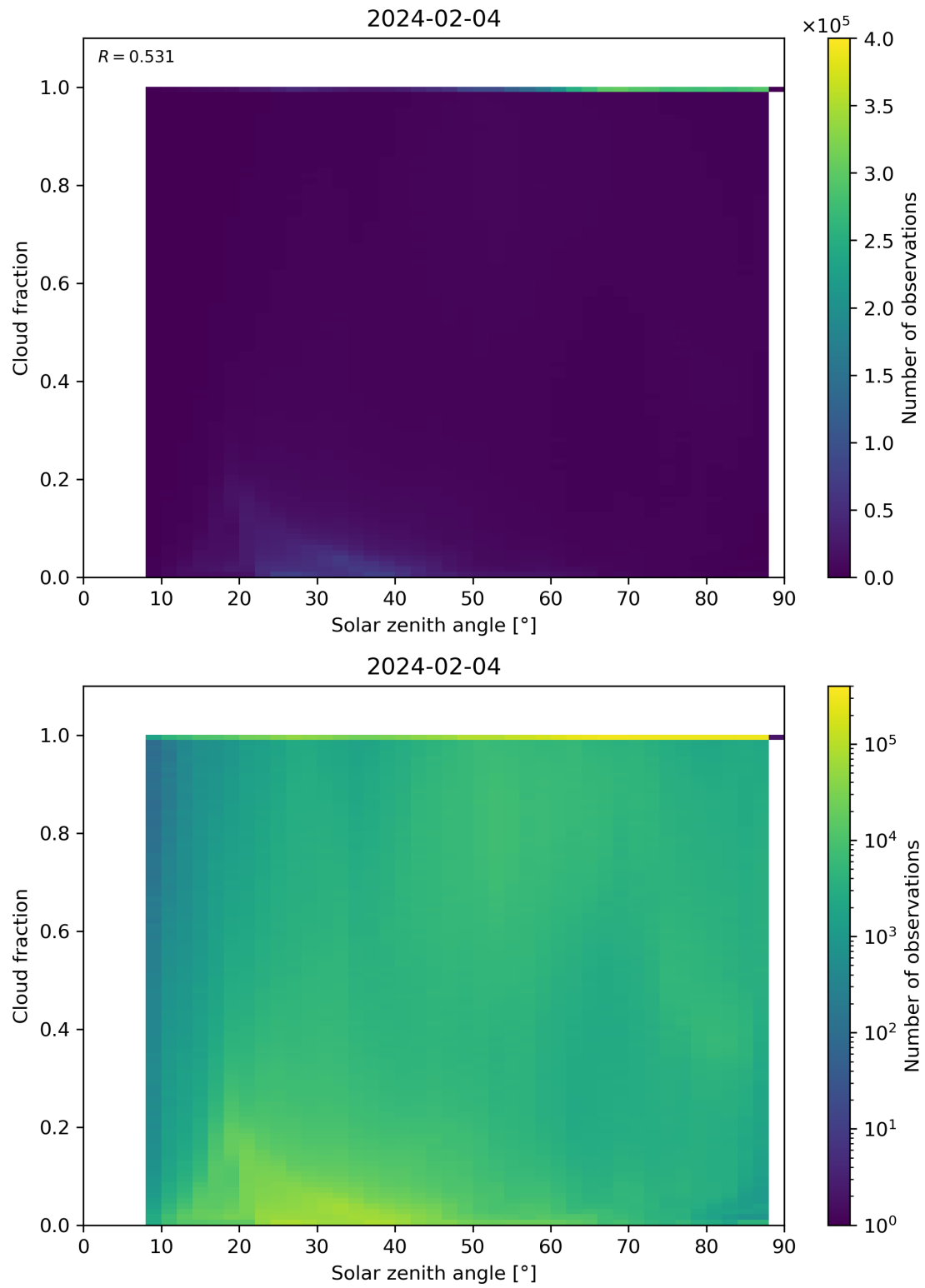
Figure 110: Scatter density plot of “Solar zenith angle” against “Cloud fraction” for 2024-02-03 to 2024-02-05.
