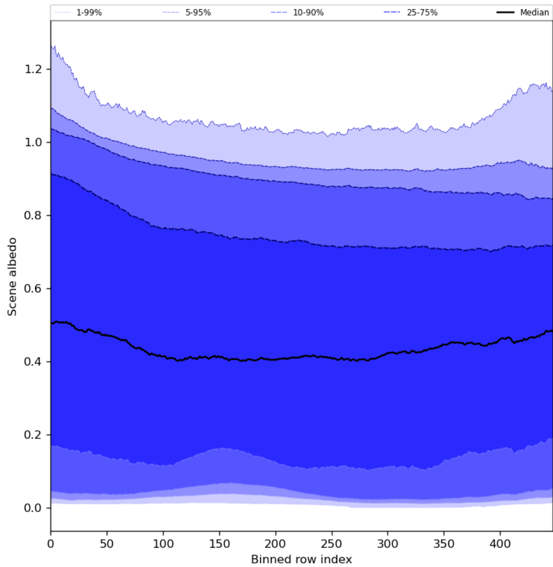
Figure 51: Along track statistics of “Scene albedo” for 2024-02-03 to 2024-02-05
