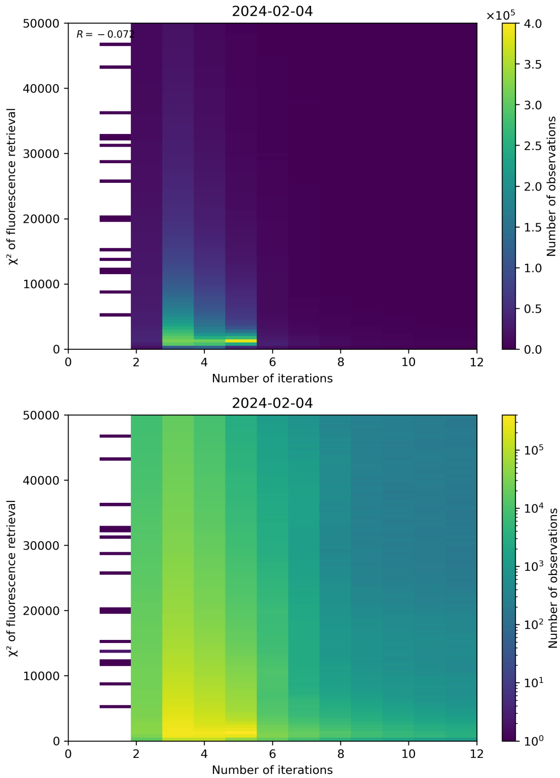
Figure 97: Scatter density plot of “Number of iterations” against “ \chi^2 of fluorescence retrieval” for 2024-02-03 to 2024-02-05.
