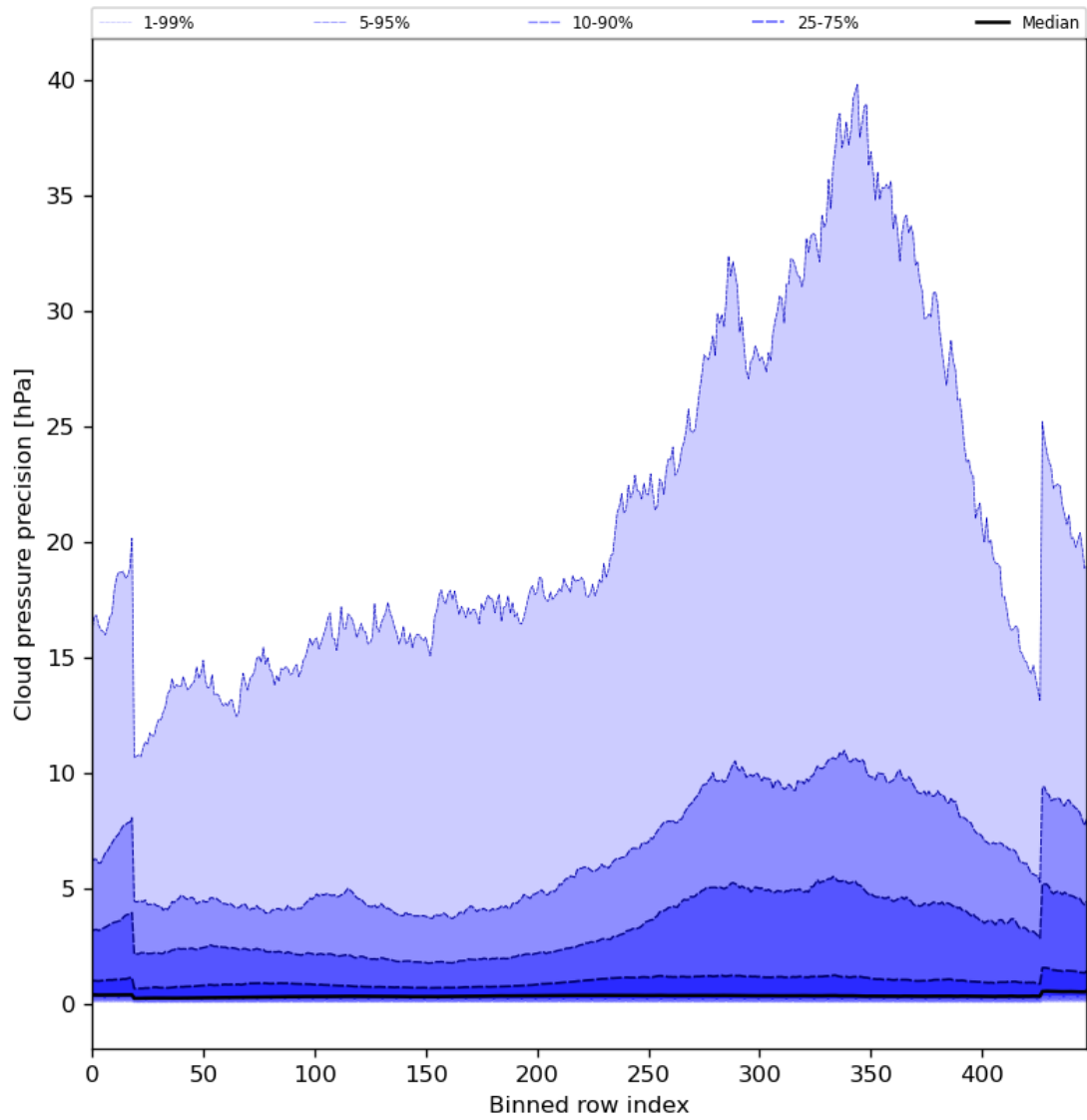
Figure 48: Along track statistics of “Cloud pressure precision” for 2024-02-03 to 2024-02-05
