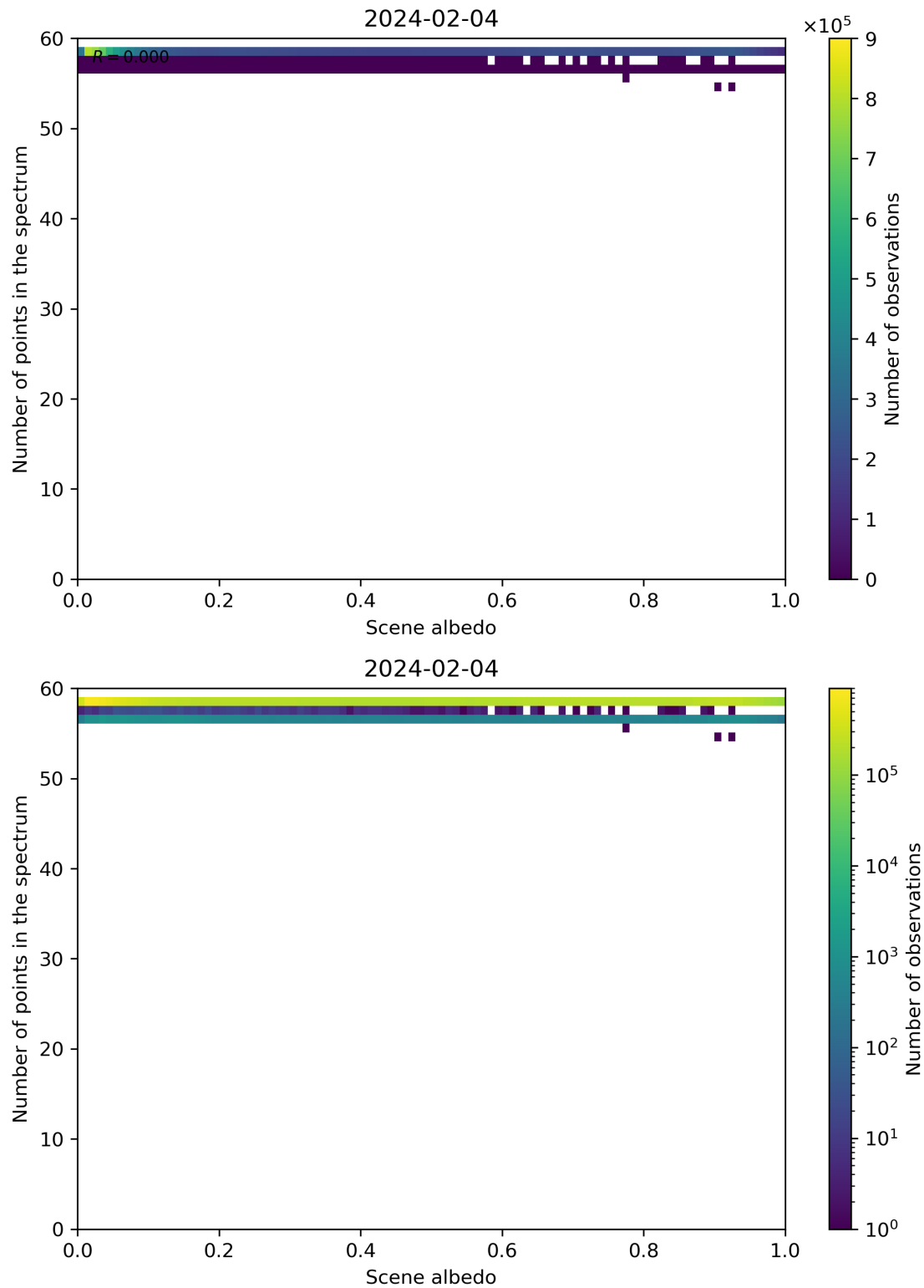
Figure 106: Scatter density plot of “Scene albedo” against “Number of points in the spectrum” for 2024-02-03 to 2024-02-05.
