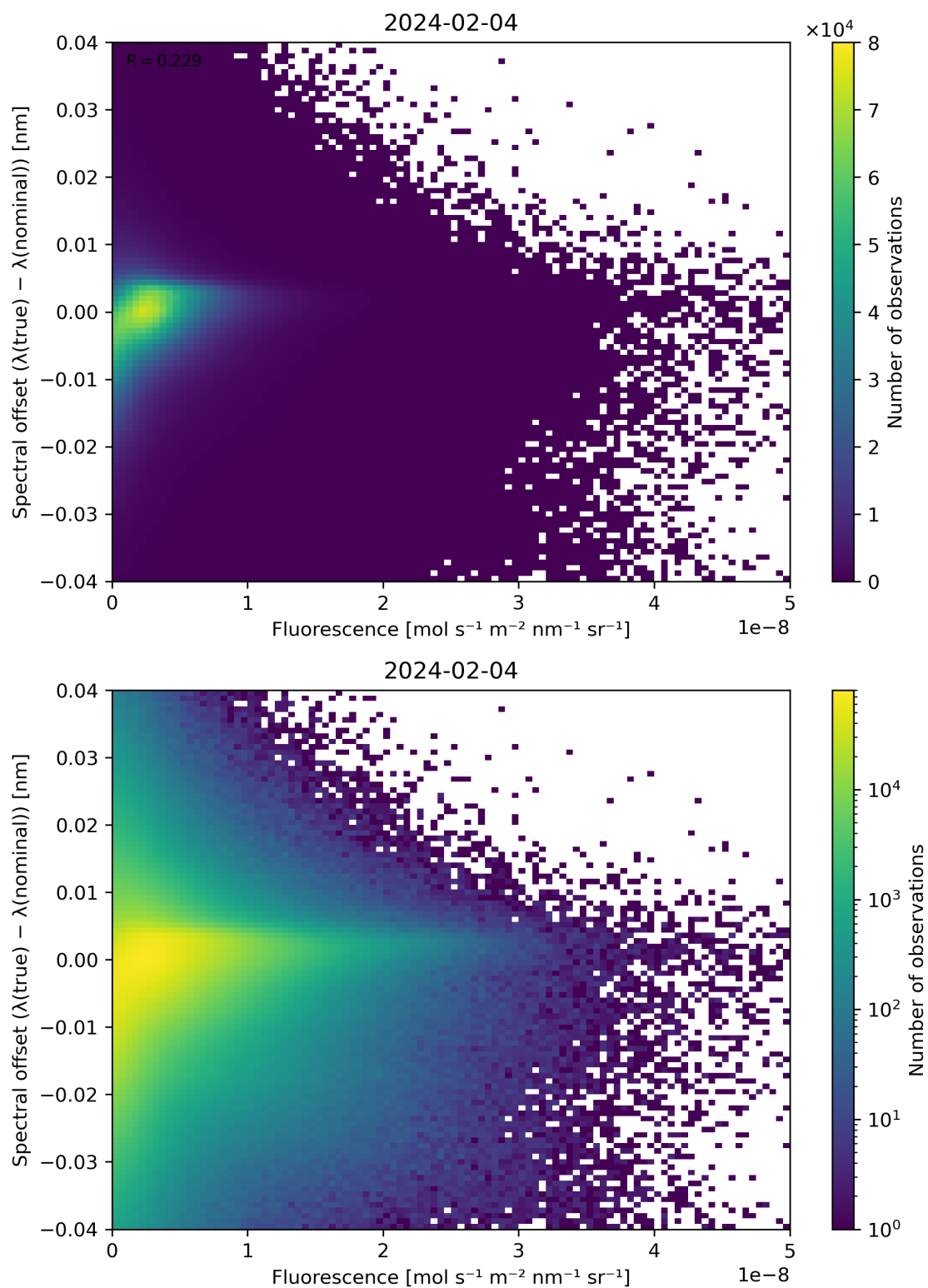
Figure 87: Scatter density plot of “Fluorescence” against “Spectral offset ( \lambda(\text{true}) - \lambda(\text{nominal}) )” for 2024-02-03 to 2024-02-05.
