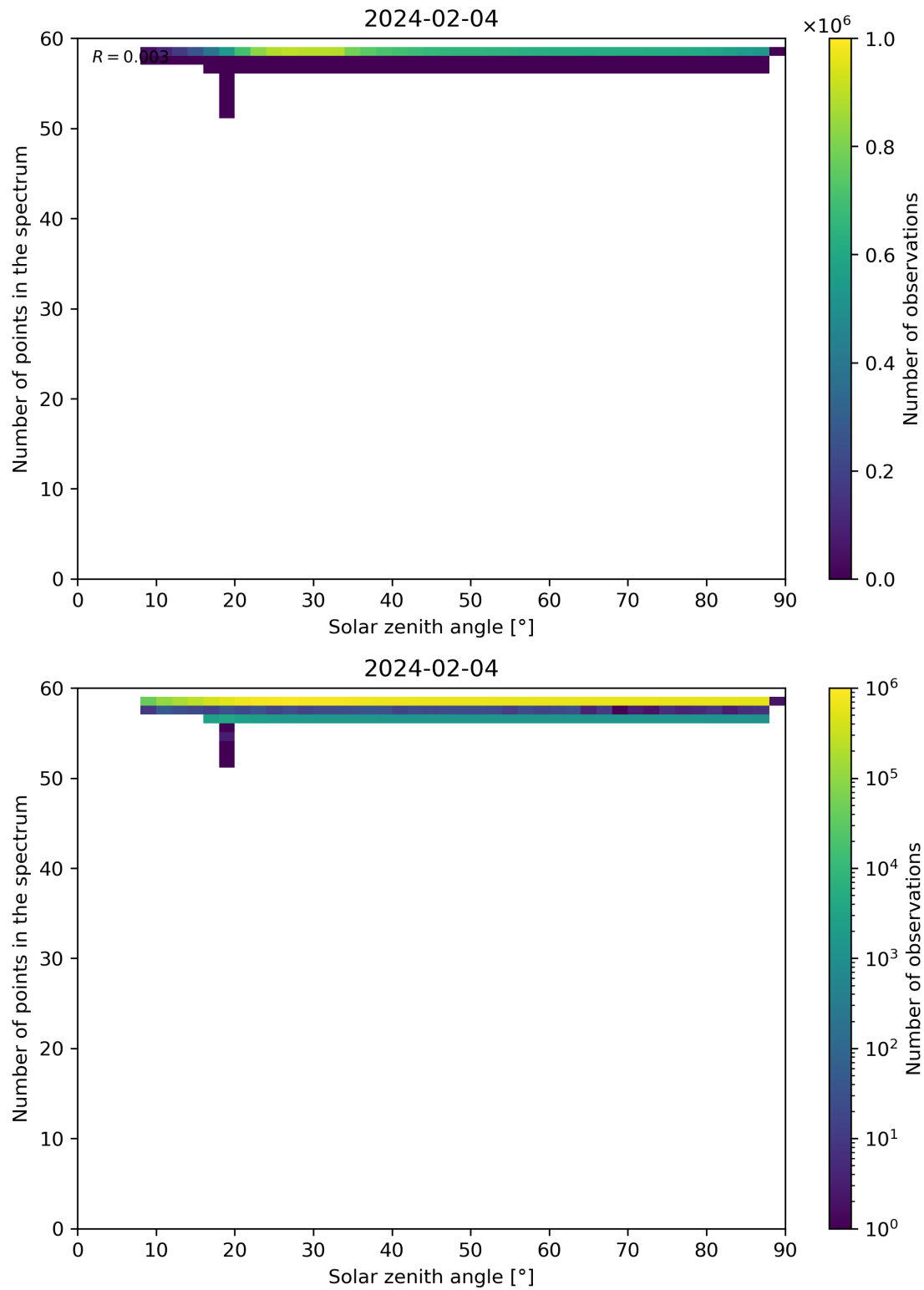
Figure 115: Scatter density plot of “Solar zenith angle” against “Number of points in the spectrum” for 2024-02-03 to 2024-02-05.
