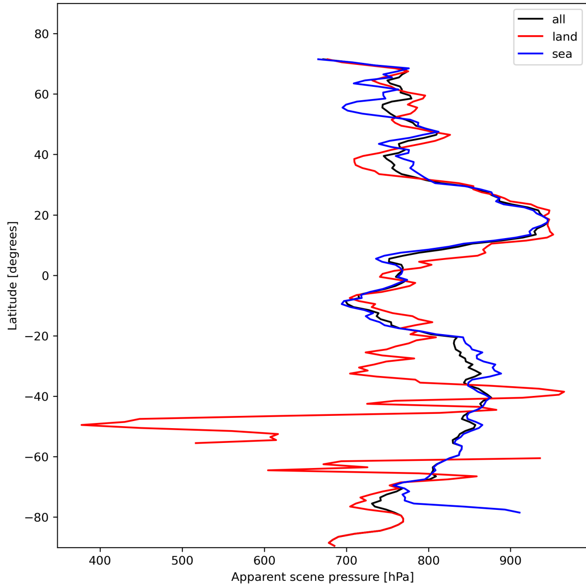
Figure 19: Zonal average of “Apparent scene pressure” for 2024-02-03 to 2024-02-05.
