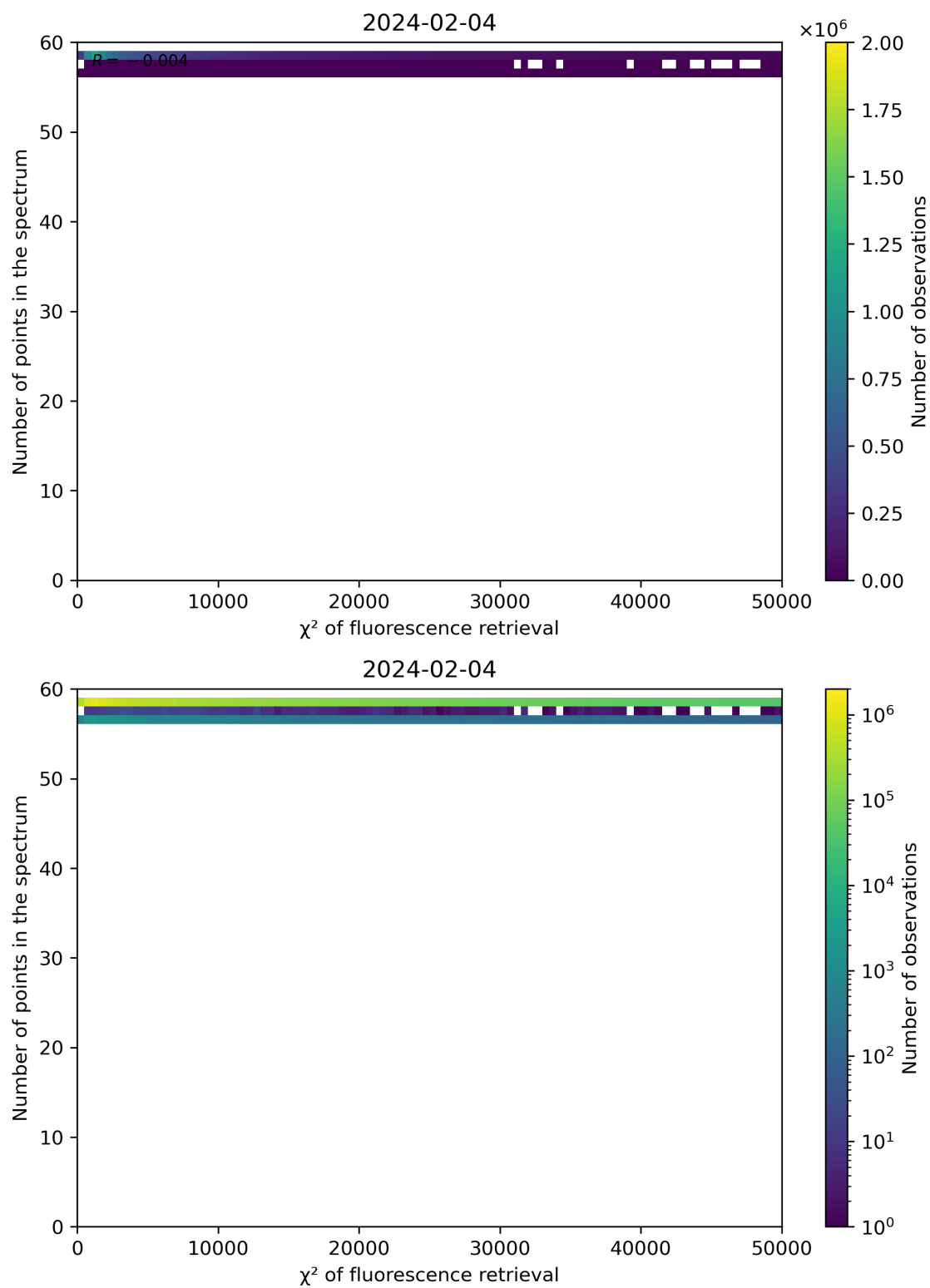
Figure 68: Scatter density plot of " \chi^2 of fluorescence retrieval" against "Number of points in the spectrum" for 2024-02-03 to 2024-02-05.
