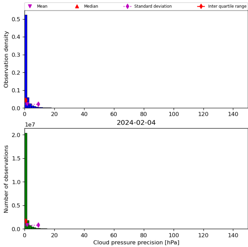
Figure 31: Histogram of “Cloud pressure precision” for 2024-02-03 to 2024-02-05
