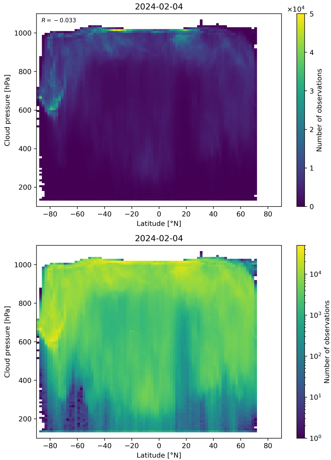
Figure 91: Scatter density plot of “Latitude” against “Cloud pressure” for 2024-02-03 to 2024-02-05.
