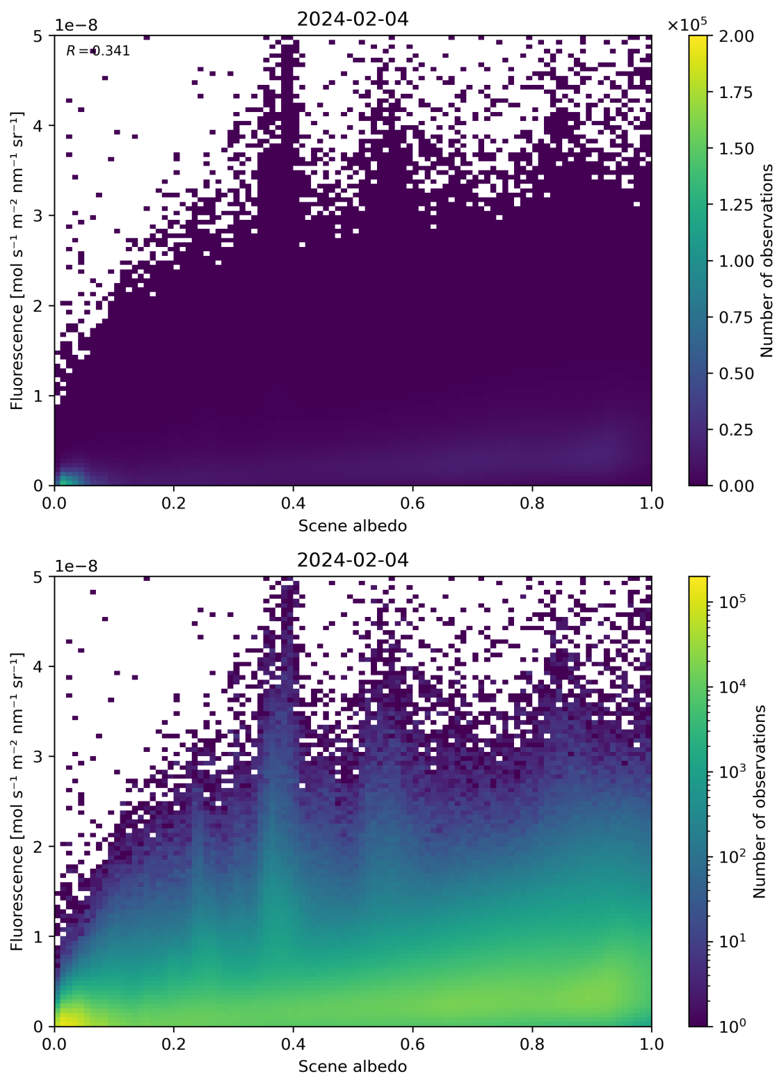
Figure 104: Scatter density plot of “Scene albedo” against “Fluorescence” for 2024-02-03 to 2024-02-05.
