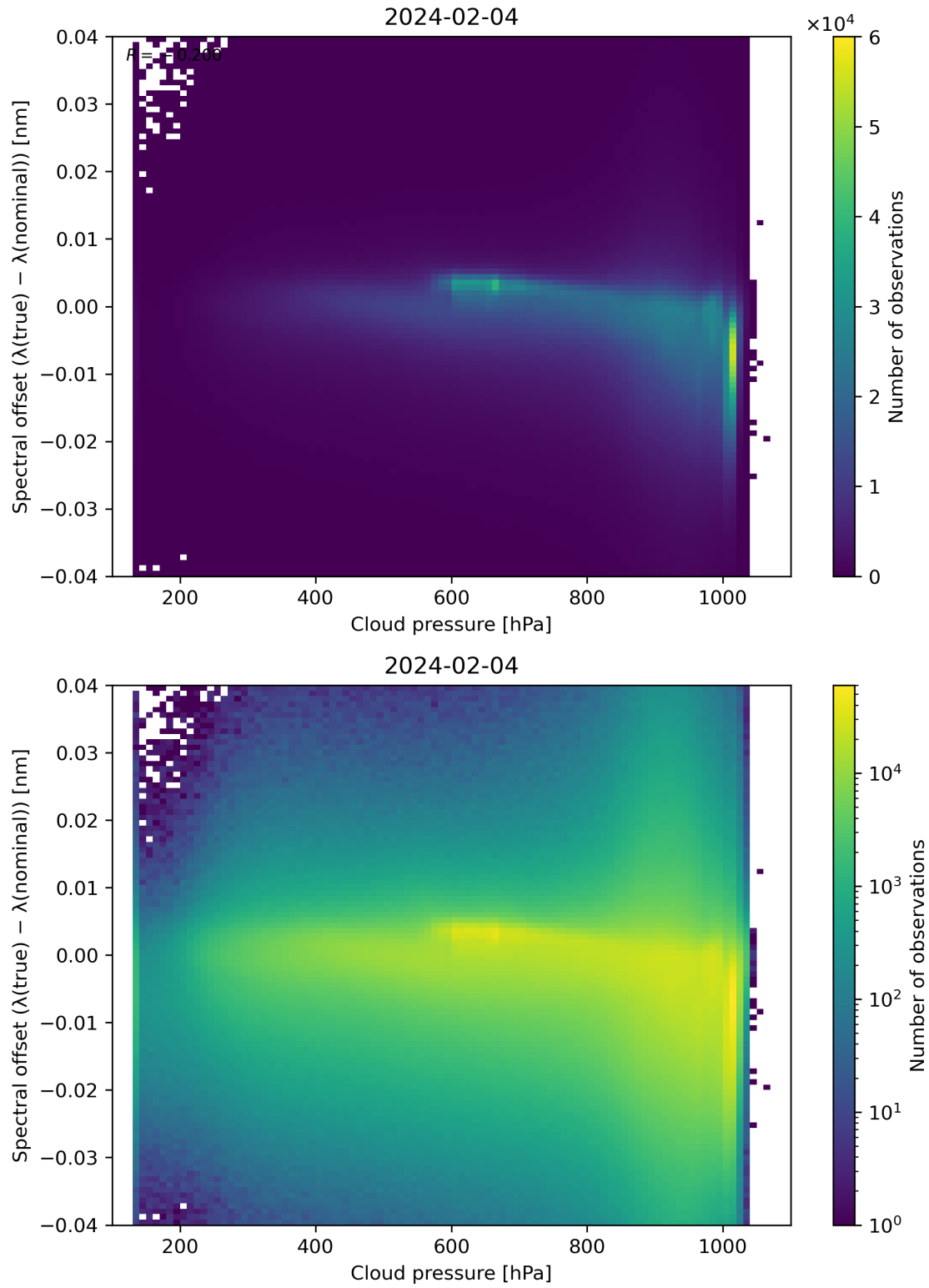
Figure 84: Scatter density plot of “Cloud pressure” against “Spectral offset ( \lambda(\text{true}) - \lambda(\text{nominal}) )” for 2024-02-03 to 2024-02-05.
