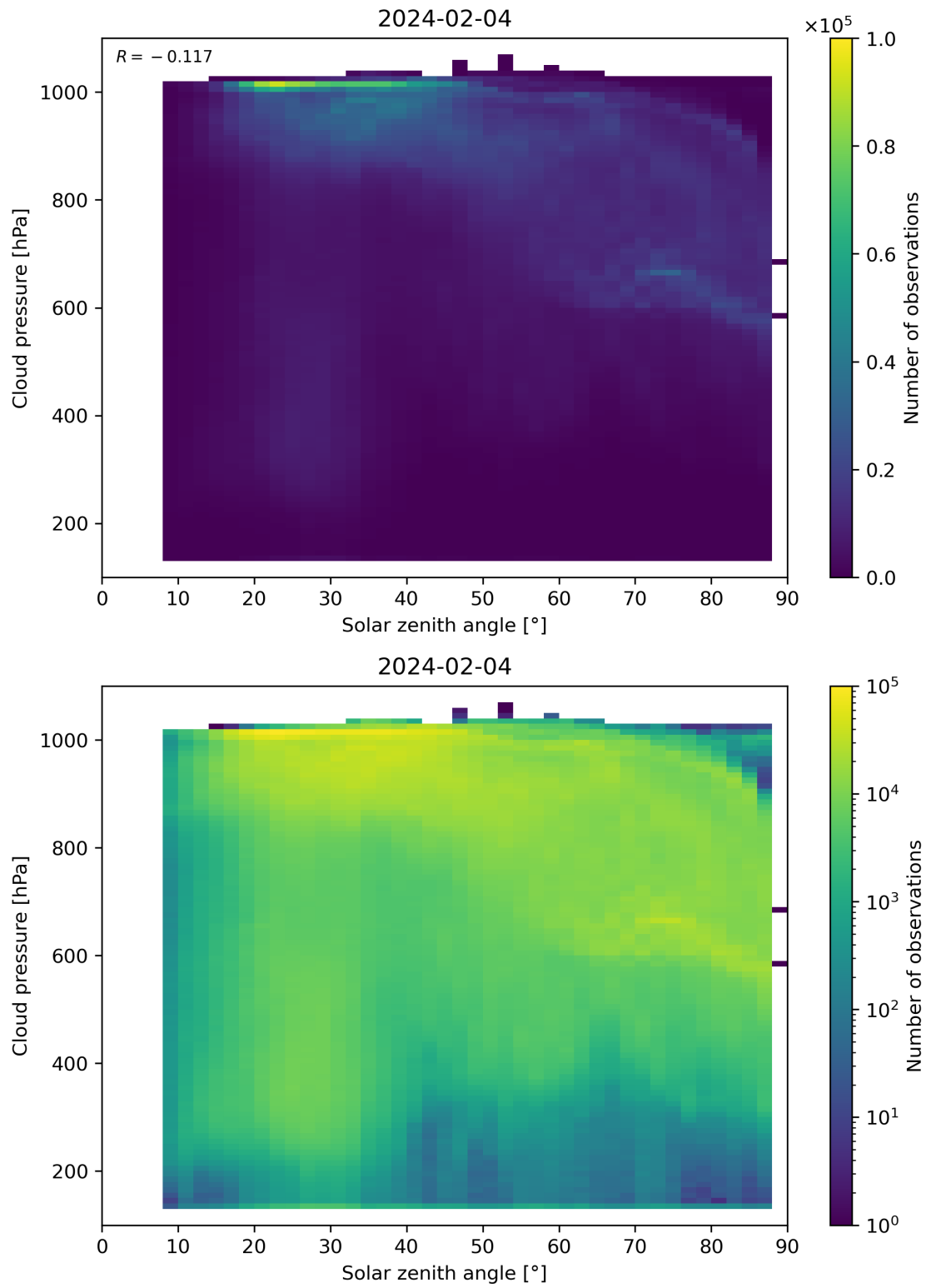
Figure 111: Scatter density plot of “Solar zenith angle” against “Cloud pressure” for 2024-02-03 to 2024-02-05.
