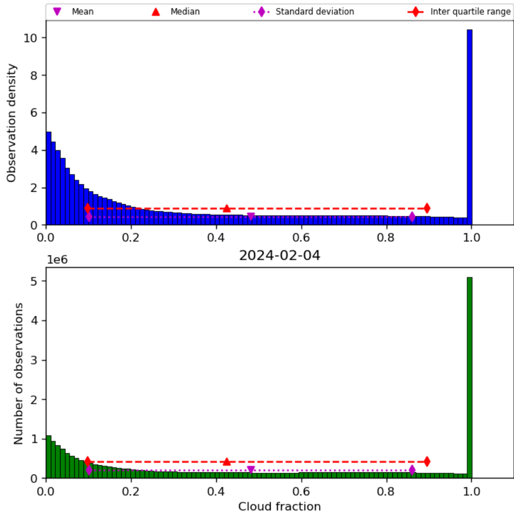
Figure 32: Histogram of “Cloud fraction” for 2024-02-03 to 2024-02-05
