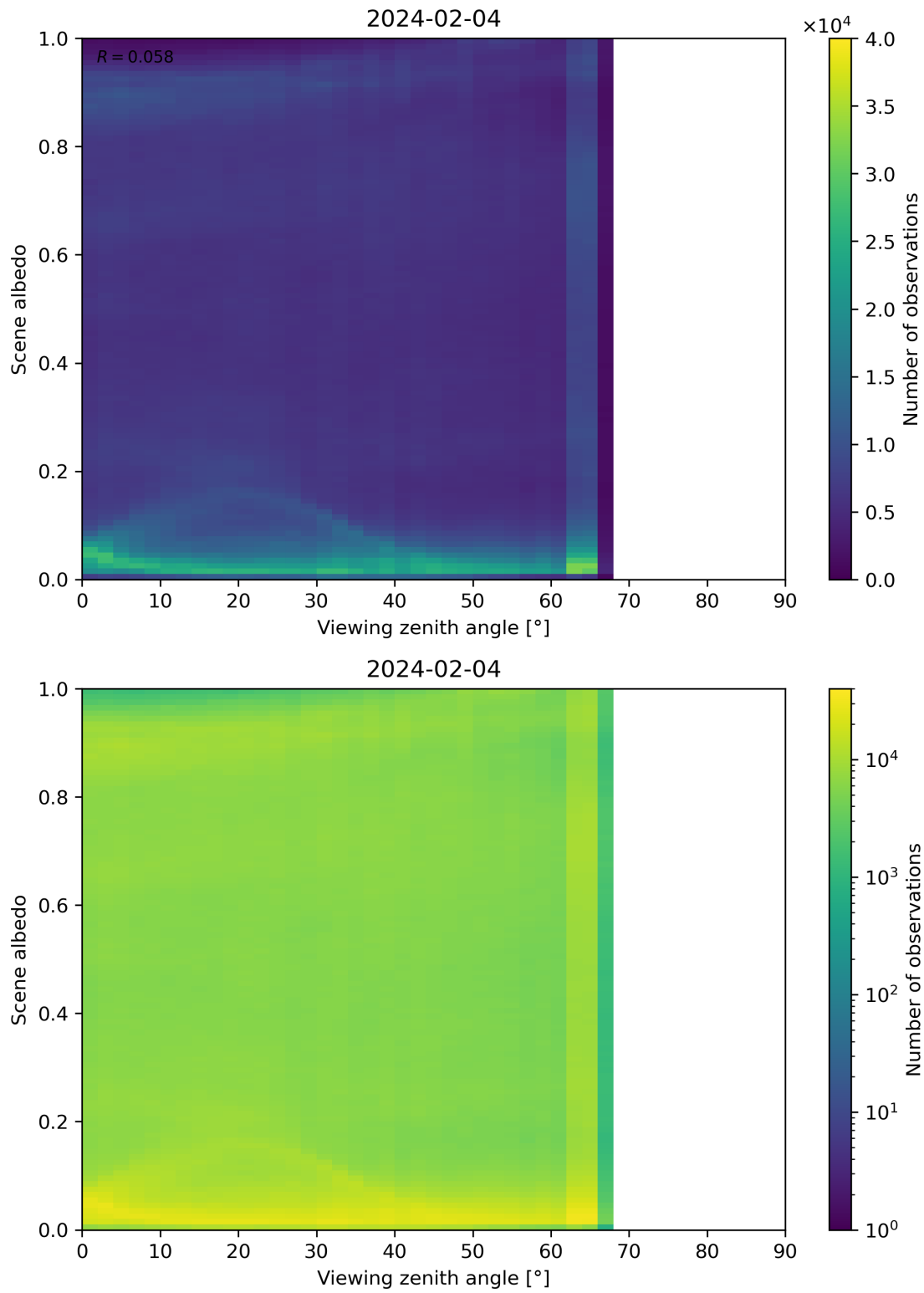
Figure 126: Scatter density plot of “Viewing zenith angle” against “Scene albedo” for 2024-02-03 to 2024-02-05.
