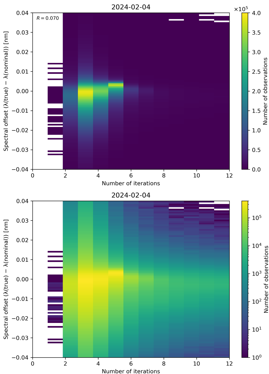
Figure 100: Scatter density plot of “Number of iterations” against “Spectral offset ( \lambda(\text{true}) - \lambda(\text{nominal}) )” for 2024-02-03 to 2024-02-05.
