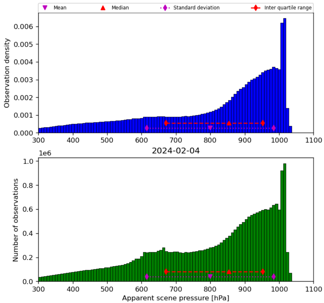
Figure 36: Histogram of “Apparent scene pressure” for 2024-02-03 to 2024-02-05
