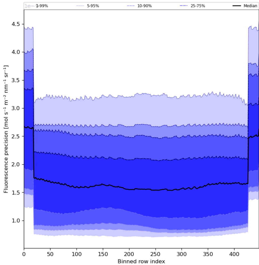
Figure 58: Along track statistics of “Fluorescence precision” for 2024-02-03 to 2024-02-05
