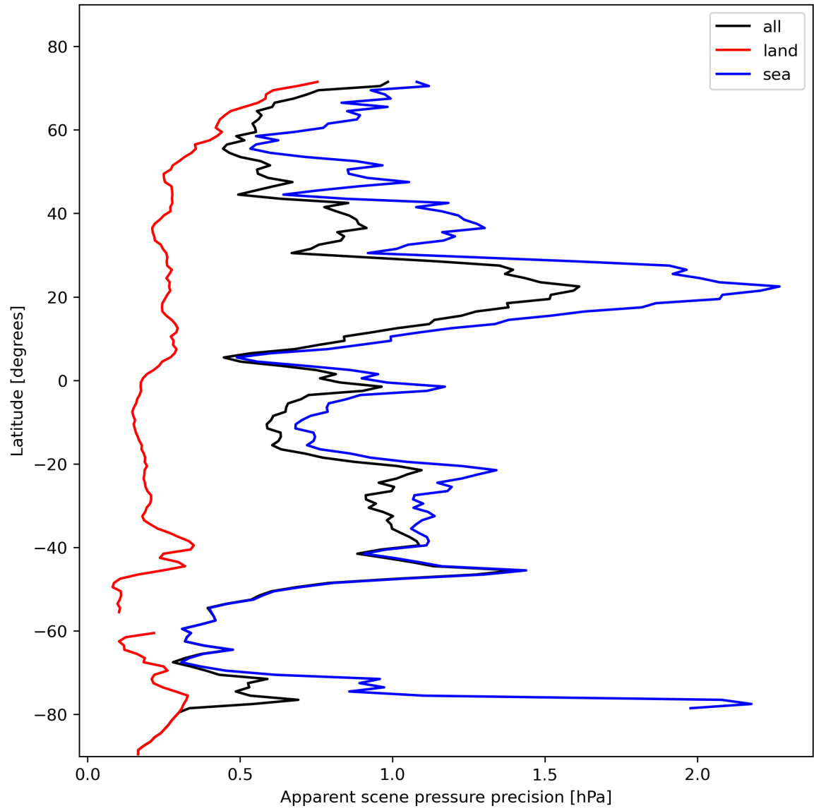
Figure 20: Zonal average of “Apparent scene pressure precision” for 2024-02-03 to 2024-02-05.
