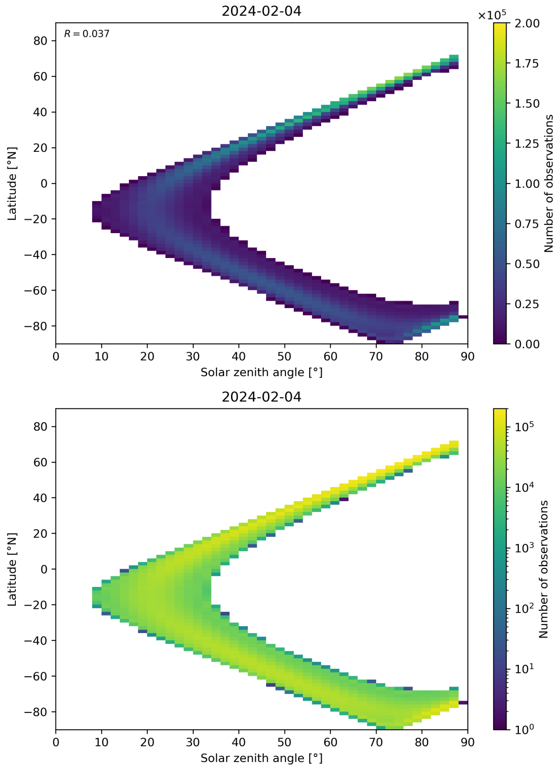
Figure 113: Scatter density plot of “Solar zenith angle” against “Latitude” for 2024-02-03 to 2024-02-05.
