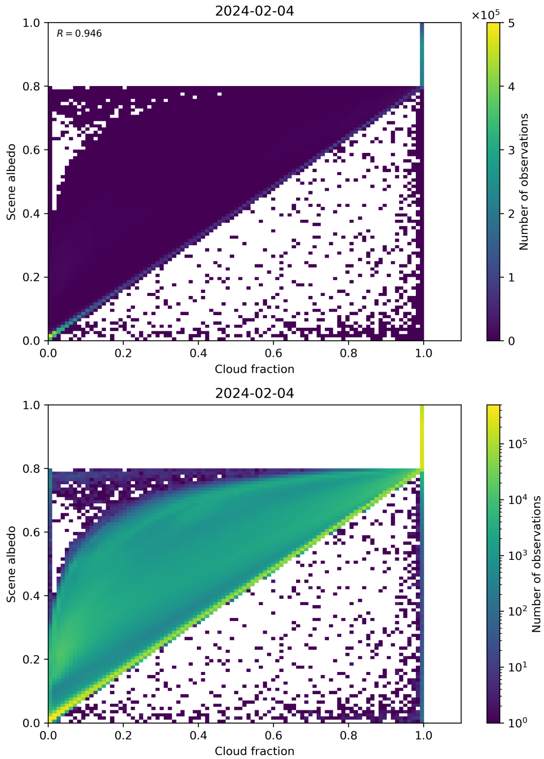
Figure 75: Scatter density plot of “Cloud fraction” against “Scene albedo” for 2024-02-03 to 2024-02-05.
