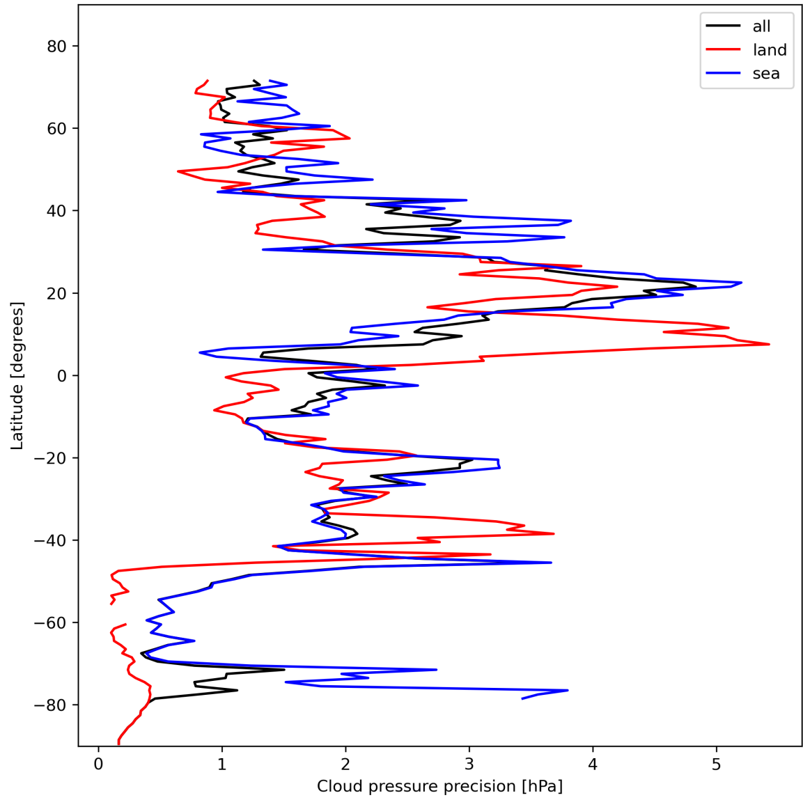
Figure 14: Zonal average of “Cloud pressure precision” for 2024-02-03 to 2024-02-05.
