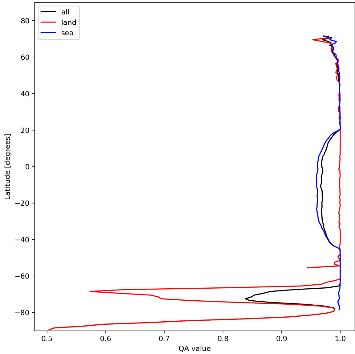
Figure 12: Zonal average of “QA value” for 2024-02-03 to 2024-02-05.
