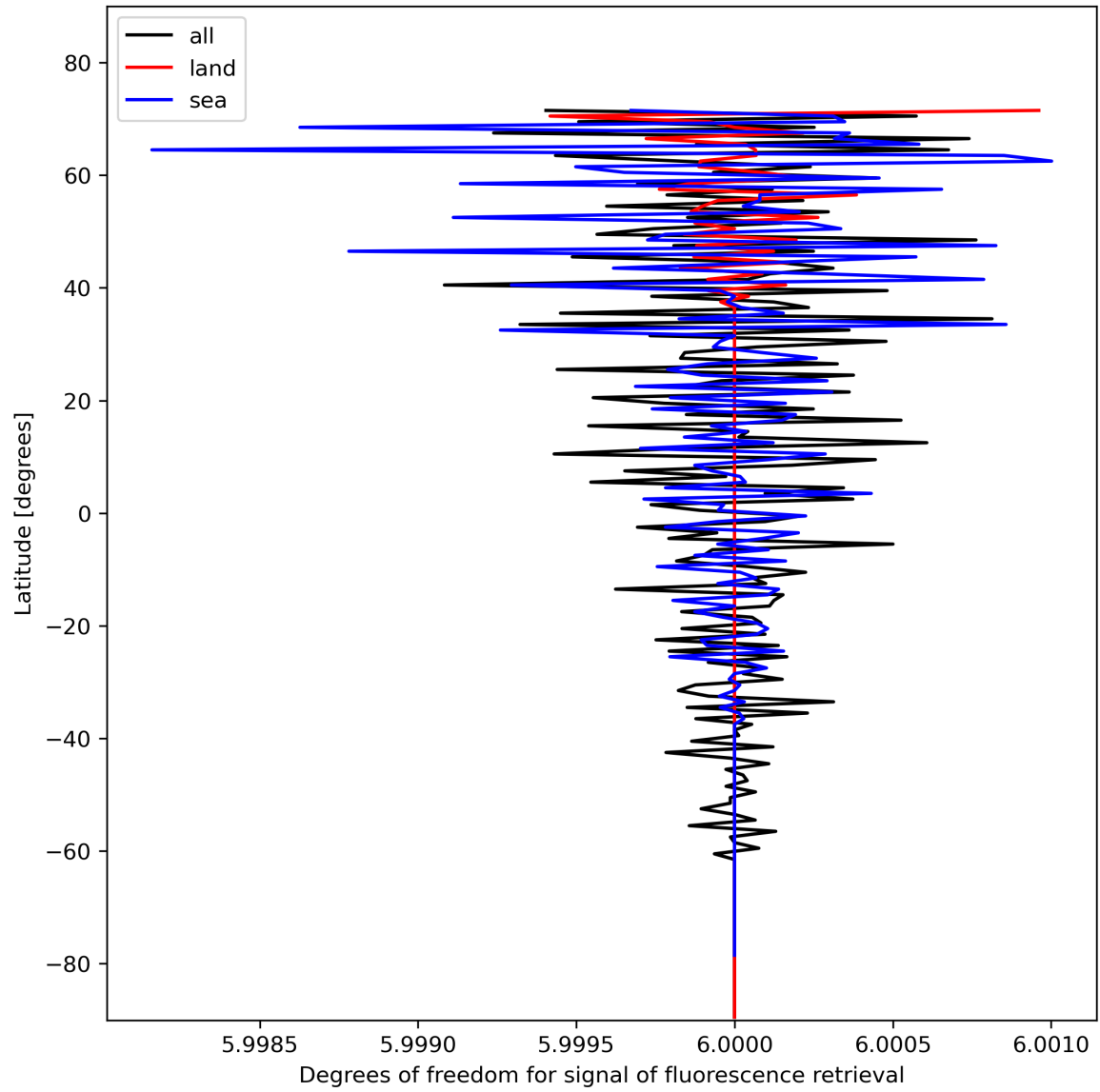
Figure 26: Zonal average of “Degrees of freedom for signal of fluorescence retrieval” for 2024-02-03 to 2024-02-05.
