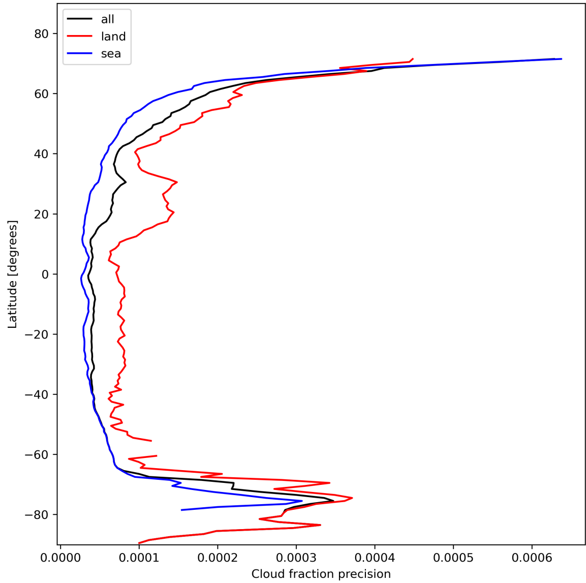
Figure 16: Zonal average of “Cloud fraction precision” for 2024-02-03 to 2024-02-05.
