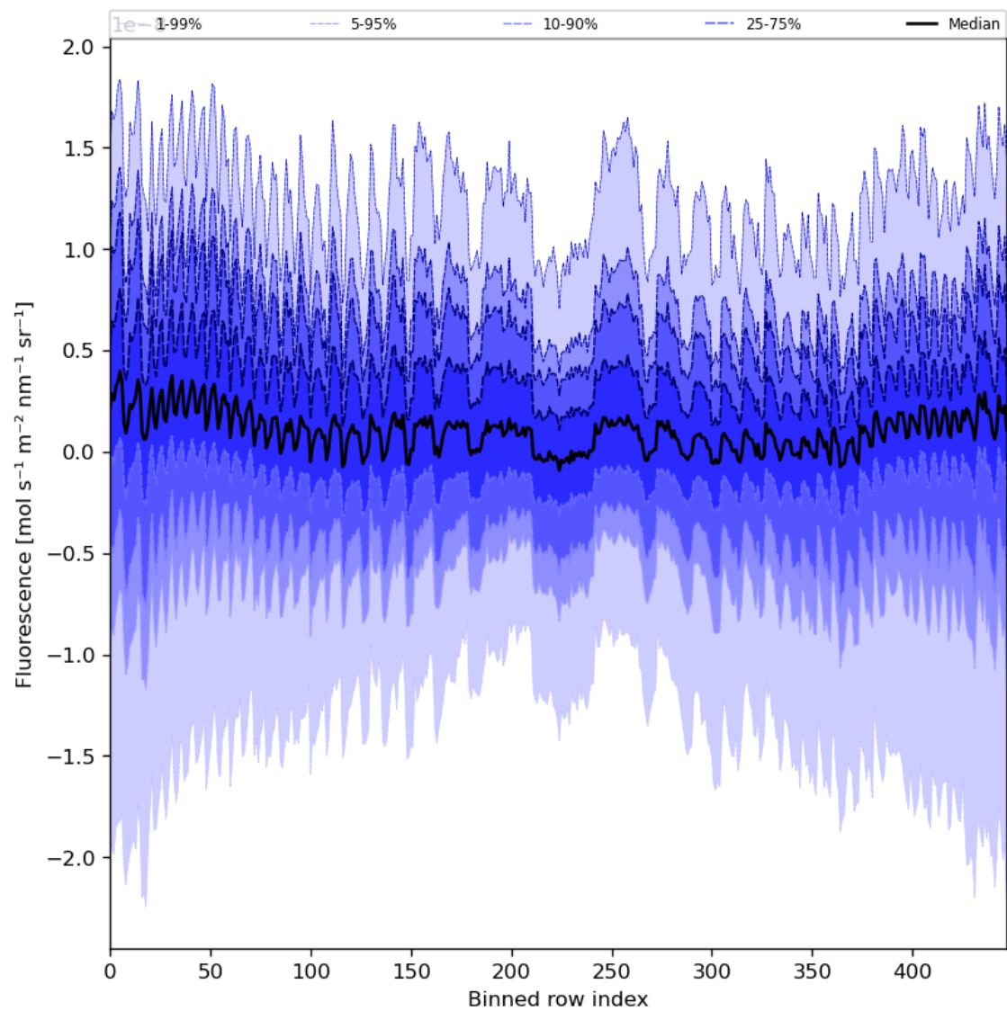
Figure 57: Along track statistics of “Fluorescence” for 2024-02-03 to 2024-02-05
