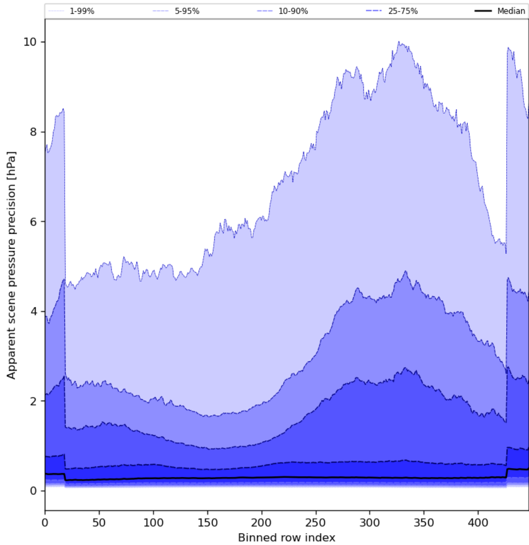
Figure 54: Along track statistics of “Apparent scene pressure precision” for 2024-02-03 to 2024-02-05
