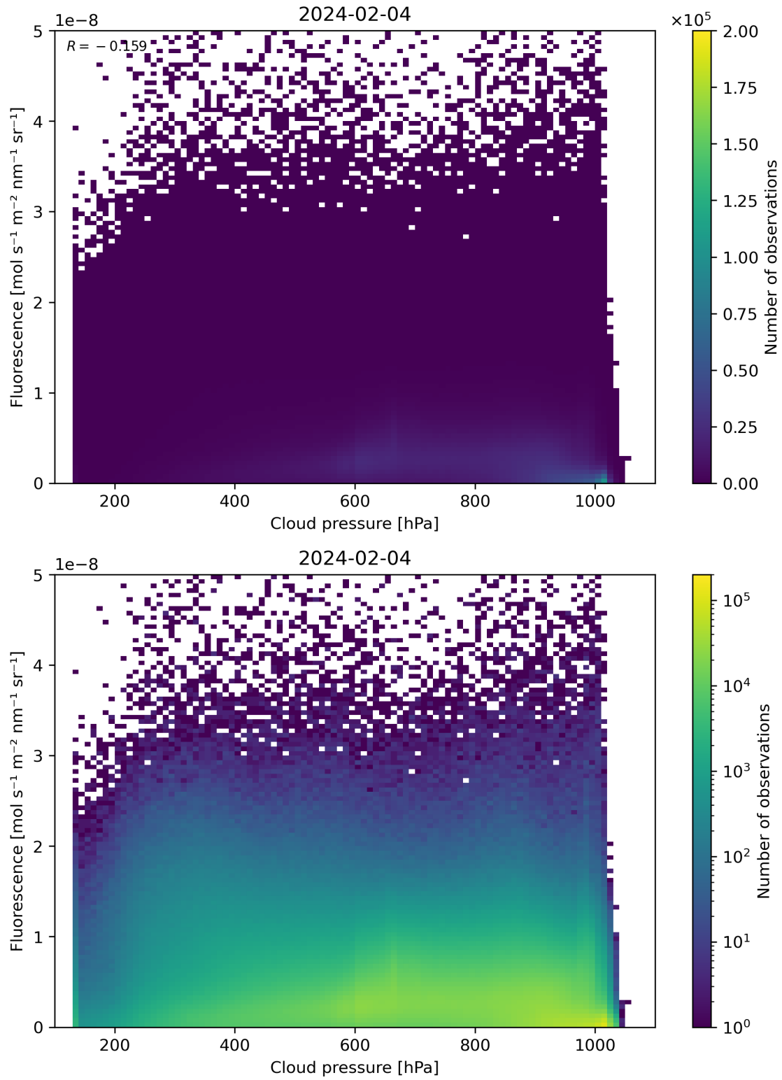
Figure 80: Scatter density plot of “Cloud pressure” against “Fluorescence” for 2024-02-03 to 2024-02-05.
