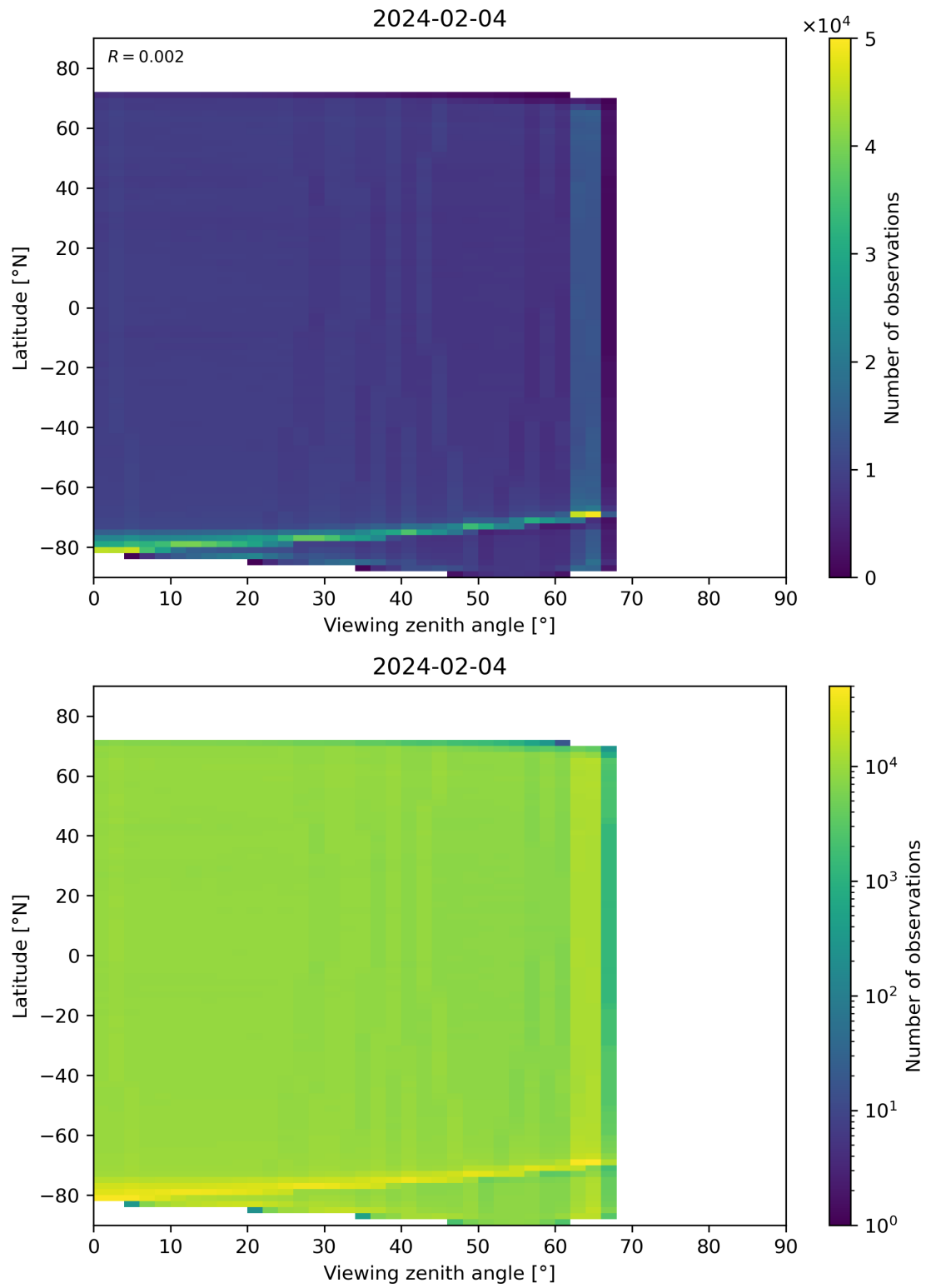
Figure 123: Scatter density plot of “Viewing zenith angle” against “Latitude” for 2024-02-03 to 2024-02-05.
