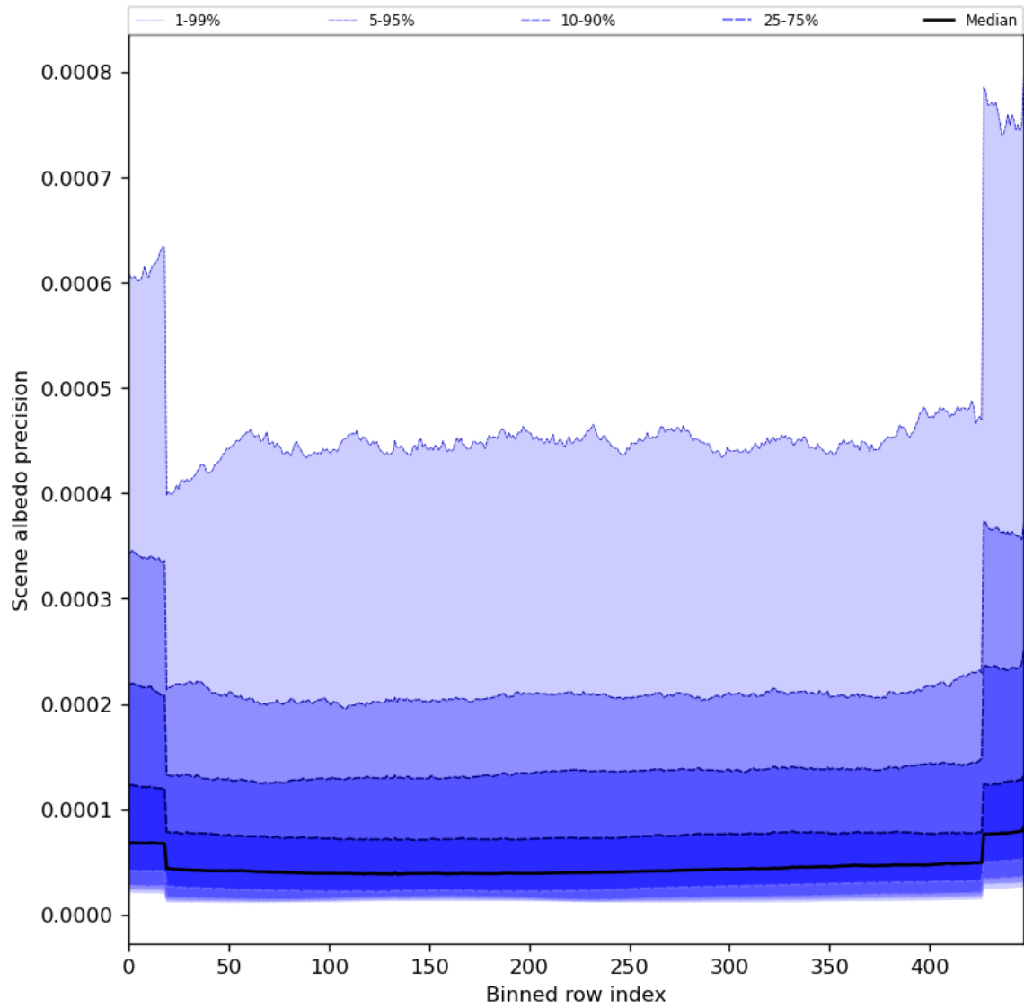
Figure 52: Along track statistics of “Scene albedo precision” for 2024-02-03 to 2024-02-05
