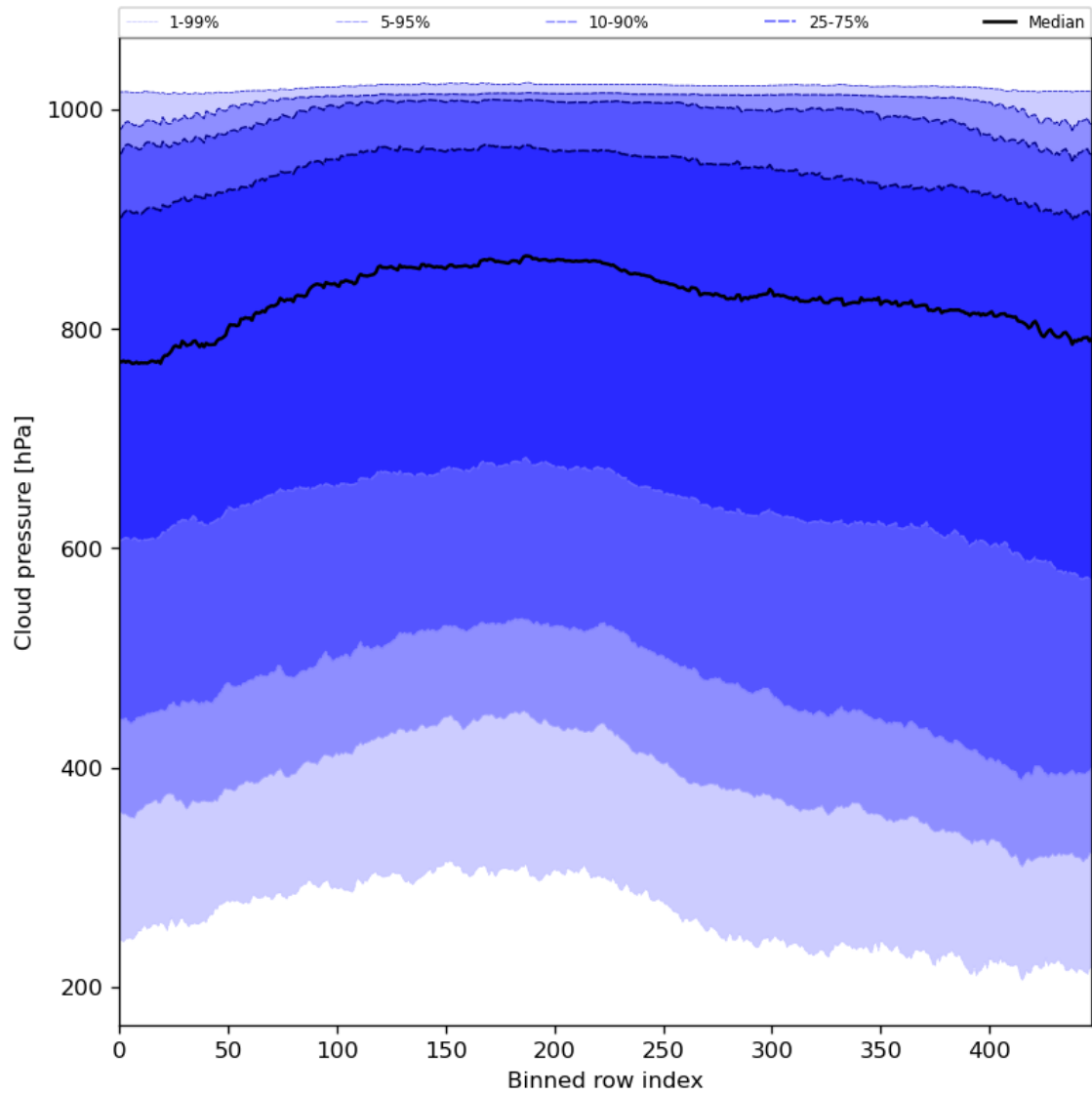
Figure 47: Along track statistics of “Cloud pressure” for 2024-02-03 to 2024-02-05
