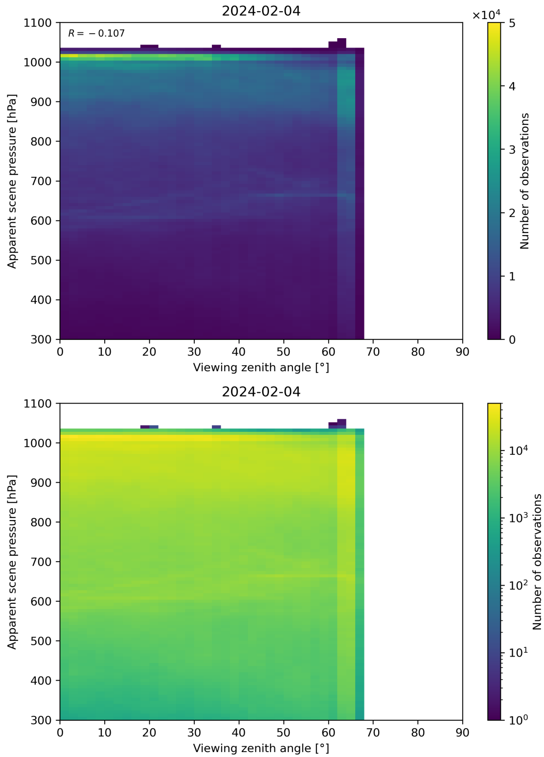
Figure 118: Scatter density plot of “Viewing zenith angle” against “Apparent scene pressure” for 2024-02-03 to 2024-02-05.
