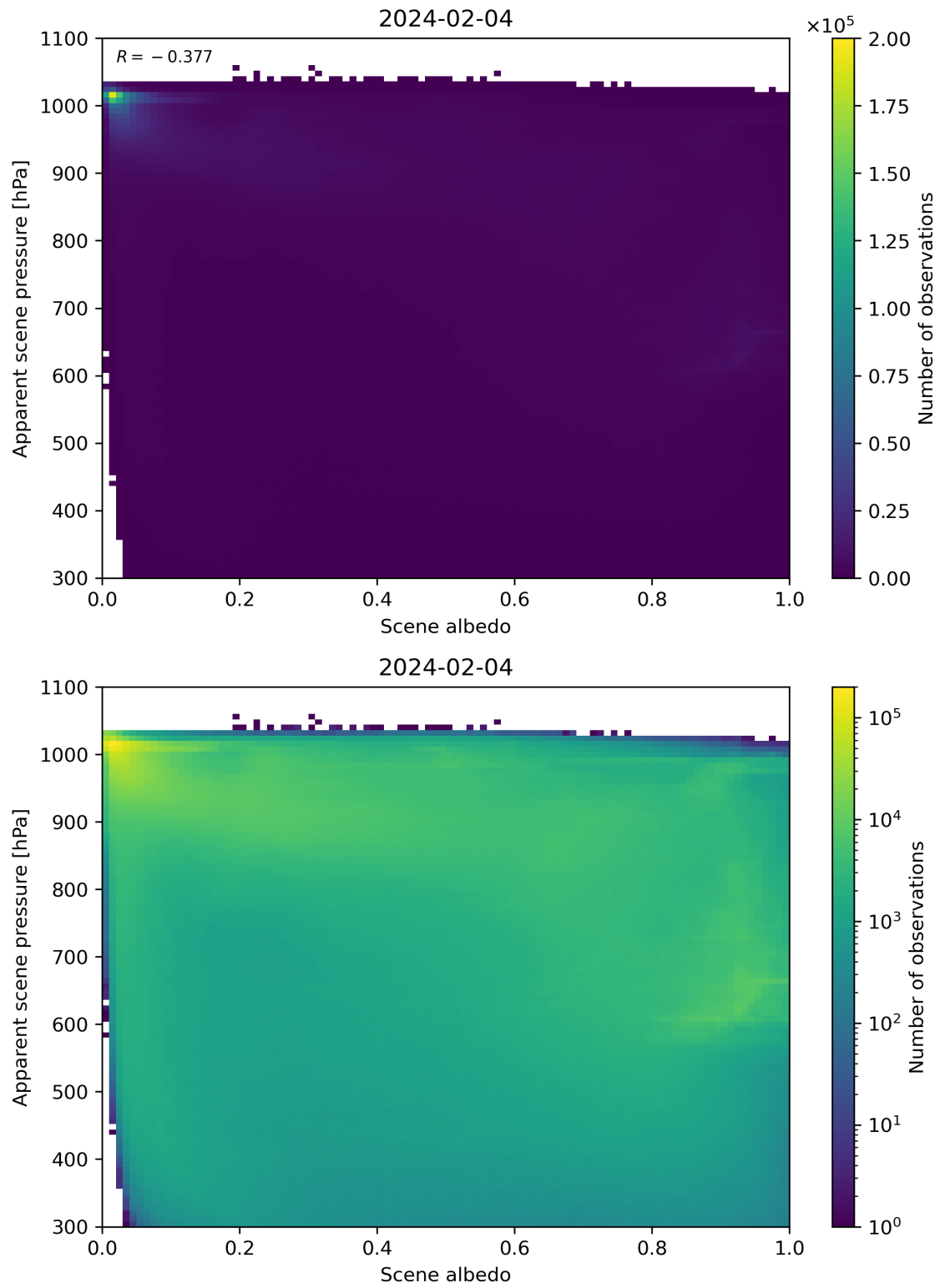
Figure 102: Scatter density plot of “Scene albedo” against “Apparent scene pressure” for 2024-02-03 to 2024-02-05.
