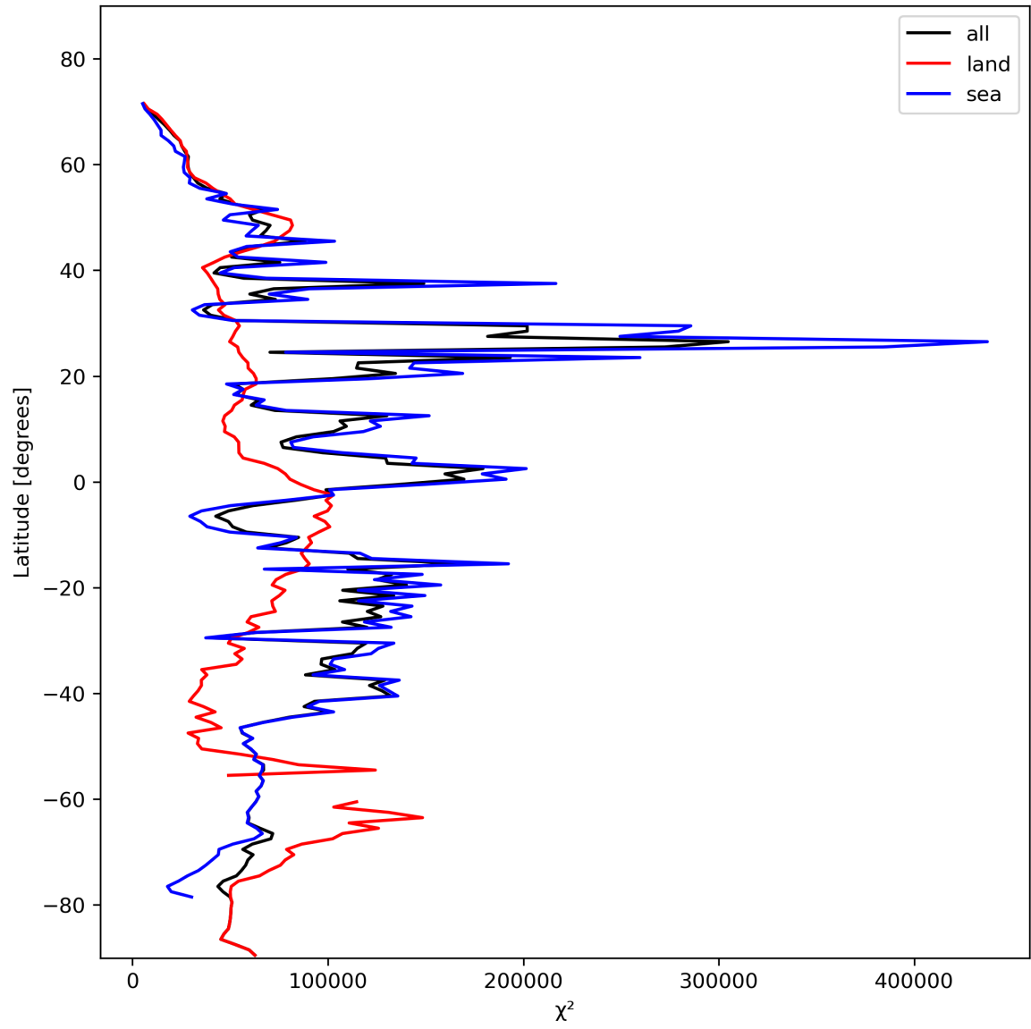
Figure 21: Zonal average of “ \chi^2 ” for 2024-02-03 to 2024-02-05.
