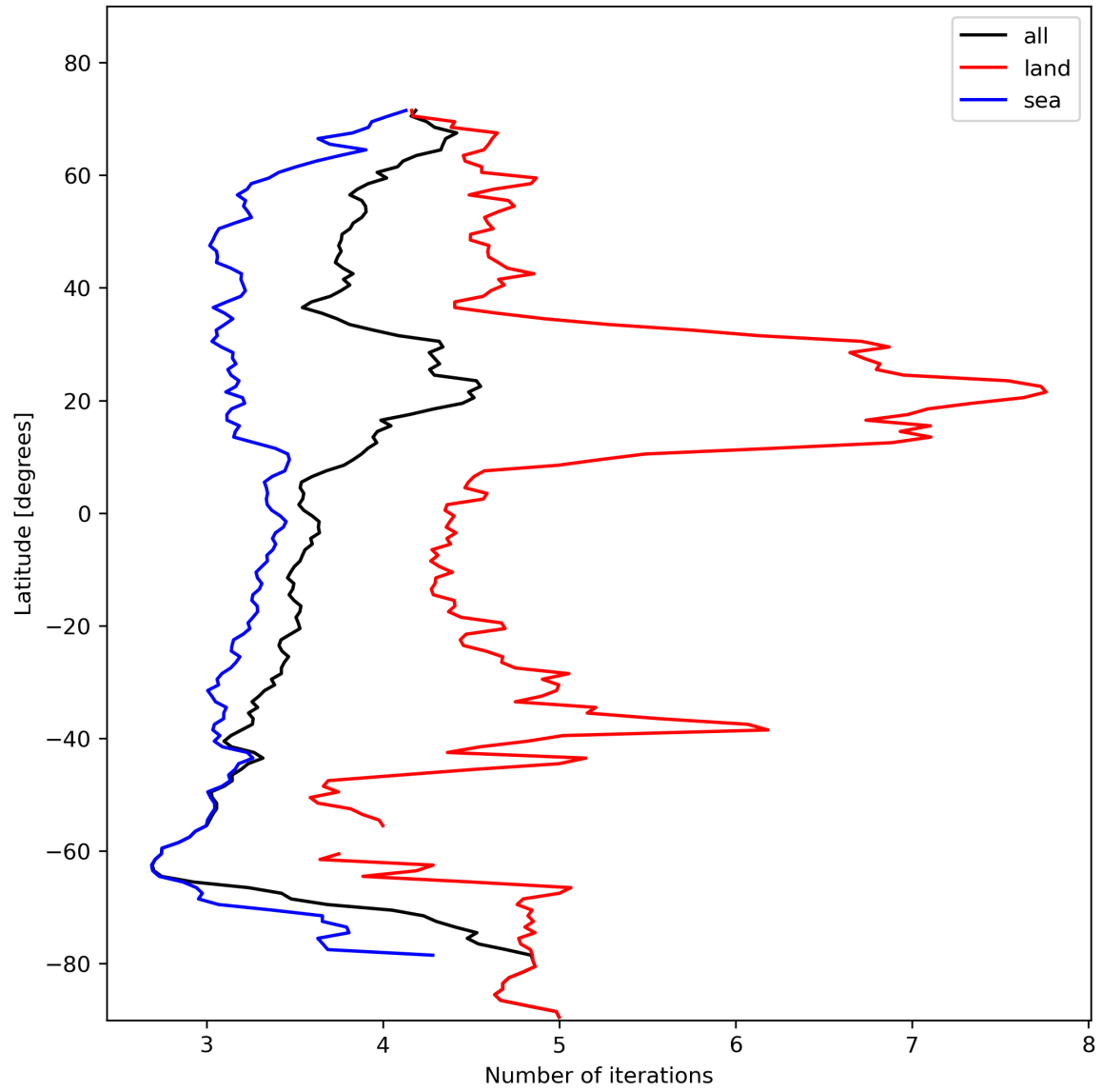
Figure 22: Zonal average of “Number of iterations” for 2024-02-03 to 2024-02-05.
