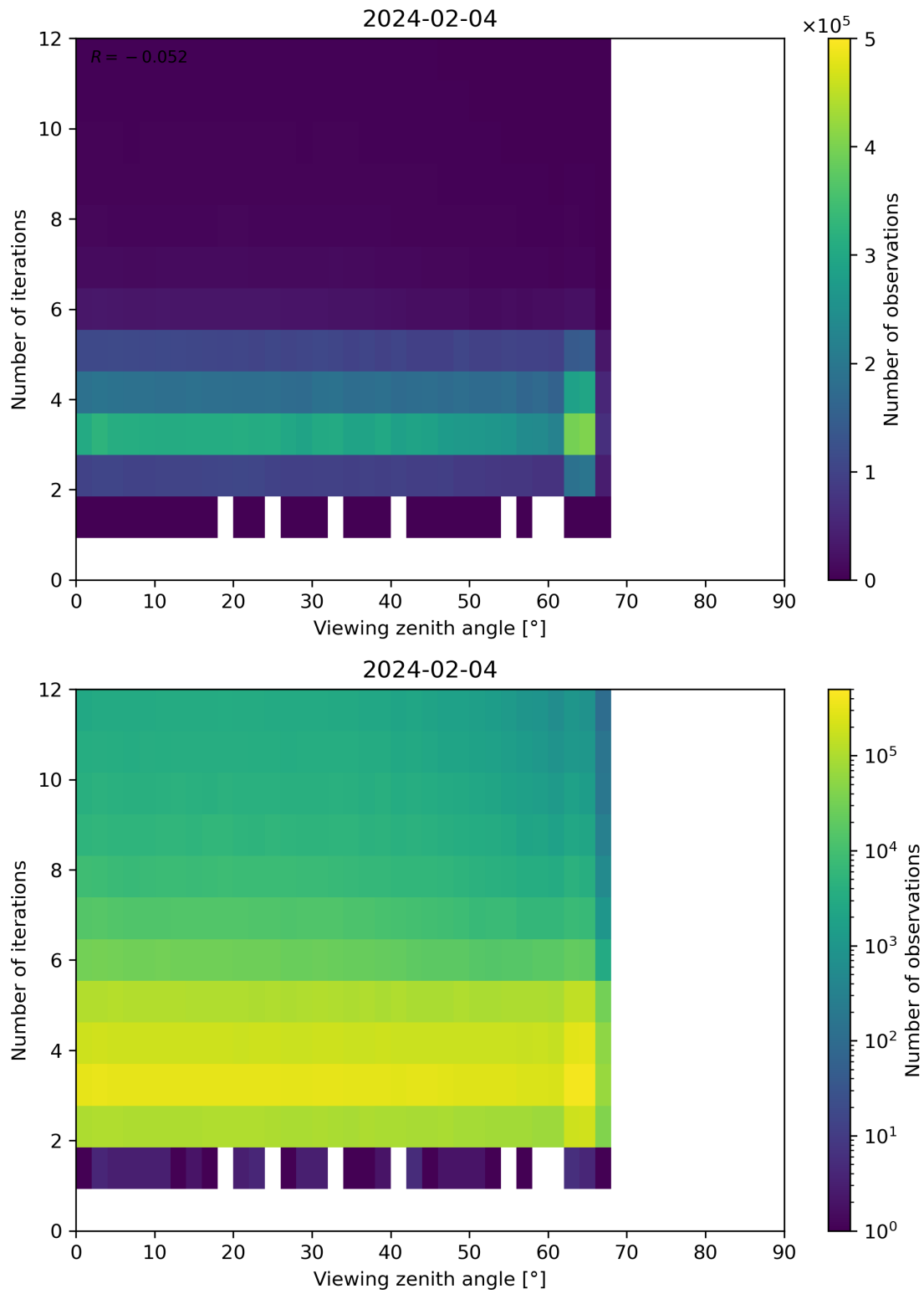
Figure 124: Scatter density plot of “Viewing zenith angle” against “Number of iterations” for 2024-02-03 to 2024-02-05.
