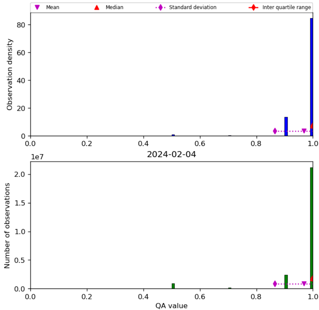
Figure 29: Histogram of “QA value” for 2024-02-03 to 2024-02-05
