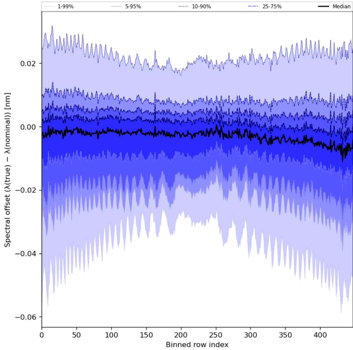
Figure 62: Along track statistics of “Spectral offset ( \lambda(\text{true}) - \lambda(\text{nominal}) )” for 2024-02-03 to 2024-02-05
