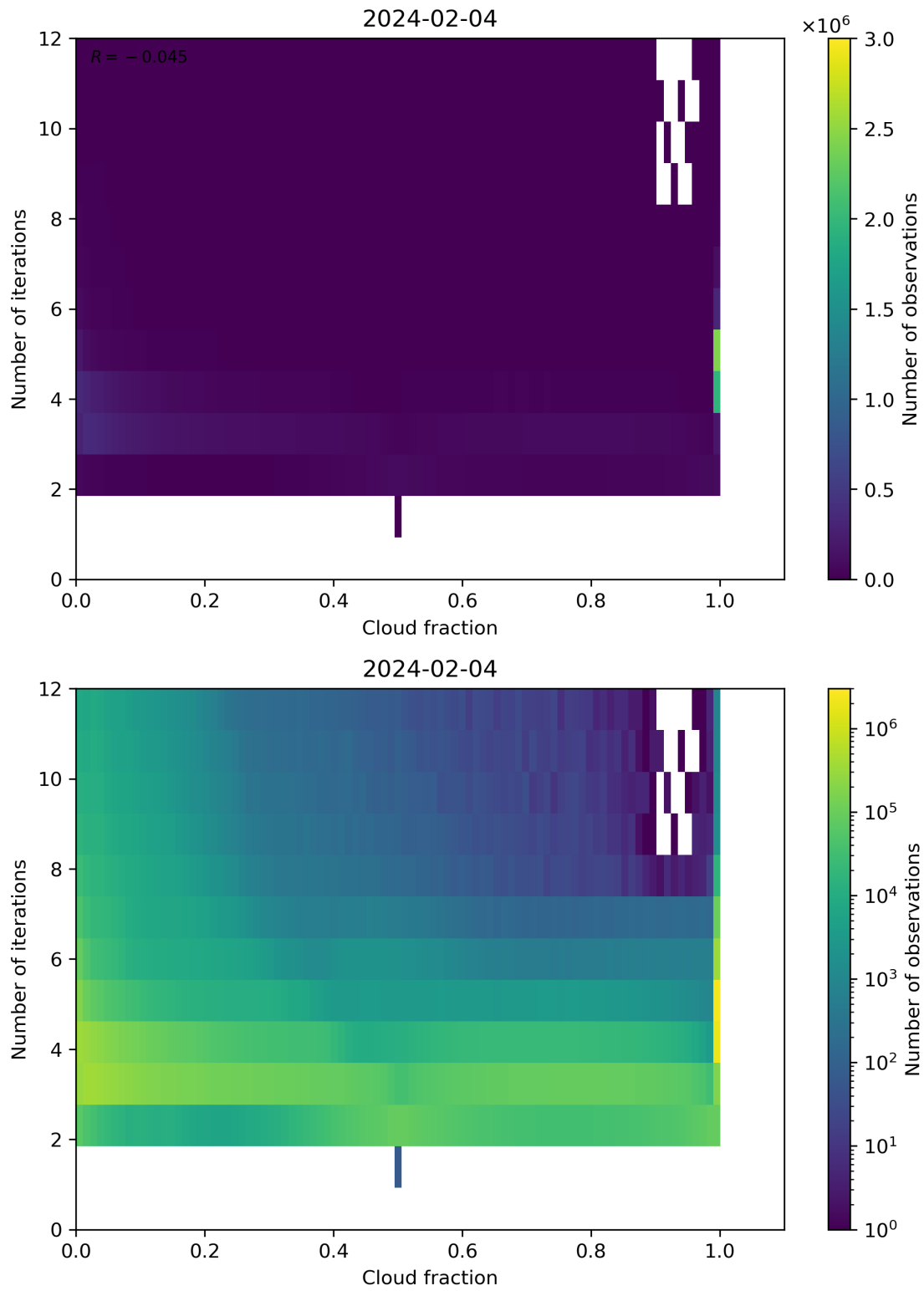
Figure 73: Scatter density plot of “Cloud fraction” against “Number of iterations” for 2024-02-03 to 2024-02-05.
