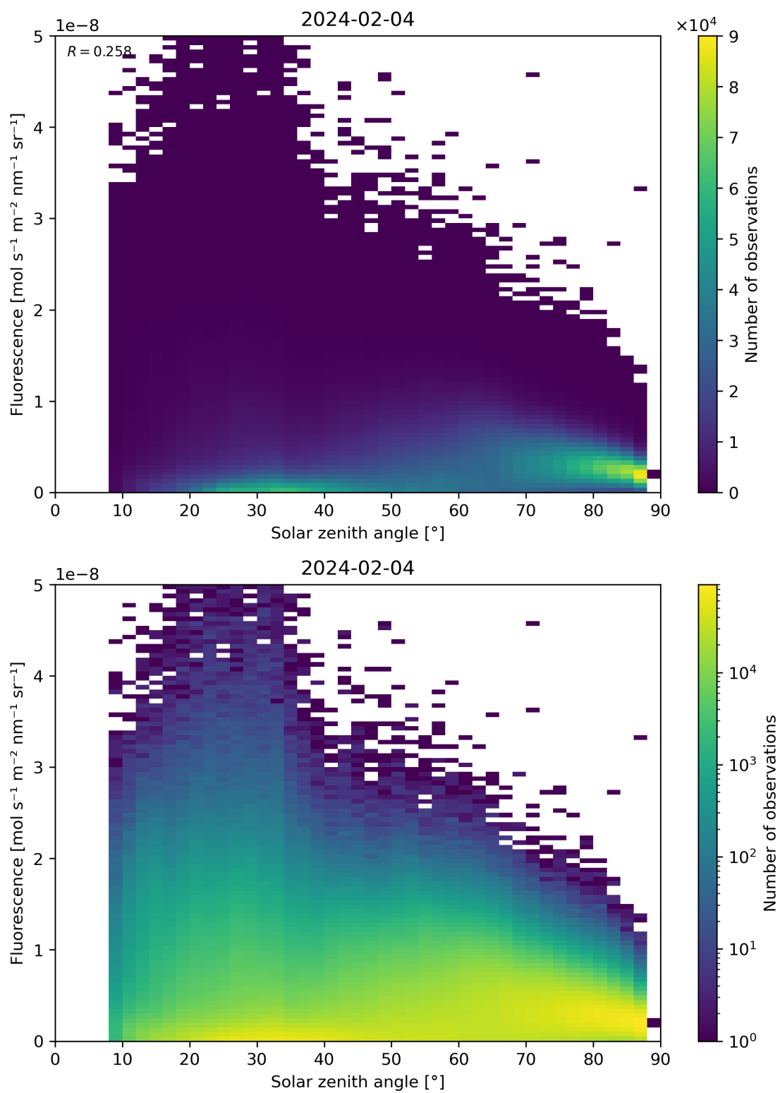
Figure 112: Scatter density plot of “Solar zenith angle” against “Fluorescence” for 2024-02-03 to 2024-02-05.
