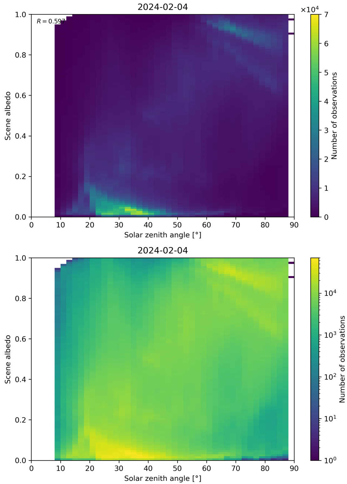
Figure 116: Scatter density plot of “Solar zenith angle” against “Scene albedo” for 2024-02-03 to 2024-02-05.
