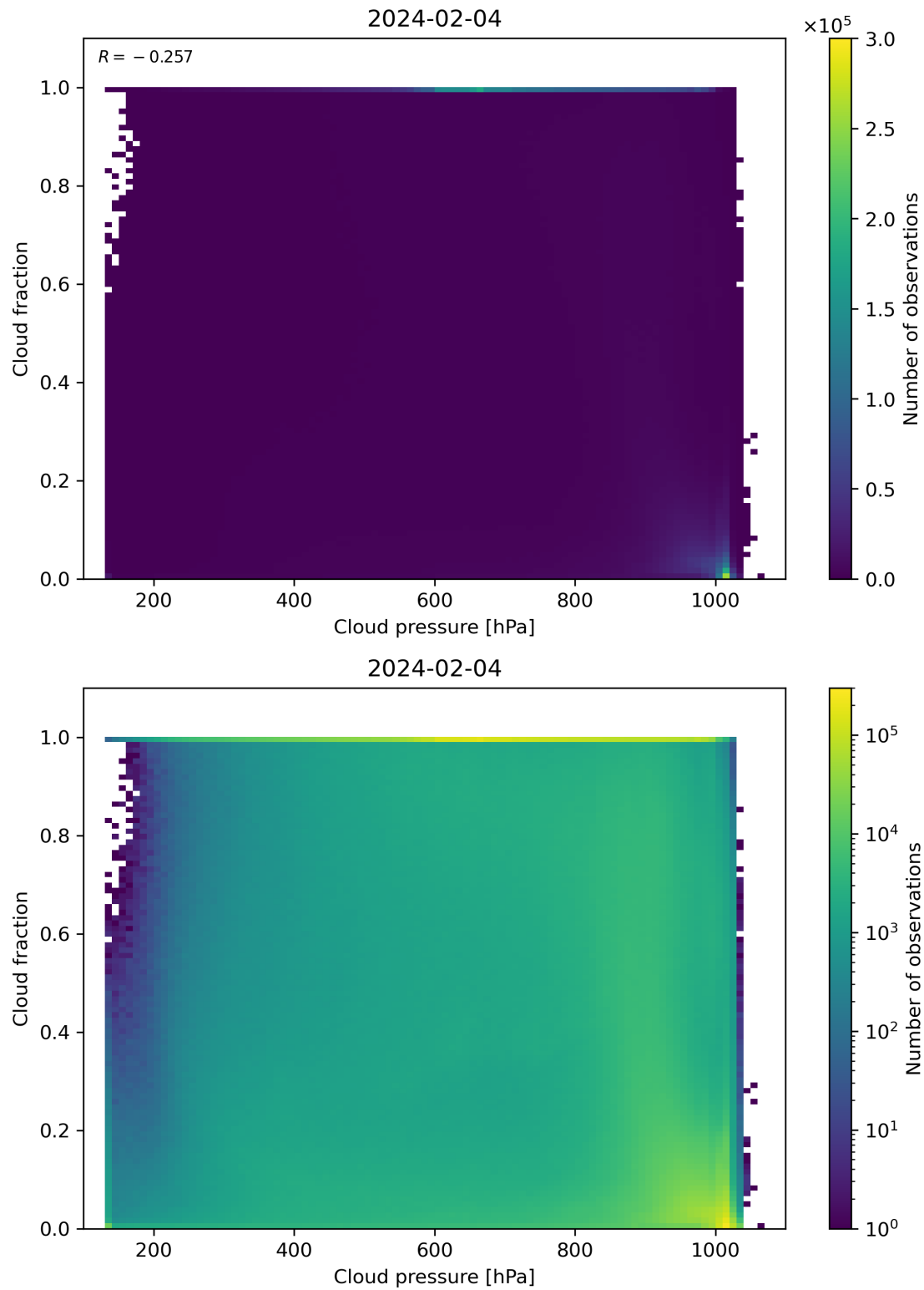
Figure 79: Scatter density plot of “Cloud pressure” against “Cloud fraction” for 2024-02-03 to 2024-02-05.
