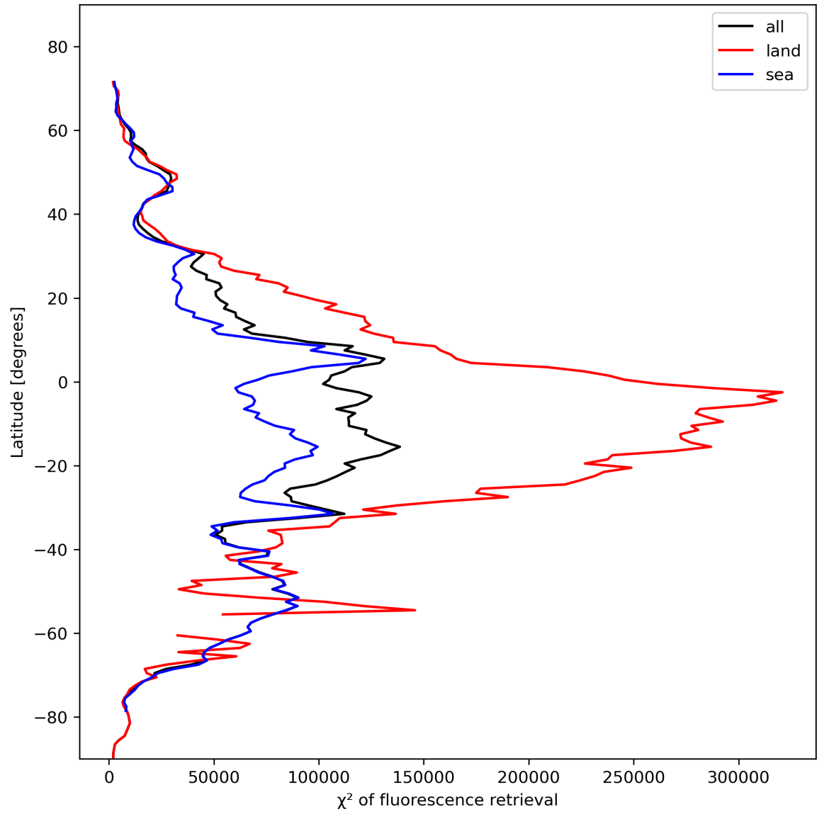
Figure 25: Zonal average of “ \chi^2 of fluorescence retrieval” for 2024-02-03 to 2024-02-05.
