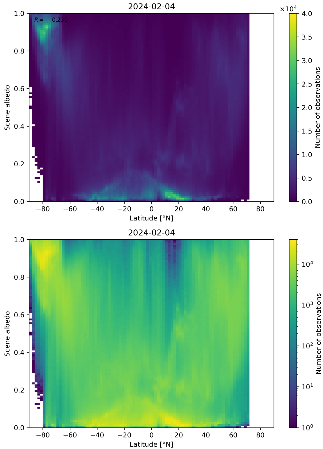
Figure 95: Scatter density plot of “Latitude” against “Scene albedo” for 2024-02-03 to 2024-02-05.
