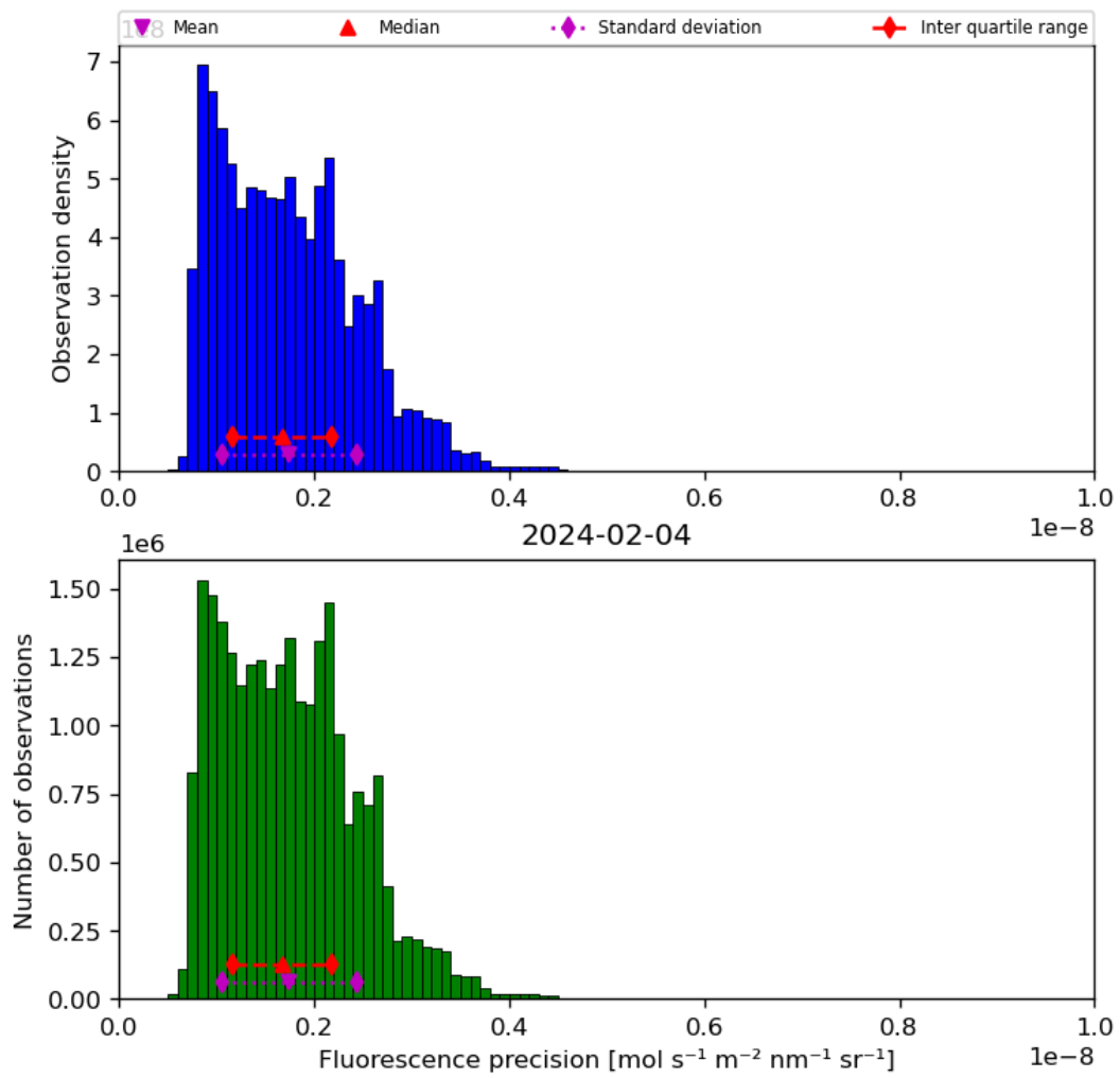
Figure 41: Histogram of “Fluorescence precision” for 2024-02-03 to 2024-02-05
