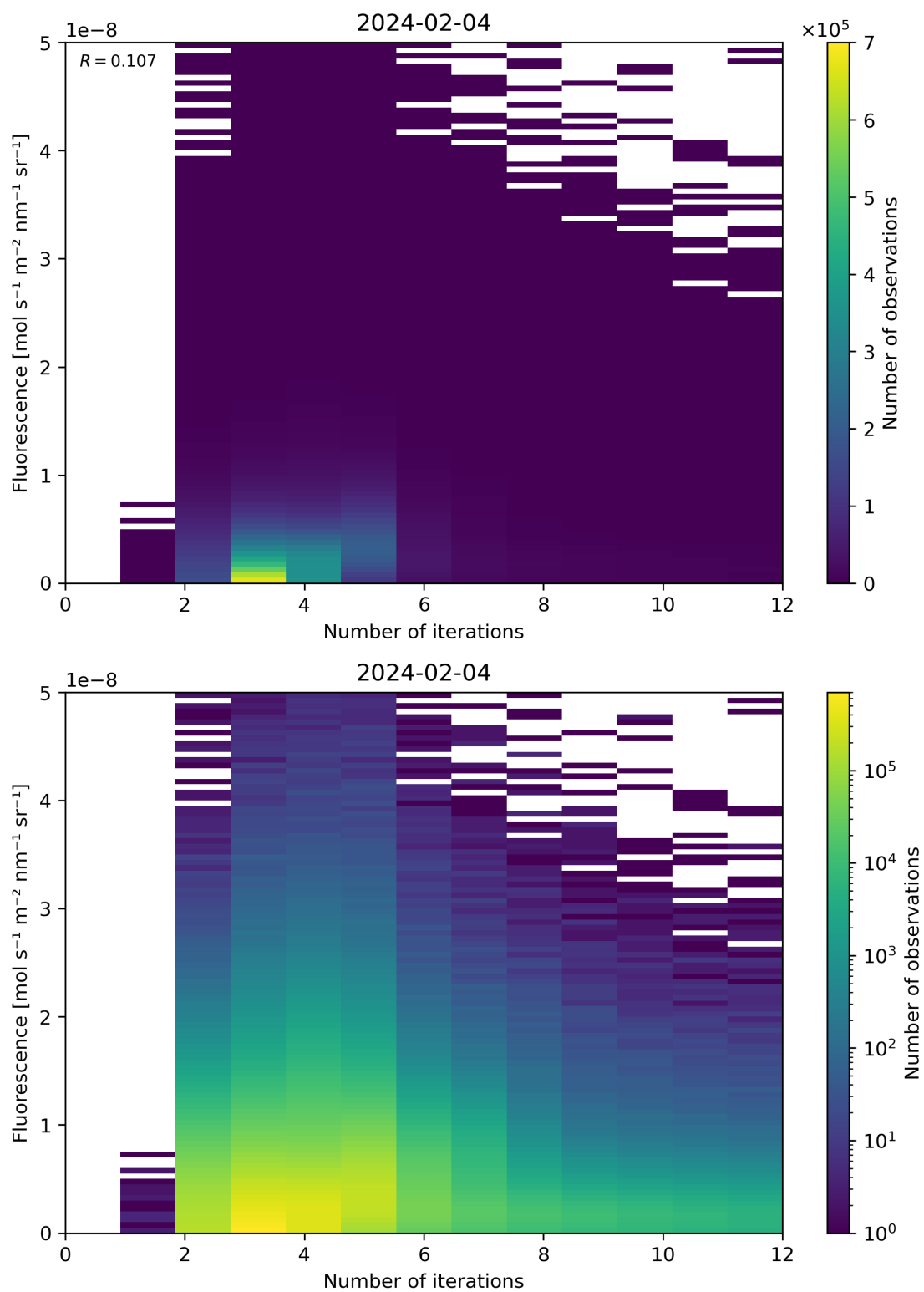
Figure 98: Scatter density plot of “Number of iterations” against “Fluorescence” for 2024-02-03 to 2024-02-05.
