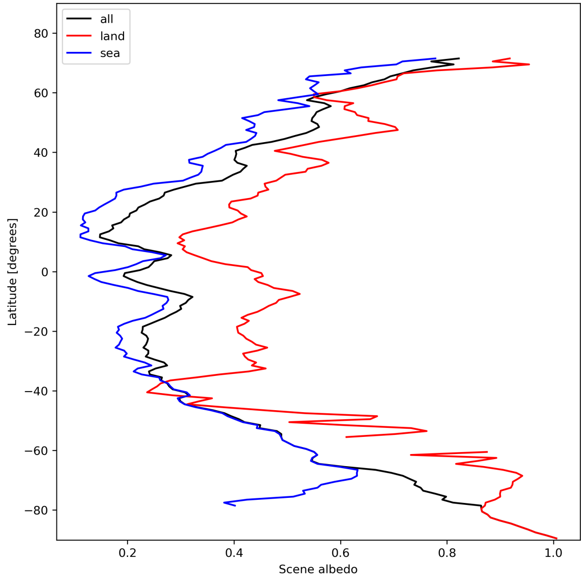
Figure 17: Zonal average of “Scene albedo” for 2024-02-03 to 2024-02-05.
