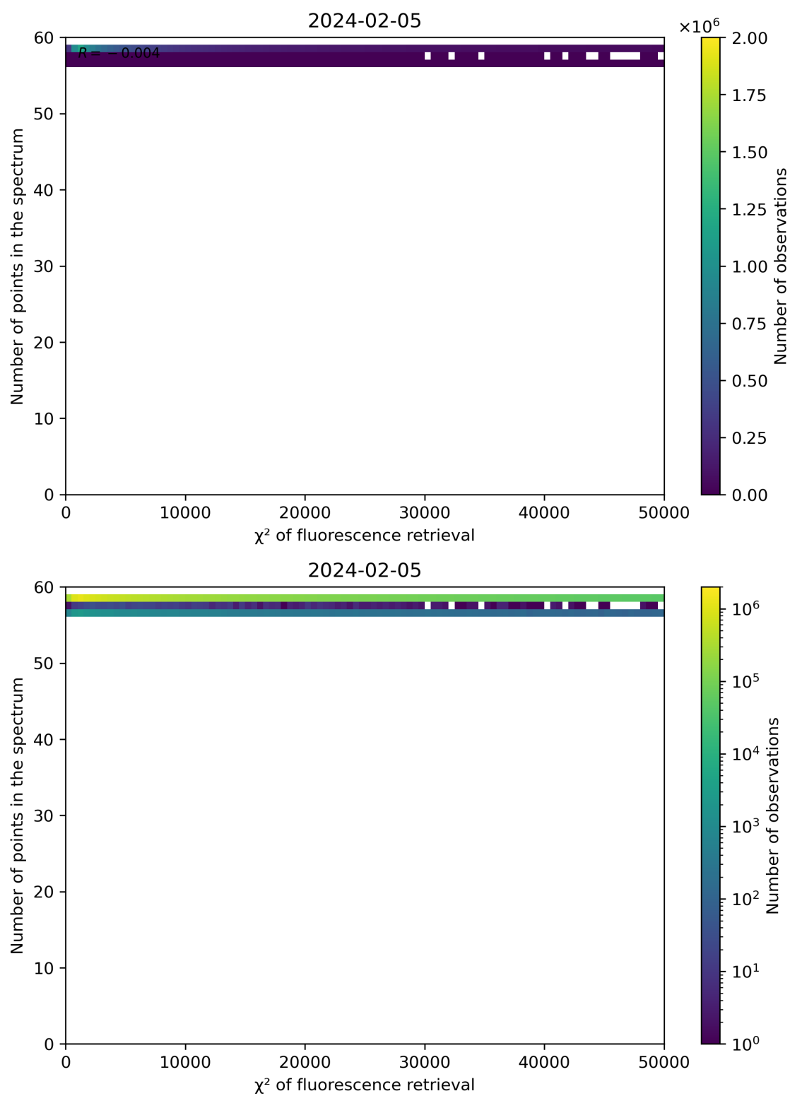
Figure 68: Scatter density plot of " \chi^2 of fluorescence retrieval" against "Number of points in the spectrum" for 2024-02-04 to 2024-02-06.
