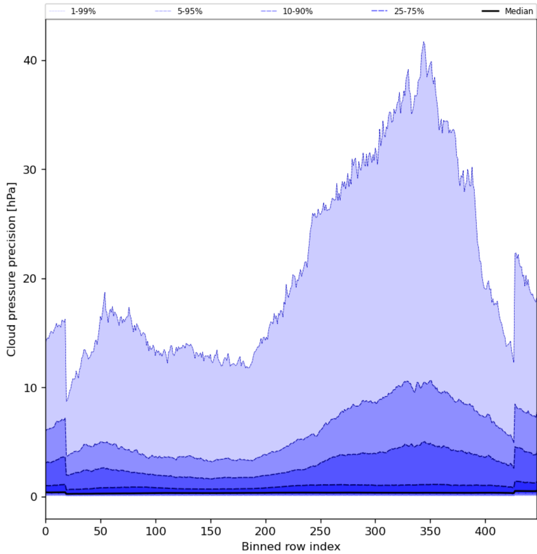
Figure 48: Along track statistics of “Cloud pressure precision” for 2024-02-04 to 2024-02-06
