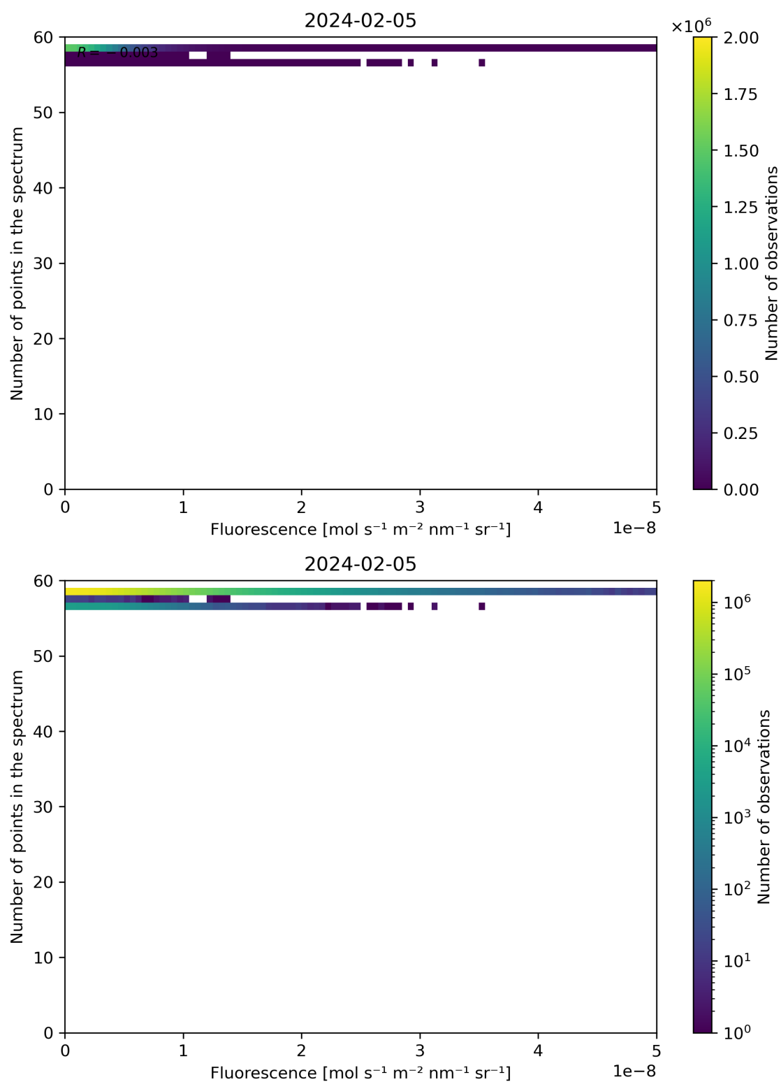
Figure 86: Scatter density plot of “Fluorescence” against “Number of points in the spectrum” for 2024-02-04 to 2024-02-06.
