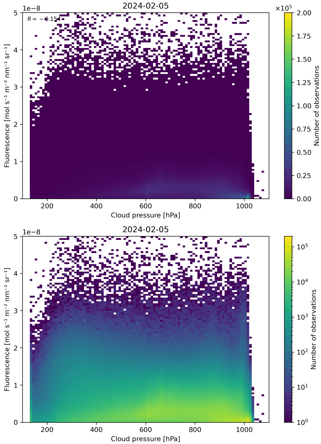
Figure 80: Scatter density plot of “Cloud pressure” against “Fluorescence” for 2024-02-04 to 2024-02-06.
