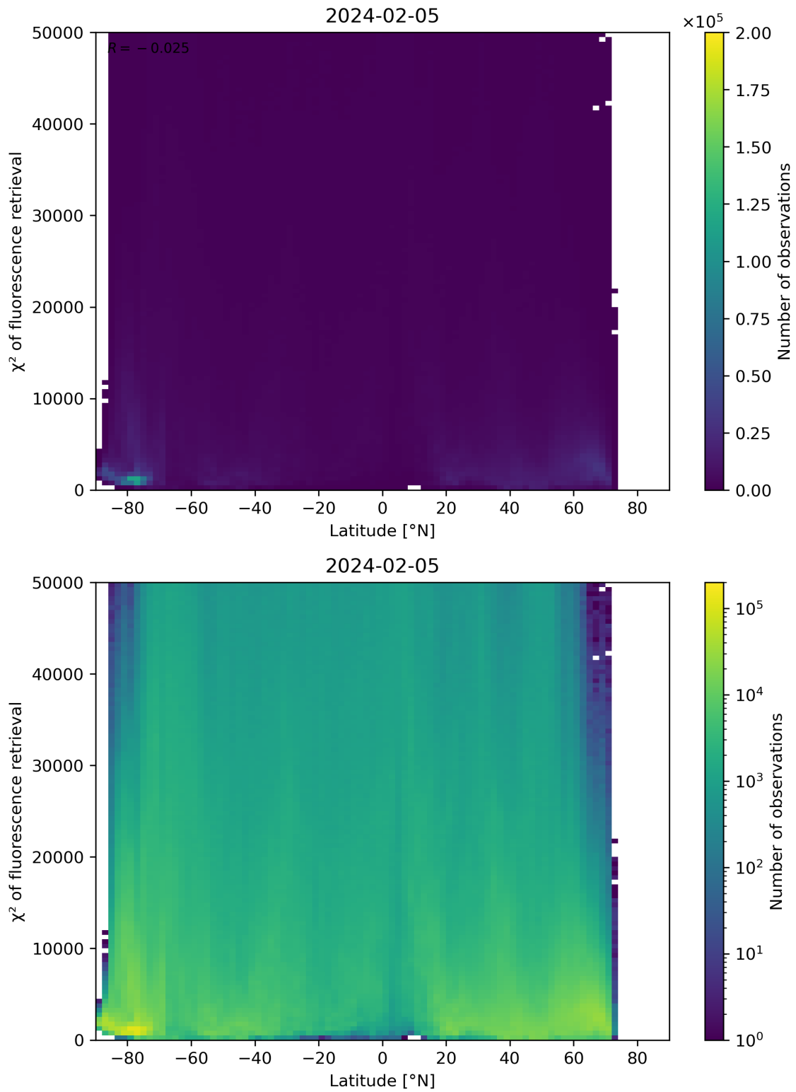
Figure 89: Scatter density plot of “Latitude” against “ \chi^2 of fluorescence retrieval” for 2024-02-04 to 2024-02-06.
