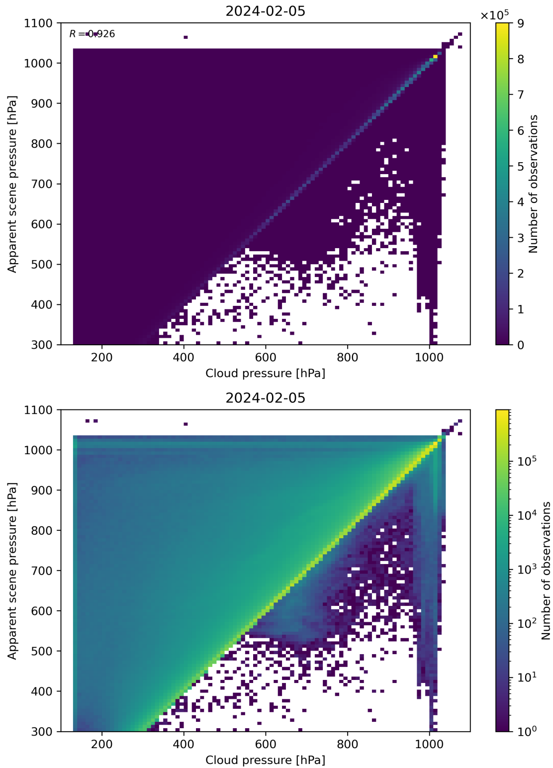
Figure 77: Scatter density plot of “Cloud pressure” against “Apparent scene pressure” for 2024-02-04 to 2024-02-06.
