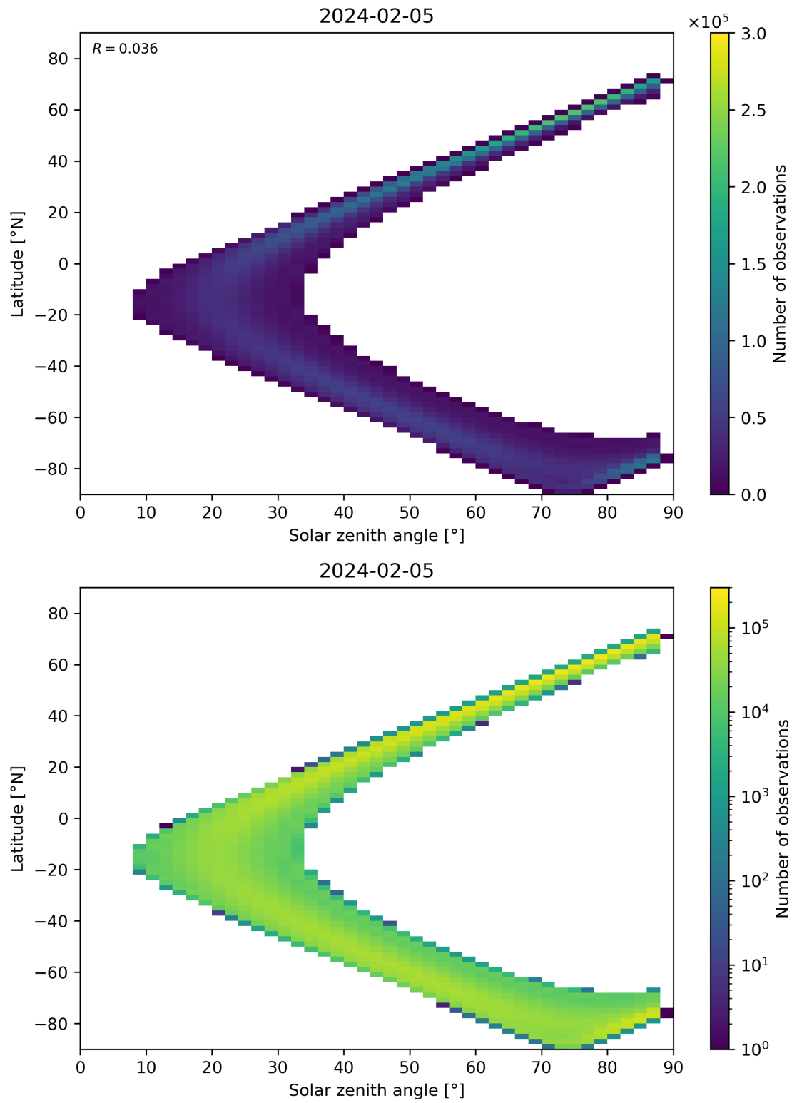
Figure 113: Scatter density plot of “Solar zenith angle” against “Latitude” for 2024-02-04 to 2024-02-06.
