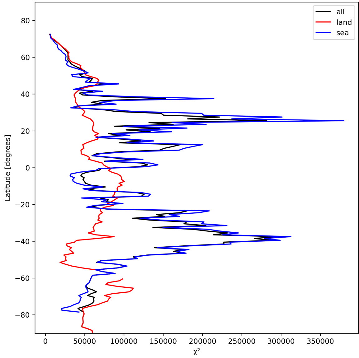
Figure 21: Zonal average of “ \chi^2 ” for 2024-02-04 to 2024-02-06.
