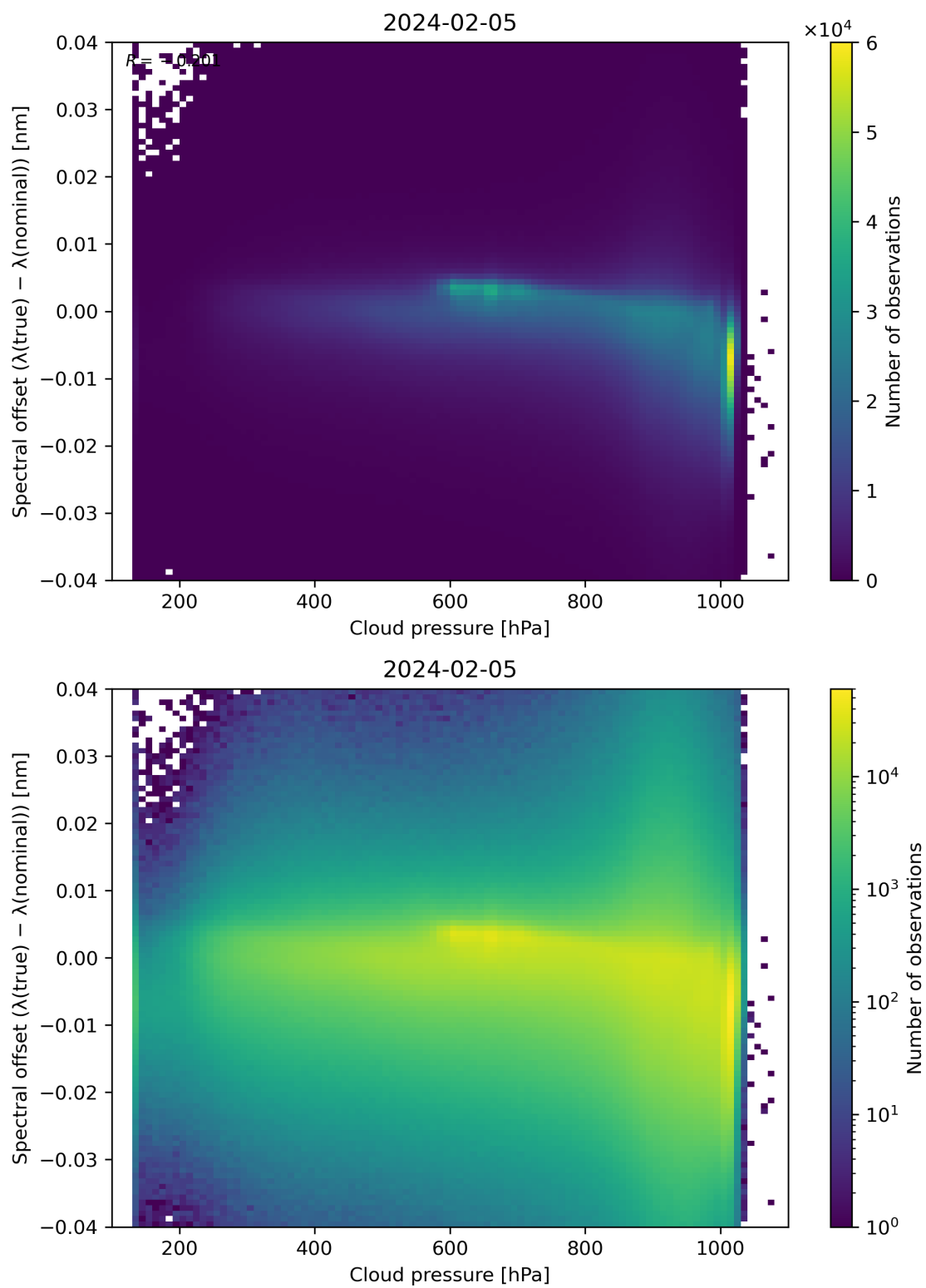
Figure 84: Scatter density plot of “Cloud pressure” against “Spectral offset ( \lambda(\text{true}) - \lambda(\text{nominal}) )” for 2024-02-04 to 2024-02-06.
