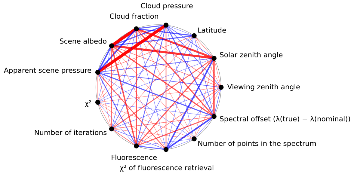
Figure 1: Map of correlation graph for 2024-02-04 to 2024-02-06.
