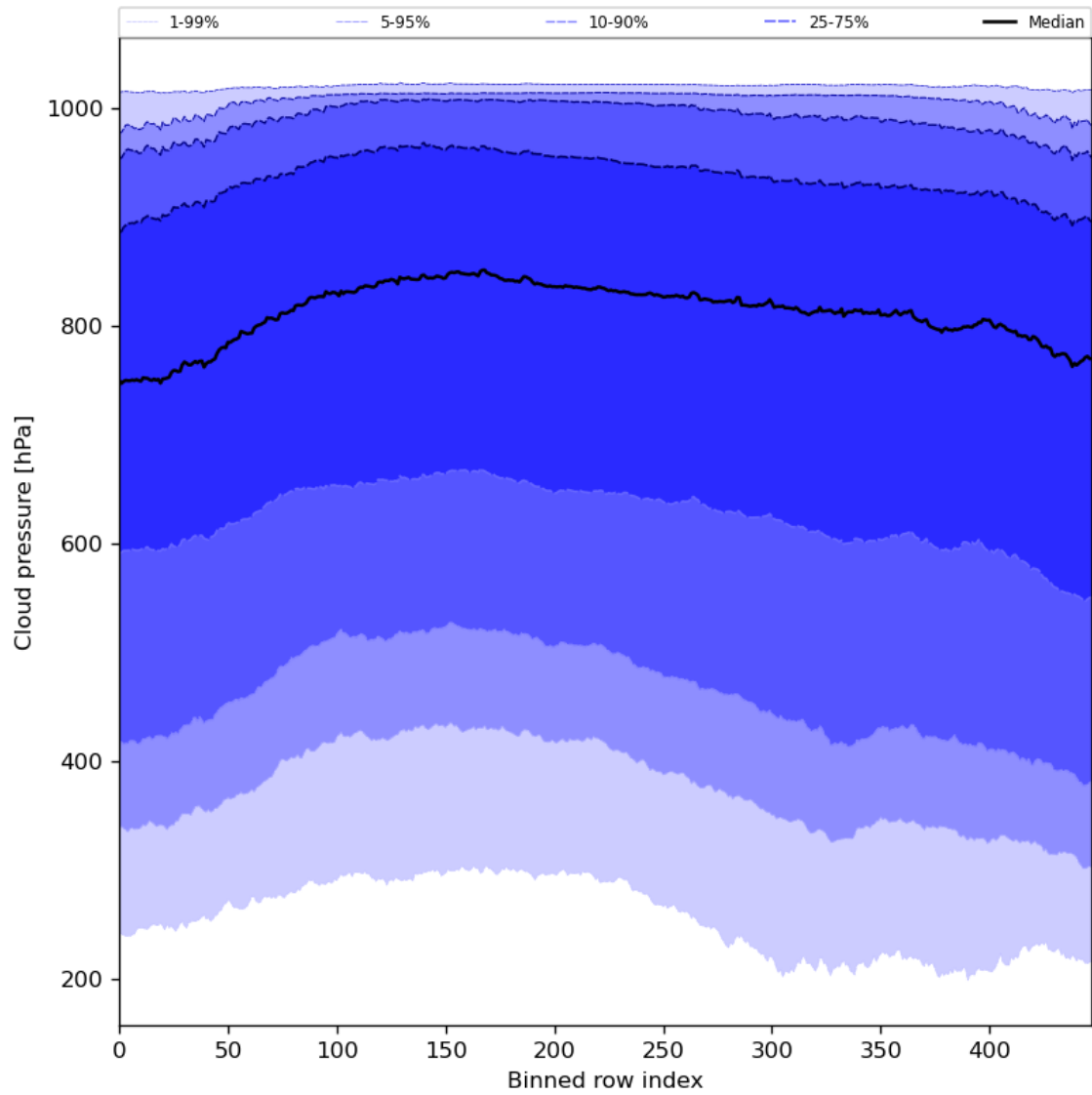
Figure 47: Along track statistics of “Cloud pressure” for 2024-02-04 to 2024-02-06
