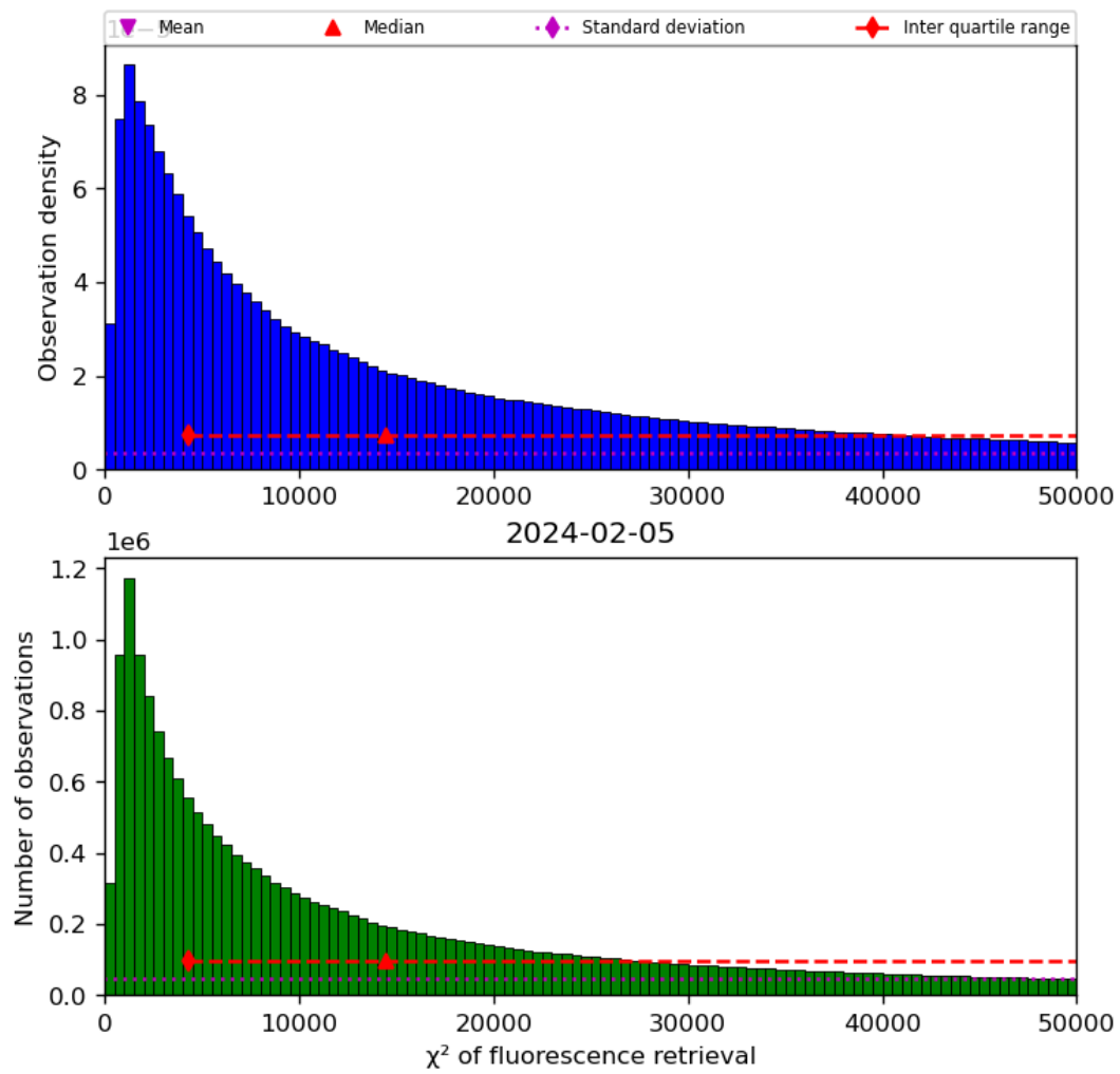
Figure 42: Histogram of “ \chi^2 of fluorescence retrieval” for 2024-02-04 to 2024-02-06
