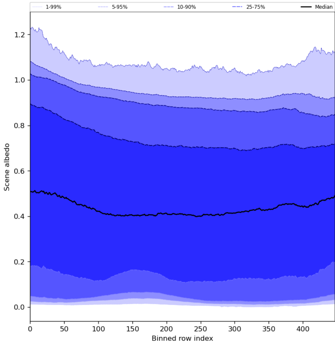
Figure 51: Along track statistics of “Scene albedo” for 2024-02-04 to 2024-02-06
