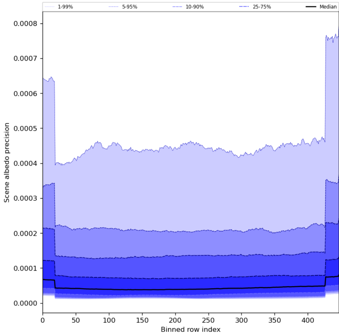
Figure 52: Along track statistics of “Scene albedo precision” for 2024-02-04 to 2024-02-06
