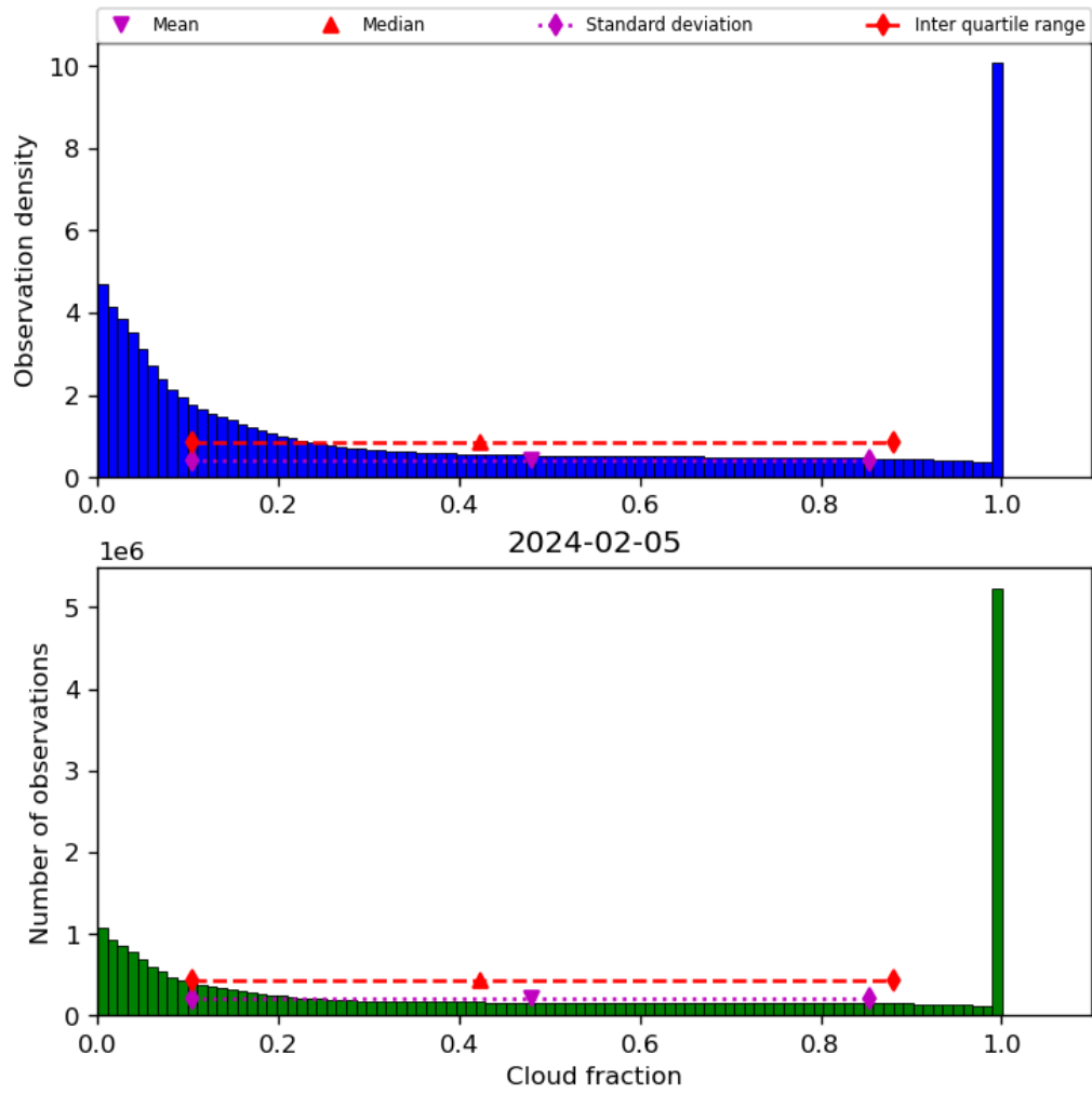
Figure 32: Histogram of “Cloud fraction” for 2024-02-04 to 2024-02-06
