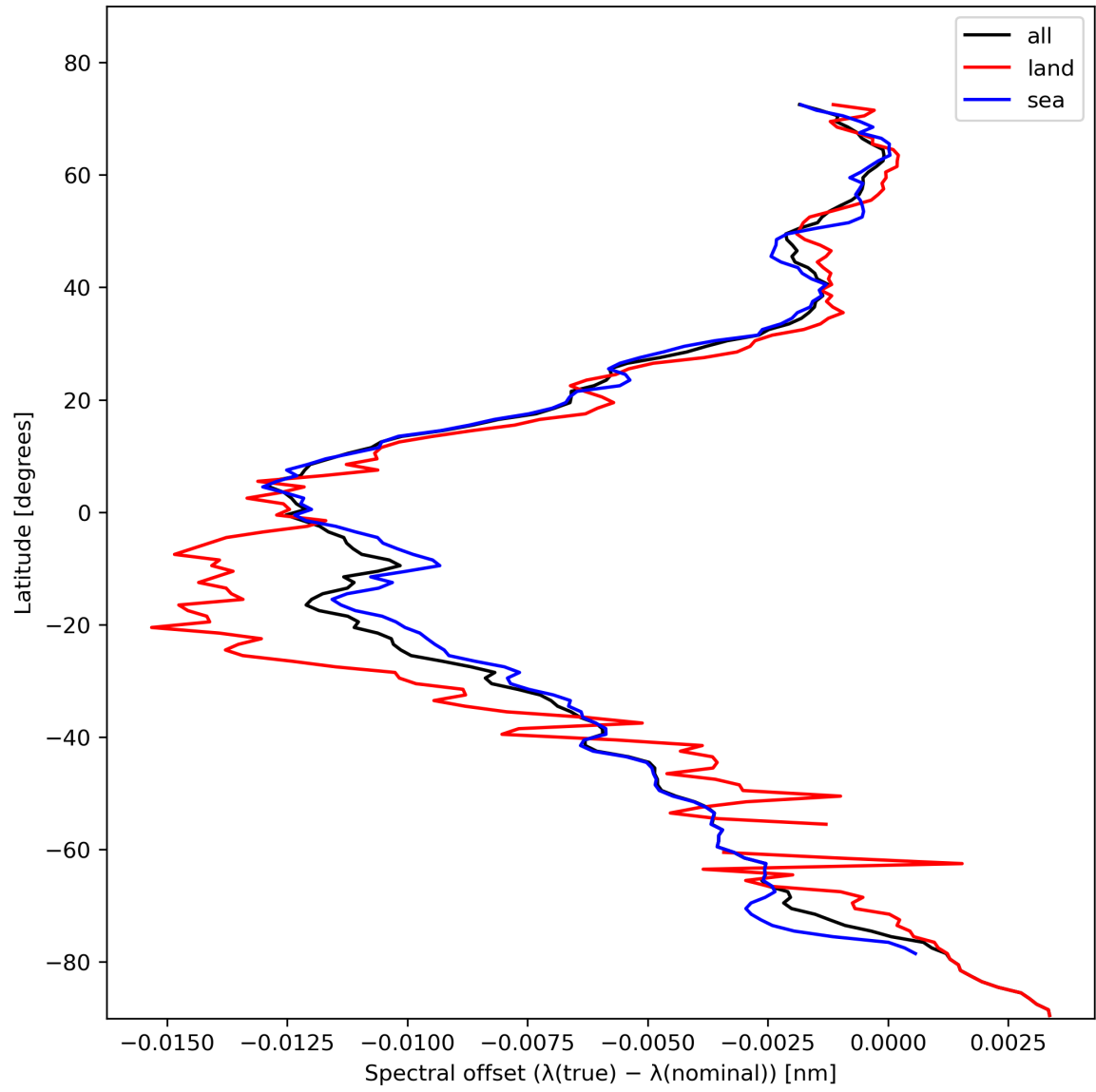
Figure 28: Zonal average of “Spectral offset ( \lambda(\text{true}) - \lambda(\text{nominal}) )” for 2024-02-04 to 2024-02-06.
