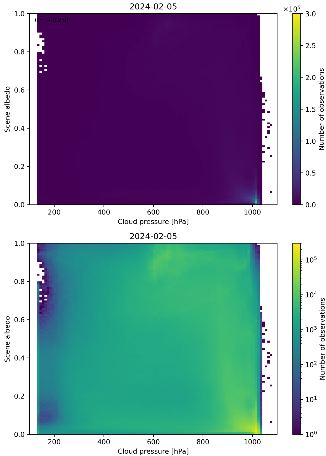
Figure 83: Scatter density plot of “Cloud pressure” against “Scene albedo” for 2024-02-04 to 2024-02-06.
