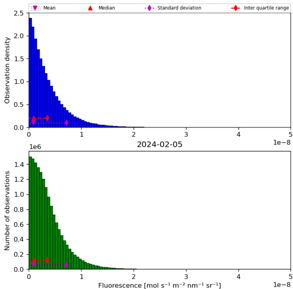
Figure 40: Histogram of “Fluorescence” for 2024-02-04 to 2024-02-06
