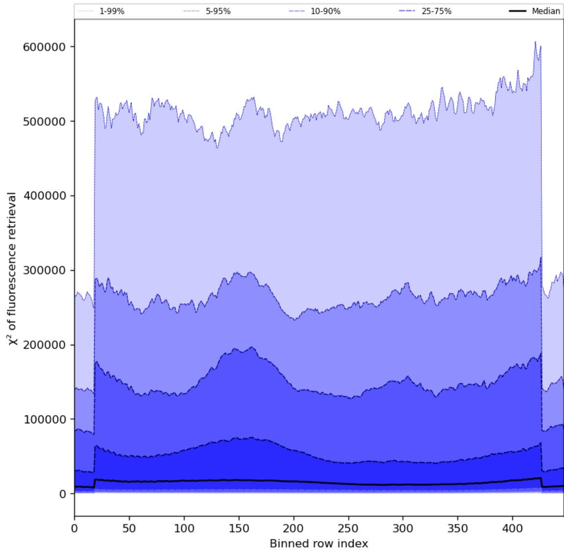
Figure 59: Along track statistics of “ \chi^2 of fluorescence retrieval” for 2024-02-04 to 2024-02-06
