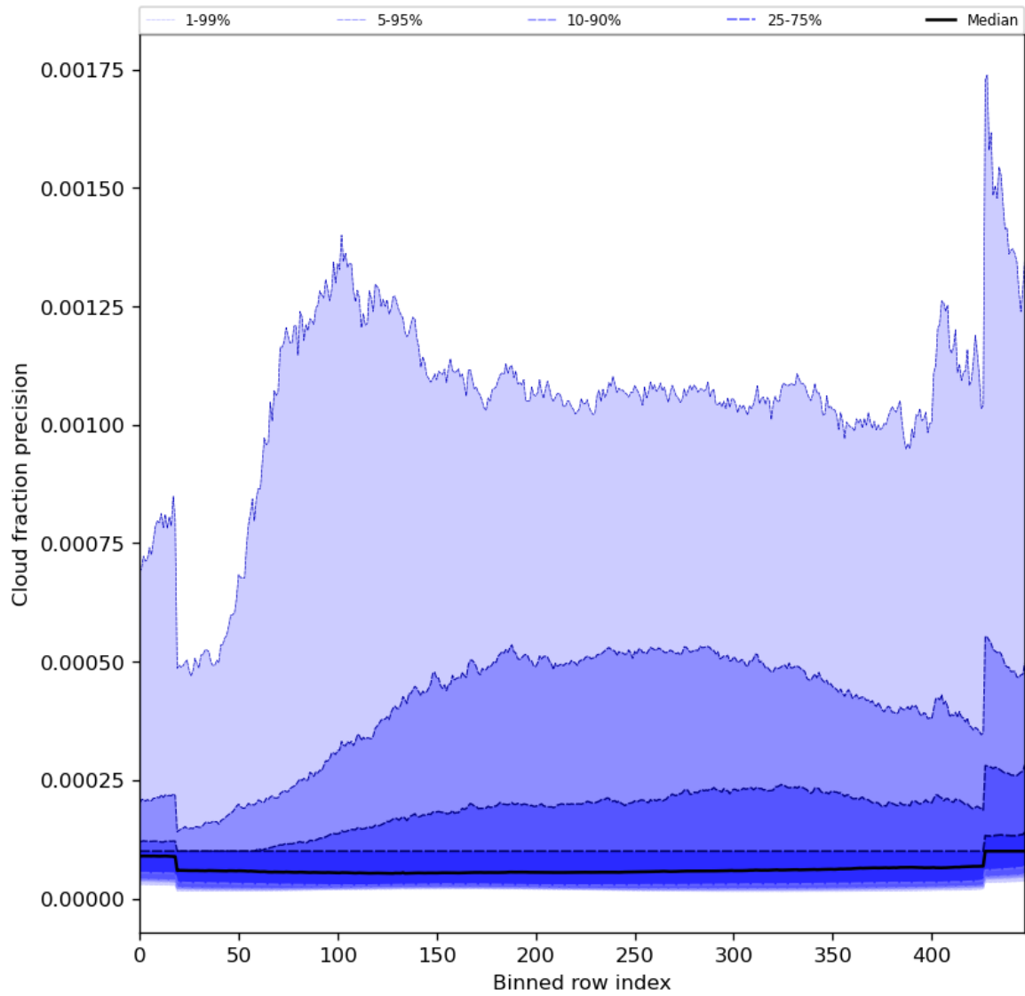
Figure 50: Along track statistics of “Cloud fraction precision” for 2024-02-04 to 2024-02-06
