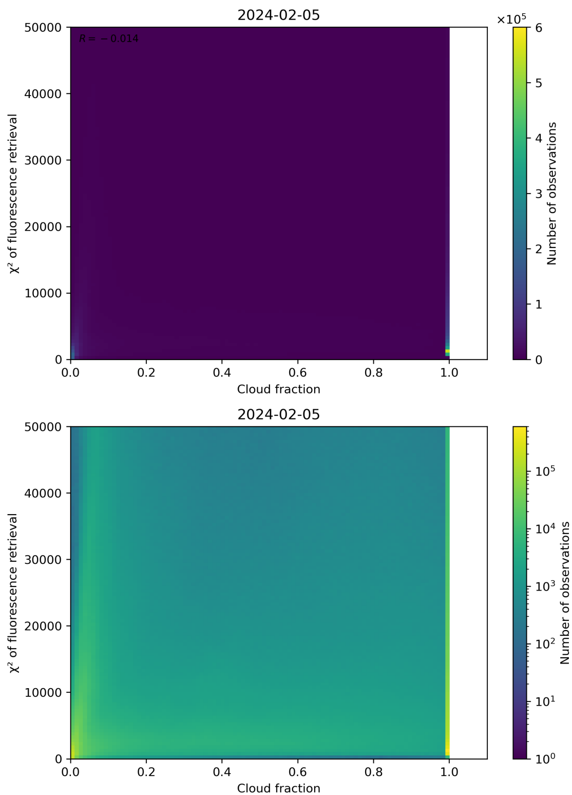
Figure 71: Scatter density plot of “Cloud fraction” against “ \chi^2 of fluorescence retrieval” for 2024-02-04 to 2024-02-06.
