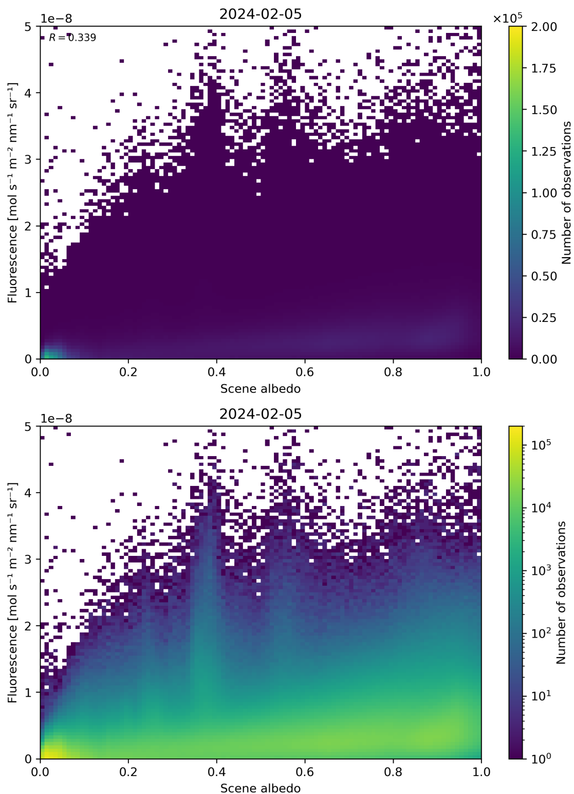
Figure 104: Scatter density plot of “Scene albedo” against “Fluorescence” for 2024-02-04 to 2024-02-06.
