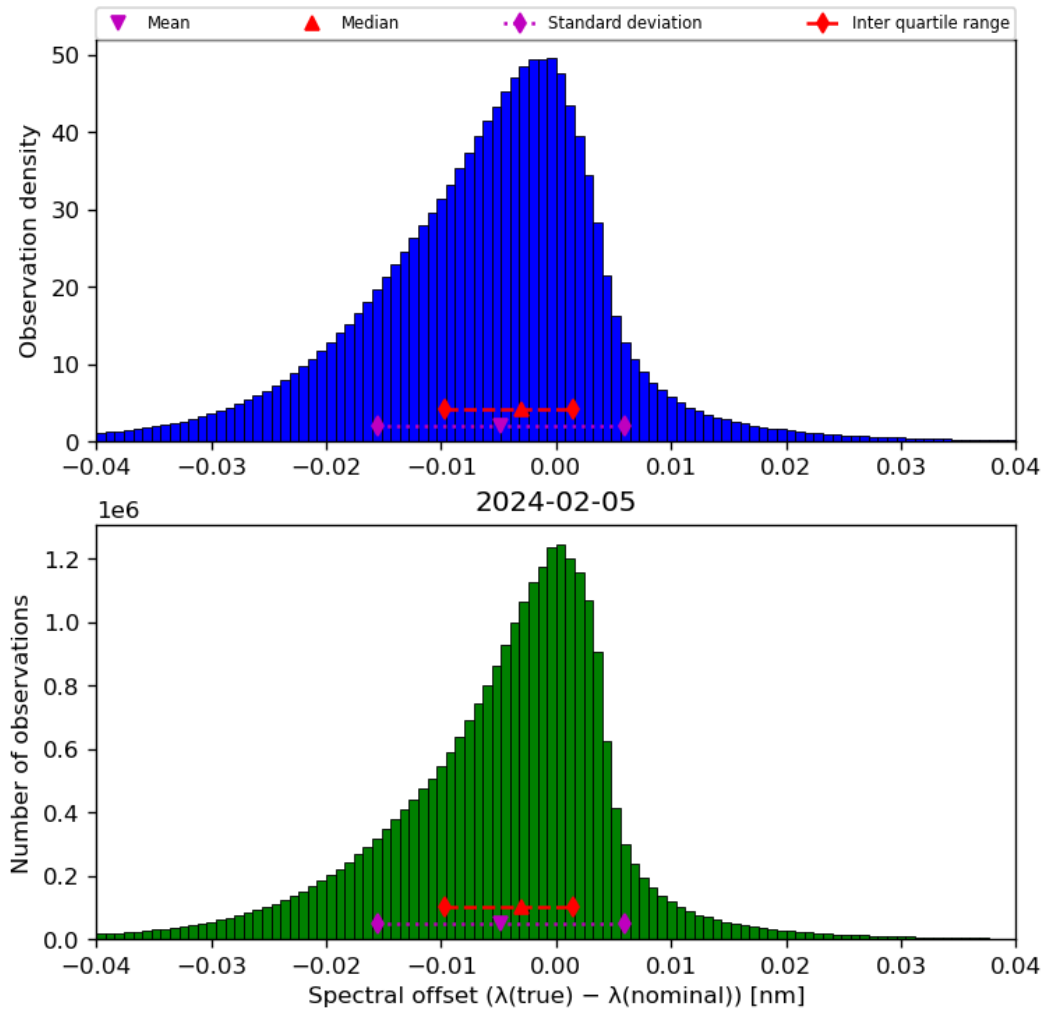
Figure 45: Histogram of “Spectral offset ( \lambda(\text{true}) - \lambda(\text{nominal}) )” for 2024-02-04 to 2024-02-06
