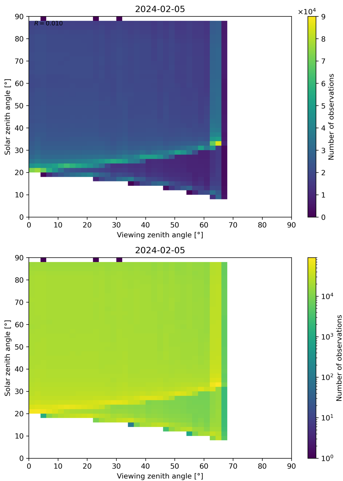
Figure 127: Scatter density plot of “Viewing zenith angle” against “Solar zenith angle” for 2024-02-04 to 2024-02-06.
