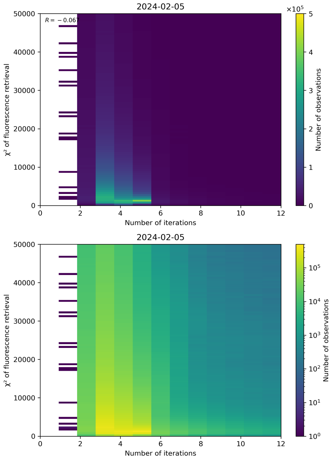
Figure 97: Scatter density plot of “Number of iterations” against “ \chi^2 of fluorescence retrieval” for 2024-02-04 to 2024-02-06.
