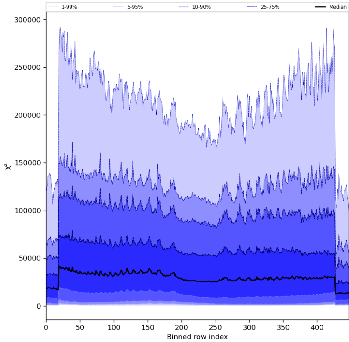
Figure 55: Along track statistics of “ \chi^2 ” for 2024-02-04 to 2024-02-06
