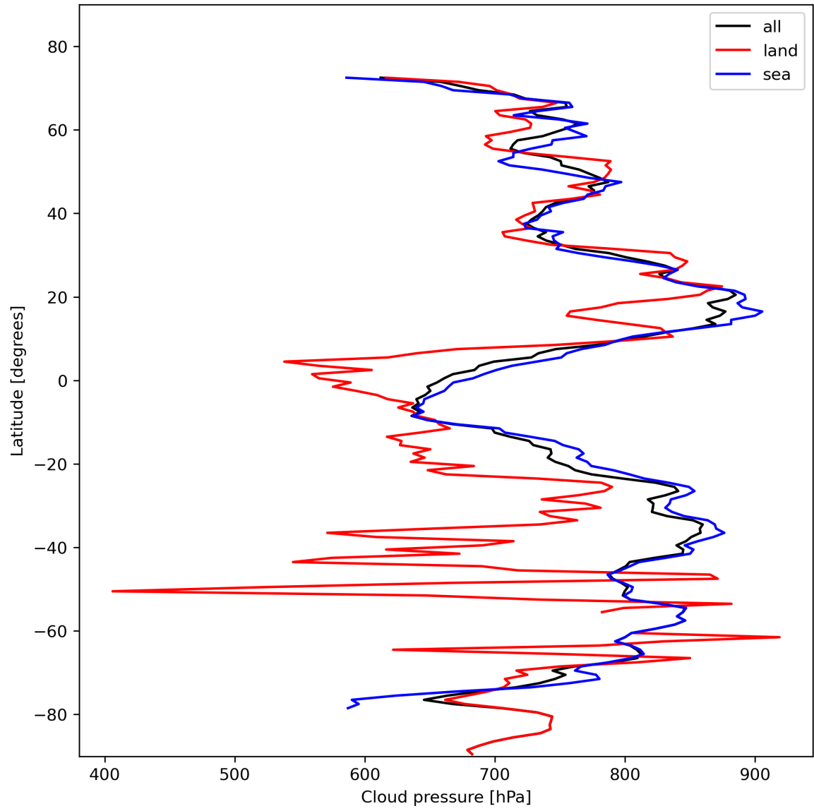
Figure 13: Zonal average of “Cloud pressure” for 2024-02-04 to 2024-02-06.
