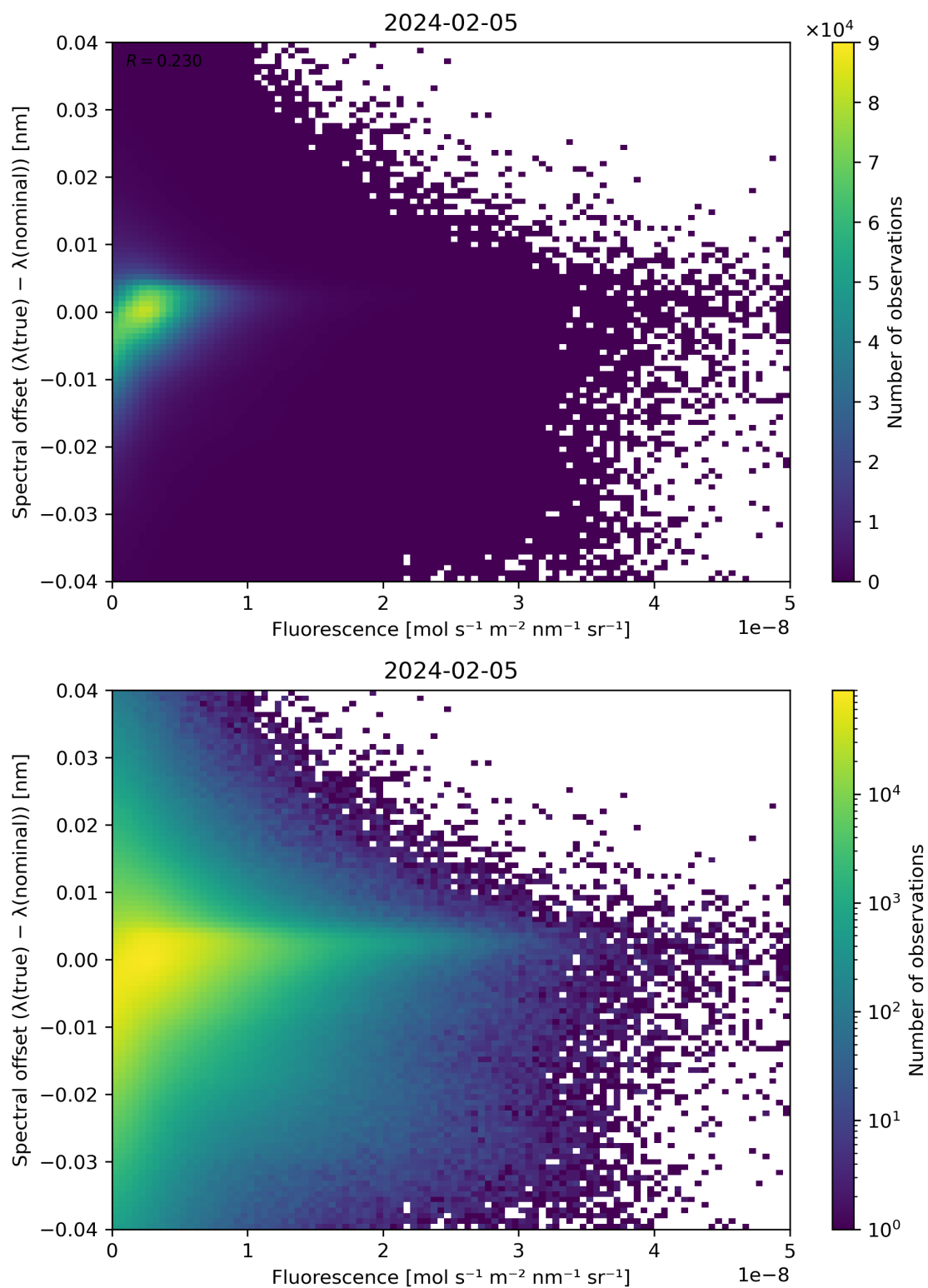
Figure 87: Scatter density plot of “Fluorescence” against “Spectral offset ( \lambda(\text{true}) - \lambda(\text{nominal}) )” for 2024-02-04 to 2024-02-06.
