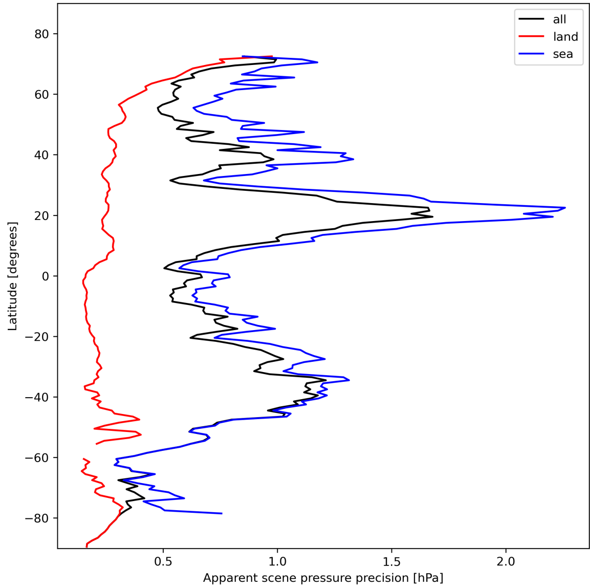
Figure 20: Zonal average of “Apparent scene pressure precision” for 2024-02-04 to 2024-02-06.
