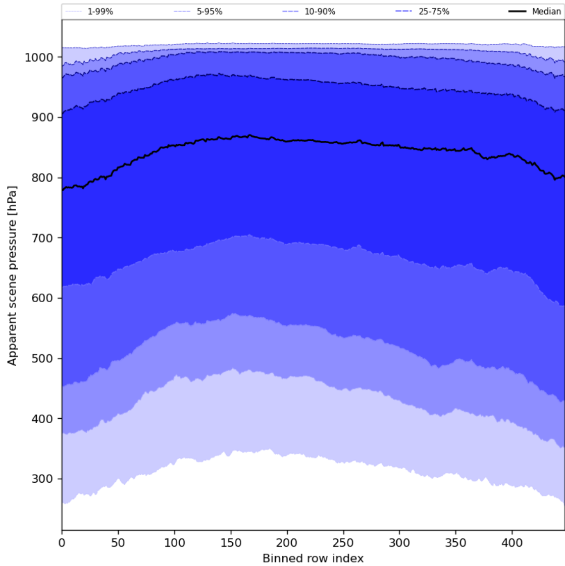
Figure 53: Along track statistics of “Apparent scene pressure” for 2024-02-04 to 2024-02-06
