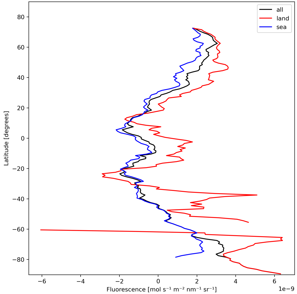
Figure 23: Zonal average of “Fluorescence” for 2024-02-04 to 2024-02-06.
