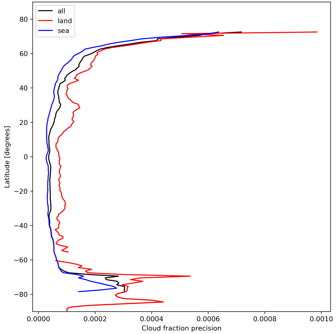
Figure 16: Zonal average of “Cloud fraction precision” for 2024-02-04 to 2024-02-06.
