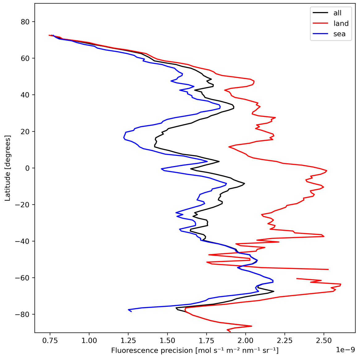
Figure 24: Zonal average of “Fluorescence precision” for 2024-02-04 to 2024-02-06.
