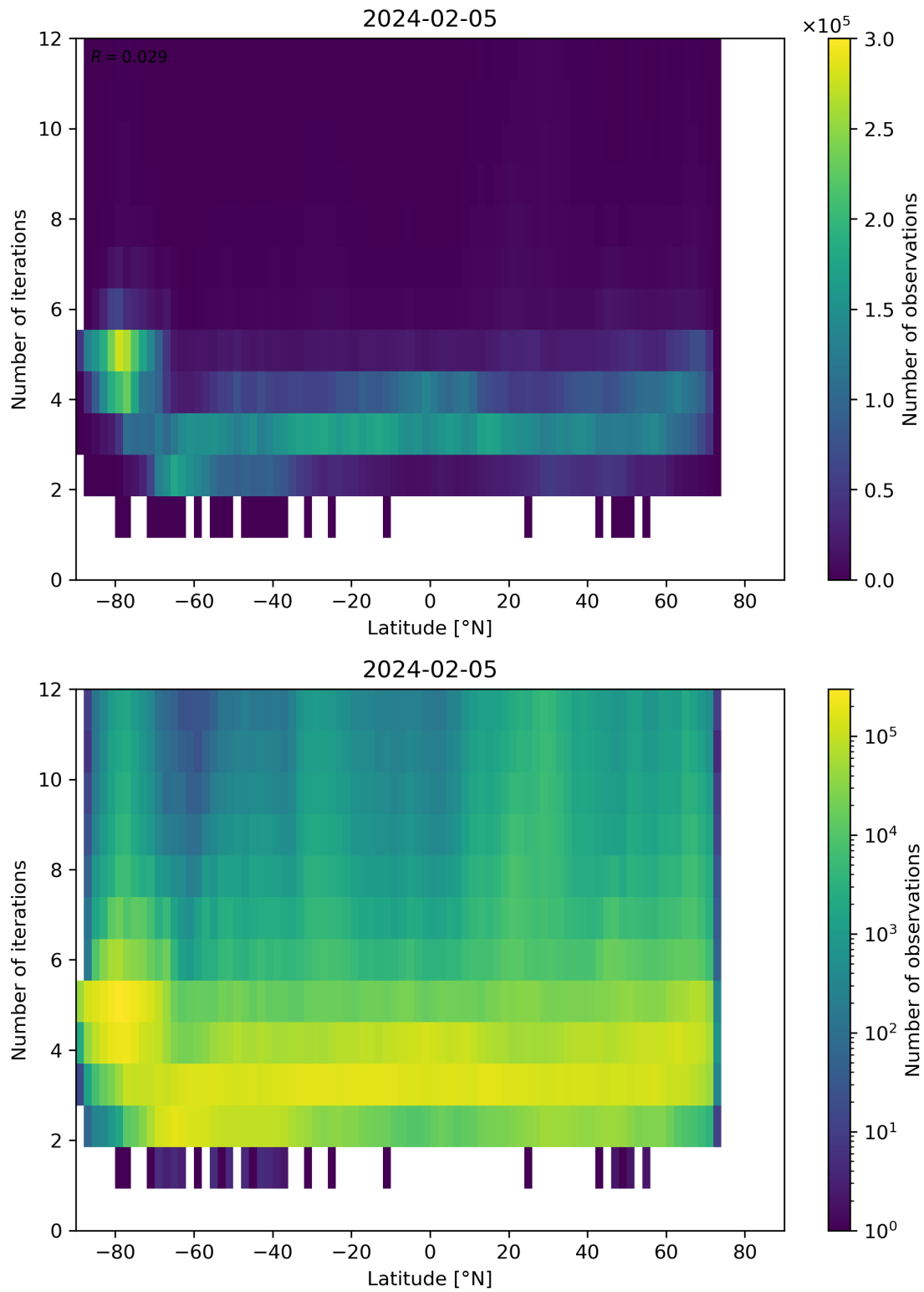
Figure 93: Scatter density plot of “Latitude” against “Number of iterations” for 2024-02-04 to 2024-02-06.
