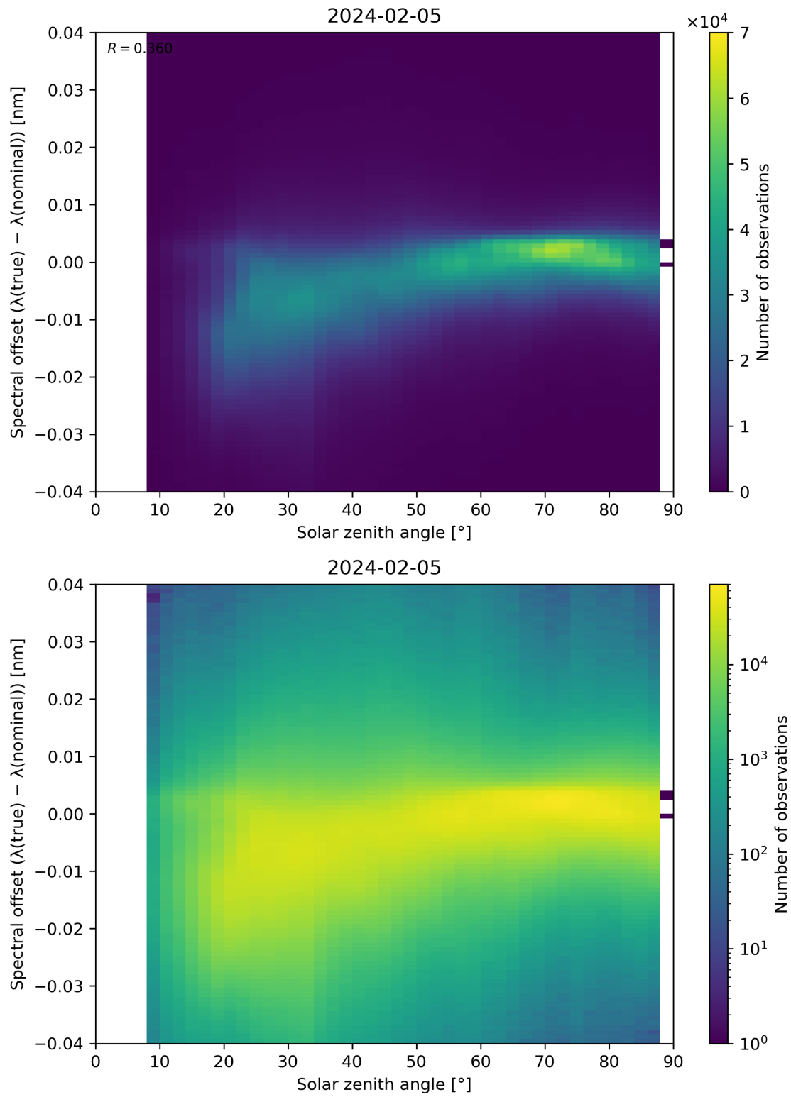
Figure 117: Scatter density plot of “Solar zenith angle” against “Spectral offset ( \lambda(\text{true}) - \lambda(\text{nominal}) )” for 2024-02-04 to 2024-02-06.
