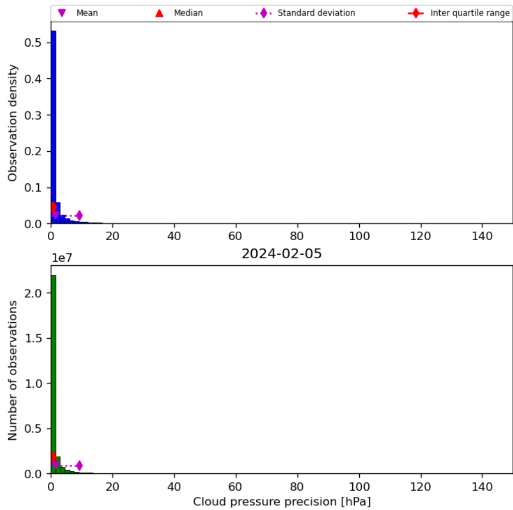
Figure 31: Histogram of “Cloud pressure precision” for 2024-02-04 to 2024-02-06
