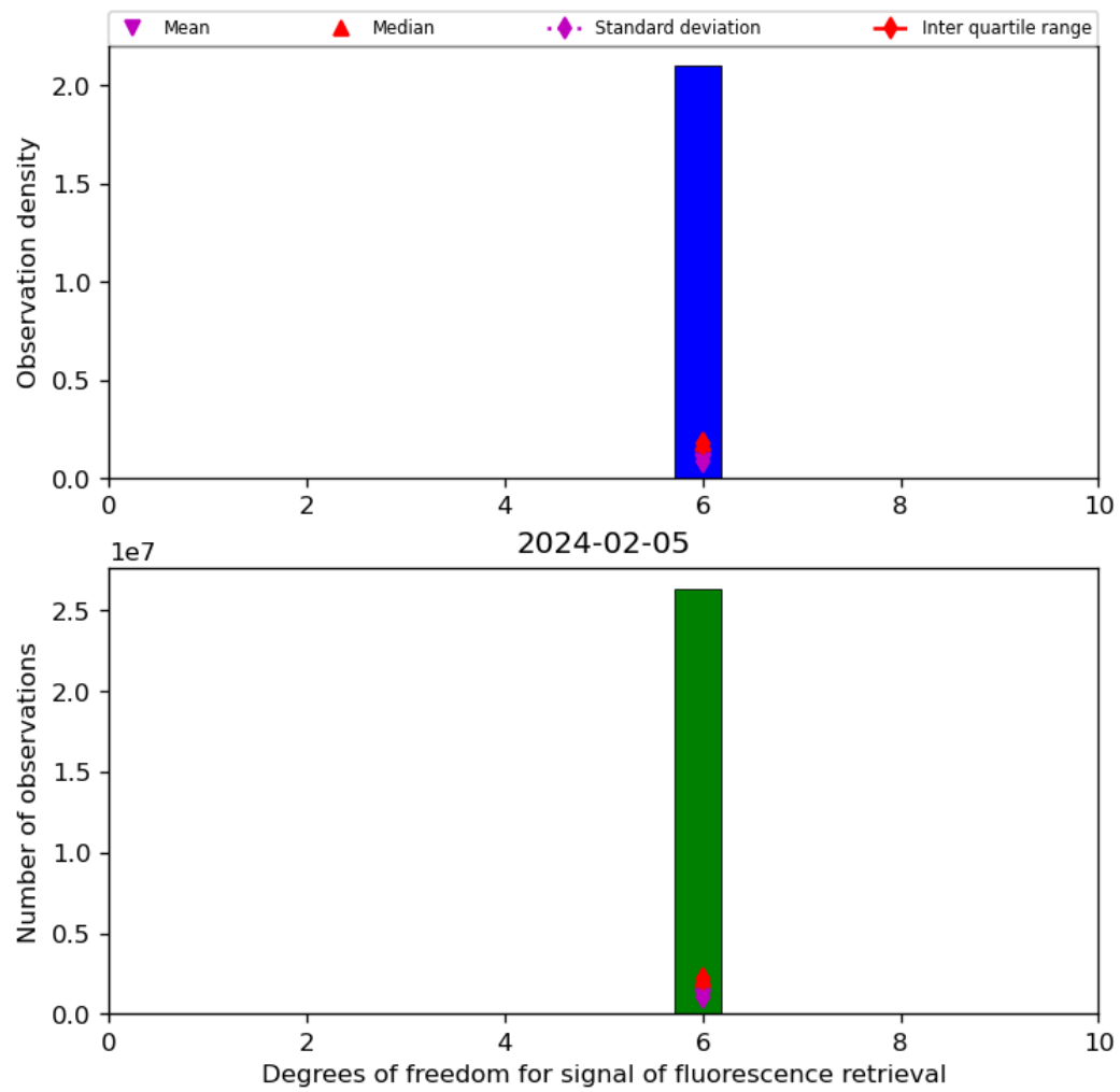
Figure 43: Histogram of “Degrees of freedom for signal of fluorescence retrieval” for 2024-02-04 to 2024-02-06
