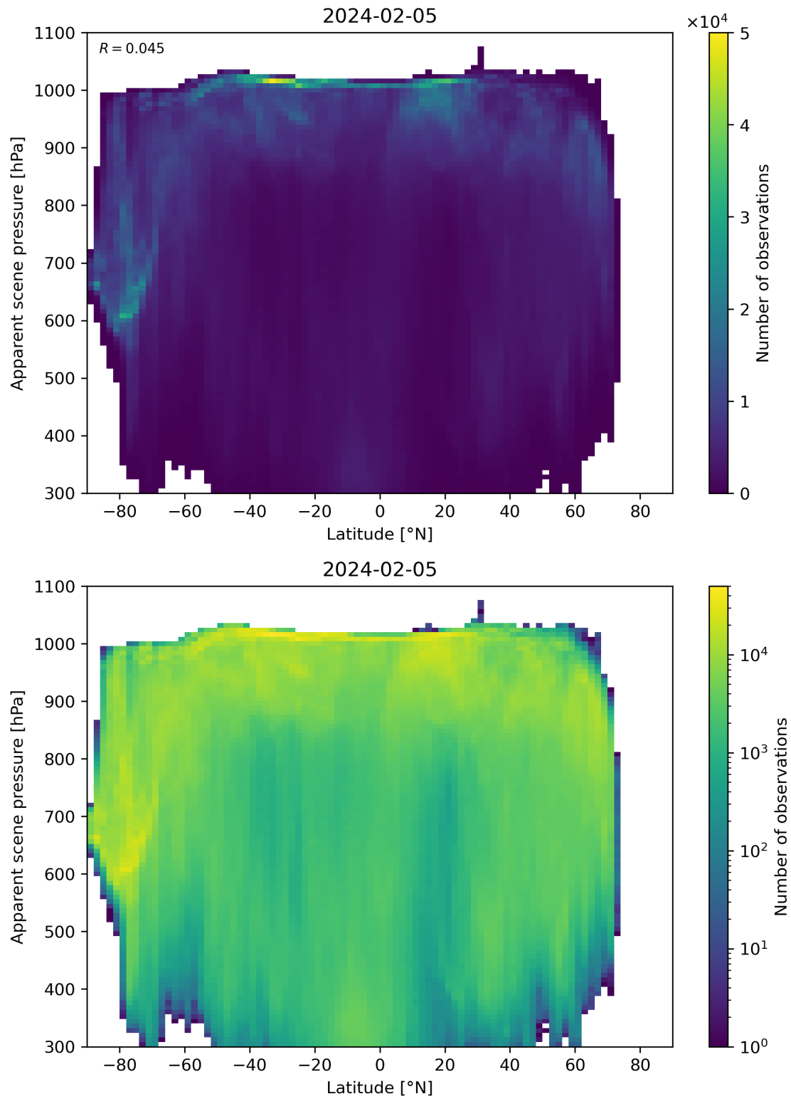
Figure 88: Scatter density plot of “Latitude” against “Apparent scene pressure” for 2024-02-04 to 2024-02-06.
