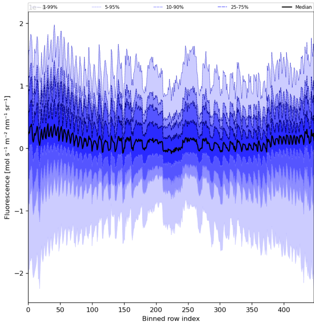
Figure 57: Along track statistics of “Fluorescence” for 2024-02-04 to 2024-02-06
