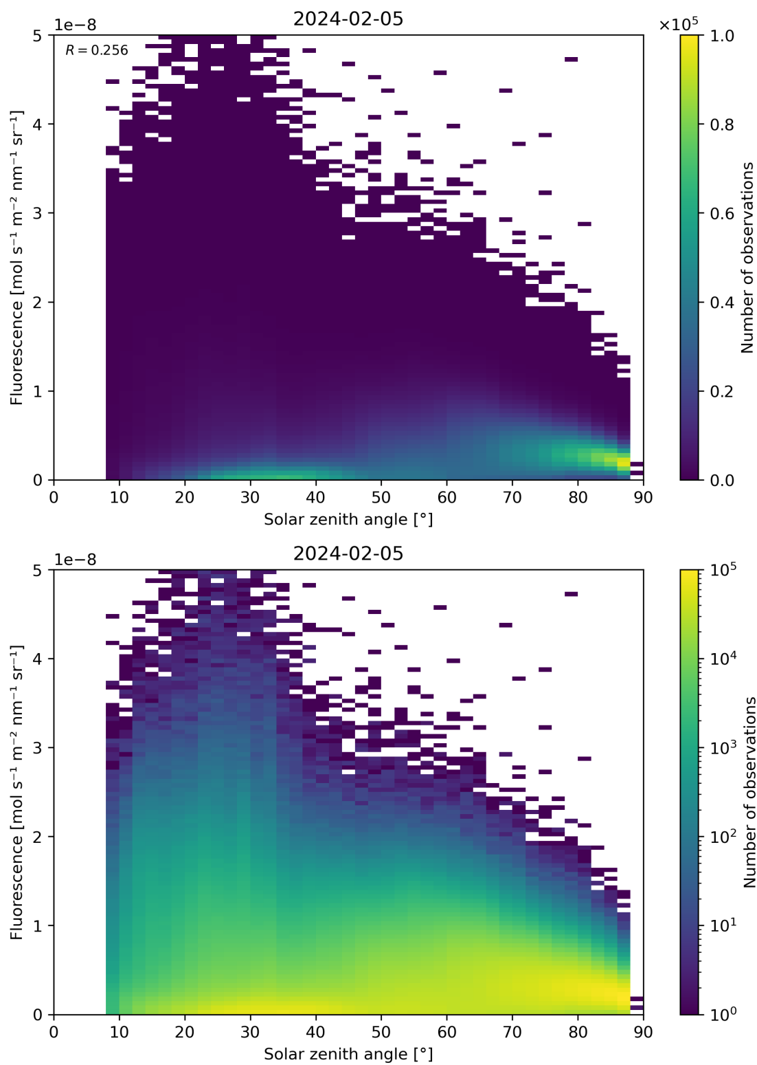
Figure 112: Scatter density plot of “Solar zenith angle” against “Fluorescence” for 2024-02-04 to 2024-02-06.
