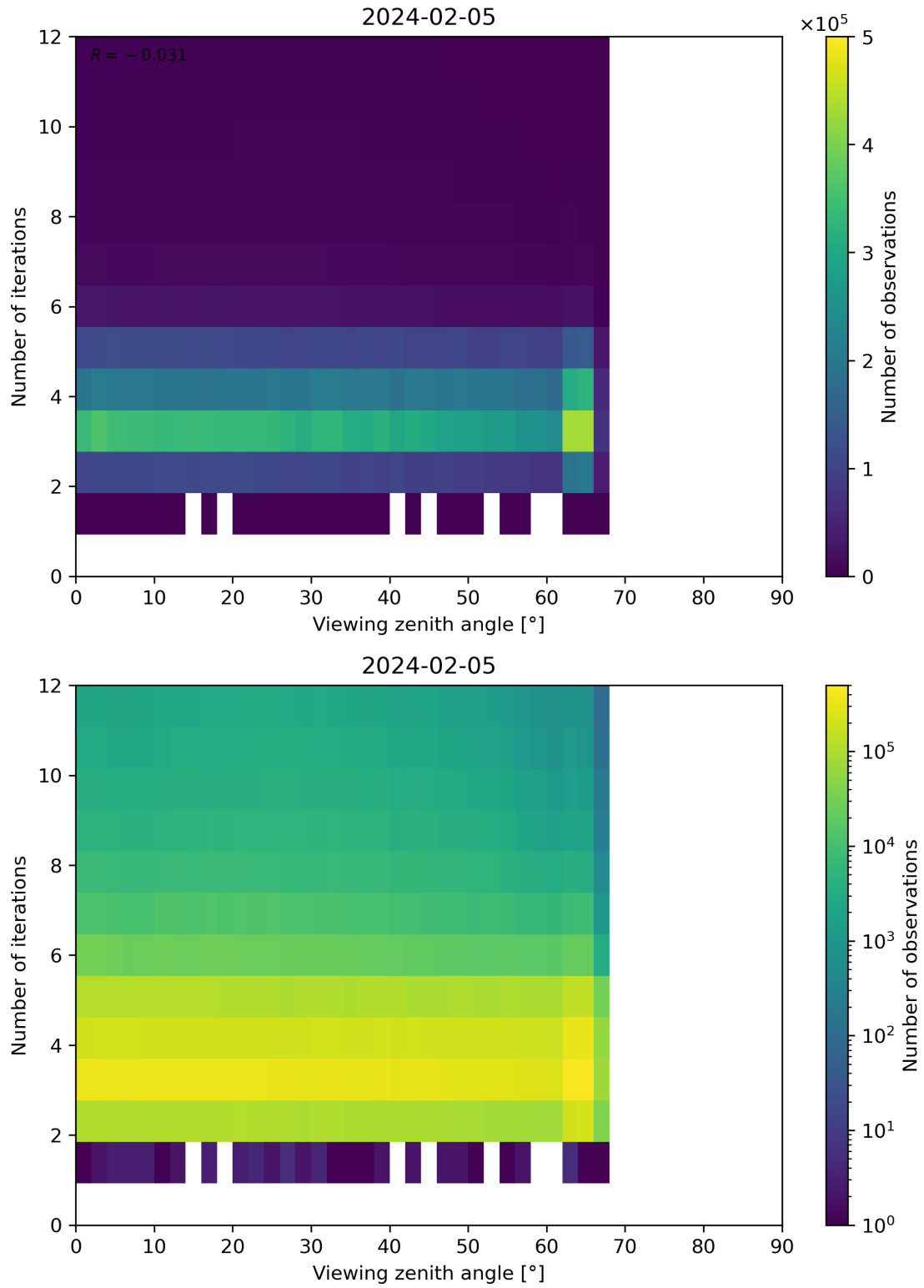
Figure 124: Scatter density plot of “Viewing zenith angle” against “Number of iterations” for 2024-02-04 to 2024-02-06.
