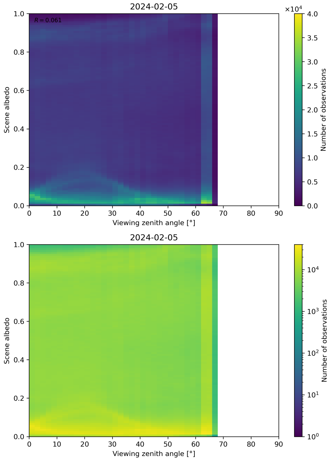
Figure 126: Scatter density plot of “Viewing zenith angle” against “Scene albedo” for 2024-02-04 to 2024-02-06.
