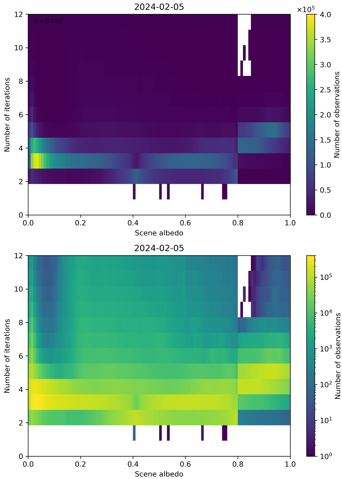
Figure 105: Scatter density plot of “Scene albedo” against “Number of iterations” for 2024-02-04 to 2024-02-06.
