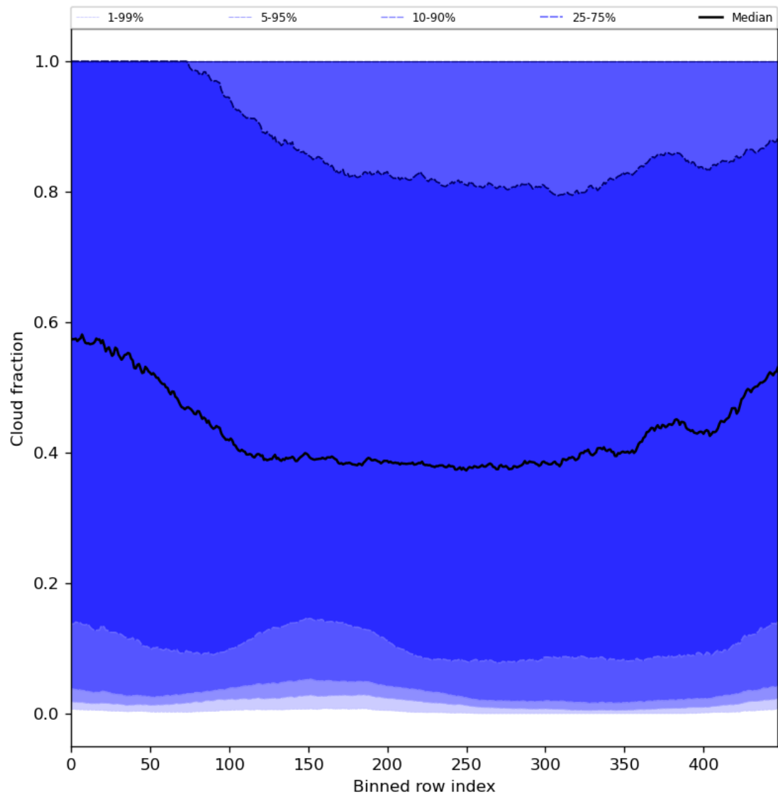
Figure 49: Along track statistics of “Cloud fraction” for 2024-02-04 to 2024-02-06
