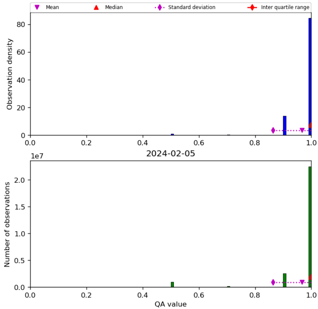
Figure 29: Histogram of “QA value” for 2024-02-04 to 2024-02-06
