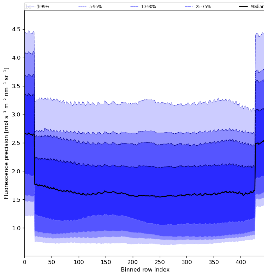
Figure 58: Along track statistics of “Fluorescence precision” for 2024-02-04 to 2024-02-06
