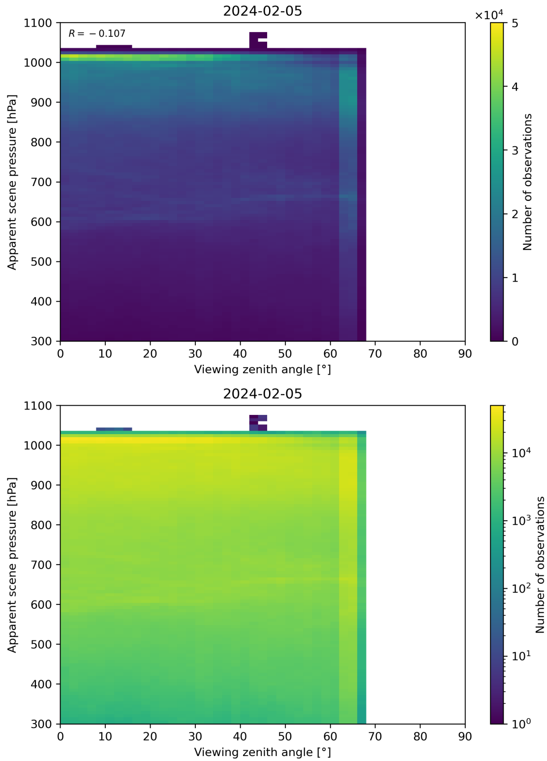
Figure 118: Scatter density plot of “Viewing zenith angle” against “Apparent scene pressure” for 2024-02-04 to 2024-02-06.
