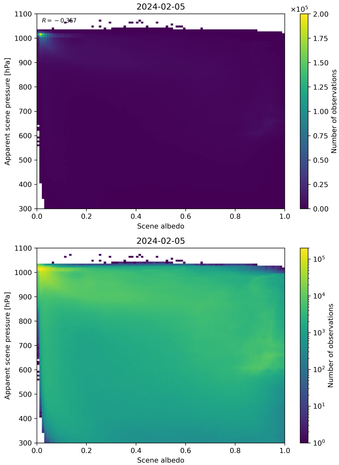
Figure 102: Scatter density plot of “Scene albedo” against “Apparent scene pressure” for 2024-02-04 to 2024-02-06.
