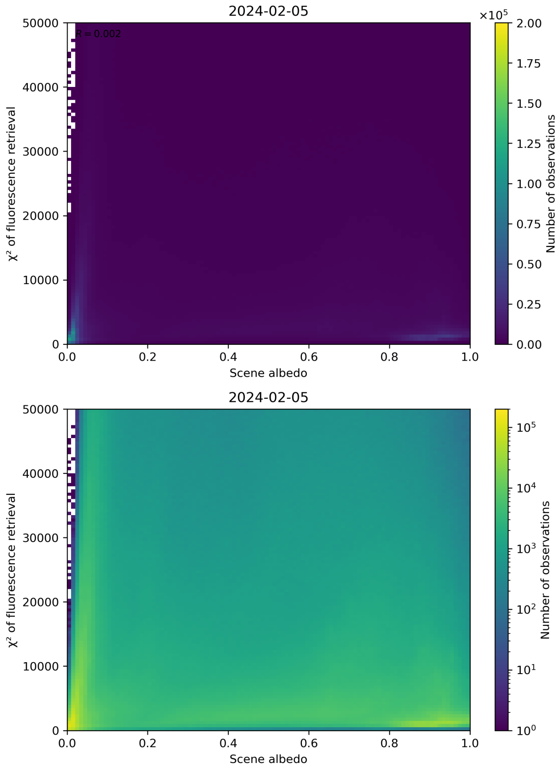
Figure 103: Scatter density plot of “Scene albedo” against “ \chi^2 of fluorescence retrieval” for 2024-02-04 to 2024-02-06.
