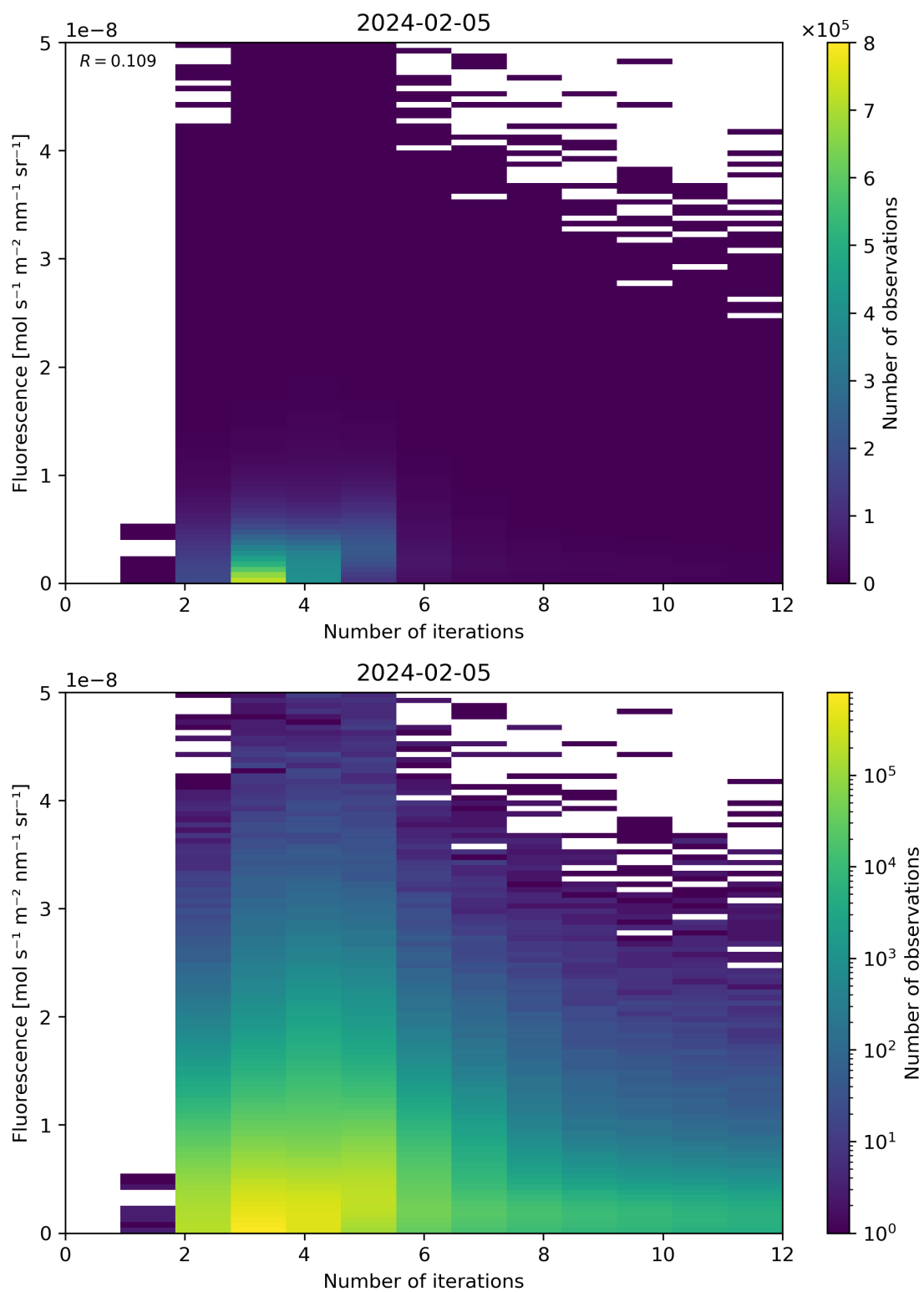
Figure 98: Scatter density plot of “Number of iterations” against “Fluorescence” for 2024-02-04 to 2024-02-06.
