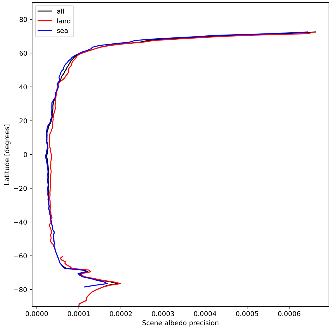
Figure 18: Zonal average of “Scene albedo precision” for 2024-02-04 to 2024-02-06.
