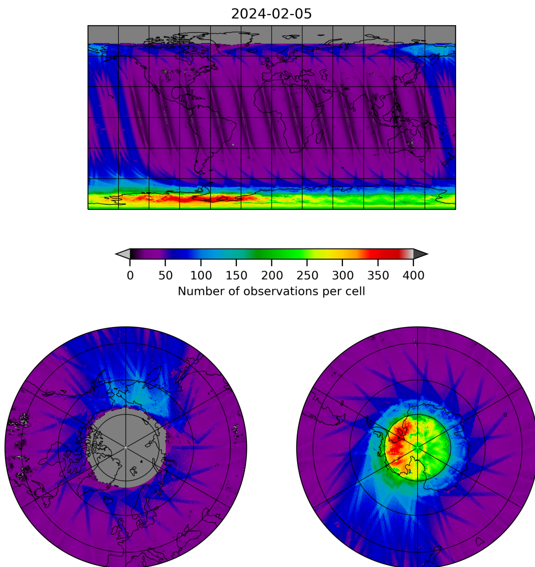
Figure 11: Map of the number of observations for 2024-02-04 to 2024-02-06
