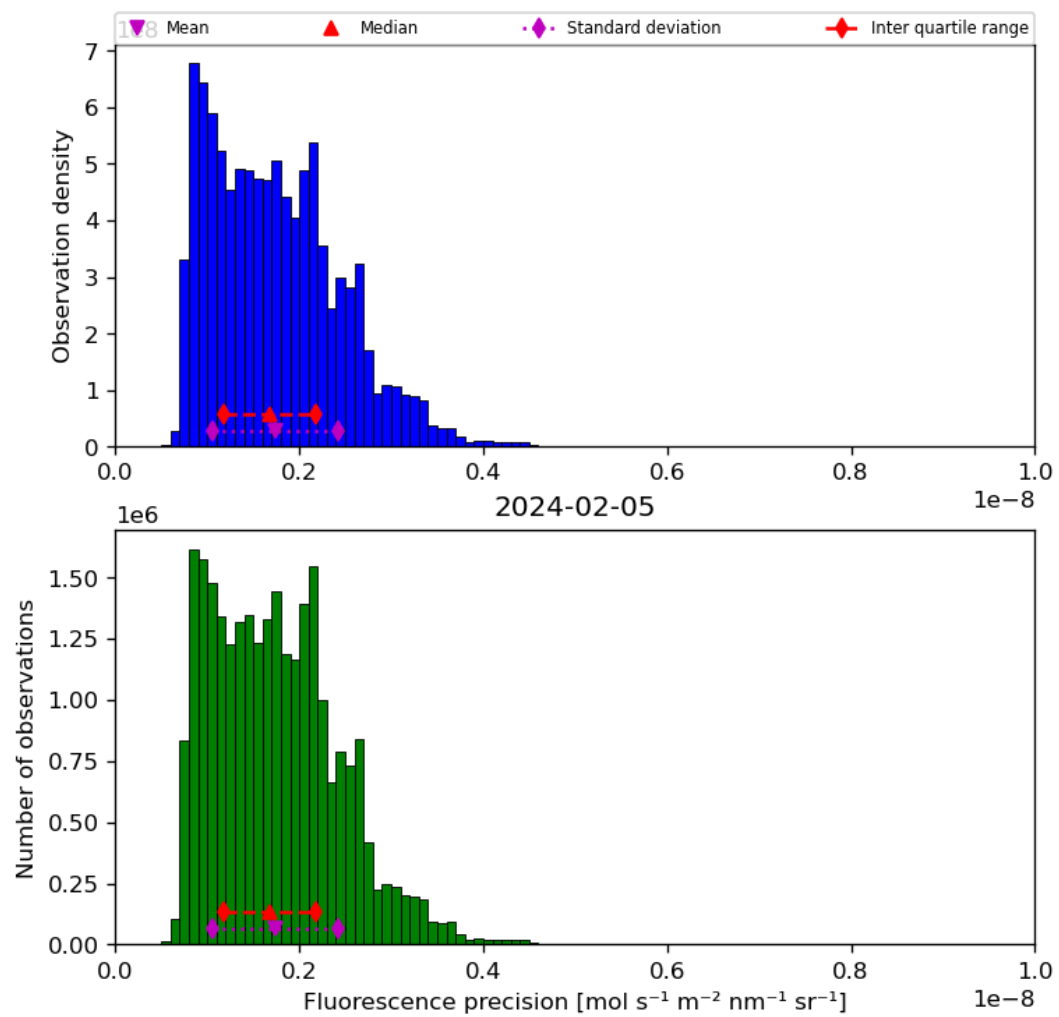
Figure 41: Histogram of “Fluorescence precision” for 2024-02-04 to 2024-02-06
