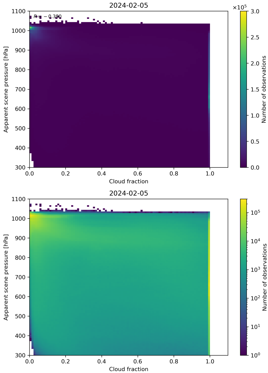
Figure 70: Scatter density plot of “Cloud fraction” against “Apparent scene pressure” for 2024-02-04 to 2024-02-06.
