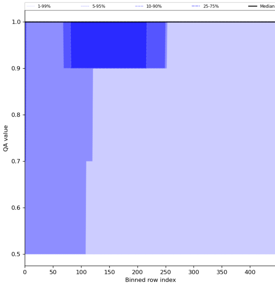
Figure 46: Along track statistics of “QA value” for 2024-02-04 to 2024-02-06
