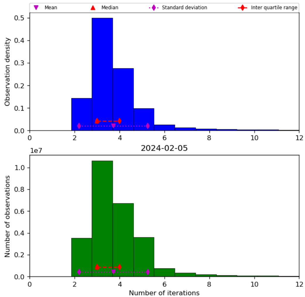
Figure 39: Histogram of “Number of iterations” for 2024-02-04 to 2024-02-06
