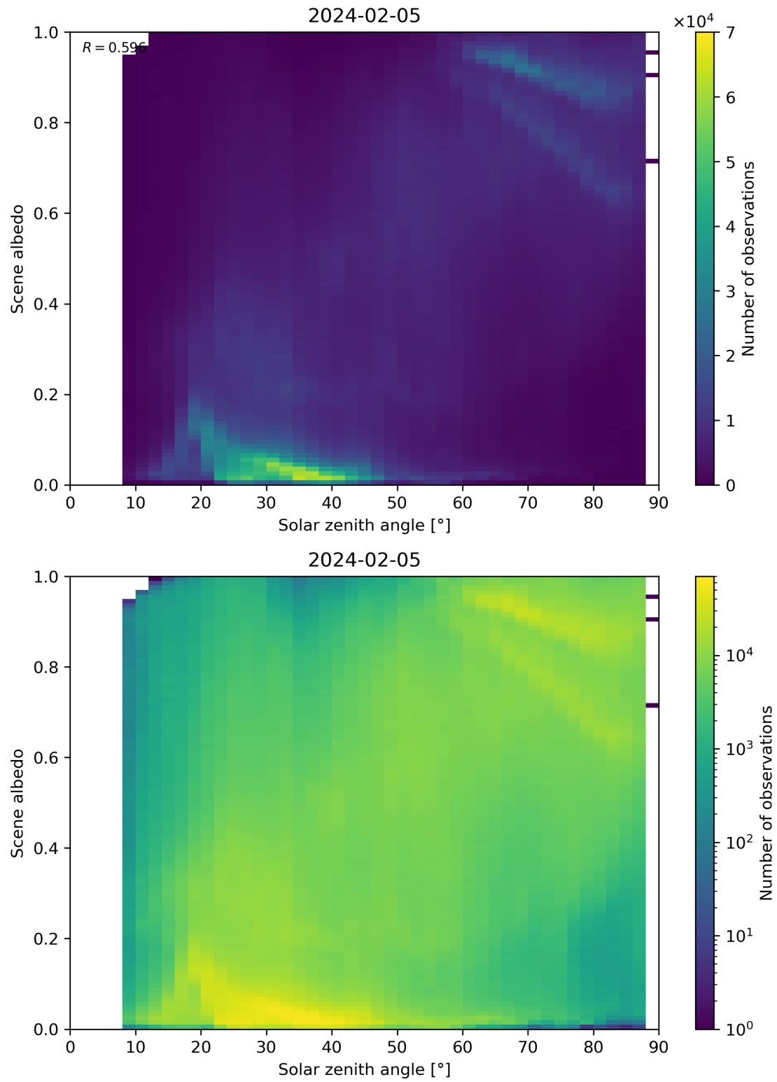
Figure 116: Scatter density plot of “Solar zenith angle” against “Scene albedo” for 2024-02-04 to 2024-02-06.
