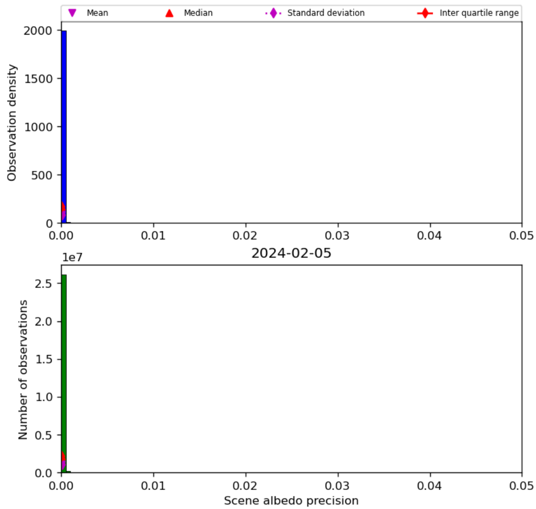
Figure 35: Histogram of “Scene albedo precision” for 2024-02-04 to 2024-02-06
