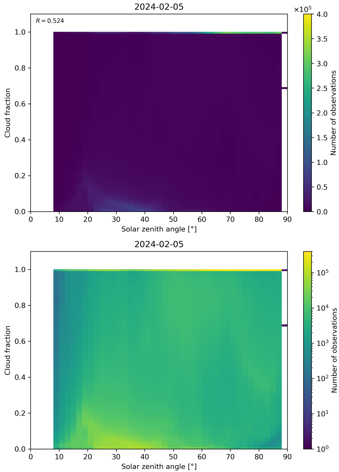
Figure 110: Scatter density plot of “Solar zenith angle” against “Cloud fraction” for 2024-02-04 to 2024-02-06.
