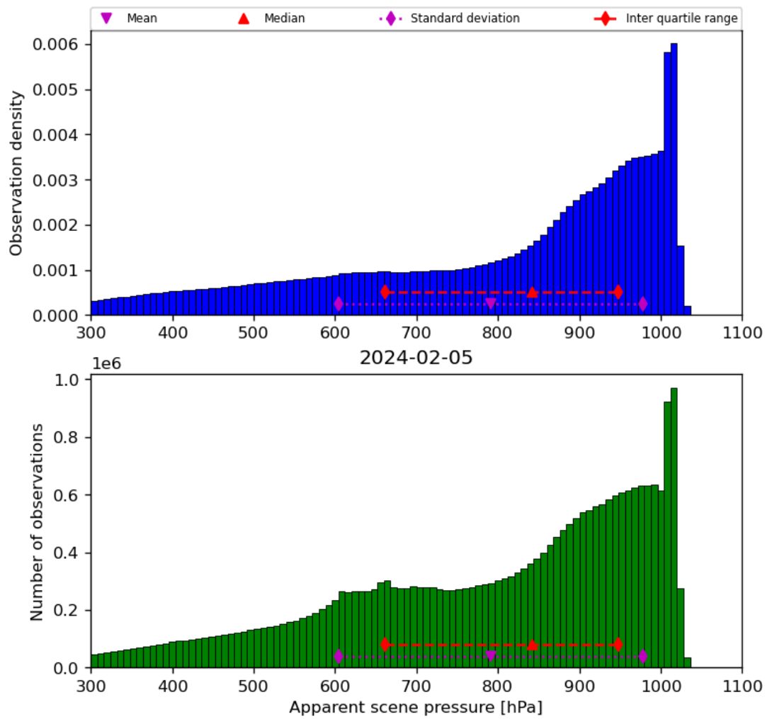
Figure 36: Histogram of “Apparent scene pressure” for 2024-02-04 to 2024-02-06
