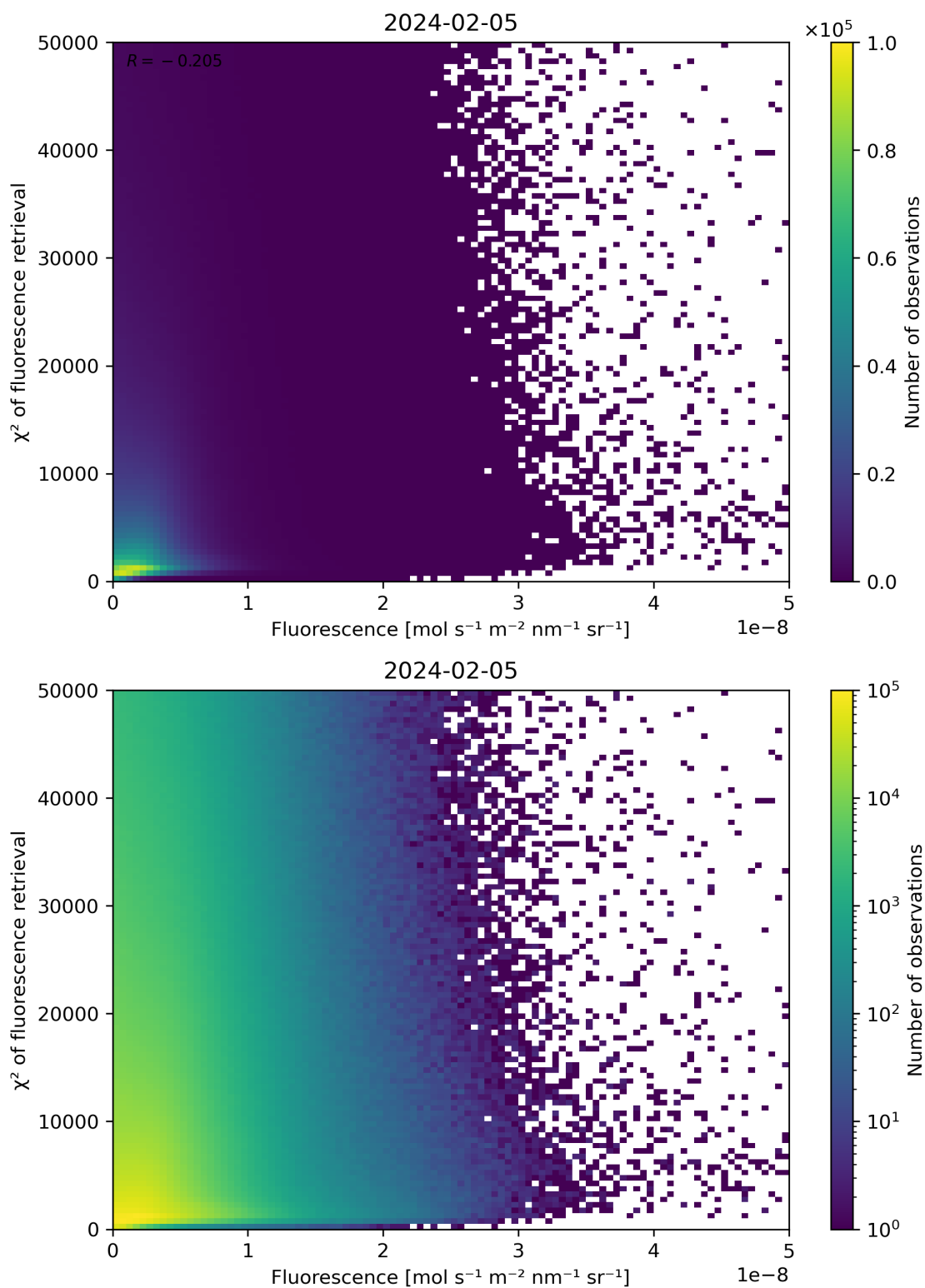
Figure 85: Scatter density plot of “Fluorescence” against “ \chi^2 of fluorescence retrieval” for 2024-02-04 to 2024-02-06.
