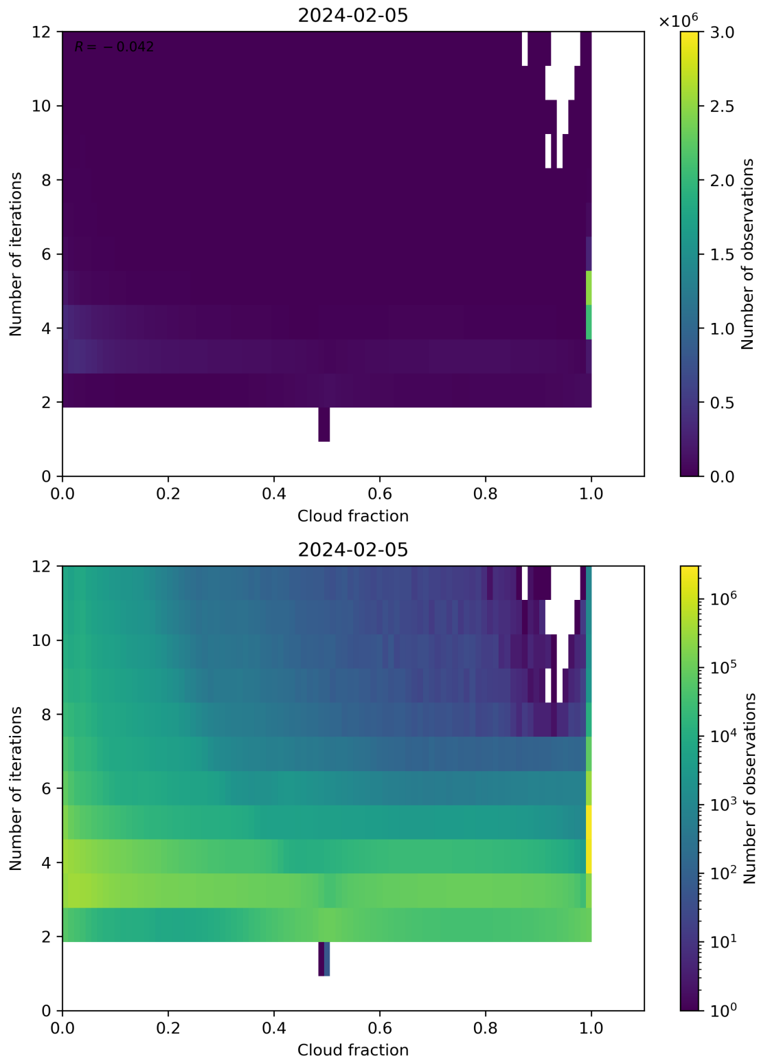
Figure 73: Scatter density plot of “Cloud fraction” against “Number of iterations” for 2024-02-04 to 2024-02-06.
