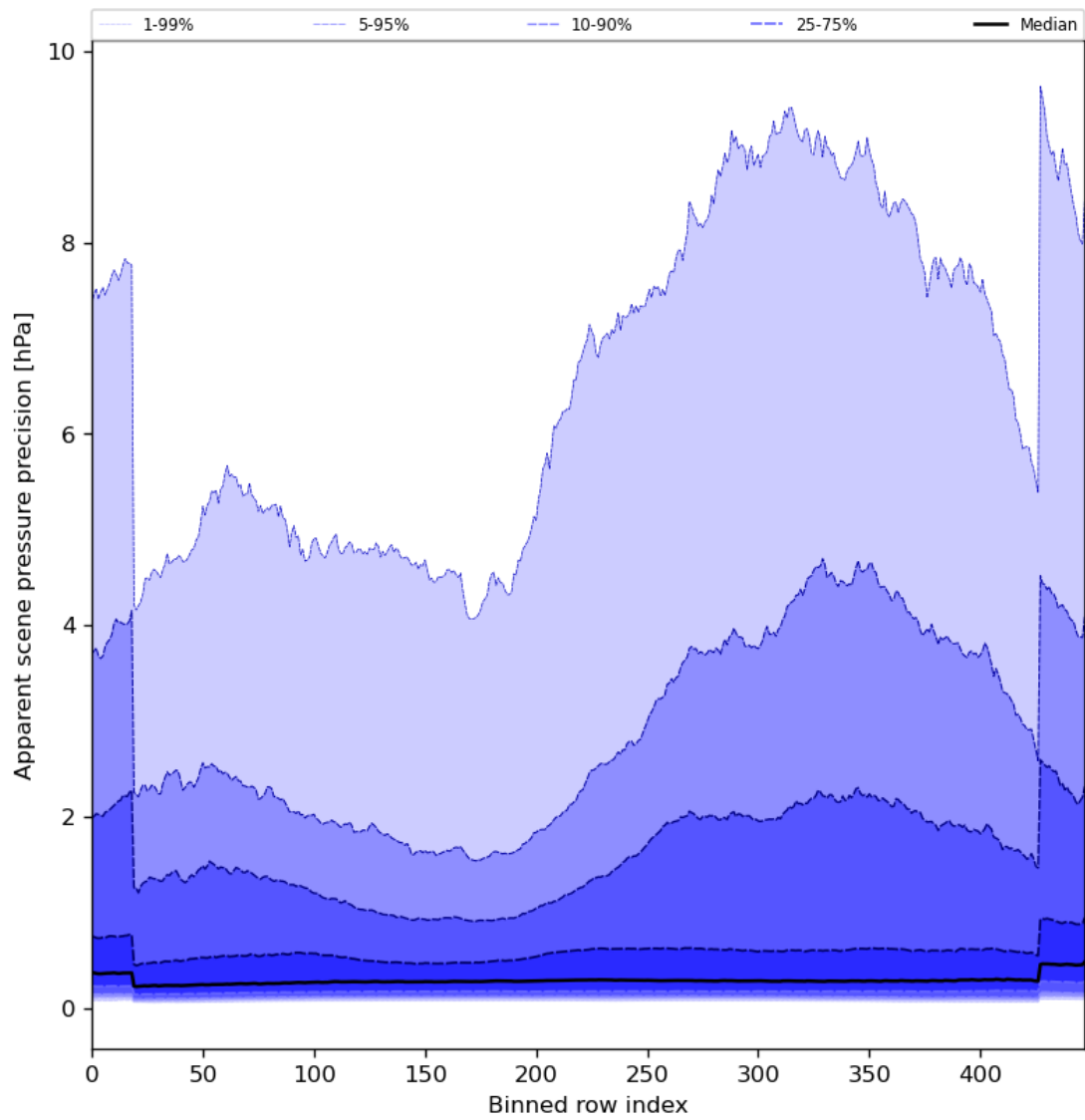
Figure 54: Along track statistics of “Apparent scene pressure precision” for 2024-02-04 to 2024-02-06
