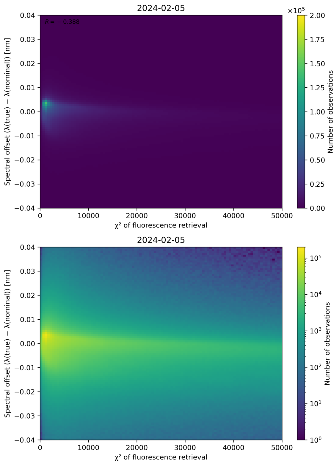
Figure 69: Scatter density plot of " \chi^2 of fluorescence retrieval" against "Spectral offset ( \lambda(\text{true}) - \lambda(\text{nominal})) " for 2024-02-04 to 2024-02-06.
