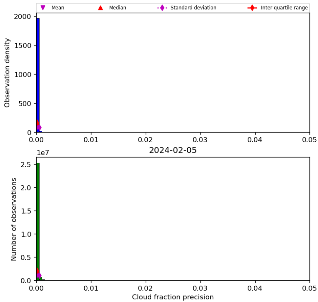
Figure 33: Histogram of “Cloud fraction precision” for 2024-02-04 to 2024-02-06
