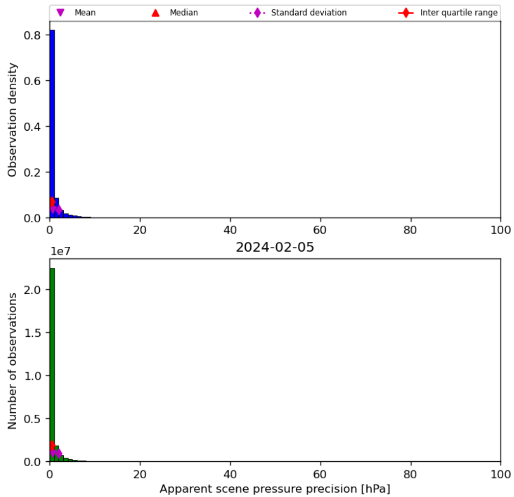
Figure 37: Histogram of “Apparent scene pressure precision” for 2024-02-04 to 2024-02-06
