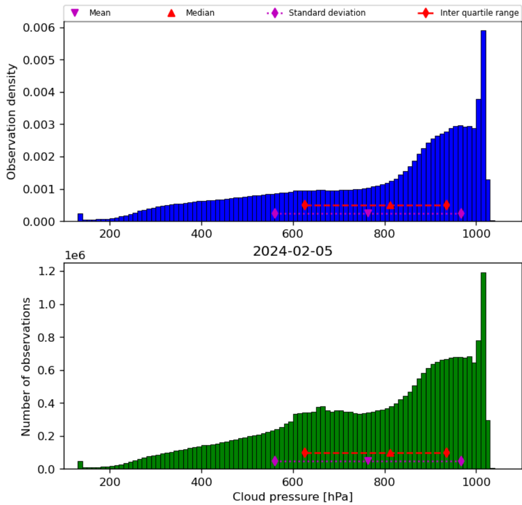
Figure 30: Histogram of “Cloud pressure” for 2024-02-04 to 2024-02-06
