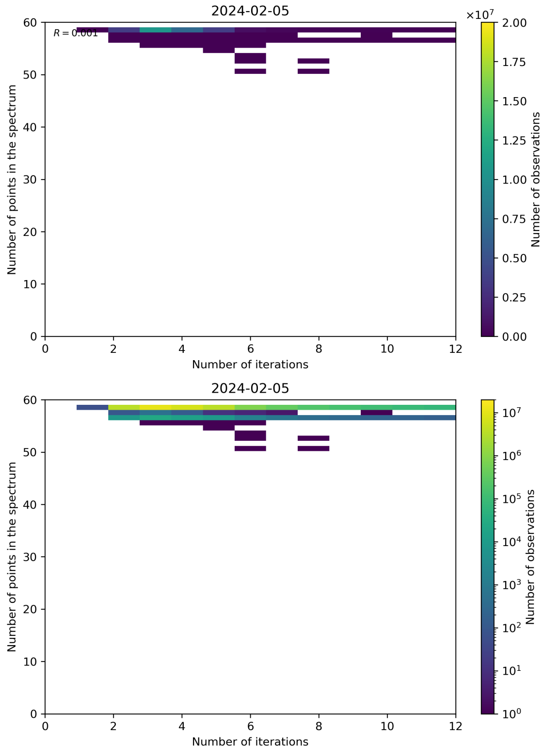
Figure 99: Scatter density plot of “Number of iterations” against “Number of points in the spectrum” for 2024-02-04 to 2024-02-06.
