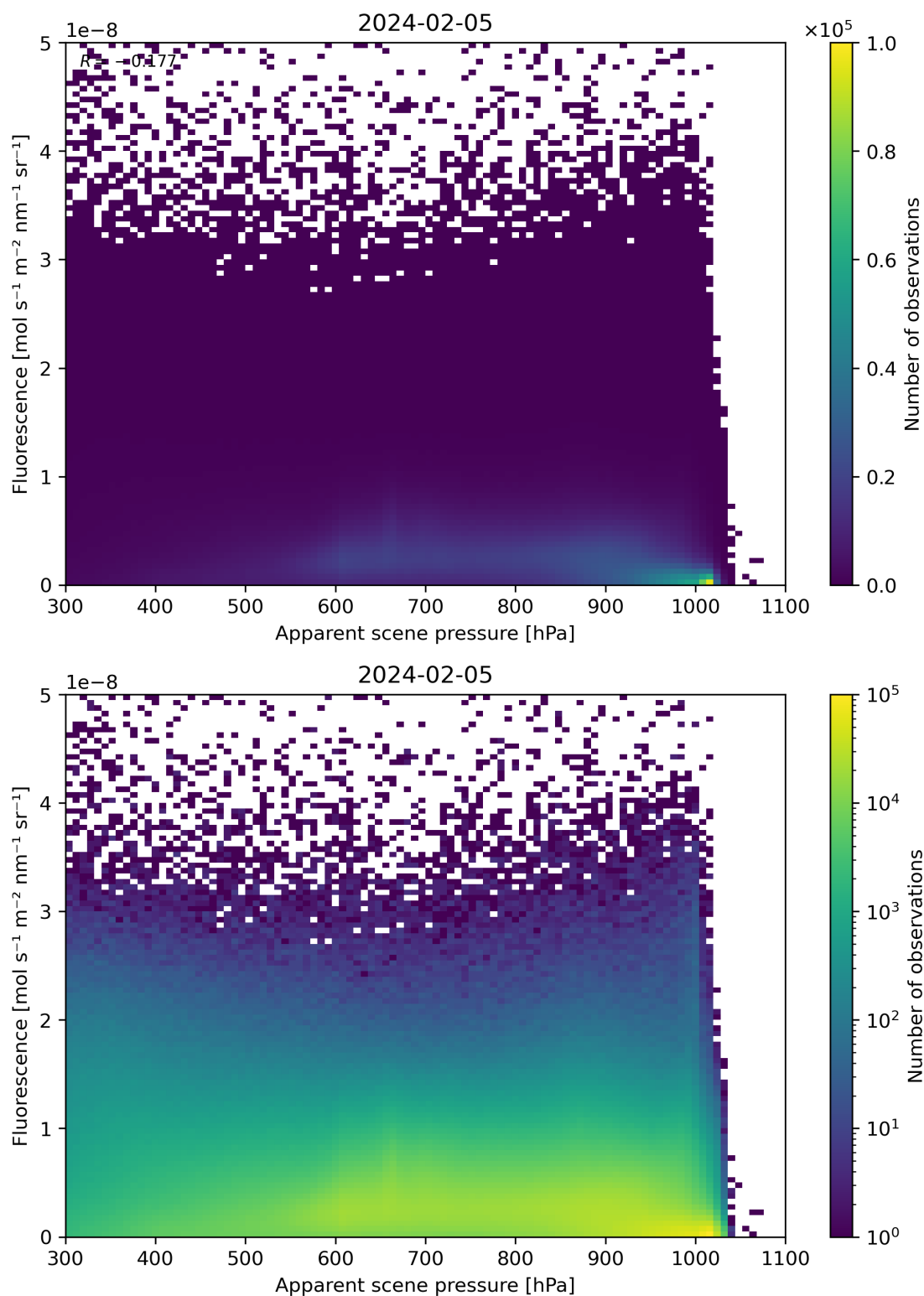
Figure 64: Scatter density plot of “Apparent scene pressure” against “Fluorescence” for 2024-02-04 to 2024-02-06.
