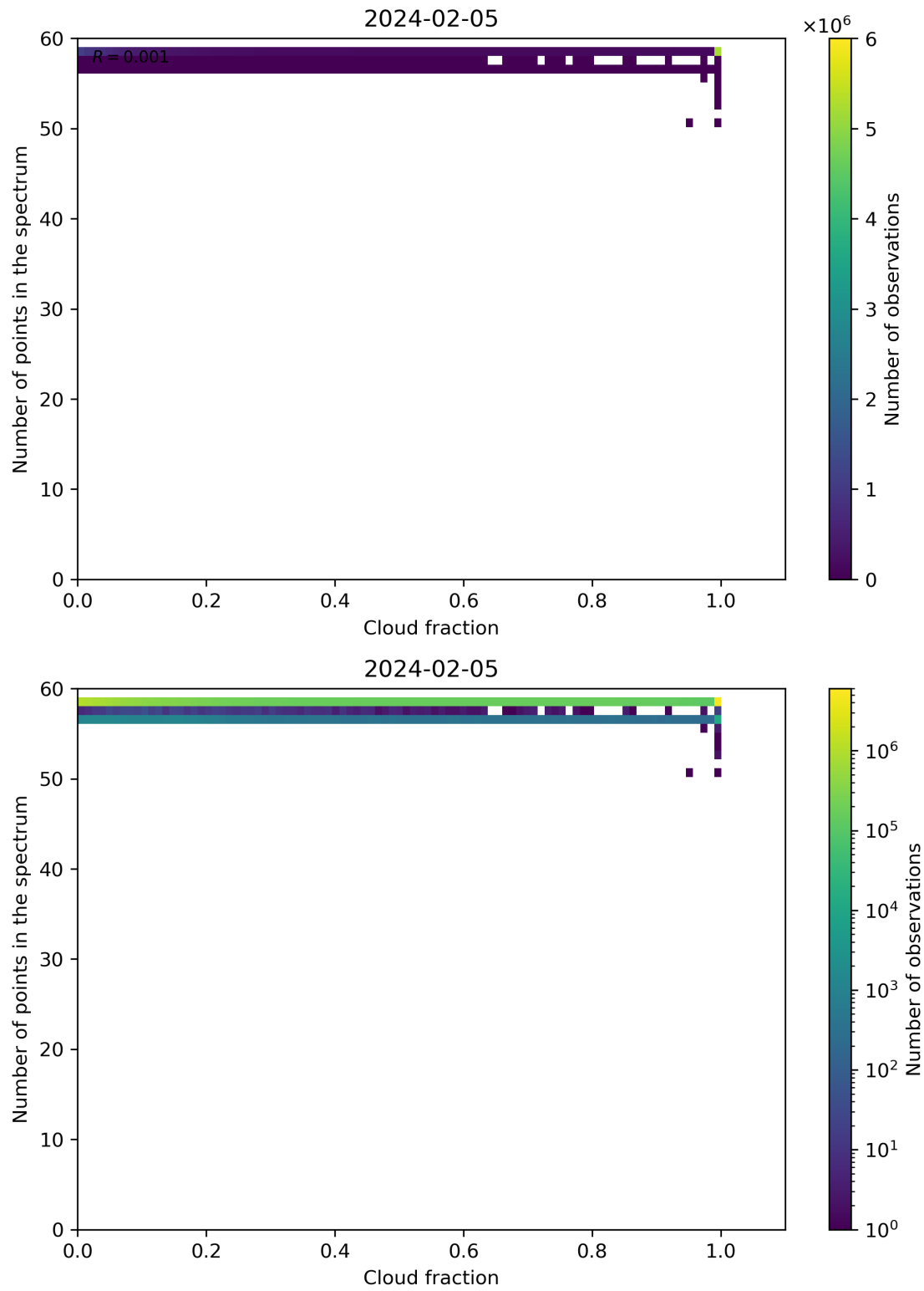
Figure 74: Scatter density plot of “Cloud fraction” against “Number of points in the spectrum” for 2024-02-04 to 2024-02-06.
