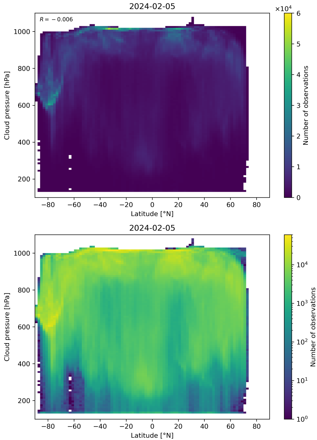
Figure 91: Scatter density plot of “Latitude” against “Cloud pressure” for 2024-02-04 to 2024-02-06.
