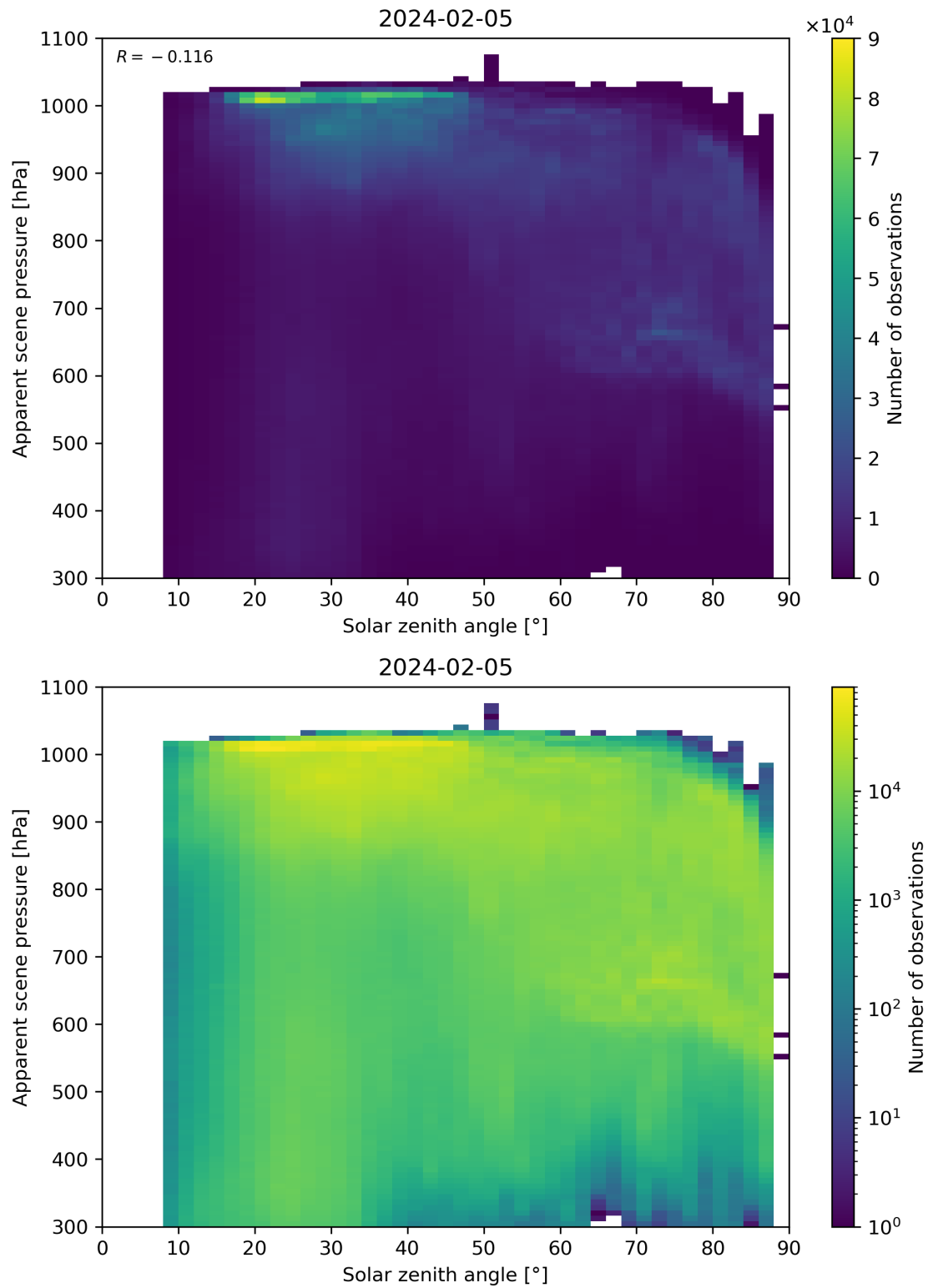
Figure 108: Scatter density plot of “Solar zenith angle” against “Apparent scene pressure” for 2024-02-04 to 2024-02-06.
