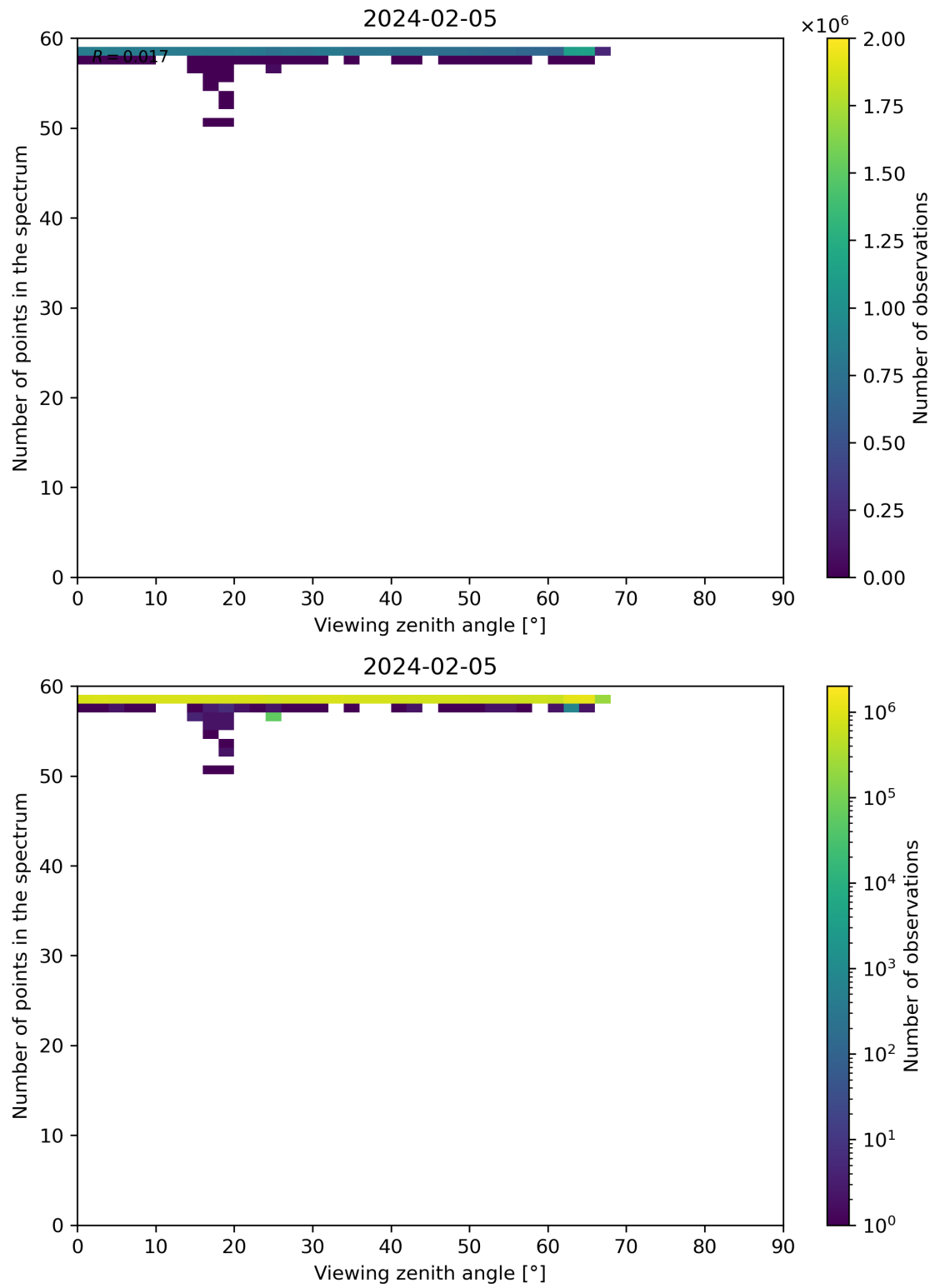
Figure 125: Scatter density plot of “Viewing zenith angle” against “Number of points in the spectrum” for 2024-02-04 to 2024-02-06.
