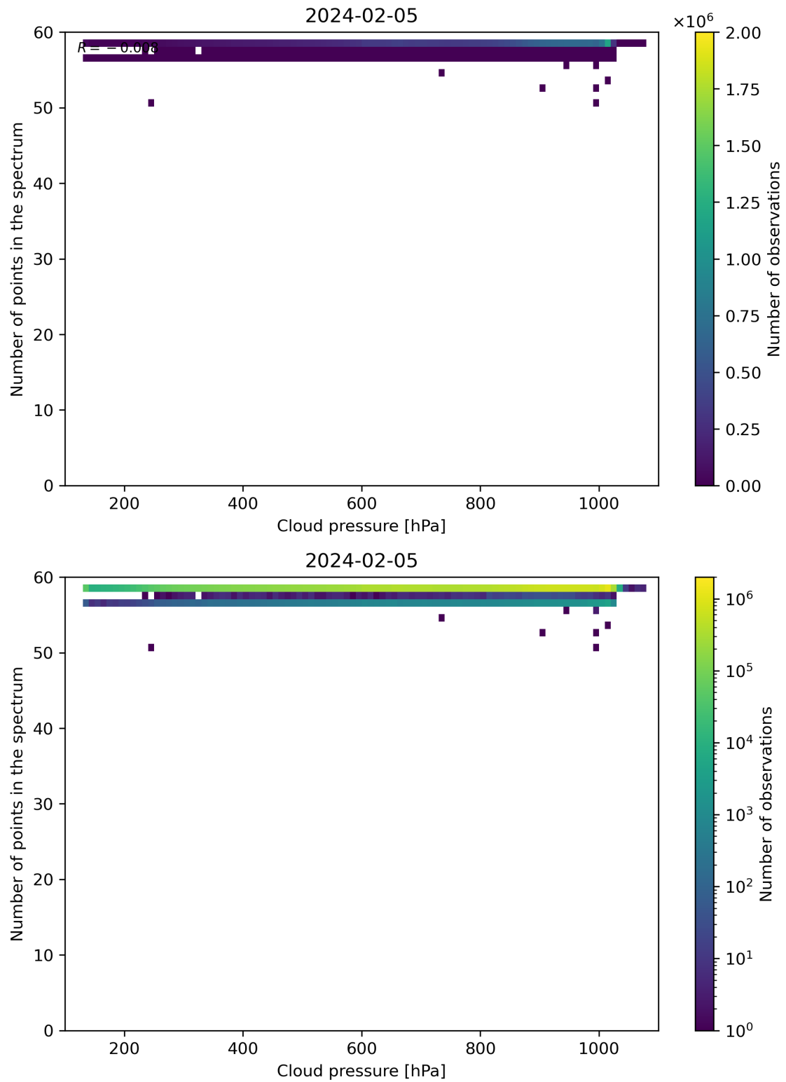
Figure 82: Scatter density plot of “Cloud pressure” against “Number of points in the spectrum” for 2024-02-04 to 2024-02-06.
