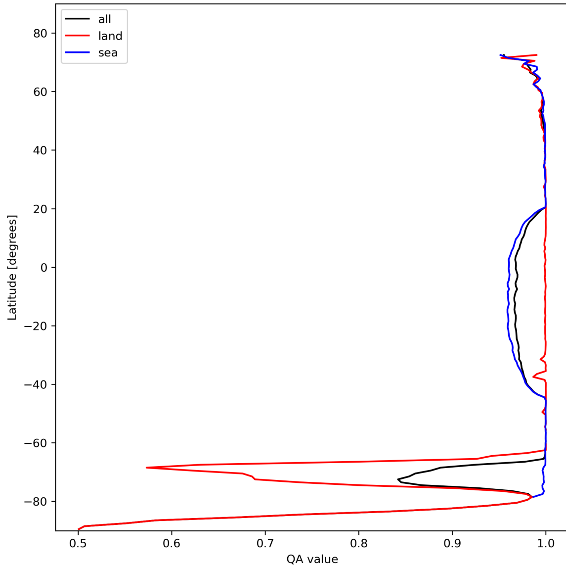
Figure 12: Zonal average of “QA value” for 2024-02-04 to 2024-02-06.
