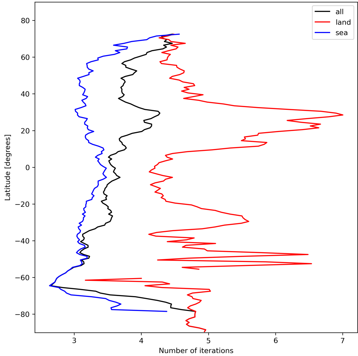
Figure 22: Zonal average of “Number of iterations” for 2024-02-04 to 2024-02-06.
