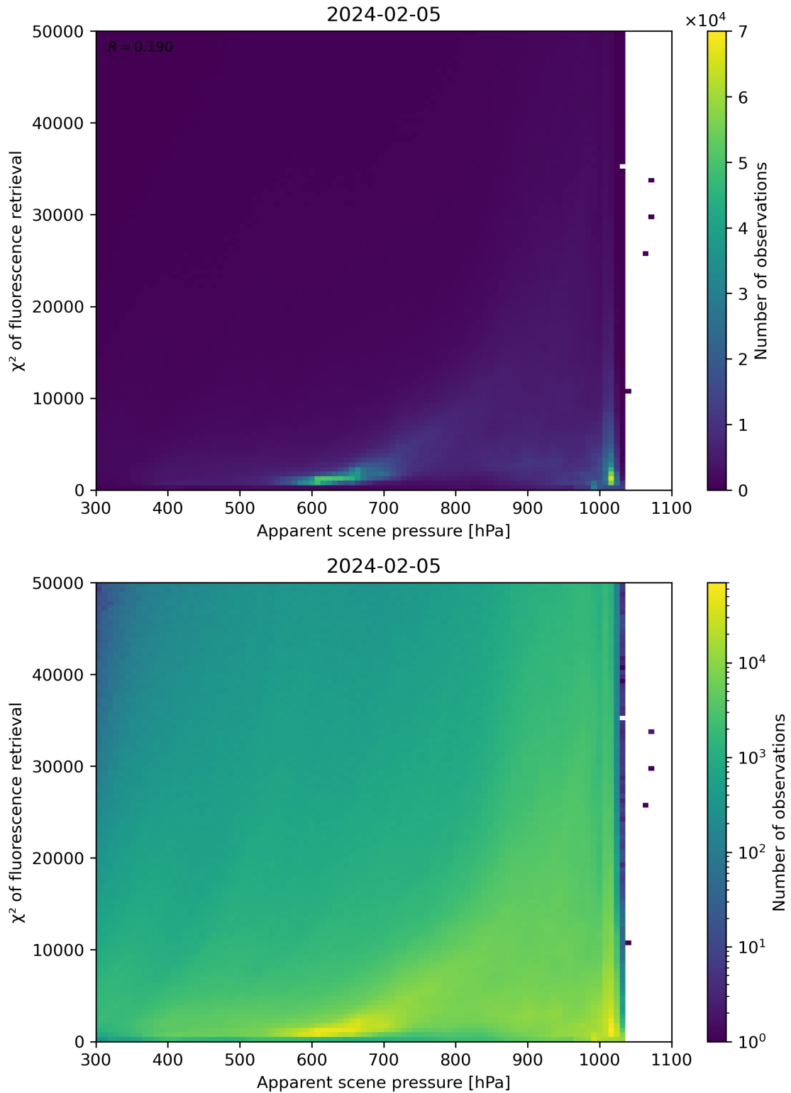
Figure 63: Scatter density plot of “Apparent scene pressure” against “ \chi^2 of fluorescence retrieval” for 2024-02-04 to 2024-02-06.
