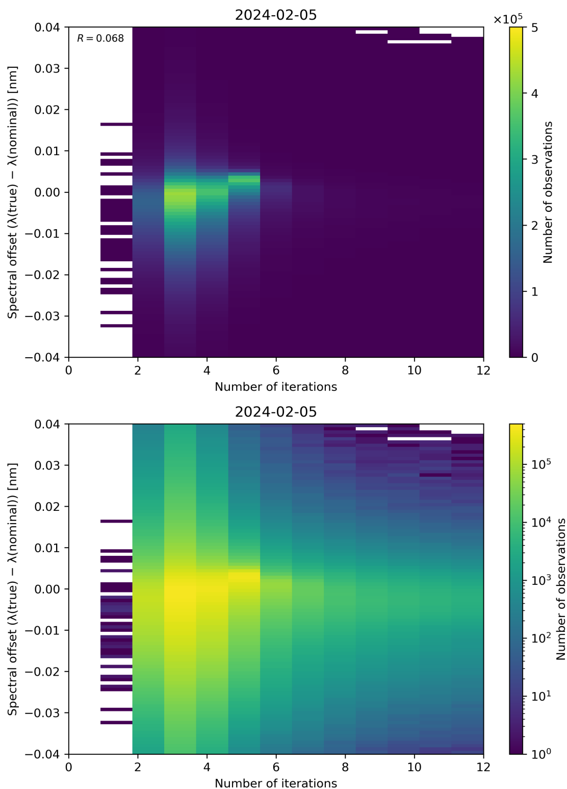
Figure 100: Scatter density plot of “Number of iterations” against “Spectral offset ( \lambda(\text{true}) - \lambda(\text{nominal}) )” for 2024-02-04 to 2024-02-06.
