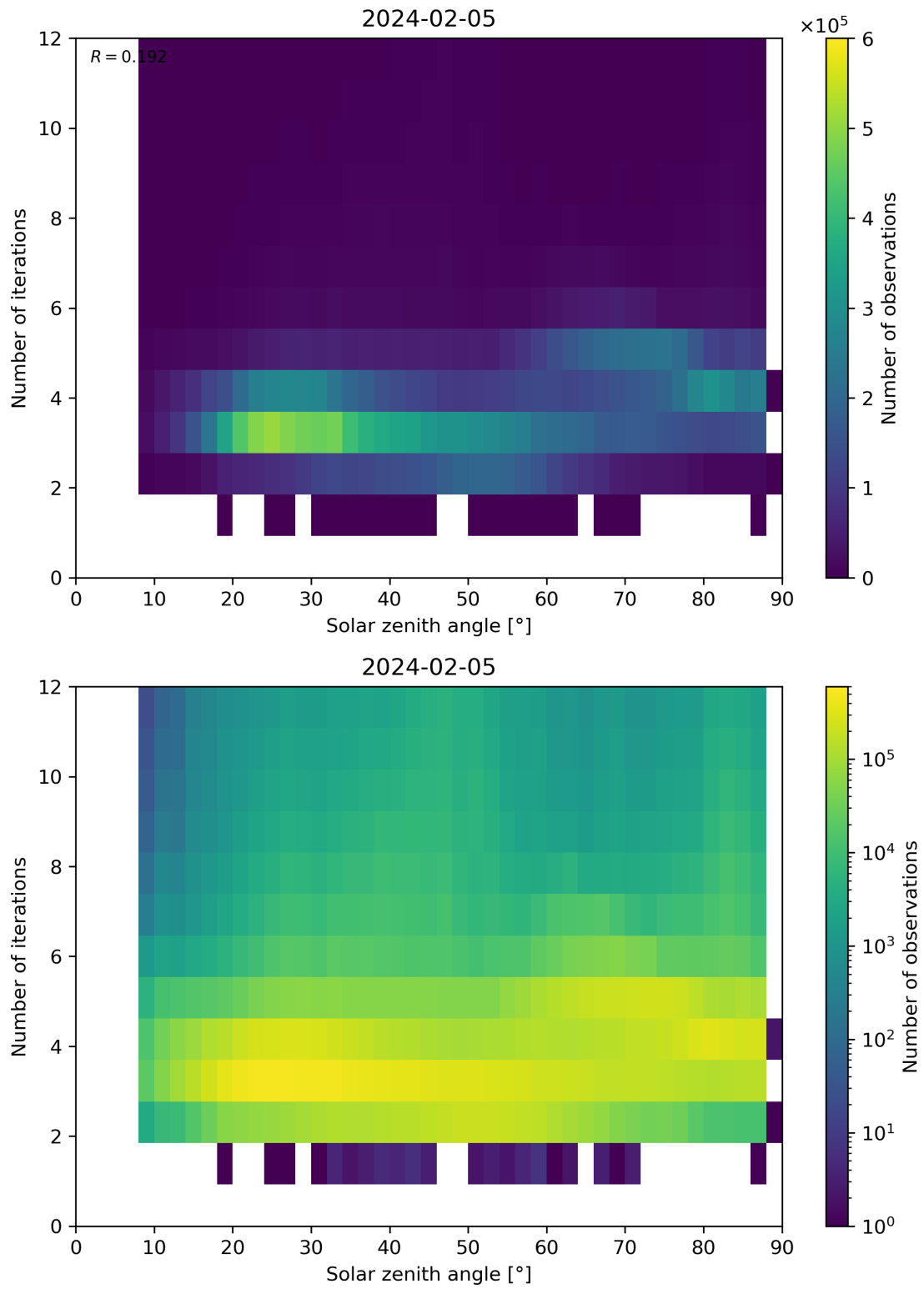
Figure 114: Scatter density plot of “Solar zenith angle” against “Number of iterations” for 2024-02-04 to 2024-02-06.
