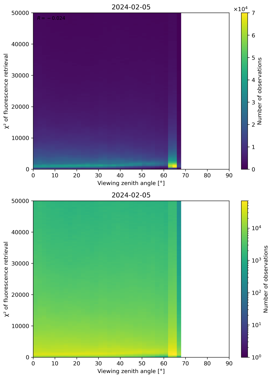
Figure 119: Scatter density plot of “Viewing zenith angle” against “ \chi^2 of fluorescence retrieval” for 2024-02-04 to 2024-02-06.
