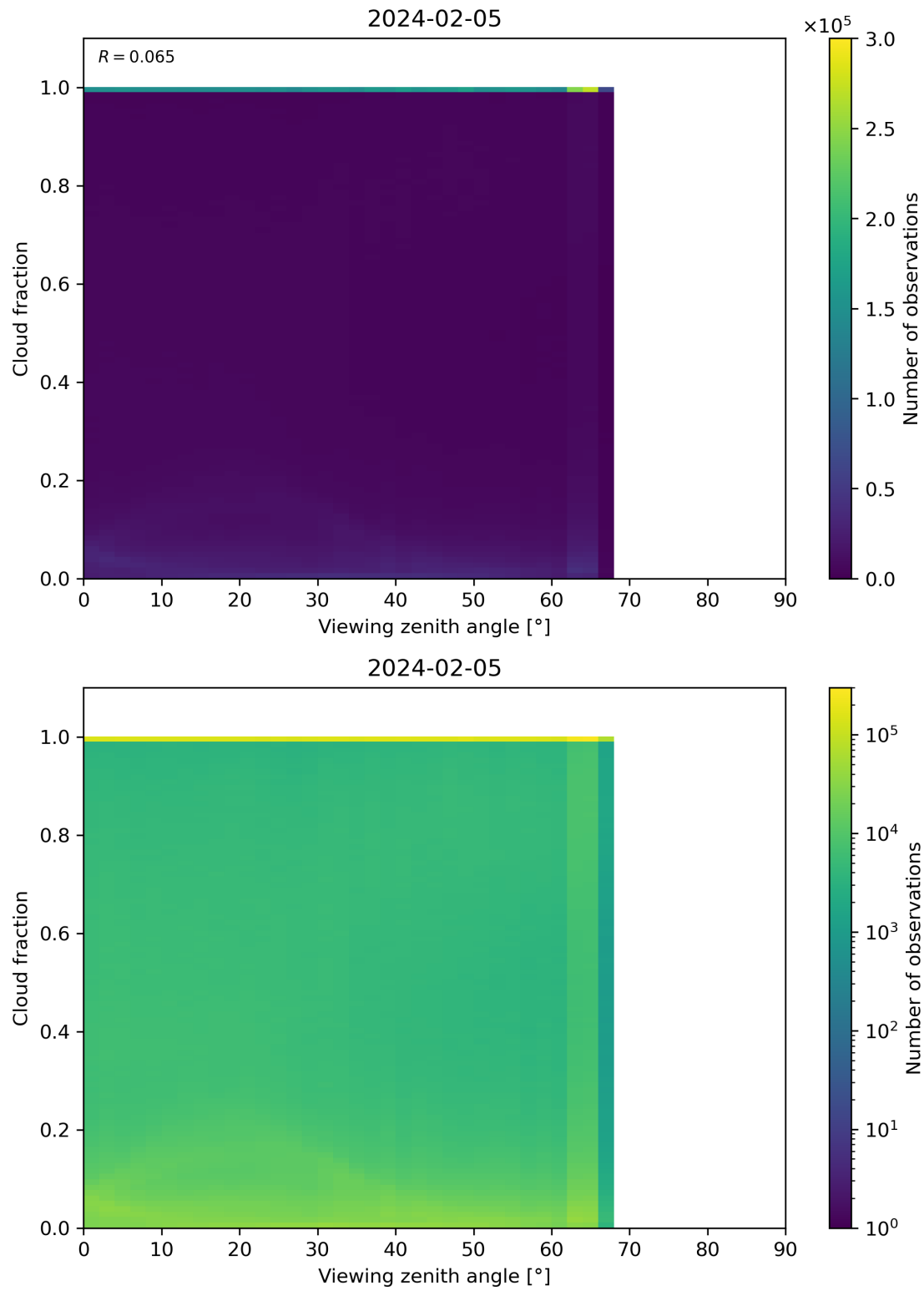
Figure 120: Scatter density plot of “Viewing zenith angle” against “Cloud fraction” for 2024-02-04 to 2024-02-06.
