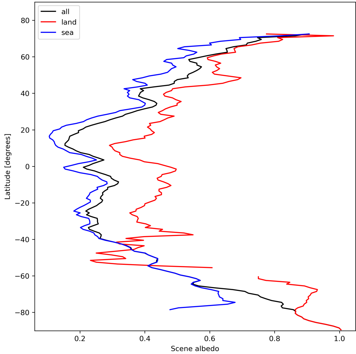
Figure 17: Zonal average of “Scene albedo” for 2024-02-04 to 2024-02-06.
