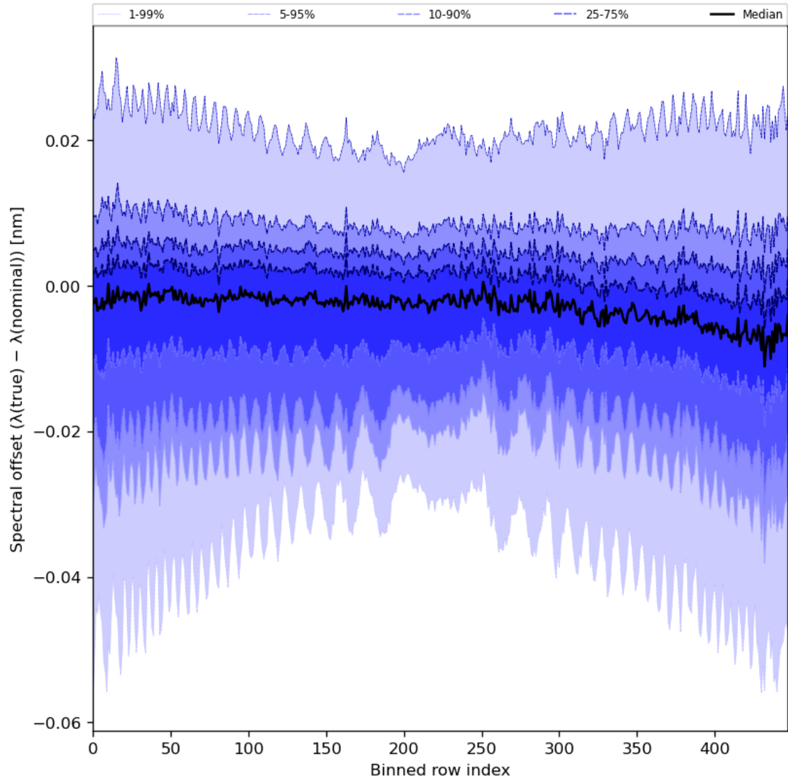
Figure 62: Along track statistics of “Spectral offset ( \lambda(\text{true}) - \lambda(\text{nominal}) )” for 2024-02-04 to 2024-02-06
