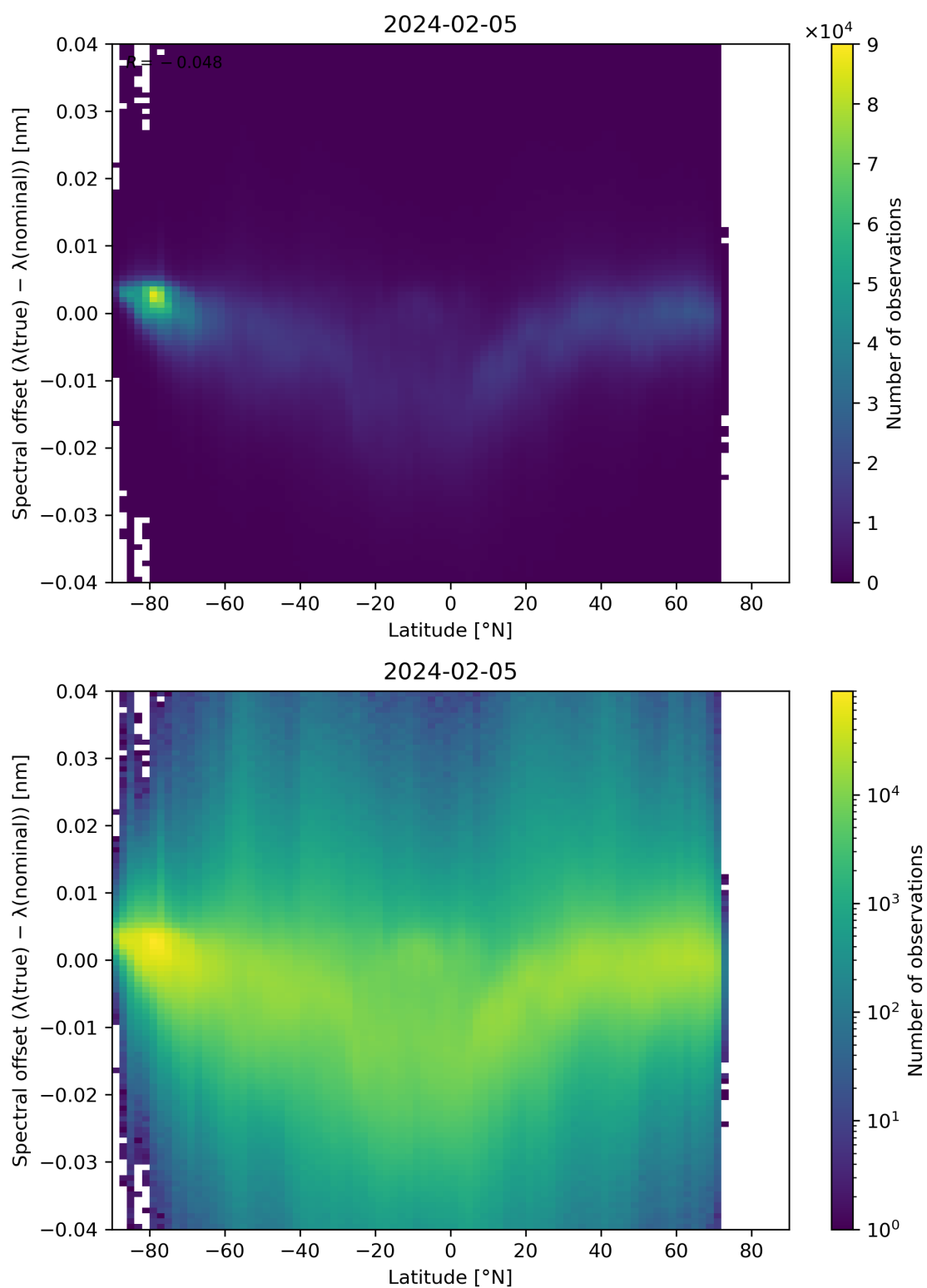
Figure 96: Scatter density plot of “Latitude” against “Spectral offset ( \lambda(\text{true}) - \lambda(\text{nominal}) )” for 2024-02-04 to 2024-02-06.
