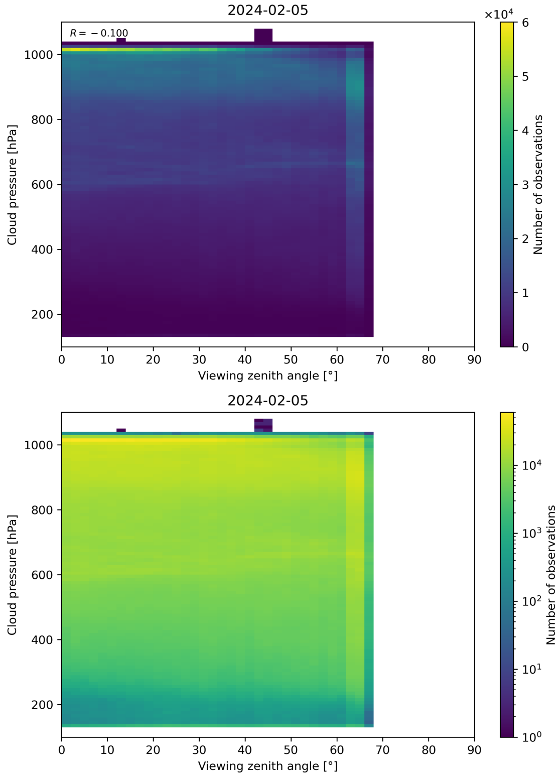
Figure 121: Scatter density plot of “Viewing zenith angle” against “Cloud pressure” for 2024-02-04 to 2024-02-06.
