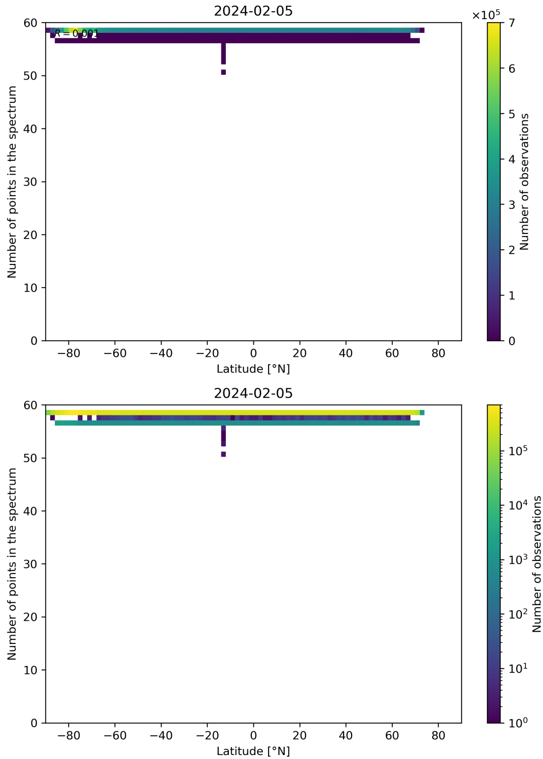
Figure 94: Scatter density plot of “Latitude” against “Number of points in the spectrum” for 2024-02-04 to 2024-02-06.
