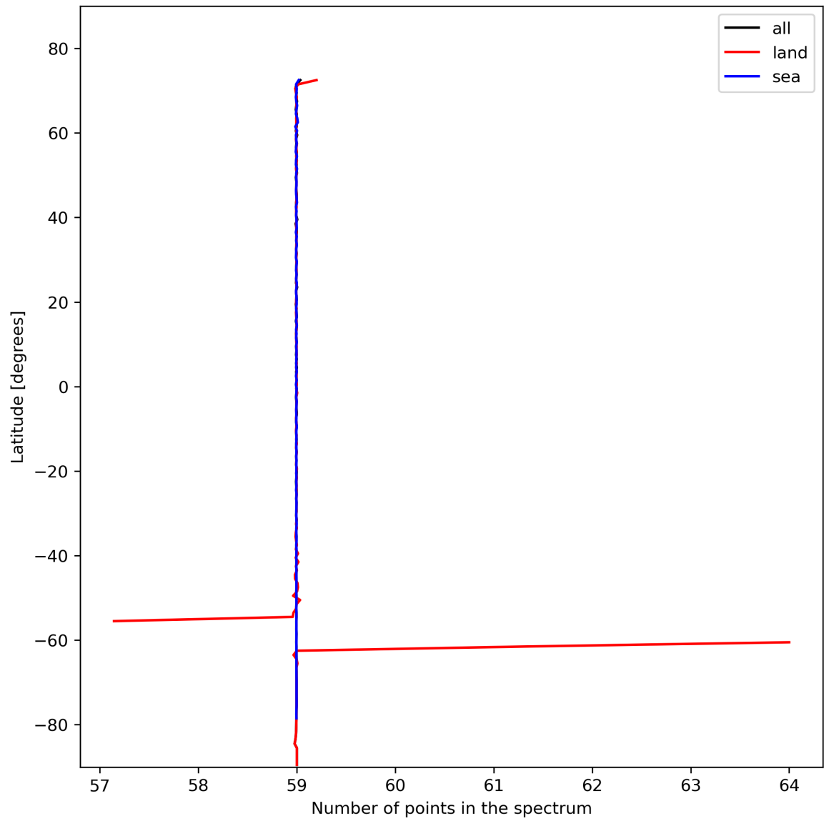
Figure 27: Zonal average of “Number of points in the spectrum” for 2024-02-04 to 2024-02-06.
