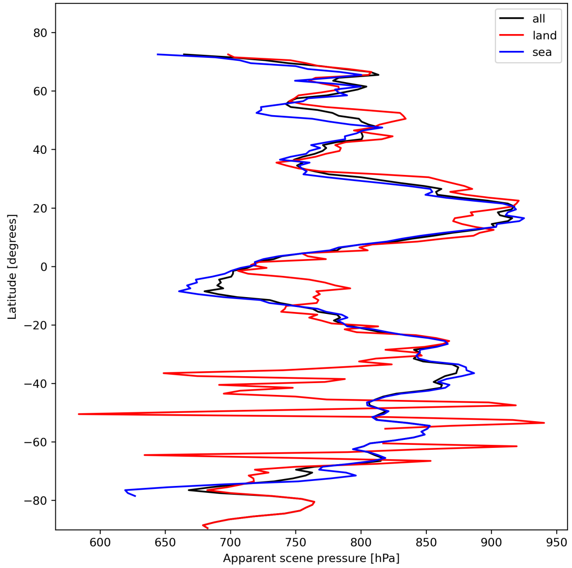
Figure 19: Zonal average of “Apparent scene pressure” for 2024-02-04 to 2024-02-06.
