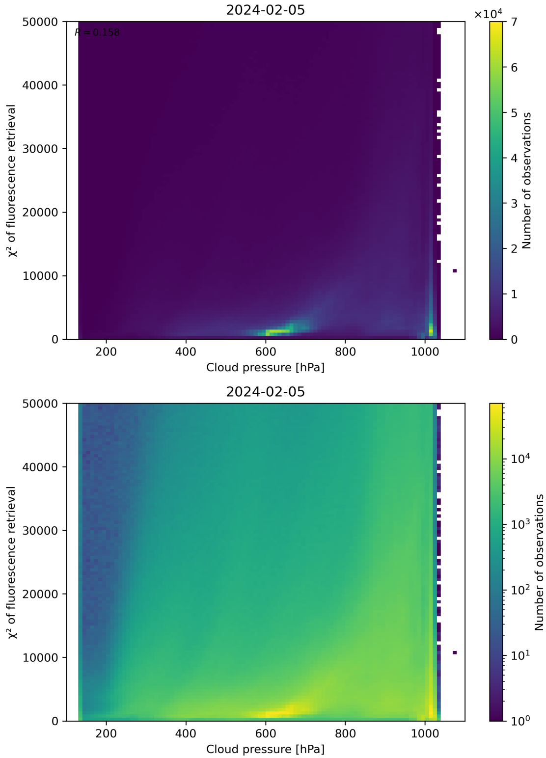
Figure 78: Scatter density plot of “Cloud pressure” against “ \chi^2 of fluorescence retrieval” for 2024-02-04 to 2024-02-06.
