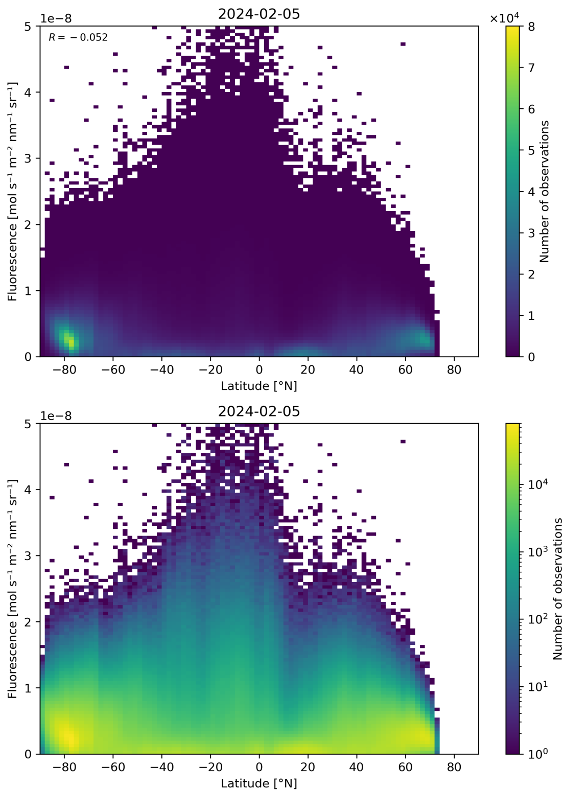
Figure 92: Scatter density plot of “Latitude” against “Fluorescence” for 2024-02-04 to 2024-02-06.
