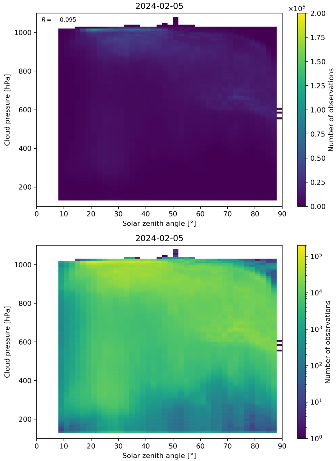
Figure 111: Scatter density plot of “Solar zenith angle” against “Cloud pressure” for 2024-02-04 to 2024-02-06.
