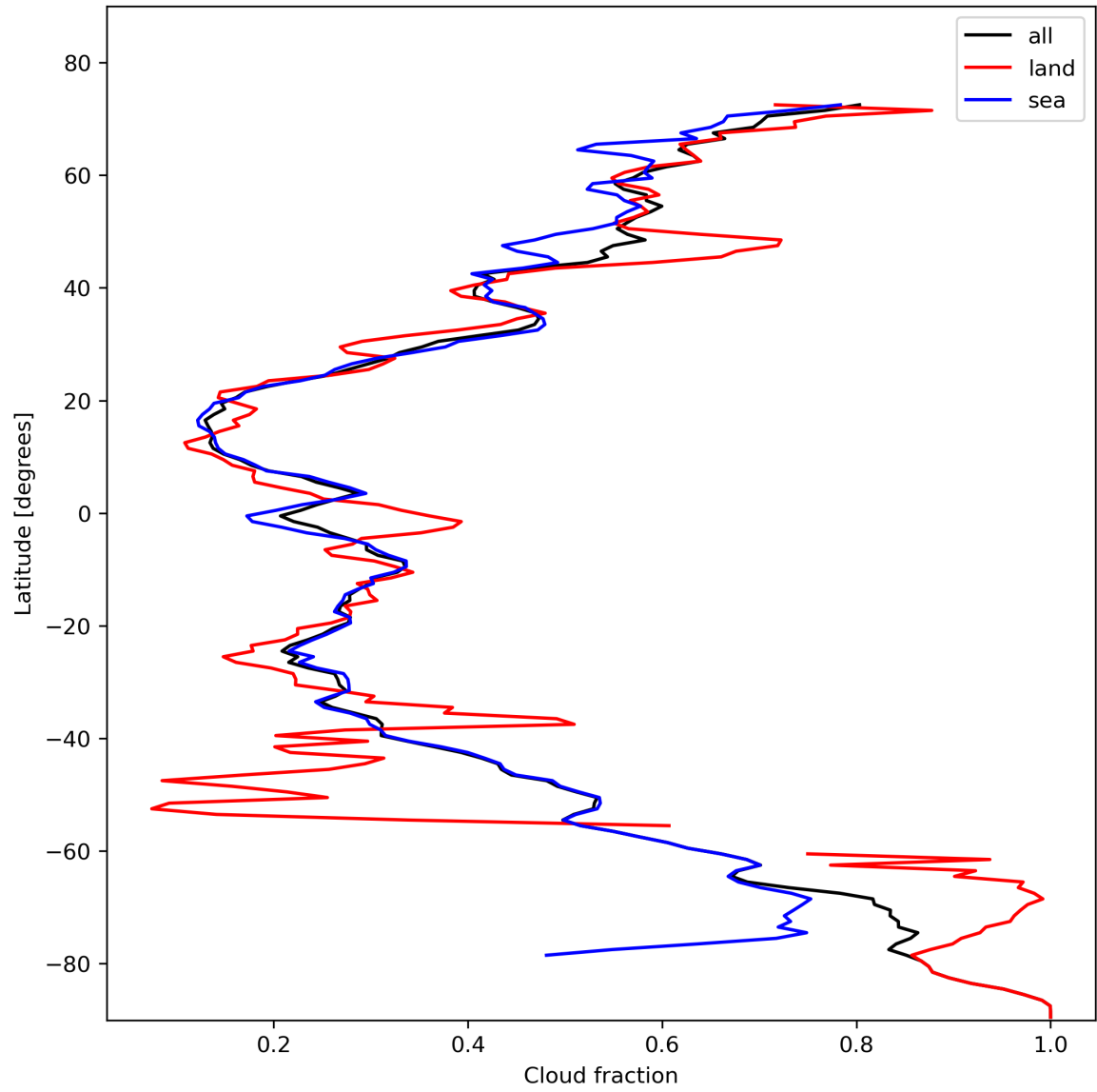
Figure 15: Zonal average of “Cloud fraction” for 2024-02-04 to 2024-02-06.
