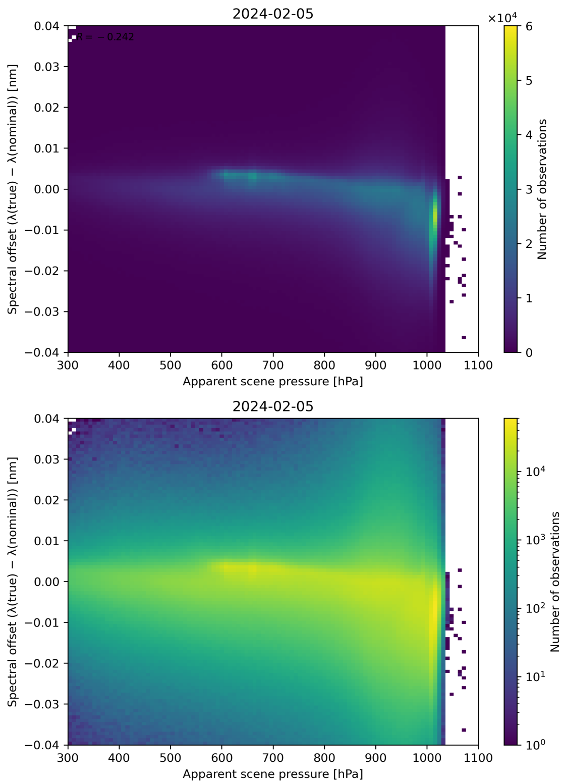
Figure 67: Scatter density plot of “Apparent scene pressure” against “Spectral offset ( \lambda(\text{true}) - \lambda(\text{nominal}) )” for 2024-02-04 to 2024-02-06.
