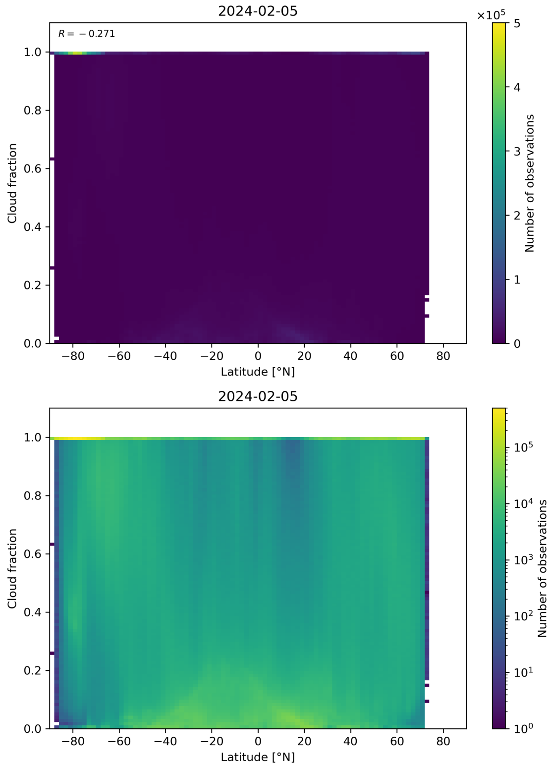
Figure 90: Scatter density plot of “Latitude” against “Cloud fraction” for 2024-02-04 to 2024-02-06.
