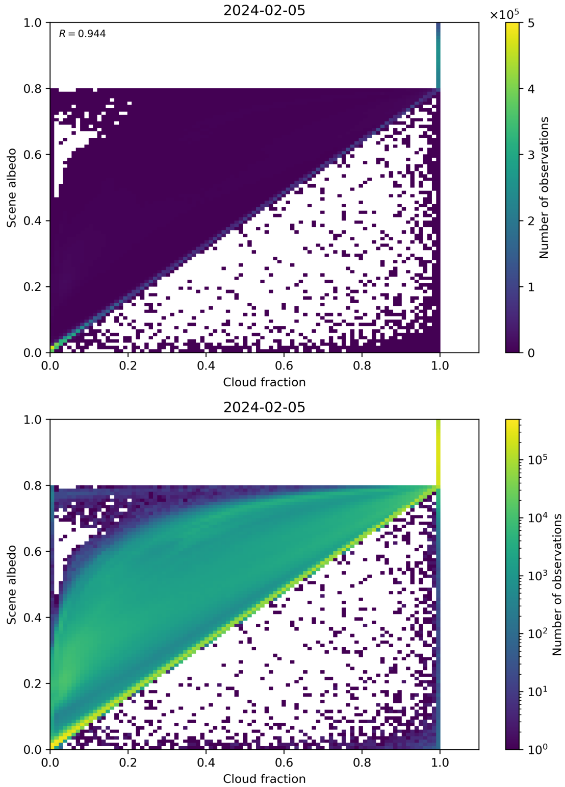
Figure 75: Scatter density plot of “Cloud fraction” against “Scene albedo” for 2024-02-04 to 2024-02-06.
