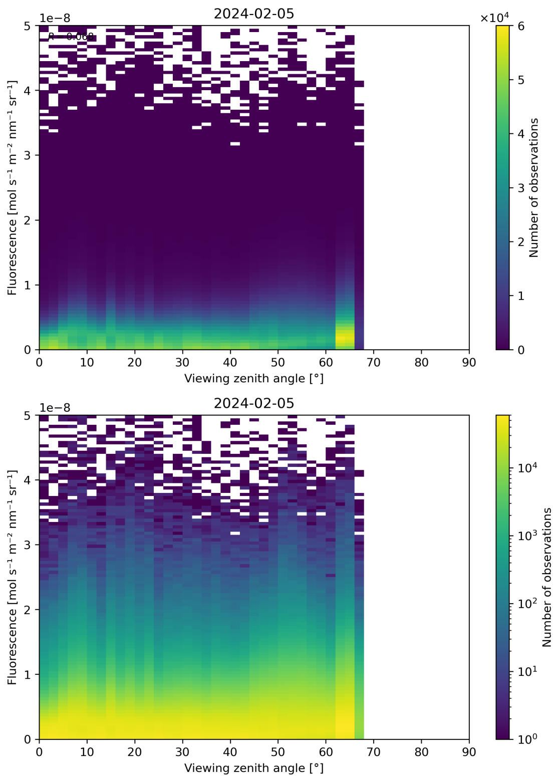
Figure 122: Scatter density plot of “Viewing zenith angle” against “Fluorescence” for 2024-02-04 to 2024-02-06.
