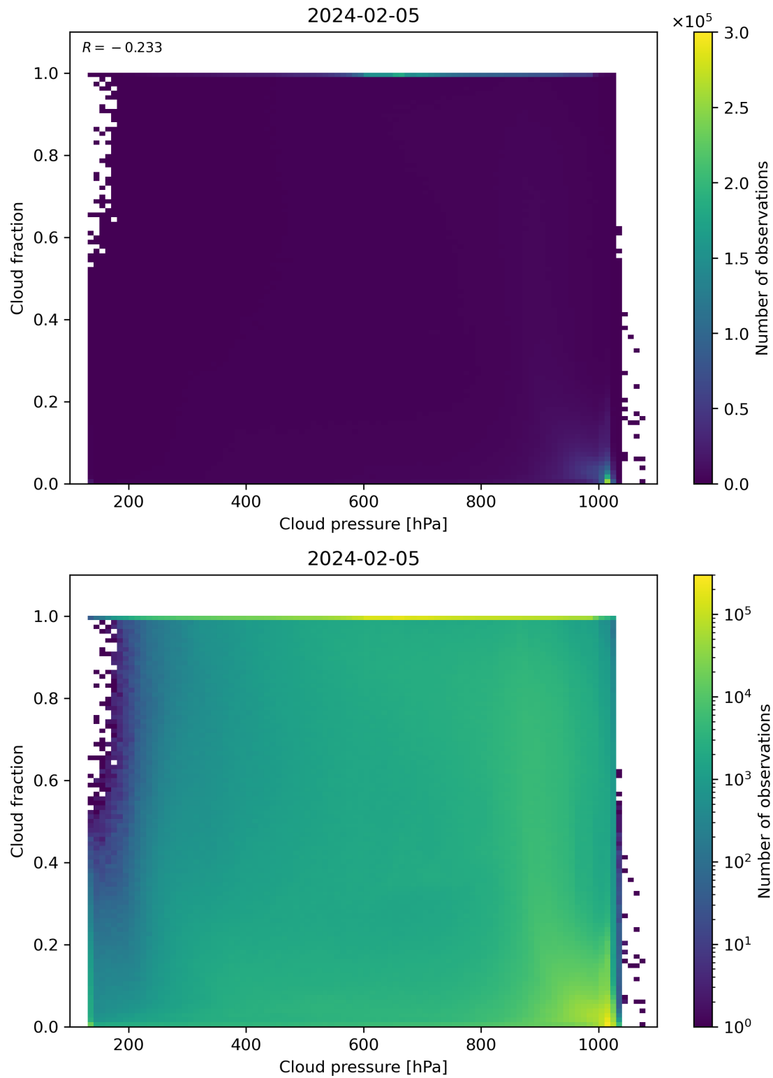
Figure 79: Scatter density plot of “Cloud pressure” against “Cloud fraction” for 2024-02-04 to 2024-02-06.
