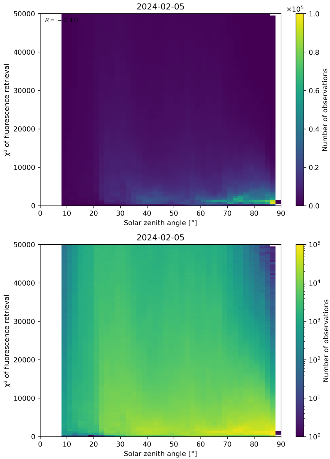
Figure 109: Scatter density plot of “Solar zenith angle” against “ \chi^2 of fluorescence retrieval” for 2024-02-04 to 2024-02-06.
