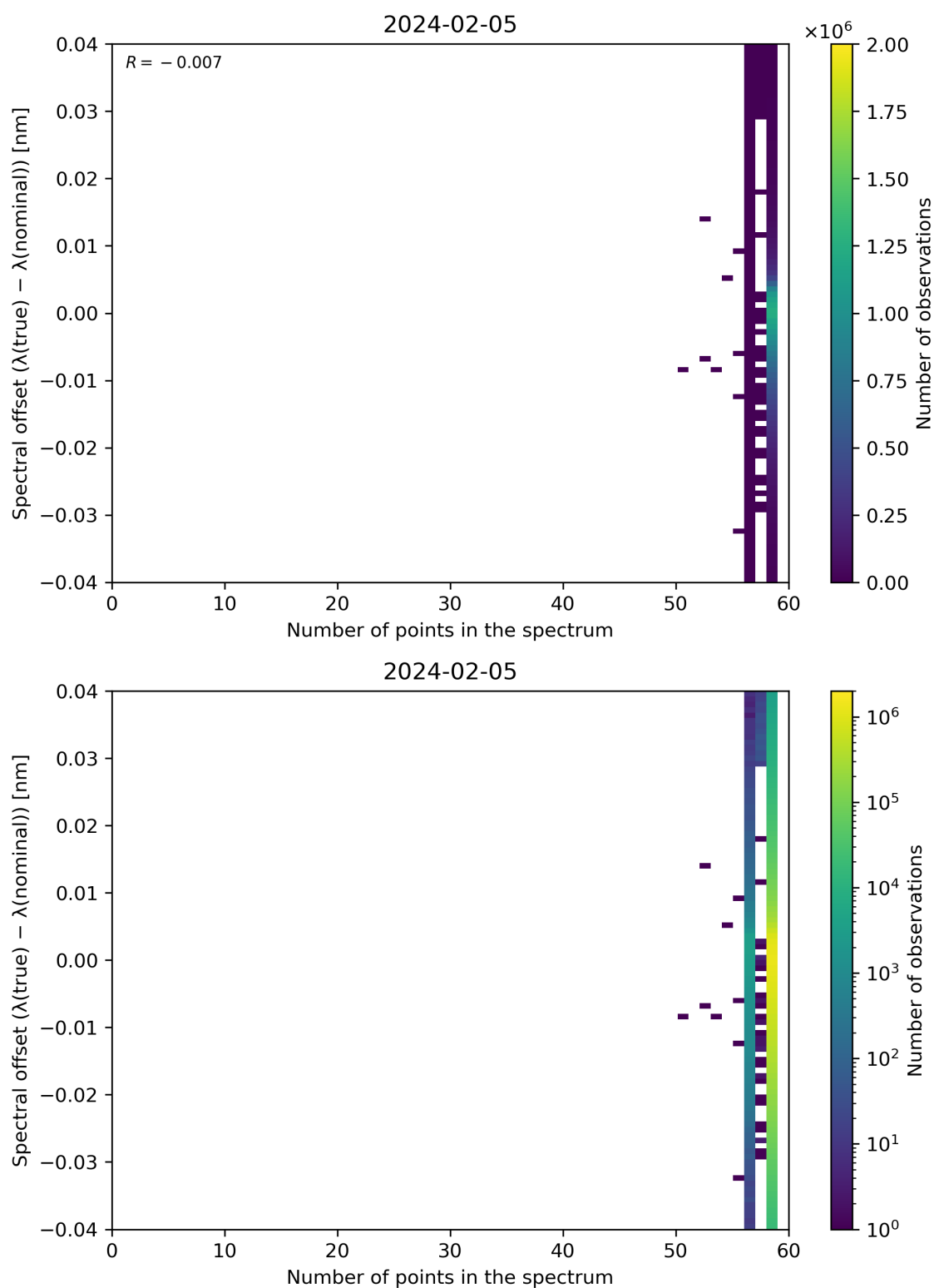
Figure 101: Scatter density plot of “Number of points in the spectrum” against “Spectral offset ( \lambda(\text{true}) - \lambda(\text{nominal}) )” for 2024-02-04 to 2024-02-06.
