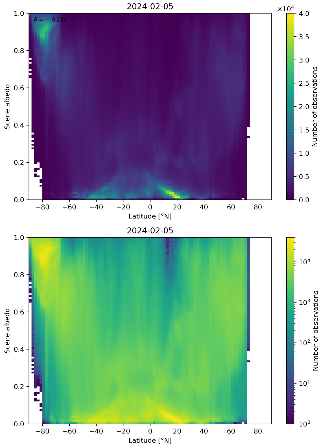
Figure 95: Scatter density plot of “Latitude” against “Scene albedo” for 2024-02-04 to 2024-02-06.
