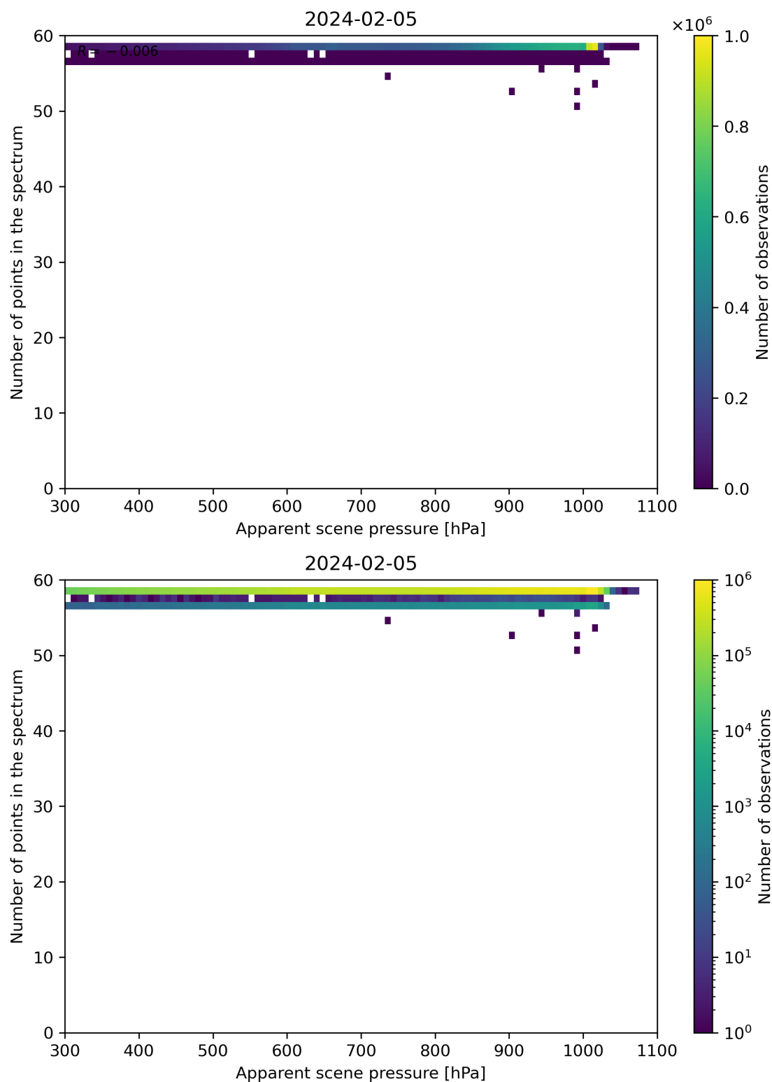
Figure 66: Scatter density plot of “Apparent scene pressure” against “Number of points in the spectrum” for 2024-02-04 to 2024-02-06.
