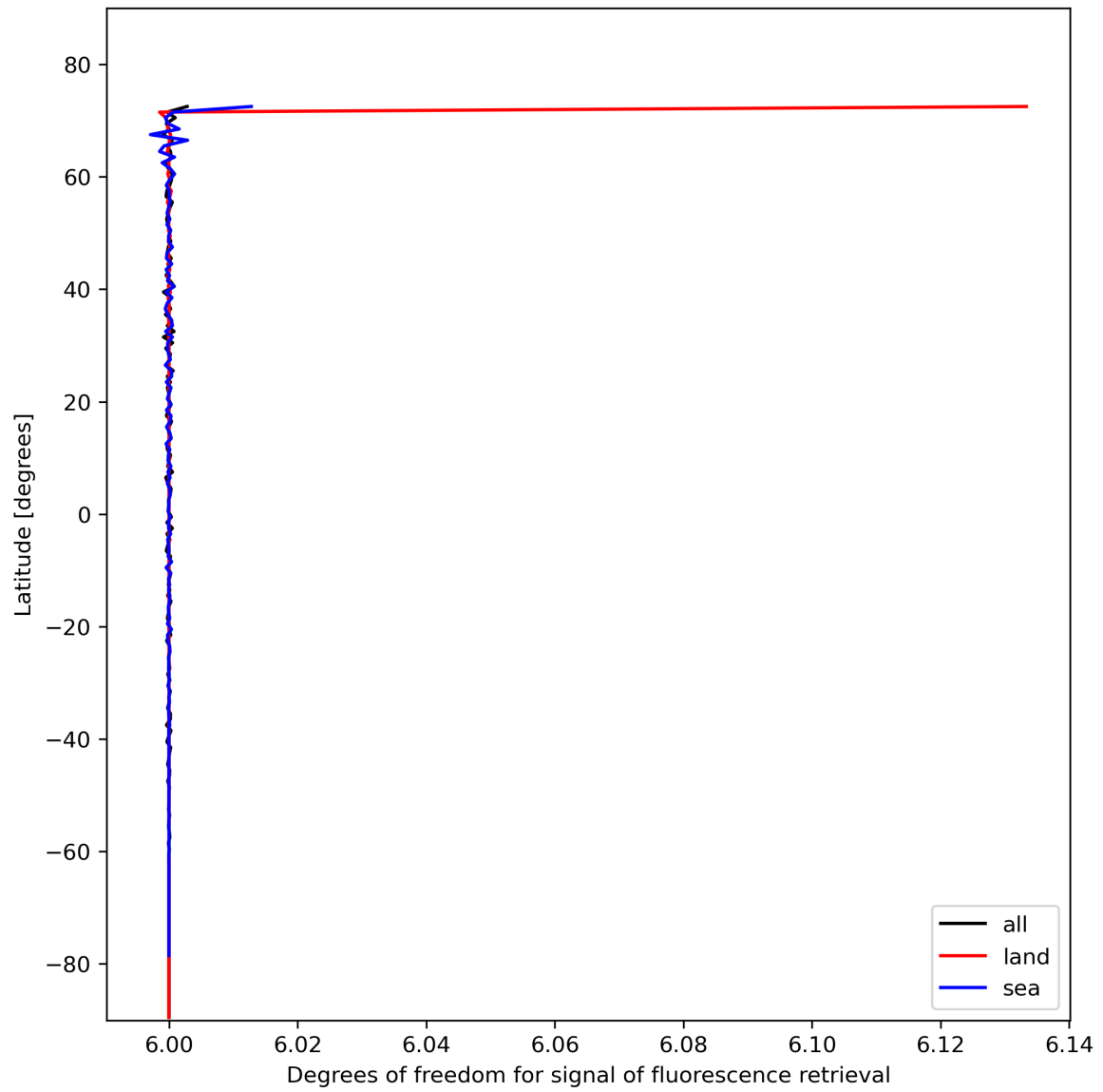
Figure 26: Zonal average of “Degrees of freedom for signal of fluorescence retrieval” for 2024-02-04 to 2024-02-06.
