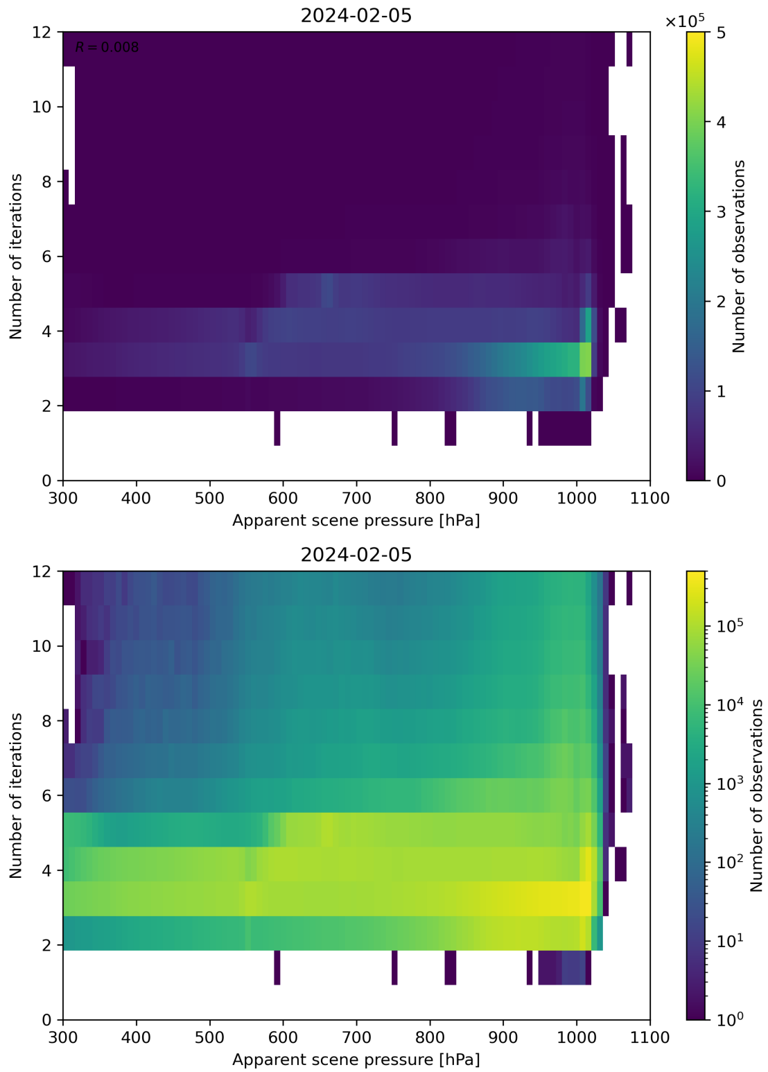
Figure 65: Scatter density plot of “Apparent scene pressure” against “Number of iterations” for 2024-02-04 to 2024-02-06.
