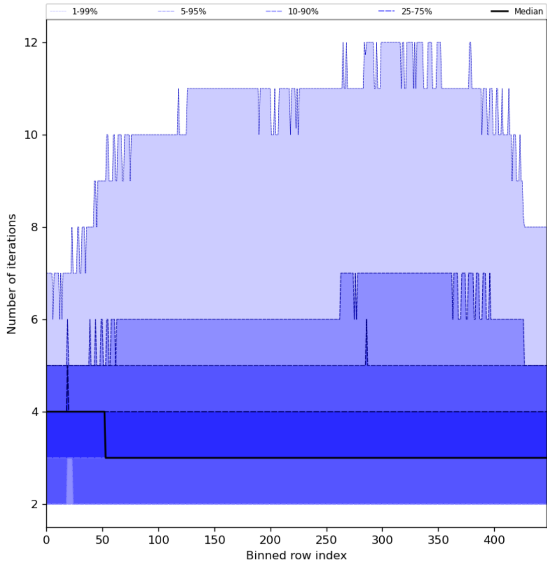
Figure 56: Along track statistics of “Number of iterations” for 2024-02-04 to 2024-02-06
