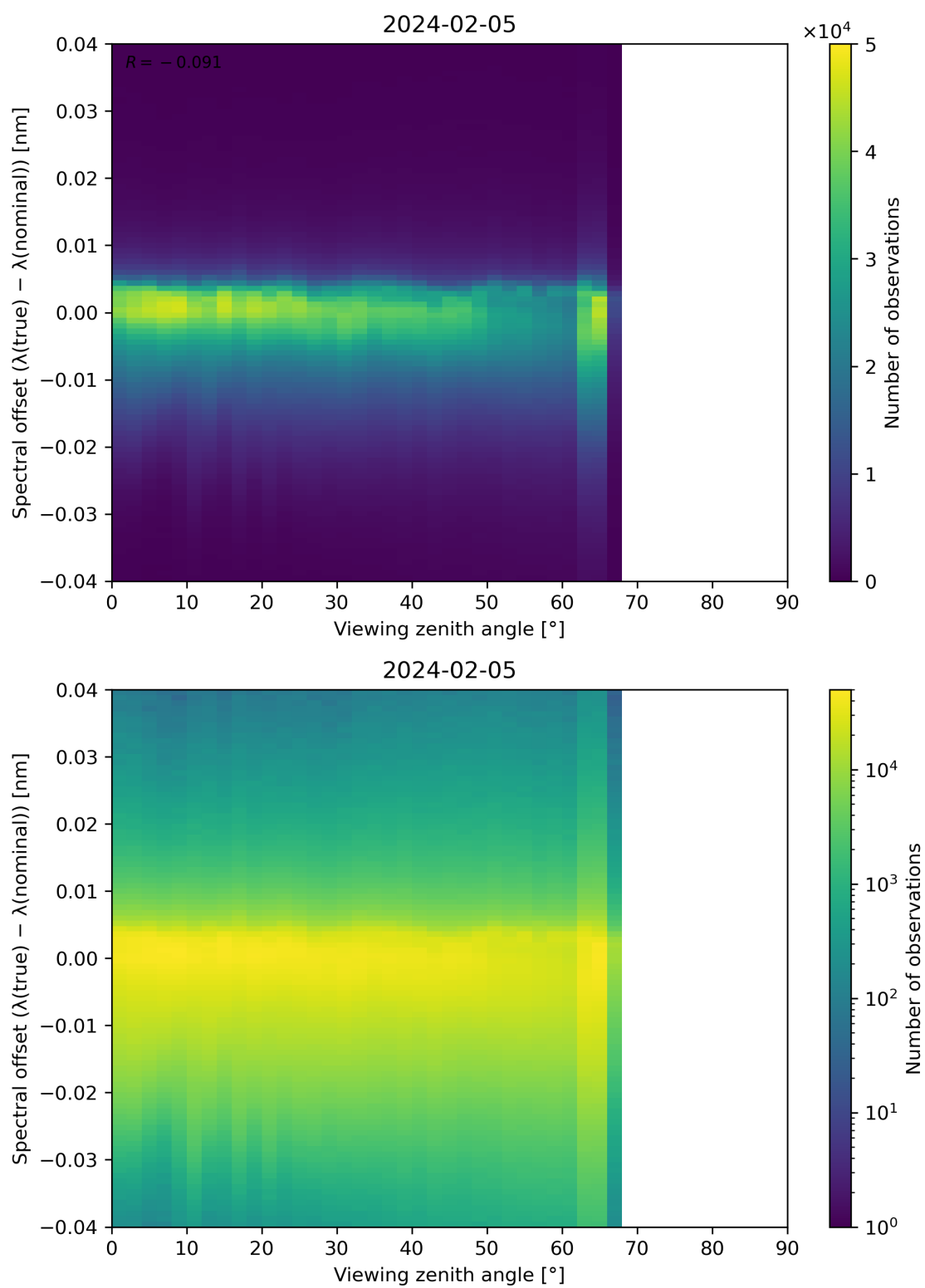
Figure 128: Scatter density plot of “Viewing zenith angle” against “Spectral offset ( \lambda(\text{true}) - \lambda(\text{nominal}) )” for 2024-02-04 to 2024-02-06.
