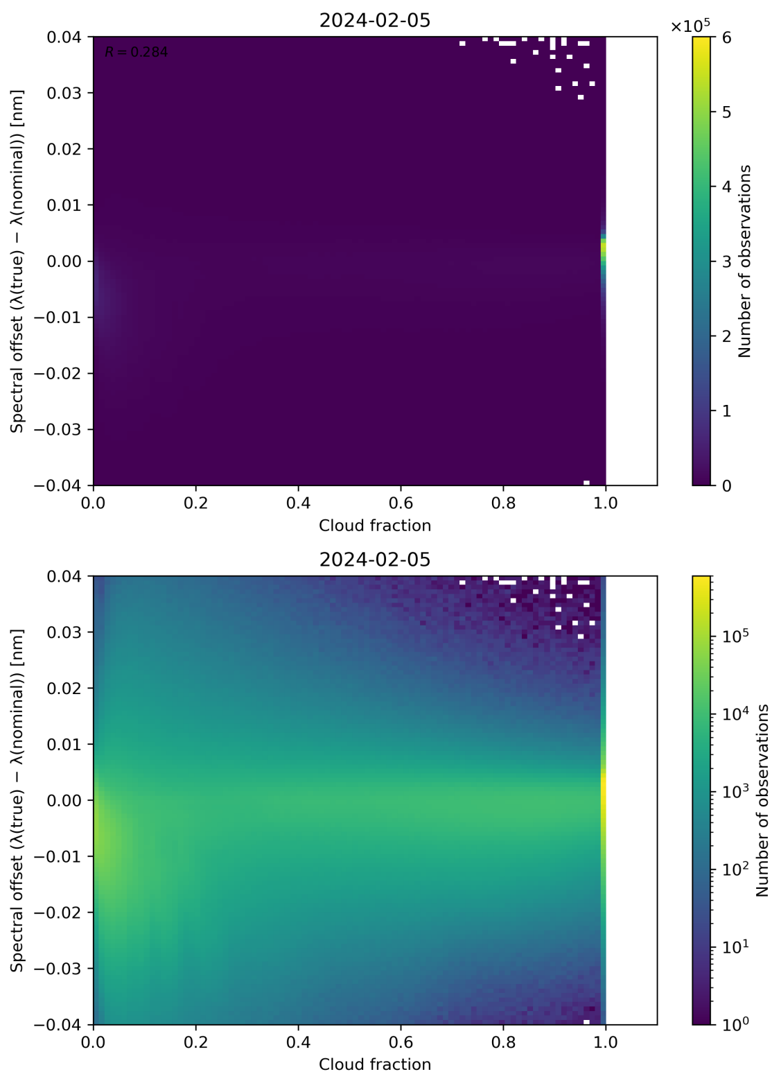
Figure 76: Scatter density plot of “Cloud fraction” against “Spectral offset ( \lambda(\text{true}) - \lambda(\text{nominal}) )” for 2024-02-04 to 2024-02-06.
