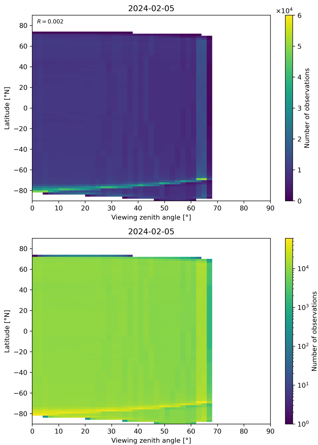
Figure 123: Scatter density plot of “Viewing zenith angle” against “Latitude” for 2024-02-04 to 2024-02-06.
