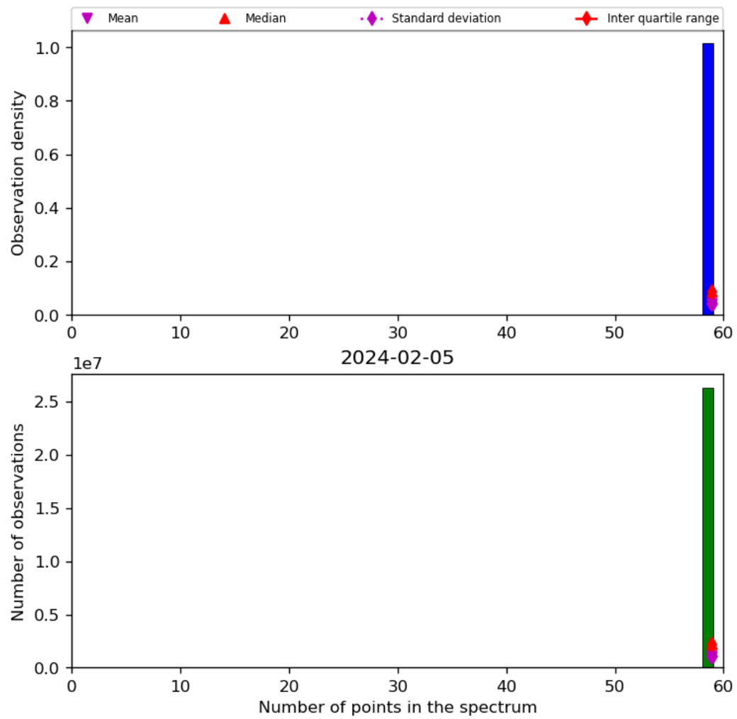
Figure 44: Histogram of "Number of points in the spectrum" for 2024-02-04 to 2024-02-06
