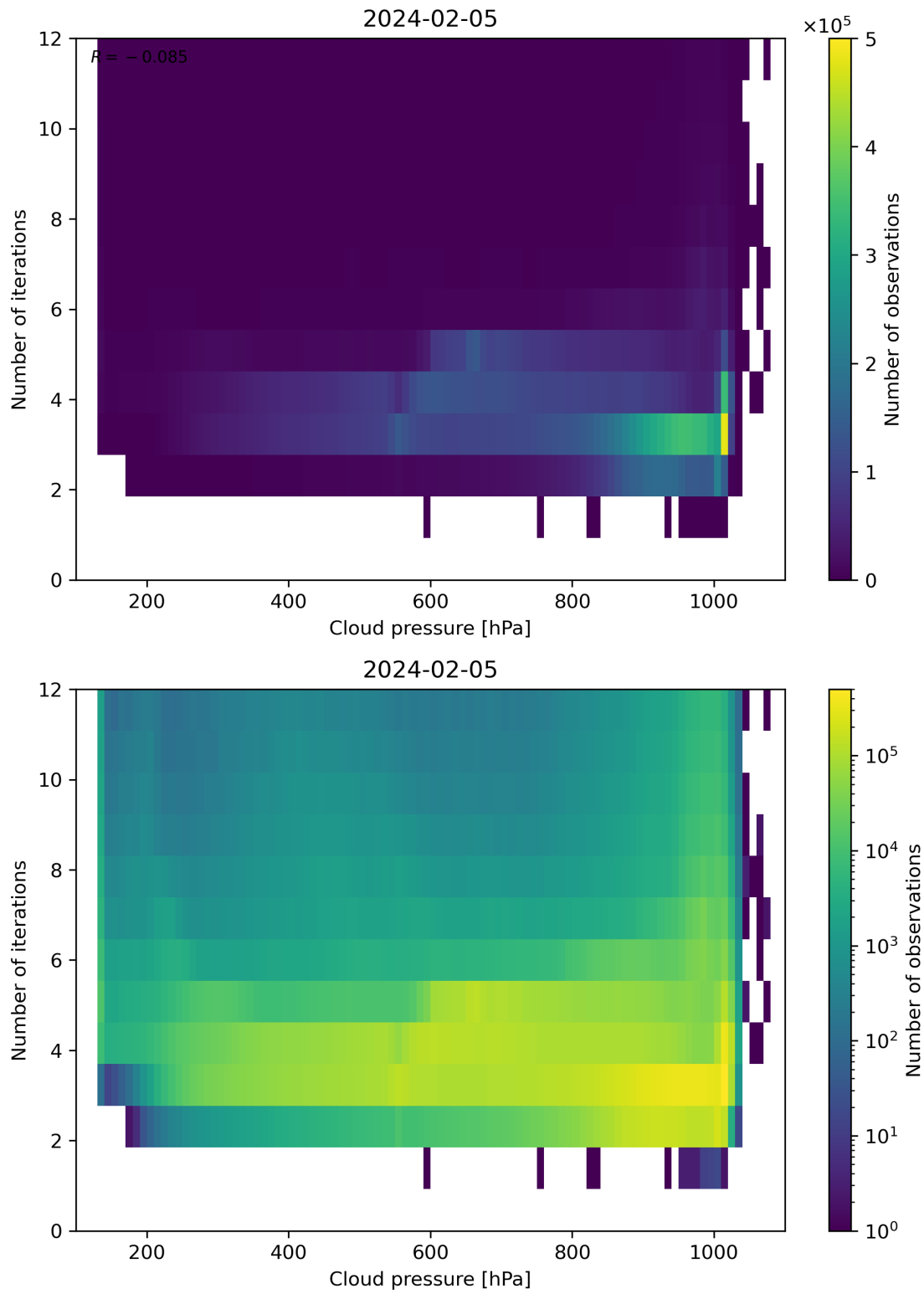
Figure 81: Scatter density plot of “Cloud pressure” against “Number of iterations” for 2024-02-04 to 2024-02-06.
