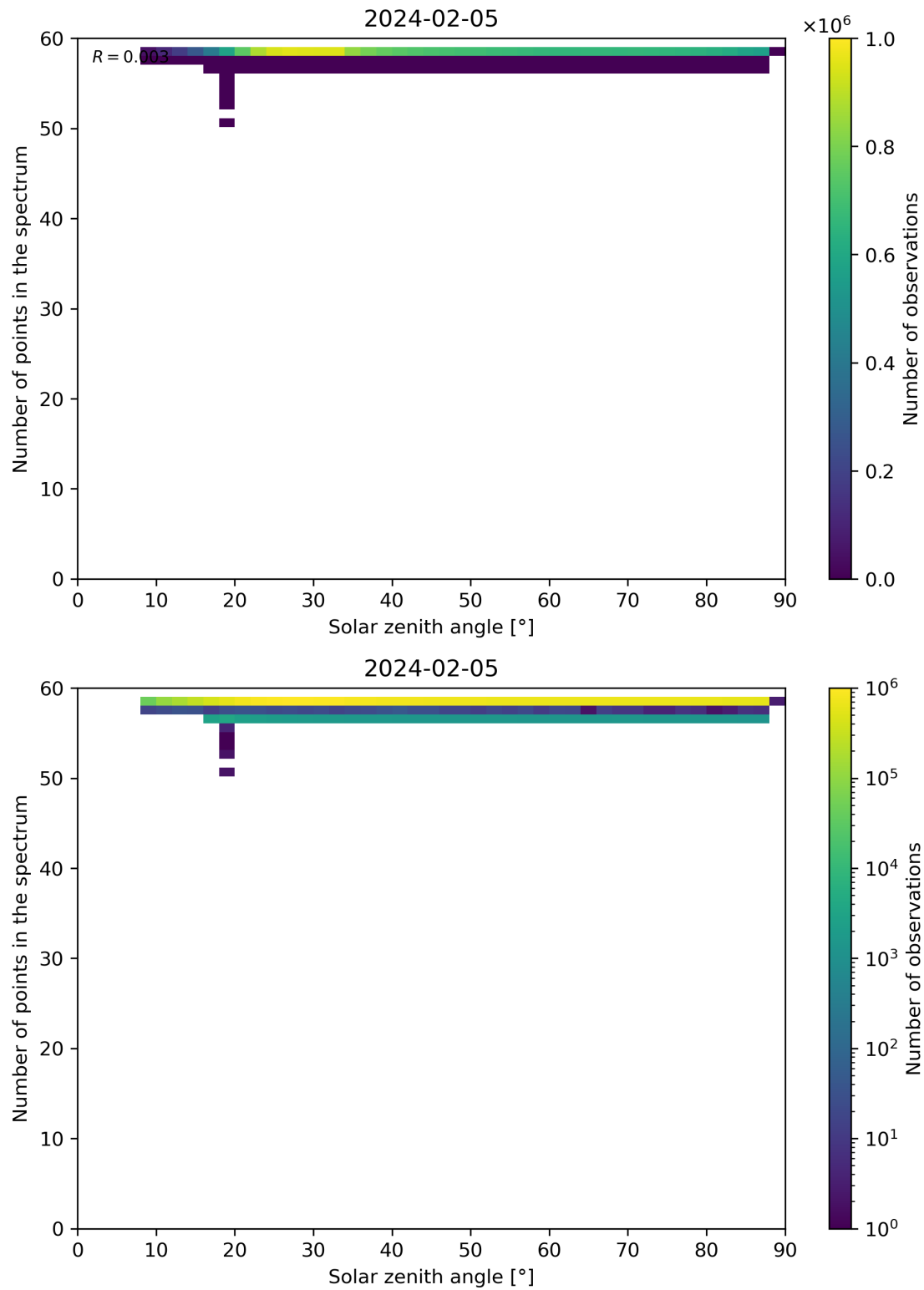
Figure 115: Scatter density plot of “Solar zenith angle” against “Number of points in the spectrum” for 2024-02-04 to 2024-02-06.
