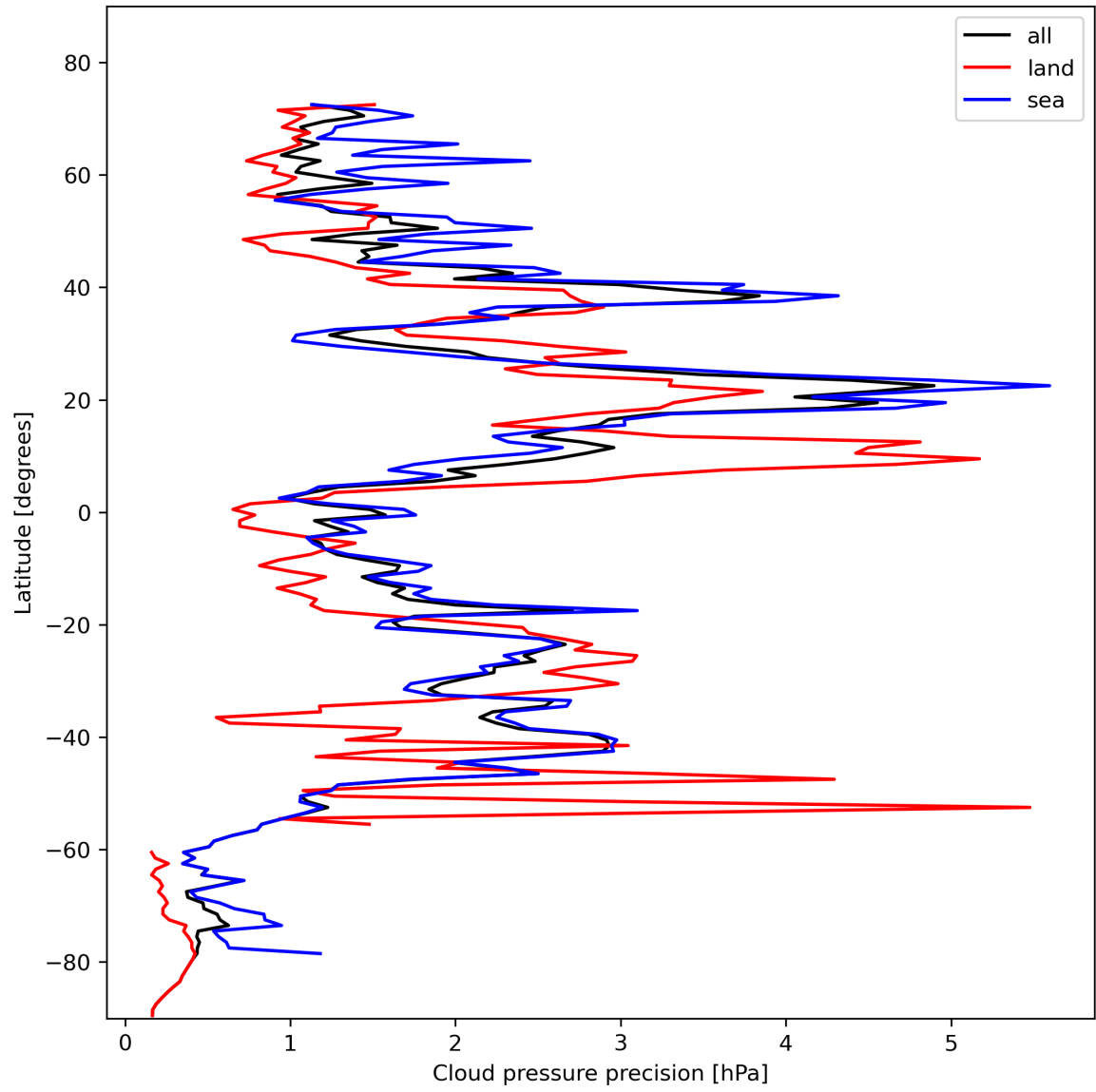
Figure 14: Zonal average of “Cloud pressure precision” for 2024-02-04 to 2024-02-06.
