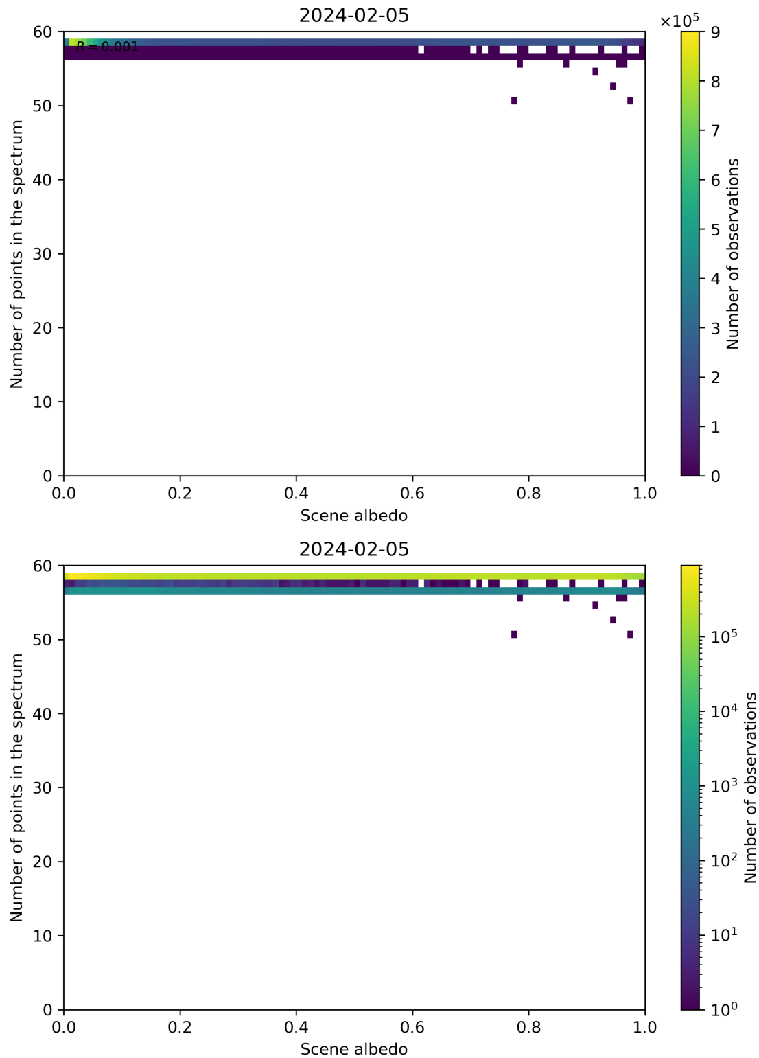
Figure 106: Scatter density plot of “Scene albedo” against “Number of points in the spectrum” for 2024-02-04 to 2024-02-06.
