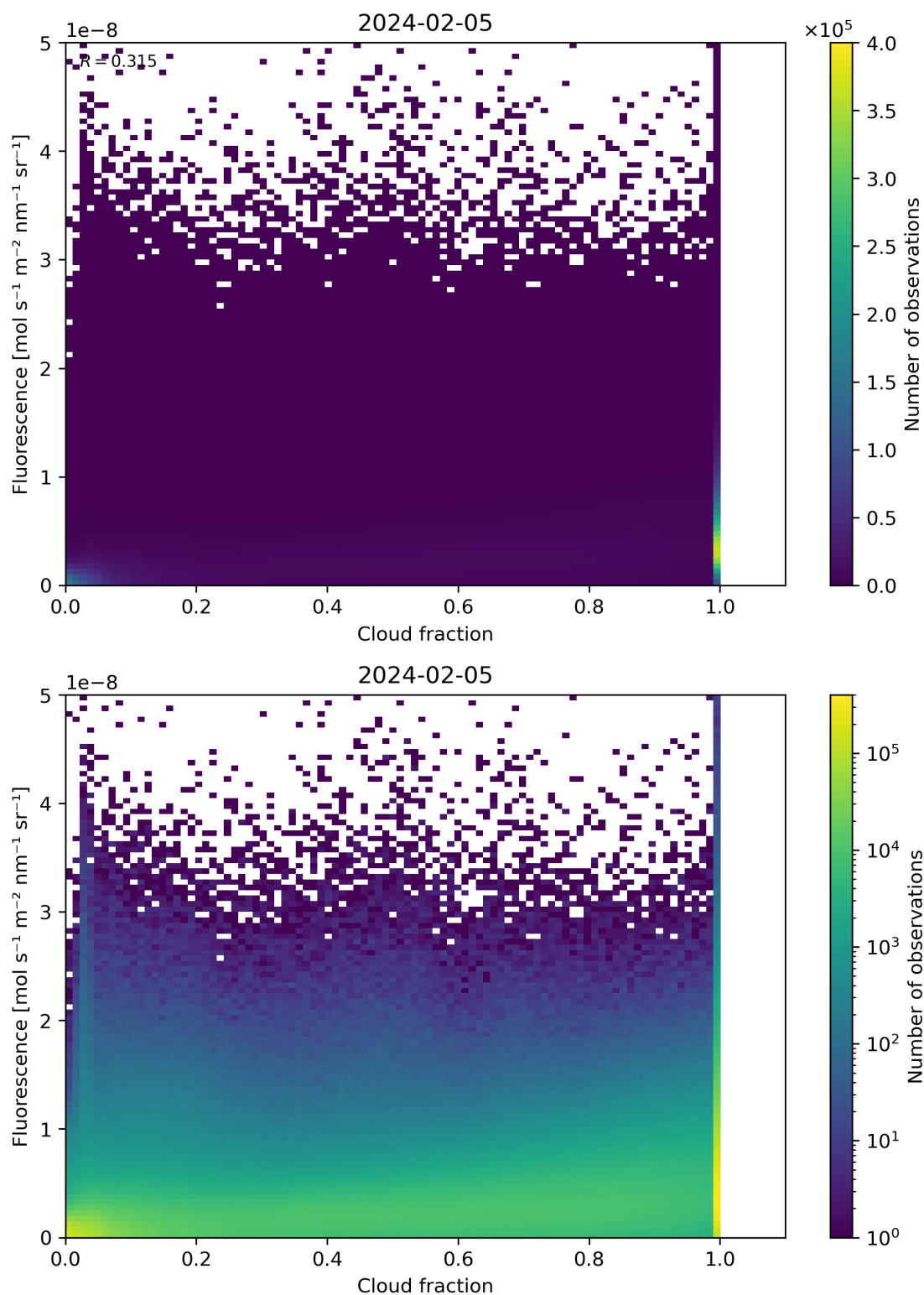
Figure 72: Scatter density plot of “Cloud fraction” against “Fluorescence” for 2024-02-04 to 2024-02-06.
