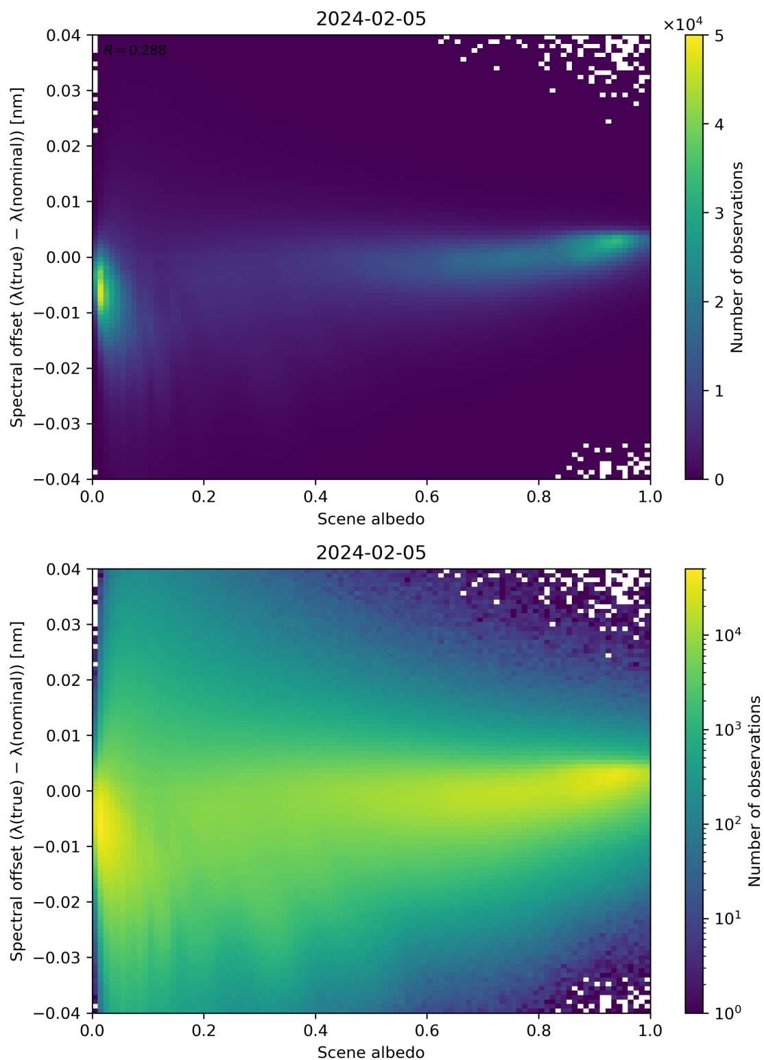
Figure 107: Scatter density plot of “Scene albedo” against “Spectral offset ( \lambda(\text{true}) - \lambda(\text{nominal}) )” for 2024-02-04 to 2024-02-06.
