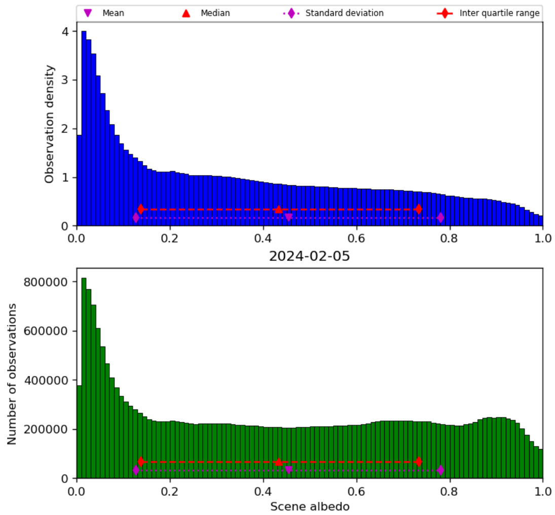
Figure 34: Histogram of “Scene albedo” for 2024-02-04 to 2024-02-06
