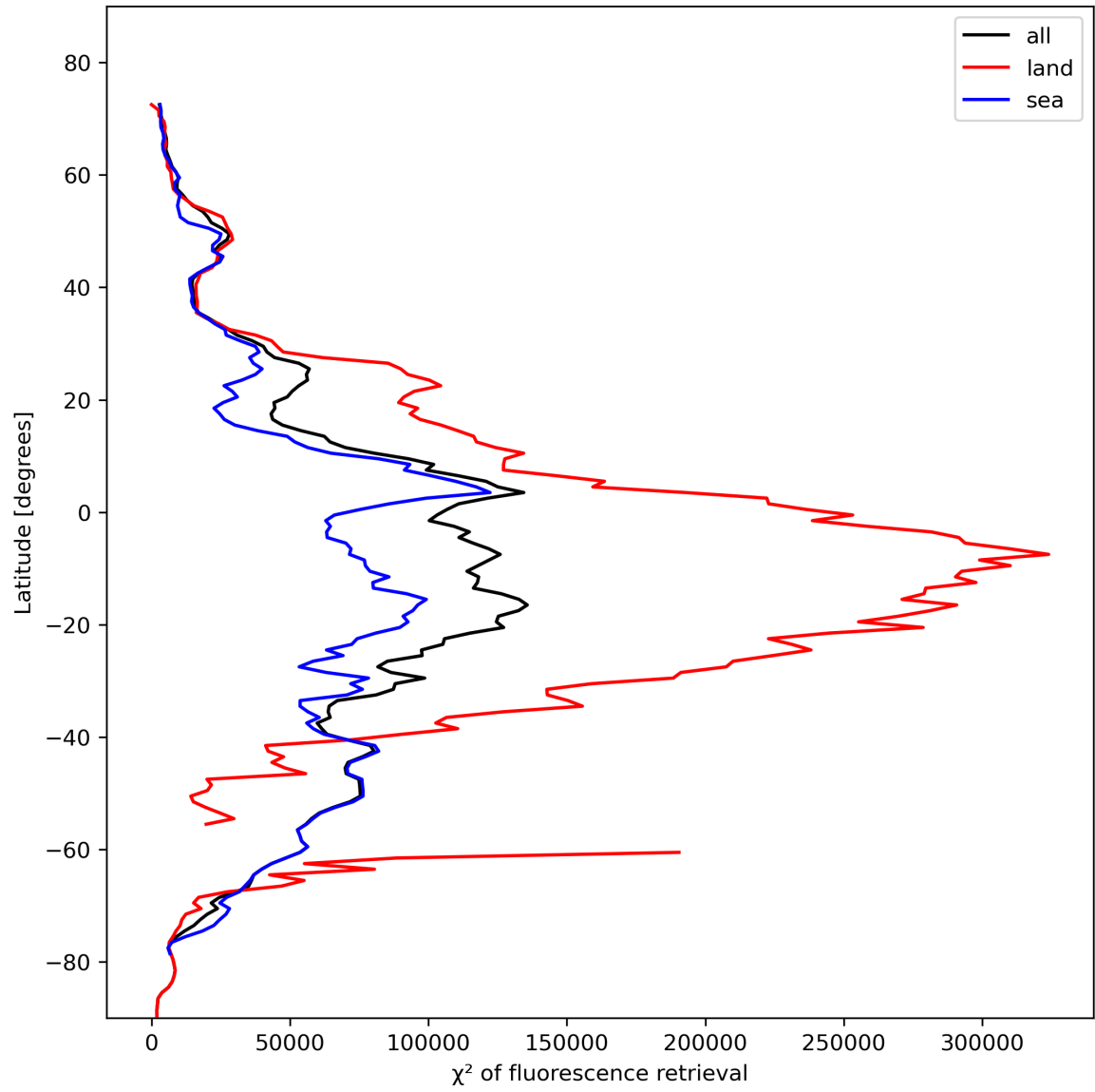
Figure 25: Zonal average of “ \chi^2 of fluorescence retrieval” for 2024-02-04 to 2024-02-06.
