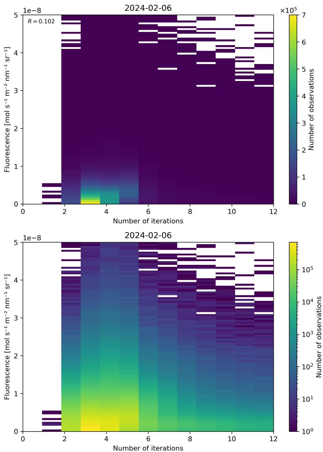
Figure 98: Scatter density plot of “Number of iterations” against “Fluorescence” for 2024-02-06 to 2024-02-07.
