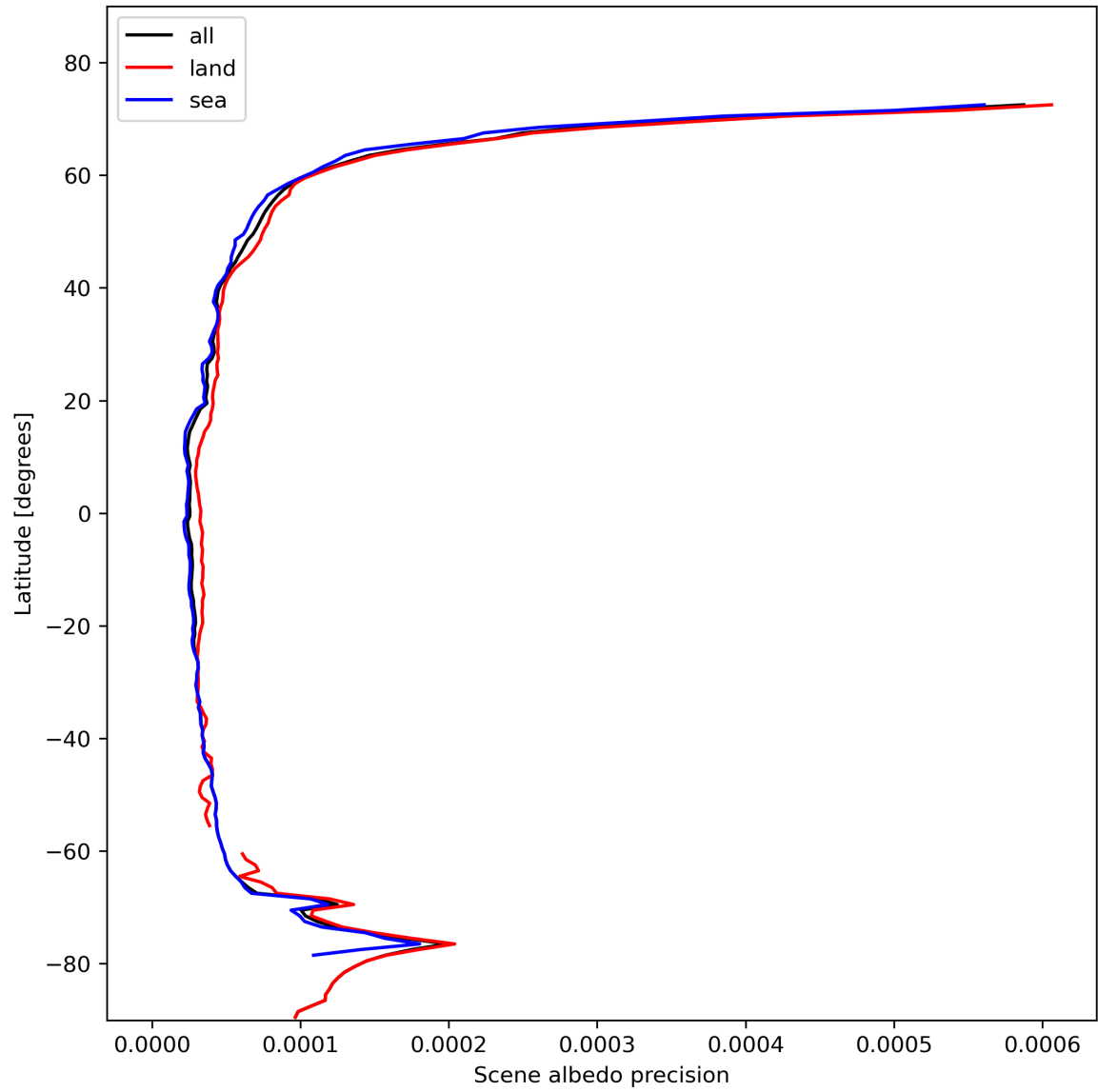
Figure 18: Zonal average of “Scene albedo precision” for 2024-02-06 to 2024-02-07.
