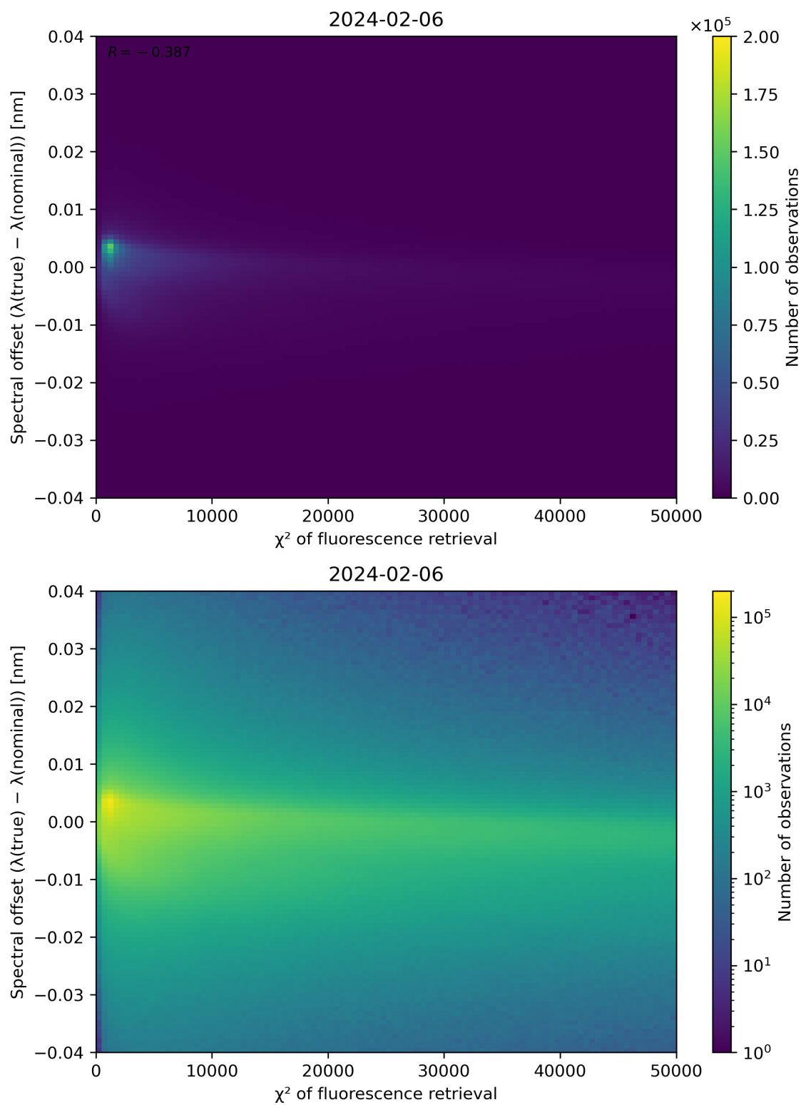
Figure 69: Scatter density plot of " \chi^2 of fluorescence retrieval" against "Spectral offset ( \lambda(\text{true}) - \lambda(\text{nominal}) )" for 2024-02-06 to 2024-02-07.
