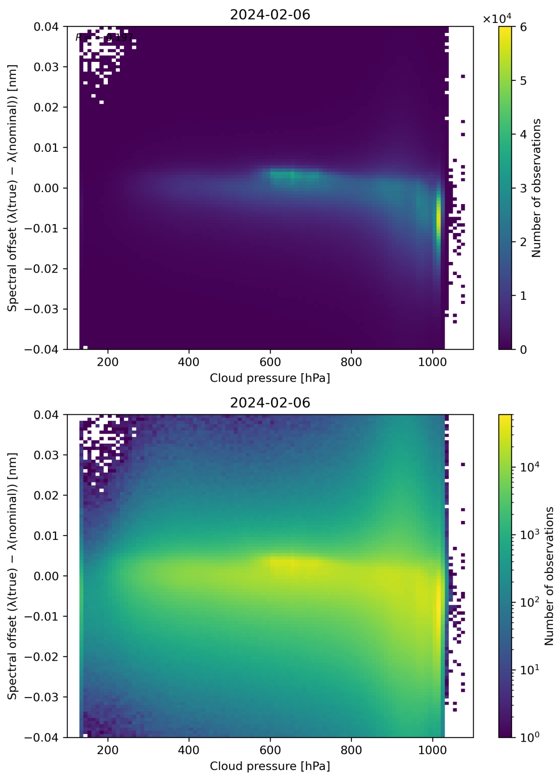
Figure 84: Scatter density plot of “Cloud pressure” against “Spectral offset ( \lambda(\text{true}) - \lambda(\text{nominal}) )” for 2024-02-06 to 2024-02-07.
