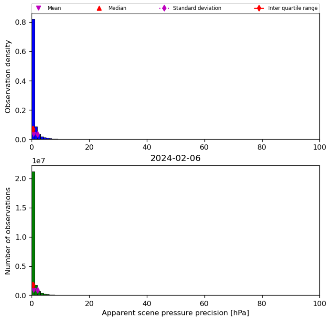
Figure 37: Histogram of “Apparent scene pressure precision” for 2024-02-06 to 2024-02-07
