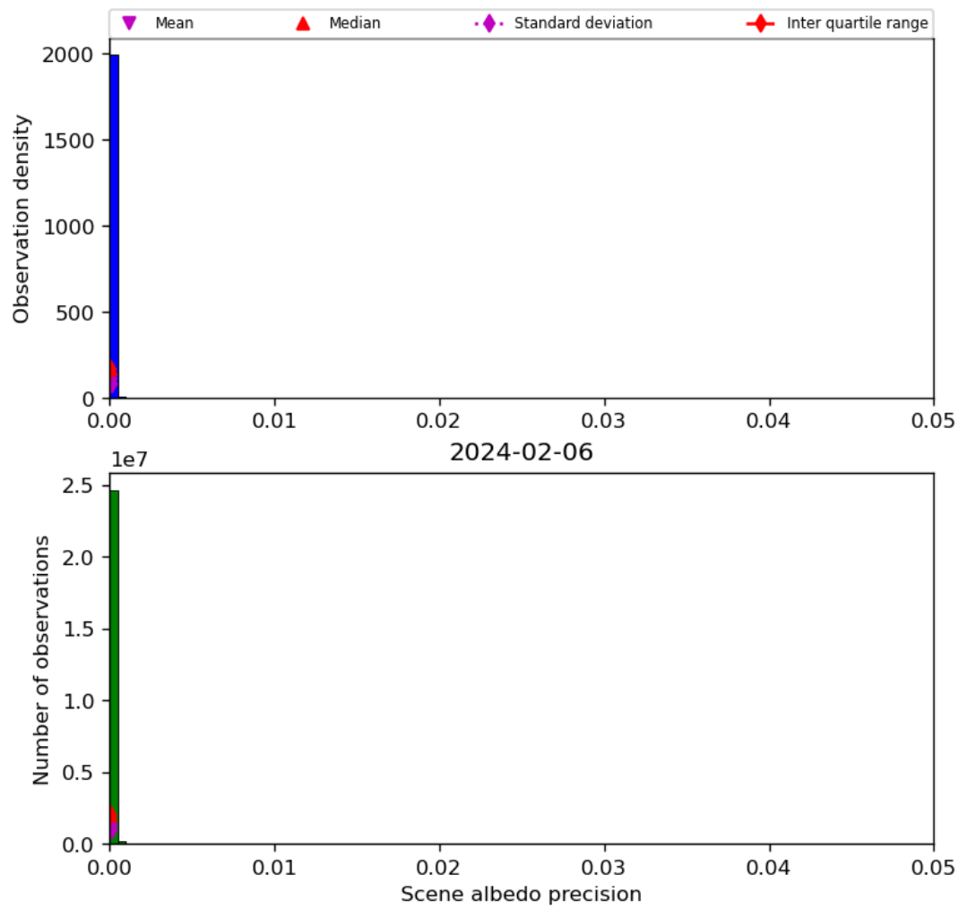
Figure 35: Histogram of “Scene albedo precision” for 2024-02-06 to 2024-02-07
