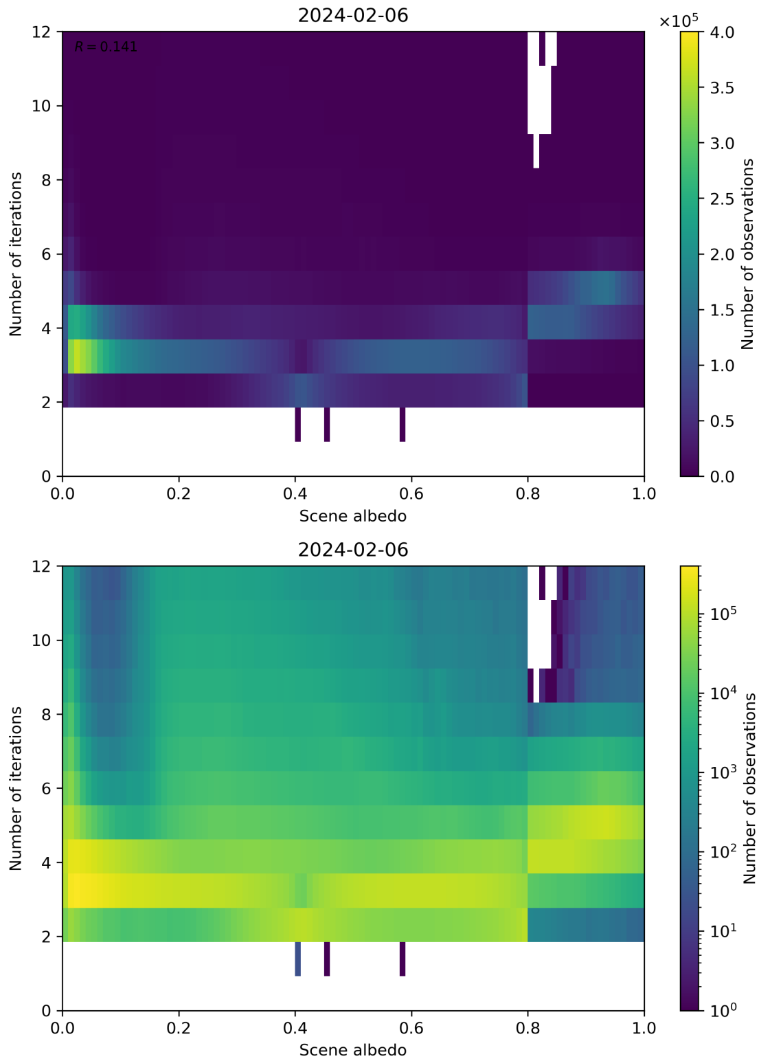
Figure 105: Scatter density plot of “Scene albedo” against “Number of iterations” for 2024-02-06 to 2024-02-07.
