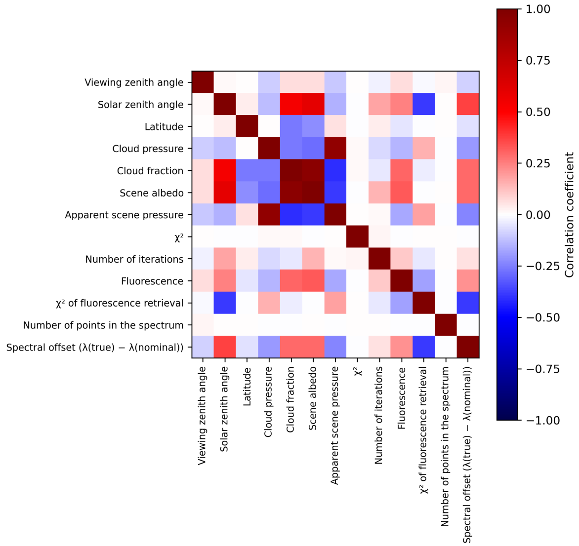
Figure 2: Map of correlation matrix for 2024-02-06 to 2024-02-07.
