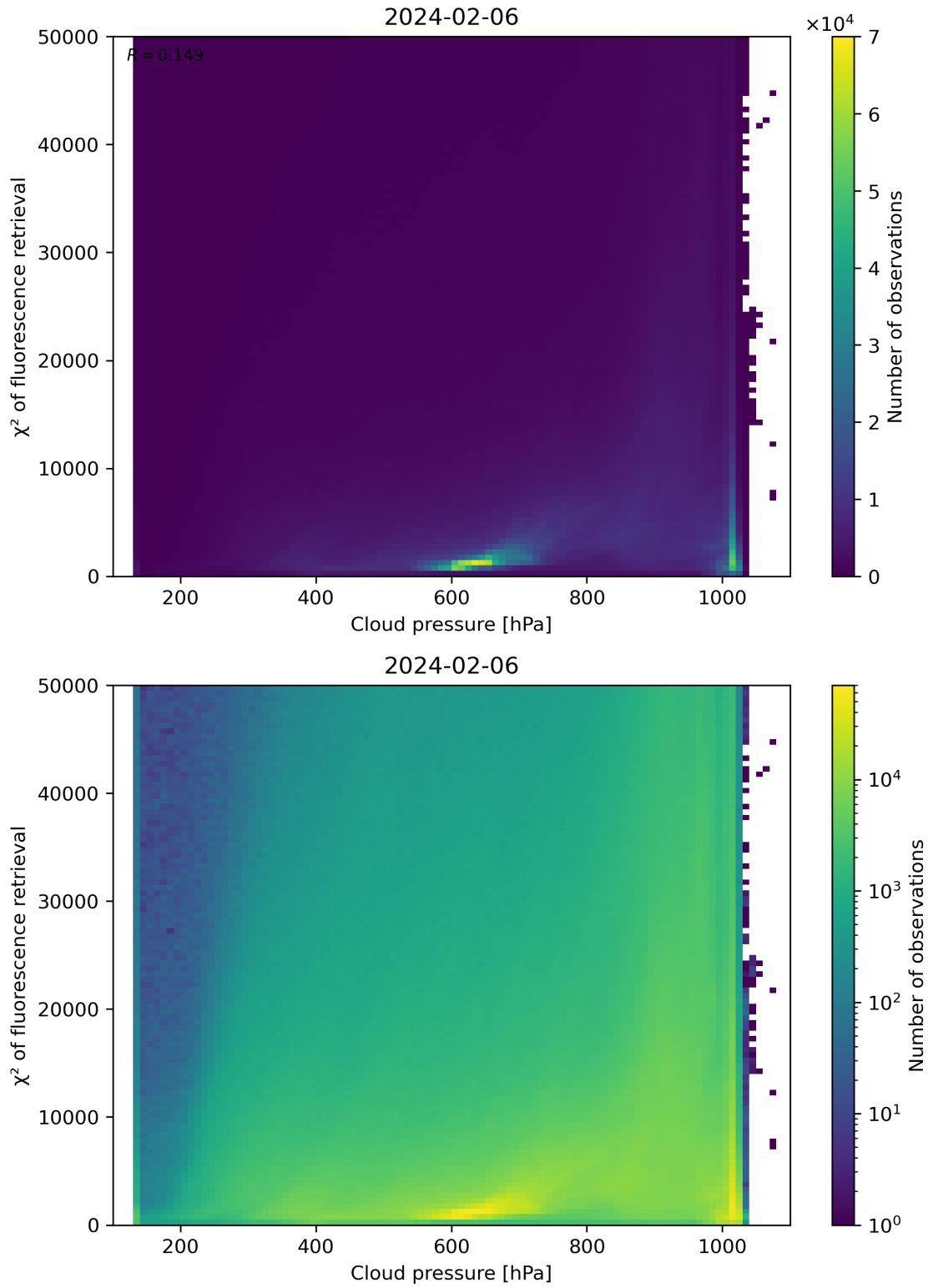
Figure 78: Scatter density plot of “Cloud pressure” against “ \chi^2 of fluorescence retrieval” for 2024-02-06 to 2024-02-07.
