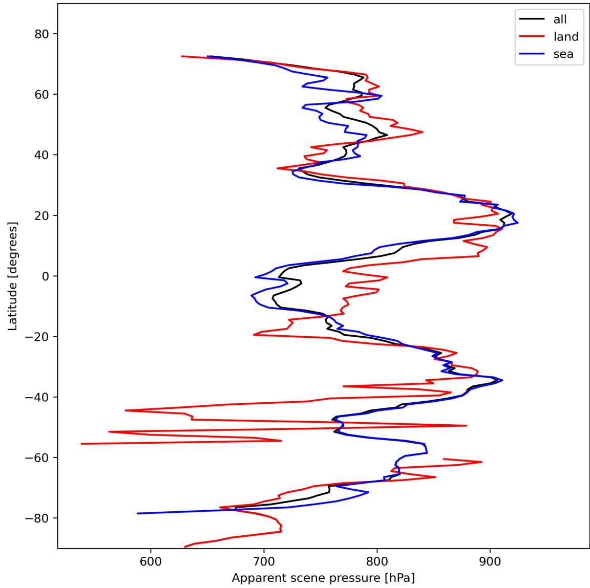
Figure 19: Zonal average of “Apparent scene pressure” for 2024-02-06 to 2024-02-07.
