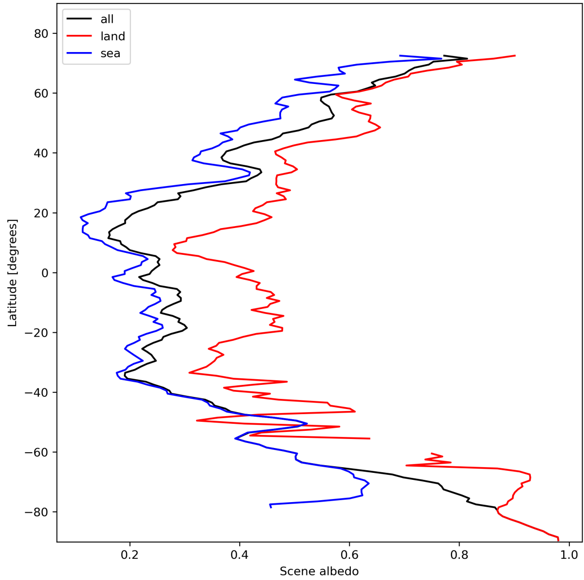
Figure 17: Zonal average of “Scene albedo” for 2024-02-06 to 2024-02-07.
