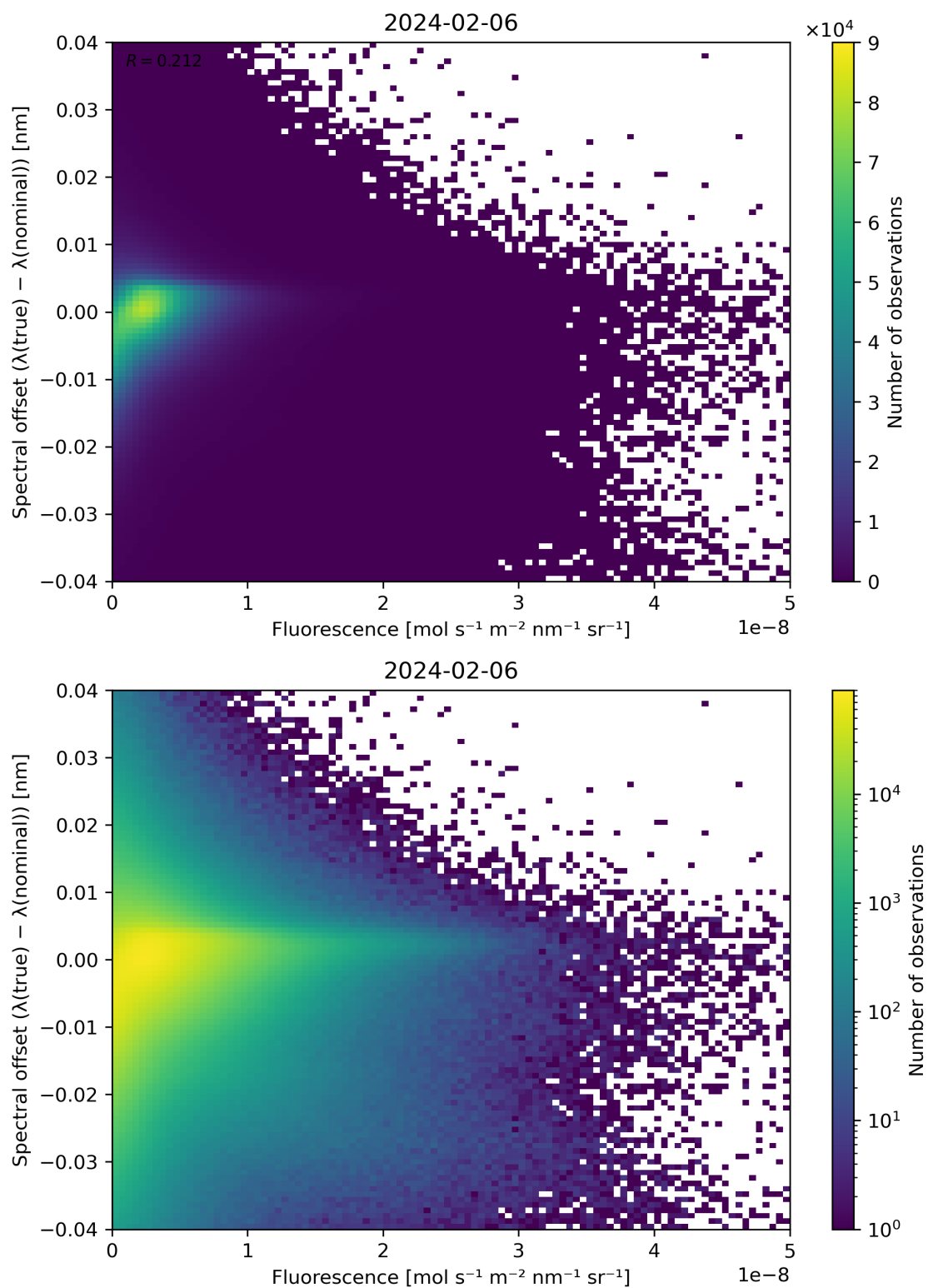
Figure 87: Scatter density plot of “Fluorescence” against “Spectral offset ( \lambda(\text{true}) - \lambda(\text{nominal}) )” for 2024-02-06 to 2024-02-07.
