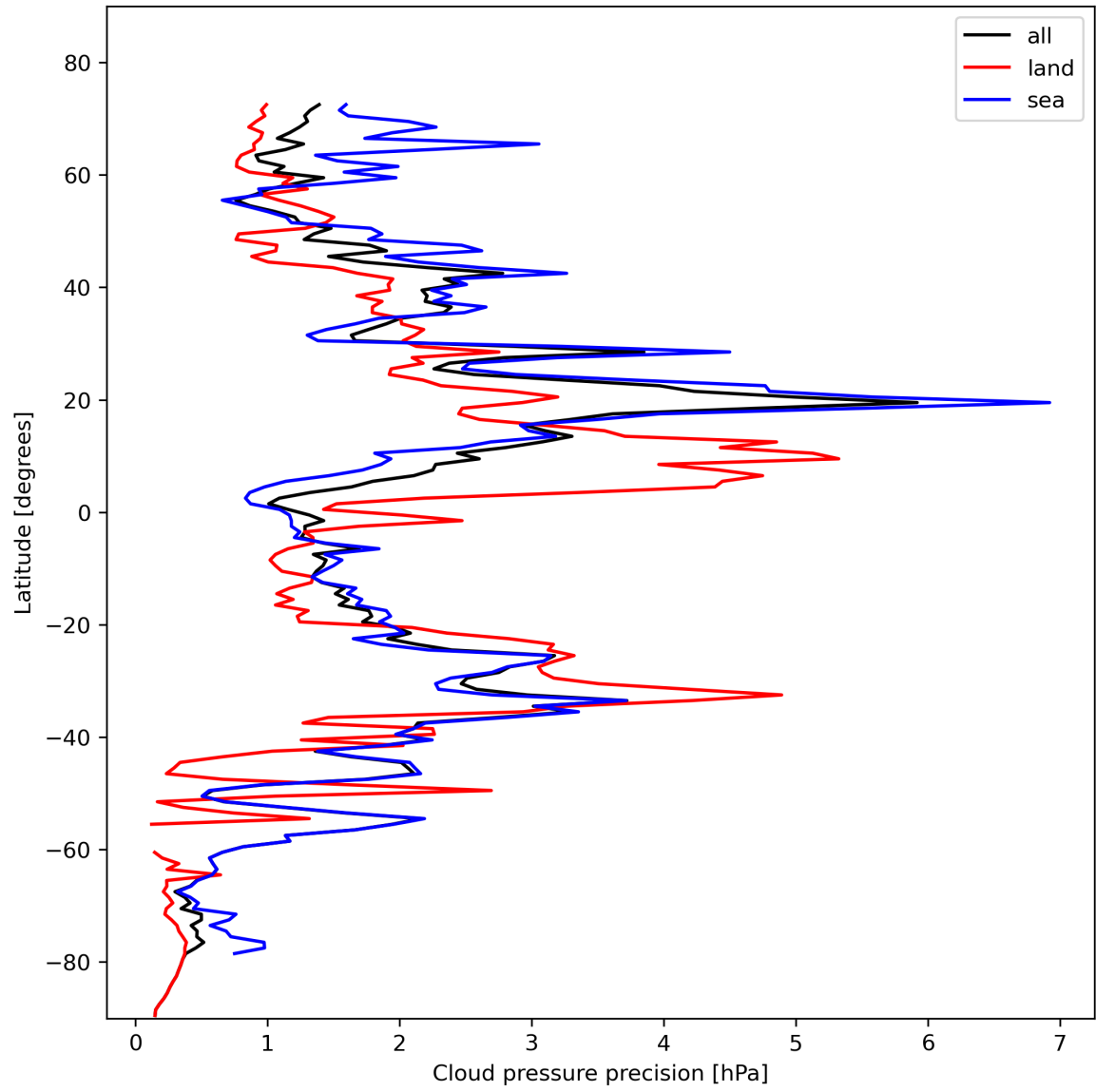
Figure 14: Zonal average of “Cloud pressure precision” for 2024-02-06 to 2024-02-07.
