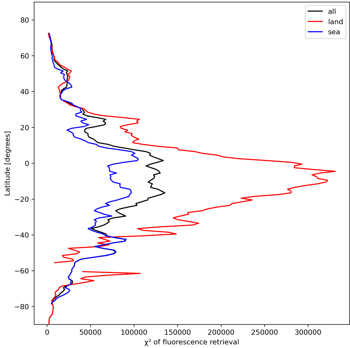
Figure 25: Zonal average of “ \chi^2 of fluorescence retrieval” for 2024-02-06 to 2024-02-07.
