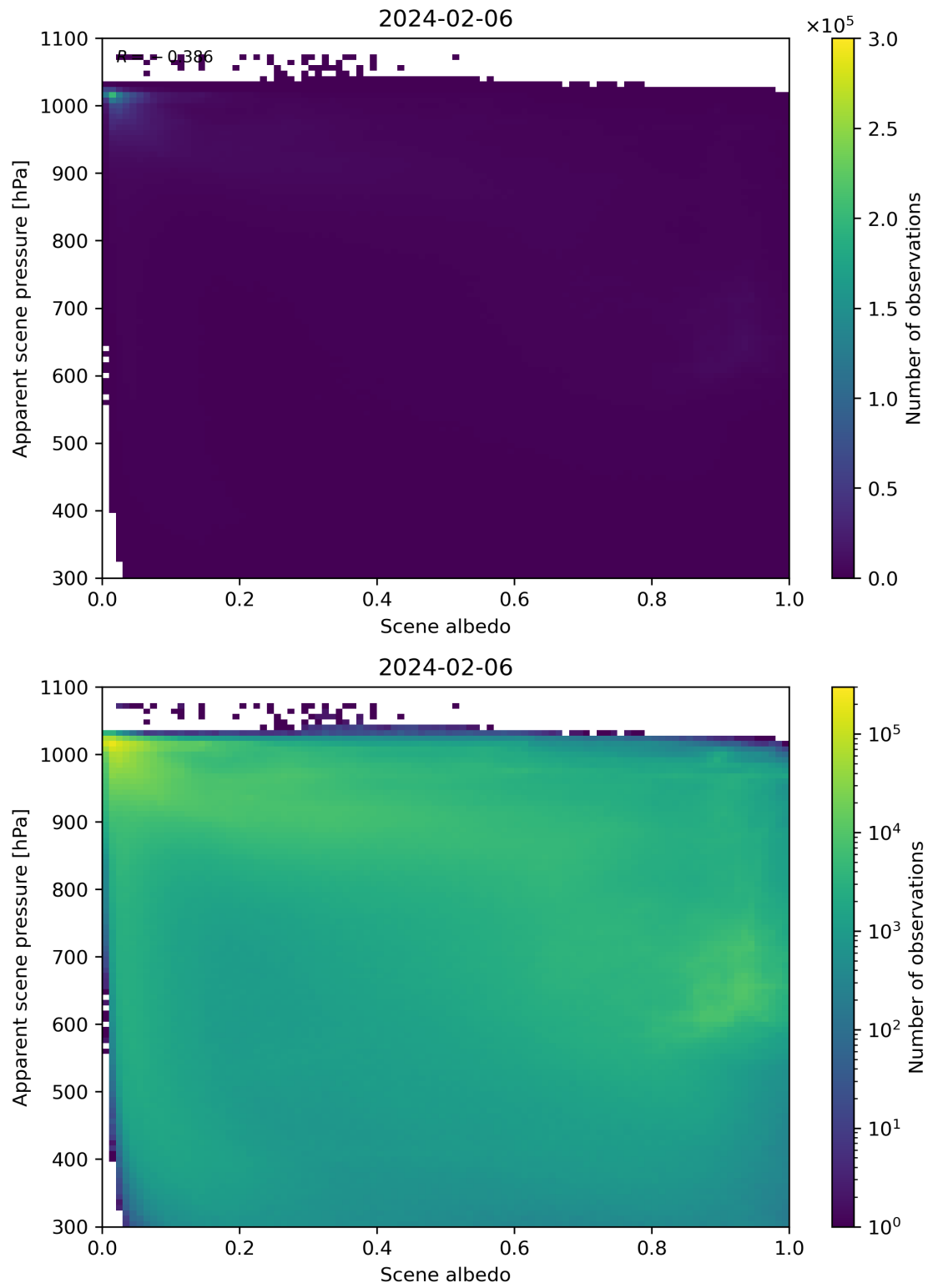
Figure 102: Scatter density plot of “Scene albedo” against “Apparent scene pressure” for 2024-02-06 to 2024-02-07.
