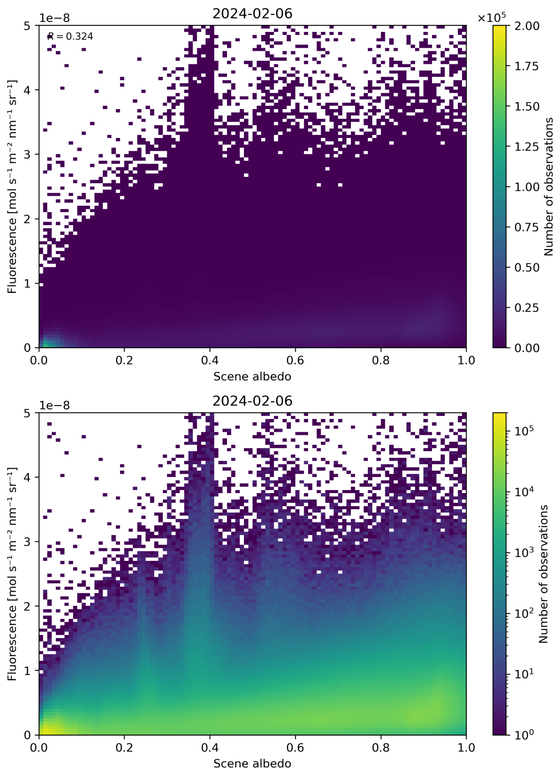
Figure 104: Scatter density plot of “Scene albedo” against “Fluorescence” for 2024-02-06 to 2024-02-07.
