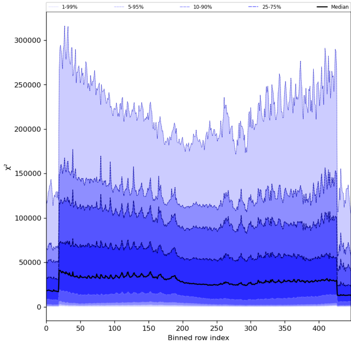
Figure 55: Along track statistics of “ \chi^2 ” for 2024-02-06 to 2024-02-07
