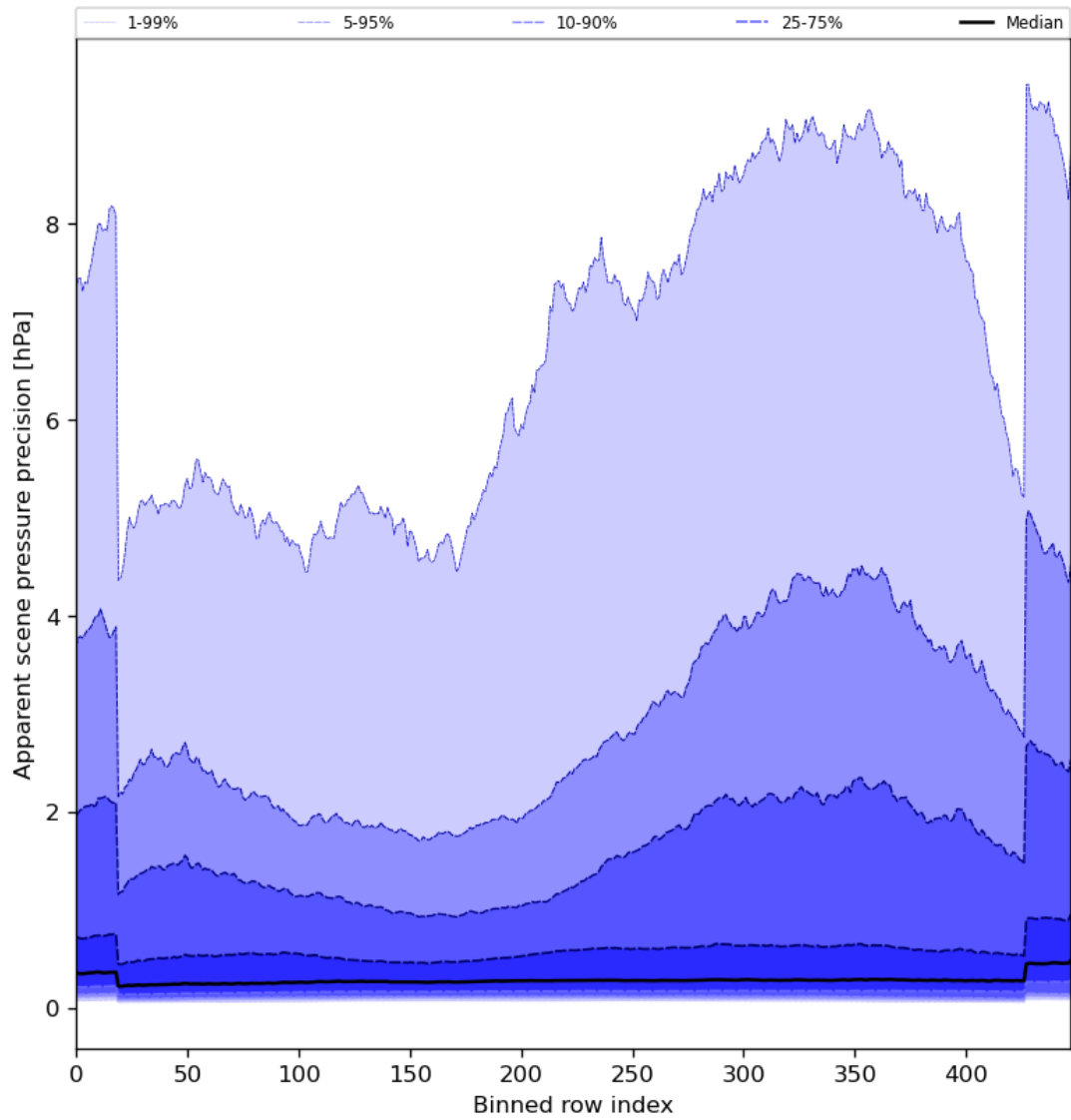
Figure 54: Along track statistics of “Apparent scene pressure precision” for 2024-02-06 to 2024-02-07
