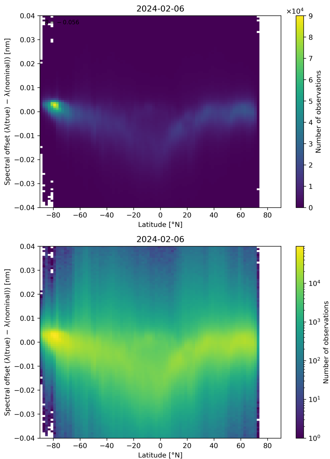
Figure 96: Scatter density plot of “Latitude” against “Spectral offset ( \lambda(\text{true}) - \lambda(\text{nominal}) )” for 2024-02-06 to 2024-02-07.
