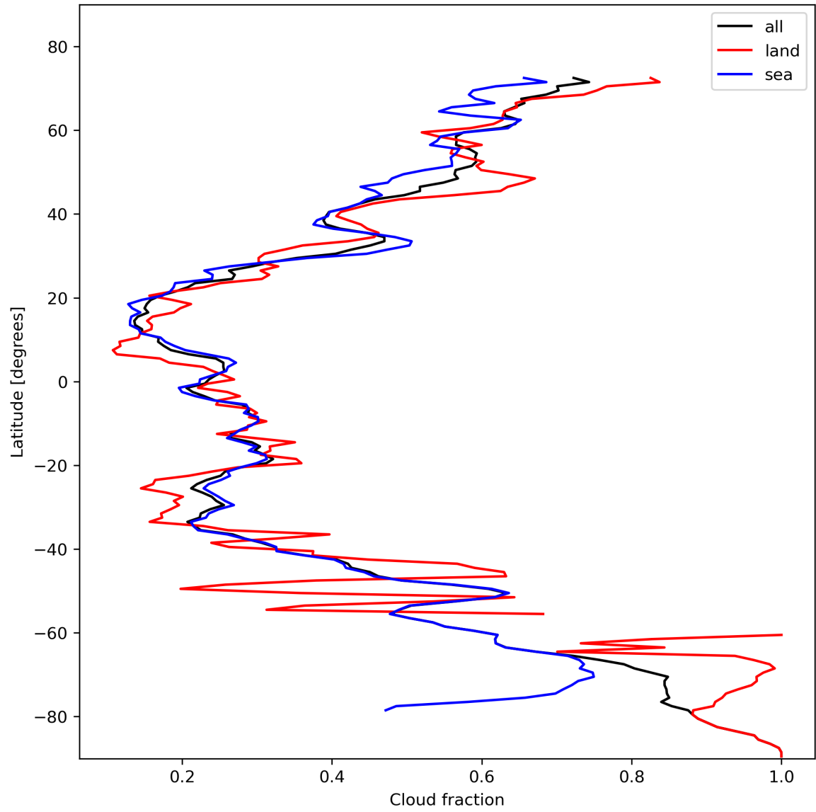
Figure 15: Zonal average of “Cloud fraction” for 2024-02-06 to 2024-02-07.
