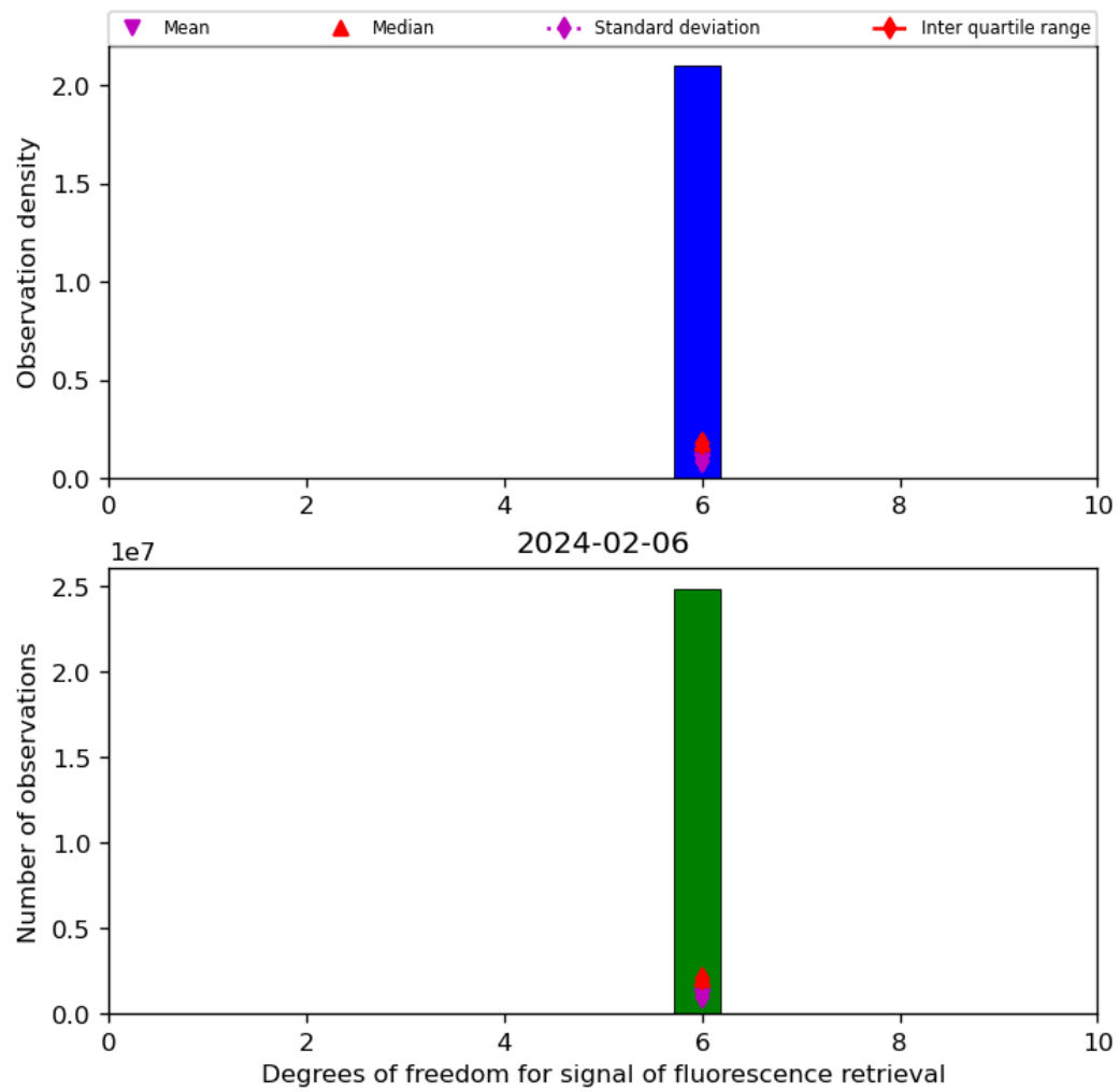
Figure 43: Histogram of “Degrees of freedom for signal of fluorescence retrieval” for 2024-02-06 to 2024-02-07
