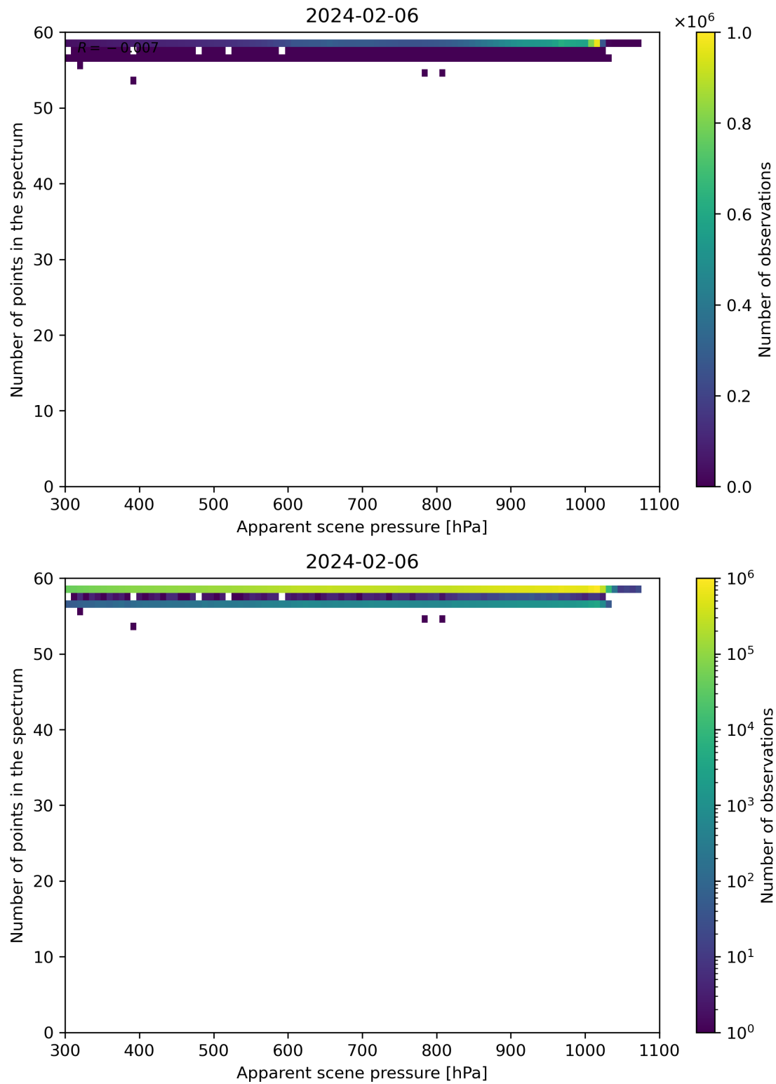
Figure 66: Scatter density plot of “Apparent scene pressure” against “Number of points in the spectrum” for 2024-02-06 to 2024-02-07.
