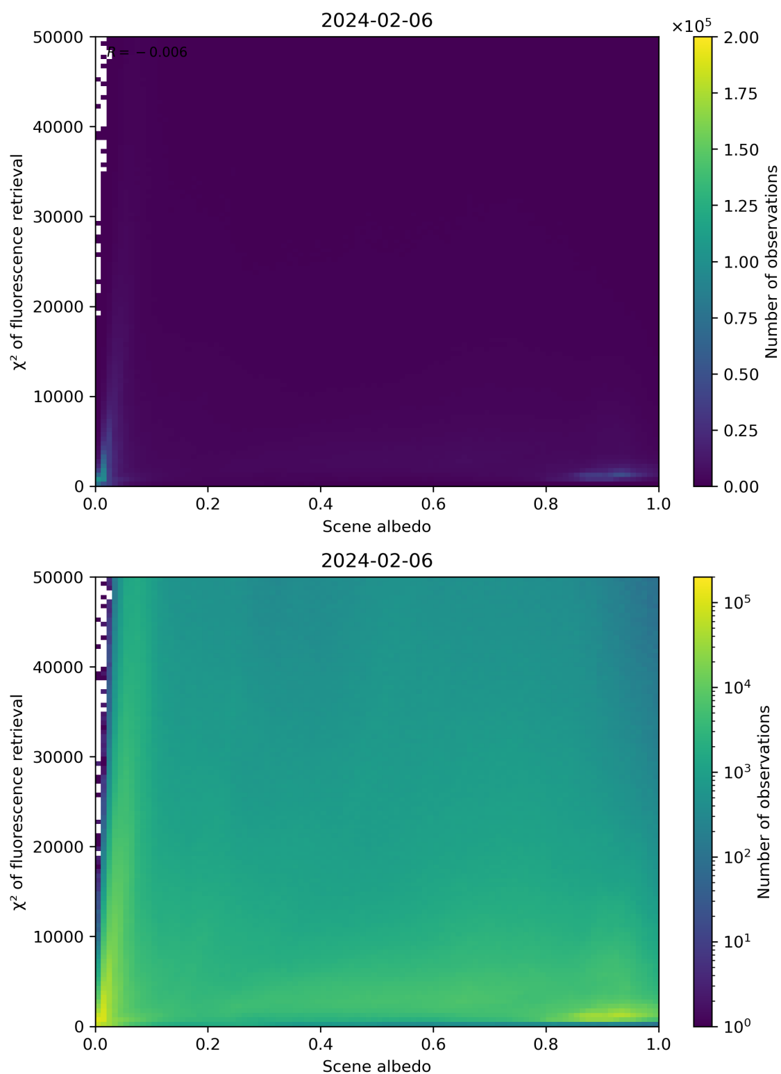
Figure 103: Scatter density plot of “Scene albedo” against “ \chi^2 of fluorescence retrieval” for 2024-02-06 to 2024-02-07.
