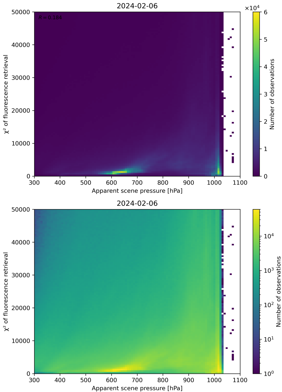
Figure 63: Scatter density plot of “Apparent scene pressure” against “ \chi^2 of fluorescence retrieval” for 2024-02-06 to 2024-02-07.
