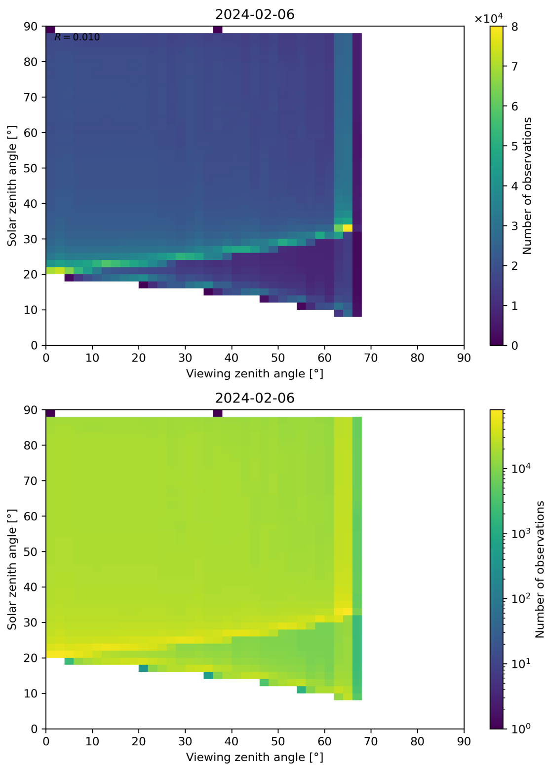
Figure 127: Scatter density plot of “Viewing zenith angle” against “Solar zenith angle” for 2024-02-06 to 2024-02-07.
