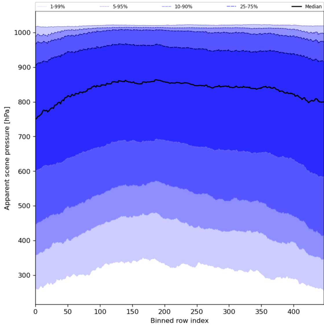
Figure 53: Along track statistics of “Apparent scene pressure” for 2024-02-06 to 2024-02-07
