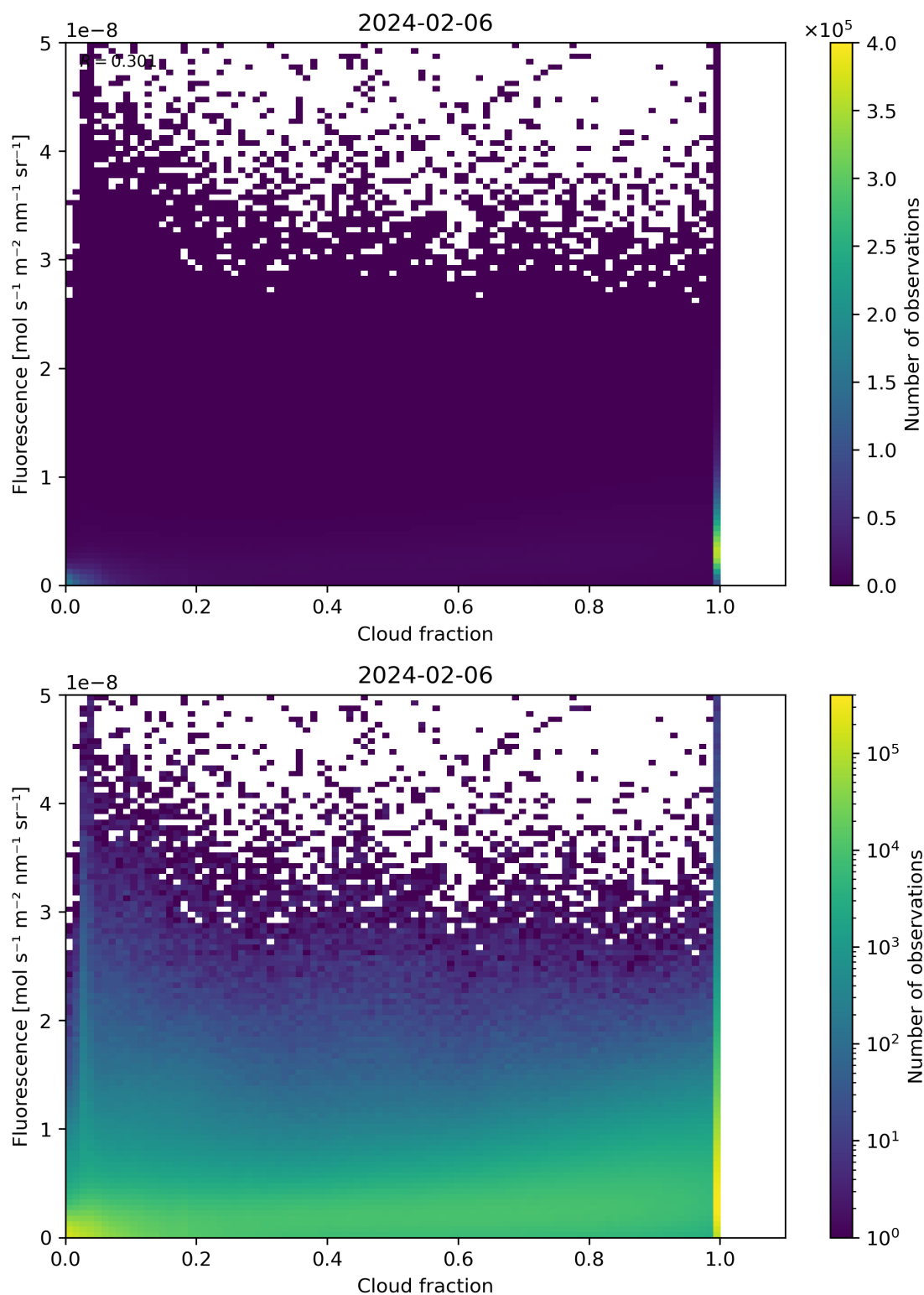
Figure 72: Scatter density plot of “Cloud fraction” against “Fluorescence” for 2024-02-06 to 2024-02-07.
