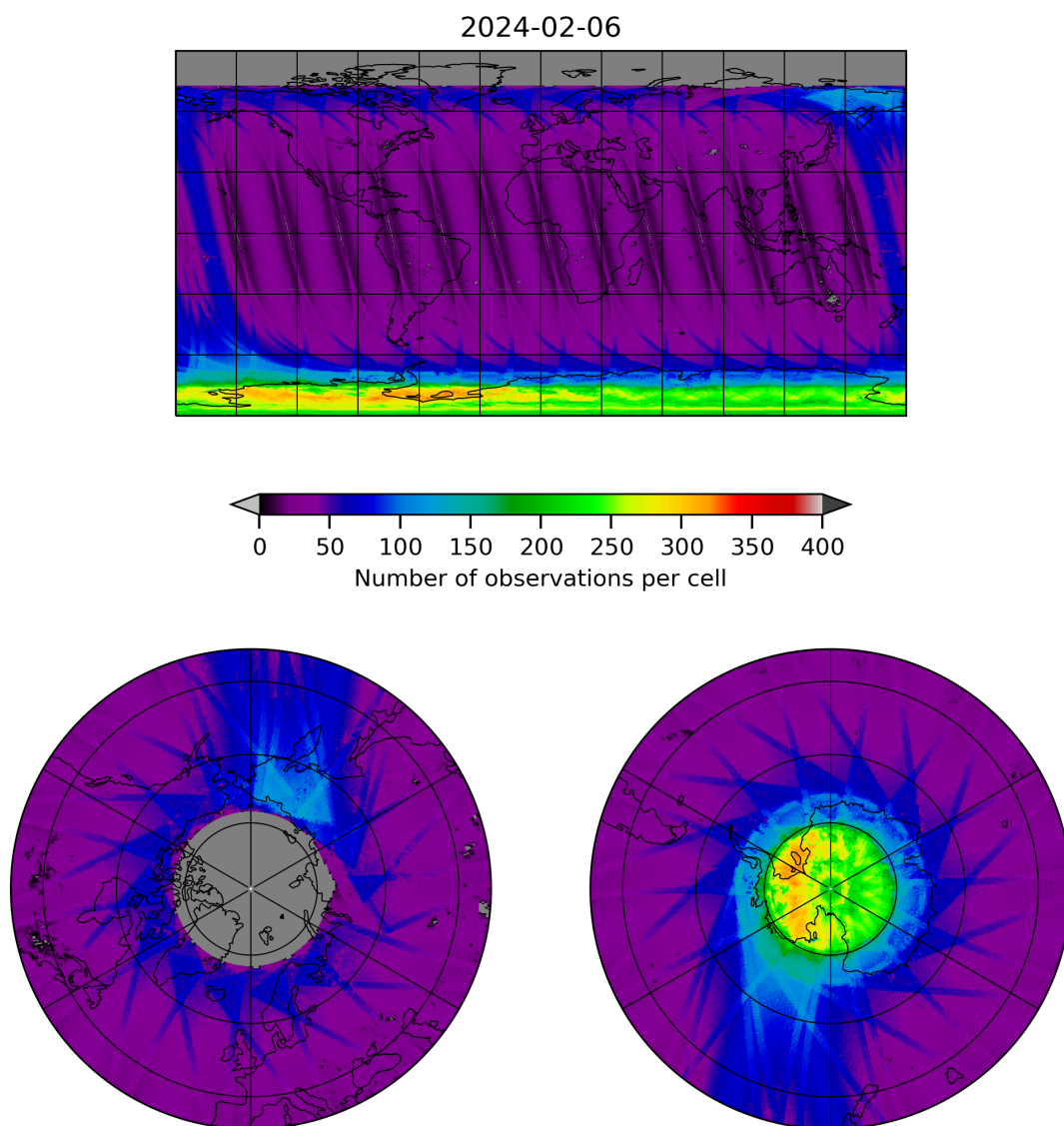
Figure 11: Map of the number of observations for 2024-02-06 to 2024-02-07
