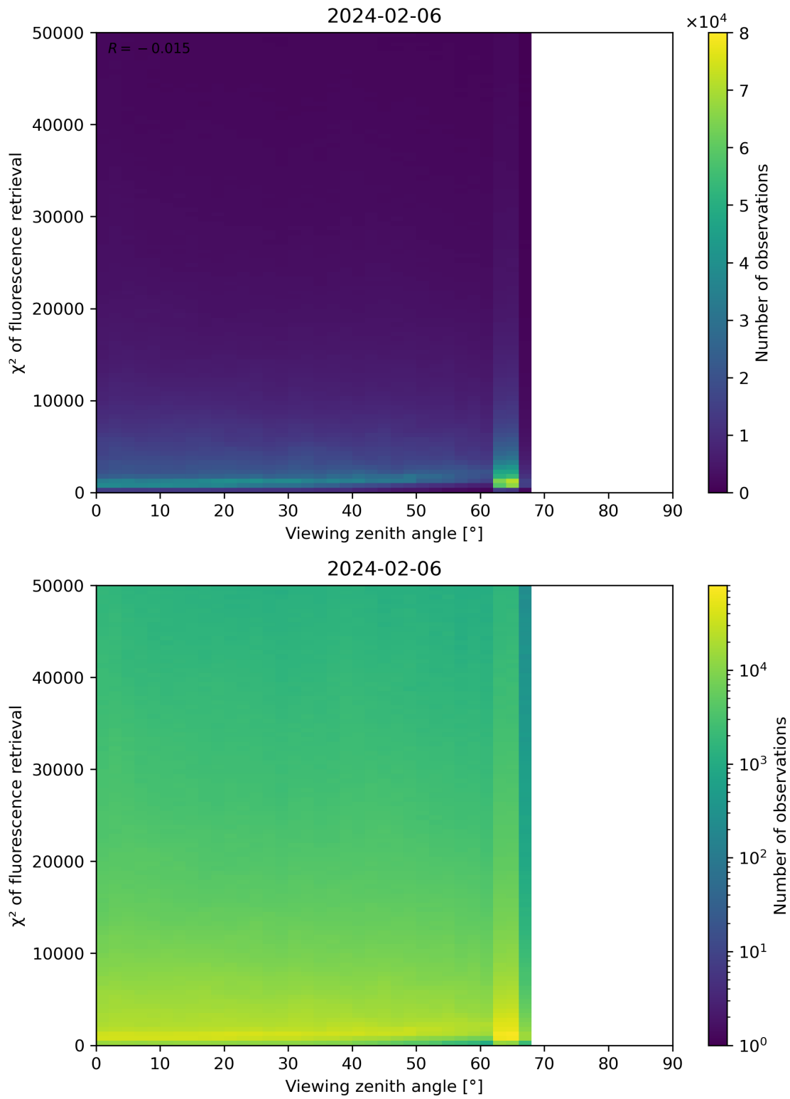
Figure 119: Scatter density plot of “Viewing zenith angle” against “ \chi^2 of fluorescence retrieval” for 2024-02-06 to 2024-02-07.
