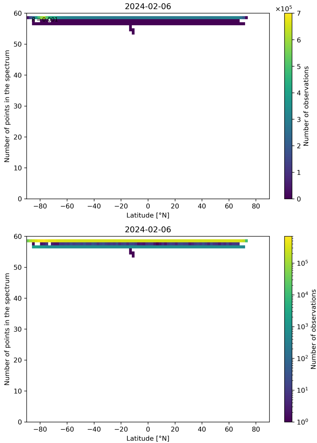
Figure 94: Scatter density plot of “Latitude” against “Number of points in the spectrum” for 2024-02-06 to 2024-02-07.
