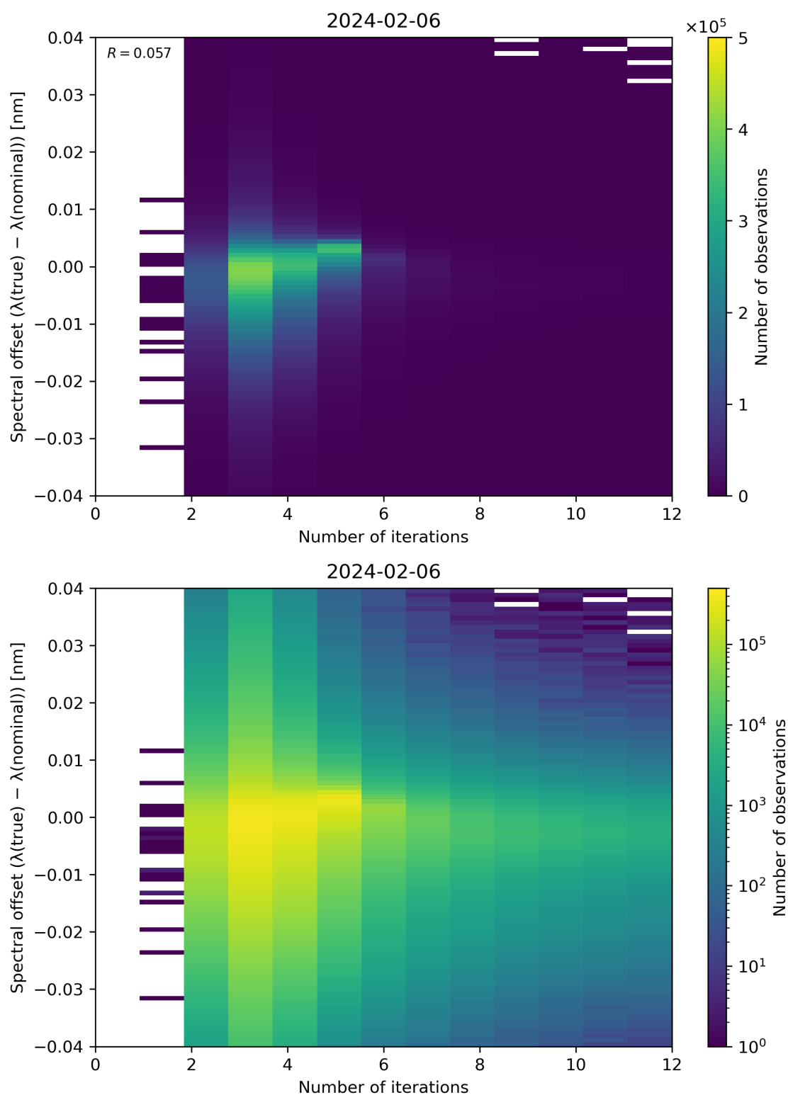
Figure 100: Scatter density plot of “Number of iterations” against “Spectral offset ( \lambda(\text{true}) - \lambda(\text{nominal}) )” for 2024-02-06 to 2024-02-07.
