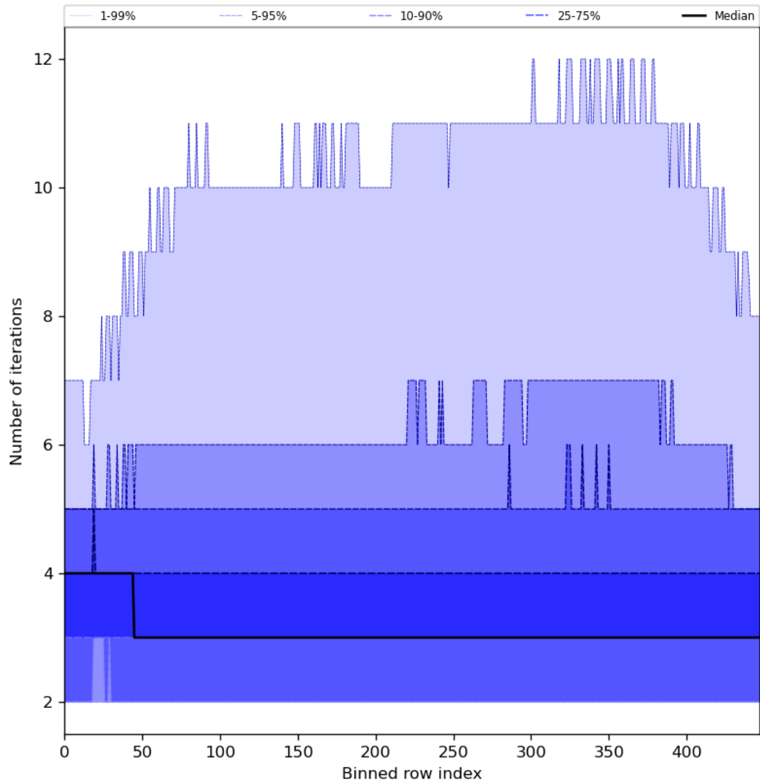
Figure 56: Along track statistics of “Number of iterations” for 2024-02-06 to 2024-02-07
