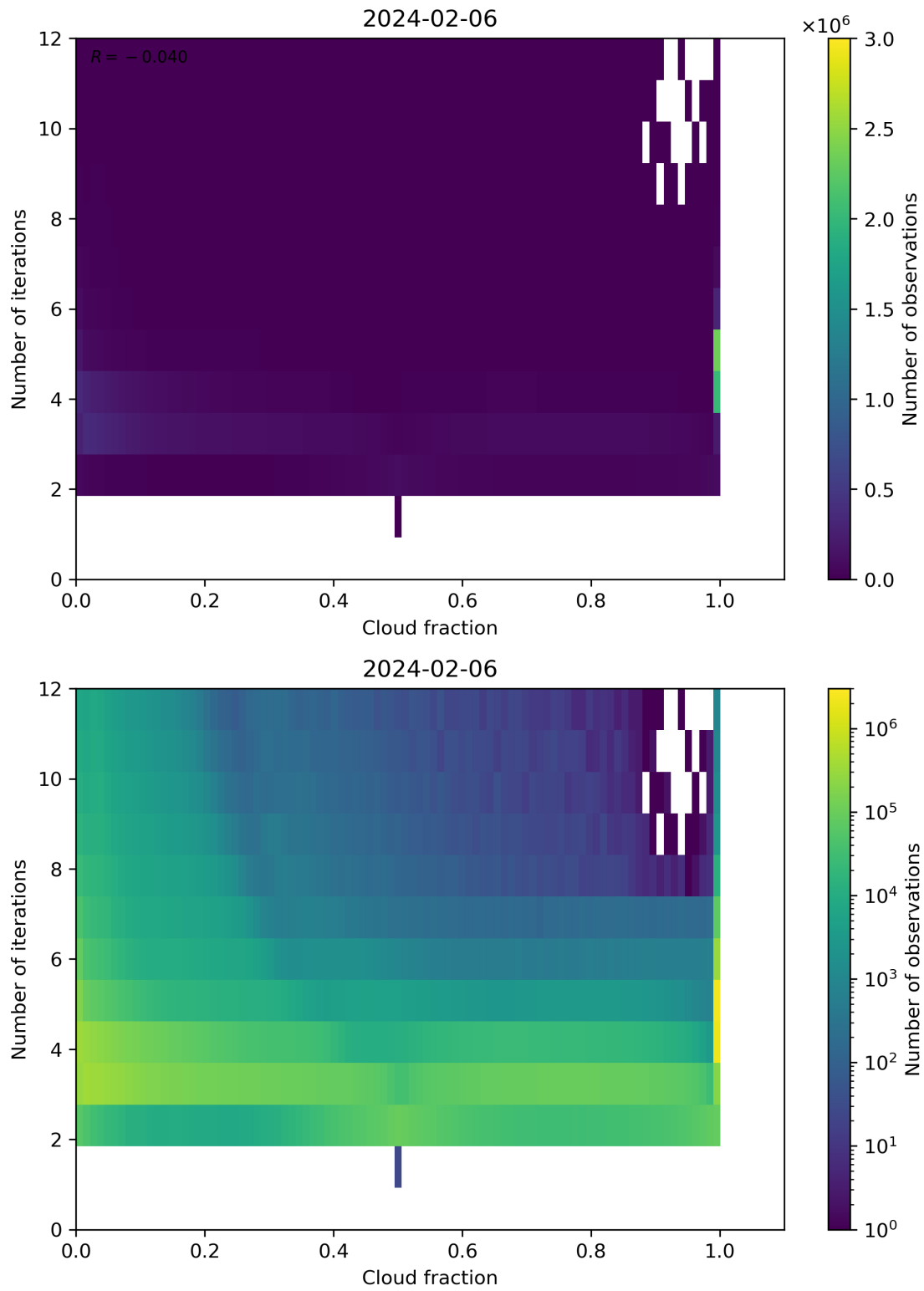
Figure 73: Scatter density plot of “Cloud fraction” against “Number of iterations” for 2024-02-06 to 2024-02-07.
