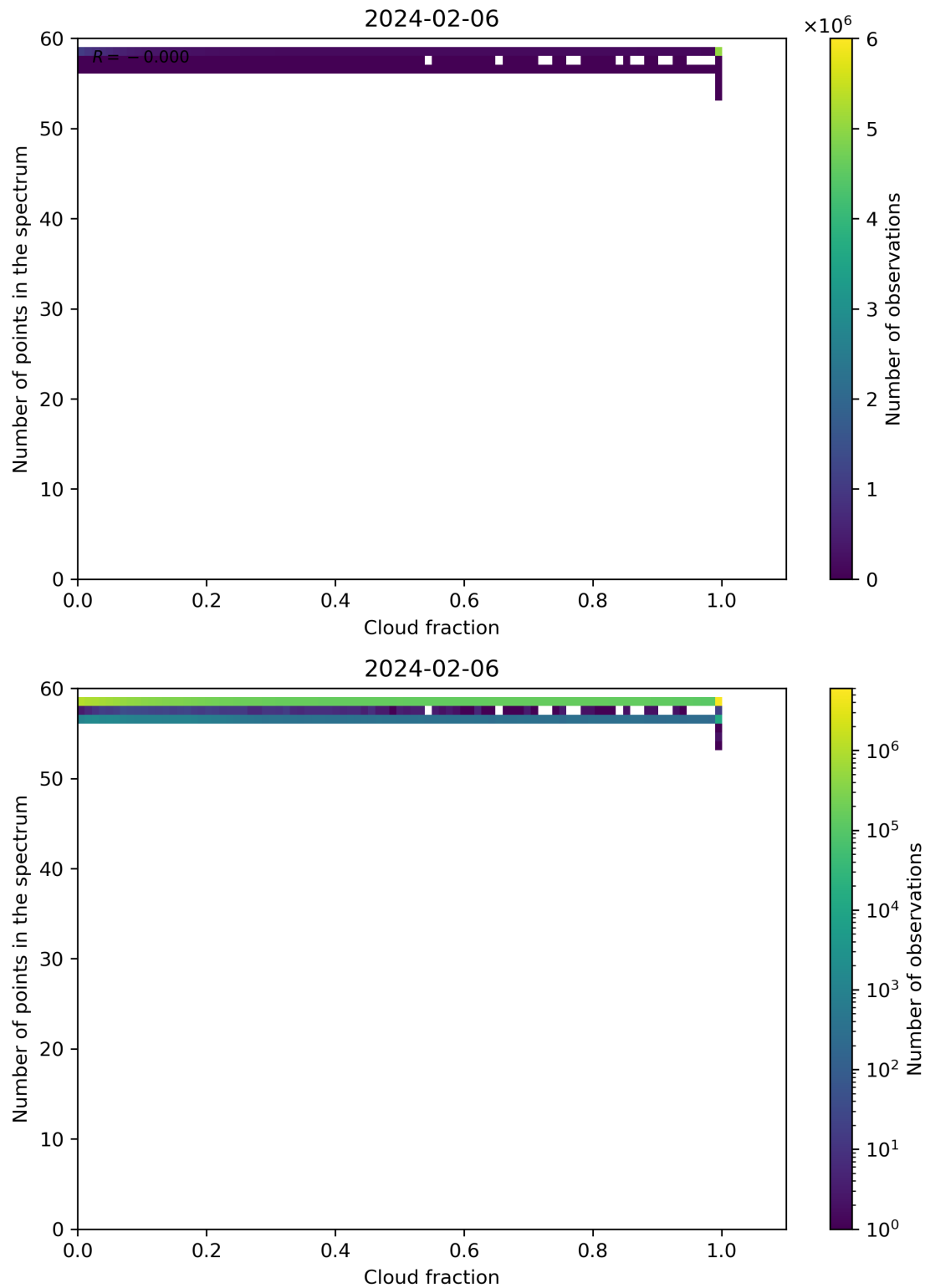
Figure 74: Scatter density plot of “Cloud fraction” against “Number of points in the spectrum” for 2024-02-06 to 2024-02-07.
