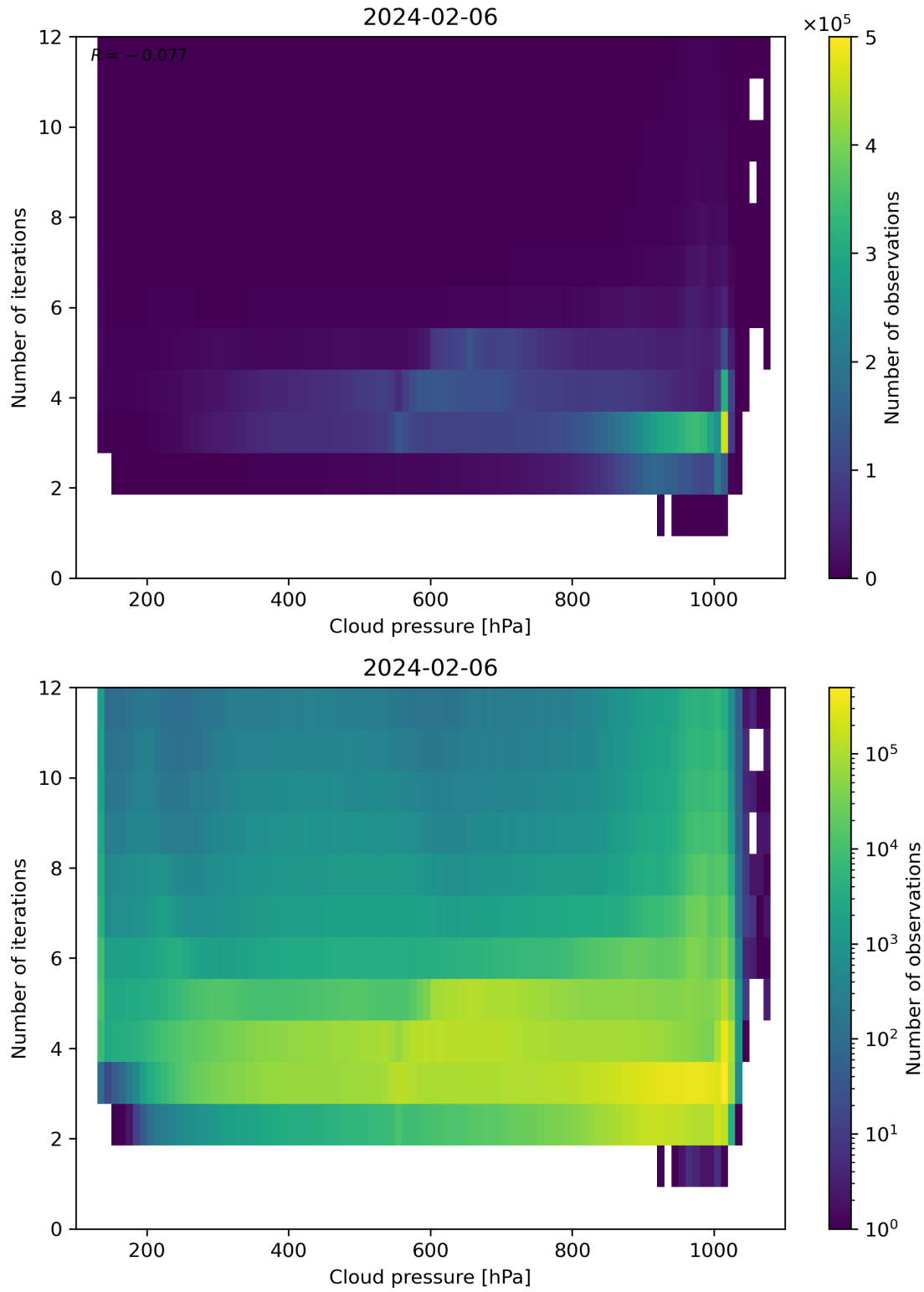
Figure 81: Scatter density plot of “Cloud pressure” against “Number of iterations” for 2024-02-06 to 2024-02-07.
