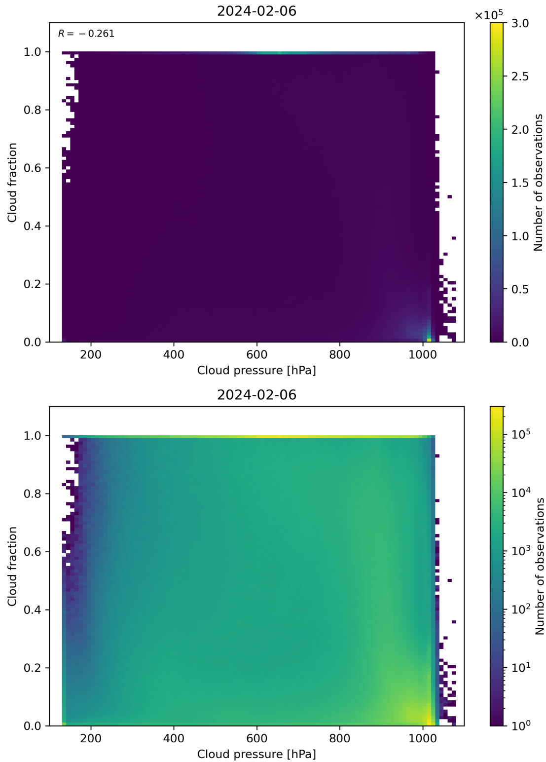
Figure 79: Scatter density plot of “Cloud pressure” against “Cloud fraction” for 2024-02-06 to 2024-02-07.
