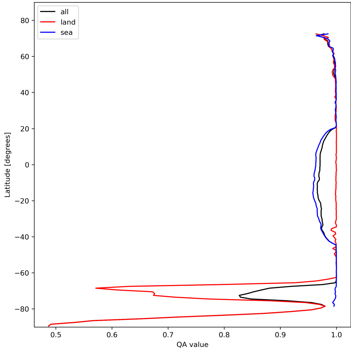
Figure 12: Zonal average of “QA value” for 2024-02-06 to 2024-02-07.
