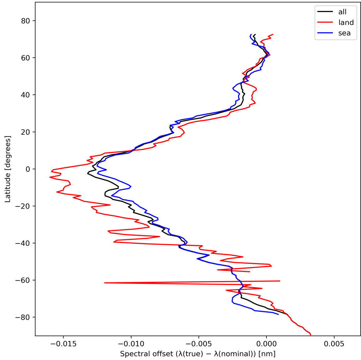
Figure 28: Zonal average of “Spectral offset ( \lambda(\text{true}) - \lambda(\text{nominal}) )” for 2024-02-06 to 2024-02-07.
