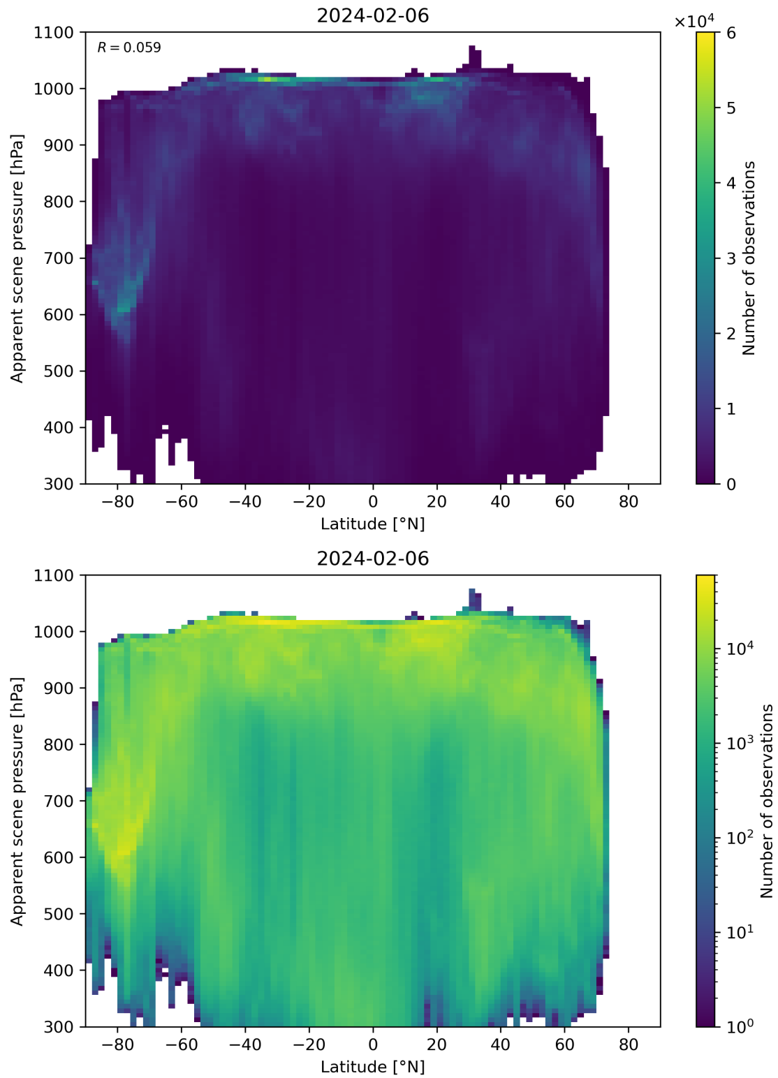
Figure 88: Scatter density plot of “Latitude” against “Apparent scene pressure” for 2024-02-06 to 2024-02-07.
