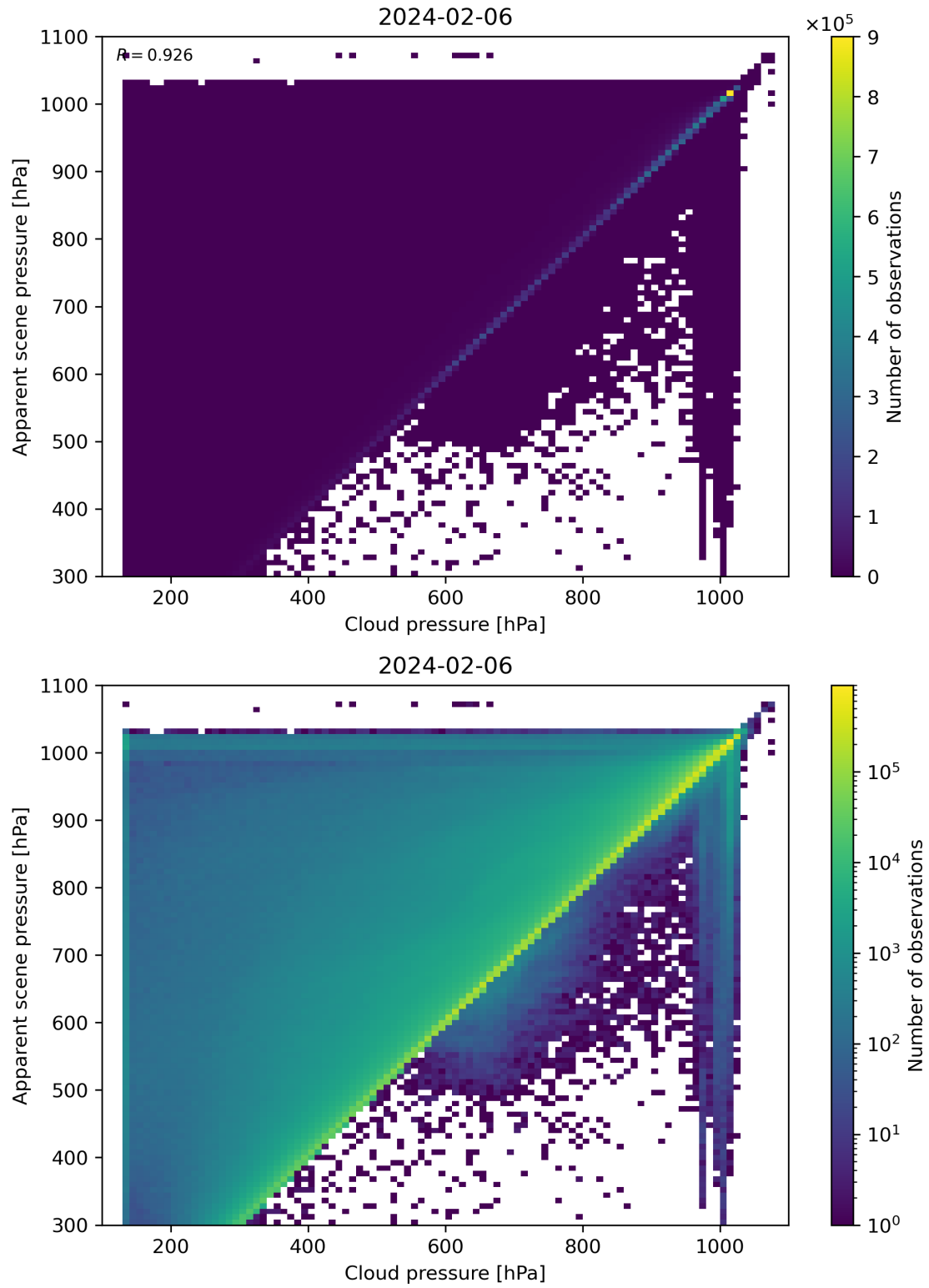
Figure 77: Scatter density plot of “Cloud pressure” against “Apparent scene pressure” for 2024-02-06 to 2024-02-07.
