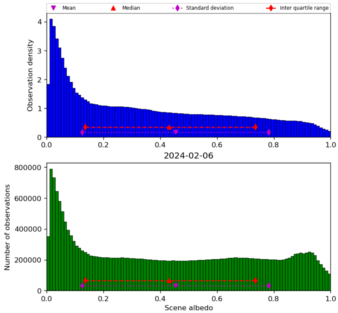
Figure 34: Histogram of “Scene albedo” for 2024-02-06 to 2024-02-07
