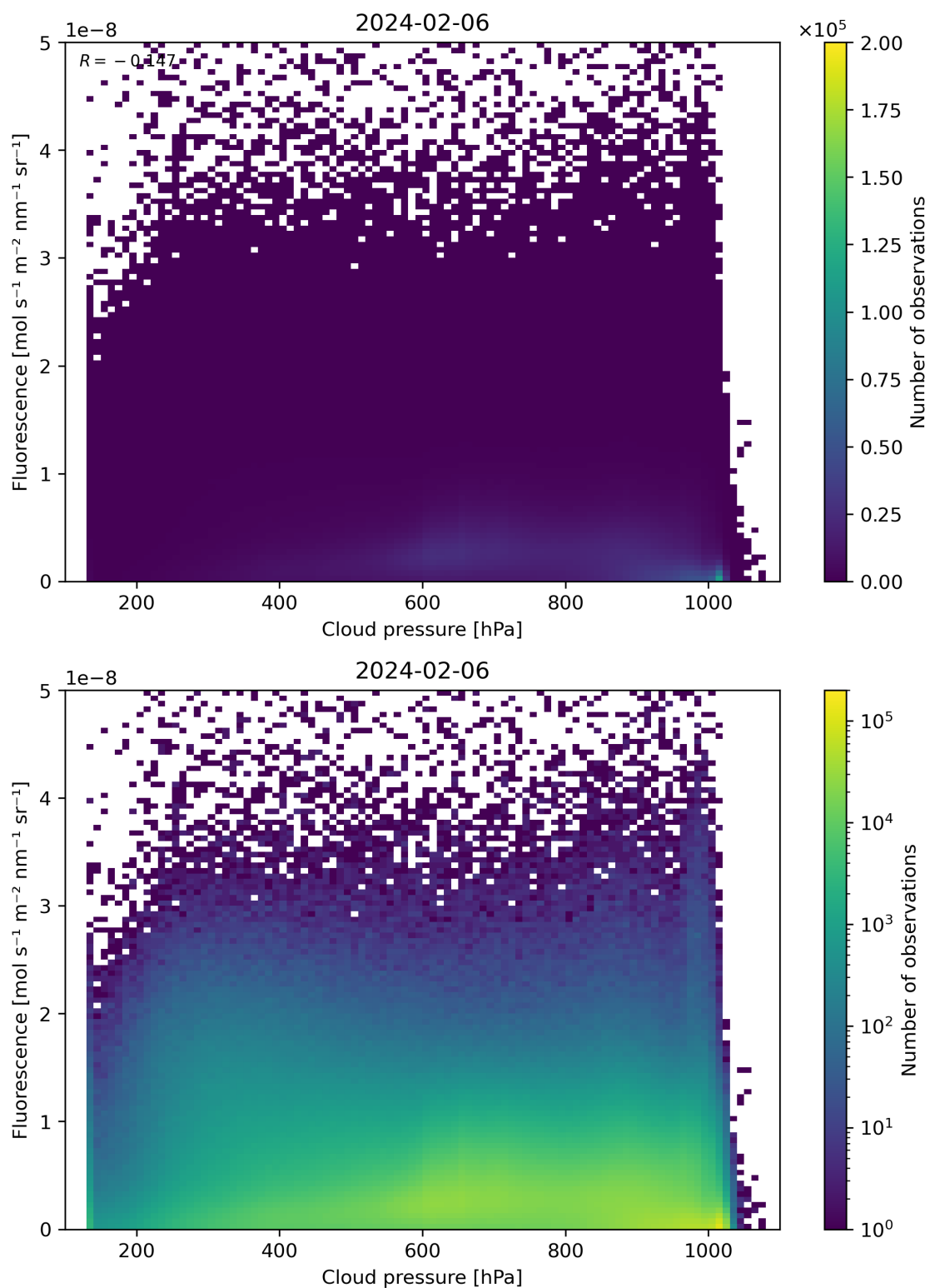
Figure 80: Scatter density plot of “Cloud pressure” against “Fluorescence” for 2024-02-06 to 2024-02-07.
