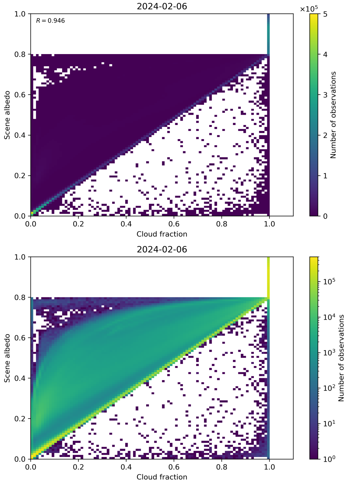
Figure 75: Scatter density plot of “Cloud fraction” against “Scene albedo” for 2024-02-06 to 2024-02-07.
