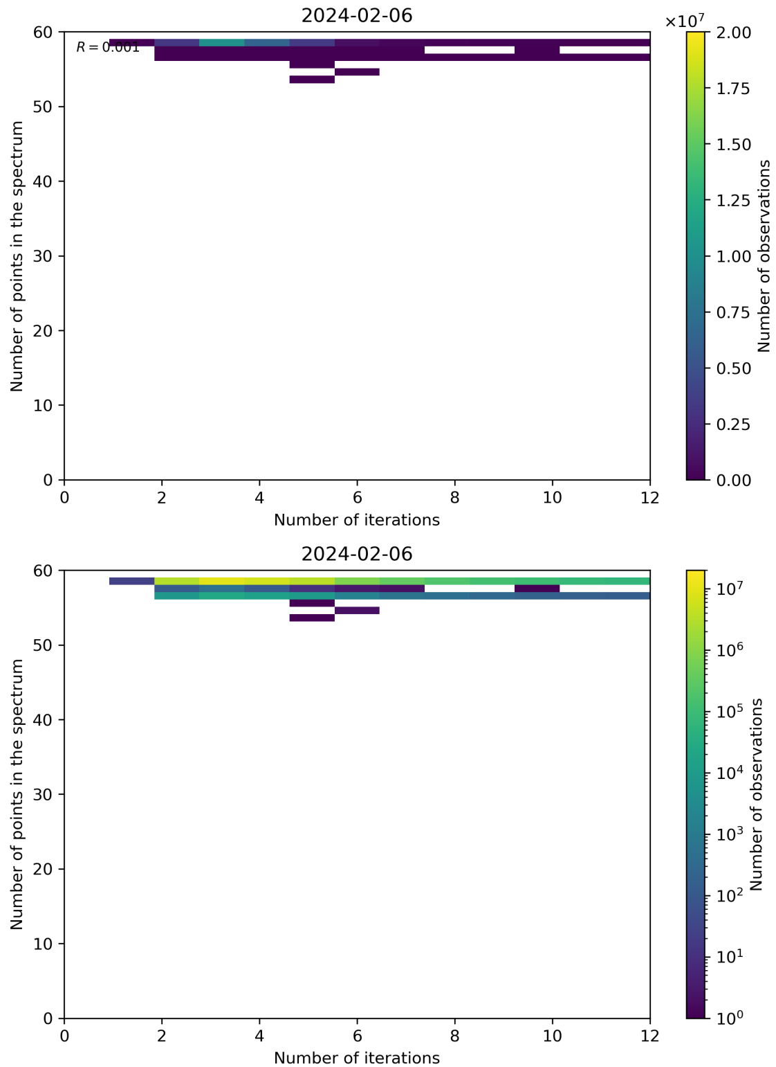
Figure 99: Scatter density plot of “Number of iterations” against “Number of points in the spectrum” for 2024-02-06 to 2024-02-07.
