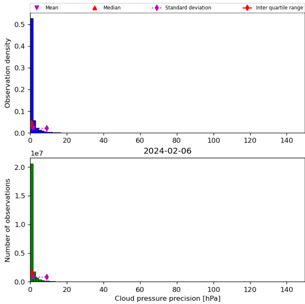
Figure 31: Histogram of “Cloud pressure precision” for 2024-02-06 to 2024-02-07
