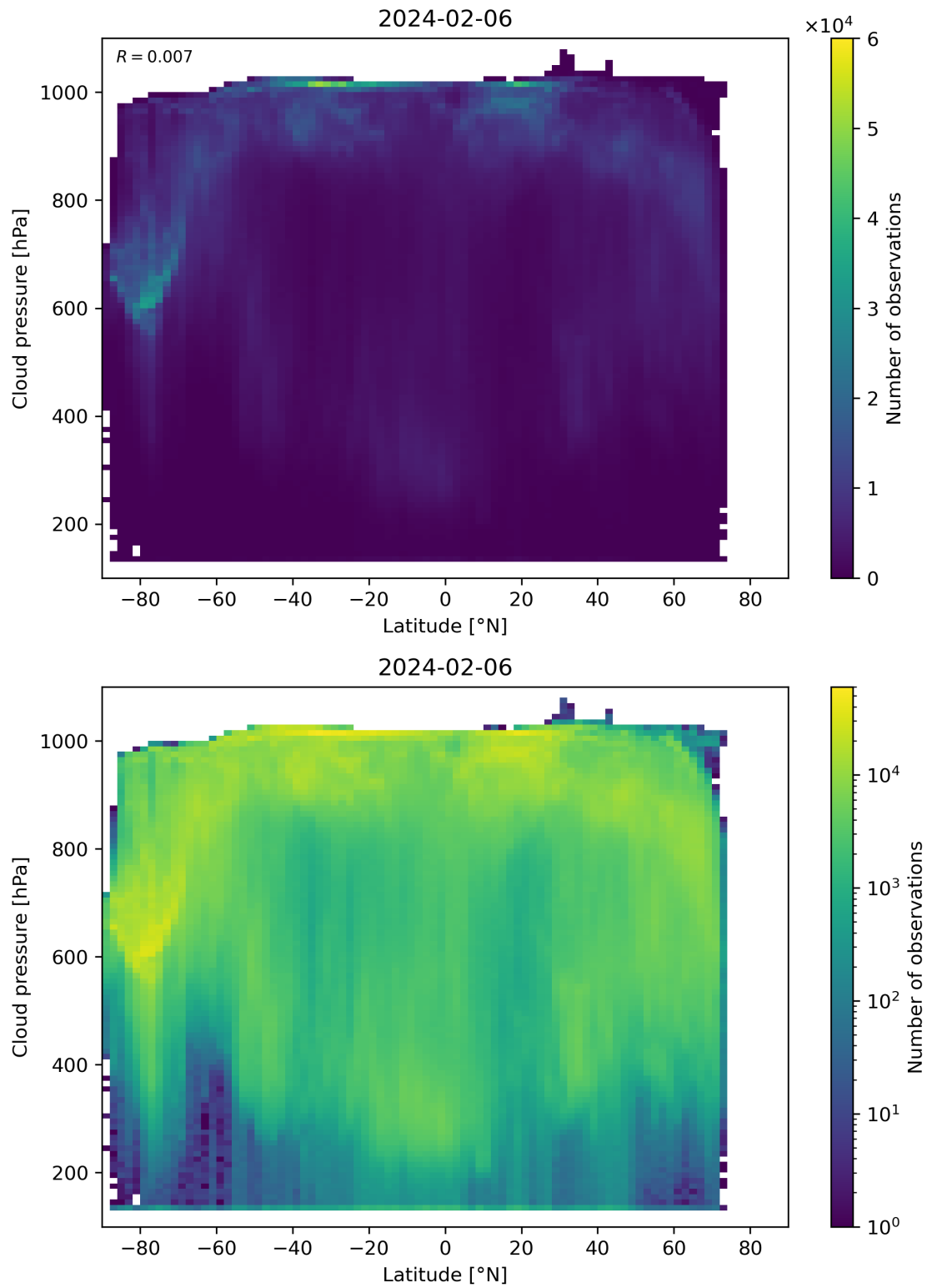
Figure 91: Scatter density plot of “Latitude” against “Cloud pressure” for 2024-02-06 to 2024-02-07.
