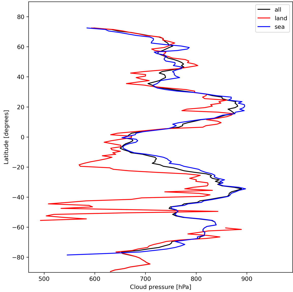
Figure 13: Zonal average of “Cloud pressure” for 2024-02-06 to 2024-02-07.
