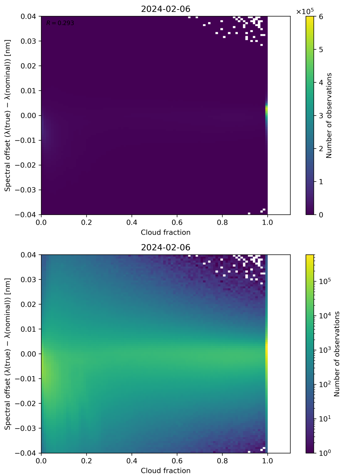
Figure 76: Scatter density plot of “Cloud fraction” against “Spectral offset ( \lambda(\text{true}) - \lambda(\text{nominal}) )” for 2024-02-06 to 2024-02-07.
