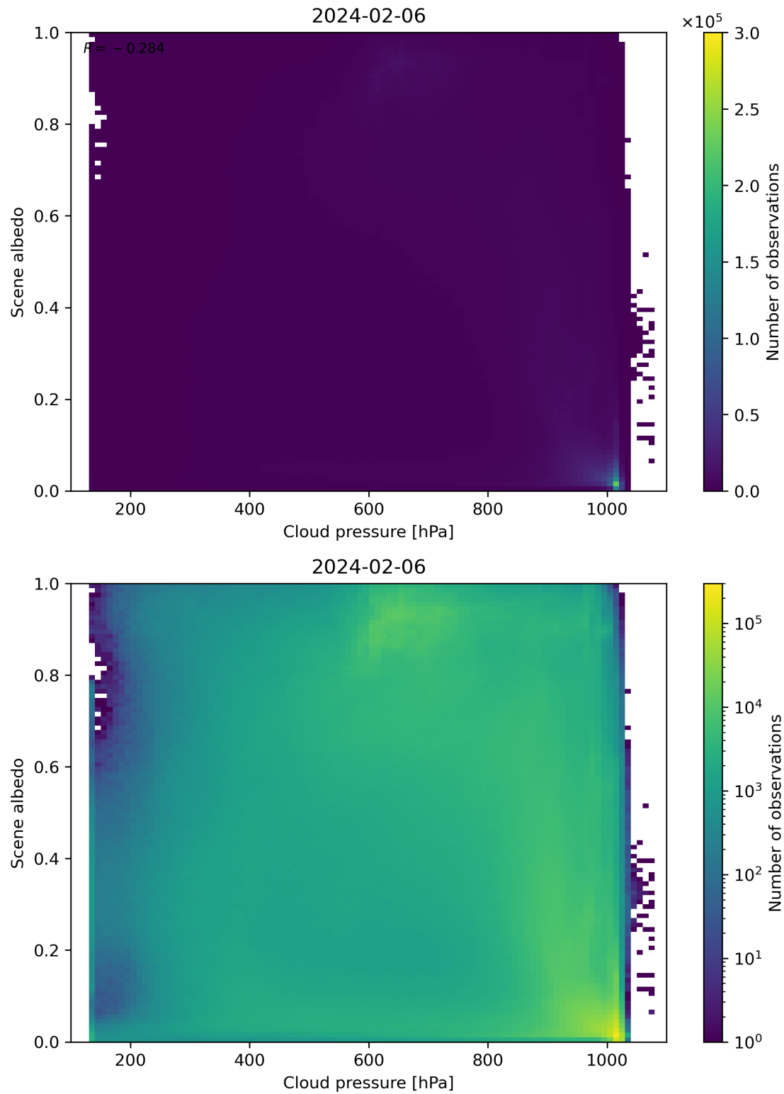
Figure 83: Scatter density plot of “Cloud pressure” against “Scene albedo” for 2024-02-06 to 2024-02-07.
