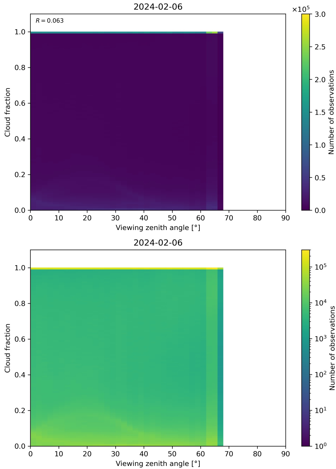
Figure 120: Scatter density plot of “Viewing zenith angle” against “Cloud fraction” for 2024-02-06 to 2024-02-07.
