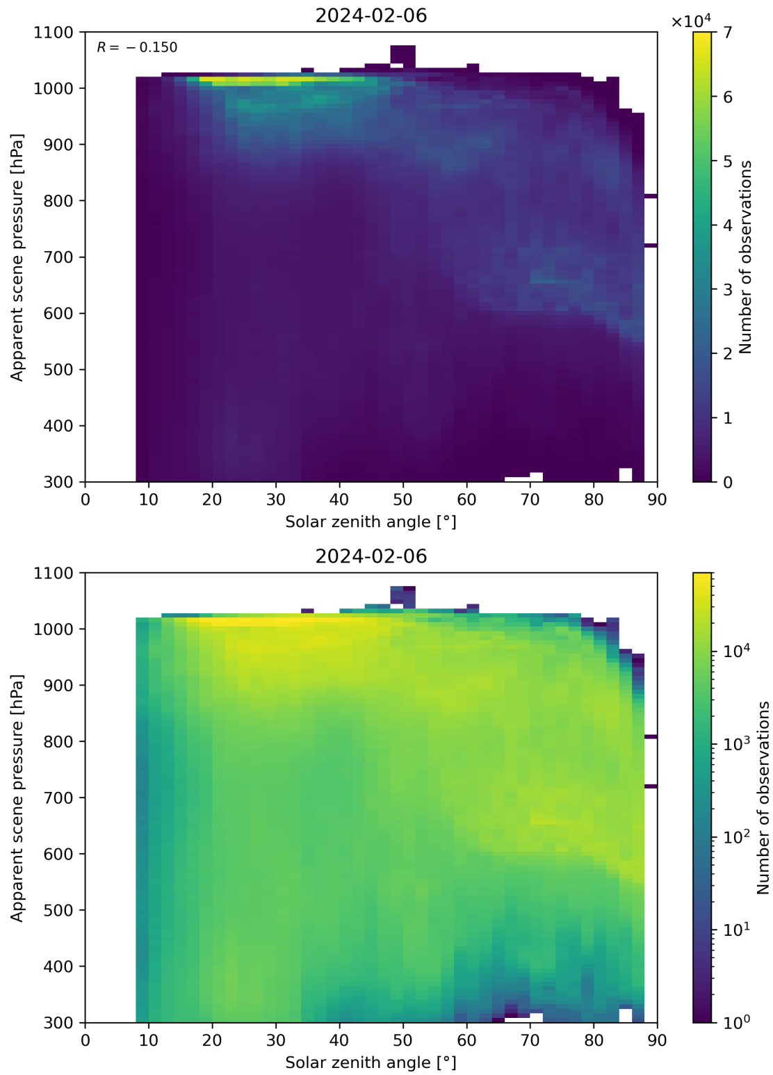
Figure 108: Scatter density plot of “Solar zenith angle” against “Apparent scene pressure” for 2024-02-06 to 2024-02-07.
