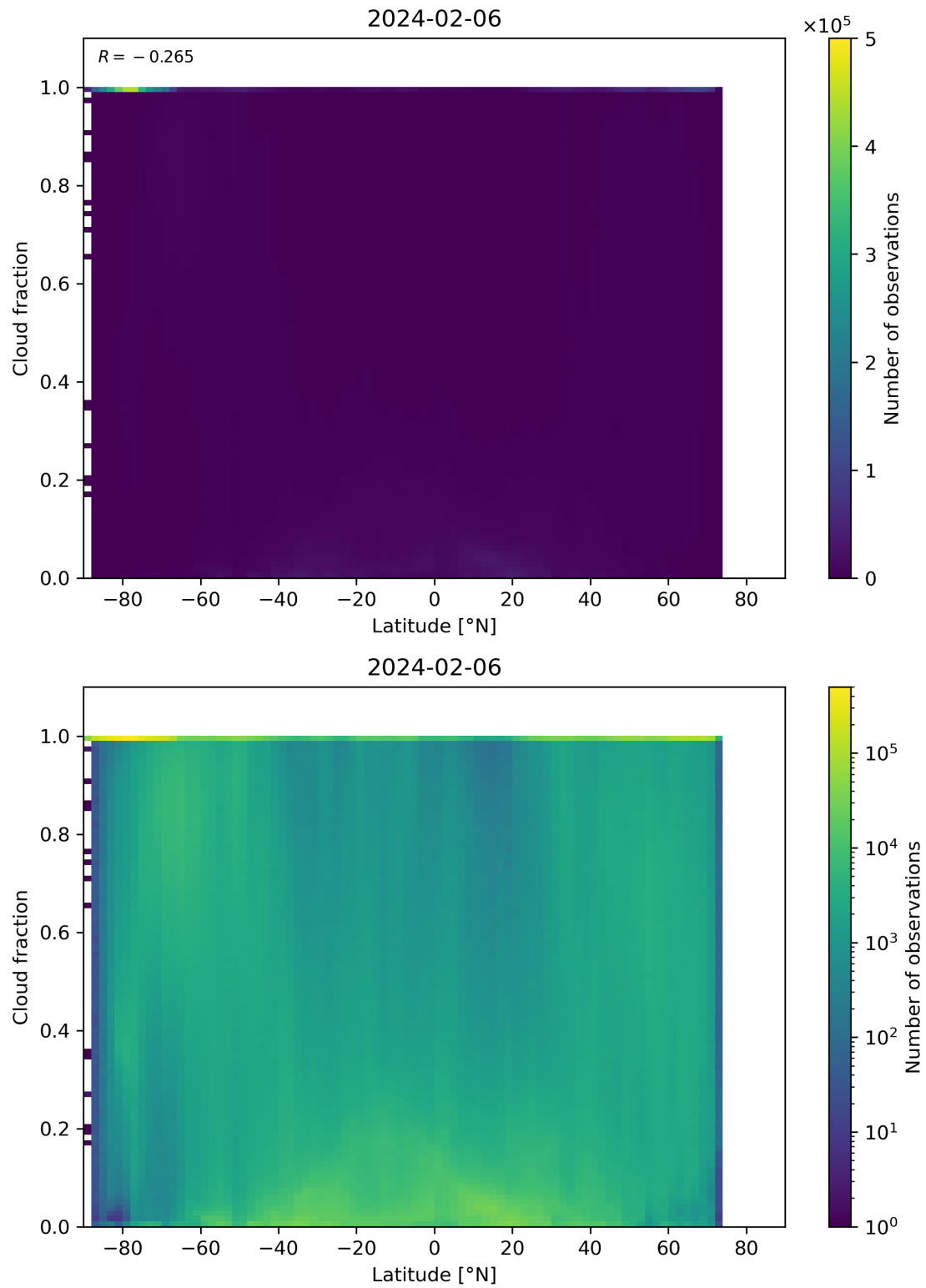
Figure 90: Scatter density plot of “Latitude” against “Cloud fraction” for 2024-02-06 to 2024-02-07.
