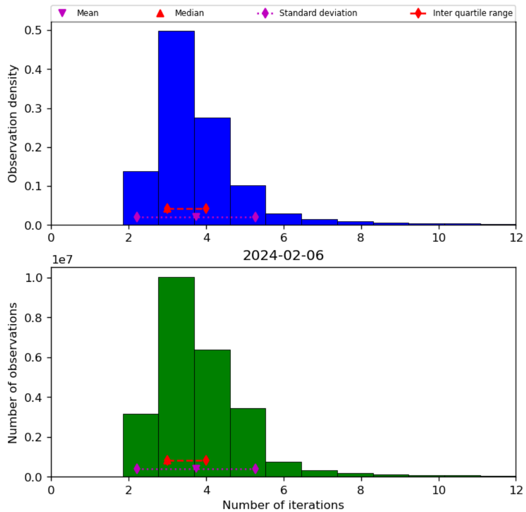
Figure 39: Histogram of “Number of iterations” for 2024-02-06 to 2024-02-07
