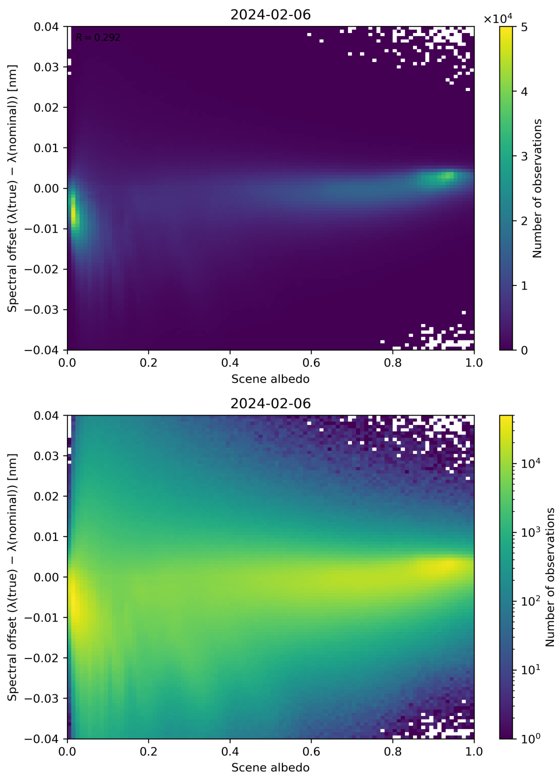
Figure 107: Scatter density plot of “Scene albedo” against “Spectral offset ( \lambda(\text{true}) - \lambda(\text{nominal}) )” for 2024-02-06 to 2024-02-07.
