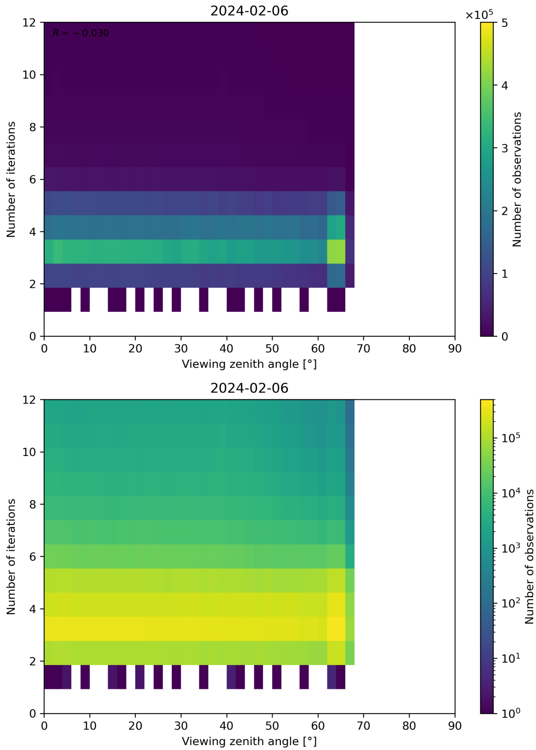
Figure 124: Scatter density plot of “Viewing zenith angle” against “Number of iterations” for 2024-02-06 to 2024-02-07.
