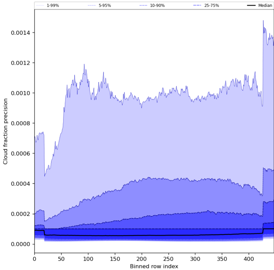
Figure 50: Along track statistics of “Cloud fraction precision” for 2024-02-06 to 2024-02-07
