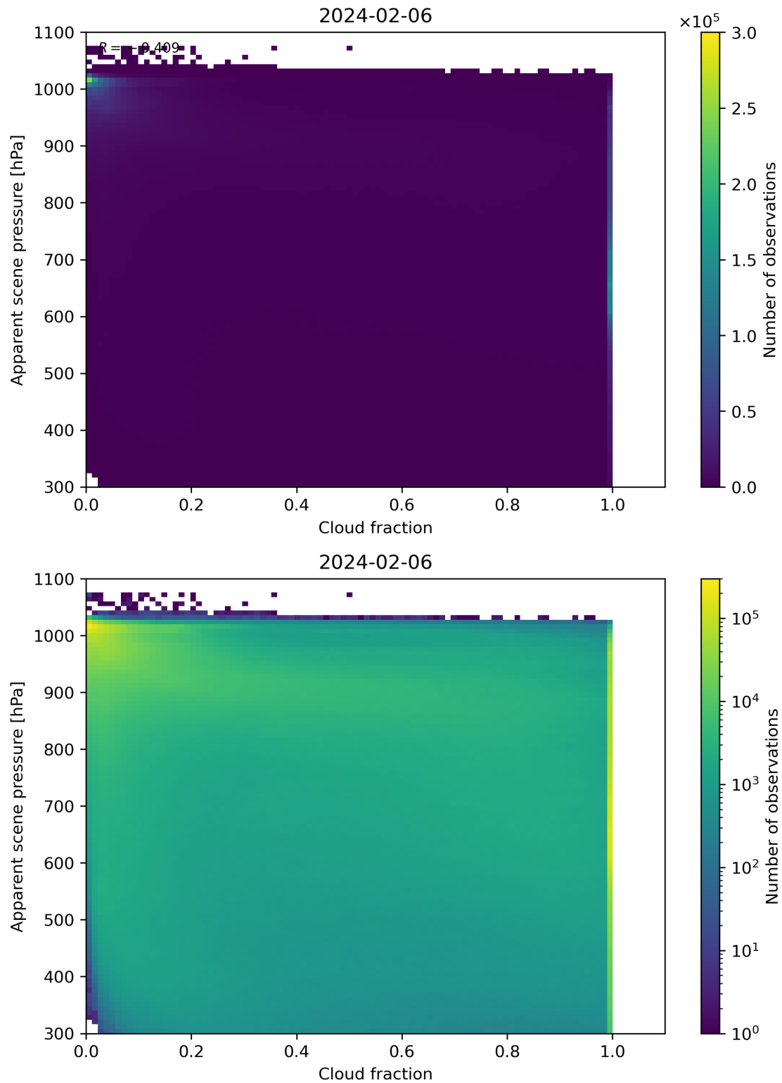
Figure 70: Scatter density plot of “Cloud fraction” against “Apparent scene pressure” for 2024-02-06 to 2024-02-07.
