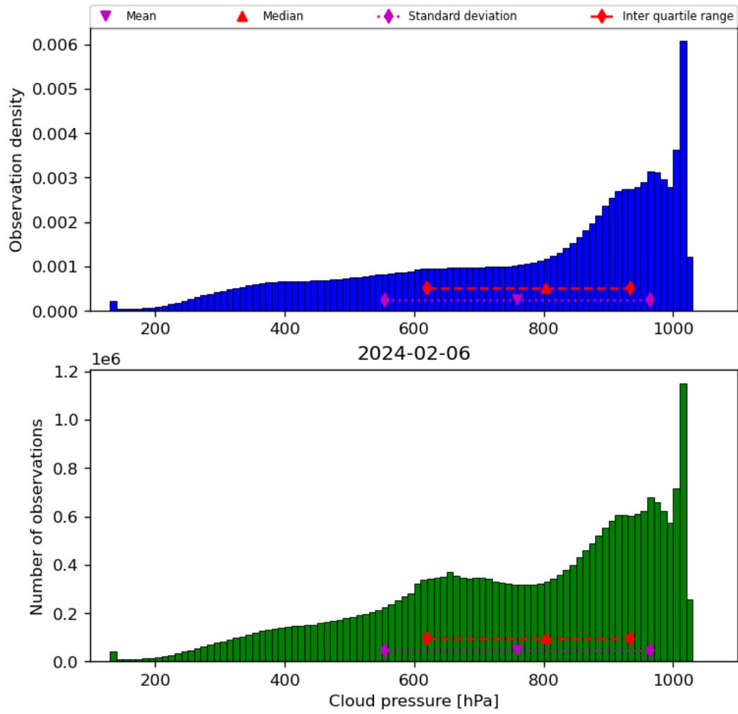
Figure 30: Histogram of “Cloud pressure” for 2024-02-06 to 2024-02-07
