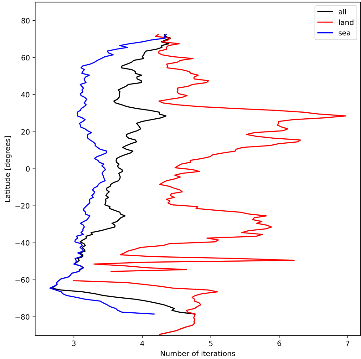
Figure 22: Zonal average of “Number of iterations” for 2024-02-06 to 2024-02-07.
