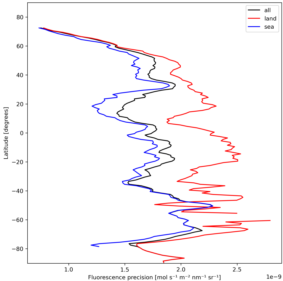
Figure 24: Zonal average of “Fluorescence precision” for 2024-02-06 to 2024-02-07.
