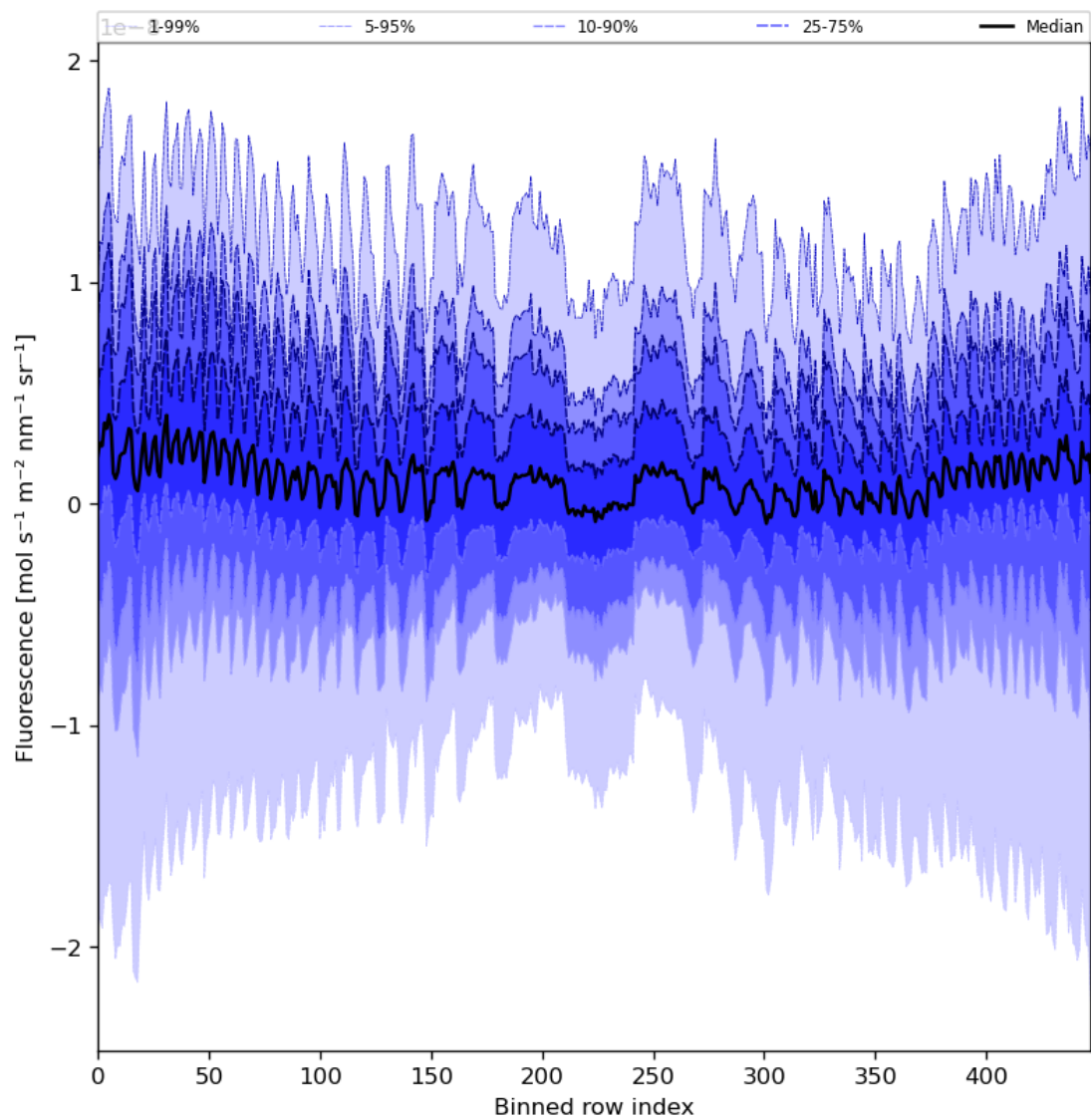
Figure 57: Along track statistics of “Fluorescence” for 2024-02-06 to 2024-02-07
