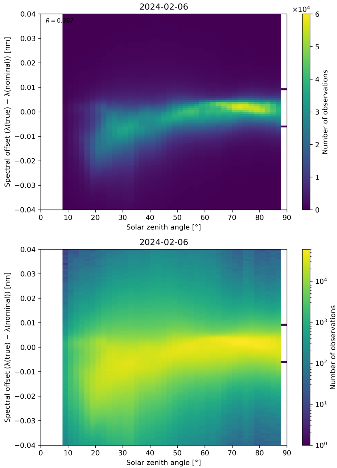
Figure 117: Scatter density plot of “Solar zenith angle” against “Spectral offset ( \lambda(\text{true}) - \lambda(\text{nominal}) )” for 2024-02-06 to 2024-02-07.
