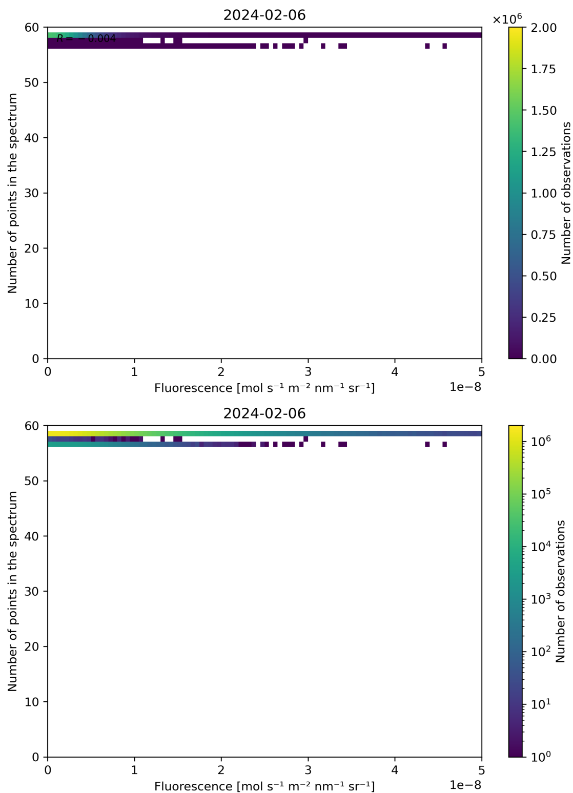
Figure 86: Scatter density plot of “Fluorescence” against “Number of points in the spectrum” for 2024-02-06 to 2024-02-07.
