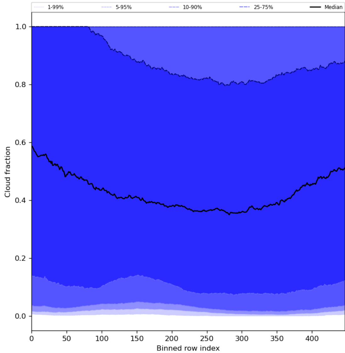
Figure 49: Along track statistics of “Cloud fraction” for 2024-02-06 to 2024-02-07
