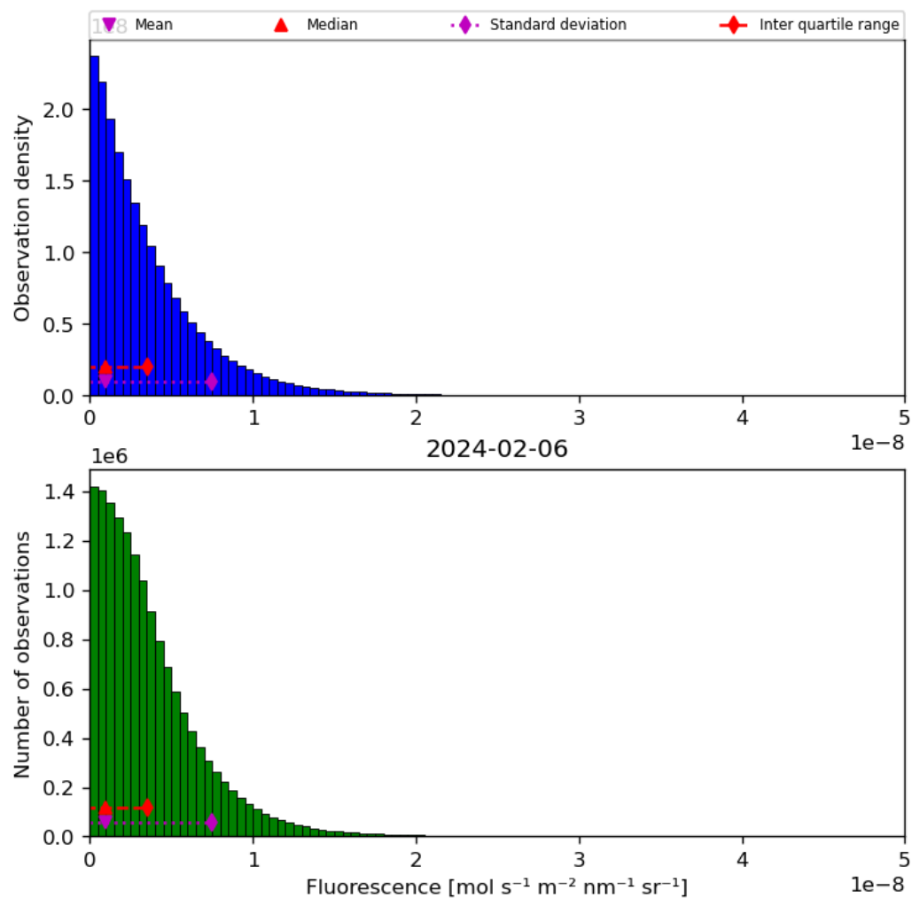
Figure 40: Histogram of “Fluorescence” for 2024-02-06 to 2024-02-07
