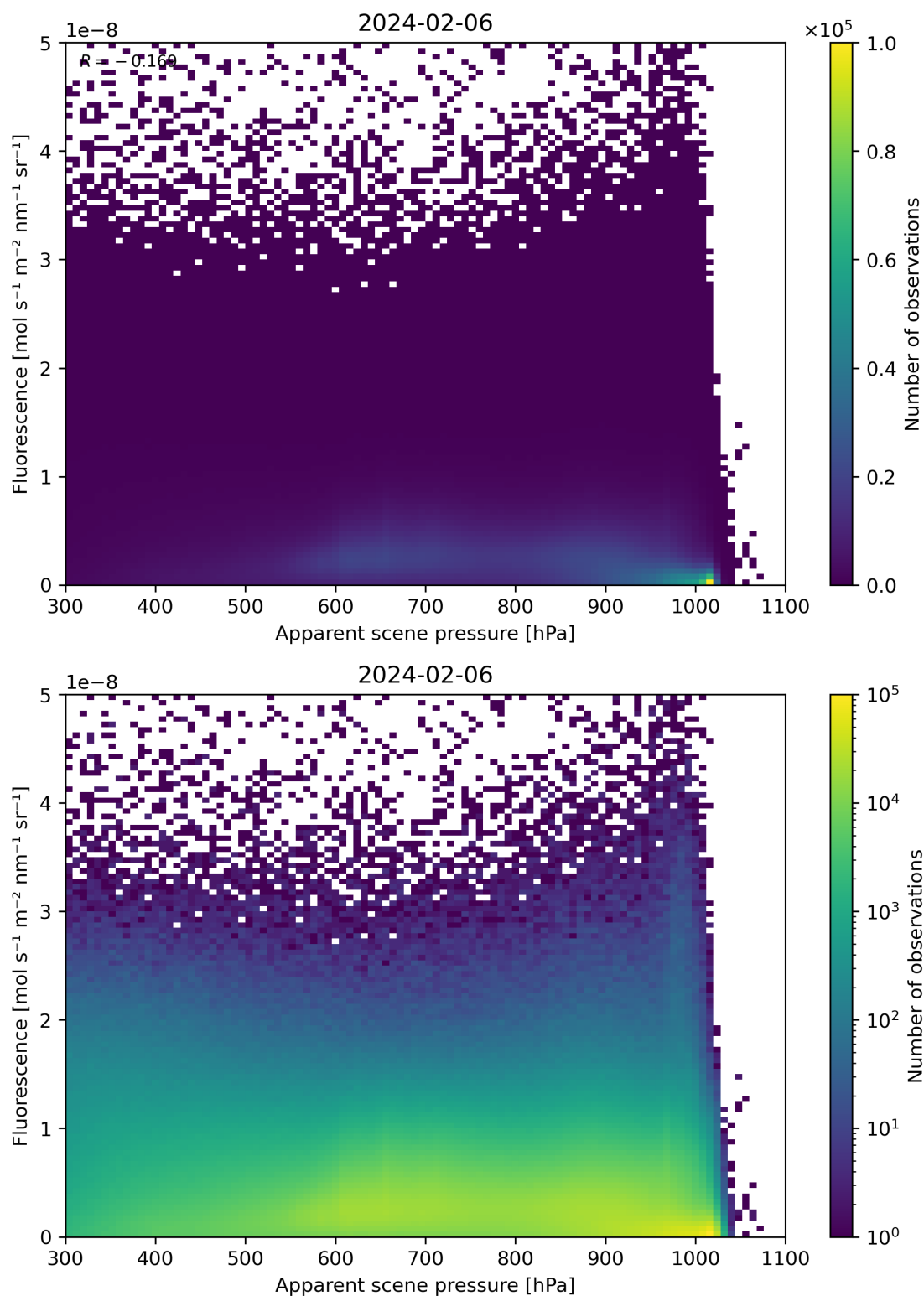
Figure 64: Scatter density plot of “Apparent scene pressure” against “Fluorescence” for 2024-02-06 to 2024-02-07.
