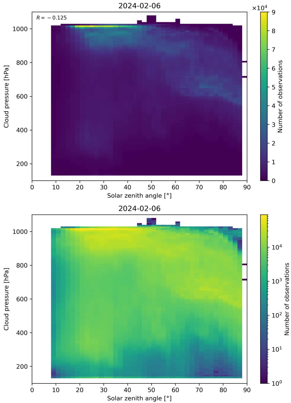
Figure 111: Scatter density plot of “Solar zenith angle” against “Cloud pressure” for 2024-02-06 to 2024-02-07.
