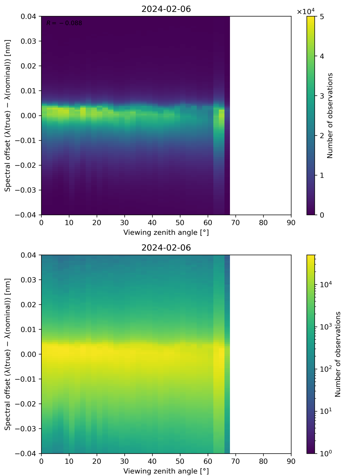
Figure 128: Scatter density plot of “Viewing zenith angle” against “Spectral offset ( \lambda(\text{true}) - \lambda(\text{nominal}) )” for 2024-02-06 to 2024-02-07.
