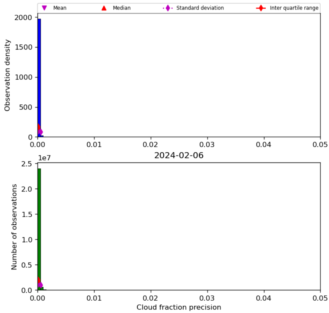
Figure 33: Histogram of “Cloud fraction precision” for 2024-02-06 to 2024-02-07
