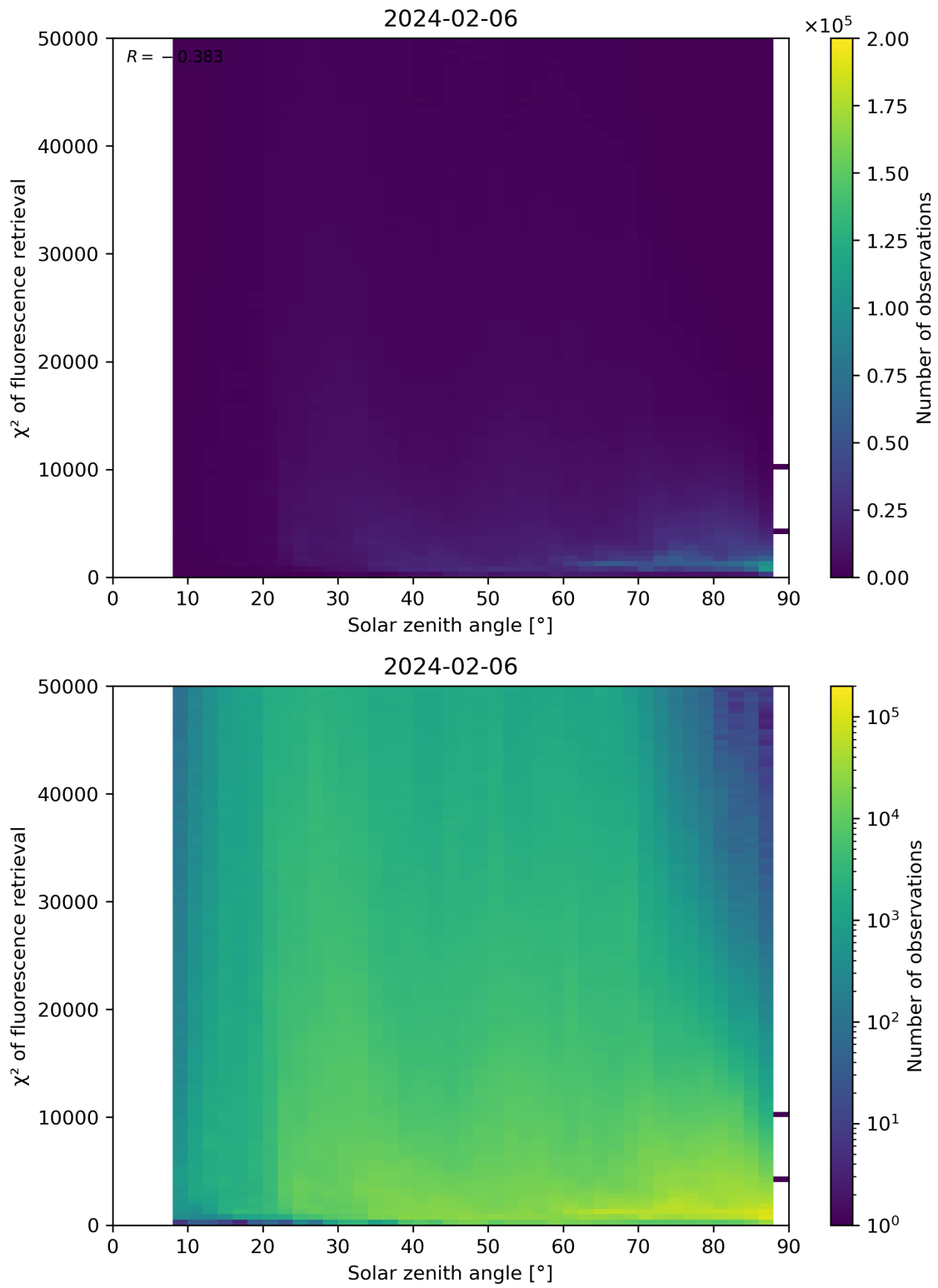
Figure 109: Scatter density plot of “Solar zenith angle” against “ \chi^2 of fluorescence retrieval” for 2024-02-06 to 2024-02-07.
