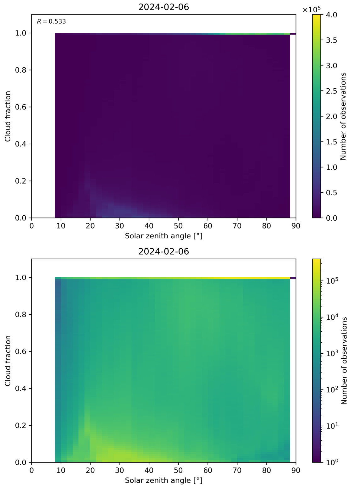
Figure 110: Scatter density plot of “Solar zenith angle” against “Cloud fraction” for 2024-02-06 to 2024-02-07.
