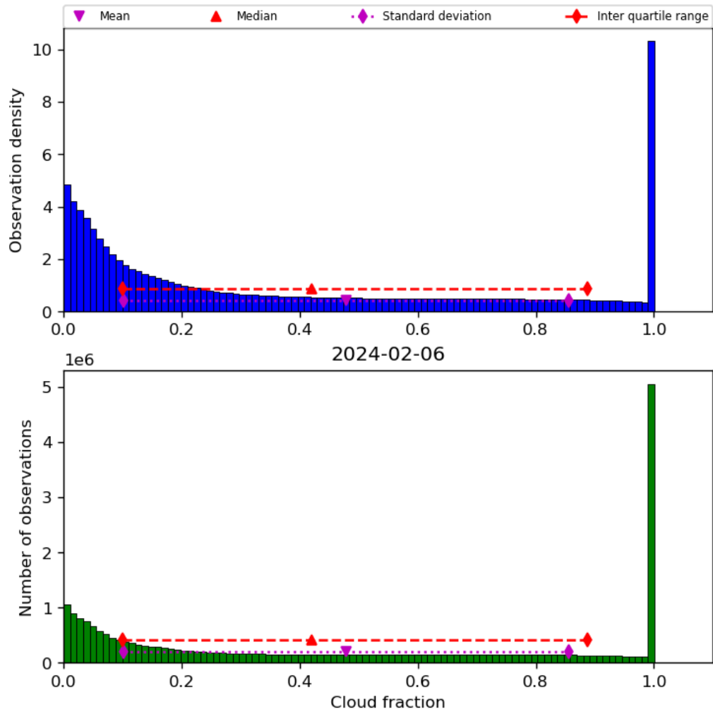
Figure 32: Histogram of “Cloud fraction” for 2024-02-06 to 2024-02-07
