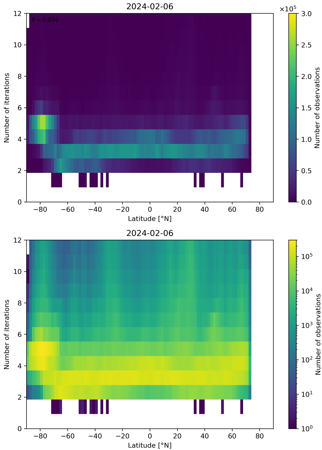
Figure 93: Scatter density plot of “Latitude” against “Number of iterations” for 2024-02-06 to 2024-02-07.
