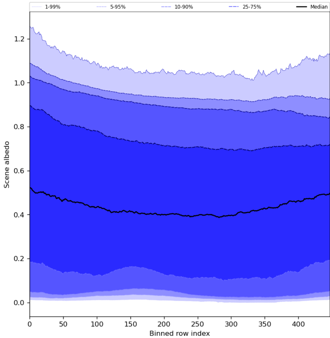
Figure 51: Along track statistics of “Scene albedo” for 2024-02-06 to 2024-02-07
