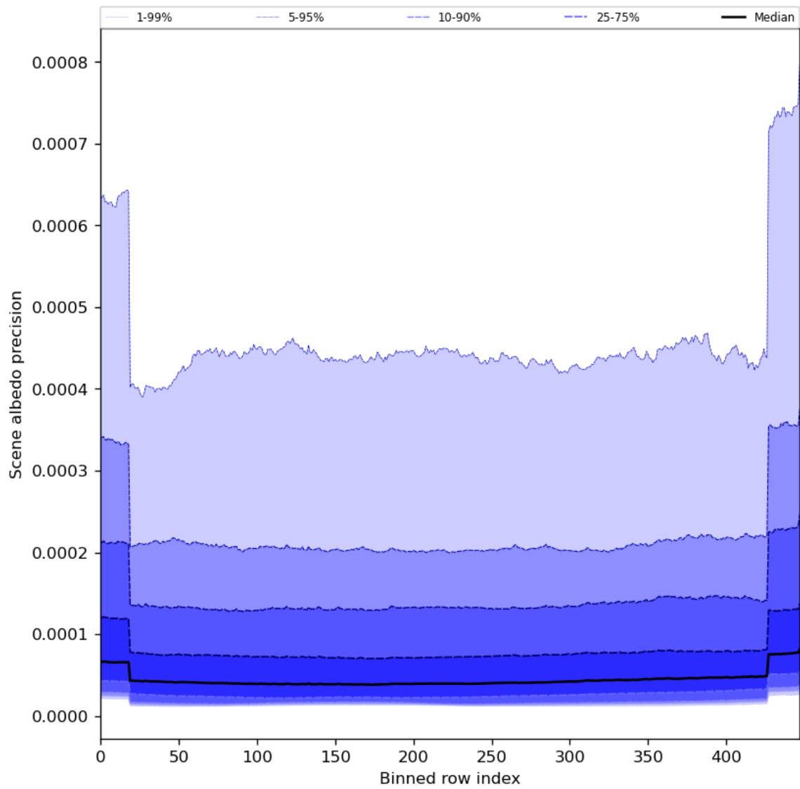
Figure 52: Along track statistics of “Scene albedo precision” for 2024-02-06 to 2024-02-07
