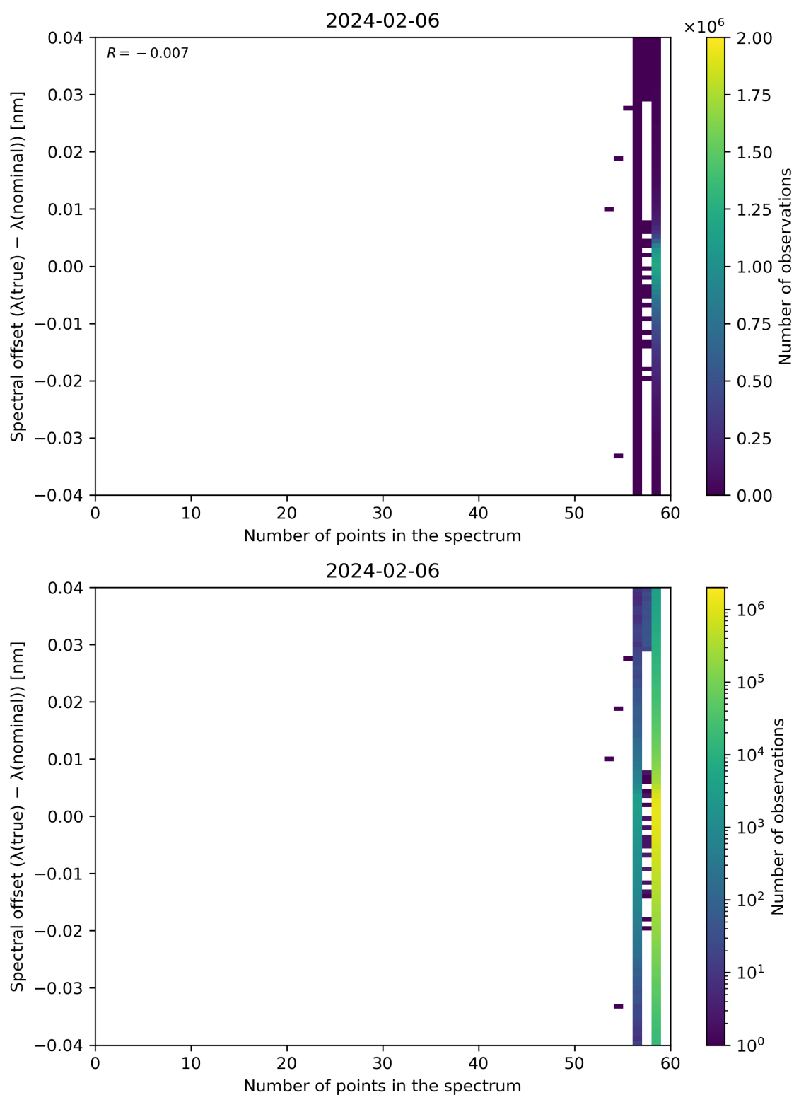
Figure 101: Scatter density plot of “Number of points in the spectrum” against “Spectral offset ( \lambda(\text{true}) - \lambda(\text{nominal}) )” for 2024-02-06 to 2024-02-07.
