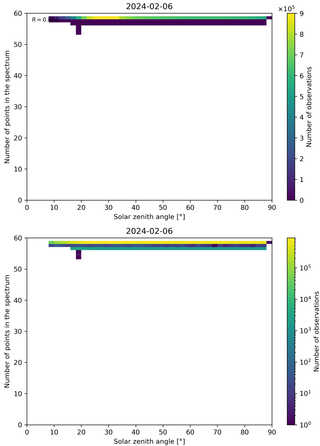
Figure 115: Scatter density plot of “Solar zenith angle” against “Number of points in the spectrum” for 2024-02-06 to 2024-02-07.
