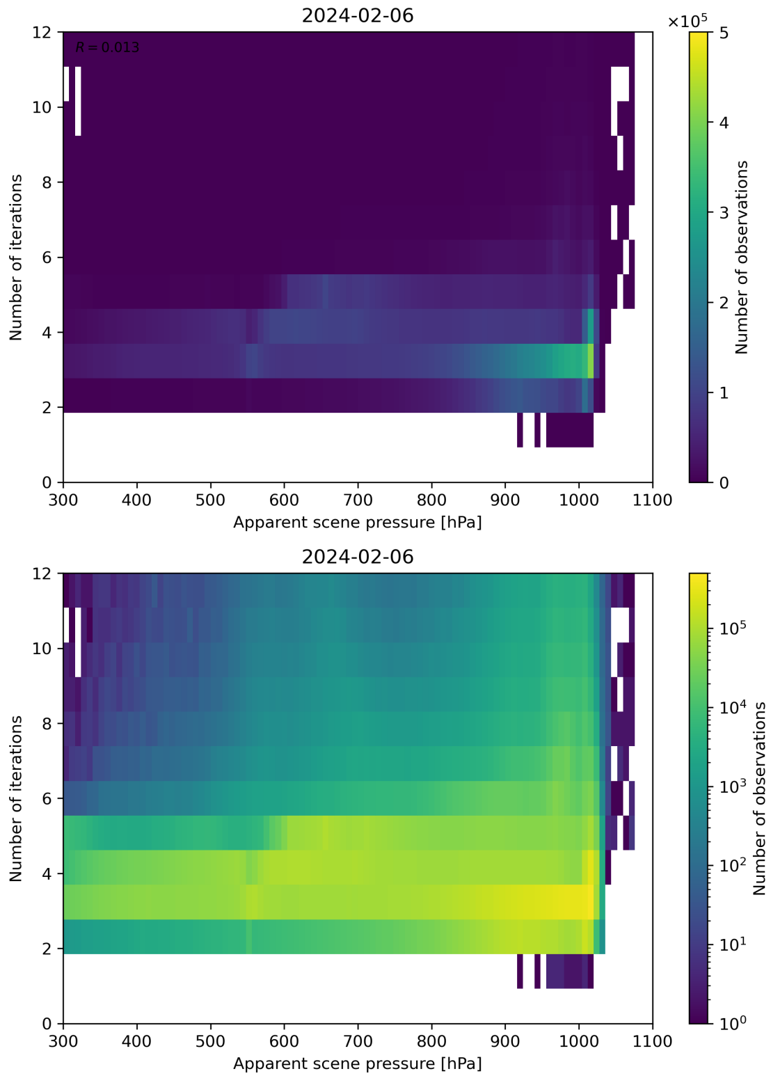
Figure 65: Scatter density plot of “Apparent scene pressure” against “Number of iterations” for 2024-02-06 to 2024-02-07.
