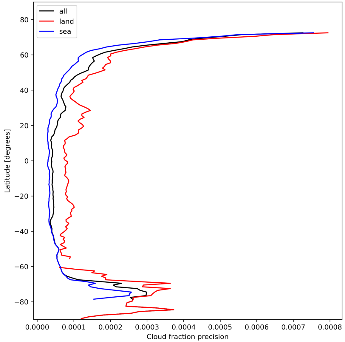
Figure 16: Zonal average of “Cloud fraction precision” for 2024-02-06 to 2024-02-07.
