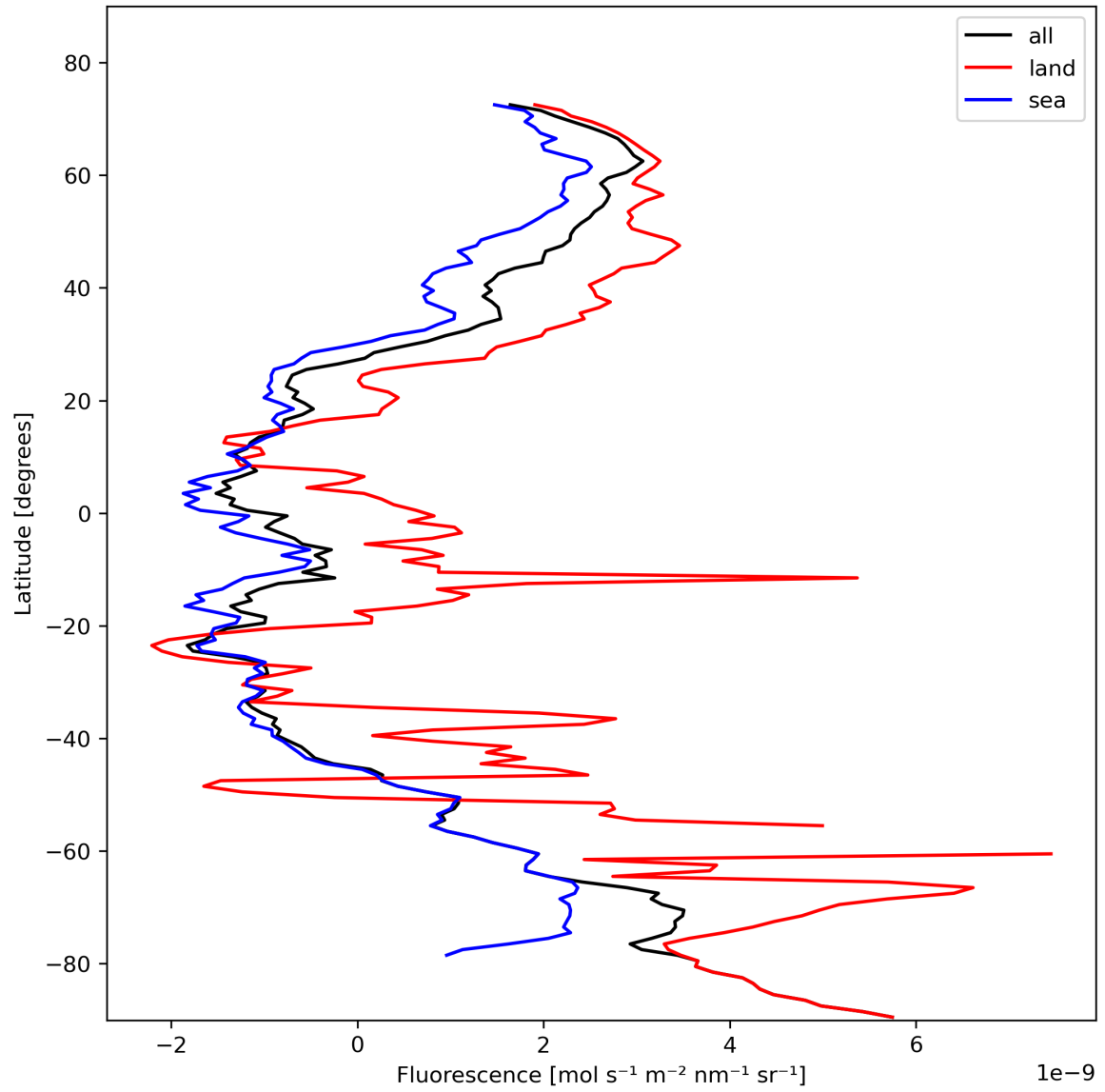
Figure 23: Zonal average of “Fluorescence” for 2024-02-06 to 2024-02-07.
