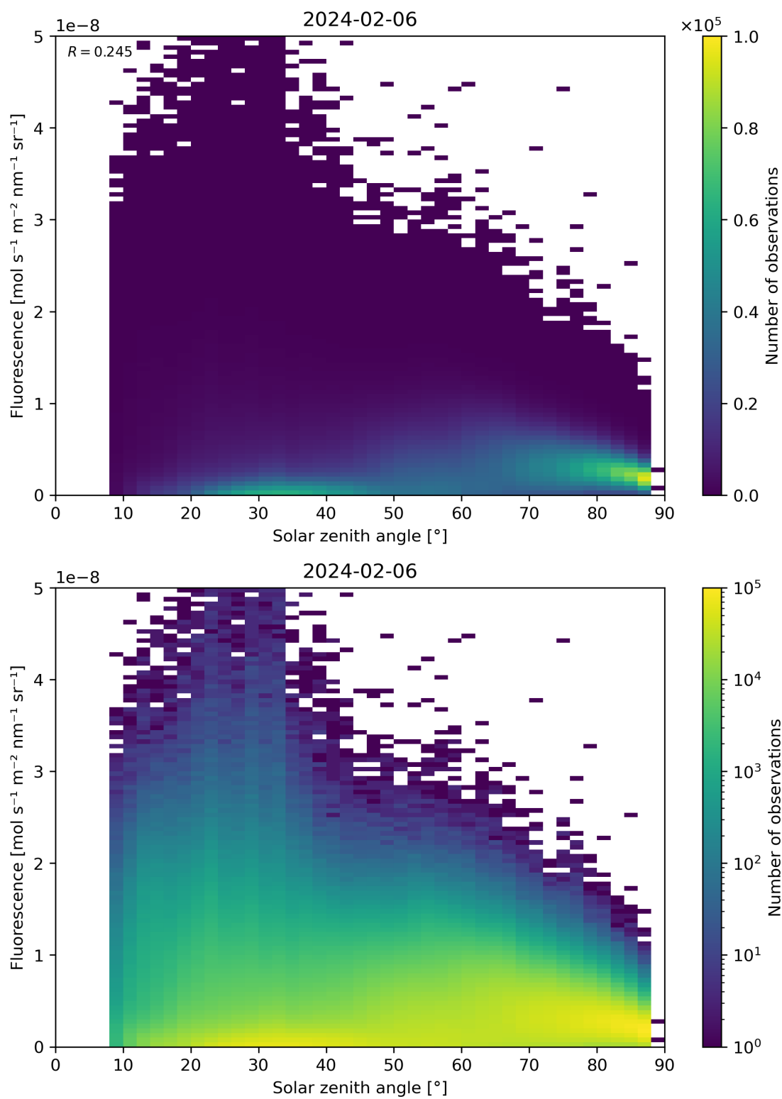
Figure 112: Scatter density plot of “Solar zenith angle” against “Fluorescence” for 2024-02-06 to 2024-02-07.
