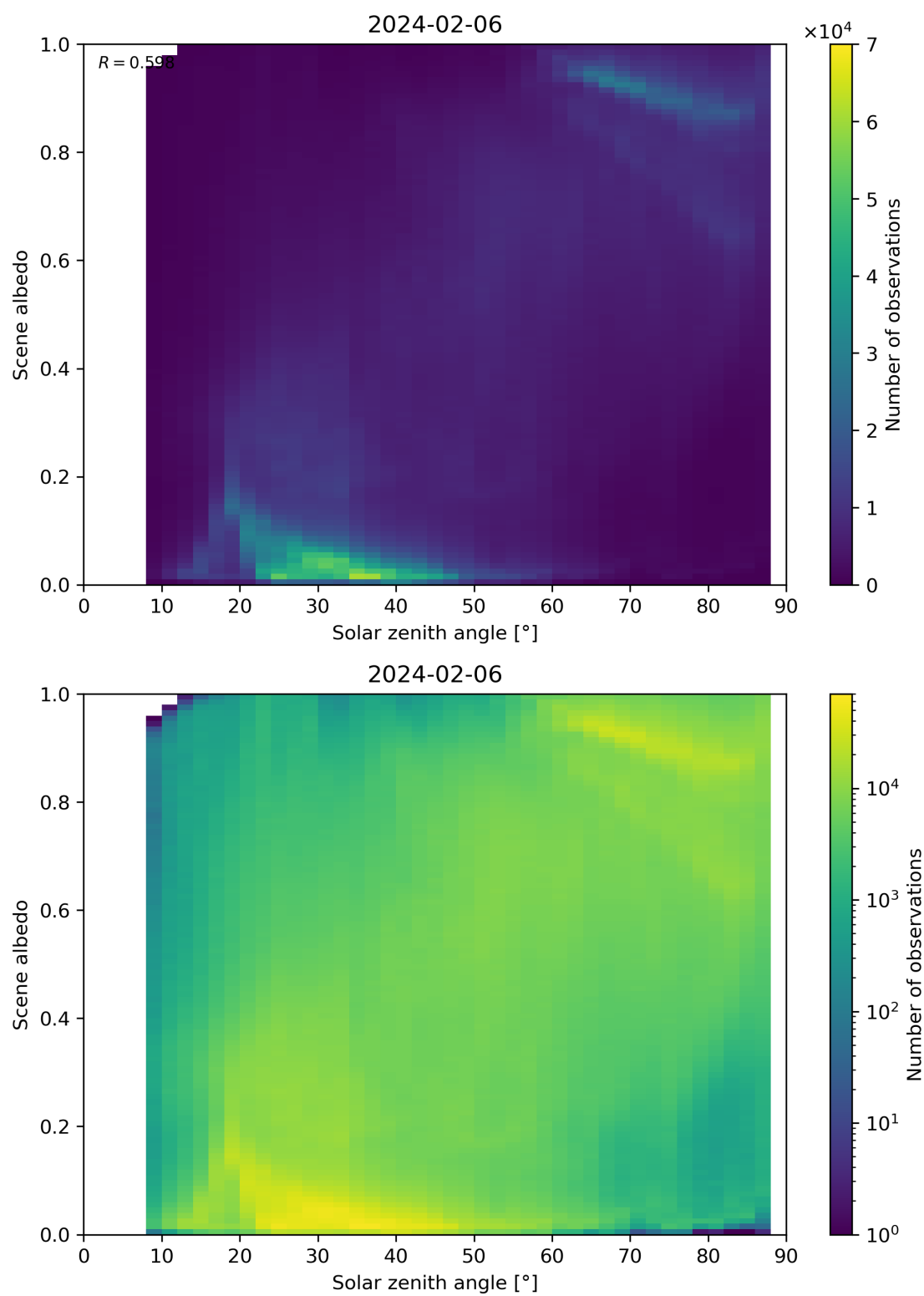
Figure 116: Scatter density plot of “Solar zenith angle” against “Scene albedo” for 2024-02-06 to 2024-02-07.
