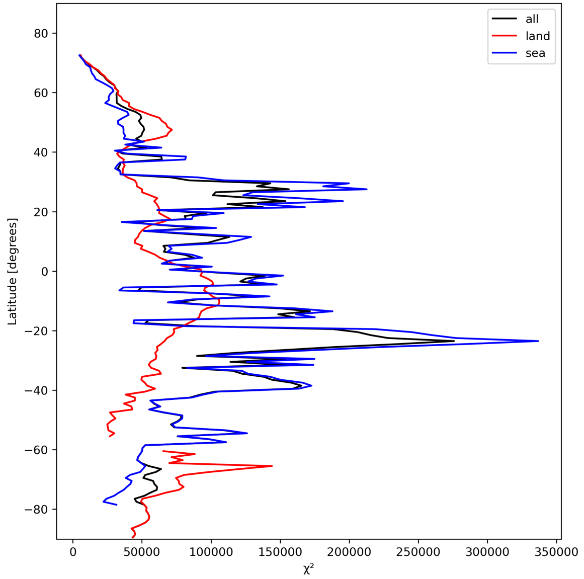
Figure 21: Zonal average of “ \chi^2 ” for 2024-02-06 to 2024-02-07.
