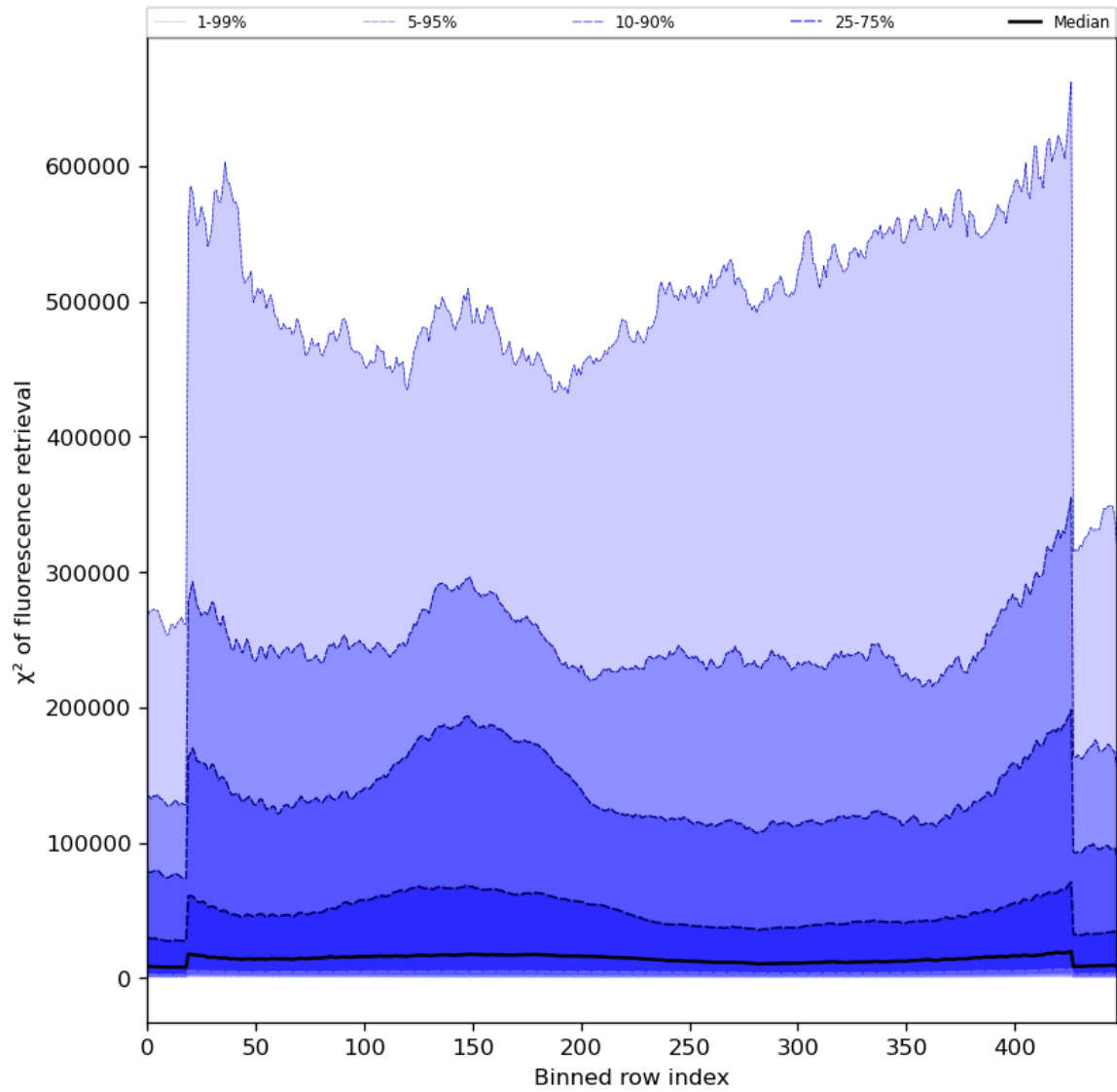
Figure 59: Along track statistics of “ \chi^2 of fluorescence retrieval” for 2024-02-06 to 2024-02-07
