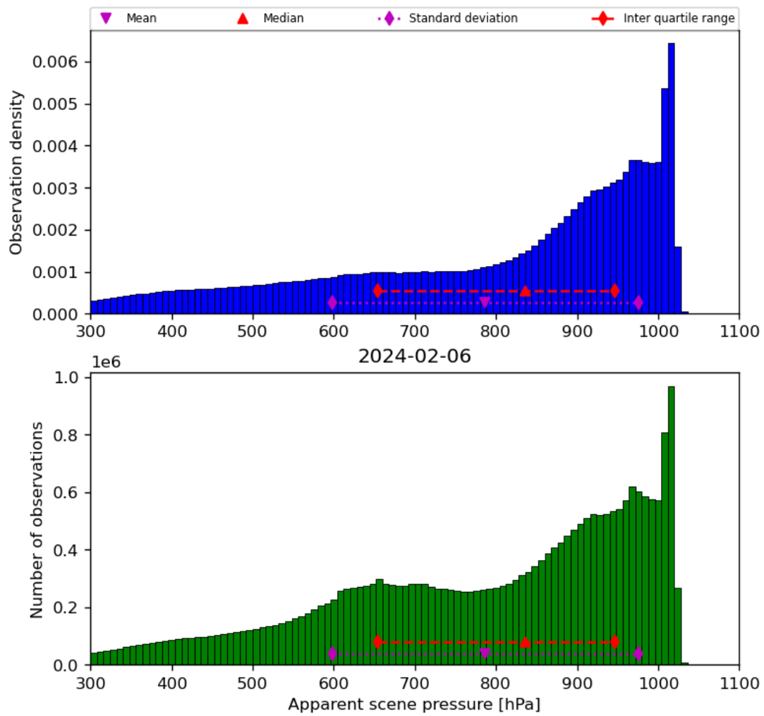
Figure 36: Histogram of “Apparent scene pressure” for 2024-02-06 to 2024-02-07
