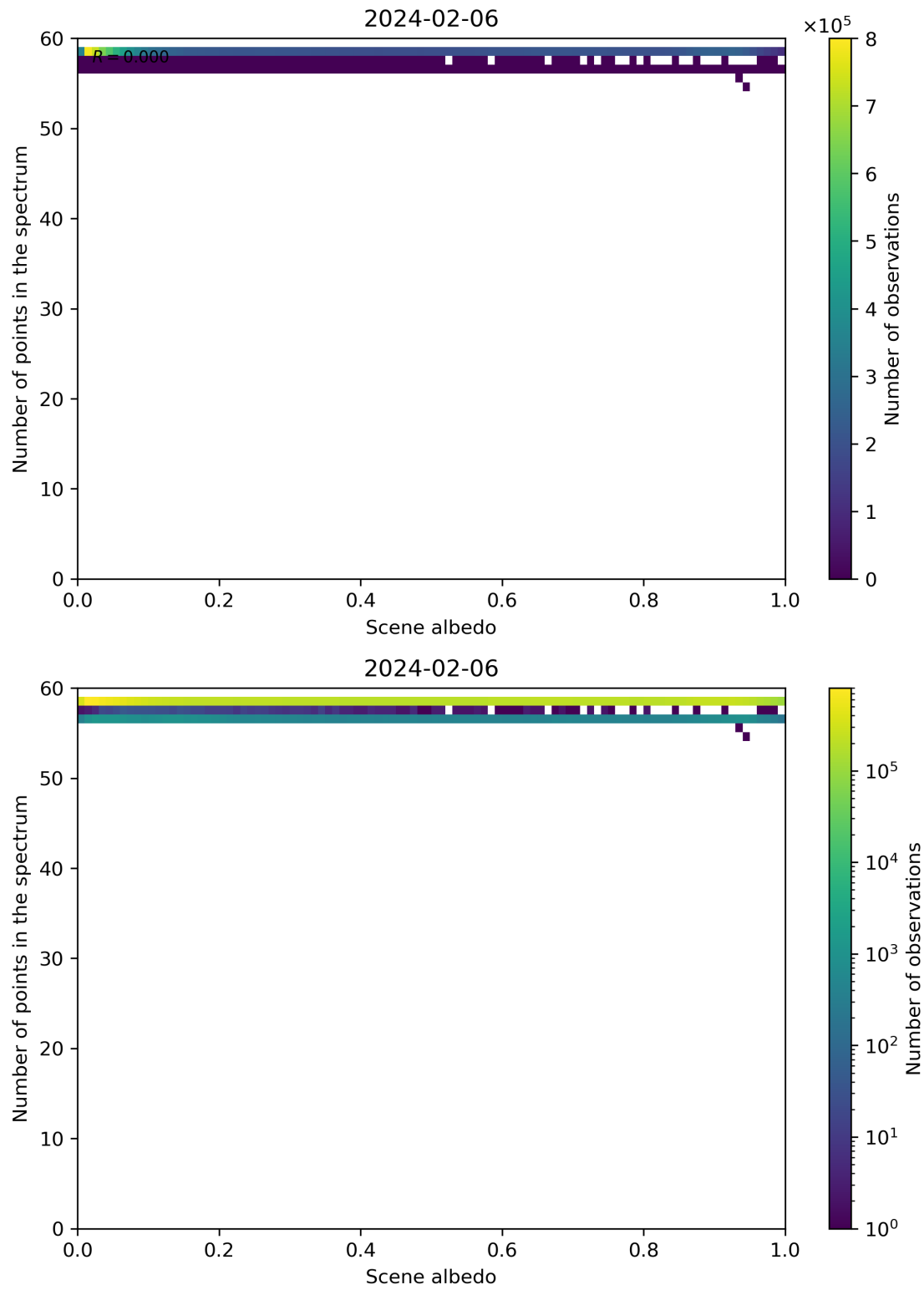
Figure 106: Scatter density plot of “Scene albedo” against “Number of points in the spectrum” for 2024-02-06 to 2024-02-07.
