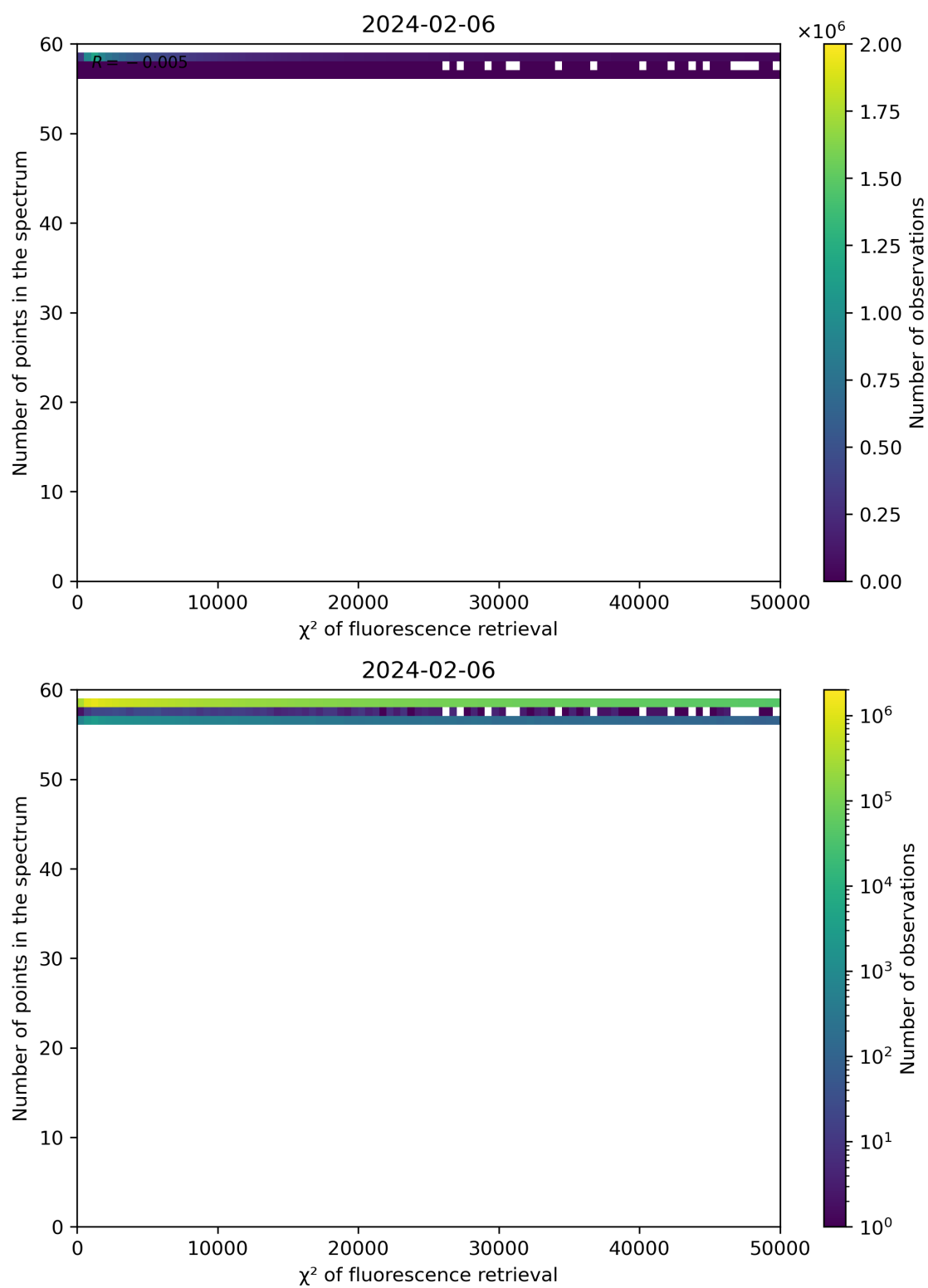
Figure 68: Scatter density plot of " \chi^2 of fluorescence retrieval" against "Number of points in the spectrum" for 2024-02-06 to 2024-02-07.
