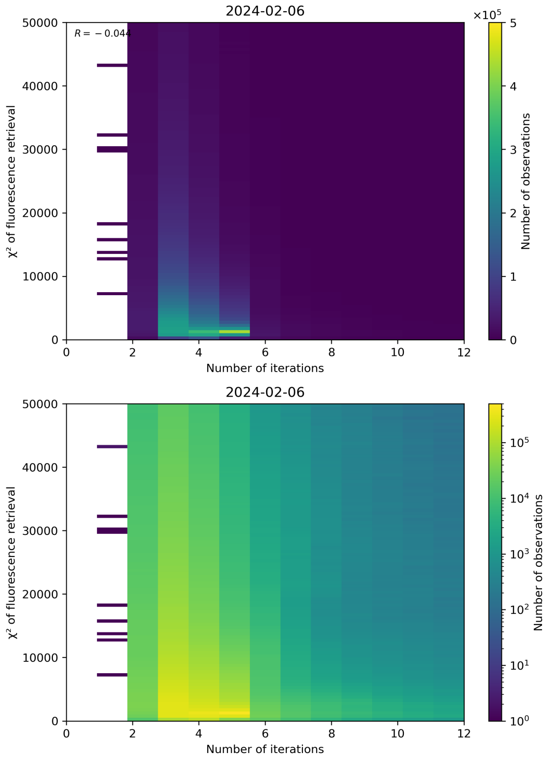
Figure 97: Scatter density plot of “Number of iterations” against “ \chi^2 of fluorescence retrieval” for 2024-02-06 to 2024-02-07.
