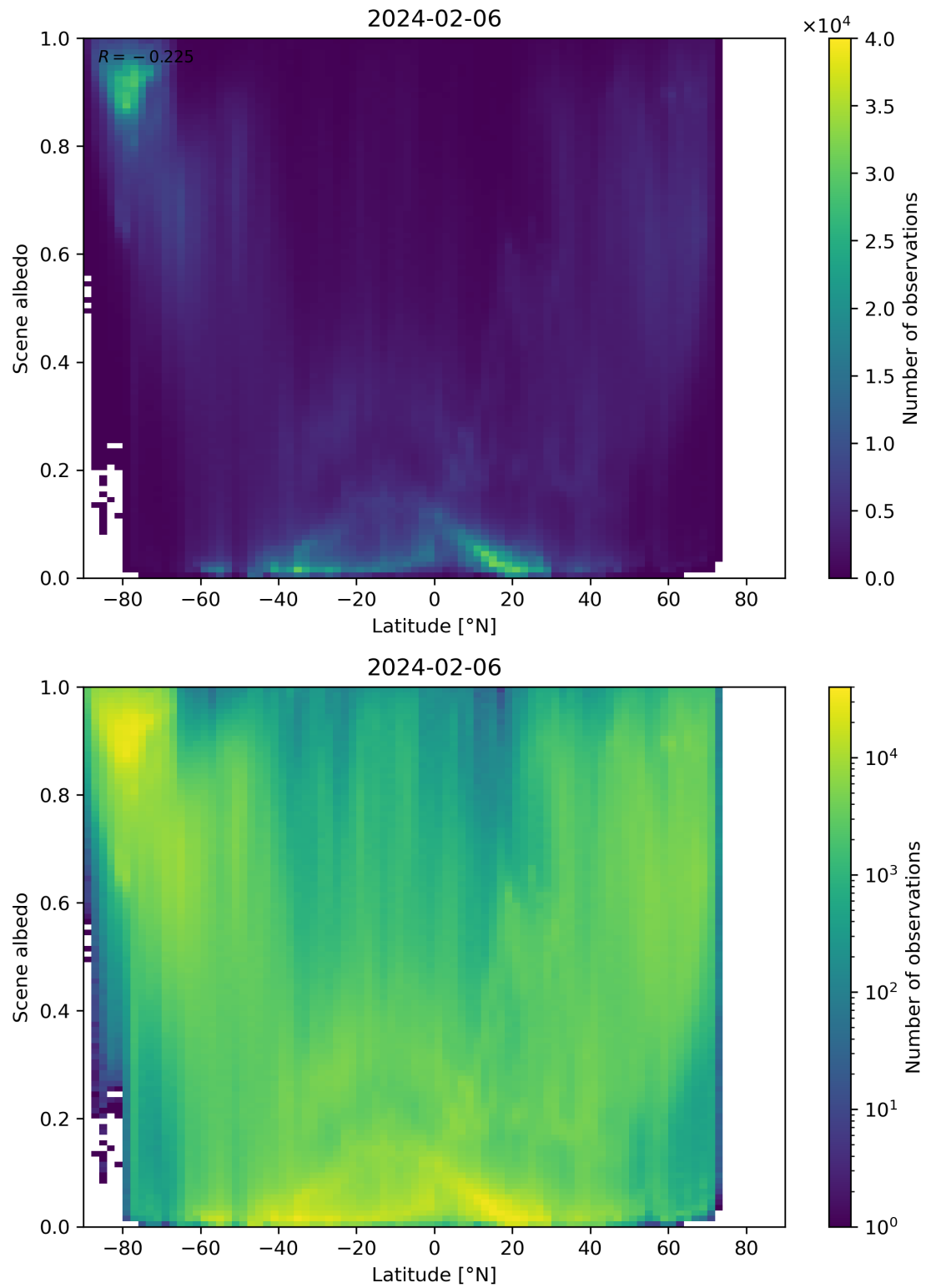
Figure 95: Scatter density plot of “Latitude” against “Scene albedo” for 2024-02-06 to 2024-02-07.
