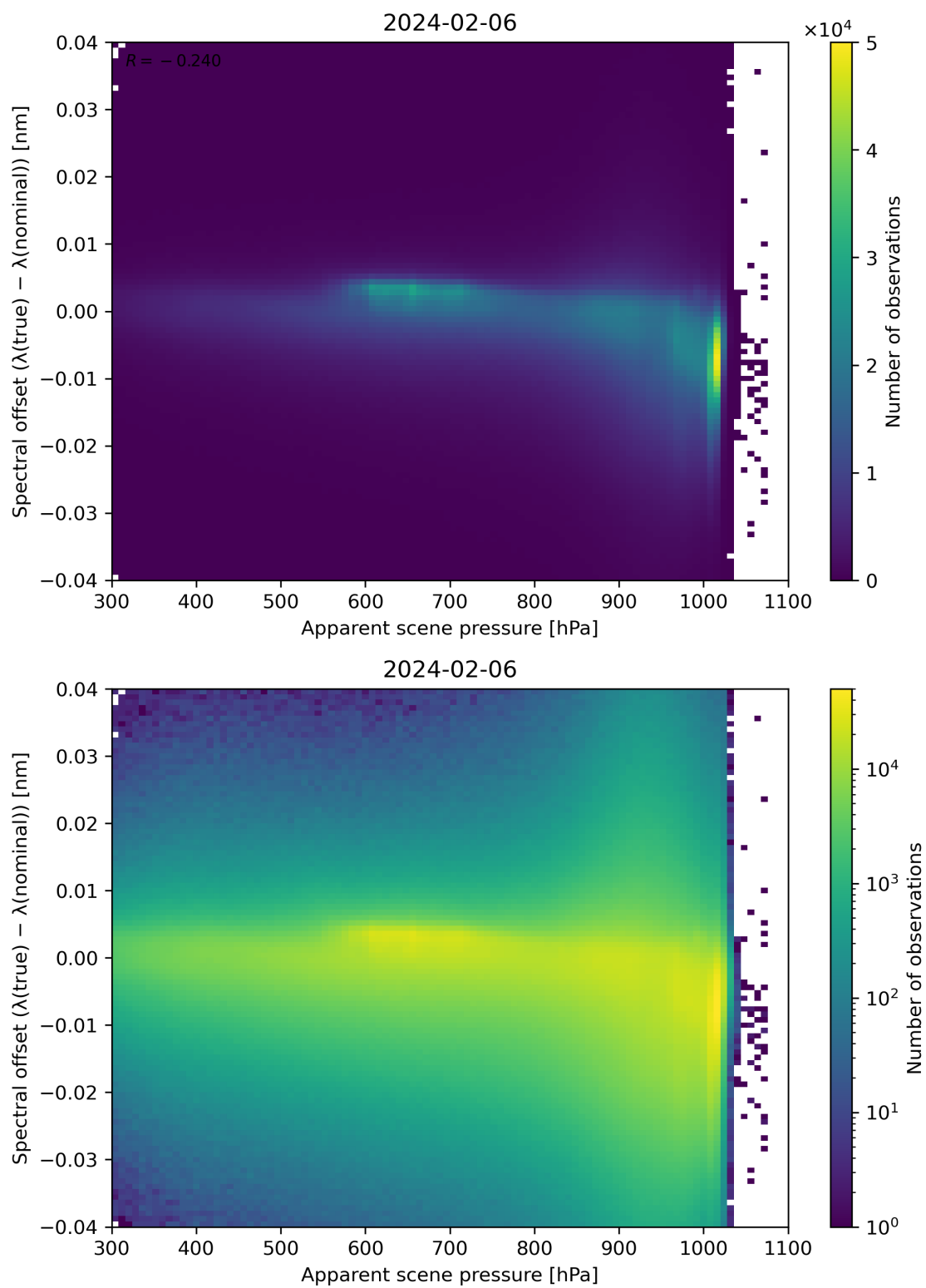
Figure 67: Scatter density plot of “Apparent scene pressure” against “Spectral offset ( \lambda(\text{true}) - \lambda(\text{nominal}) )” for 2024-02-06 to 2024-02-07.
