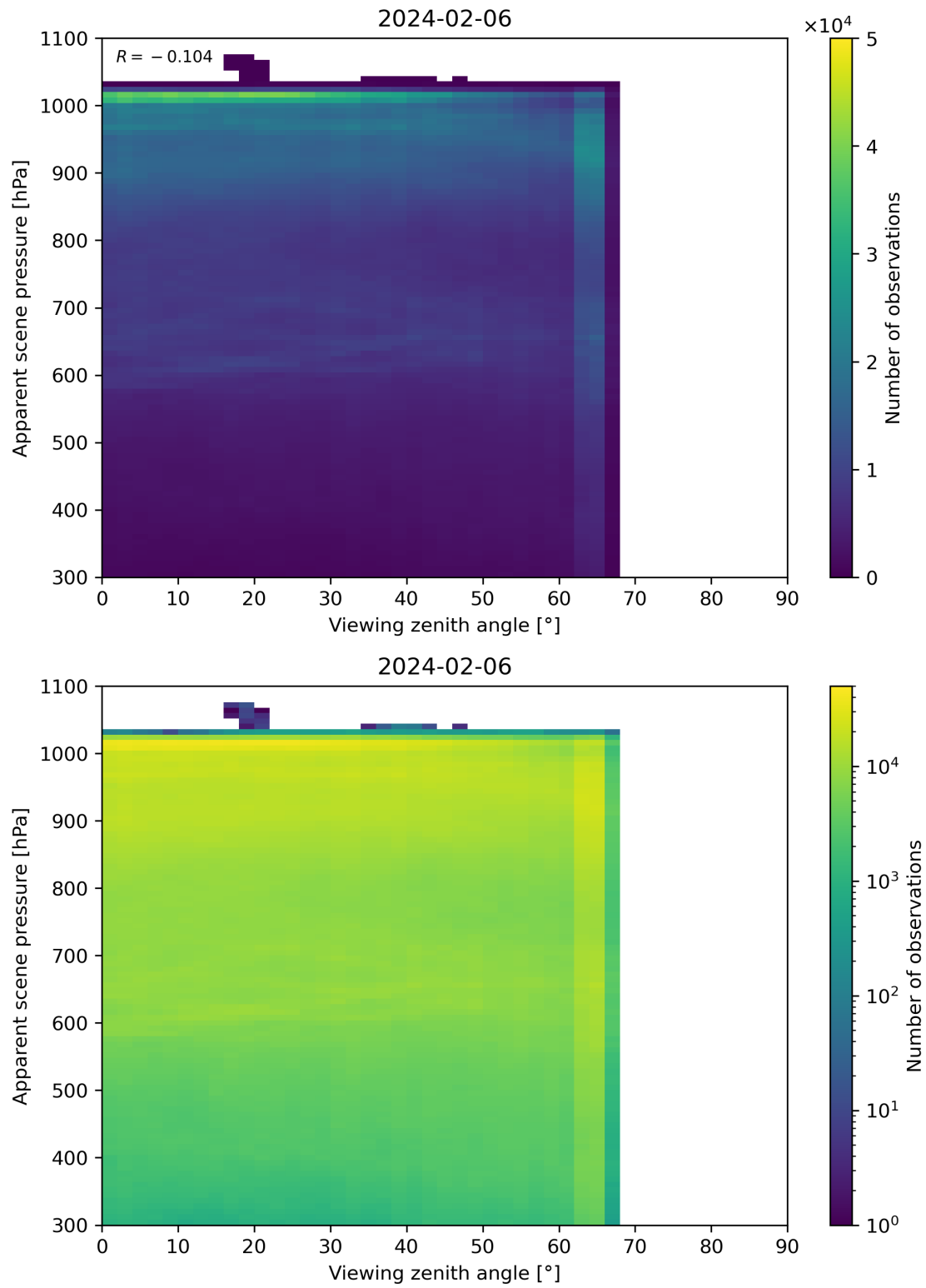
Figure 118: Scatter density plot of “Viewing zenith angle” against “Apparent scene pressure” for 2024-02-06 to 2024-02-07.
