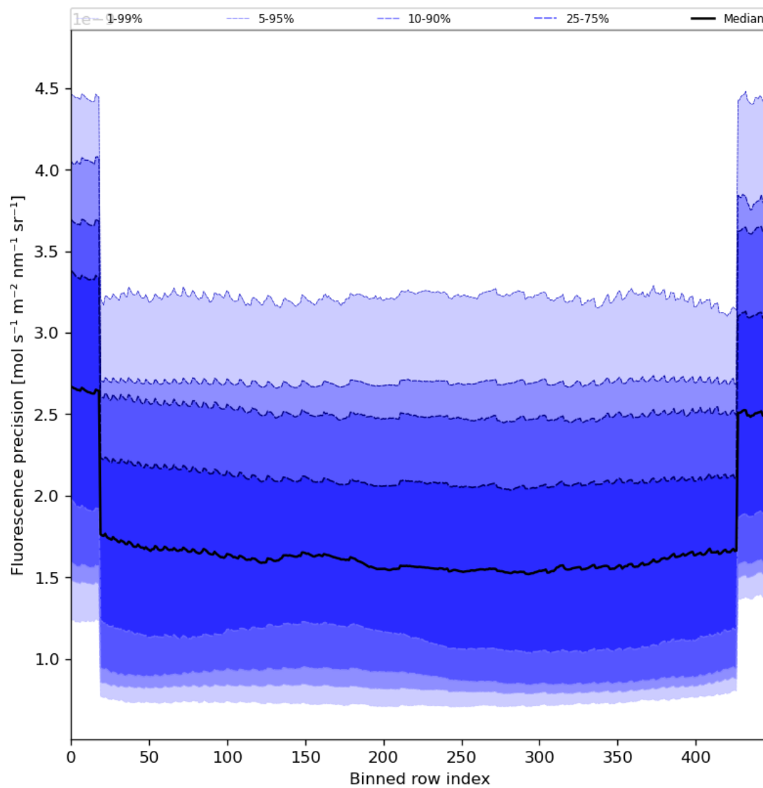
Figure 58: Along track statistics of “Fluorescence precision” for 2024-02-06 to 2024-02-07
