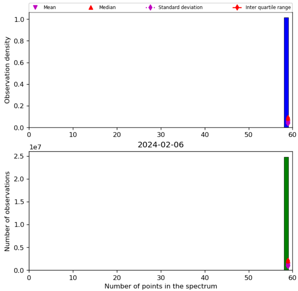
Figure 44: Histogram of “Number of points in the spectrum” for 2024-02-06 to 2024-02-07
