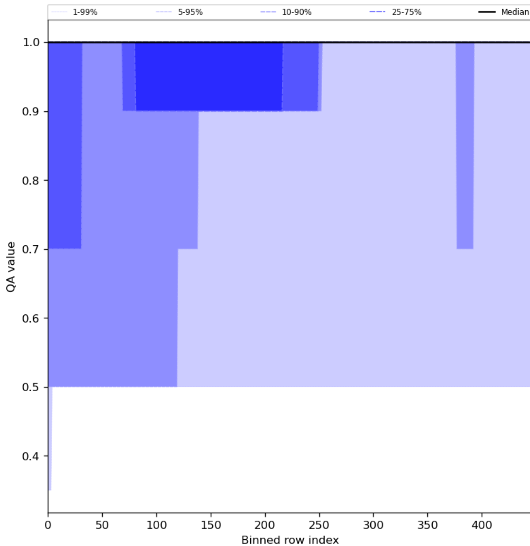
Figure 46: Along track statistics of “QA value” for 2024-02-06 to 2024-02-07
