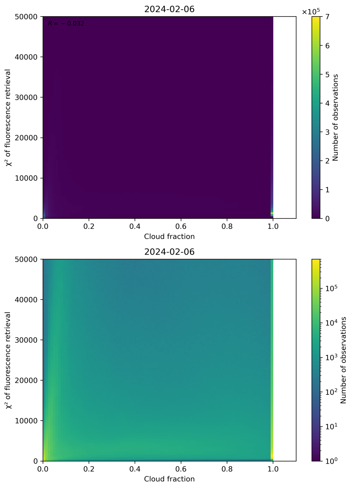
Figure 71: Scatter density plot of “Cloud fraction” against “ \chi^2 of fluorescence retrieval” for 2024-02-06 to 2024-02-07.
