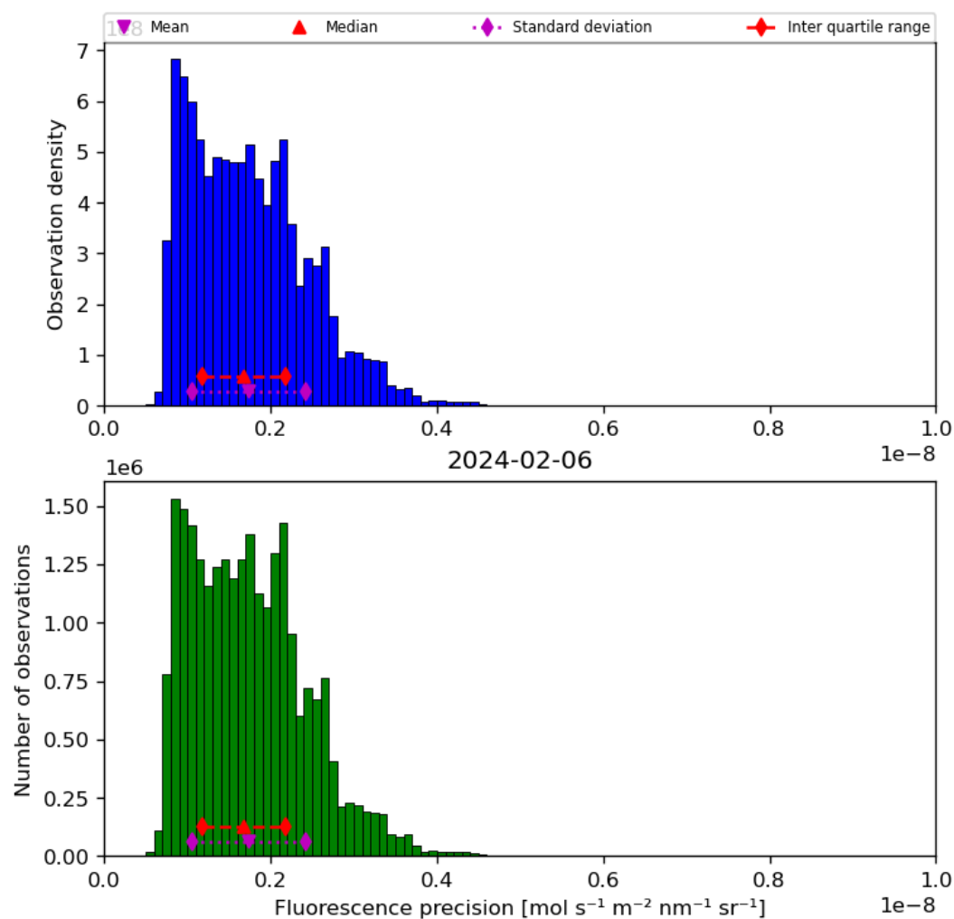
Figure 41: Histogram of “Fluorescence precision” for 2024-02-06 to 2024-02-07
