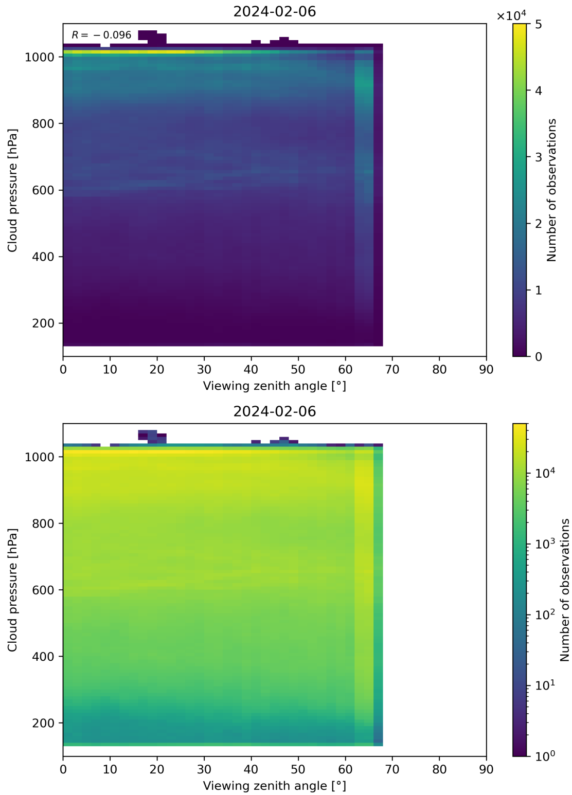
Figure 121: Scatter density plot of “Viewing zenith angle” against “Cloud pressure” for 2024-02-06 to 2024-02-07.
