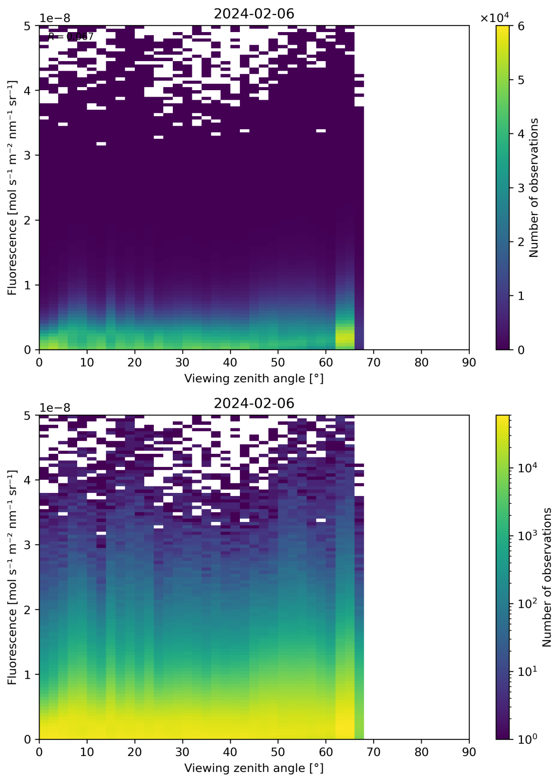
Figure 122: Scatter density plot of “Viewing zenith angle” against “Fluorescence” for 2024-02-06 to 2024-02-07.
