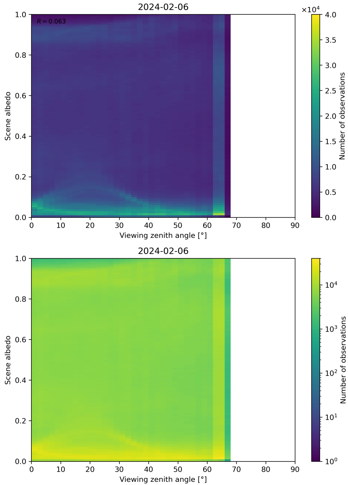
Figure 126: Scatter density plot of “Viewing zenith angle” against “Scene albedo” for 2024-02-06 to 2024-02-07.
