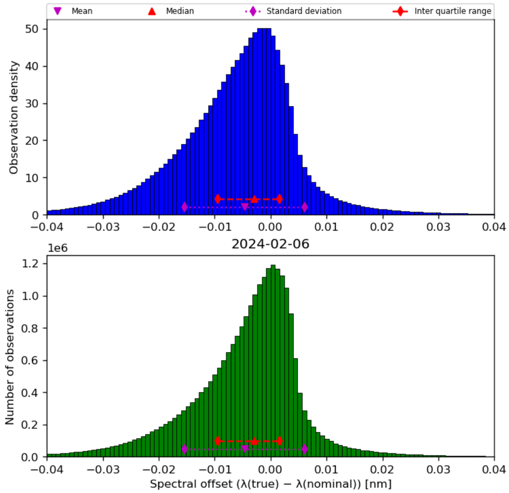
Figure 45: Histogram of “Spectral offset ( \lambda(\text{true}) - \lambda(\text{nominal}) )” for 2024-02-06 to 2024-02-07
