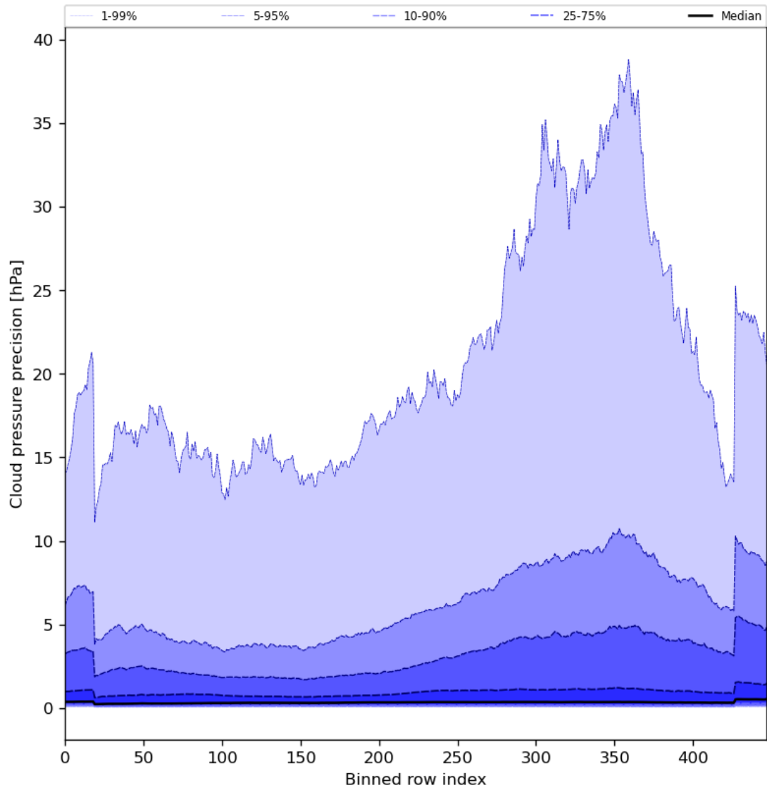
Figure 48: Along track statistics of “Cloud pressure precision” for 2024-02-06 to 2024-02-07
