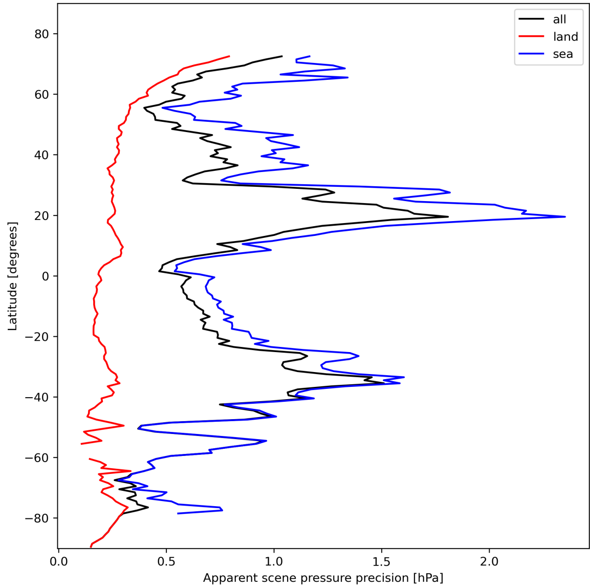
Figure 20: Zonal average of “Apparent scene pressure precision” for 2024-02-06 to 2024-02-07.
