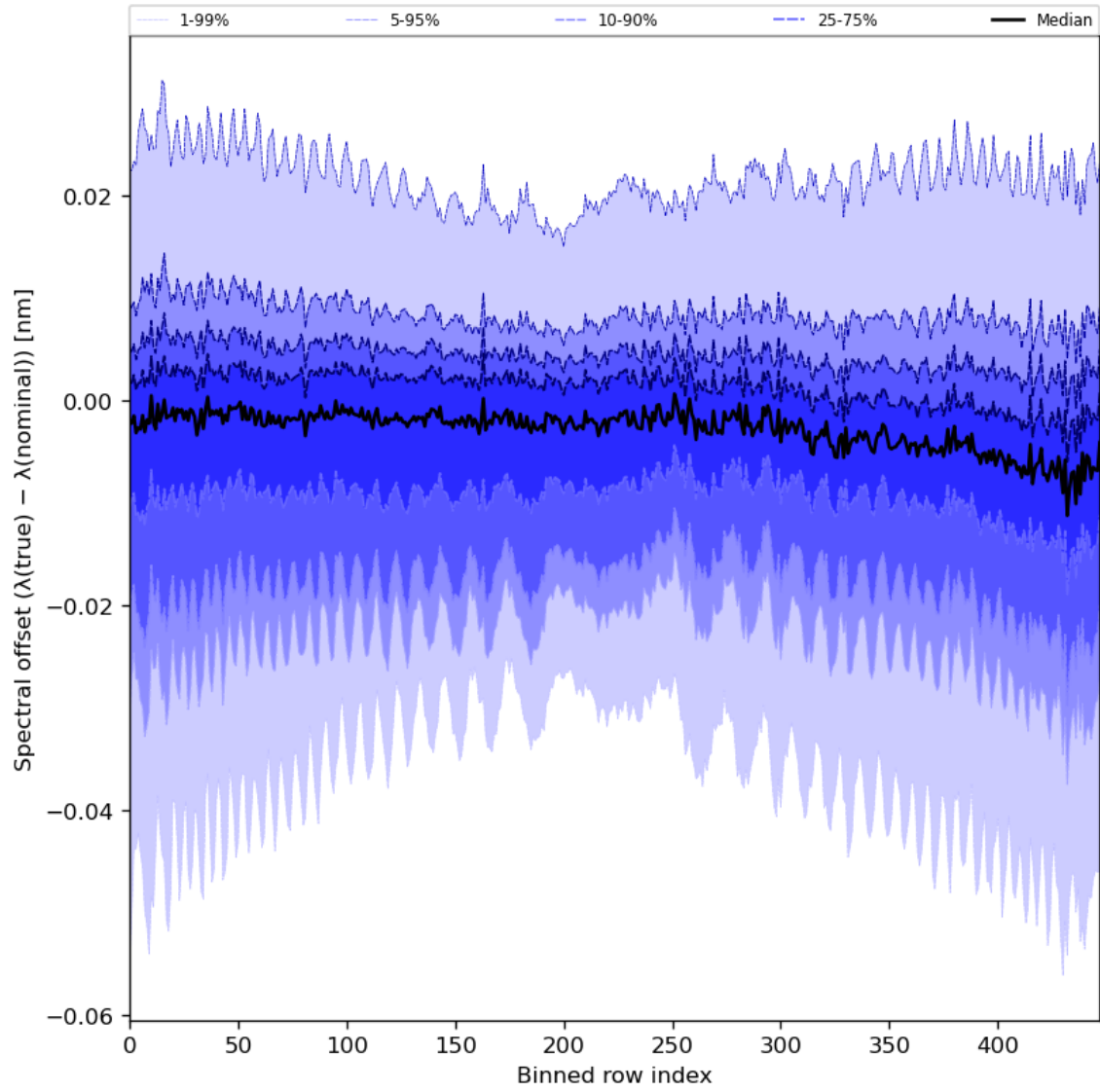
Figure 62: Along track statistics of “Spectral offset ( \lambda(\text{true}) - \lambda(\text{nominal}) )” for 2024-02-06 to 2024-02-07
