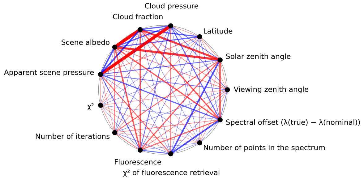
Figure 1: Map of correlation graph for 2024-02-06 to 2024-02-07.
