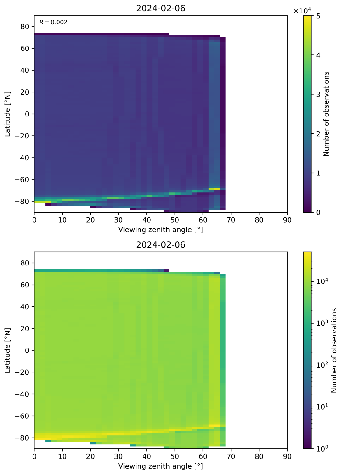
Figure 123: Scatter density plot of “Viewing zenith angle” against “Latitude” for 2024-02-06 to 2024-02-07.
