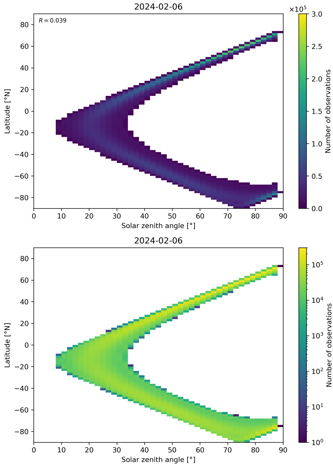
Figure 113: Scatter density plot of “Solar zenith angle” against “Latitude” for 2024-02-06 to 2024-02-07.
