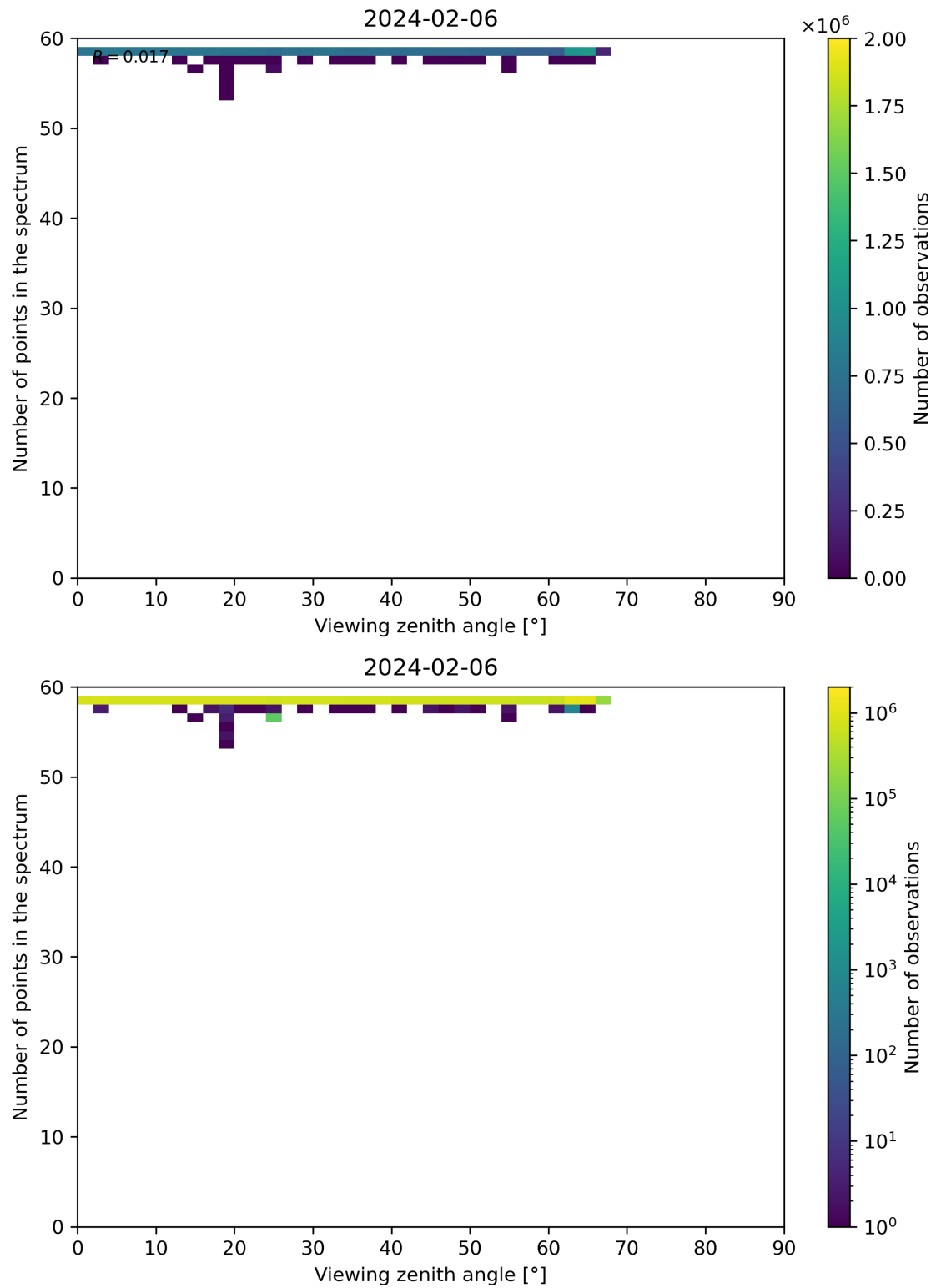
Figure 125: Scatter density plot of “Viewing zenith angle” against “Number of points in the spectrum” for 2024-02-06 to 2024-02-07.
