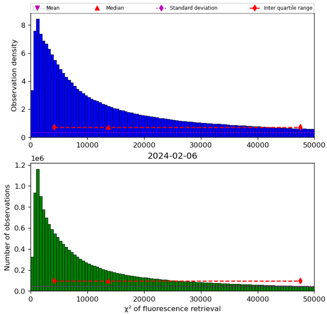
Figure 42: Histogram of “ \chi^2 of fluorescence retrieval” for 2024-02-06 to 2024-02-07
