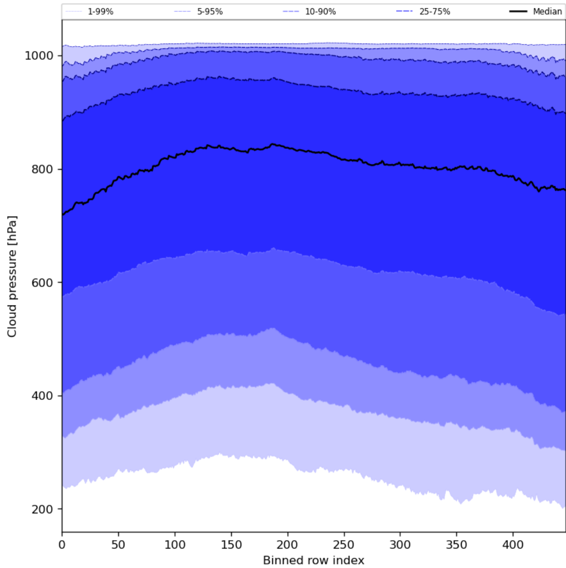
Figure 47: Along track statistics of “Cloud pressure” for 2024-02-06 to 2024-02-07
