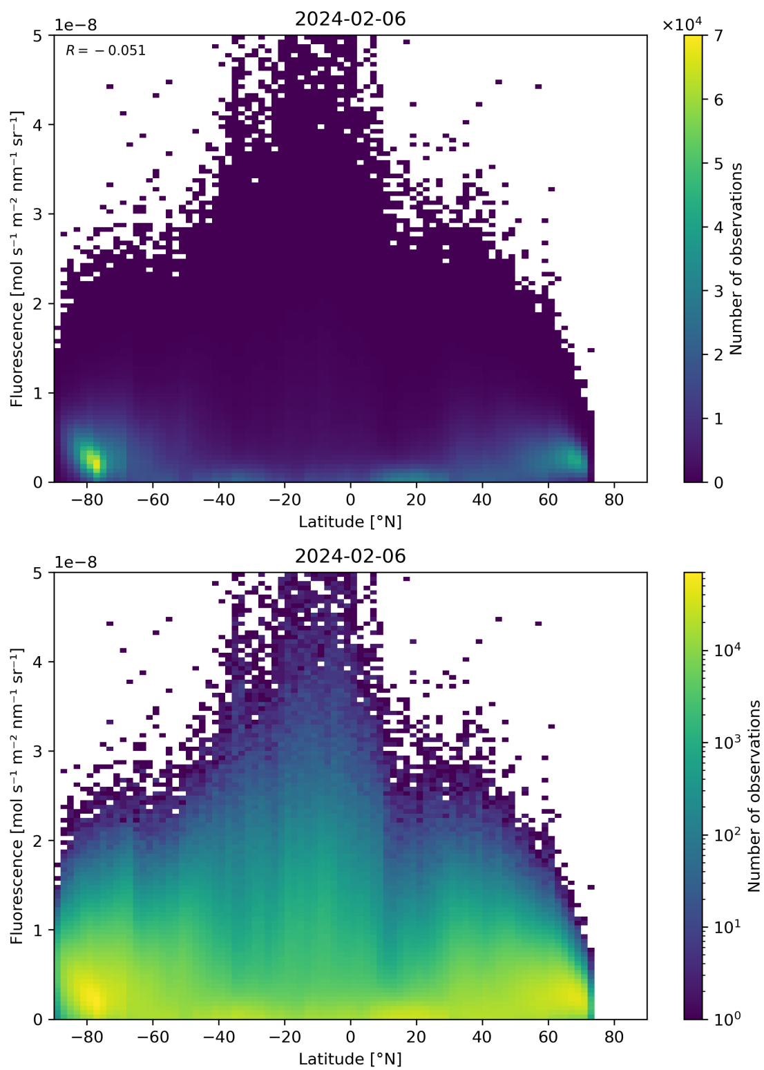
Figure 92: Scatter density plot of “Latitude” against “Fluorescence” for 2024-02-06 to 2024-02-07.
