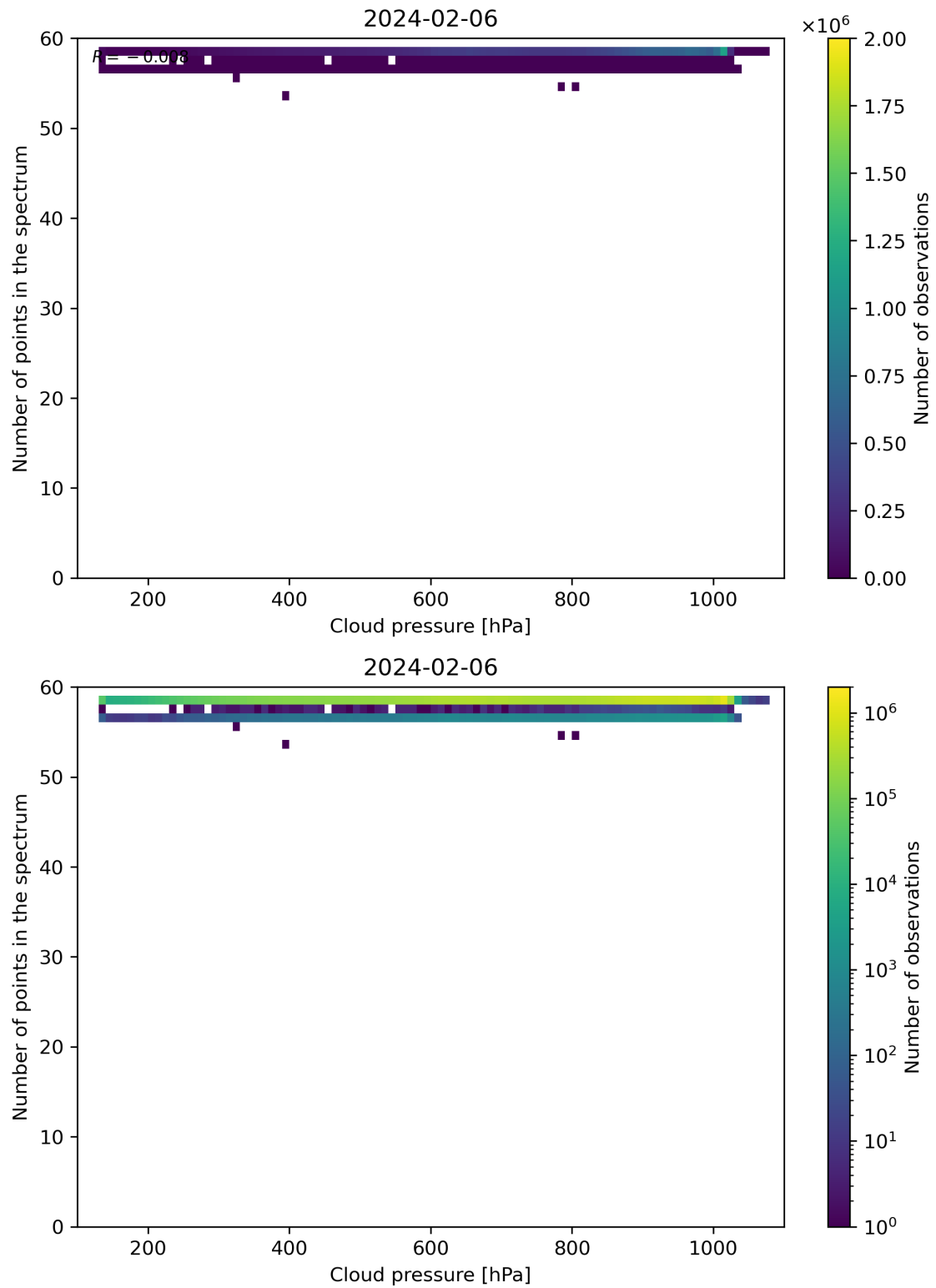
Figure 82: Scatter density plot of “Cloud pressure” against “Number of points in the spectrum” for 2024-02-06 to 2024-02-07.
