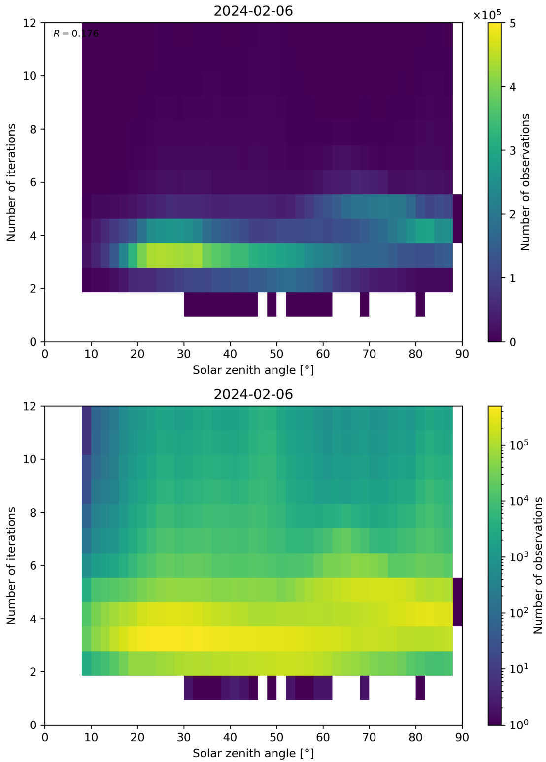
Figure 114: Scatter density plot of “Solar zenith angle” against “Number of iterations” for 2024-02-06 to 2024-02-07.
