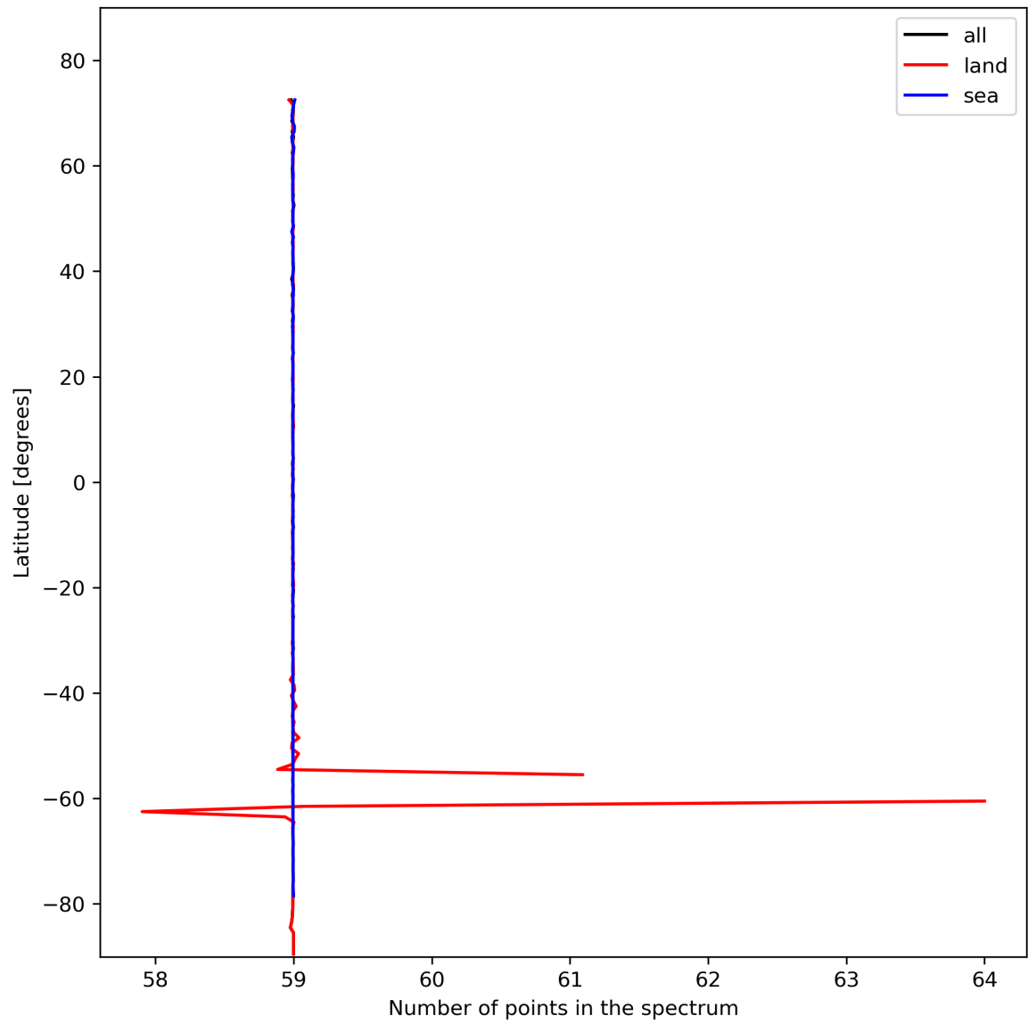
Figure 27: Zonal average of “Number of points in the spectrum” for 2024-02-06 to 2024-02-07.
