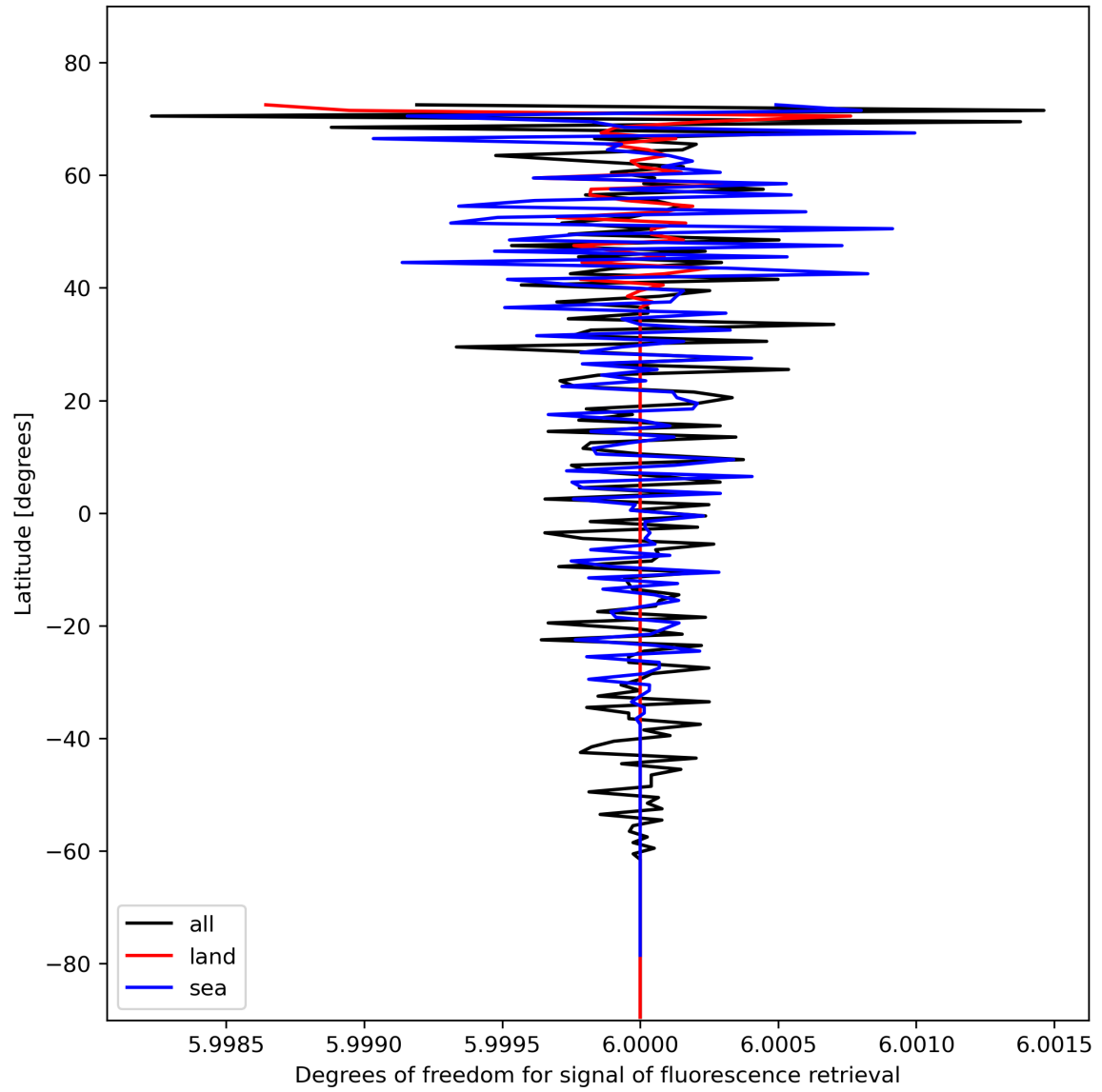
Figure 26: Zonal average of “Degrees of freedom for signal of fluorescence retrieval” for 2024-02-06 to 2024-02-07.
