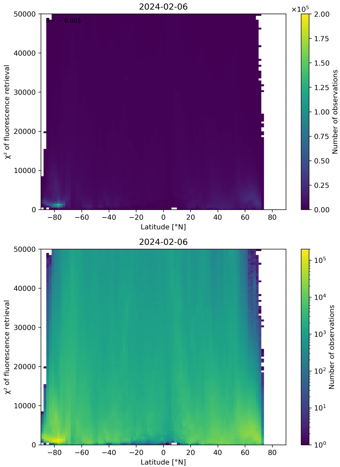
Figure 89: Scatter density plot of “Latitude” against “ \chi^2 of fluorescence retrieval” for 2024-02-06 to 2024-02-07.
