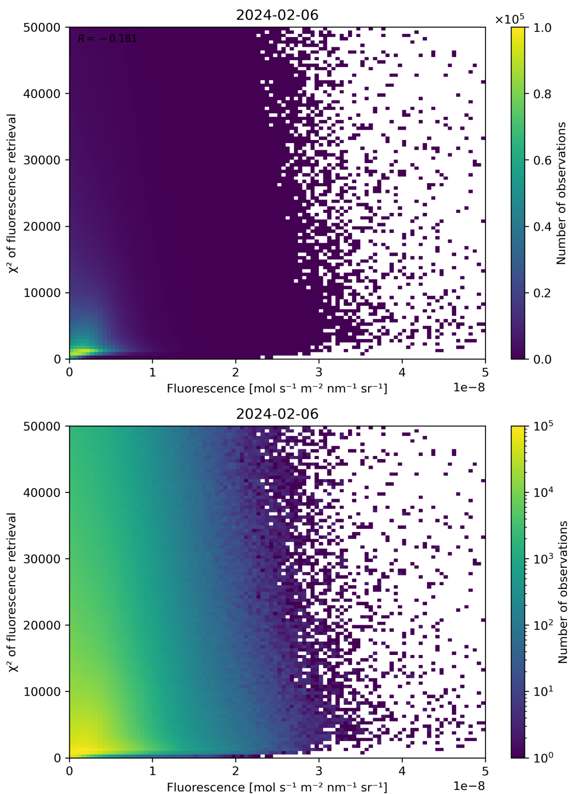
Figure 85: Scatter density plot of “Fluorescence” against “ \chi^2 of fluorescence retrieval” for 2024-02-06 to 2024-02-07.
