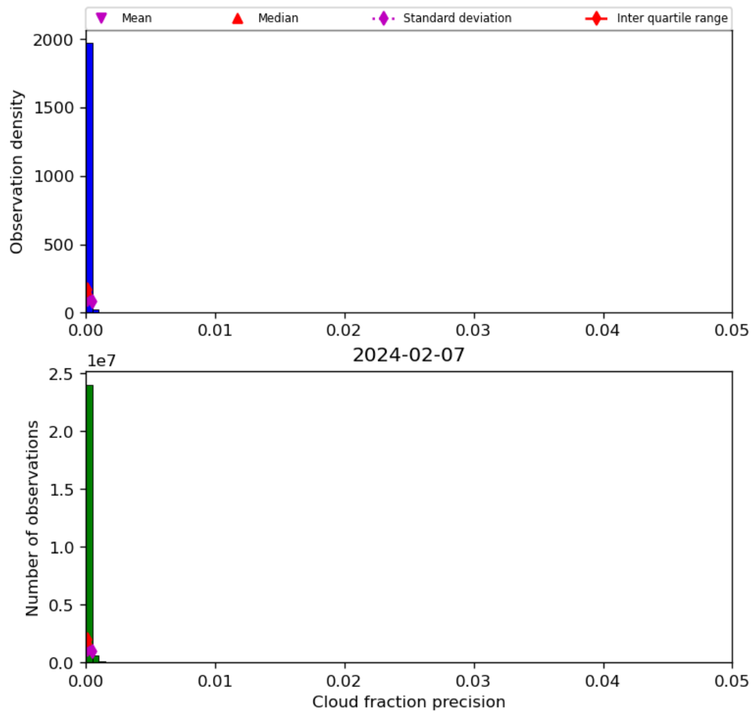
Figure 33: Histogram of “Cloud fraction precision” for 2024-02-06 to 2024-02-08
