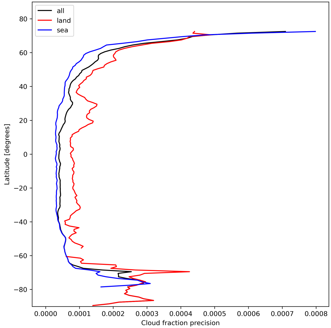
Figure 16: Zonal average of “Cloud fraction precision” for 2024-02-06 to 2024-02-08.
