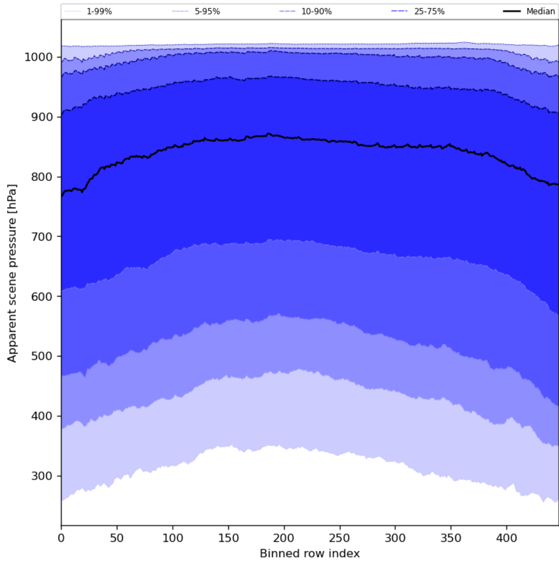
Figure 53: Along track statistics of “Apparent scene pressure” for 2024-02-06 to 2024-02-08
