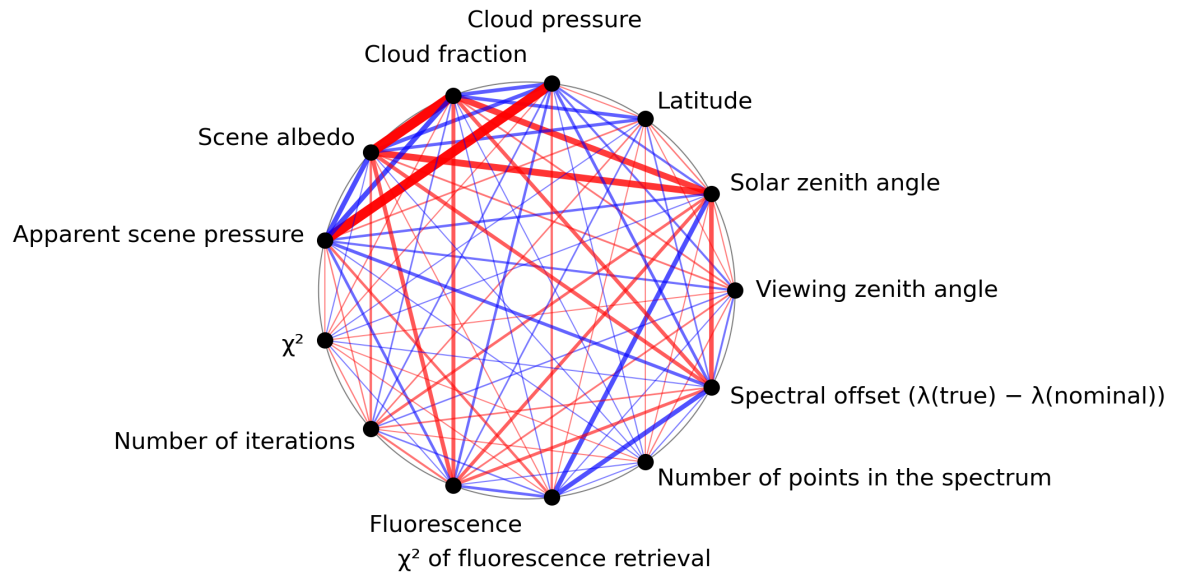
Figure 1: Map of correlation graph for 2024-02-06 to 2024-02-08.
