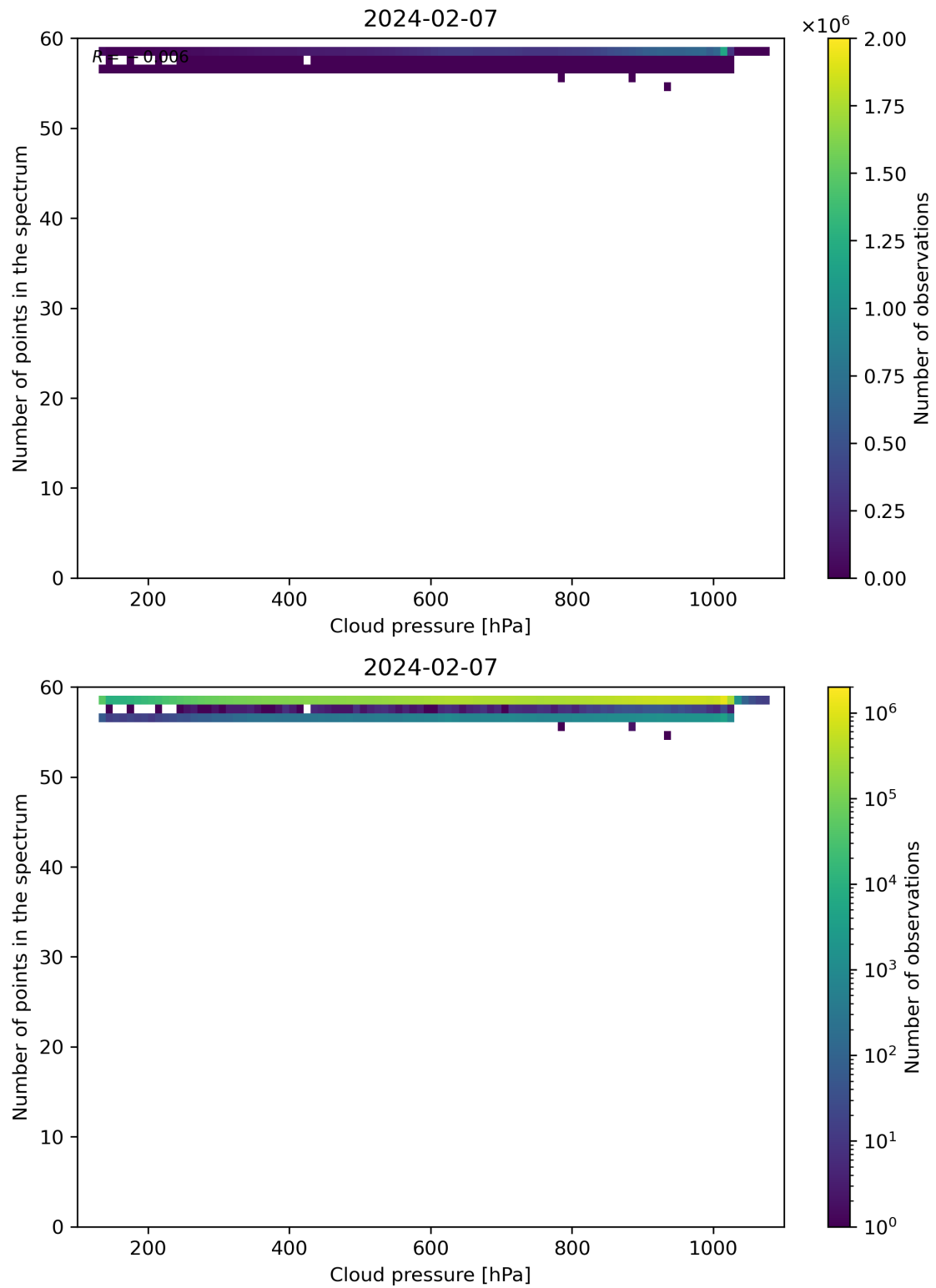
Figure 82: Scatter density plot of “Cloud pressure” against “Number of points in the spectrum” for 2024-02-06 to 2024-02-08.
