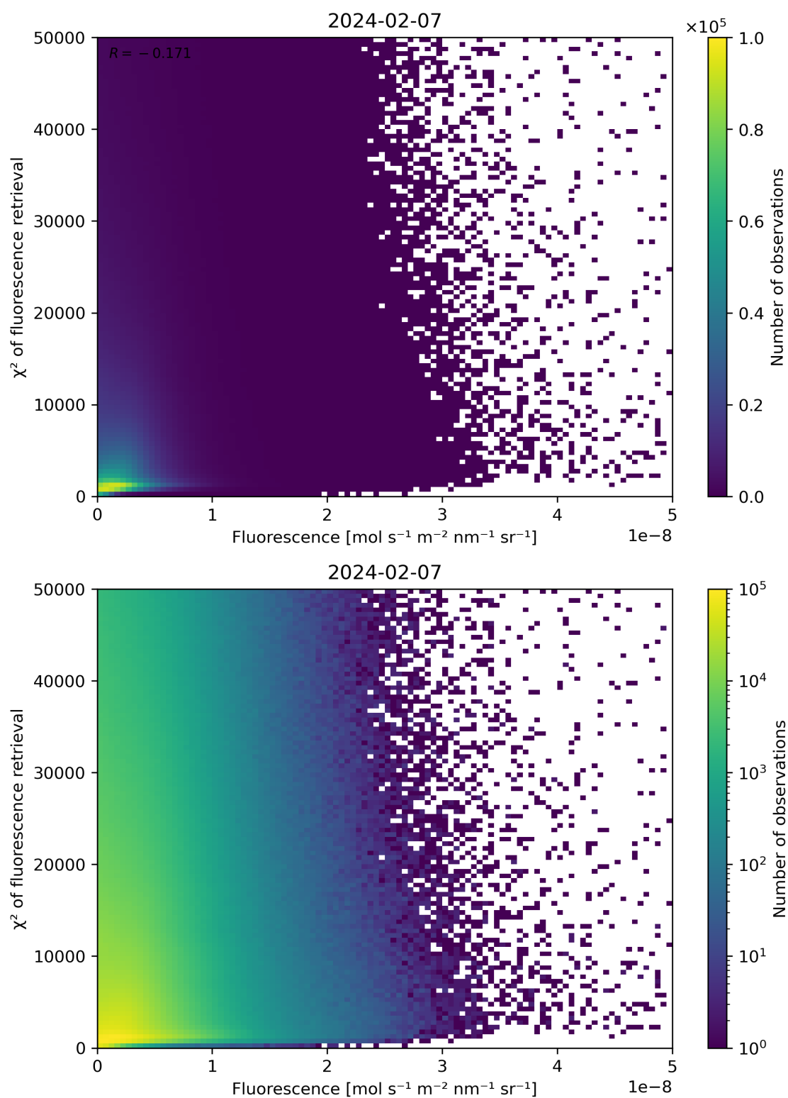
Figure 85: Scatter density plot of “Fluorescence” against “ \chi^2 of fluorescence retrieval” for 2024-02-06 to 2024-02-08.
