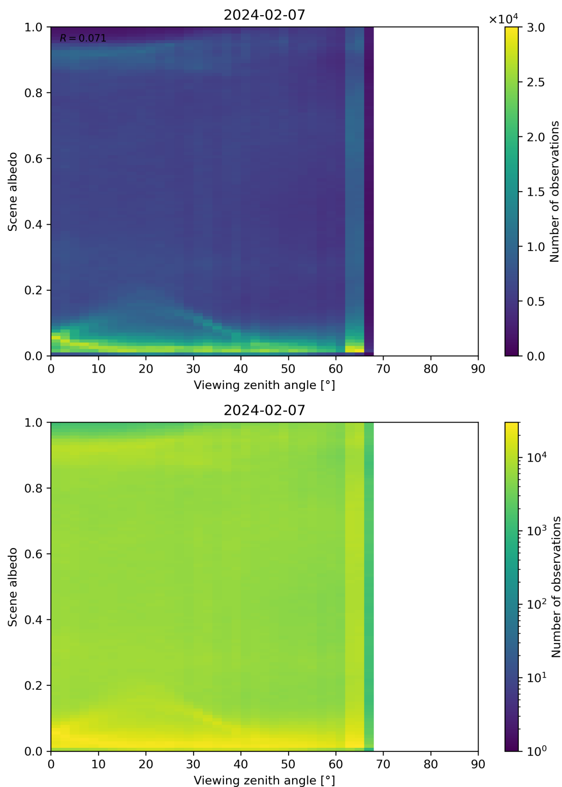
Figure 126: Scatter density plot of “Viewing zenith angle” against “Scene albedo” for 2024-02-06 to 2024-02-08.
