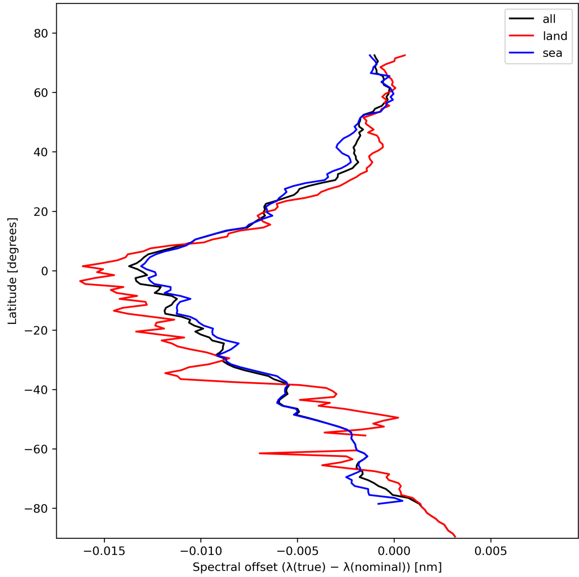
Figure 28: Zonal average of “Spectral offset ( \lambda(\text{true}) - \lambda(\text{nominal}) )” for 2024-02-06 to 2024-02-08.
