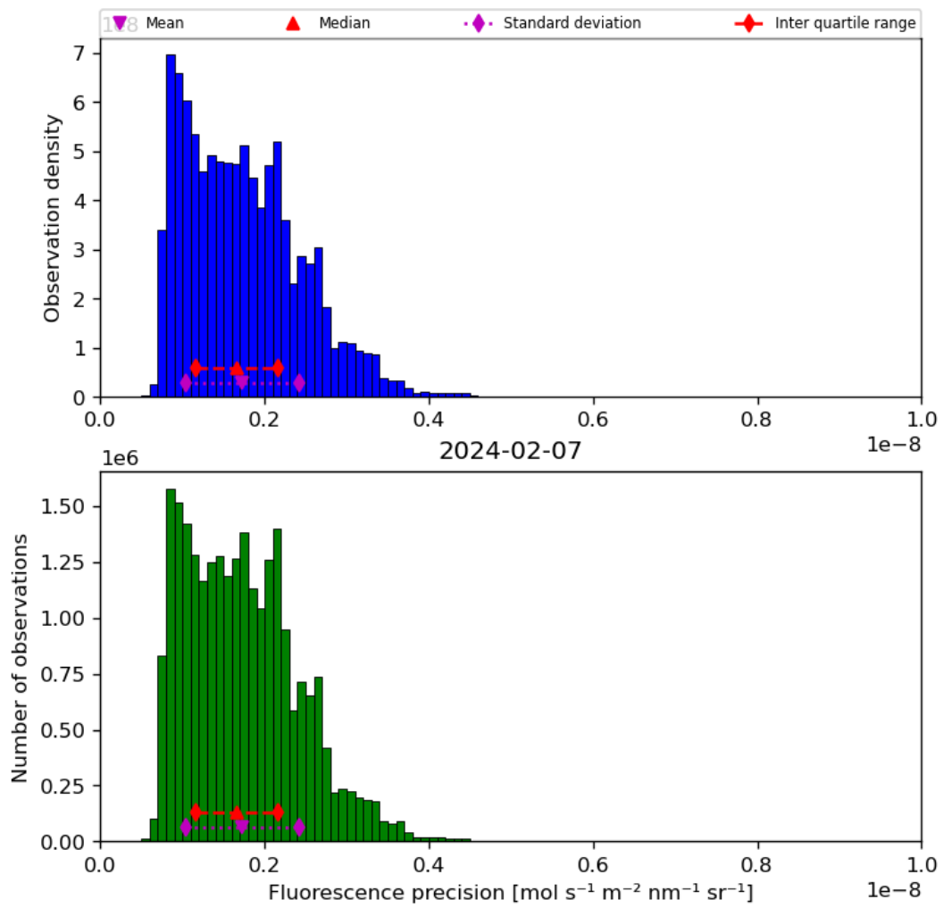
Figure 41: Histogram of “Fluorescence precision” for 2024-02-06 to 2024-02-08
