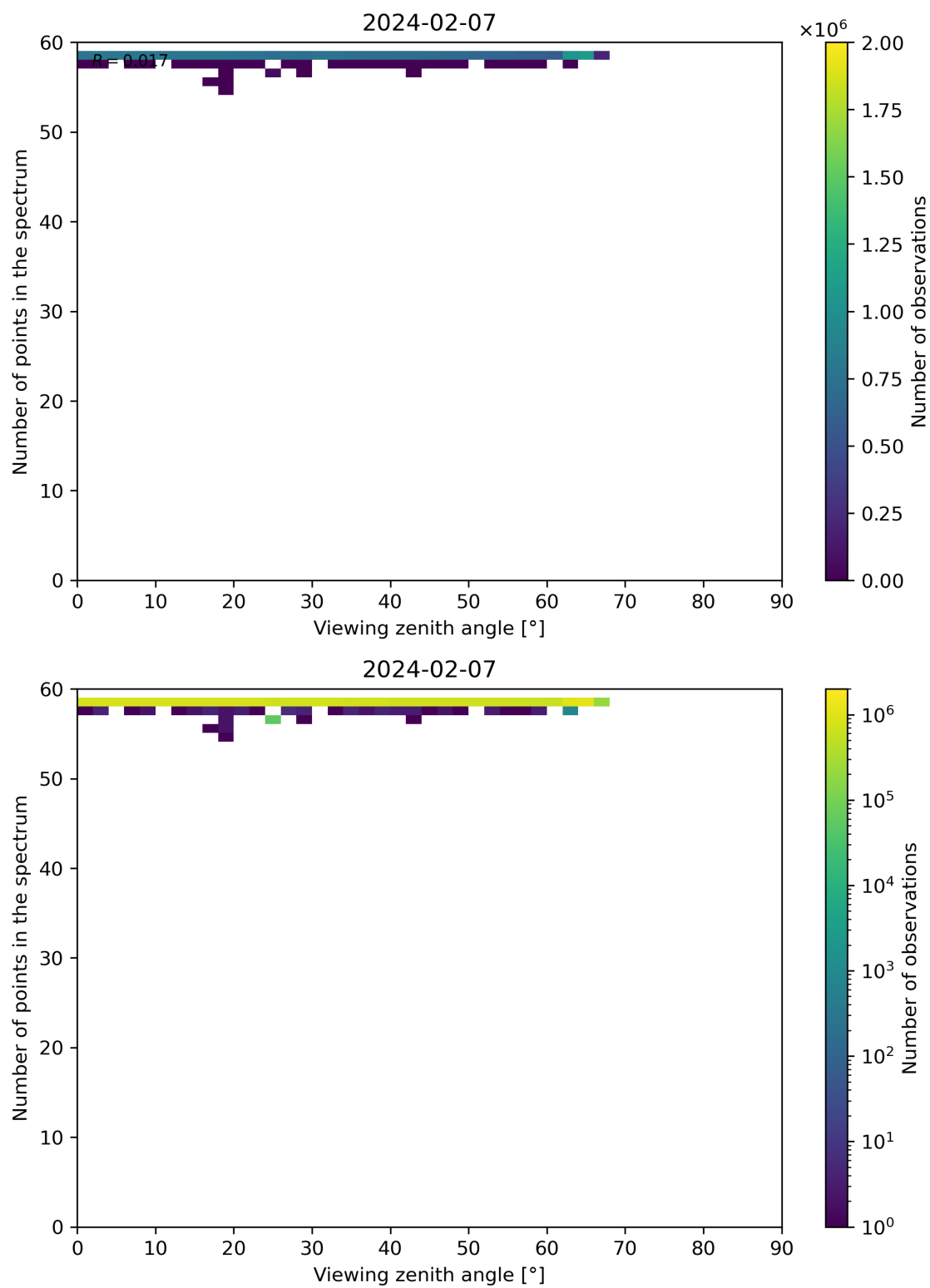
Figure 125: Scatter density plot of “Viewing zenith angle” against “Number of points in the spectrum” for 2024-02-06 to 2024-02-08.
