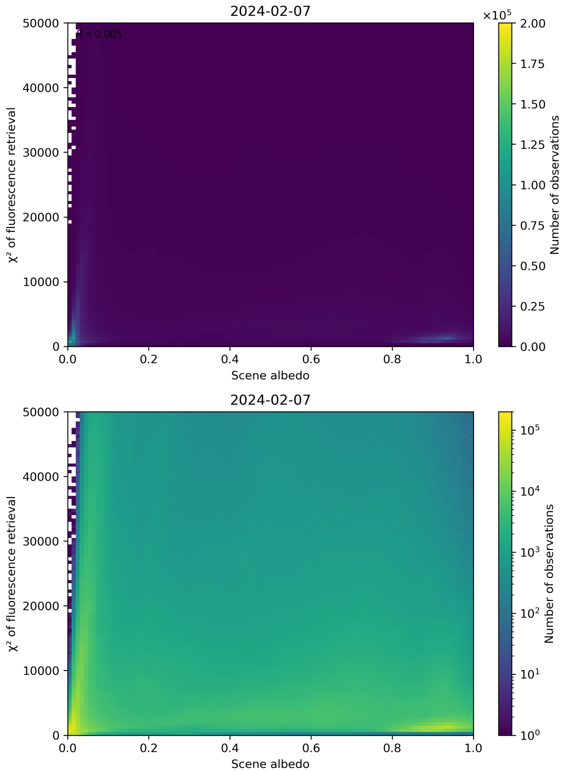
Figure 103: Scatter density plot of “Scene albedo” against “ \chi^2 of fluorescence retrieval” for 2024-02-06 to 2024-02-08.
