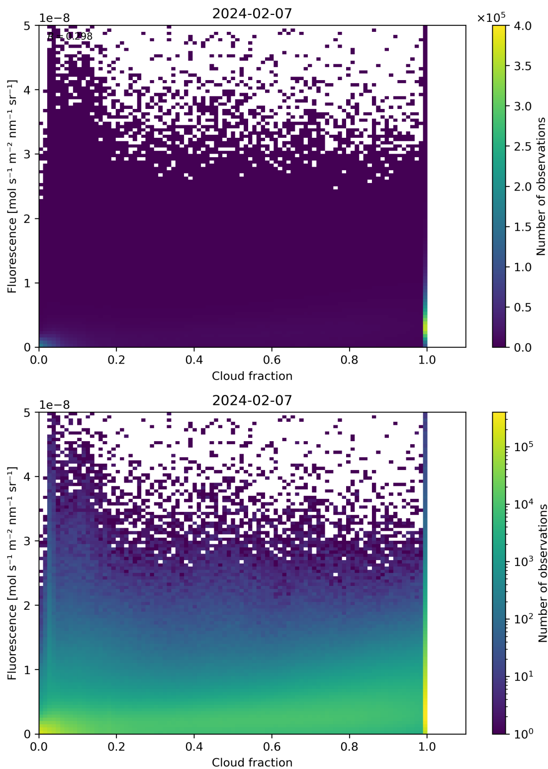
Figure 72: Scatter density plot of “Cloud fraction” against “Fluorescence” for 2024-02-06 to 2024-02-08.
