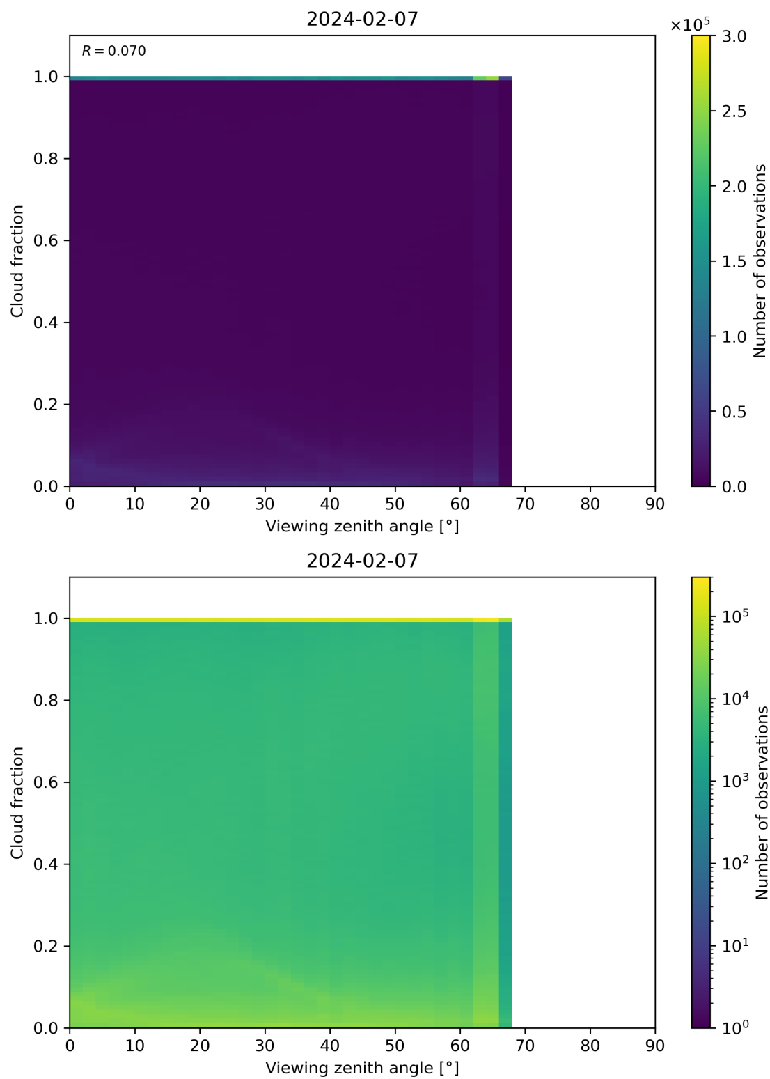
Figure 120: Scatter density plot of “Viewing zenith angle” against “Cloud fraction” for 2024-02-06 to 2024-02-08.
