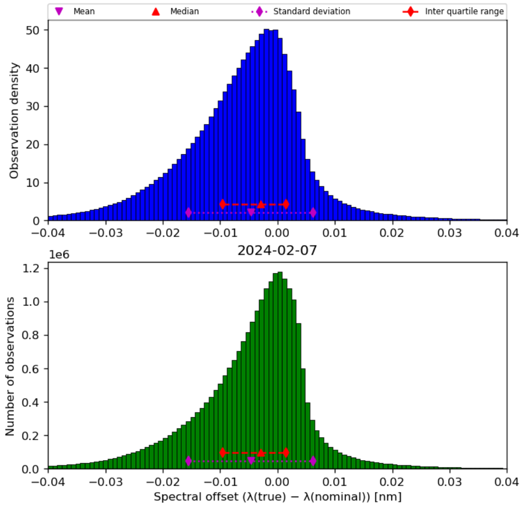
Figure 45: Histogram of “Spectral offset ( \lambda(\text{true}) - \lambda(\text{nominal}) )” for 2024-02-06 to 2024-02-08
