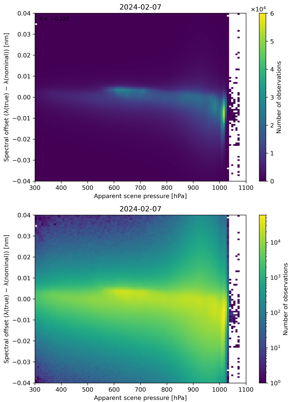
Figure 67: Scatter density plot of “Apparent scene pressure” against “Spectral offset ( \lambda(\text{true}) - \lambda(\text{nominal}) )” for 2024-02-06 to 2024-02-08.
