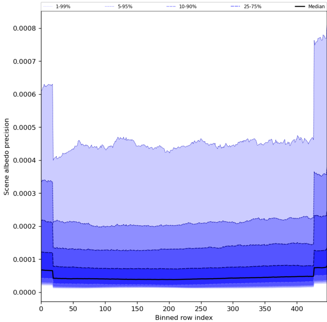
Figure 52: Along track statistics of “Scene albedo precision” for 2024-02-06 to 2024-02-08
