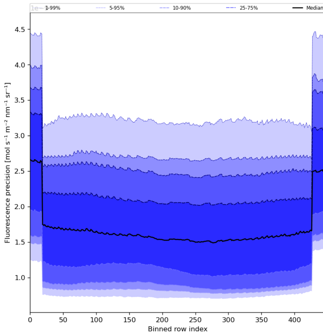
Figure 58: Along track statistics of “Fluorescence precision” for 2024-02-06 to 2024-02-08
