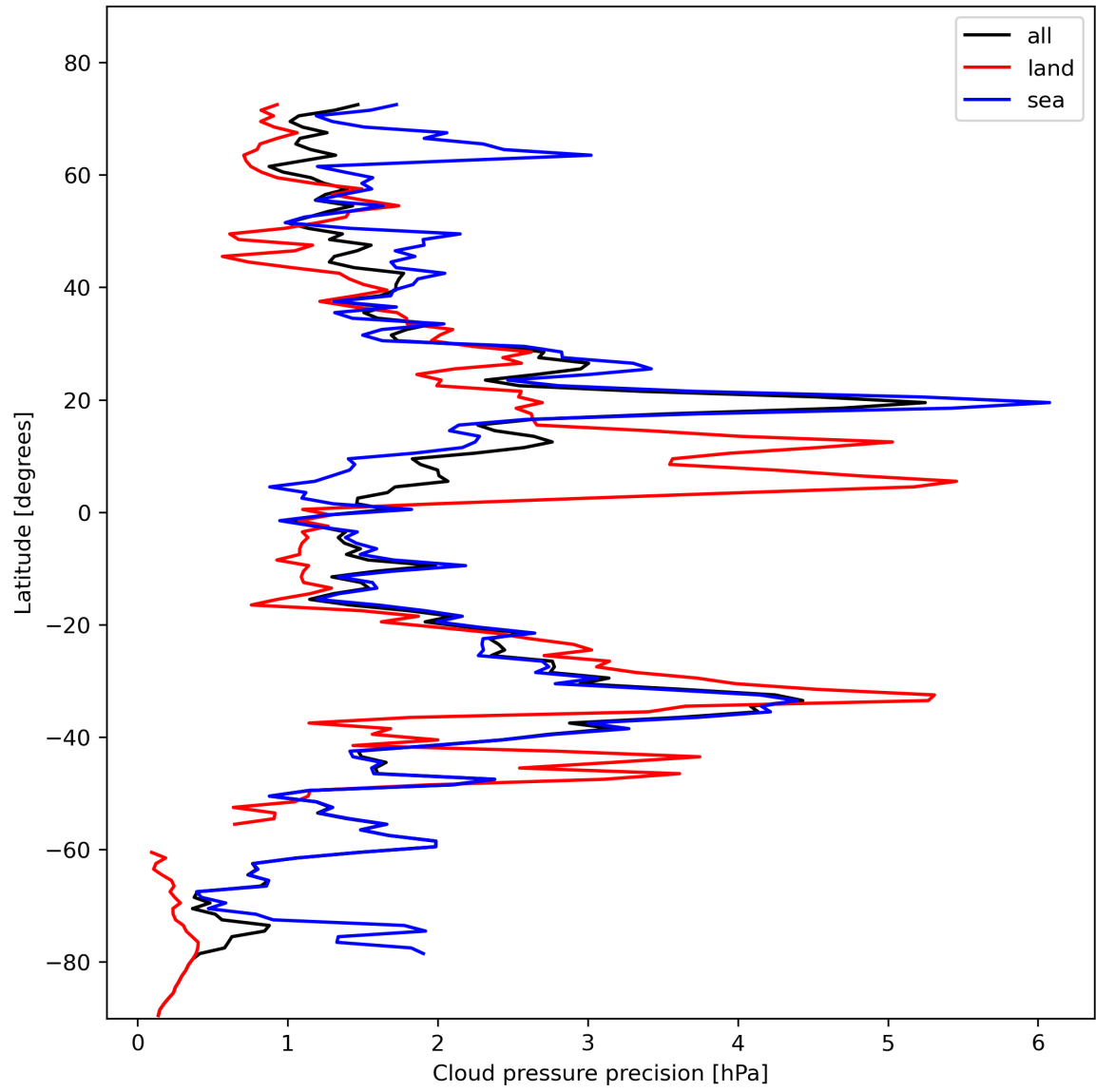
Figure 14: Zonal average of "Cloud pressure precision" for 2024-02-06 to 2024-02-08.
