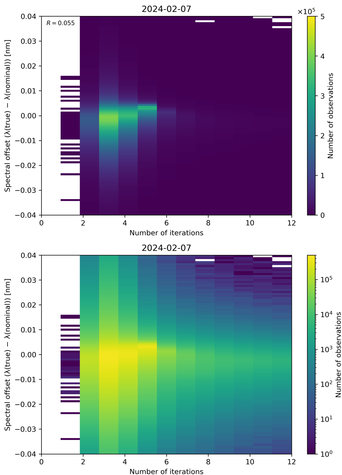
Figure 100: Scatter density plot of “Number of iterations” against “Spectral offset ( \lambda(\text{true}) - \lambda(\text{nominal}) )” for 2024-02-06 to 2024-02-08.
