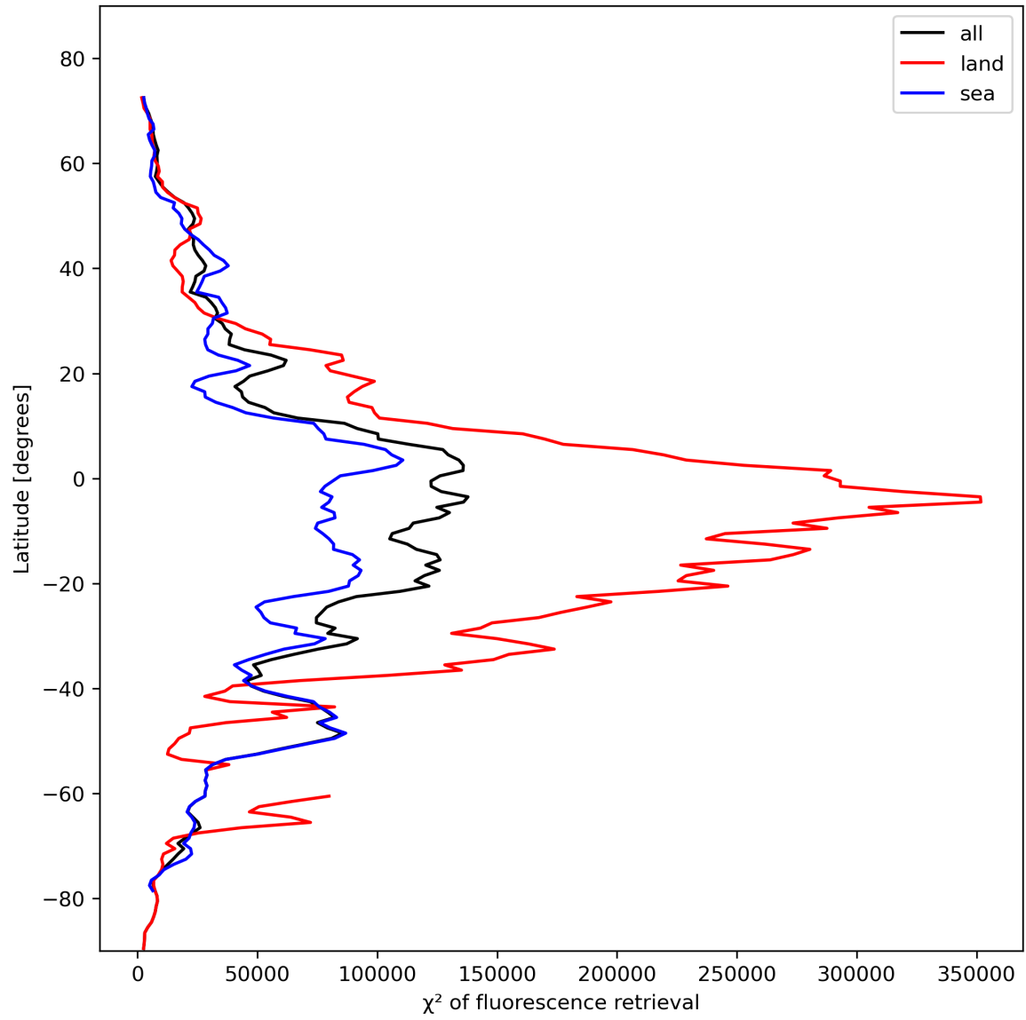
Figure 25: Zonal average of “ \chi^2 of fluorescence retrieval” for 2024-02-06 to 2024-02-08.
