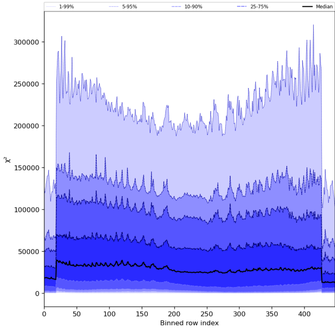
Figure 55: Along track statistics of “ \chi^2 ” for 2024-02-06 to 2024-02-08
