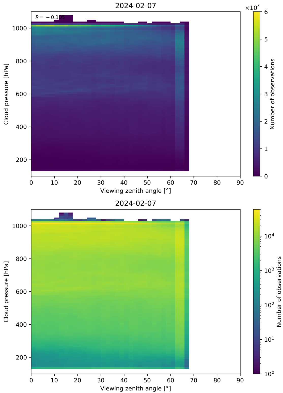
Figure 121: Scatter density plot of “Viewing zenith angle” against “Cloud pressure” for 2024-02-06 to 2024-02-08.
