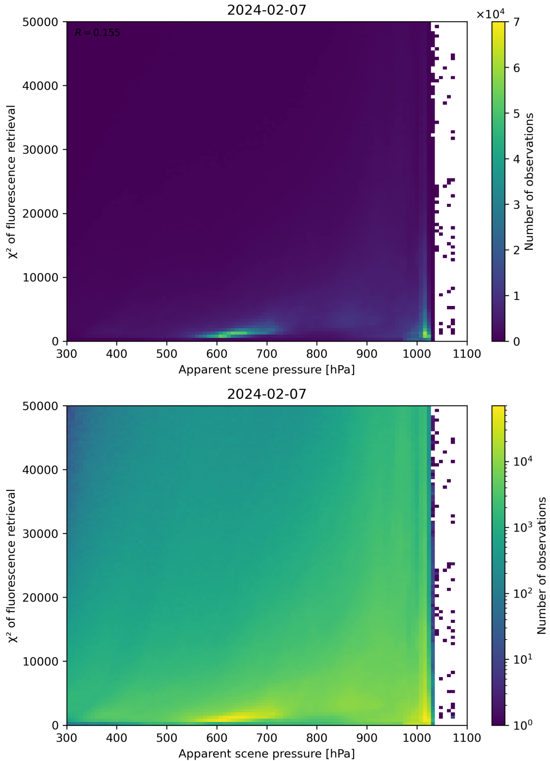
Figure 63: Scatter density plot of “Apparent scene pressure” against “ \chi^2 of fluorescence retrieval” for 2024-02-06 to 2024-02-08.
