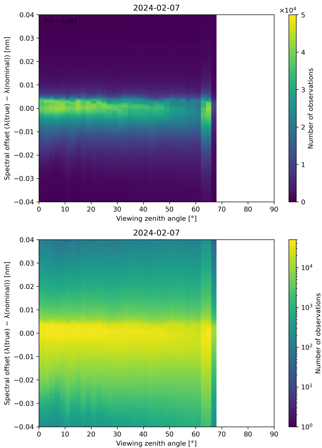
Figure 128: Scatter density plot of “Viewing zenith angle” against “Spectral offset ( \lambda(\text{true}) - \lambda(\text{nominal}) )” for 2024-02-06 to 2024-02-08.
