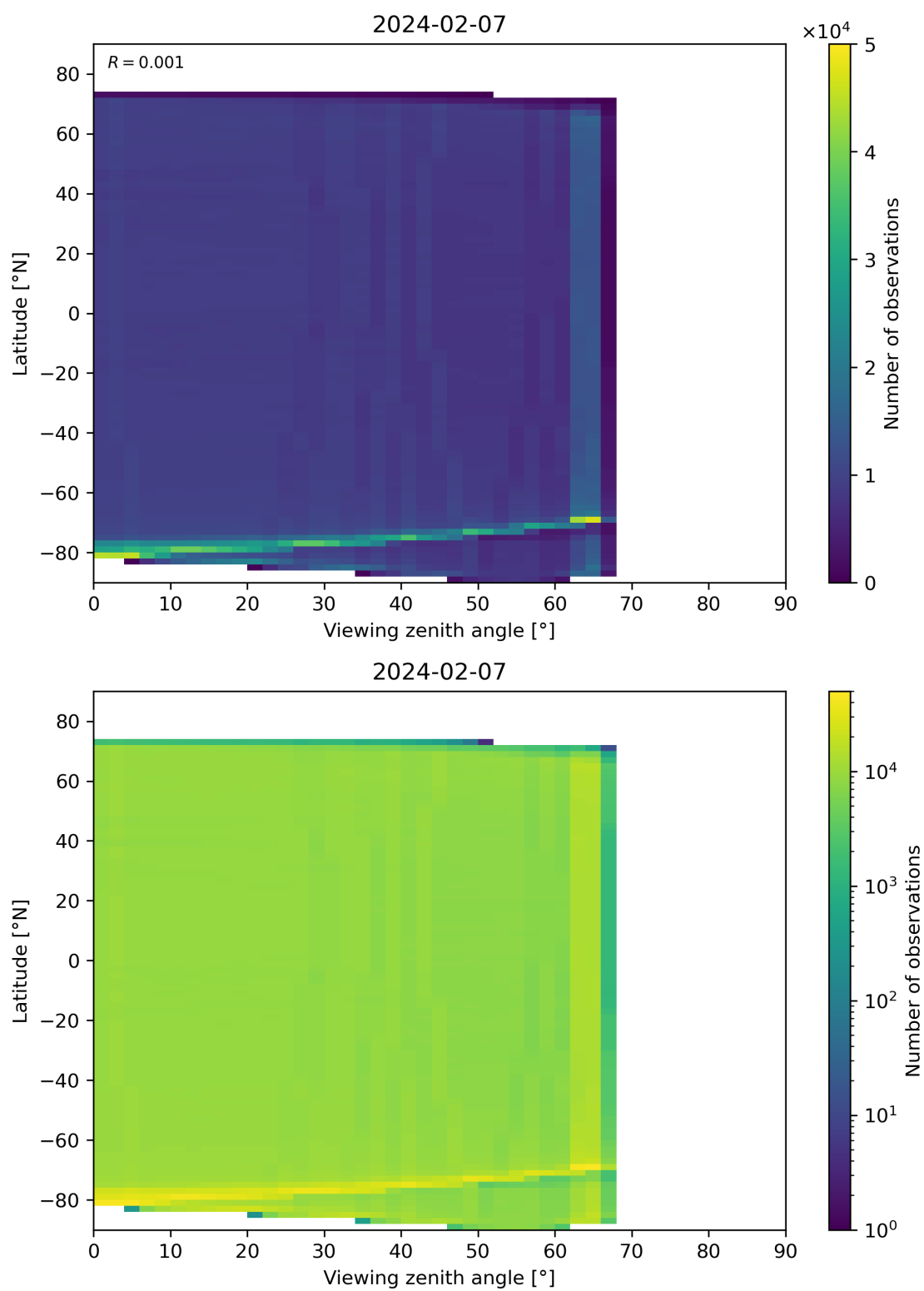
Figure 123: Scatter density plot of “Viewing zenith angle” against “Latitude” for 2024-02-06 to 2024-02-08.
