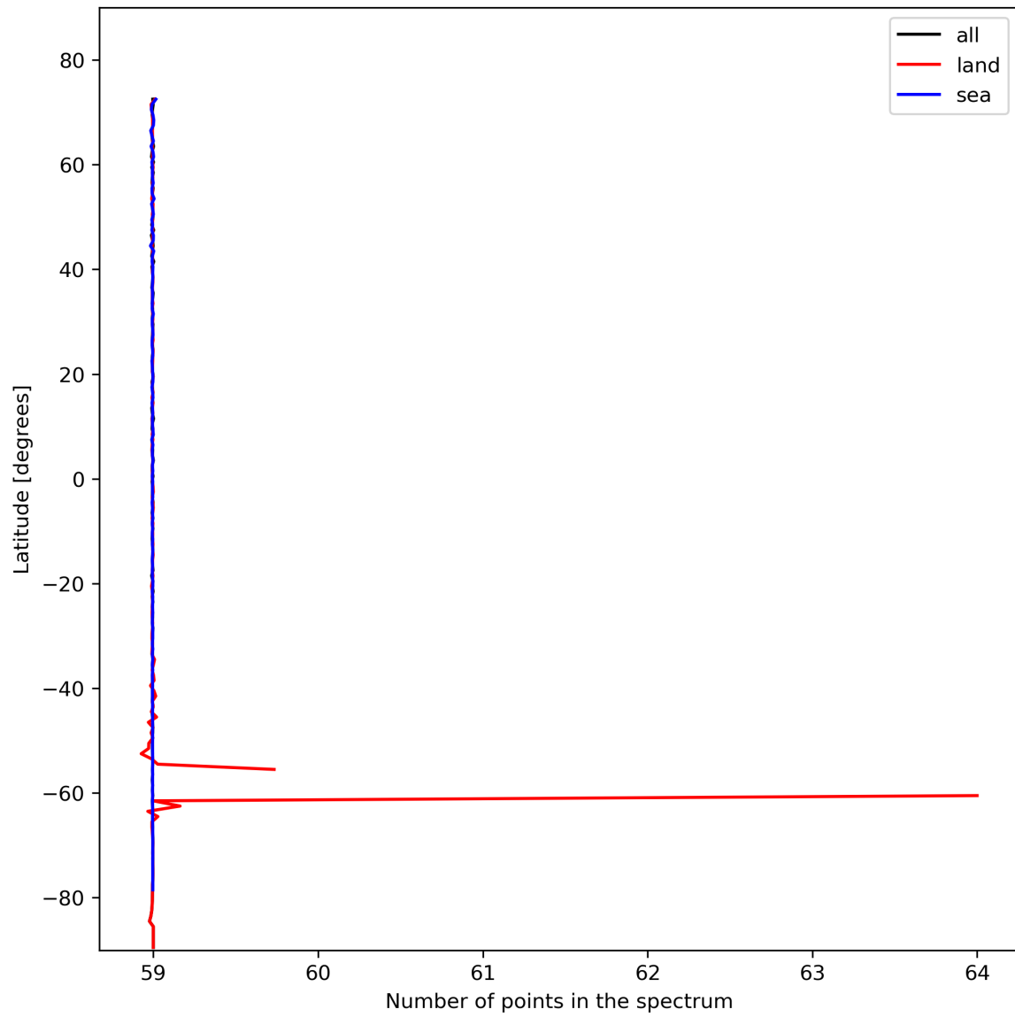
Figure 27: Zonal average of “Number of points in the spectrum” for 2024-02-06 to 2024-02-08.
