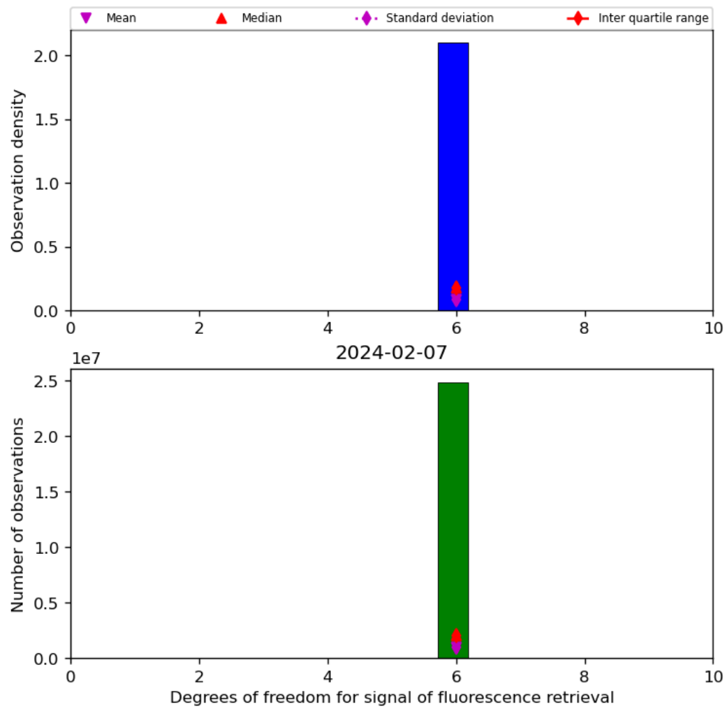
Figure 43: Histogram of “Degrees of freedom for signal of fluorescence retrieval” for 2024-02-06 to 2024-02-08
