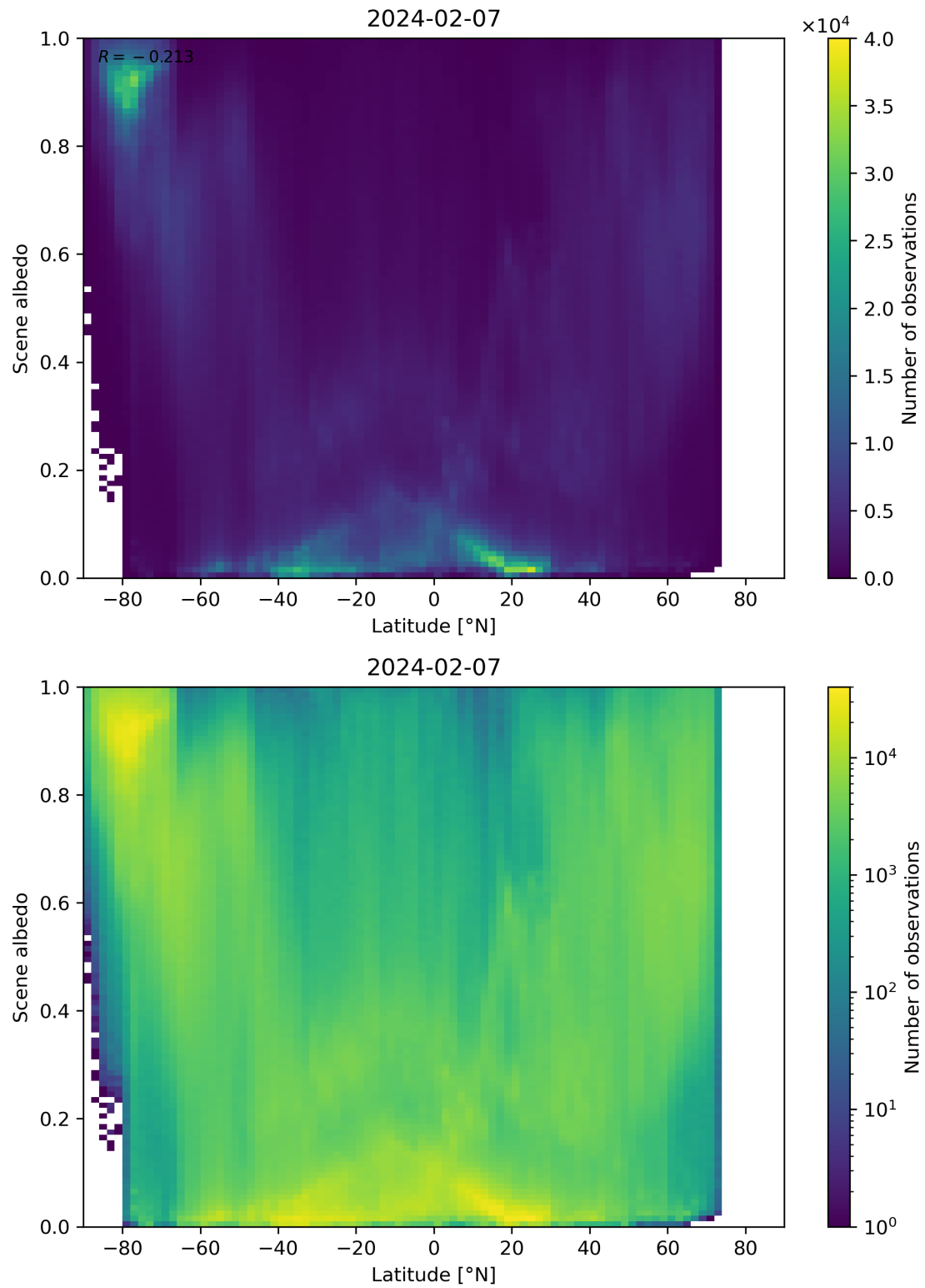
Figure 95: Scatter density plot of “Latitude” against “Scene albedo” for 2024-02-06 to 2024-02-08.
