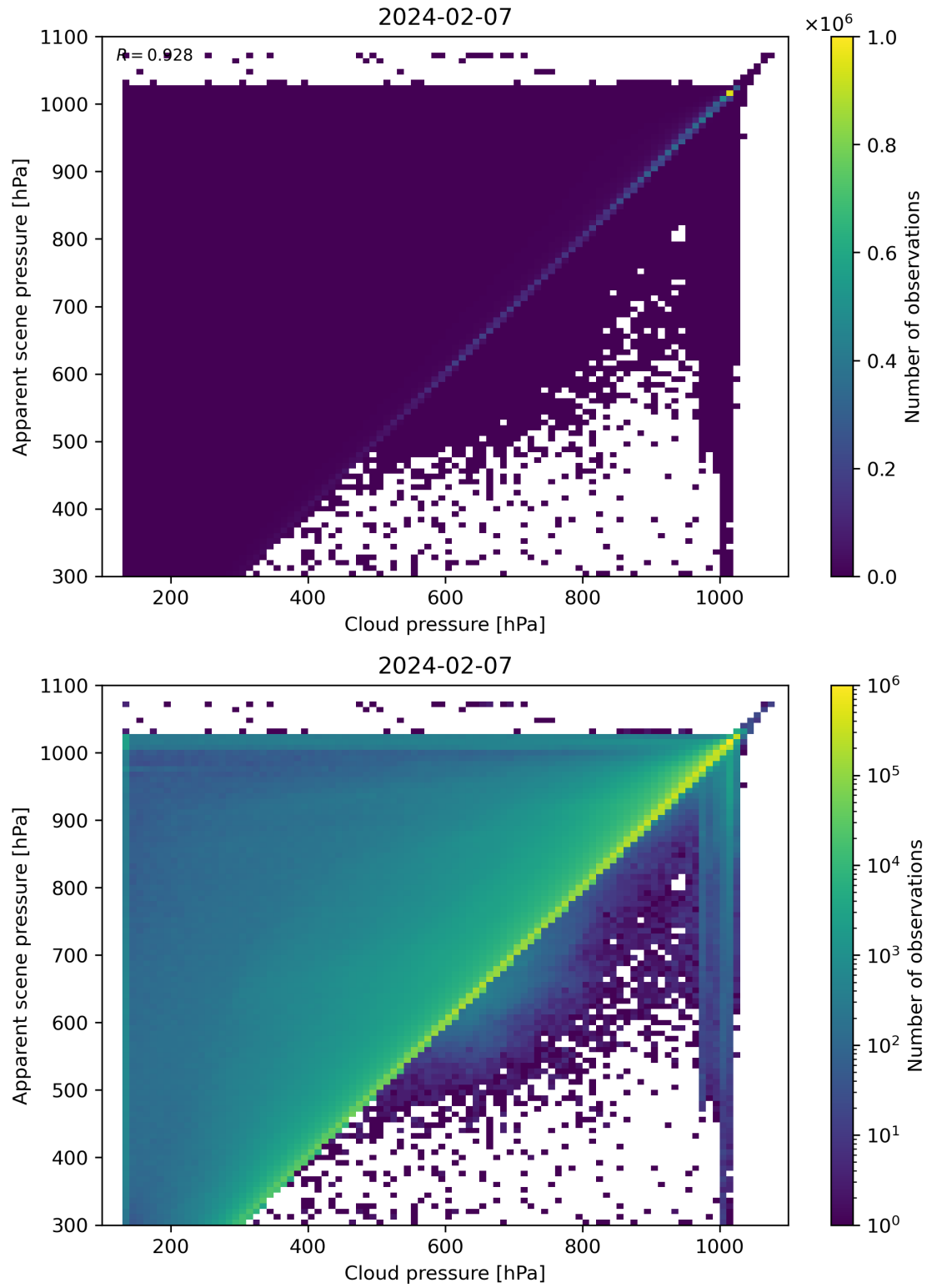
Figure 77: Scatter density plot of “Cloud pressure” against “Apparent scene pressure” for 2024-02-06 to 2024-02-08.
