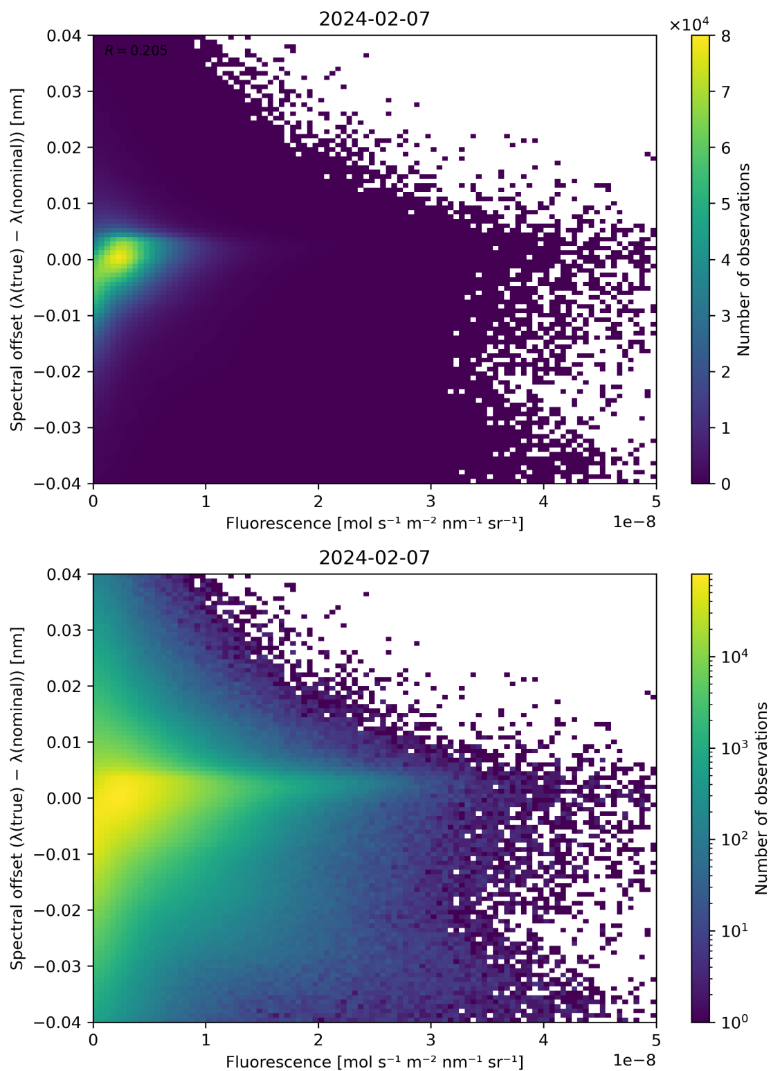
Figure 87: Scatter density plot of “Fluorescence” against “Spectral offset ( \lambda(\text{true}) - \lambda(\text{nominal}) )” for 2024-02-06 to 2024-02-08.
