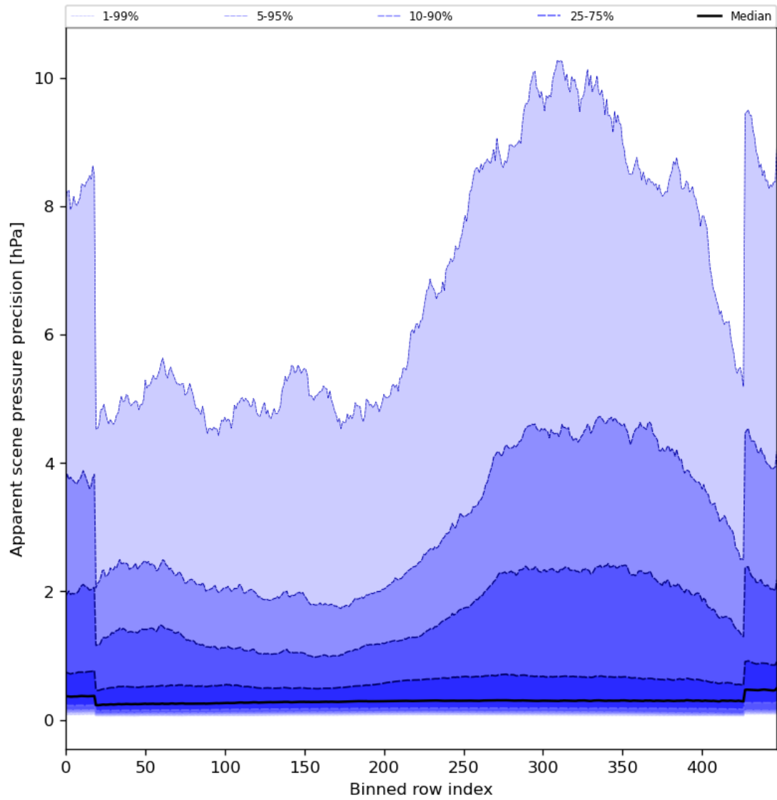
Figure 54: Along track statistics of “Apparent scene pressure precision” for 2024-02-06 to 2024-02-08
