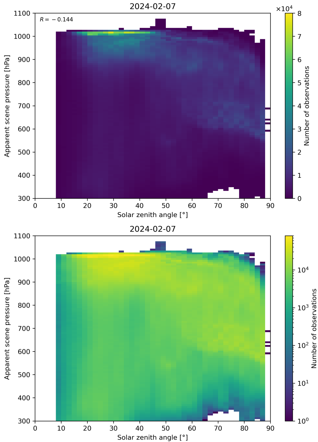
Figure 108: Scatter density plot of “Solar zenith angle” against “Apparent scene pressure” for 2024-02-06 to 2024-02-08.
