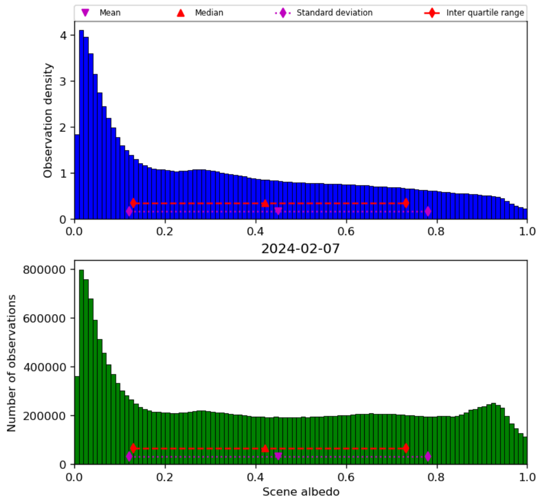
Figure 34: Histogram of “Scene albedo” for 2024-02-06 to 2024-02-08
