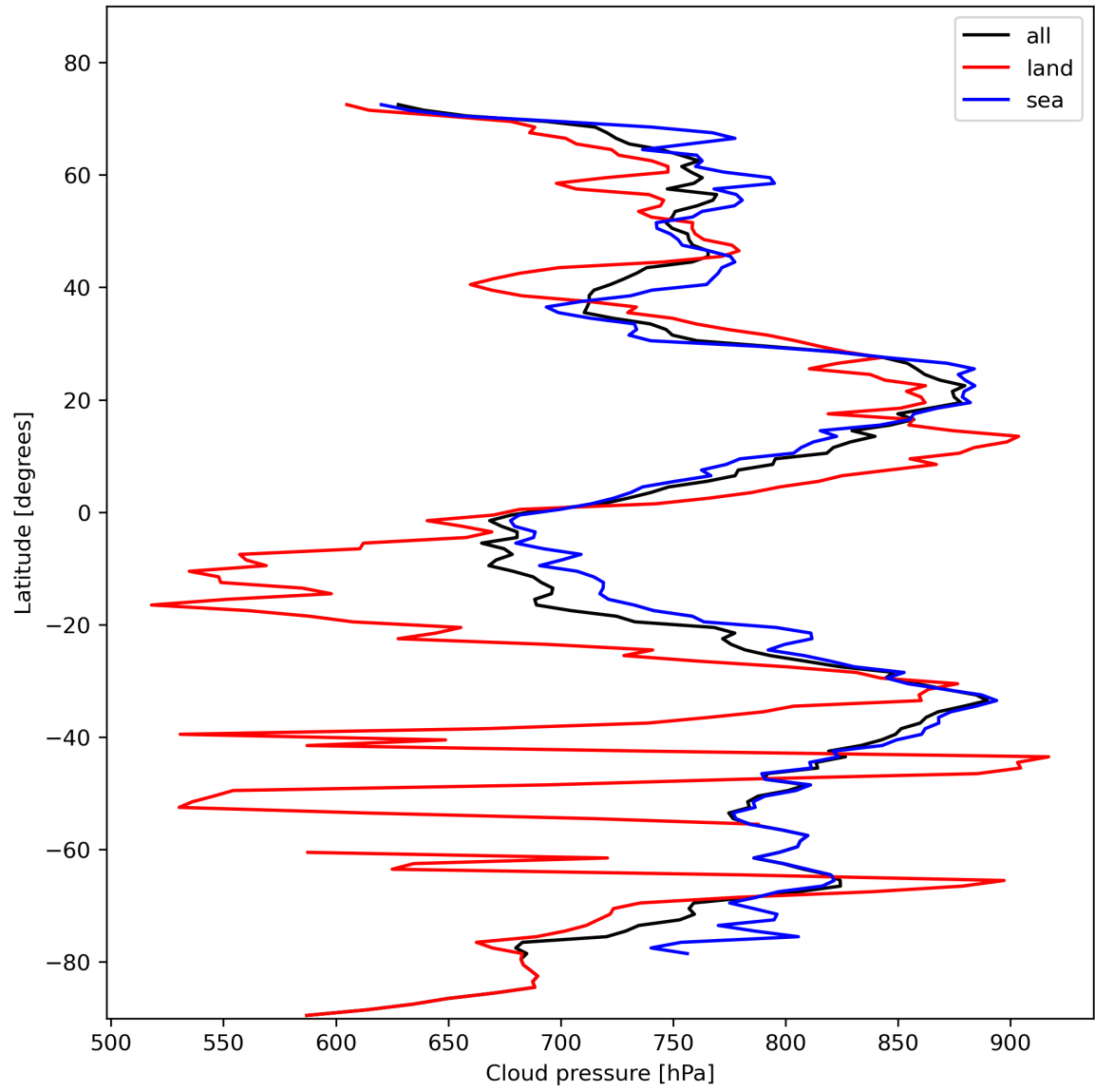
Figure 13: Zonal average of “Cloud pressure” for 2024-02-06 to 2024-02-08.
