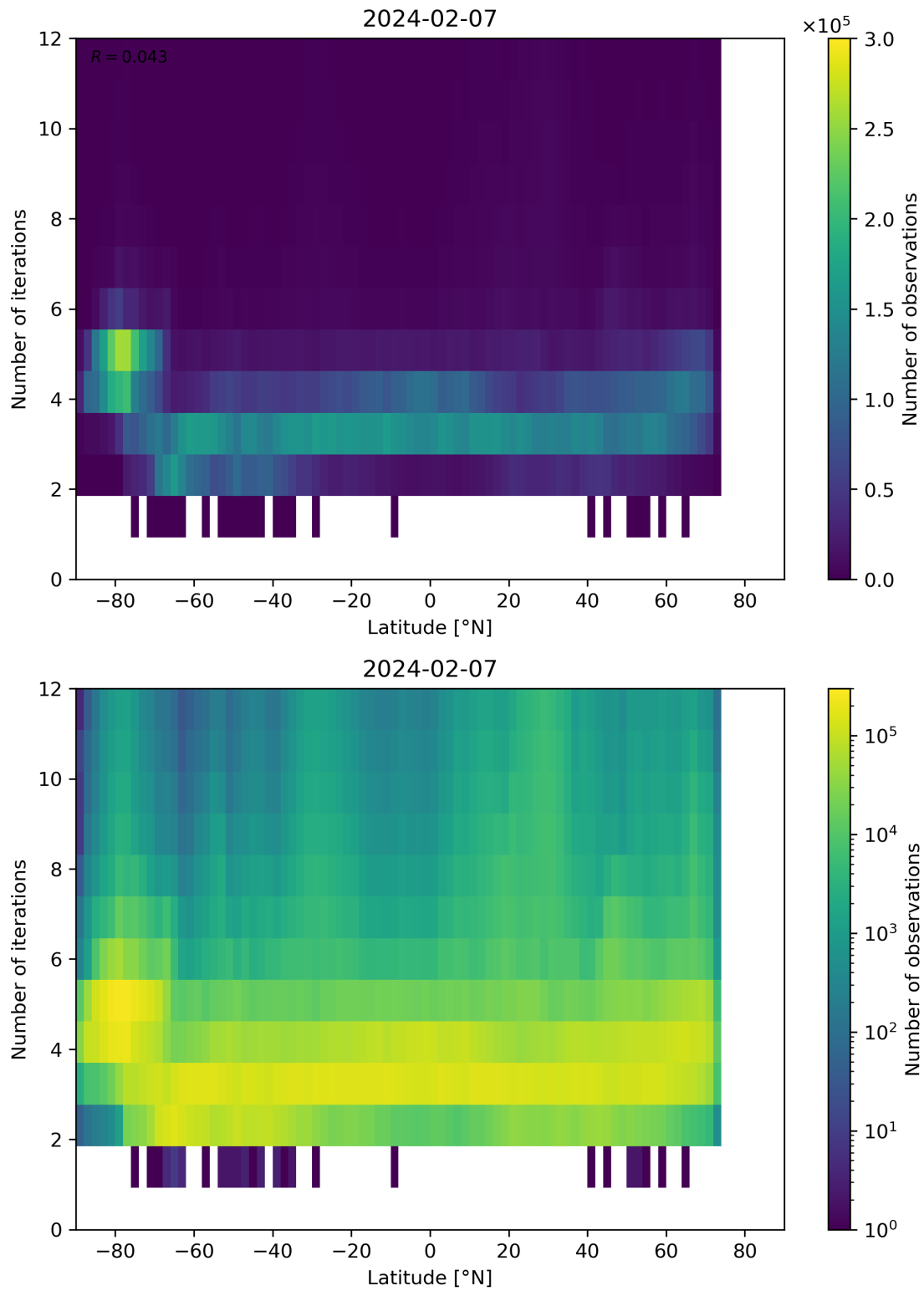
Figure 93: Scatter density plot of “Latitude” against “Number of iterations” for 2024-02-06 to 2024-02-08.
