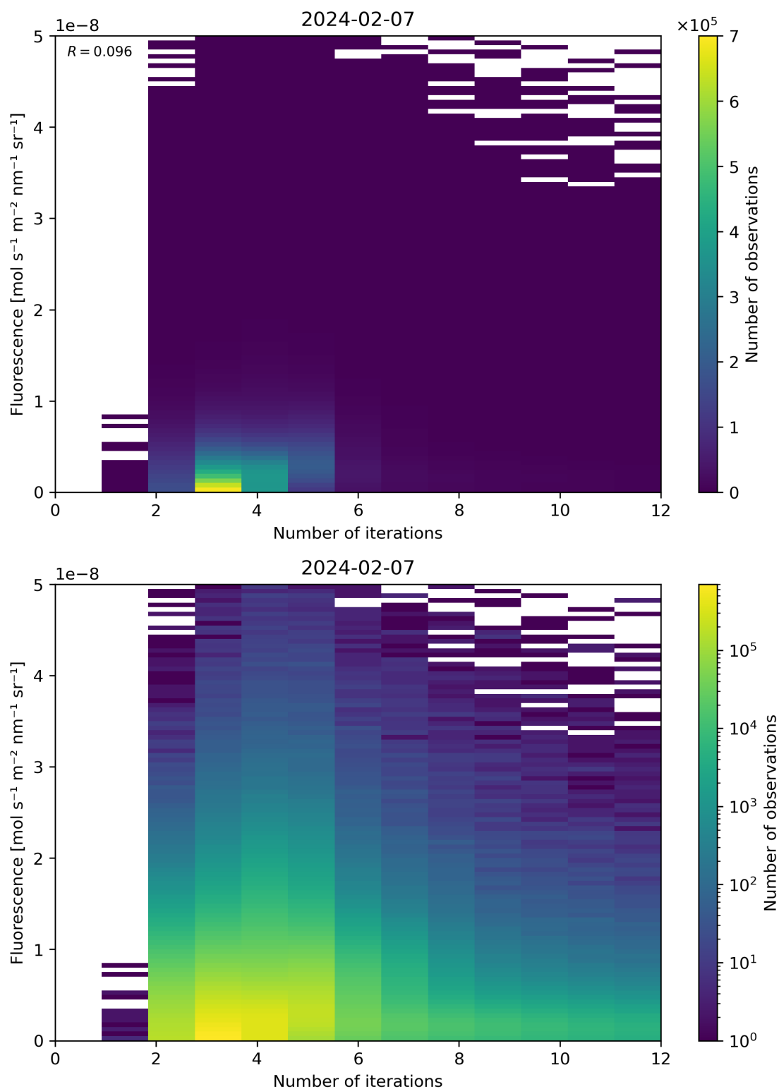
Figure 98: Scatter density plot of “Number of iterations” against “Fluorescence” for 2024-02-06 to 2024-02-08.
