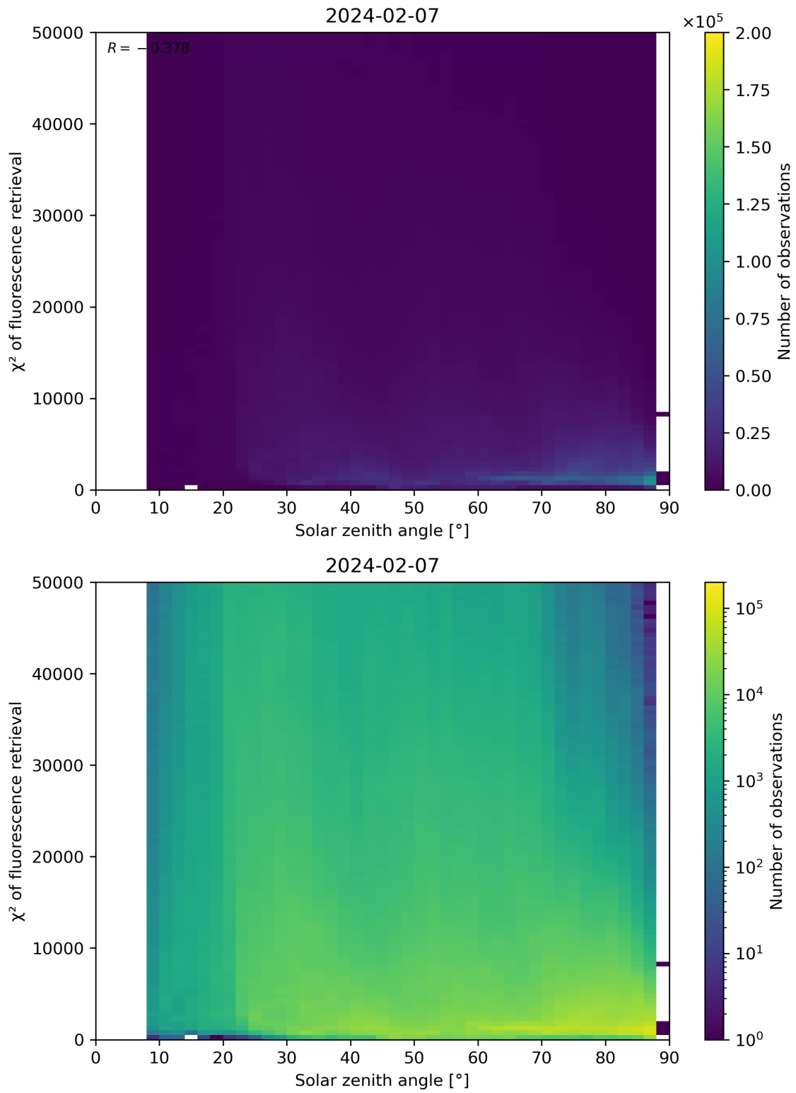
Figure 109: Scatter density plot of “Solar zenith angle” against “ \chi^2 of fluorescence retrieval” for 2024-02-06 to 2024-02-08.
