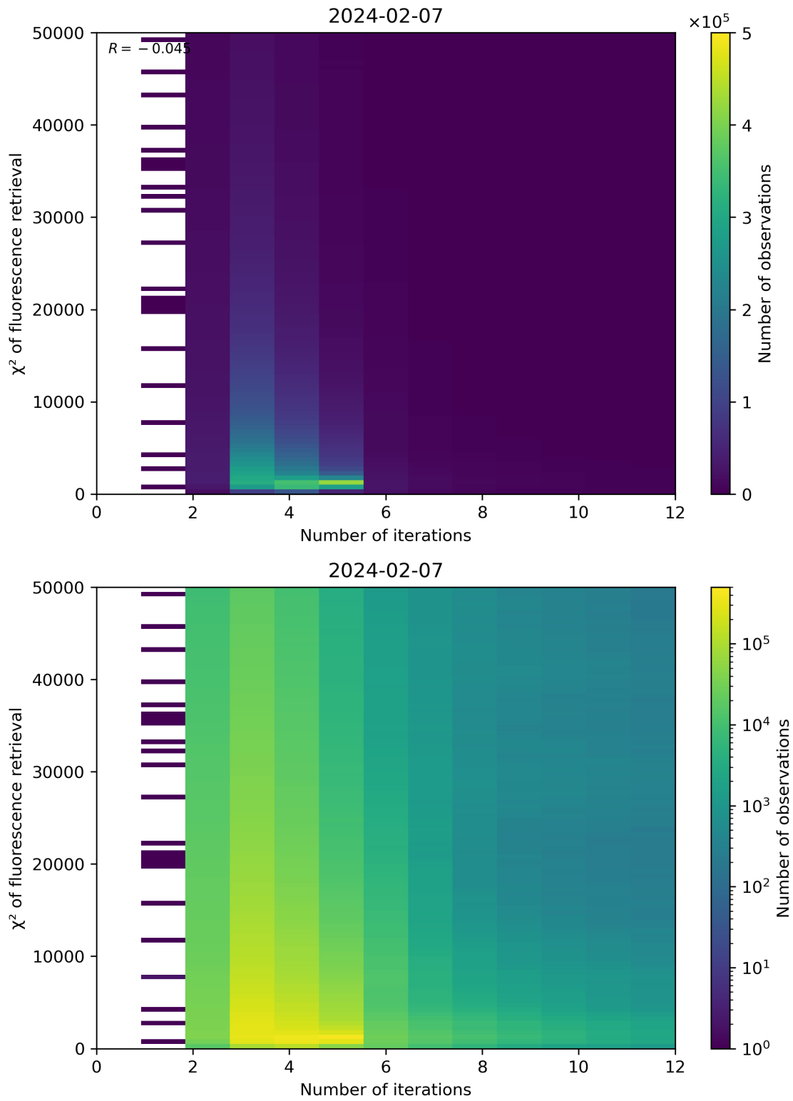
Figure 97: Scatter density plot of “Number of iterations” against “ \chi^2 of fluorescence retrieval” for 2024-02-06 to 2024-02-08.
