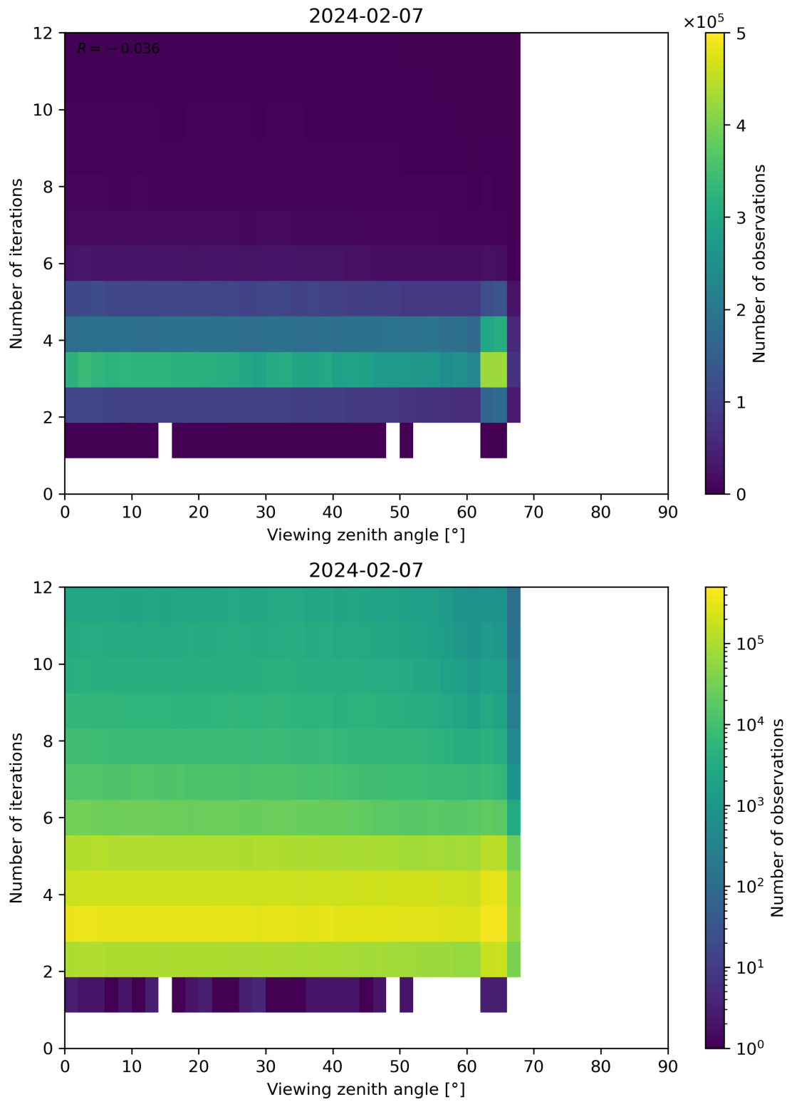
Figure 124: Scatter density plot of “Viewing zenith angle” against “Number of iterations” for 2024-02-06 to 2024-02-08.
