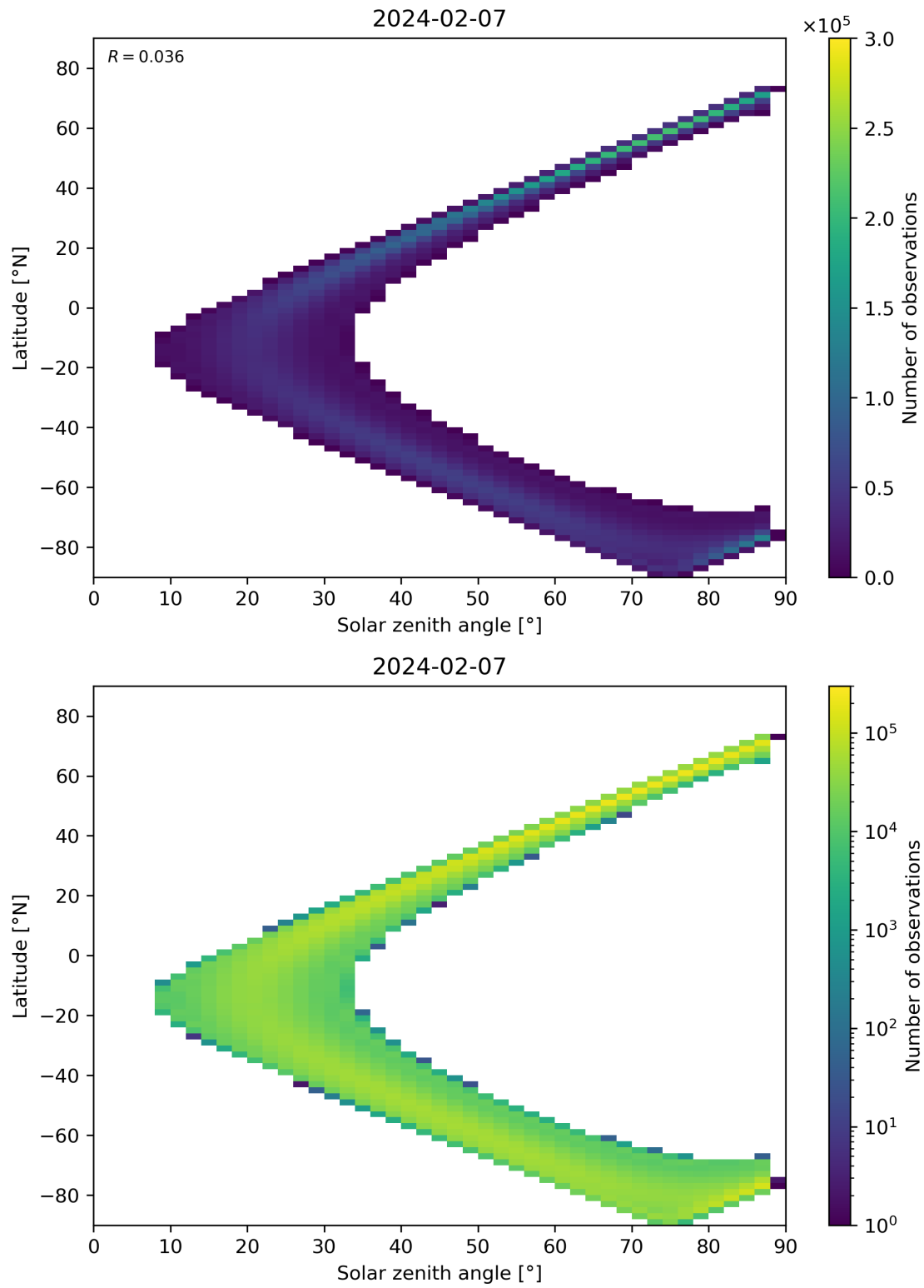
Figure 113: Scatter density plot of “Solar zenith angle” against “Latitude” for 2024-02-06 to 2024-02-08.
