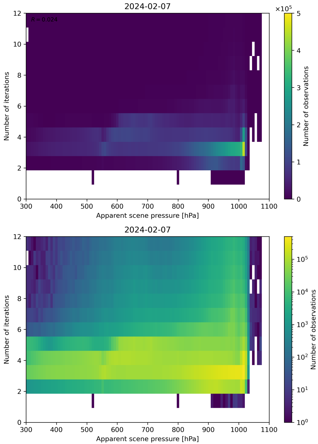
Figure 65: Scatter density plot of “Apparent scene pressure” against “Number of iterations” for 2024-02-06 to 2024-02-08.
