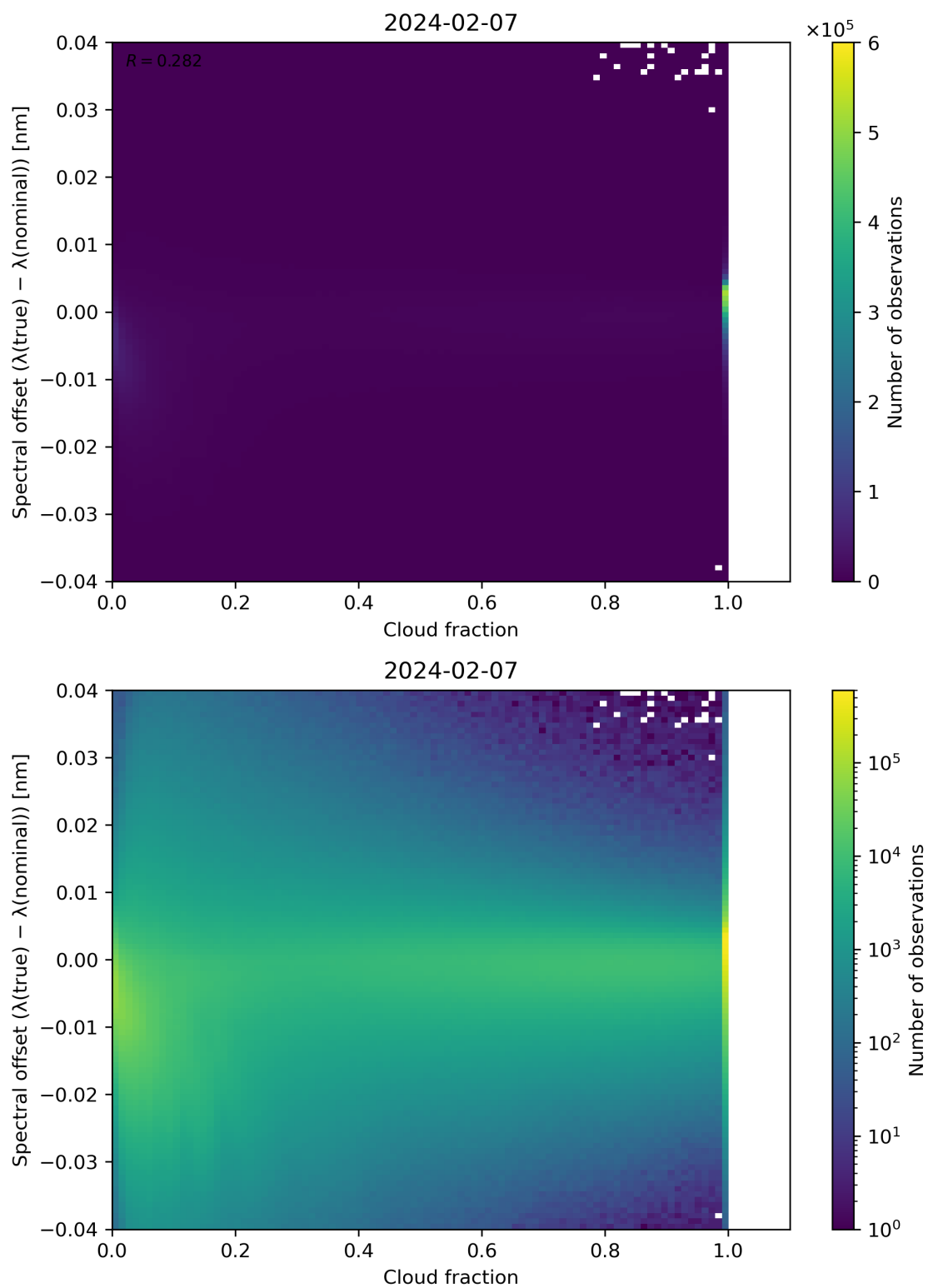
Figure 76: Scatter density plot of “Cloud fraction” against “Spectral offset ( \lambda(\text{true}) - \lambda(\text{nominal}) )” for 2024-02-06 to 2024-02-08.
