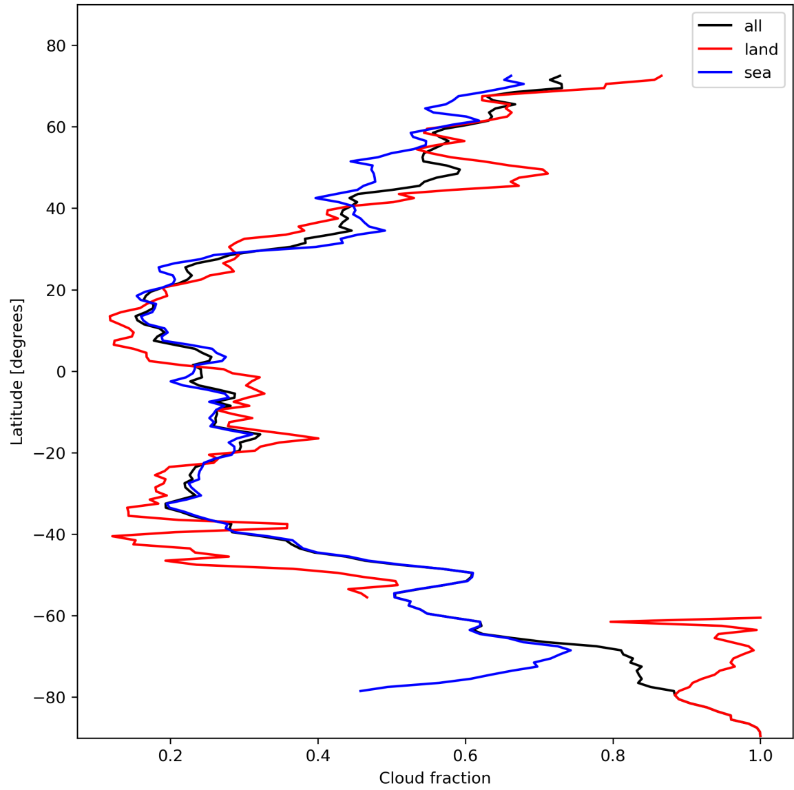
Figure 15: Zonal average of “Cloud fraction” for 2024-02-06 to 2024-02-08.
