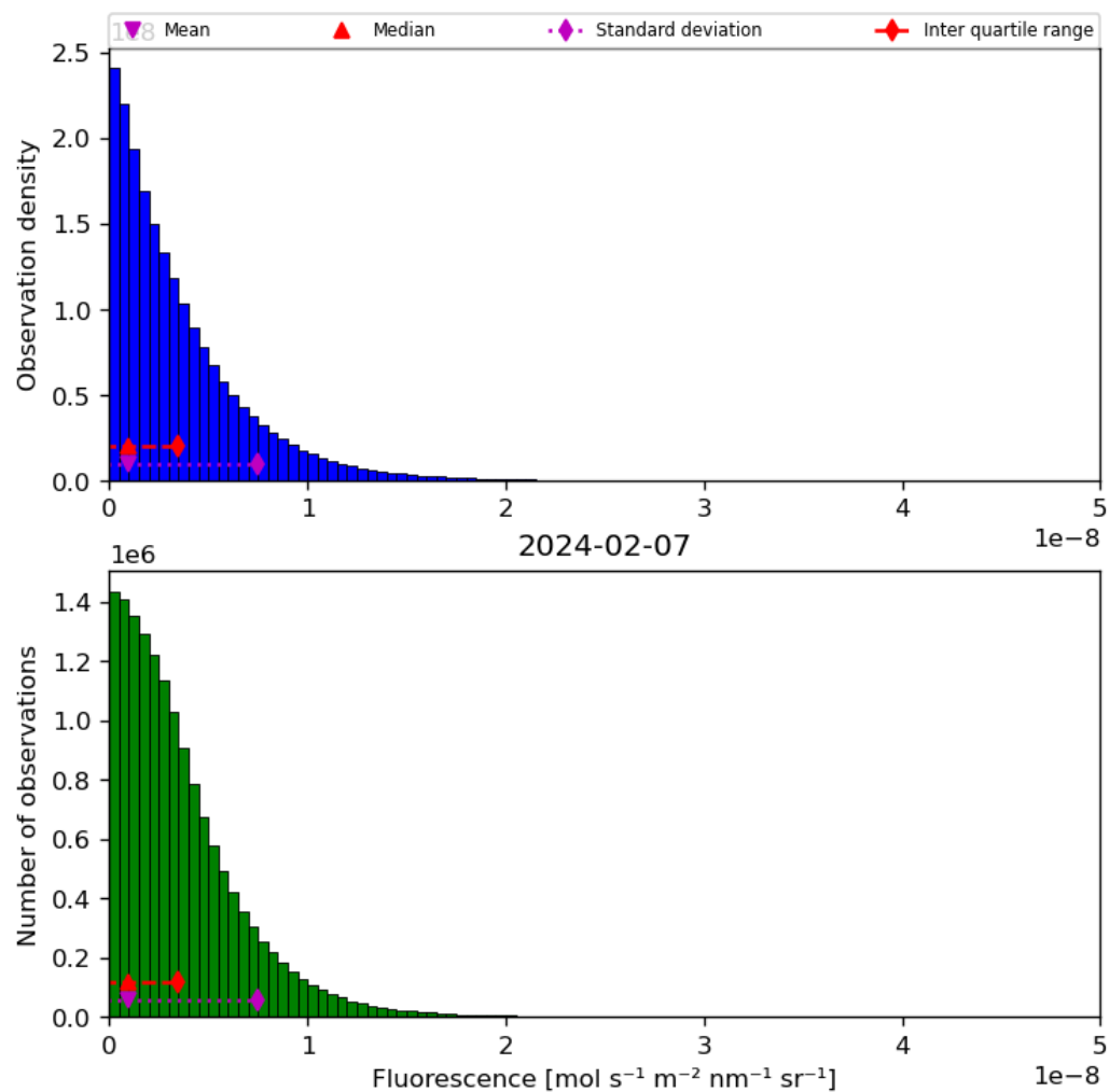
Figure 40: Histogram of “Fluorescence” for 2024-02-06 to 2024-02-08
