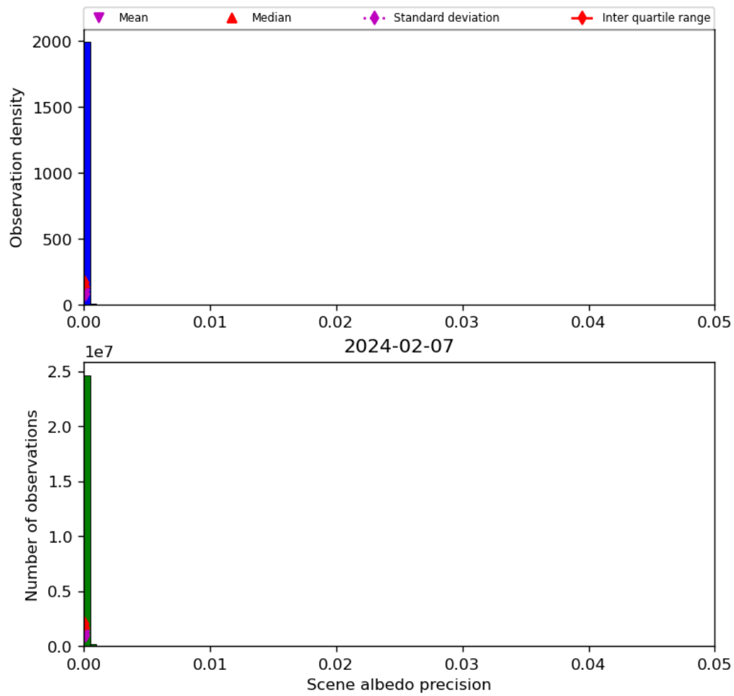
Figure 35: Histogram of “Scene albedo precision” for 2024-02-06 to 2024-02-08
