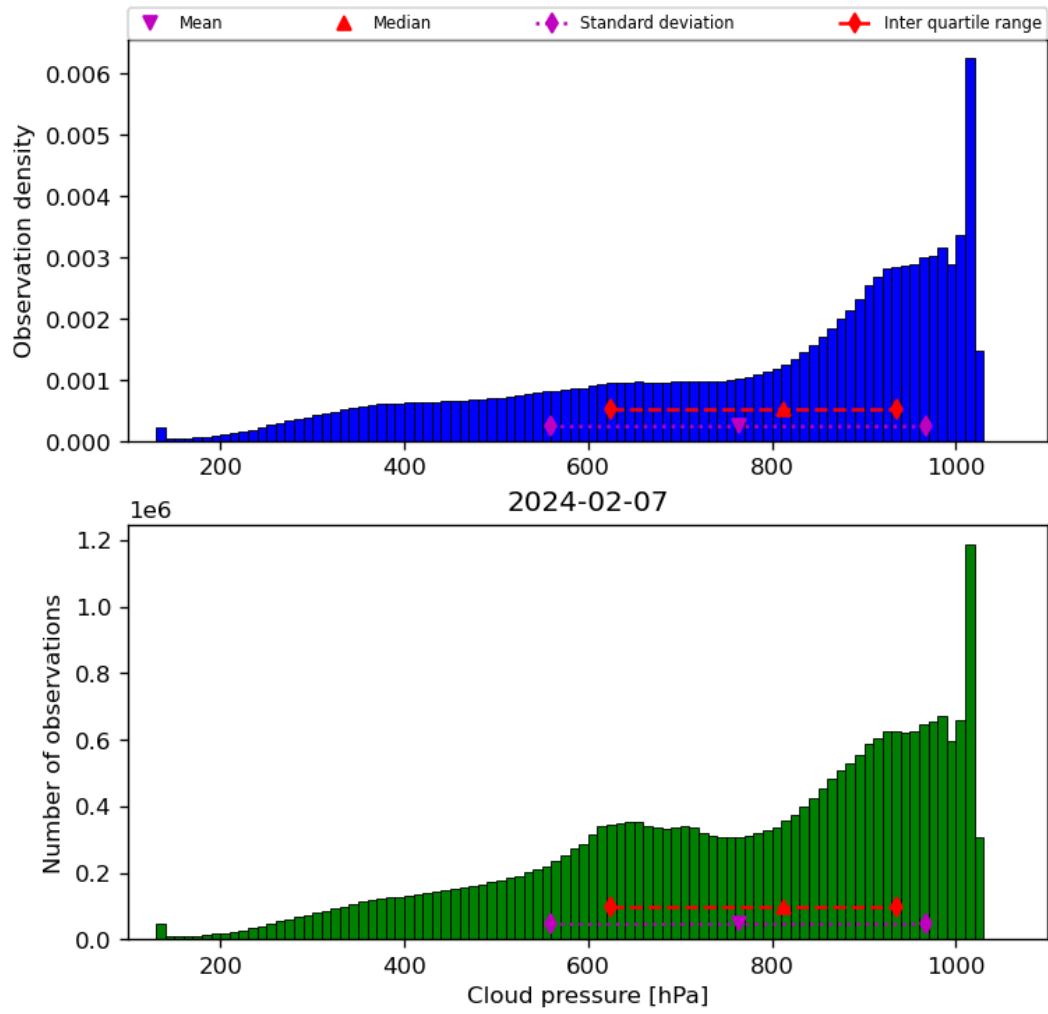
Figure 30: Histogram of “Cloud pressure” for 2024-02-06 to 2024-02-08
