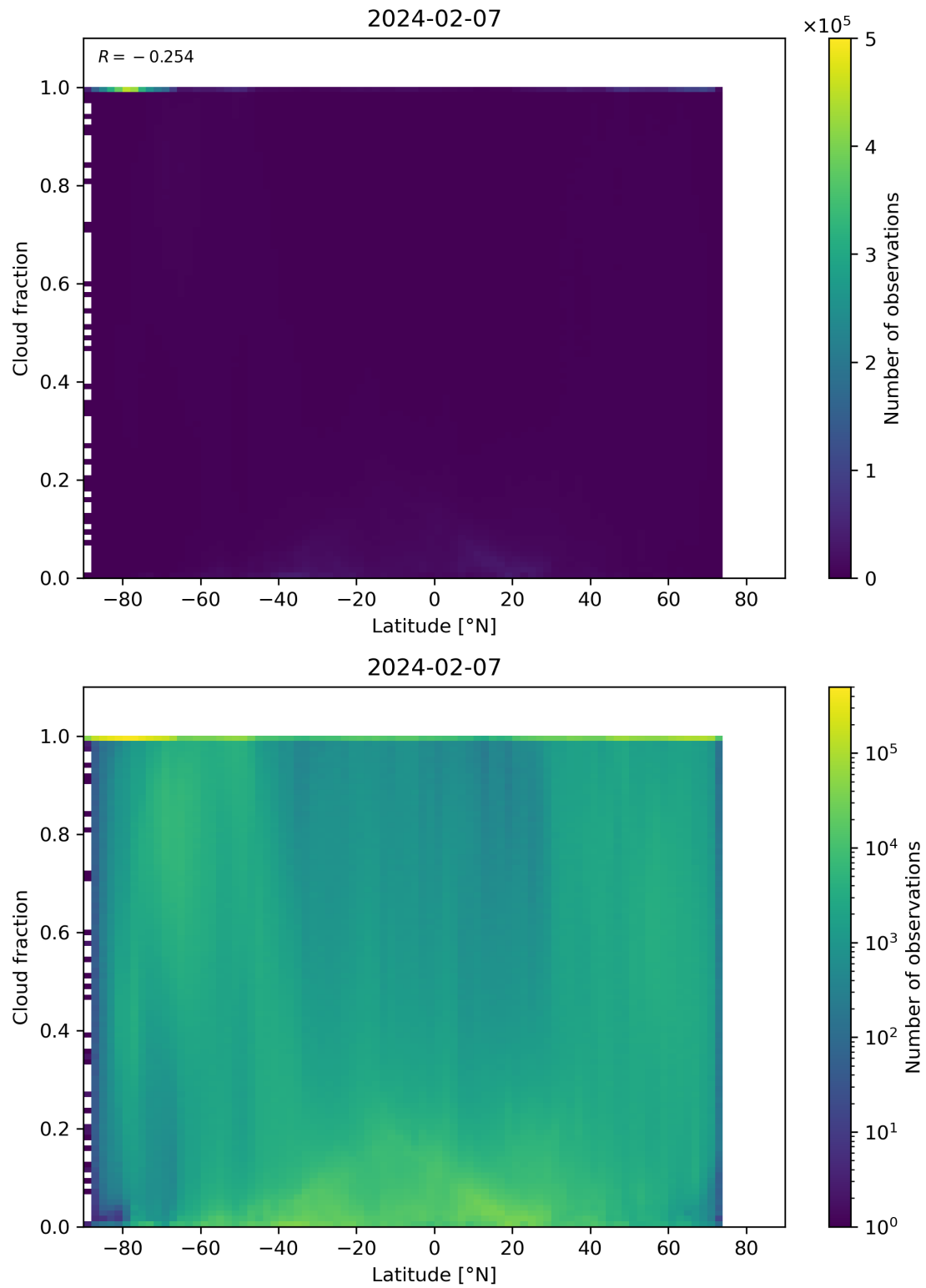
Figure 90: Scatter density plot of “Latitude” against “Cloud fraction” for 2024-02-06 to 2024-02-08.
