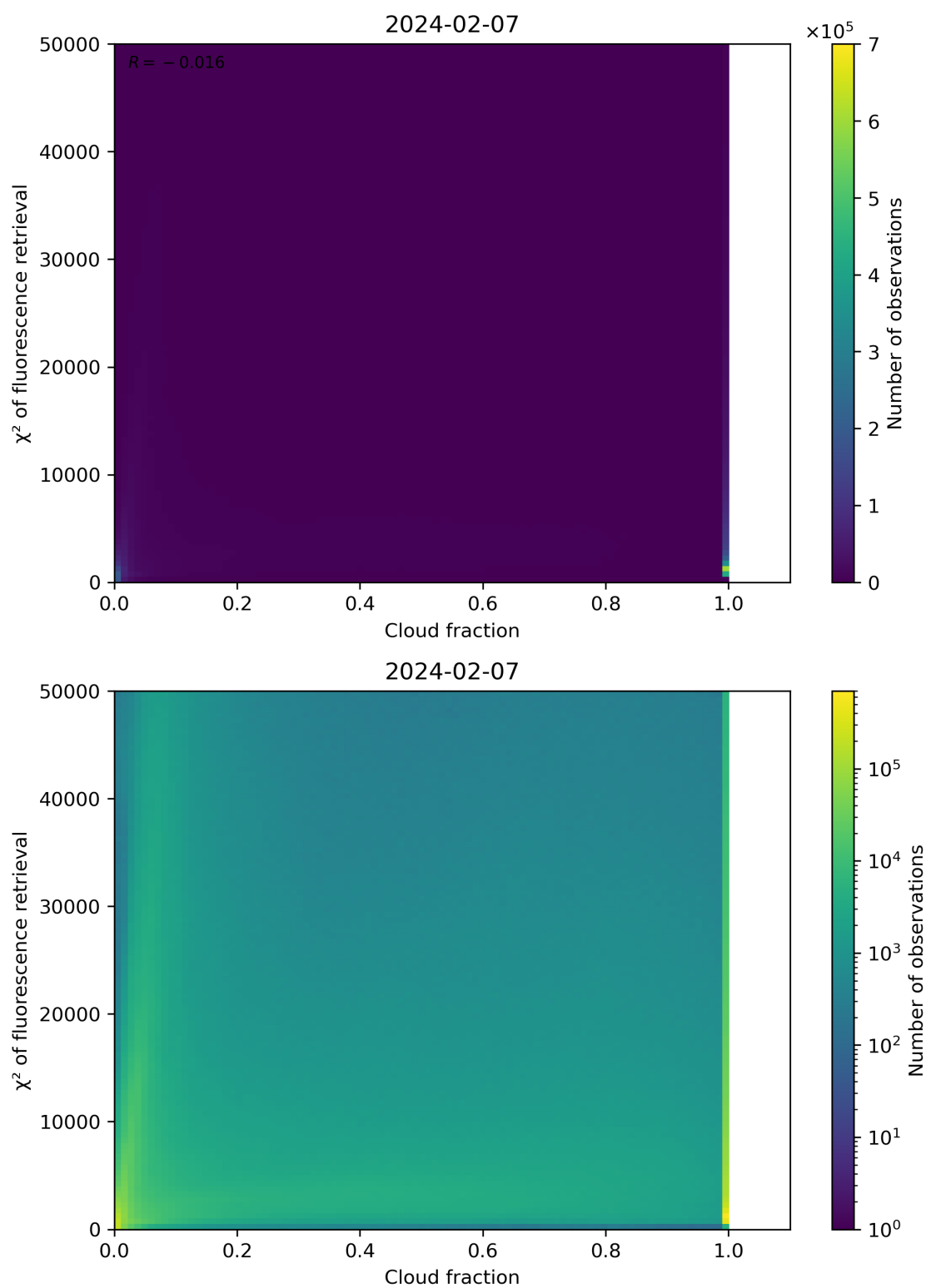
Figure 71: Scatter density plot of “Cloud fraction” against “ \chi^2 of fluorescence retrieval” for 2024-02-06 to 2024-02-08.
