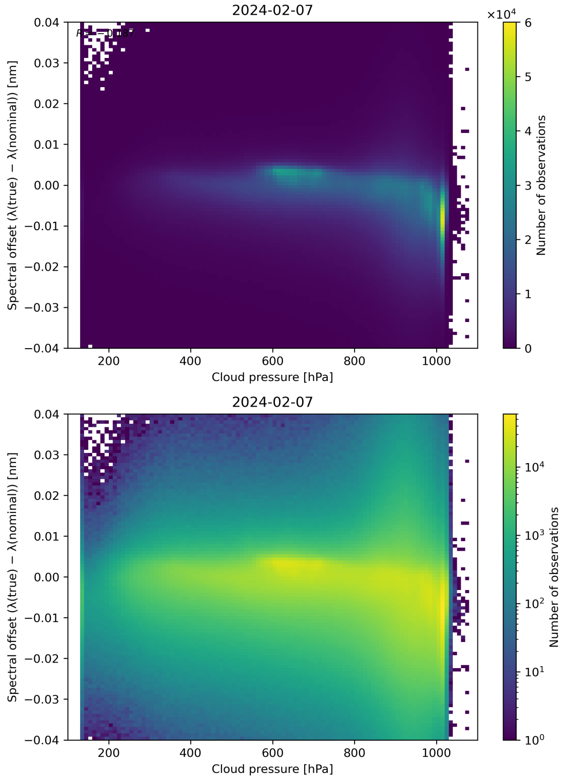
Figure 84: Scatter density plot of “Cloud pressure” against “Spectral offset ( \lambda(\text{true}) - \lambda(\text{nominal}) )” for 2024-02-06 to 2024-02-08.
