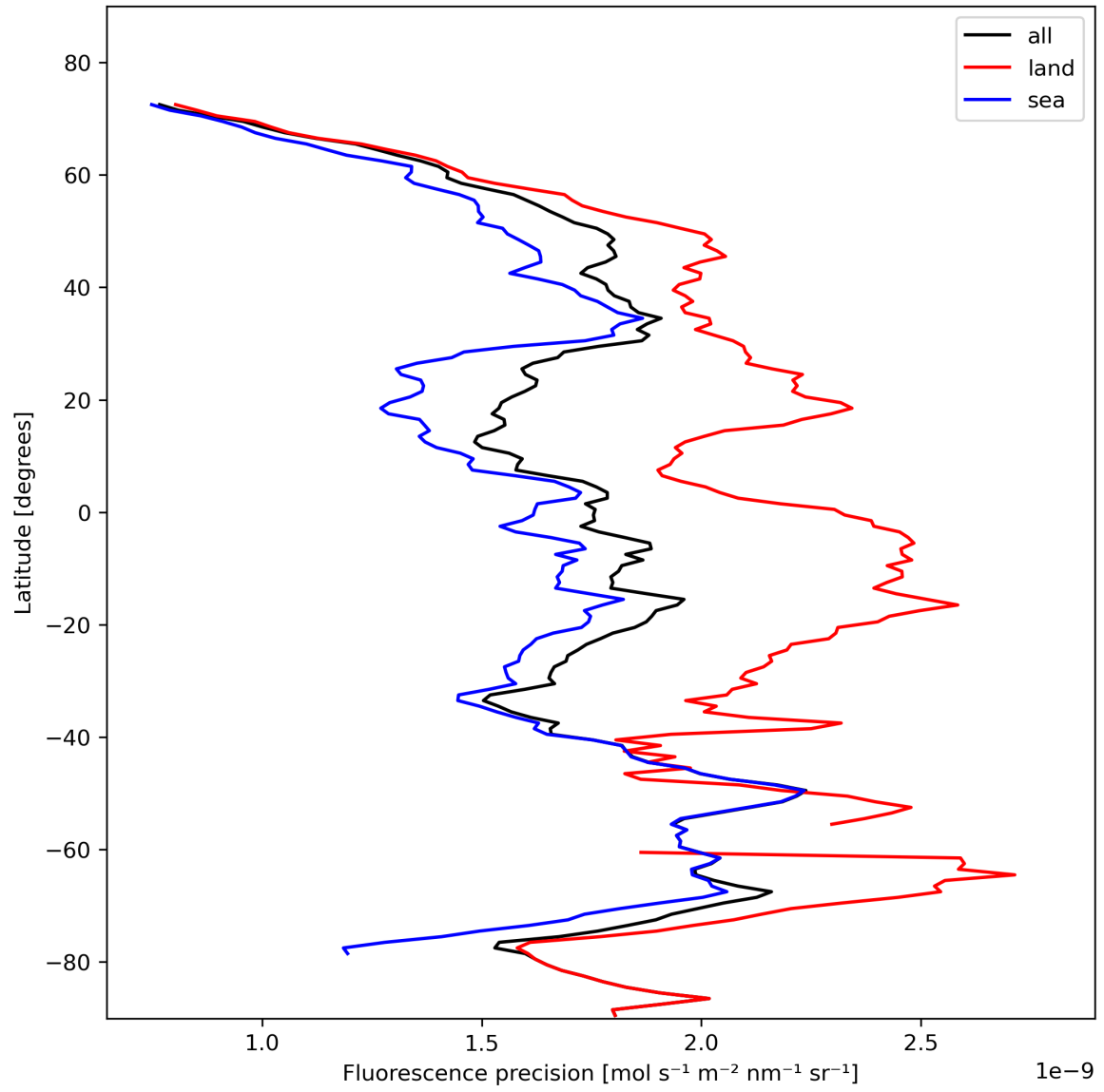
Figure 24: Zonal average of “Fluorescence precision” for 2024-02-06 to 2024-02-08.
