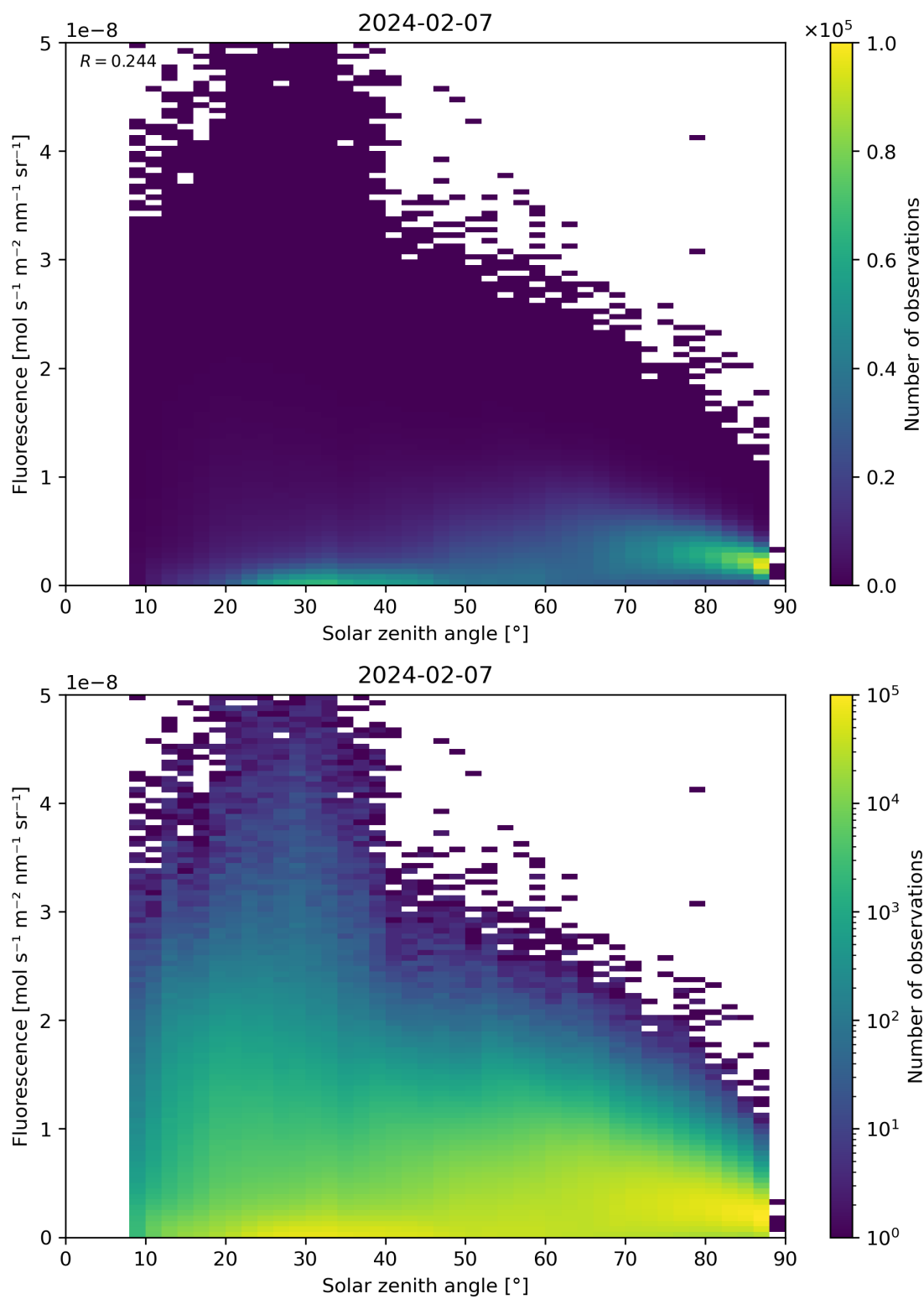
Figure 112: Scatter density plot of “Solar zenith angle” against “Fluorescence” for 2024-02-06 to 2024-02-08.
