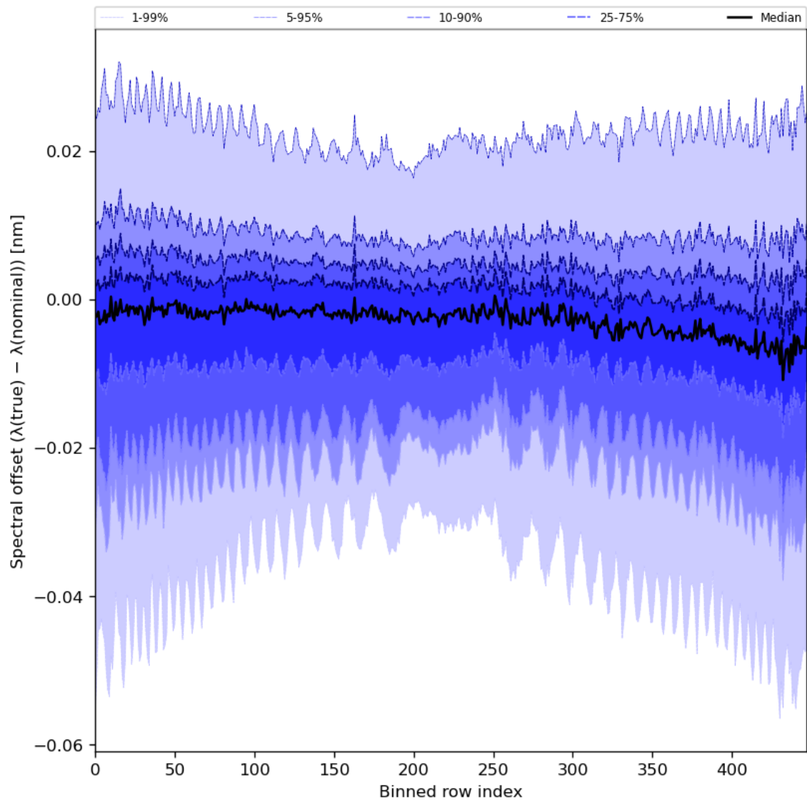
Figure 62: Along track statistics of “Spectral offset ( \lambda(\text{true}) - \lambda(\text{nominal}) )” for 2024-02-06 to 2024-02-08
