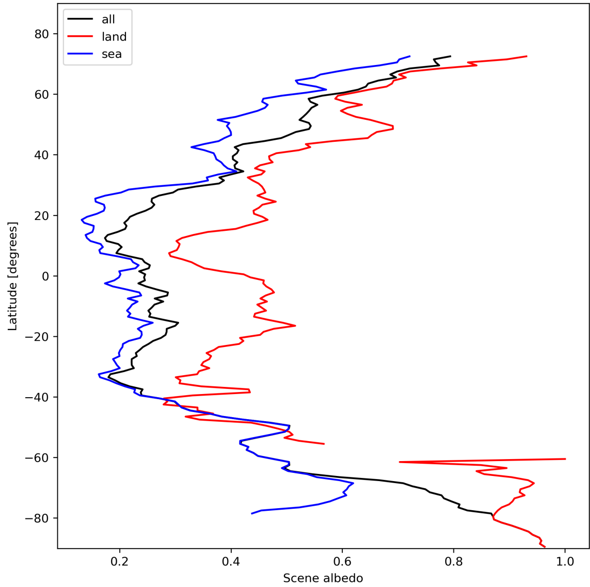
Figure 17: Zonal average of “Scene albedo” for 2024-02-06 to 2024-02-08.
