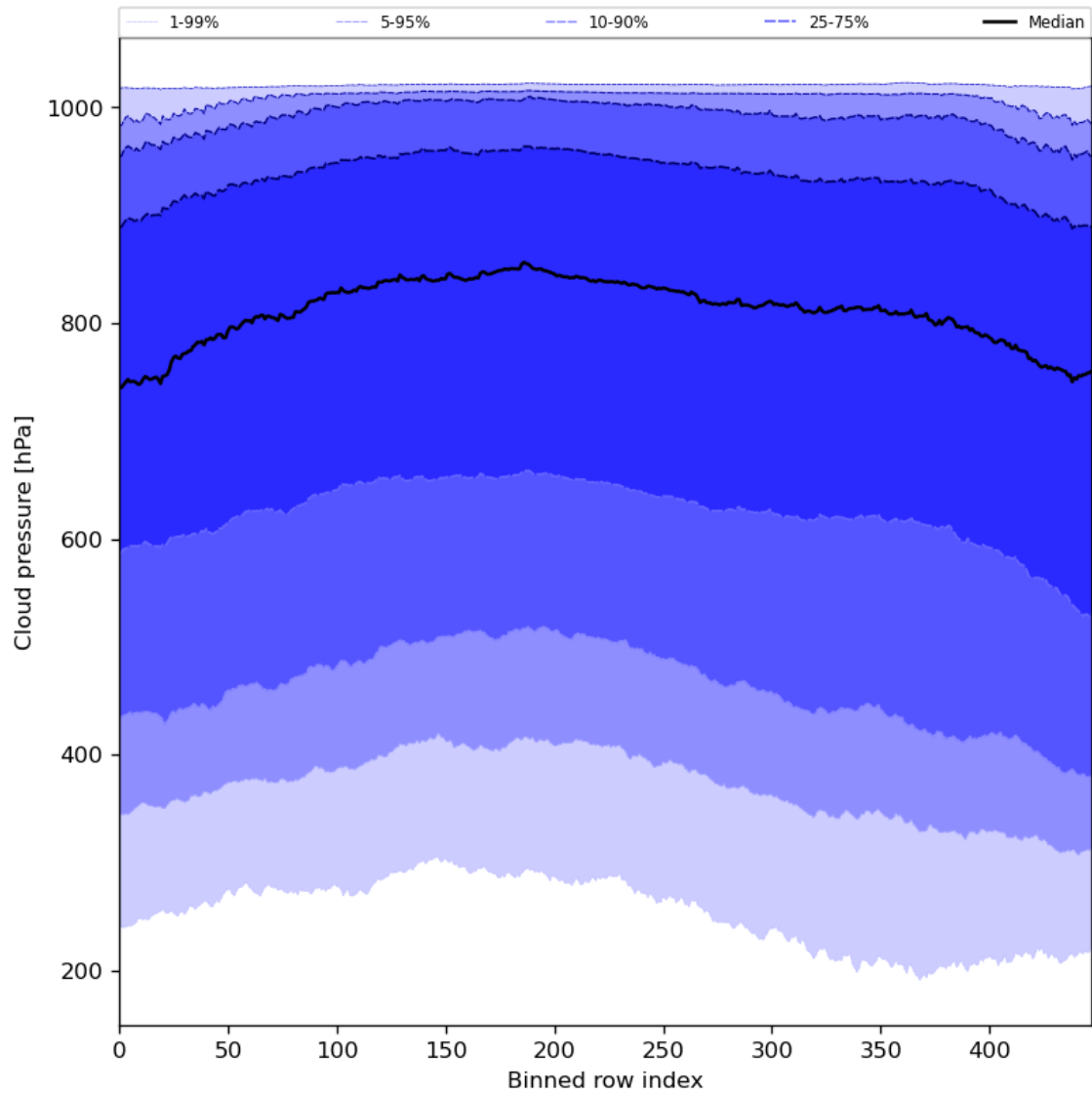
Figure 47: Along track statistics of “Cloud pressure” for 2024-02-06 to 2024-02-08
