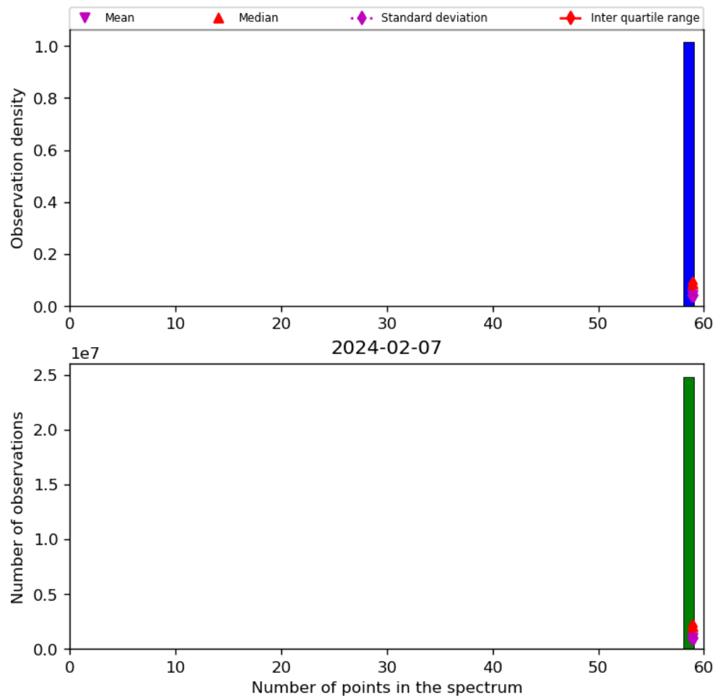
Figure 44: Histogram of “Number of points in the spectrum” for 2024-02-06 to 2024-02-08
