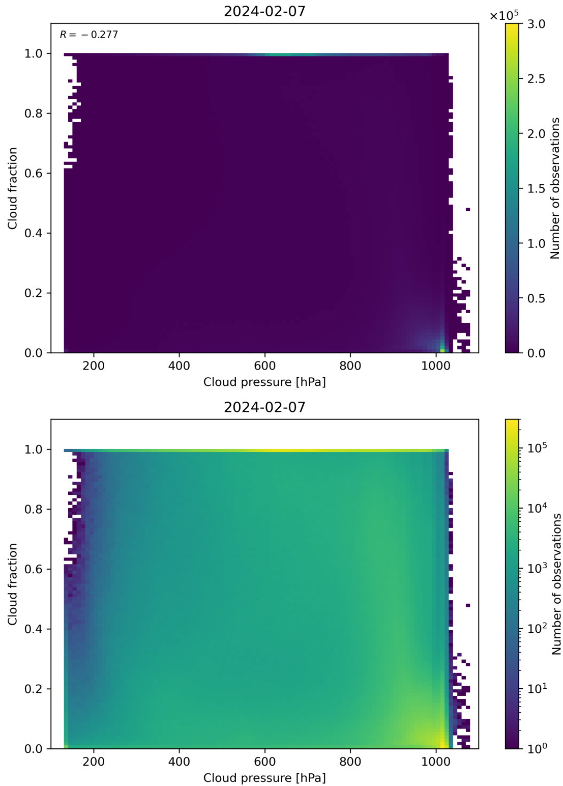
Figure 79: Scatter density plot of “Cloud pressure” against “Cloud fraction” for 2024-02-06 to 2024-02-08.
