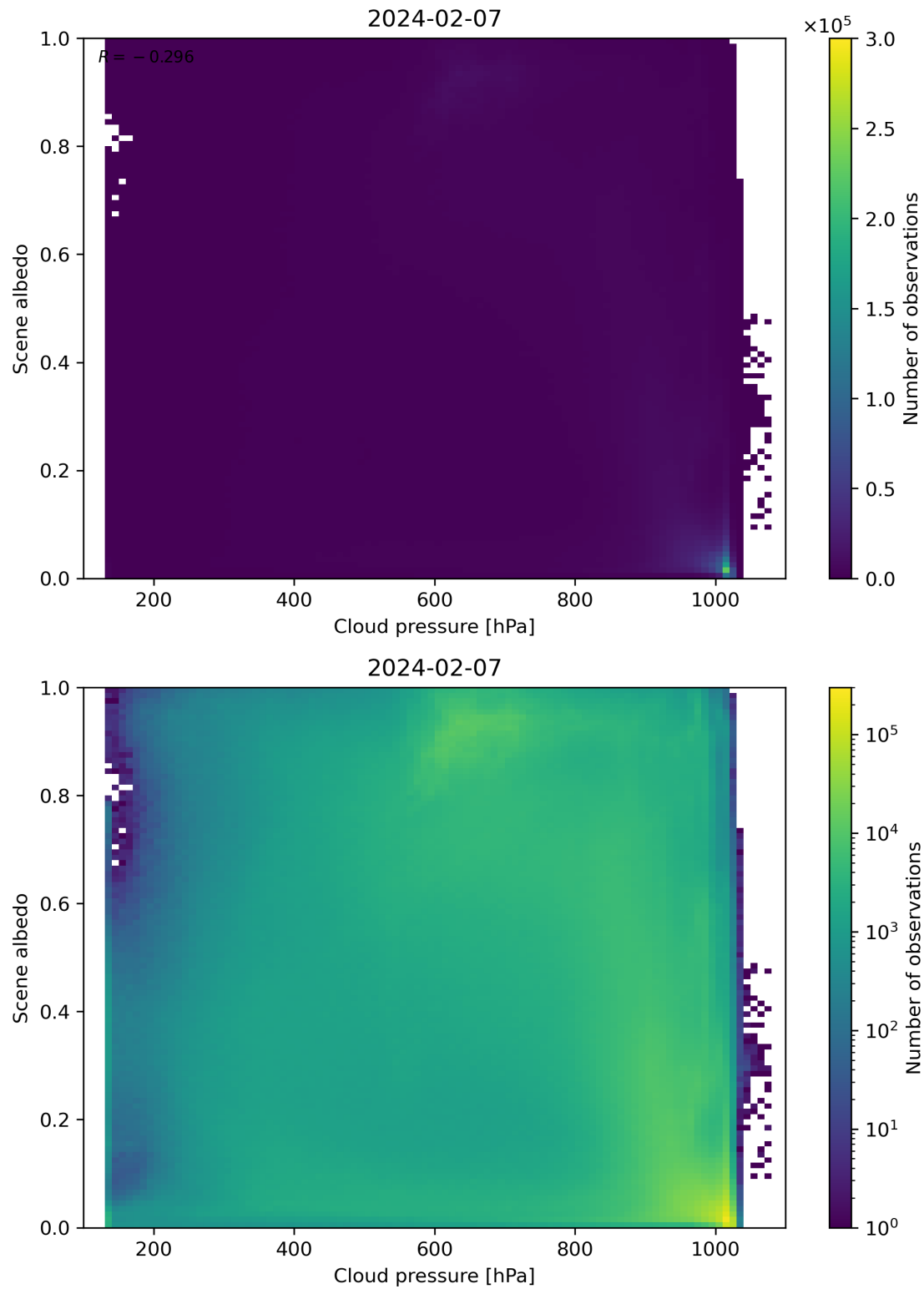
Figure 83: Scatter density plot of “Cloud pressure” against “Scene albedo” for 2024-02-06 to 2024-02-08.
