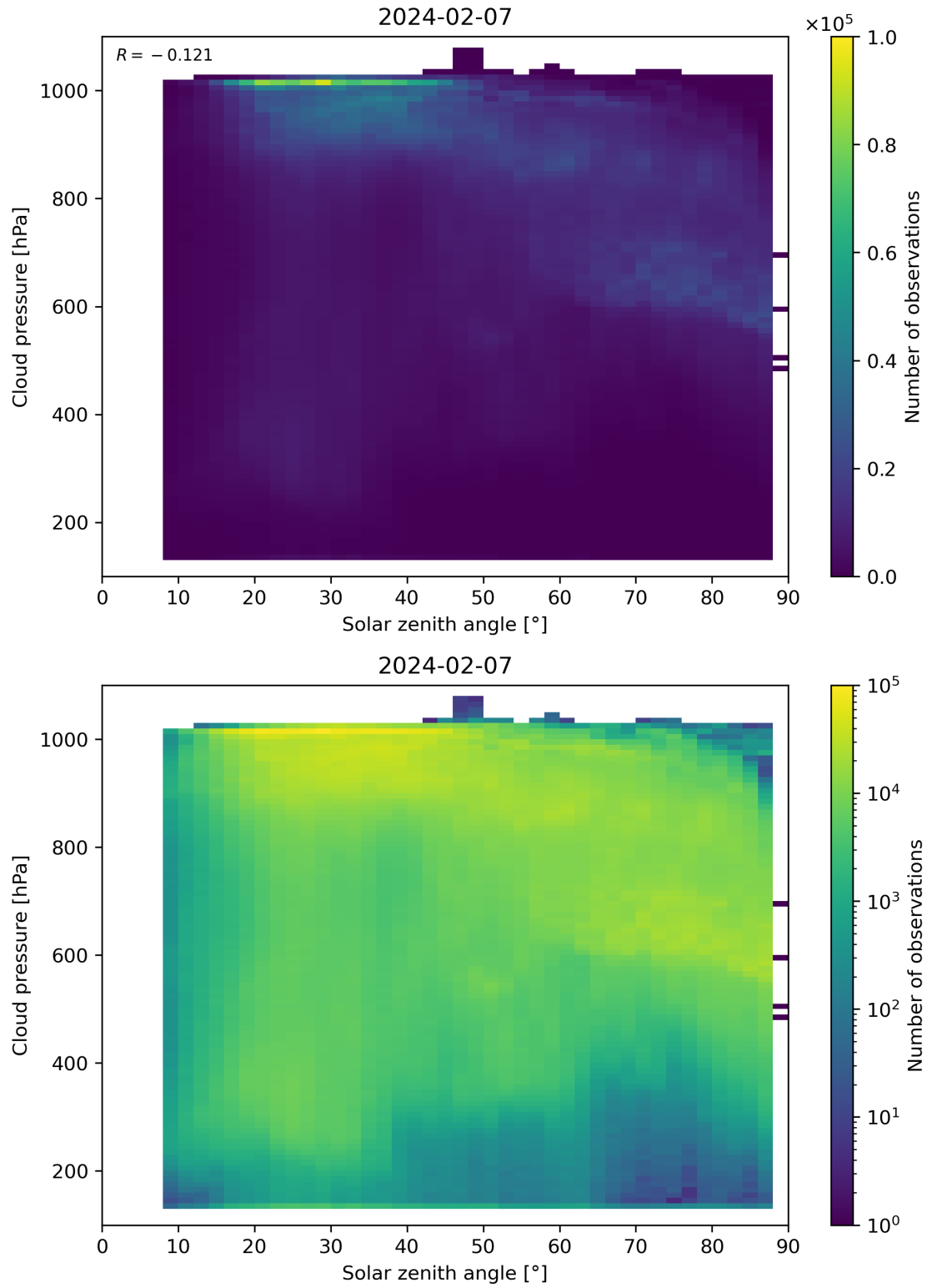
Figure 111: Scatter density plot of “Solar zenith angle” against “Cloud pressure” for 2024-02-06 to 2024-02-08.
