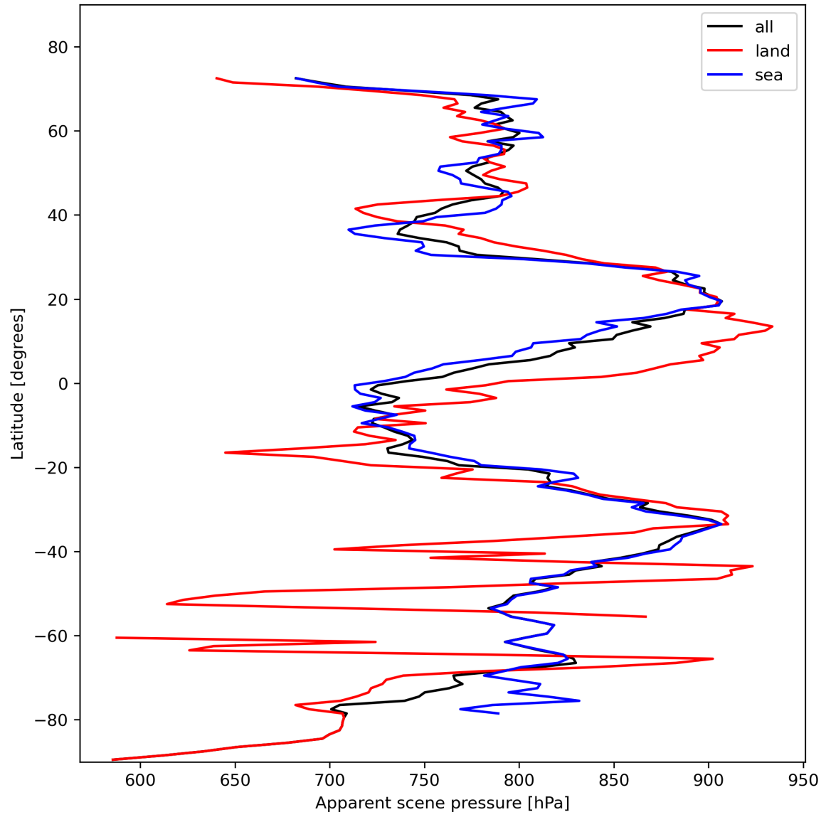
Figure 19: Zonal average of “Apparent scene pressure” for 2024-02-06 to 2024-02-08.
