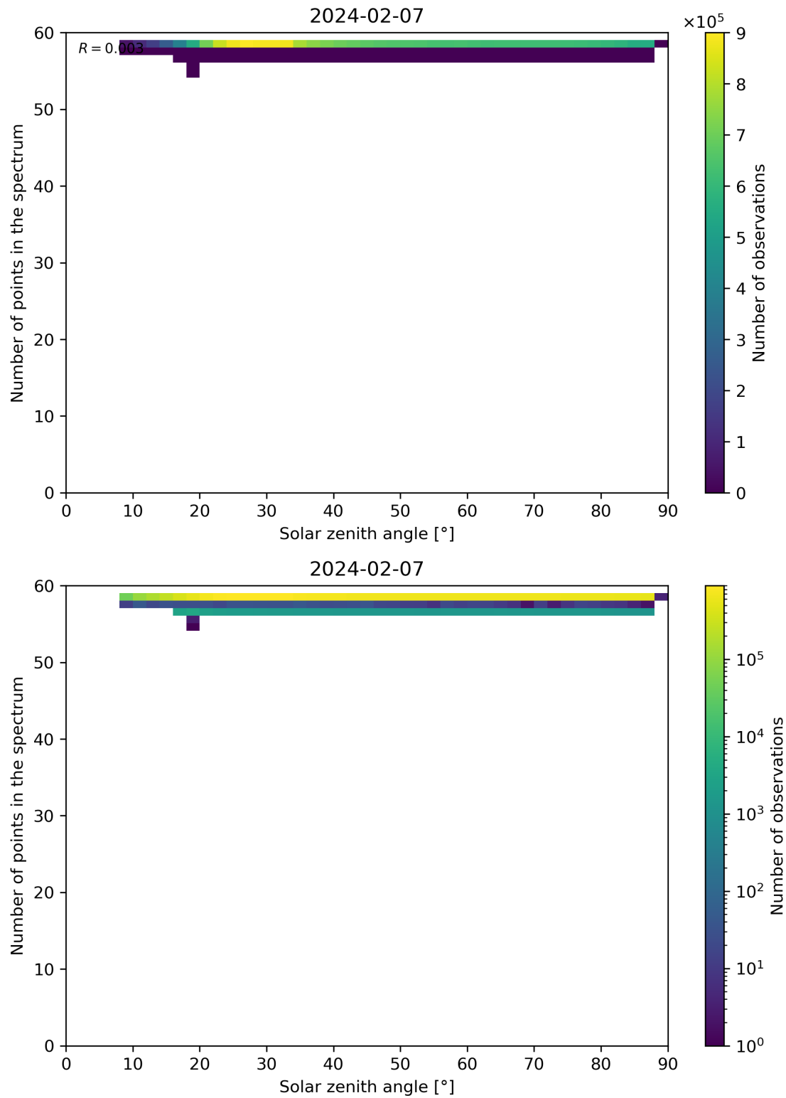
Figure 115: Scatter density plot of “Solar zenith angle” against “Number of points in the spectrum” for 2024-02-06 to 2024-02-08.
