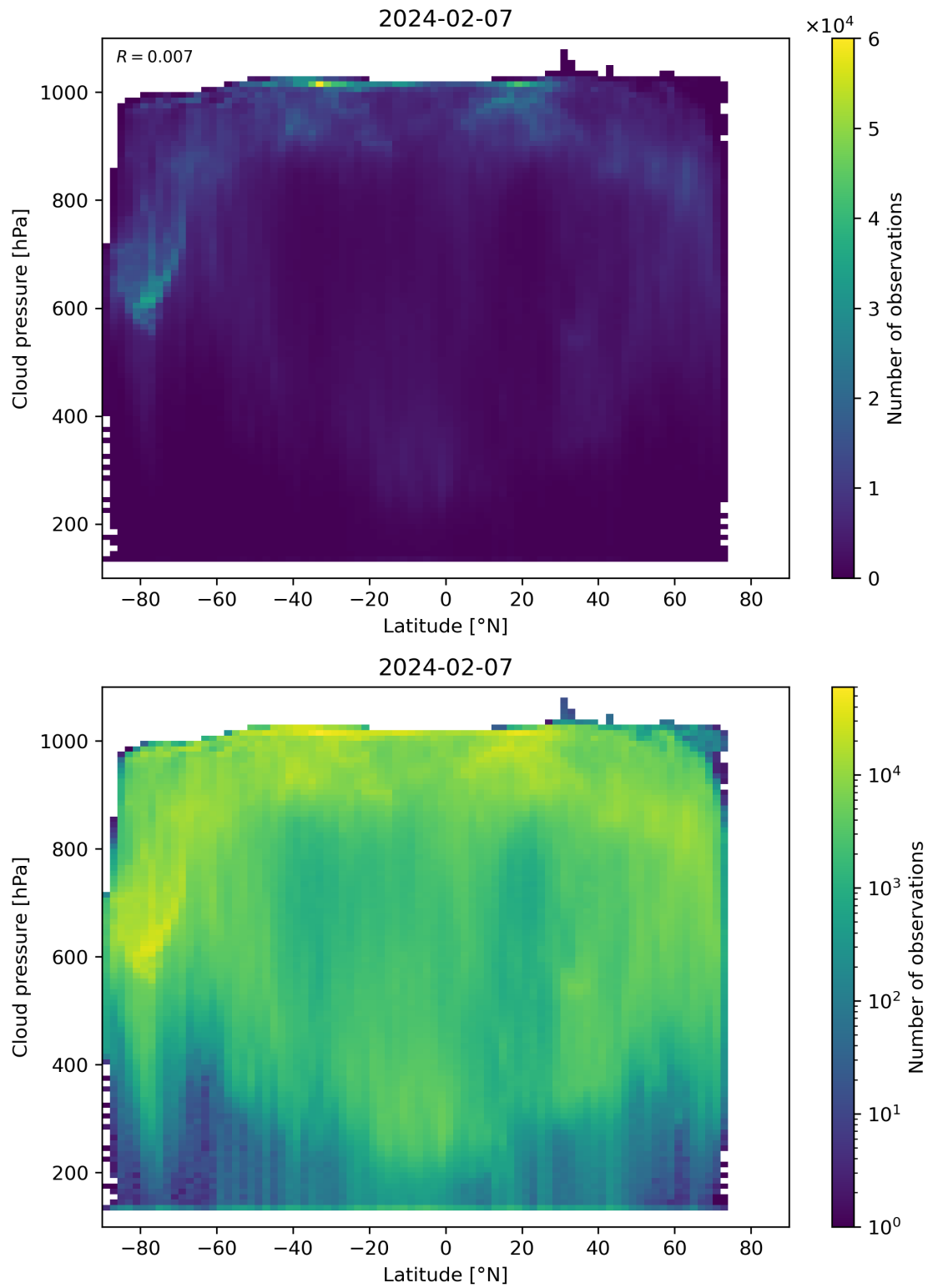
Figure 91: Scatter density plot of “Latitude” against “Cloud pressure” for 2024-02-06 to 2024-02-08.
