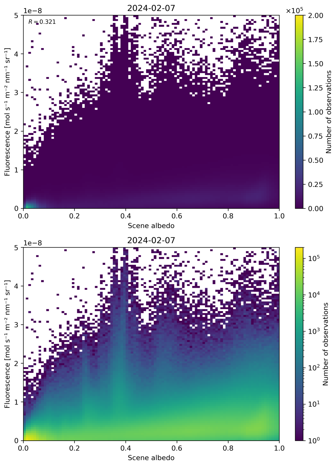
Figure 104: Scatter density plot of “Scene albedo” against “Fluorescence” for 2024-02-06 to 2024-02-08.
