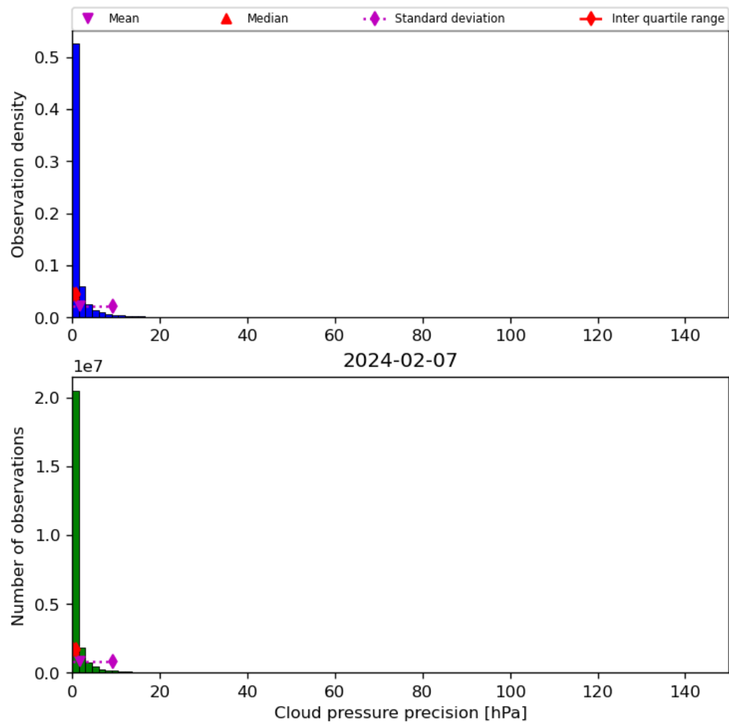
Figure 31: Histogram of “Cloud pressure precision” for 2024-02-06 to 2024-02-08
