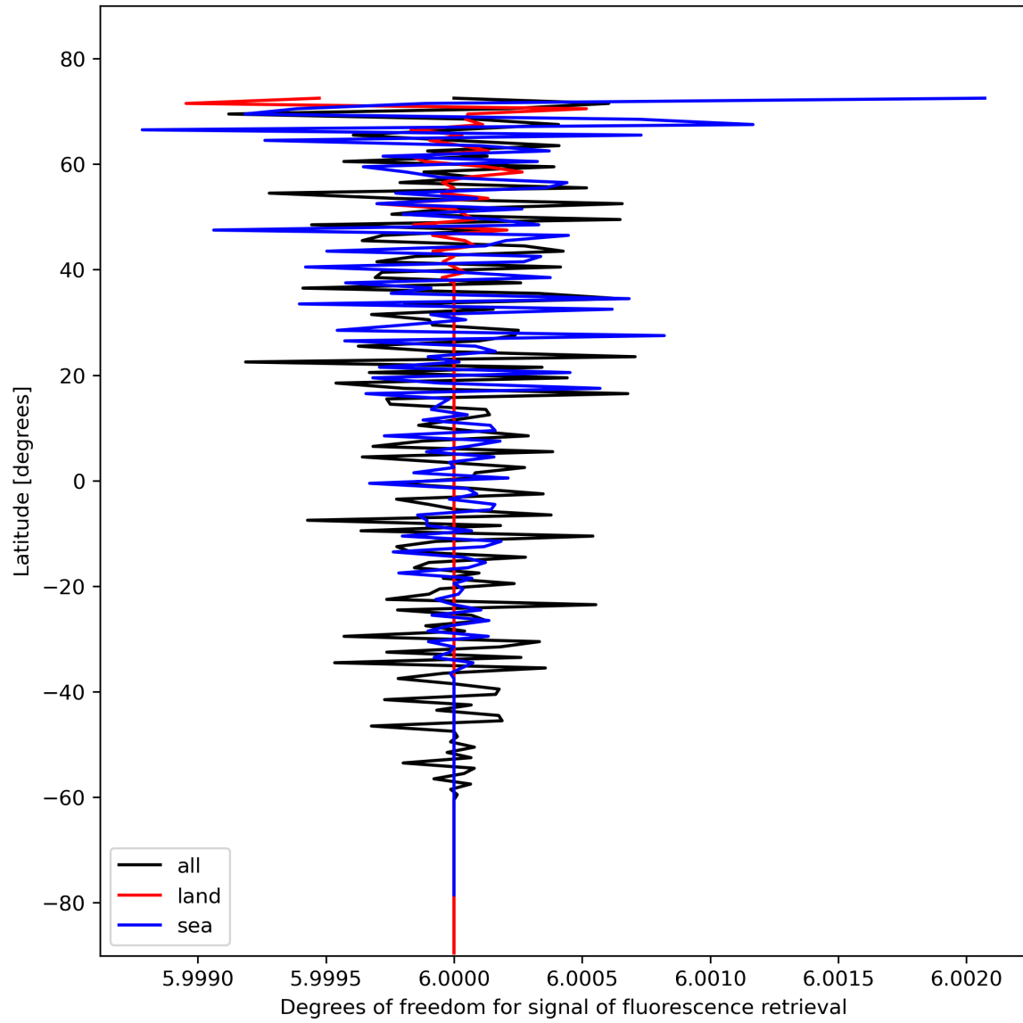
Figure 26: Zonal average of “Degrees of freedom for signal of fluorescence retrieval” for 2024-02-06 to 2024-02-08.
