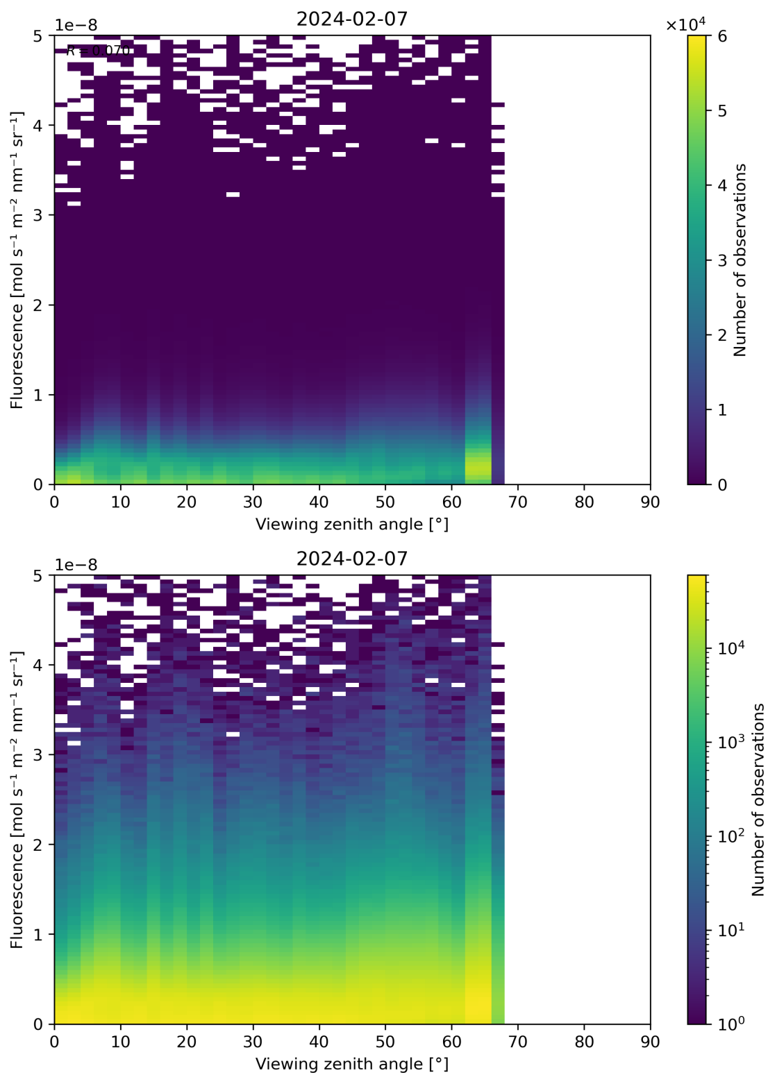
Figure 122: Scatter density plot of “Viewing zenith angle” against “Fluorescence” for 2024-02-06 to 2024-02-08.
