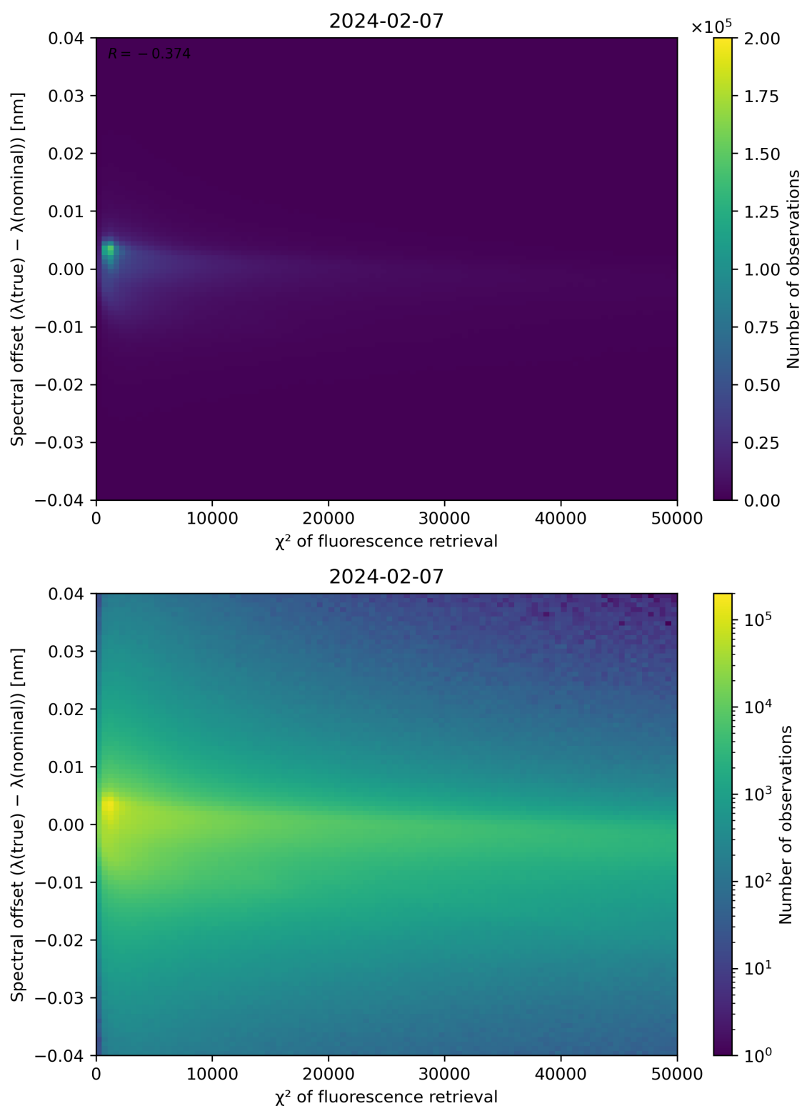
Figure 69: Scatter density plot of " \chi^2 of fluorescence retrieval" against "Spectral offset ( \lambda(\text{true}) - \lambda(\text{nominal}) )" for 2024-02-06 to 2024-02-08.
