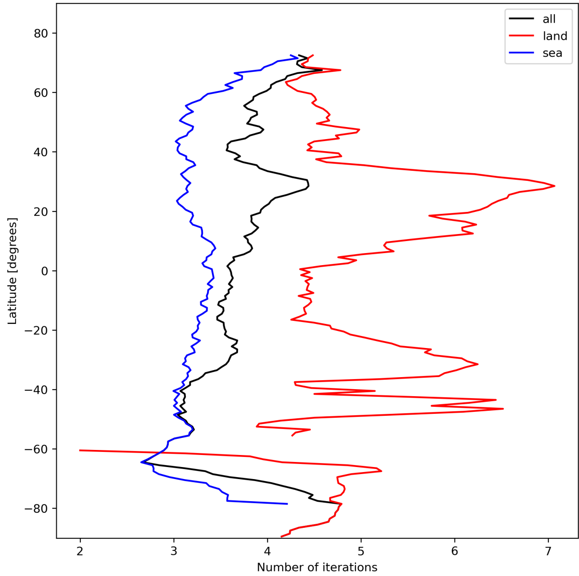
Figure 22: Zonal average of “Number of iterations” for 2024-02-06 to 2024-02-08.
