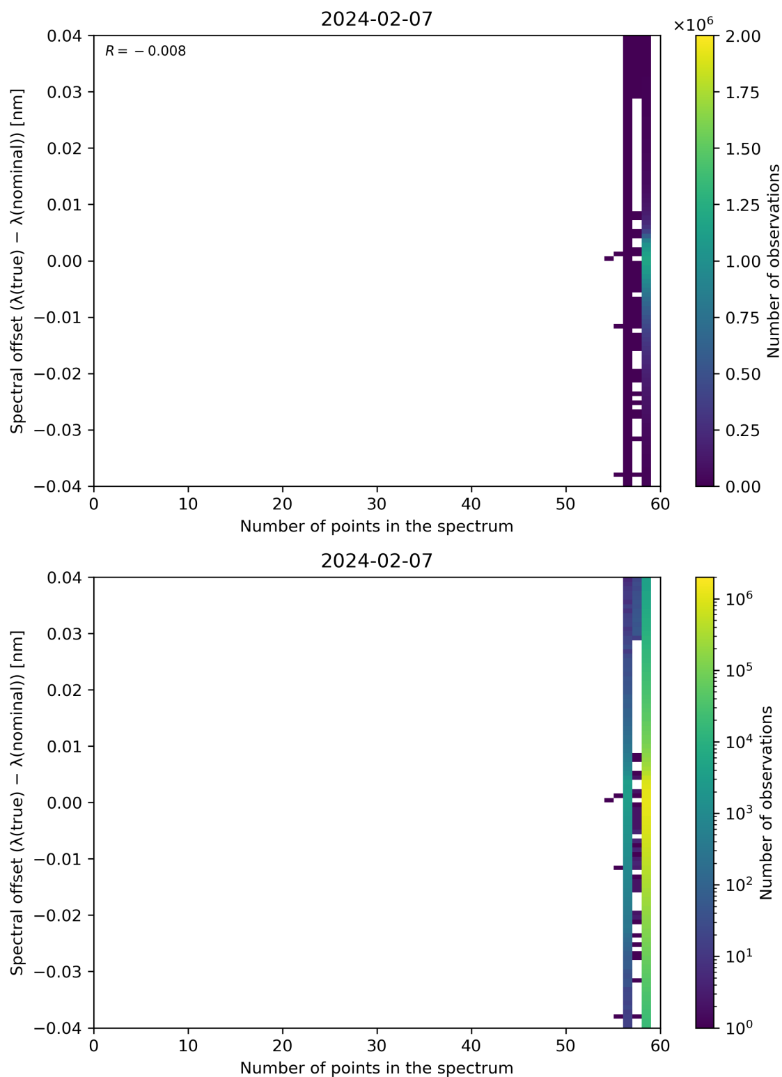
Figure 101: Scatter density plot of “Number of points in the spectrum” against “Spectral offset ( \lambda(\text{true}) - \lambda(\text{nominal}) )” for 2024-02-06 to 2024-02-08.
