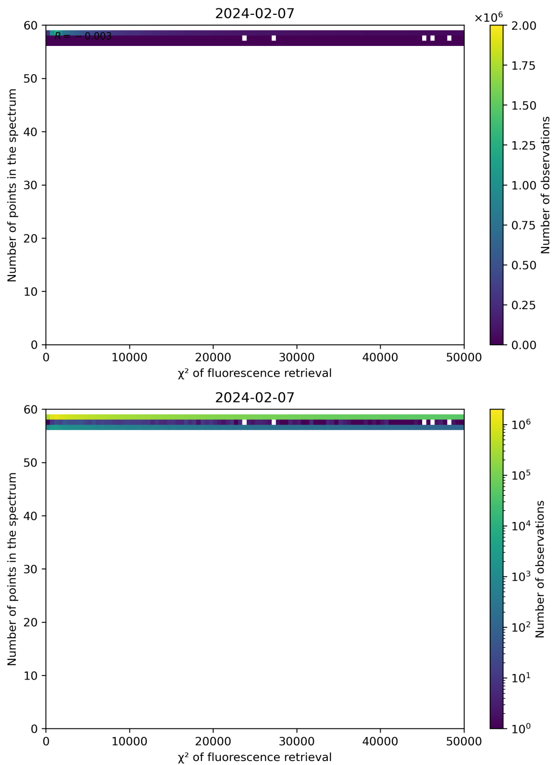
Figure 68: Scatter density plot of " \chi^2 of fluorescence retrieval" against "Number of points in the spectrum" for 2024-02-06 to 2024-02-08.
