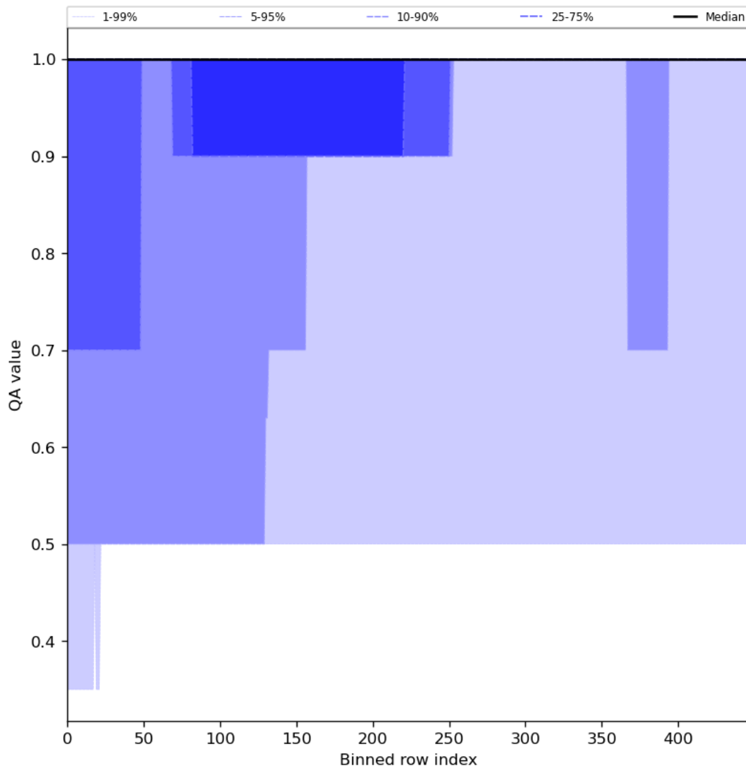
Figure 46: Along track statistics of “QA value” for 2024-02-06 to 2024-02-08
