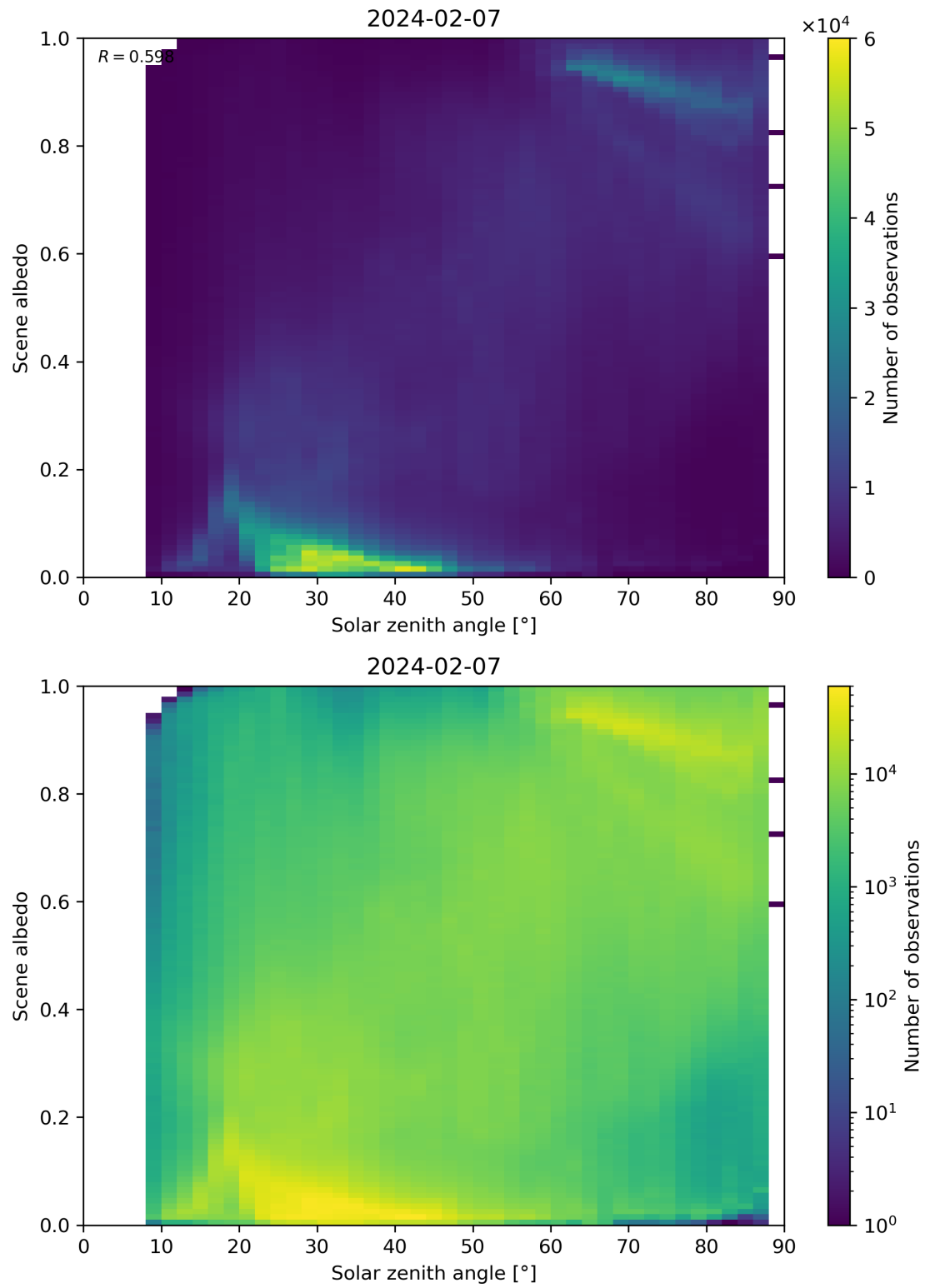
Figure 116: Scatter density plot of “Solar zenith angle” against “Scene albedo” for 2024-02-06 to 2024-02-08.
