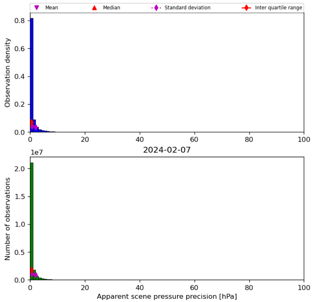
Figure 37: Histogram of “Apparent scene pressure precision” for 2024-02-06 to 2024-02-08
