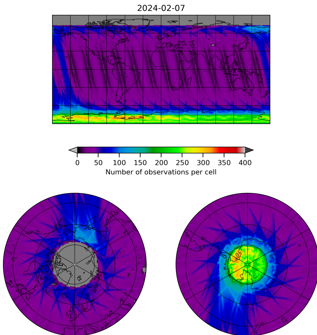
Figure 11: Map of the number of observations for 2024-02-06 to 2024-02-08
