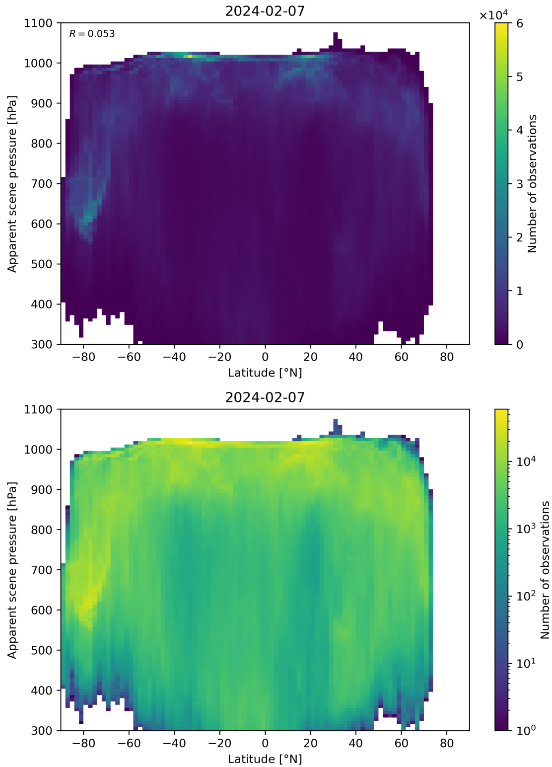
Figure 88: Scatter density plot of “Latitude” against “Apparent scene pressure” for 2024-02-06 to 2024-02-08.
