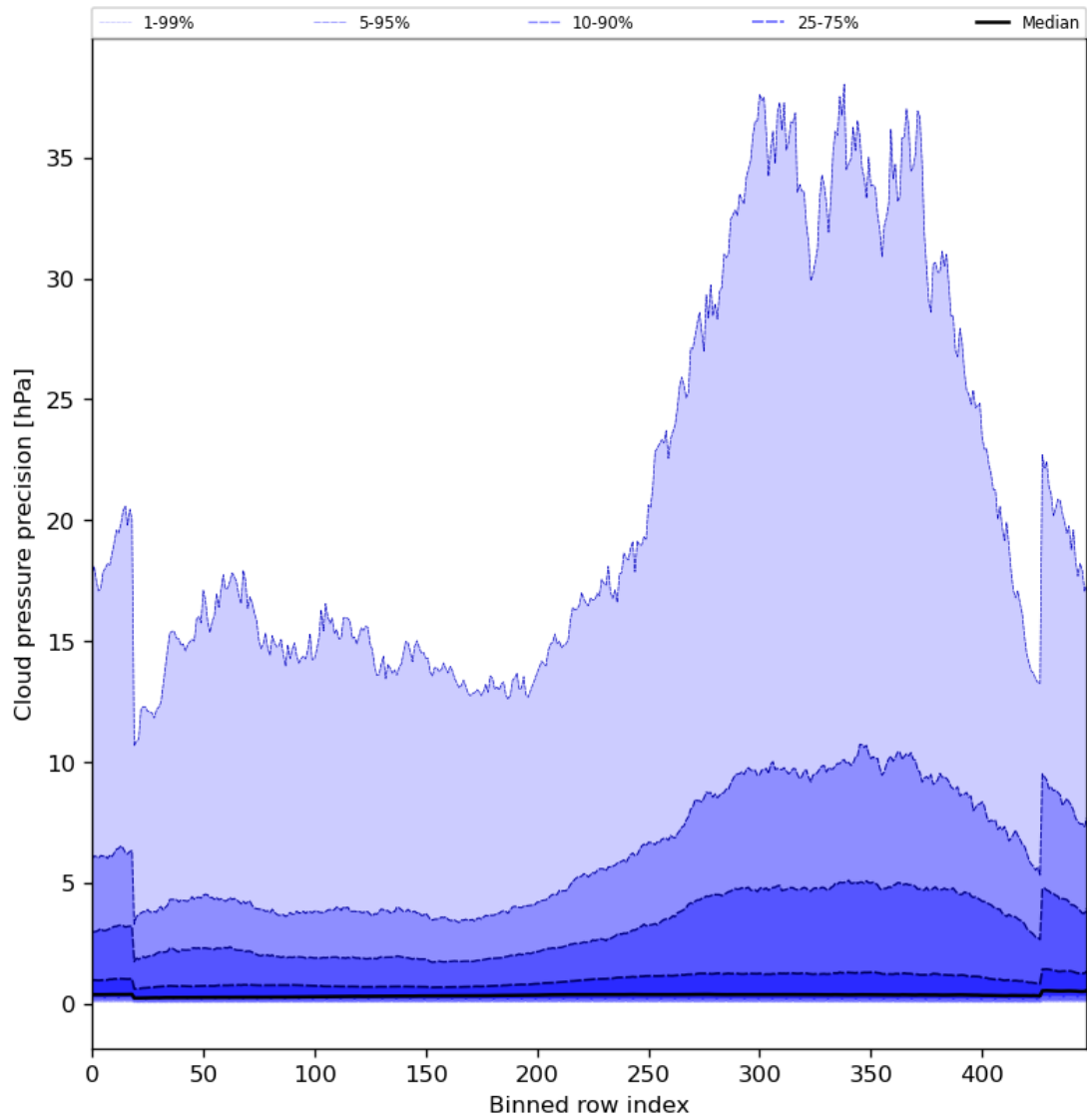
Figure 48: Along track statistics of “Cloud pressure precision” for 2024-02-06 to 2024-02-08
