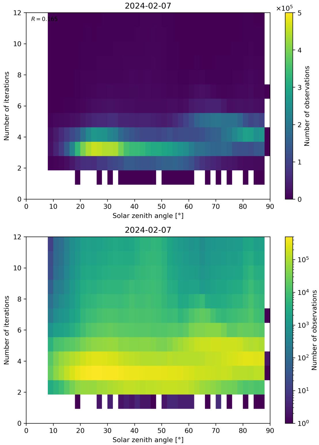
Figure 114: Scatter density plot of “Solar zenith angle” against “Number of iterations” for 2024-02-06 to 2024-02-08.
