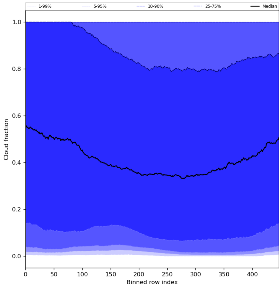
Figure 49: Along track statistics of “Cloud fraction” for 2024-02-06 to 2024-02-08
