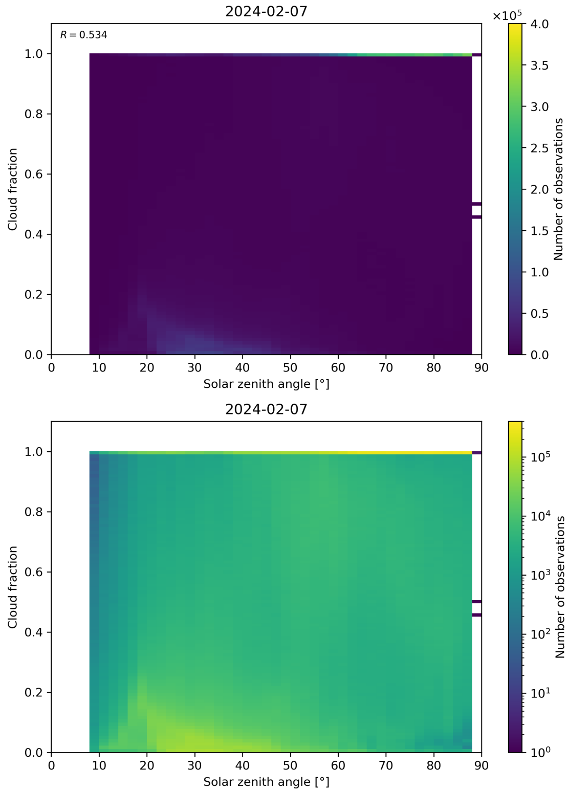
Figure 110: Scatter density plot of “Solar zenith angle” against “Cloud fraction” for 2024-02-06 to 2024-02-08.
