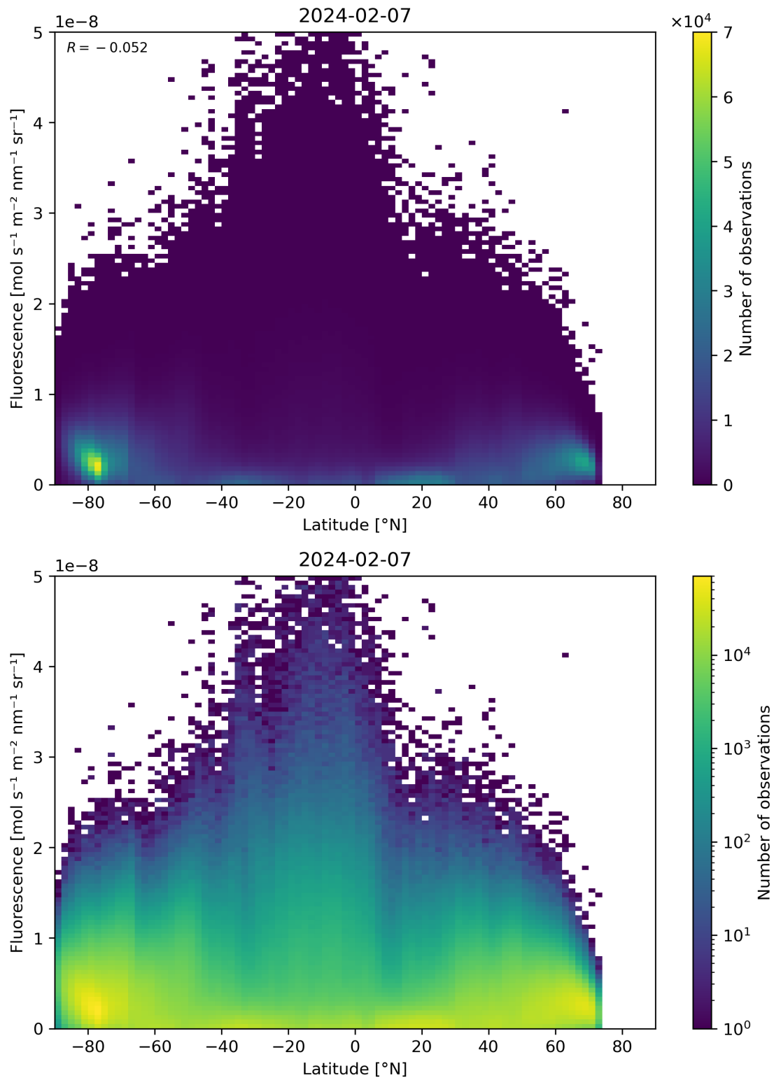
Figure 92: Scatter density plot of “Latitude” against “Fluorescence” for 2024-02-06 to 2024-02-08.
