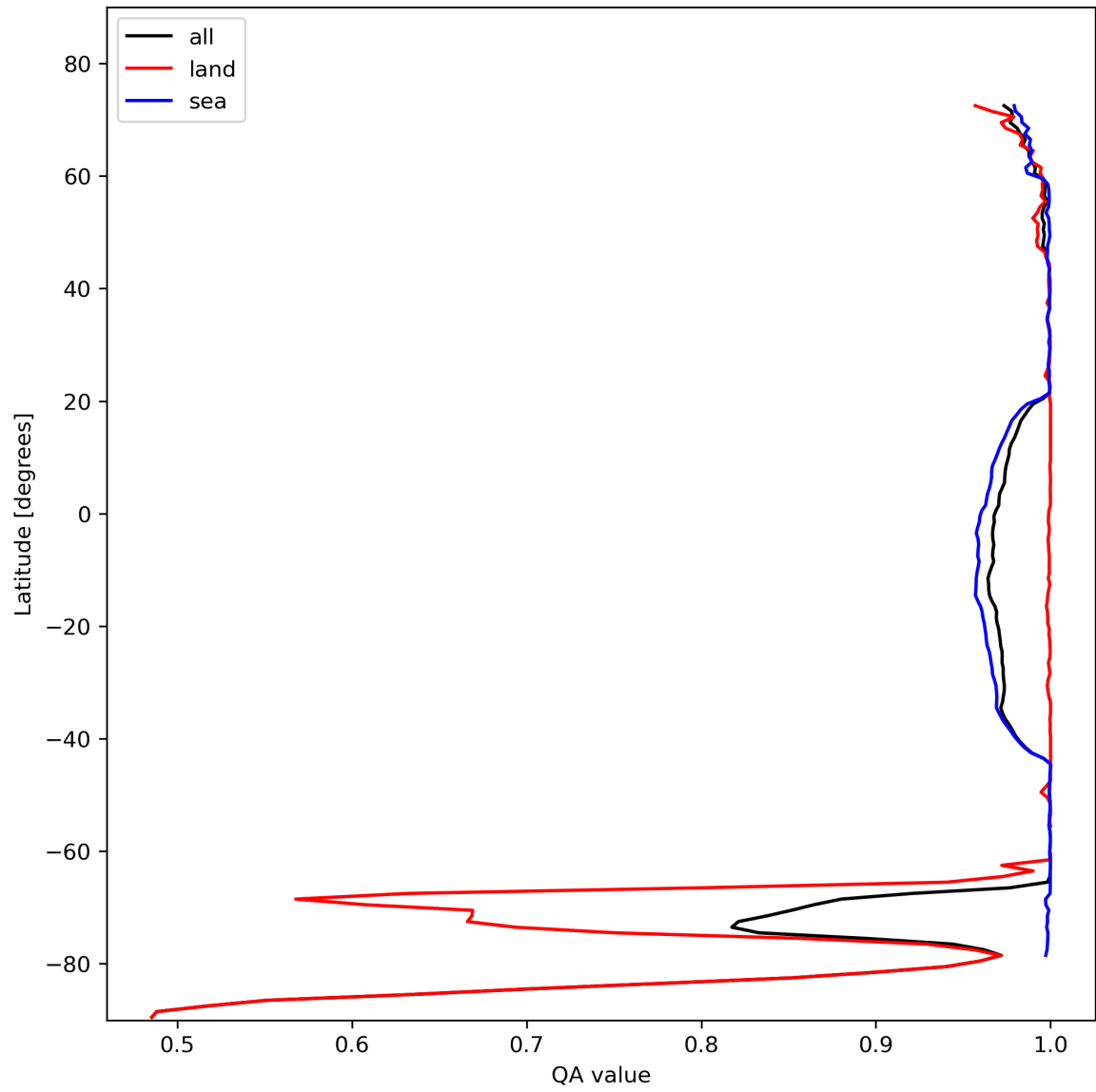
Figure 12: Zonal average of “QA value” for 2024-02-06 to 2024-02-08.
