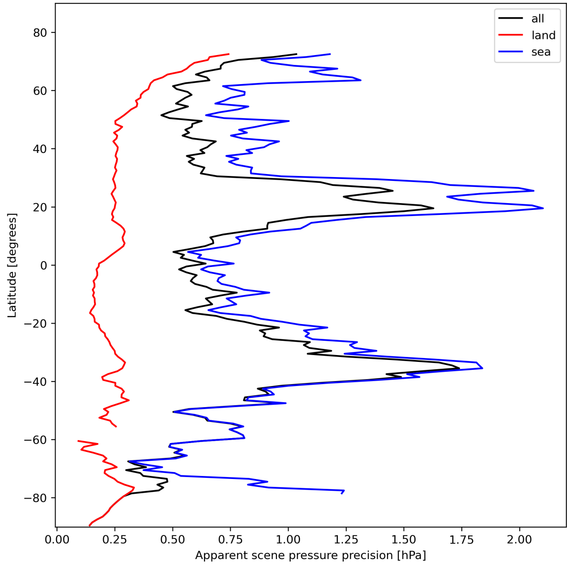
Figure 20: Zonal average of “Apparent scene pressure precision” for 2024-02-06 to 2024-02-08.
