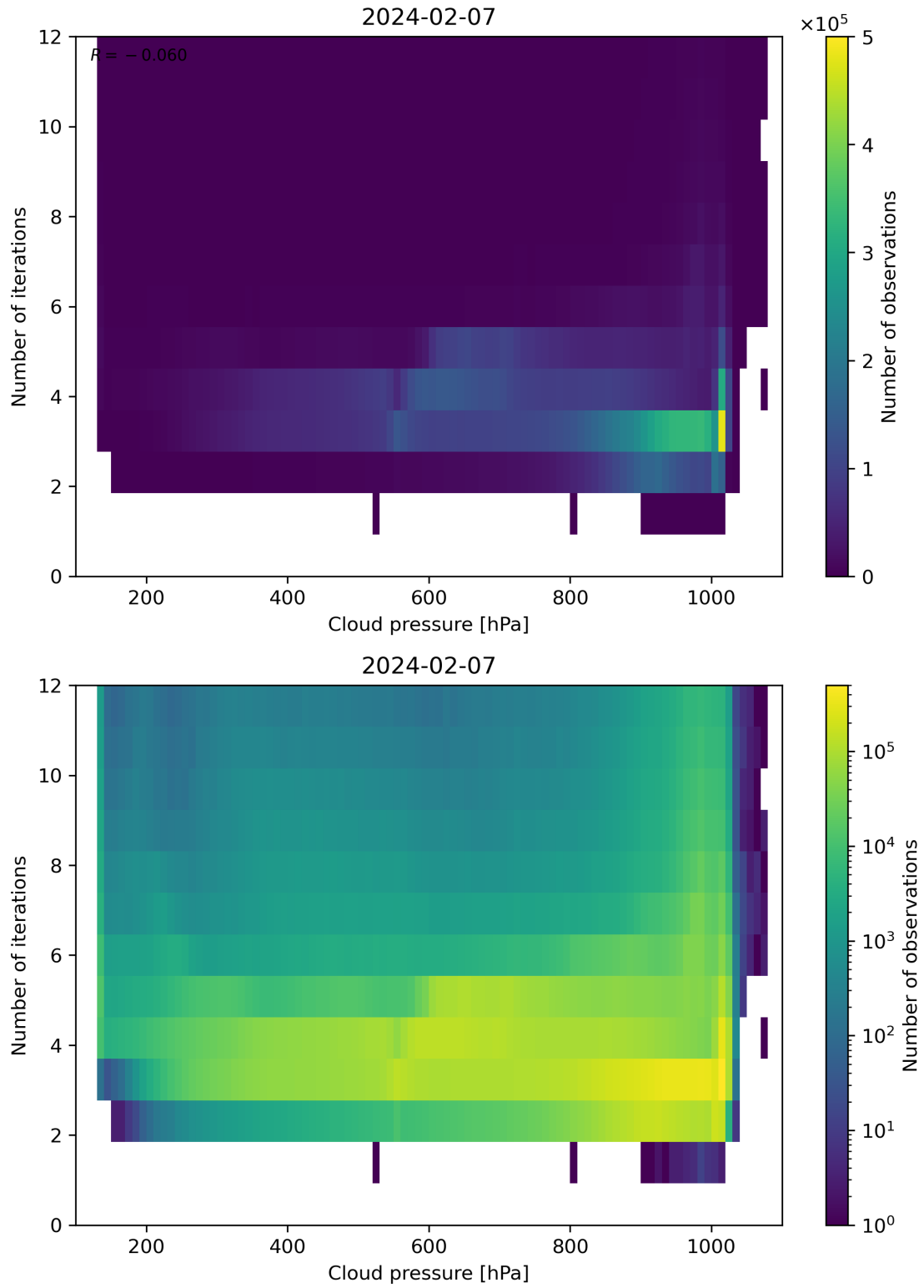
Figure 81: Scatter density plot of “Cloud pressure” against “Number of iterations” for 2024-02-06 to 2024-02-08.
