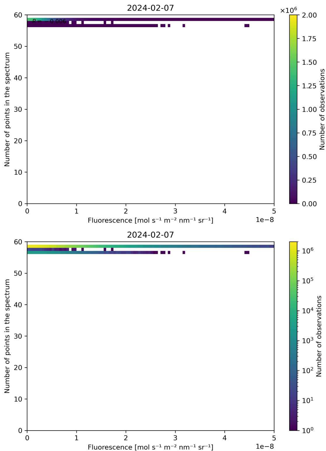
Figure 86: Scatter density plot of “Fluorescence” against “Number of points in the spectrum” for 2024-02-06 to 2024-02-08.
