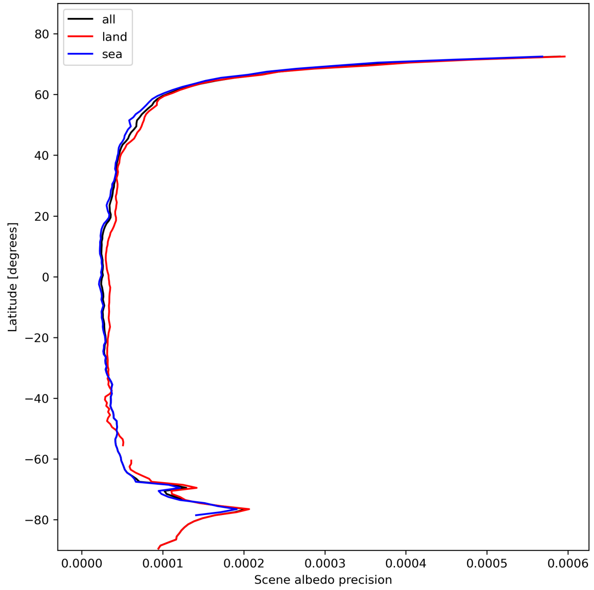
Figure 18: Zonal average of “Scene albedo precision” for 2024-02-06 to 2024-02-08.
