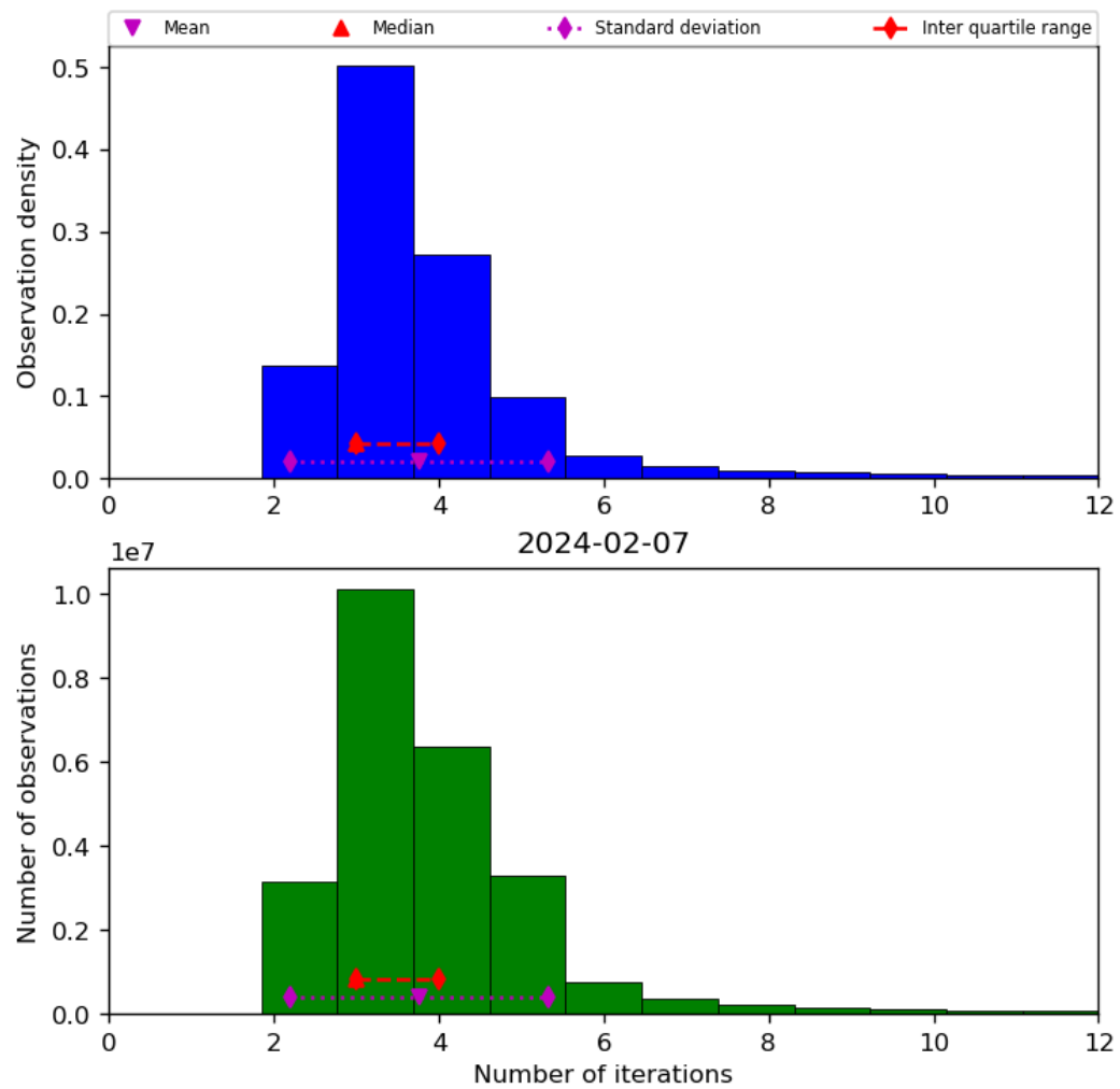
Figure 39: Histogram of “Number of iterations” for 2024-02-06 to 2024-02-08
