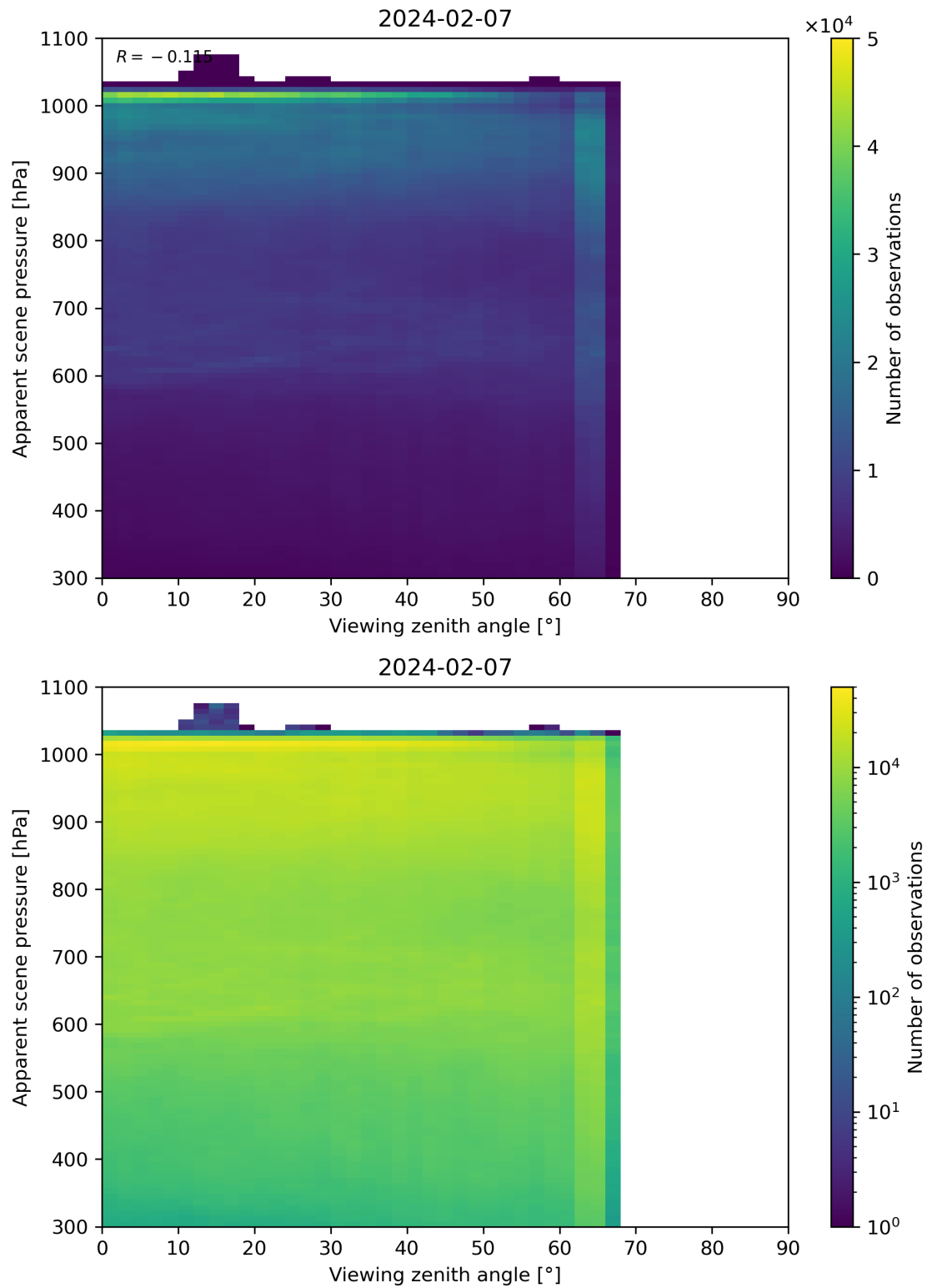
Figure 118: Scatter density plot of “Viewing zenith angle” against “Apparent scene pressure” for 2024-02-06 to 2024-02-08.
