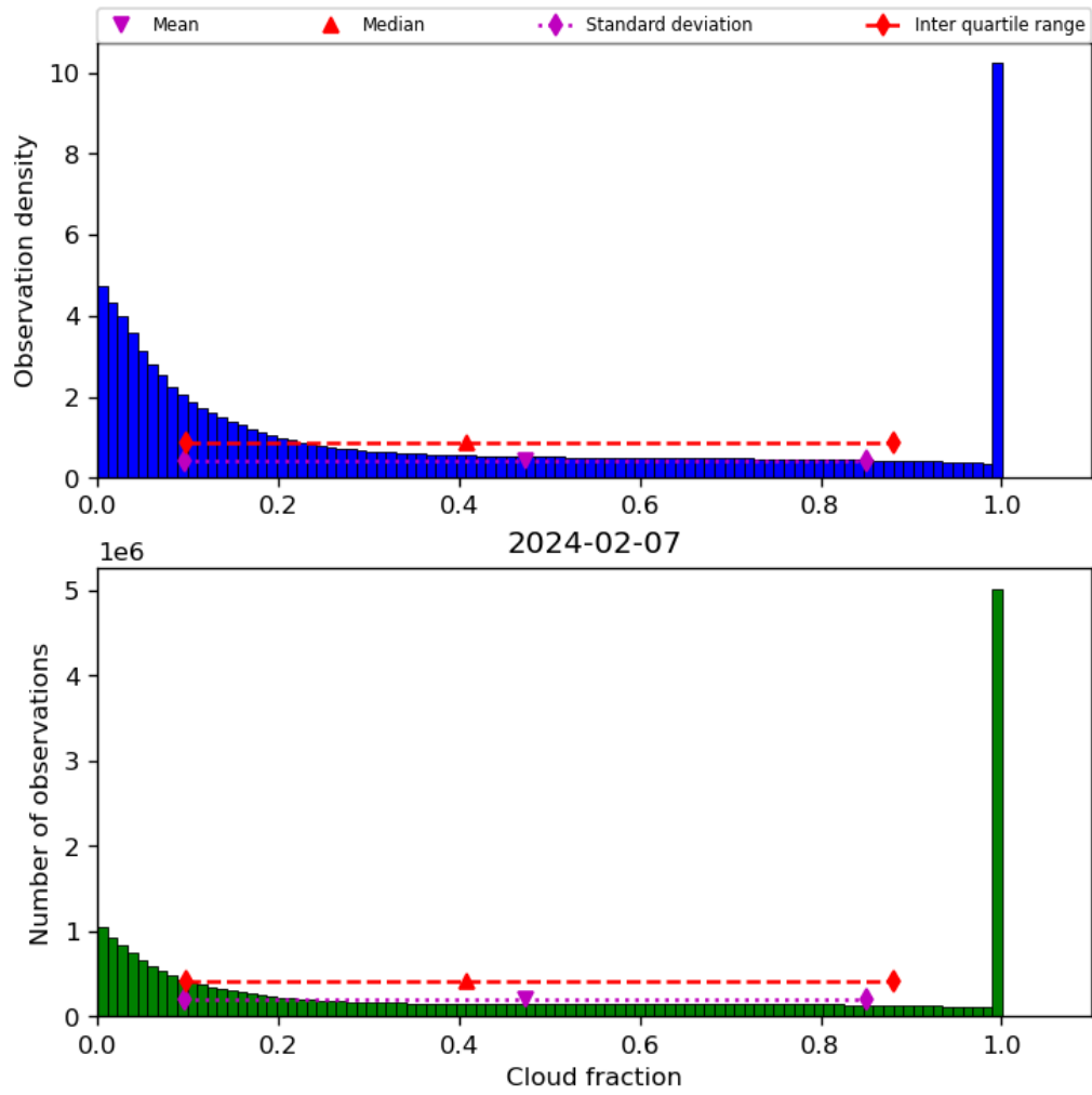
Figure 32: Histogram of “Cloud fraction” for 2024-02-06 to 2024-02-08
