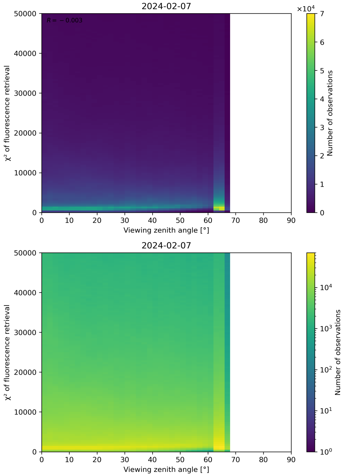
Figure 119: Scatter density plot of “Viewing zenith angle” against “ \chi^2 of fluorescence retrieval” for 2024-02-06 to 2024-02-08.
