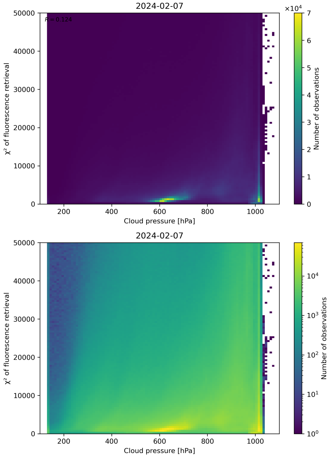
Figure 78: Scatter density plot of “Cloud pressure” against “ \chi^2 of fluorescence retrieval” for 2024-02-06 to 2024-02-08.
