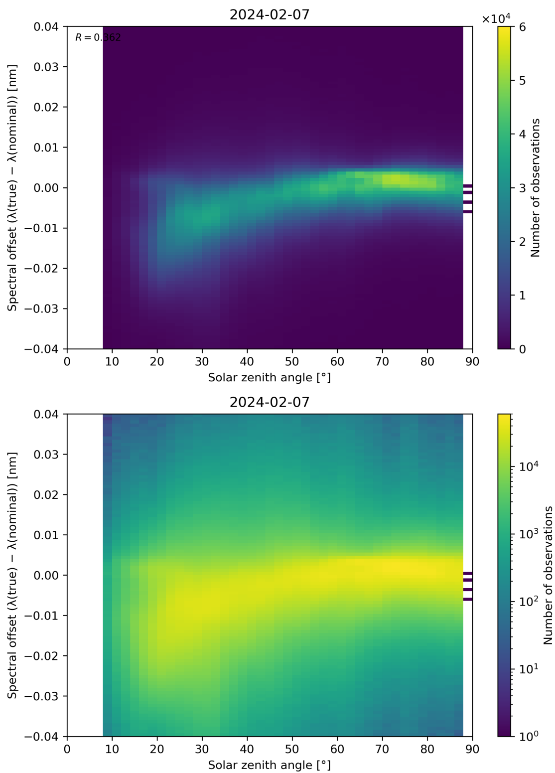
Figure 117: Scatter density plot of “Solar zenith angle” against “Spectral offset ( \lambda(\text{true}) - \lambda(\text{nominal}) )” for 2024-02-06 to 2024-02-08.
