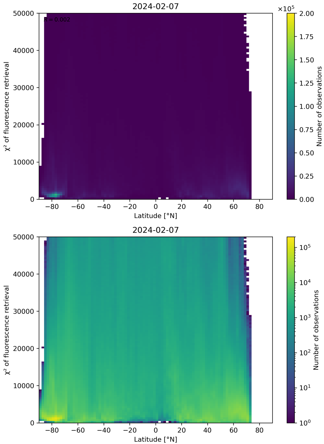
Figure 89: Scatter density plot of “Latitude” against “ \chi^2 of fluorescence retrieval” for 2024-02-06 to 2024-02-08.
