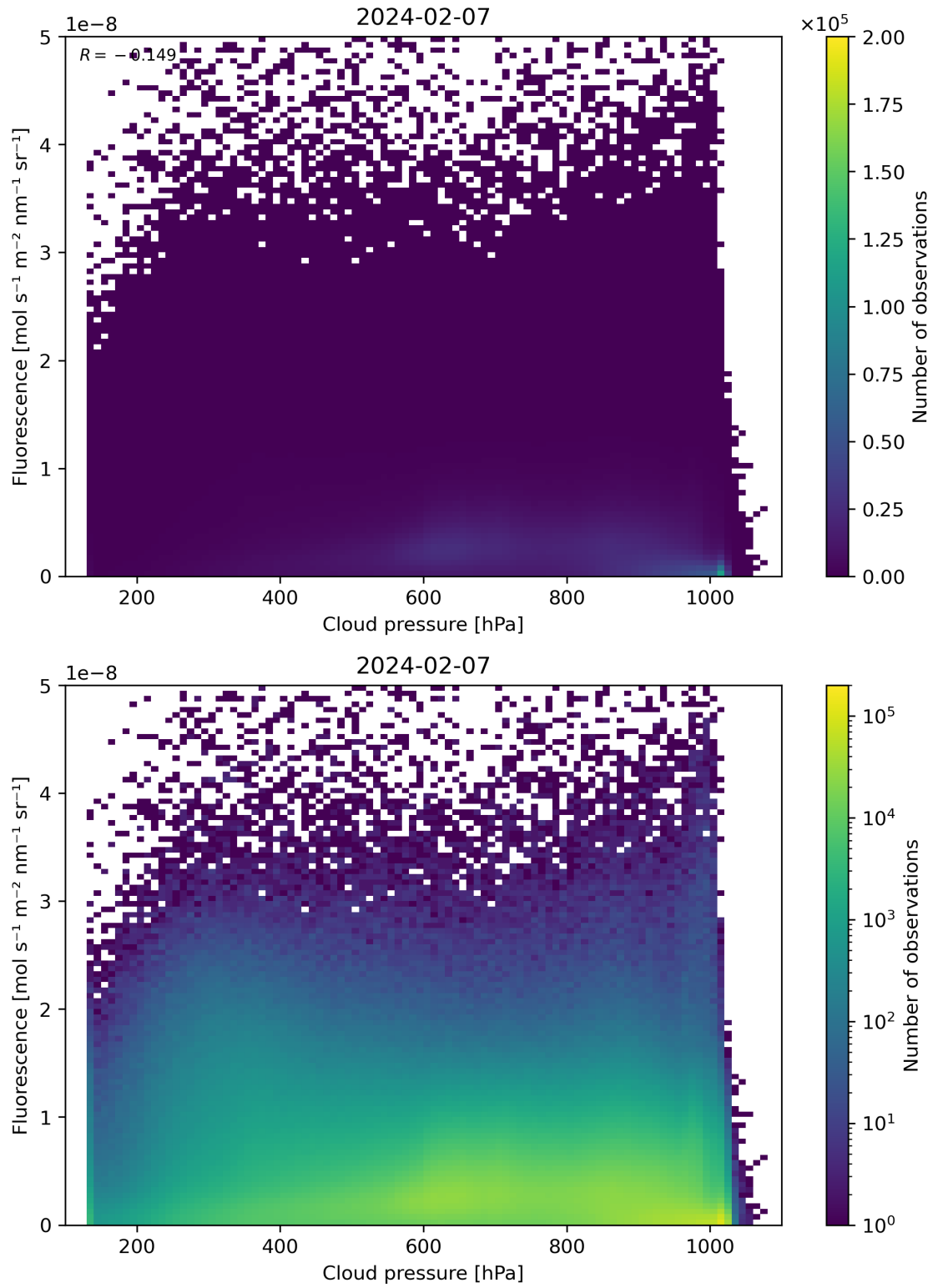
Figure 80: Scatter density plot of “Cloud pressure” against “Fluorescence” for 2024-02-06 to 2024-02-08.
