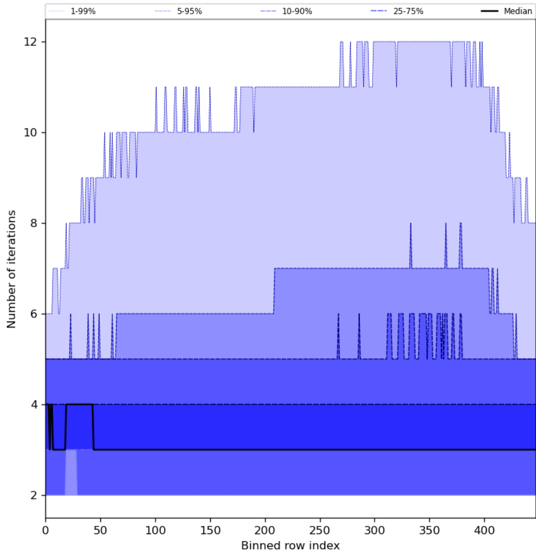
Figure 56: Along track statistics of “Number of iterations” for 2024-02-06 to 2024-02-08
