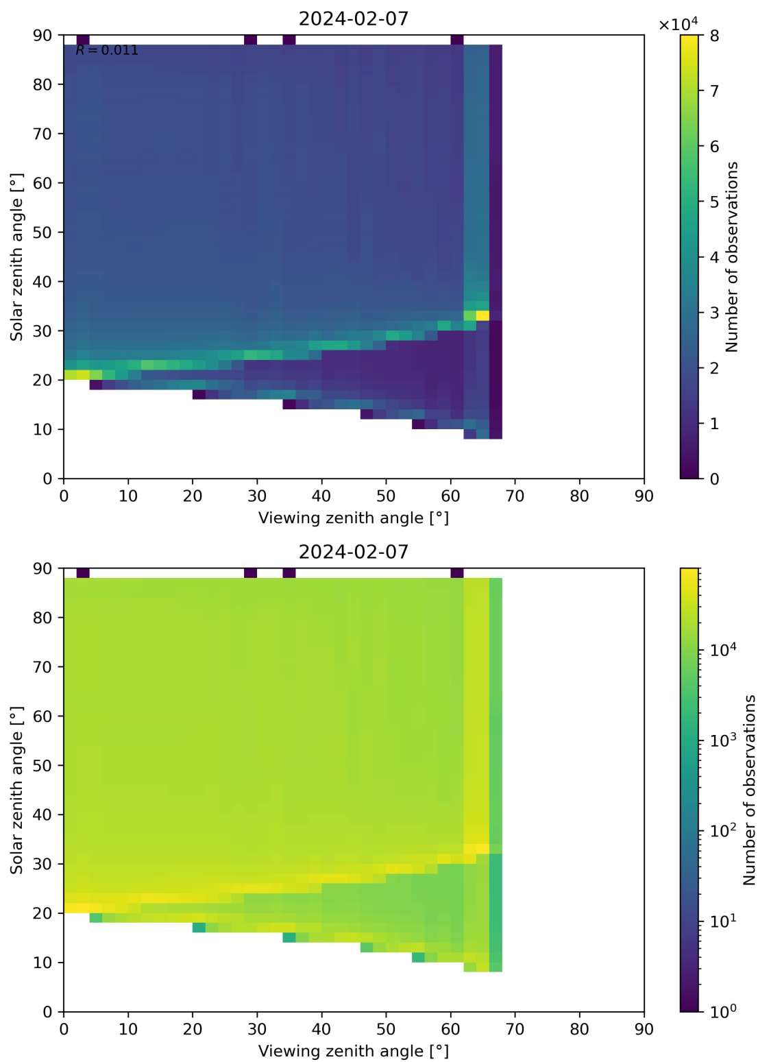
Figure 127: Scatter density plot of “Viewing zenith angle” against “Solar zenith angle” for 2024-02-06 to 2024-02-08.
