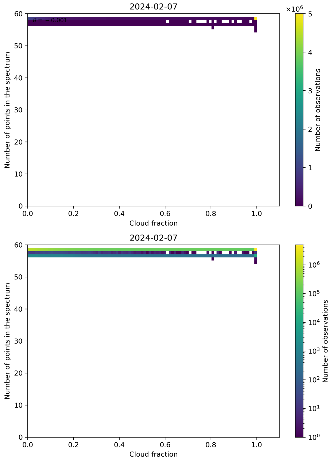
Figure 74: Scatter density plot of “Cloud fraction” against “Number of points in the spectrum” for 2024-02-06 to 2024-02-08.
