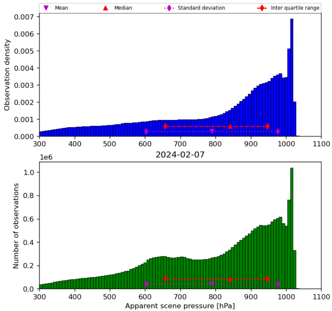
Figure 36: Histogram of “Apparent scene pressure” for 2024-02-06 to 2024-02-08
