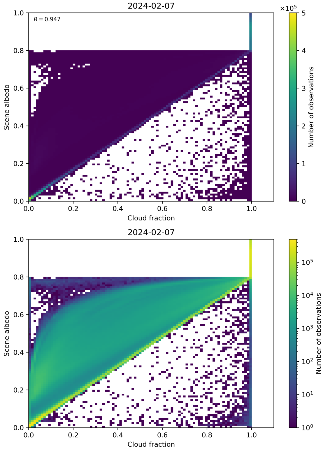
Figure 75: Scatter density plot of “Cloud fraction” against “Scene albedo” for 2024-02-06 to 2024-02-08.
