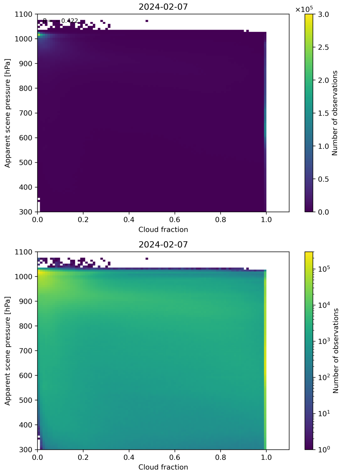
Figure 70: Scatter density plot of “Cloud fraction” against “Apparent scene pressure” for 2024-02-06 to 2024-02-08.
