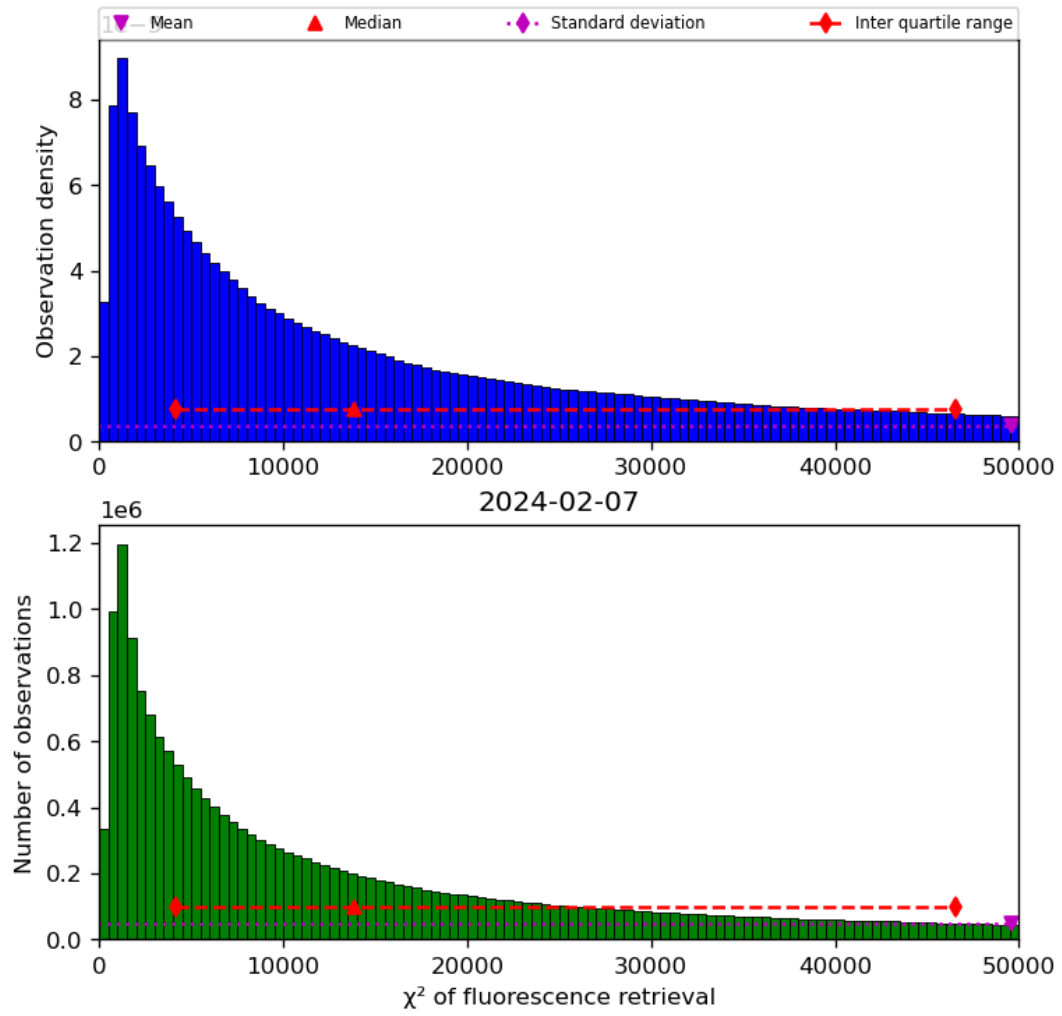
Figure 42: Histogram of “ \chi^2 of fluorescence retrieval” for 2024-02-06 to 2024-02-08
