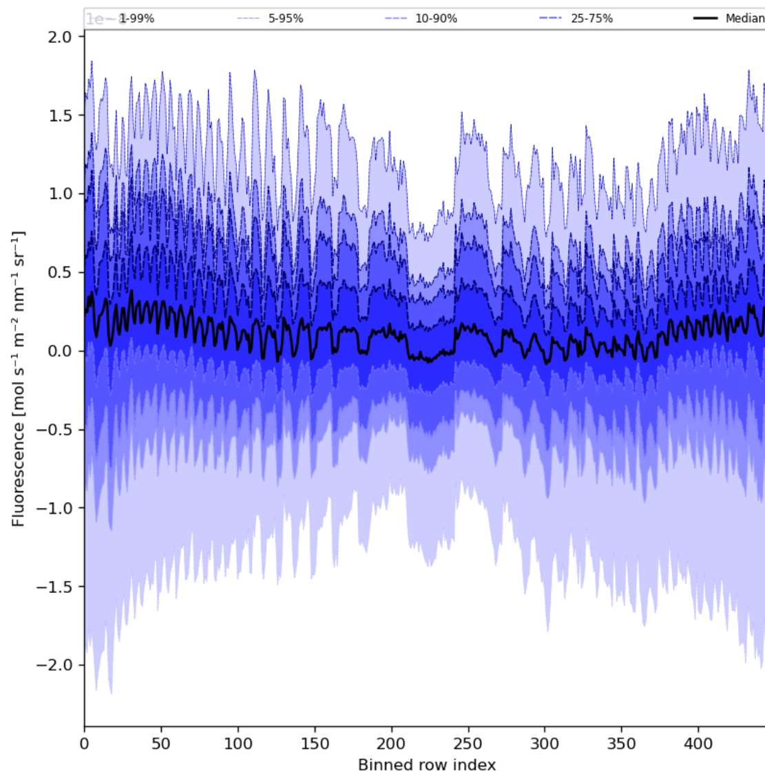
Figure 57: Along track statistics of “Fluorescence” for 2024-02-06 to 2024-02-08
