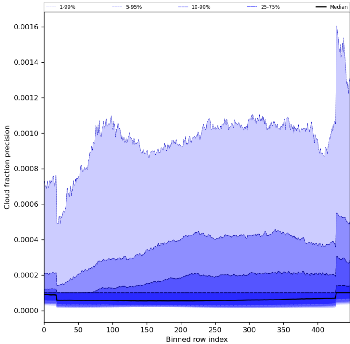
Figure 50: Along track statistics of “Cloud fraction precision” for 2024-02-06 to 2024-02-08
