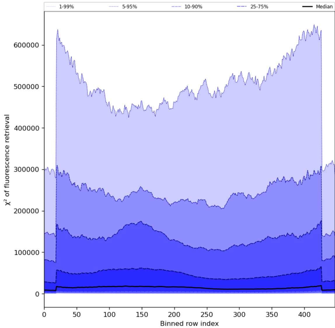
Figure 59: Along track statistics of “ \chi^2 of fluorescence retrieval” for 2024-02-06 to 2024-02-08
