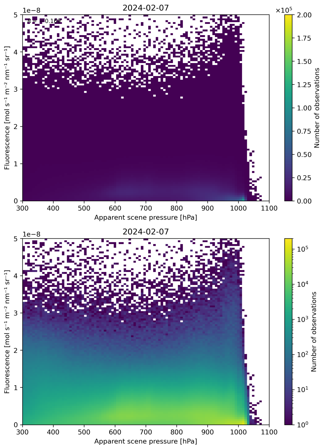
Figure 64: Scatter density plot of “Apparent scene pressure” against “Fluorescence” for 2024-02-06 to 2024-02-08.
