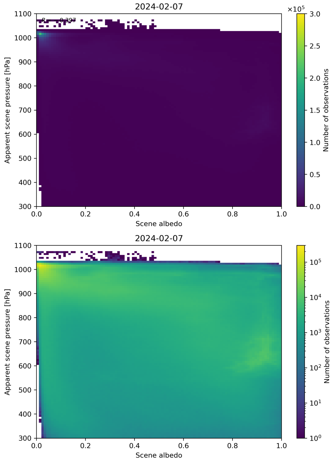
Figure 102: Scatter density plot of “Scene albedo” against “Apparent scene pressure” for 2024-02-06 to 2024-02-08.
