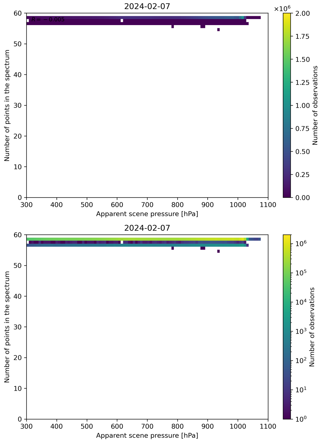
Figure 66: Scatter density plot of “Apparent scene pressure” against “Number of points in the spectrum” for 2024-02-06 to 2024-02-08.
