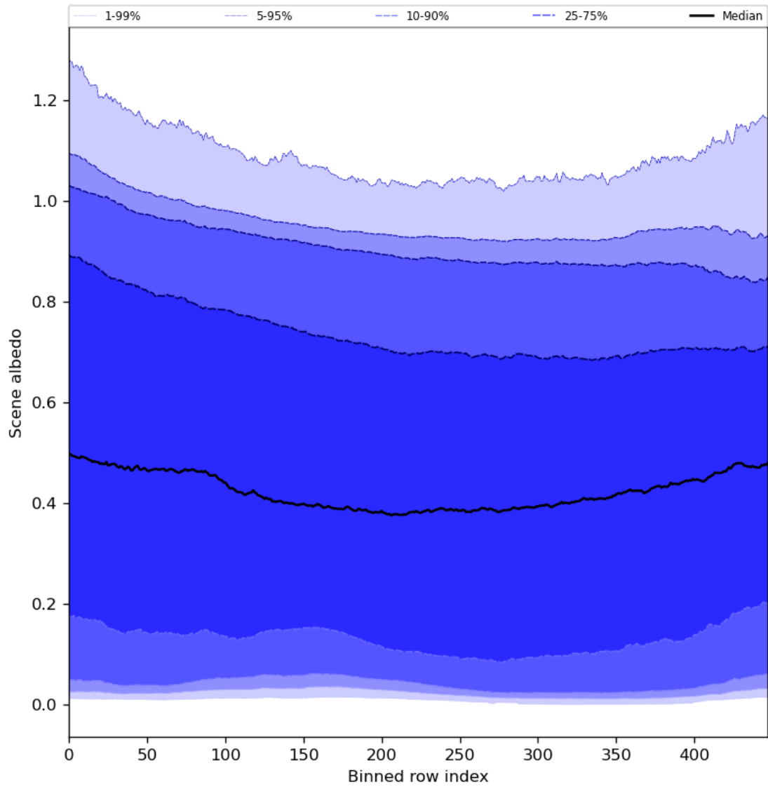
Figure 51: Along track statistics of “Scene albedo” for 2024-02-06 to 2024-02-08
