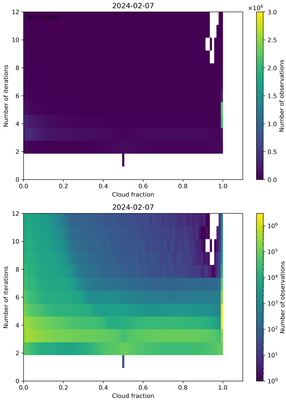
Figure 73: Scatter density plot of “Cloud fraction” against “Number of iterations” for 2024-02-06 to 2024-02-08.
