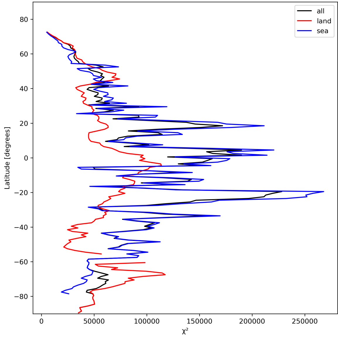
Figure 21: Zonal average of “ \chi^2 ” for 2024-02-06 to 2024-02-08.
