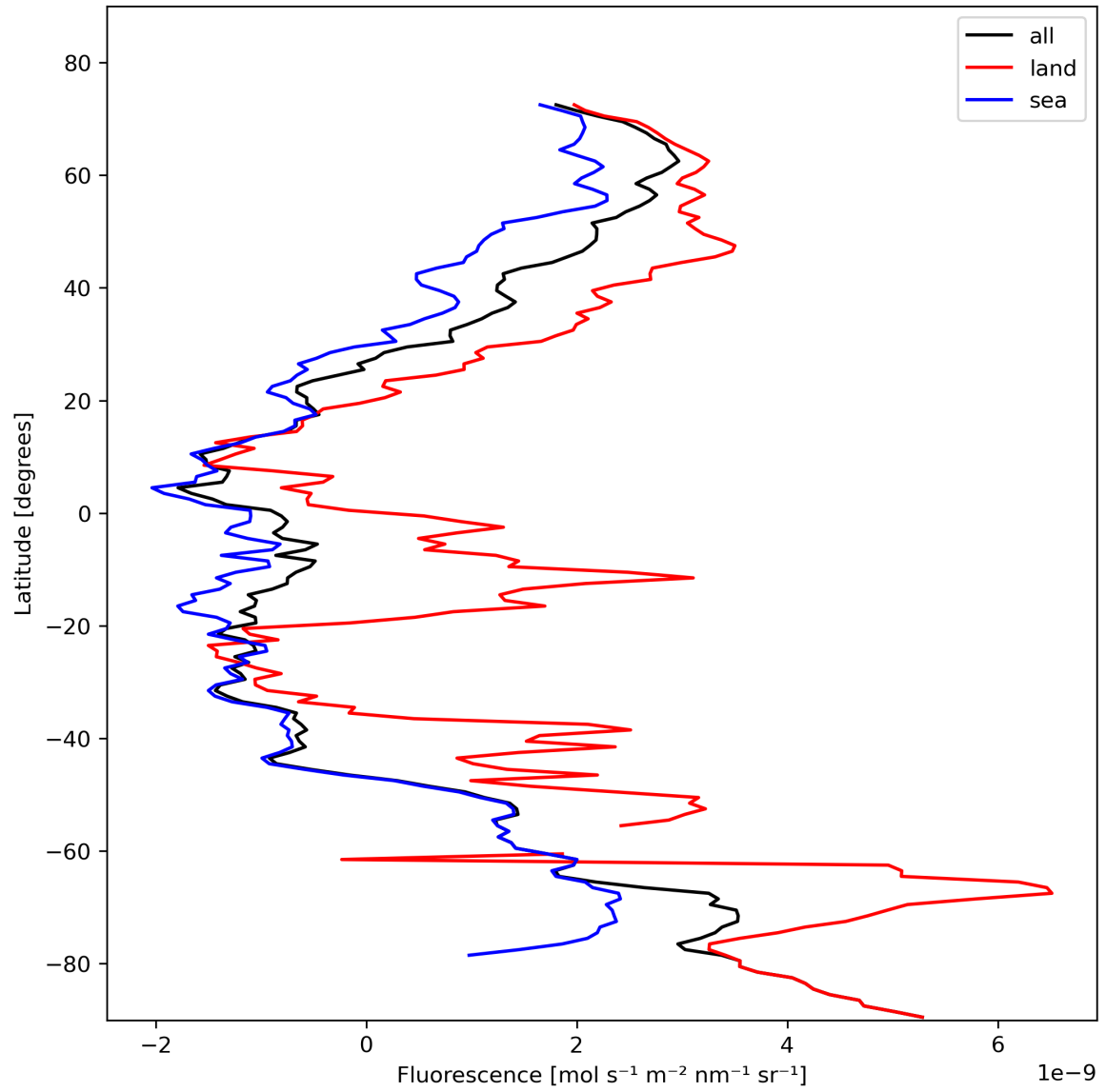
Figure 23: Zonal average of “Fluorescence” for 2024-02-06 to 2024-02-08.
