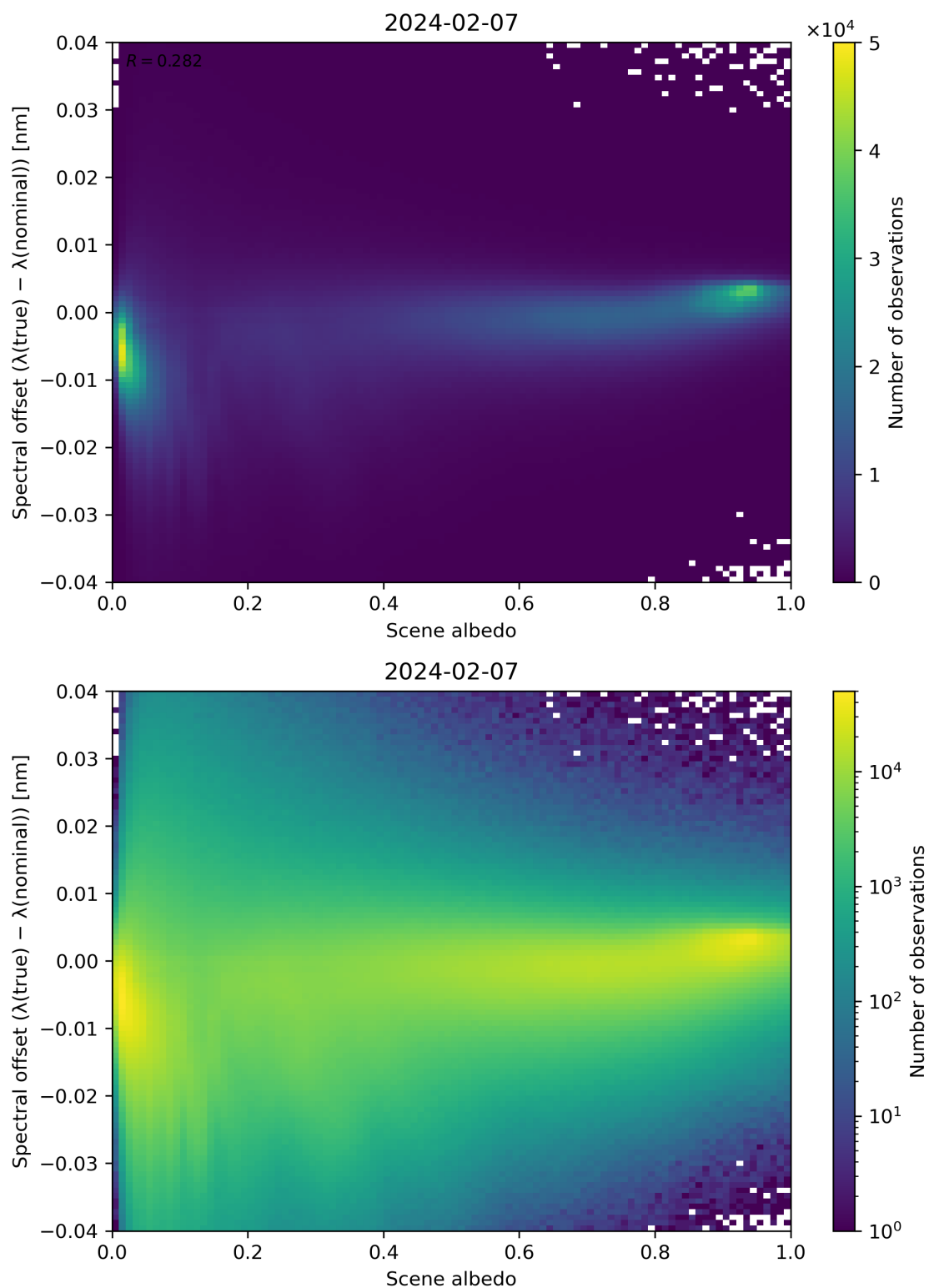
Figure 107: Scatter density plot of “Scene albedo” against “Spectral offset ( \lambda(\text{true}) - \lambda(\text{nominal}) )” for 2024-02-06 to 2024-02-08.
