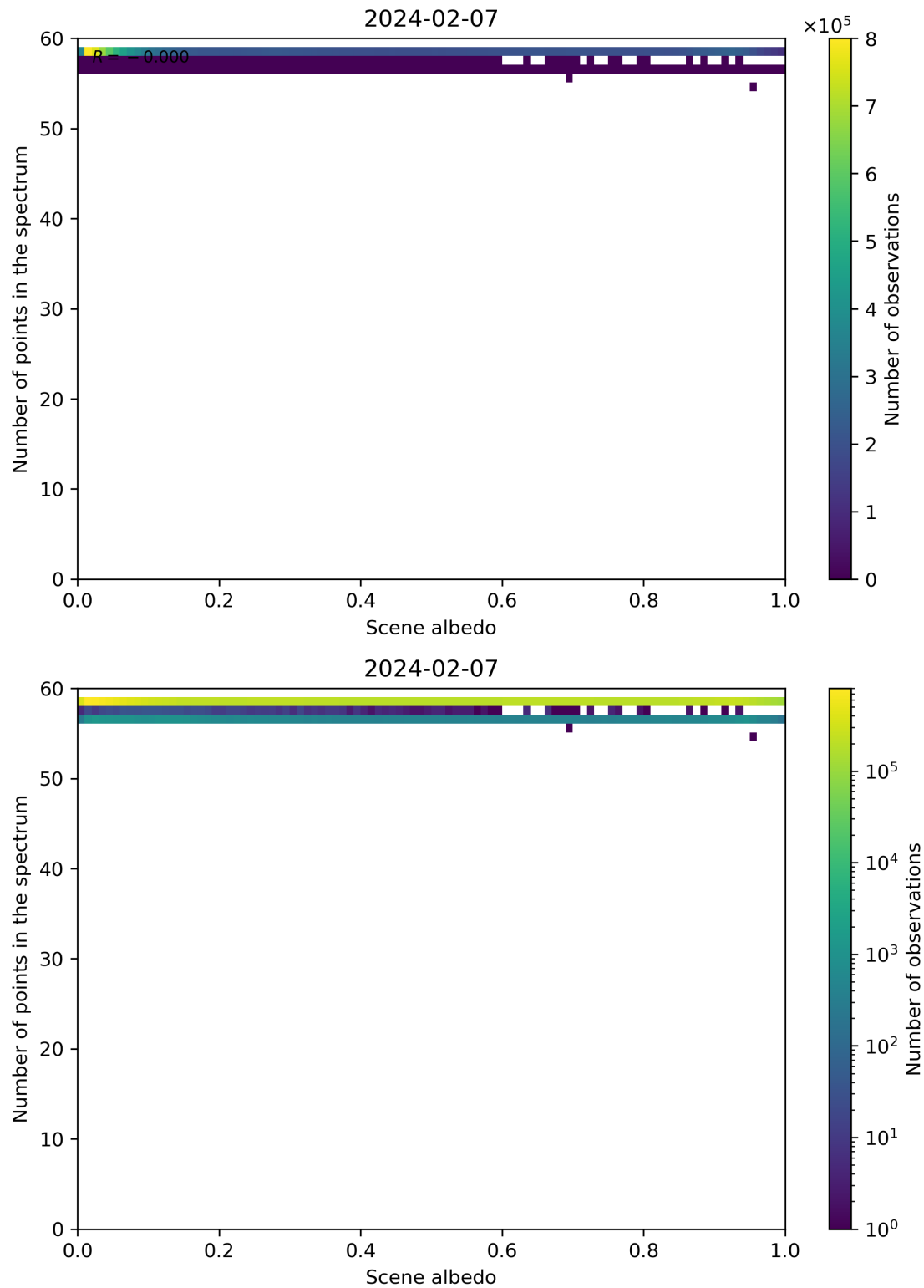
Figure 106: Scatter density plot of “Scene albedo” against “Number of points in the spectrum” for 2024-02-06 to 2024-02-08.
