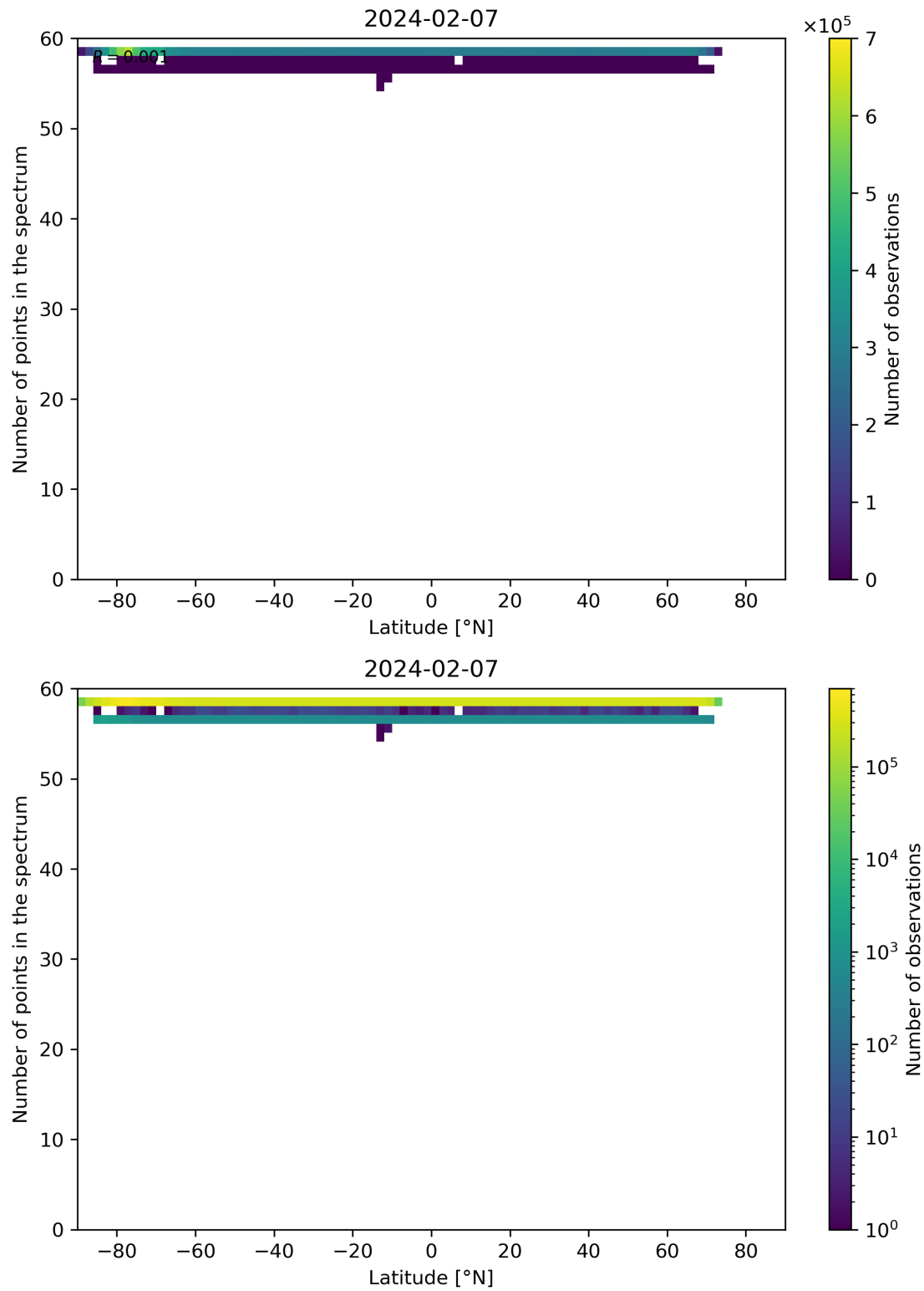
Figure 94: Scatter density plot of “Latitude” against “Number of points in the spectrum” for 2024-02-06 to 2024-02-08.
