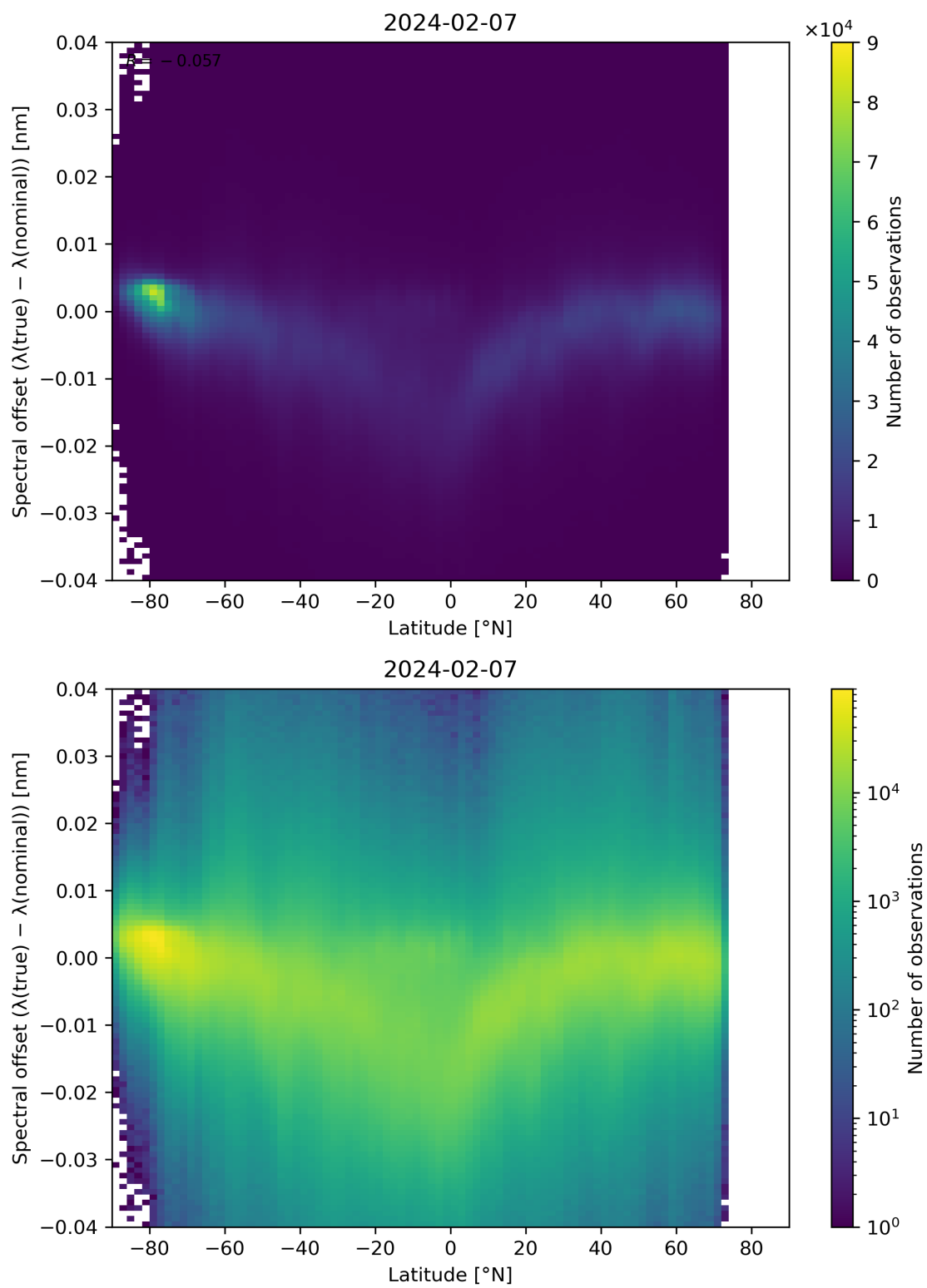
Figure 96: Scatter density plot of “Latitude” against “Spectral offset ( \lambda(\text{true}) - \lambda(\text{nominal}) )” for 2024-02-06 to 2024-02-08.
