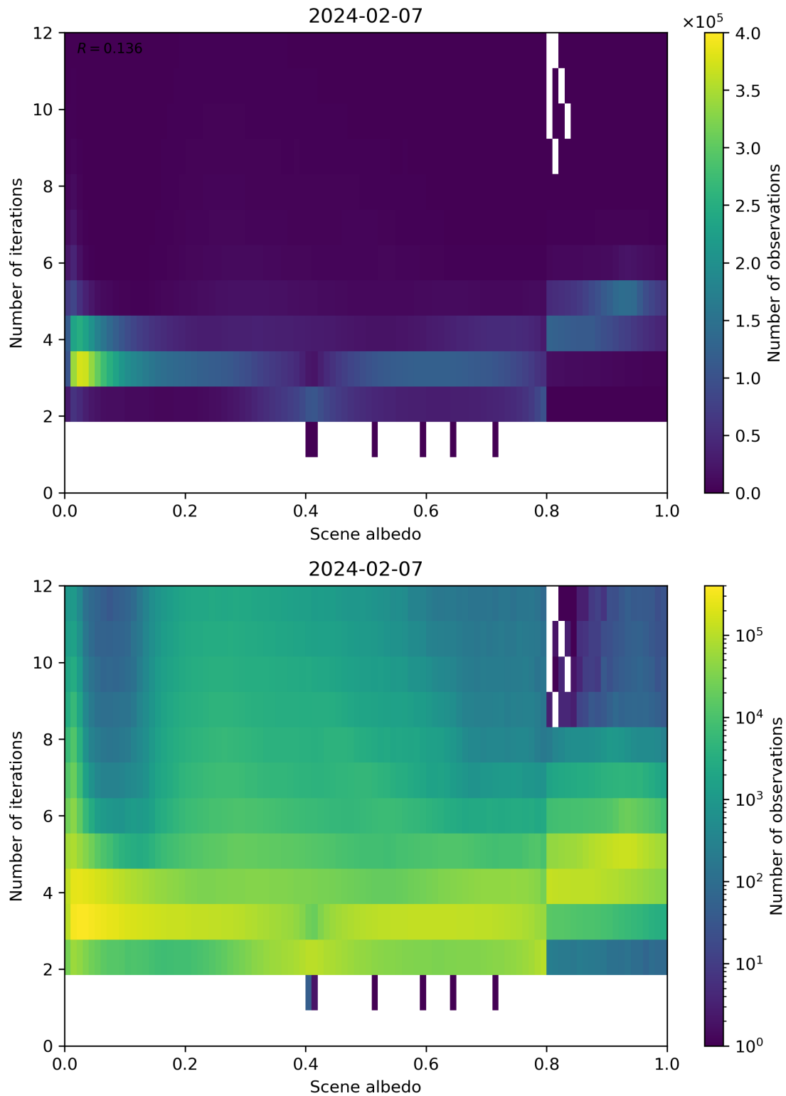
Figure 105: Scatter density plot of “Scene albedo” against “Number of iterations” for 2024-02-06 to 2024-02-08.
