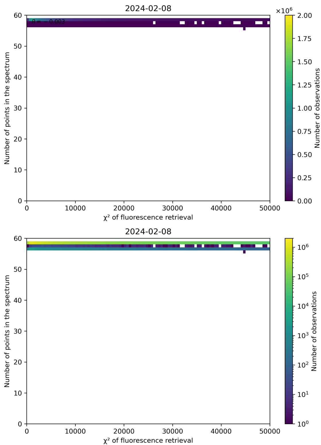
Figure 68: Scatter density plot of “ \chi^2 of fluorescence retrieval” against “Number of points in the spectrum” for 2024-02-07 to 2024-02-09.
