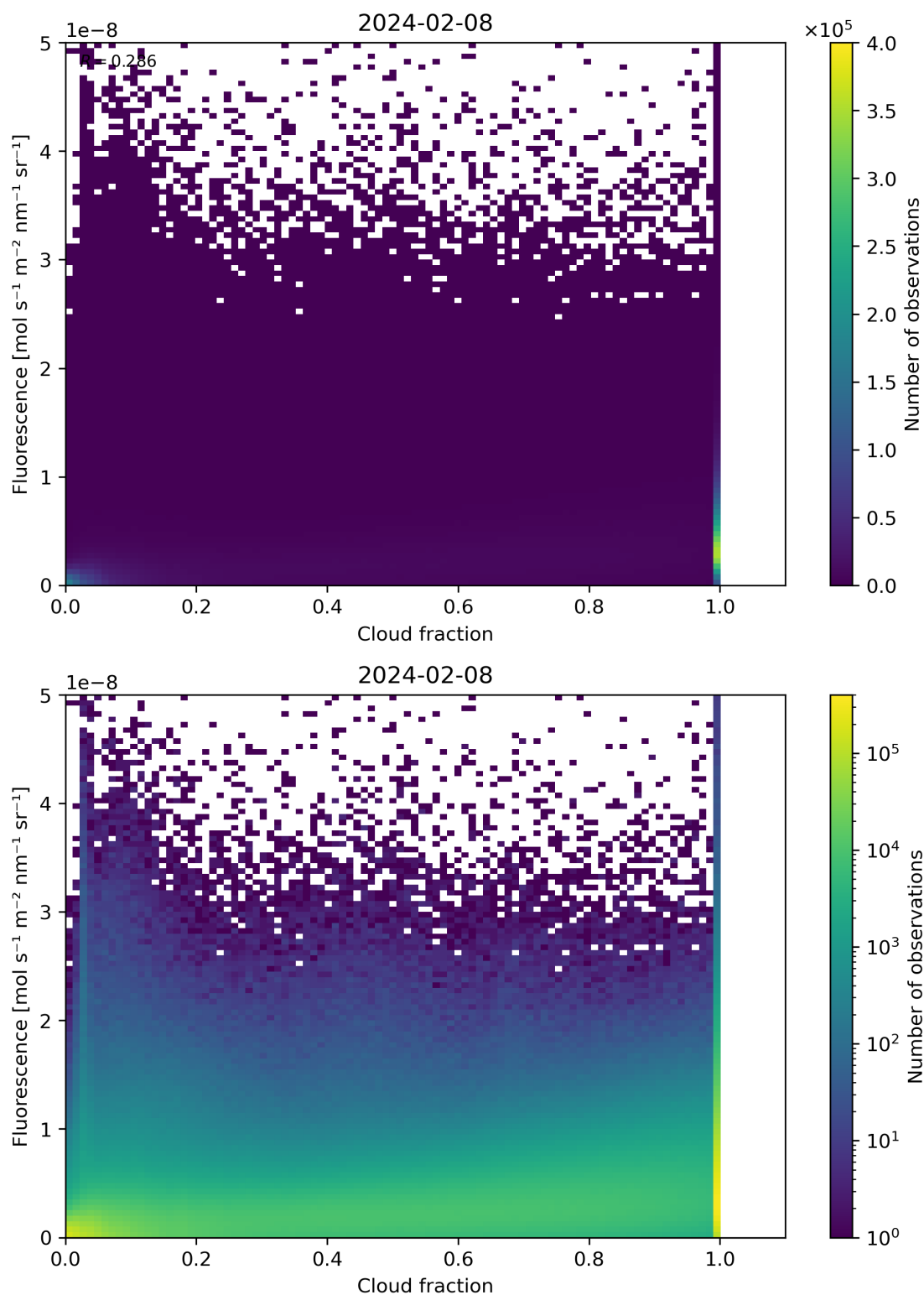
Figure 72: Scatter density plot of “Cloud fraction” against “Fluorescence” for 2024-02-07 to 2024-02-09.
