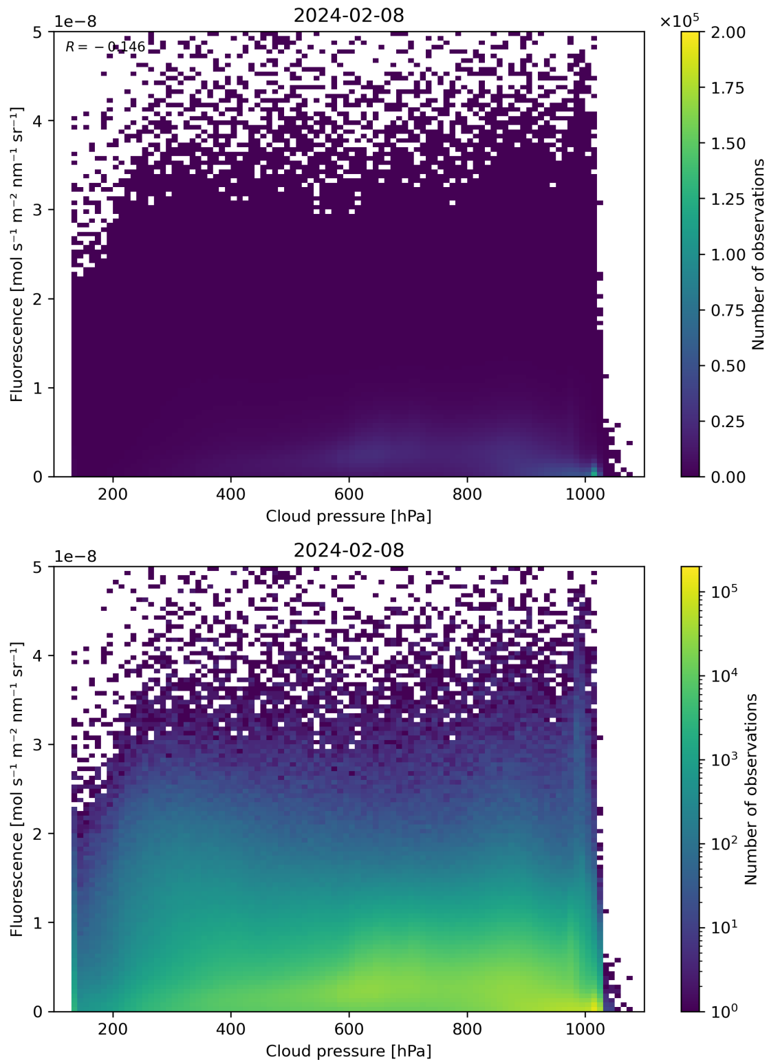
Figure 80: Scatter density plot of “Cloud pressure” against “Fluorescence” for 2024-02-07 to 2024-02-09.
