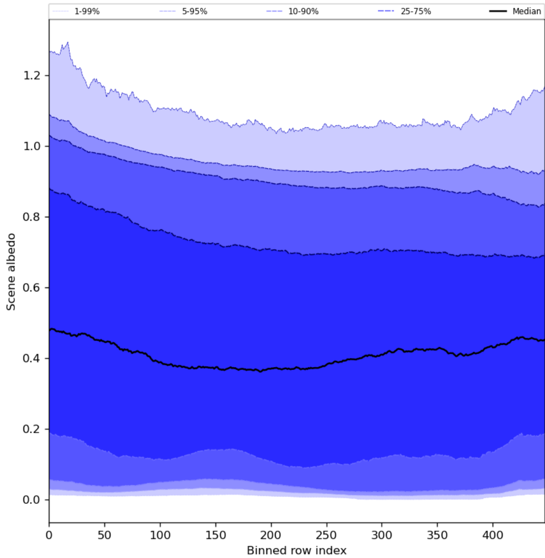
Figure 51: Along track statistics of “Scene albedo” for 2024-02-07 to 2024-02-09
