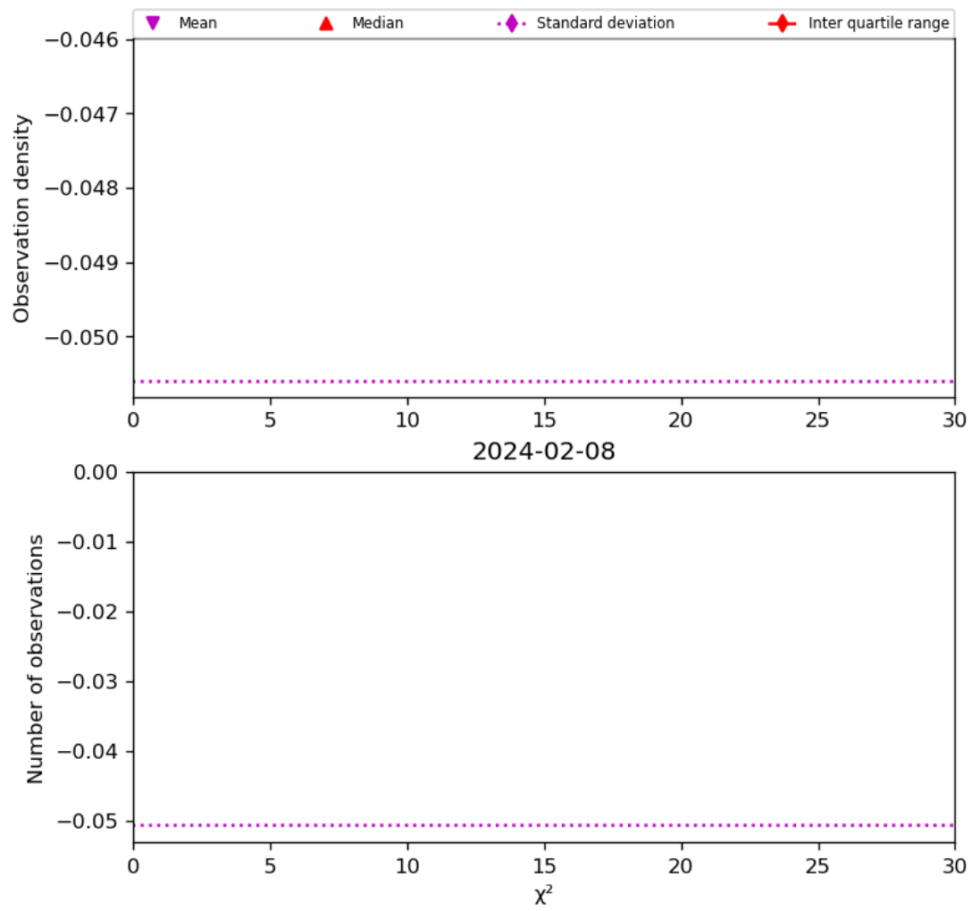
Figure 38: Histogram of “ \chi^2 ” for 2024-02-07 to 2024-02-09
