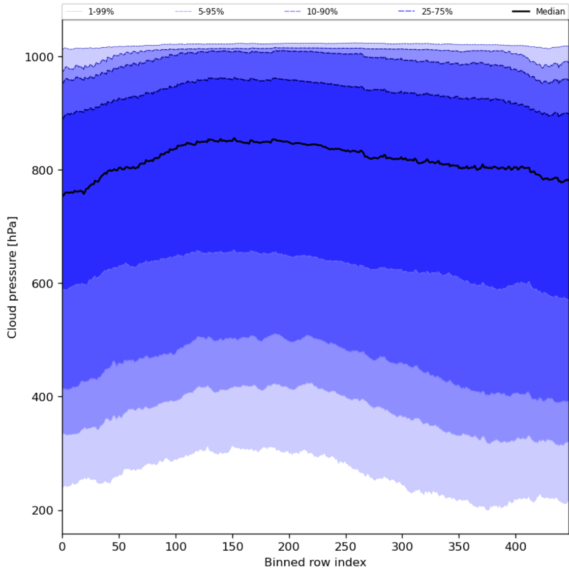
Figure 47: Along track statistics of “Cloud pressure” for 2024-02-07 to 2024-02-09
