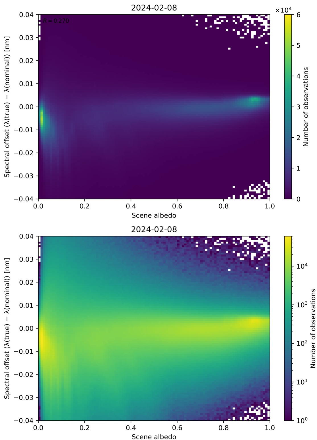
Figure 107: Scatter density plot of “Scene albedo” against “Spectral offset ( \lambda(\text{true}) - \lambda(\text{nominal}) )” for 2024-02-07 to 2024-02-09.
