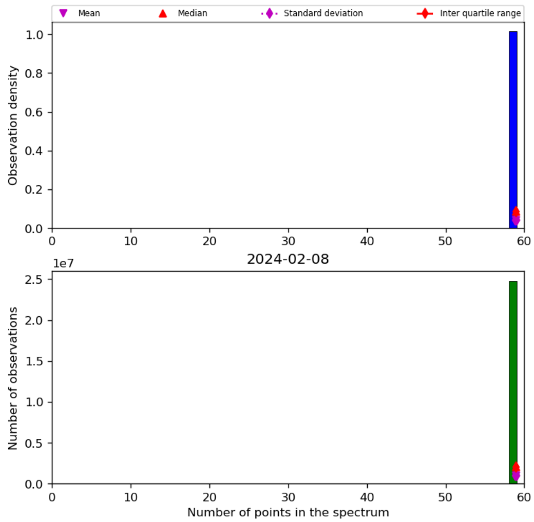
Figure 44: Histogram of “Number of points in the spectrum” for 2024-02-07 to 2024-02-09
