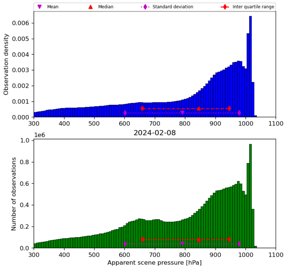
Figure 36: Histogram of “Apparent scene pressure” for 2024-02-07 to 2024-02-09
