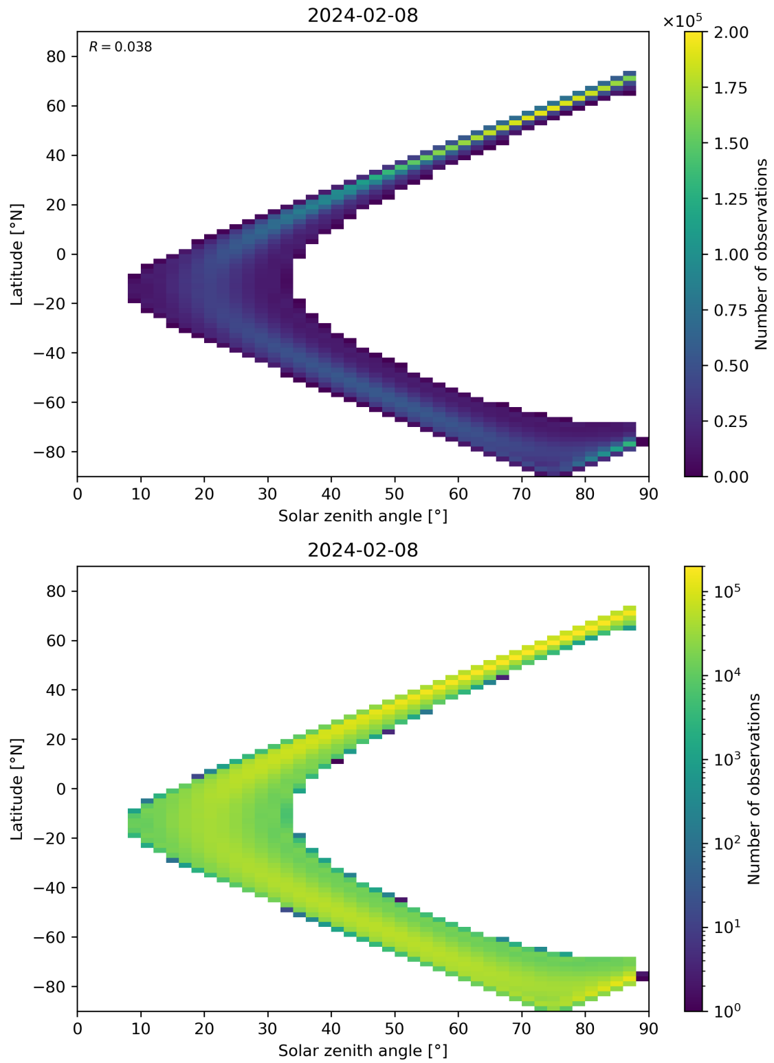
Figure 113: Scatter density plot of “Solar zenith angle” against “Latitude” for 2024-02-07 to 2024-02-09.
