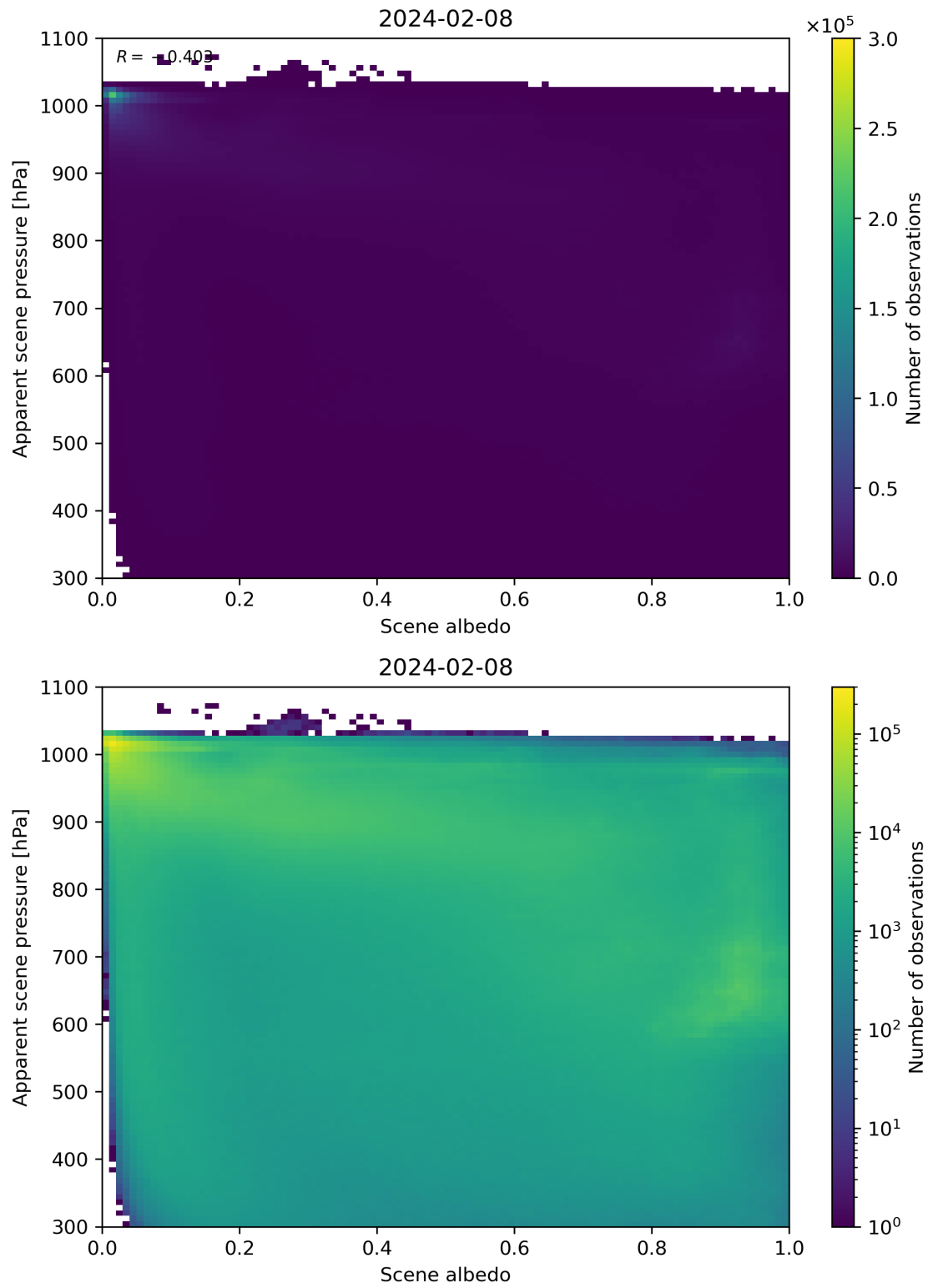
Figure 102: Scatter density plot of “Scene albedo” against “Apparent scene pressure” for 2024-02-07 to 2024-02-09.
