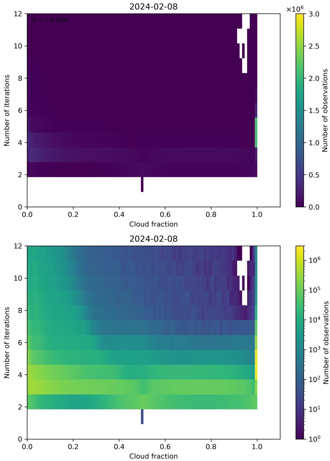
Figure 73: Scatter density plot of “Cloud fraction” against “Number of iterations” for 2024-02-07 to 2024-02-09.
