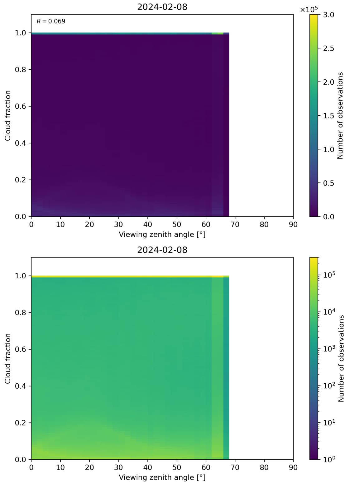
Figure 120: Scatter density plot of “Viewing zenith angle” against “Cloud fraction” for 2024-02-07 to 2024-02-09.
