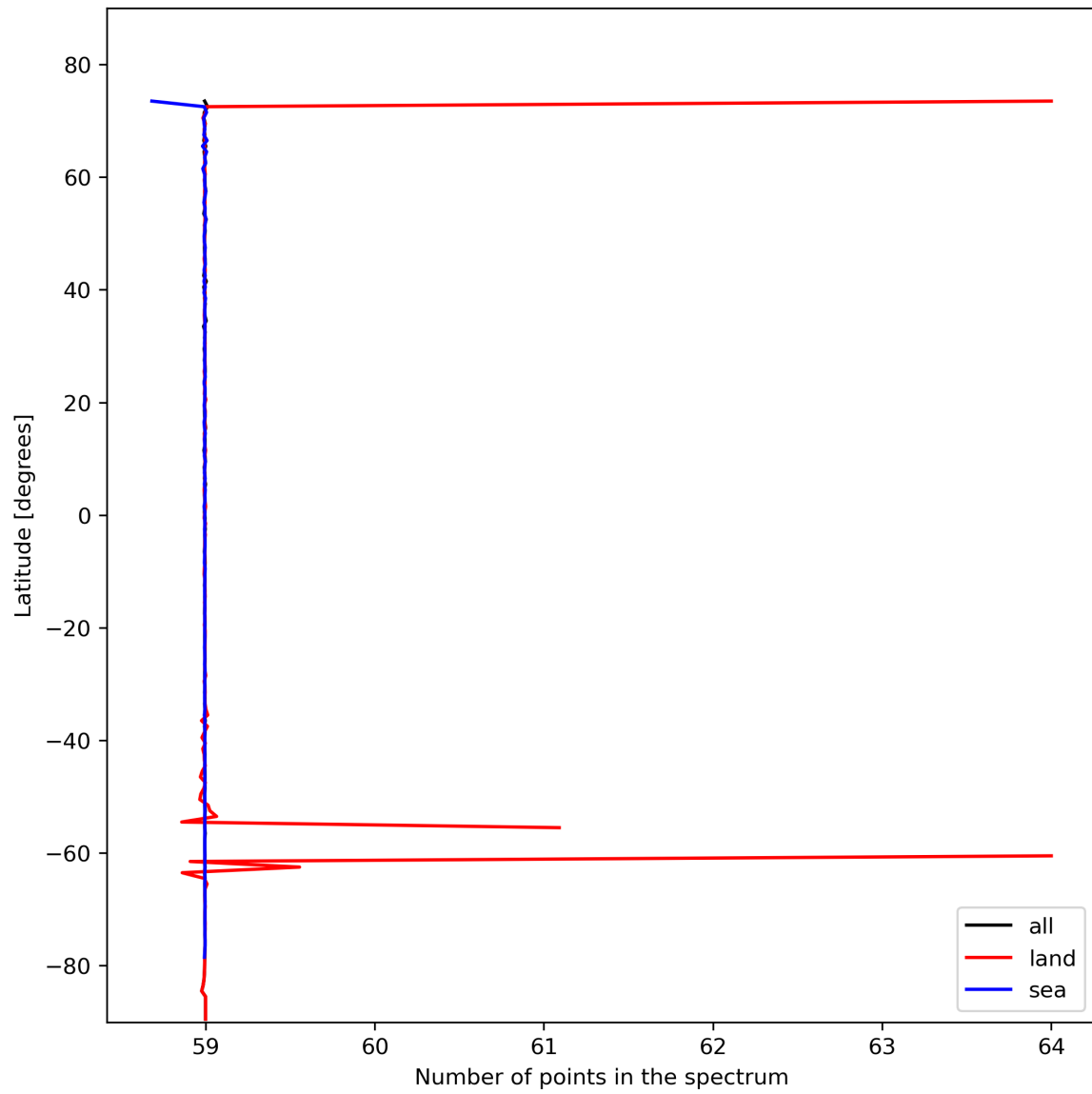
Figure 27: Zonal average of “Number of points in the spectrum” for 2024-02-07 to 2024-02-09.
