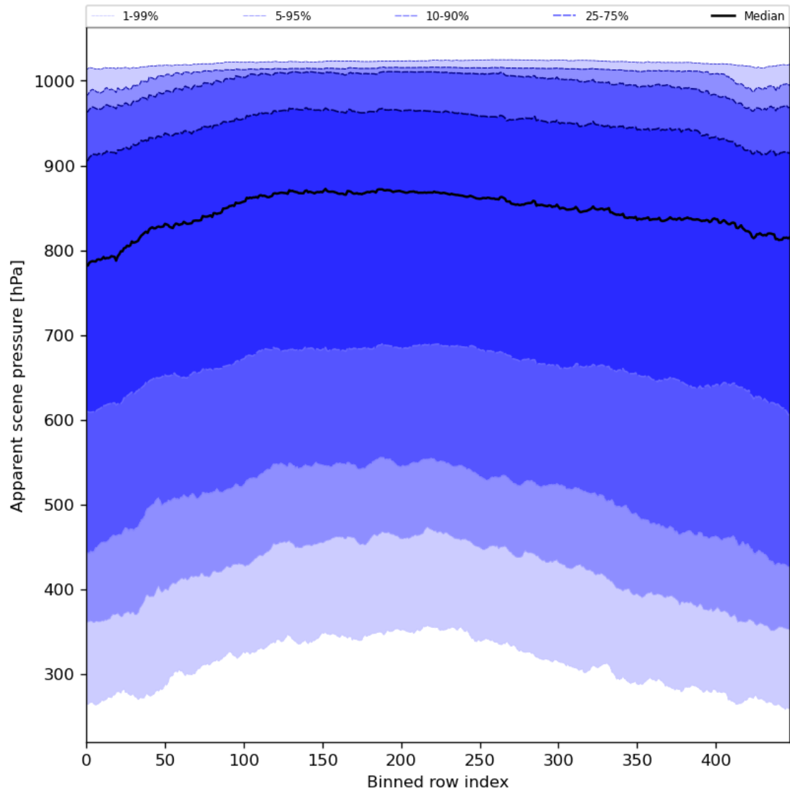
Figure 53: Along track statistics of “Apparent scene pressure” for 2024-02-07 to 2024-02-09
