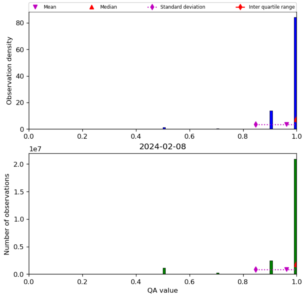
Figure 29: Histogram of “QA value” for 2024-02-07 to 2024-02-09
