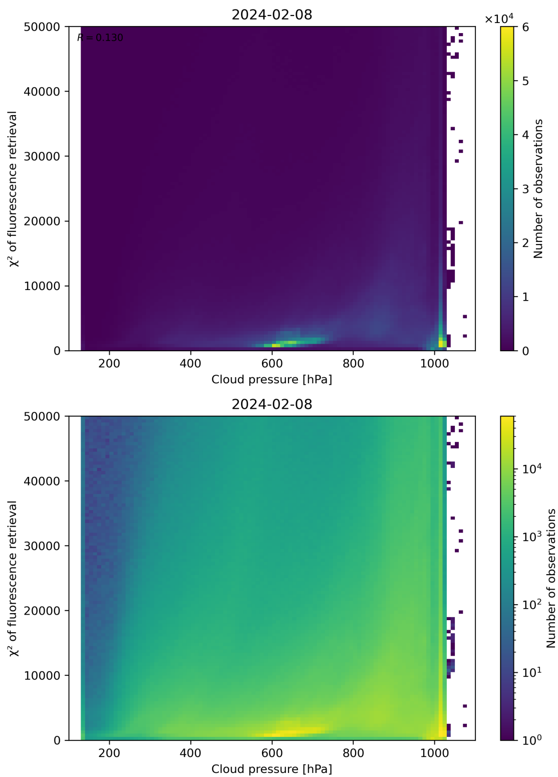
Figure 78: Scatter density plot of “Cloud pressure” against “ \chi^2 of fluorescence retrieval” for 2024-02-07 to 2024-02-09.
