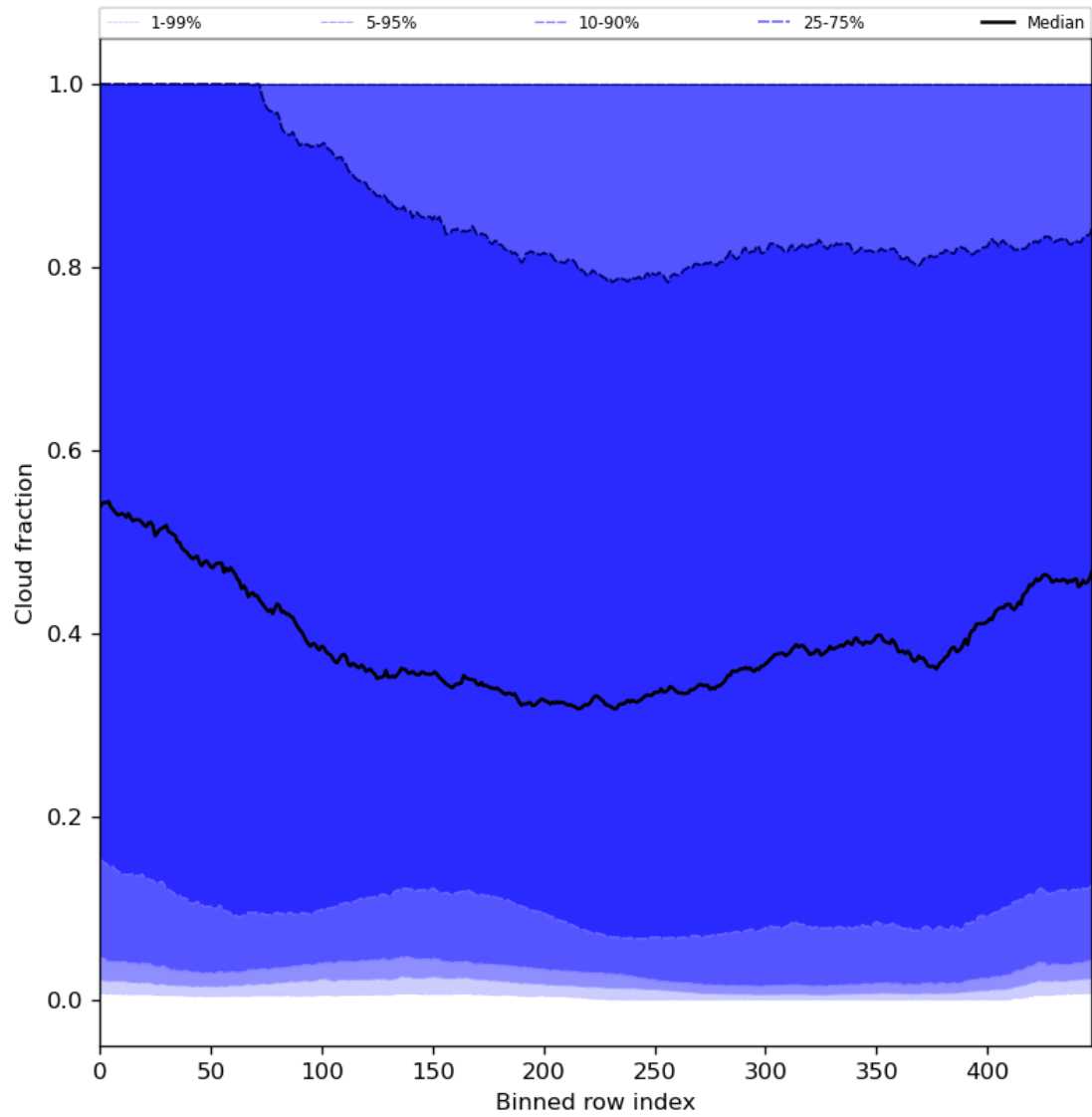
Figure 49: Along track statistics of “Cloud fraction” for 2024-02-07 to 2024-02-09
