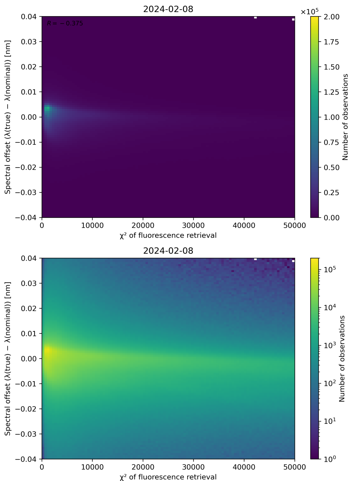
Figure 69: Scatter density plot of " \chi^2 of fluorescence retrieval" against "Spectral offset ( \lambda(\text{true}) - \lambda(\text{nominal})) " for 2024-02-07 to 2024-02-09.
