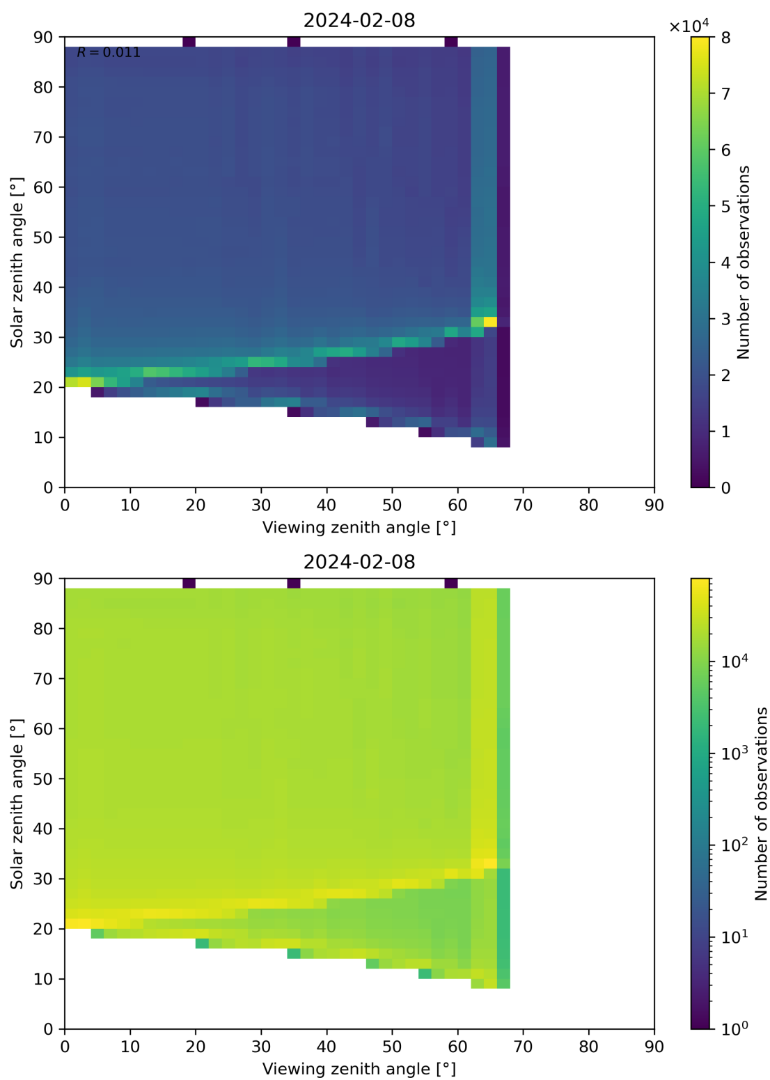
Figure 127: Scatter density plot of “Viewing zenith angle” against “Solar zenith angle” for 2024-02-07 to 2024-02-09.
