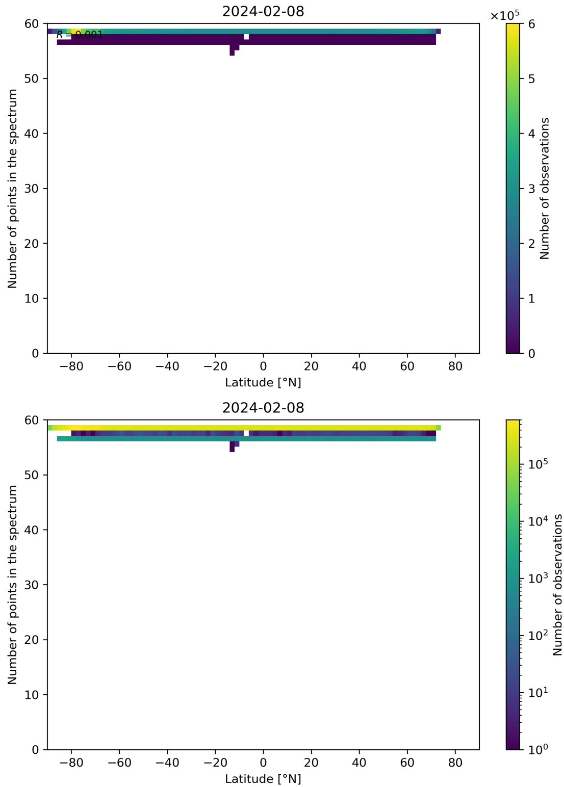
Figure 94: Scatter density plot of “Latitude” against “Number of points in the spectrum” for 2024-02-07 to 2024-02-09.
