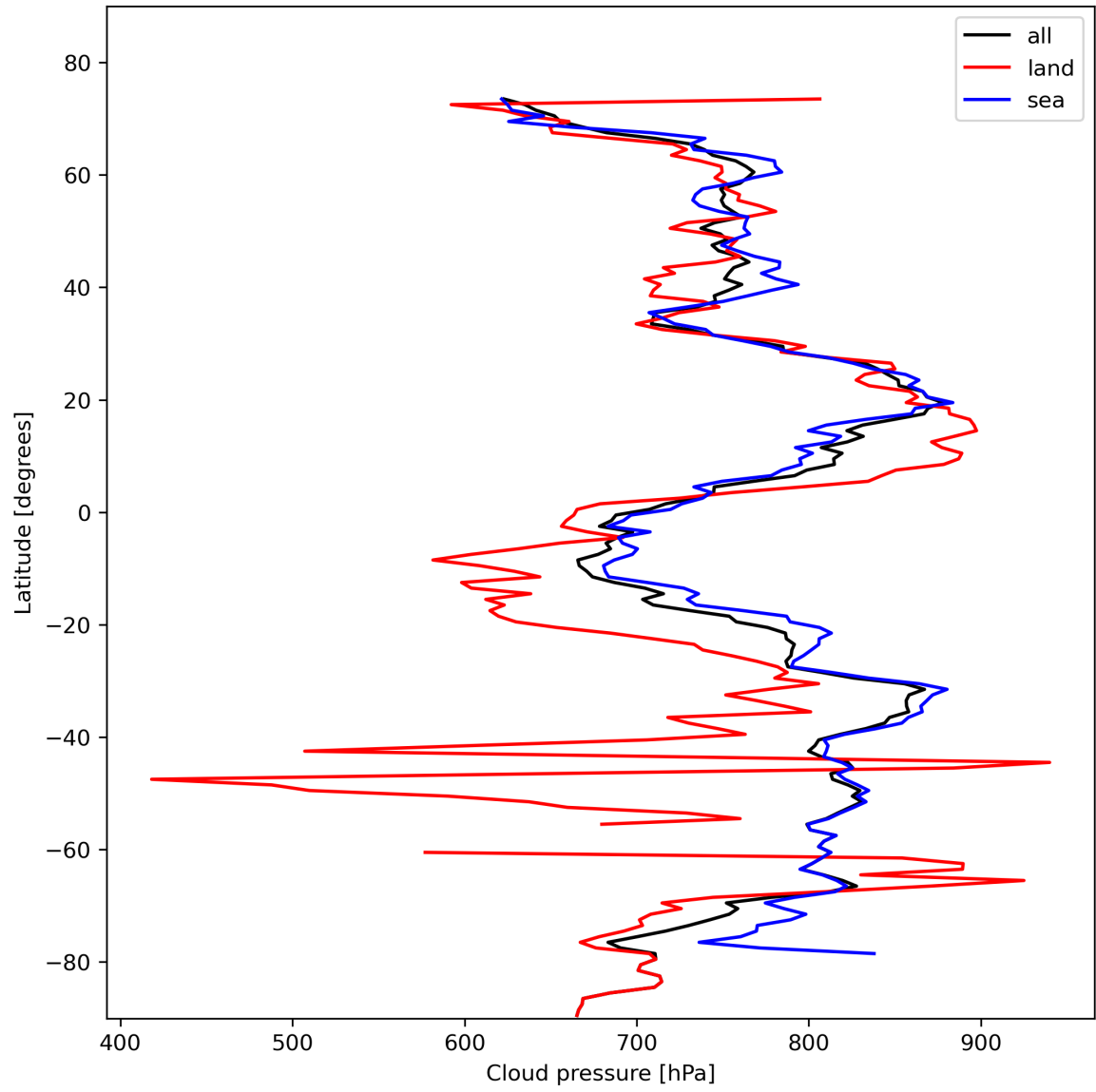
Figure 13: Zonal average of “Cloud pressure” for 2024-02-07 to 2024-02-09.
