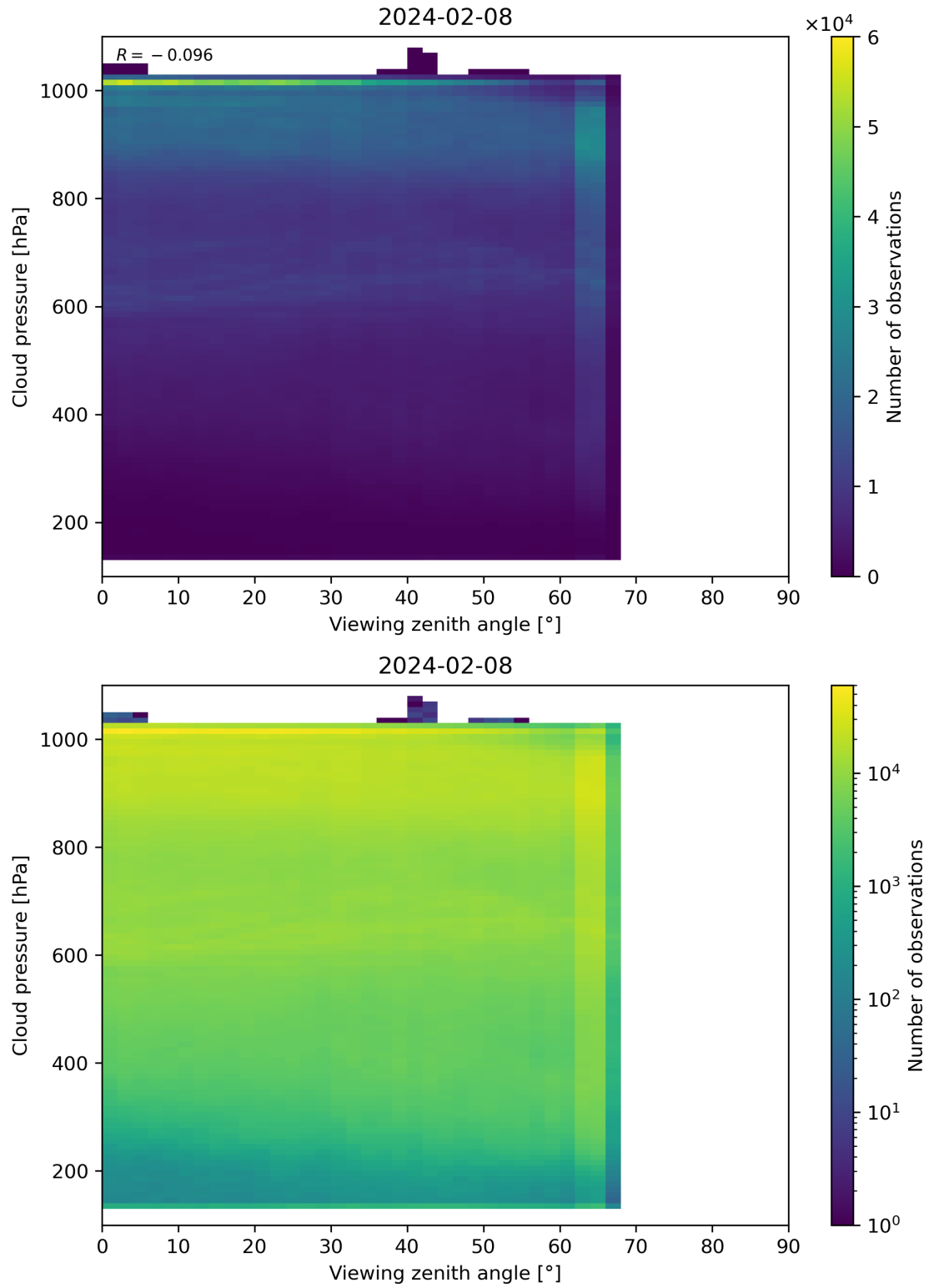
Figure 121: Scatter density plot of “Viewing zenith angle” against “Cloud pressure” for 2024-02-07 to 2024-02-09.
