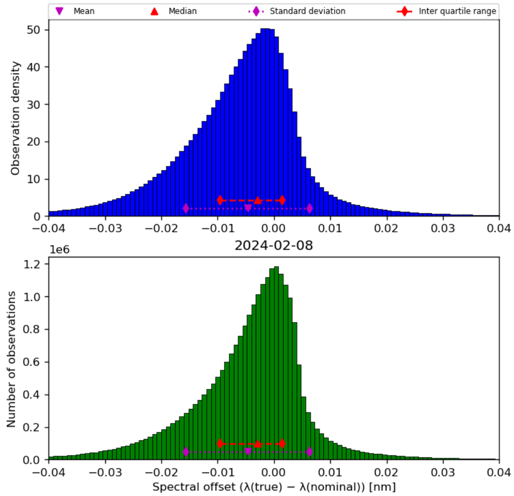
Figure 45: Histogram of “Spectral offset ( \lambda(\text{true}) - \lambda(\text{nominal}) )” for 2024-02-07 to 2024-02-09
