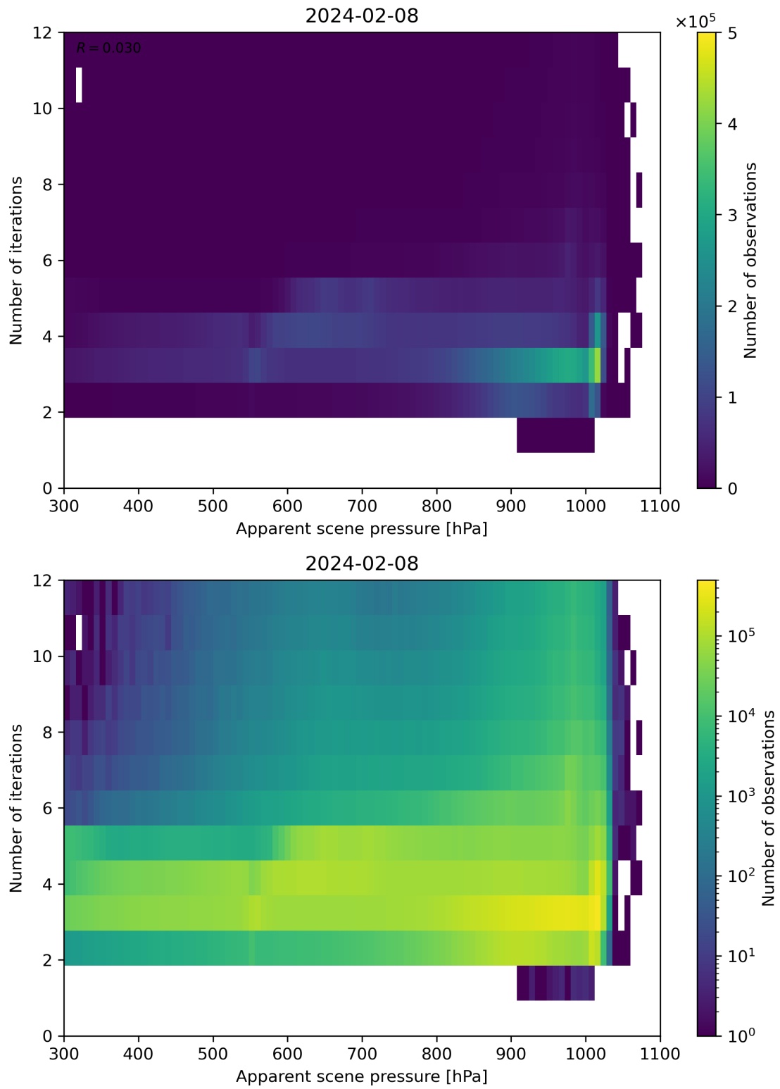
Figure 65: Scatter density plot of “Apparent scene pressure” against “Number of iterations” for 2024-02-07 to 2024-02-09.
