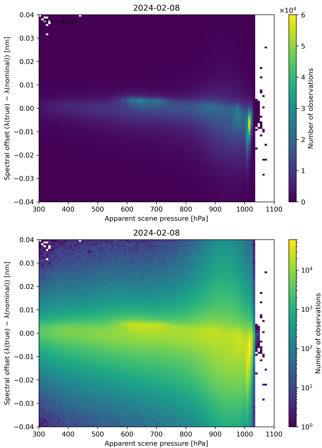
Figure 67: Scatter density plot of “Apparent scene pressure” against “Spectral offset ( \lambda(\text{true}) - \lambda(\text{nominal}) )” for 2024-02-07 to 2024-02-09.
