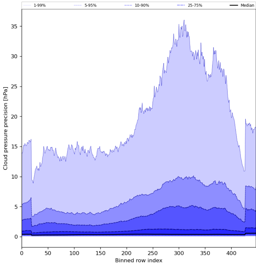
Figure 48: Along track statistics of “Cloud pressure precision” for 2024-02-07 to 2024-02-09
