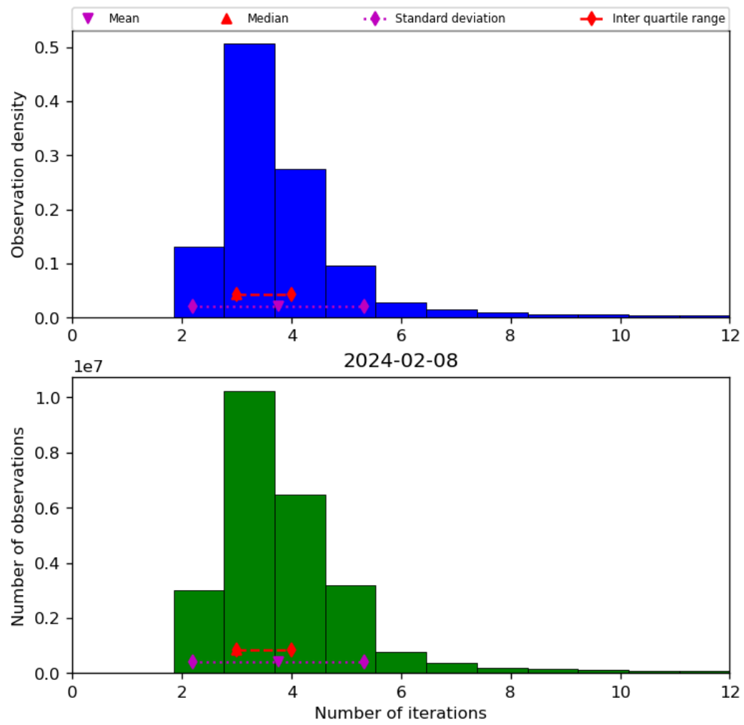
Figure 39: Histogram of “Number of iterations” for 2024-02-07 to 2024-02-09
