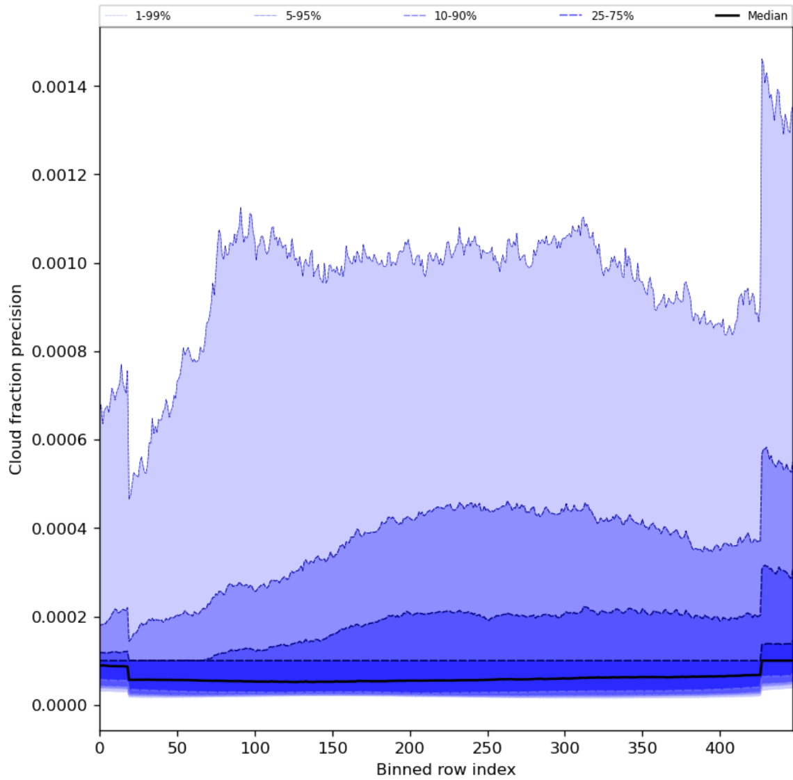
Figure 50: Along track statistics of “Cloud fraction precision” for 2024-02-07 to 2024-02-09
