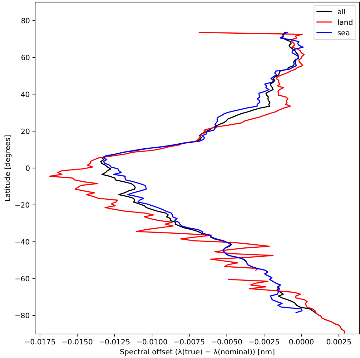
Figure 28: Zonal average of “Spectral offset ( \lambda(\text{true}) - \lambda(\text{nominal}) )” for 2024-02-07 to 2024-02-09.
