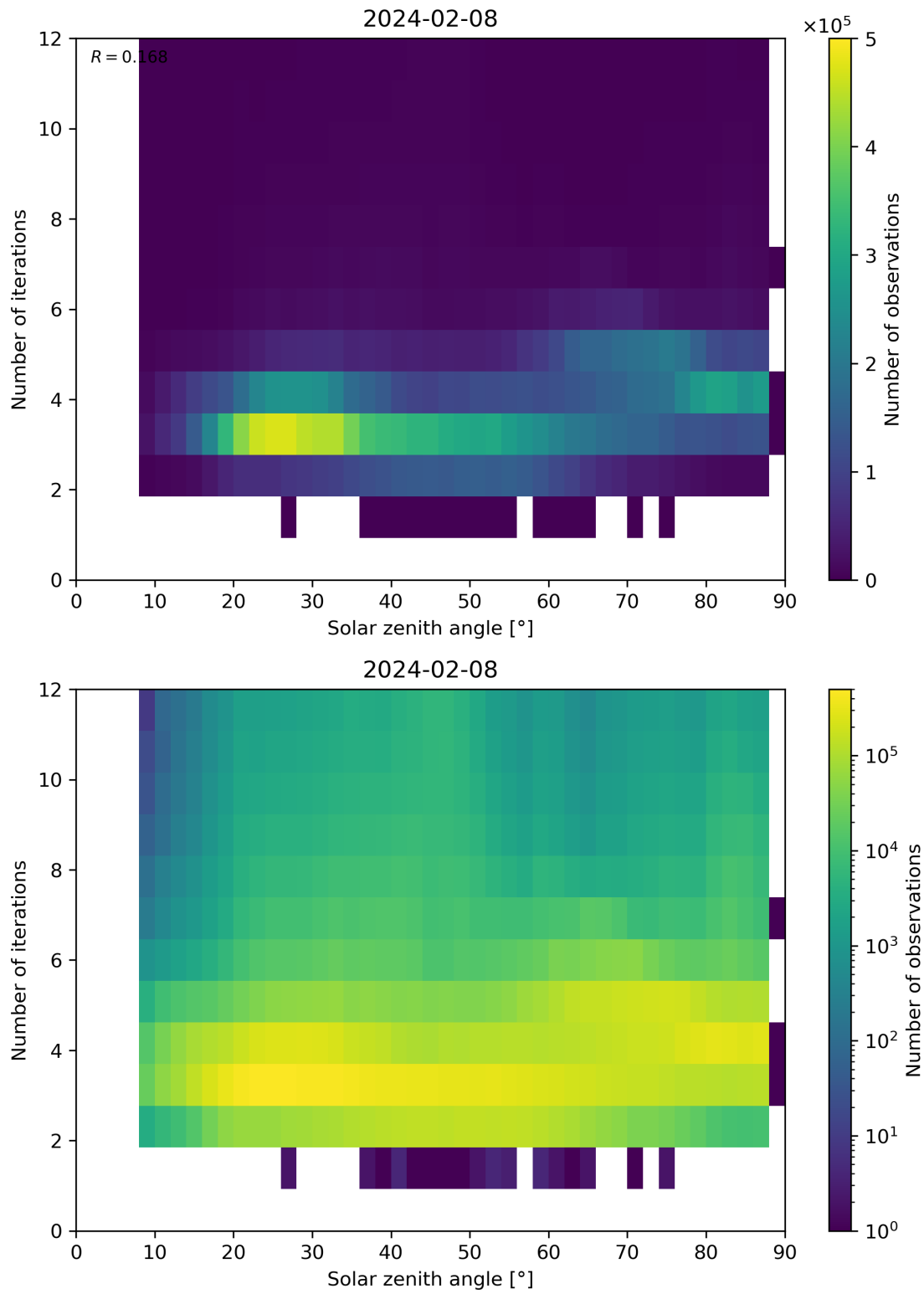
Figure 114: Scatter density plot of “Solar zenith angle” against “Number of iterations” for 2024-02-07 to 2024-02-09.
