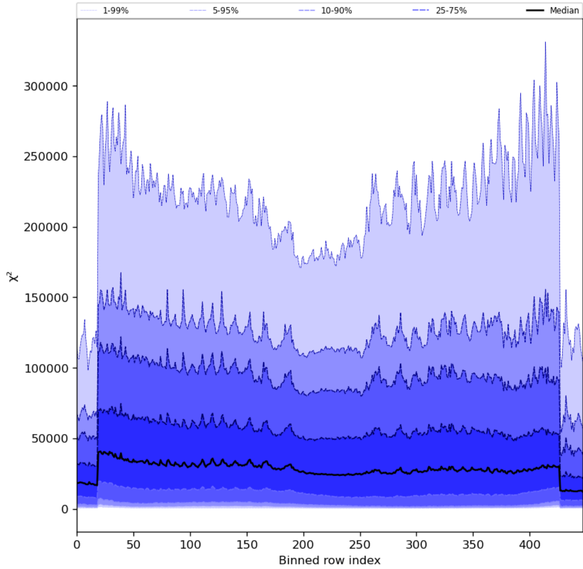
Figure 55: Along track statistics of “ \chi^2 ” for 2024-02-07 to 2024-02-09
