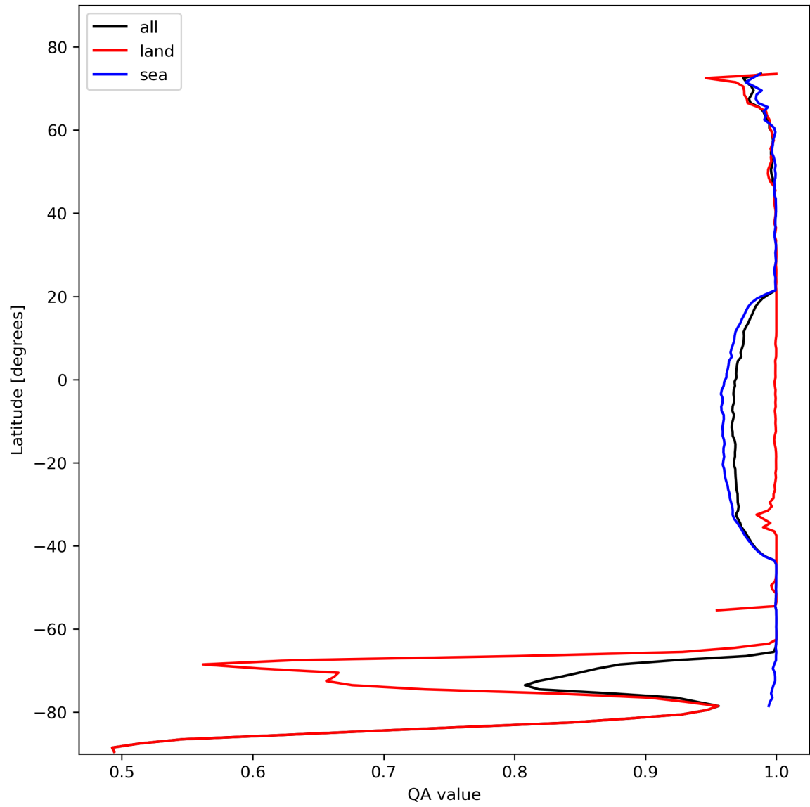
Figure 12: Zonal average of “QA value” for 2024-02-07 to 2024-02-09.
