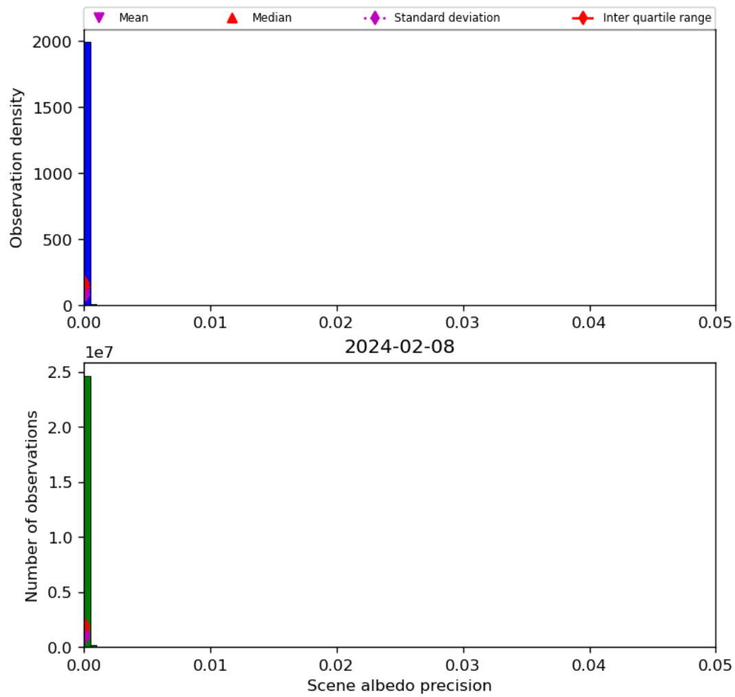
Figure 35: Histogram of “Scene albedo precision” for 2024-02-07 to 2024-02-09
