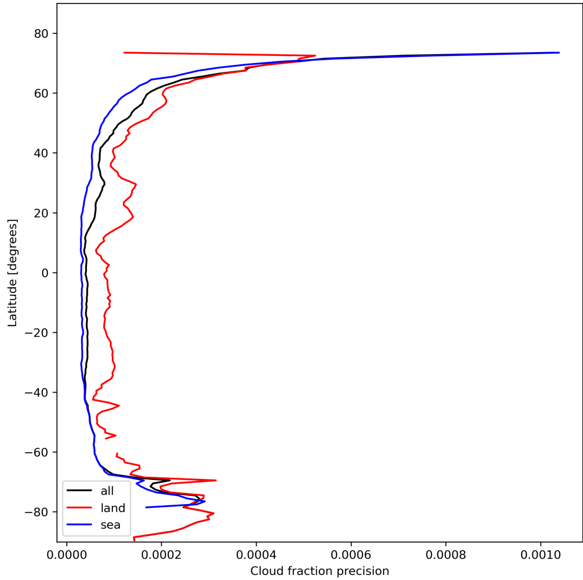
Figure 16: Zonal average of “Cloud fraction precision” for 2024-02-07 to 2024-02-09.
