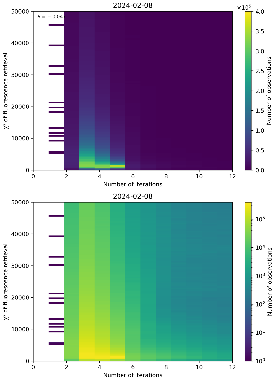
Figure 97: Scatter density plot of “Number of iterations” against “ \chi^2 of fluorescence retrieval” for 2024-02-07 to 2024-02-09.
