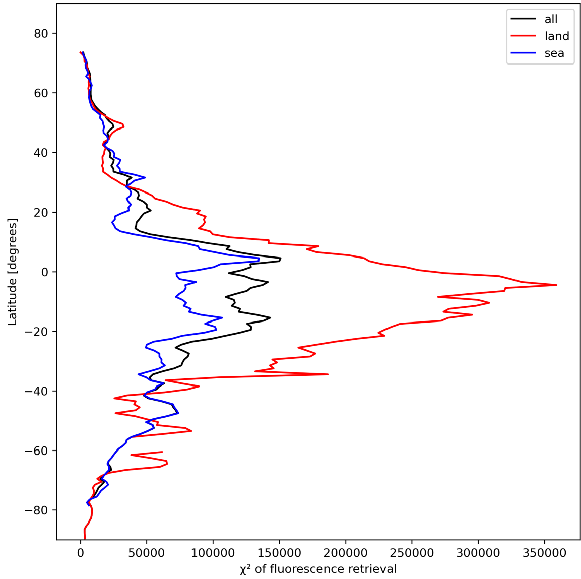
Figure 25: Zonal average of “ \chi^2 of fluorescence retrieval” for 2024-02-07 to 2024-02-09.
