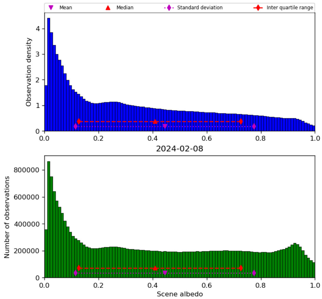
Figure 34: Histogram of “Scene albedo” for 2024-02-07 to 2024-02-09
