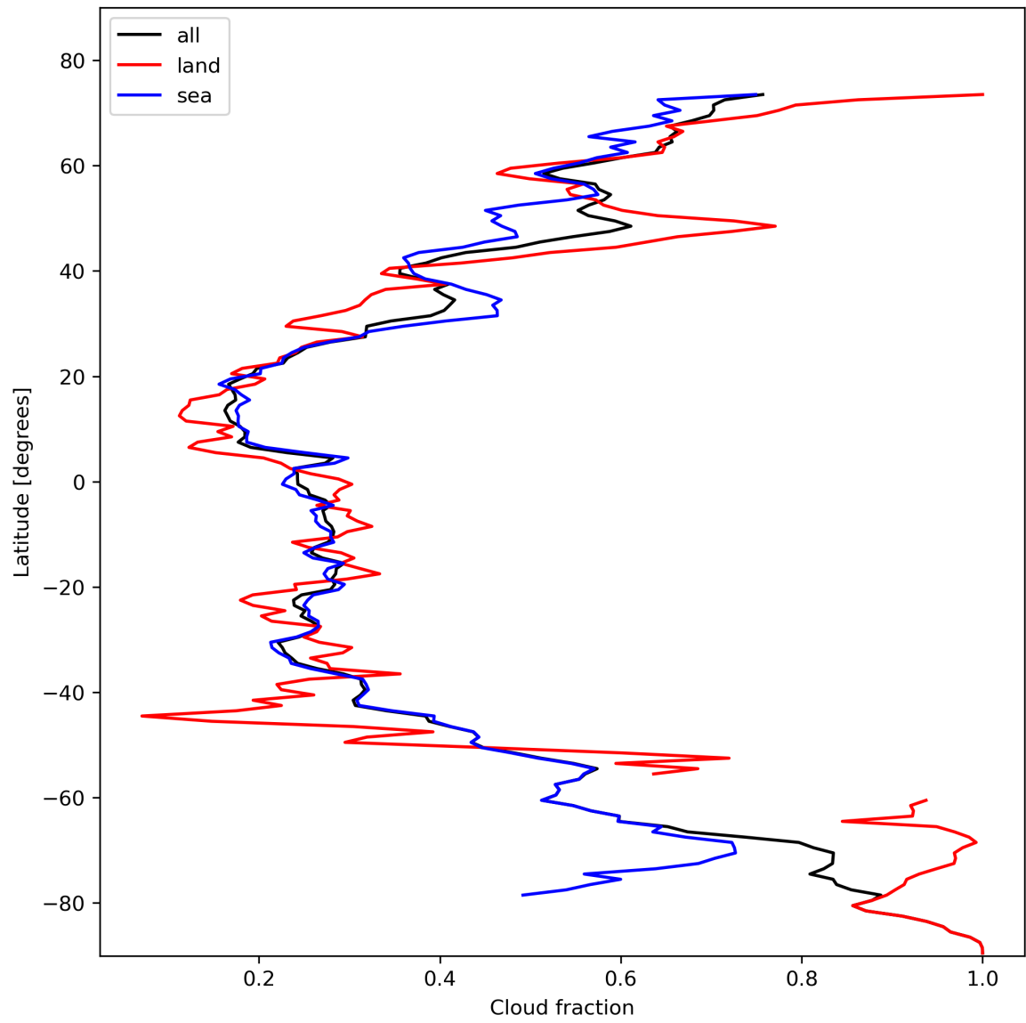
Figure 15: Zonal average of “Cloud fraction” for 2024-02-07 to 2024-02-09.
