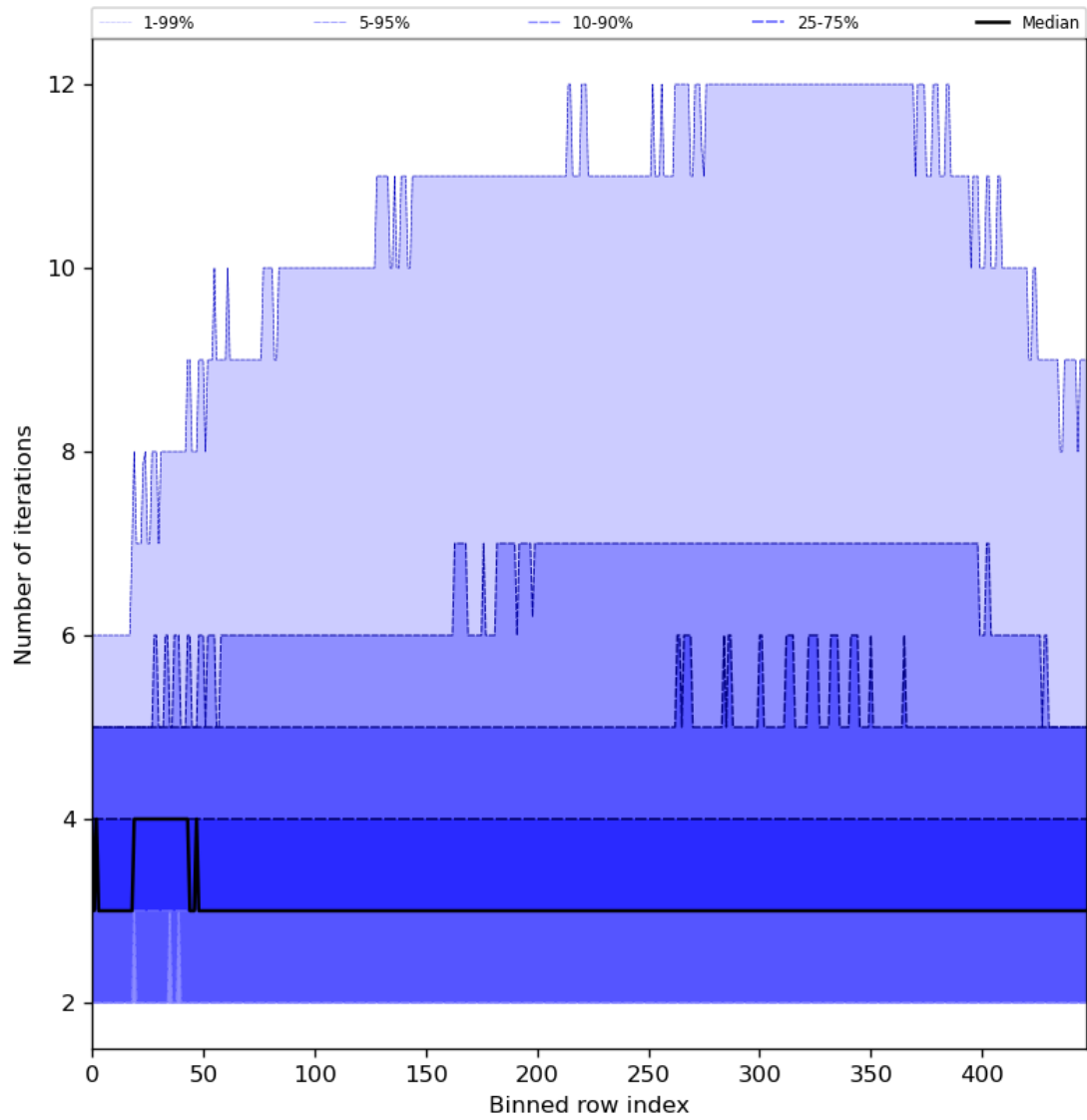
Figure 56: Along track statistics of “Number of iterations” for 2024-02-07 to 2024-02-09
