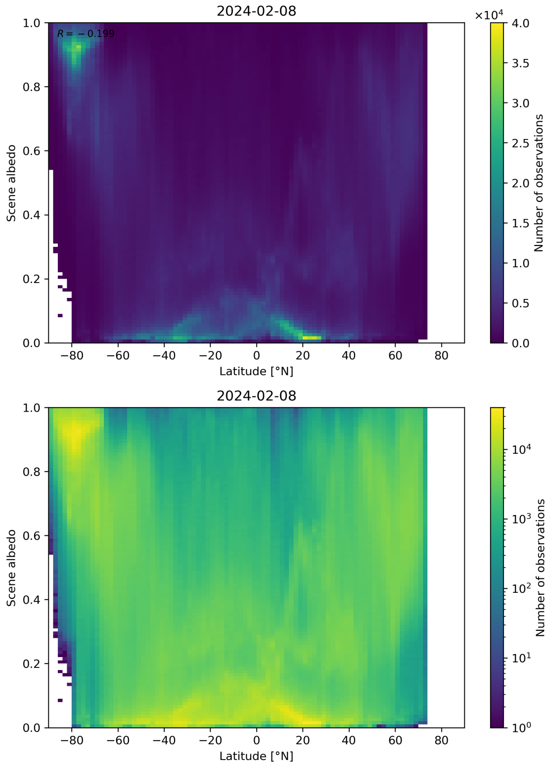
Figure 95: Scatter density plot of “Latitude” against “Scene albedo” for 2024-02-07 to 2024-02-09.
