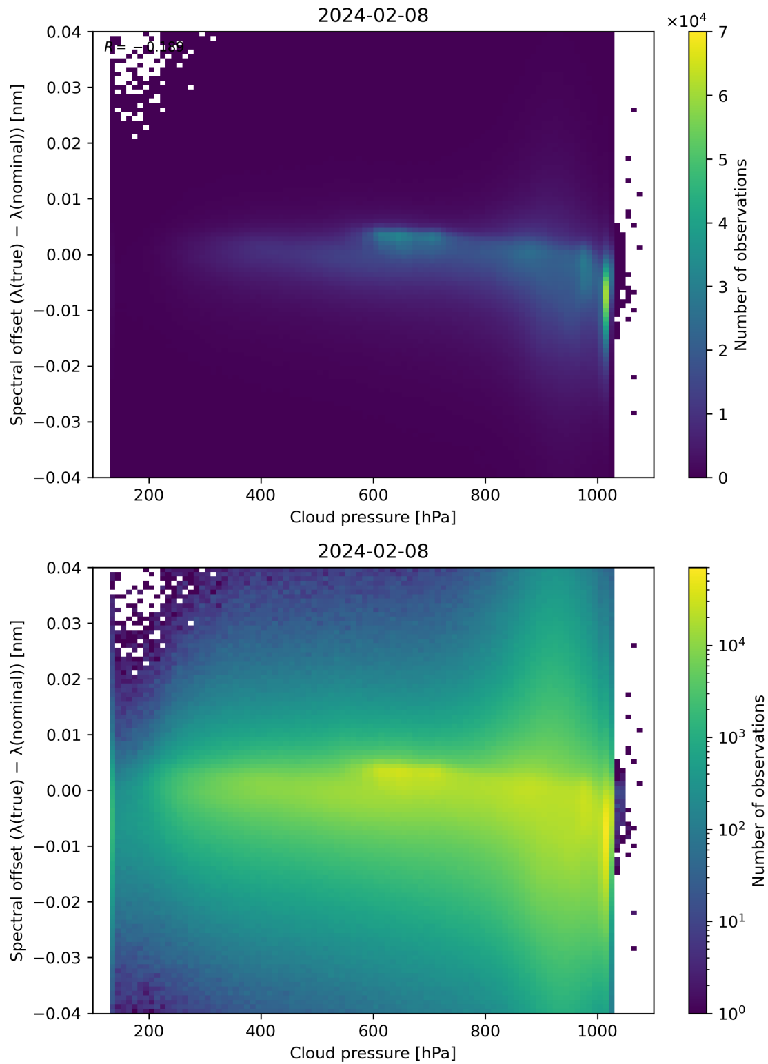
Figure 84: Scatter density plot of “Cloud pressure” against “Spectral offset ( \lambda(\text{true}) - \lambda(\text{nominal}) )” for 2024-02-07 to 2024-02-09.
