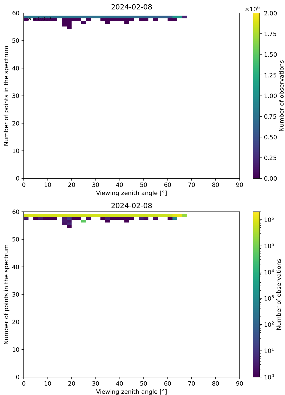
Figure 125: Scatter density plot of “Viewing zenith angle” against “Number of points in the spectrum” for 2024-02-07 to 2024-02-09.
