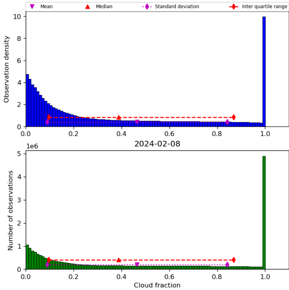
Figure 32: Histogram of “Cloud fraction” for 2024-02-07 to 2024-02-09
