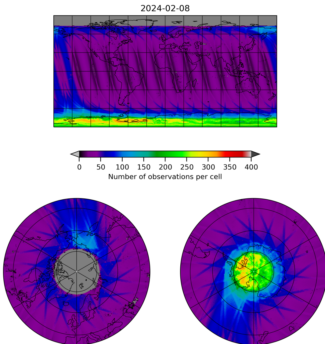
Figure 11: Map of the number of observations for 2024-02-07 to 2024-02-09
