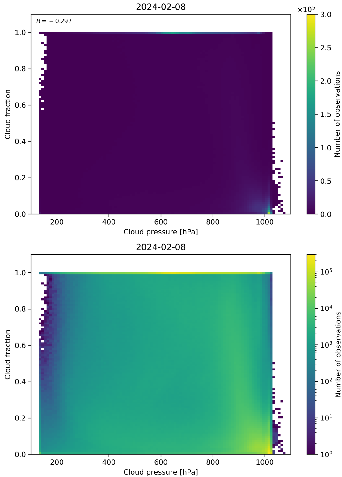
Figure 79: Scatter density plot of “Cloud pressure” against “Cloud fraction” for 2024-02-07 to 2024-02-09.
