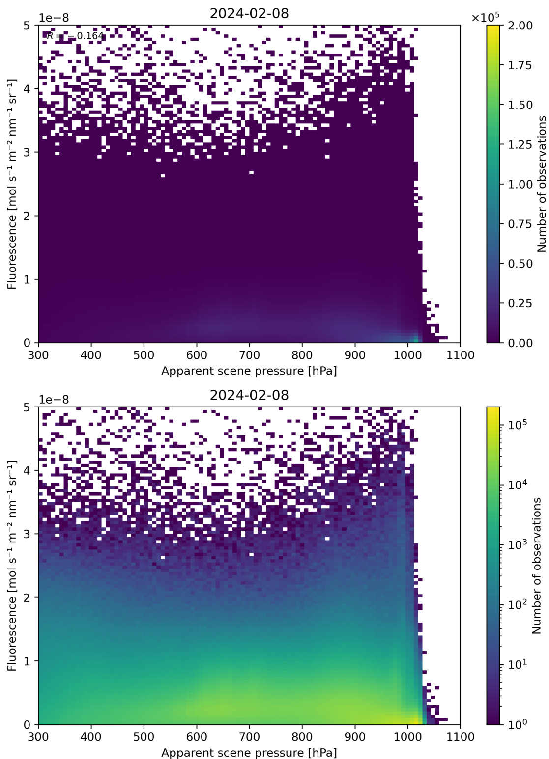
Figure 64: Scatter density plot of “Apparent scene pressure” against “Fluorescence” for 2024-02-07 to 2024-02-09.
