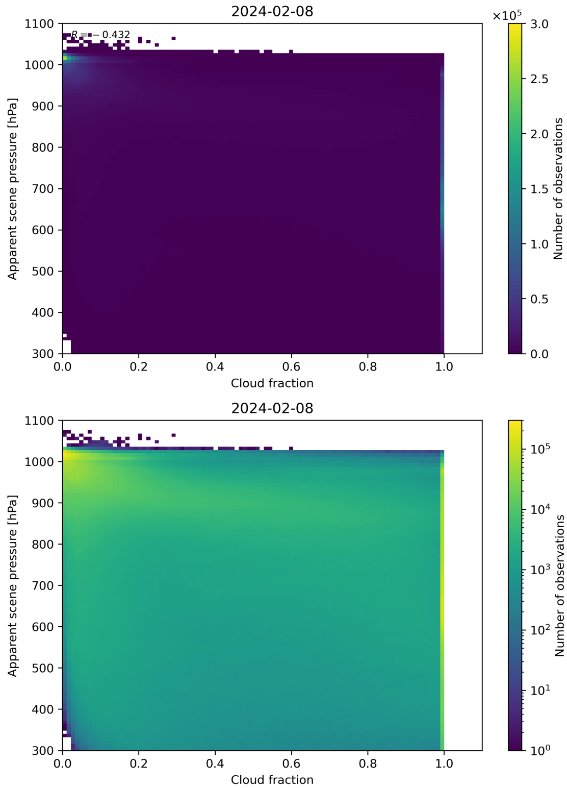
Figure 70: Scatter density plot of “Cloud fraction” against “Apparent scene pressure” for 2024-02-07 to 2024-02-09.
