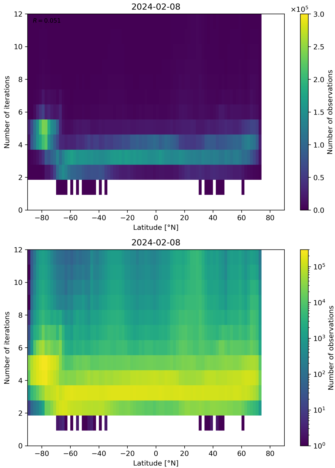
Figure 93: Scatter density plot of “Latitude” against “Number of iterations” for 2024-02-07 to 2024-02-09.
