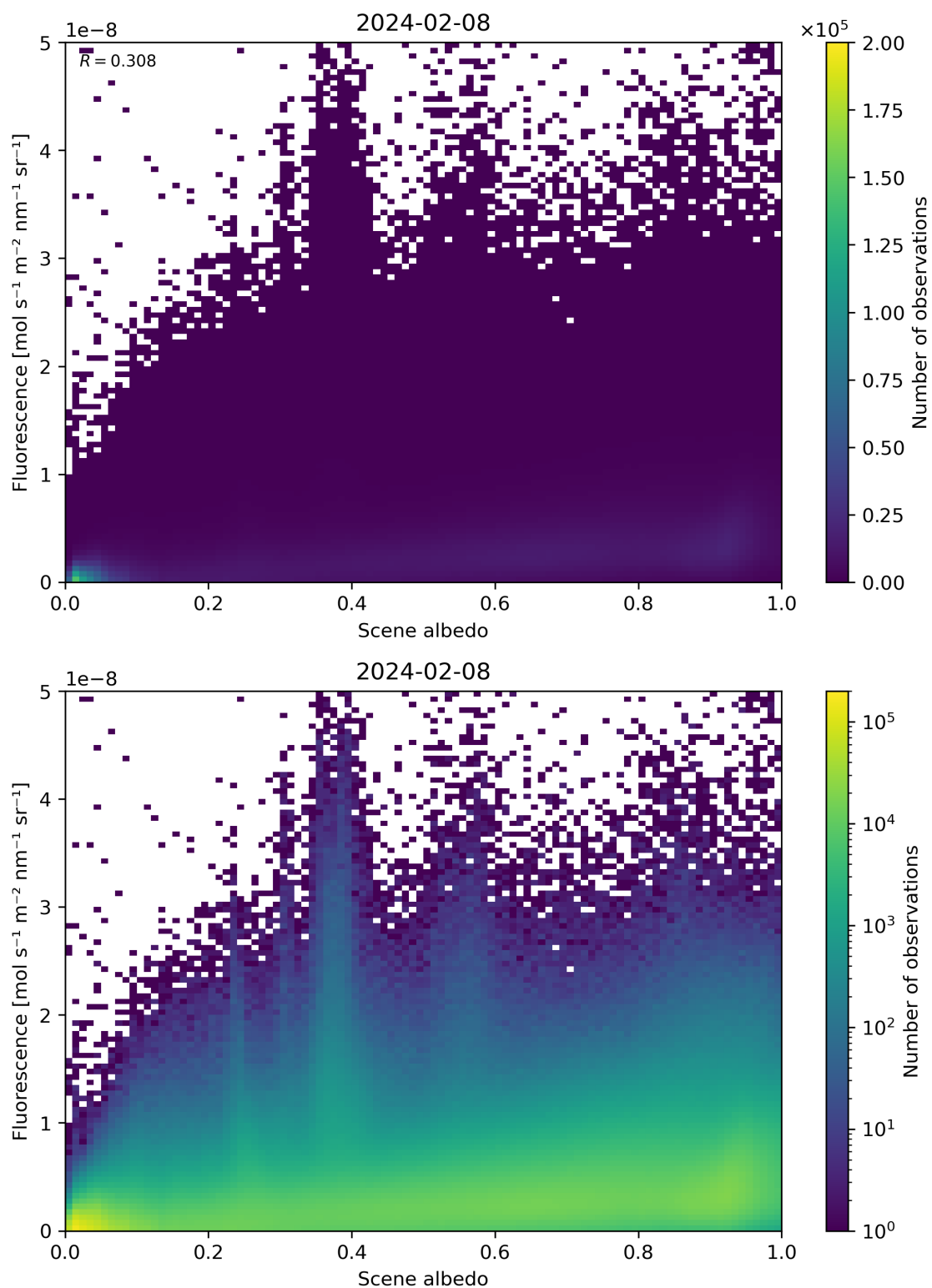
Figure 104: Scatter density plot of “Scene albedo” against “Fluorescence” for 2024-02-07 to 2024-02-09.
