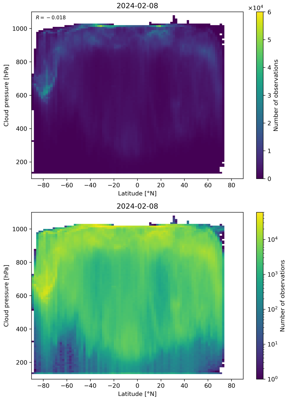
Figure 91: Scatter density plot of “Latitude” against “Cloud pressure” for 2024-02-07 to 2024-02-09.
