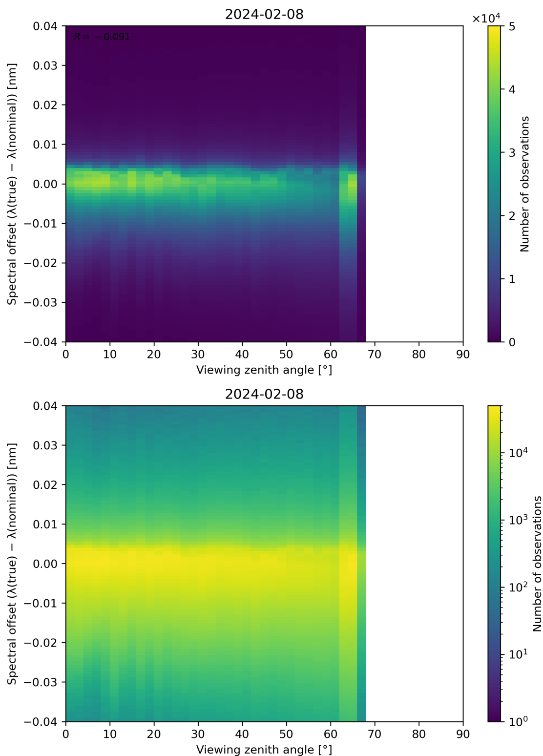
Figure 128: Scatter density plot of “Viewing zenith angle” against “Spectral offset ( \lambda(\text{true}) - \lambda(\text{nominal}) )” for 2024-02-07 to 2024-02-09.
