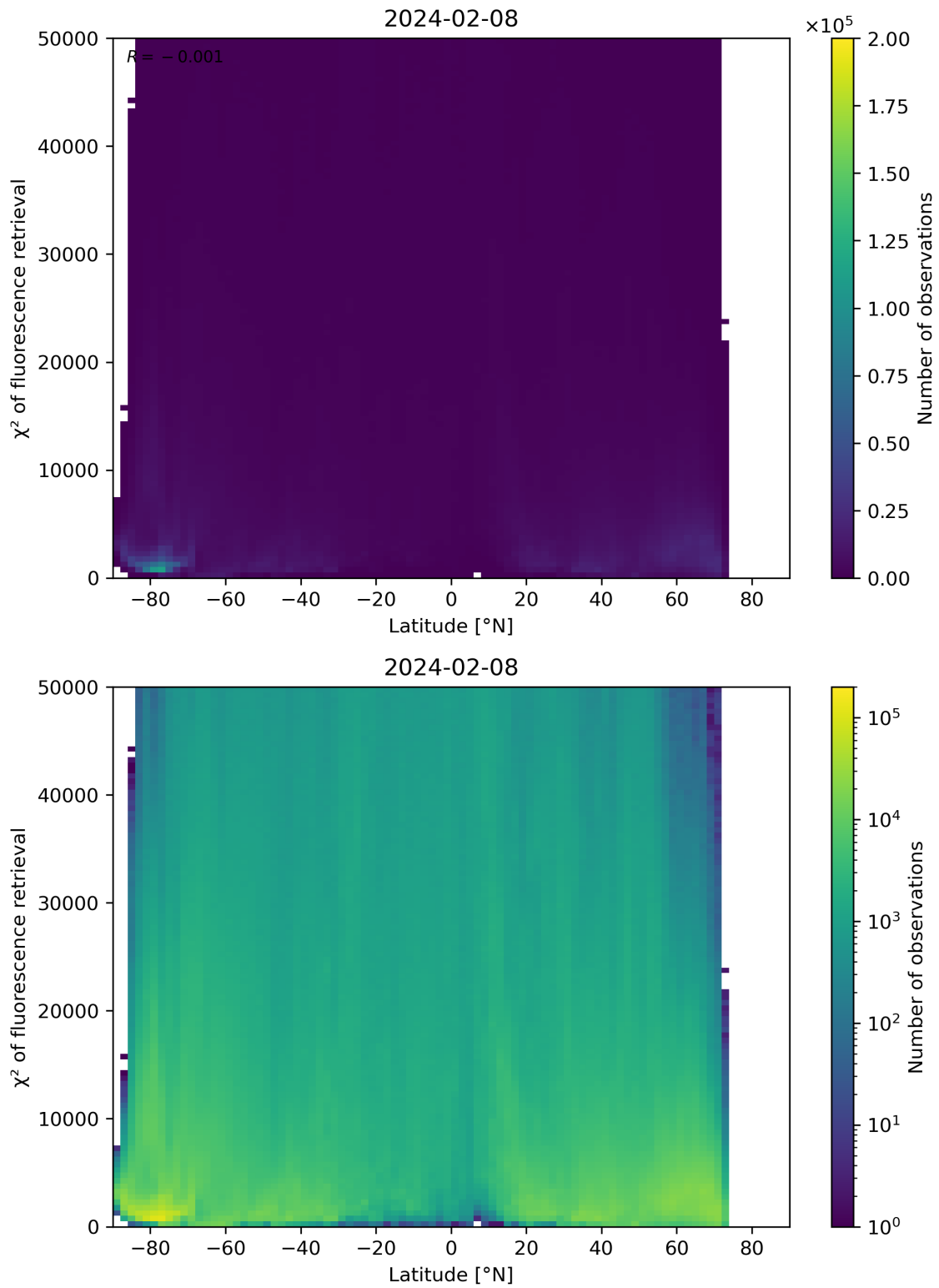
Figure 89: Scatter density plot of “Latitude” against “ \chi^2 of fluorescence retrieval” for 2024-02-07 to 2024-02-09.
