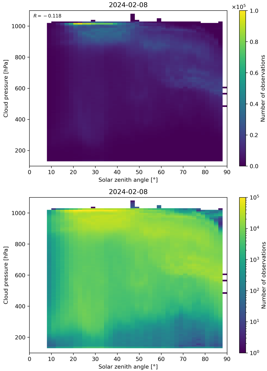
Figure 111: Scatter density plot of “Solar zenith angle” against “Cloud pressure” for 2024-02-07 to 2024-02-09.
