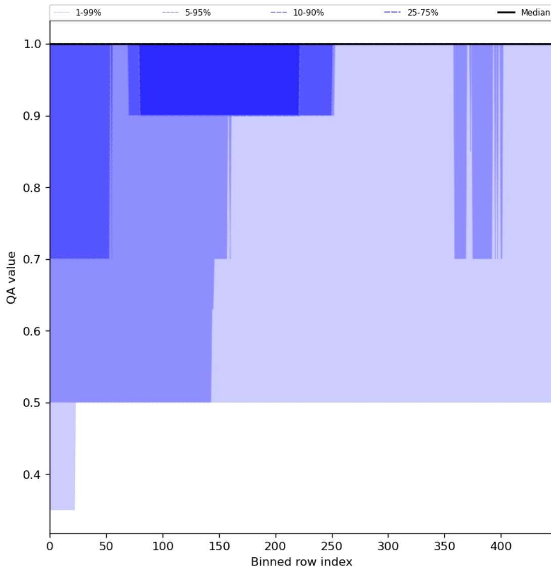
Figure 46: Along track statistics of “QA value” for 2024-02-07 to 2024-02-09
