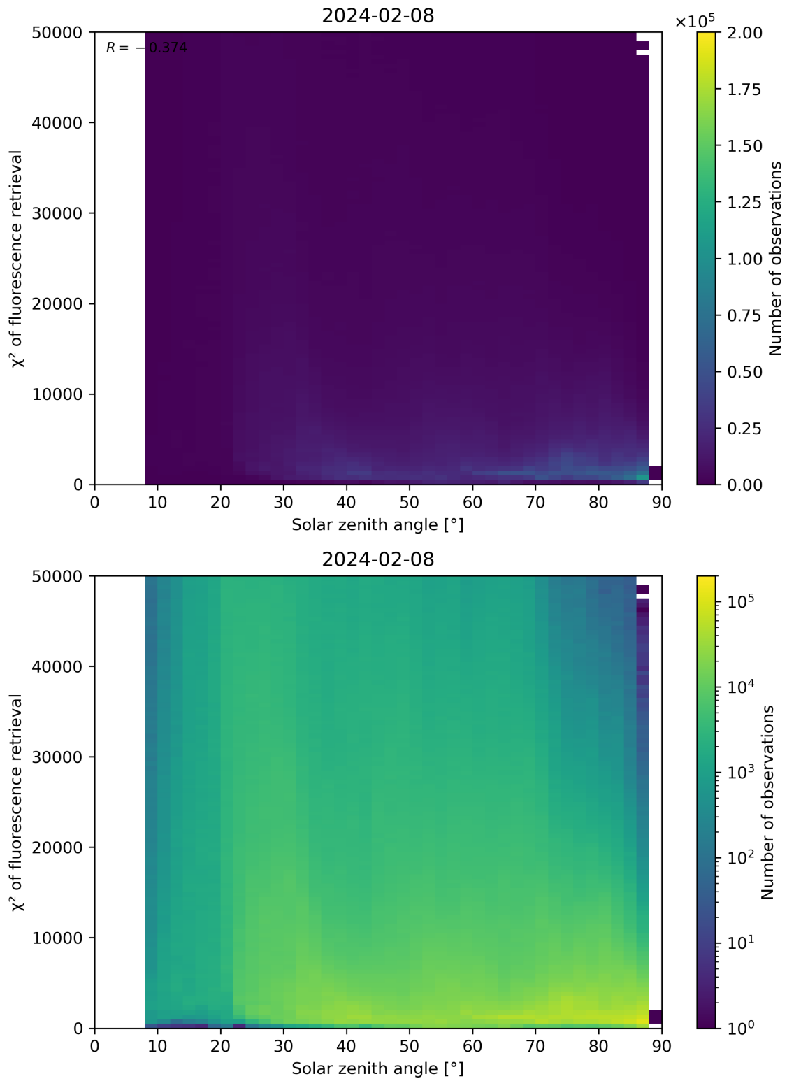
Figure 109: Scatter density plot of “Solar zenith angle” against “ \chi^2 of fluorescence retrieval” for 2024-02-07 to 2024-02-09.
