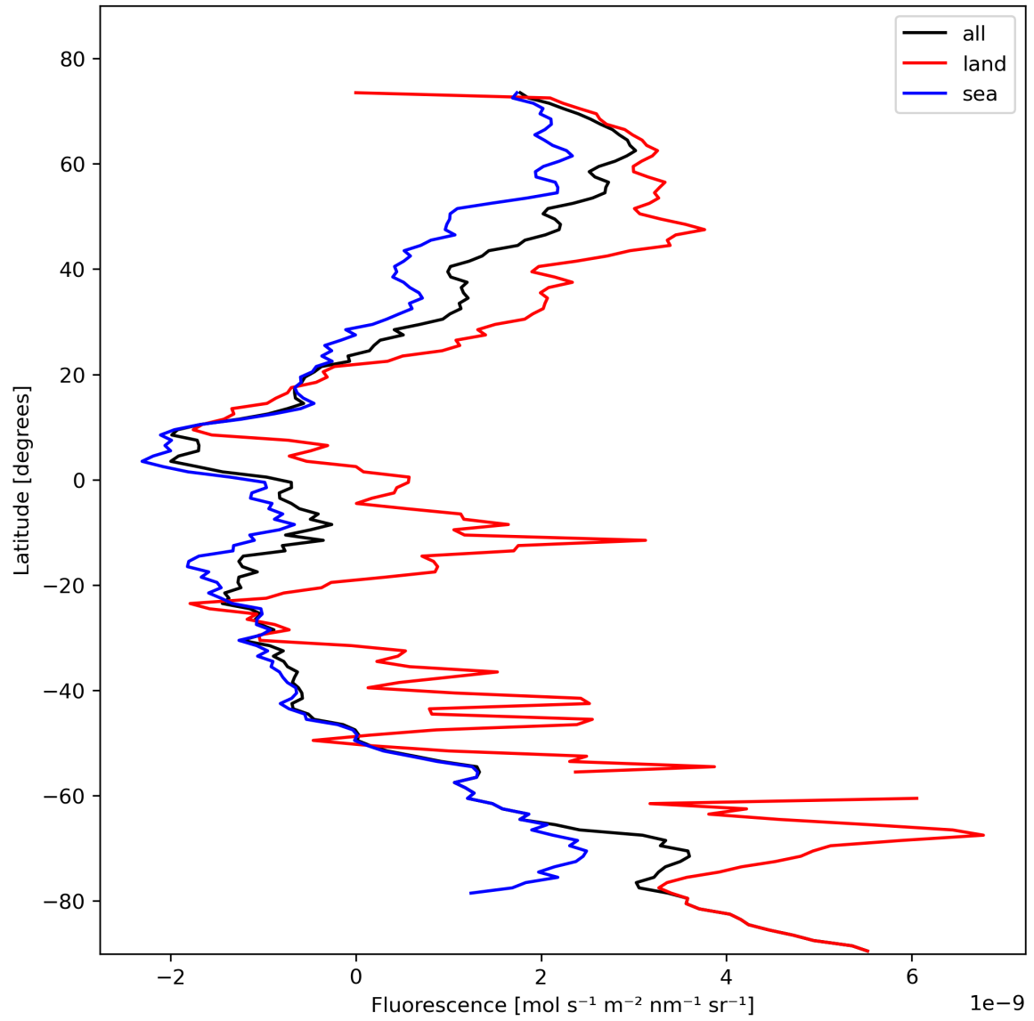
Figure 23: Zonal average of “Fluorescence” for 2024-02-07 to 2024-02-09.
