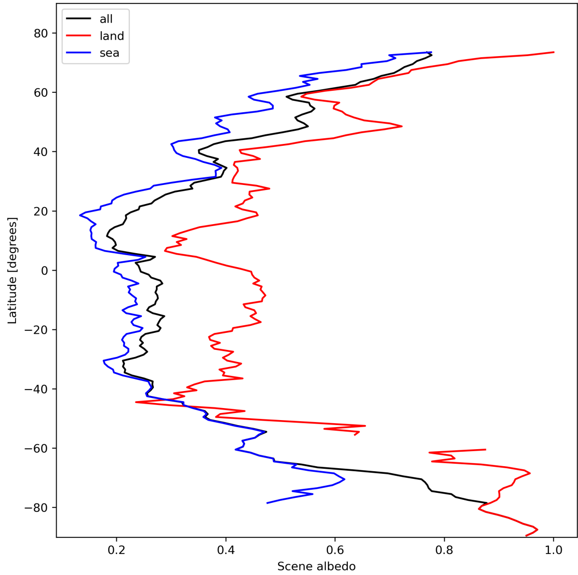
Figure 17: Zonal average of “Scene albedo” for 2024-02-07 to 2024-02-09.
