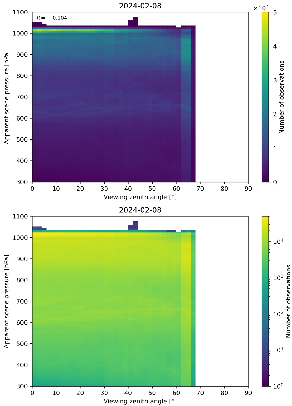
Figure 118: Scatter density plot of “Viewing zenith angle” against “Apparent scene pressure” for 2024-02-07 to 2024-02-09.
