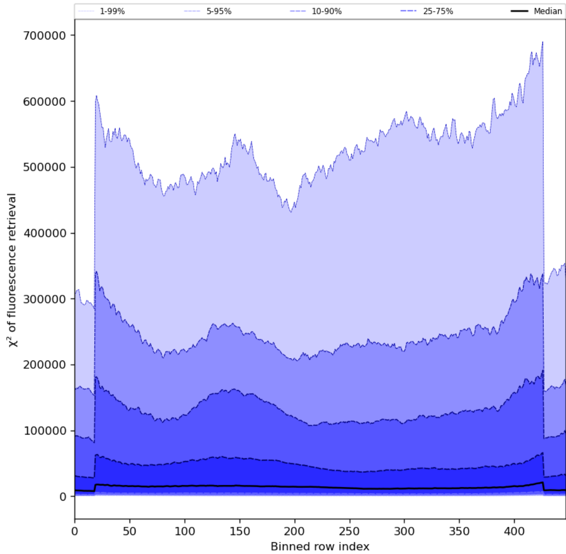
Figure 59: Along track statistics of “ \chi^2 of fluorescence retrieval” for 2024-02-07 to 2024-02-09
