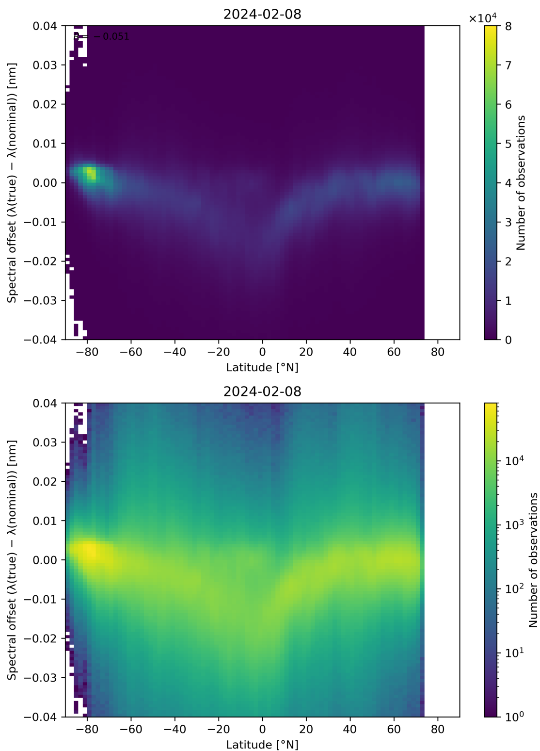
Figure 96: Scatter density plot of “Latitude” against “Spectral offset ( \lambda(\text{true}) - \lambda(\text{nominal}) )” for 2024-02-07 to 2024-02-09.
