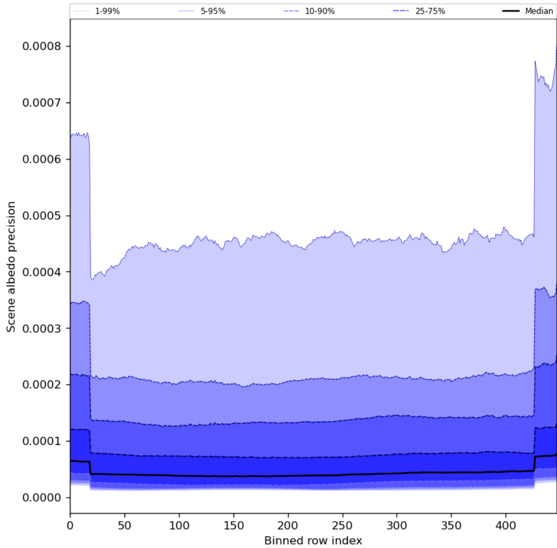
Figure 52: Along track statistics of “Scene albedo precision” for 2024-02-07 to 2024-02-09
