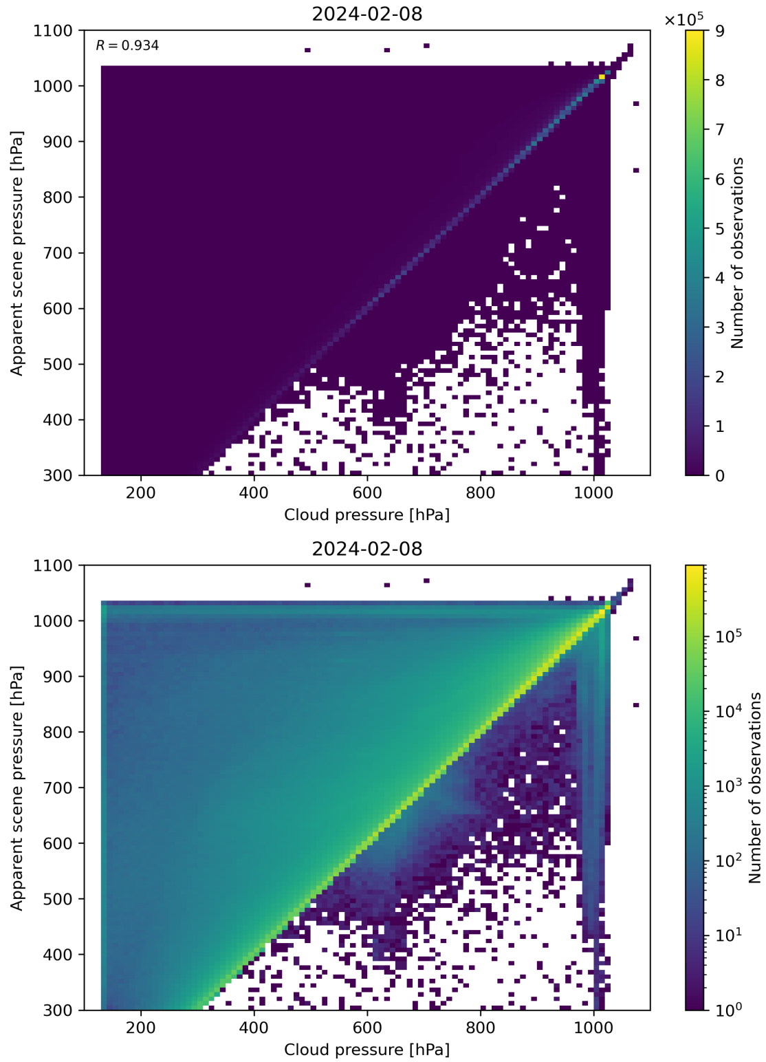
Figure 77: Scatter density plot of “Cloud pressure” against “Apparent scene pressure” for 2024-02-07 to 2024-02-09.
