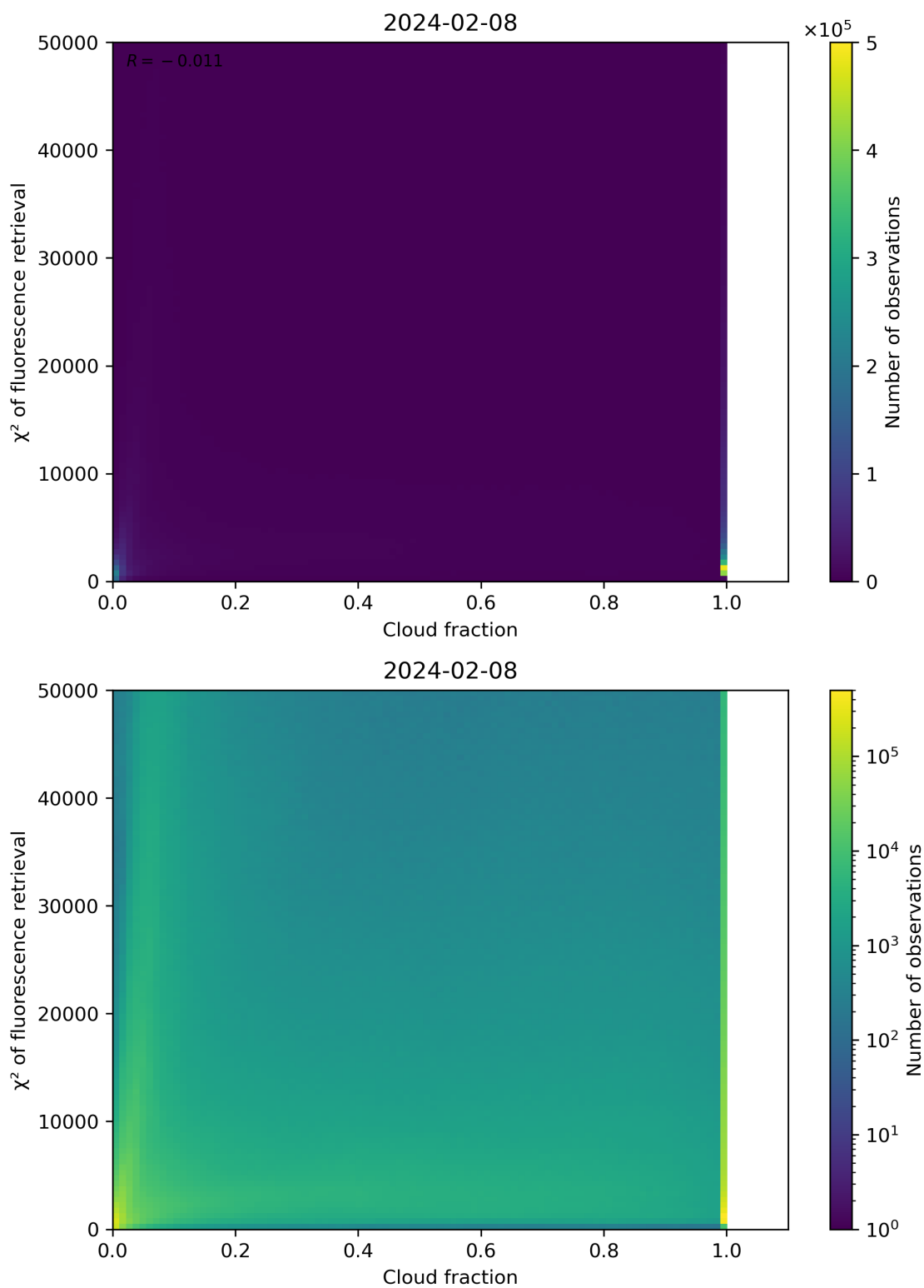
Figure 71: Scatter density plot of “Cloud fraction” against “ \chi^2 of fluorescence retrieval” for 2024-02-07 to 2024-02-09.
