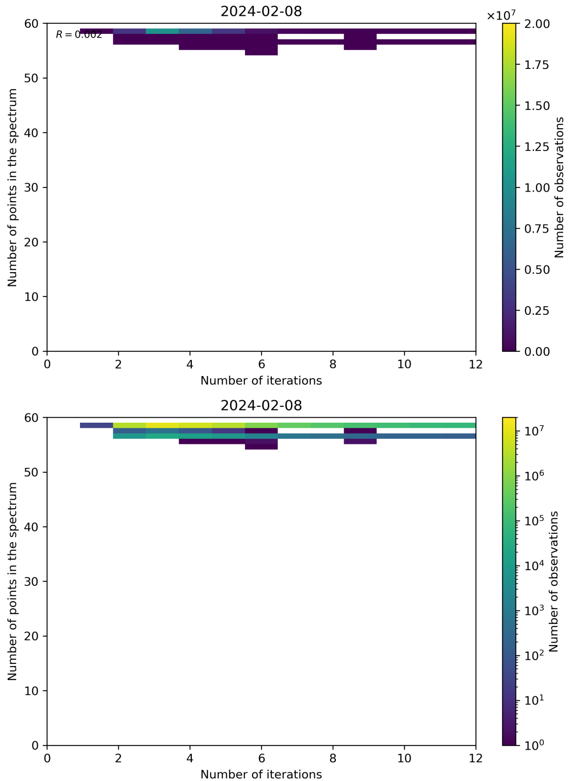
Figure 99: Scatter density plot of “Number of iterations” against “Number of points in the spectrum” for 2024-02-07 to 2024-02-09.
