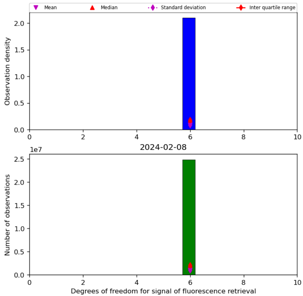
Figure 43: Histogram of “Degrees of freedom for signal of fluorescence retrieval” for 2024-02-07 to 2024-02-09
