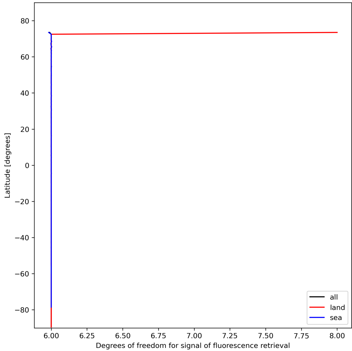
Figure 26: Zonal average of “Degrees of freedom for signal of fluorescence retrieval” for 2024-02-07 to 2024-02-09.
