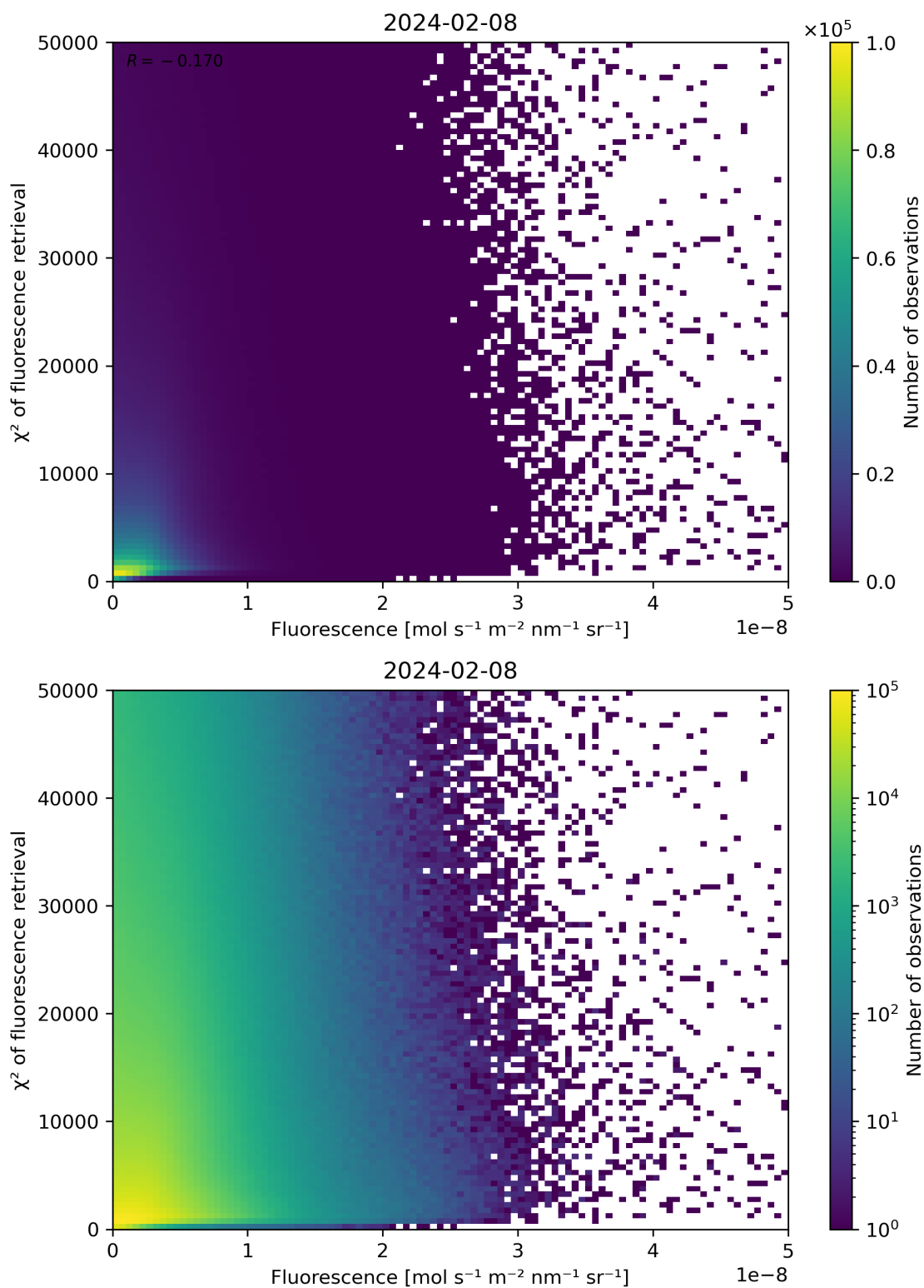
Figure 85: Scatter density plot of “Fluorescence” against “ \chi^2 of fluorescence retrieval” for 2024-02-07 to 2024-02-09.
