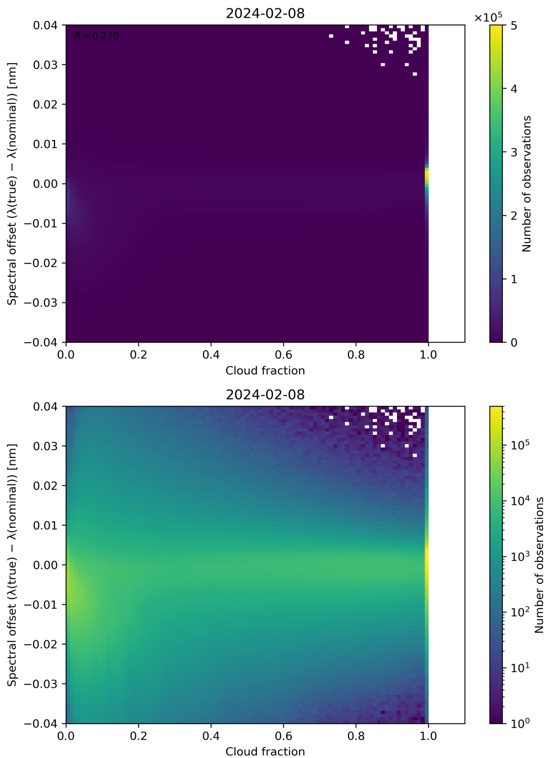
Figure 76: Scatter density plot of “Cloud fraction” against “Spectral offset ( \lambda(\text{true}) - \lambda(\text{nominal}) )” for 2024-02-07 to 2024-02-09.
