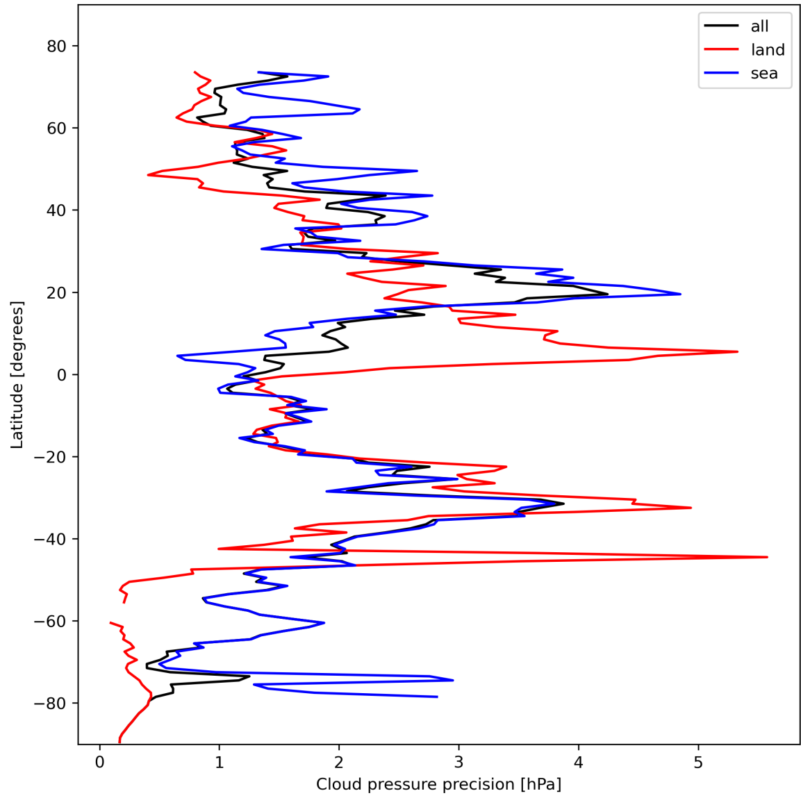
Figure 14: Zonal average of “Cloud pressure precision” for 2024-02-07 to 2024-02-09.
