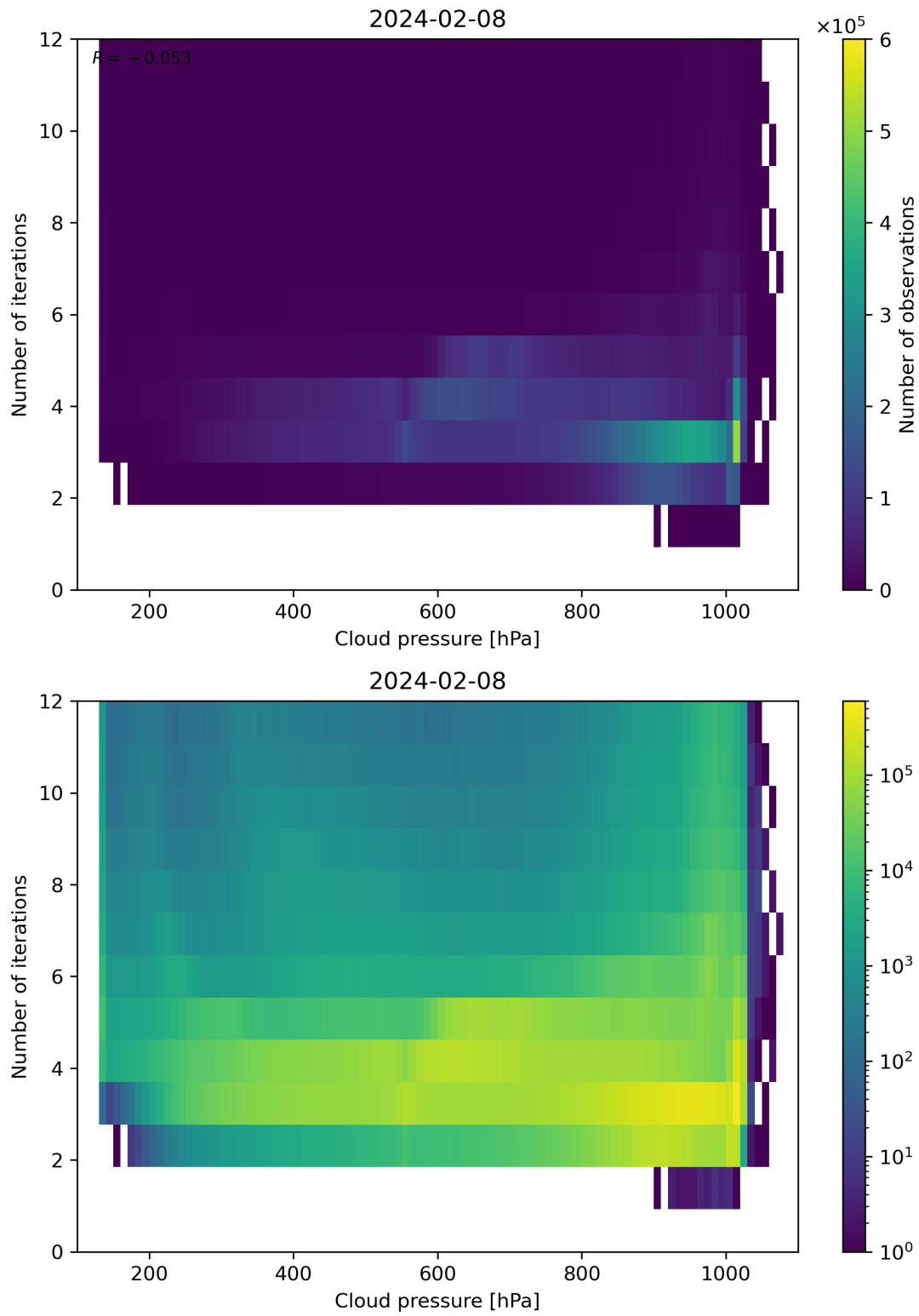
Figure 81: Scatter density plot of “Cloud pressure” against “Number of iterations” for 2024-02-07 to 2024-02-09.
