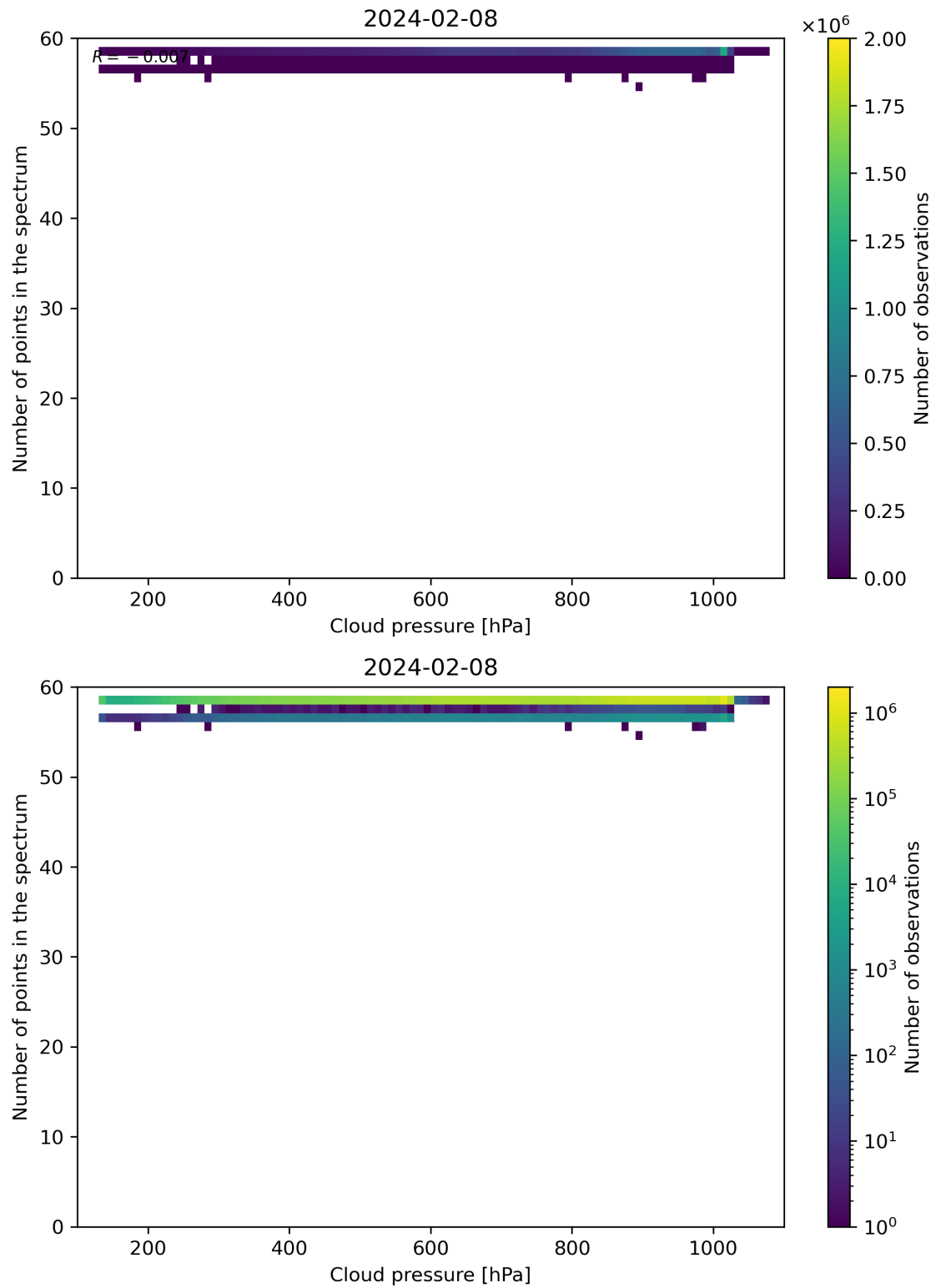
Figure 82: Scatter density plot of “Cloud pressure” against “Number of points in the spectrum” for 2024-02-07 to 2024-02-09.
