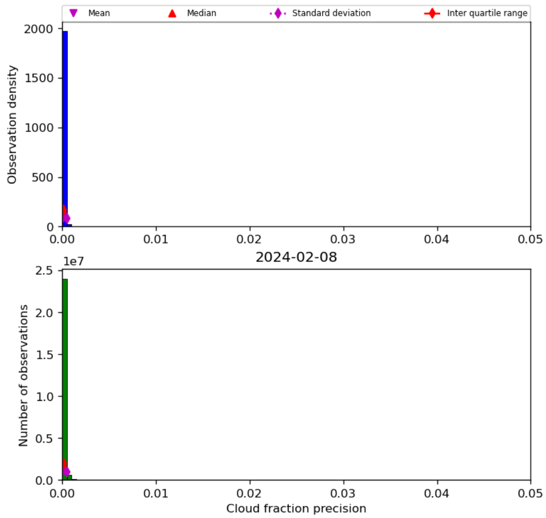
Figure 33: Histogram of “Cloud fraction precision” for 2024-02-07 to 2024-02-09
