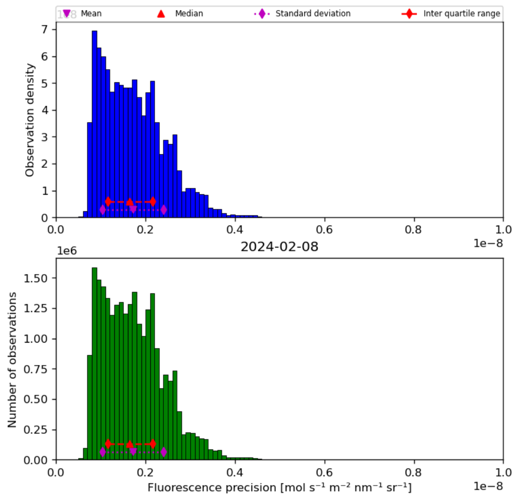
Figure 41: Histogram of “Fluorescence precision” for 2024-02-07 to 2024-02-09
