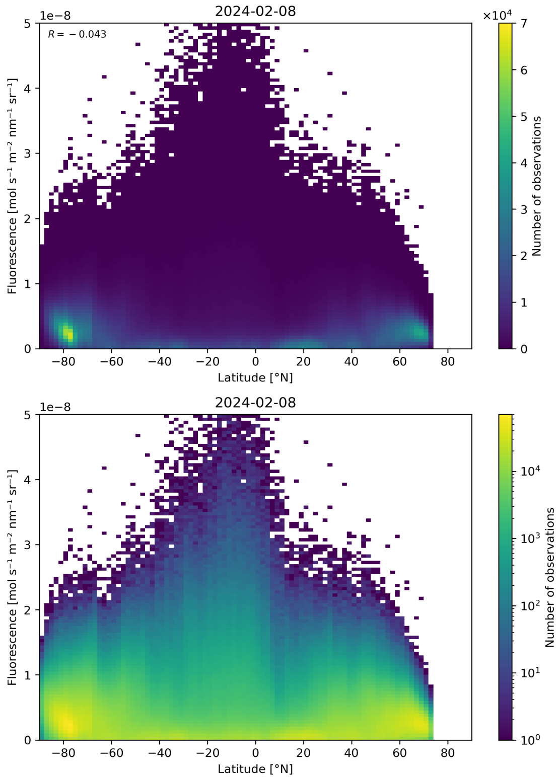
Figure 92: Scatter density plot of “Latitude” against “Fluorescence” for 2024-02-07 to 2024-02-09.
