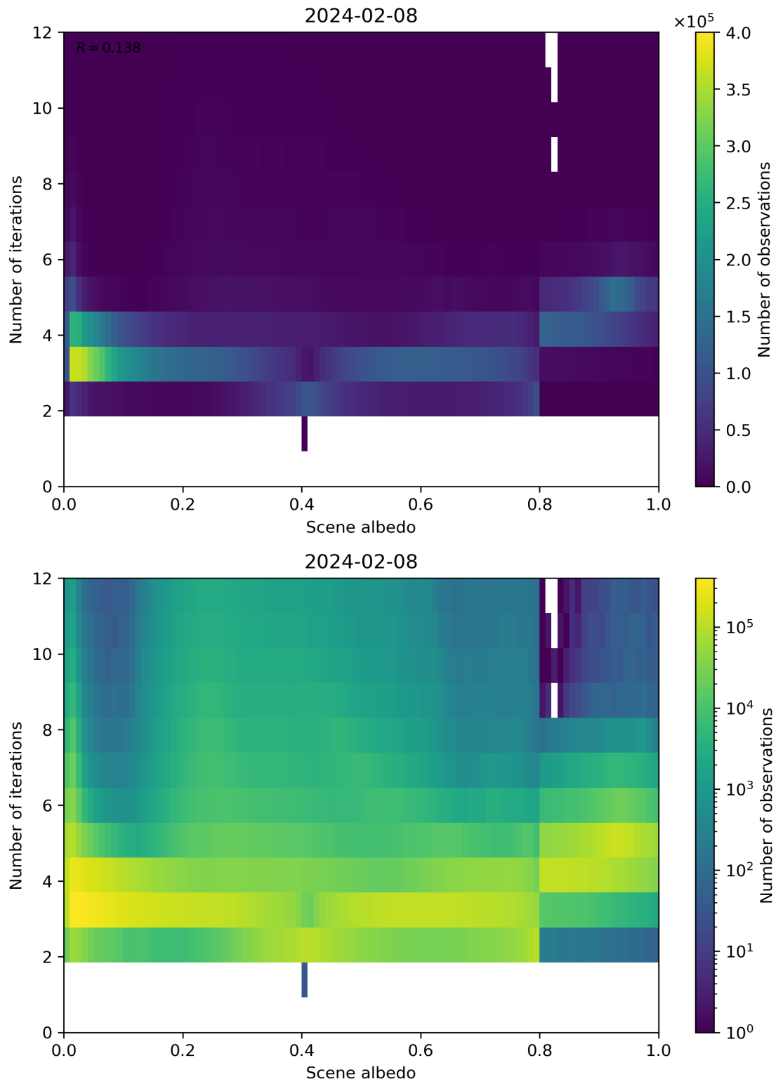
Figure 105: Scatter density plot of “Scene albedo” against “Number of iterations” for 2024-02-07 to 2024-02-09.
