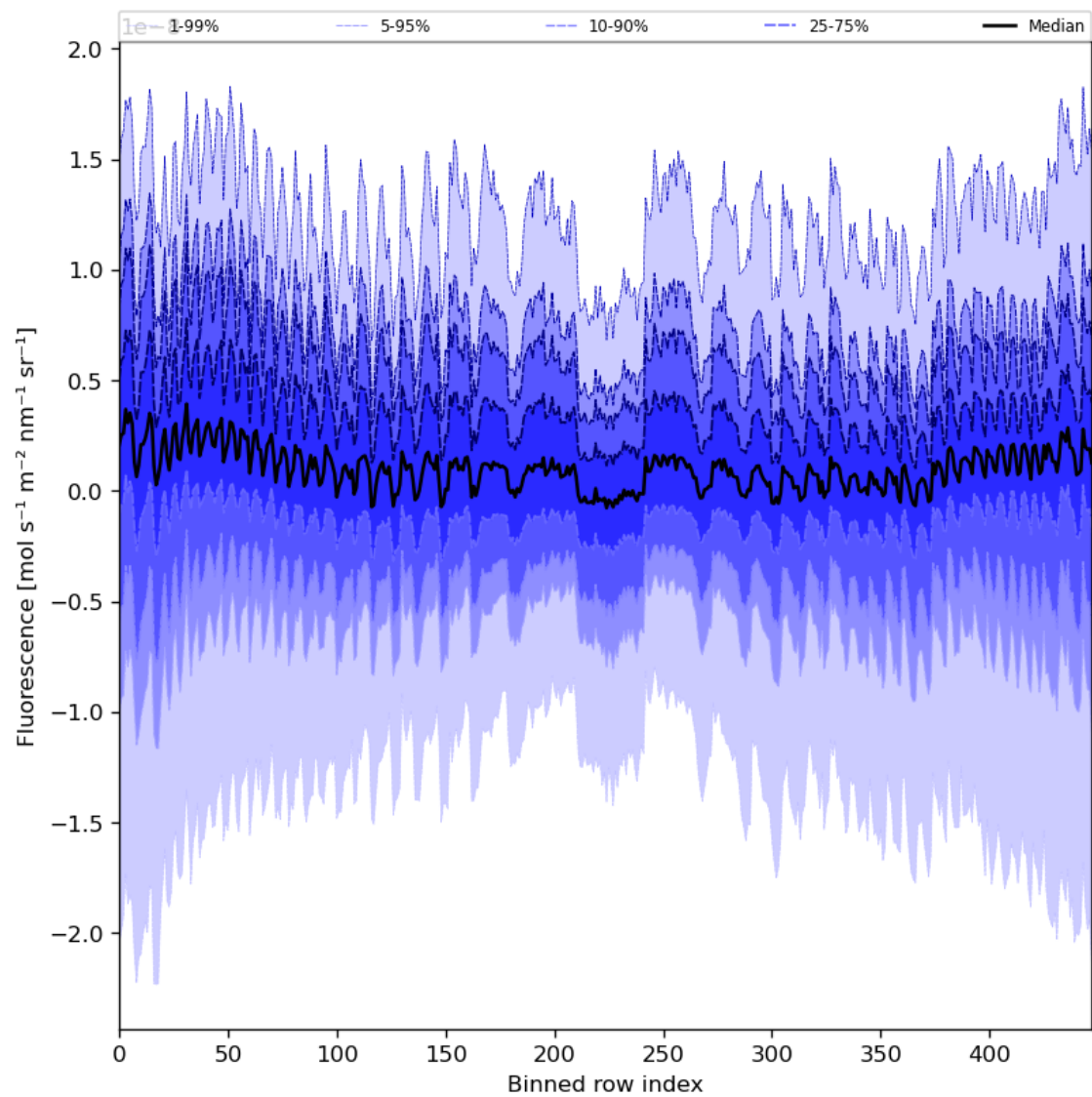
Figure 57: Along track statistics of “Fluorescence” for 2024-02-07 to 2024-02-09
