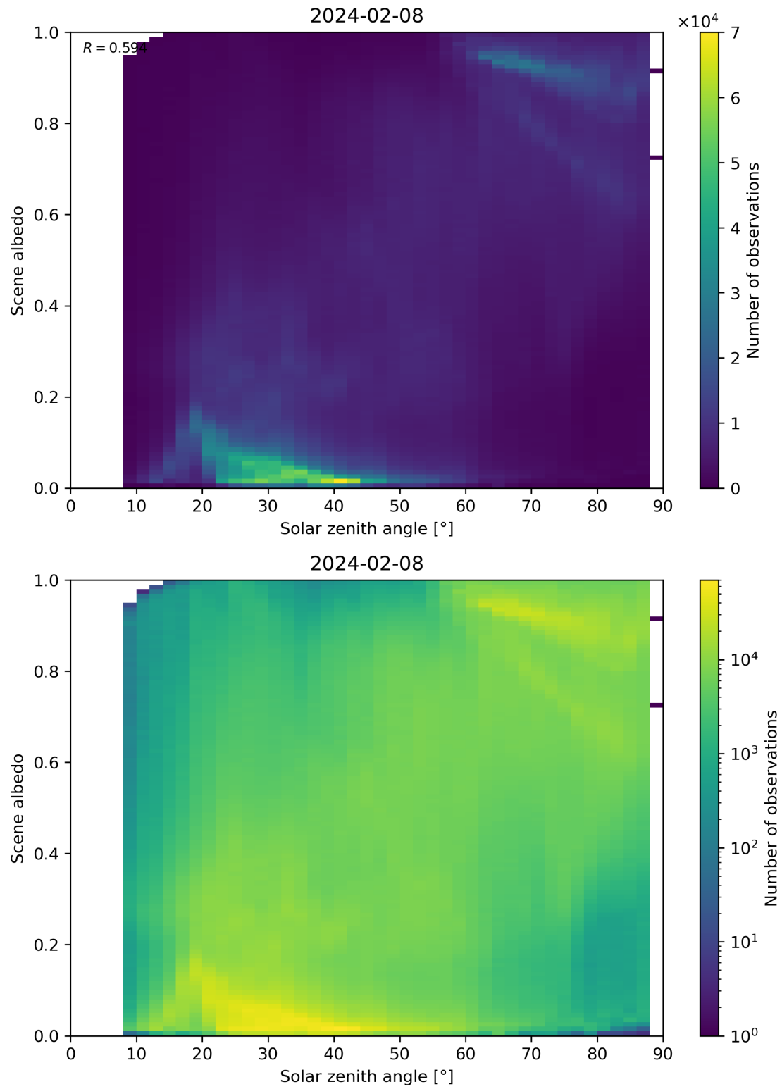
Figure 116: Scatter density plot of “Solar zenith angle” against “Scene albedo” for 2024-02-07 to 2024-02-09.
