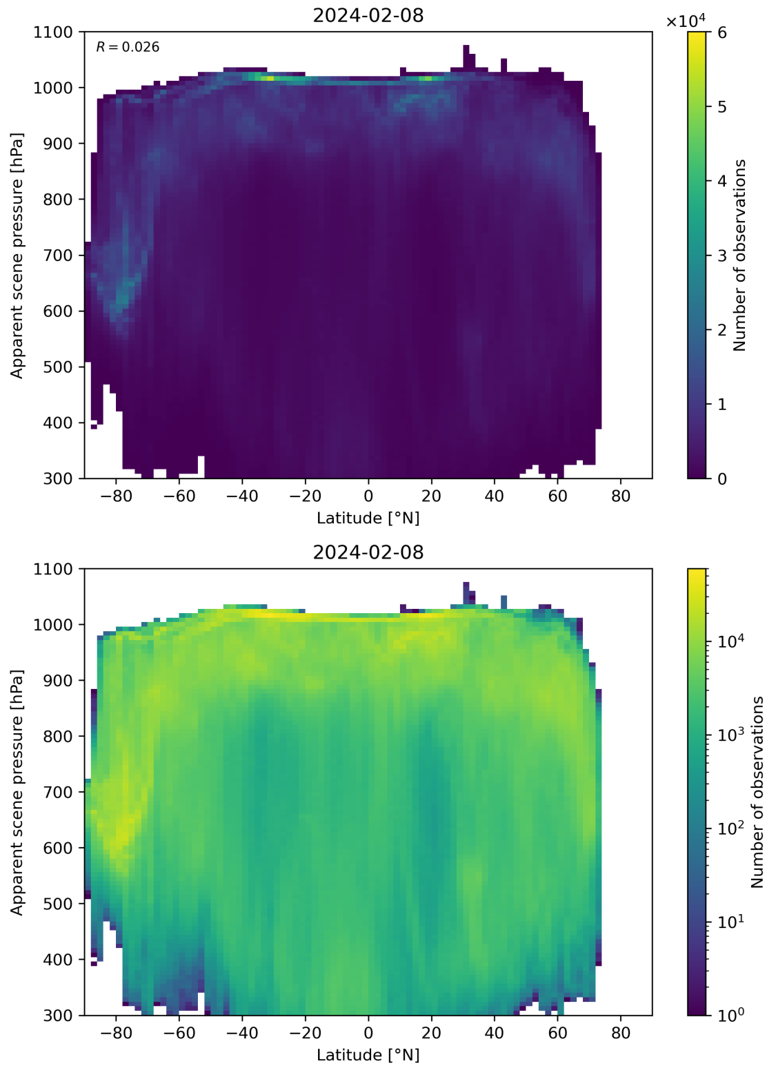
Figure 88: Scatter density plot of “Latitude” against “Apparent scene pressure” for 2024-02-07 to 2024-02-09.
