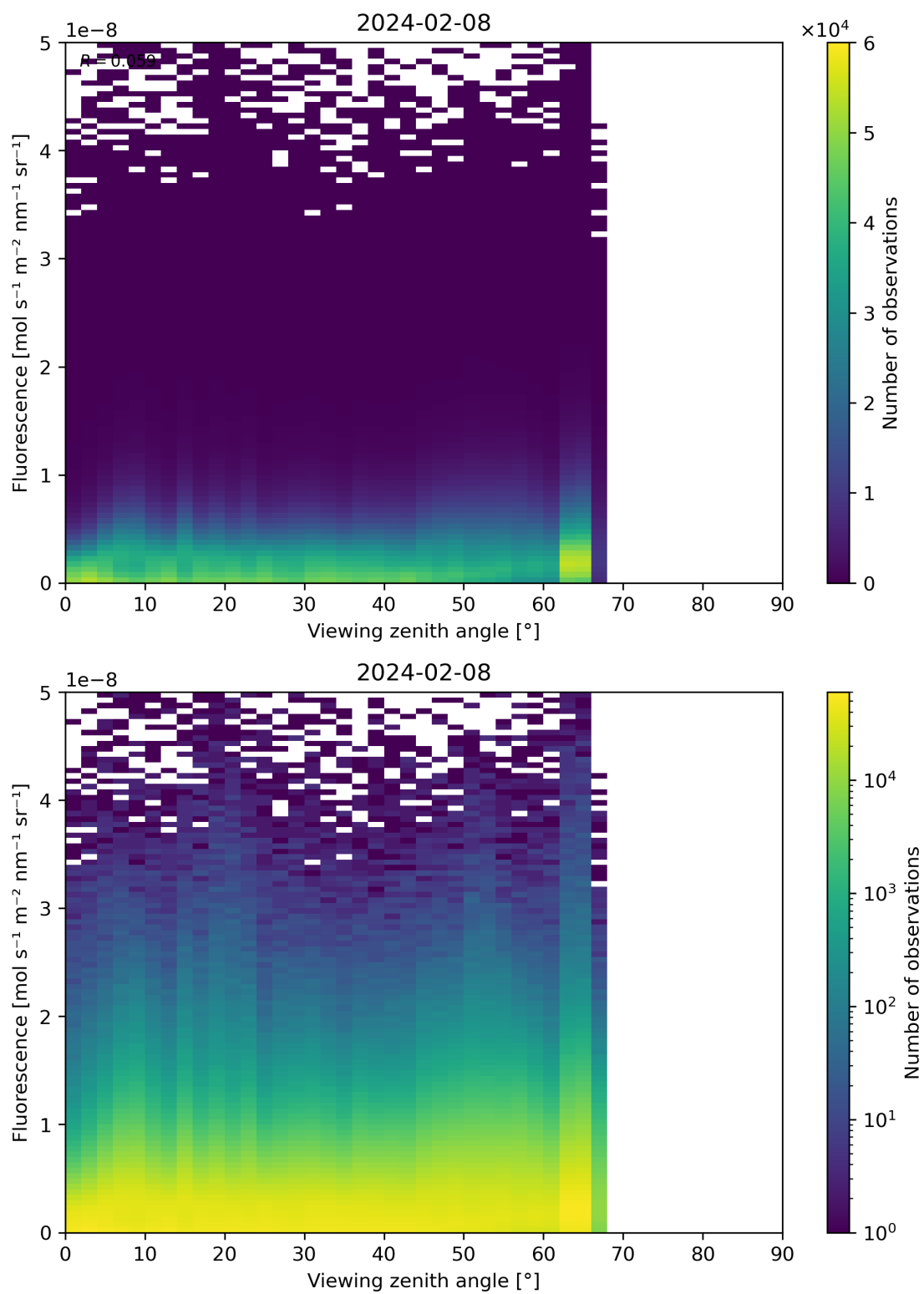
Figure 122: Scatter density plot of “Viewing zenith angle” against “Fluorescence” for 2024-02-07 to 2024-02-09.
