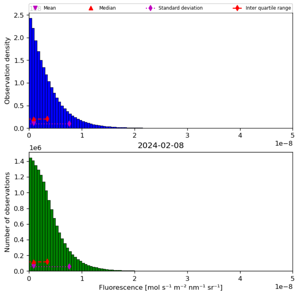
Figure 40: Histogram of “Fluorescence” for 2024-02-07 to 2024-02-09
