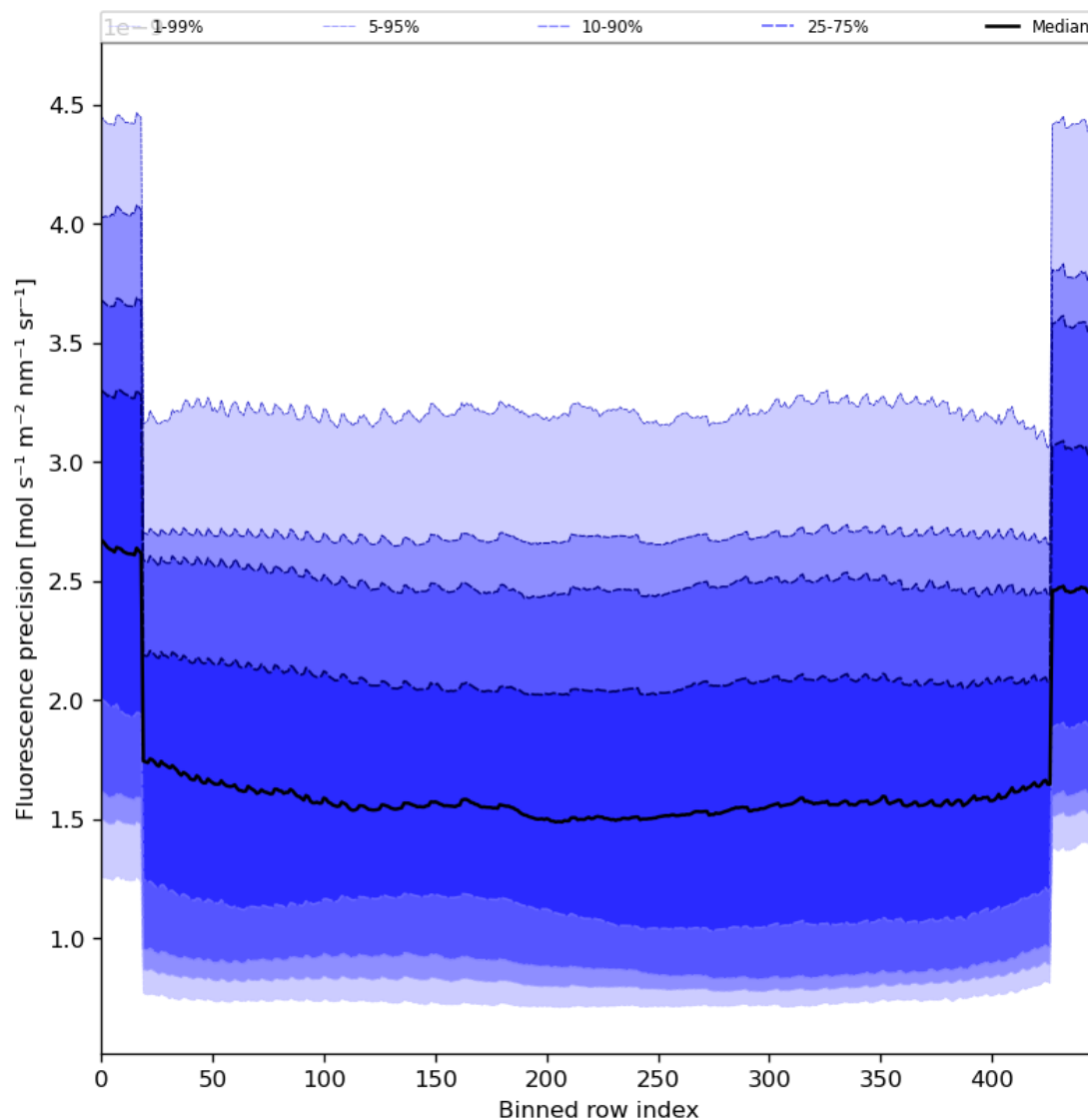
Figure 58: Along track statistics of “Fluorescence precision” for 2024-02-07 to 2024-02-09
