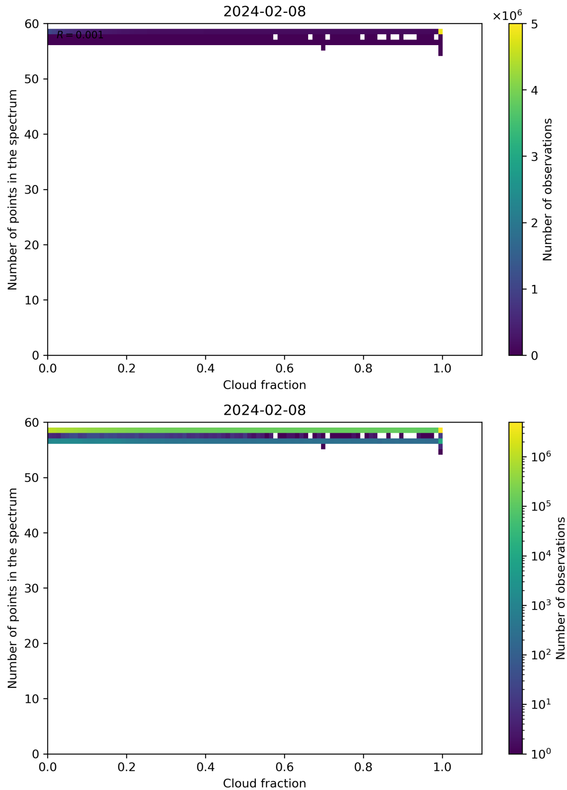
Figure 74: Scatter density plot of “Cloud fraction” against “Number of points in the spectrum” for 2024-02-07 to 2024-02-09.
