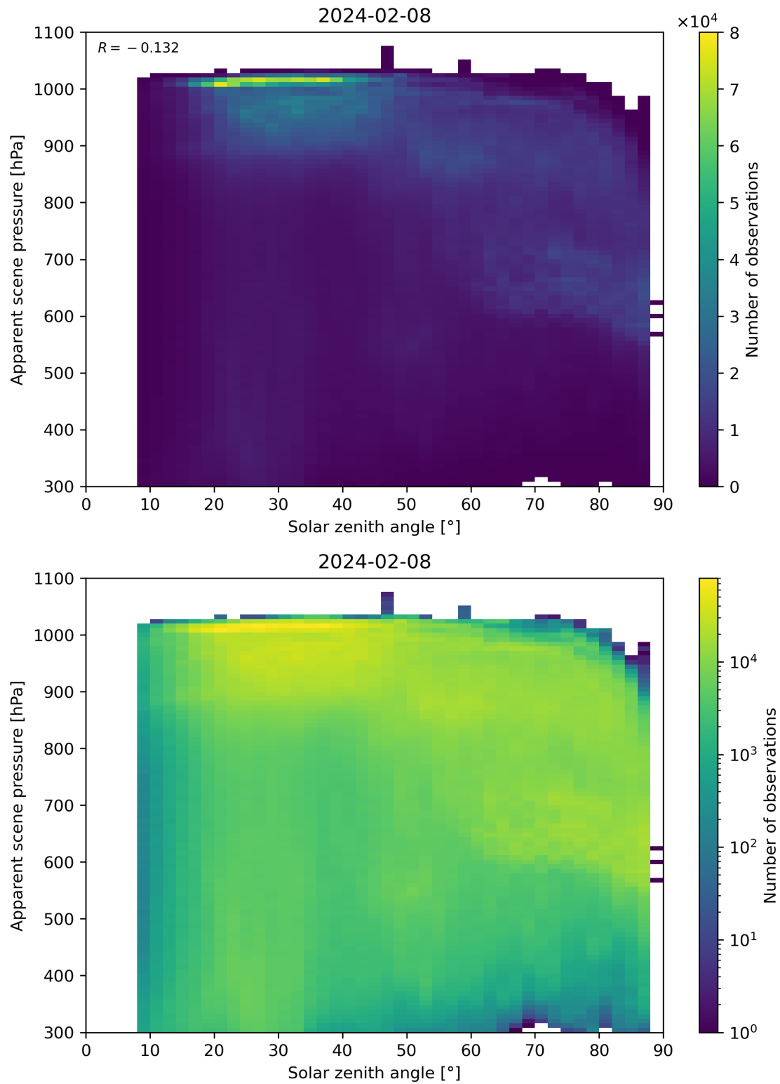
Figure 108: Scatter density plot of “Solar zenith angle” against “Apparent scene pressure” for 2024-02-07 to 2024-02-09.
