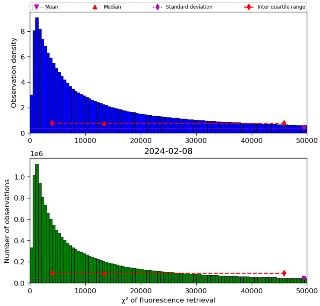
Figure 42: Histogram of “ \chi^2 of fluorescence retrieval” for 2024-02-07 to 2024-02-09
