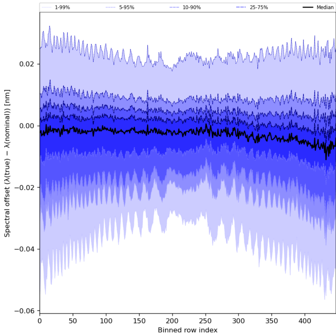
Figure 62: Along track statistics of “Spectral offset ( \lambda(\text{true}) - \lambda(\text{nominal}) )” for 2024-02-07 to 2024-02-09
