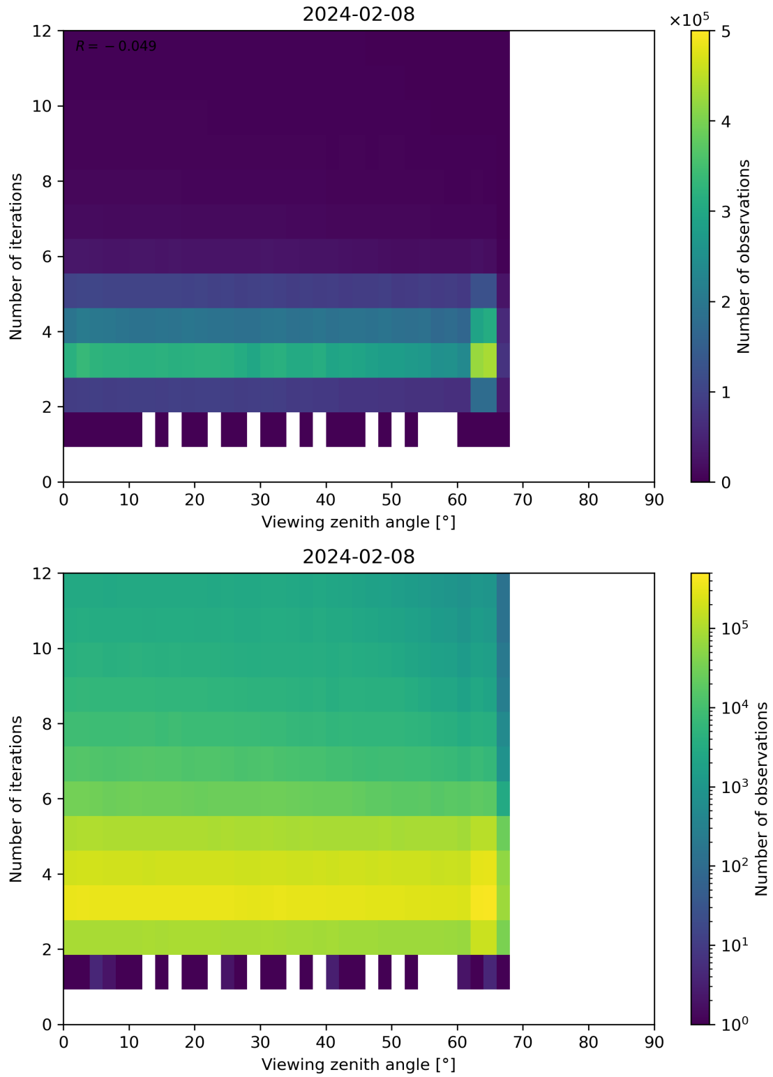
Figure 124: Scatter density plot of “Viewing zenith angle” against “Number of iterations” for 2024-02-07 to 2024-02-09.
