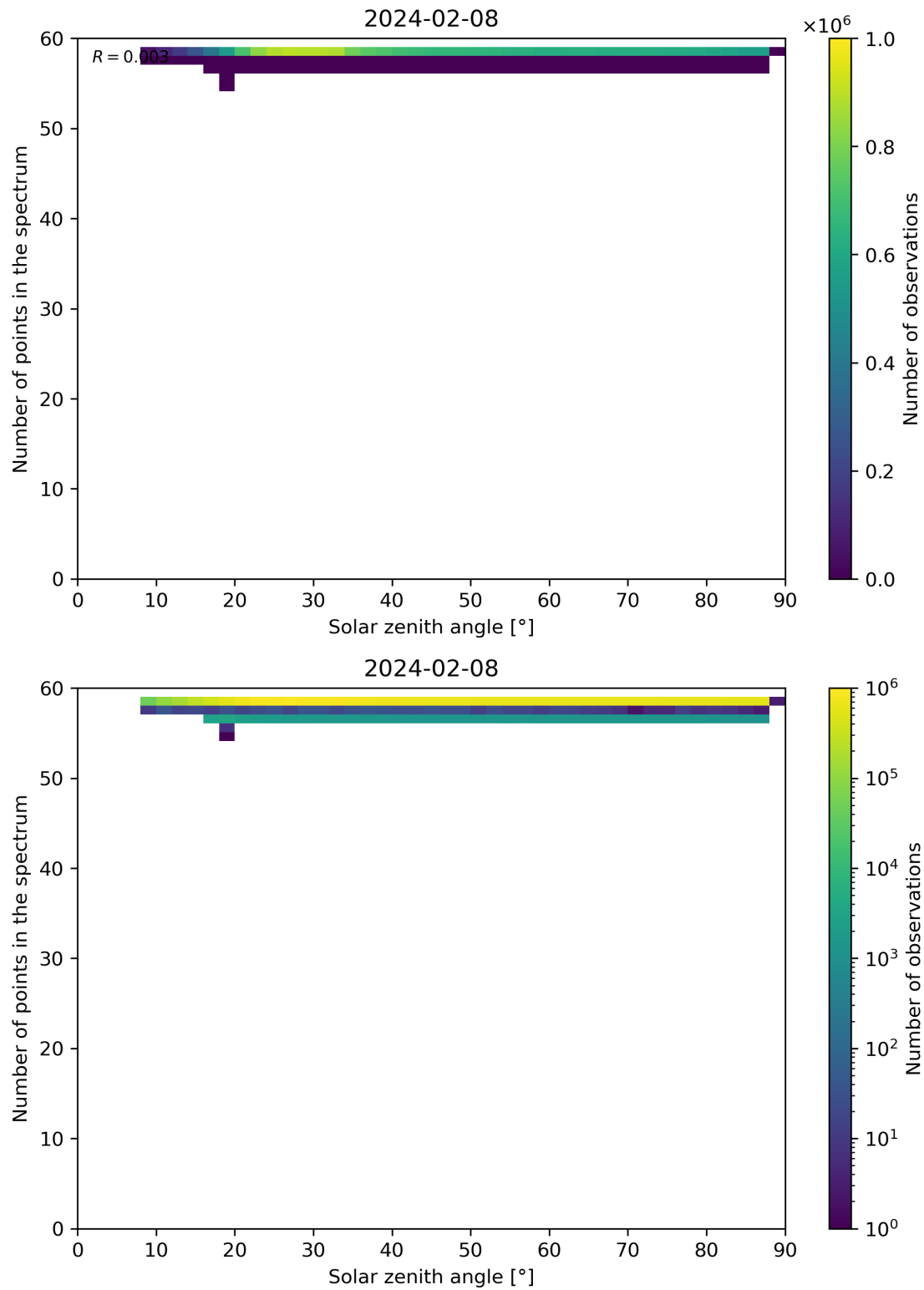
Figure 115: Scatter density plot of “Solar zenith angle” against “Number of points in the spectrum” for 2024-02-07 to 2024-02-09.
