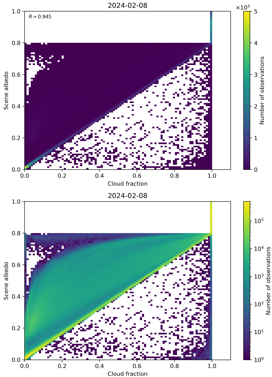
Figure 75: Scatter density plot of “Cloud fraction” against “Scene albedo” for 2024-02-07 to 2024-02-09.
