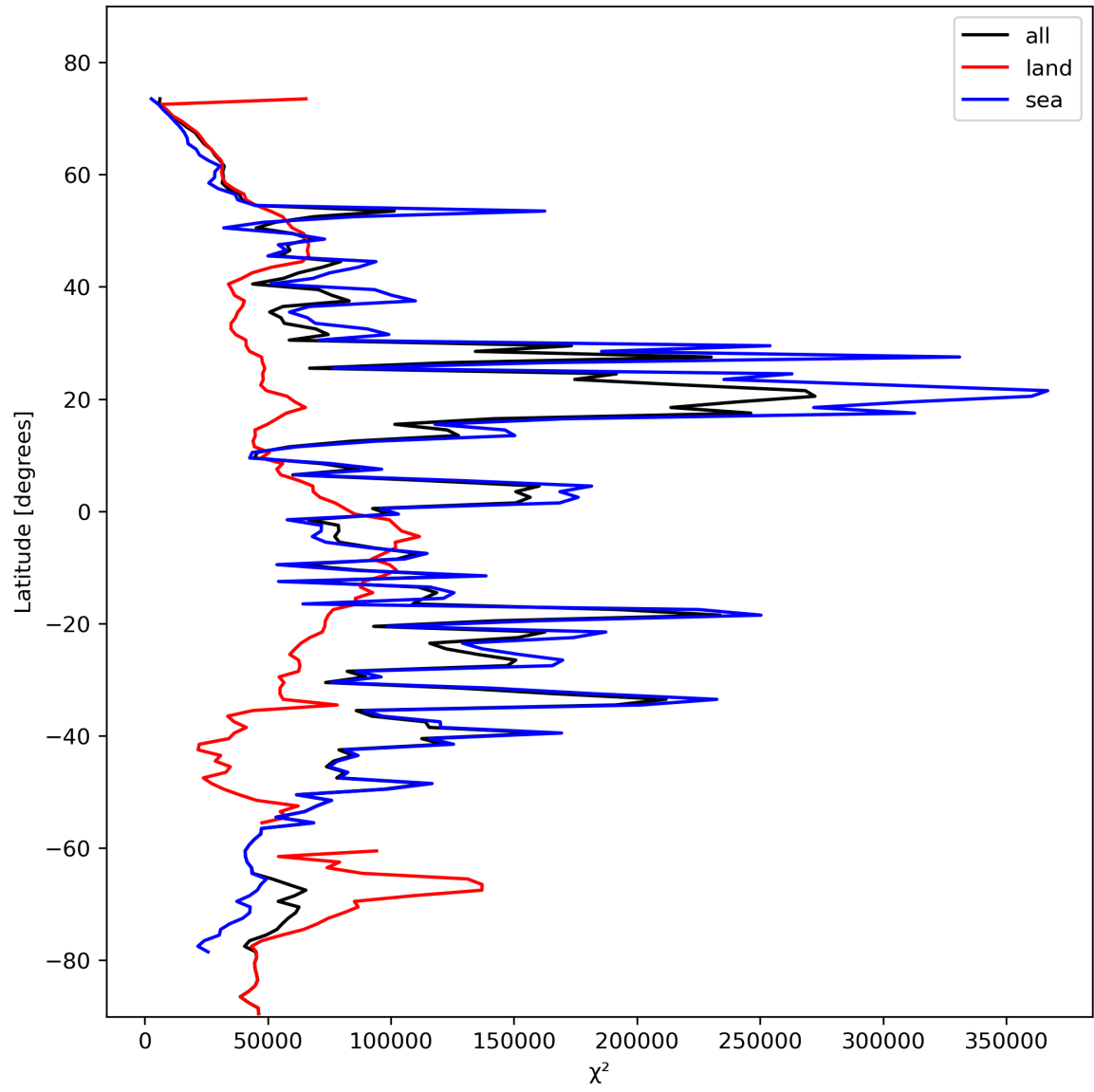
Figure 21: Zonal average of “ \chi^2 ” for 2024-02-07 to 2024-02-09.
