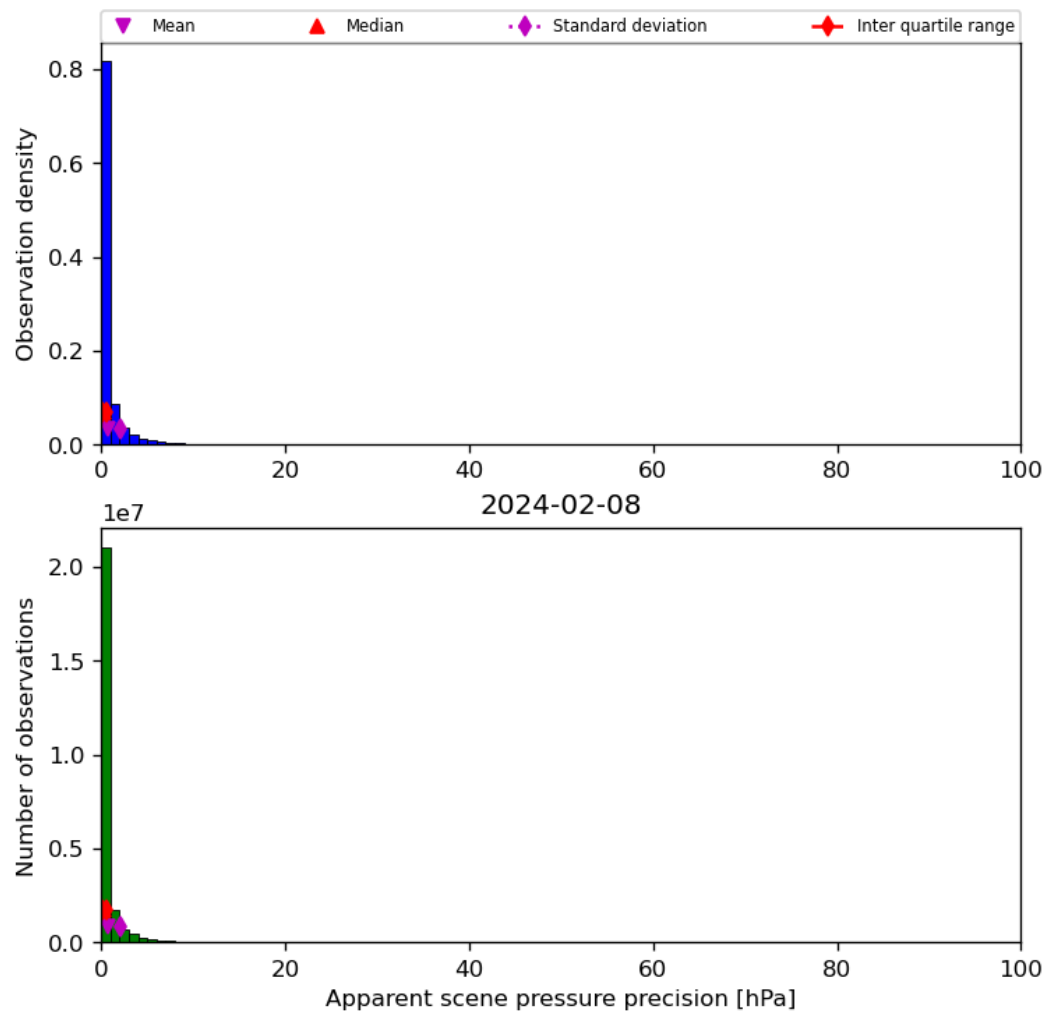
Figure 37: Histogram of "Apparent scene pressure precision" for 2024-02-07 to 2024-02-09
