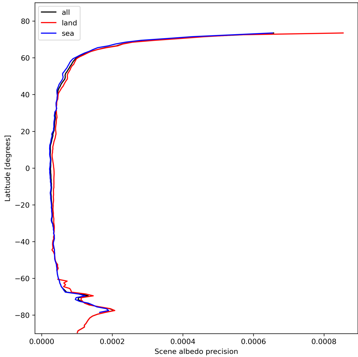
Figure 18: Zonal average of “Scene albedo precision” for 2024-02-07 to 2024-02-09.
