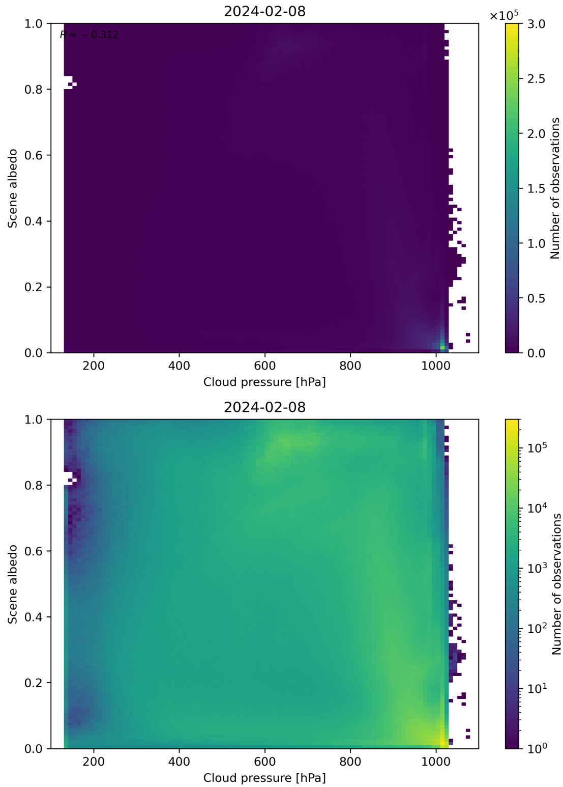
Figure 83: Scatter density plot of “Cloud pressure” against “Scene albedo” for 2024-02-07 to 2024-02-09.
