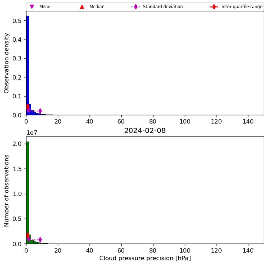
Figure 31: Histogram of “Cloud pressure precision” for 2024-02-07 to 2024-02-09
