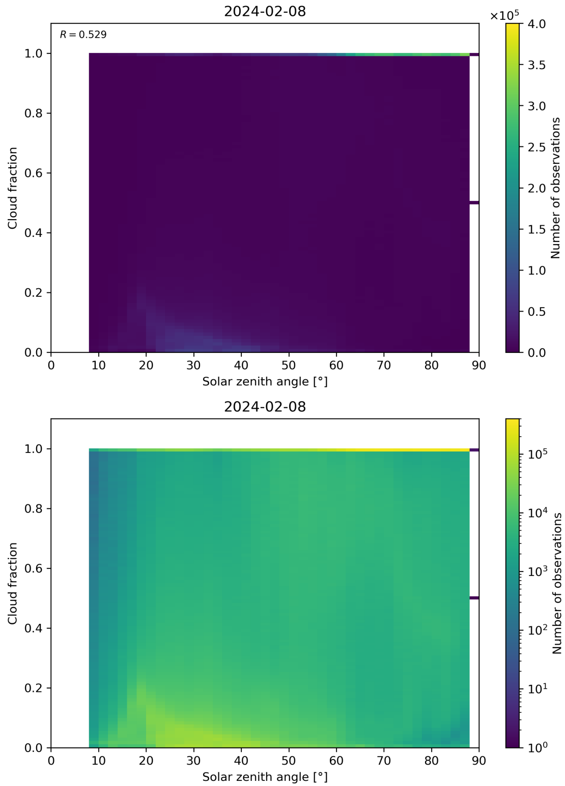
Figure 110: Scatter density plot of “Solar zenith angle” against “Cloud fraction” for 2024-02-07 to 2024-02-09.
