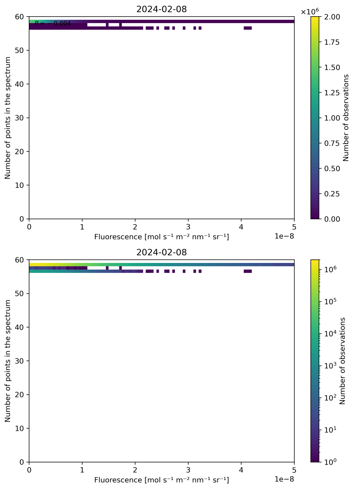
Figure 86: Scatter density plot of “Fluorescence” against “Number of points in the spectrum” for 2024-02-07 to 2024-02-09.
