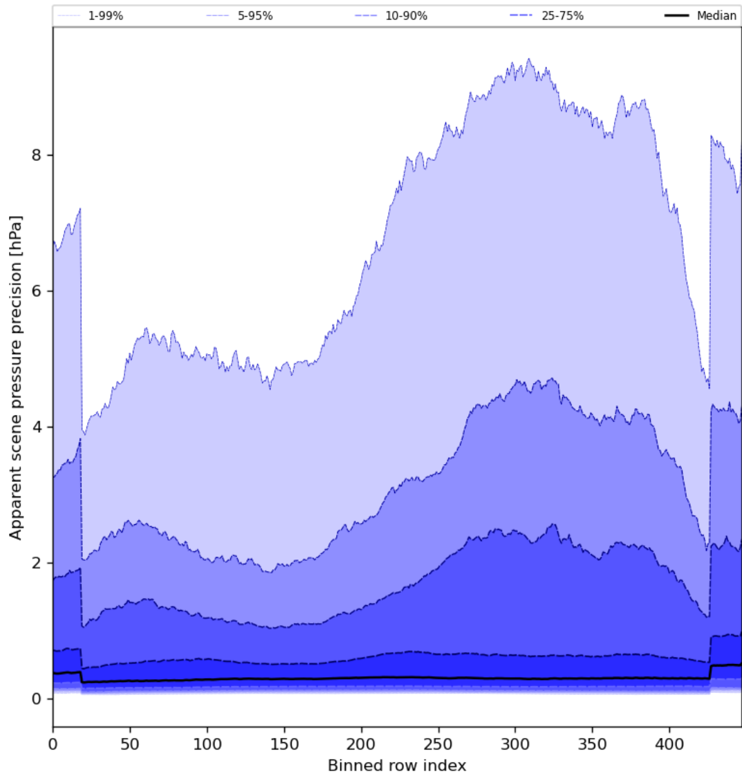
Figure 54: Along track statistics of “Apparent scene pressure precision” for 2024-02-07 to 2024-02-09
