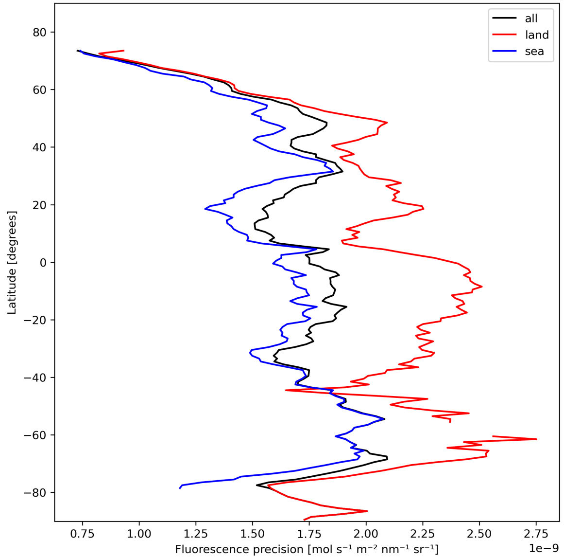
Figure 24: Zonal average of “Fluorescence precision” for 2024-02-07 to 2024-02-09.
