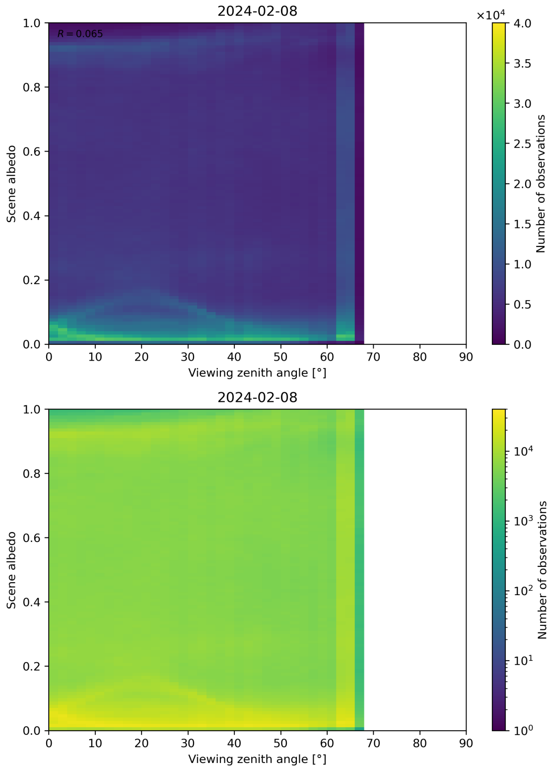
Figure 126: Scatter density plot of “Viewing zenith angle” against “Scene albedo” for 2024-02-07 to 2024-02-09.
