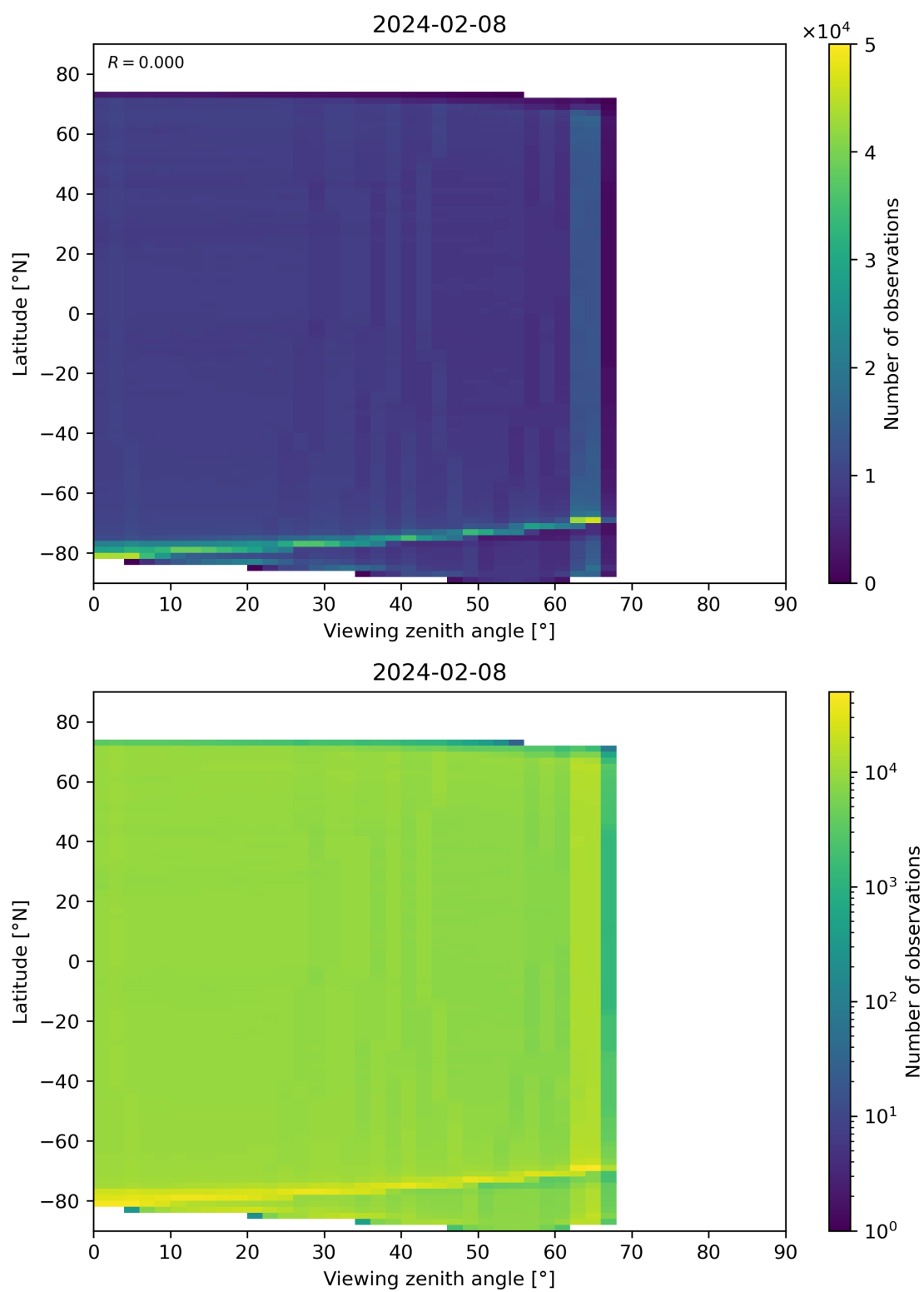
Figure 123: Scatter density plot of “Viewing zenith angle” against “Latitude” for 2024-02-07 to 2024-02-09.
