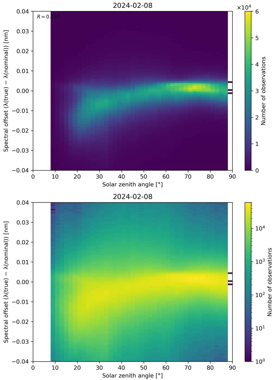
Figure 117: Scatter density plot of “Solar zenith angle” against “Spectral offset ( \lambda(\text{true}) - \lambda(\text{nominal}) )” for 2024-02-07 to 2024-02-09.
