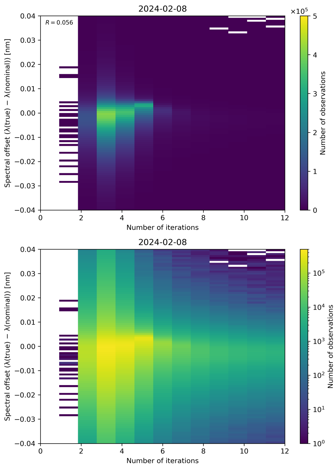
Figure 100: Scatter density plot of “Number of iterations” against “Spectral offset ( \lambda(\text{true}) - \lambda(\text{nominal}) )” for 2024-02-07 to 2024-02-09.
