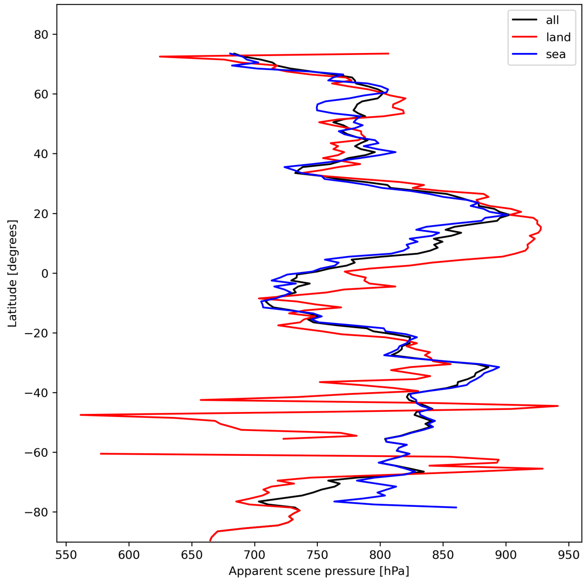
Figure 19: Zonal average of “Apparent scene pressure” for 2024-02-07 to 2024-02-09.
