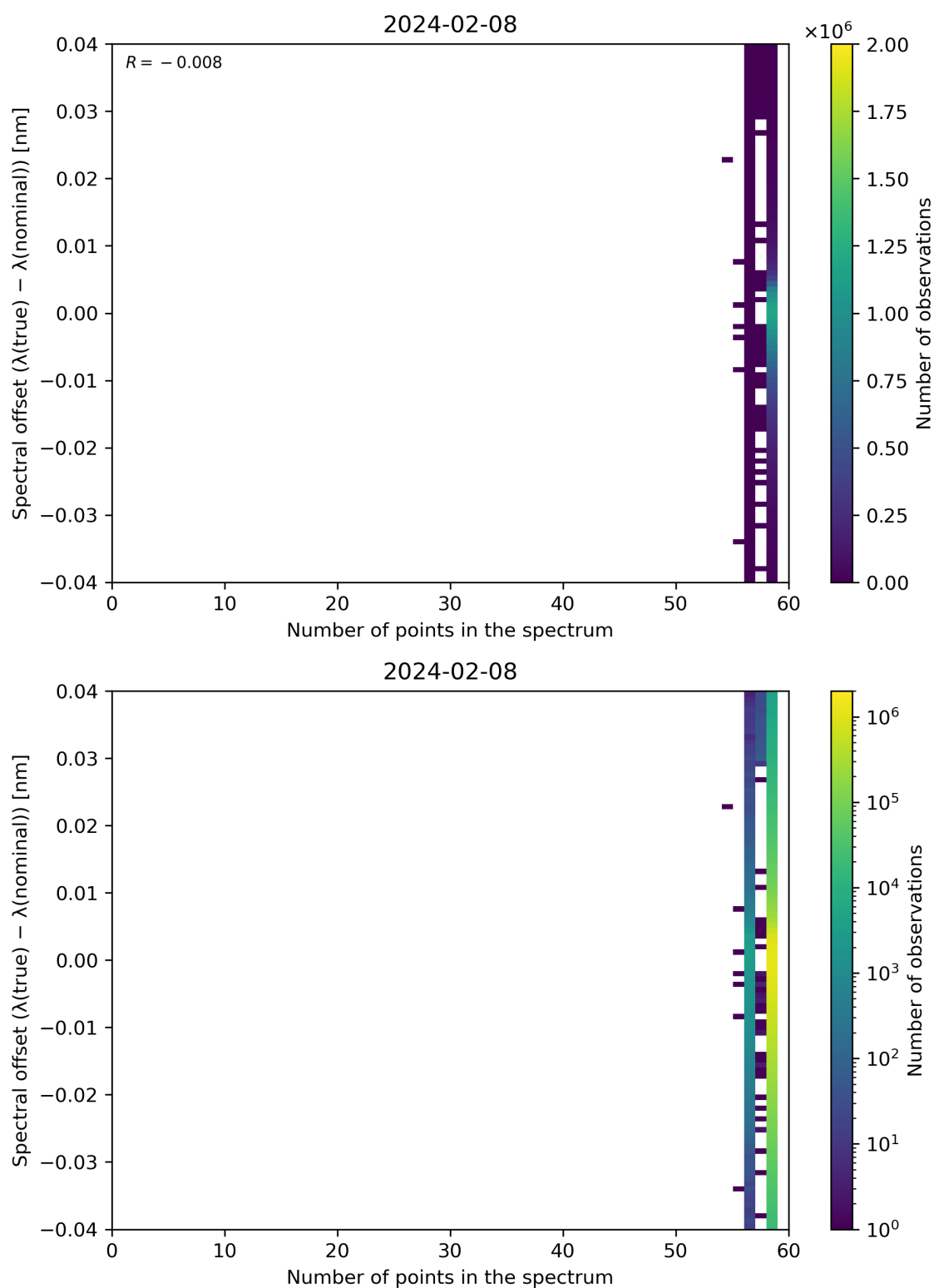
Figure 101: Scatter density plot of “Number of points in the spectrum” against “Spectral offset ( \lambda(\text{true}) - \lambda(\text{nominal}) )” for 2024-02-07 to 2024-02-09.
