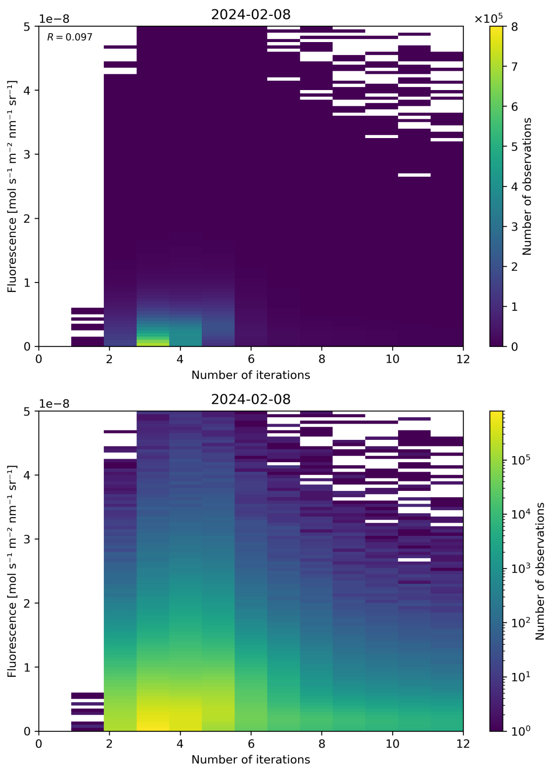
Figure 98: Scatter density plot of “Number of iterations” against “Fluorescence” for 2024-02-07 to 2024-02-09.
