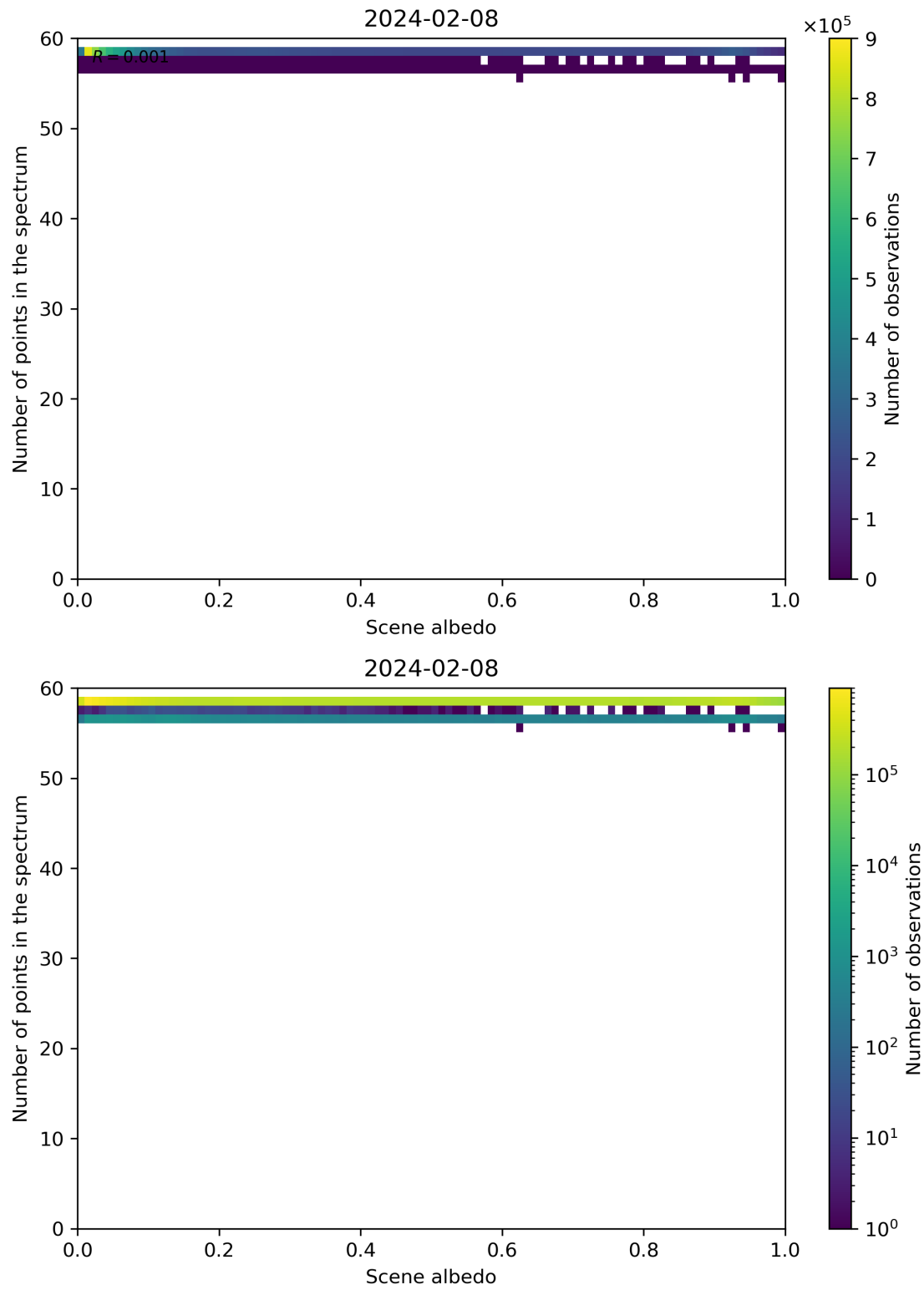
Figure 106: Scatter density plot of “Scene albedo” against “Number of points in the spectrum” for 2024-02-07 to 2024-02-09.
