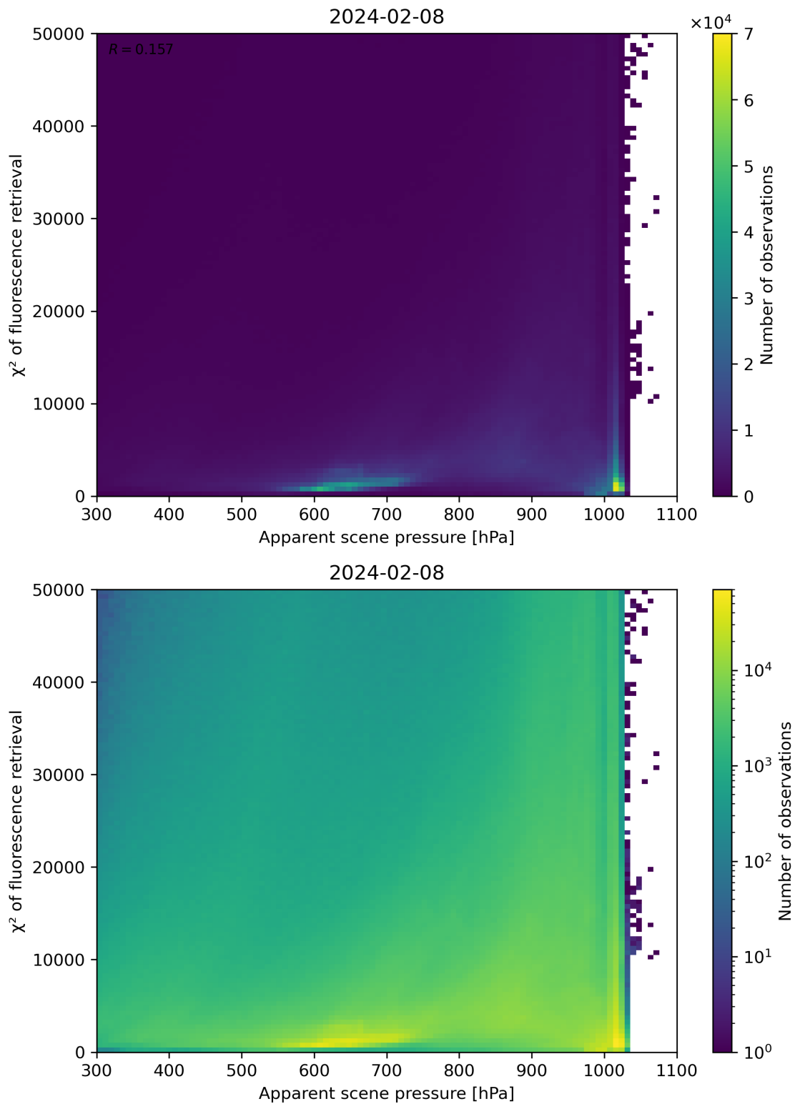
Figure 63: Scatter density plot of “Apparent scene pressure” against “ \chi^2 of fluorescence retrieval” for 2024-02-07 to 2024-02-09.
