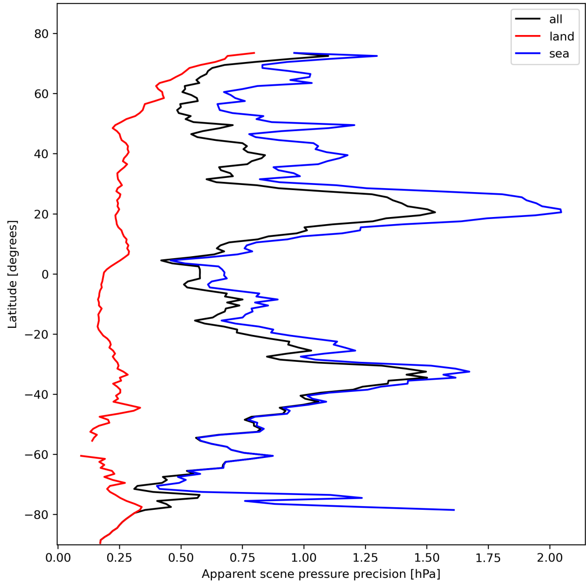
Figure 20: Zonal average of “Apparent scene pressure precision” for 2024-02-07 to 2024-02-09.
