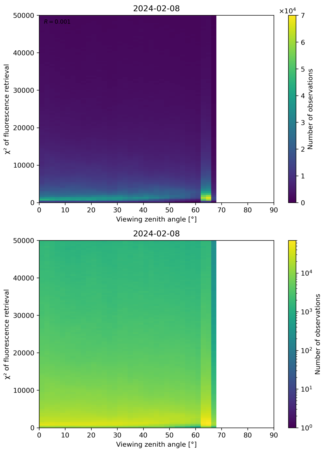
Figure 119: Scatter density plot of “Viewing zenith angle” against “ \chi^2 of fluorescence retrieval” for 2024-02-07 to 2024-02-09.
