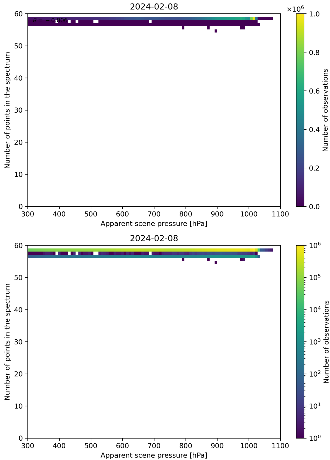
Figure 66: Scatter density plot of “Apparent scene pressure” against “Number of points in the spectrum” for 2024-02-07 to 2024-02-09.
