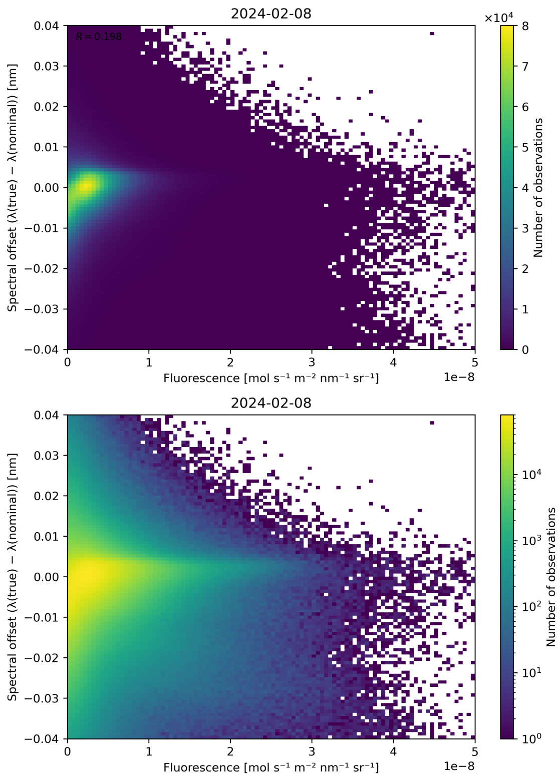
Figure 87: Scatter density plot of “Fluorescence” against “Spectral offset ( \lambda(\text{true}) - \lambda(\text{nominal}) )” for 2024-02-07 to 2024-02-09.
