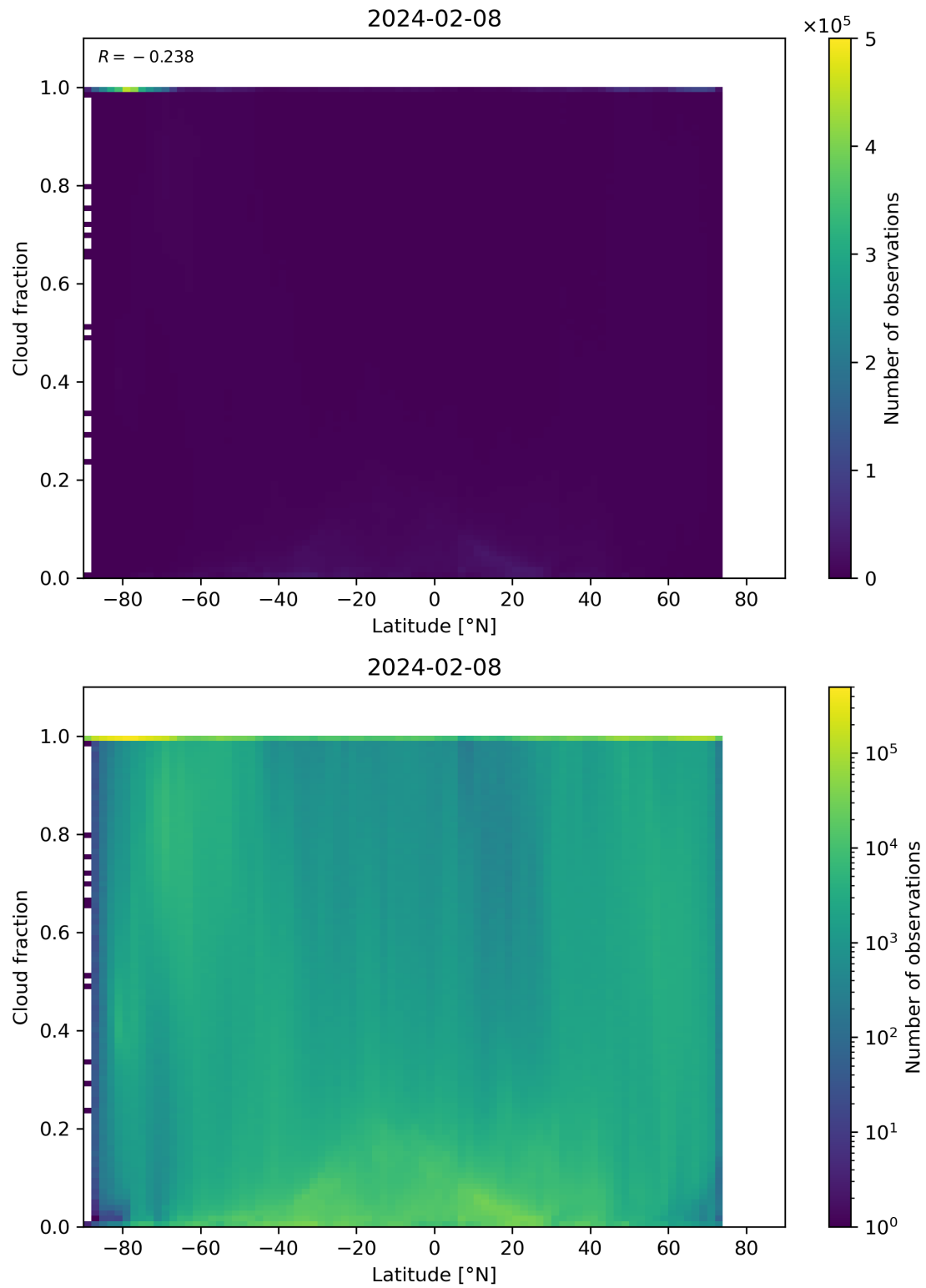
Figure 90: Scatter density plot of “Latitude” against “Cloud fraction” for 2024-02-07 to 2024-02-09.
