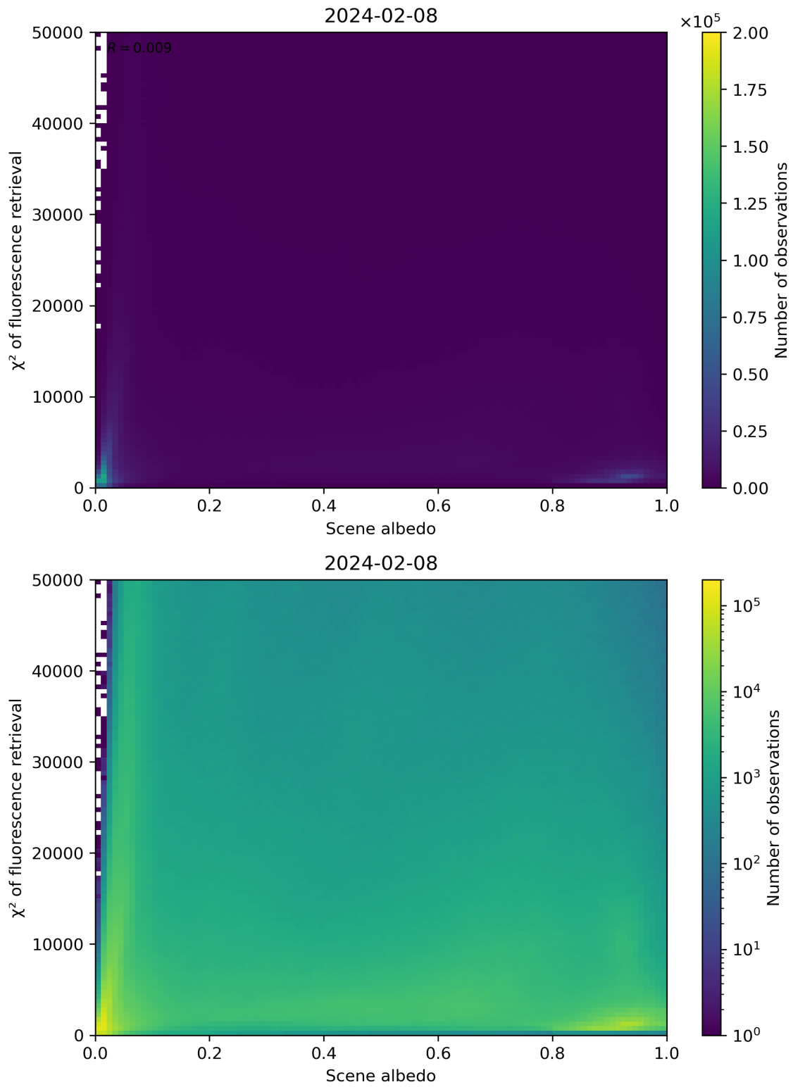
Figure 103: Scatter density plot of “Scene albedo” against “ \chi^2 of fluorescence retrieval” for 2024-02-07 to 2024-02-09.
