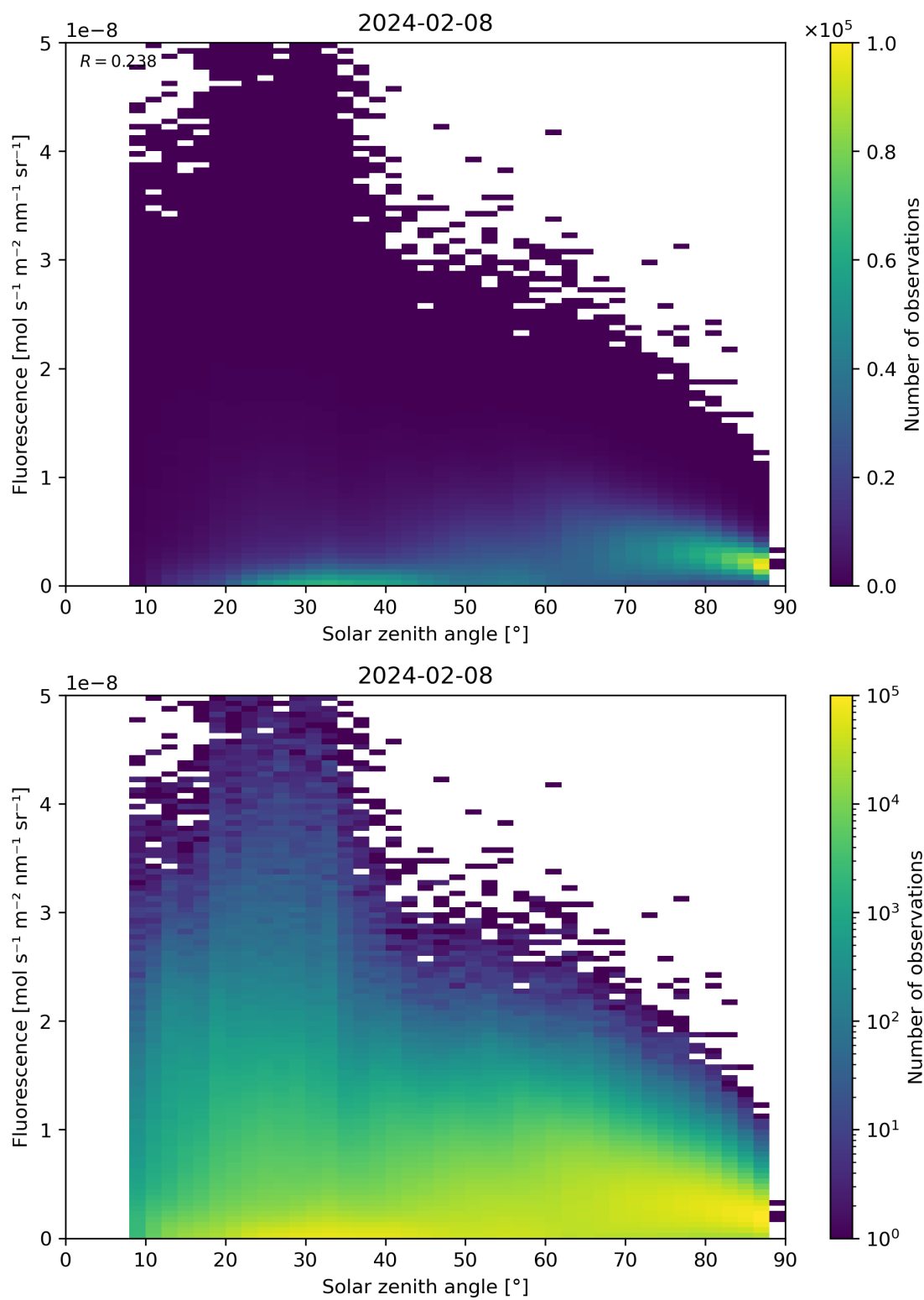
Figure 112: Scatter density plot of “Solar zenith angle” against “Fluorescence” for 2024-02-07 to 2024-02-09.
