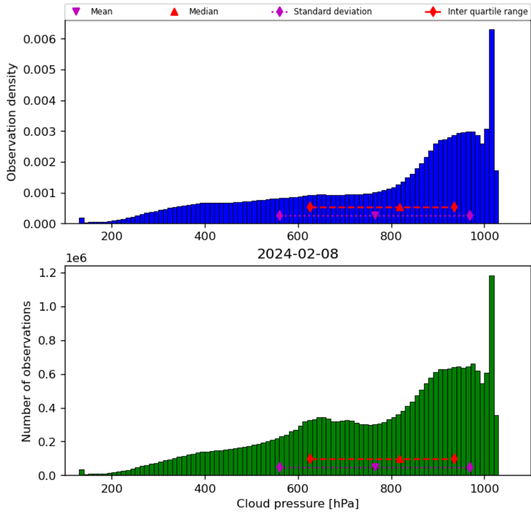
Figure 30: Histogram of “Cloud pressure” for 2024-02-07 to 2024-02-09
