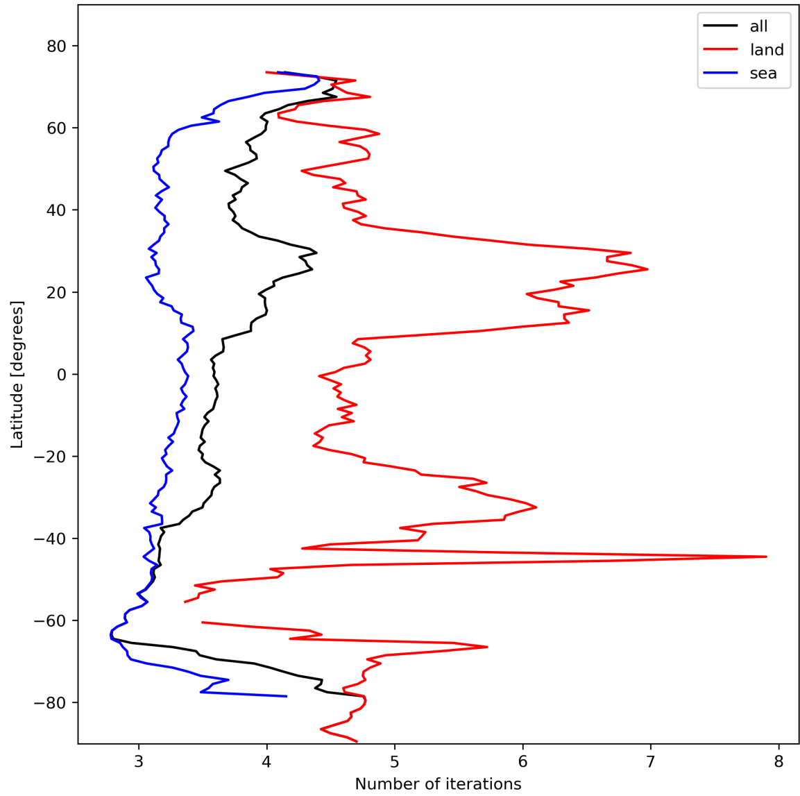
Figure 22: Zonal average of “Number of iterations” for 2024-02-07 to 2024-02-09.
