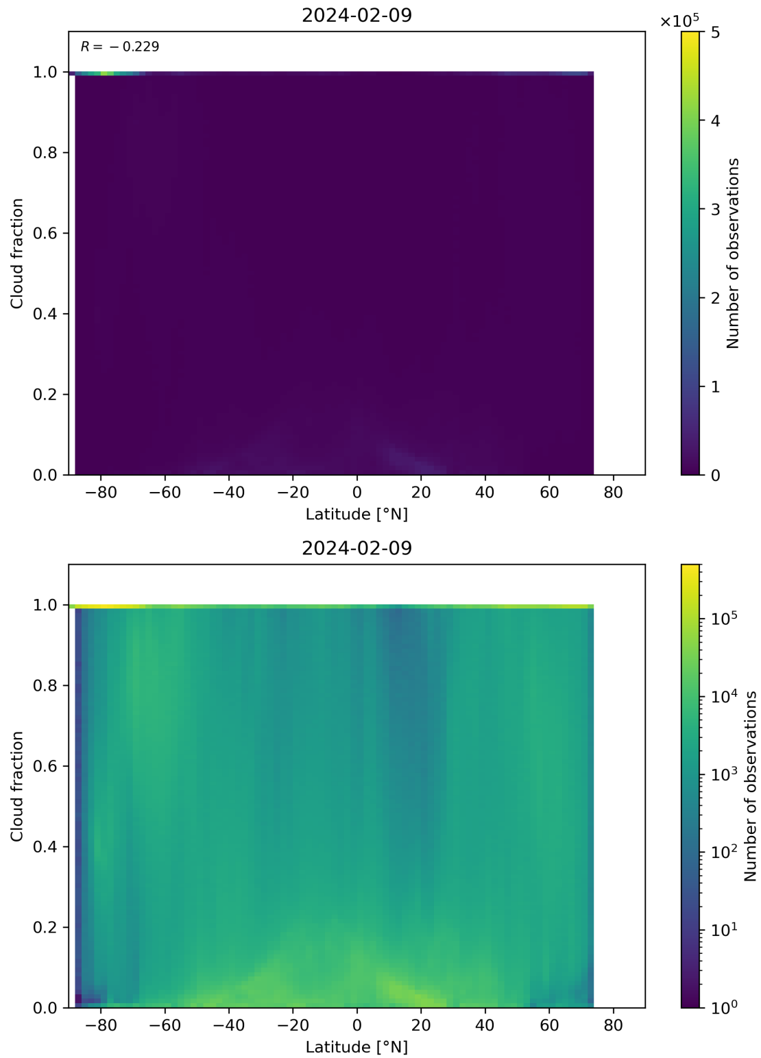
Figure 90: Scatter density plot of “Latitude” against “Cloud fraction” for 2024-02-08 to 2024-02-10.
