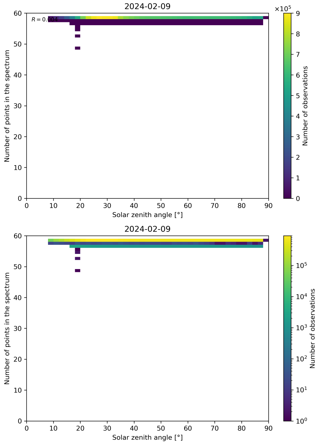
Figure 115: Scatter density plot of “Solar zenith angle” against “Number of points in the spectrum” for 2024-02-08 to 2024-02-10.
