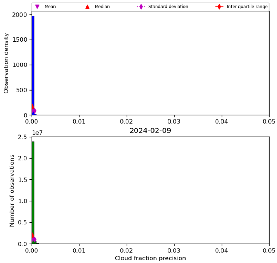
Figure 33: Histogram of “Cloud fraction precision” for 2024-02-08 to 2024-02-10
