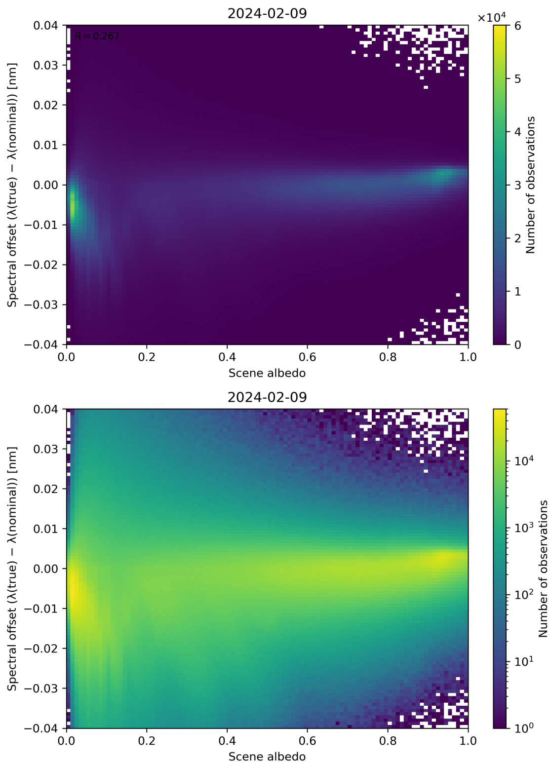
Figure 107: Scatter density plot of “Scene albedo” against “Spectral offset ( \lambda(\text{true}) - \lambda(\text{nominal}) )” for 2024-02-08 to 2024-02-10.
