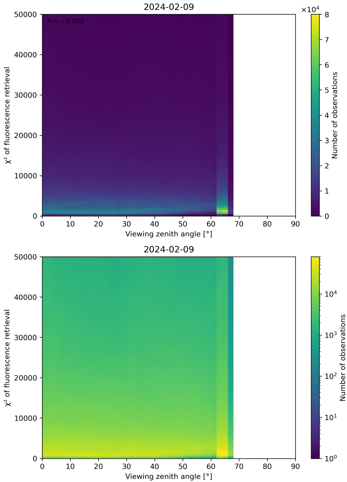
Figure 119: Scatter density plot of “Viewing zenith angle” against “ \chi^2 of fluorescence retrieval” for 2024-02-08 to 2024-02-10.
