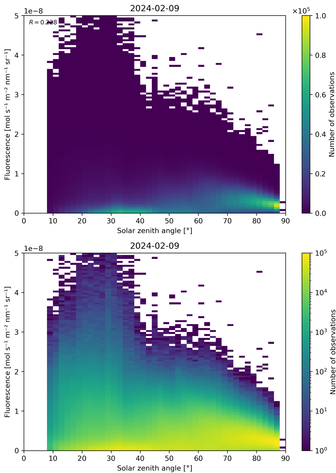
Figure 112: Scatter density plot of “Solar zenith angle” against “Fluorescence” for 2024-02-08 to 2024-02-10.
