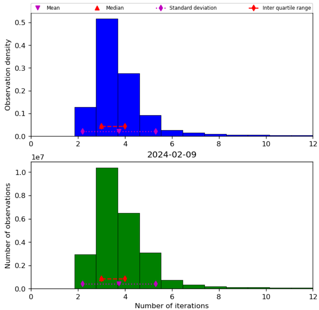
Figure 39: Histogram of “Number of iterations” for 2024-02-08 to 2024-02-10
