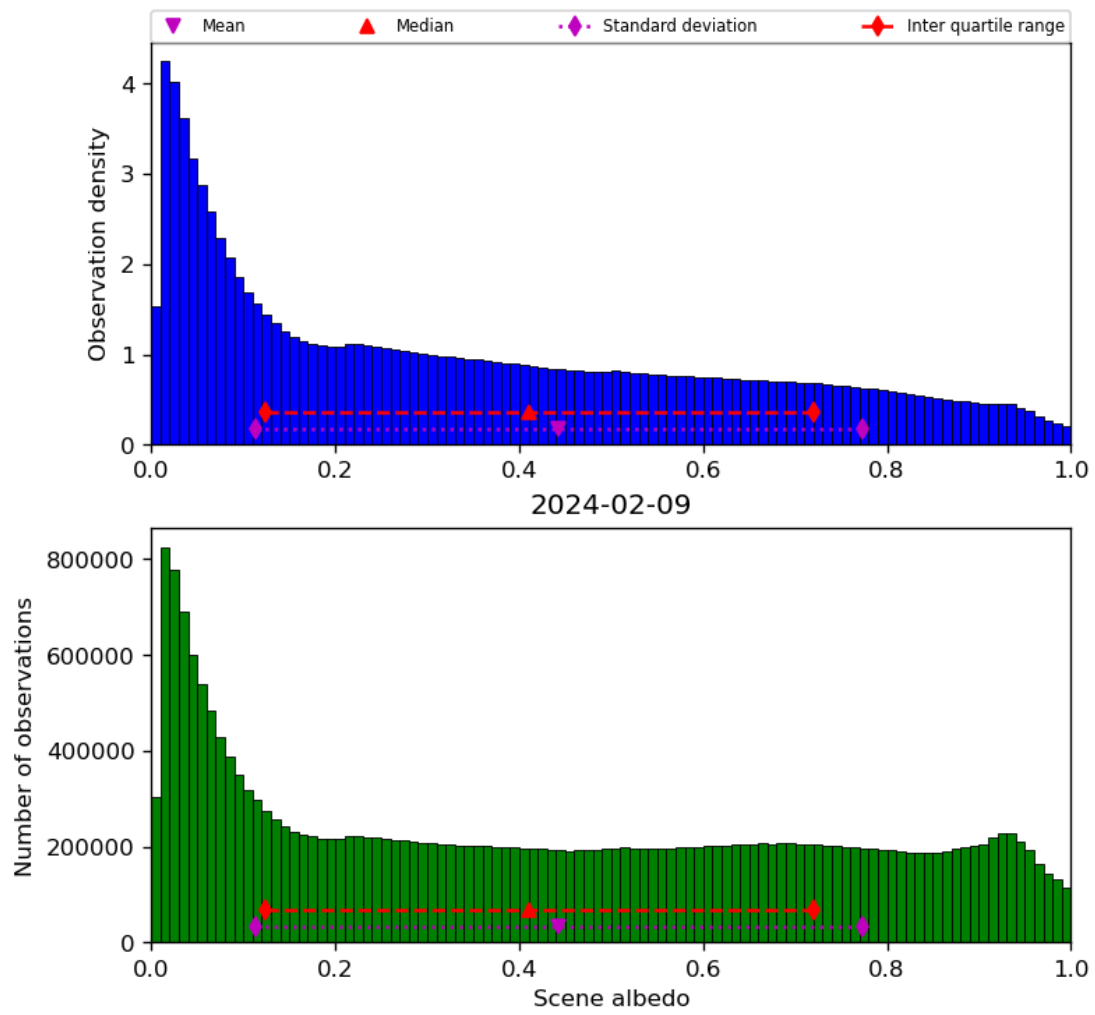
Figure 34: Histogram of “Scene albedo” for 2024-02-08 to 2024-02-10
