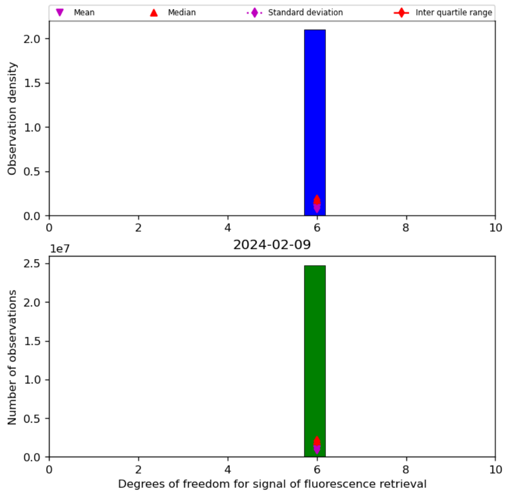
Figure 43: Histogram of “Degrees of freedom for signal of fluorescence retrieval” for 2024-02-08 to 2024-02-10
