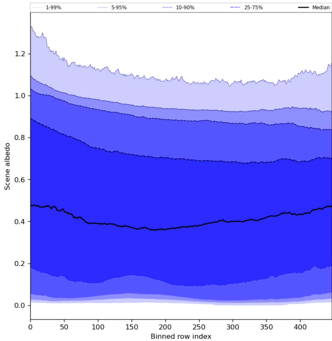
Figure 51: Along track statistics of “Scene albedo” for 2024-02-08 to 2024-02-10
