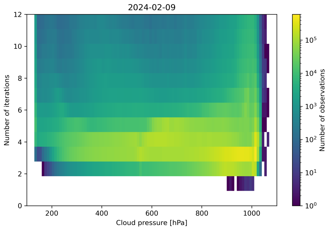
Figure 81: Scatter density plot of “Cloud pressure” against “Number of iterations” for 2024-02-08 to 2024-02-10.
