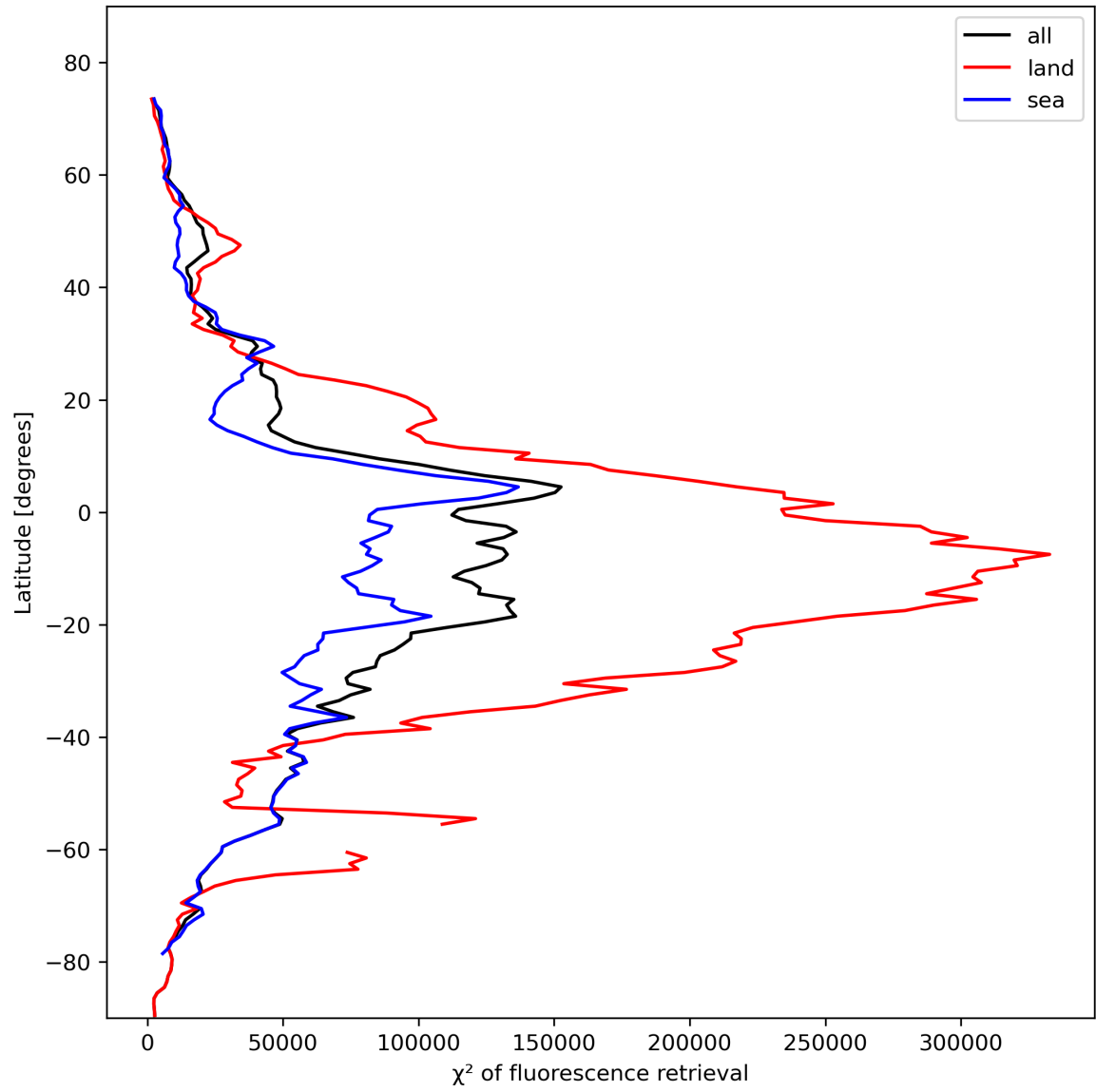
Figure 25: Zonal average of “ \chi^2 of fluorescence retrieval” for 2024-02-08 to 2024-02-10.
