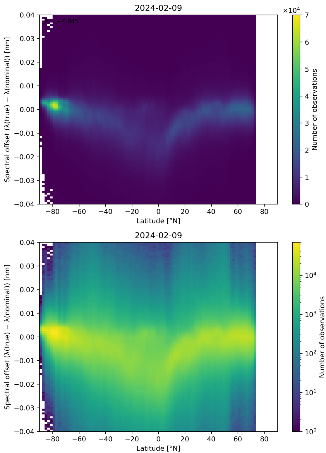
Figure 96: Scatter density plot of “Latitude” against “Spectral offset ( \lambda(\text{true}) - \lambda(\text{nominal}) )” for 2024-02-08 to 2024-02-10.
