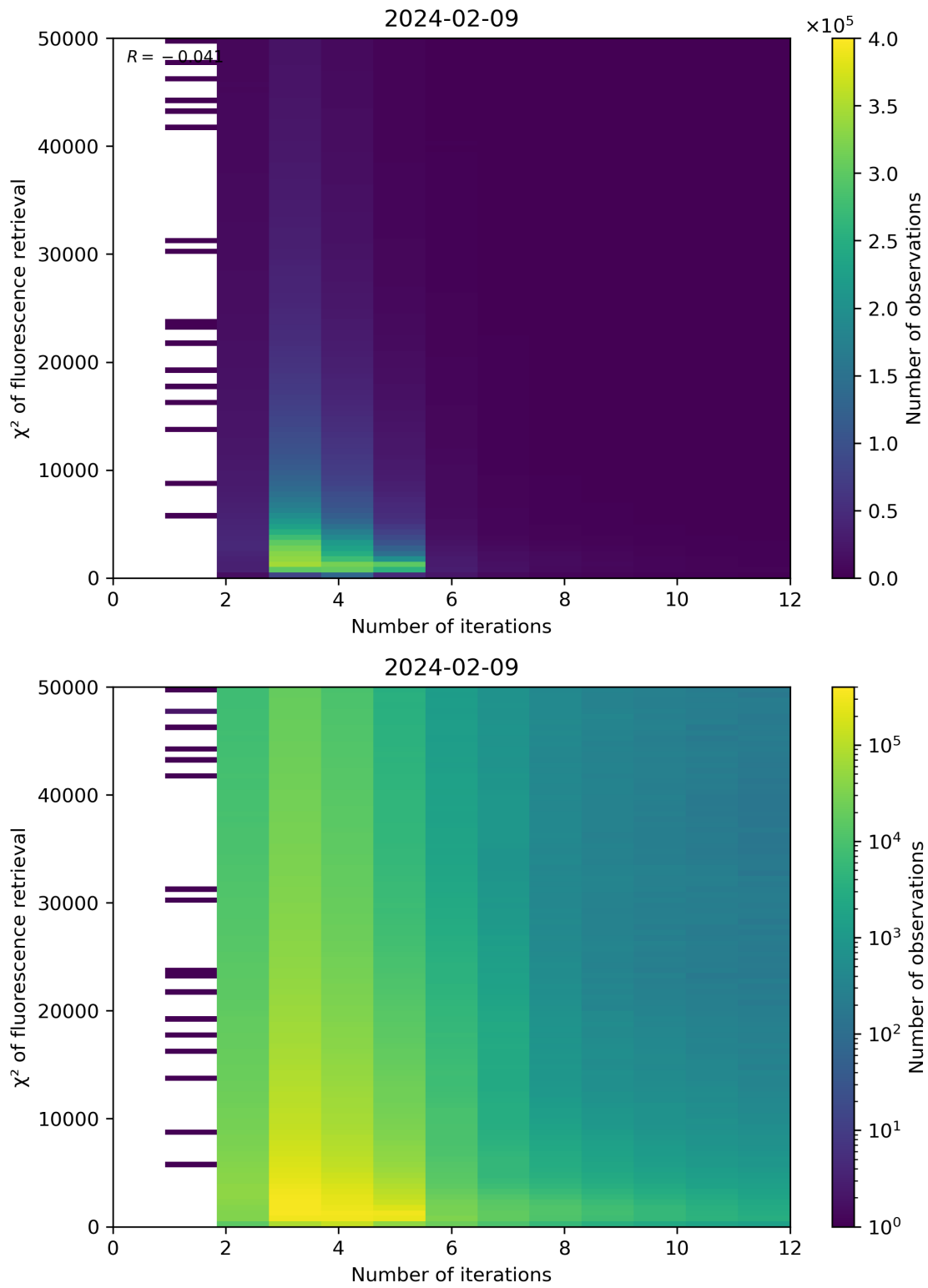
Figure 97: Scatter density plot of “Number of iterations” against “ \chi^2 of fluorescence retrieval” for 2024-02-08 to 2024-02-10.
