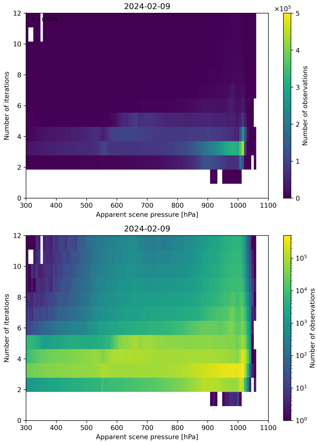
Figure 65: Scatter density plot of “Apparent scene pressure” against “Number of iterations” for 2024-02-08 to 2024-02-10.
