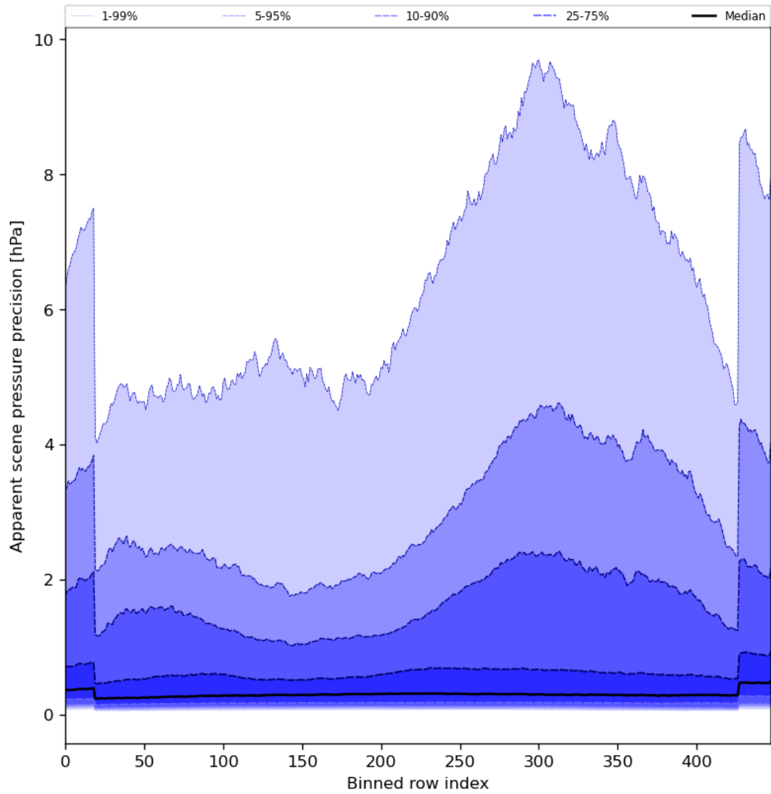
Figure 54: Along track statistics of “Apparent scene pressure precision” for 2024-02-08 to 2024-02-10
