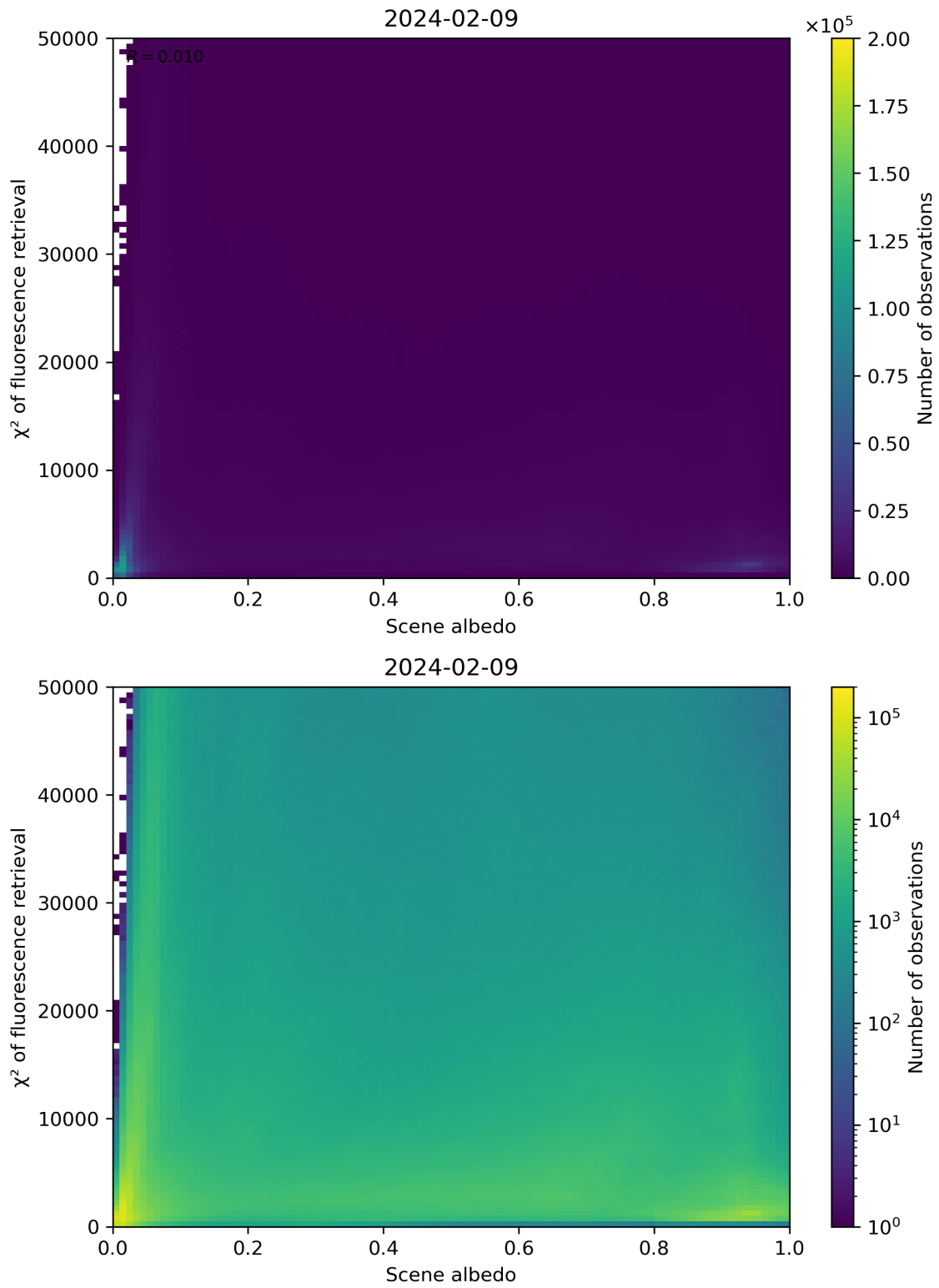
Figure 103: Scatter density plot of “Scene albedo” against “ \chi^2 of fluorescence retrieval” for 2024-02-08 to 2024-02-10.
