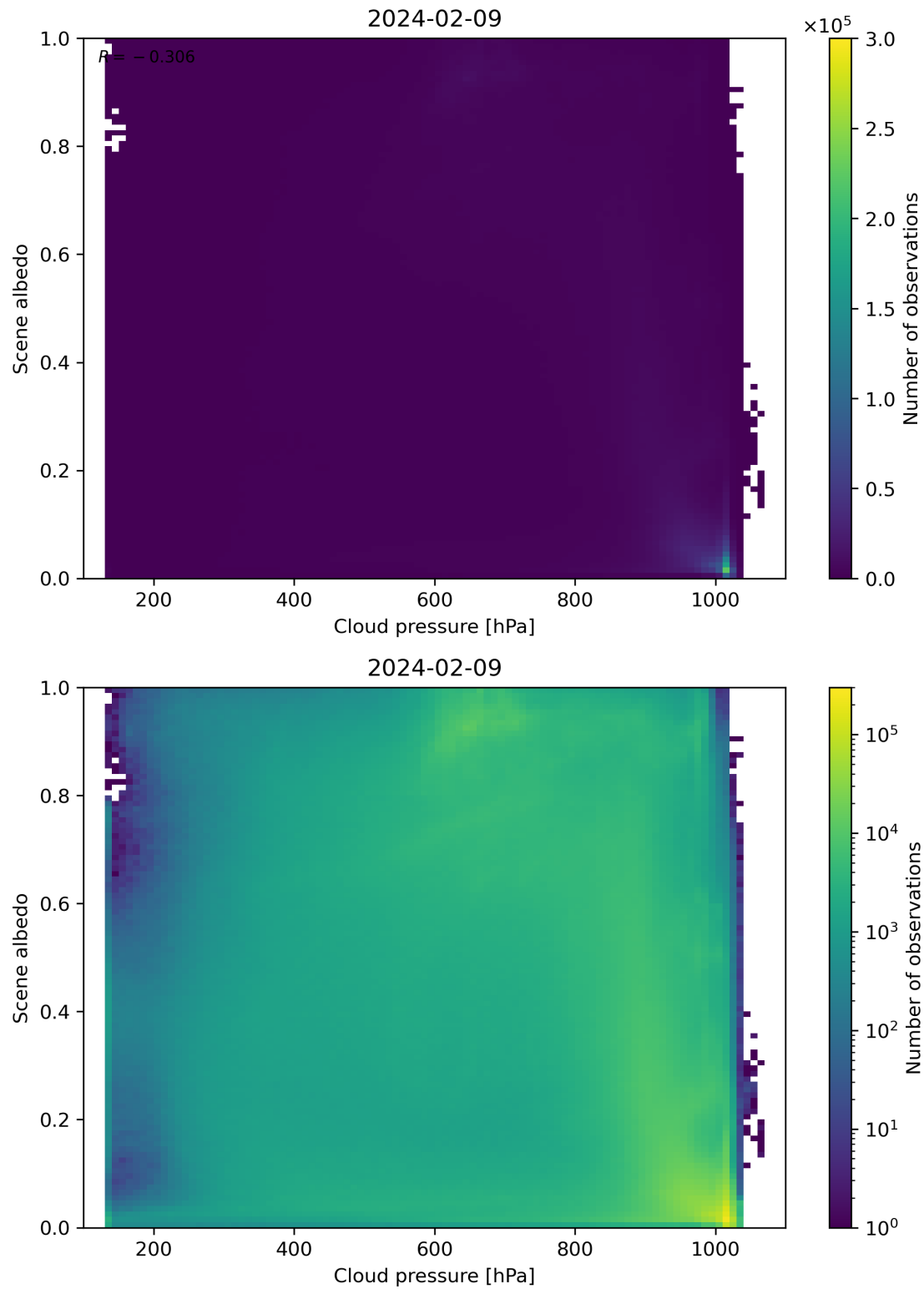
Figure 83: Scatter density plot of “Cloud pressure” against “Scene albedo” for 2024-02-08 to 2024-02-10.
