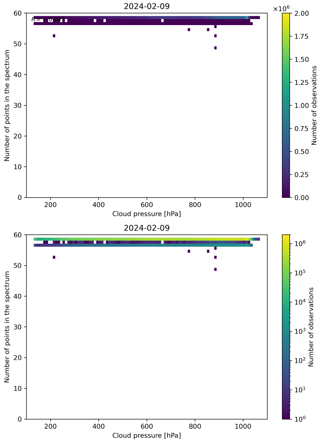
Figure 82: Scatter density plot of “Cloud pressure” against “Number of points in the spectrum” for 2024-02-08 to 2024-02-10.
