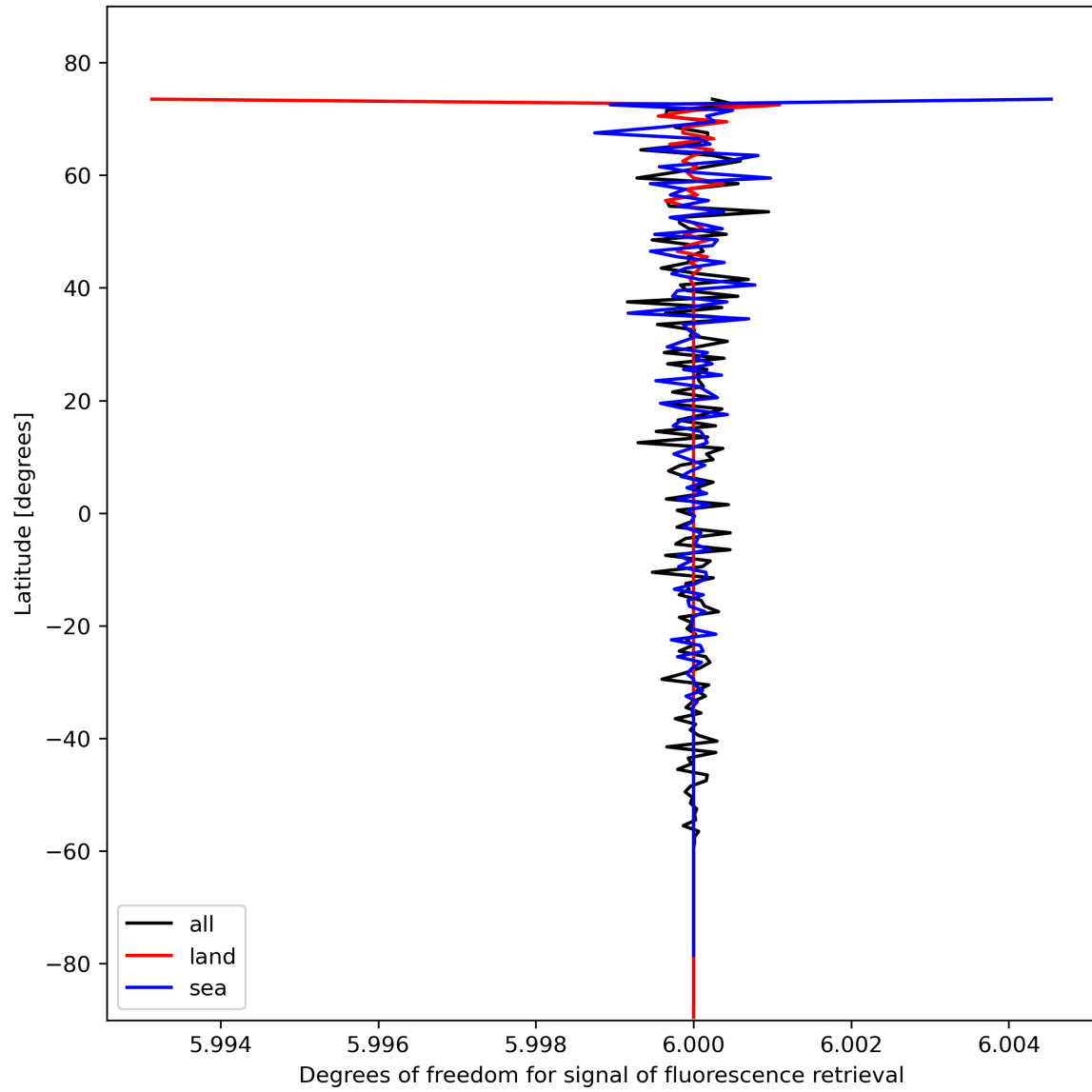
Figure 26: Zonal average of “Degrees of freedom for signal of fluorescence retrieval” for 2024-02-08 to 2024-02-10.
