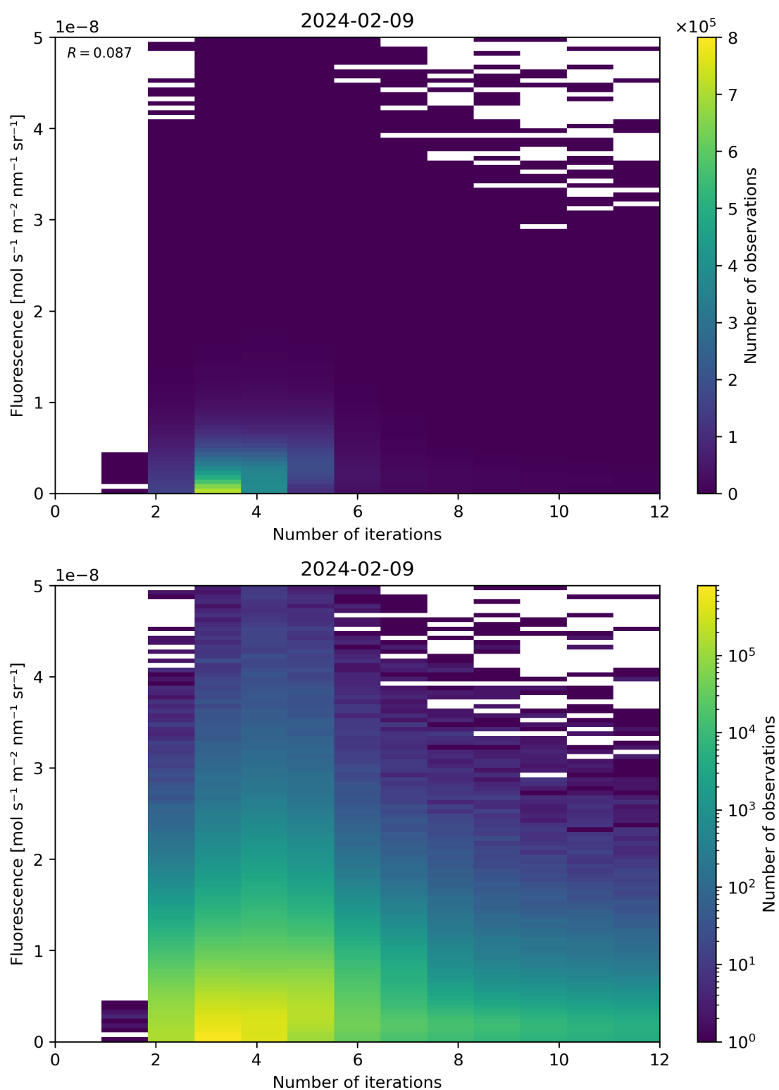
Figure 98: Scatter density plot of “Number of iterations” against “Fluorescence” for 2024-02-08 to 2024-02-10.
