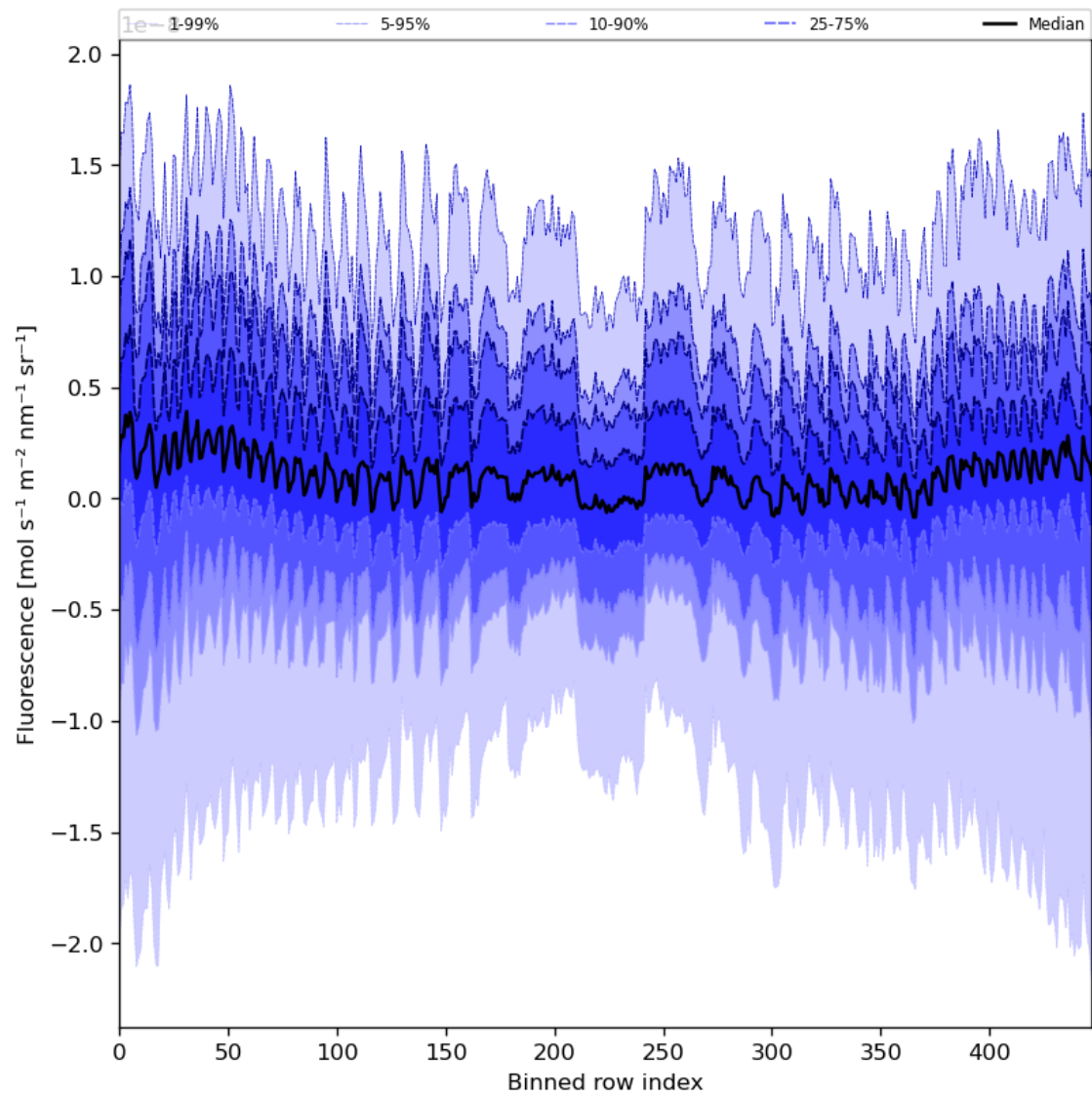
Figure 57: Along track statistics of “Fluorescence” for 2024-02-08 to 2024-02-10
