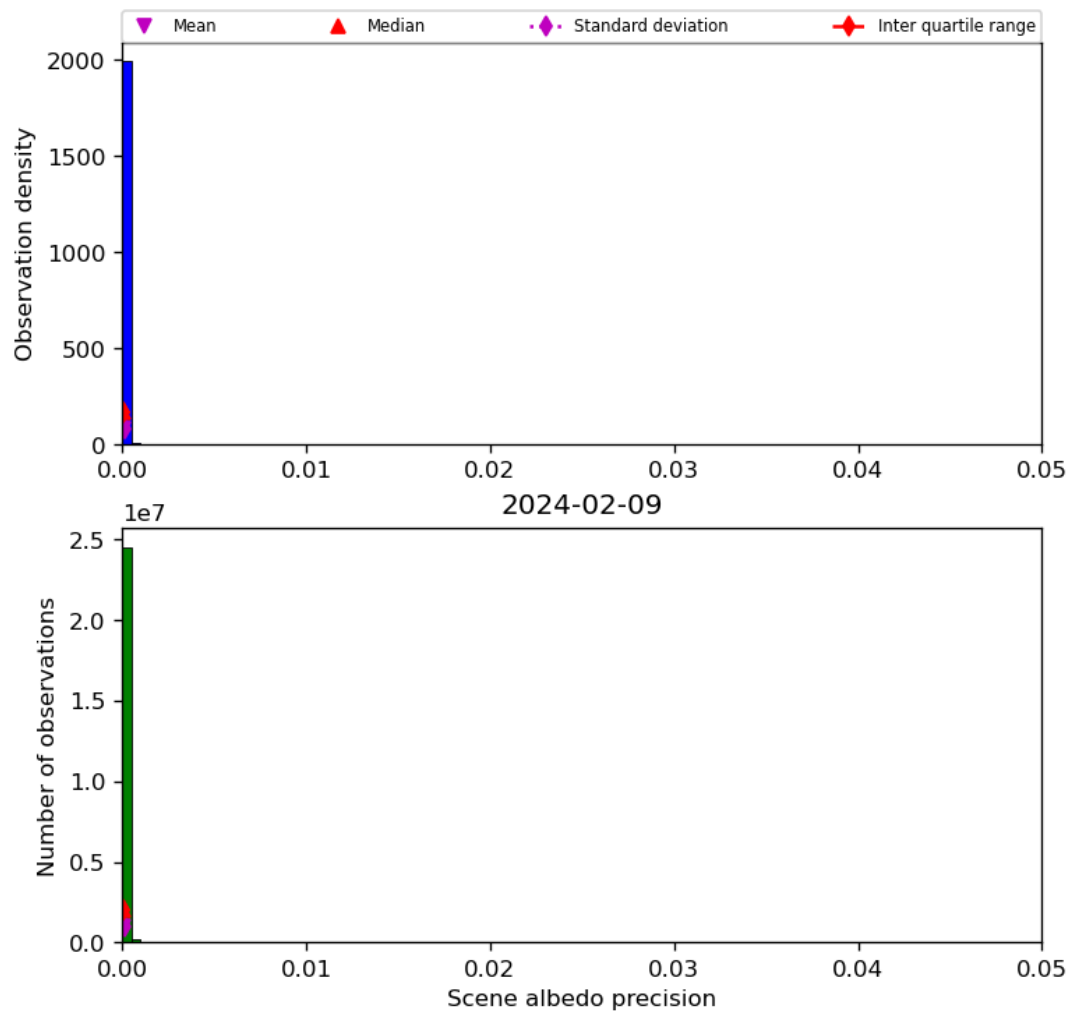
Figure 35: Histogram of “Scene albedo precision” for 2024-02-08 to 2024-02-10
