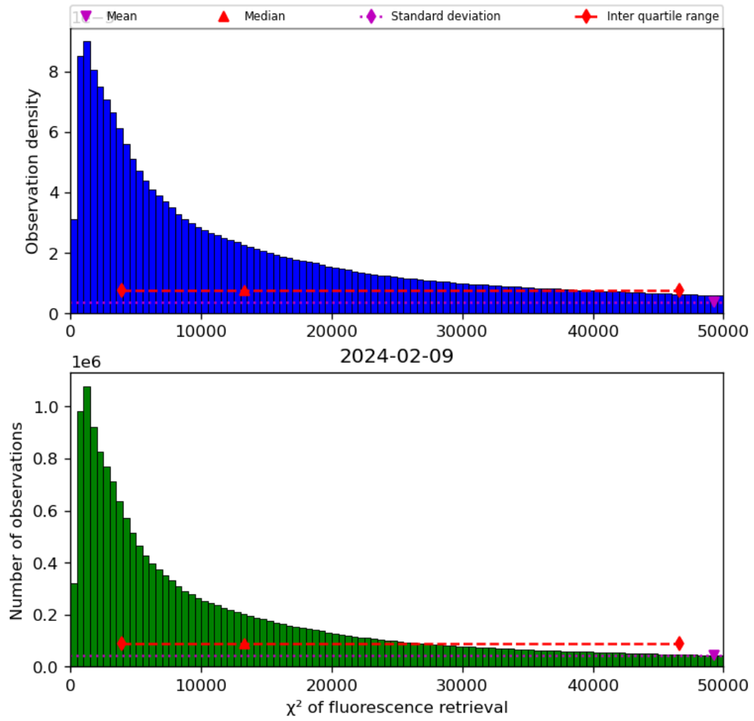
Figure 42: Histogram of “ \chi^2 of fluorescence retrieval” for 2024-02-08 to 2024-02-10
