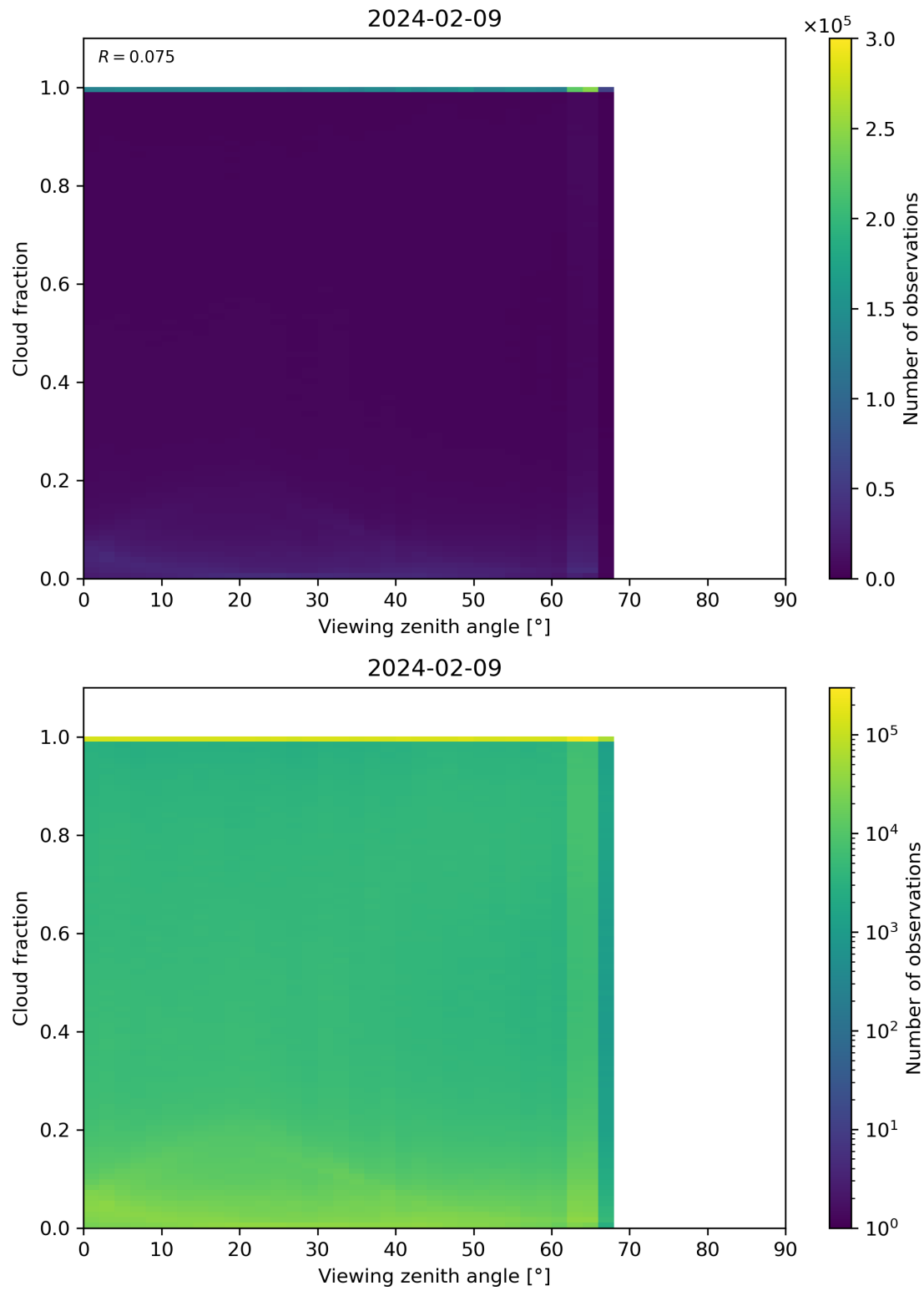
Figure 120: Scatter density plot of “Viewing zenith angle” against “Cloud fraction” for 2024-02-08 to 2024-02-10.
