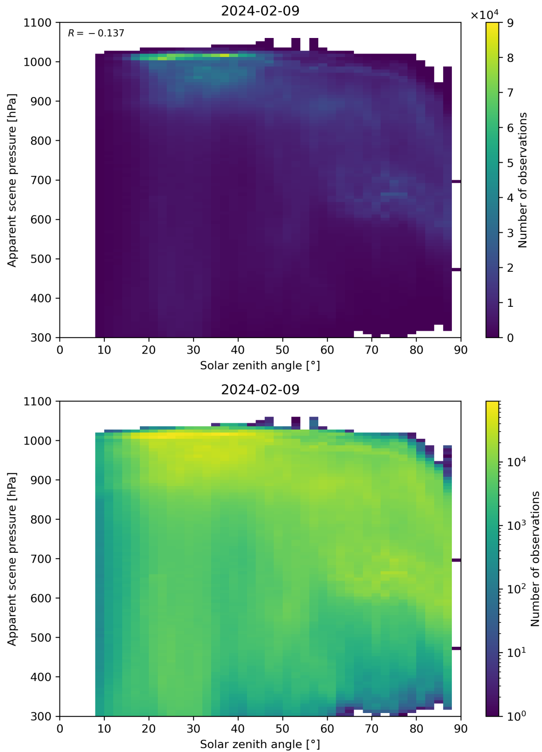
Figure 108: Scatter density plot of “Solar zenith angle” against “Apparent scene pressure” for 2024-02-08 to 2024-02-10.
