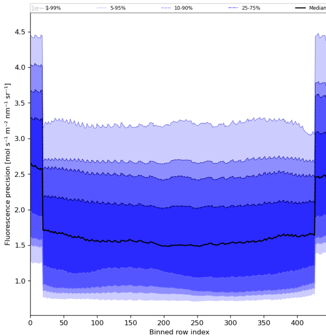
Figure 58: Along track statistics of “Fluorescence precision” for 2024-02-08 to 2024-02-10
