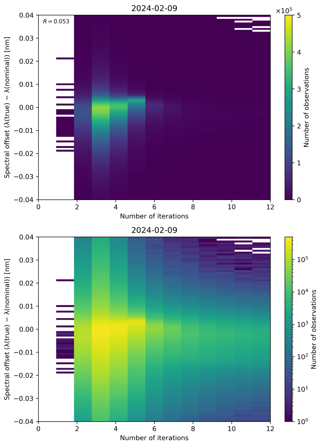
Figure 100: Scatter density plot of “Number of iterations” against “Spectral offset ( \lambda(\text{true}) - \lambda(\text{nominal}) )” for 2024-02-08 to 2024-02-10.
