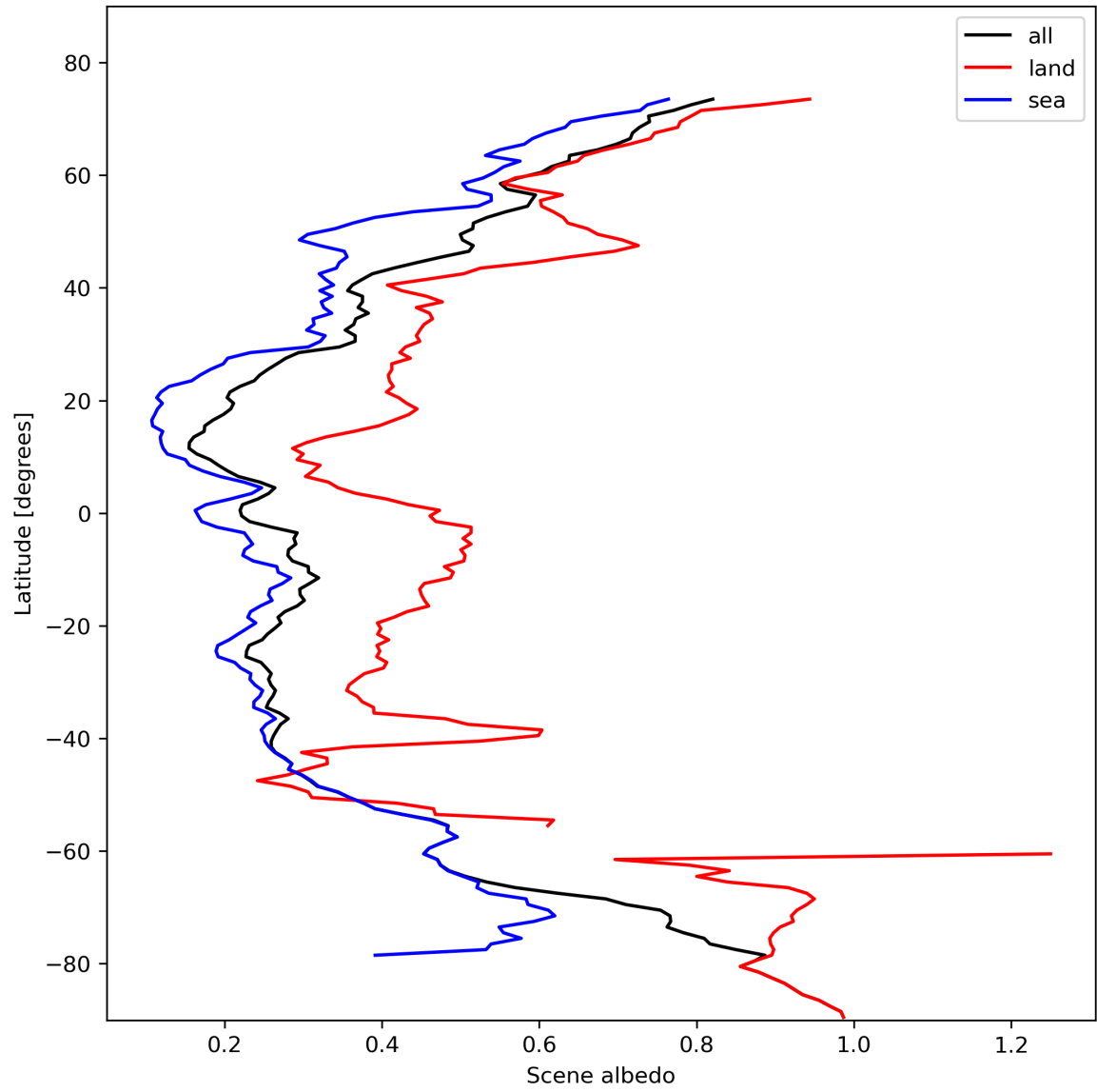
Figure 17: Zonal average of “Scene albedo” for 2024-02-08 to 2024-02-10.
