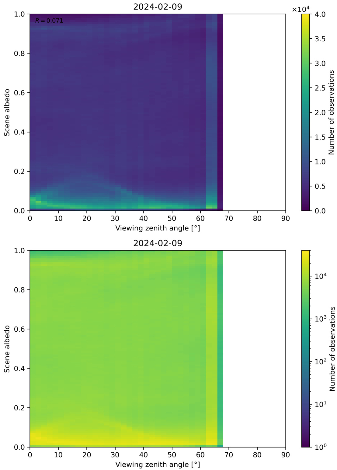
Figure 126: Scatter density plot of “Viewing zenith angle” against “Scene albedo” for 2024-02-08 to 2024-02-10.
