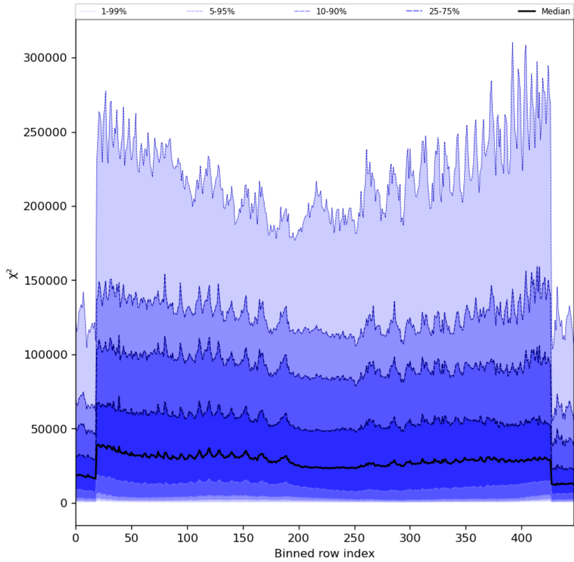
Figure 55: Along track statistics of “ \chi^2 ” for 2024-02-08 to 2024-02-10
