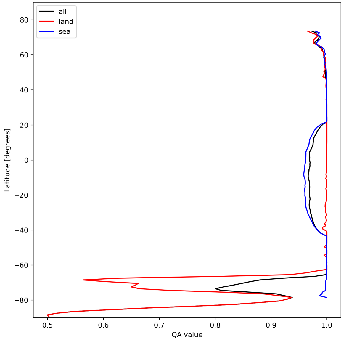
Figure 12: Zonal average of “QA value” for 2024-02-08 to 2024-02-10.
