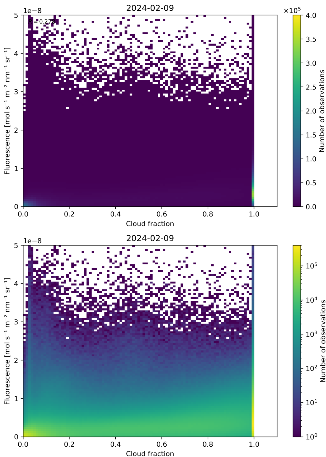
Figure 72: Scatter density plot of “Cloud fraction” against “Fluorescence” for 2024-02-08 to 2024-02-10.
