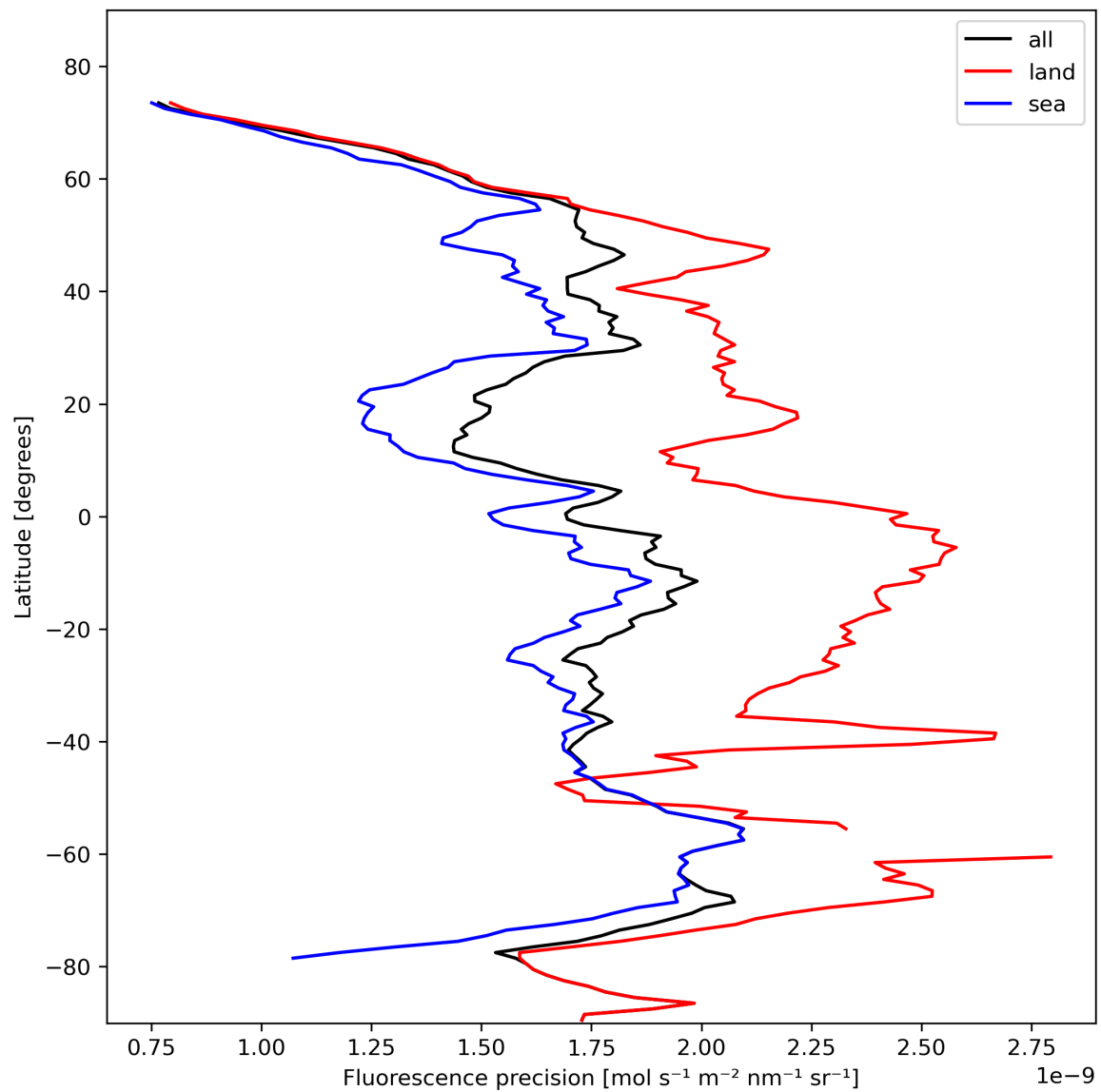
Figure 24: Zonal average of “Fluorescence precision” for 2024-02-08 to 2024-02-10.
