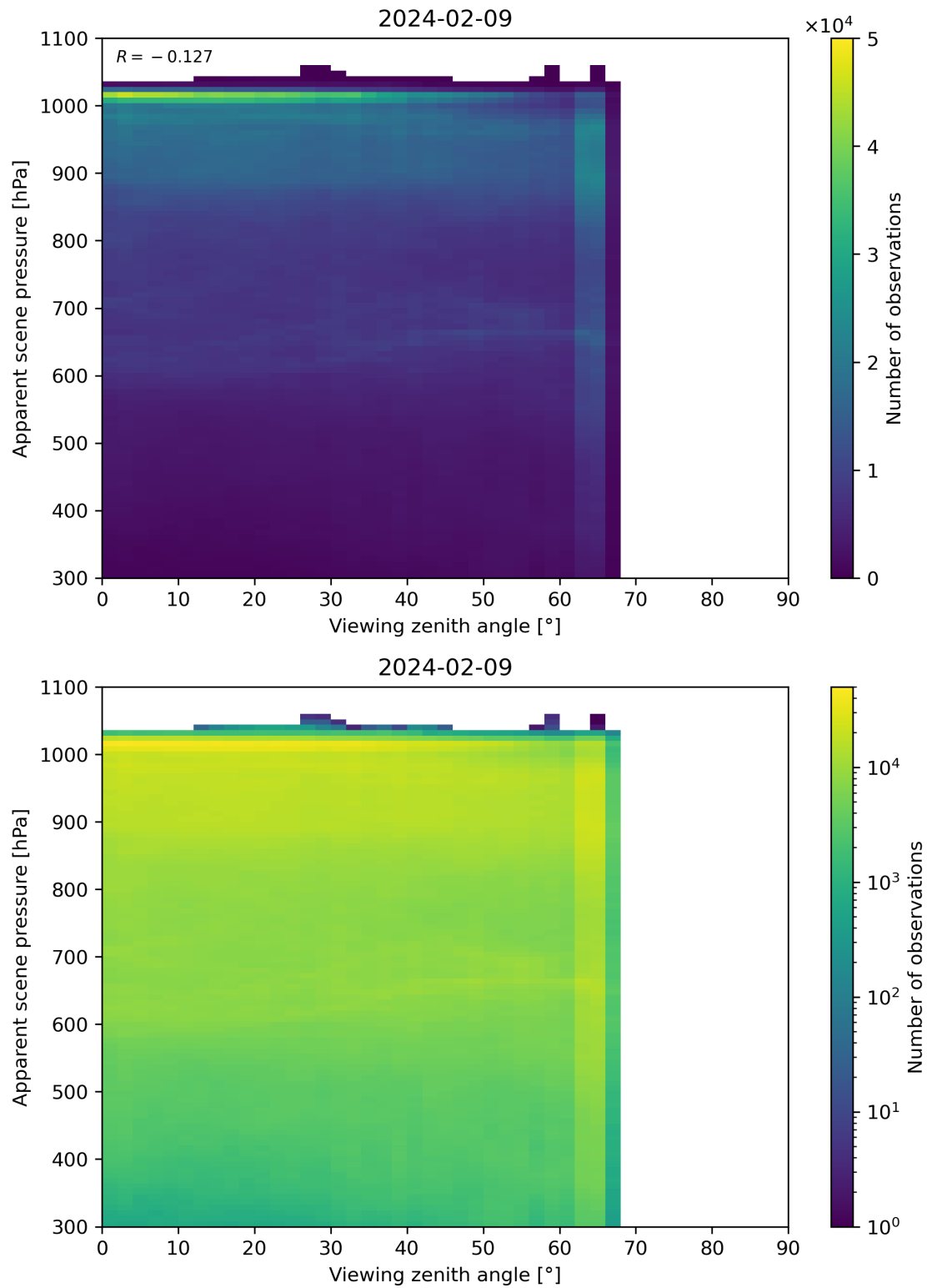
Figure 118: Scatter density plot of “Viewing zenith angle” against “Apparent scene pressure” for 2024-02-08 to 2024-02-10.
