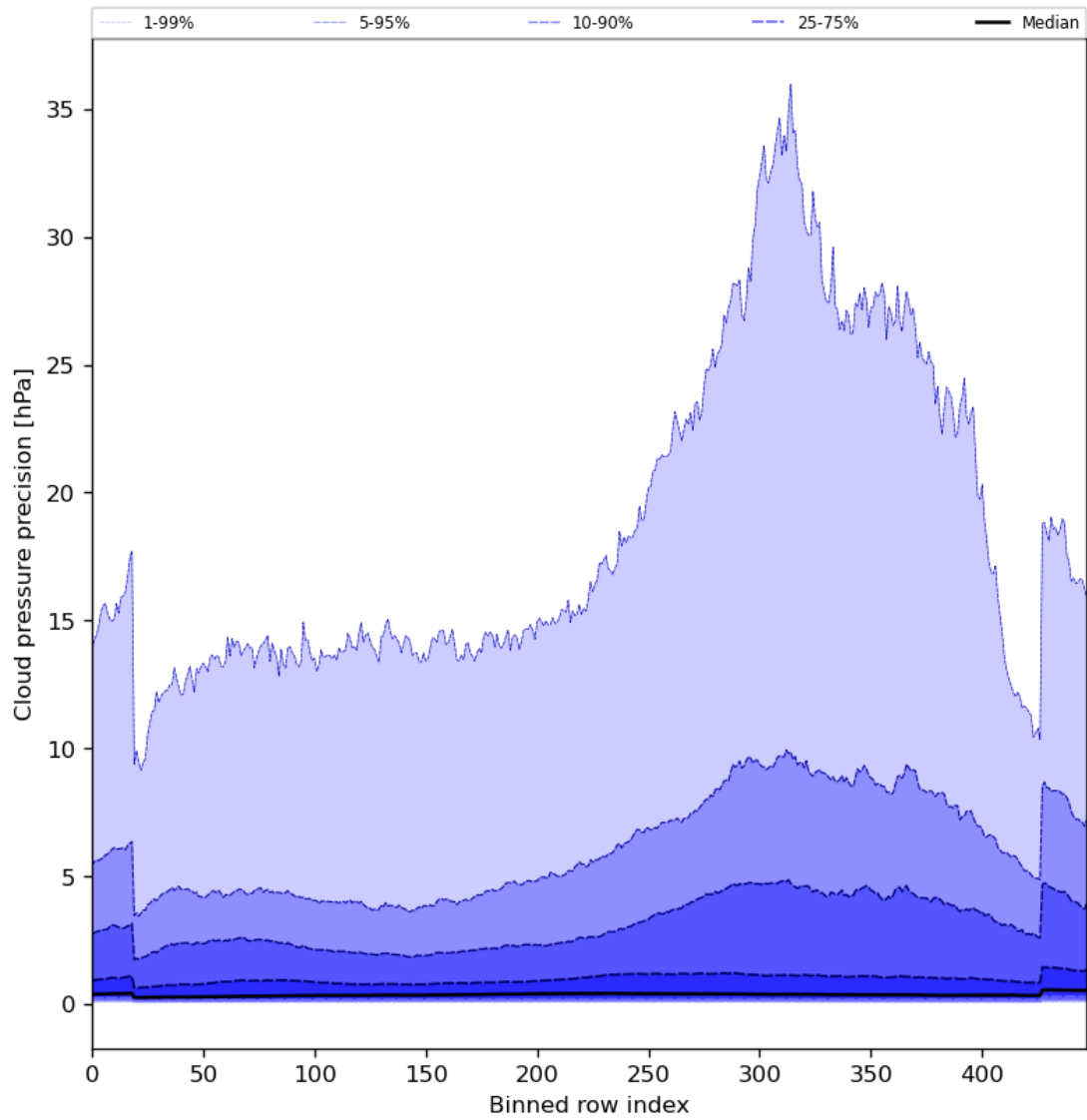
Figure 48: Along track statistics of “Cloud pressure precision” for 2024-02-08 to 2024-02-10
