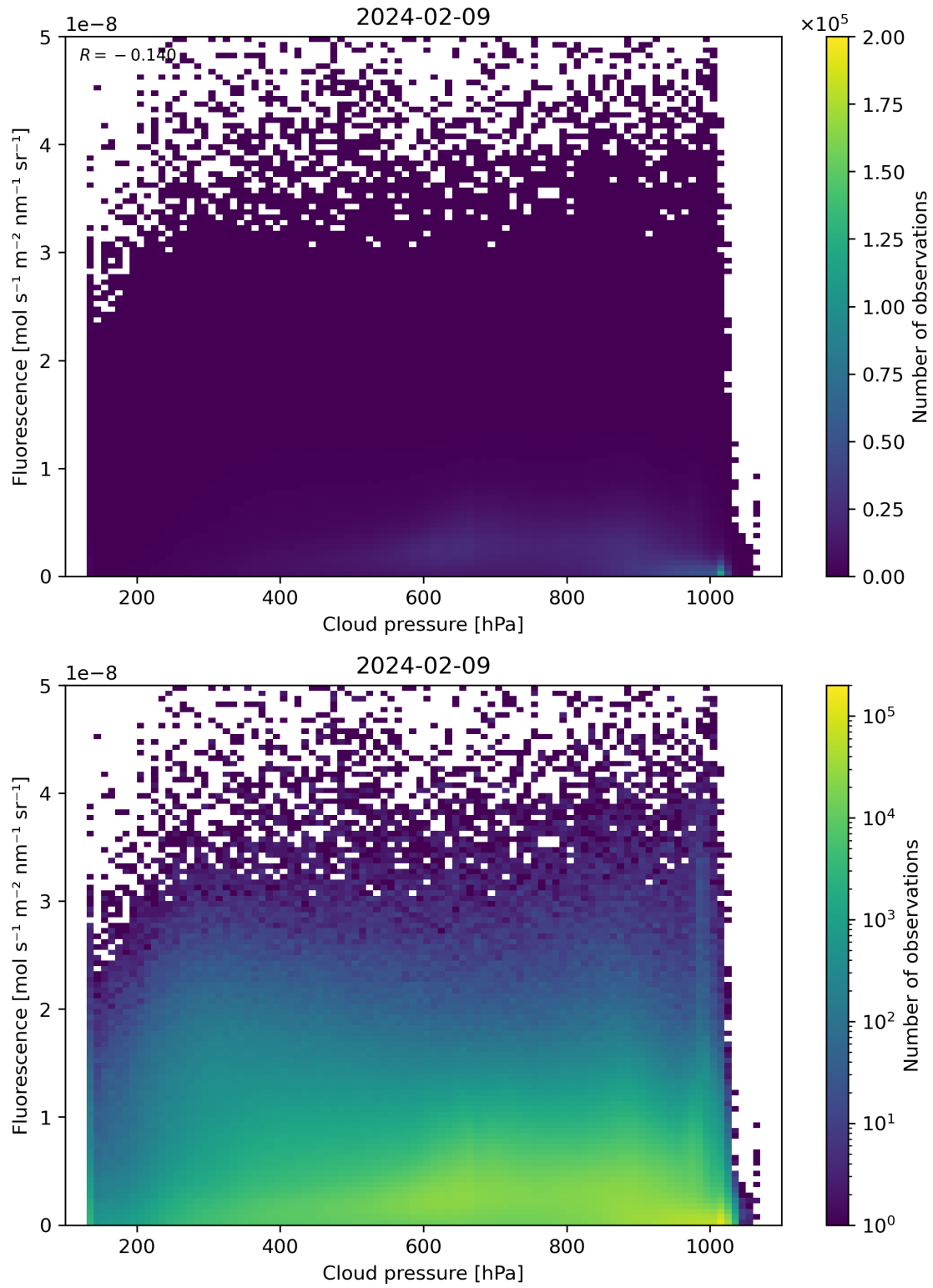
Figure 80: Scatter density plot of “Cloud pressure” against “Fluorescence” for 2024-02-08 to 2024-02-10.
