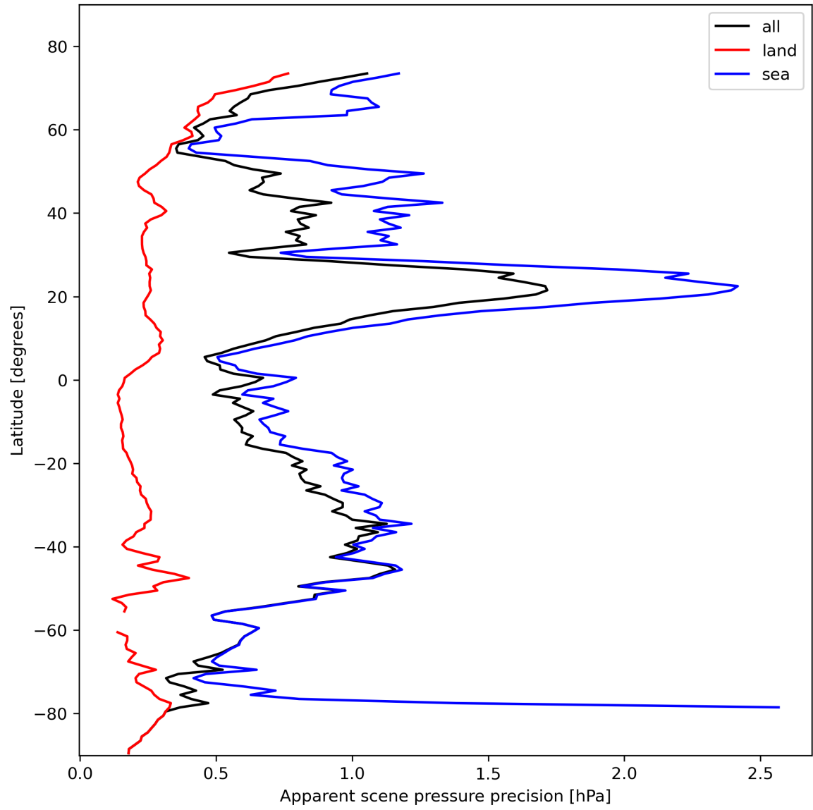
Figure 20: Zonal average of “Apparent scene pressure precision” for 2024-02-08 to 2024-02-10.
