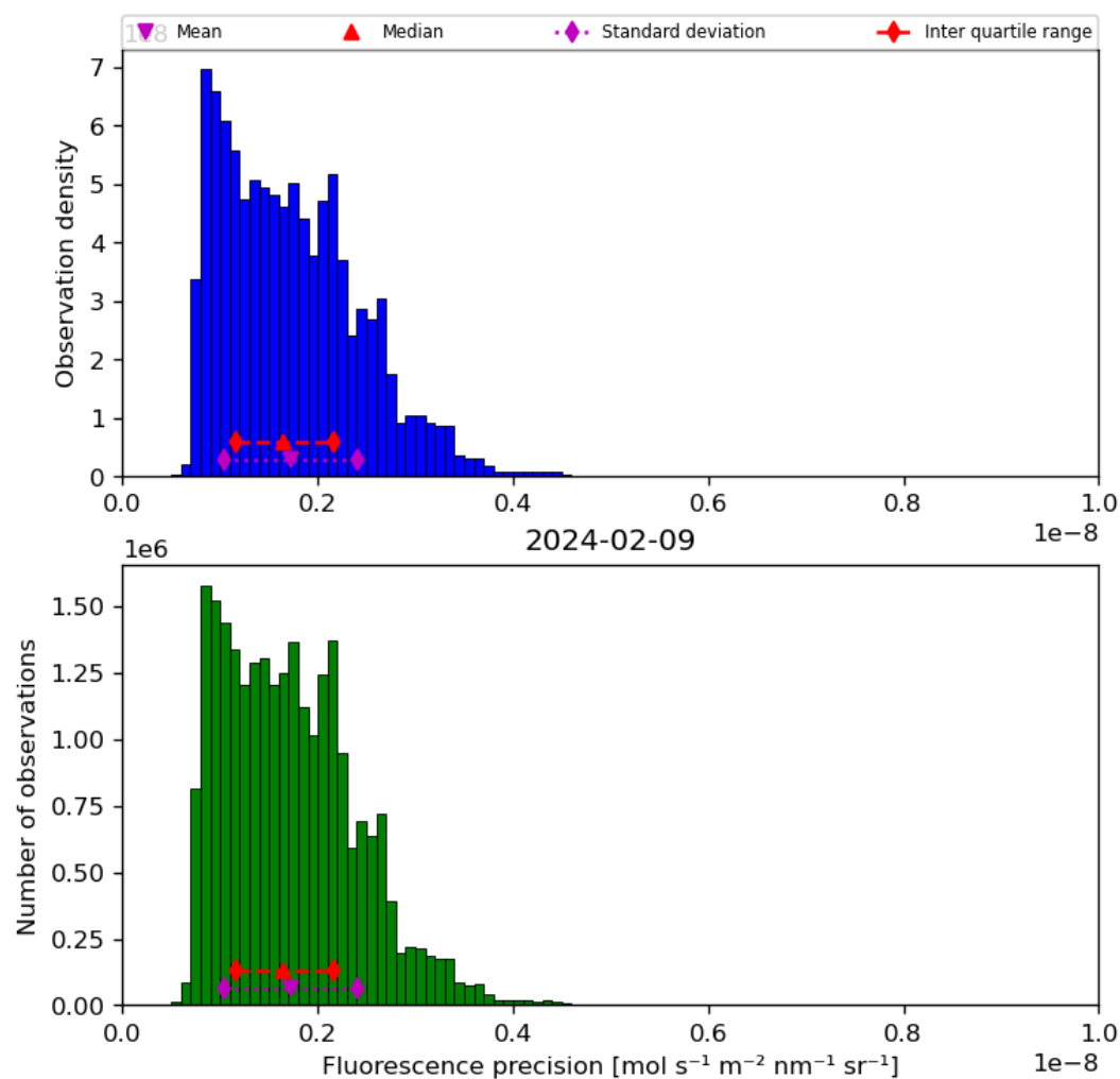
Figure 41: Histogram of “Fluorescence precision” for 2024-02-08 to 2024-02-10
