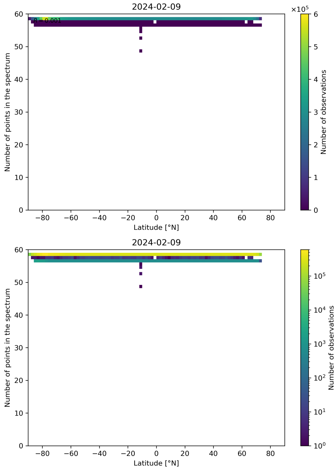
Figure 94: Scatter density plot of “Latitude” against “Number of points in the spectrum” for 2024-02-08 to 2024-02-10.
