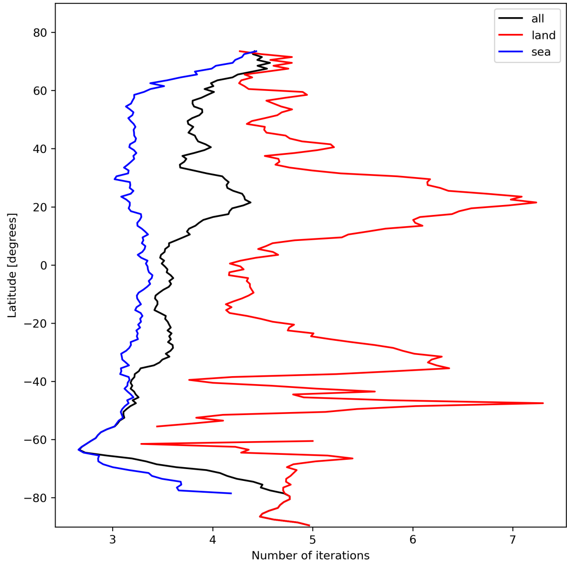
Figure 22: Zonal average of “Number of iterations” for 2024-02-08 to 2024-02-10.
