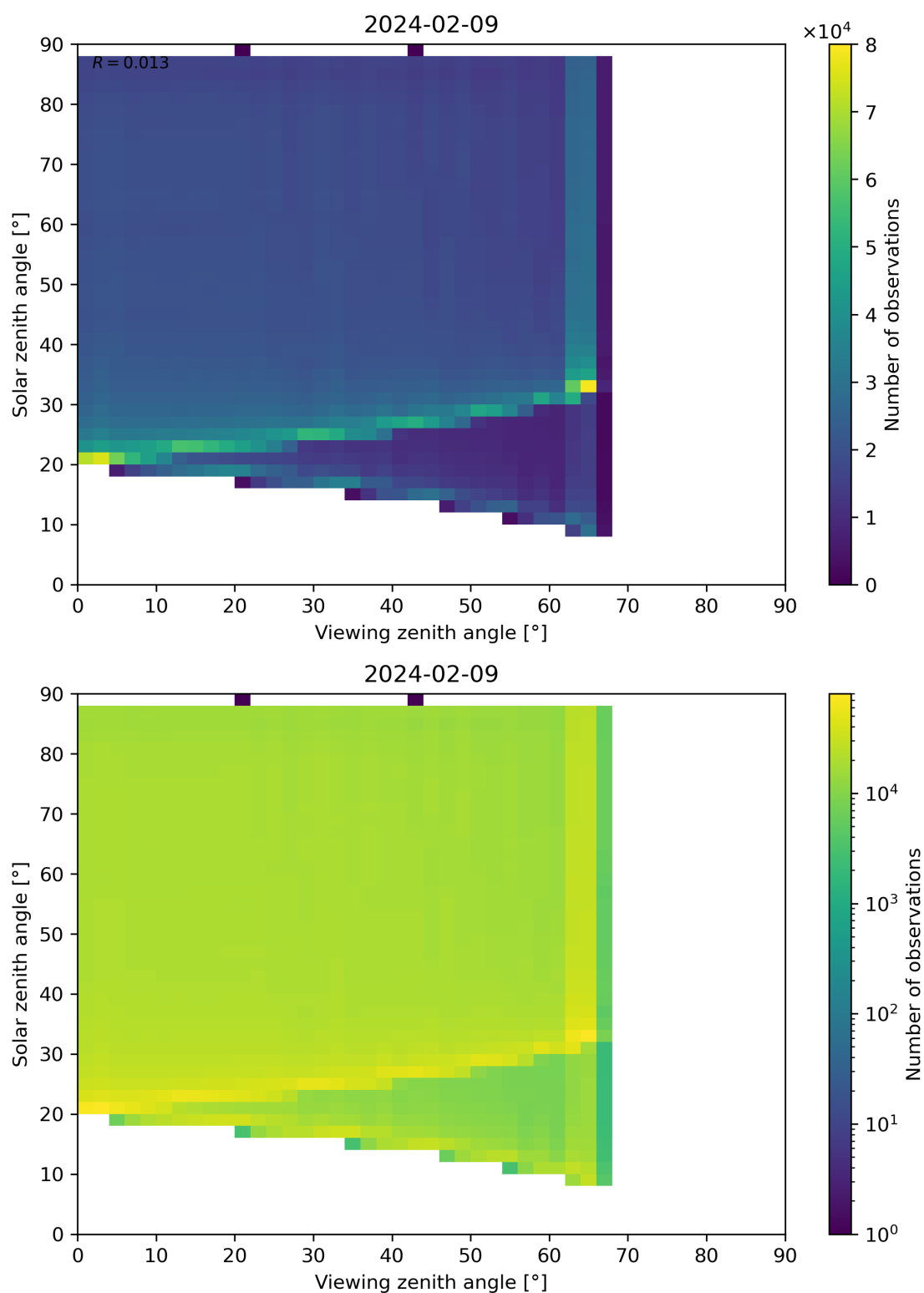
Figure 127: Scatter density plot of “Viewing zenith angle” against “Solar zenith angle” for 2024-02-08 to 2024-02-10.
