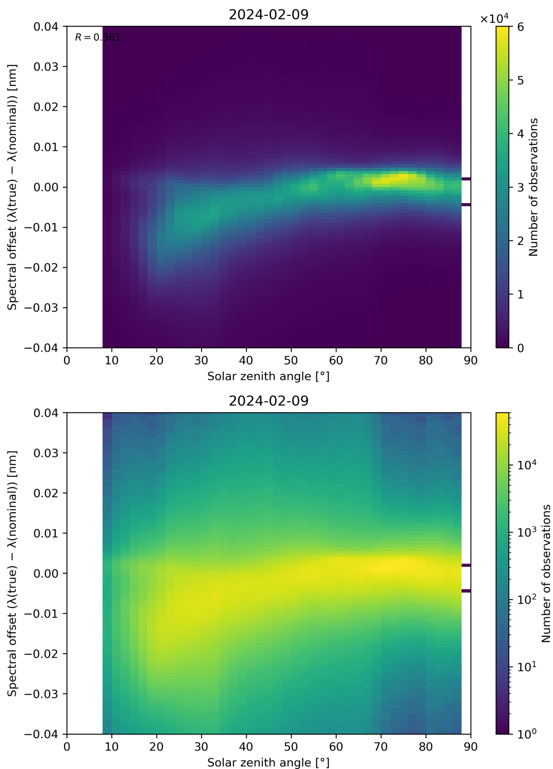
Figure 117: Scatter density plot of “Solar zenith angle” against “Spectral offset ( \lambda(\text{true}) - \lambda(\text{nominal}) )” for 2024-02-08 to 2024-02-10.
