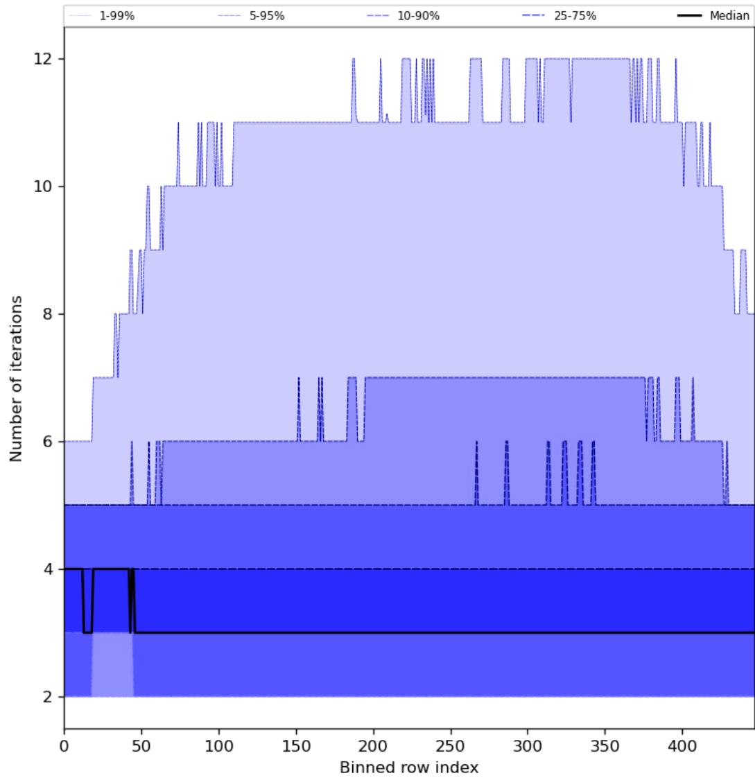
Figure 56: Along track statistics of “Number of iterations” for 2024-02-08 to 2024-02-10
