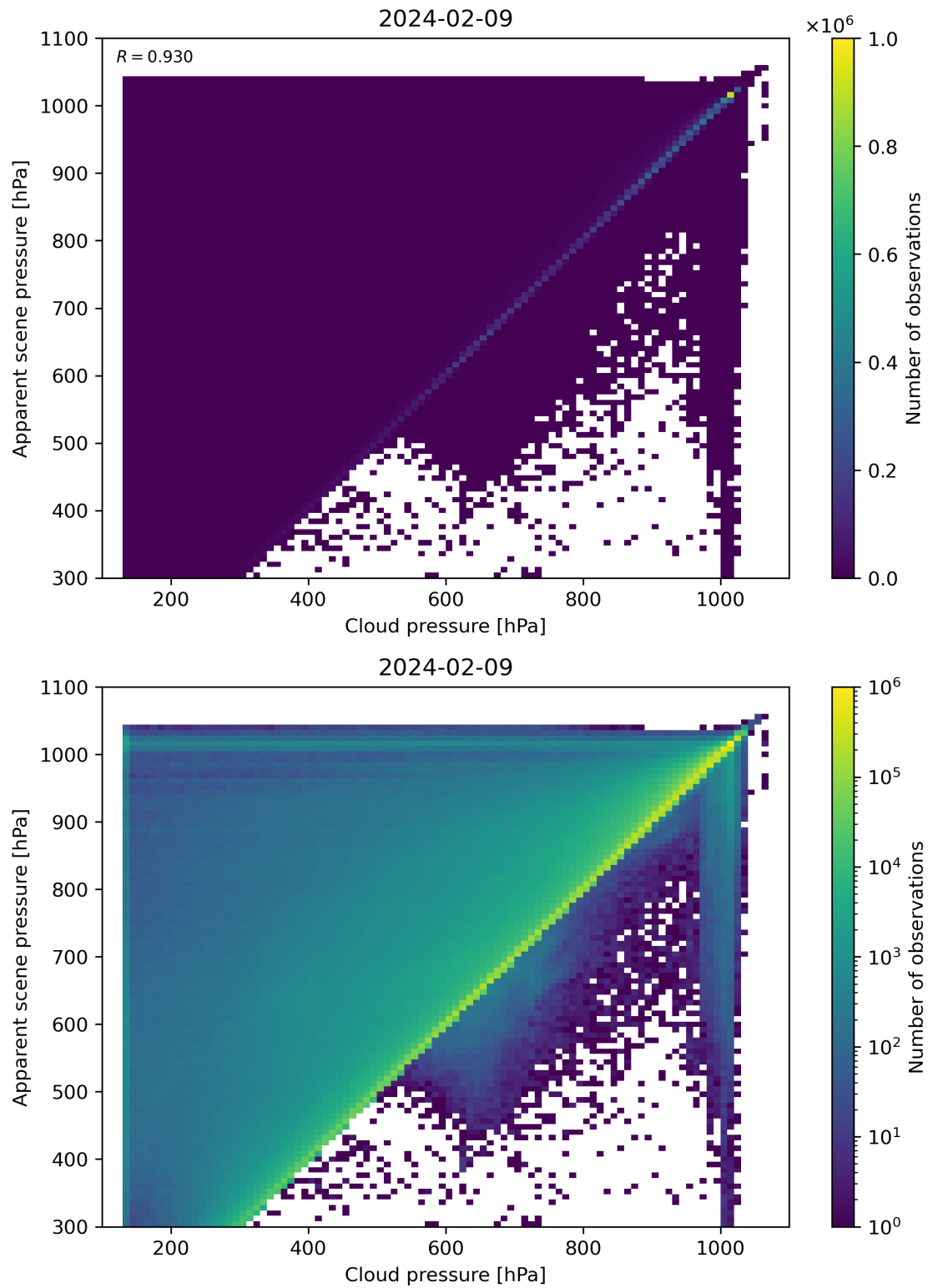
Figure 77: Scatter density plot of “Cloud pressure” against “Apparent scene pressure” for 2024-02-08 to 2024-02-10.
