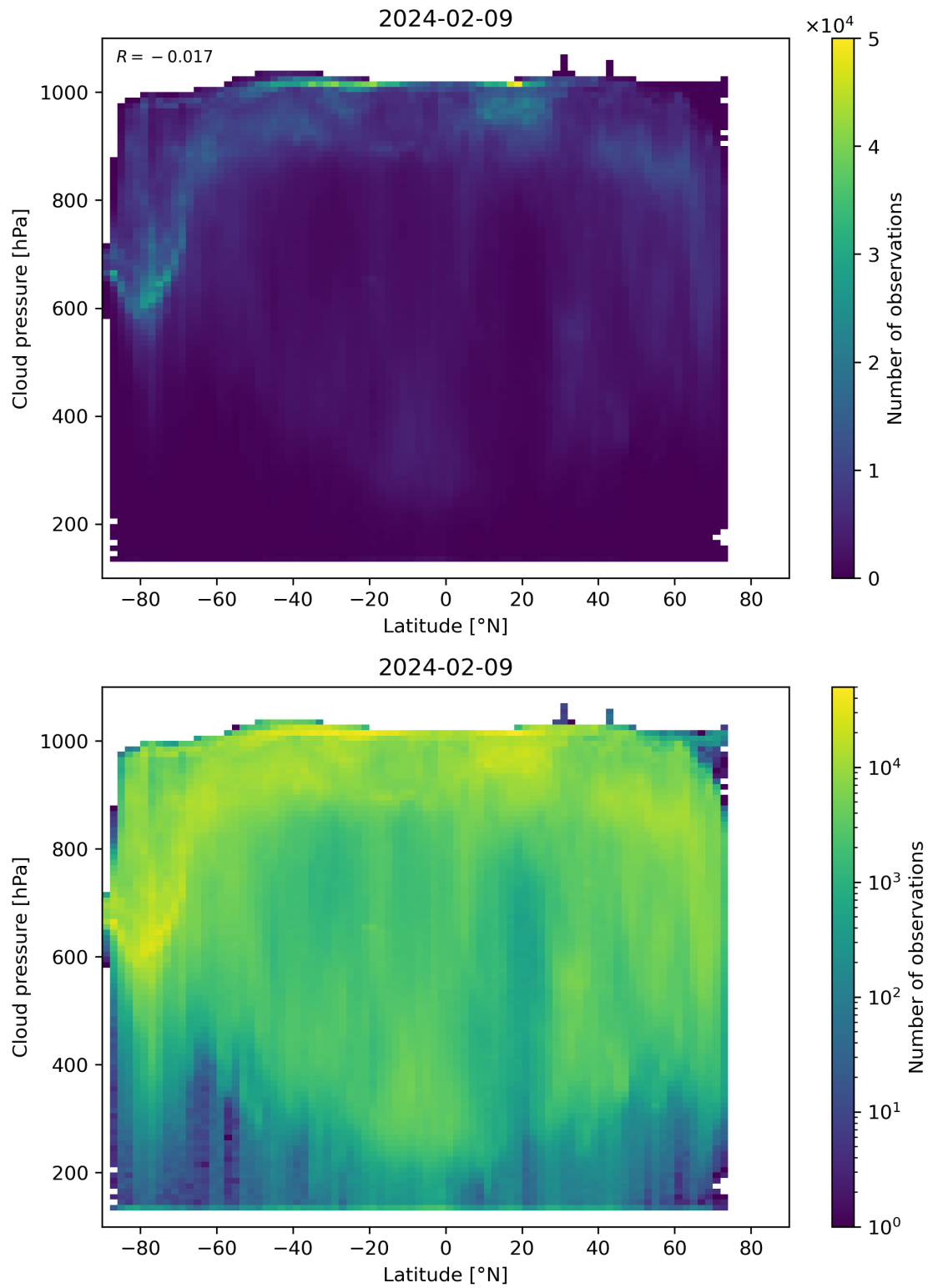
Figure 91: Scatter density plot of “Latitude” against “Cloud pressure” for 2024-02-08 to 2024-02-10.
