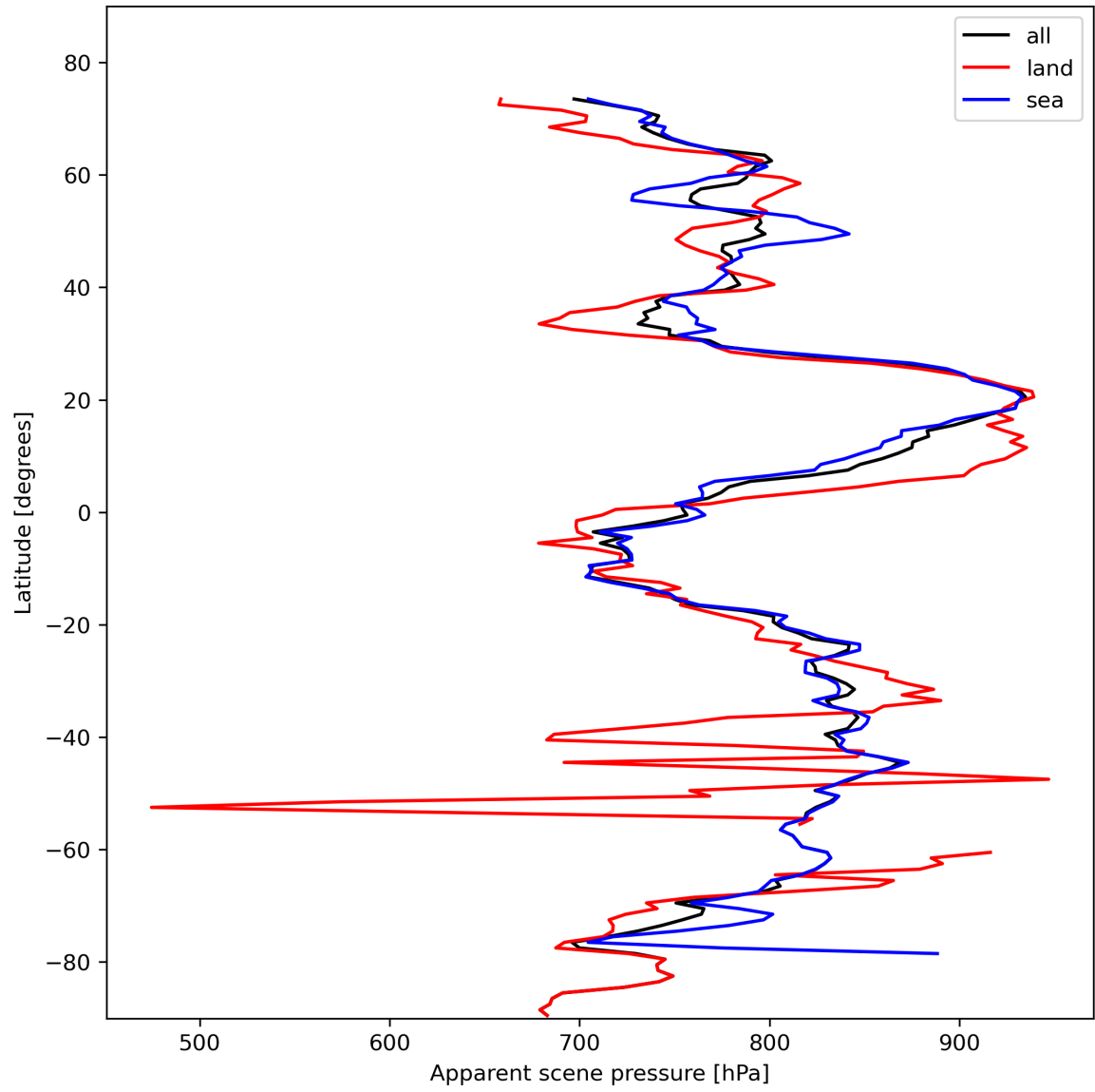
Figure 19: Zonal average of “Apparent scene pressure” for 2024-02-08 to 2024-02-10.
