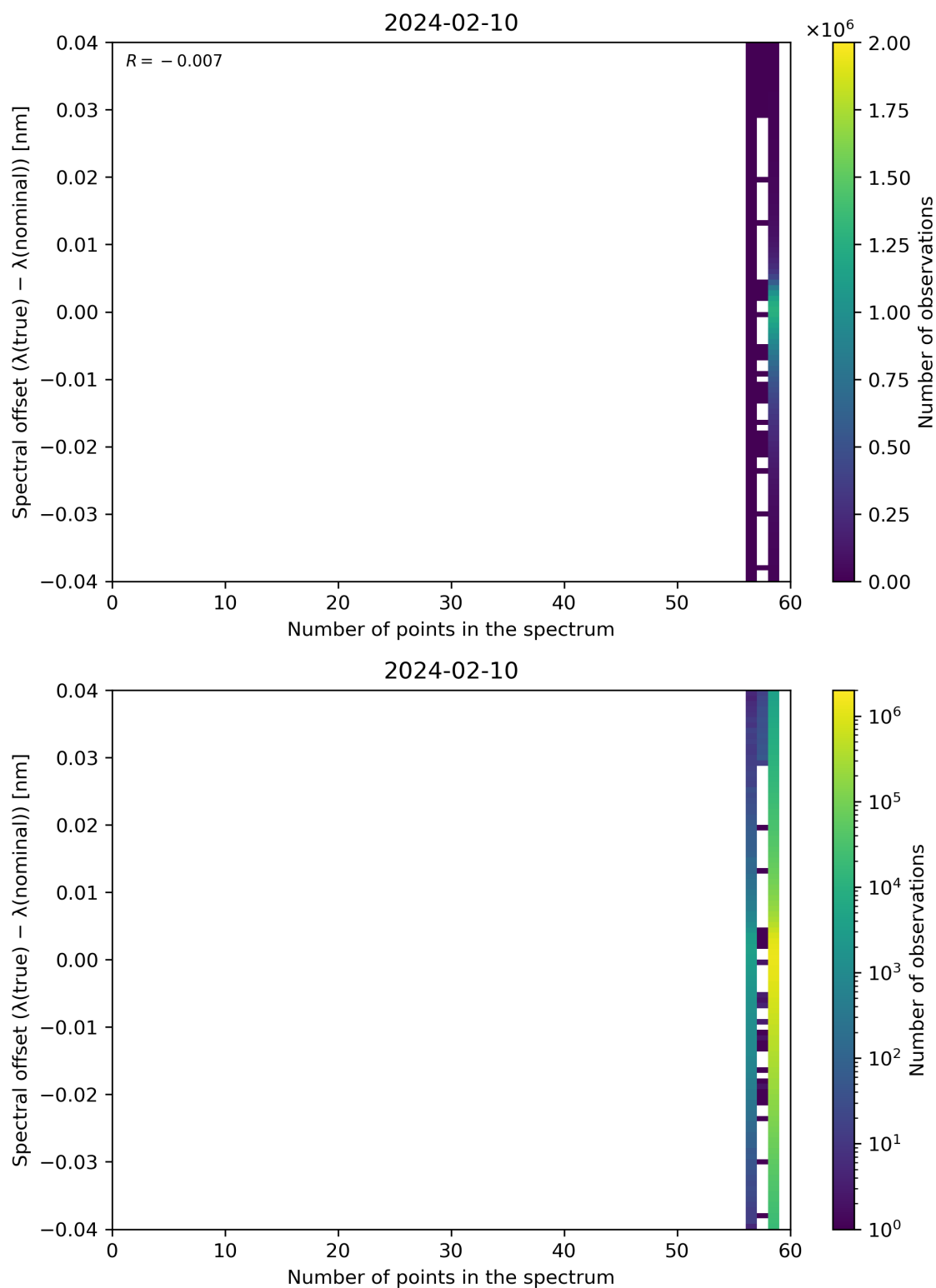
Figure 101: Scatter density plot of “Number of points in the spectrum” against “Spectral offset ( \lambda(\text{true}) - \lambda(\text{nominal}) )” for 2024-02-09 to 2024-02-11.
