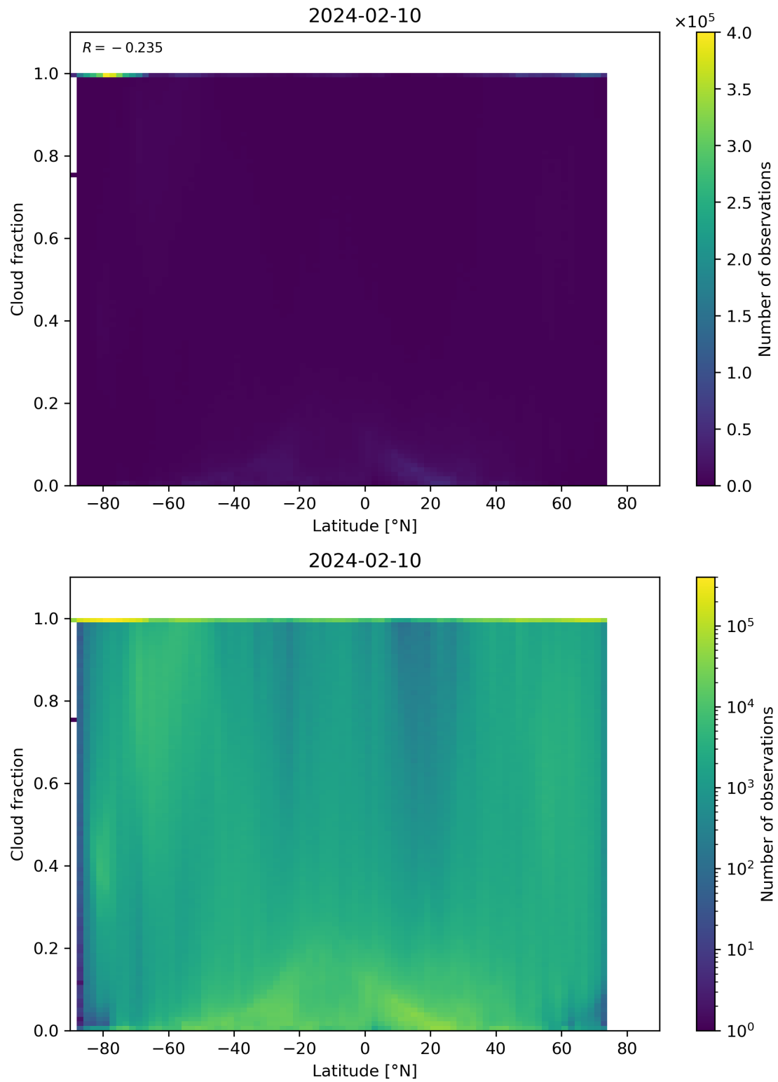
Figure 90: Scatter density plot of “Latitude” against “Cloud fraction” for 2024-02-09 to 2024-02-11.
