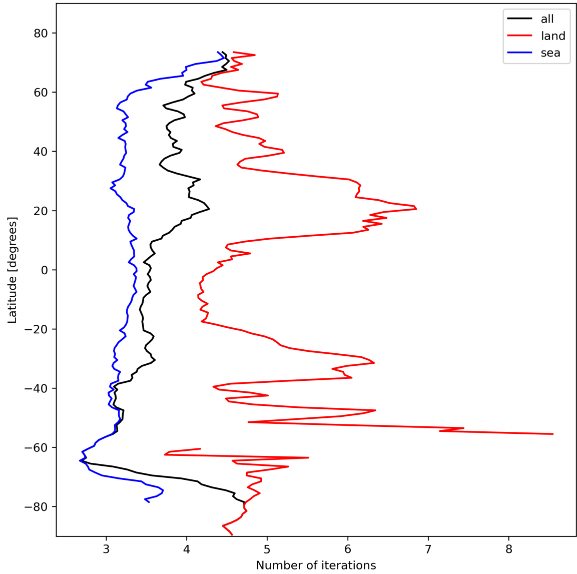
Figure 22: Zonal average of “Number of iterations” for 2024-02-09 to 2024-02-11.
