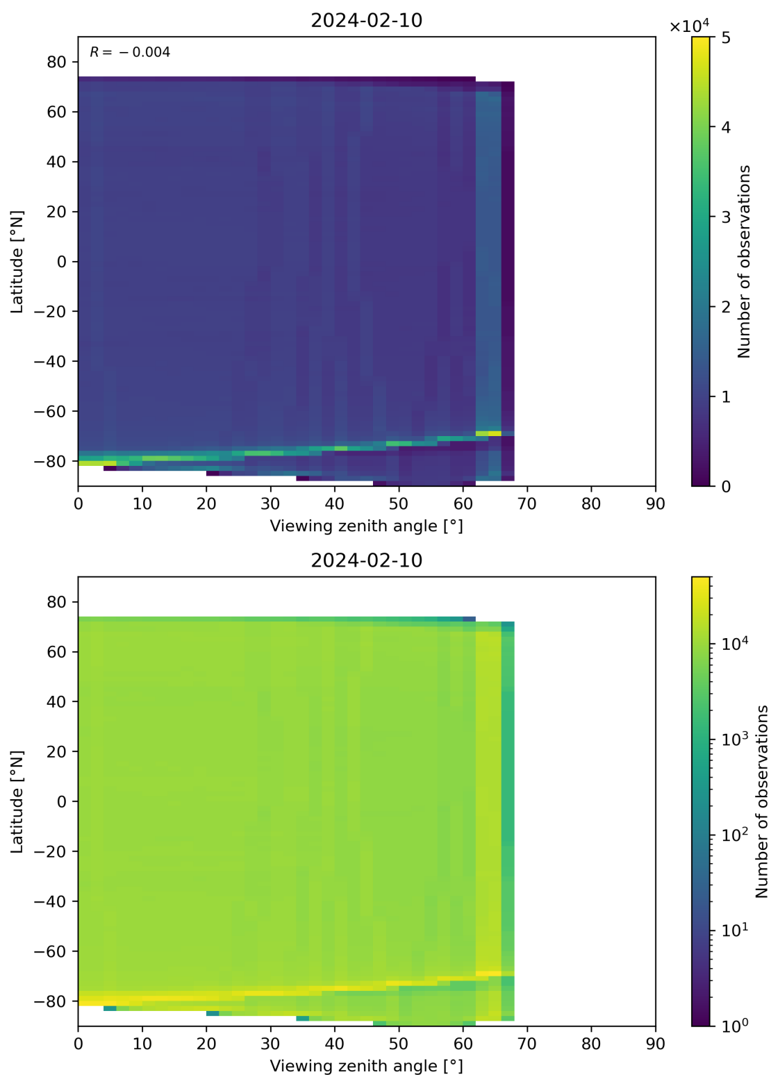
Figure 123: Scatter density plot of “Viewing zenith angle” against “Latitude” for 2024-02-09 to 2024-02-11.
