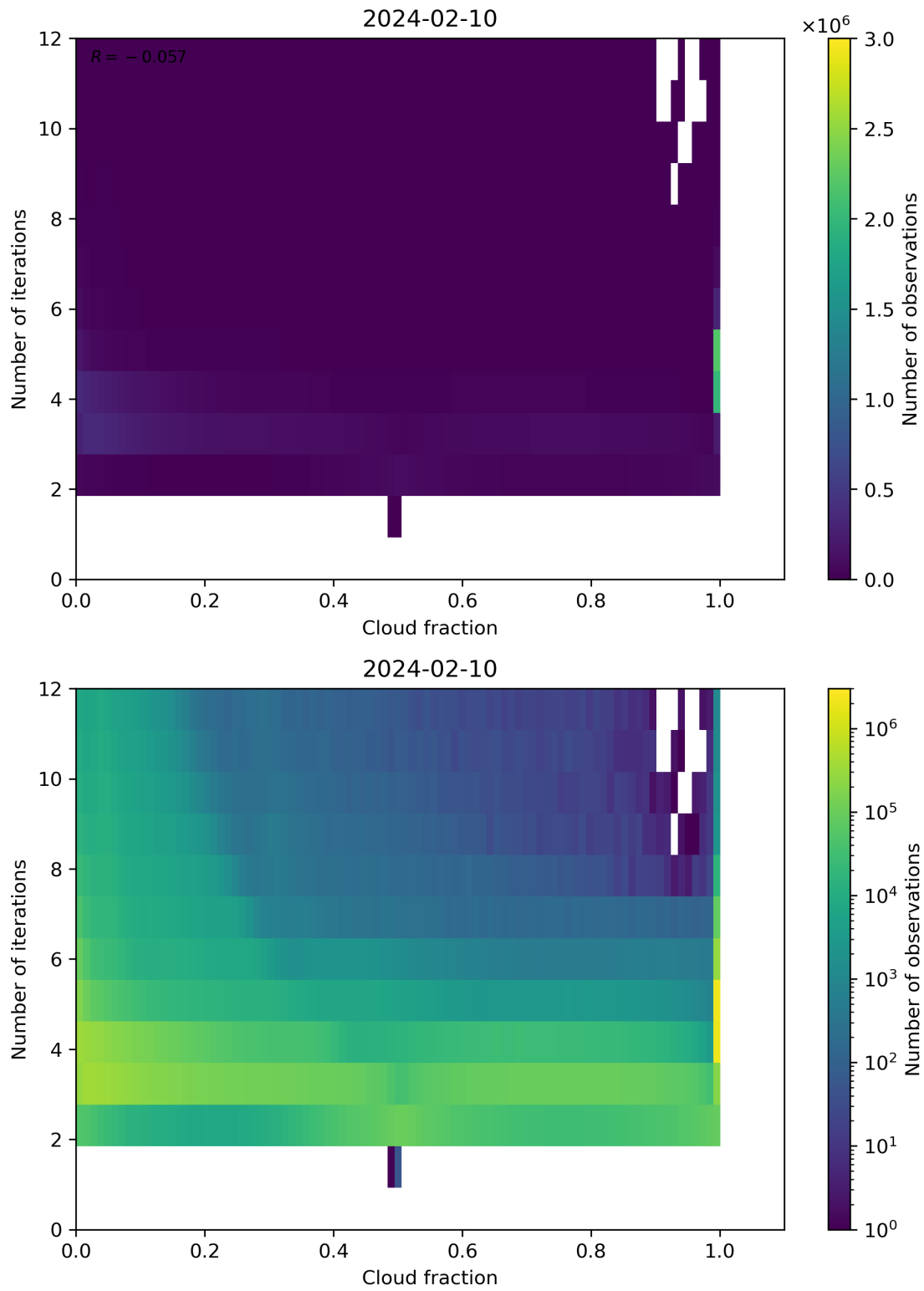
Figure 73: Scatter density plot of “Cloud fraction” against “Number of iterations” for 2024-02-09 to 2024-02-11.
