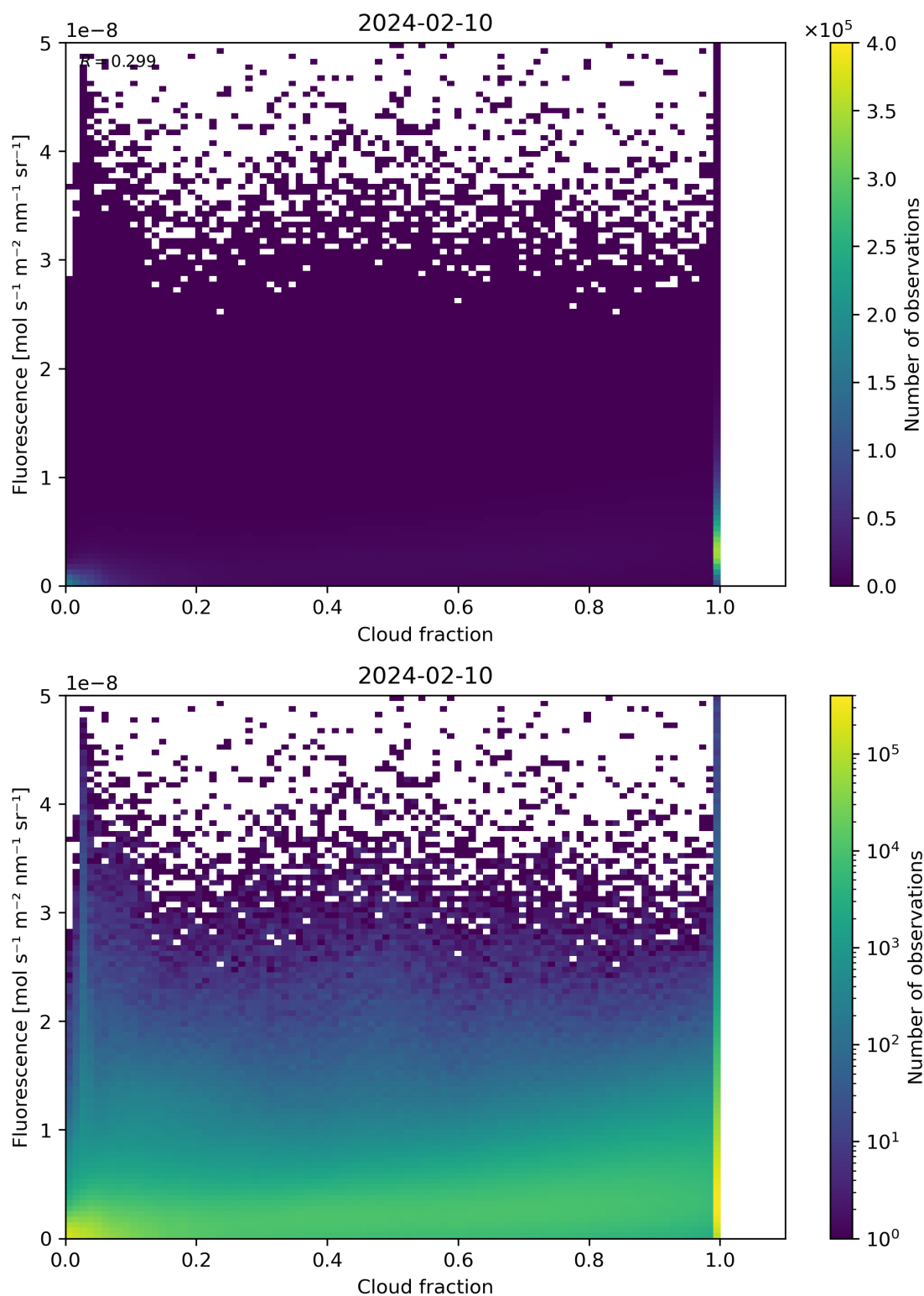
Figure 72: Scatter density plot of “Cloud fraction” against “Fluorescence” for 2024-02-09 to 2024-02-11.
