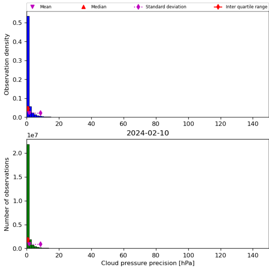
Figure 31: Histogram of “Cloud pressure precision” for 2024-02-09 to 2024-02-11
