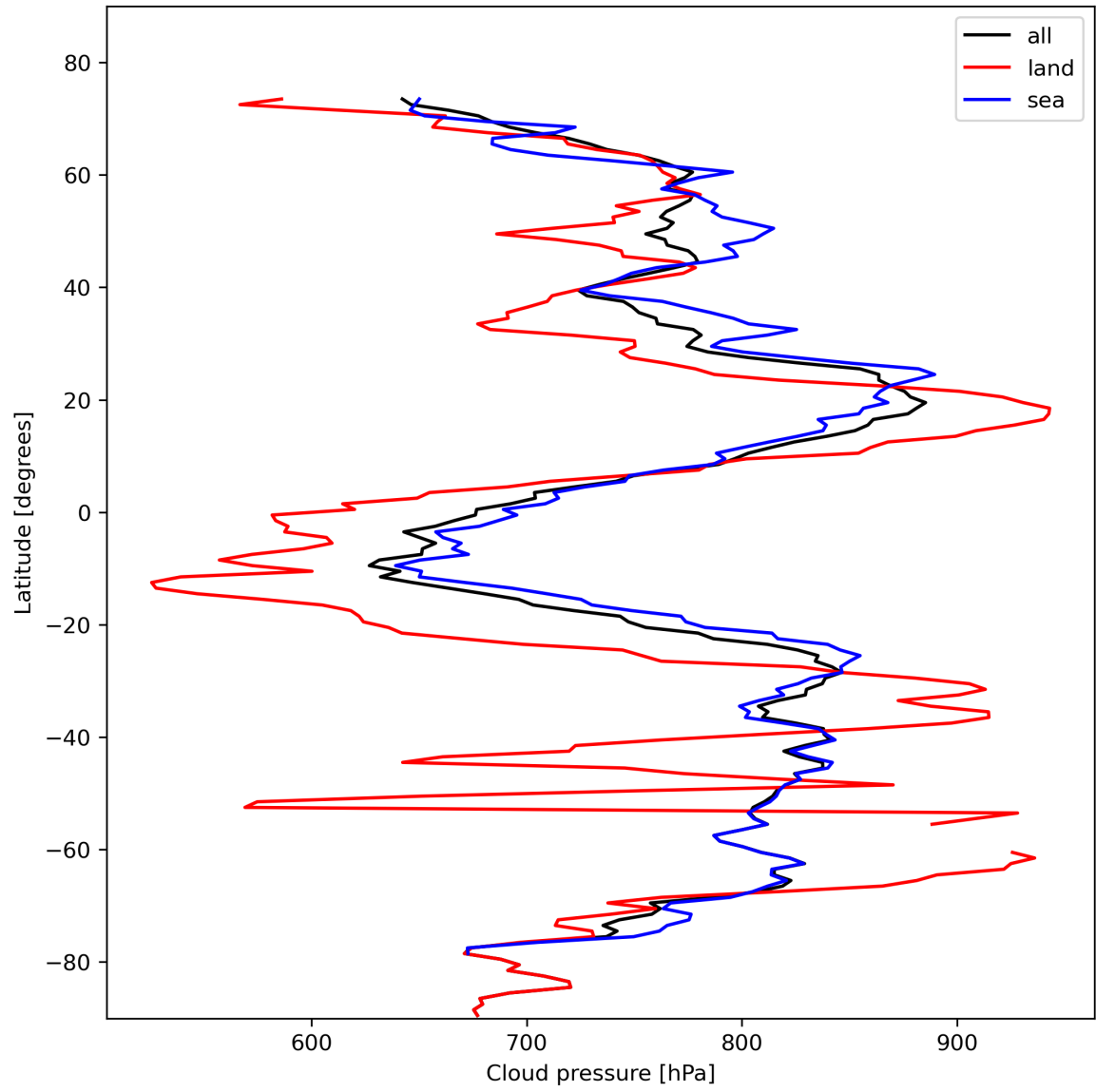
Figure 13: Zonal average of “Cloud pressure” for 2024-02-09 to 2024-02-11.
