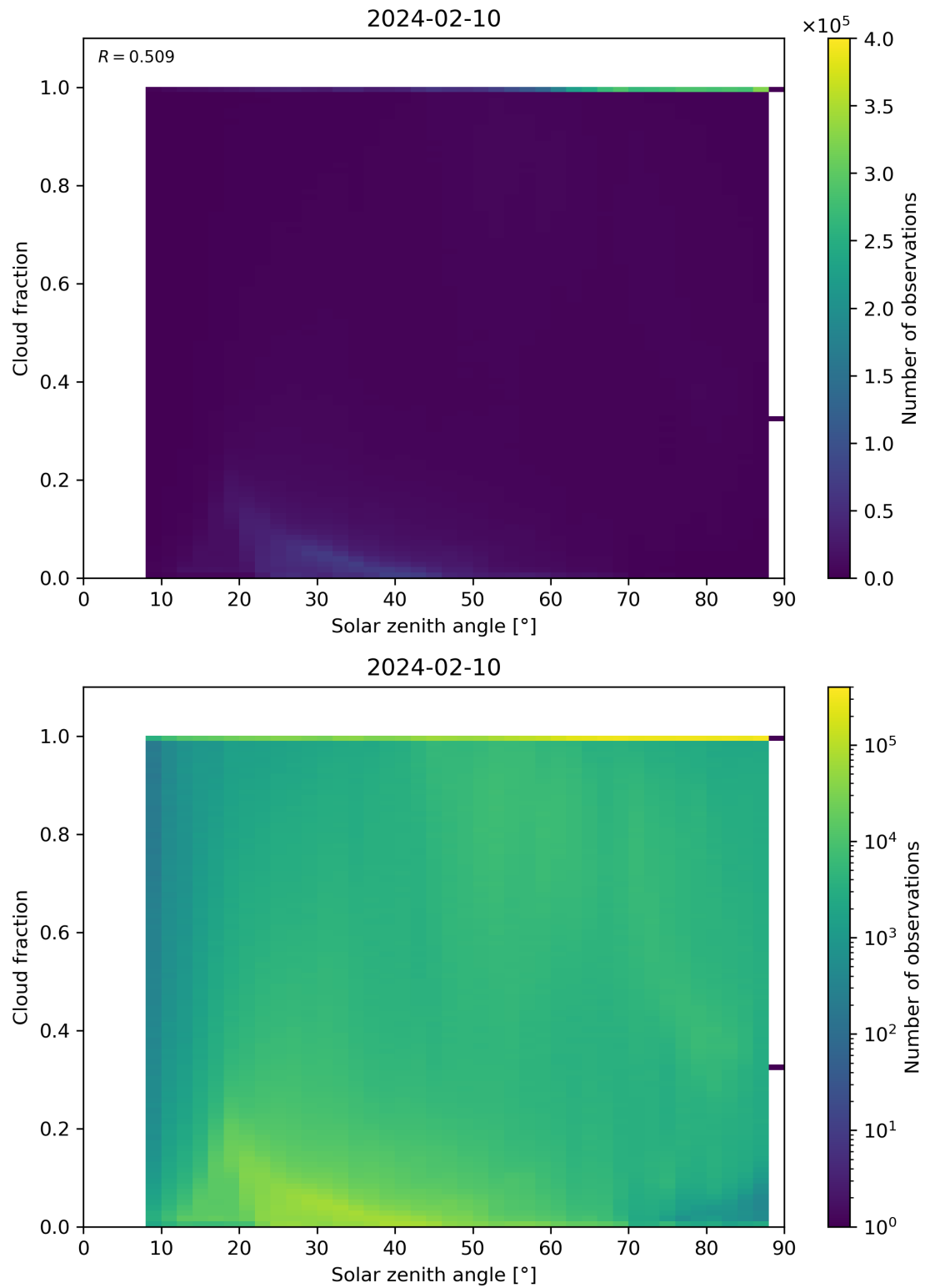
Figure 110: Scatter density plot of “Solar zenith angle” against “Cloud fraction” for 2024-02-09 to 2024-02-11.
