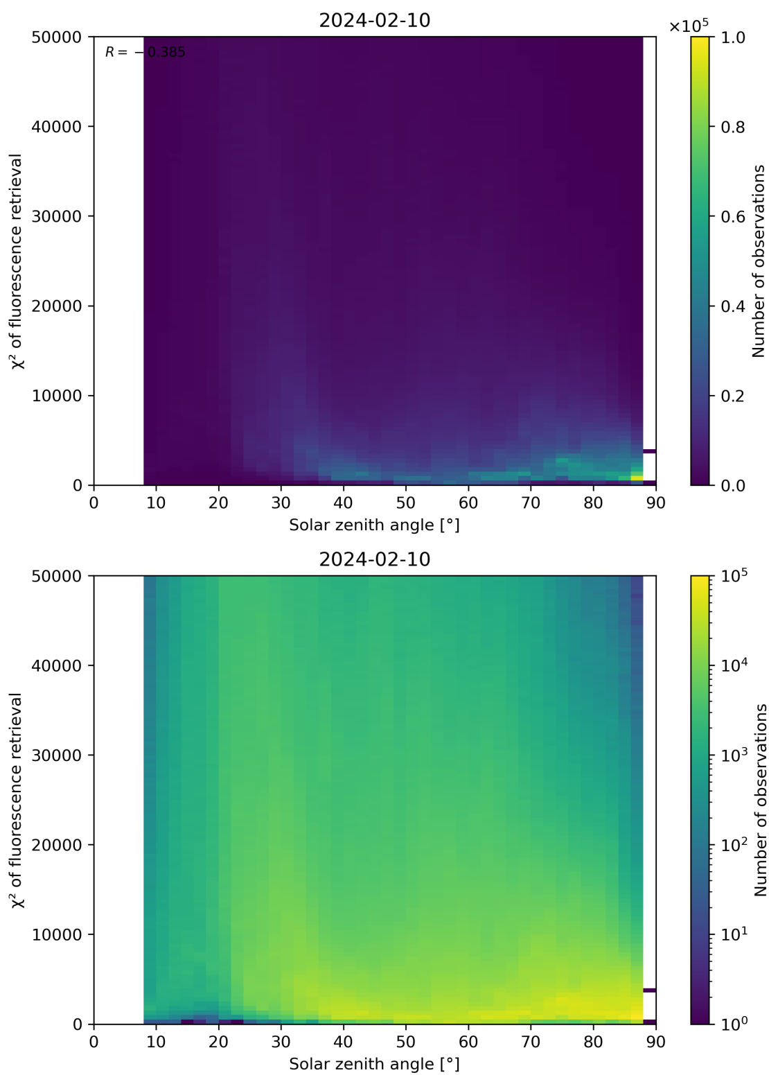
Figure 109: Scatter density plot of “Solar zenith angle” against “ \chi^2 of fluorescence retrieval” for 2024-02-09 to 2024-02-11.
