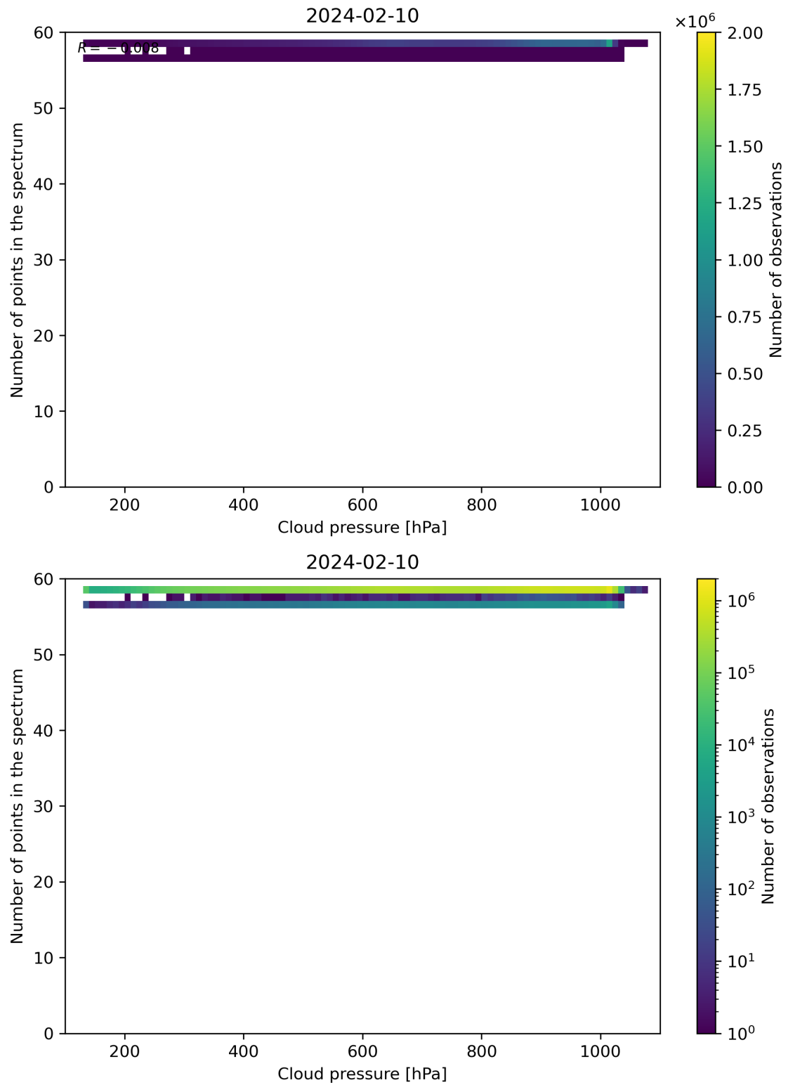
Figure 82: Scatter density plot of “Cloud pressure” against “Number of points in the spectrum” for 2024-02-09 to 2024-02-11.
