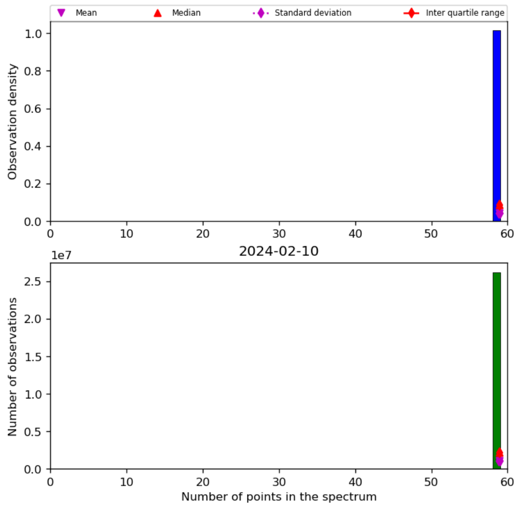
Figure 44: Histogram of “Number of points in the spectrum” for 2024-02-09 to 2024-02-11
