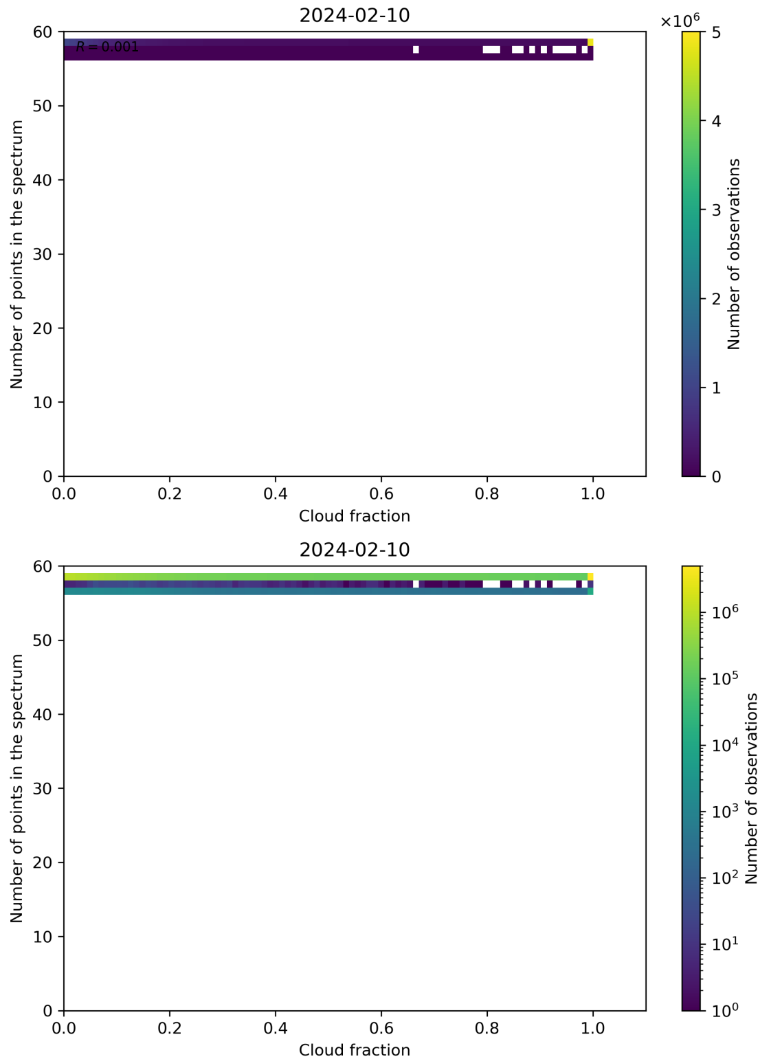
Figure 74: Scatter density plot of “Cloud fraction” against “Number of points in the spectrum” for 2024-02-09 to 2024-02-11.
