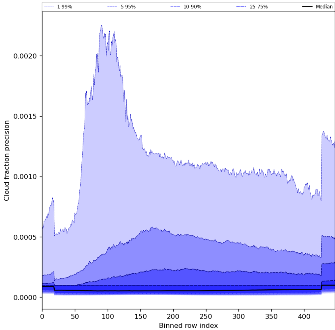
Figure 50: Along track statistics of “Cloud fraction precision” for 2024-02-09 to 2024-02-11
