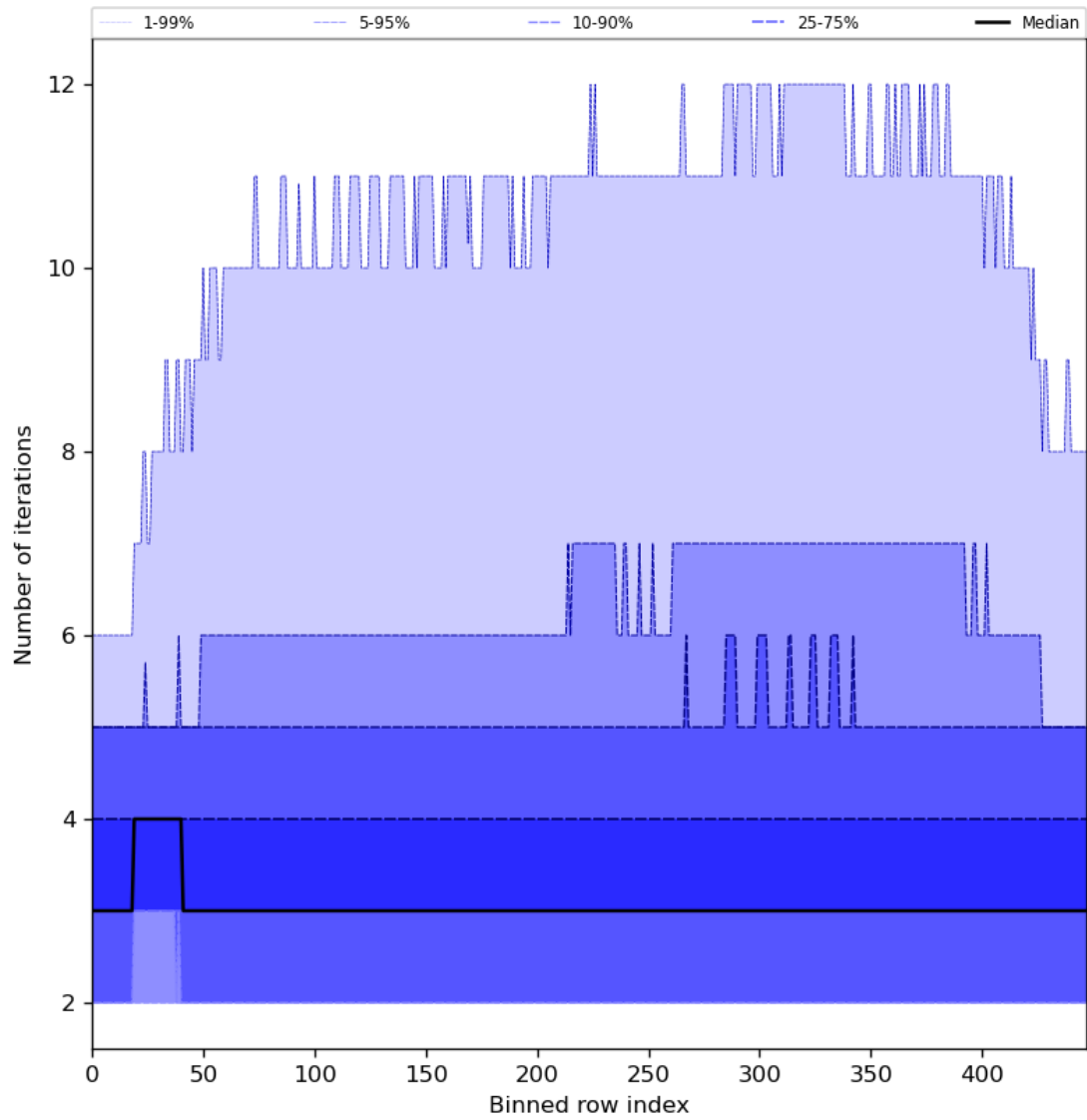
Figure 56: Along track statistics of “Number of iterations” for 2024-02-09 to 2024-02-11
