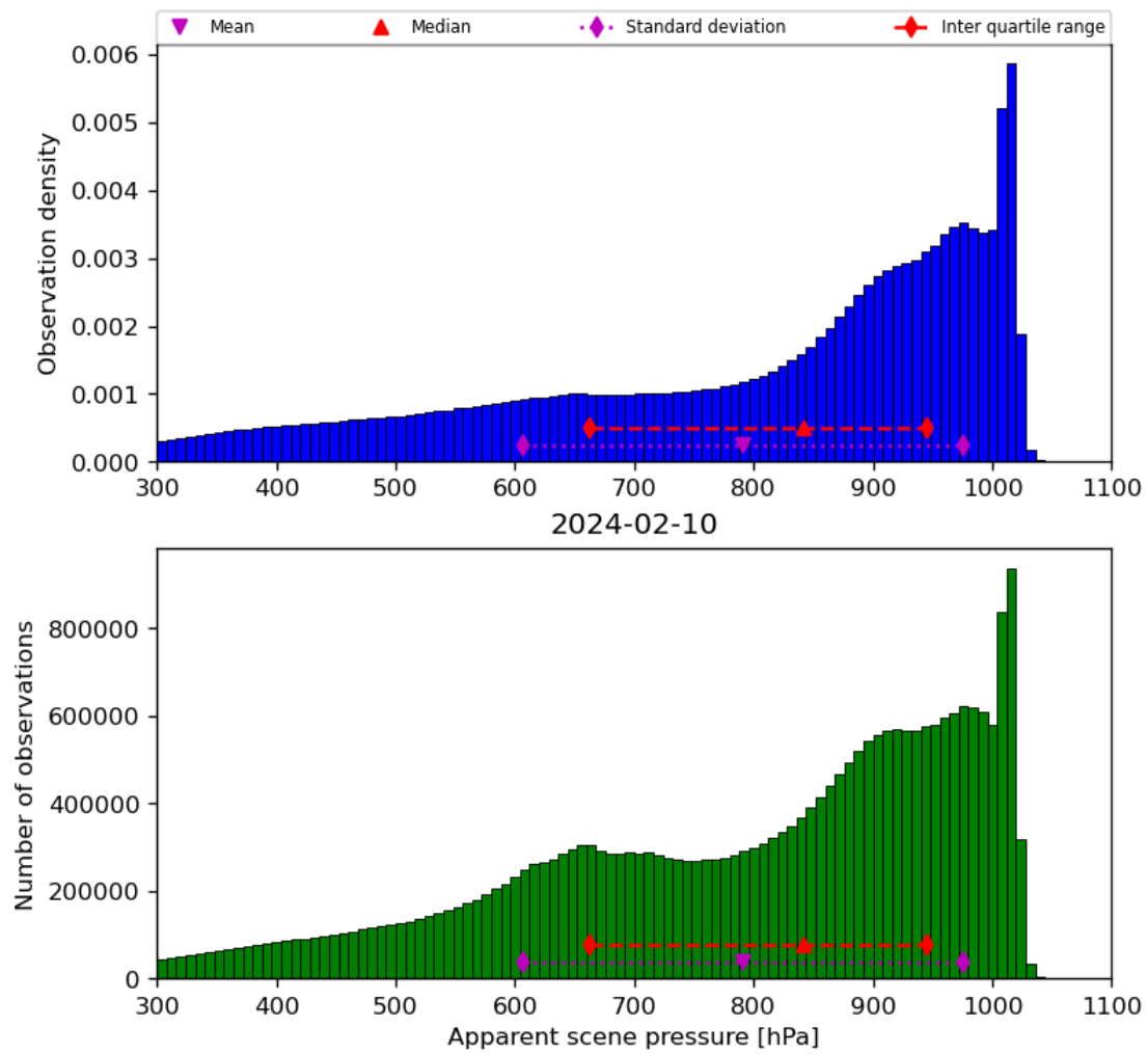
Figure 36: Histogram of “Apparent scene pressure” for 2024-02-09 to 2024-02-11
