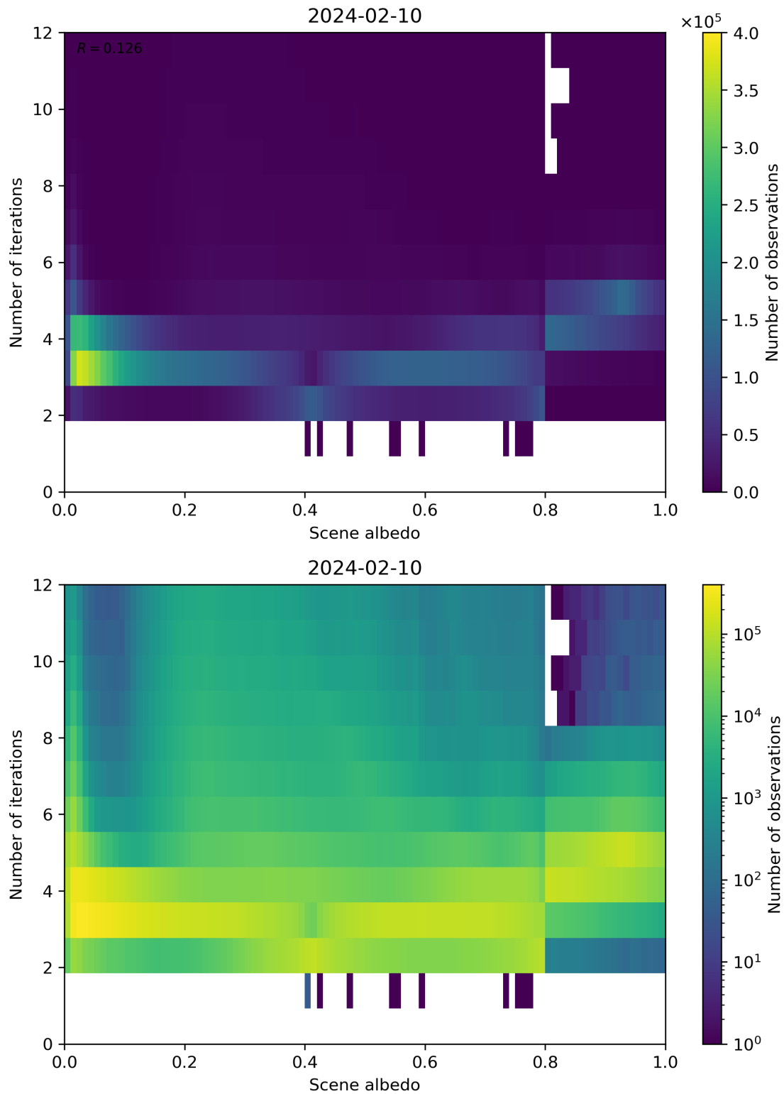
Figure 105: Scatter density plot of “Scene albedo” against “Number of iterations” for 2024-02-09 to 2024-02-11.
