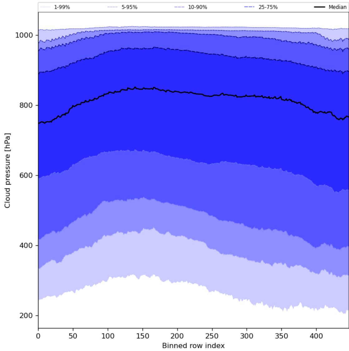
Figure 47: Along track statistics of “Cloud pressure” for 2024-02-09 to 2024-02-11
