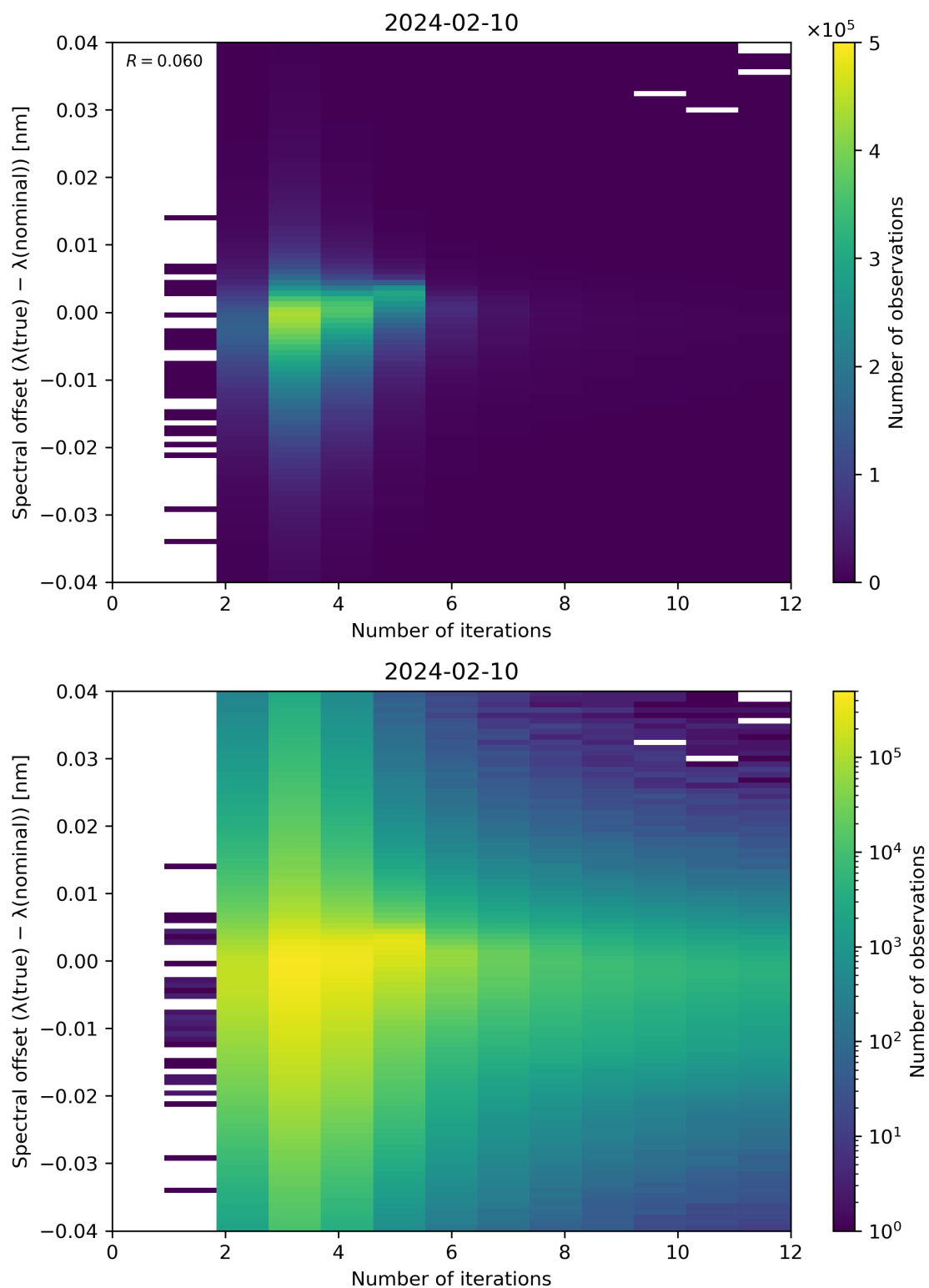
Figure 100: Scatter density plot of “Number of iterations” against “Spectral offset ( \lambda(\text{true}) - \lambda(\text{nominal}) )” for 2024-02-09 to 2024-02-11.
