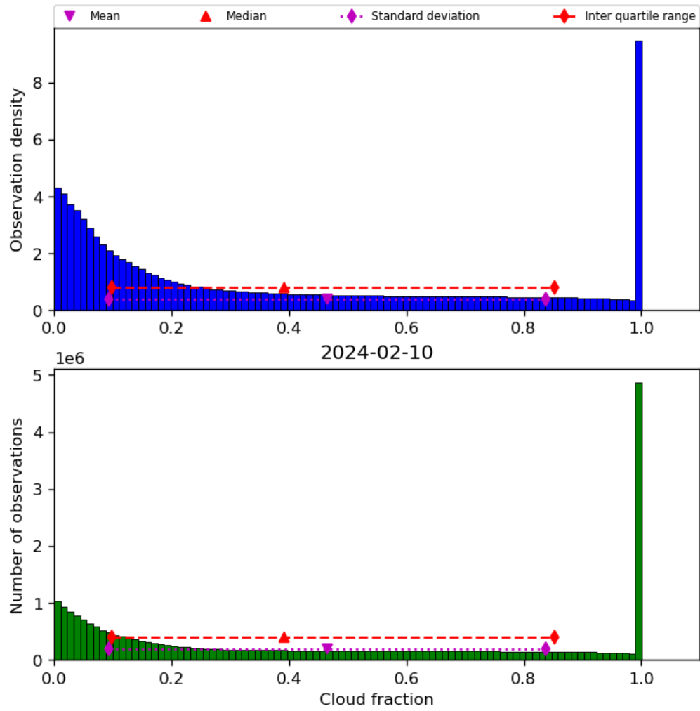
Figure 32: Histogram of “Cloud fraction” for 2024-02-09 to 2024-02-11
