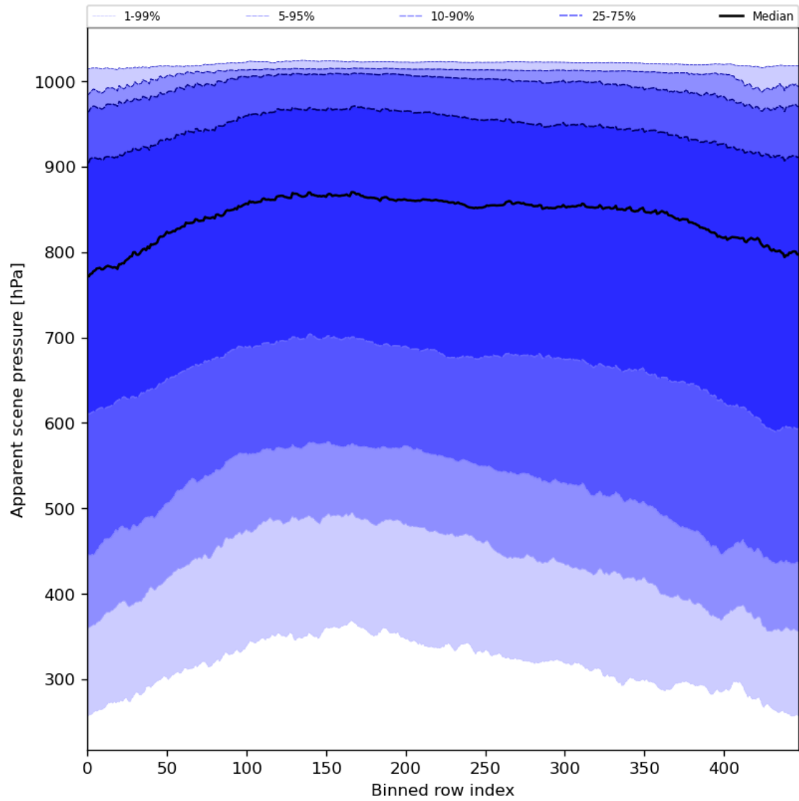
Figure 53: Along track statistics of “Apparent scene pressure” for 2024-02-09 to 2024-02-11
