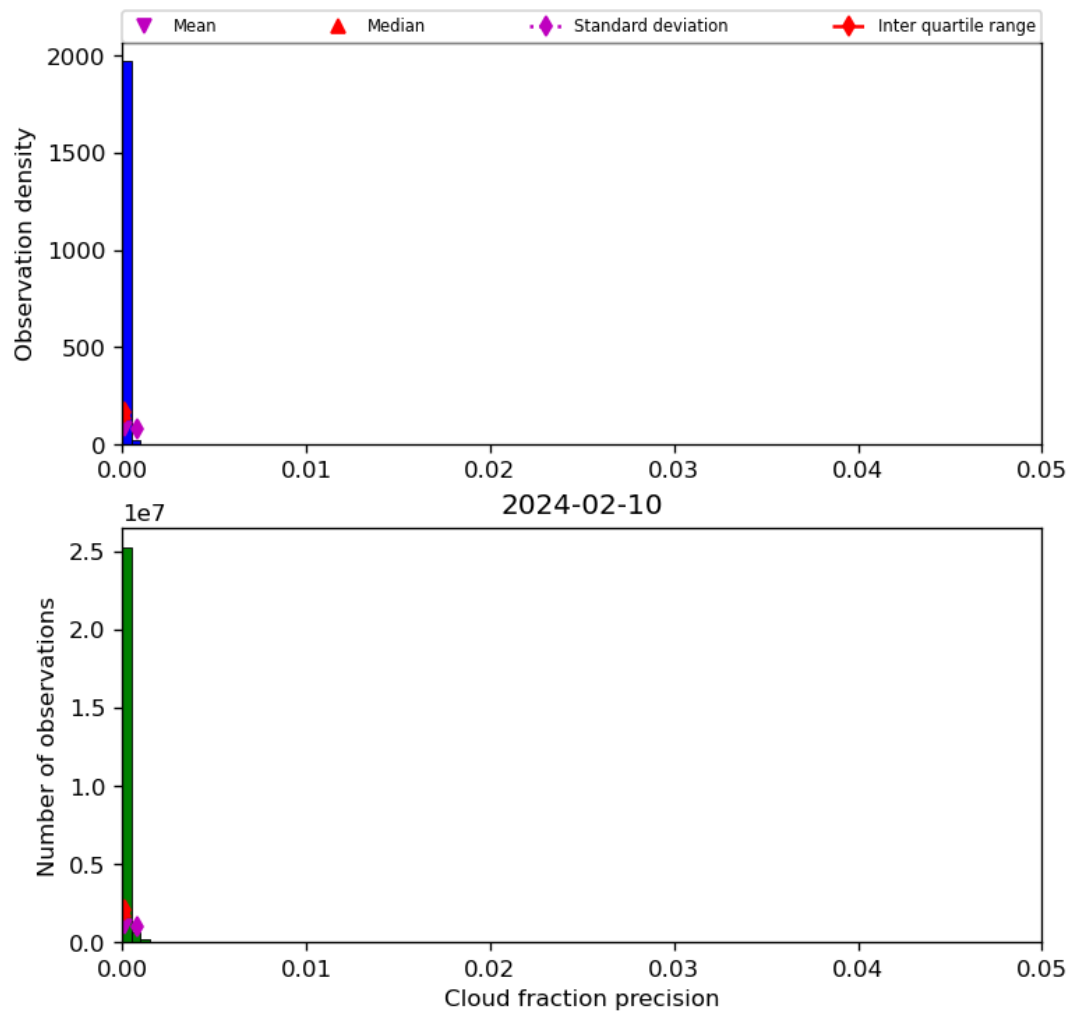
Figure 33: Histogram of “Cloud fraction precision” for 2024-02-09 to 2024-02-11
