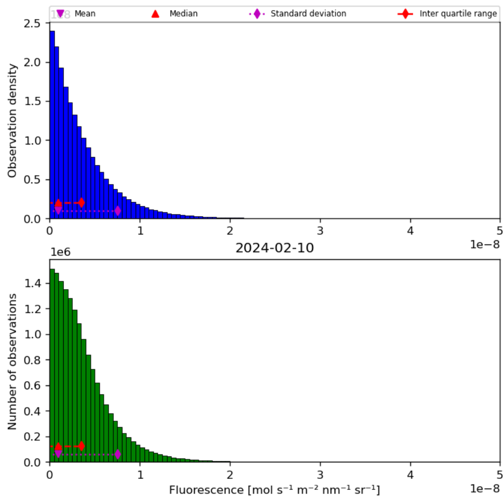
Figure 40: Histogram of “Fluorescence” for 2024-02-09 to 2024-02-11
