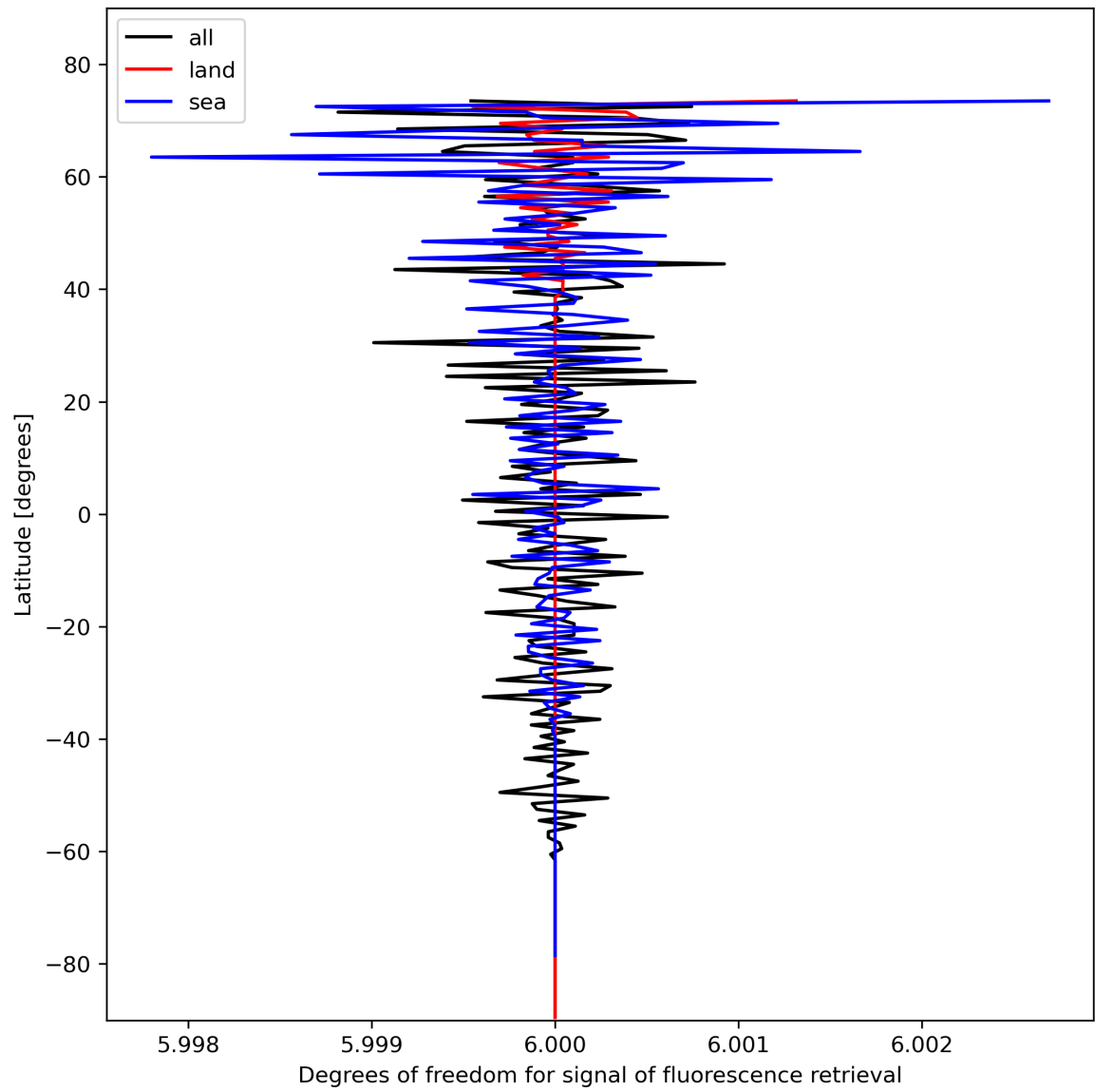
Figure 26: Zonal average of “Degrees of freedom for signal of fluorescence retrieval” for 2024-02-09 to 2024-02-11.
