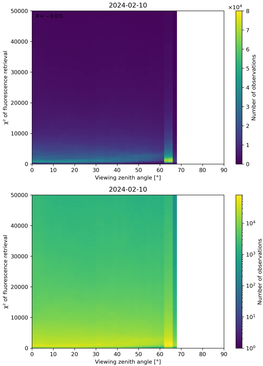
Figure 119: Scatter density plot of “Viewing zenith angle” against “ \chi^2 of fluorescence retrieval” for 2024-02-09 to 2024-02-11.
