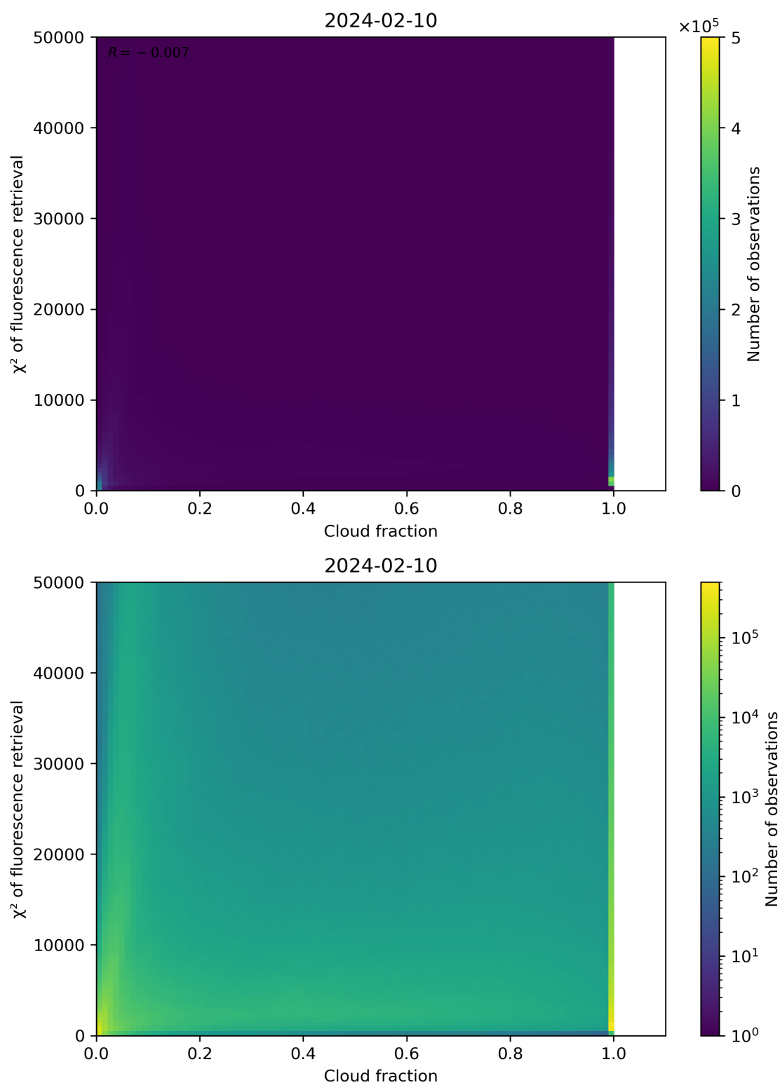
Figure 71: Scatter density plot of “Cloud fraction” against “ \chi^2 of fluorescence retrieval” for 2024-02-09 to 2024-02-11.
