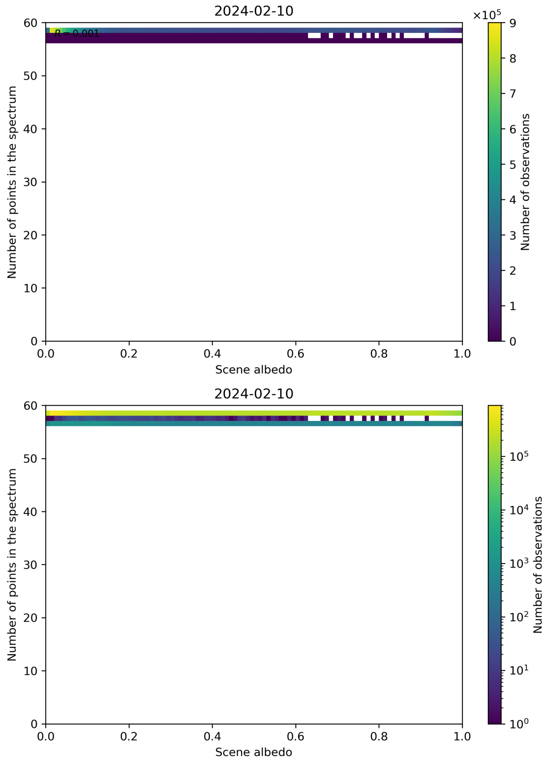
Figure 106: Scatter density plot of “Scene albedo” against “Number of points in the spectrum” for 2024-02-09 to 2024-02-11.
