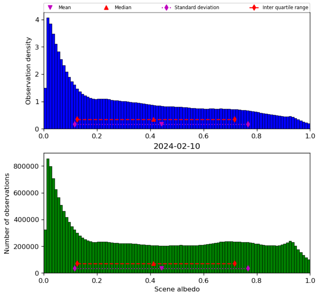
Figure 34: Histogram of “Scene albedo” for 2024-02-09 to 2024-02-11
