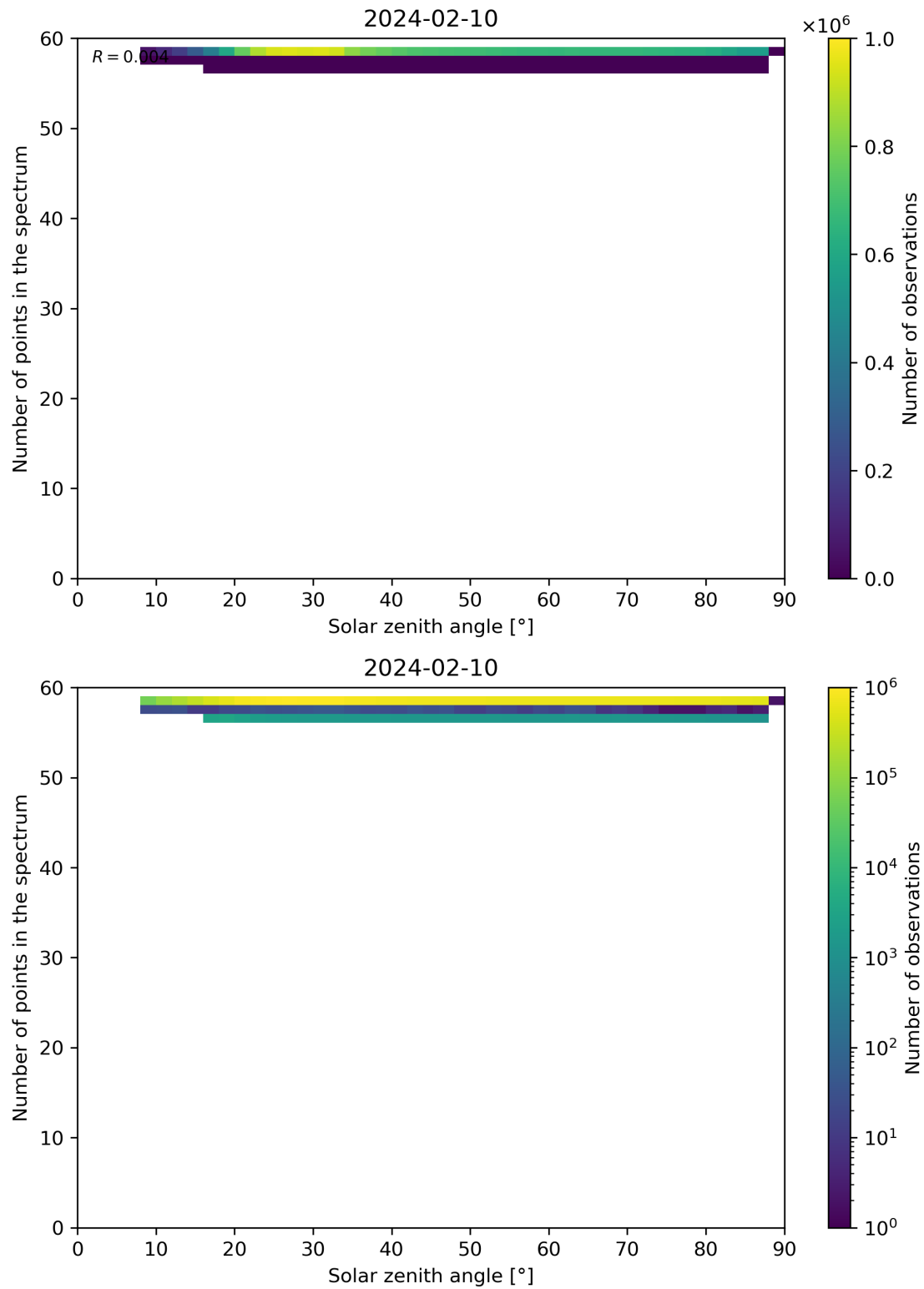
Figure 115: Scatter density plot of “Solar zenith angle” against “Number of points in the spectrum” for 2024-02-09 to 2024-02-11.
