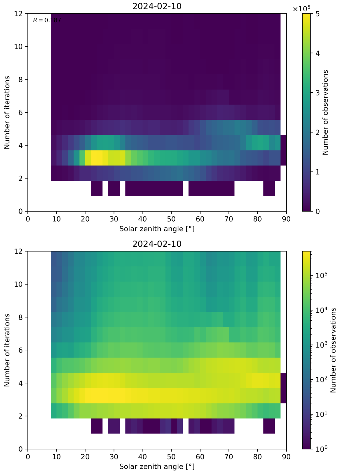
Figure 114: Scatter density plot of “Solar zenith angle” against “Number of iterations” for 2024-02-09 to 2024-02-11.
