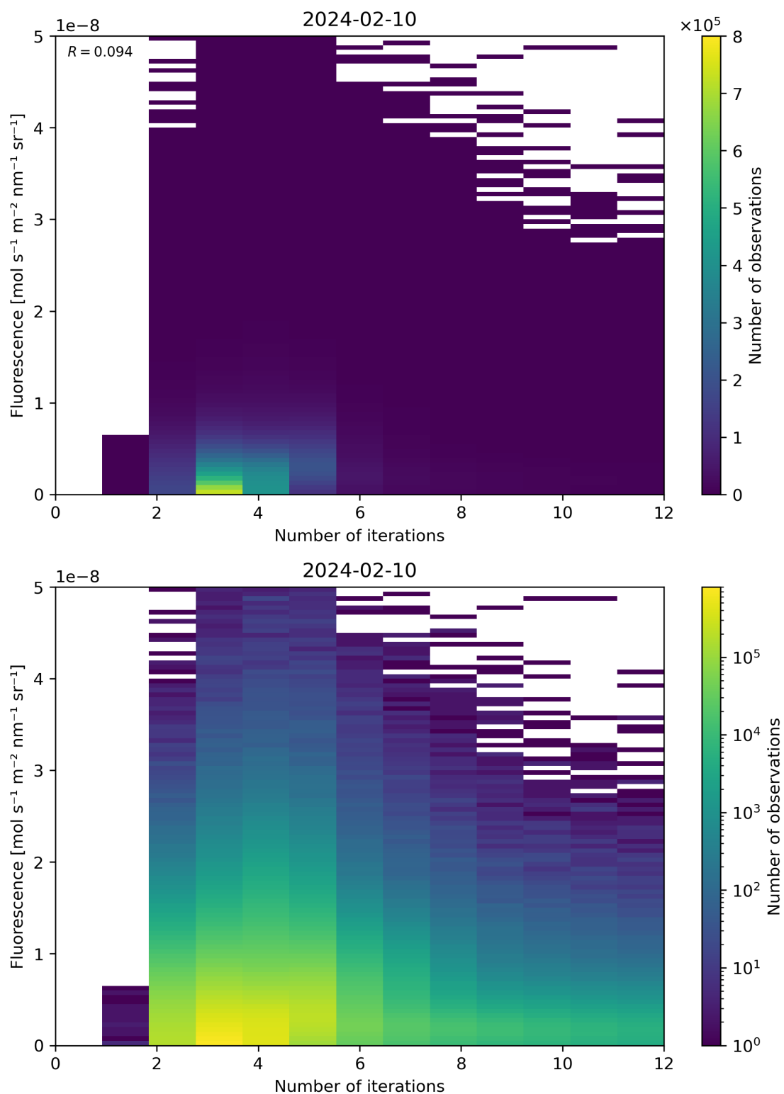
Figure 98: Scatter density plot of “Number of iterations” against “Fluorescence” for 2024-02-09 to 2024-02-11.
