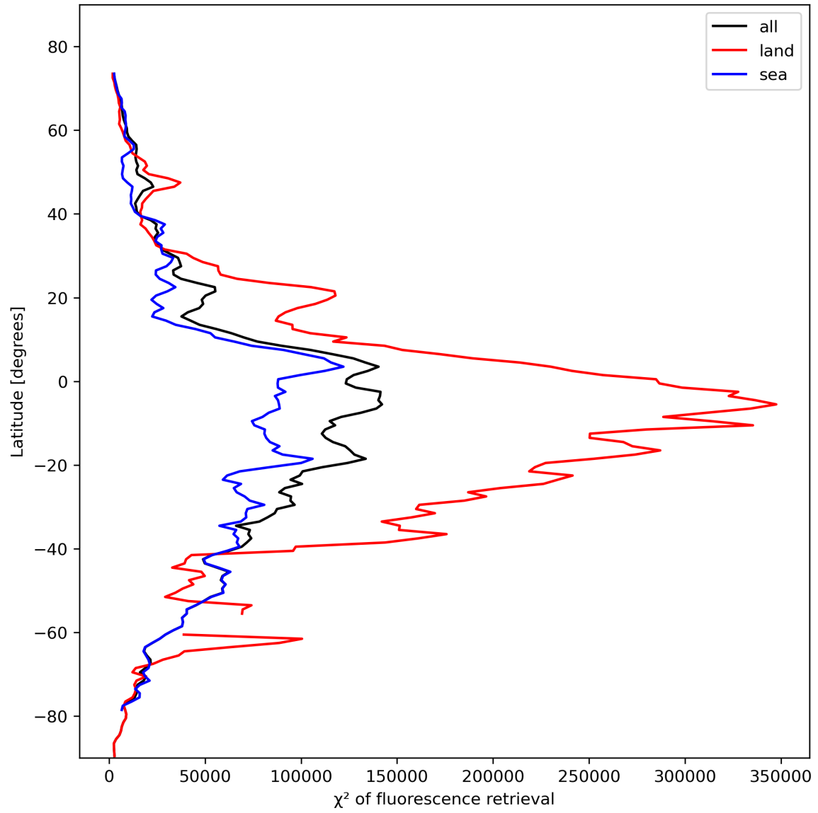
Figure 25: Zonal average of “ \chi^2 of fluorescence retrieval” for 2024-02-09 to 2024-02-11.
