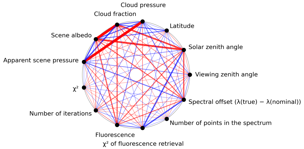
Figure 1: Map of correlation graph for 2024-02-09 to 2024-02-11.
