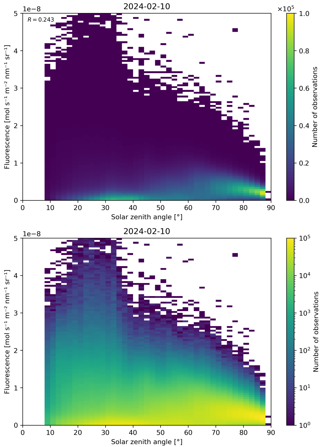
Figure 112: Scatter density plot of “Solar zenith angle” against “Fluorescence” for 2024-02-09 to 2024-02-11.
