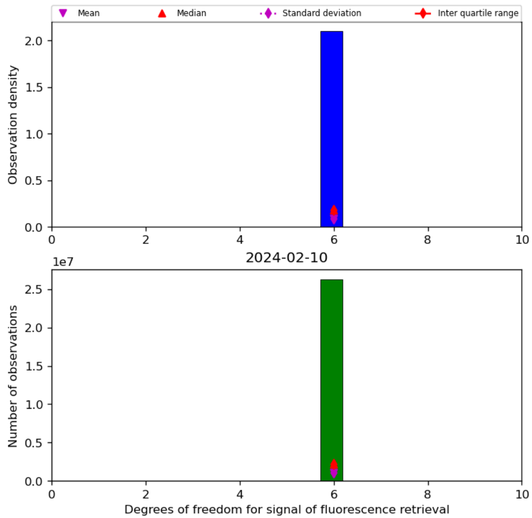
Figure 43: Histogram of “Degrees of freedom for signal of fluorescence retrieval” for 2024-02-09 to 2024-02-11
