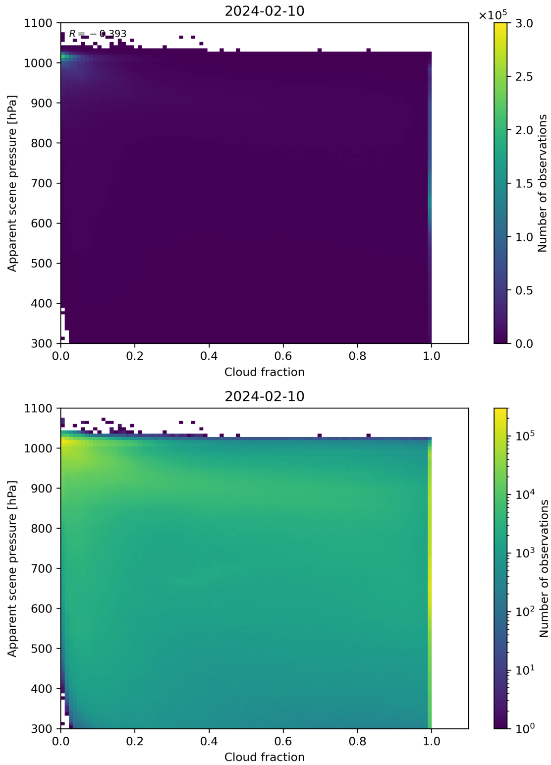
Figure 70: Scatter density plot of “Cloud fraction” against “Apparent scene pressure” for 2024-02-09 to 2024-02-11.
