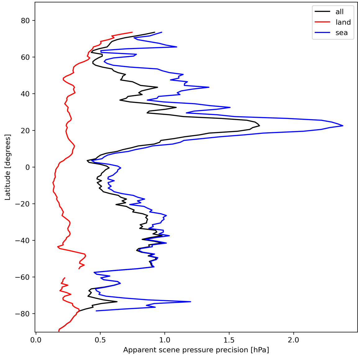
Figure 20: Zonal average of “Apparent scene pressure precision” for 2024-02-09 to 2024-02-11.
