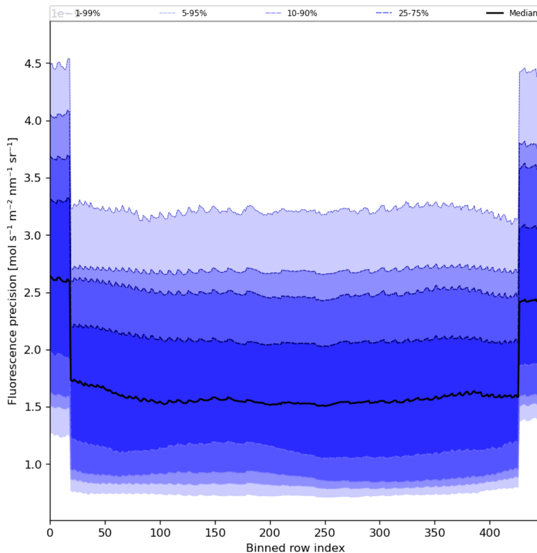
Figure 58: Along track statistics of “Fluorescence precision” for 2024-02-09 to 2024-02-11
