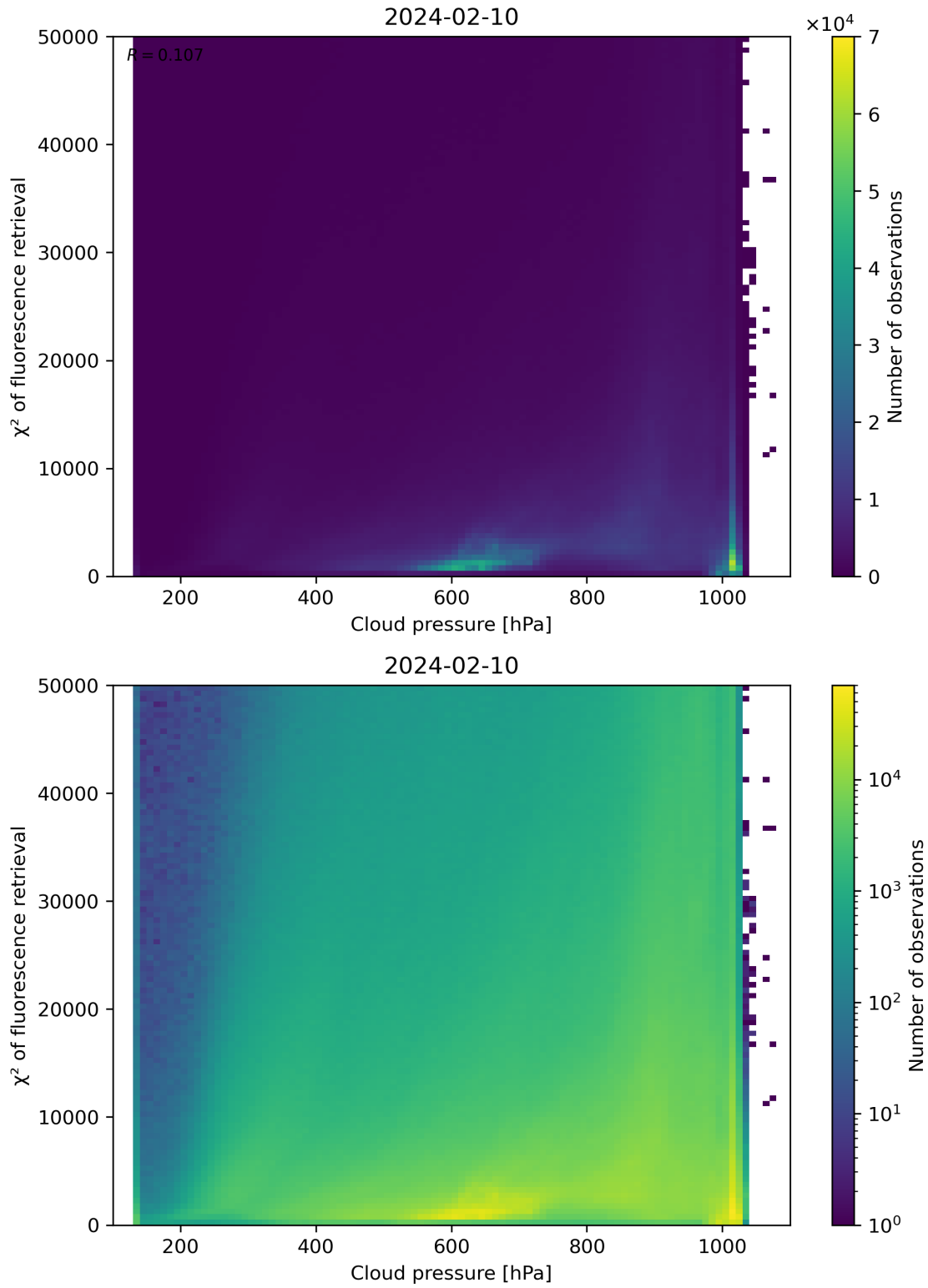
Figure 78: Scatter density plot of “Cloud pressure” against “ \chi^2 of fluorescence retrieval” for 2024-02-09 to 2024-02-11.
