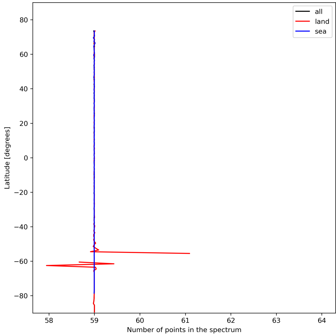
Figure 27: Zonal average of “Number of points in the spectrum” for 2024-02-09 to 2024-02-11.
