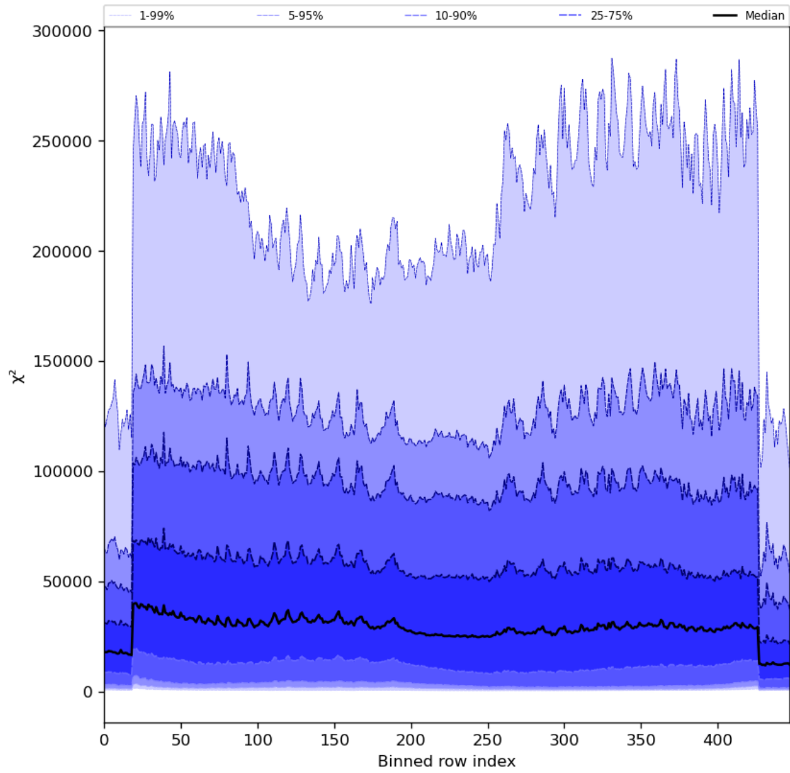
Figure 55: Along track statistics of “ \chi^2 ” for 2024-02-09 to 2024-02-11
