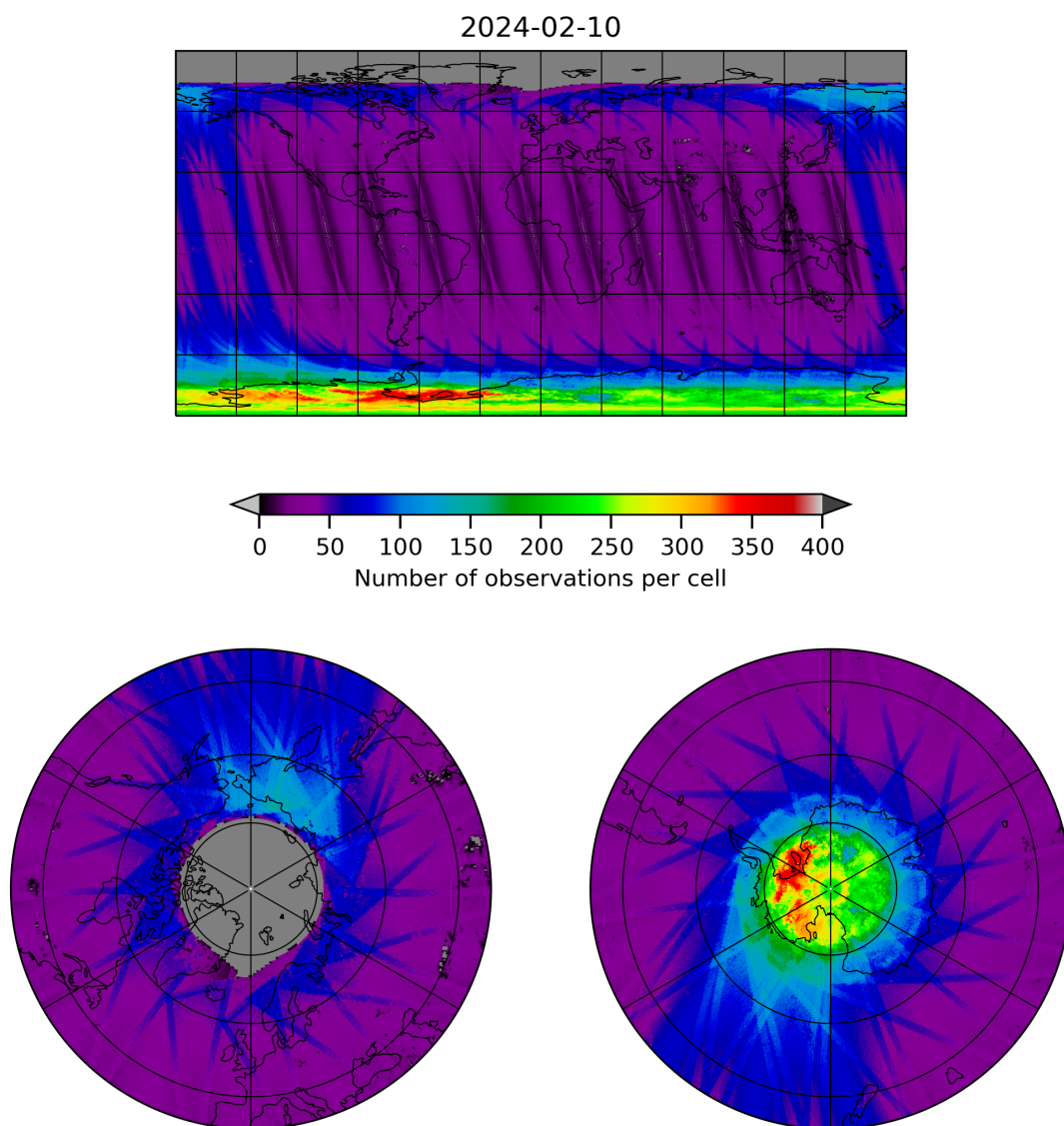
Figure 11: Map of the number of observations for 2024-02-09 to 2024-02-11
