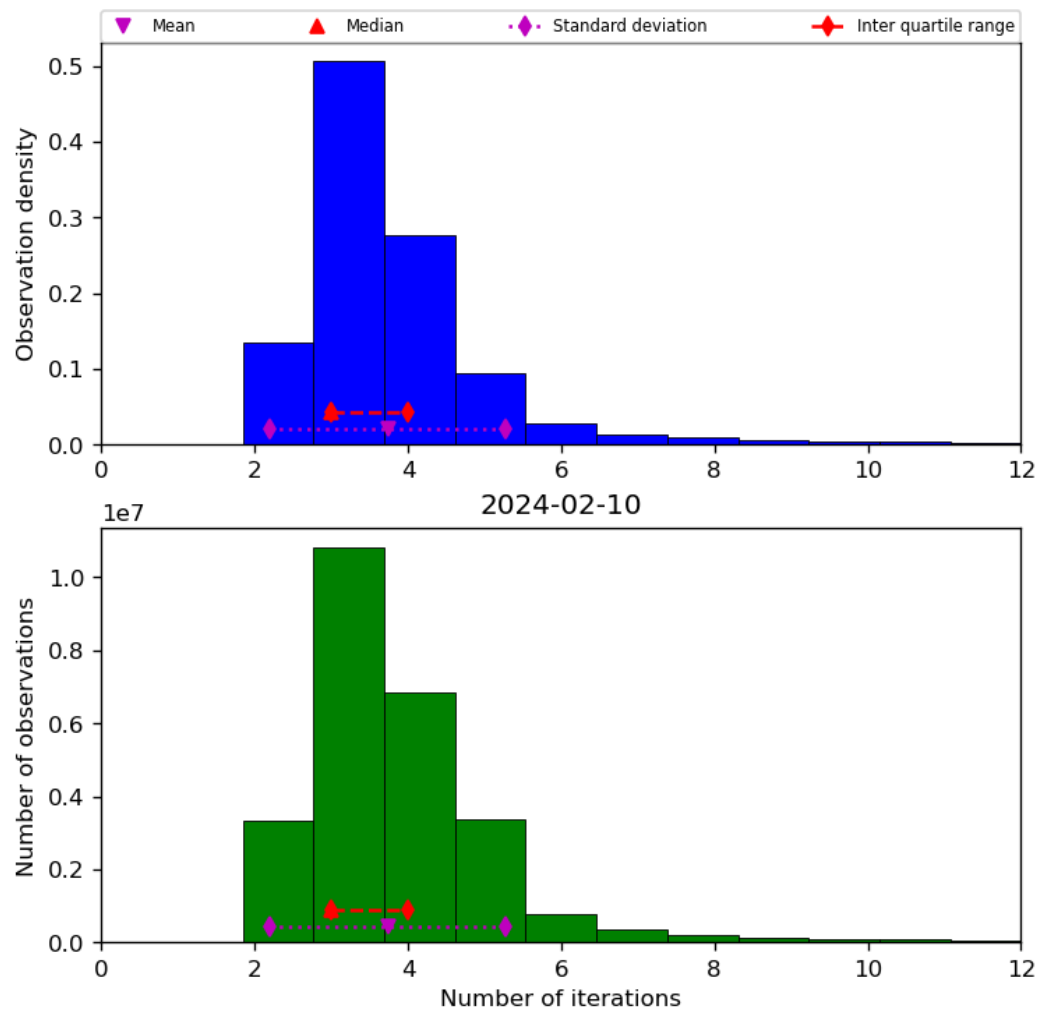
Figure 39: Histogram of “Number of iterations” for 2024-02-09 to 2024-02-11
