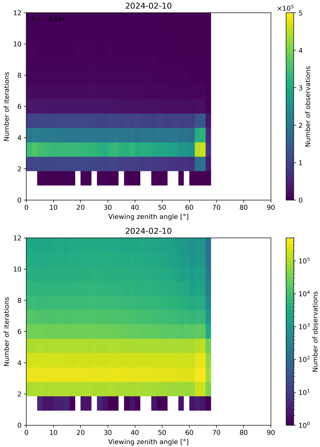
Figure 124: Scatter density plot of “Viewing zenith angle” against “Number of iterations” for 2024-02-09 to 2024-02-11.
