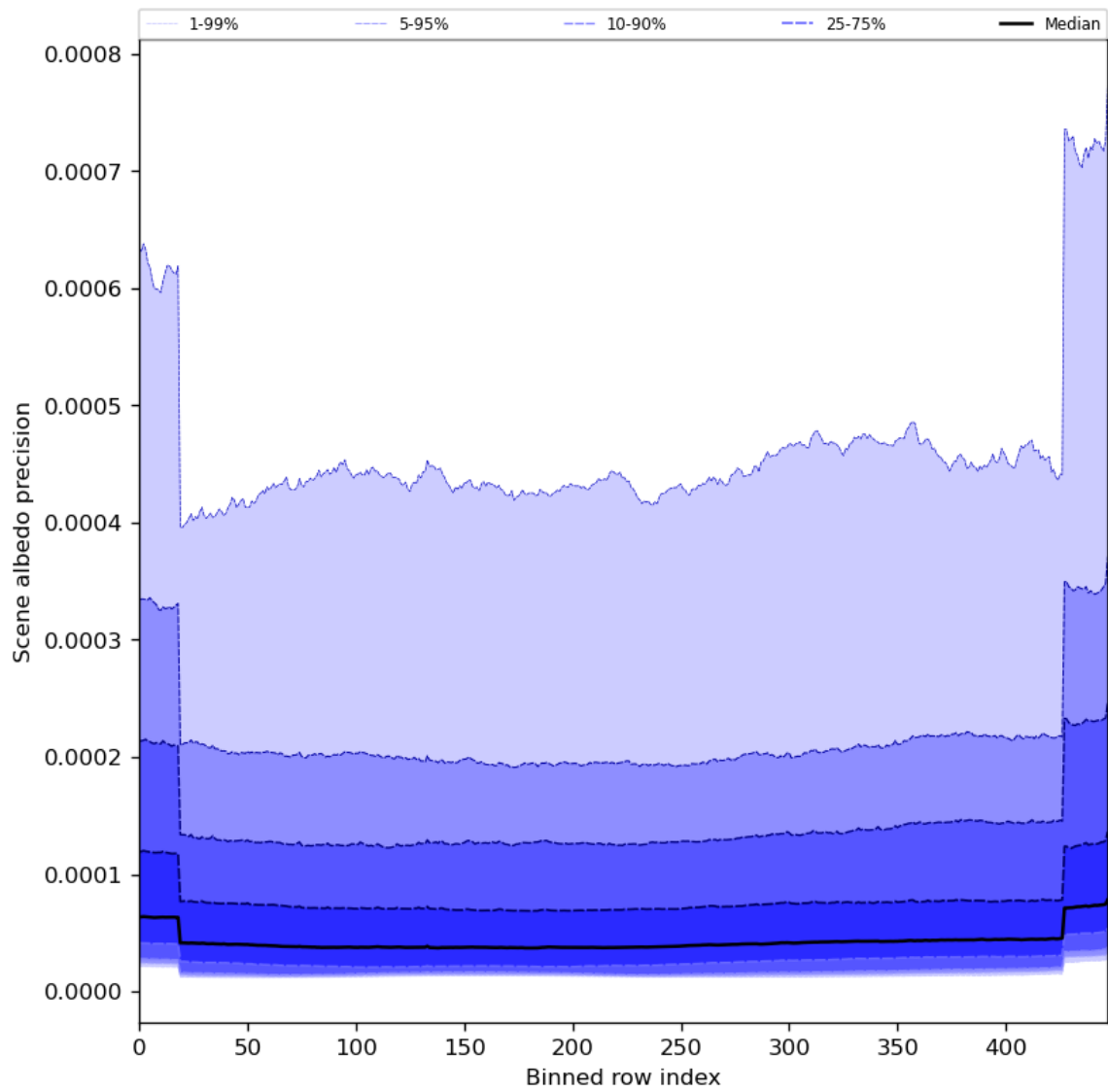
Figure 52: Along track statistics of “Scene albedo precision” for 2024-02-09 to 2024-02-11
