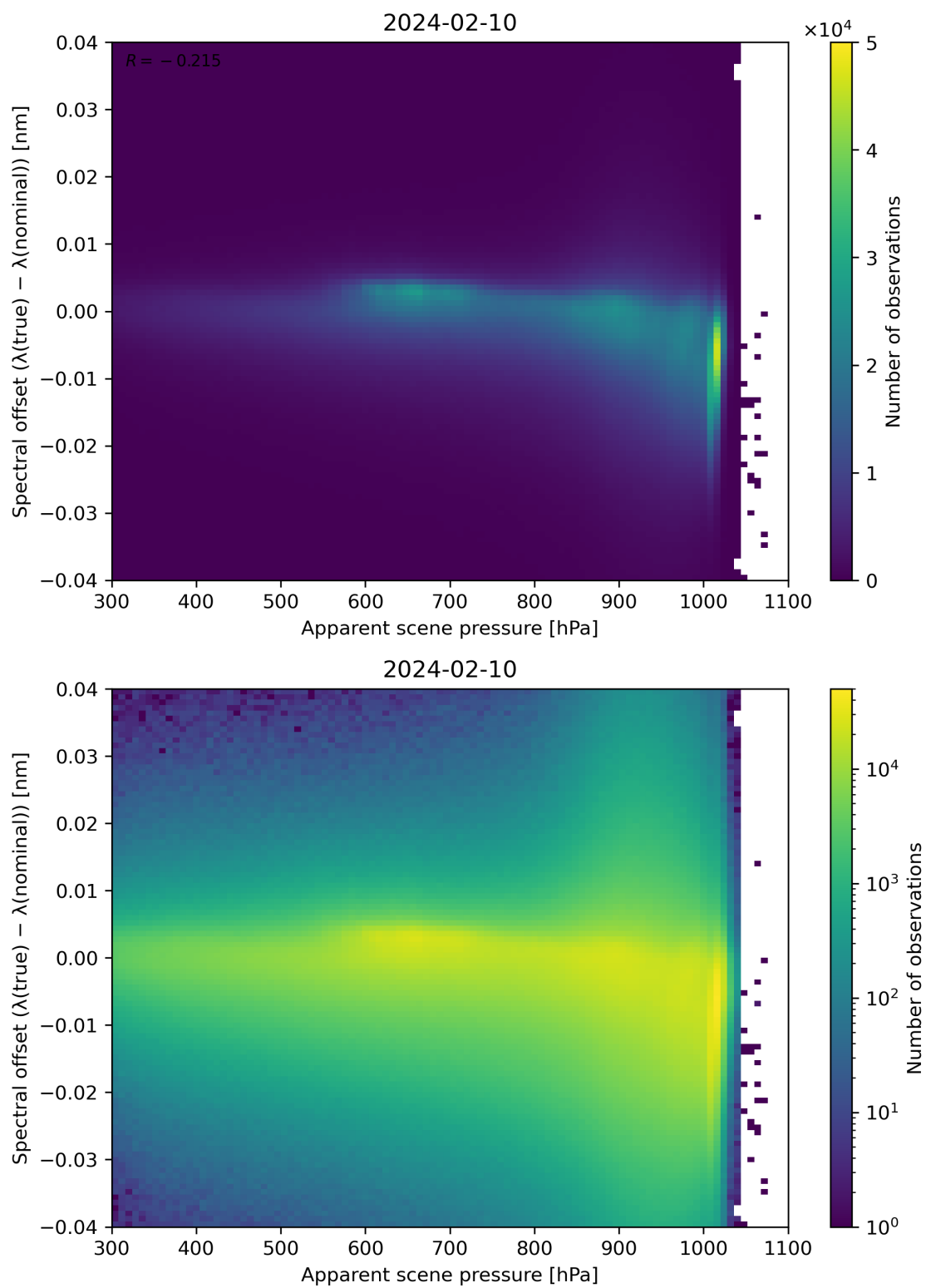
Figure 67: Scatter density plot of “Apparent scene pressure” against “Spectral offset ( \lambda(\text{true}) - \lambda(\text{nominal}) )” for 2024-02-09 to 2024-02-11.
