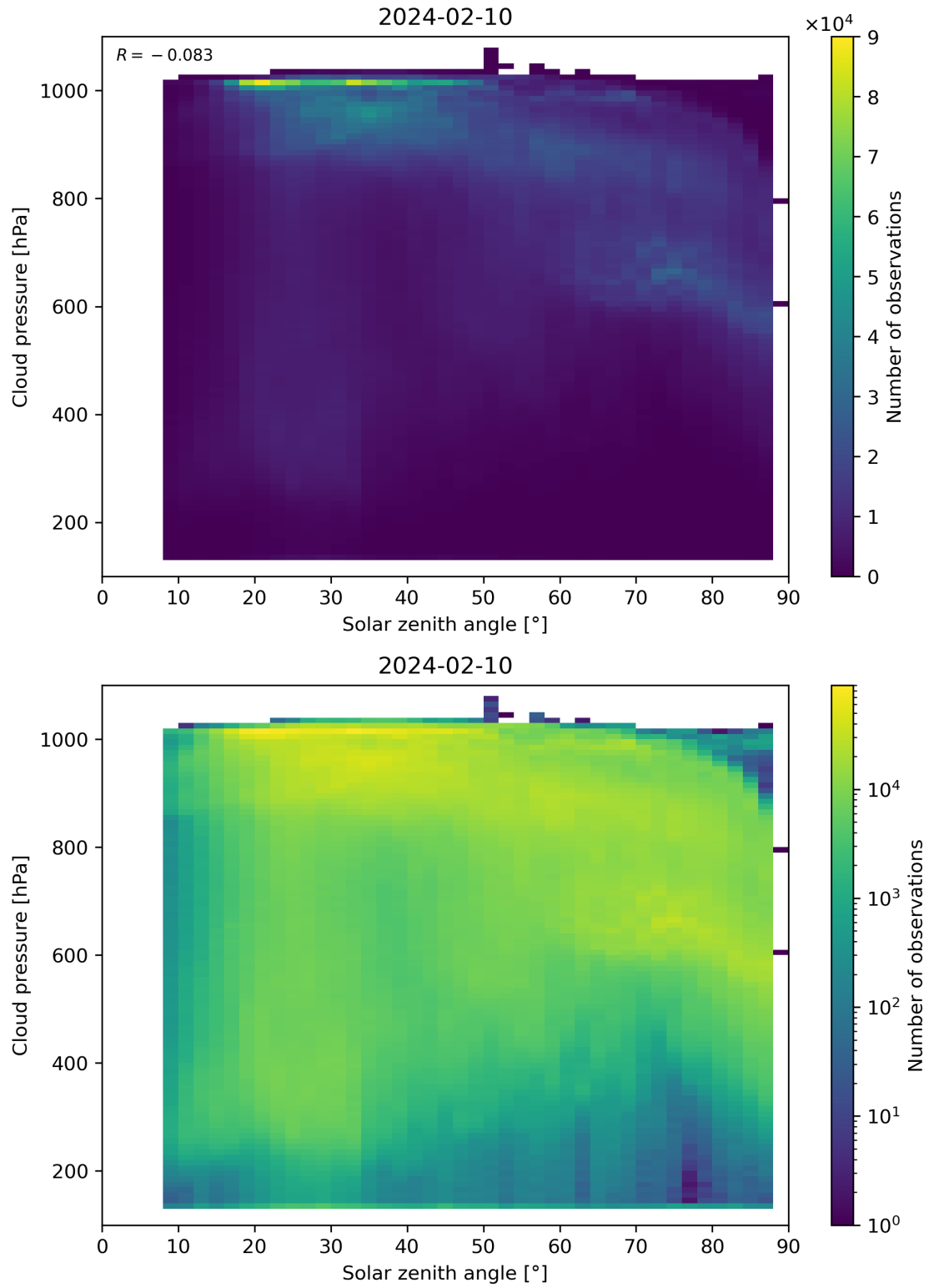
Figure 111: Scatter density plot of “Solar zenith angle” against “Cloud pressure” for 2024-02-09 to 2024-02-11.
