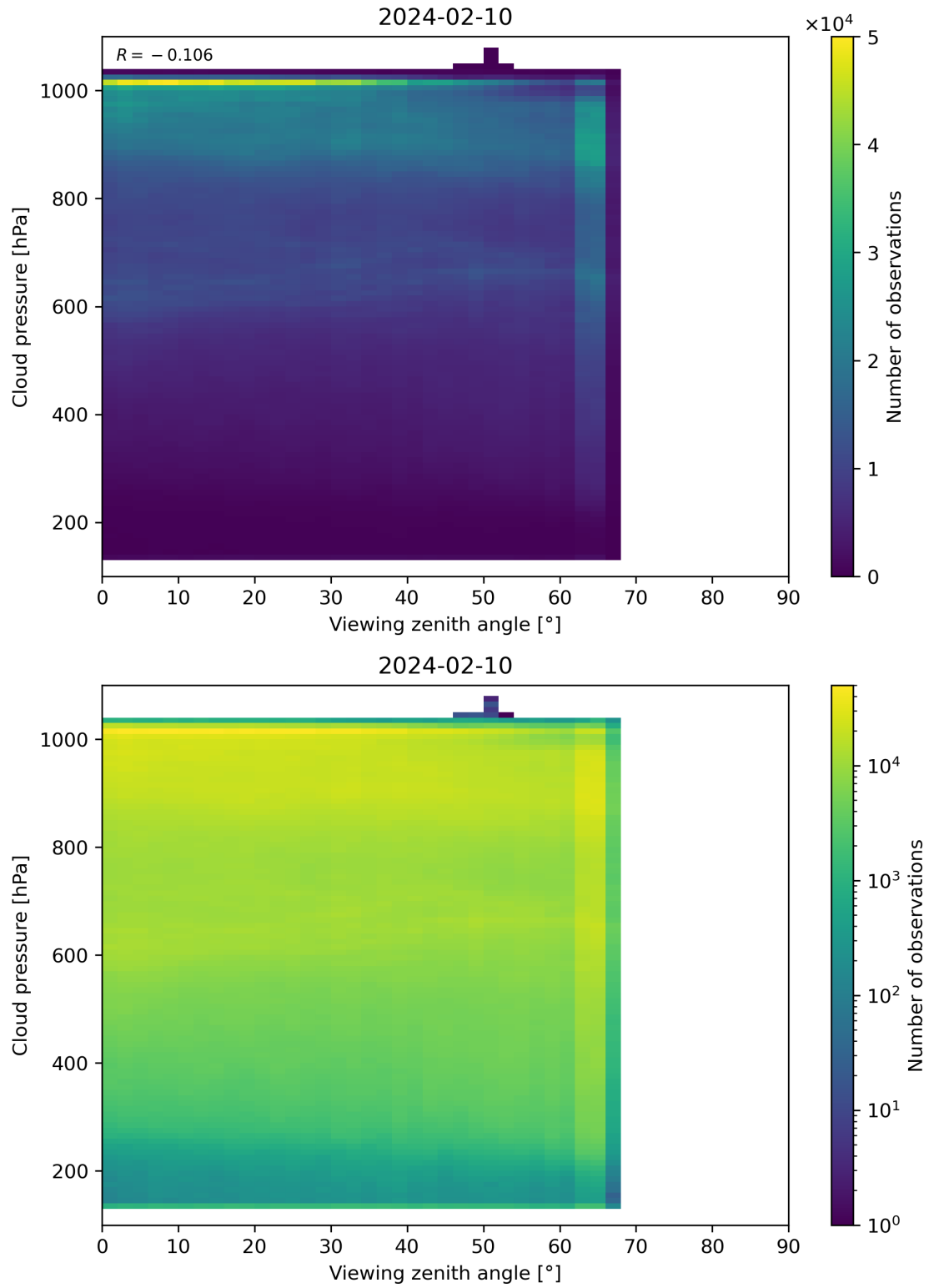
Figure 121: Scatter density plot of “Viewing zenith angle” against “Cloud pressure” for 2024-02-09 to 2024-02-11.
