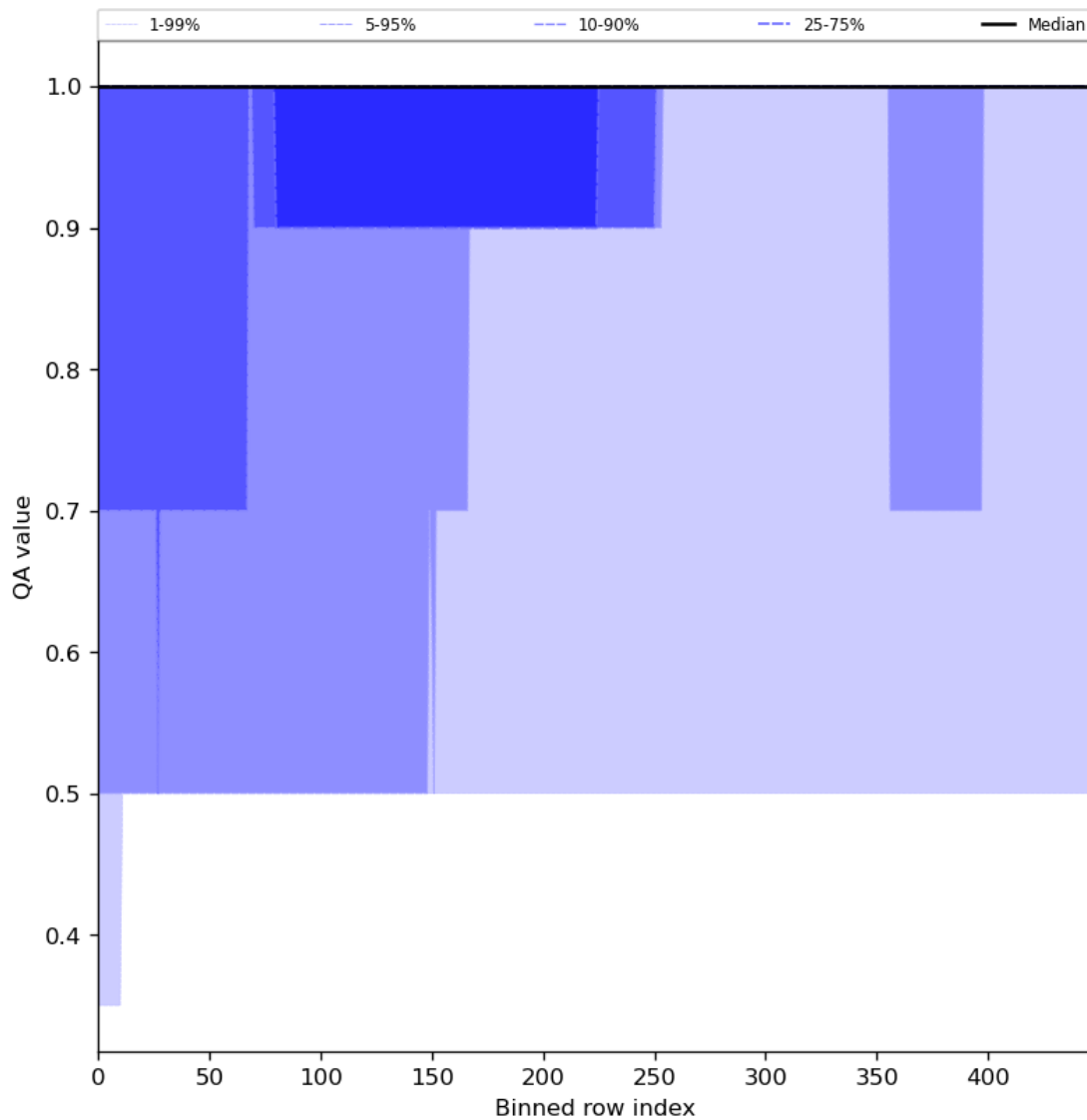
Figure 46: Along track statistics of “QA value” for 2024-02-09 to 2024-02-11
