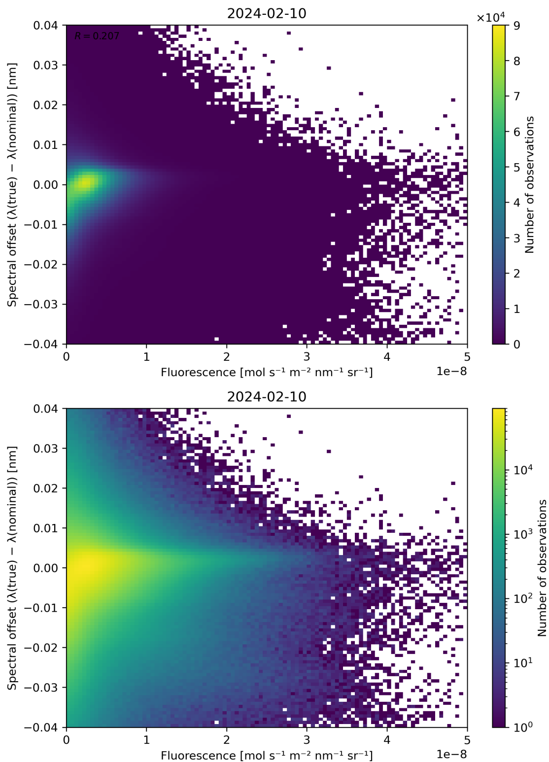
Figure 87: Scatter density plot of “Fluorescence” against “Spectral offset ( \lambda(\text{true}) - \lambda(\text{nominal}) )” for 2024-02-09 to 2024-02-11.
