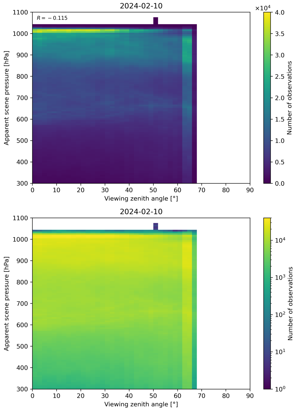
Figure 118: Scatter density plot of “Viewing zenith angle” against “Apparent scene pressure” for 2024-02-09 to 2024-02-11.
