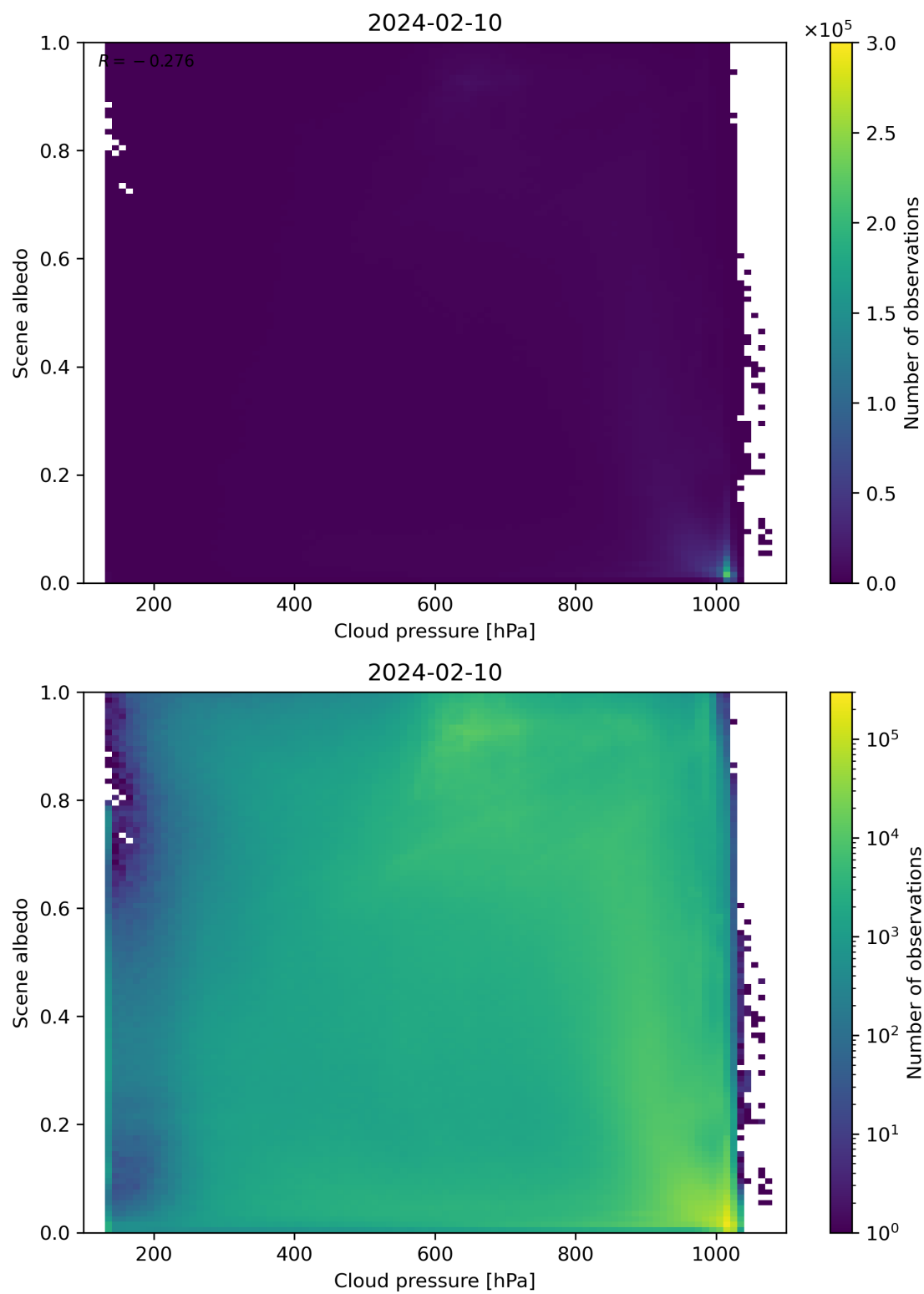
Figure 83: Scatter density plot of “Cloud pressure” against “Scene albedo” for 2024-02-09 to 2024-02-11.
