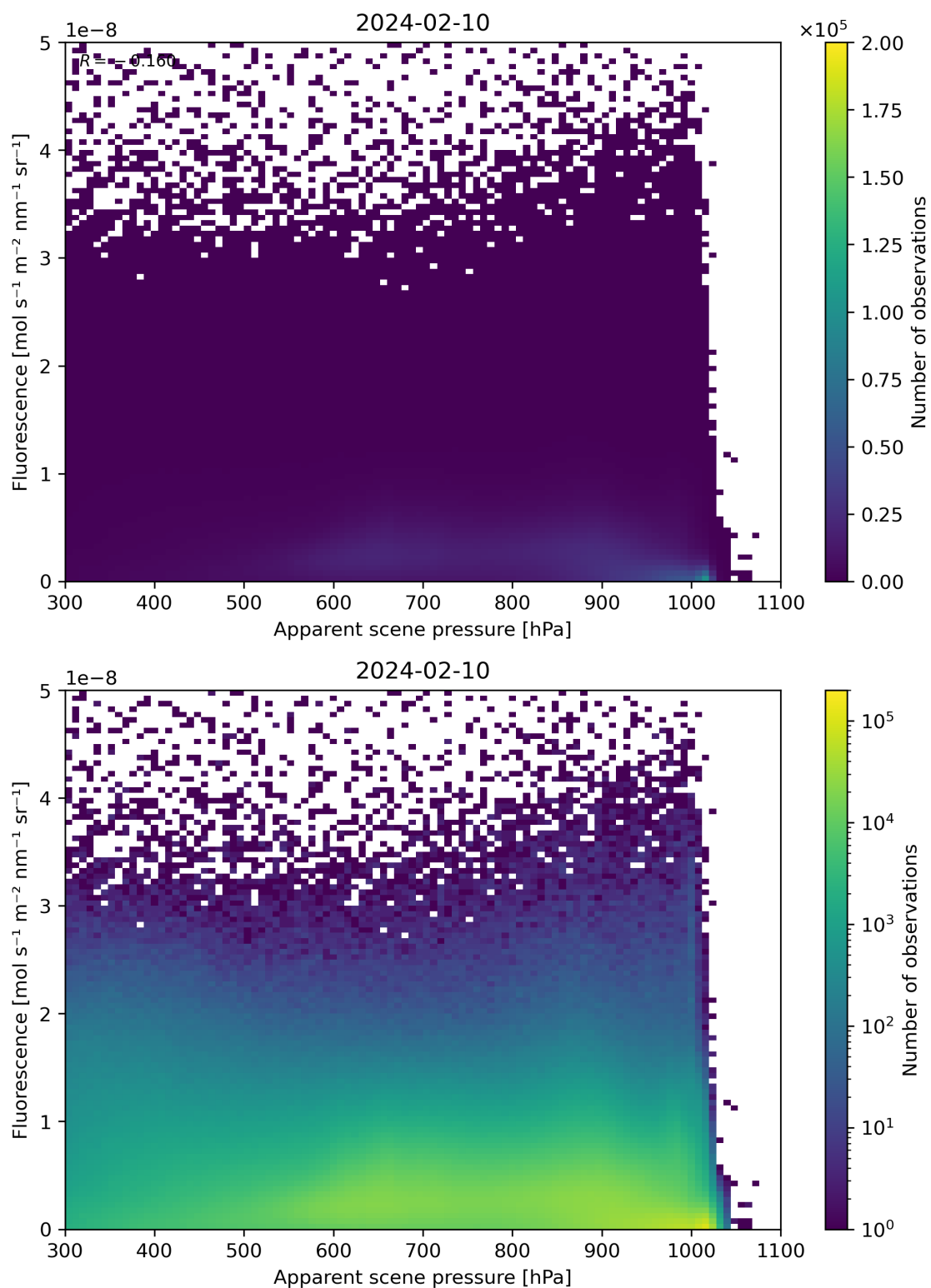
Figure 64: Scatter density plot of “Apparent scene pressure” against “Fluorescence” for 2024-02-09 to 2024-02-11.
