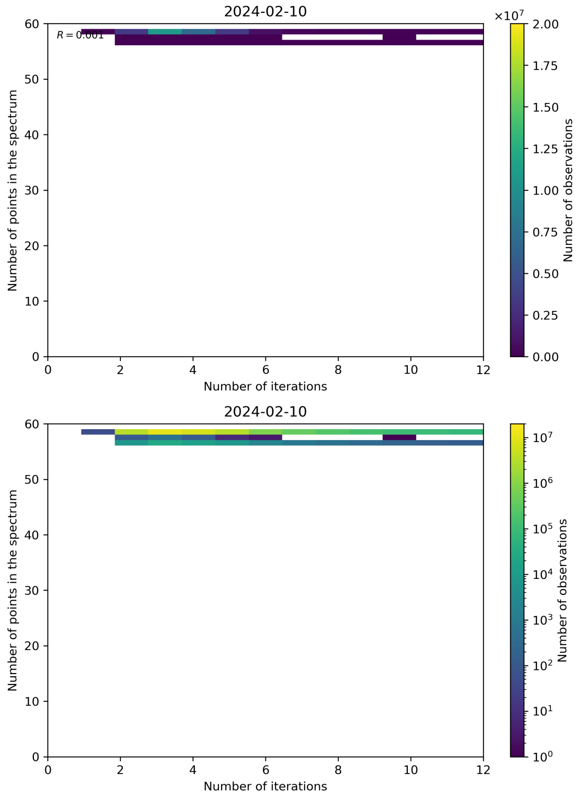
Figure 99: Scatter density plot of “Number of iterations” against “Number of points in the spectrum” for 2024-02-09 to 2024-02-11.
