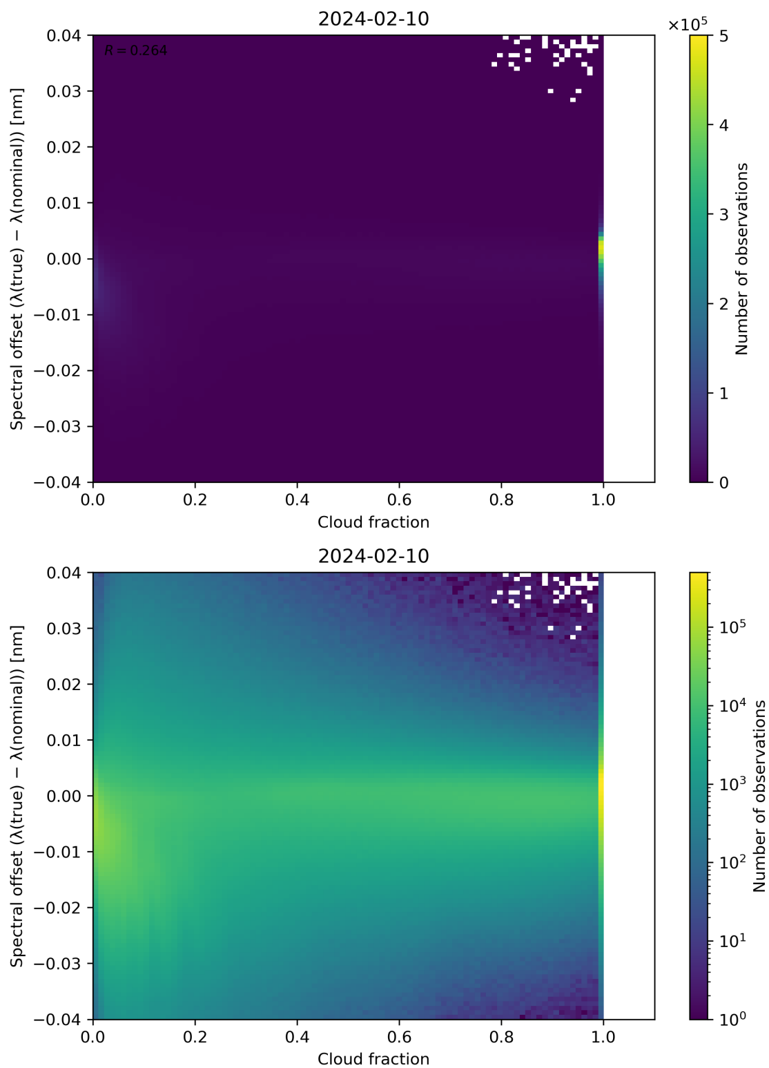
Figure 76: Scatter density plot of “Cloud fraction” against “Spectral offset ( \lambda(\text{true}) - \lambda(\text{nominal}) )” for 2024-02-09 to 2024-02-11.
