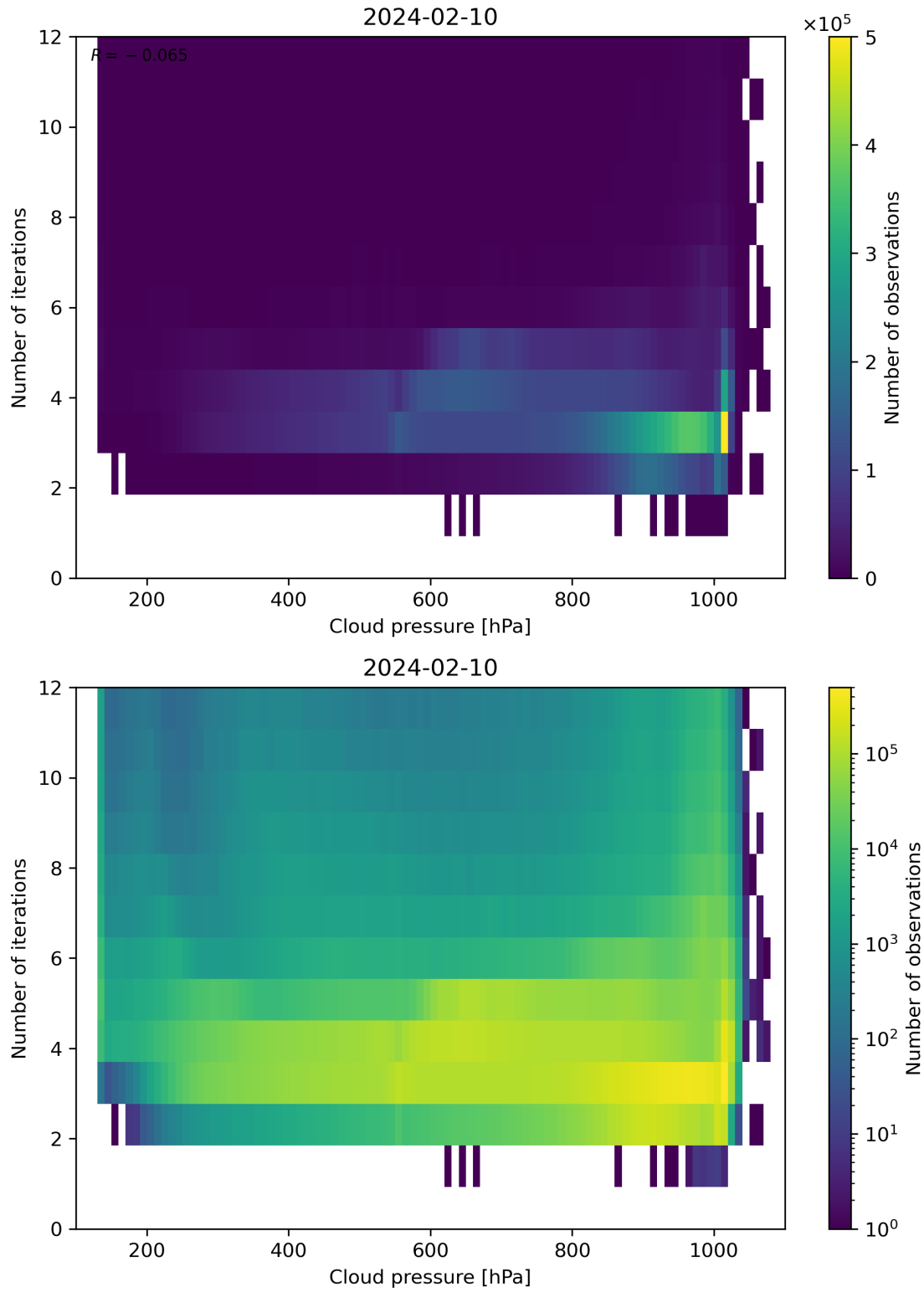
Figure 81: Scatter density plot of “Cloud pressure” against “Number of iterations” for 2024-02-09 to 2024-02-11.
