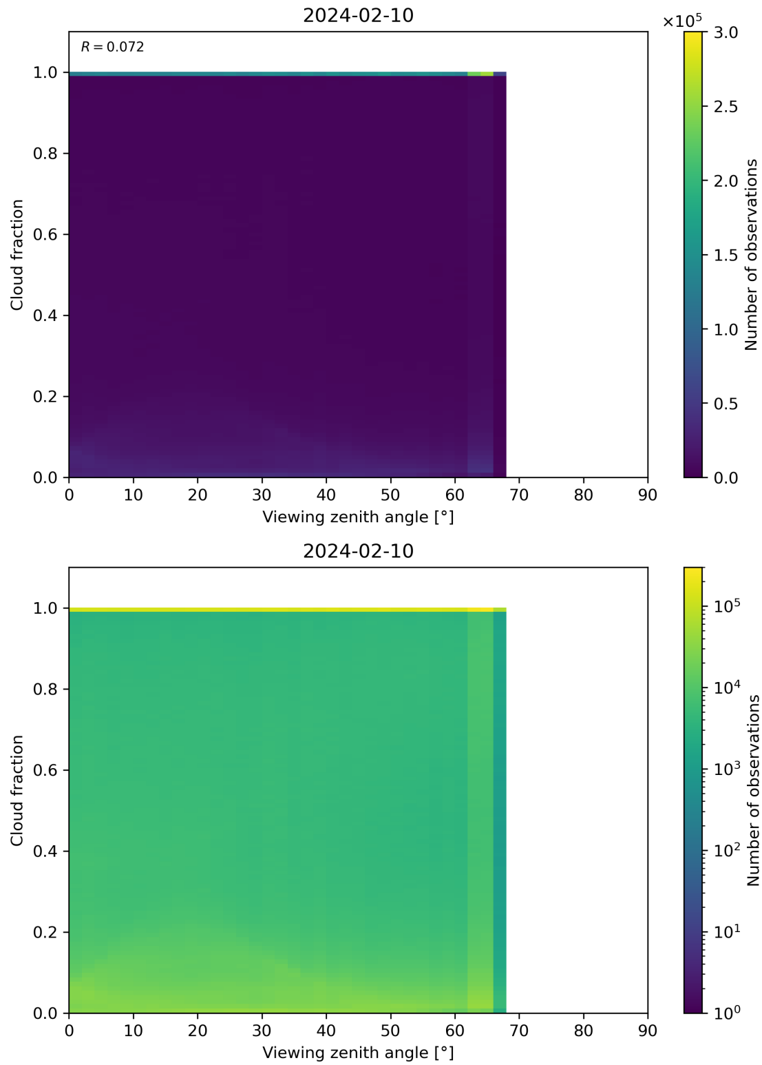
Figure 120: Scatter density plot of “Viewing zenith angle” against “Cloud fraction” for 2024-02-09 to 2024-02-11.
