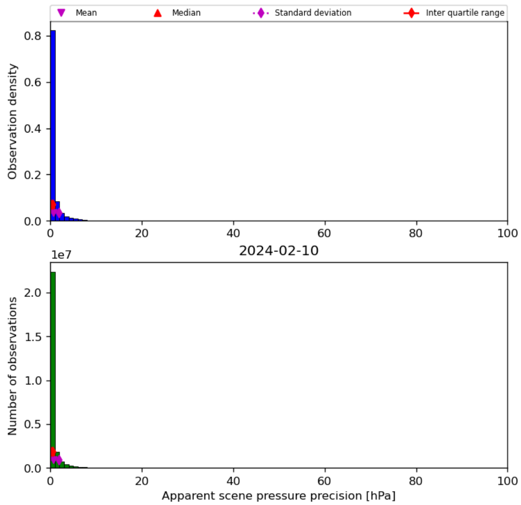
Figure 37: Histogram of “Apparent scene pressure precision” for 2024-02-09 to 2024-02-11
