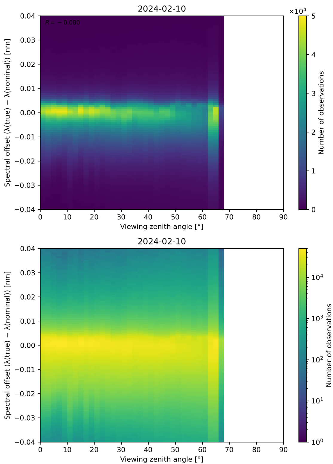
Figure 128: Scatter density plot of “Viewing zenith angle” against “Spectral offset ( \lambda(\text{true}) - \lambda(\text{nominal}) )” for 2024-02-09 to 2024-02-11.
