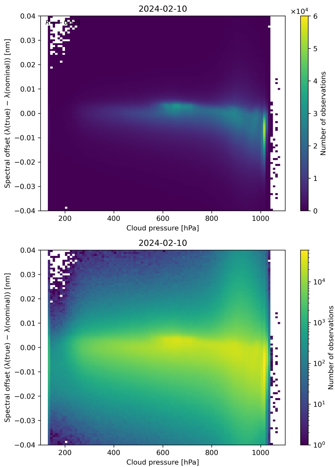
Figure 84: Scatter density plot of “Cloud pressure” against “Spectral offset ( \lambda(\text{true}) - \lambda(\text{nominal}) )” for 2024-02-09 to 2024-02-11.
