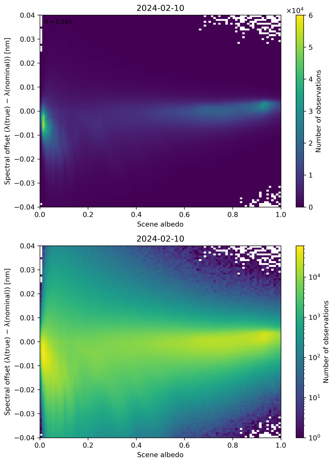
Figure 107: Scatter density plot of “Scene albedo” against “Spectral offset ( \lambda(\text{true}) - \lambda(\text{nominal}) )” for 2024-02-09 to 2024-02-11.
