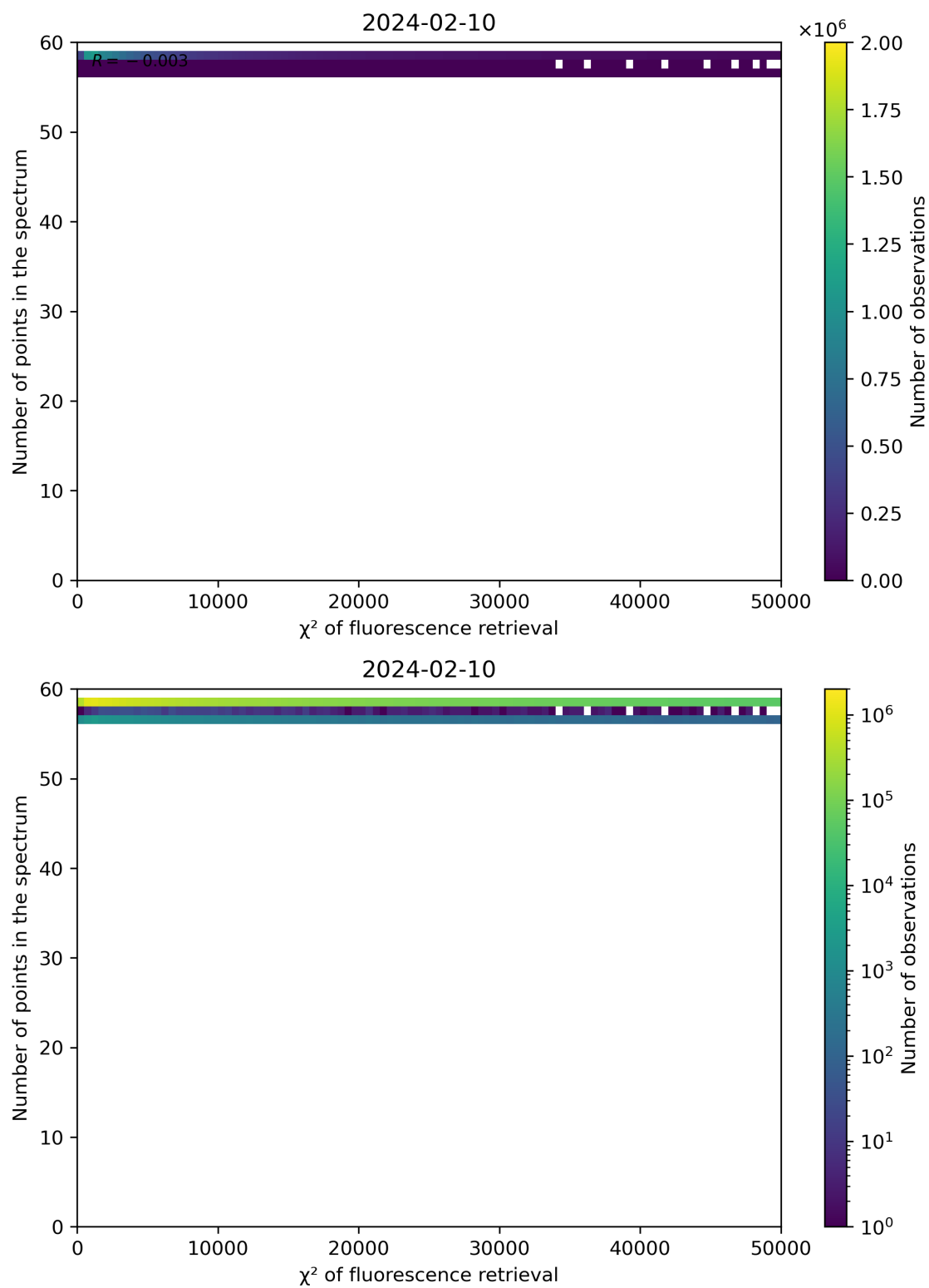
Figure 68: Scatter density plot of " \chi^2 of fluorescence retrieval" against "Number of points in the spectrum" for 2024-02-09 to 2024-02-11.
