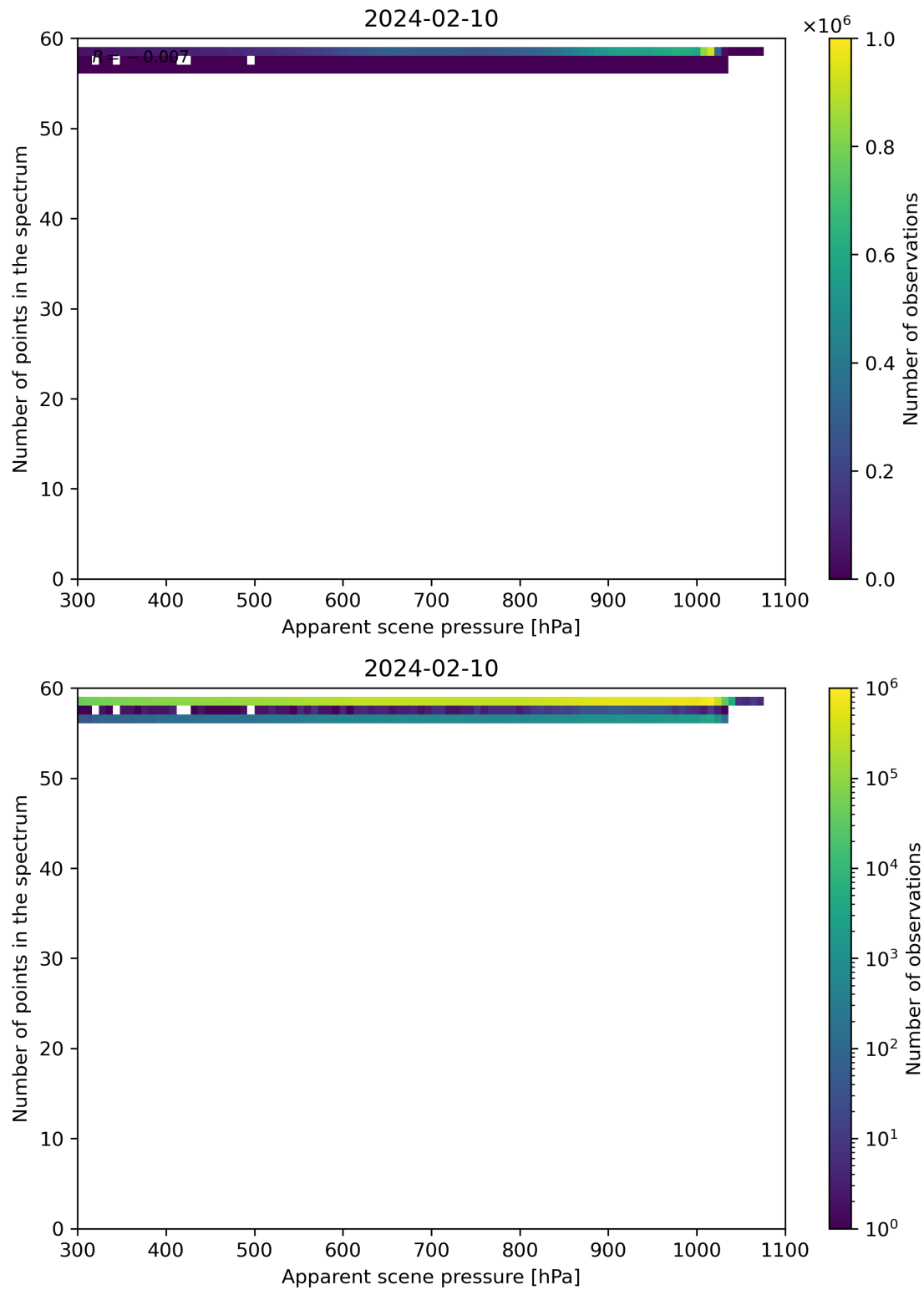
Figure 66: Scatter density plot of “Apparent scene pressure” against “Number of points in the spectrum” for 2024-02-09 to 2024-02-11.
