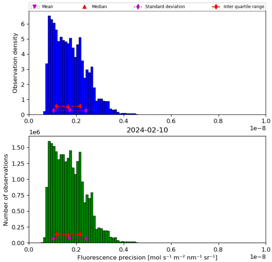
Figure 41: Histogram of “Fluorescence precision” for 2024-02-09 to 2024-02-11
