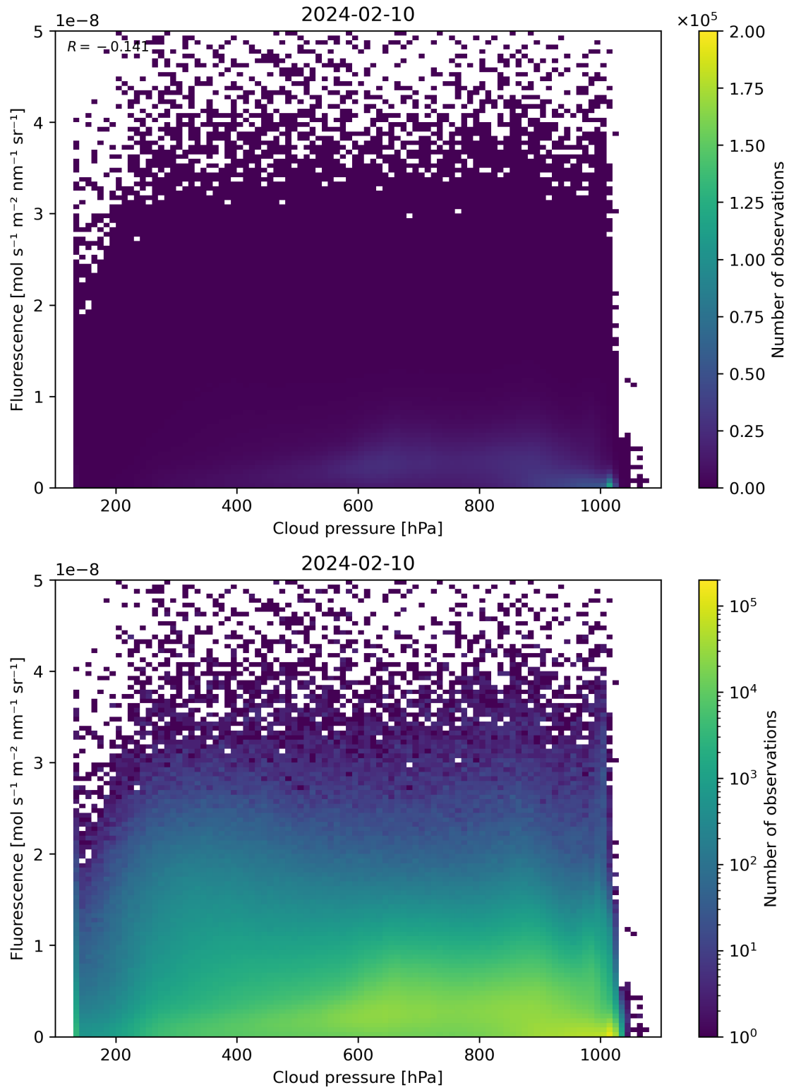
Figure 80: Scatter density plot of “Cloud pressure” against “Fluorescence” for 2024-02-09 to 2024-02-11.
