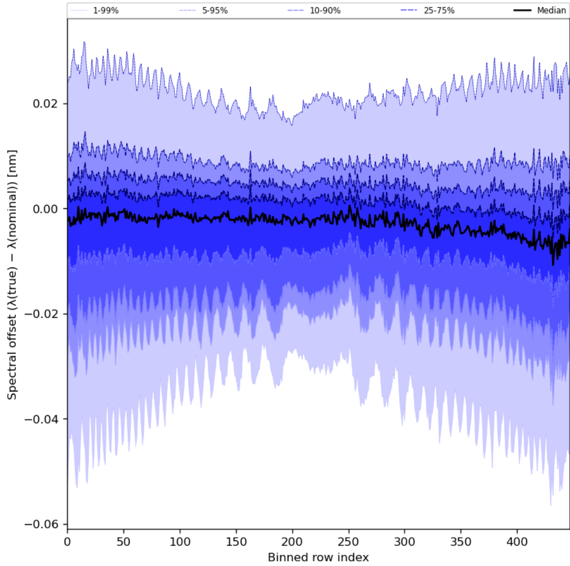
Figure 62: Along track statistics of “Spectral offset ( \lambda(\text{true}) - \lambda(\text{nominal}) )” for 2024-02-09 to 2024-02-11
