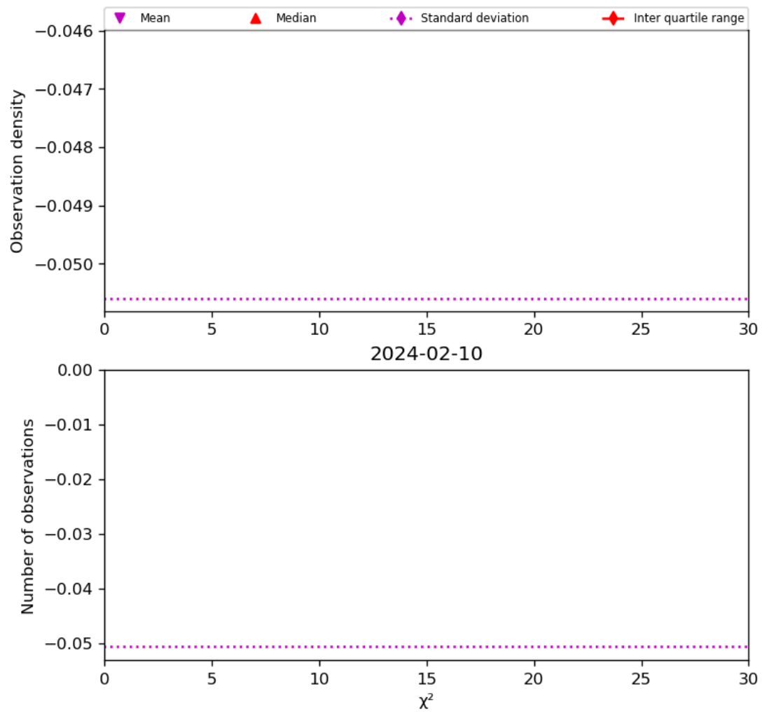
Figure 38: Histogram of “ \chi^2 ” for 2024-02-09 to 2024-02-11
