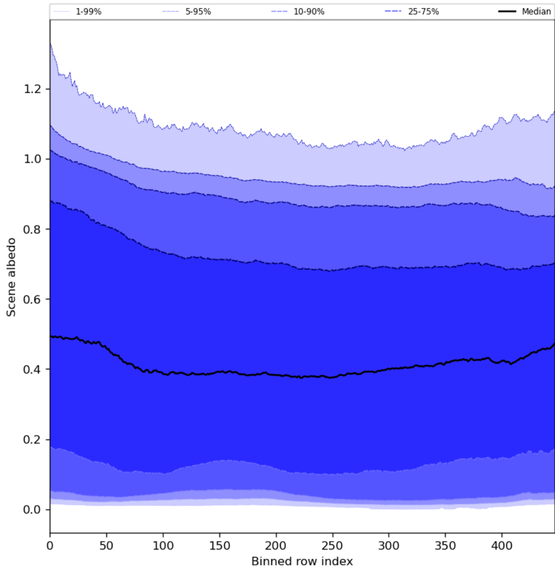
Figure 51: Along track statistics of “Scene albedo” for 2024-02-09 to 2024-02-11
