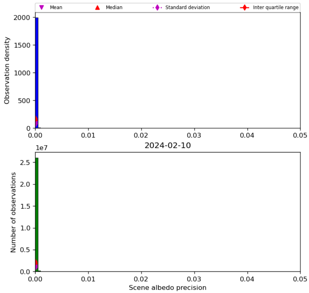
Figure 35: Histogram of “Scene albedo precision” for 2024-02-09 to 2024-02-11
