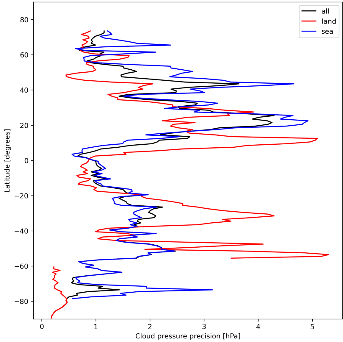
Figure 14: Zonal average of “Cloud pressure precision” for 2024-02-09 to 2024-02-11.
