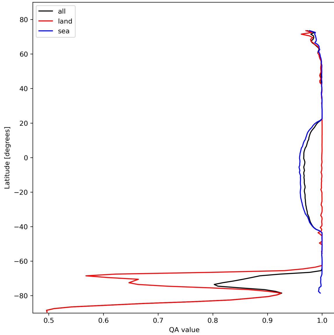
Figure 12: Zonal average of “QA value” for 2024-02-09 to 2024-02-11.
