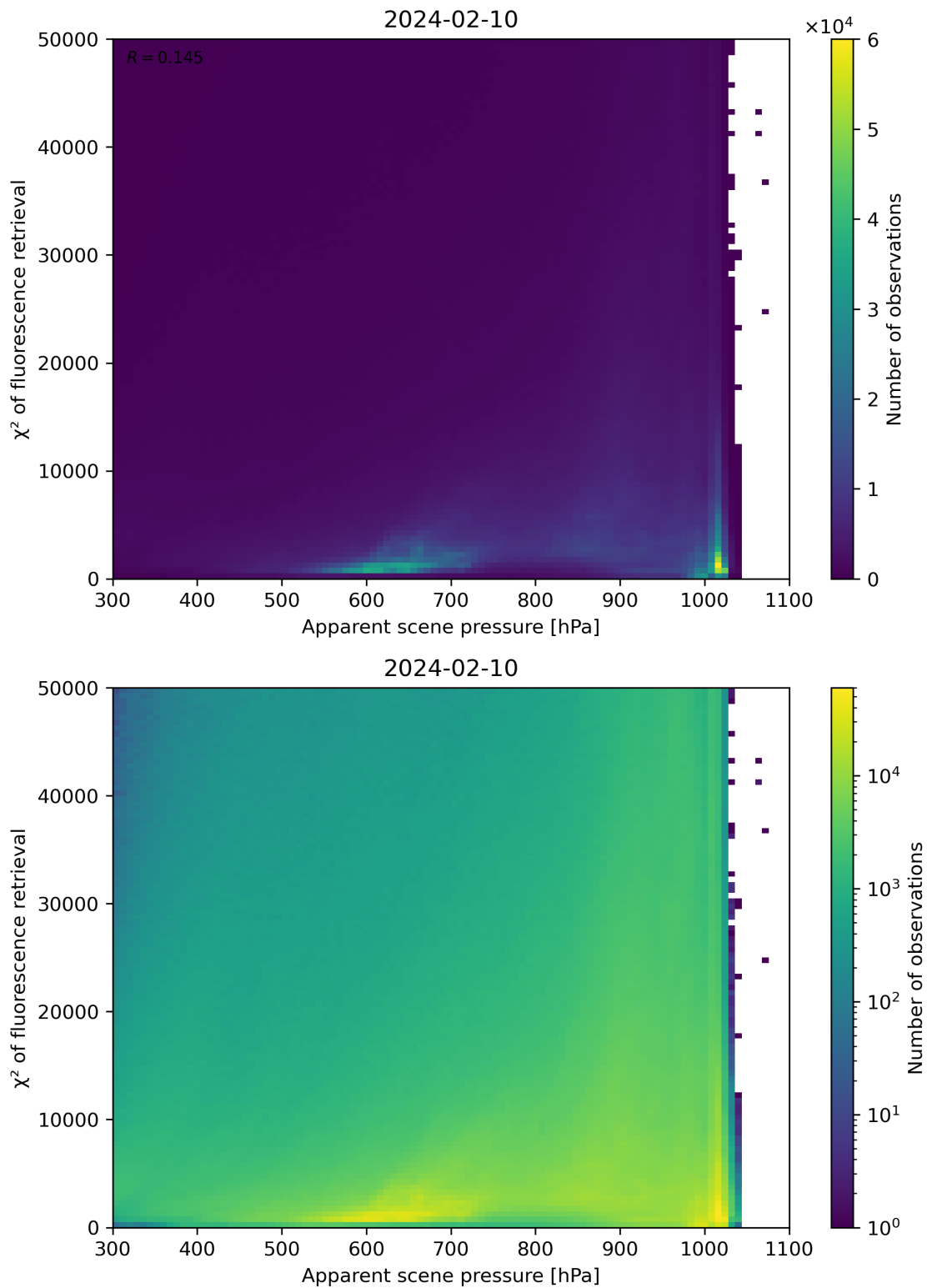
Figure 63: Scatter density plot of “Apparent scene pressure” against “ \chi^2 of fluorescence retrieval” for 2024-02-09 to 2024-02-11.
