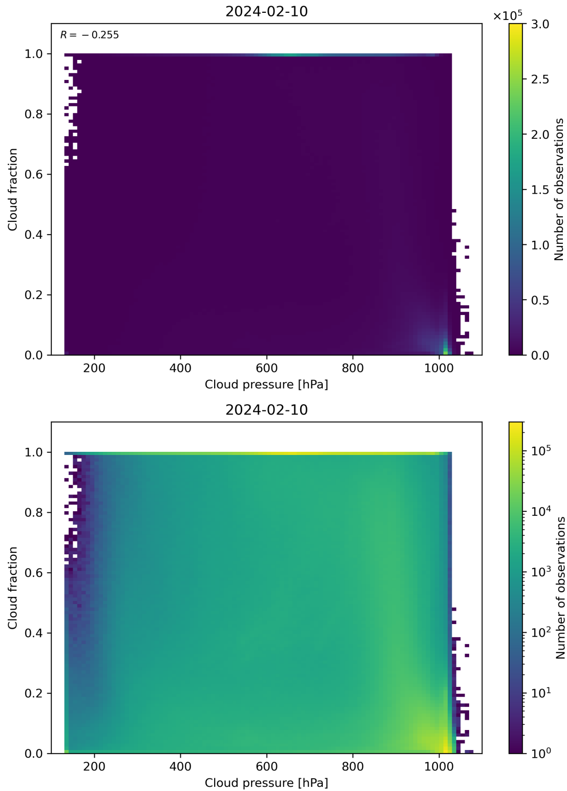
Figure 79: Scatter density plot of “Cloud pressure” against “Cloud fraction” for 2024-02-09 to 2024-02-11.
