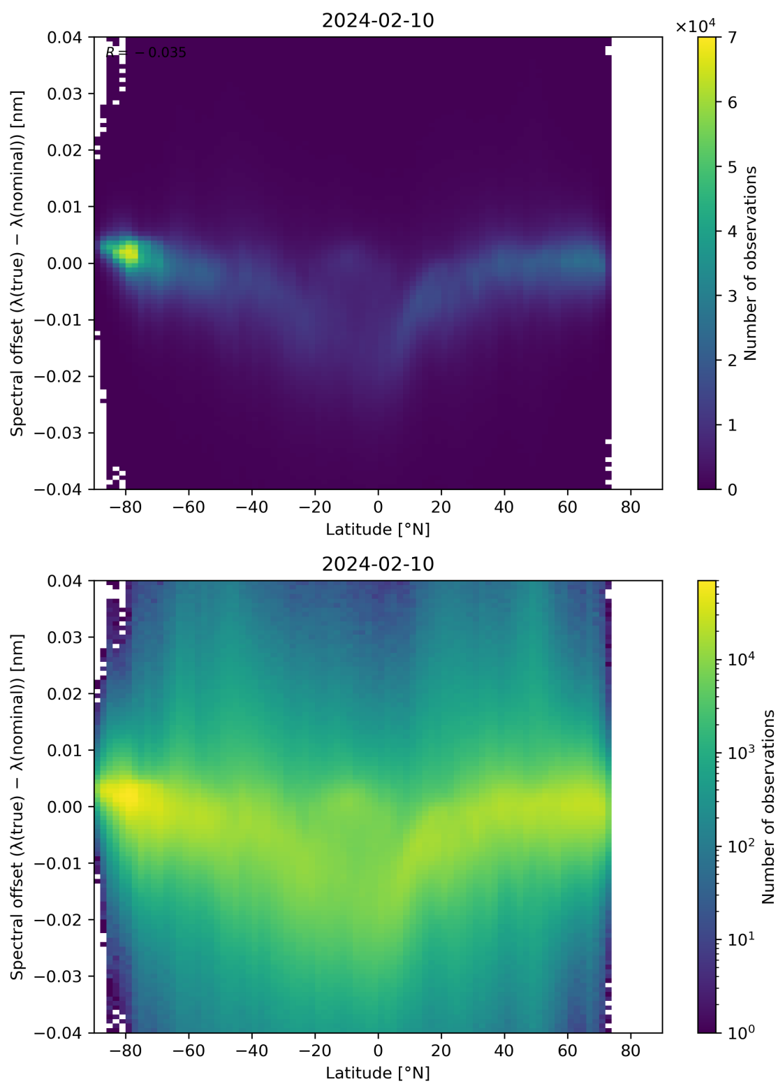
Figure 96: Scatter density plot of “Latitude” against “Spectral offset ( \lambda(\text{true}) - \lambda(\text{nominal}) )” for 2024-02-09 to 2024-02-11.
