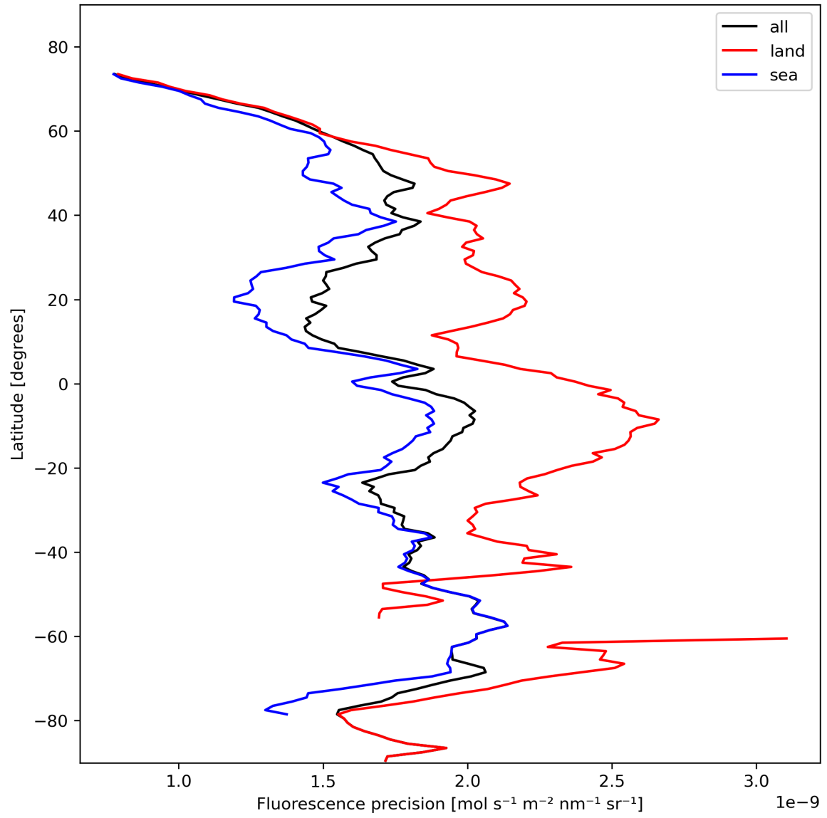
Figure 24: Zonal average of “Fluorescence precision” for 2024-02-09 to 2024-02-11.
