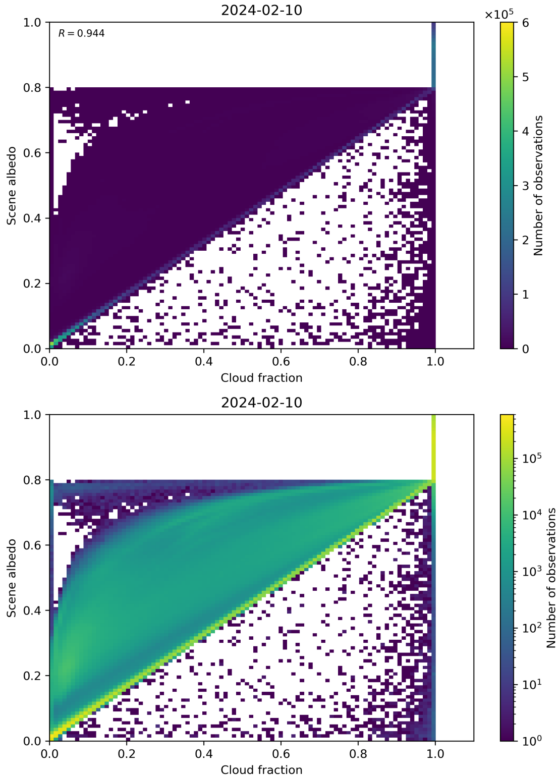
Figure 75: Scatter density plot of “Cloud fraction” against “Scene albedo” for 2024-02-09 to 2024-02-11.
