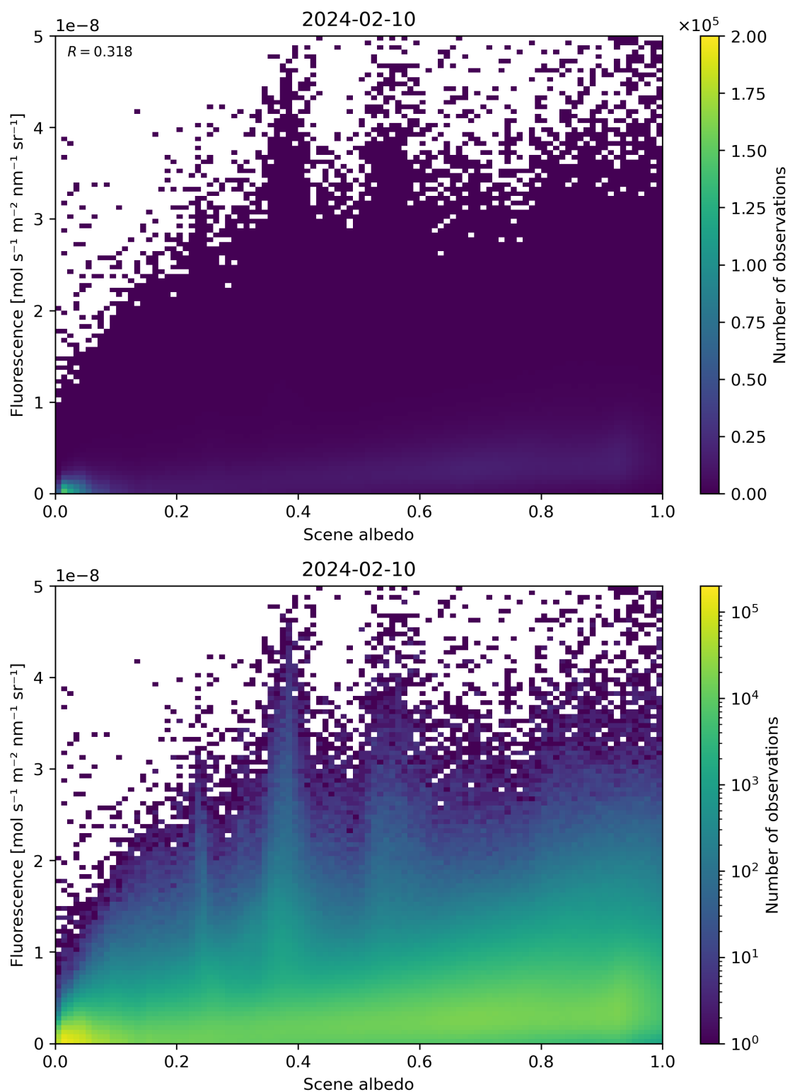
Figure 104: Scatter density plot of “Scene albedo” against “Fluorescence” for 2024-02-09 to 2024-02-11.
