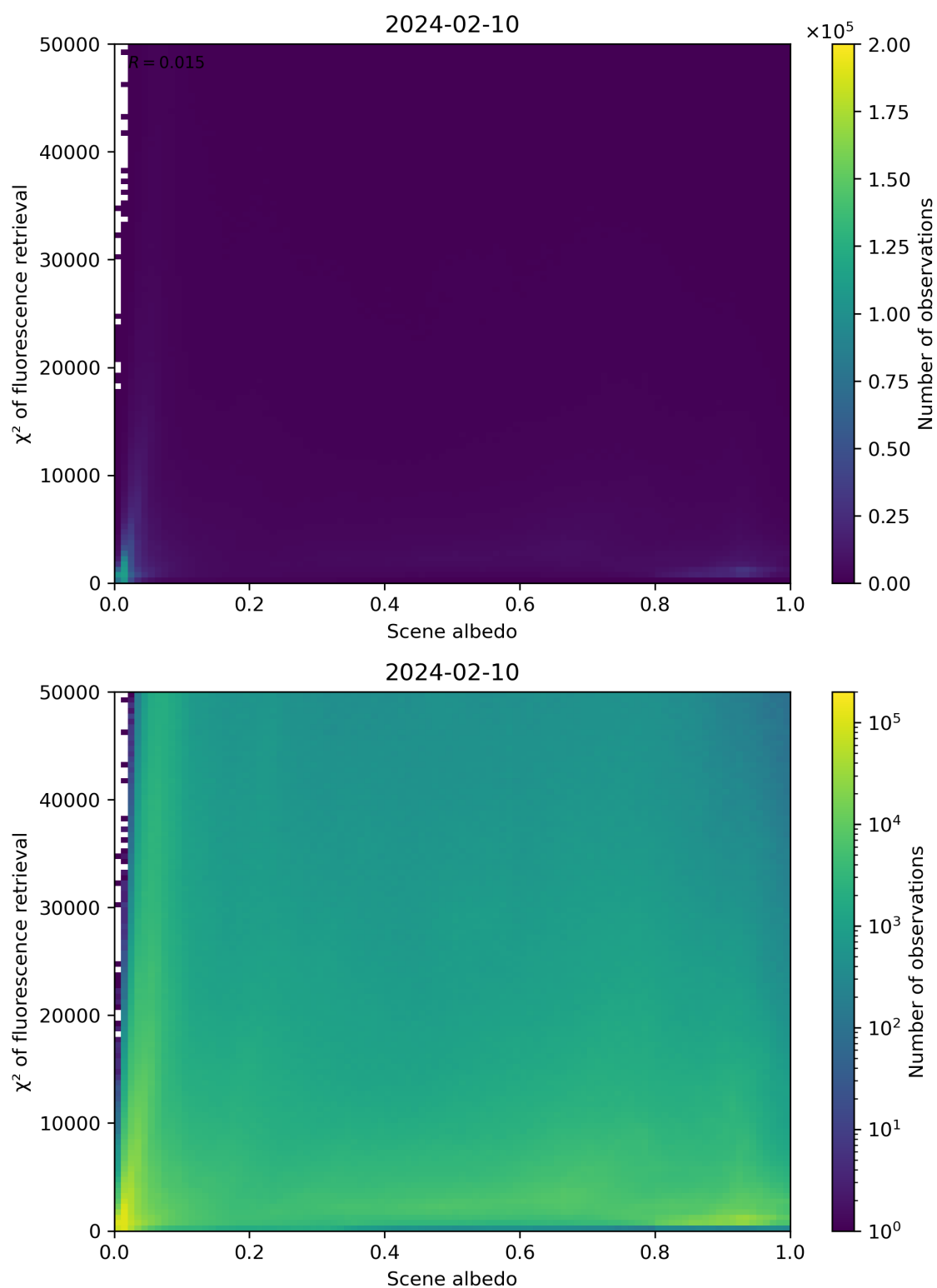
Figure 103: Scatter density plot of “Scene albedo” against “ \chi^2 of fluorescence retrieval” for 2024-02-09 to 2024-02-11.
