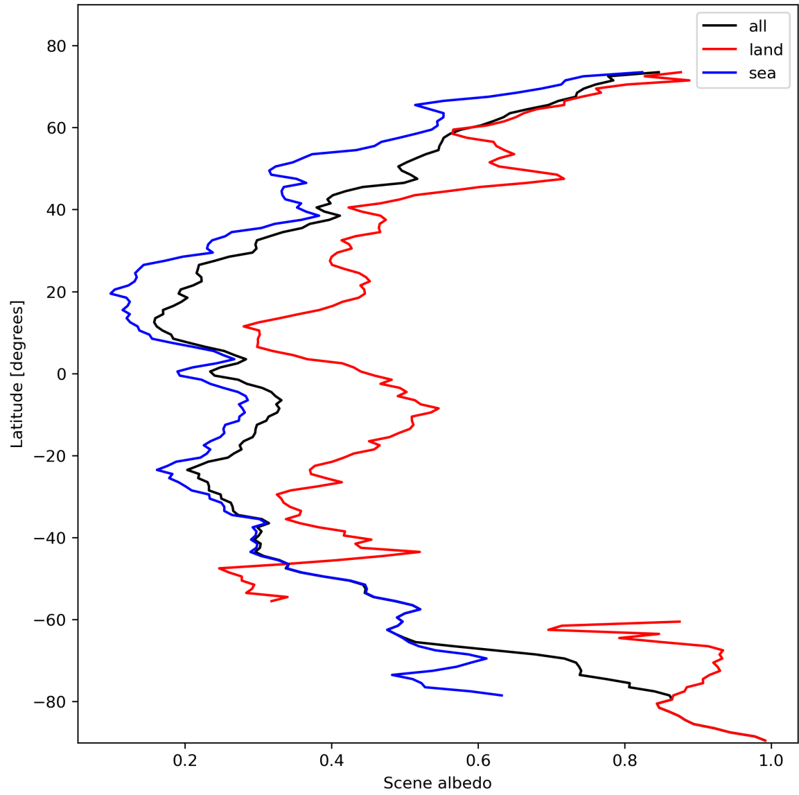
Figure 17: Zonal average of “Scene albedo” for 2024-02-09 to 2024-02-11.
