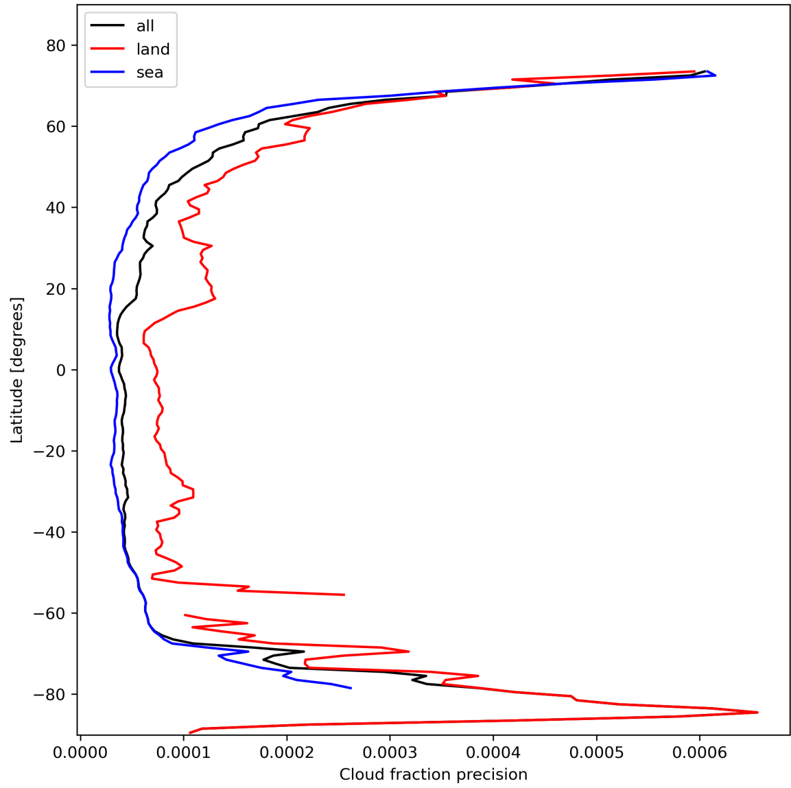
Figure 16: Zonal average of “Cloud fraction precision” for 2024-02-09 to 2024-02-11.
