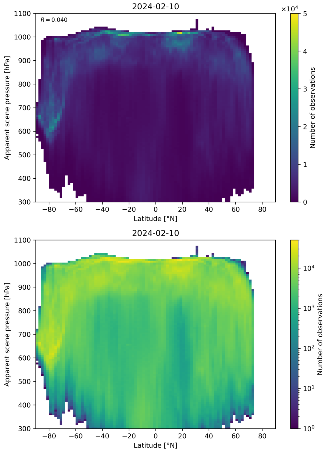
Figure 88: Scatter density plot of “Latitude” against “Apparent scene pressure” for 2024-02-09 to 2024-02-11.
