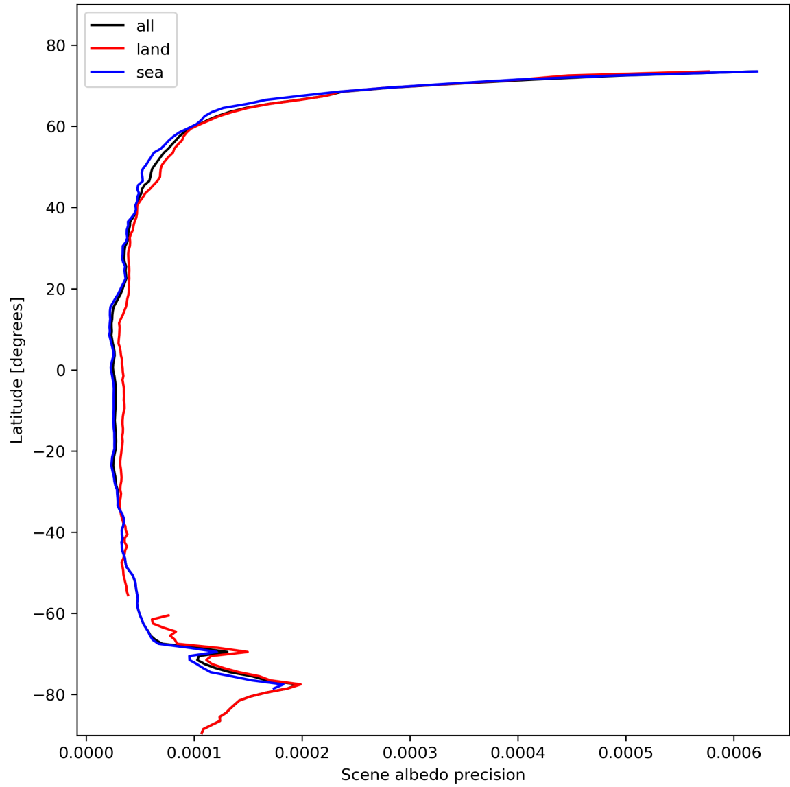
Figure 18: Zonal average of “Scene albedo precision” for 2024-02-09 to 2024-02-11.
