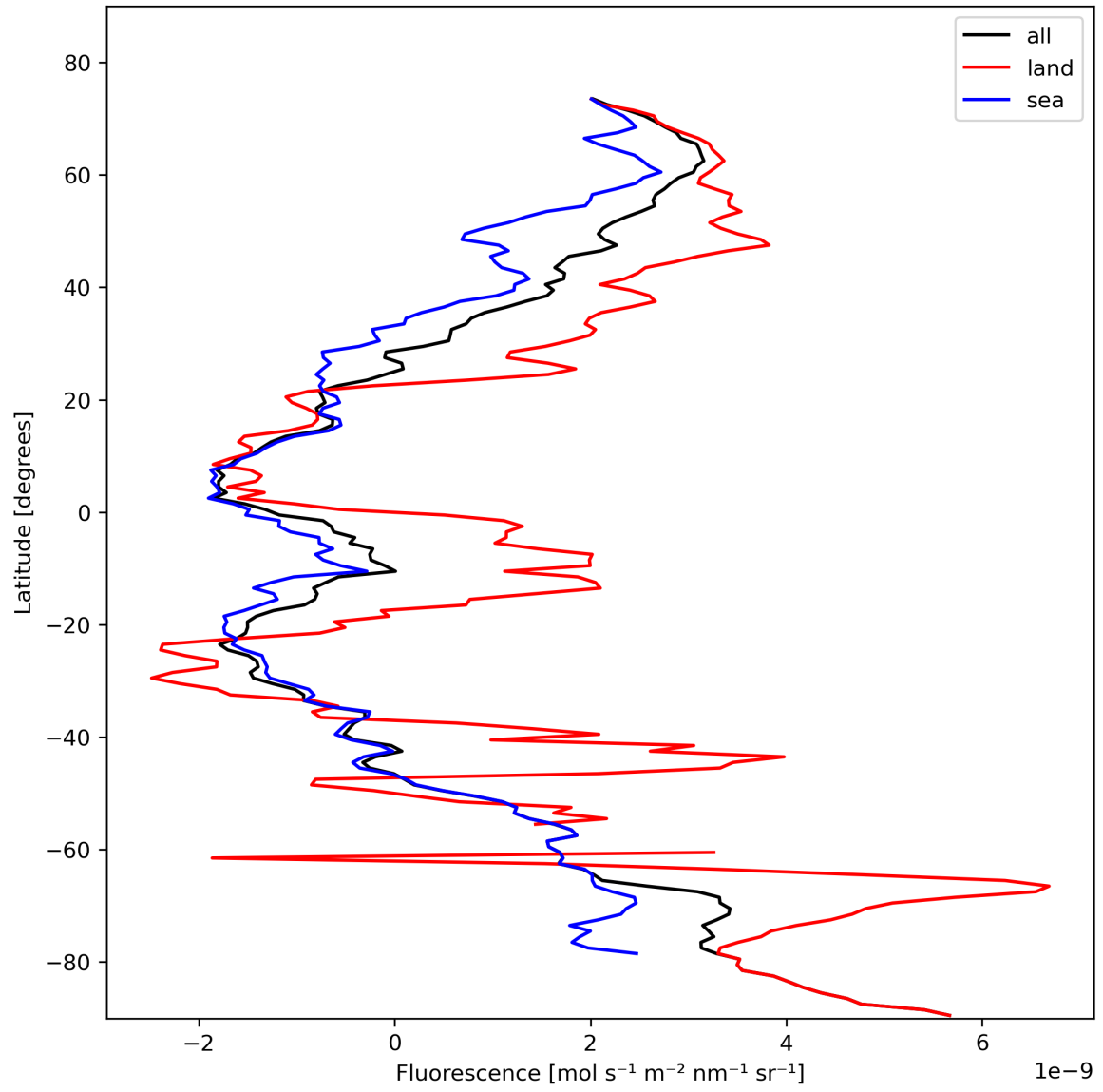
Figure 23: Zonal average of “Fluorescence” for 2024-02-09 to 2024-02-11.
