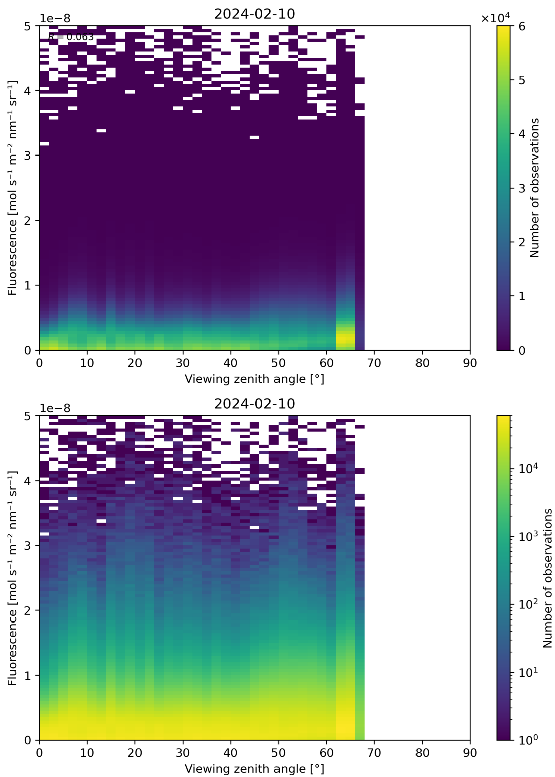
Figure 122: Scatter density plot of “Viewing zenith angle” against “Fluorescence” for 2024-02-09 to 2024-02-11.
