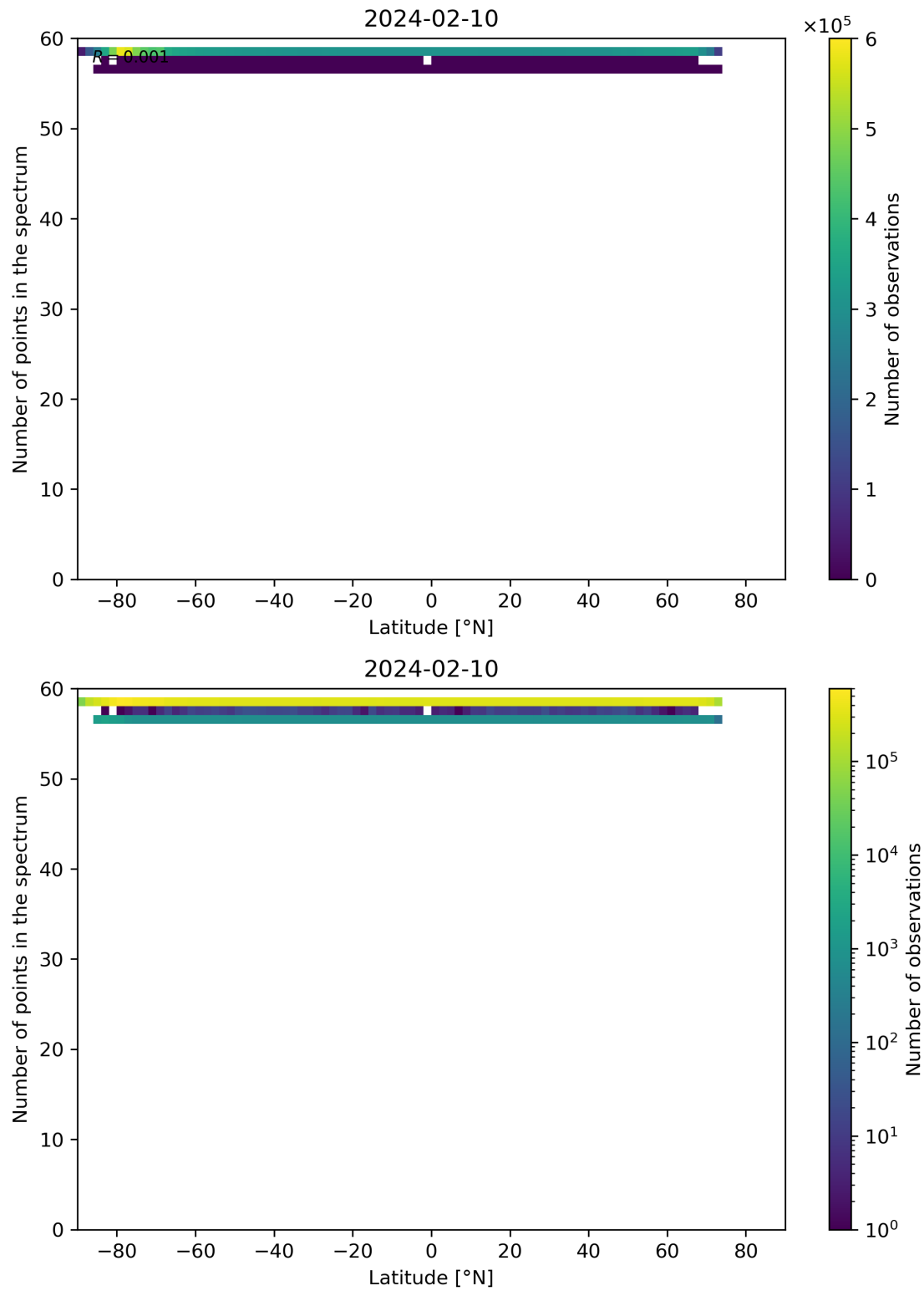
Figure 94: Scatter density plot of “Latitude” against “Number of points in the spectrum” for 2024-02-09 to 2024-02-11.
