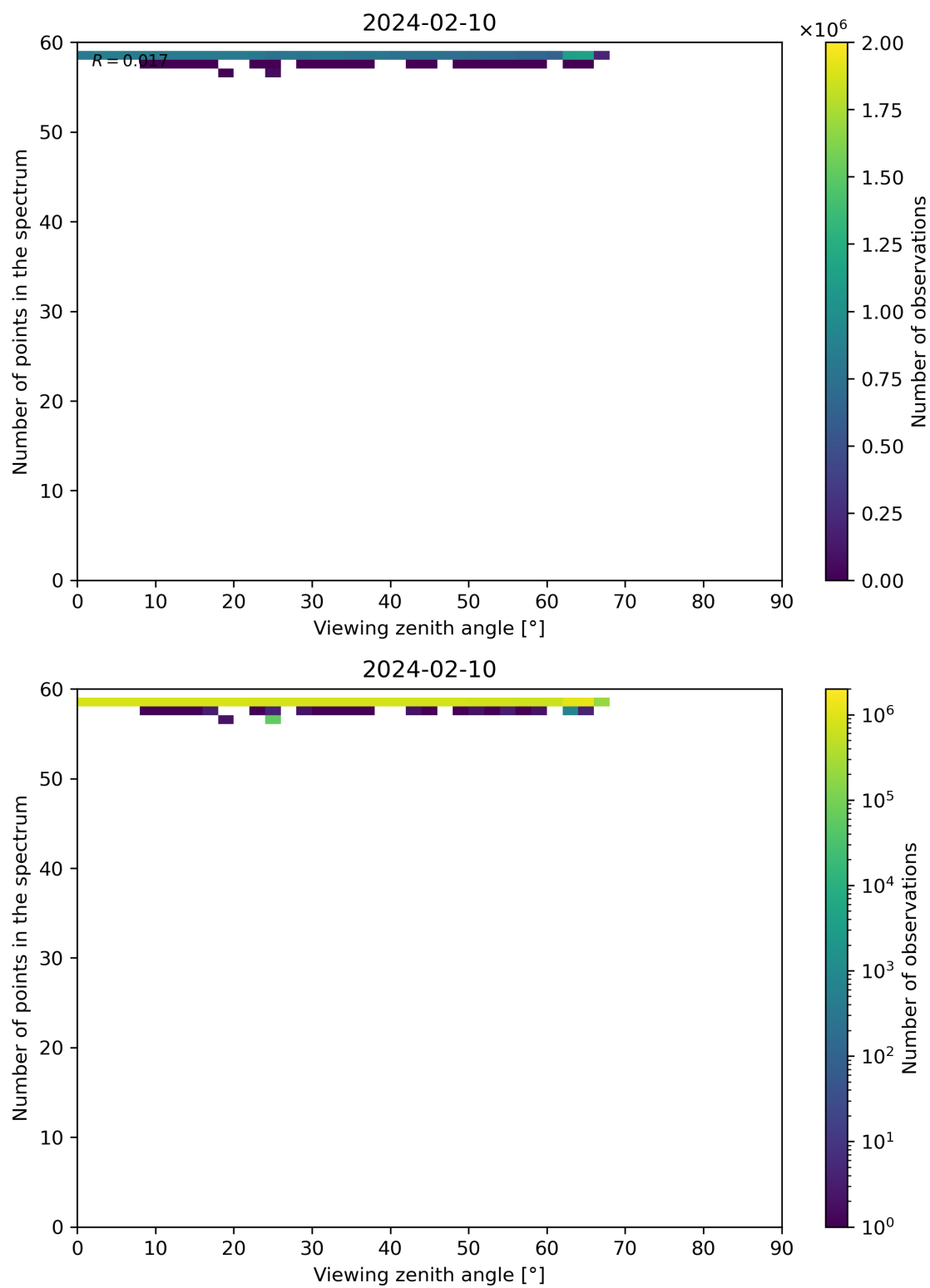
Figure 125: Scatter density plot of “Viewing zenith angle” against “Number of points in the spectrum” for 2024-02-09 to 2024-02-11.
