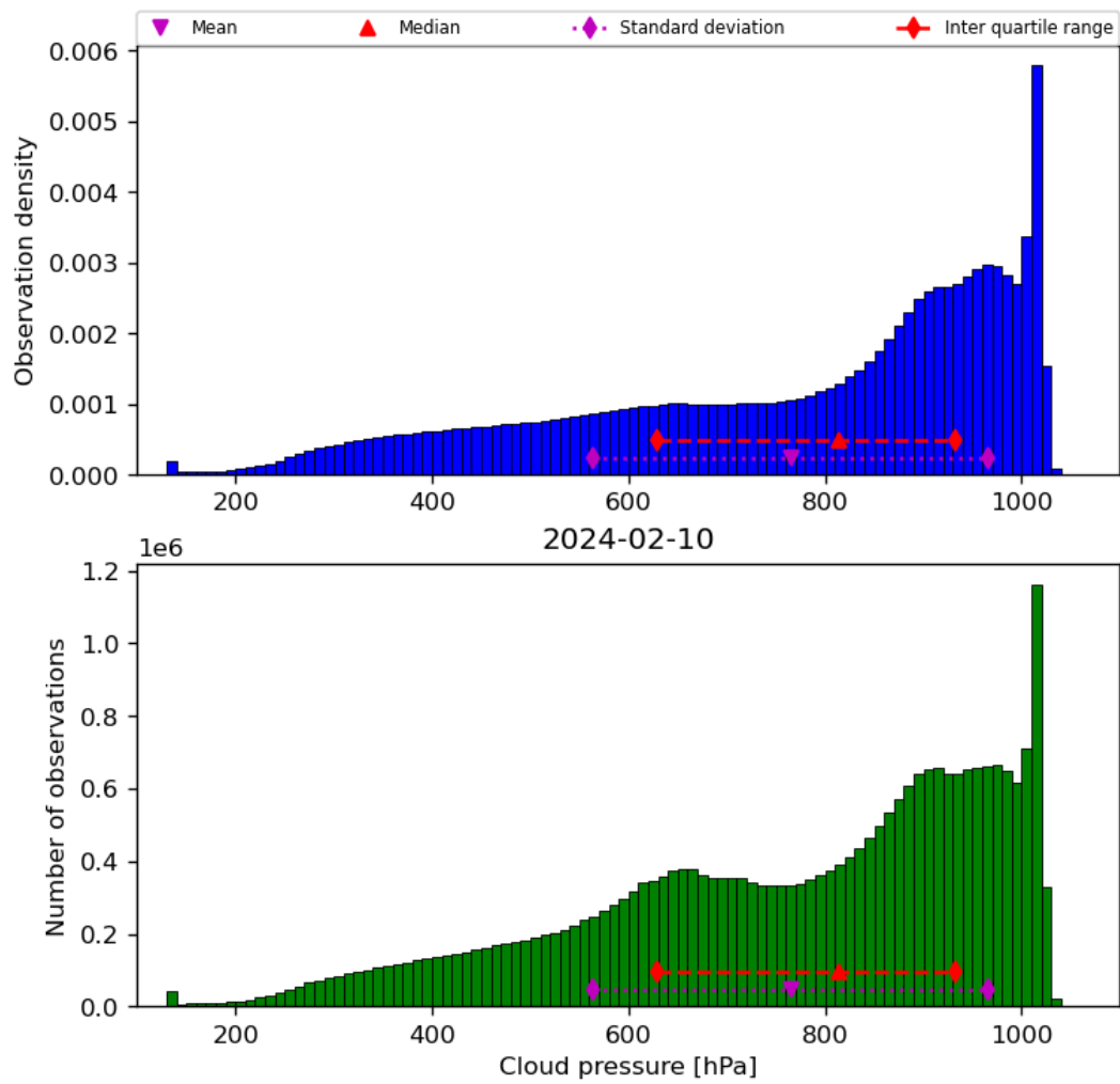
Figure 30: Histogram of “Cloud pressure” for 2024-02-09 to 2024-02-11
