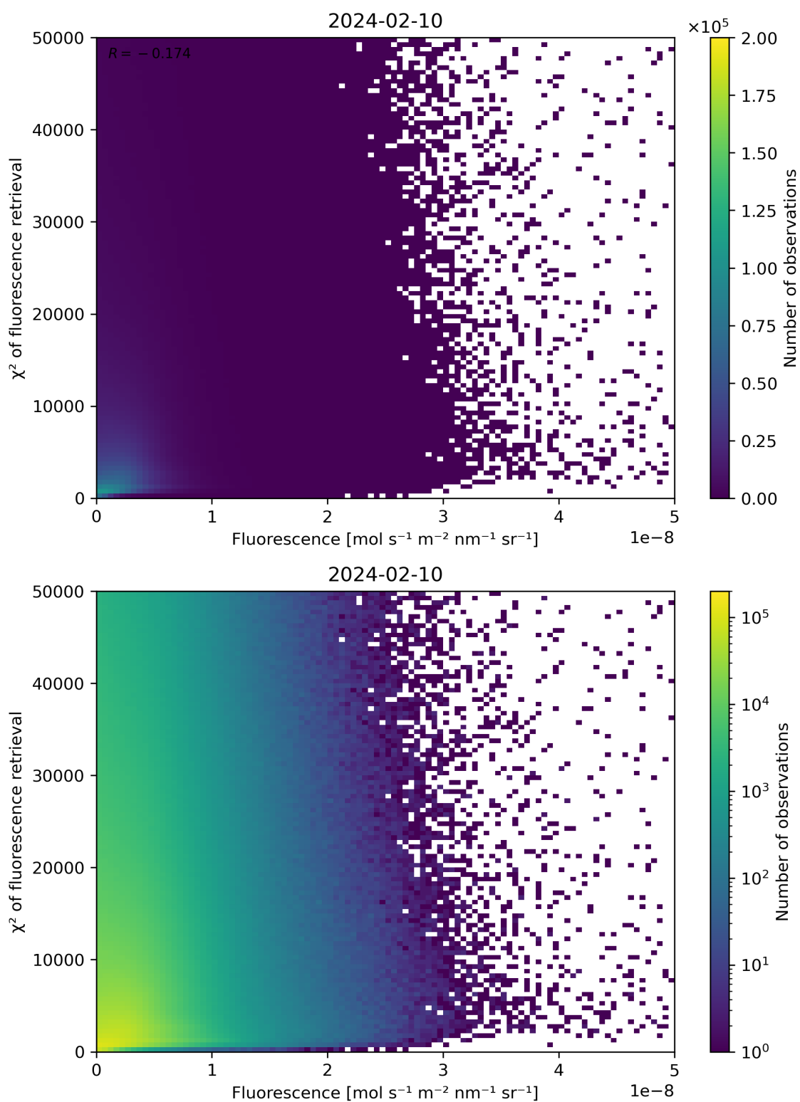
Figure 85: Scatter density plot of “Fluorescence” against “ \chi^2 of fluorescence retrieval” for 2024-02-09 to 2024-02-11.
