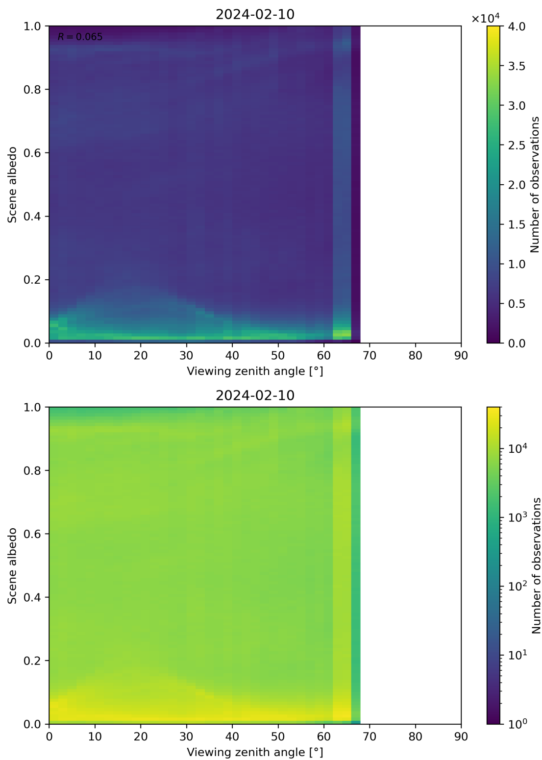
Figure 126: Scatter density plot of “Viewing zenith angle” against “Scene albedo” for 2024-02-09 to 2024-02-11.
