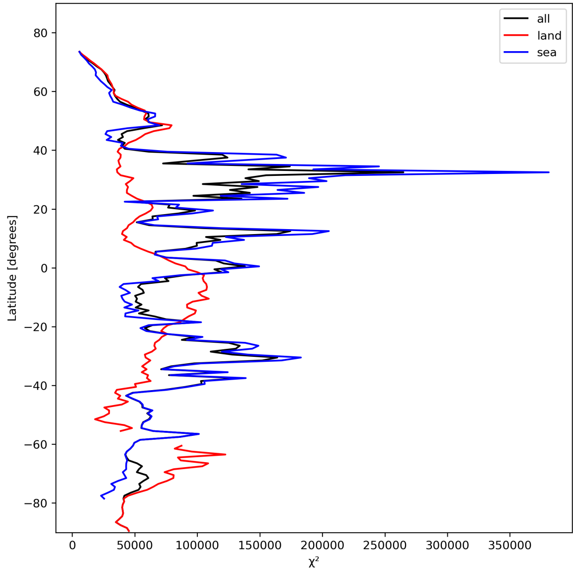
Figure 21: Zonal average of “ \chi^2 ” for 2024-02-09 to 2024-02-11.
