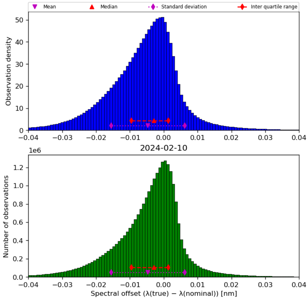
Figure 45: Histogram of “Spectral offset ( \lambda(\text{true}) - \lambda(\text{nominal}) )” for 2024-02-09 to 2024-02-11
