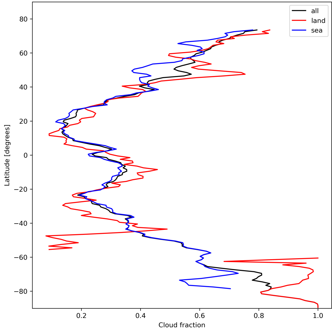
Figure 15: Zonal average of “Cloud fraction” for 2024-02-09 to 2024-02-11.
