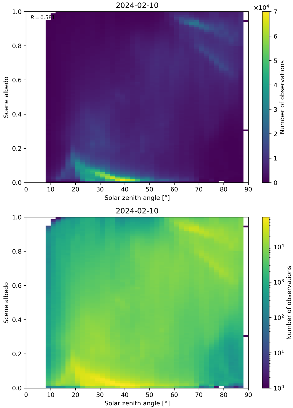
Figure 116: Scatter density plot of “Solar zenith angle” against “Scene albedo” for 2024-02-09 to 2024-02-11.
