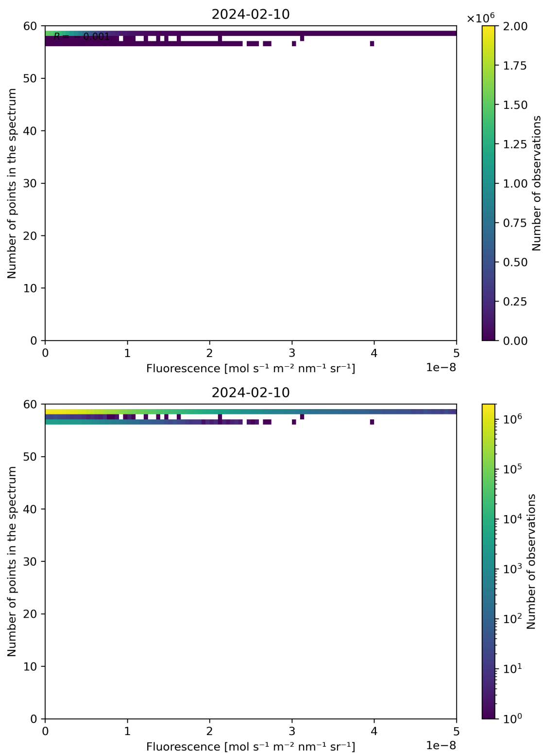
Figure 86: Scatter density plot of “Fluorescence” against “Number of points in the spectrum” for 2024-02-09 to 2024-02-11.
