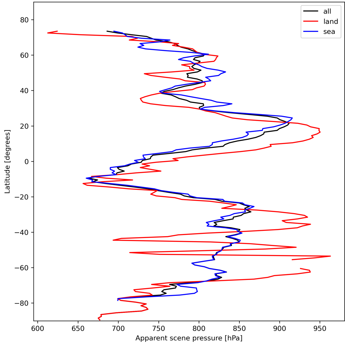
Figure 19: Zonal average of “Apparent scene pressure” for 2024-02-09 to 2024-02-11.
