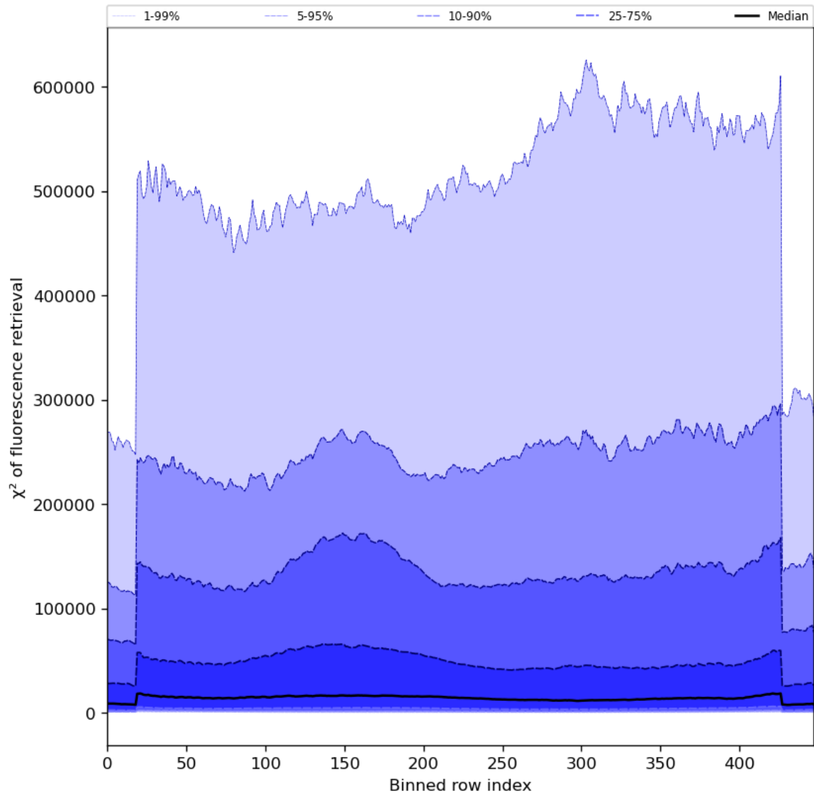
Figure 59: Along track statistics of “ \chi^2 of fluorescence retrieval” for 2024-02-09 to 2024-02-11
