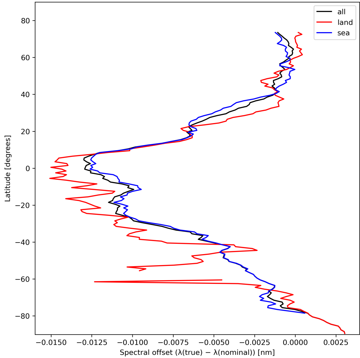
Figure 28: Zonal average of “Spectral offset ( \lambda(\text{true}) - \lambda(\text{nominal}) )” for 2024-02-09 to 2024-02-11.
