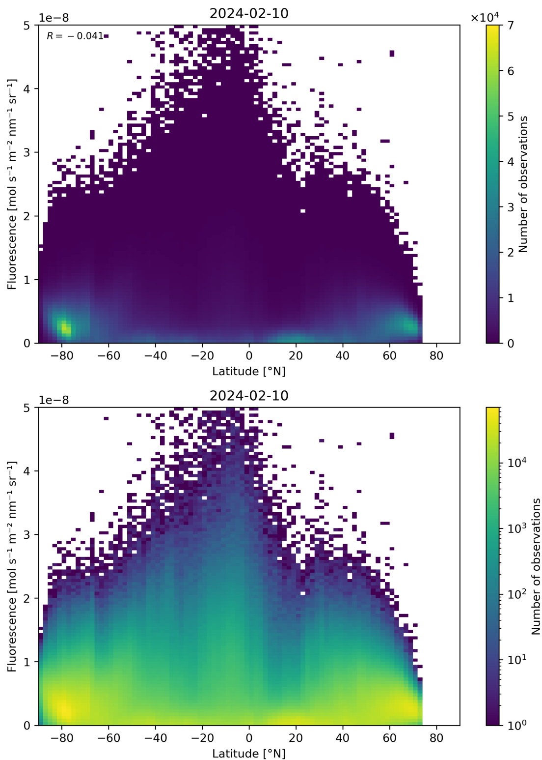
Figure 92: Scatter density plot of “Latitude” against “Fluorescence” for 2024-02-09 to 2024-02-11.
