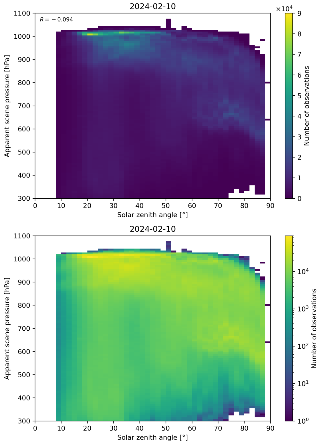
Figure 108: Scatter density plot of “Solar zenith angle” against “Apparent scene pressure” for 2024-02-09 to 2024-02-11.
