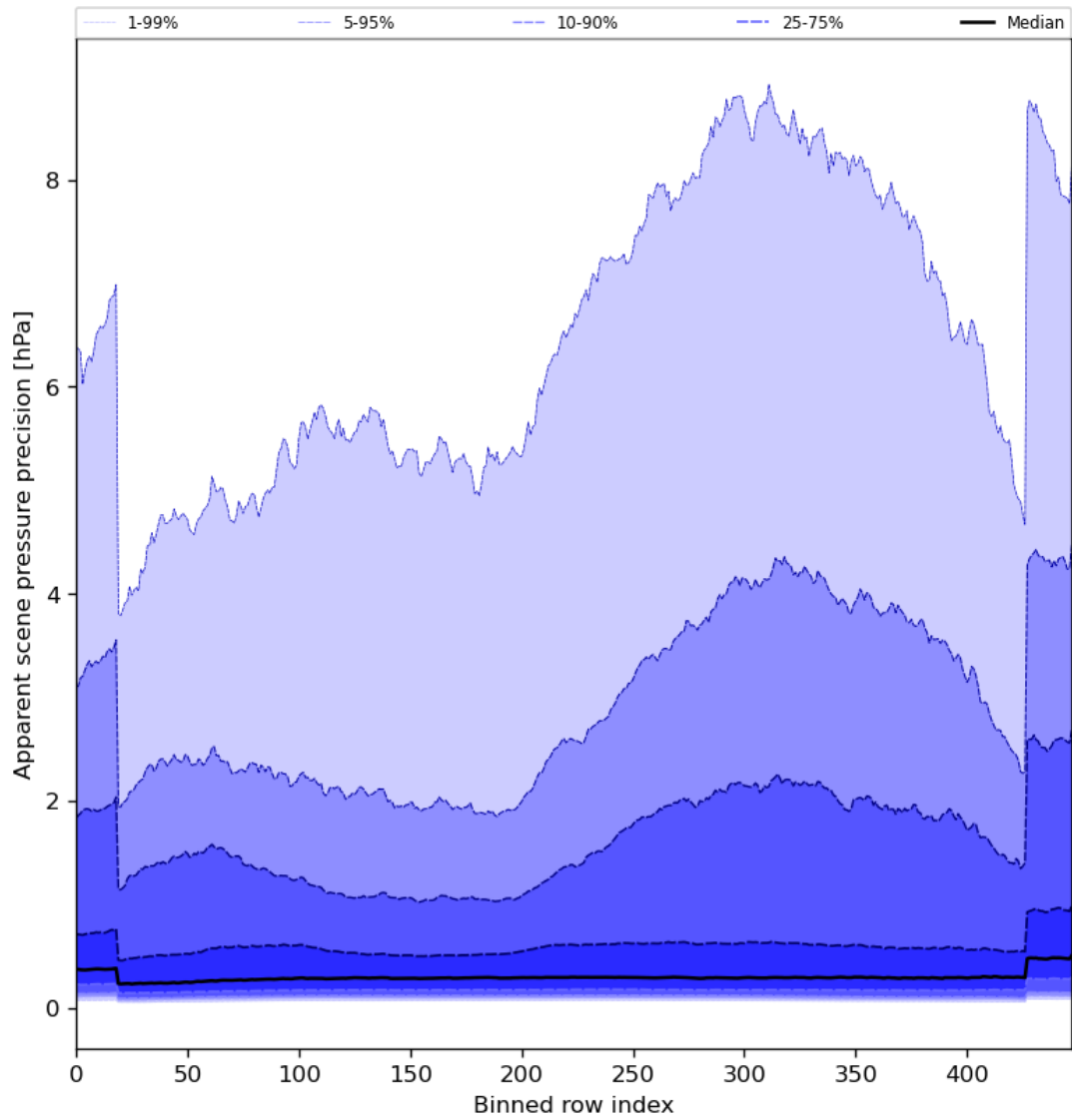
Figure 54: Along track statistics of “Apparent scene pressure precision” for 2024-02-09 to 2024-02-11
