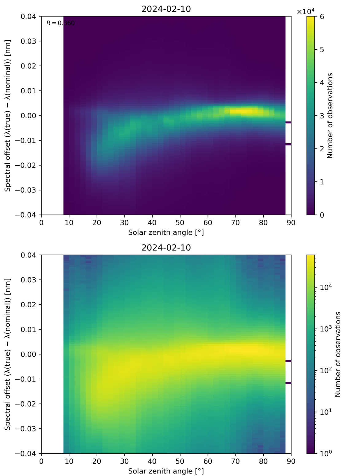
Figure 117: Scatter density plot of “Solar zenith angle” against “Spectral offset ( \lambda(\text{true}) - \lambda(\text{nominal}) )” for 2024-02-09 to 2024-02-11.
