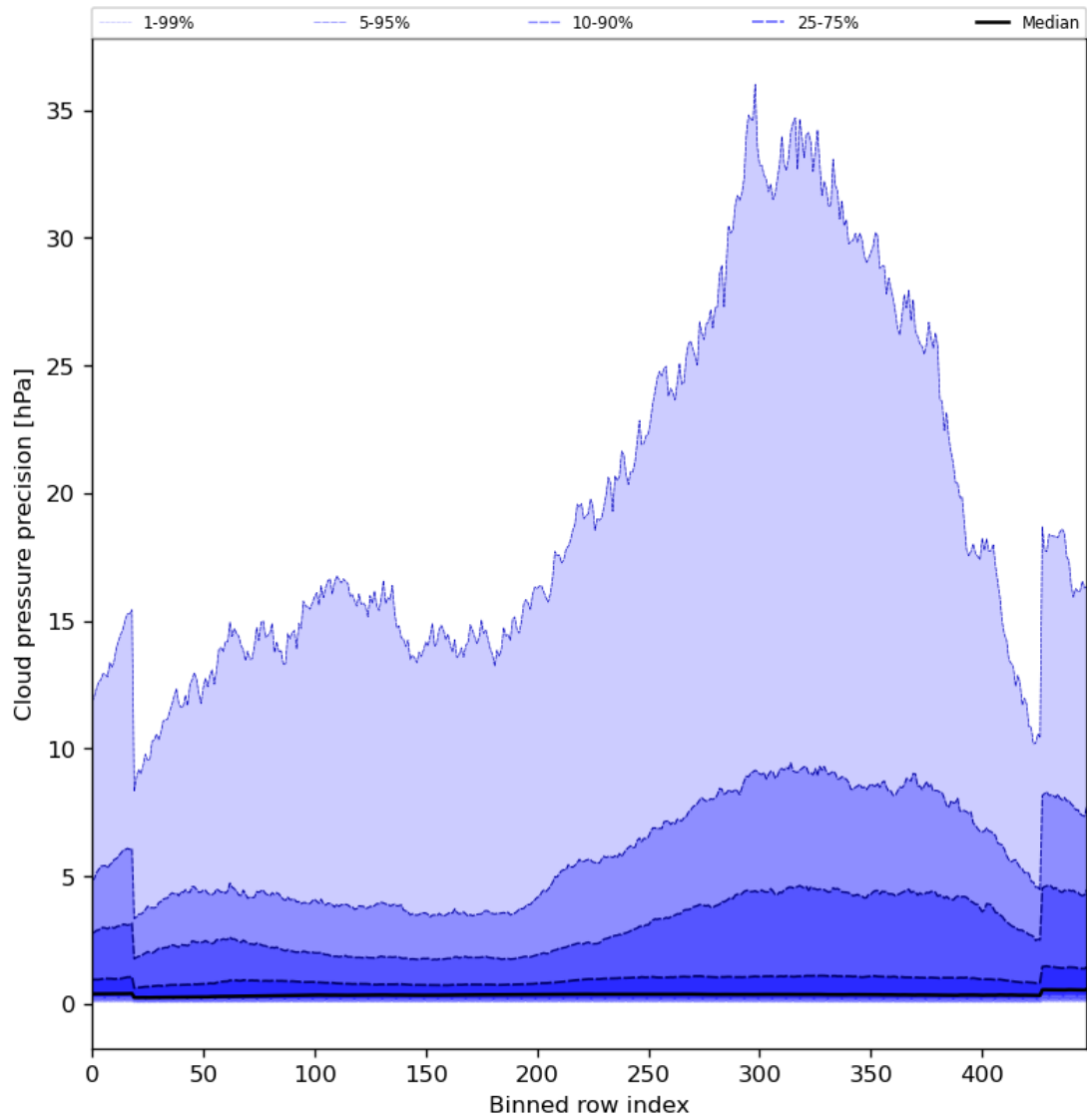
Figure 48: Along track statistics of “Cloud pressure precision” for 2024-02-09 to 2024-02-11
