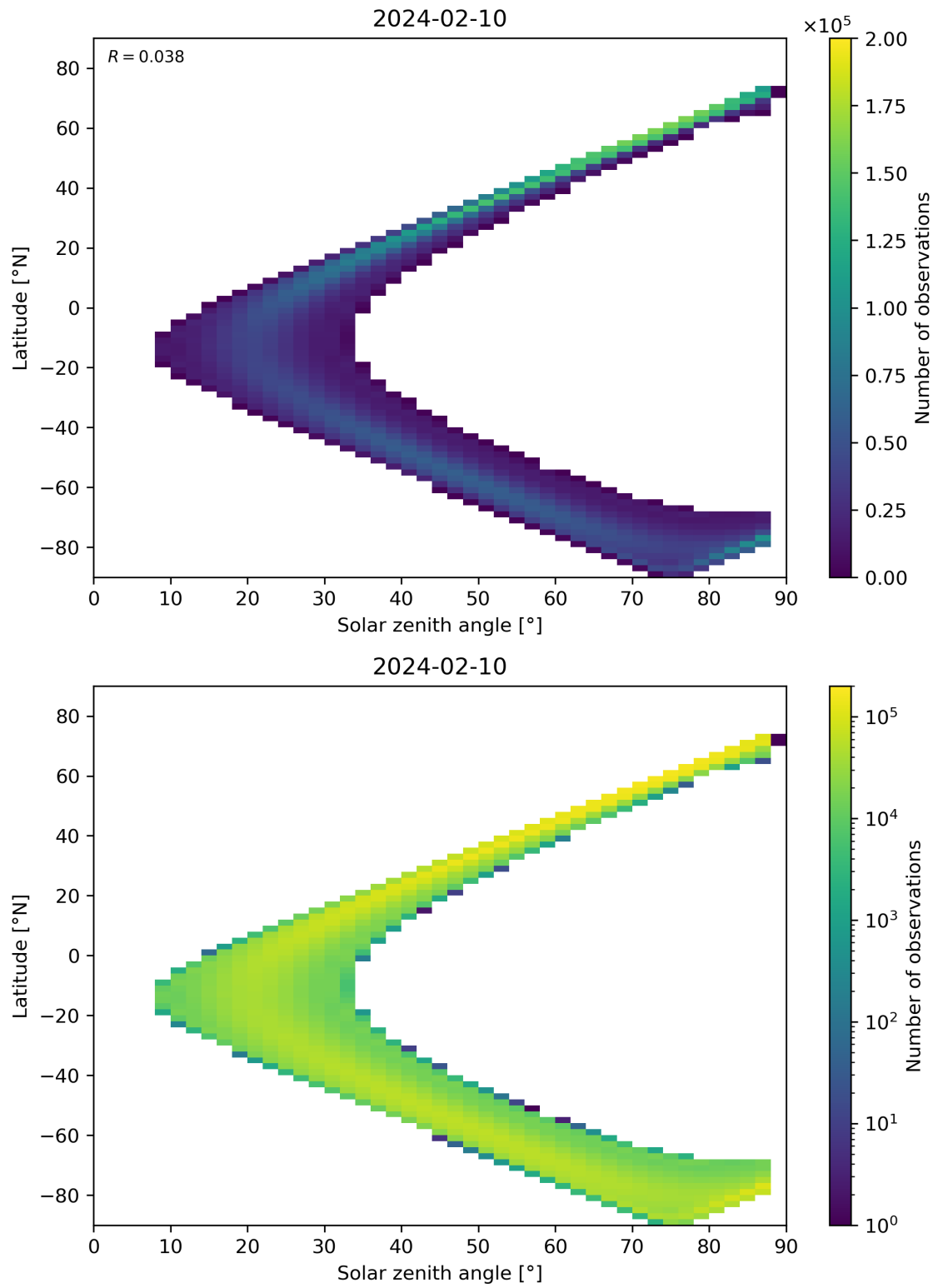
Figure 113: Scatter density plot of “Solar zenith angle” against “Latitude” for 2024-02-09 to 2024-02-11.
