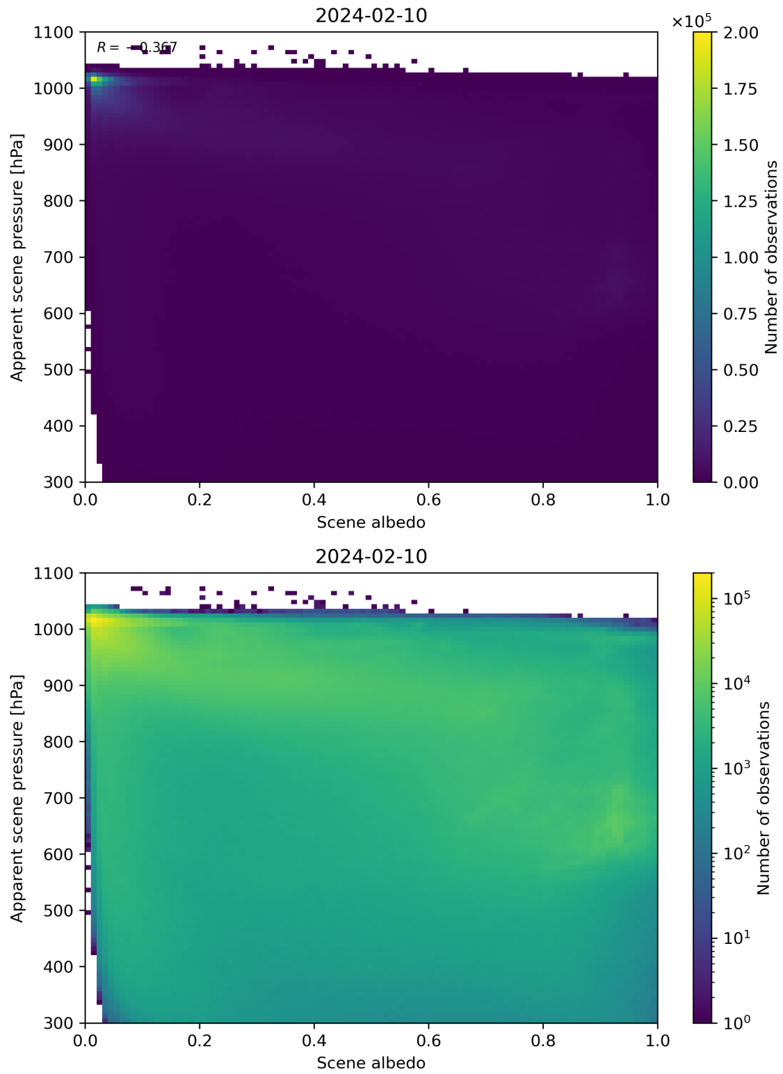
Figure 102: Scatter density plot of “Scene albedo” against “Apparent scene pressure” for 2024-02-09 to 2024-02-11.
