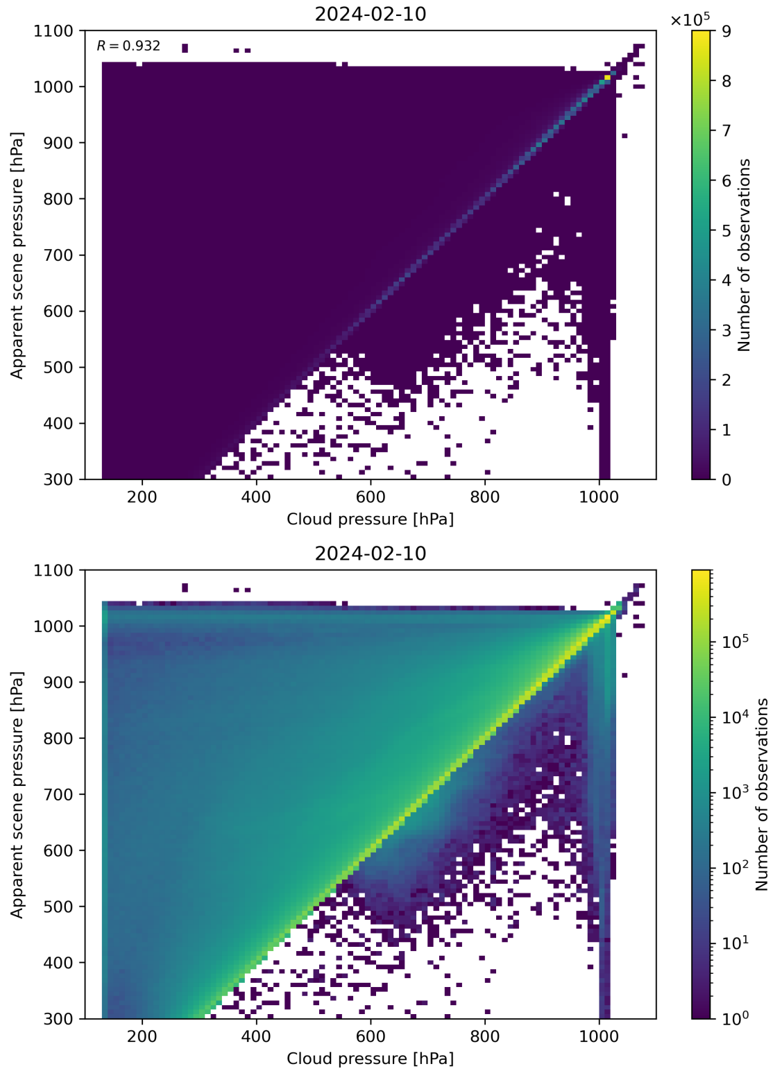
Figure 77: Scatter density plot of “Cloud pressure” against “Apparent scene pressure” for 2024-02-09 to 2024-02-11.
