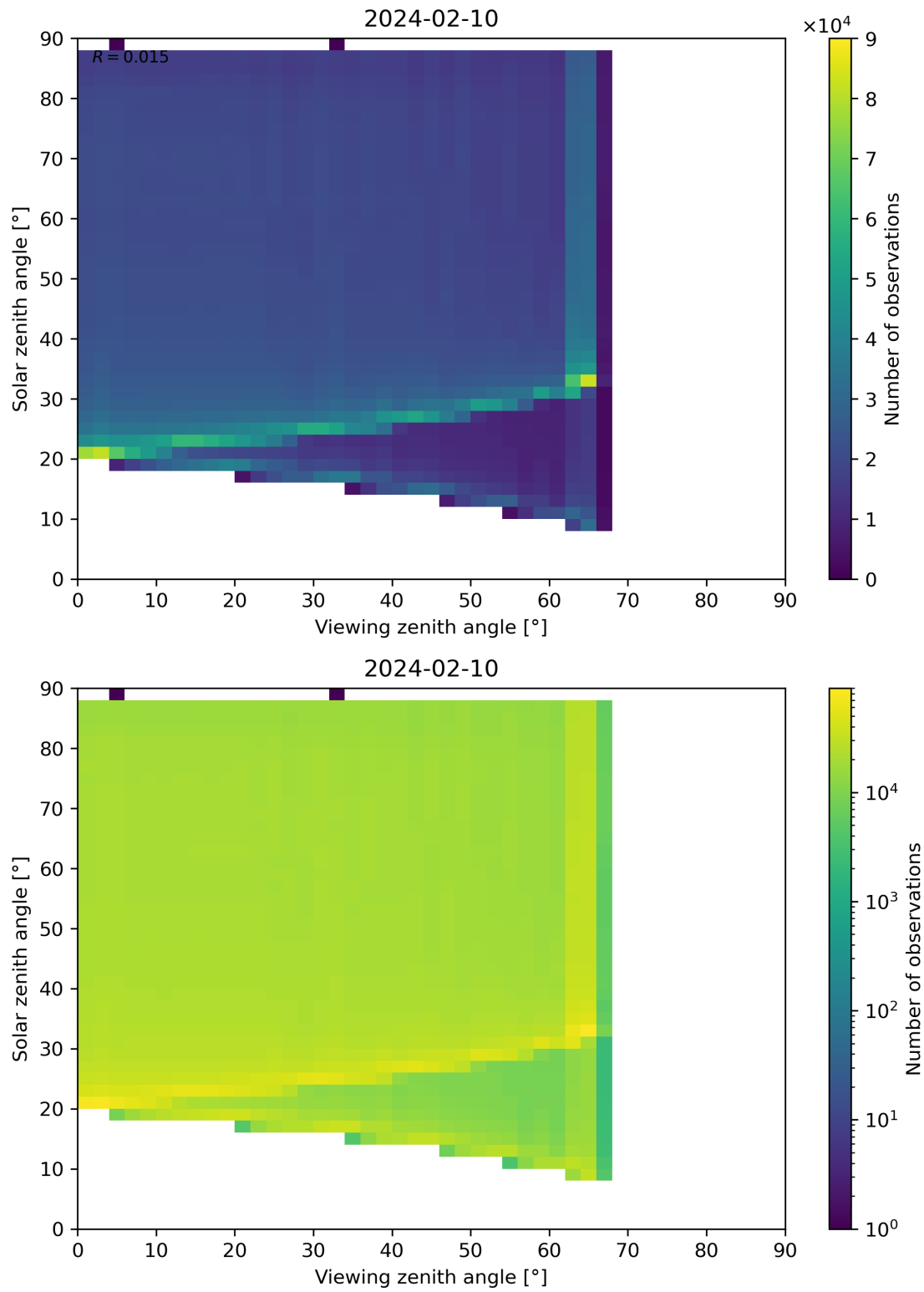
Figure 127: Scatter density plot of “Viewing zenith angle” against “Solar zenith angle” for 2024-02-09 to 2024-02-11.
