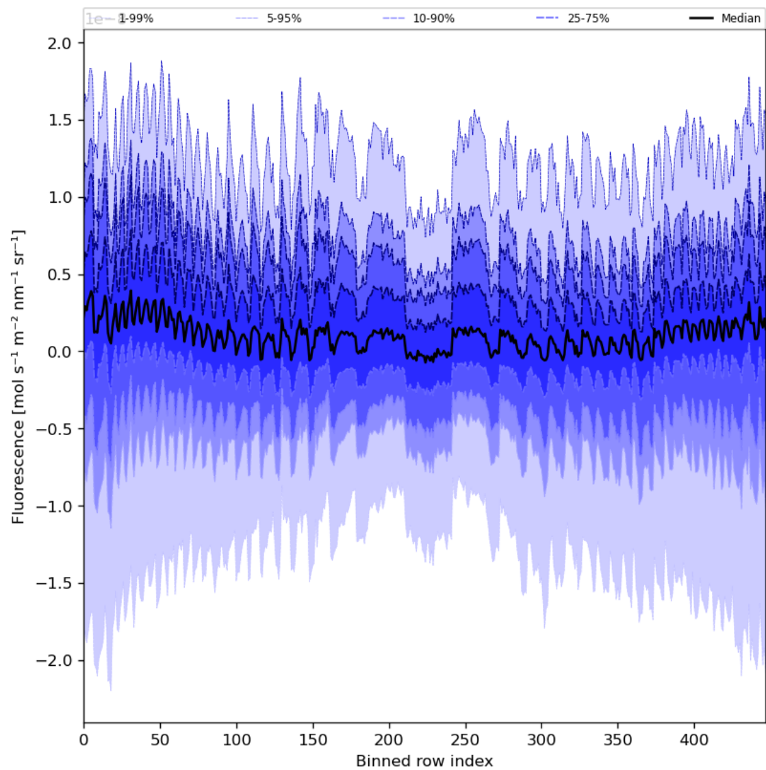
Figure 57: Along track statistics of “Fluorescence” for 2024-02-09 to 2024-02-11
