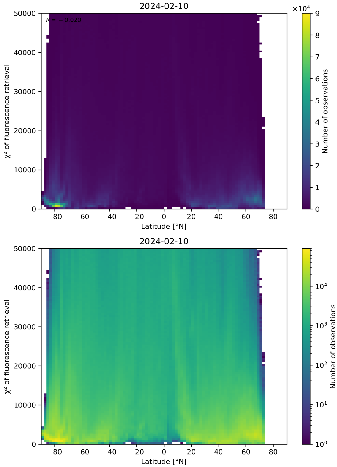
Figure 89: Scatter density plot of “Latitude” against “ \chi^2 of fluorescence retrieval” for 2024-02-09 to 2024-02-11.
