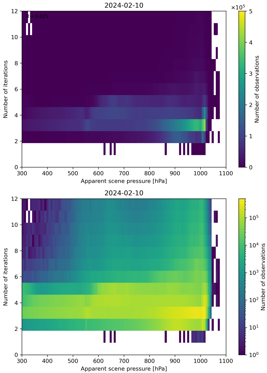
Figure 65: Scatter density plot of “Apparent scene pressure” against “Number of iterations” for 2024-02-09 to 2024-02-11.
