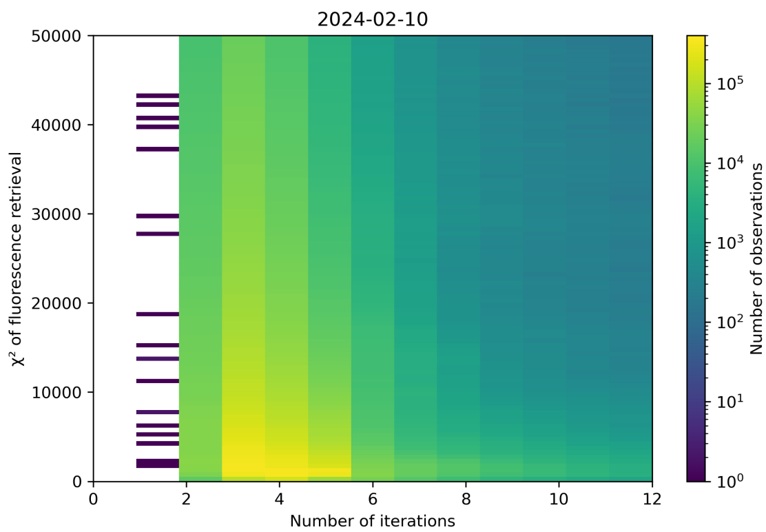
Figure 97: Scatter density plot of “Number of iterations” against “ \chi^2 of fluorescence retrieval” for 2024-02-09 to 2024-02-11.
