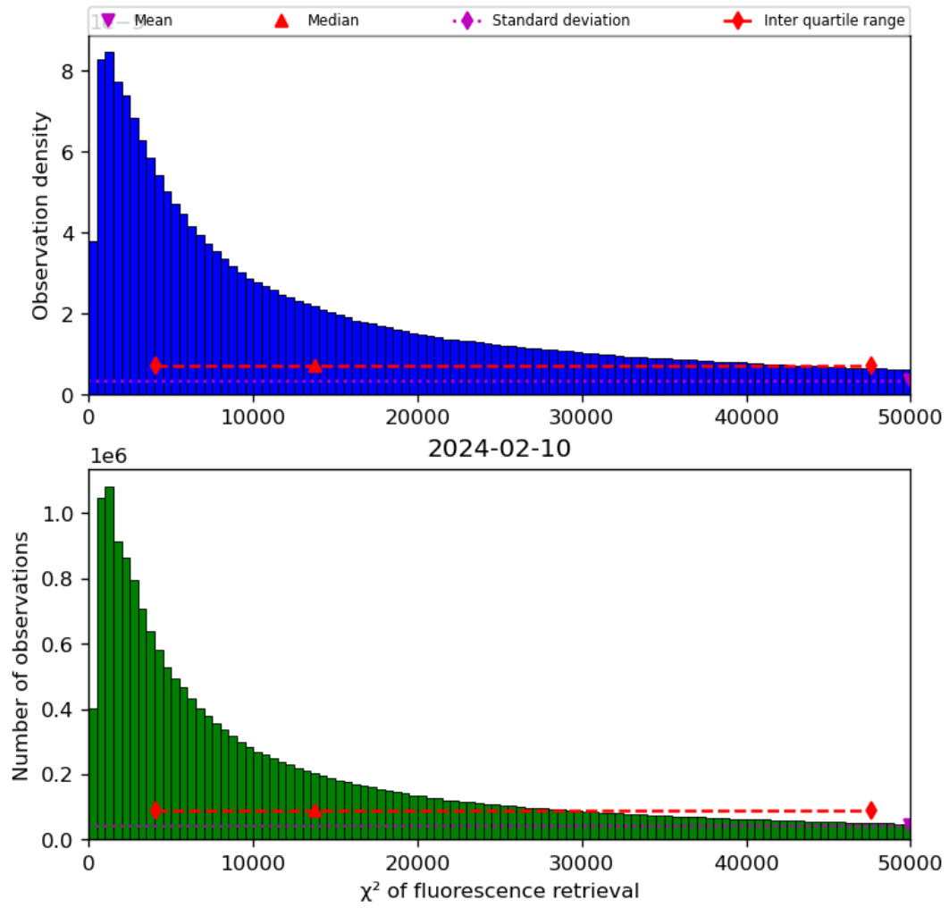
Figure 42: Histogram of “ \chi^2 of fluorescence retrieval” for 2024-02-09 to 2024-02-11
