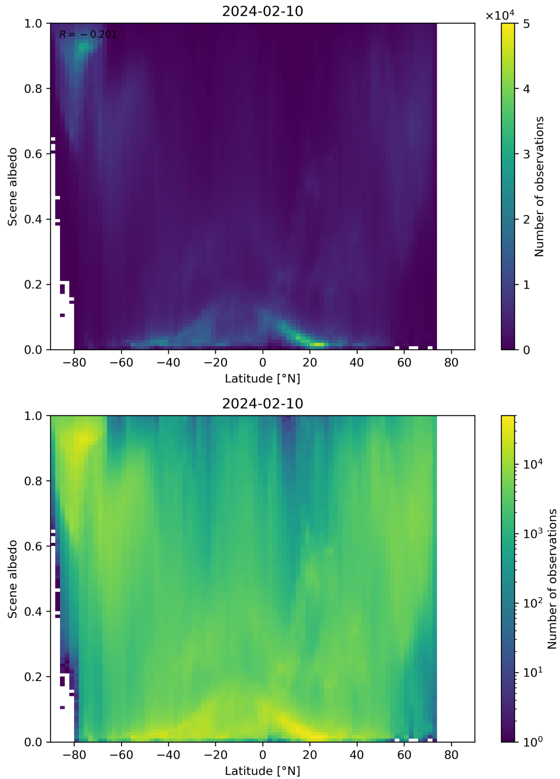
Figure 95: Scatter density plot of “Latitude” against “Scene albedo” for 2024-02-09 to 2024-02-11.
