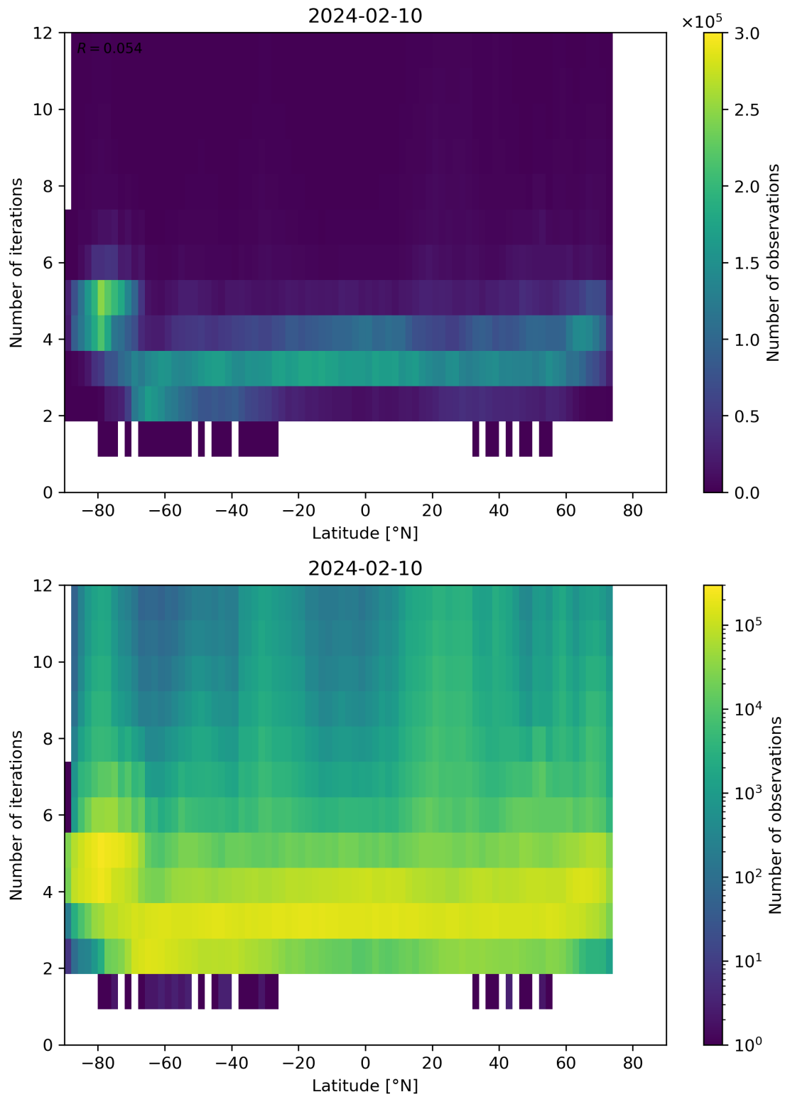
Figure 93: Scatter density plot of “Latitude” against “Number of iterations” for 2024-02-09 to 2024-02-11.
