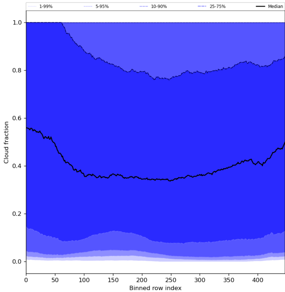
Figure 49: Along track statistics of “Cloud fraction” for 2024-02-09 to 2024-02-11
