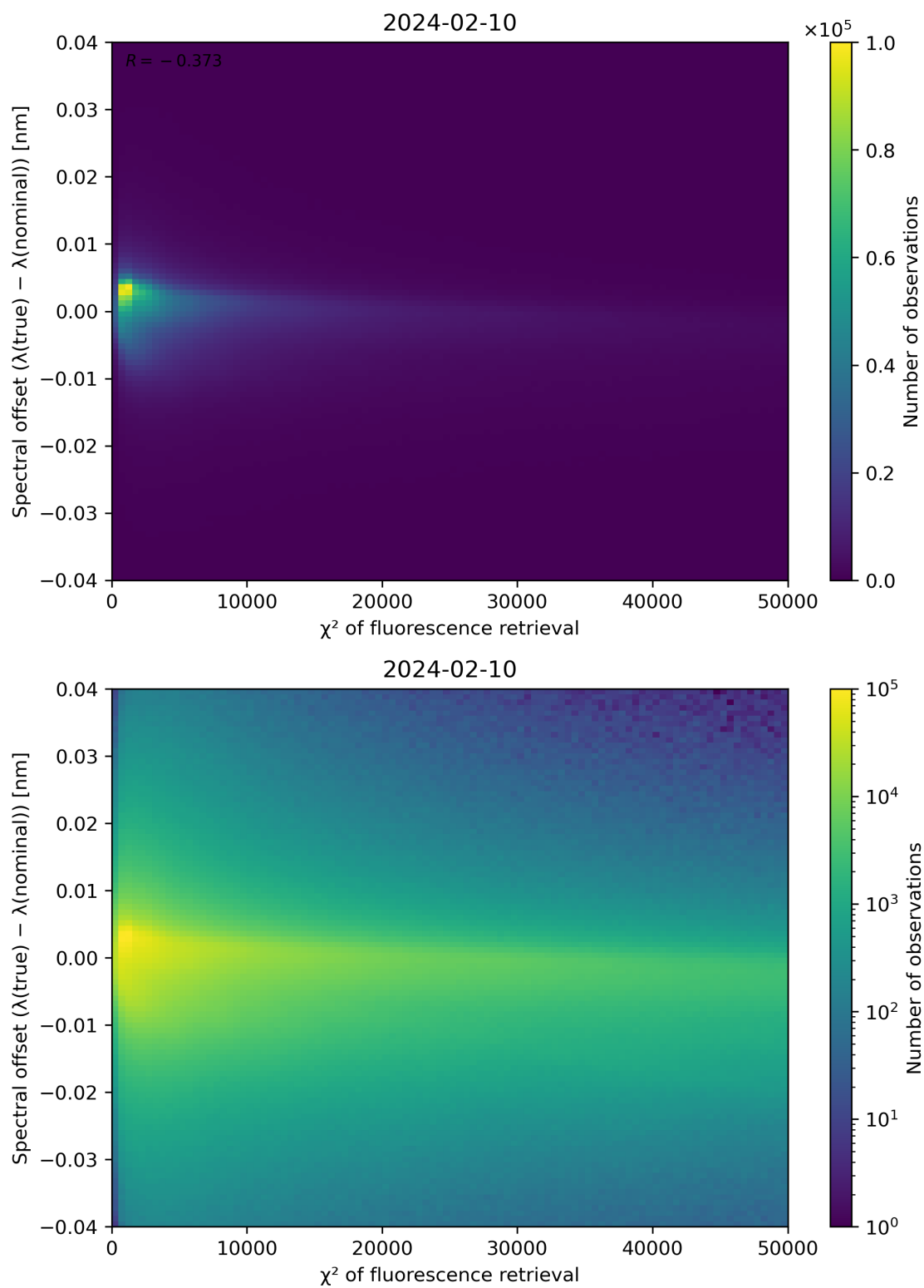
Figure 69: Scatter density plot of " \chi^2 of fluorescence retrieval" against "Spectral offset ( \lambda(\text{true}) - \lambda(\text{nominal}) )" for 2024-02-09 to 2024-02-11.
