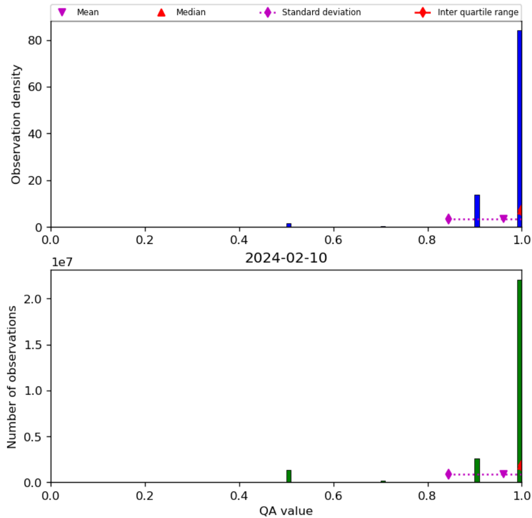
Figure 29: Histogram of “QA value” for 2024-02-09 to 2024-02-11
