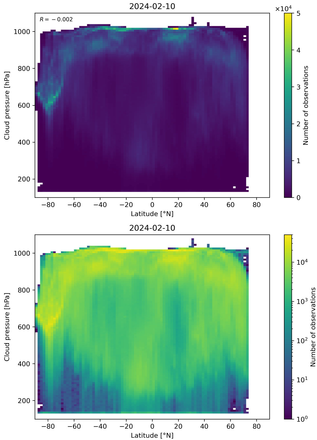
Figure 91: Scatter density plot of “Latitude” against “Cloud pressure” for 2024-02-09 to 2024-02-11.
