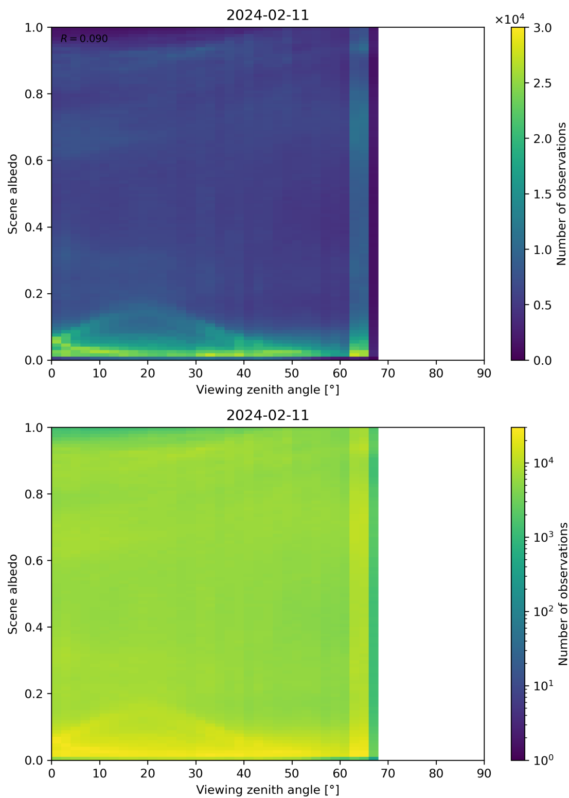
Figure 126: Scatter density plot of “Viewing zenith angle” against “Scene albedo” for 2024-02-11 to 2024-02-12.
