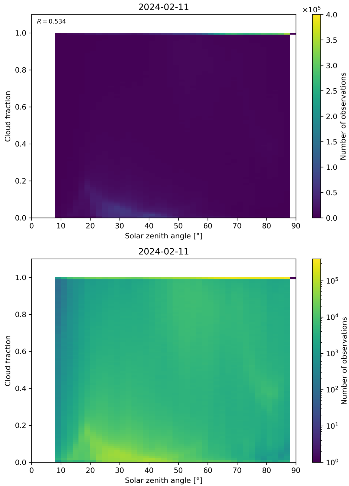
Figure 110: Scatter density plot of “Solar zenith angle” against “Cloud fraction” for 2024-02-11 to 2024-02-12.
