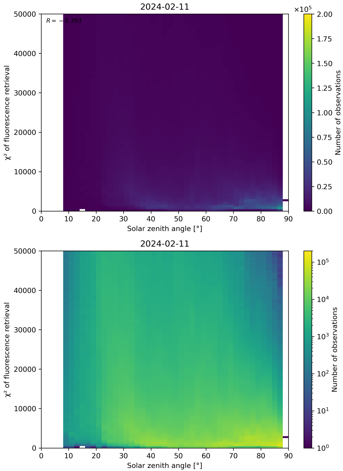
Figure 109: Scatter density plot of “Solar zenith angle” against “ \chi^2 of fluorescence retrieval” for 2024-02-11 to 2024-02-12.
