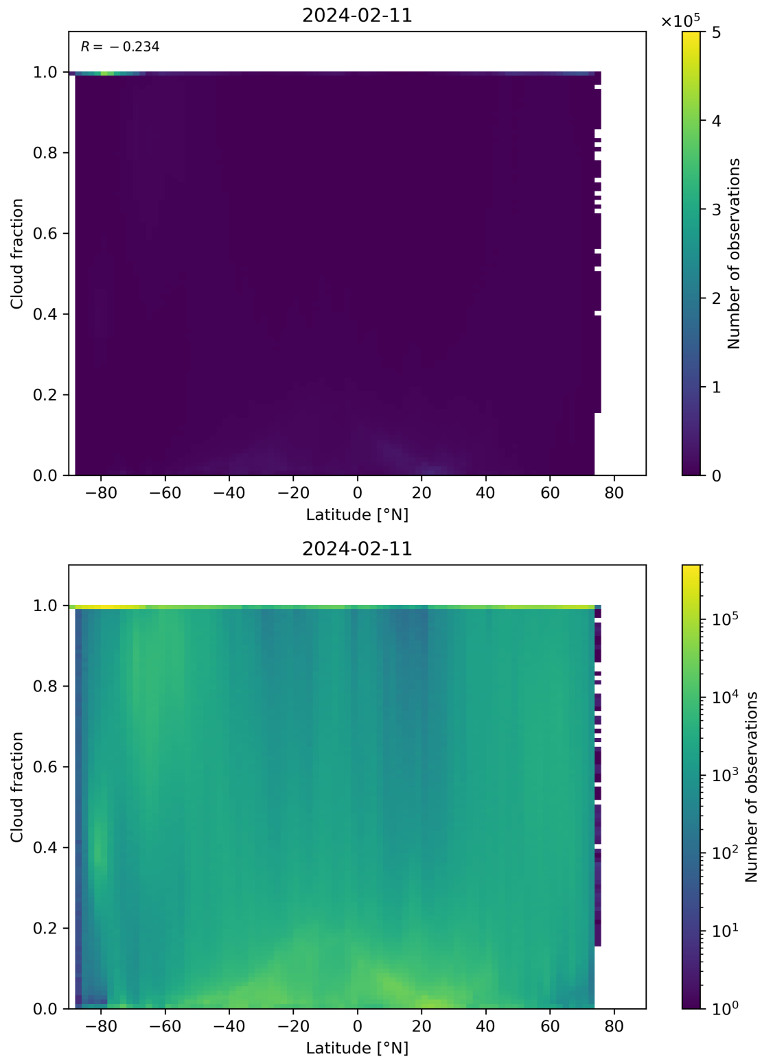
Figure 90: Scatter density plot of “Latitude” against “Cloud fraction” for 2024-02-11 to 2024-02-12.
