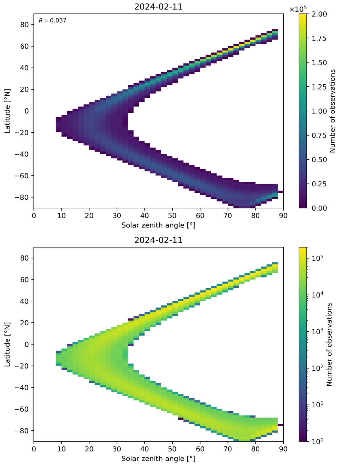
Figure 113: Scatter density plot of “Solar zenith angle” against “Latitude” for 2024-02-11 to 2024-02-12.
