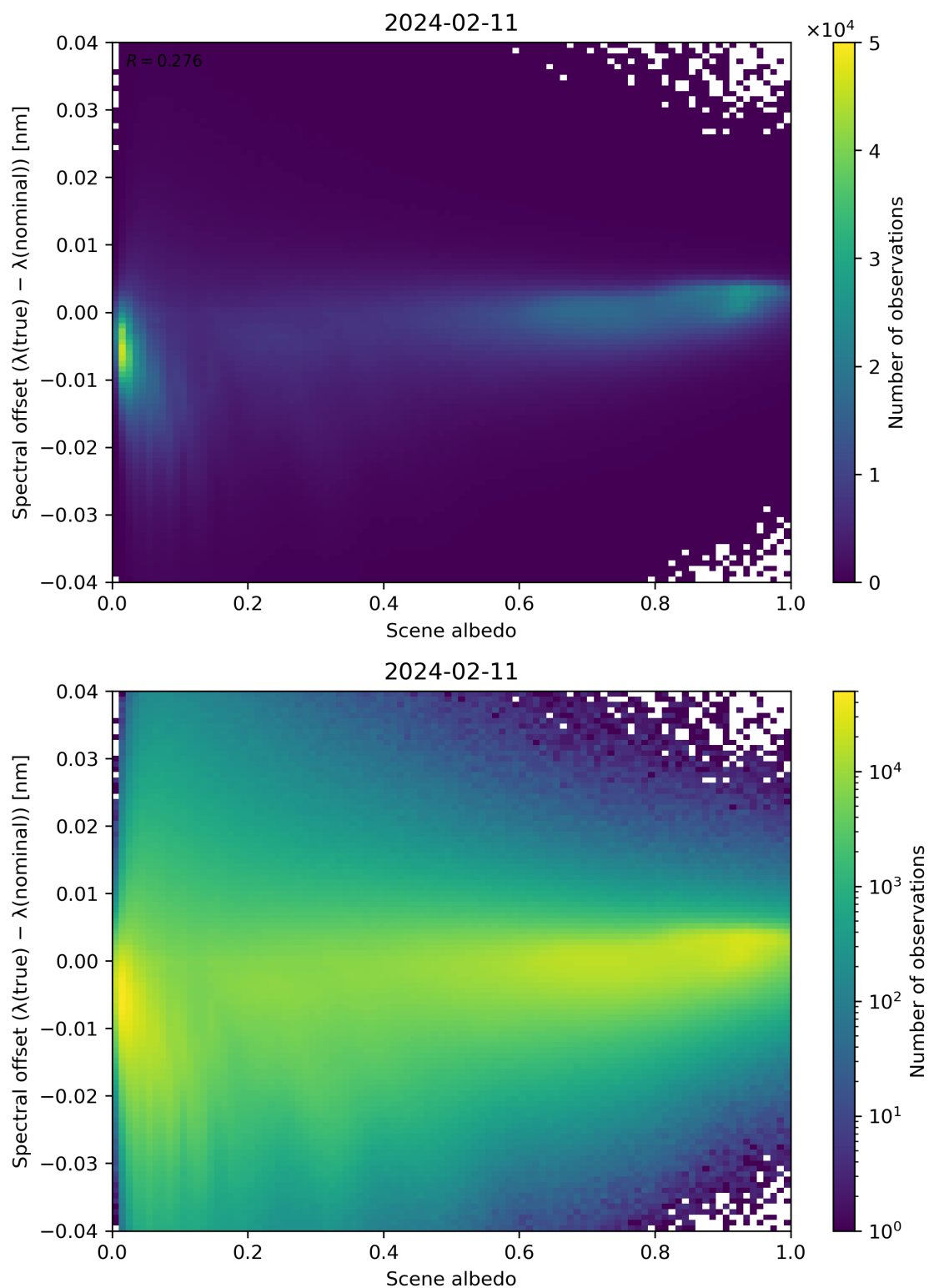
Figure 107: Scatter density plot of “Scene albedo” against “Spectral offset ( \lambda(\text{true}) - \lambda(\text{nominal}) )” for 2024-02-11 to 2024-02-12.
