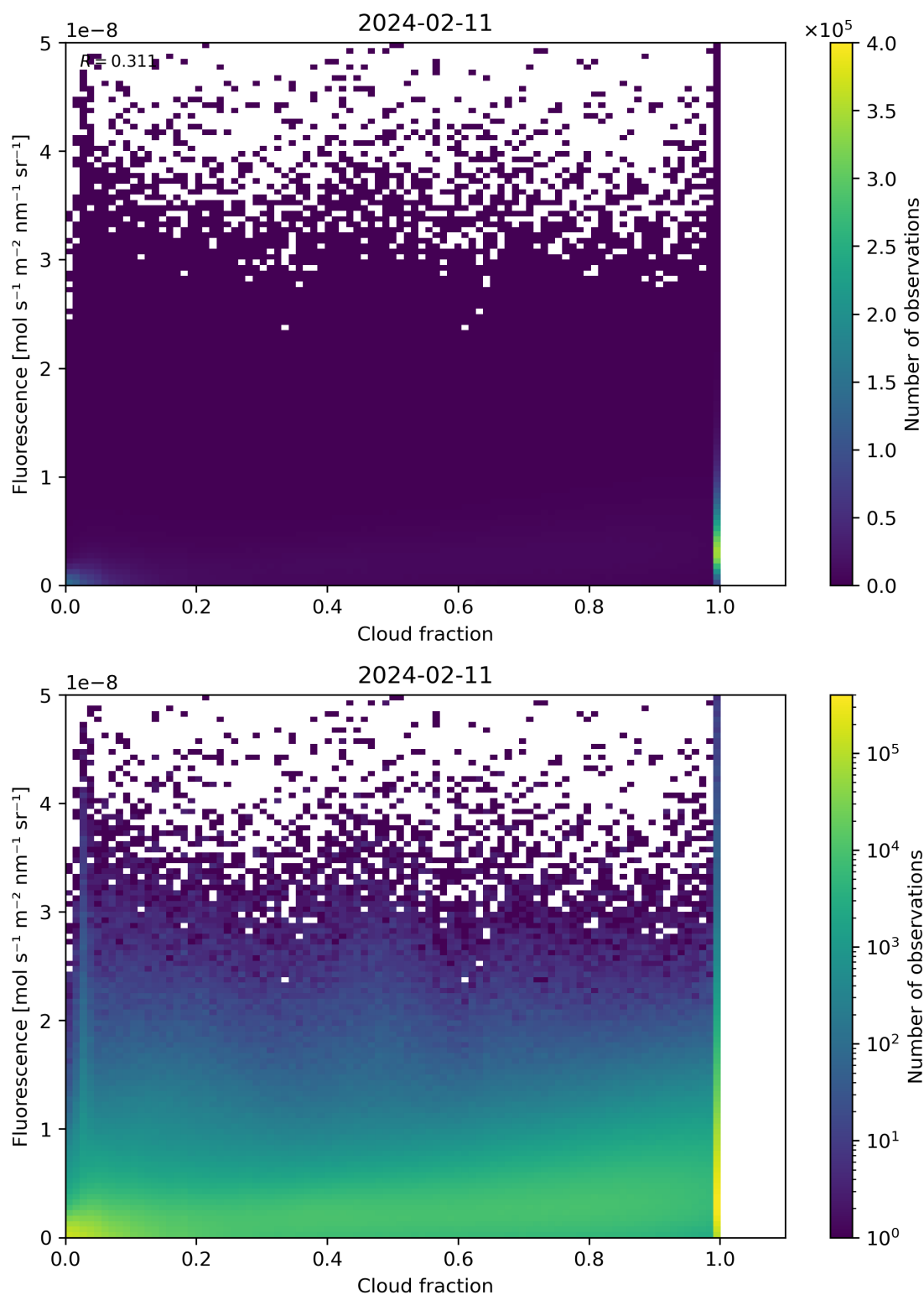
Figure 72: Scatter density plot of “Cloud fraction” against “Fluorescence” for 2024-02-11 to 2024-02-12.
