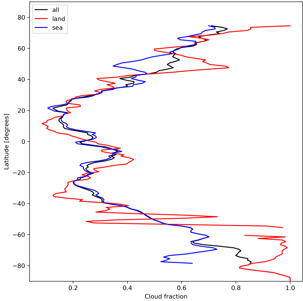
Figure 15: Zonal average of “Cloud fraction” for 2024-02-11 to 2024-02-12.
