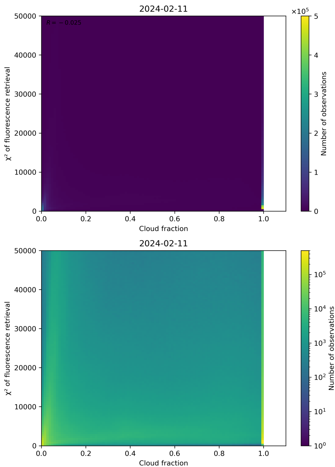
Figure 71: Scatter density plot of “Cloud fraction” against “ \chi^2 of fluorescence retrieval” for 2024-02-11 to 2024-02-12.
