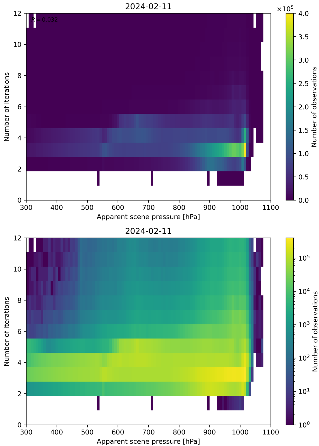
Figure 65: Scatter density plot of “Apparent scene pressure” against “Number of iterations” for 2024-02-11 to 2024-02-12.
