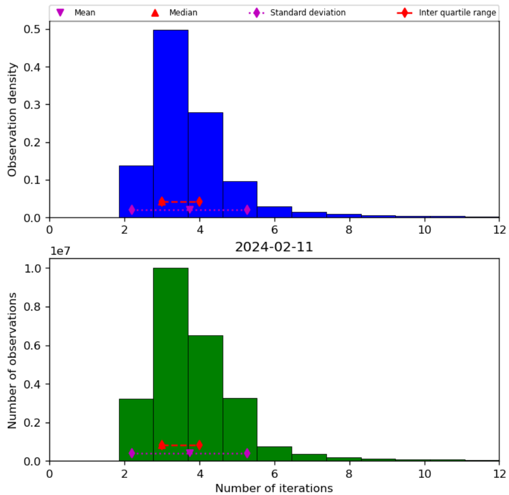
Figure 39: Histogram of “Number of iterations” for 2024-02-11 to 2024-02-12
