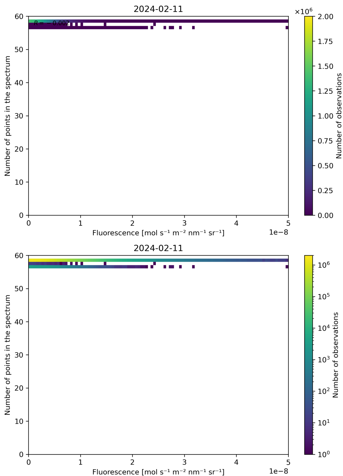
Figure 86: Scatter density plot of “Fluorescence” against “Number of points in the spectrum” for 2024-02-11 to 2024-02-12.
