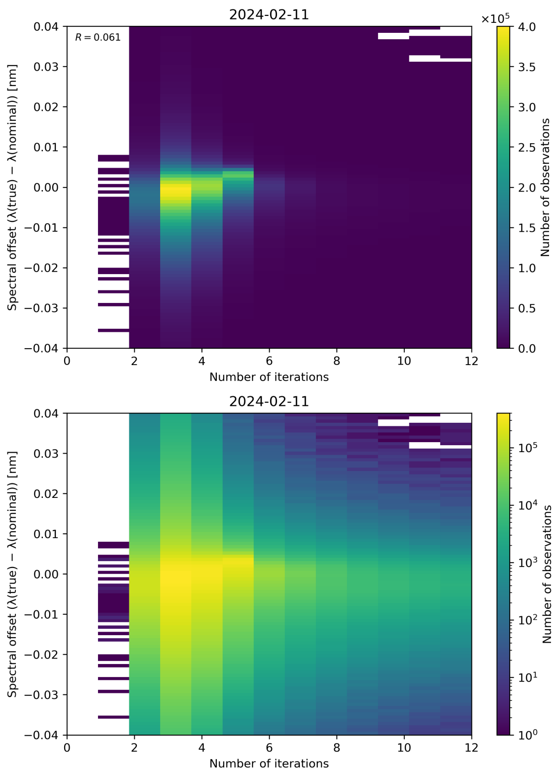
Figure 100: Scatter density plot of “Number of iterations” against “Spectral offset ( \lambda(\text{true}) - \lambda(\text{nominal}) )” for 2024-02-11 to 2024-02-12.
