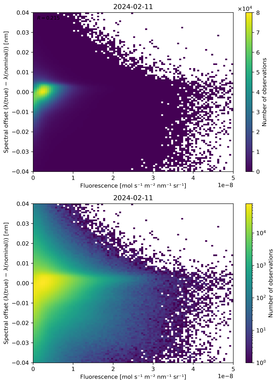
Figure 87: Scatter density plot of “Fluorescence” against “Spectral offset ( \lambda(\text{true}) - \lambda(\text{nominal}) )” for 2024-02-11 to 2024-02-12.
