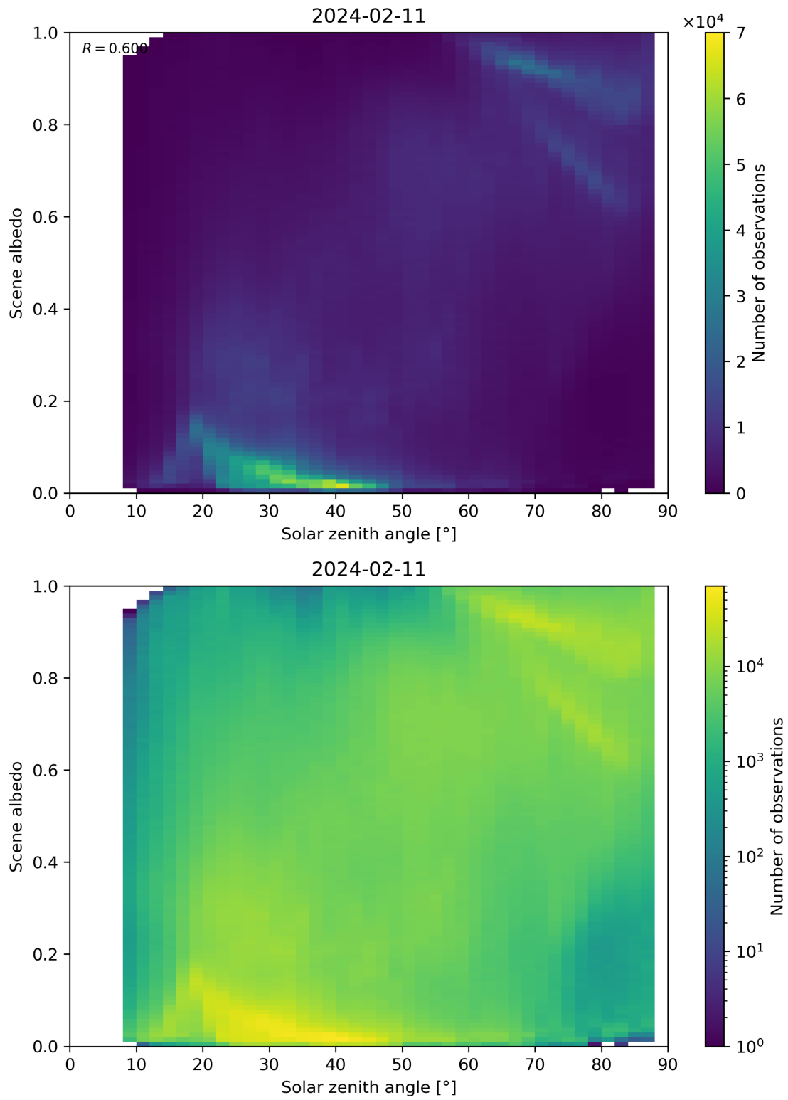
Figure 116: Scatter density plot of “Solar zenith angle” against “Scene albedo” for 2024-02-11 to 2024-02-12.
