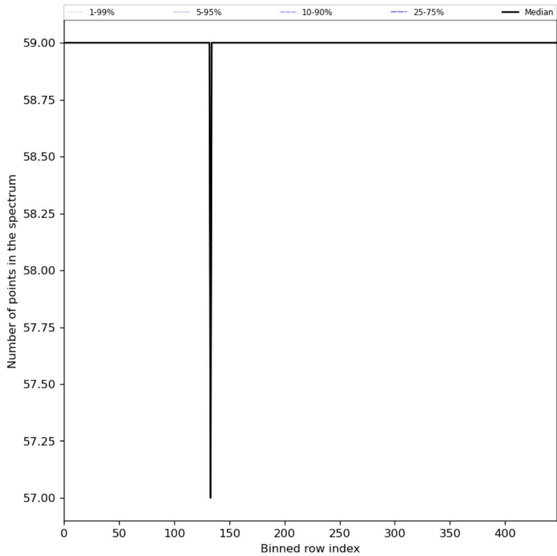
Figure 61: Along track statistics of “Number of points in the spectrum” for 2024-02-11 to 2024-02-12
