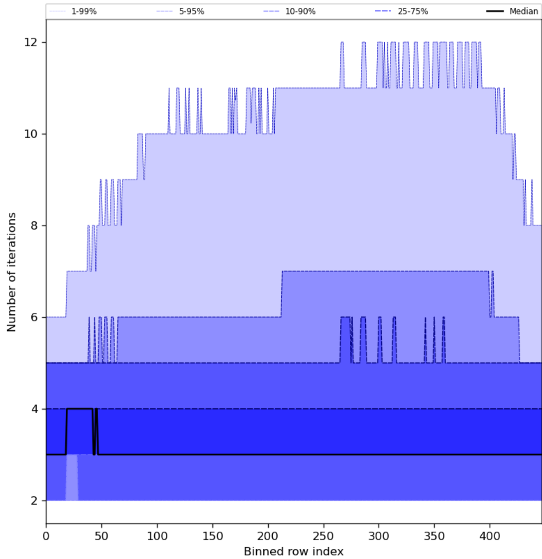
Figure 56: Along track statistics of “Number of iterations” for 2024-02-11 to 2024-02-12
