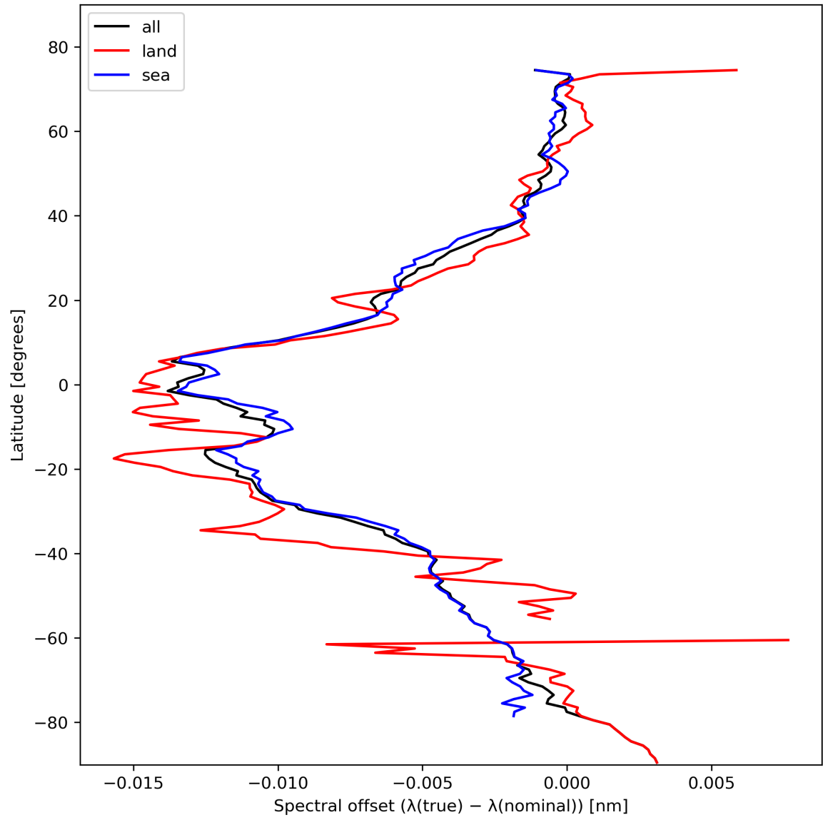
Figure 28: Zonal average of “Spectral offset ( \lambda(\text{true}) - \lambda(\text{nominal}) )” for 2024-02-11 to 2024-02-12.
