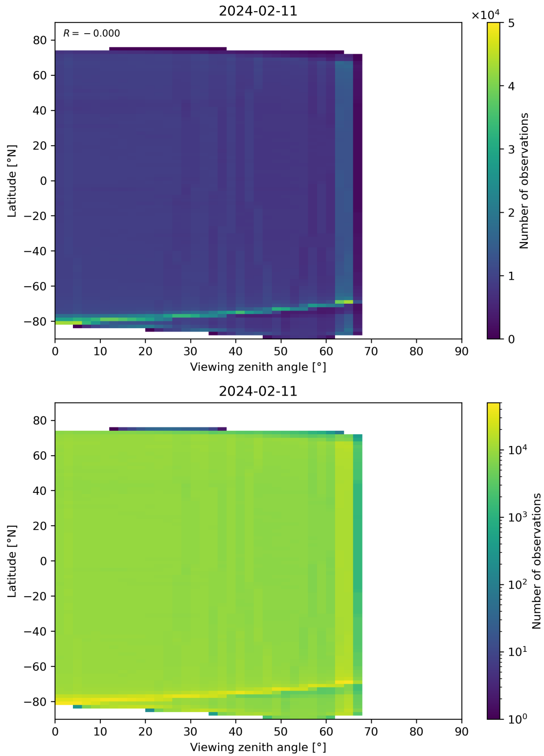
Figure 123: Scatter density plot of “Viewing zenith angle” against “Latitude” for 2024-02-11 to 2024-02-12.
