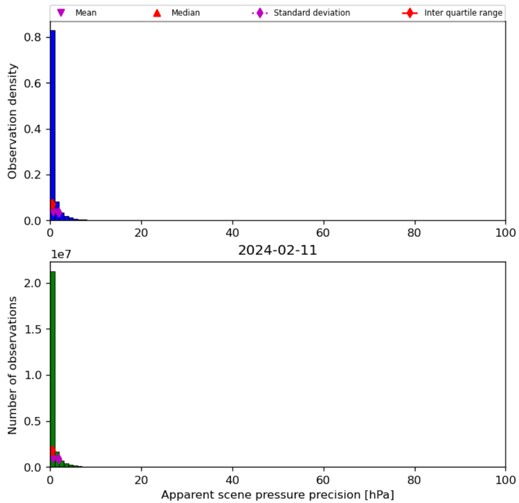
Figure 37: Histogram of “Apparent scene pressure precision” for 2024-02-11 to 2024-02-12
