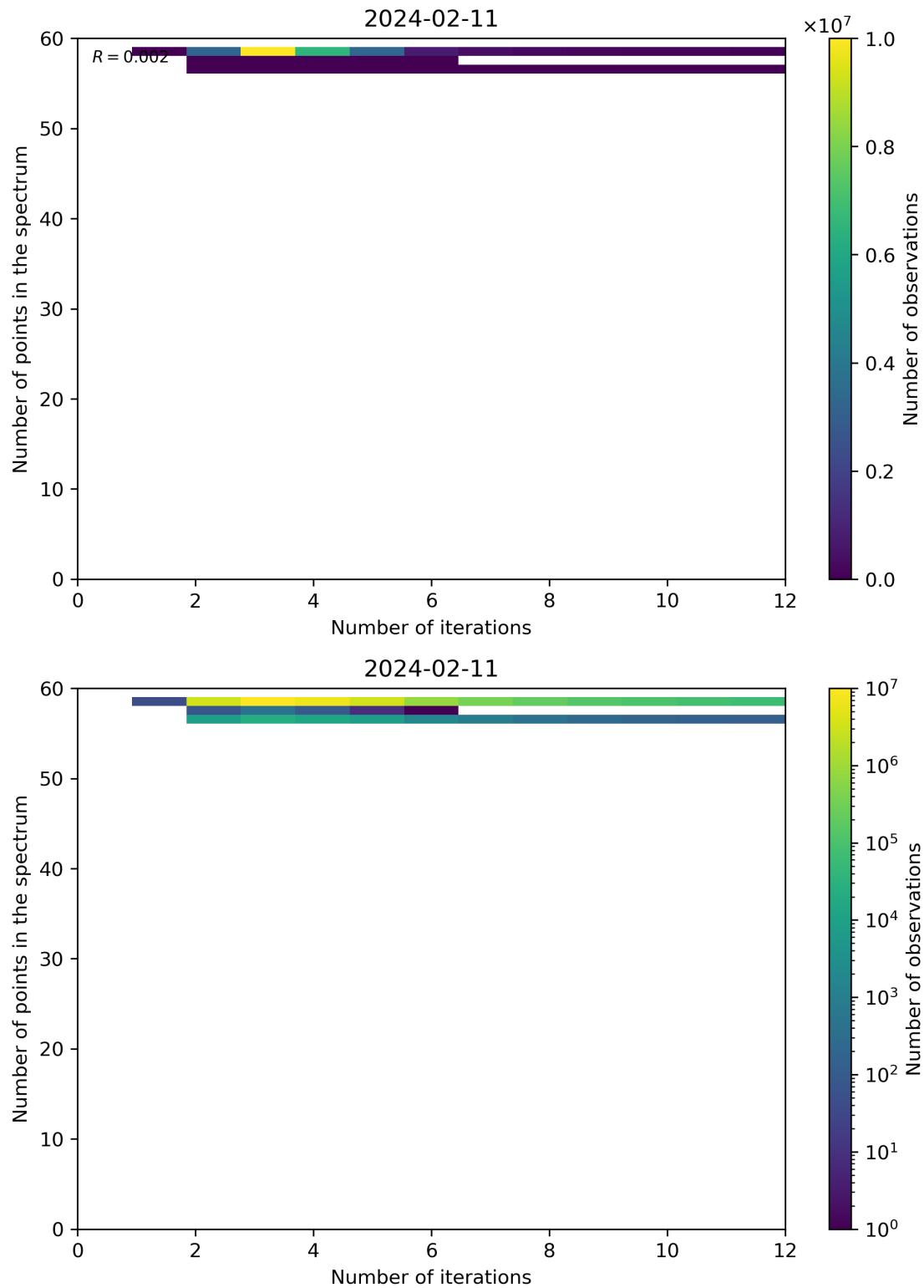
Figure 99: Scatter density plot of “Number of iterations” against “Number of points in the spectrum” for 2024-02-11 to 2024-02-12.
