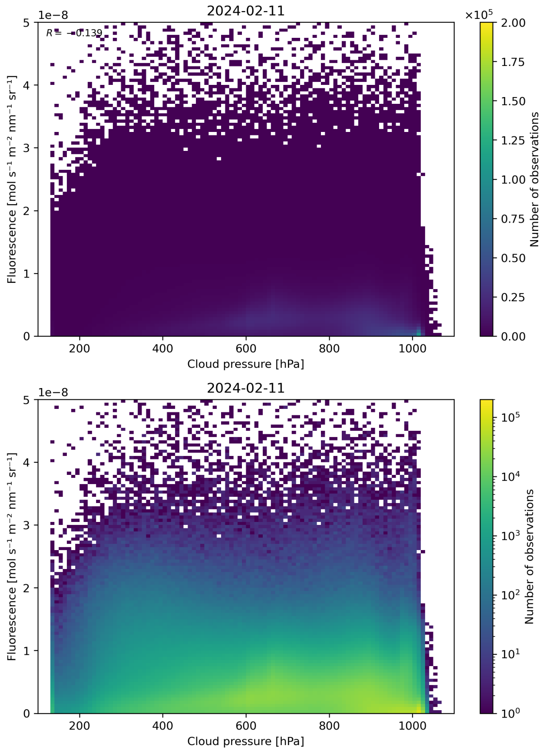
Figure 80: Scatter density plot of “Cloud pressure” against “Fluorescence” for 2024-02-11 to 2024-02-12.
