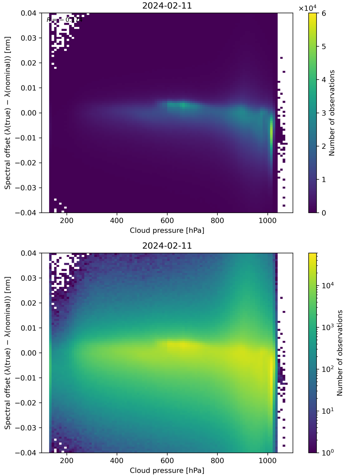
Figure 84: Scatter density plot of “Cloud pressure” against “Spectral offset ( \lambda(\text{true}) - \lambda(\text{nominal}) )” for 2024-02-11 to 2024-02-12.
