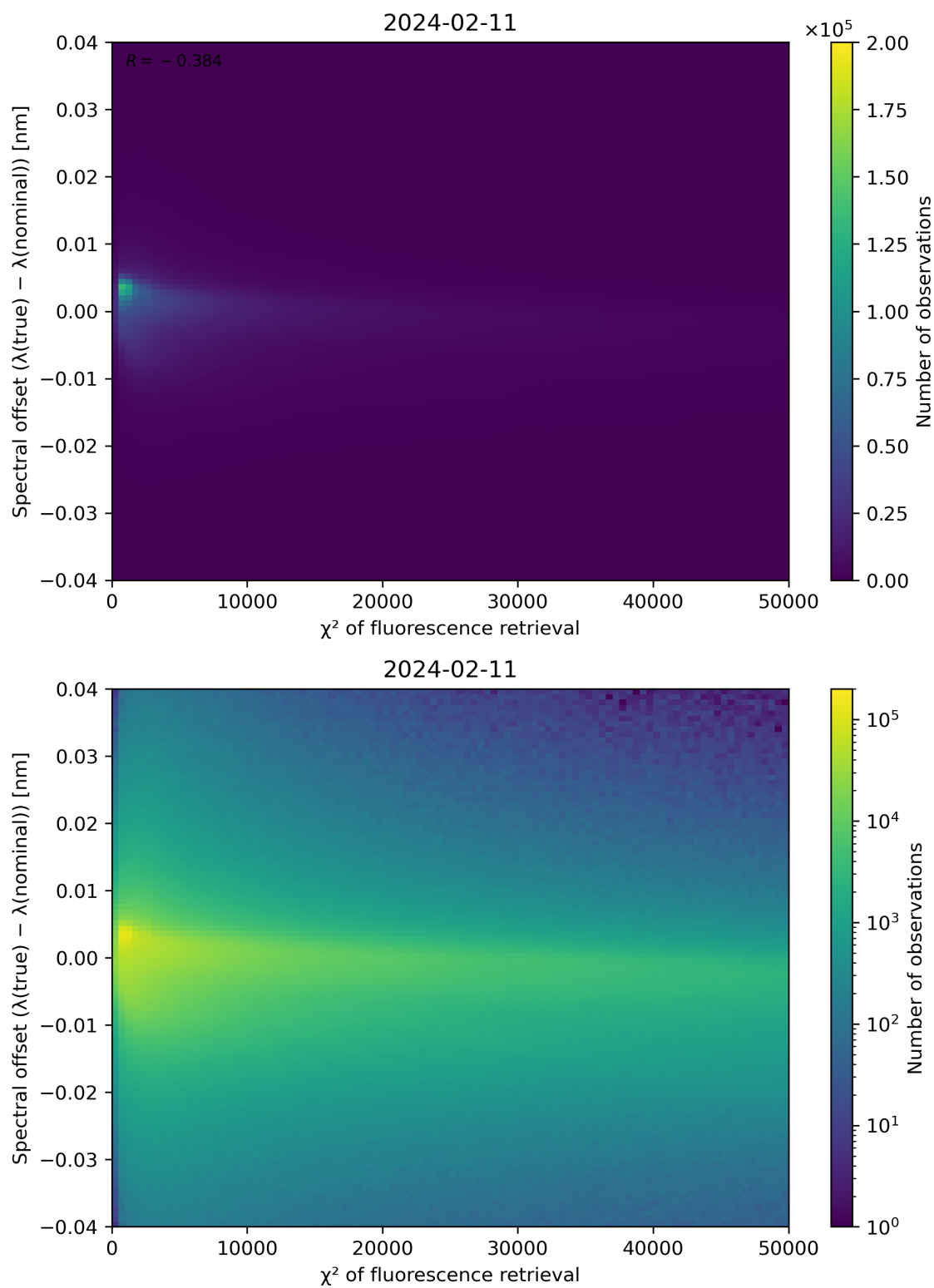
Figure 69: Scatter density plot of " \chi^2 of fluorescence retrieval" against "Spectral offset ( \lambda(\text{true}) - \lambda(\text{nominal}) )" for 2024-02-11 to 2024-02-12.
