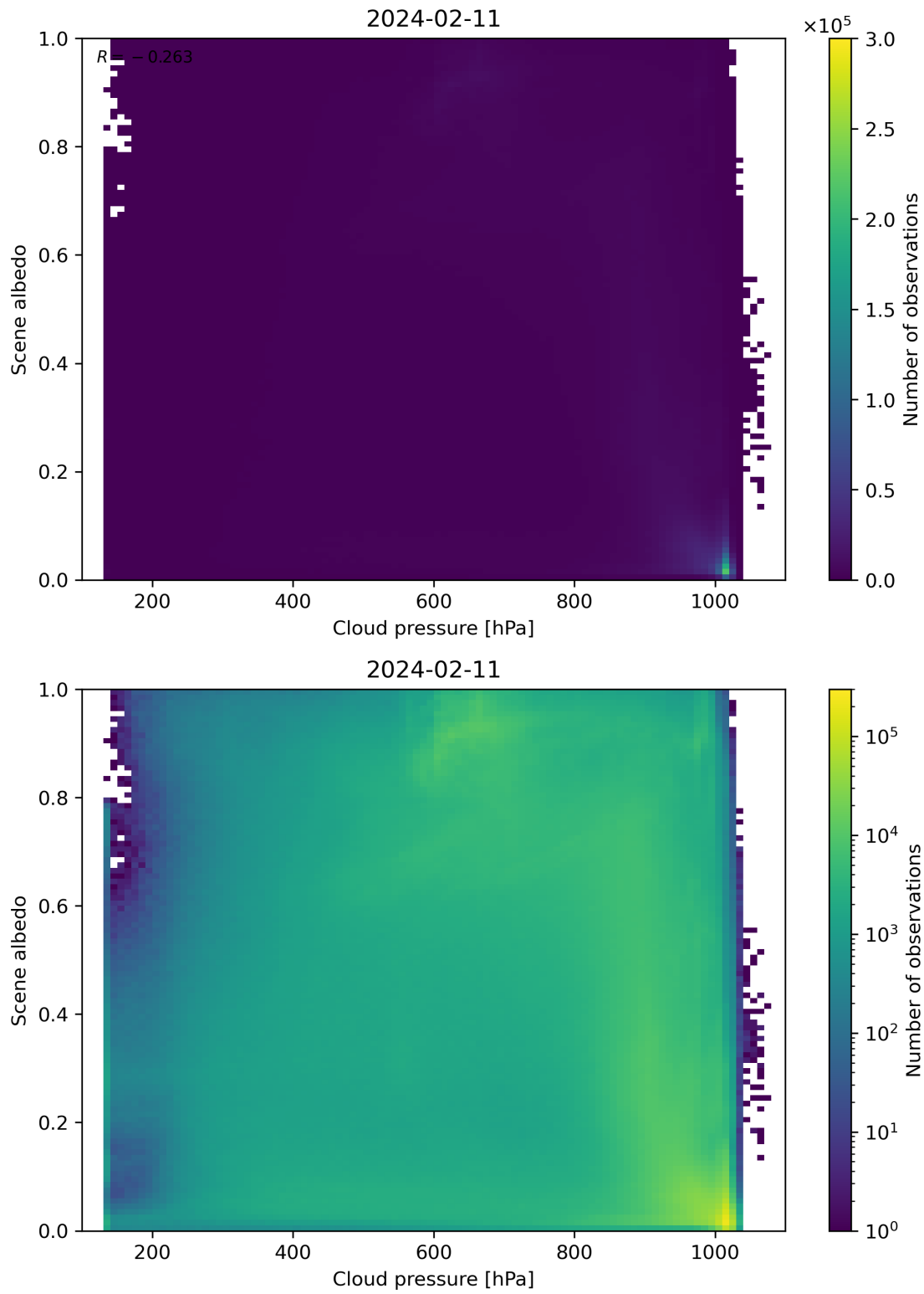
Figure 83: Scatter density plot of “Cloud pressure” against “Scene albedo” for 2024-02-11 to 2024-02-12.
