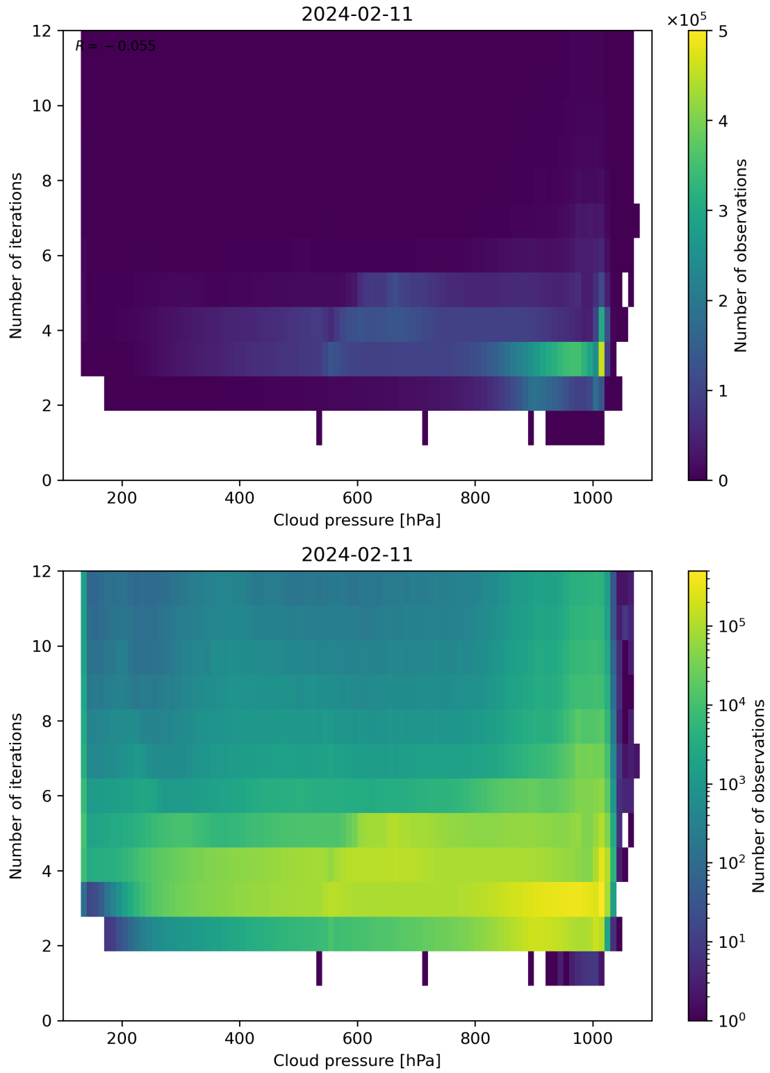
Figure 81: Scatter density plot of “Cloud pressure” against “Number of iterations” for 2024-02-11 to 2024-02-12.
