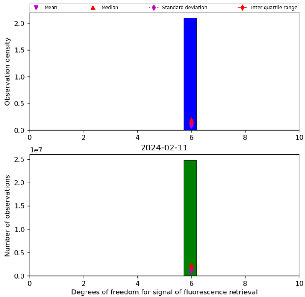
Figure 43: Histogram of “Degrees of freedom for signal of fluorescence retrieval” for 2024-02-11 to 2024-02-12
