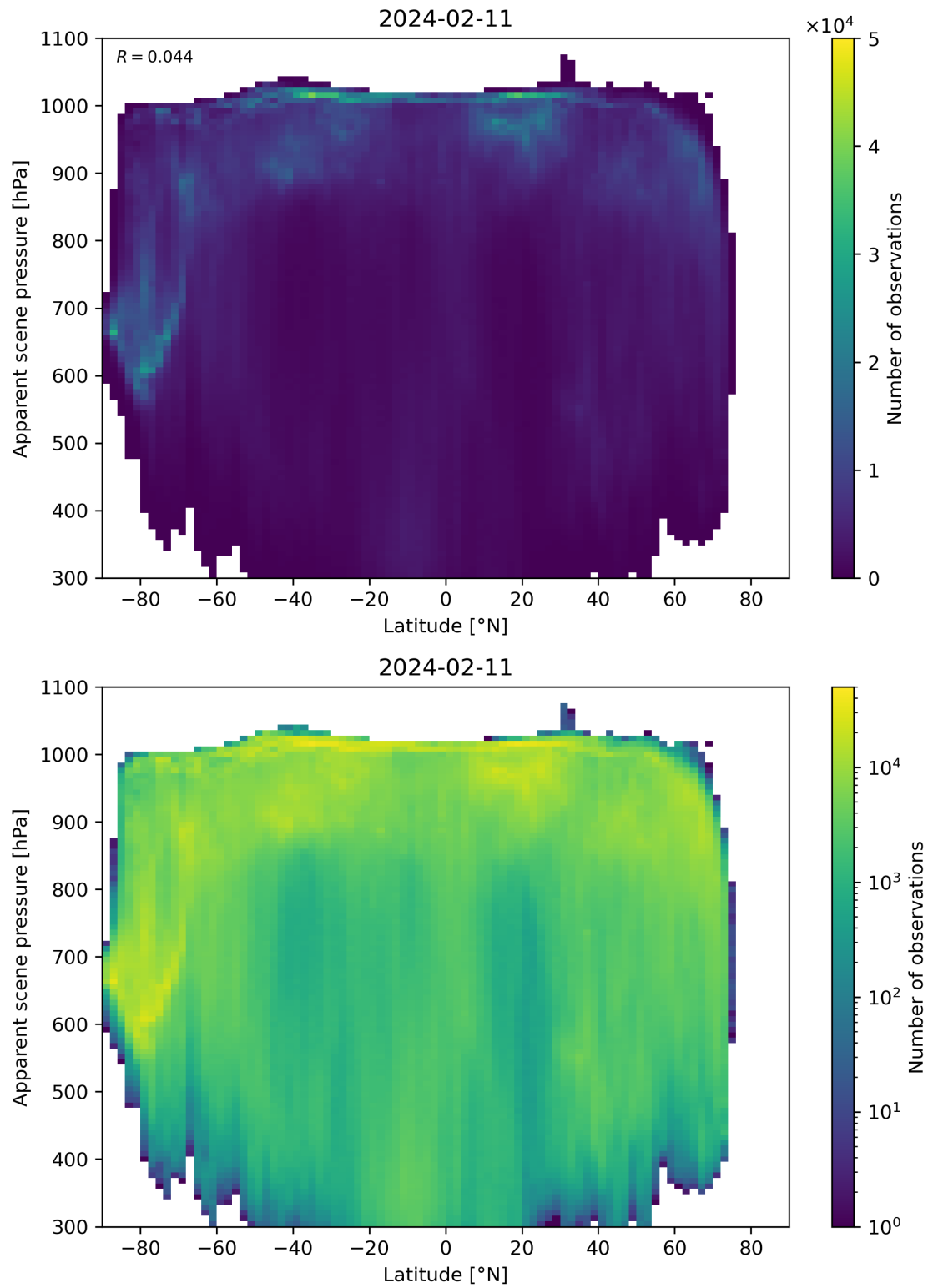
Figure 88: Scatter density plot of “Latitude” against “Apparent scene pressure” for 2024-02-11 to 2024-02-12.
