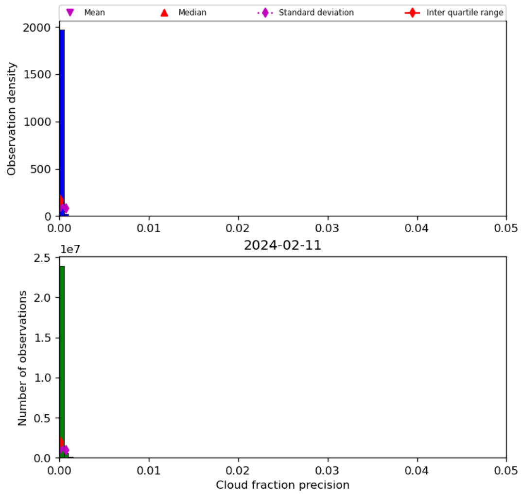
Figure 33: Histogram of “Cloud fraction precision” for 2024-02-11 to 2024-02-12
