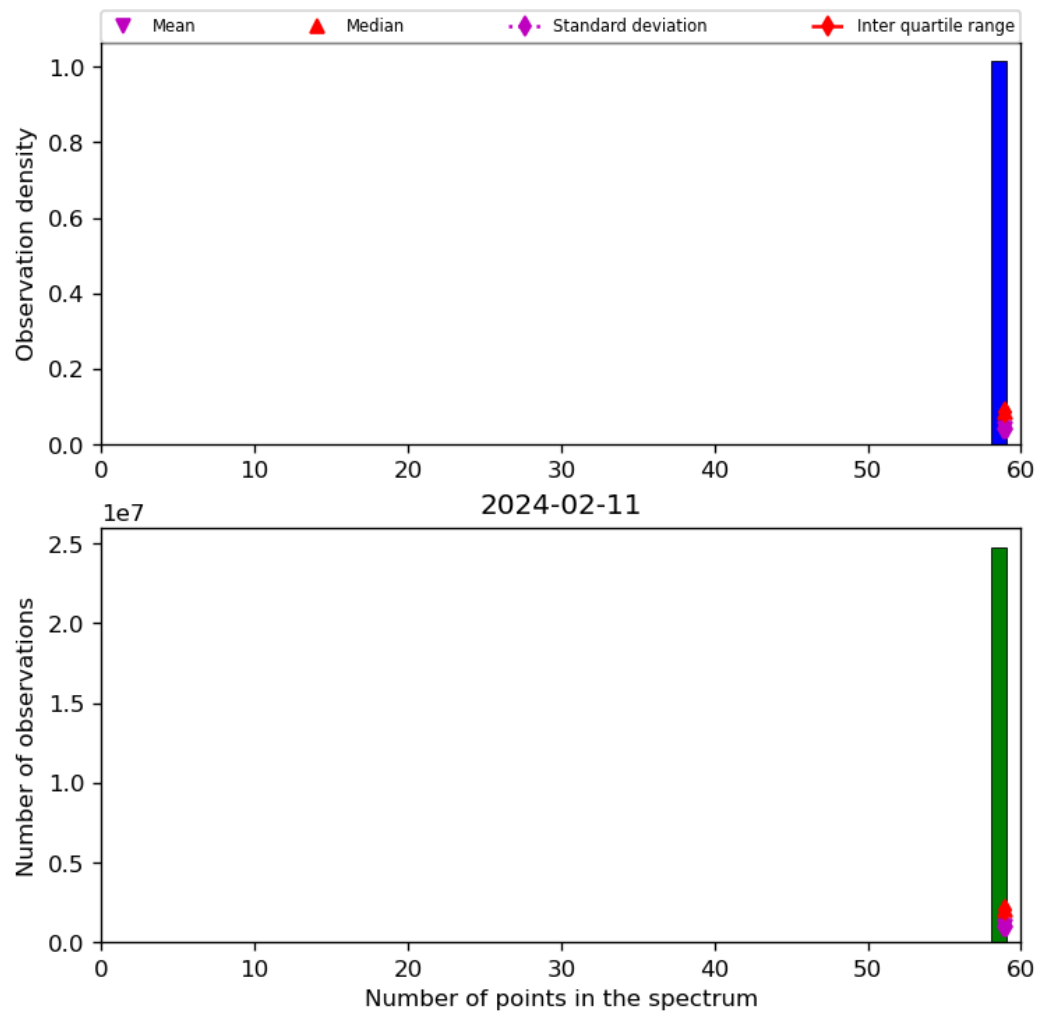
Figure 44: Histogram of “Number of points in the spectrum” for 2024-02-11 to 2024-02-12
