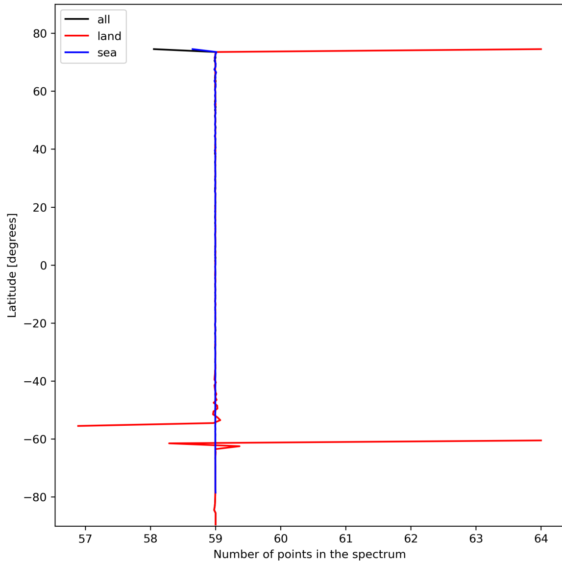
Figure 27: Zonal average of “Number of points in the spectrum” for 2024-02-11 to 2024-02-12.
