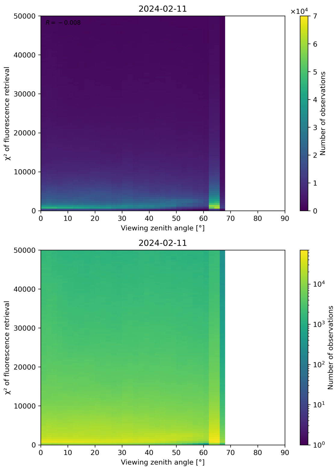
Figure 119: Scatter density plot of “Viewing zenith angle” against “ \chi^2 of fluorescence retrieval” for 2024-02-11 to 2024-02-12.
