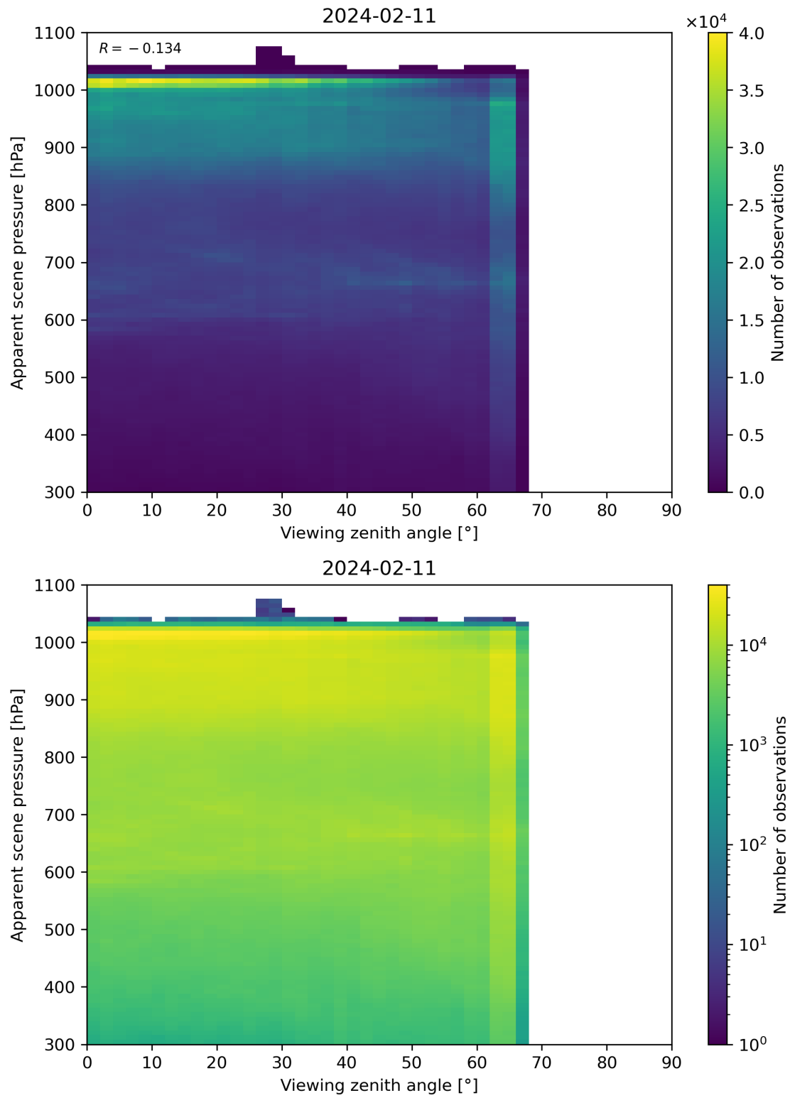
Figure 118: Scatter density plot of “Viewing zenith angle” against “Apparent scene pressure” for 2024-02-11 to 2024-02-12.
