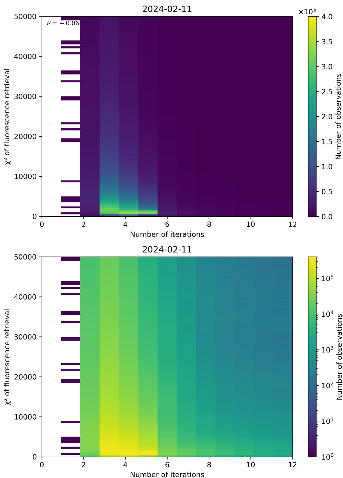
Figure 97: Scatter density plot of “Number of iterations” against “ \chi^2 of fluorescence retrieval” for 2024-02-11 to 2024-02-12.
