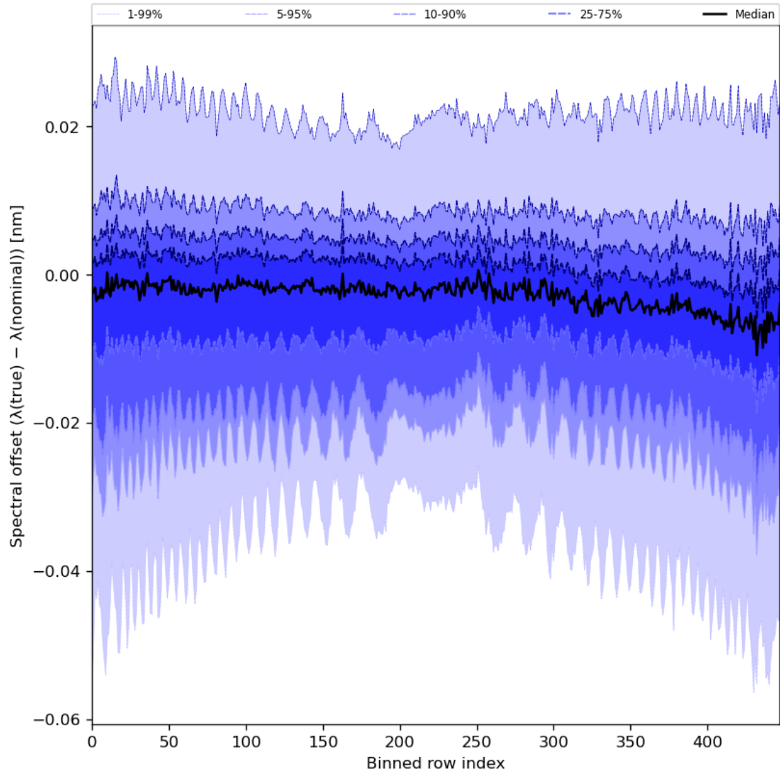
Figure 62: Along track statistics of “Spectral offset ( \lambda(\text{true}) - \lambda(\text{nominal}) )” for 2024-02-11 to 2024-02-12
