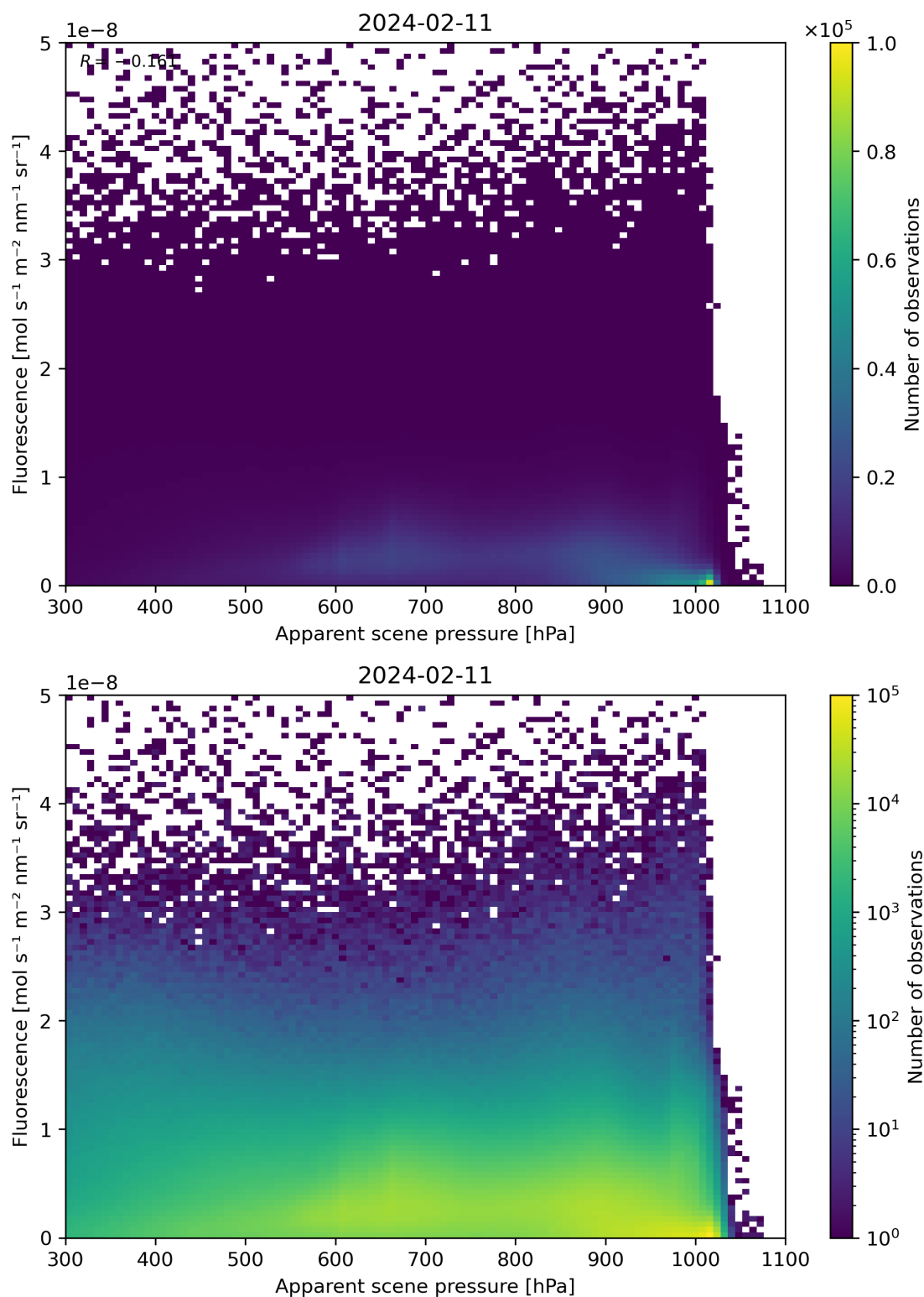
Figure 64: Scatter density plot of “Apparent scene pressure” against “Fluorescence” for 2024-02-11 to 2024-02-12.
