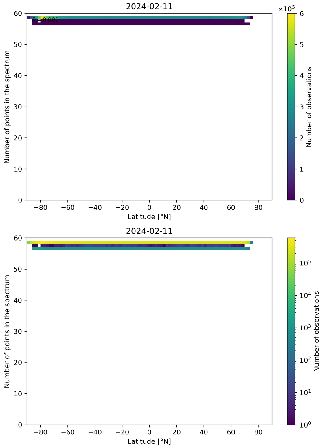
Figure 94: Scatter density plot of “Latitude” against “Number of points in the spectrum” for 2024-02-11 to 2024-02-12.
