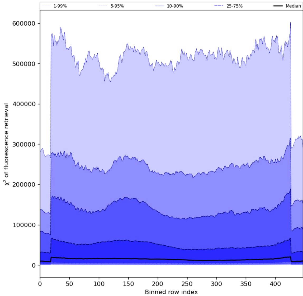
Figure 59: Along track statistics of “ \chi^2 of fluorescence retrieval” for 2024-02-11 to 2024-02-12
