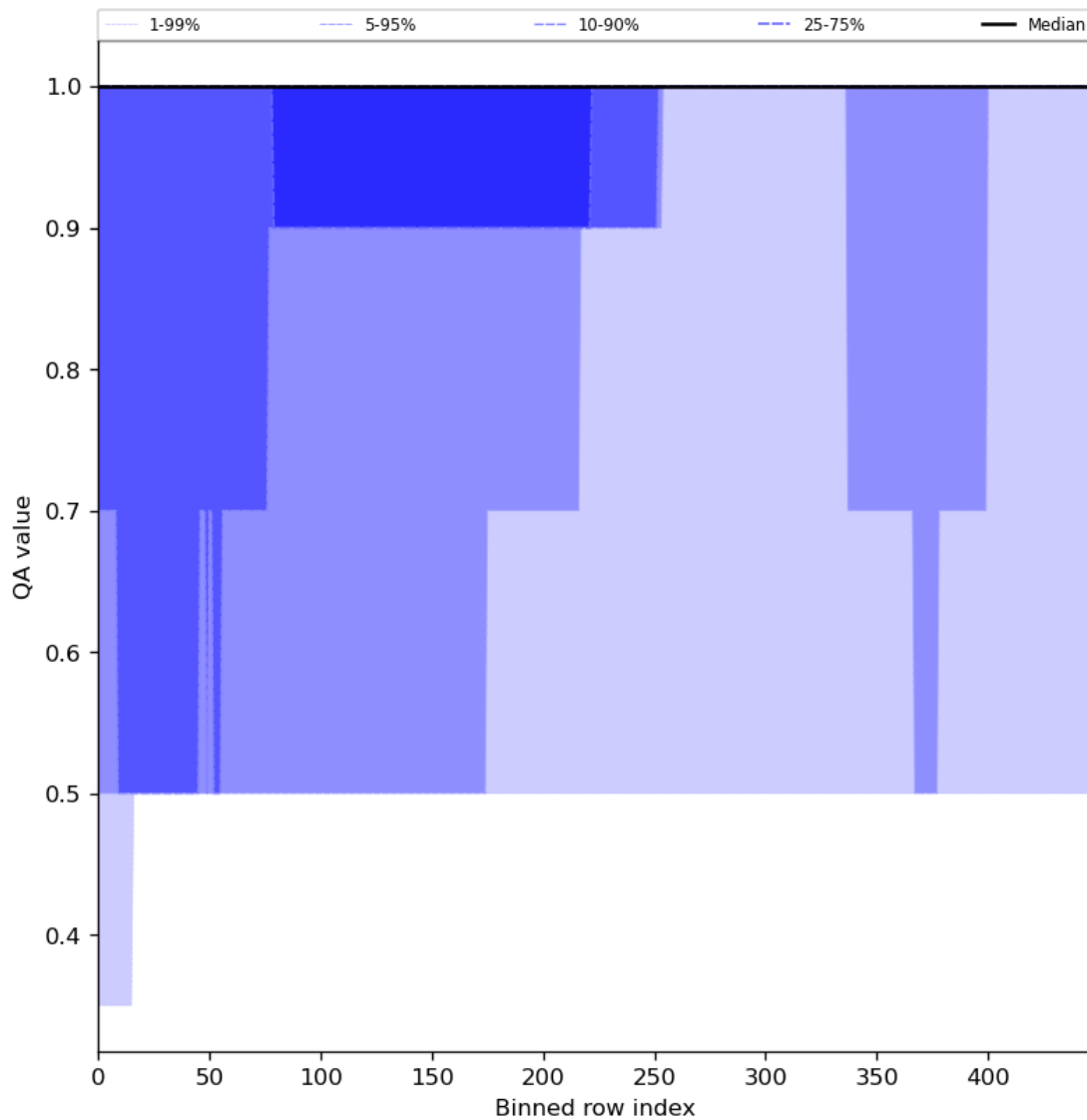
Figure 46: Along track statistics of “QA value” for 2024-02-11 to 2024-02-12
