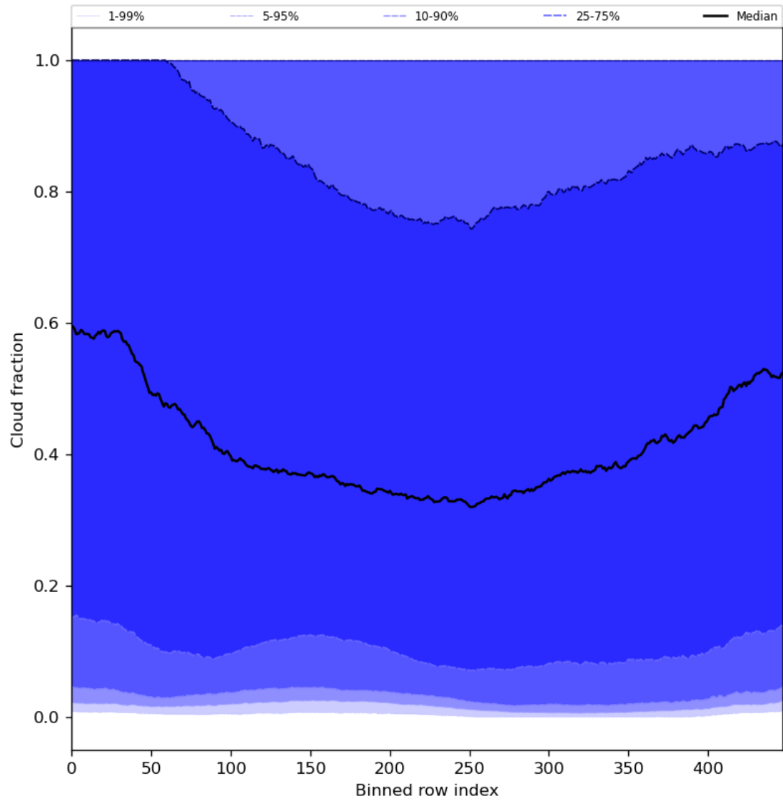
Figure 49: Along track statistics of “Cloud fraction” for 2024-02-11 to 2024-02-12
