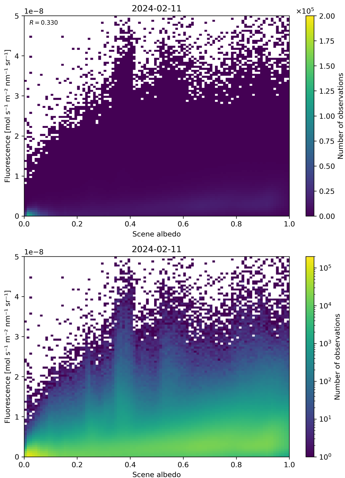
Figure 104: Scatter density plot of “Scene albedo” against “Fluorescence” for 2024-02-11 to 2024-02-12.
