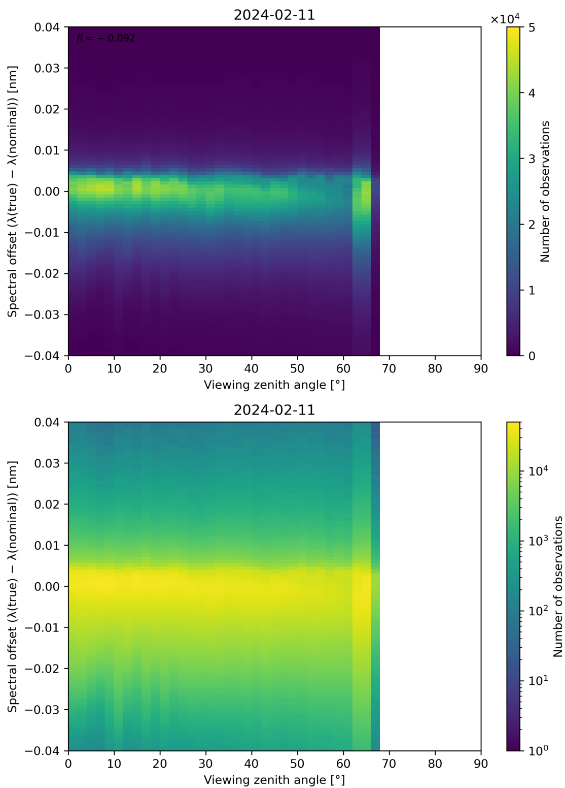
Figure 128: Scatter density plot of “Viewing zenith angle” against “Spectral offset ( \lambda(\text{true}) - \lambda(\text{nominal}) )” for 2024-02-11 to 2024-02-12.
