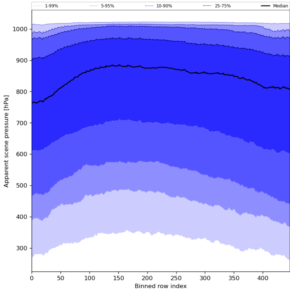
Figure 53: Along track statistics of “Apparent scene pressure” for 2024-02-11 to 2024-02-12
