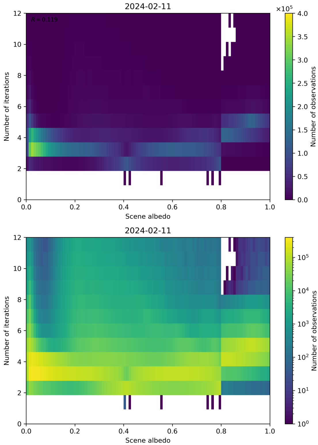
Figure 105: Scatter density plot of “Scene albedo” against “Number of iterations” for 2024-02-11 to 2024-02-12.
