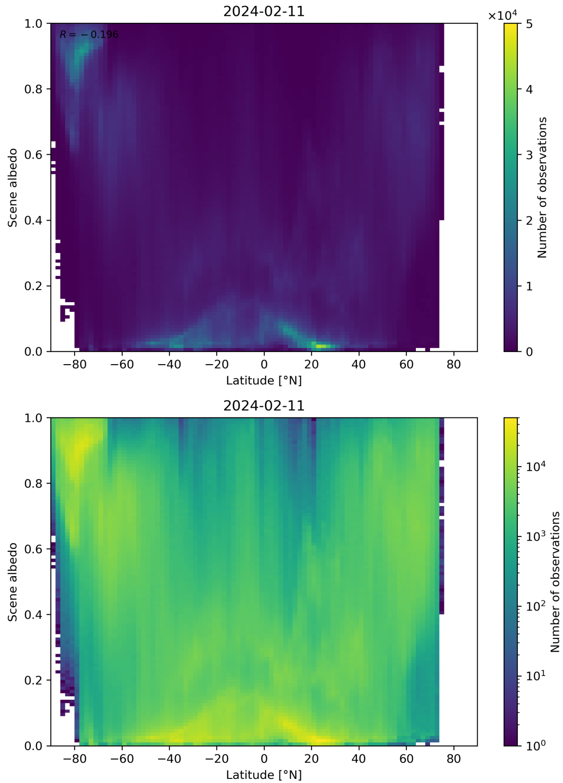
Figure 95: Scatter density plot of “Latitude” against “Scene albedo” for 2024-02-11 to 2024-02-12.
