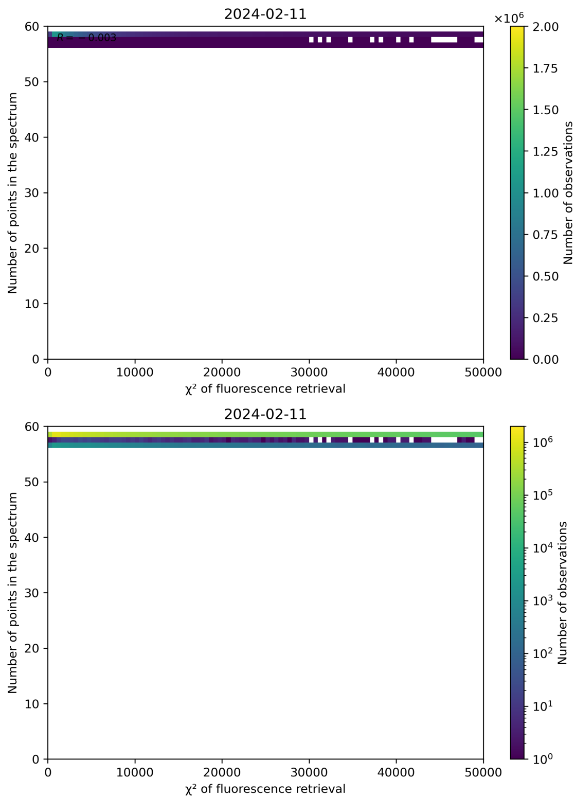
Figure 68: Scatter density plot of " \chi^2 of fluorescence retrieval" against "Number of points in the spectrum" for 2024-02-11 to 2024-02-12.
