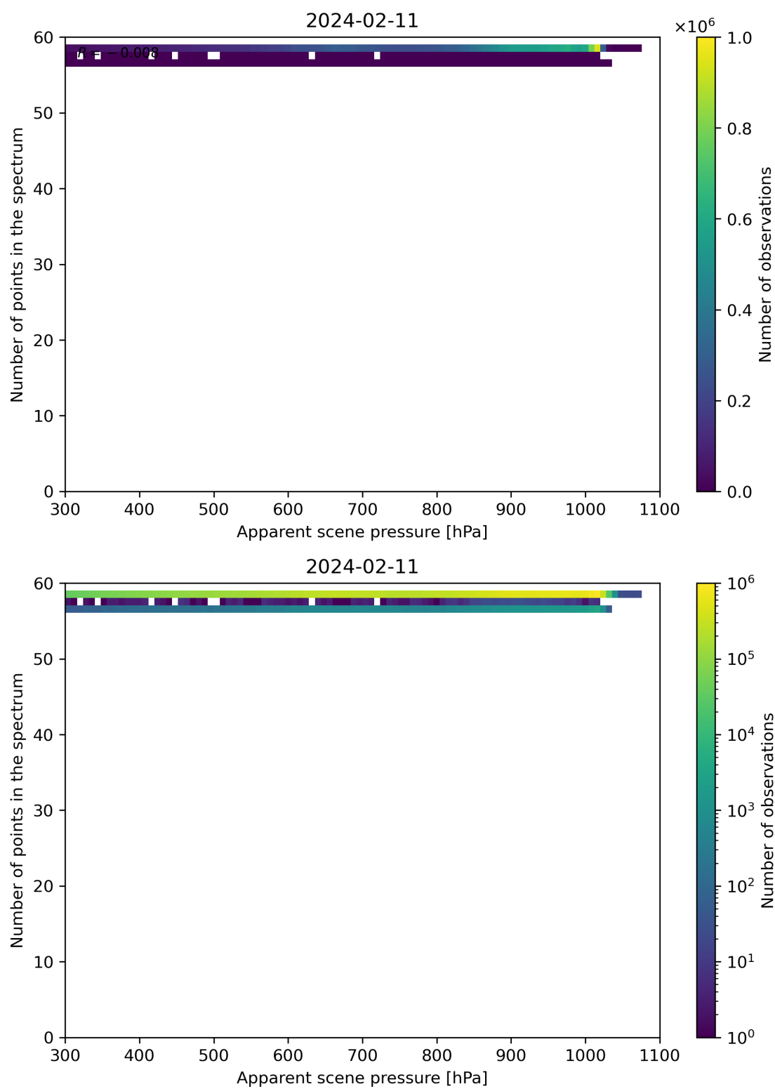
Figure 66: Scatter density plot of “Apparent scene pressure” against “Number of points in the spectrum” for 2024-02-11 to 2024-02-12.
