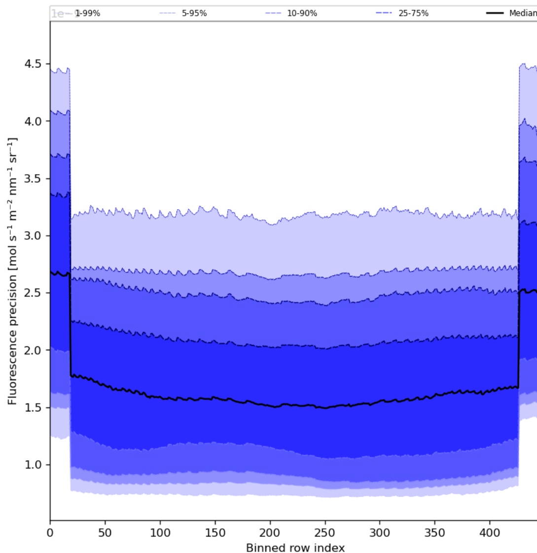
Figure 58: Along track statistics of “Fluorescence precision” for 2024-02-11 to 2024-02-12
