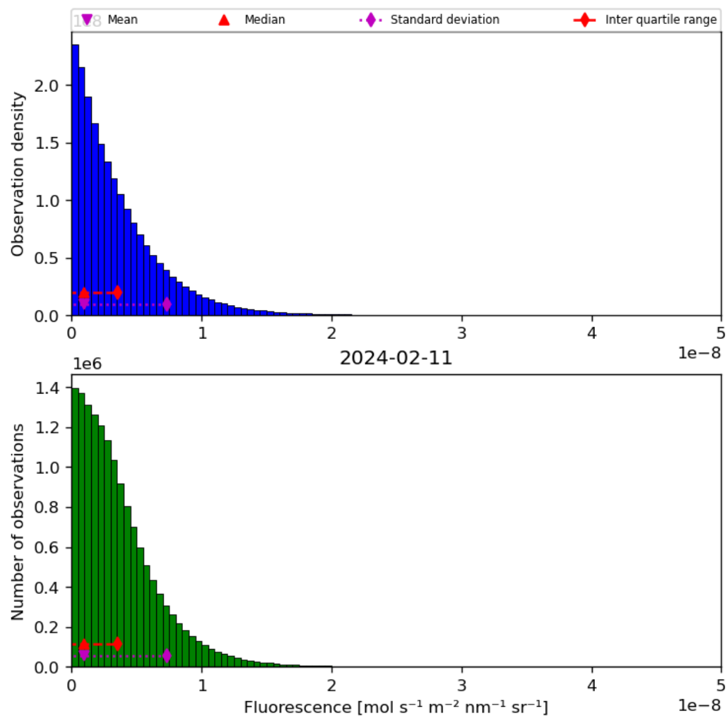
Figure 40: Histogram of “Fluorescence” for 2024-02-11 to 2024-02-12
