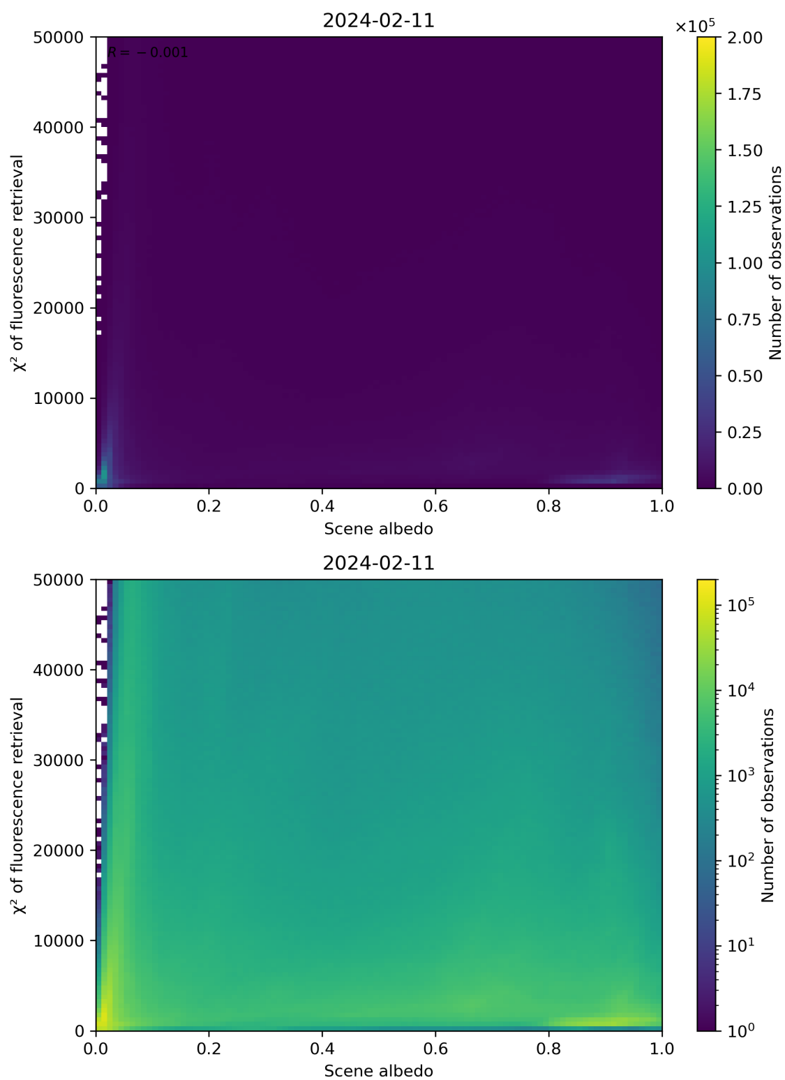
Figure 103: Scatter density plot of “Scene albedo” against “ \chi^2 of fluorescence retrieval” for 2024-02-11 to 2024-02-12.
