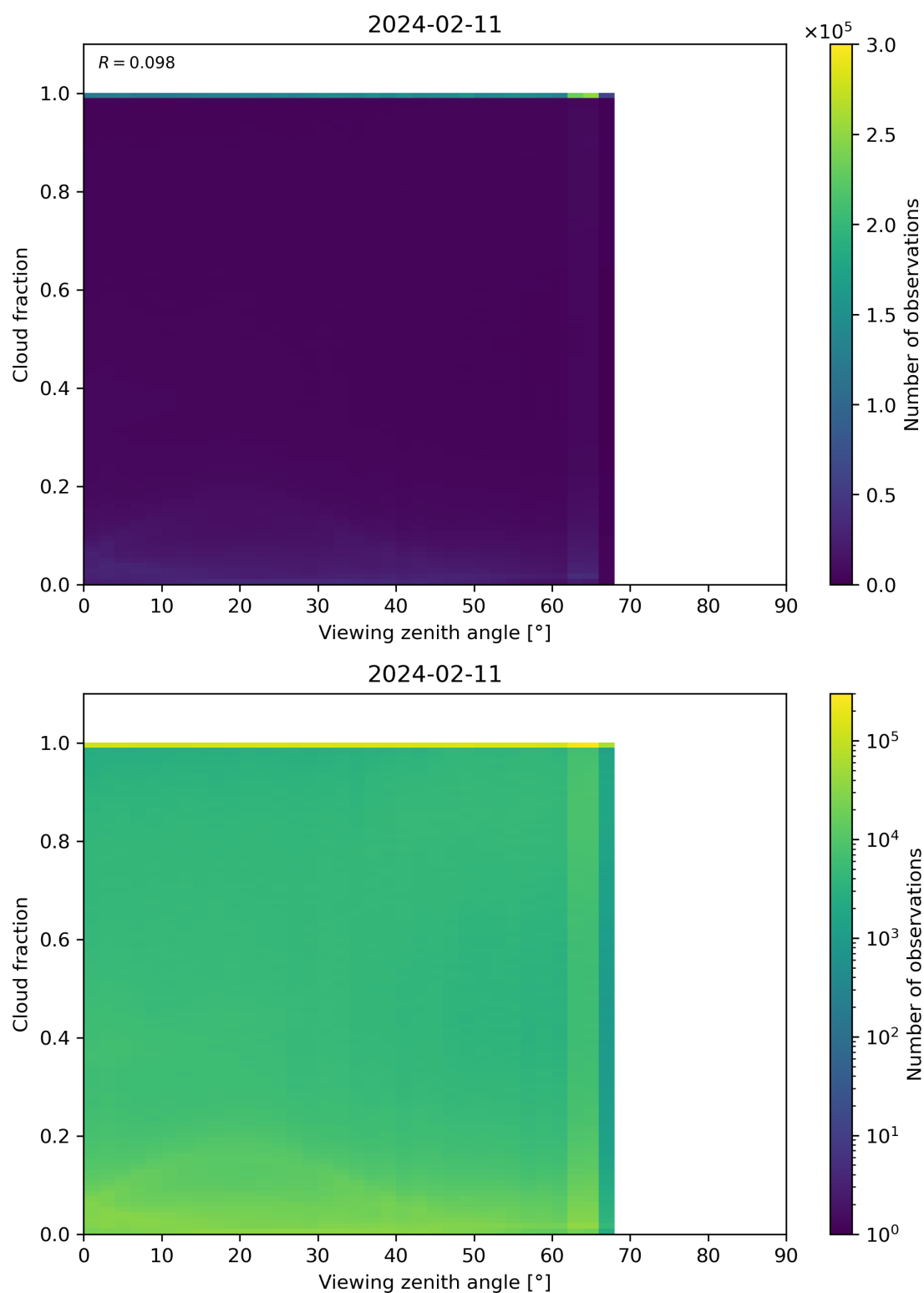
Figure 120: Scatter density plot of “Viewing zenith angle” against “Cloud fraction” for 2024-02-11 to 2024-02-12.
