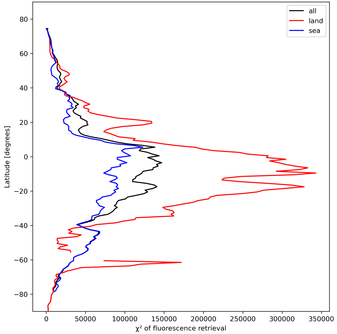
Figure 25: Zonal average of “ \chi^2 of fluorescence retrieval” for 2024-02-11 to 2024-02-12.
