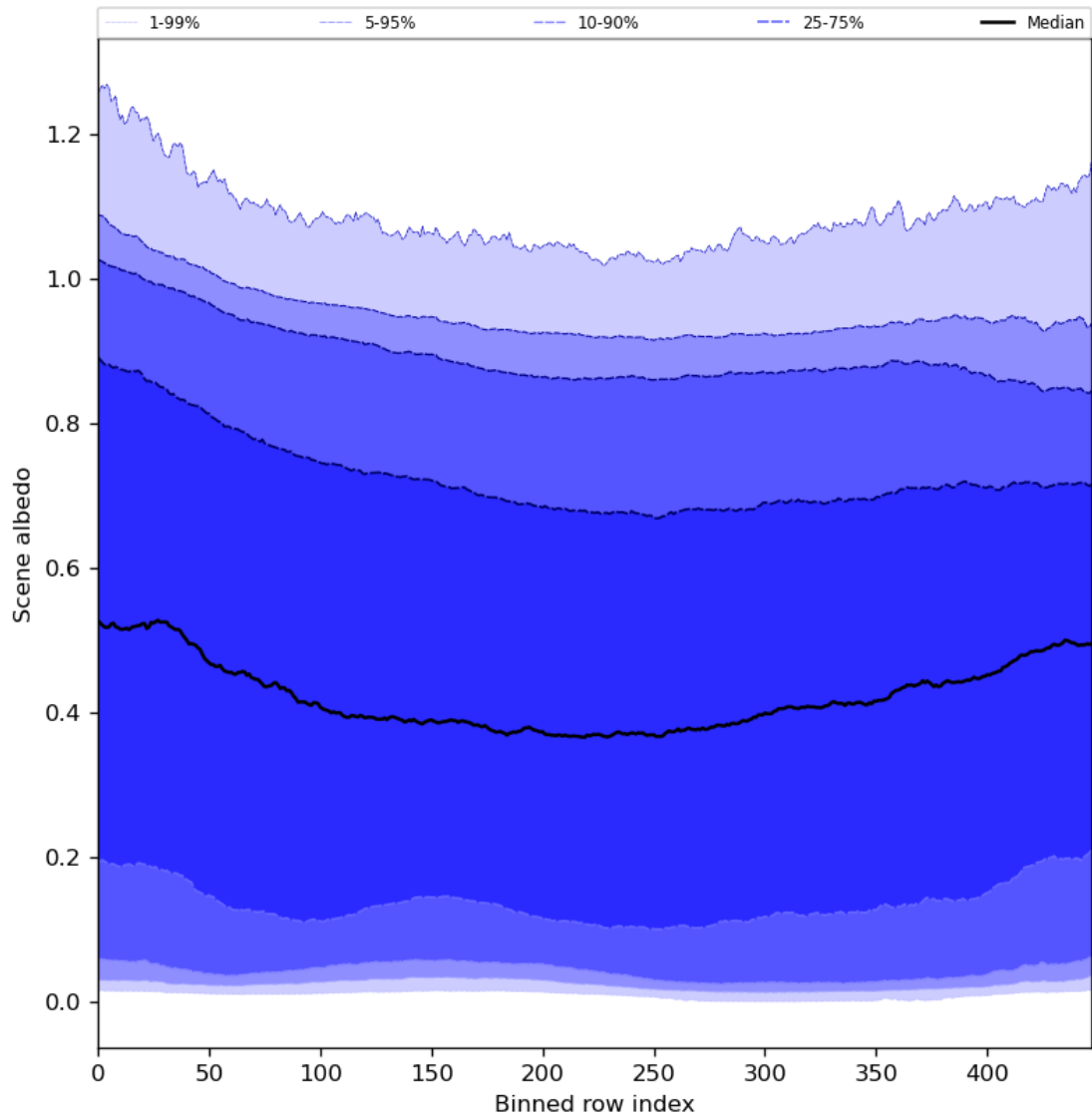
Figure 51: Along track statistics of “Scene albedo” for 2024-02-11 to 2024-02-12
