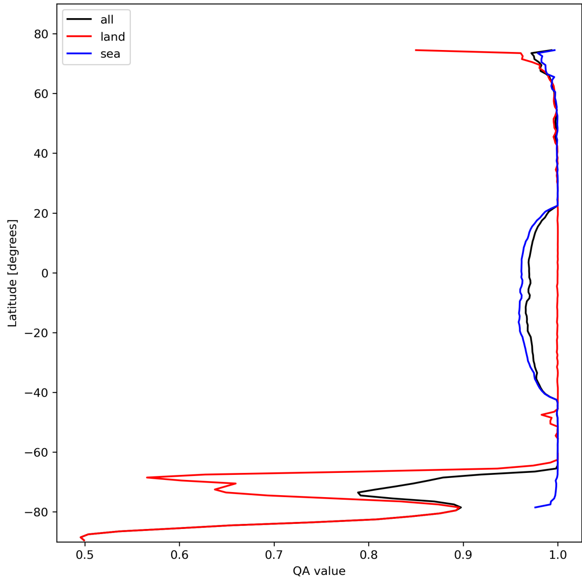
Figure 12: Zonal average of “QA value” for 2024-02-11 to 2024-02-12.
