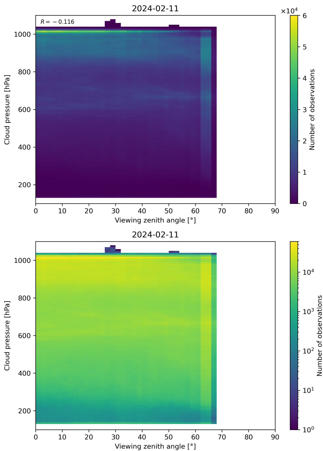
Figure 121: Scatter density plot of “Viewing zenith angle” against “Cloud pressure” for 2024-02-11 to 2024-02-12.
