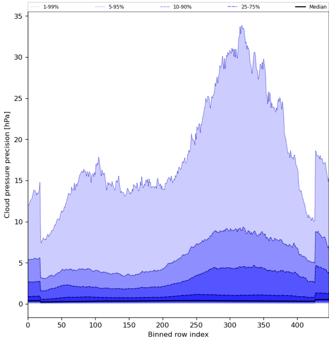
Figure 48: Along track statistics of “Cloud pressure precision” for 2024-02-11 to 2024-02-12
