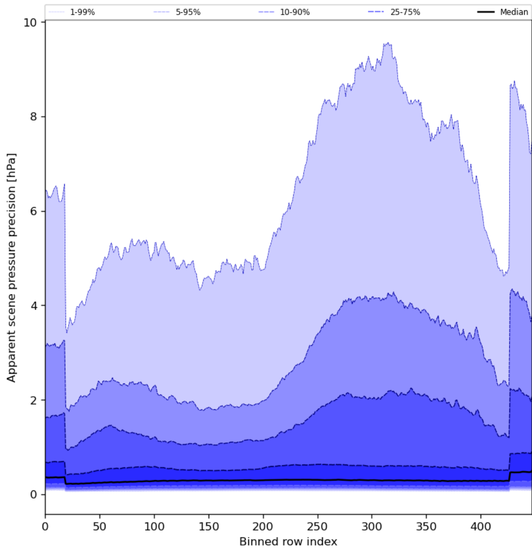
Figure 54: Along track statistics of “Apparent scene pressure precision” for 2024-02-11 to 2024-02-12
