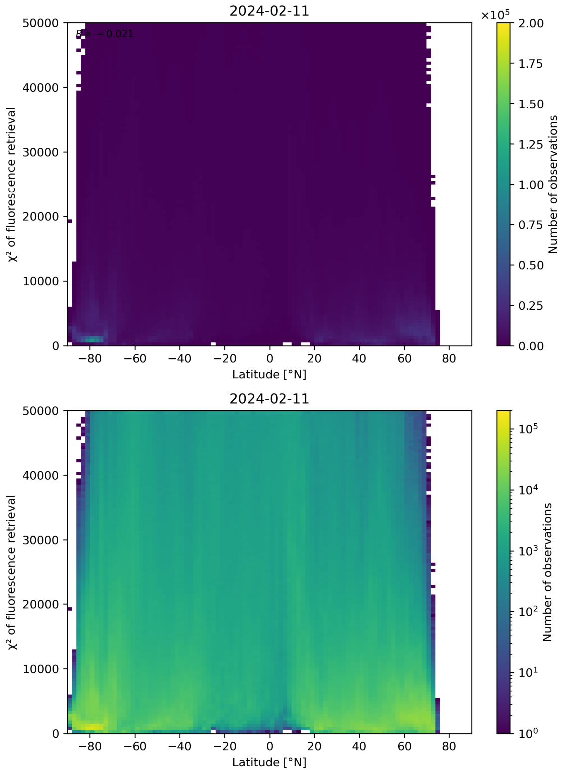
Figure 89: Scatter density plot of “Latitude” against “ \chi^2 of fluorescence retrieval” for 2024-02-11 to 2024-02-12.
