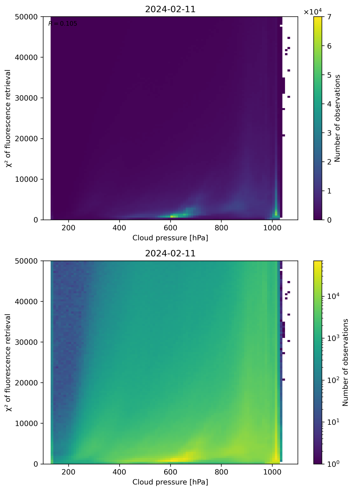
Figure 78: Scatter density plot of “Cloud pressure” against “ \chi^2 of fluorescence retrieval” for 2024-02-11 to 2024-02-12.
