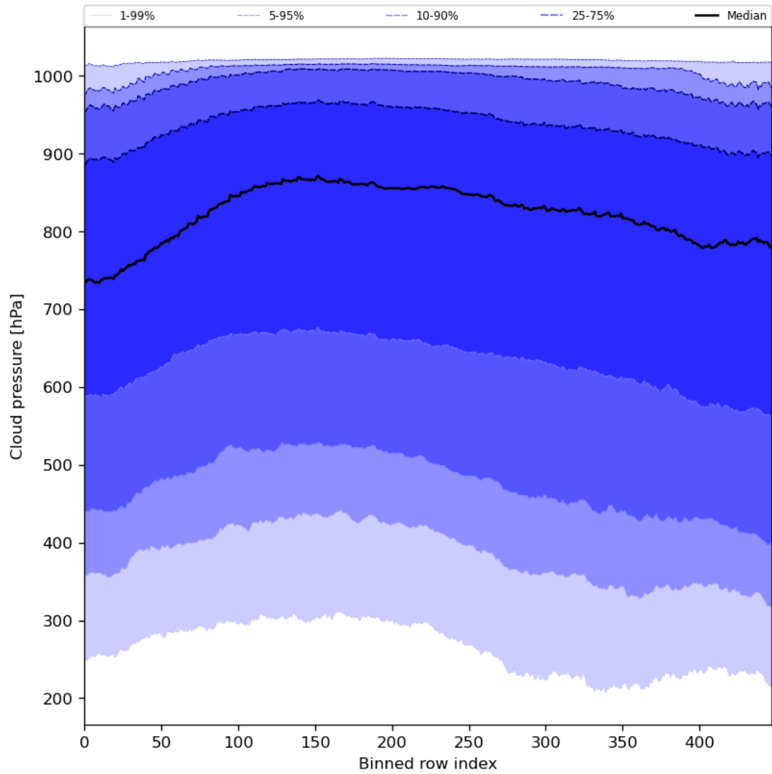
Figure 47: Along track statistics of “Cloud pressure” for 2024-02-11 to 2024-02-12
