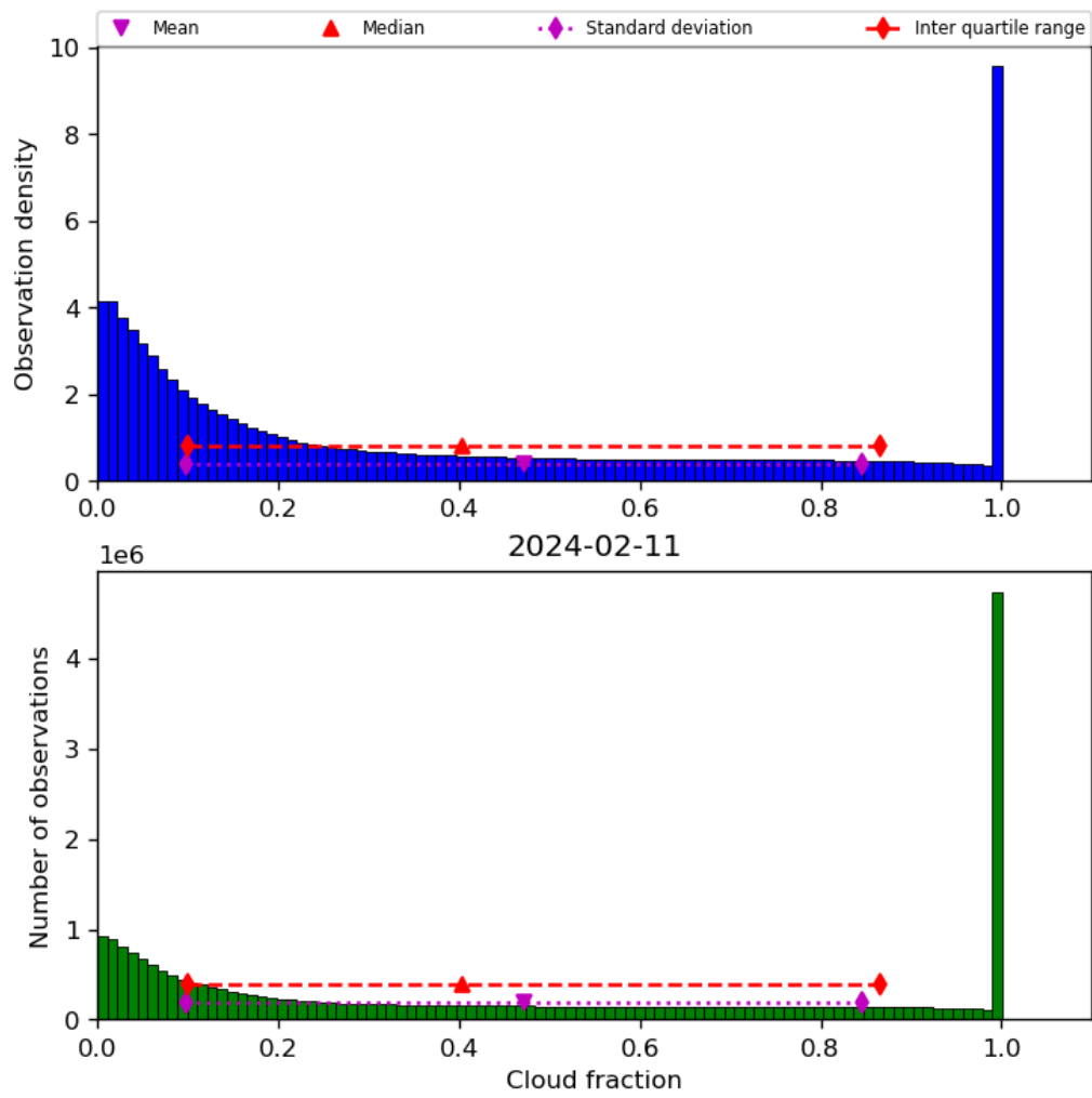
Figure 32: Histogram of “Cloud fraction” for 2024-02-11 to 2024-02-12
