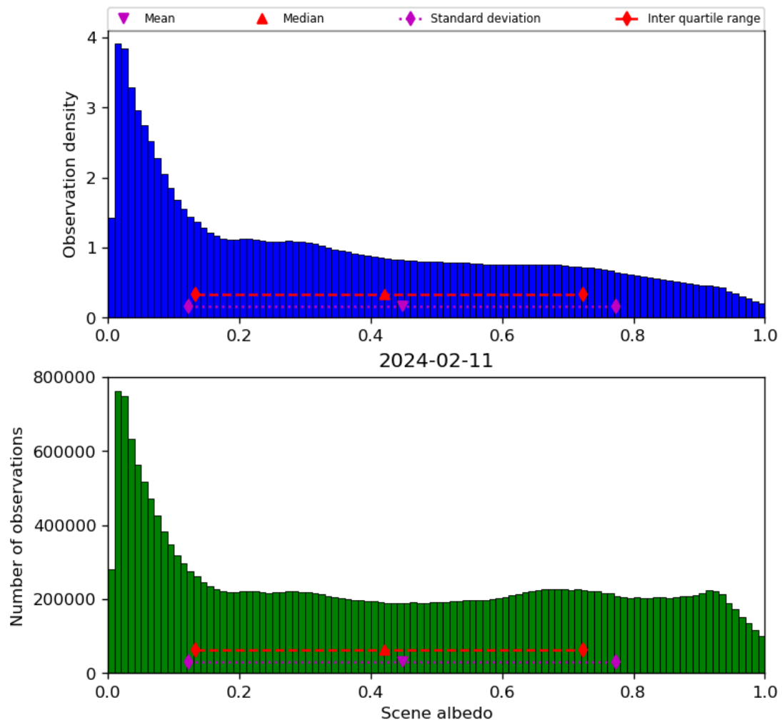
Figure 34: Histogram of “Scene albedo” for 2024-02-11 to 2024-02-12
