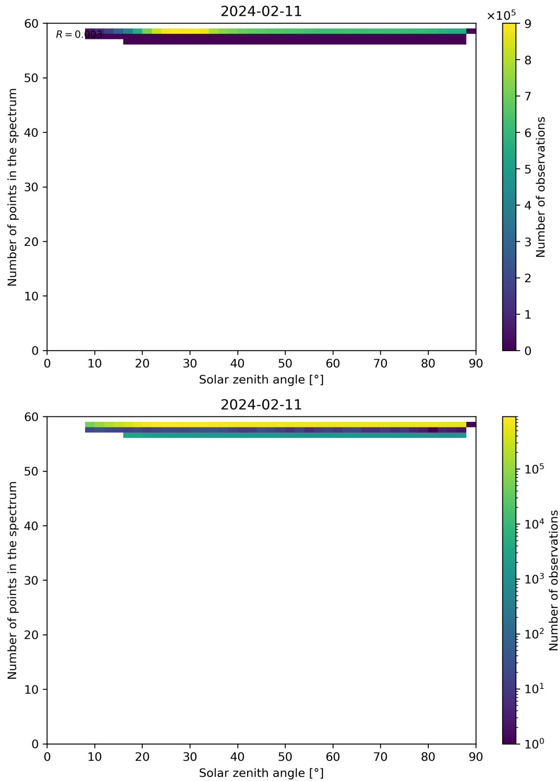
Figure 115: Scatter density plot of “Solar zenith angle” against “Number of points in the spectrum” for 2024-02-11 to 2024-02-12.
