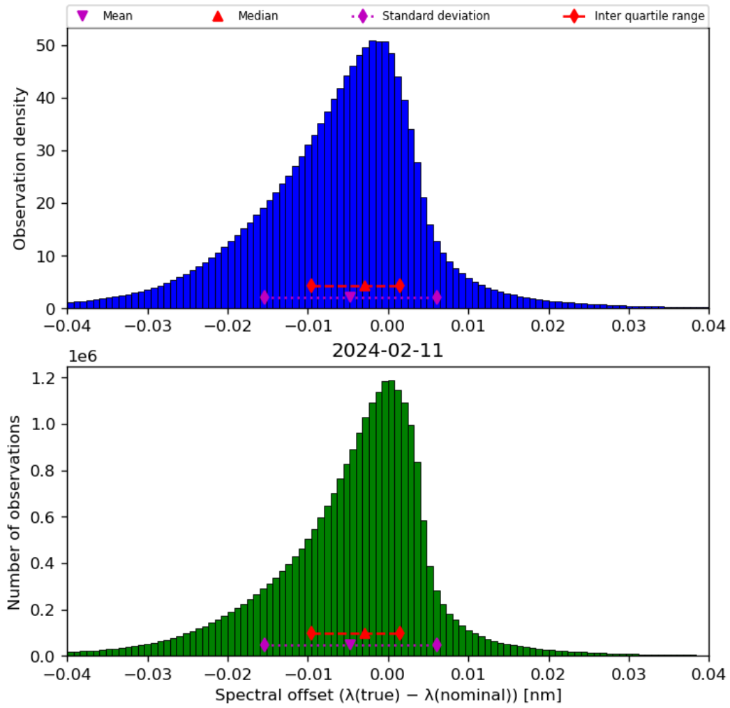
Figure 45: Histogram of “Spectral offset ( \lambda(\text{true}) - \lambda(\text{nominal}) )” for 2024-02-11 to 2024-02-12
