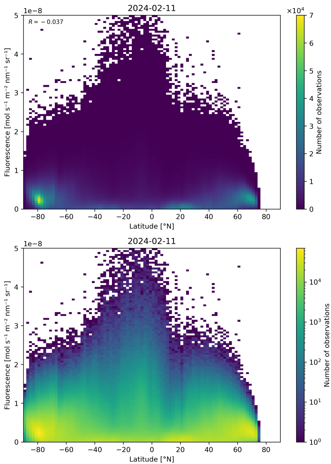
Figure 92: Scatter density plot of “Latitude” against “Fluorescence” for 2024-02-11 to 2024-02-12.
