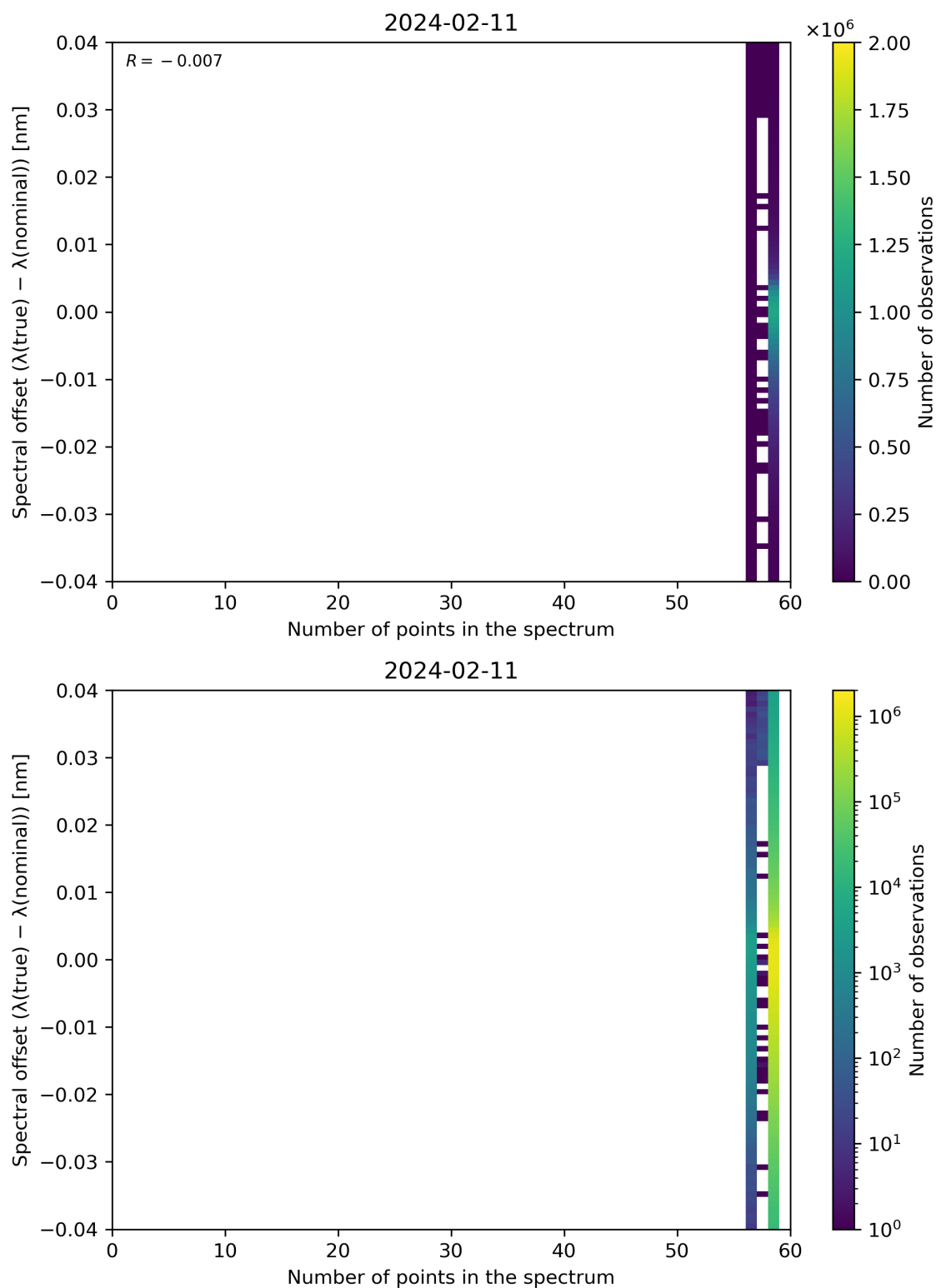
Figure 101: Scatter density plot of “Number of points in the spectrum” against “Spectral offset ( \lambda(\text{true}) - \lambda(\text{nominal}) )” for 2024-02-11 to 2024-02-12.
