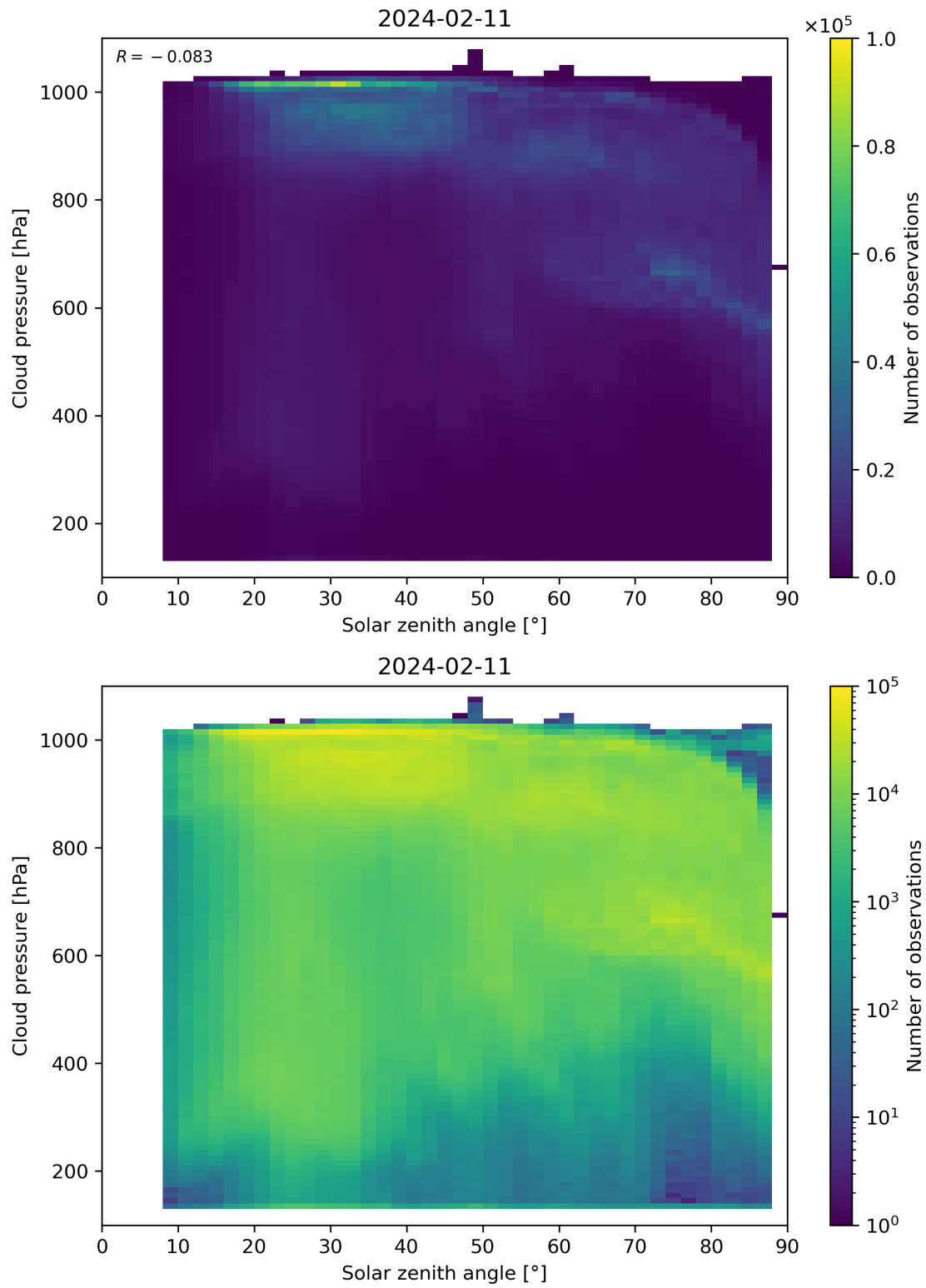
Figure 111: Scatter density plot of “Solar zenith angle” against “Cloud pressure” for 2024-02-11 to 2024-02-12.
