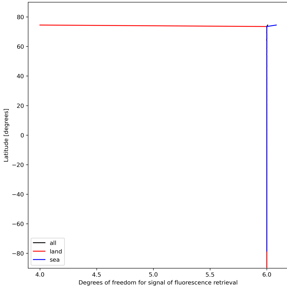
Figure 26: Zonal average of “Degrees of freedom for signal of fluorescence retrieval” for 2024-02-11 to 2024-02-12.
