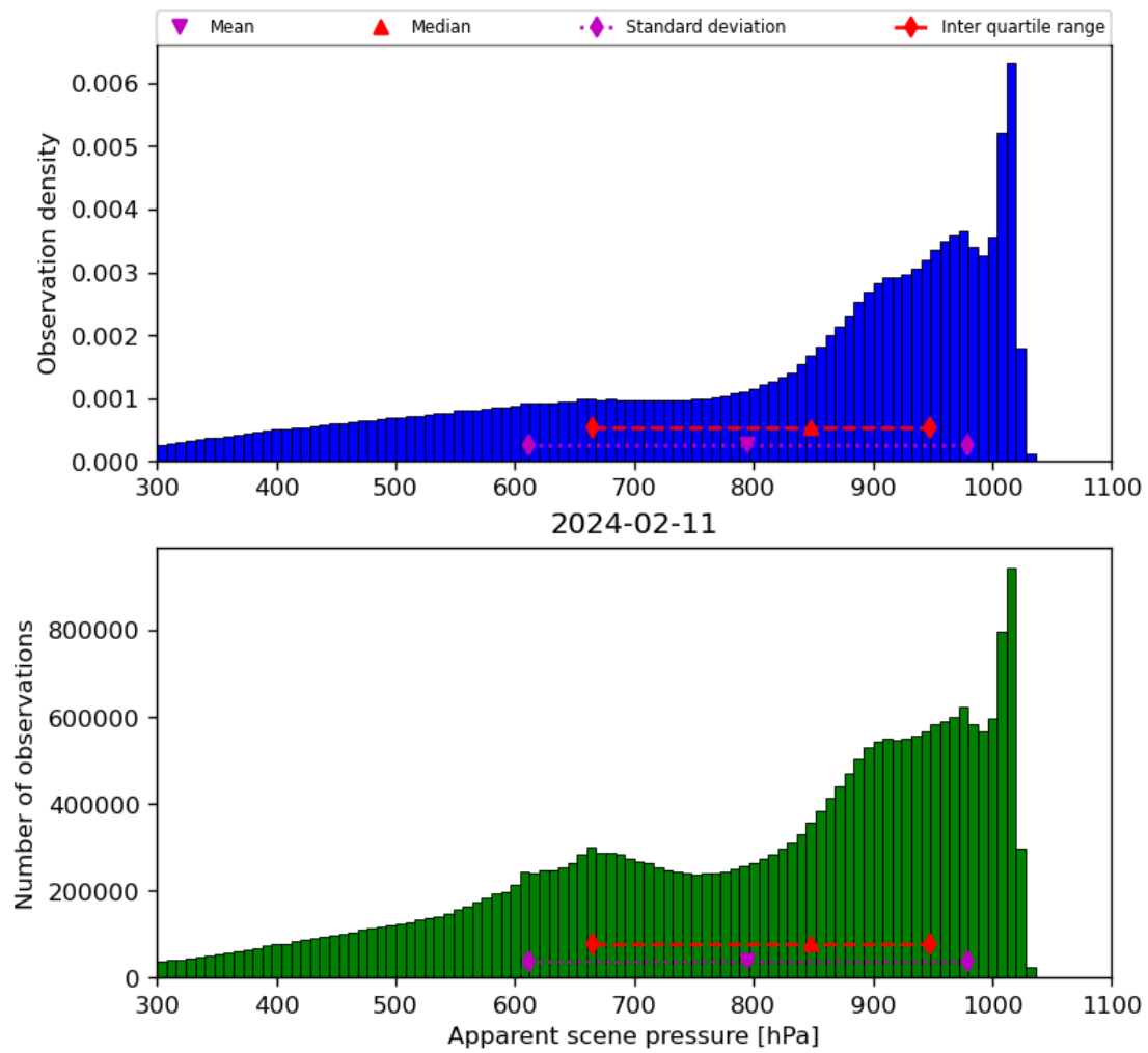
Figure 36: Histogram of “Apparent scene pressure” for 2024-02-11 to 2024-02-12
