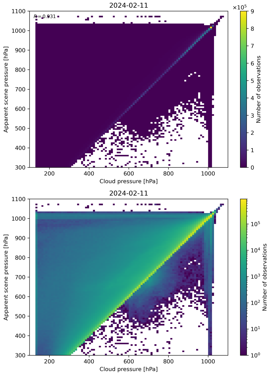
Figure 77: Scatter density plot of “Cloud pressure” against “Apparent scene pressure” for 2024-02-11 to 2024-02-12.
