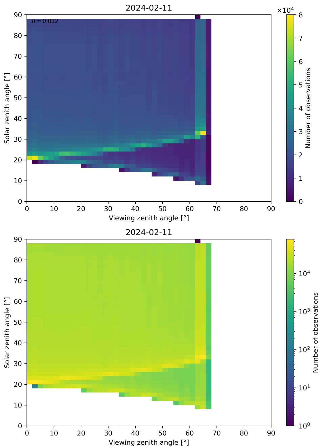
Figure 127: Scatter density plot of “Viewing zenith angle” against “Solar zenith angle” for 2024-02-11 to 2024-02-12.
