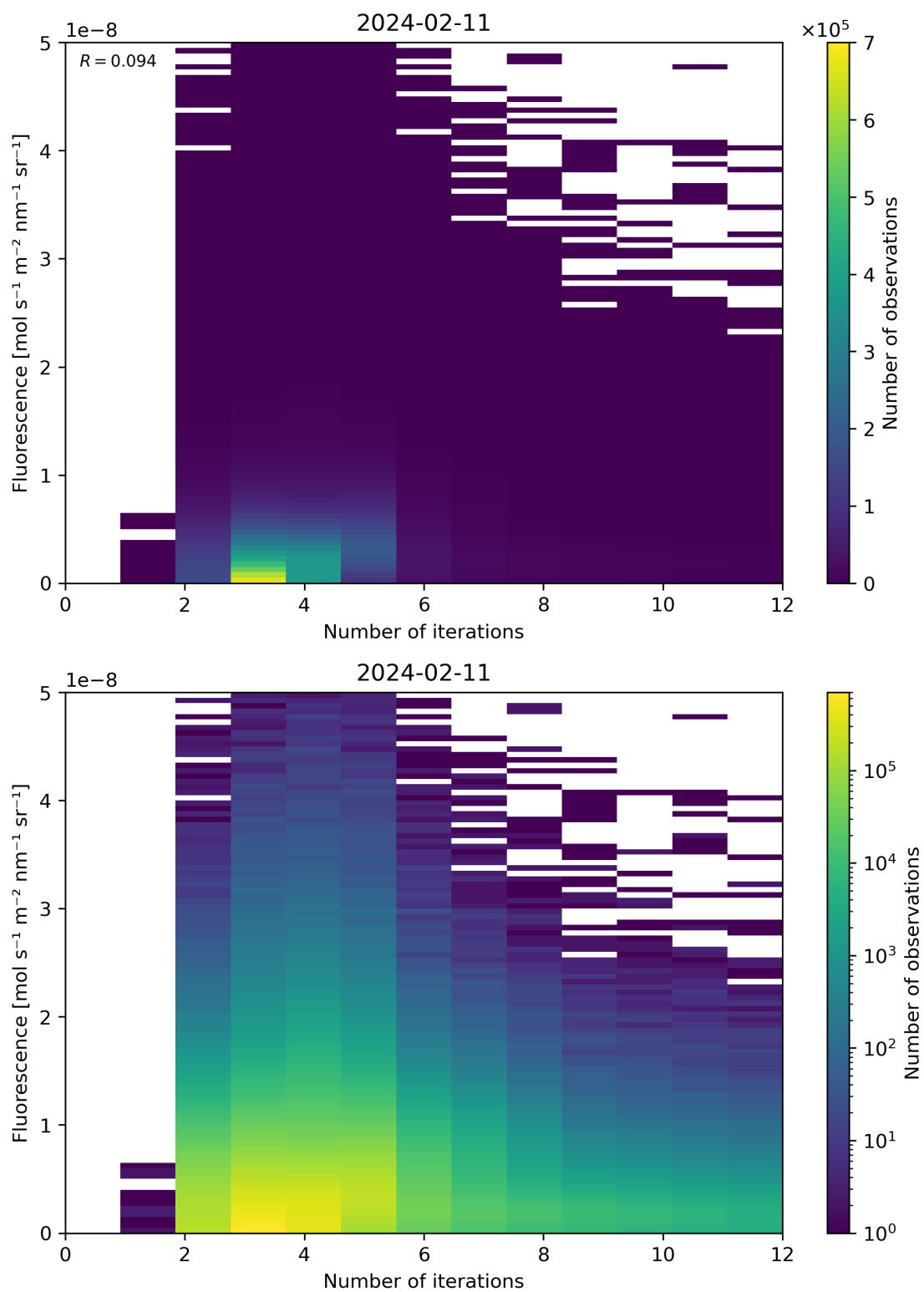
Figure 98: Scatter density plot of “Number of iterations” against “Fluorescence” for 2024-02-11 to 2024-02-12.
