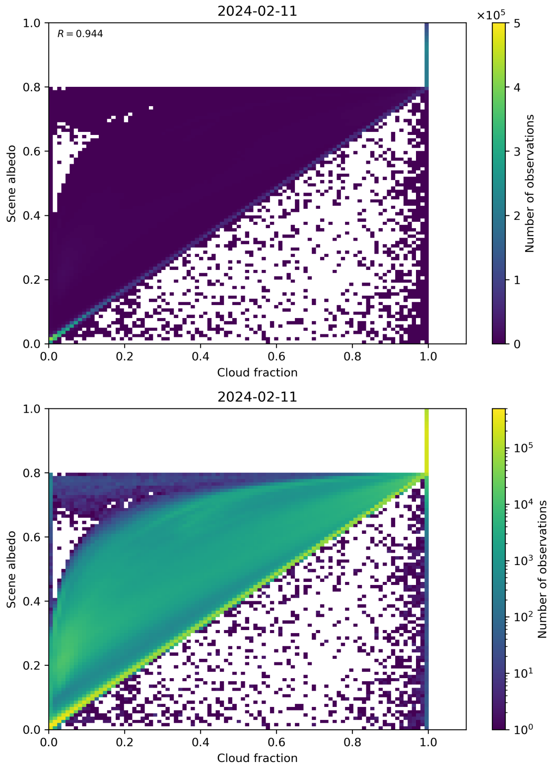
Figure 75: Scatter density plot of “Cloud fraction” against “Scene albedo” for 2024-02-11 to 2024-02-12.
