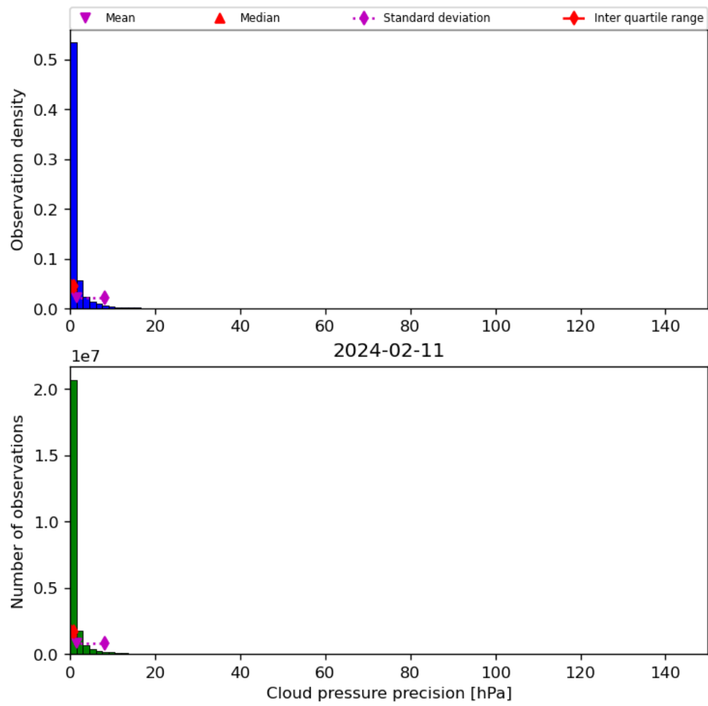
Figure 31: Histogram of “Cloud pressure precision” for 2024-02-11 to 2024-02-12
