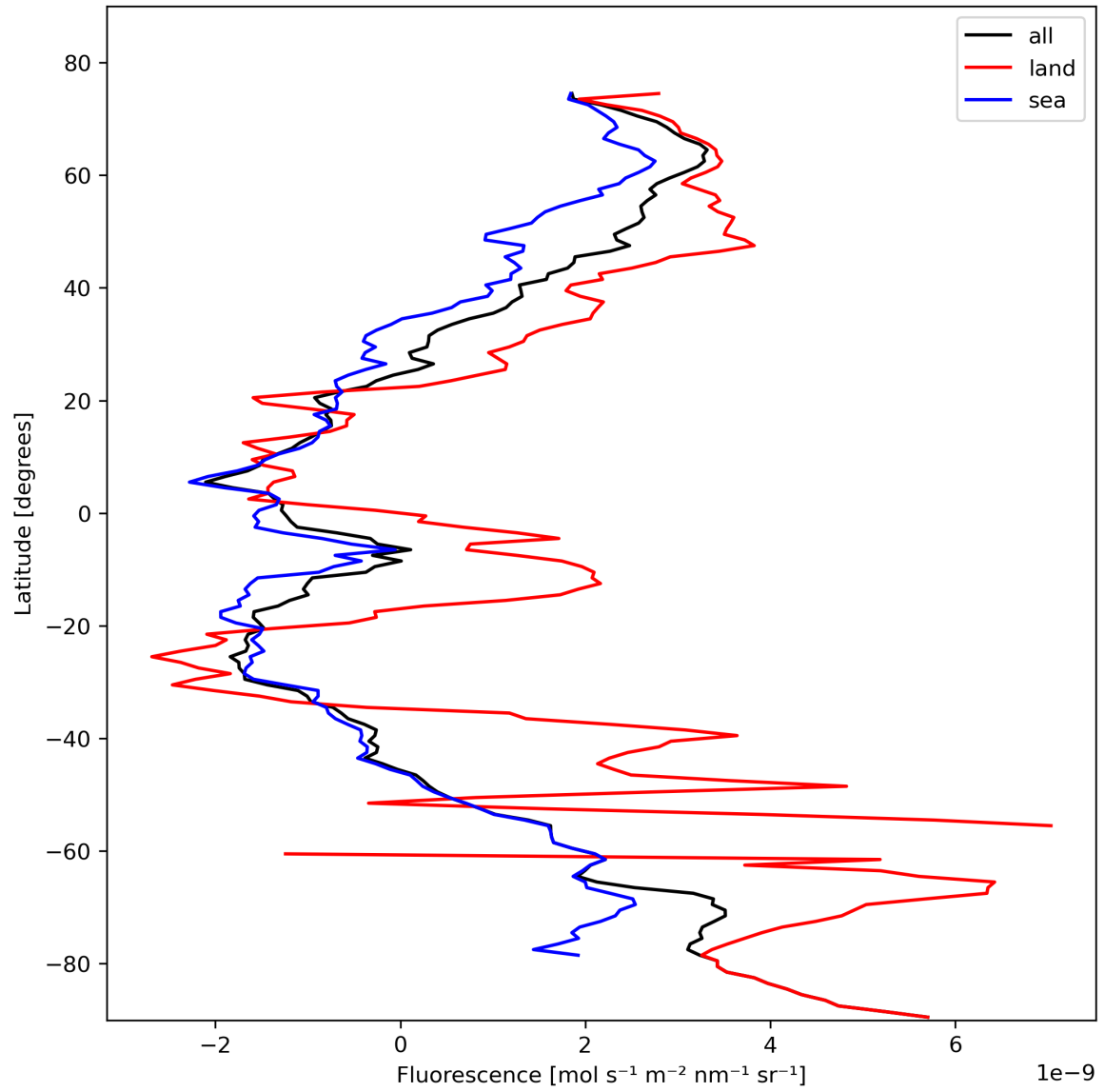
Figure 23: Zonal average of “Fluorescence” for 2024-02-11 to 2024-02-12.
