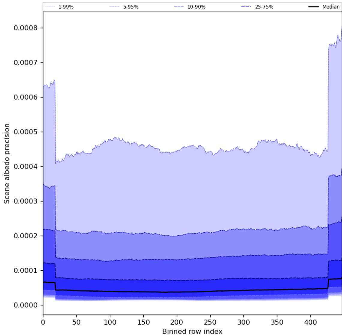
Figure 52: Along track statistics of “Scene albedo precision” for 2024-02-11 to 2024-02-12
