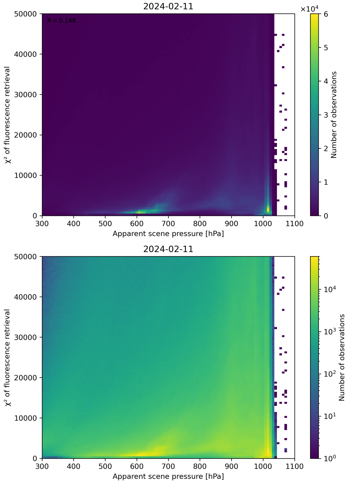
Figure 63: Scatter density plot of “Apparent scene pressure” against “ \chi^2 of fluorescence retrieval” for 2024-02-11 to 2024-02-12.
