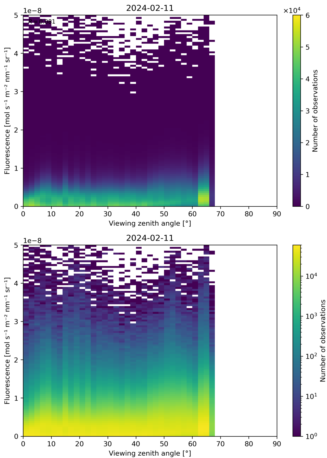
Figure 122: Scatter density plot of “Viewing zenith angle” against “Fluorescence” for 2024-02-11 to 2024-02-12.
