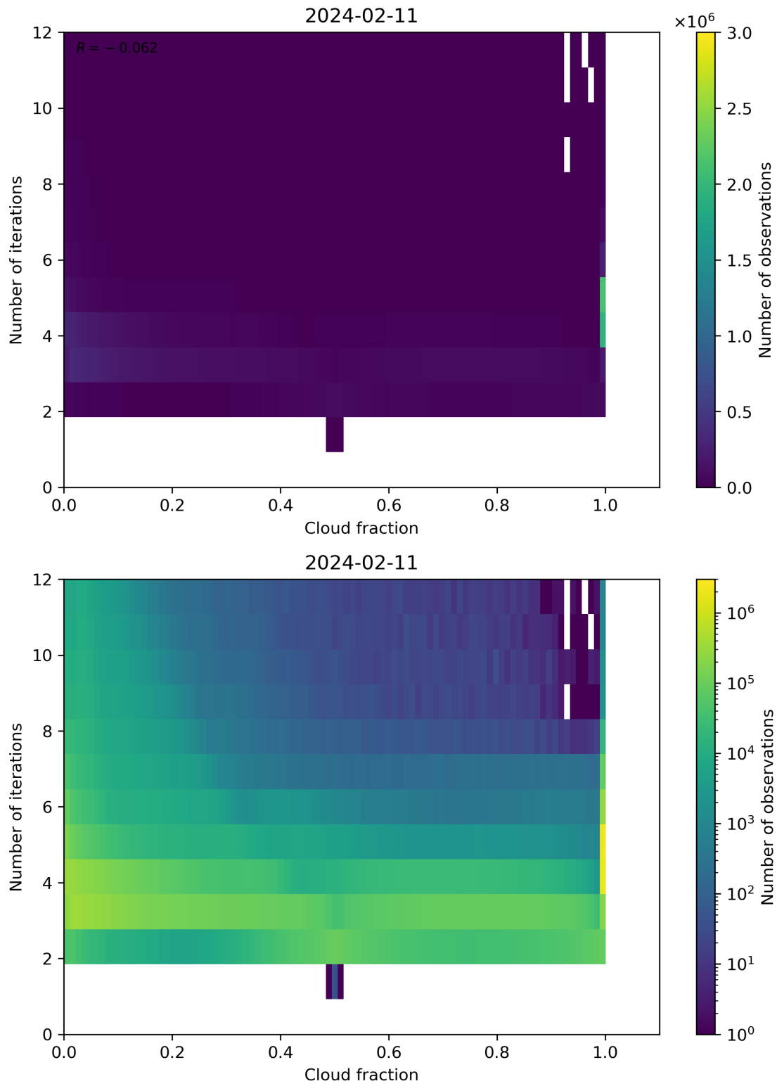
Figure 73: Scatter density plot of “Cloud fraction” against “Number of iterations” for 2024-02-11 to 2024-02-12.
