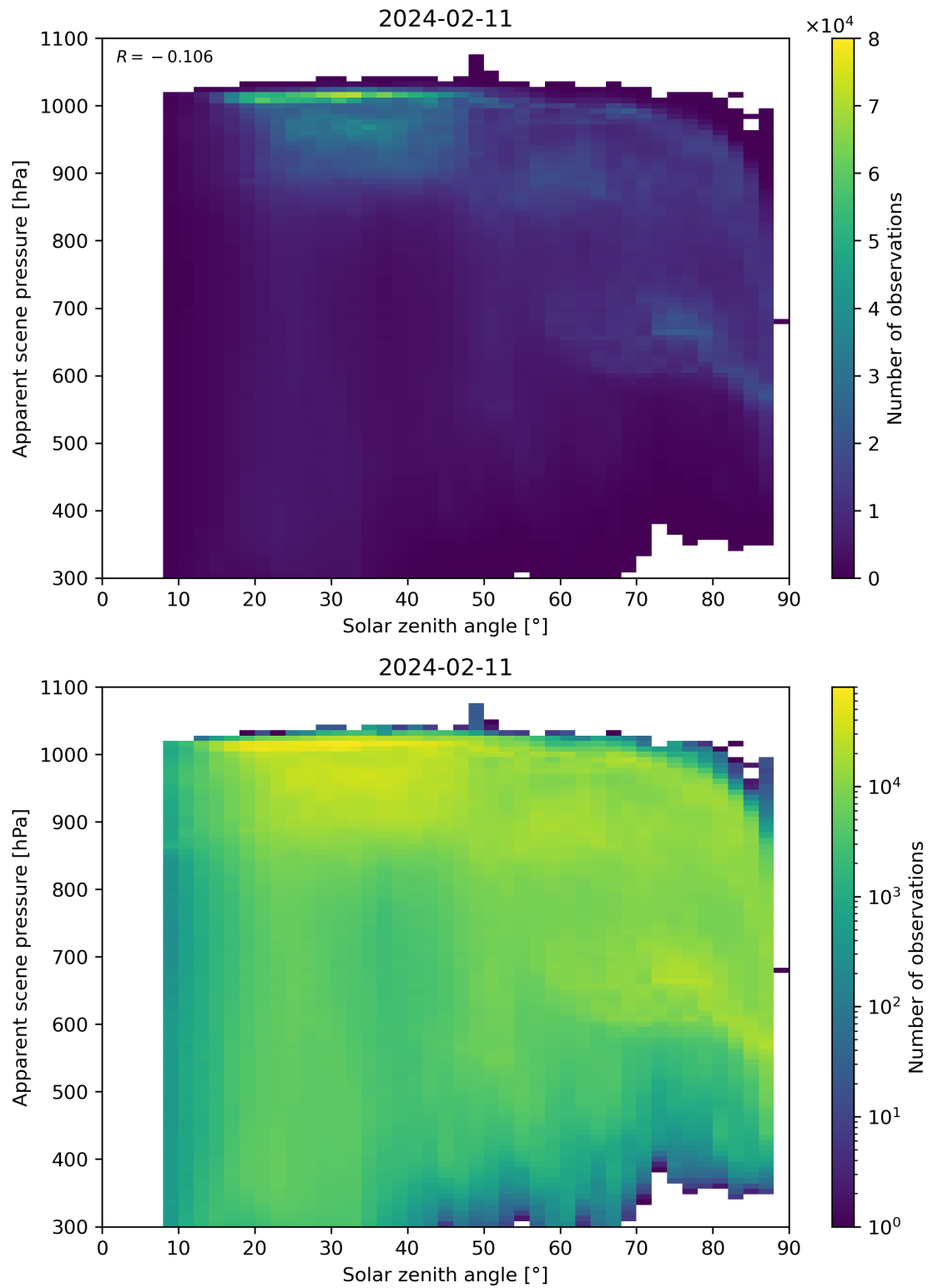
Figure 108: Scatter density plot of “Solar zenith angle” against “Apparent scene pressure” for 2024-02-11 to 2024-02-12.
