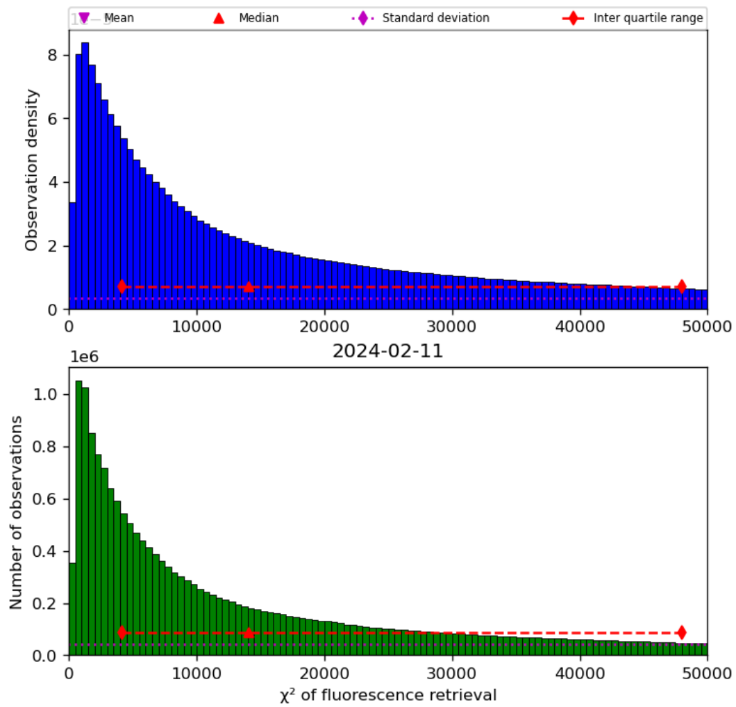
Figure 42: Histogram of “ \chi^2 of fluorescence retrieval” for 2024-02-11 to 2024-02-12
