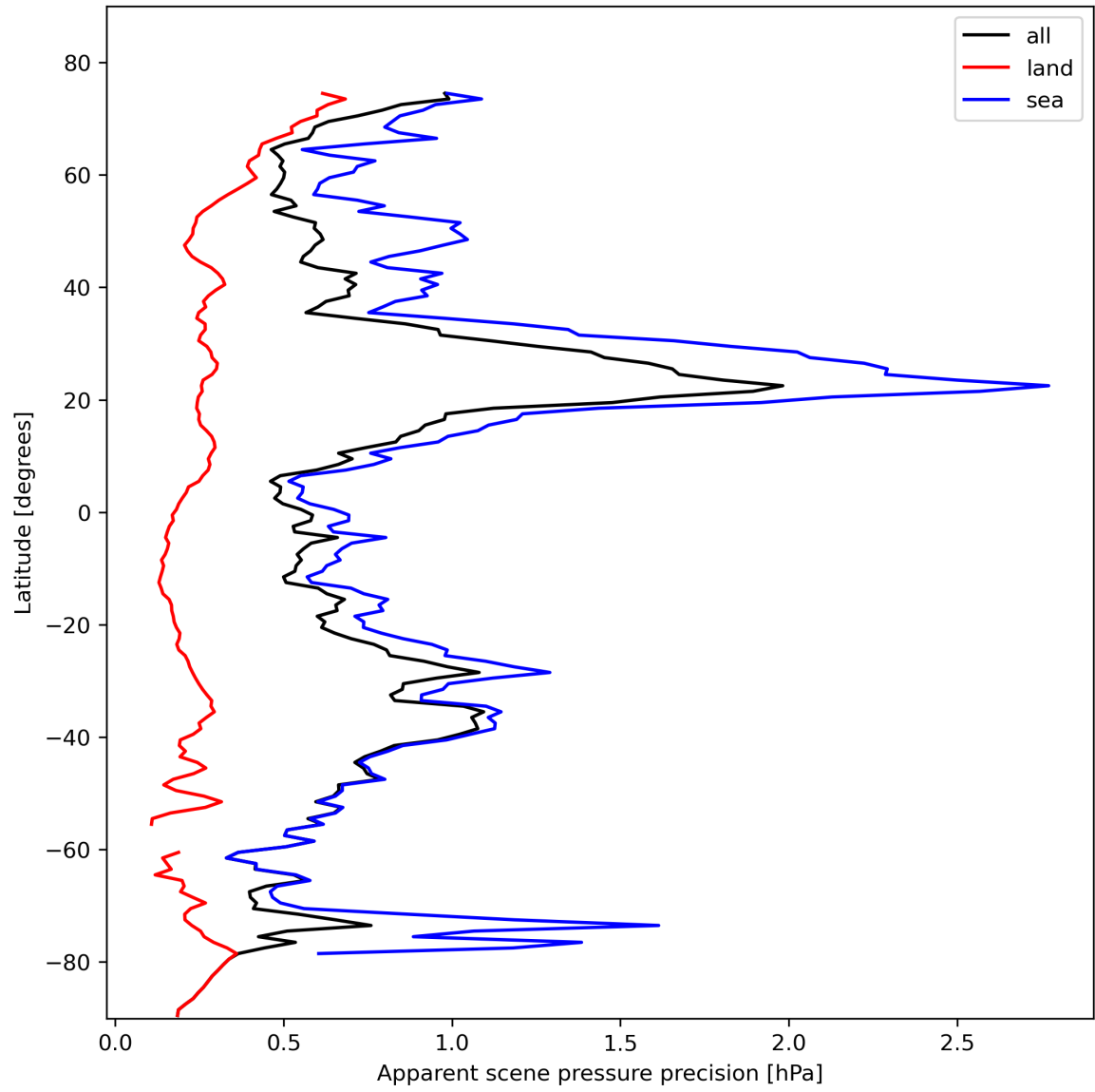
Figure 20: Zonal average of “Apparent scene pressure precision” for 2024-02-11 to 2024-02-12.
