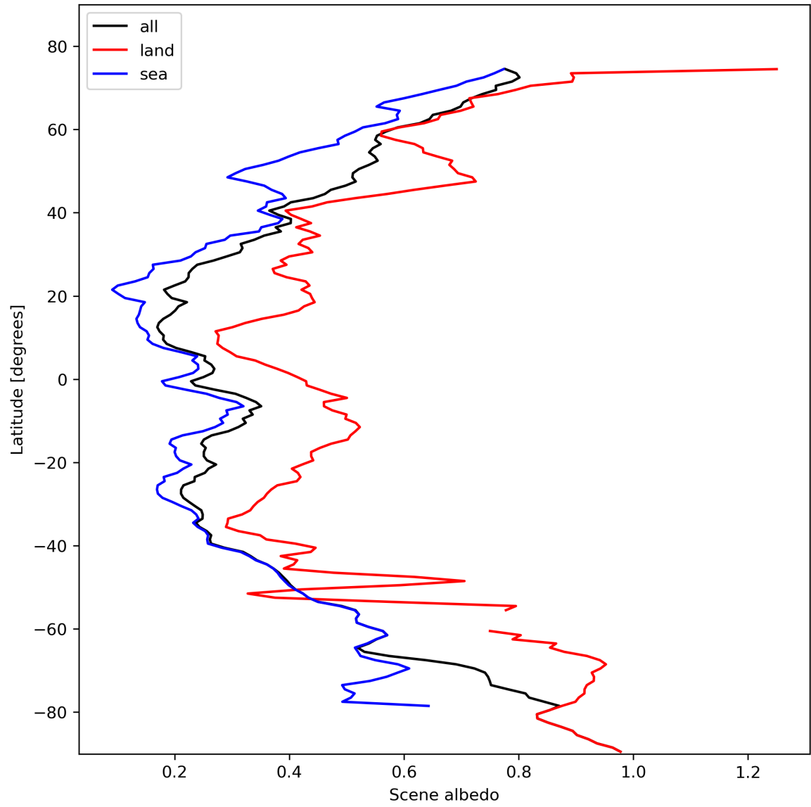
Figure 17: Zonal average of “Scene albedo” for 2024-02-11 to 2024-02-12.
