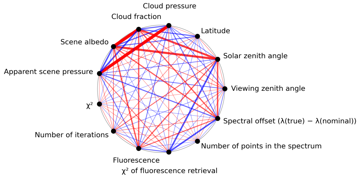
Figure 1: Map of correlation graph for 2024-02-11 to 2024-02-12.
