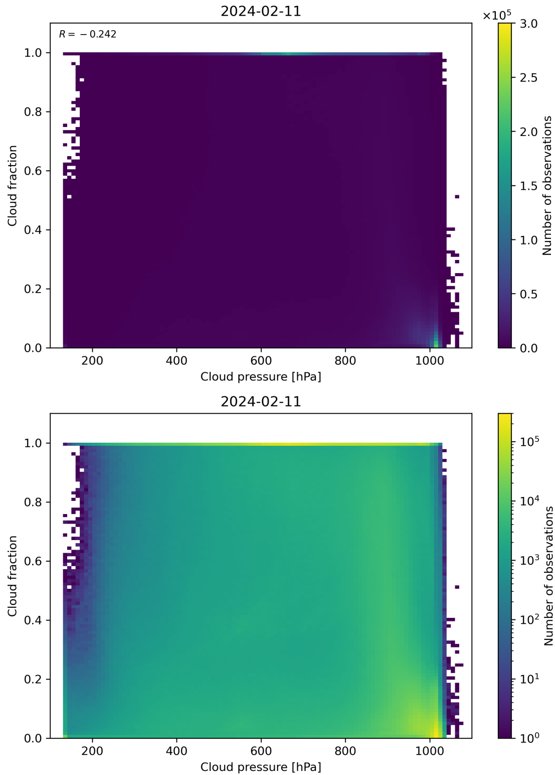
Figure 79: Scatter density plot of “Cloud pressure” against “Cloud fraction” for 2024-02-11 to 2024-02-12.
