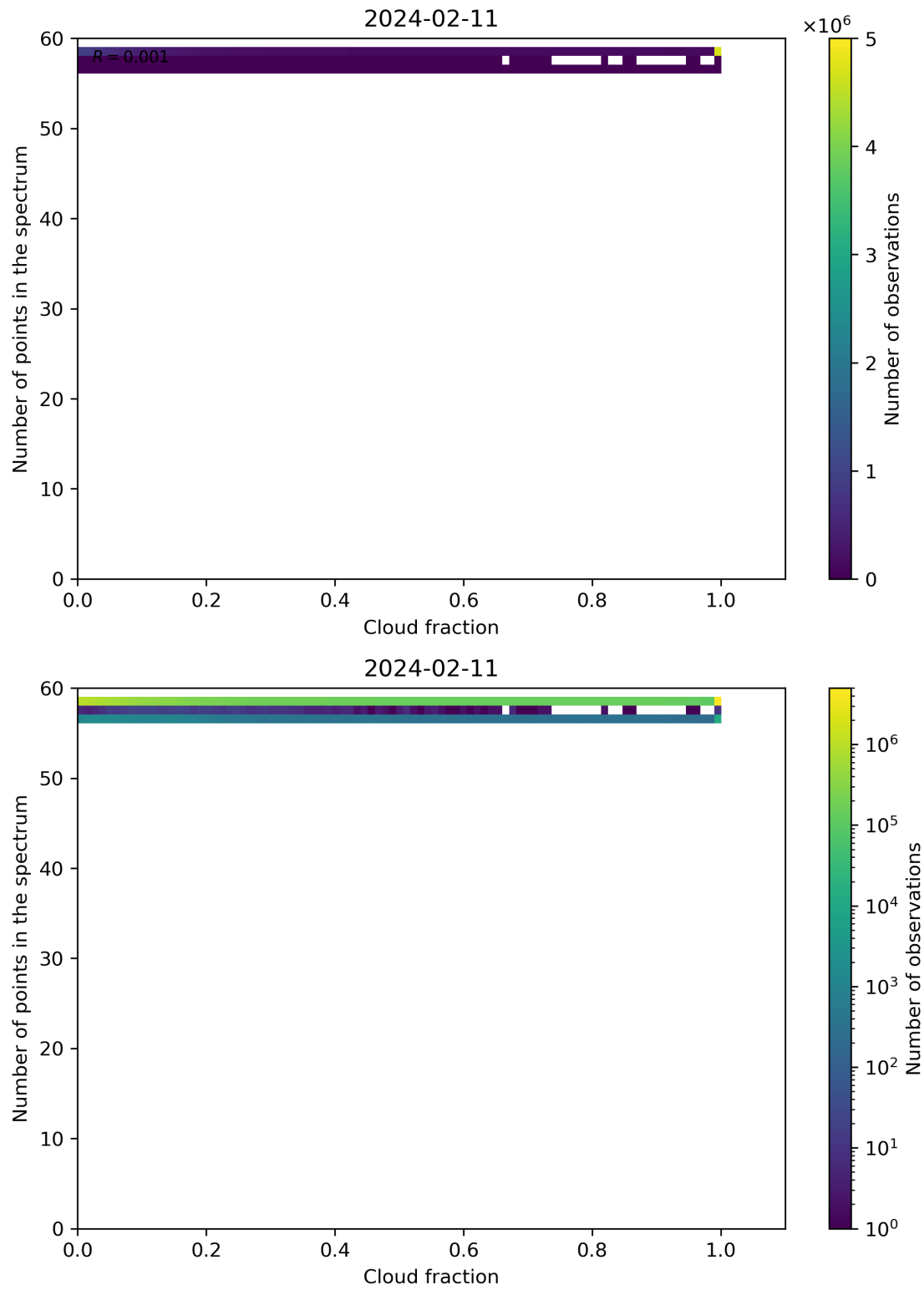
Figure 74: Scatter density plot of “Cloud fraction” against “Number of points in the spectrum” for 2024-02-11 to 2024-02-12.
