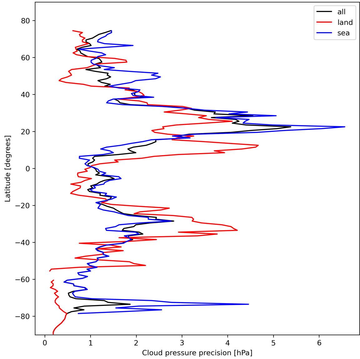
Figure 14: Zonal average of "Cloud pressure precision" for 2024-02-11 to 2024-02-12.
