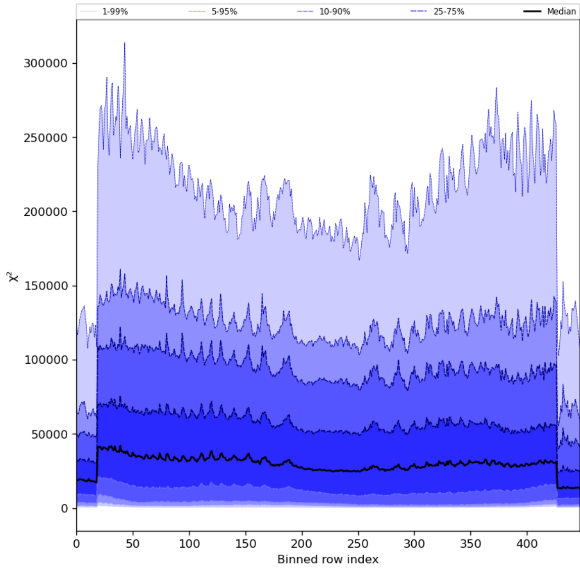
Figure 55: Along track statistics of “ \chi^2 ” for 2024-02-11 to 2024-02-12
