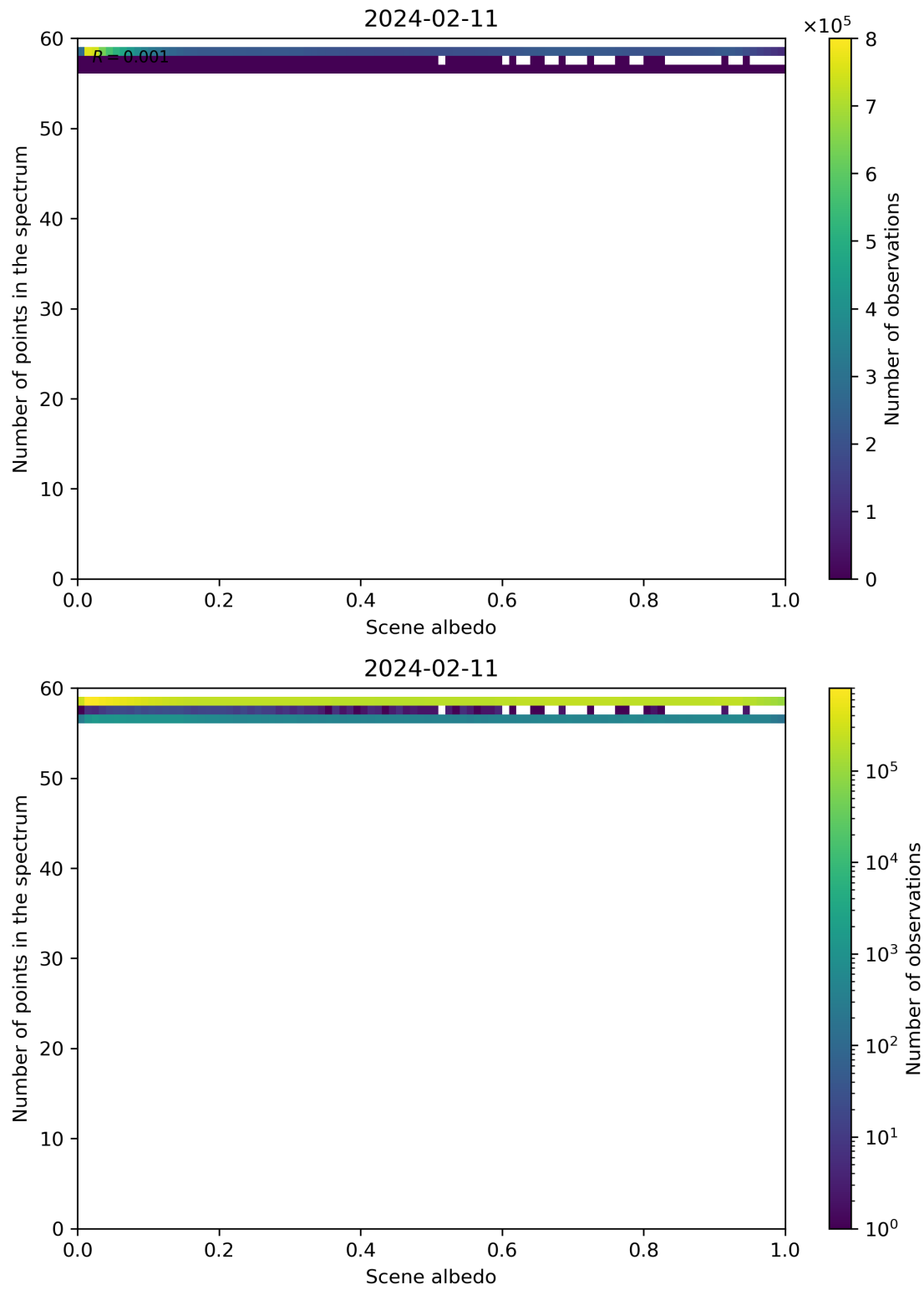
Figure 106: Scatter density plot of “Scene albedo” against “Number of points in the spectrum” for 2024-02-11 to 2024-02-12.
