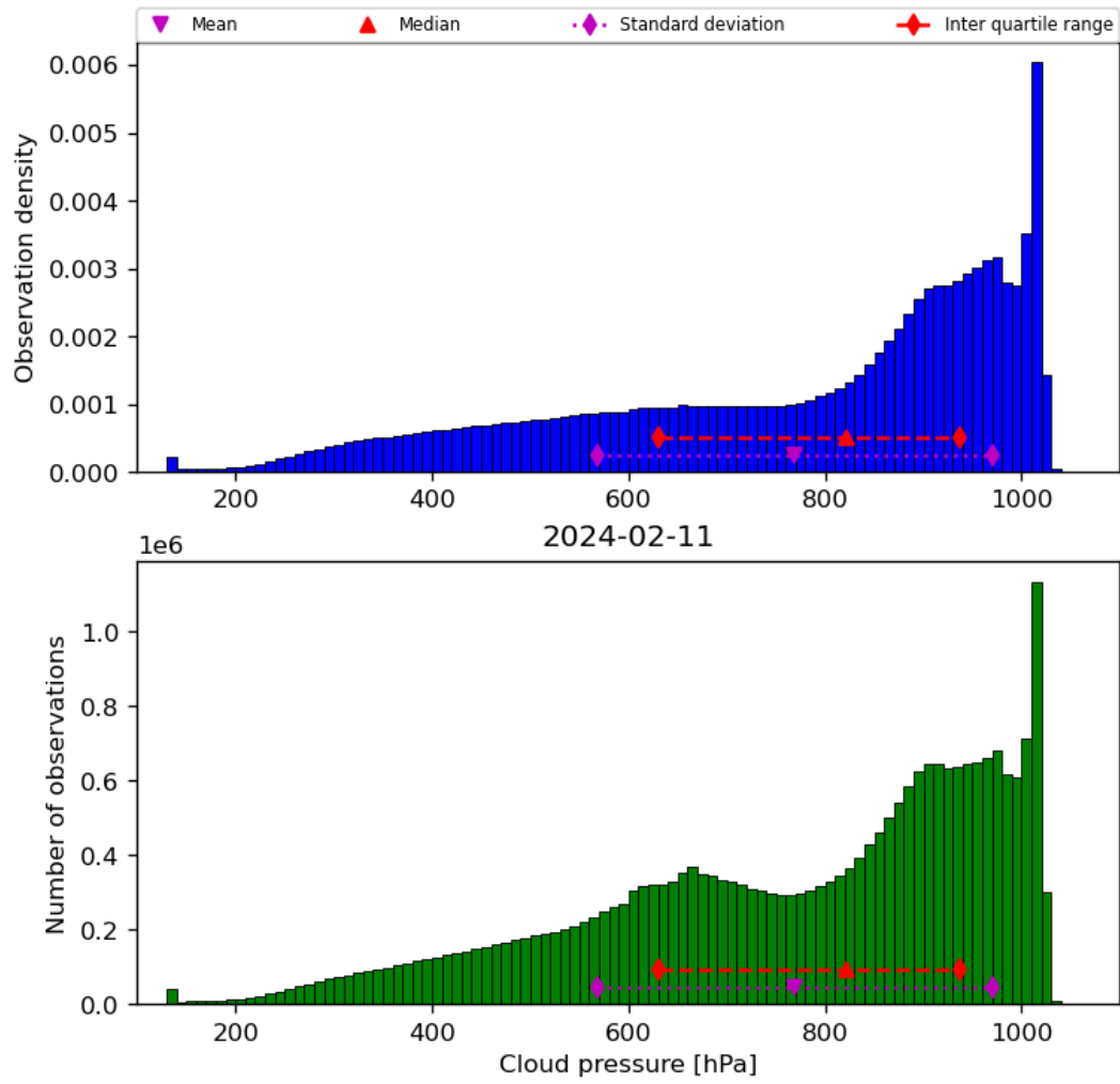
Figure 30: Histogram of “Cloud pressure” for 2024-02-11 to 2024-02-12
