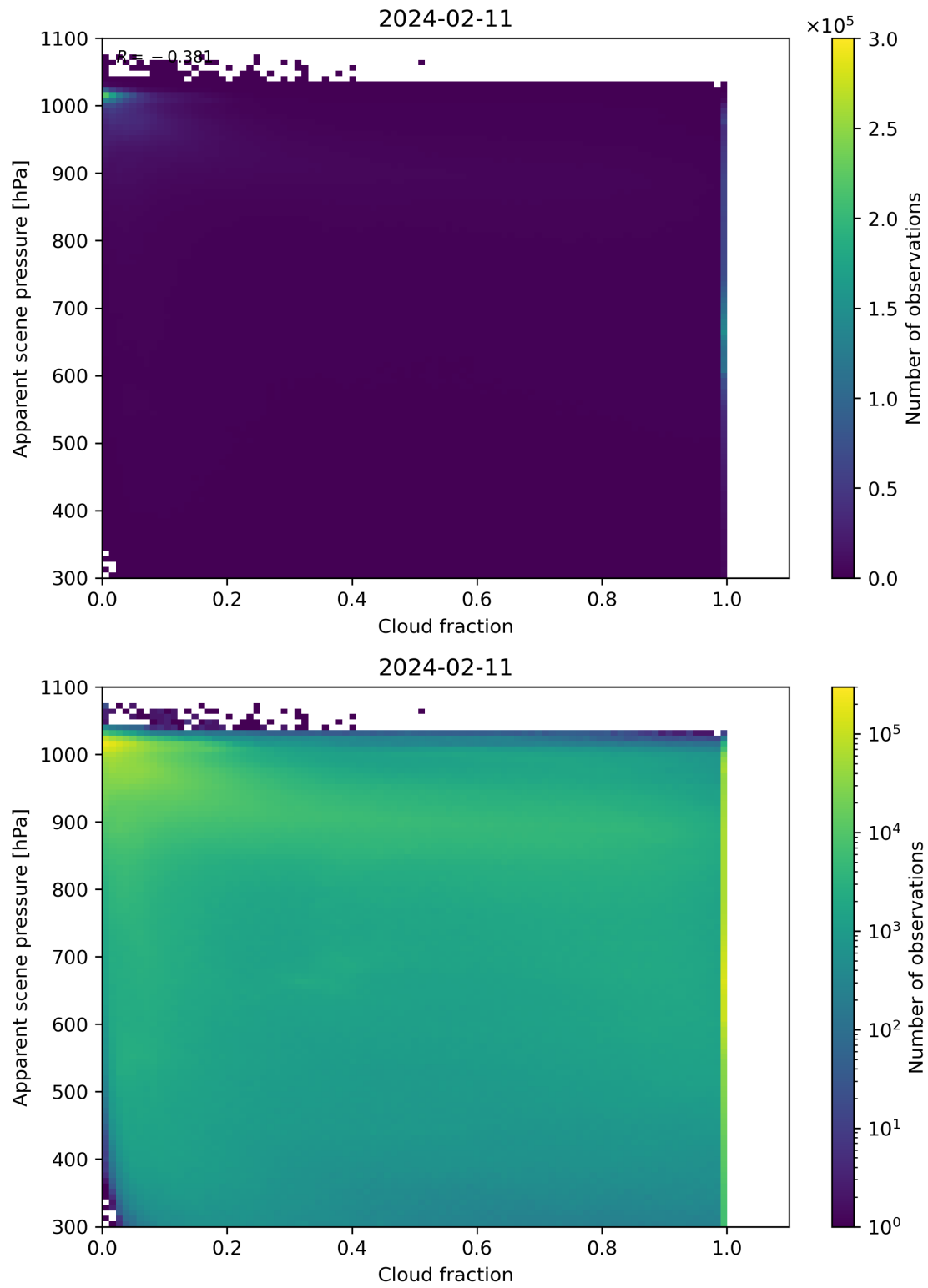
Figure 70: Scatter density plot of “Cloud fraction” against “Apparent scene pressure” for 2024-02-11 to 2024-02-12.
