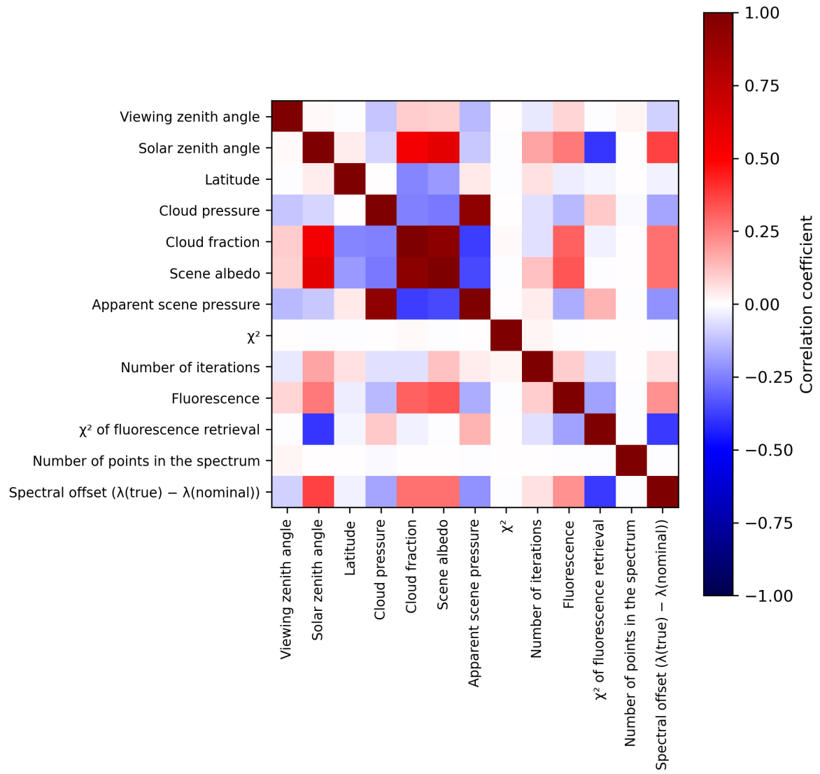
Figure 2: Map of correlation matrix for 2024-02-11 to 2024-02-12.
