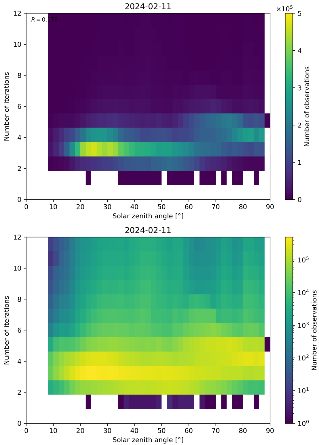
Figure 114: Scatter density plot of “Solar zenith angle” against “Number of iterations” for 2024-02-11 to 2024-02-12.
