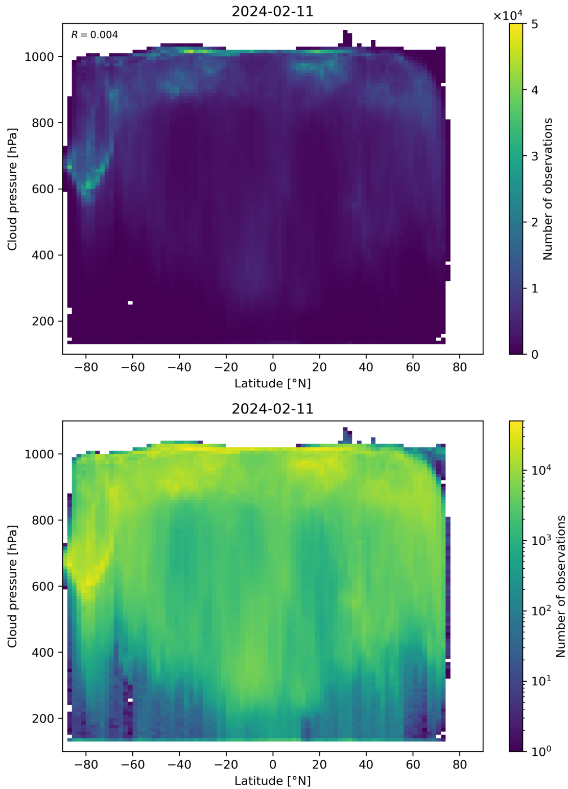
Figure 91: Scatter density plot of “Latitude” against “Cloud pressure” for 2024-02-11 to 2024-02-12.
