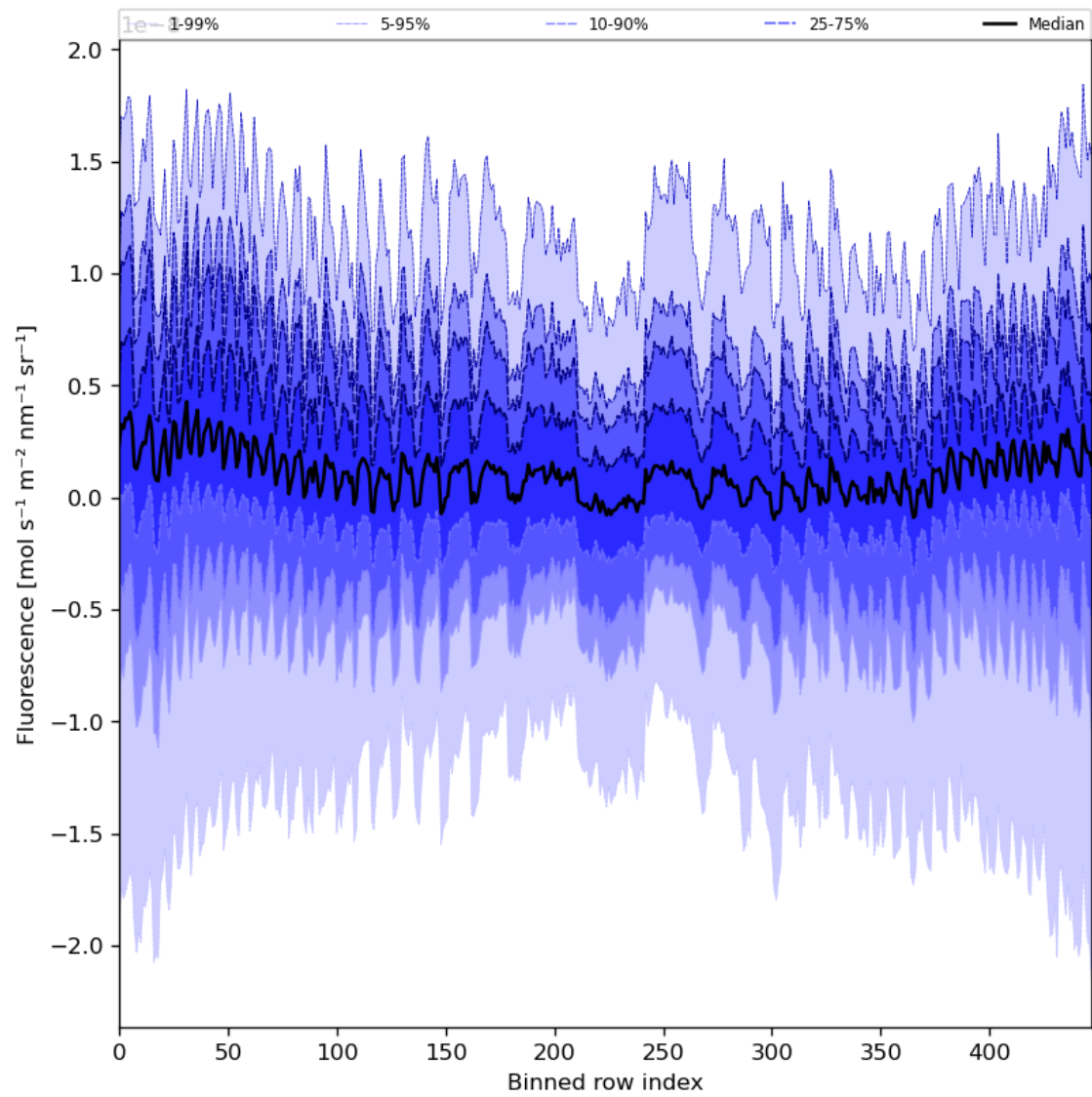
Figure 57: Along track statistics of “Fluorescence” for 2024-02-11 to 2024-02-12
