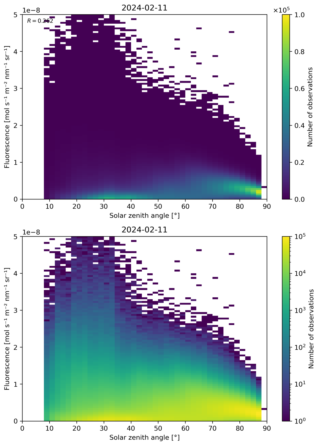
Figure 112: Scatter density plot of “Solar zenith angle” against “Fluorescence” for 2024-02-11 to 2024-02-12.
