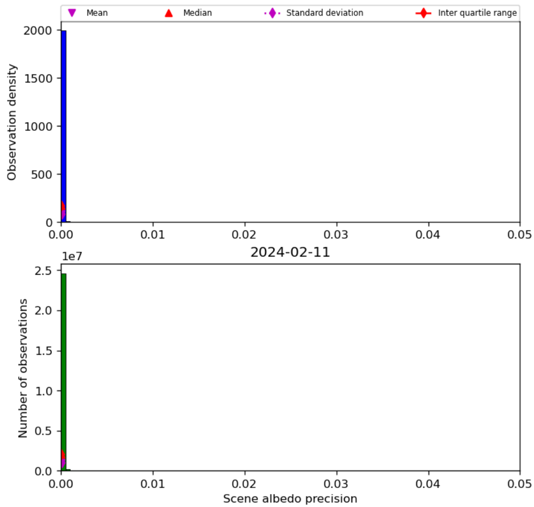
Figure 35: Histogram of “Scene albedo precision” for 2024-02-11 to 2024-02-12
