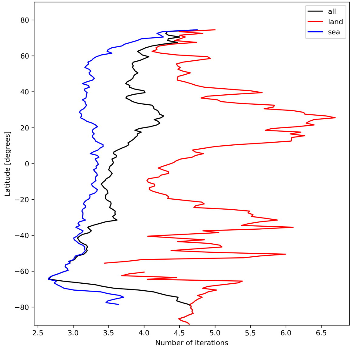
Figure 22: Zonal average of “Number of iterations” for 2024-02-11 to 2024-02-12.
