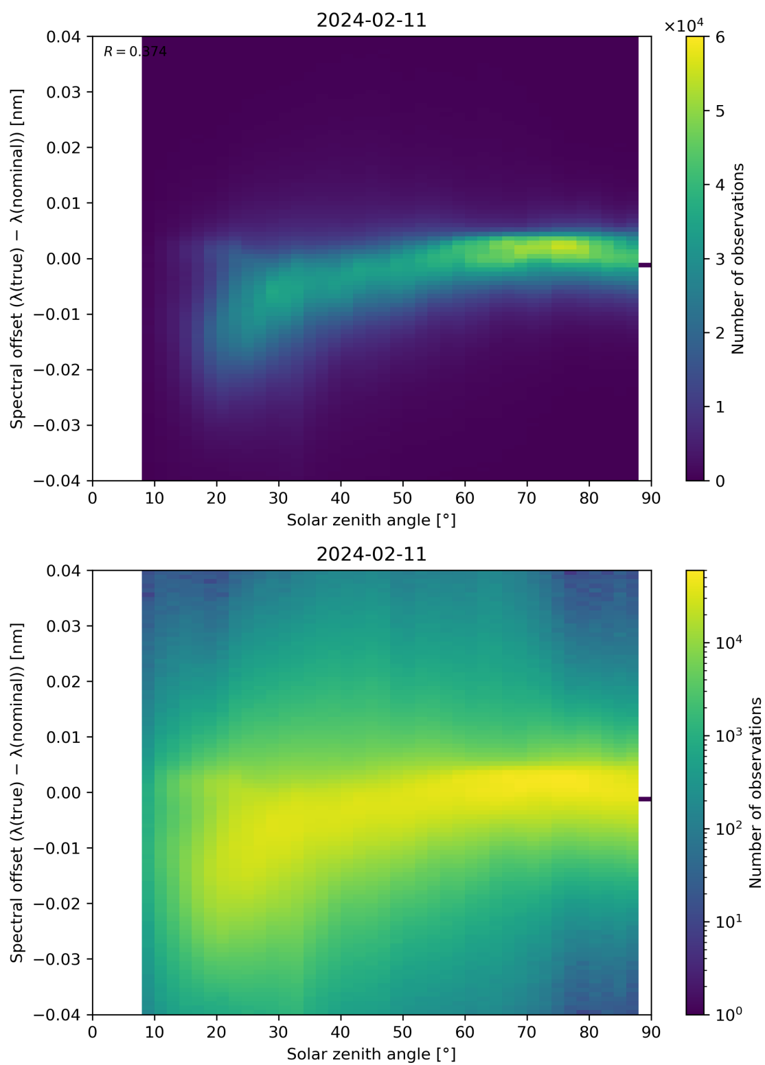
Figure 117: Scatter density plot of “Solar zenith angle” against “Spectral offset ( \lambda(\text{true}) - \lambda(\text{nominal}) )” for 2024-02-11 to 2024-02-12.
