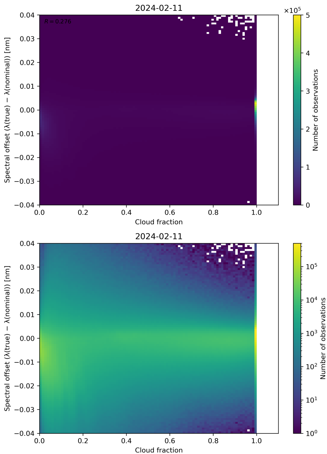
Figure 76: Scatter density plot of “Cloud fraction” against “Spectral offset ( \lambda(\text{true}) - \lambda(\text{nominal}) )” for 2024-02-11 to 2024-02-12.
