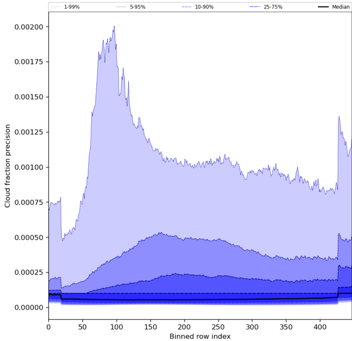
Figure 50: Along track statistics of “Cloud fraction precision” for 2024-02-11 to 2024-02-12
