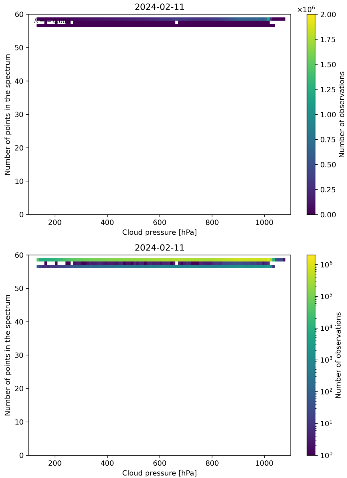
Figure 82: Scatter density plot of “Cloud pressure” against “Number of points in the spectrum” for 2024-02-11 to 2024-02-12.
