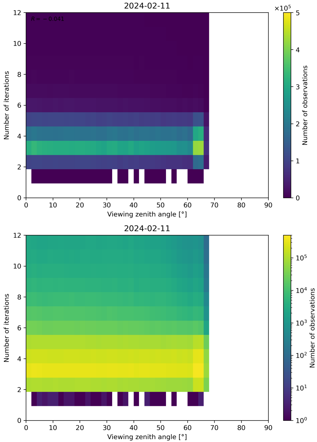
Figure 124: Scatter density plot of “Viewing zenith angle” against “Number of iterations” for 2024-02-11 to 2024-02-12.
