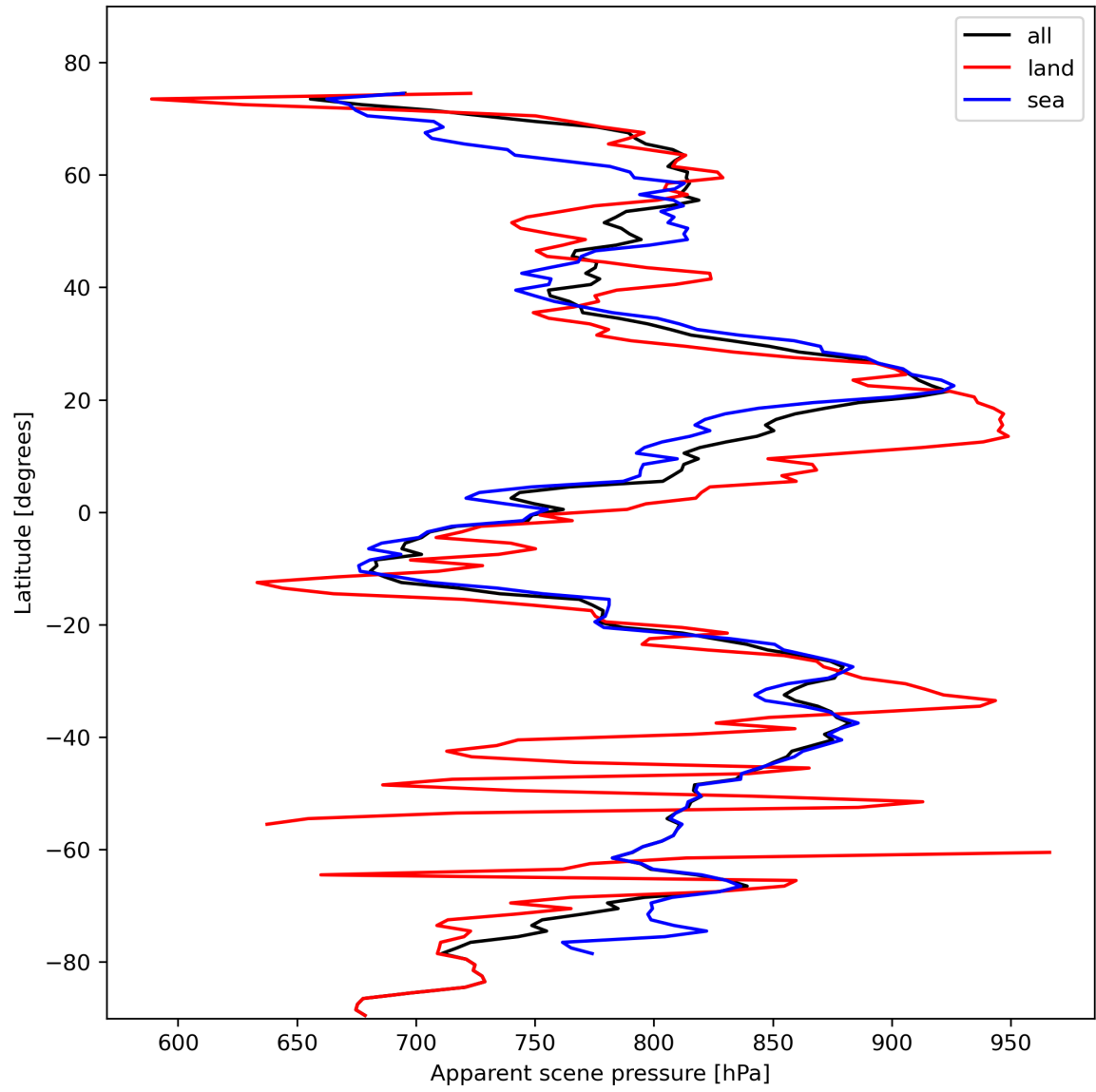
Figure 19: Zonal average of “Apparent scene pressure” for 2024-02-11 to 2024-02-12.
