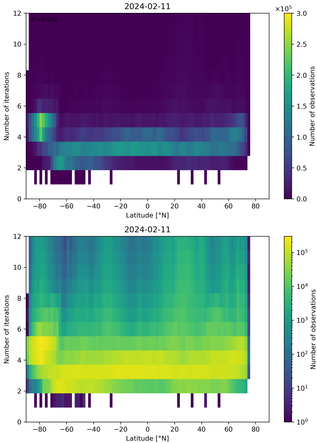
Figure 93: Scatter density plot of “Latitude” against “Number of iterations” for 2024-02-11 to 2024-02-12.
