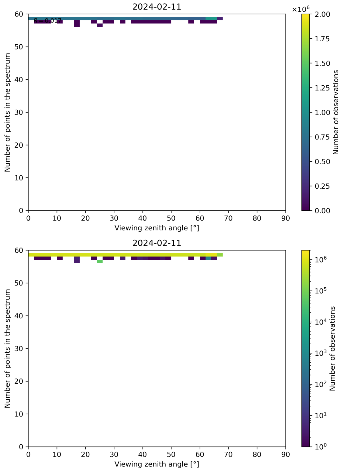
Figure 125: Scatter density plot of “Viewing zenith angle” against “Number of points in the spectrum” for 2024-02-11 to 2024-02-12.
