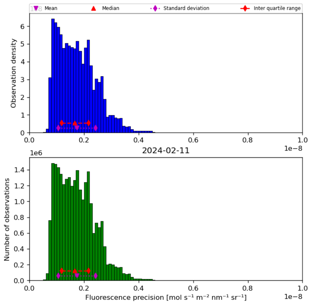
Figure 41: Histogram of “Fluorescence precision” for 2024-02-11 to 2024-02-12
