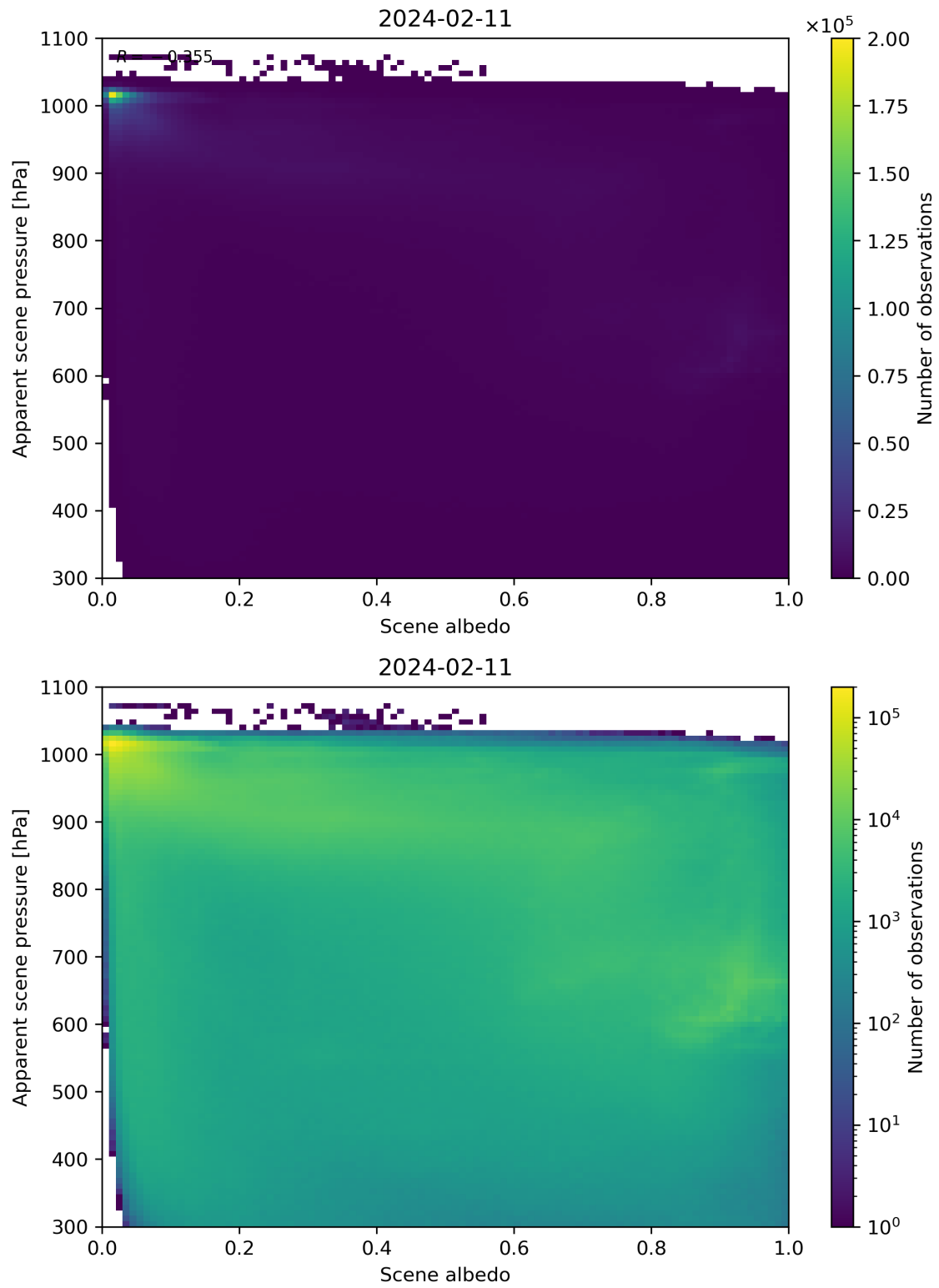
Figure 102: Scatter density plot of “Scene albedo” against “Apparent scene pressure” for 2024-02-11 to 2024-02-12.
