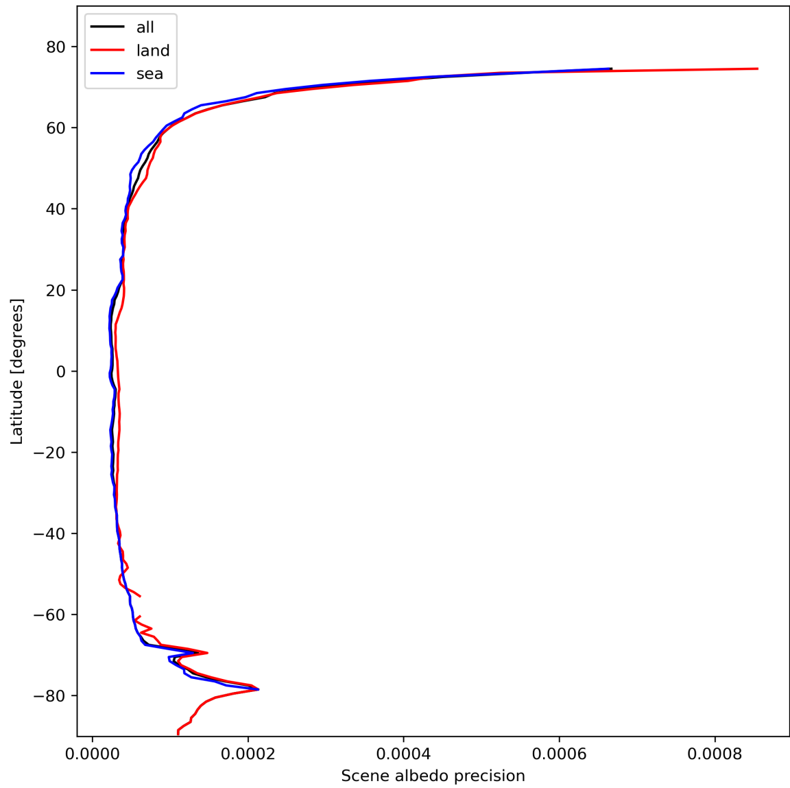
Figure 18: Zonal average of “Scene albedo precision” for 2024-02-11 to 2024-02-12.
