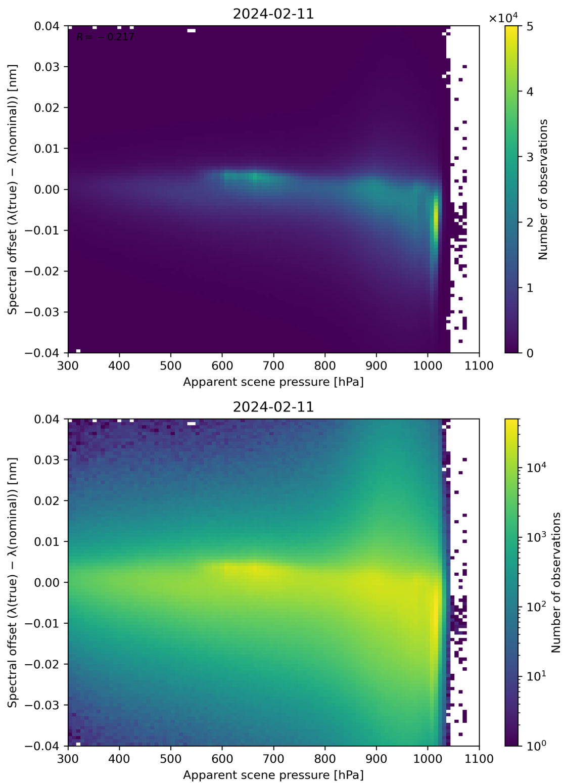
Figure 67: Scatter density plot of “Apparent scene pressure” against “Spectral offset ( \lambda(\text{true}) - \lambda(\text{nominal}) )” for 2024-02-11 to 2024-02-12.
