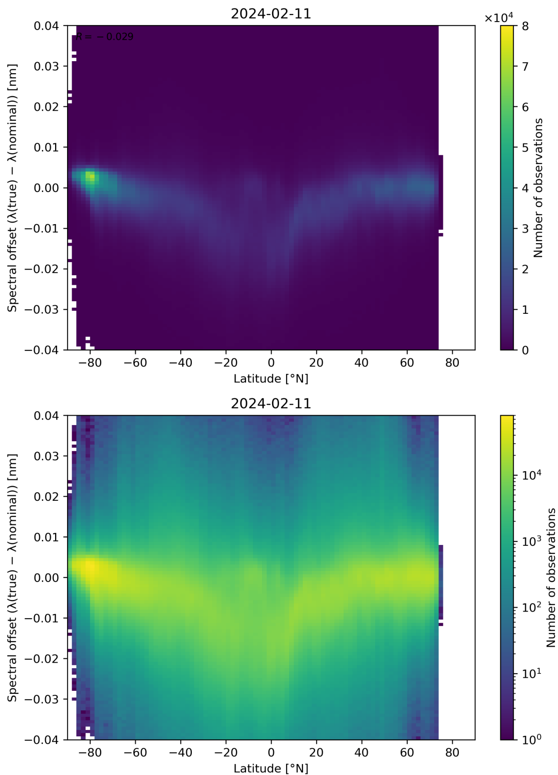
Figure 96: Scatter density plot of “Latitude” against “Spectral offset ( \lambda(\text{true}) - \lambda(\text{nominal}) )” for 2024-02-11 to 2024-02-12.
