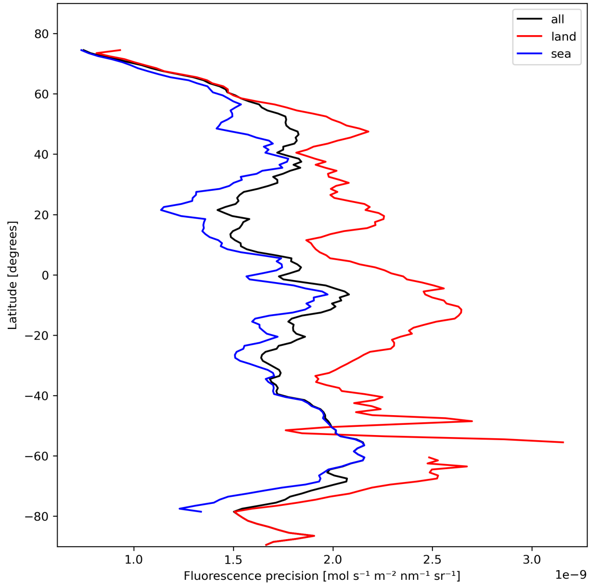
Figure 24: Zonal average of “Fluorescence precision” for 2024-02-11 to 2024-02-12.
