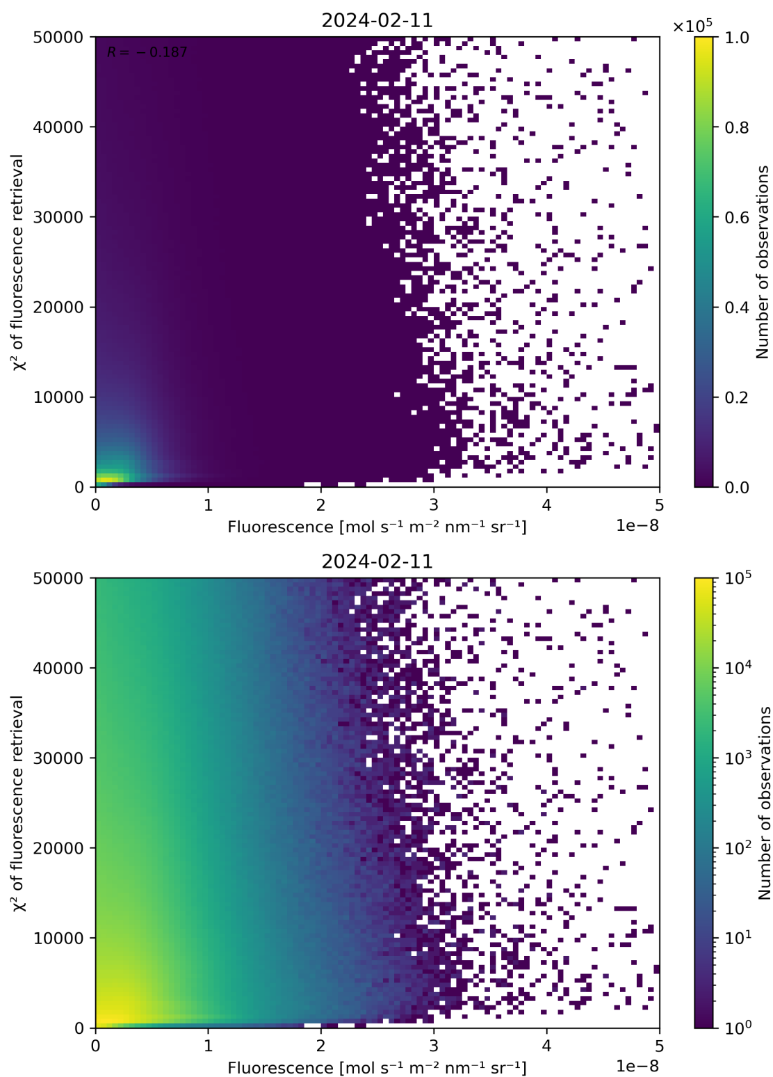
Figure 85: Scatter density plot of “Fluorescence” against “ \chi^2 of fluorescence retrieval” for 2024-02-11 to 2024-02-12.
