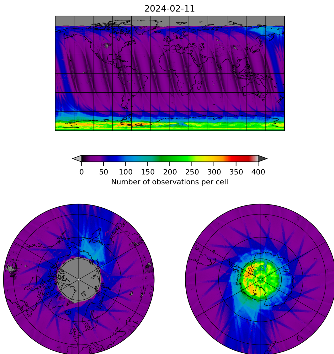
Figure 11: Map of the number of observations for 2024-02-11 to 2024-02-12
