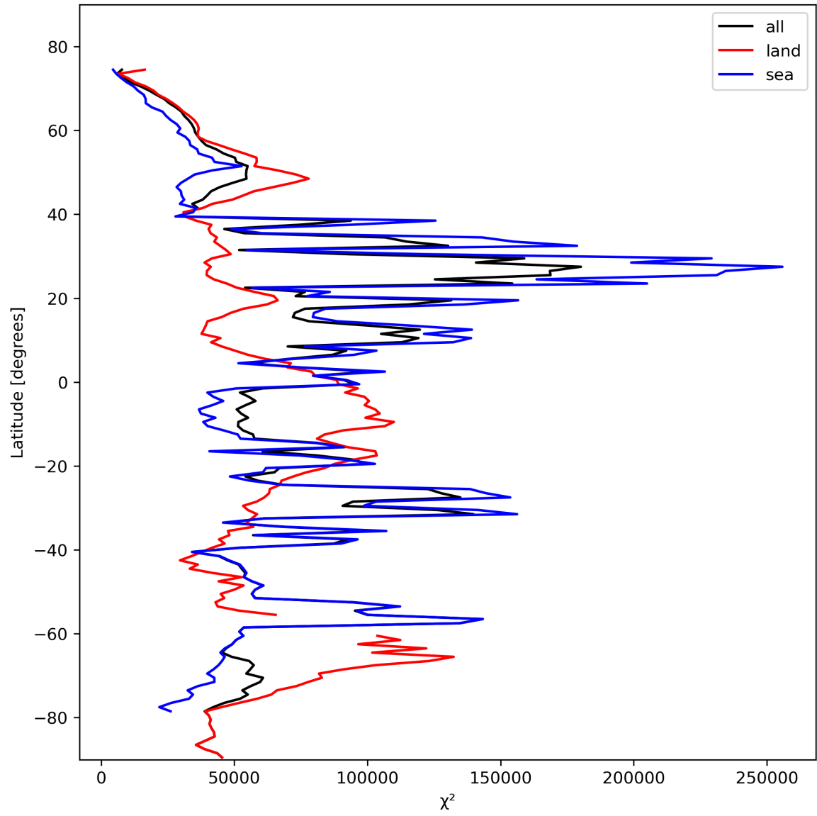
Figure 21: Zonal average of “ \chi^2 ” for 2024-02-11 to 2024-02-12.
