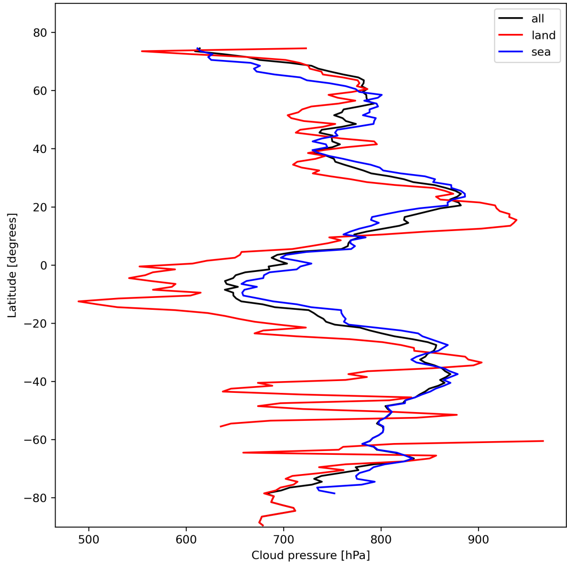
Figure 13: Zonal average of “Cloud pressure” for 2024-02-11 to 2024-02-12.
