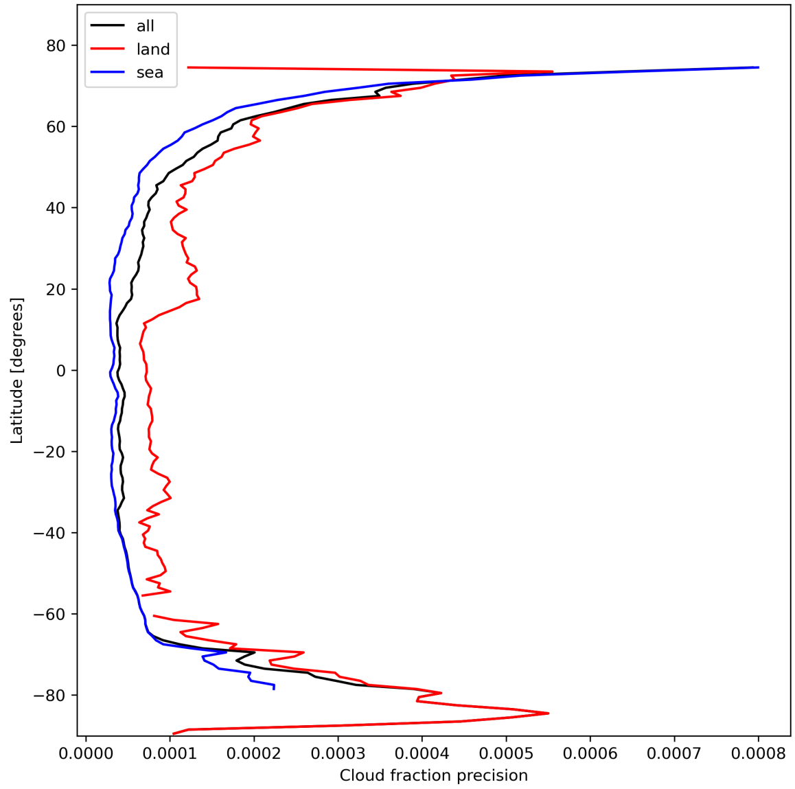
Figure 16: Zonal average of “Cloud fraction precision” for 2024-02-11 to 2024-02-12.
