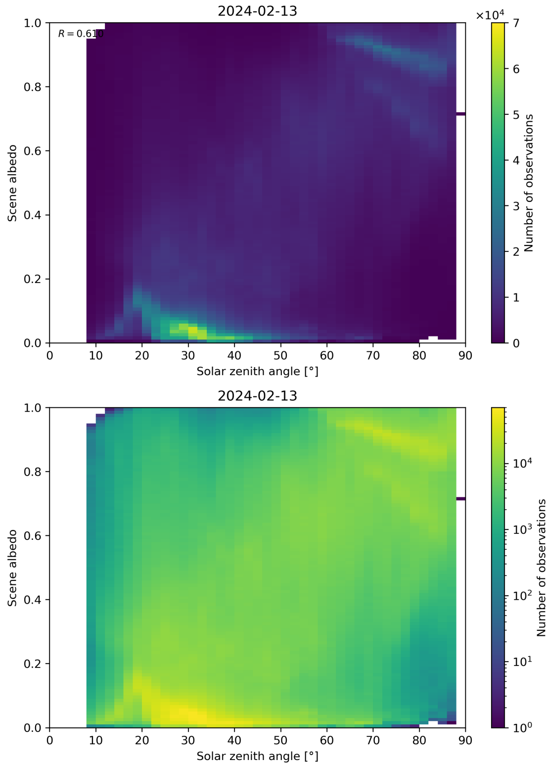
Figure 116: Scatter density plot of “Solar zenith angle” against “Scene albedo” for 2024-02-12 to 2024-02-14.
