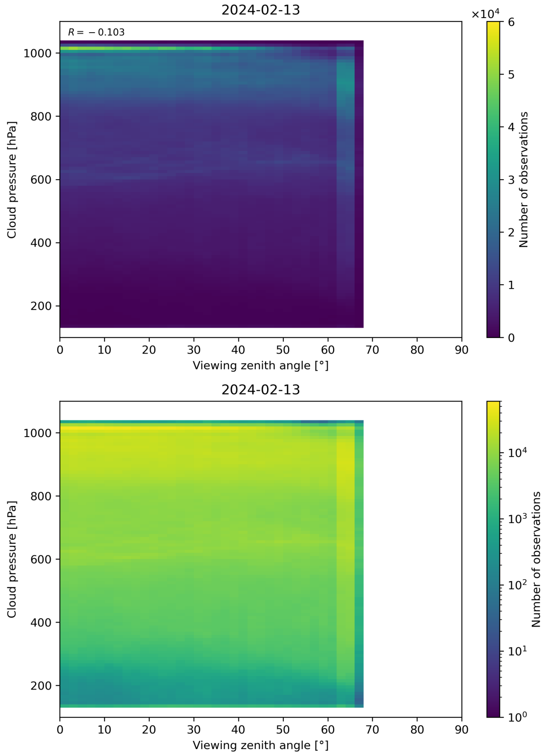
Figure 121: Scatter density plot of “Viewing zenith angle” against “Cloud pressure” for 2024-02-12 to 2024-02-14.
