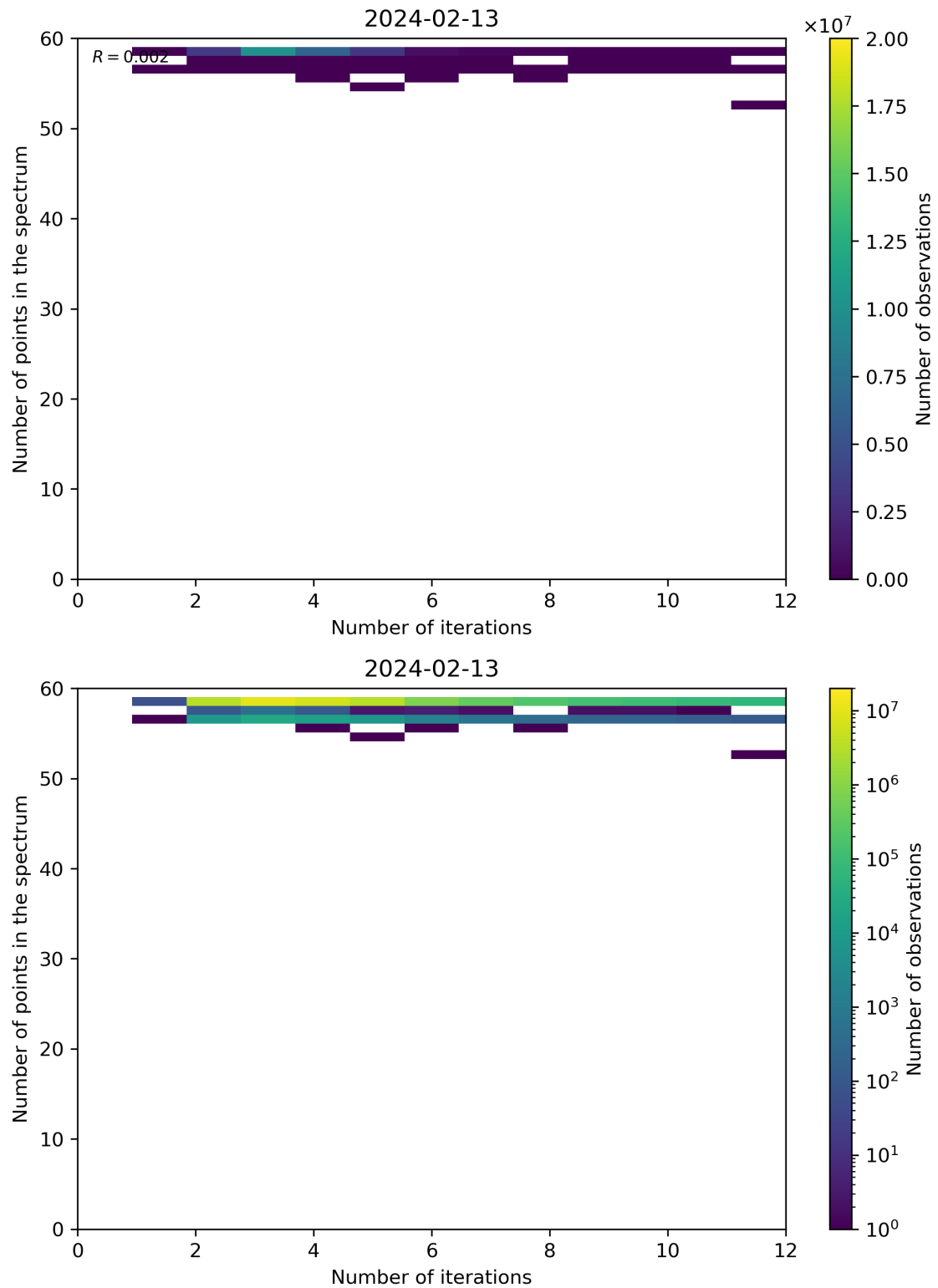
Figure 99: Scatter density plot of “Number of iterations” against “Number of points in the spectrum” for 2024-02-12 to 2024-02-14.
