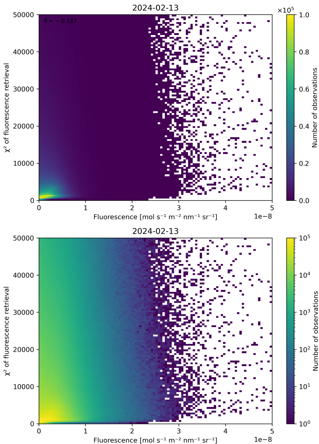
Figure 85: Scatter density plot of “Fluorescence” against “ \chi^2 of fluorescence retrieval” for 2024-02-12 to 2024-02-14.
