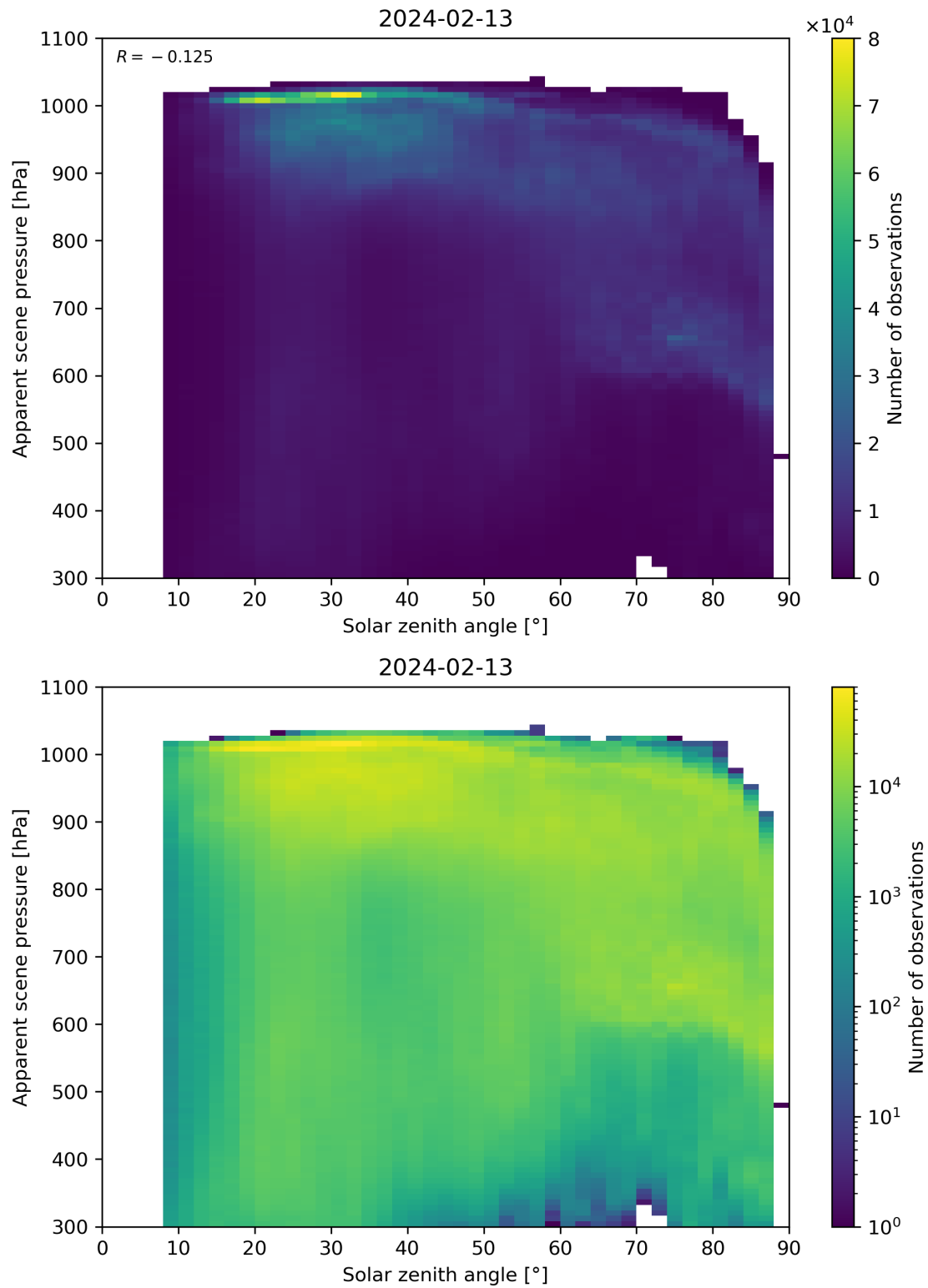
Figure 108: Scatter density plot of “Solar zenith angle” against “Apparent scene pressure” for 2024-02-12 to 2024-02-14.
