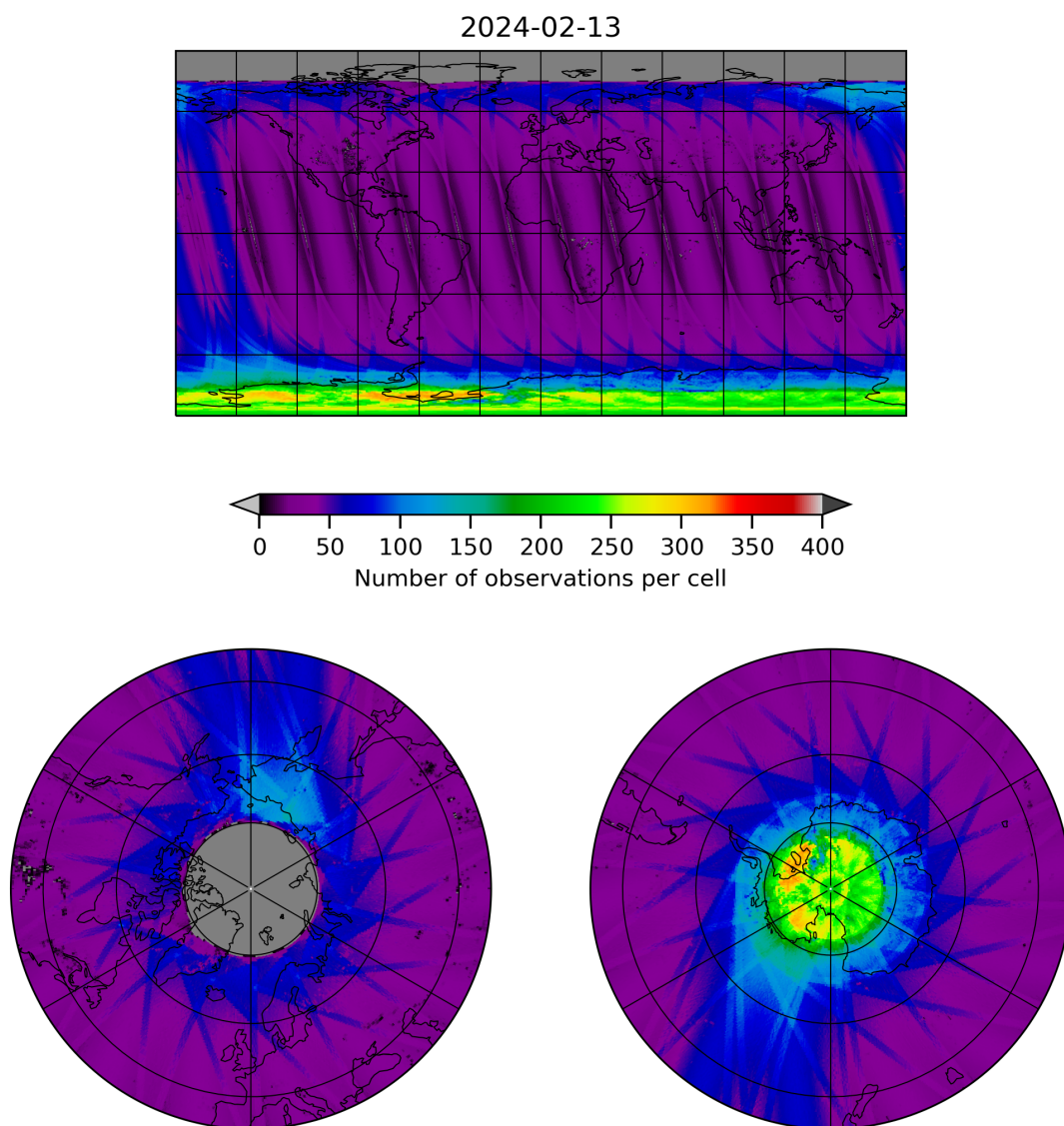
Figure 11: Map of the number of observations for 2024-02-12 to 2024-02-14
