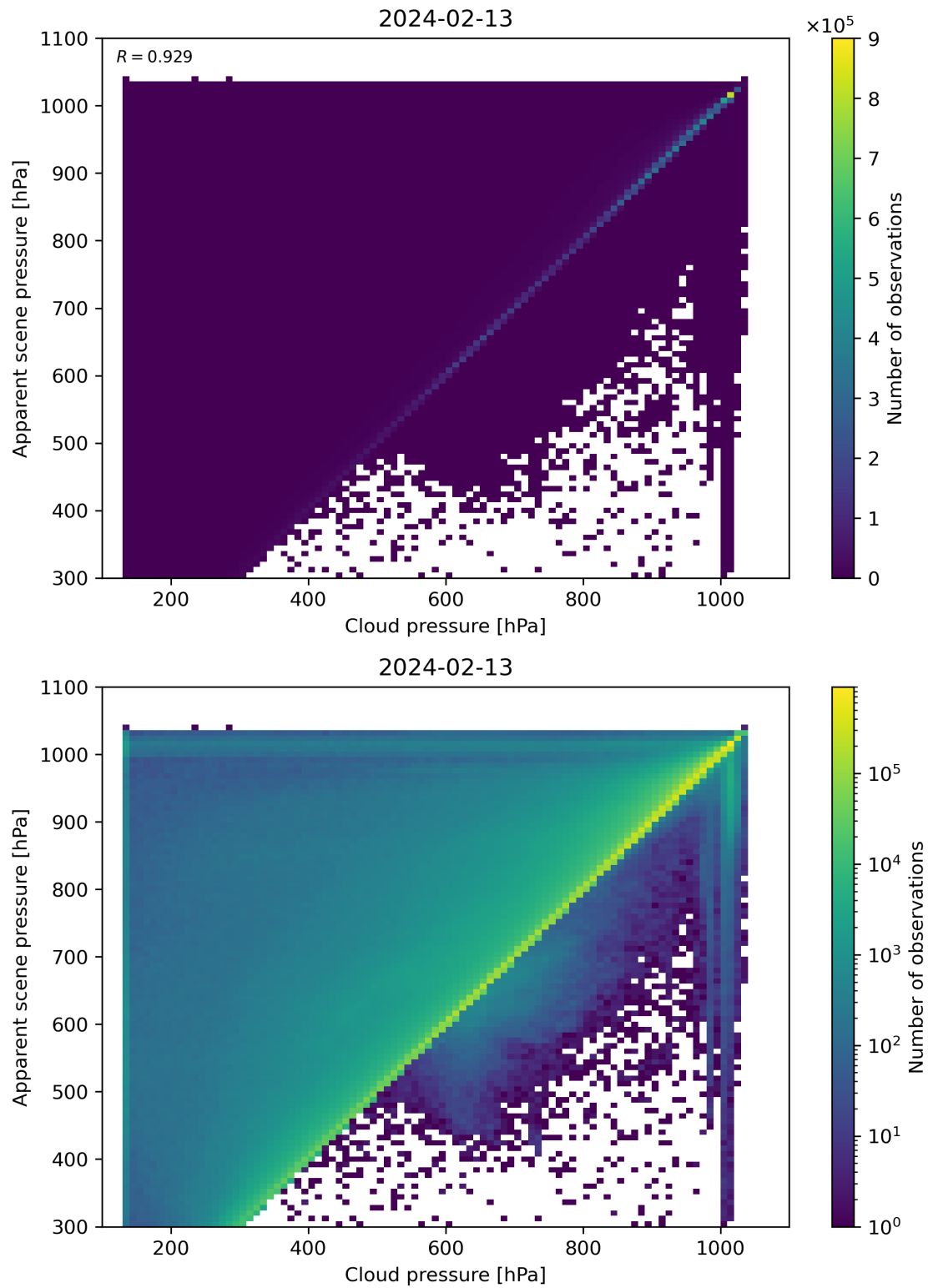
Figure 77: Scatter density plot of “Cloud pressure” against “Apparent scene pressure” for 2024-02-12 to 2024-02-14.
