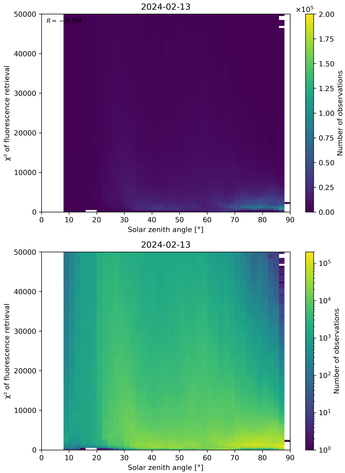
Figure 109: Scatter density plot of “Solar zenith angle” against “ \chi^2 of fluorescence retrieval” for 2024-02-12 to 2024-02-14.
