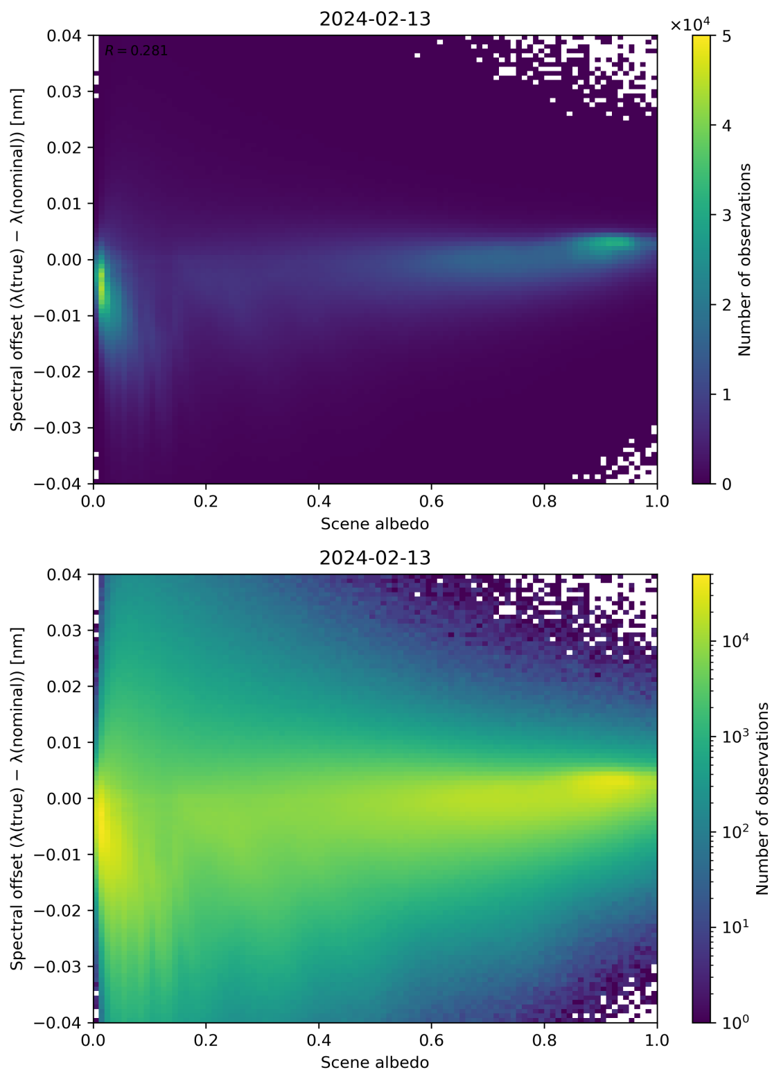
Figure 107: Scatter density plot of “Scene albedo” against “Spectral offset ( \lambda(\text{true}) - \lambda(\text{nominal}) )” for 2024-02-12 to 2024-02-14.
