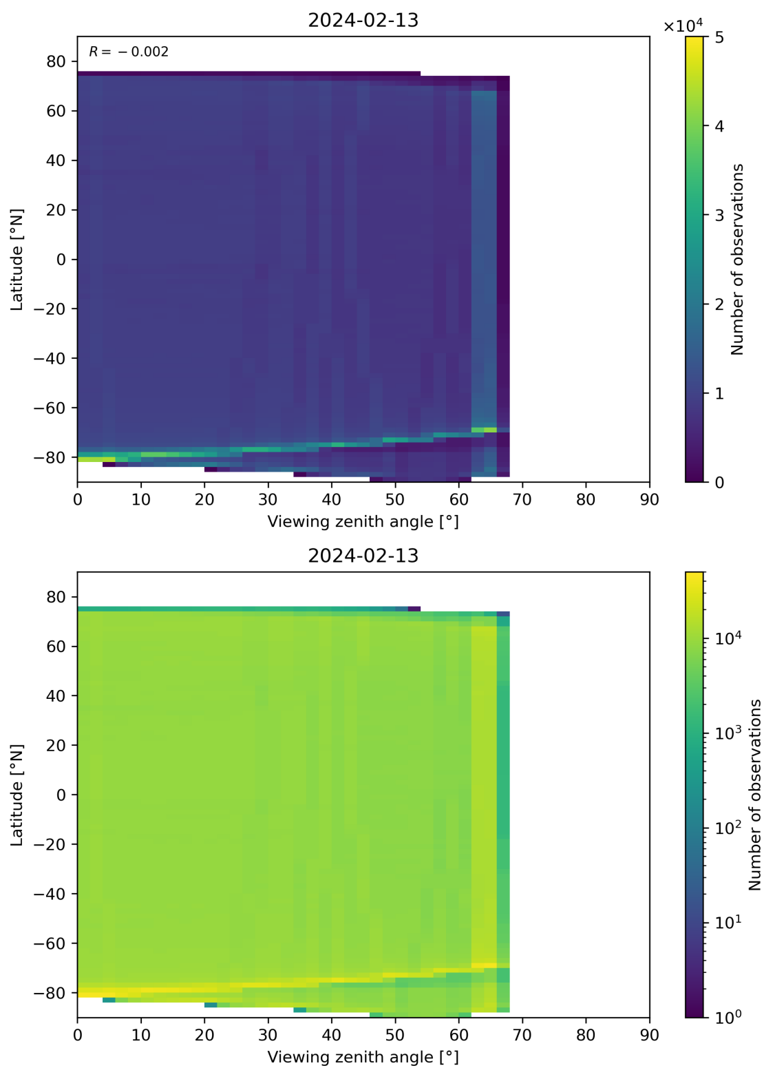
Figure 123: Scatter density plot of “Viewing zenith angle” against “Latitude” for 2024-02-12 to 2024-02-14.
