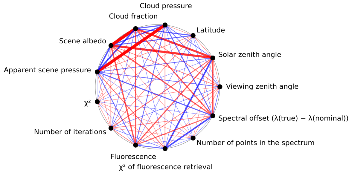
Figure 1: Map of correlation graph for 2024-02-12 to 2024-02-14.
