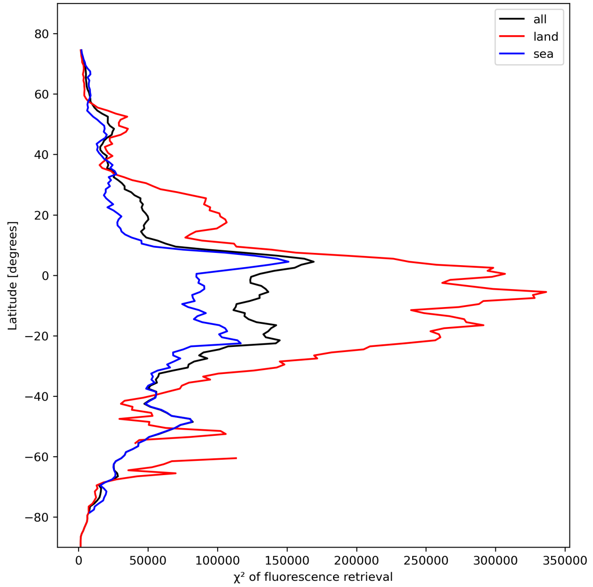
Figure 25: Zonal average of “ \chi^2 of fluorescence retrieval” for 2024-02-12 to 2024-02-14.
