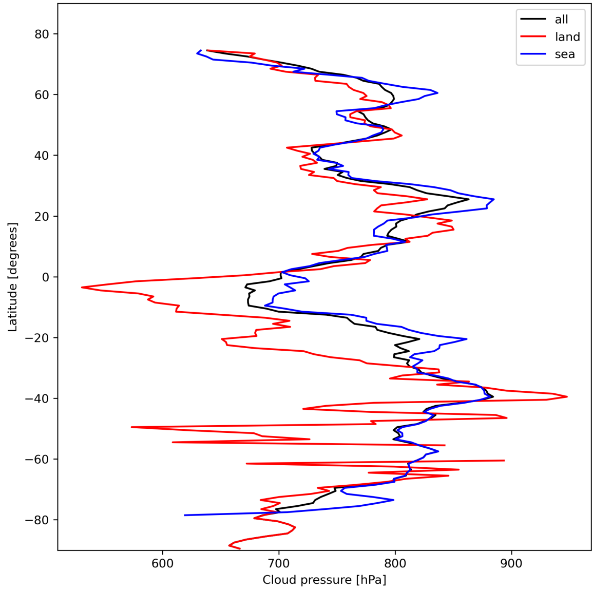
Figure 13: Zonal average of “Cloud pressure” for 2024-02-12 to 2024-02-14.
