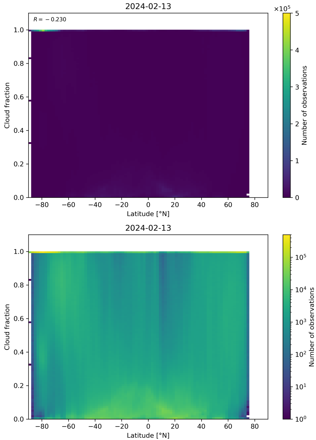
Figure 90: Scatter density plot of “Latitude” against “Cloud fraction” for 2024-02-12 to 2024-02-14.
