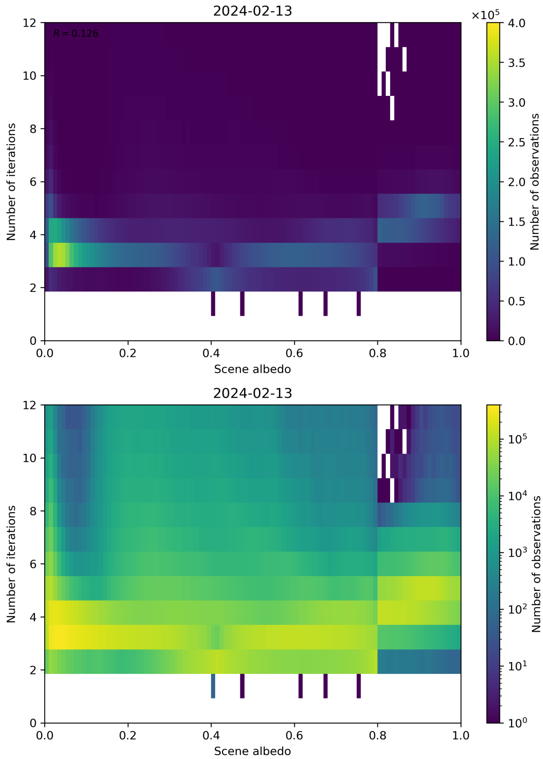
Figure 105: Scatter density plot of “Scene albedo” against “Number of iterations” for 2024-02-12 to 2024-02-14.
