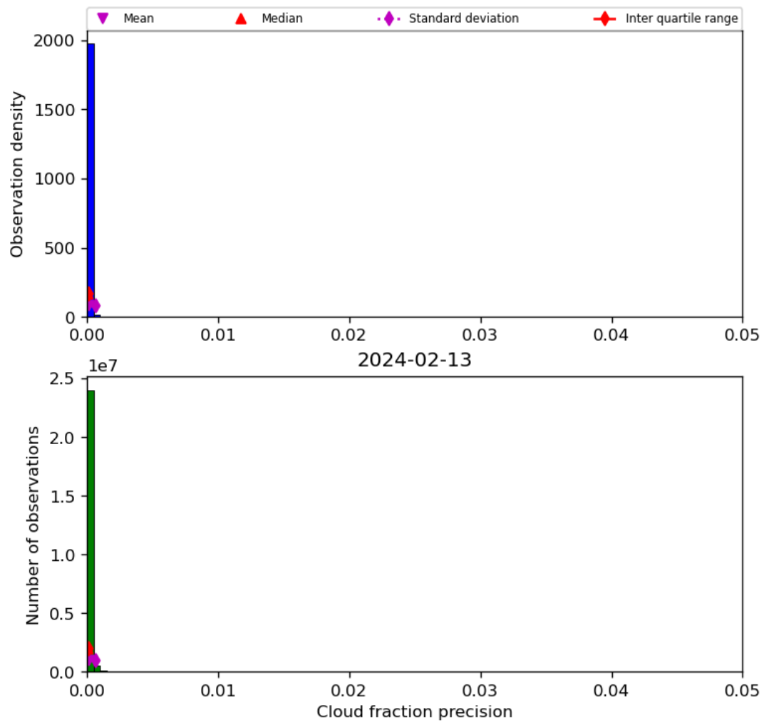
Figure 33: Histogram of “Cloud fraction precision” for 2024-02-12 to 2024-02-14
