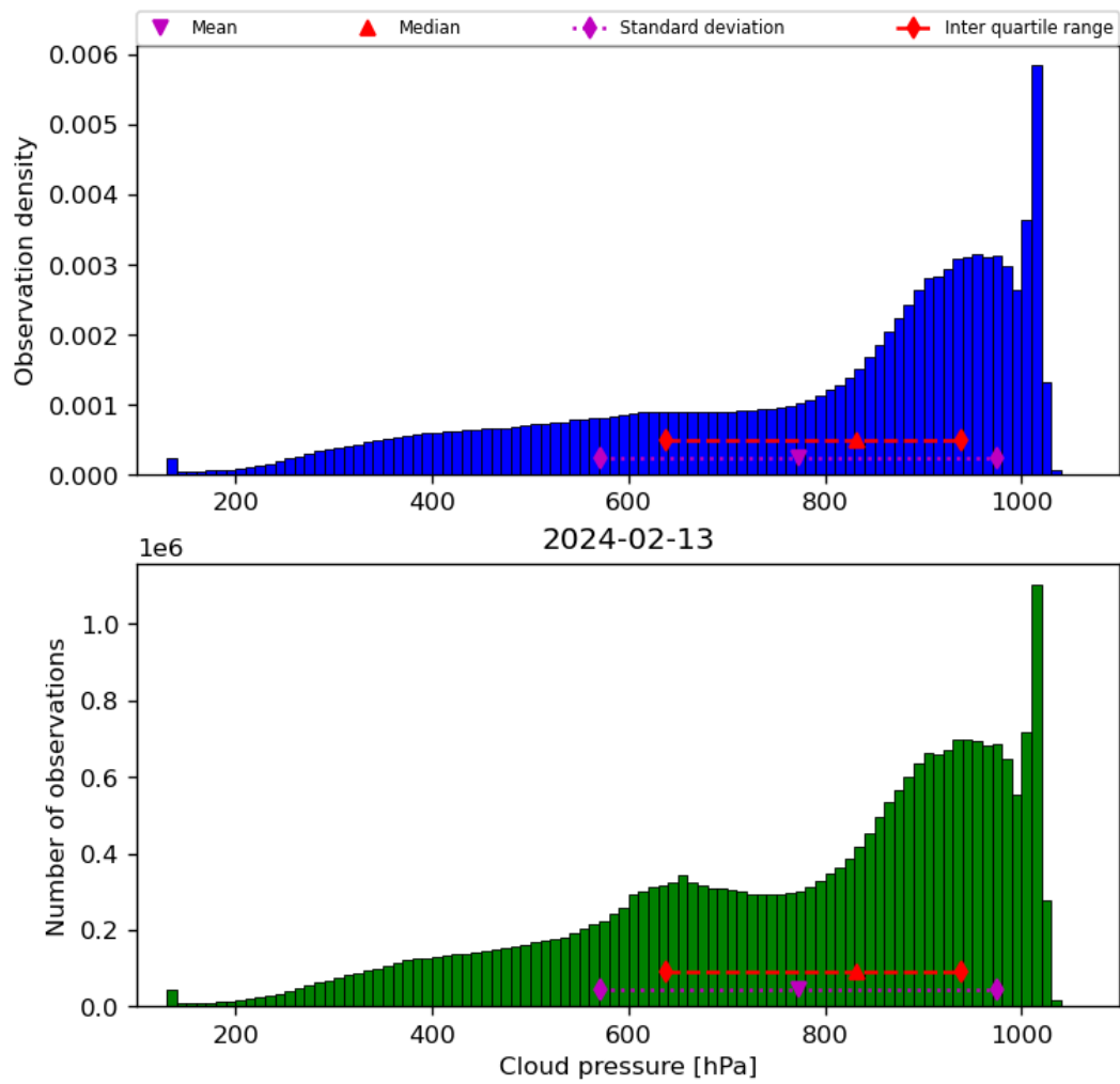
Figure 30: Histogram of “Cloud pressure” for 2024-02-12 to 2024-02-14
