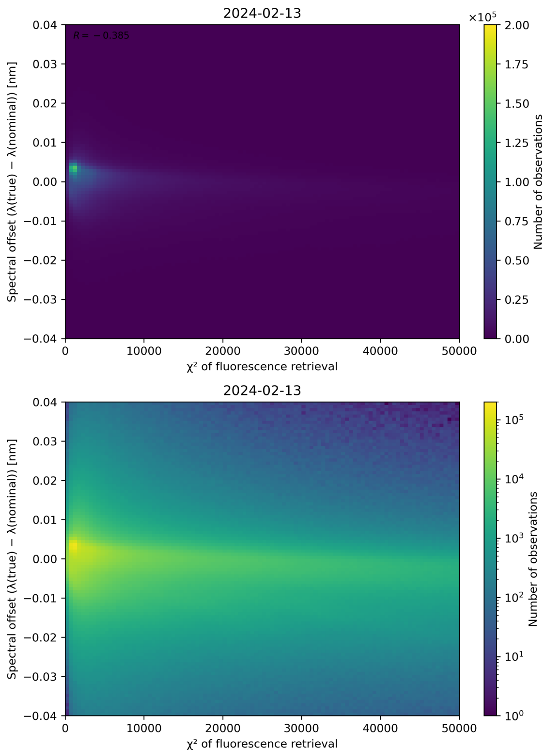
Figure 69: Scatter density plot of “ \chi^2 of fluorescence retrieval” against “Spectral offset ( \lambda(\text{true}) - \lambda(\text{nominal}) )” for 2024-02-12 to 2024-02-14.
