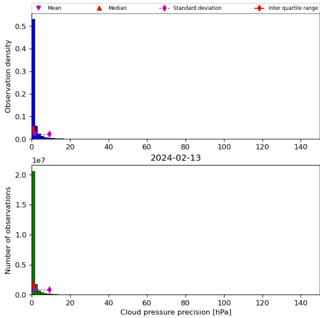
Figure 31: Histogram of “Cloud pressure precision” for 2024-02-12 to 2024-02-14
