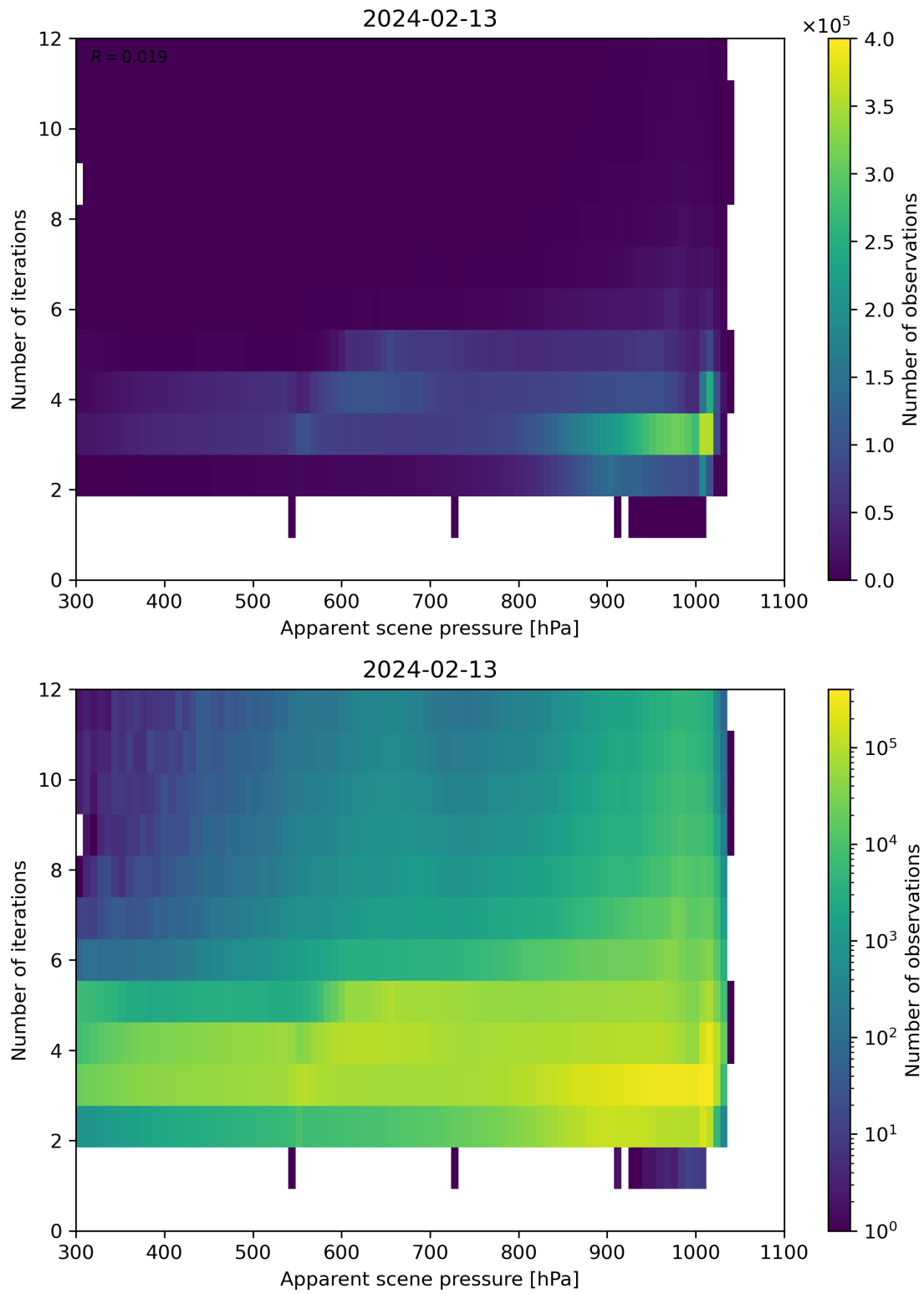
Figure 65: Scatter density plot of “Apparent scene pressure” against “Number of iterations” for 2024-02-12 to 2024-02-14.
