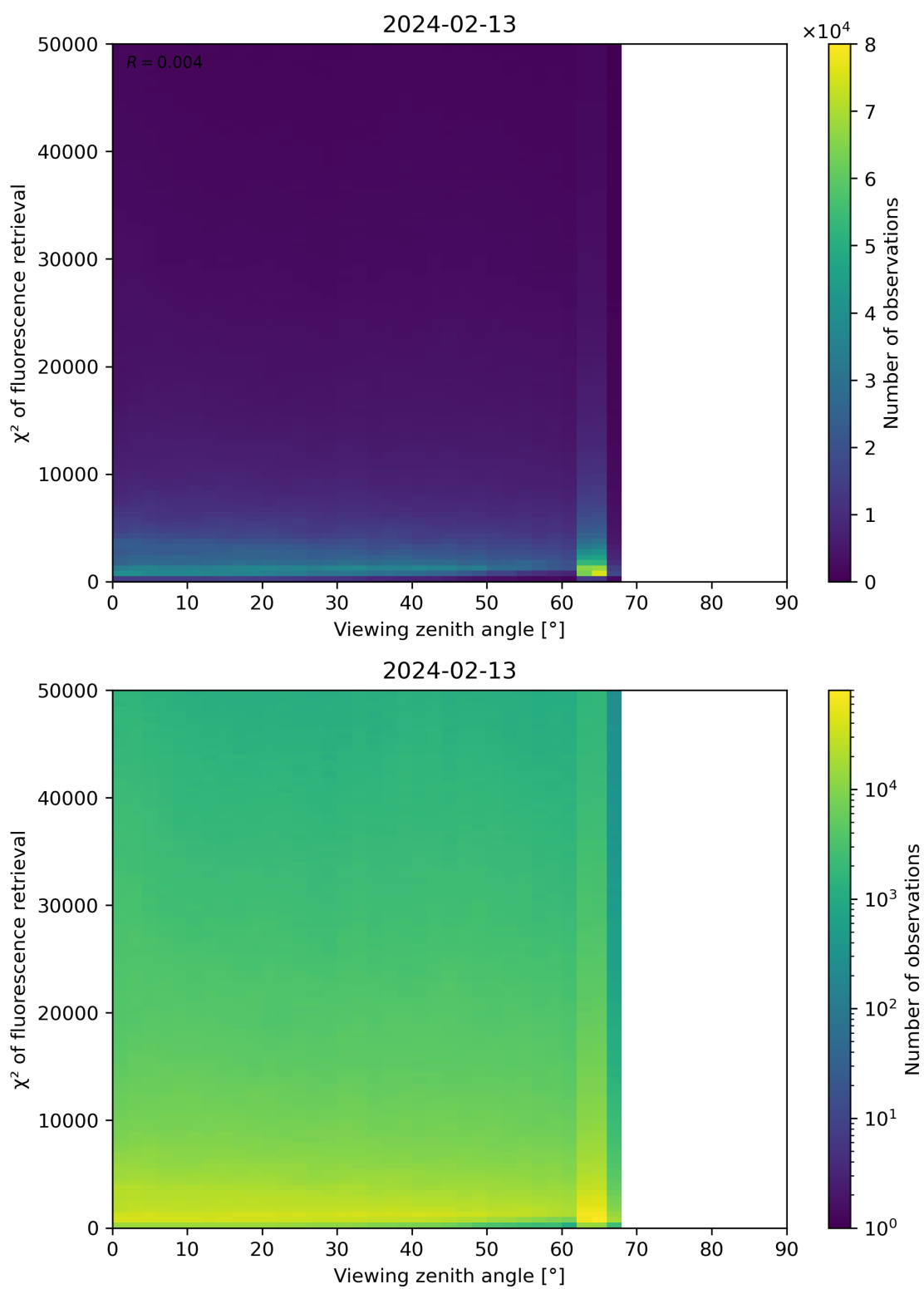
Figure 119: Scatter density plot of “Viewing zenith angle” against “ \chi^2 of fluorescence retrieval” for 2024-02-12 to 2024-02-14.
