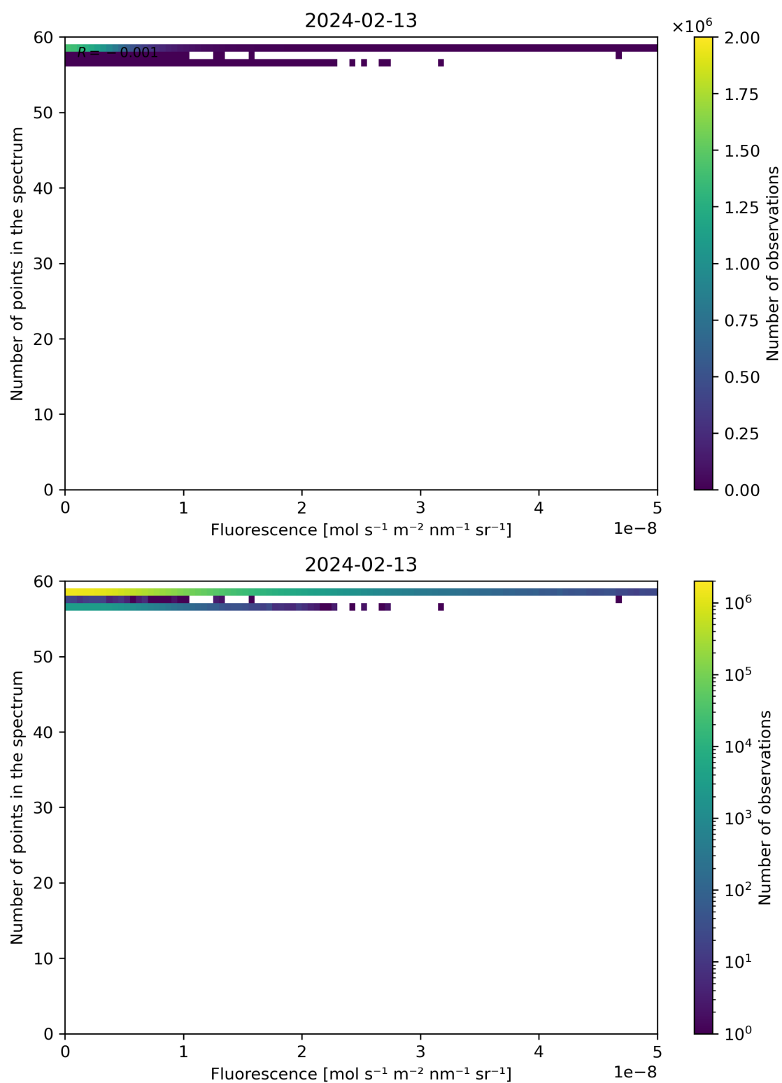
Figure 86: Scatter density plot of “Fluorescence” against “Number of points in the spectrum” for 2024-02-12 to 2024-02-14.
