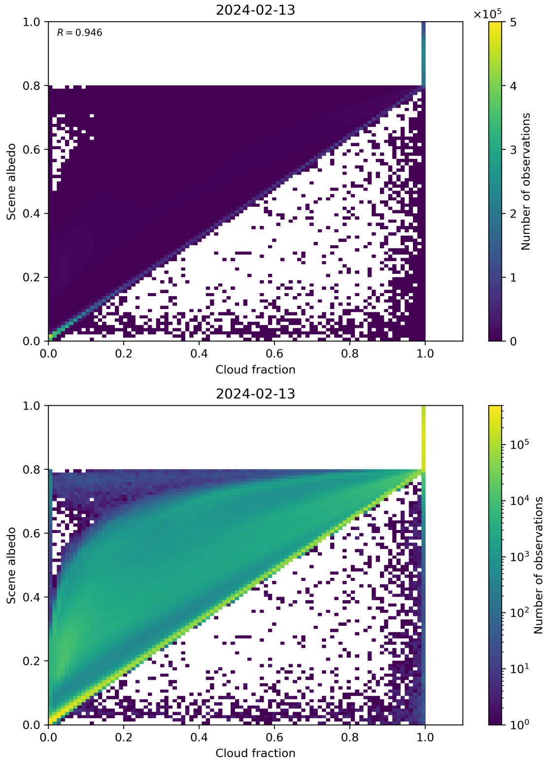
Figure 75: Scatter density plot of “Cloud fraction” against “Scene albedo” for 2024-02-12 to 2024-02-14.
