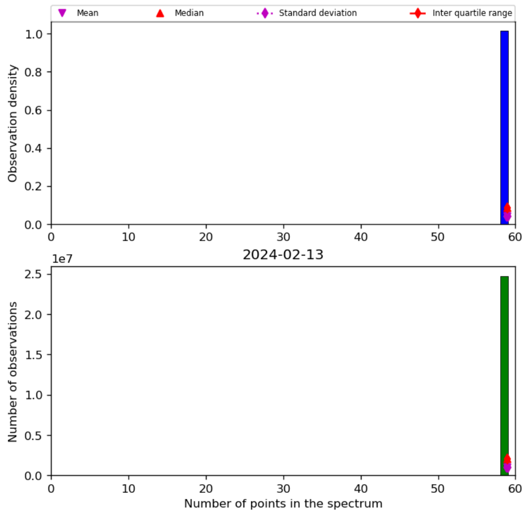
Figure 44: Histogram of “Number of points in the spectrum” for 2024-02-12 to 2024-02-14
