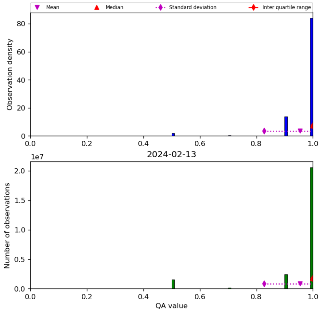
Figure 29: Histogram of “QA value” for 2024-02-12 to 2024-02-14
