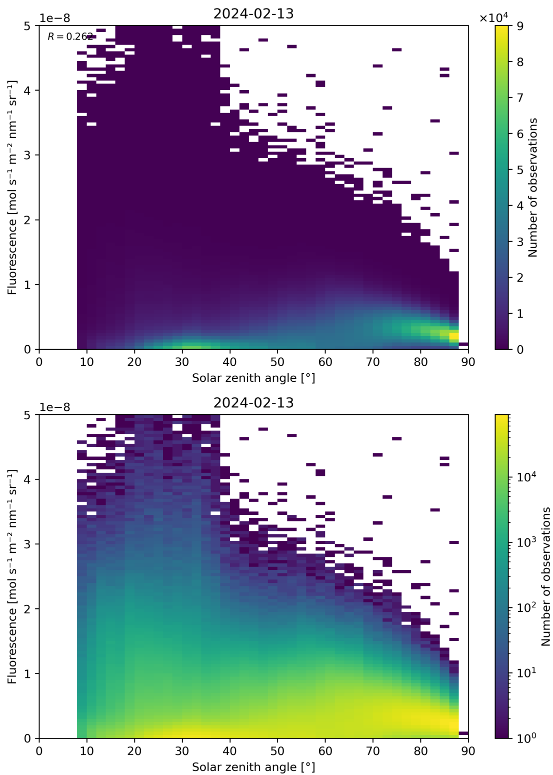
Figure 112: Scatter density plot of “Solar zenith angle” against “Fluorescence” for 2024-02-12 to 2024-02-14.
