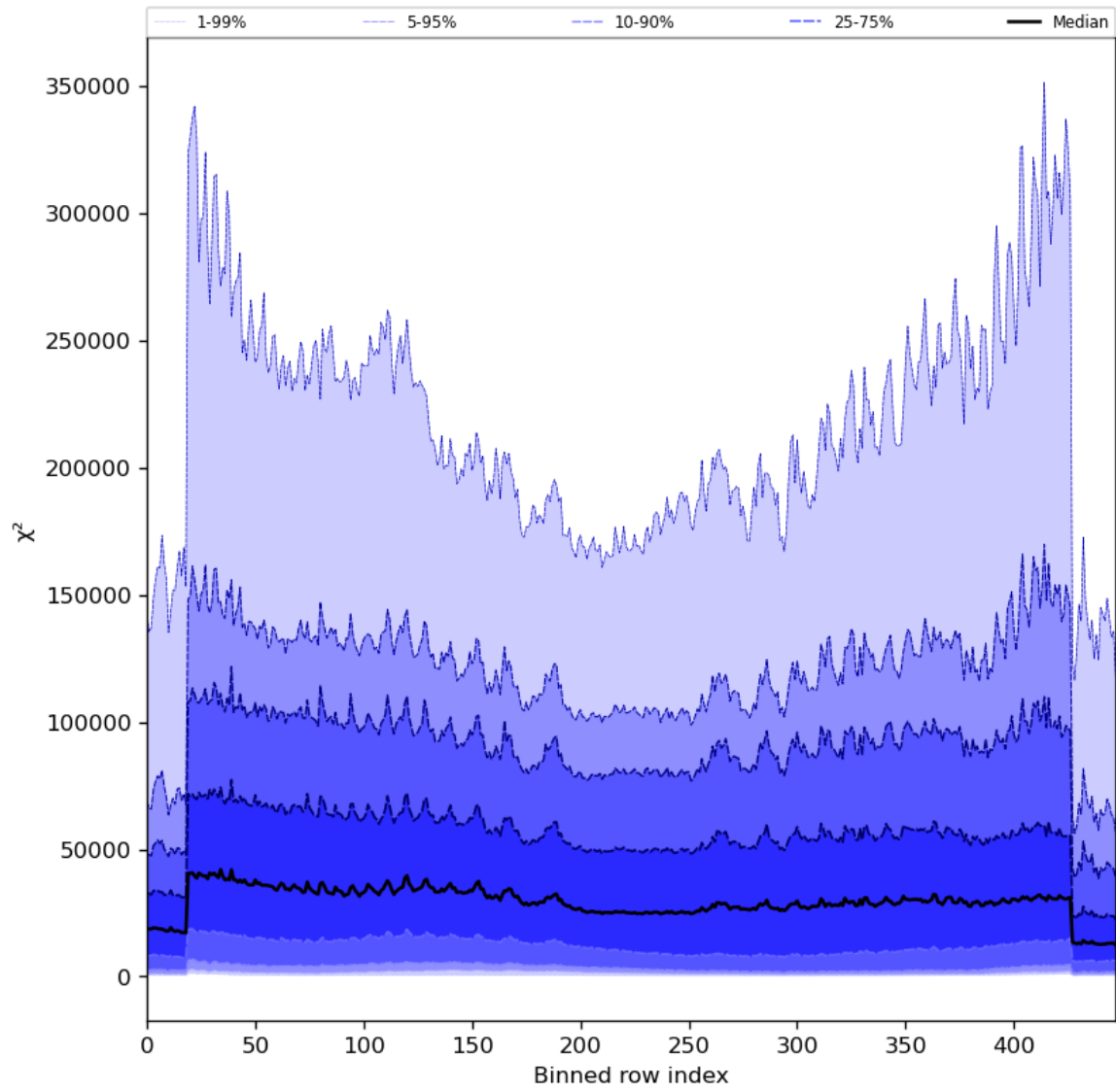
Figure 55: Along track statistics of “ \chi^2 ” for 2024-02-12 to 2024-02-14
