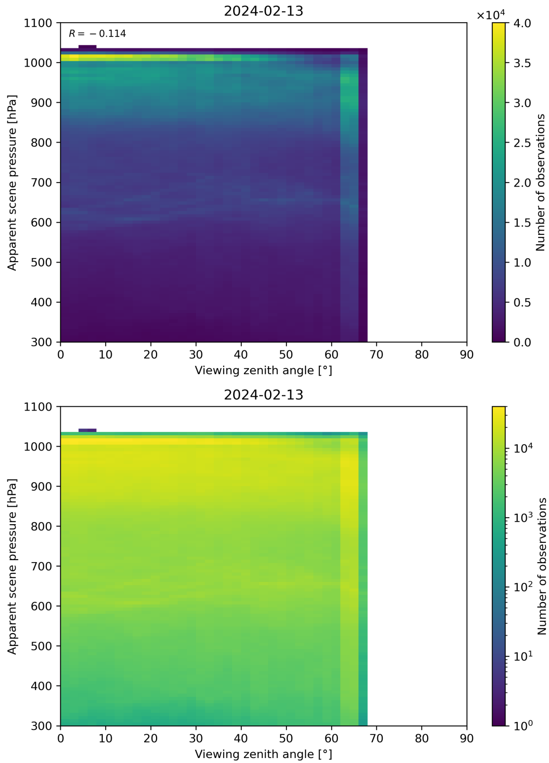
Figure 118: Scatter density plot of “Viewing zenith angle” against “Apparent scene pressure” for 2024-02-12 to 2024-02-14.
