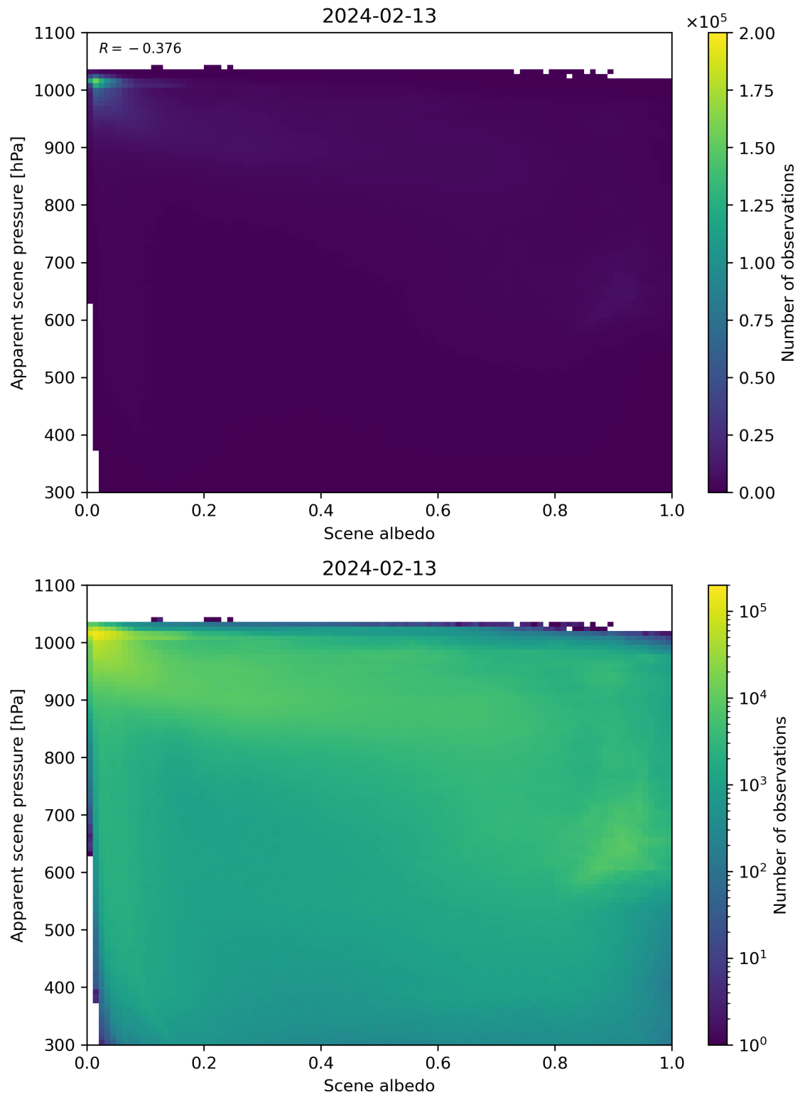
Figure 102: Scatter density plot of “Scene albedo” against “Apparent scene pressure” for 2024-02-12 to 2024-02-14.
