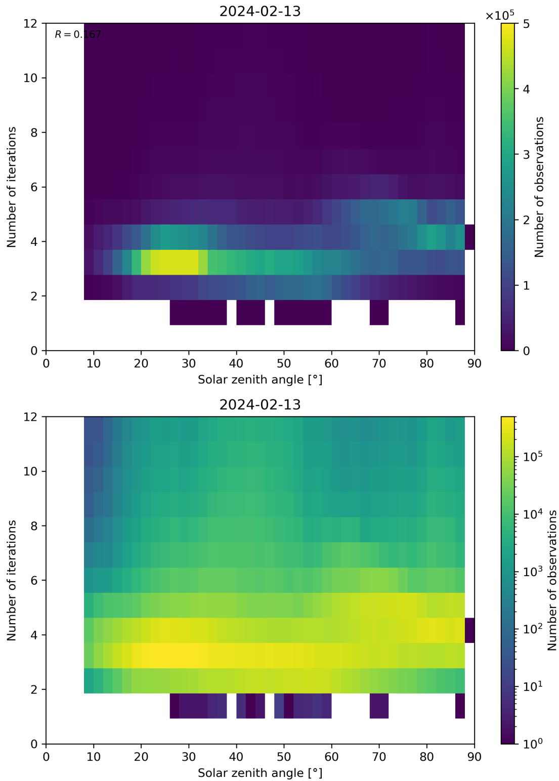
Figure 114: Scatter density plot of “Solar zenith angle” against “Number of iterations” for 2024-02-12 to 2024-02-14.
