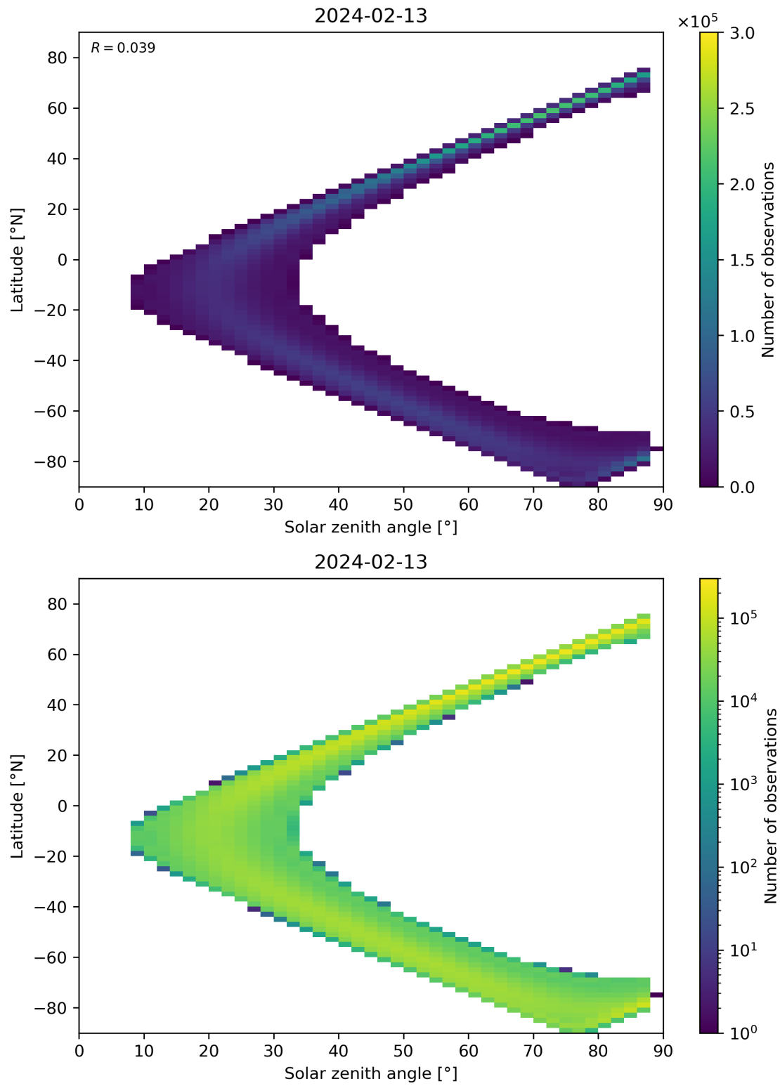
Figure 113: Scatter density plot of “Solar zenith angle” against “Latitude” for 2024-02-12 to 2024-02-14.
