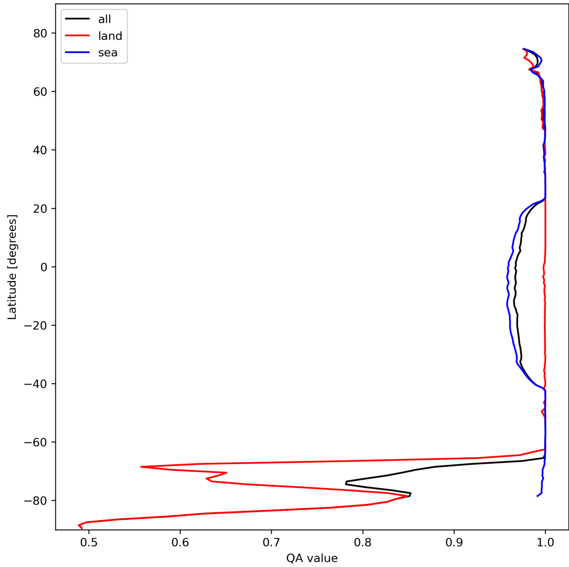
Figure 12: Zonal average of “QA value” for 2024-02-12 to 2024-02-14.
