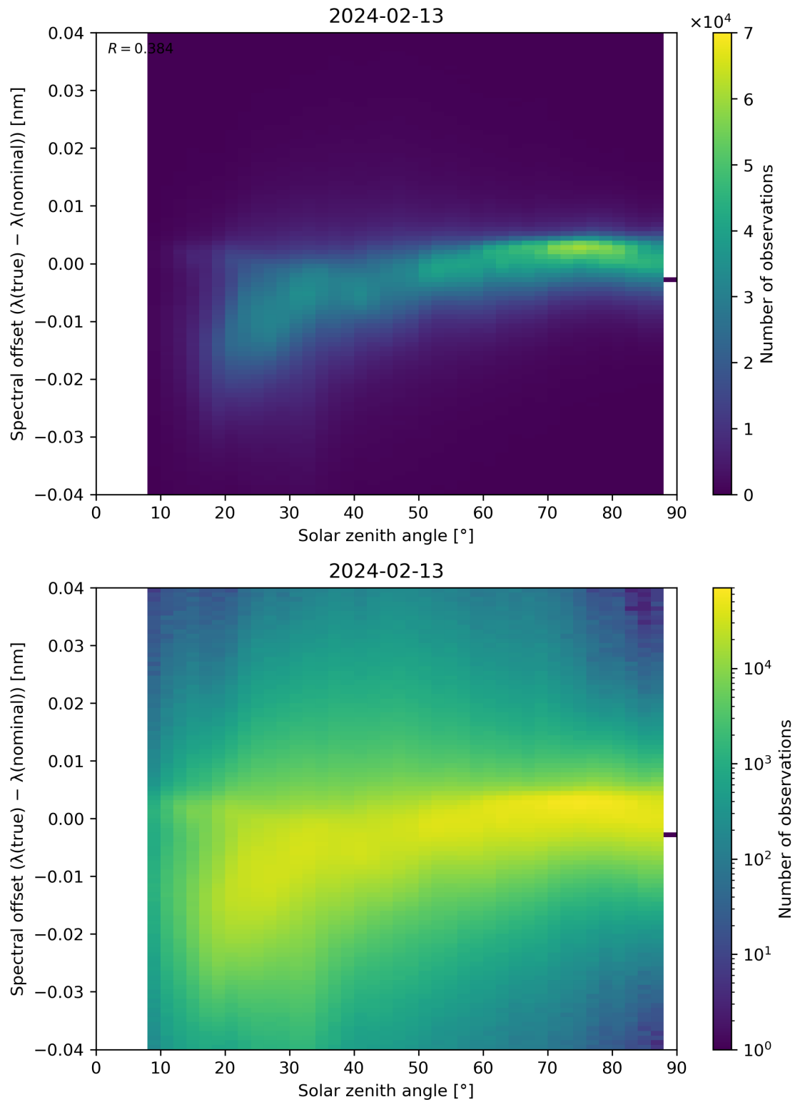
Figure 117: Scatter density plot of “Solar zenith angle” against “Spectral offset ( \lambda(\text{true}) - \lambda(\text{nominal}) )” for 2024-02-12 to 2024-02-14.
