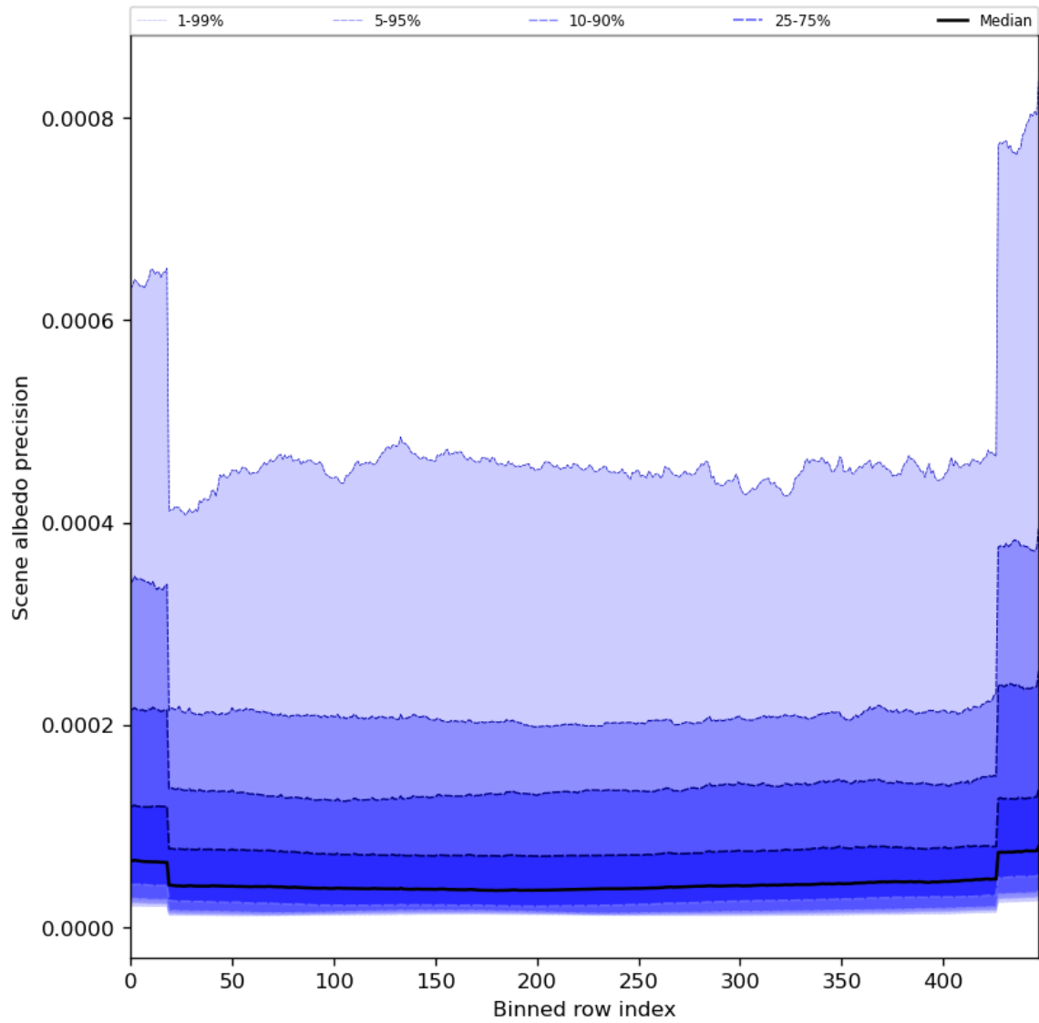
Figure 52: Along track statistics of “Scene albedo precision” for 2024-02-12 to 2024-02-14
