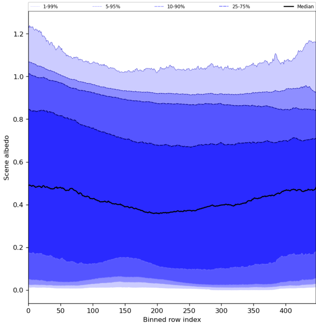
Figure 51: Along track statistics of “Scene albedo” for 2024-02-12 to 2024-02-14
