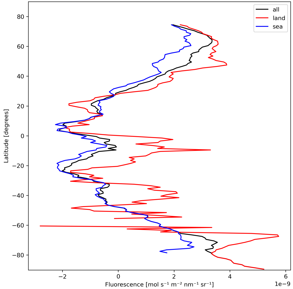
Figure 23: Zonal average of “Fluorescence” for 2024-02-12 to 2024-02-14.
