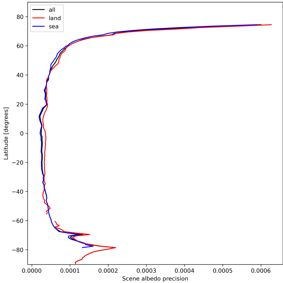
Figure 18: Zonal average of “Scene albedo precision” for 2024-02-12 to 2024-02-14.
