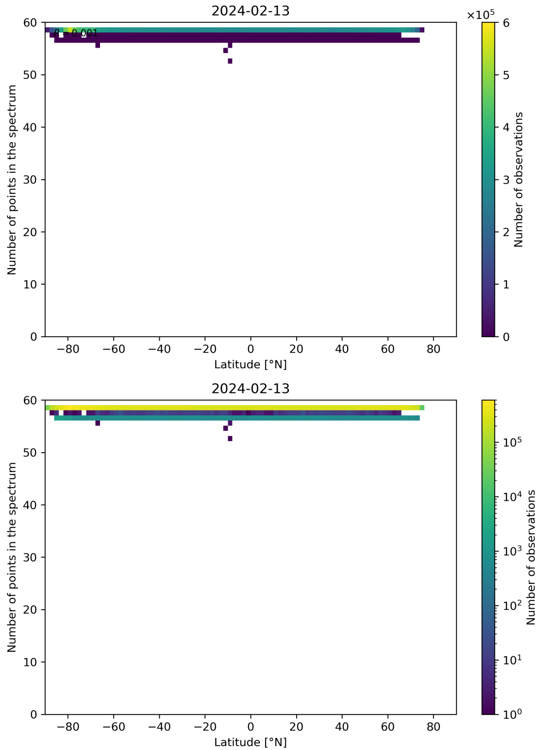
Figure 94: Scatter density plot of “Latitude” against “Number of points in the spectrum” for 2024-02-12 to 2024-02-14.
