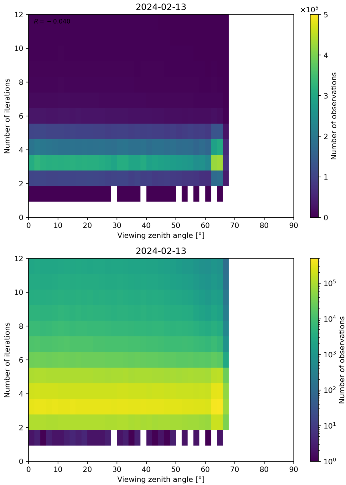
Figure 124: Scatter density plot of “Viewing zenith angle” against “Number of iterations” for 2024-02-12 to 2024-02-14.
