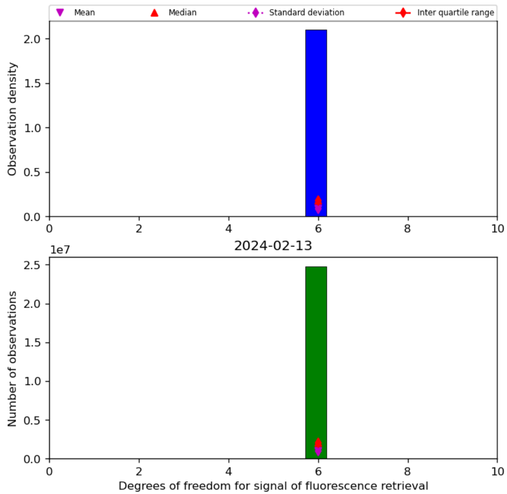
Figure 43: Histogram of “Degrees of freedom for signal of fluorescence retrieval” for 2024-02-12 to 2024-02-14
