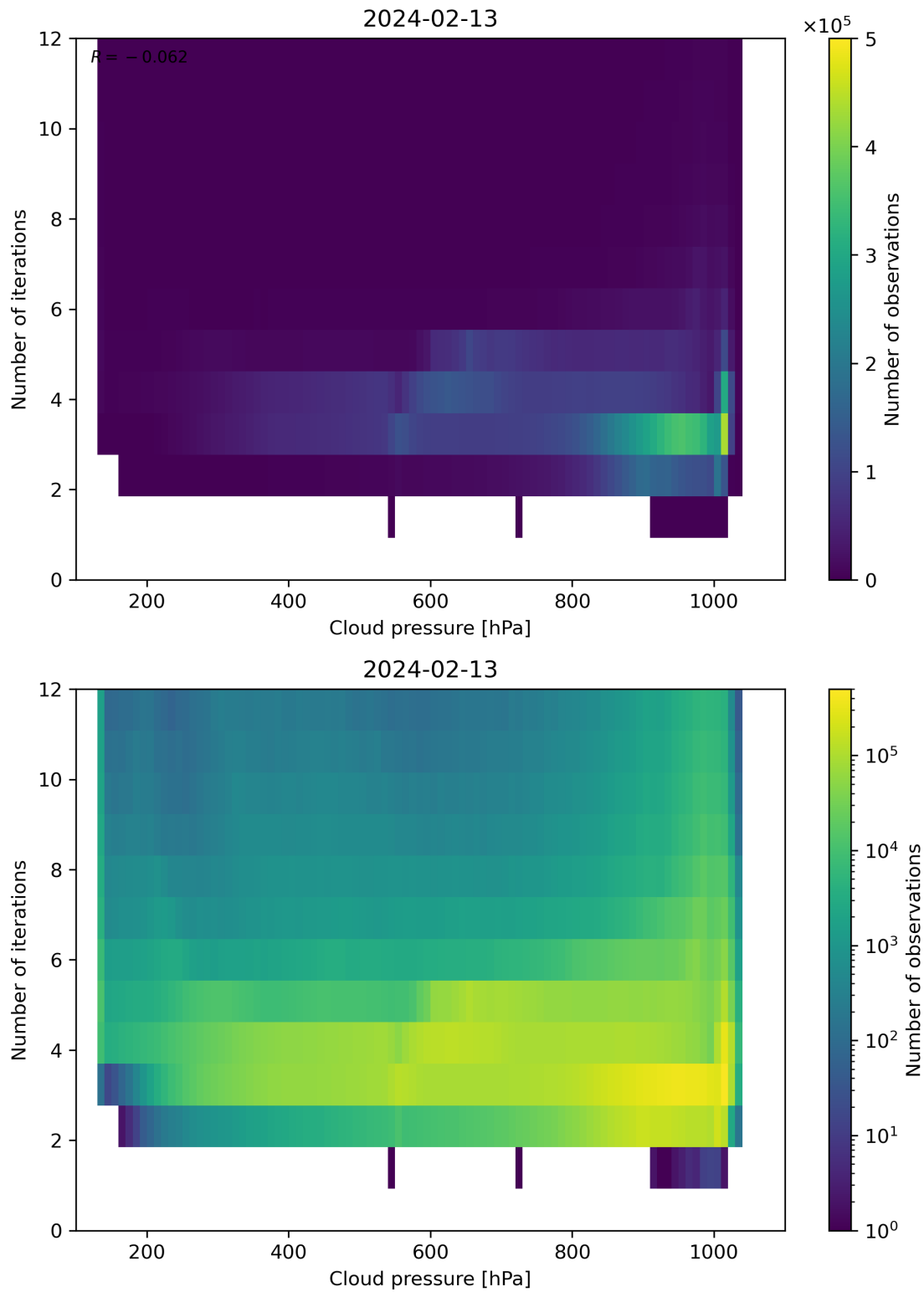
Figure 81: Scatter density plot of “Cloud pressure” against “Number of iterations” for 2024-02-12 to 2024-02-14.
