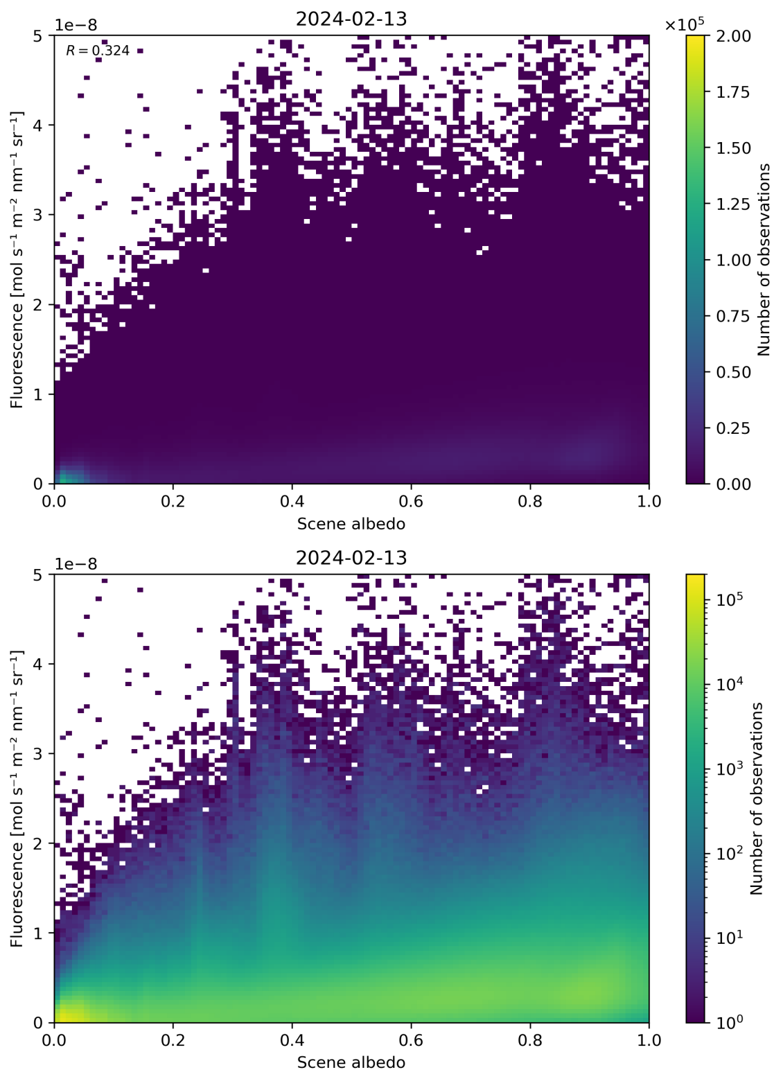
Figure 104: Scatter density plot of “Scene albedo” against “Fluorescence” for 2024-02-12 to 2024-02-14.
