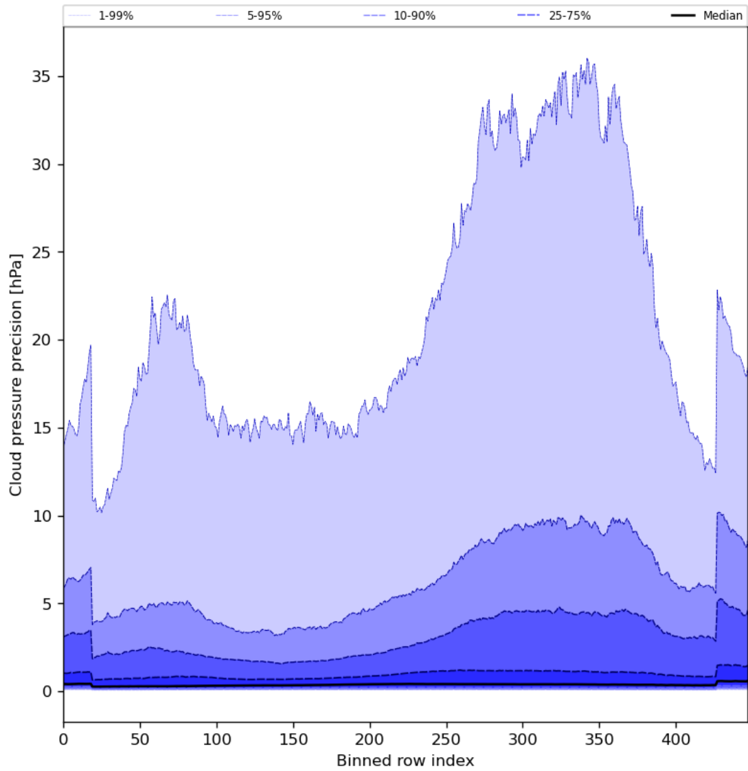
Figure 48: Along track statistics of “Cloud pressure precision” for 2024-02-12 to 2024-02-14
