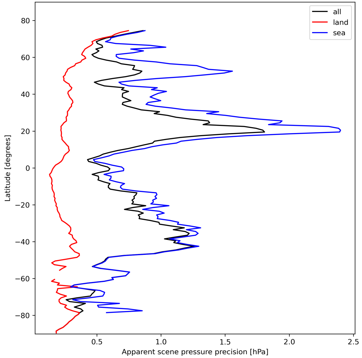
Figure 20: Zonal average of “Apparent scene pressure precision” for 2024-02-12 to 2024-02-14.
