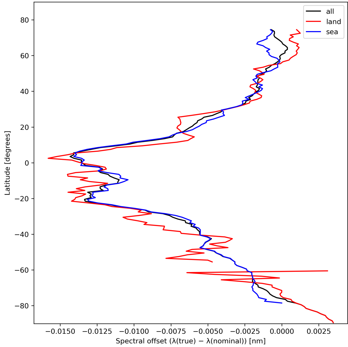
Figure 28: Zonal average of “Spectral offset ( \lambda(\text{true}) - \lambda(\text{nominal}) )” for 2024-02-12 to 2024-02-14.
