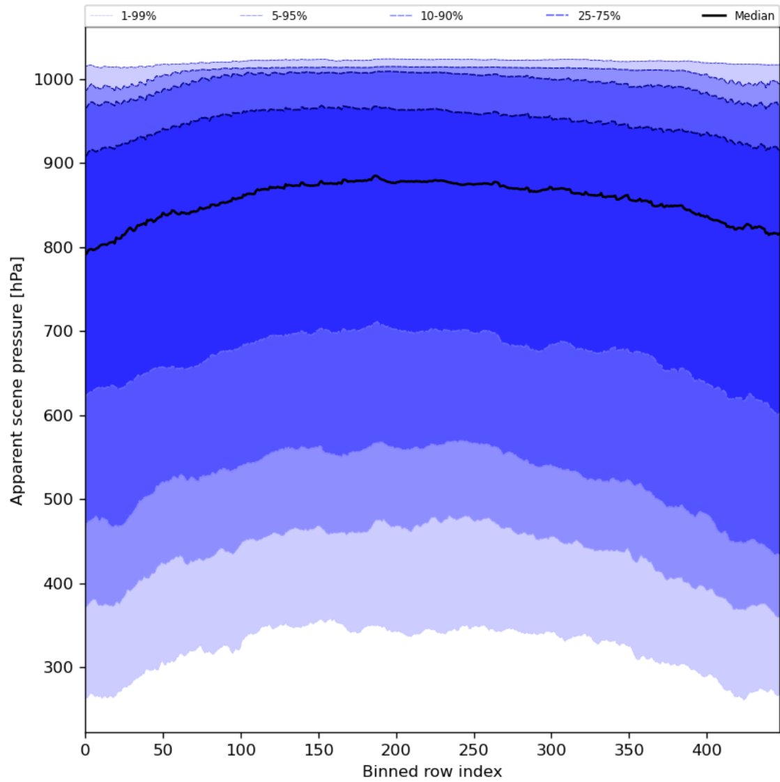
Figure 53: Along track statistics of “Apparent scene pressure” for 2024-02-12 to 2024-02-14
