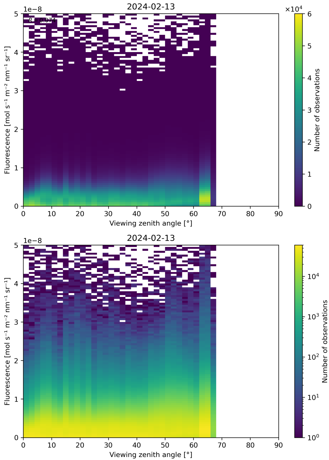
Figure 122: Scatter density plot of “Viewing zenith angle” against “Fluorescence” for 2024-02-12 to 2024-02-14.
