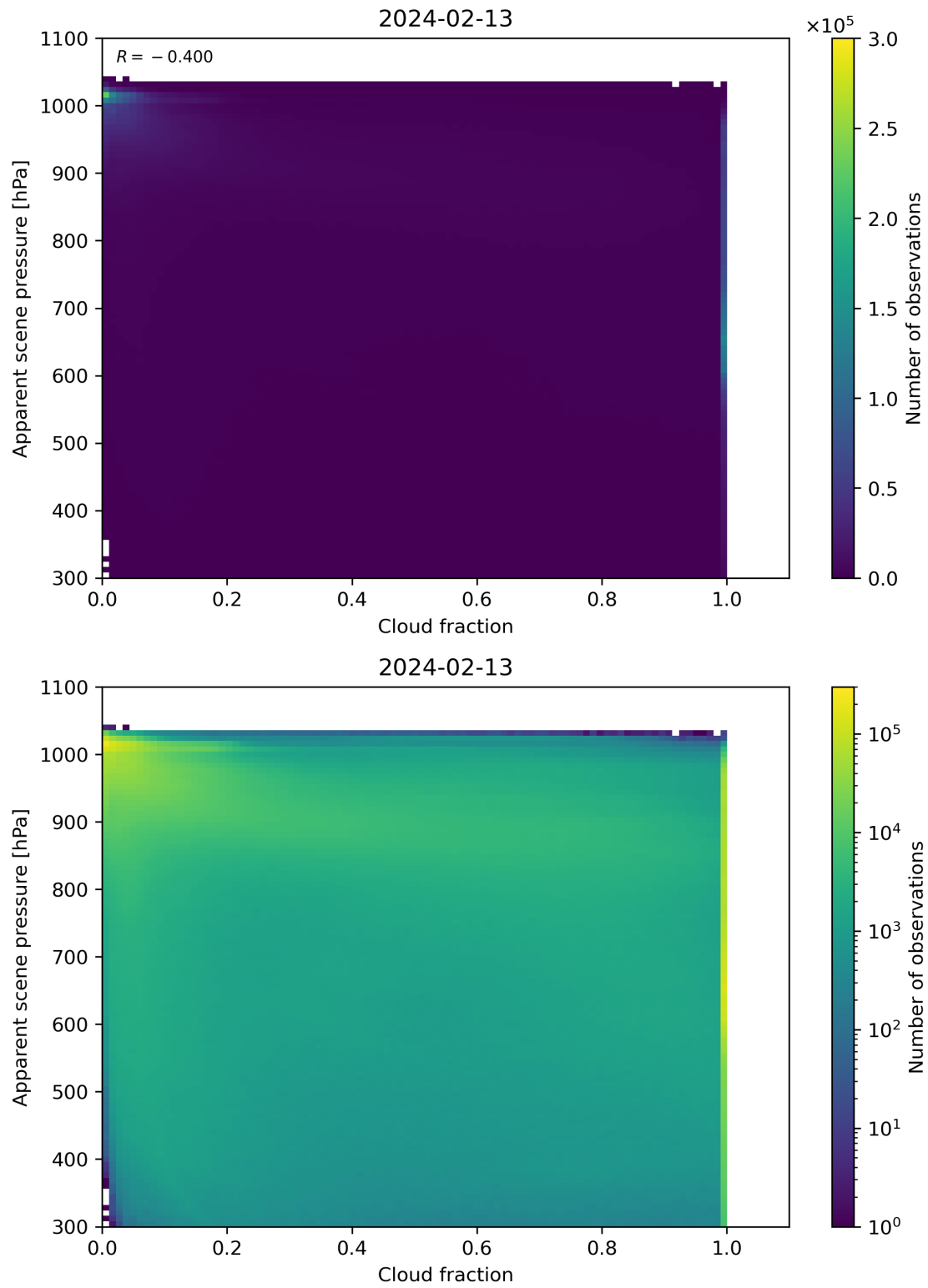
Figure 70: Scatter density plot of “Cloud fraction” against “Apparent scene pressure” for 2024-02-12 to 2024-02-14.
