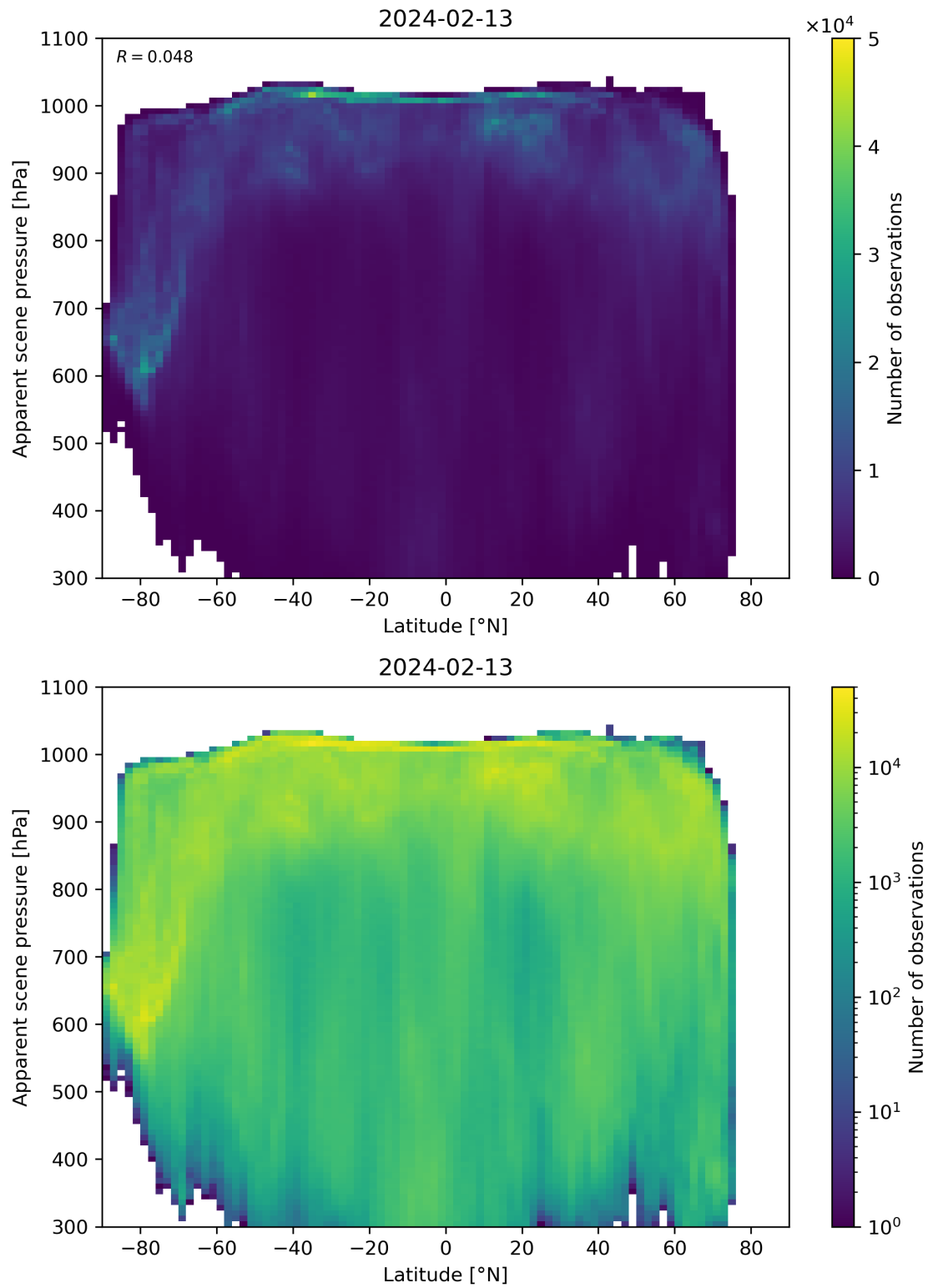
Figure 88: Scatter density plot of “Latitude” against “Apparent scene pressure” for 2024-02-12 to 2024-02-14.
