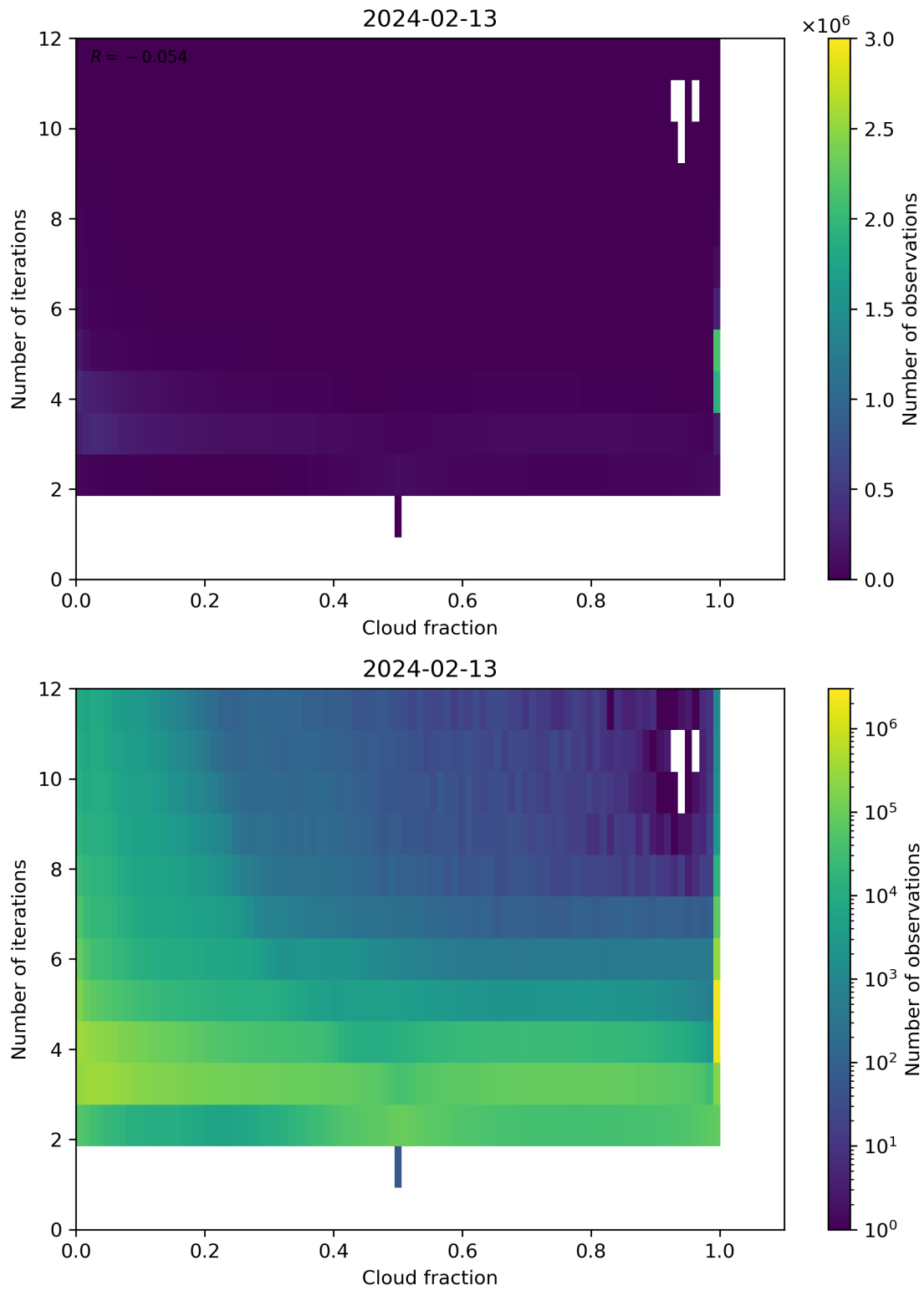
Figure 73: Scatter density plot of “Cloud fraction” against “Number of iterations” for 2024-02-12 to 2024-02-14.
