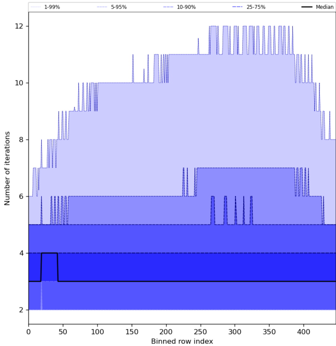
Figure 56: Along track statistics of “Number of iterations” for 2024-02-12 to 2024-02-14
