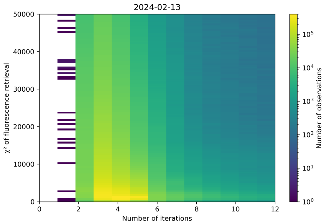
Figure 97: Scatter density plot of “Number of iterations” against “ \chi^2 of fluorescence retrieval” for 2024-02-12 to 2024-02-14.
