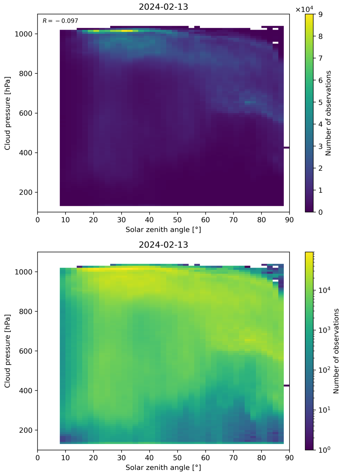
Figure 111: Scatter density plot of “Solar zenith angle” against “Cloud pressure” for 2024-02-12 to 2024-02-14.
