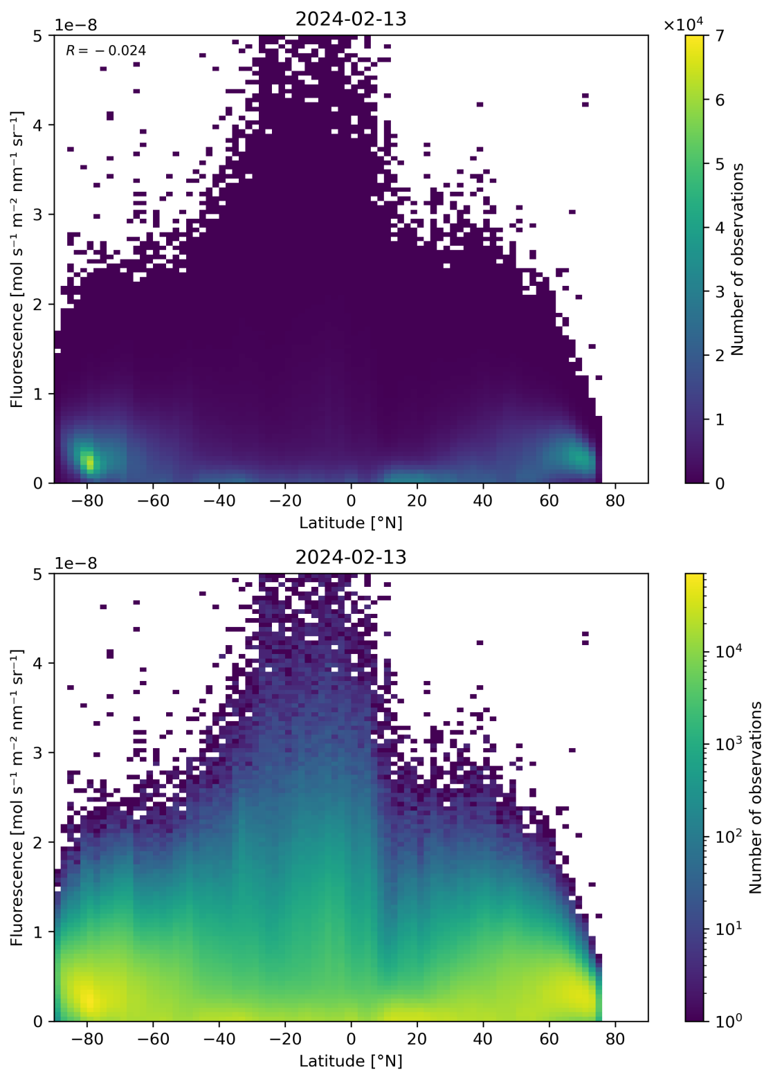
Figure 92: Scatter density plot of “Latitude” against “Fluorescence” for 2024-02-12 to 2024-02-14.
