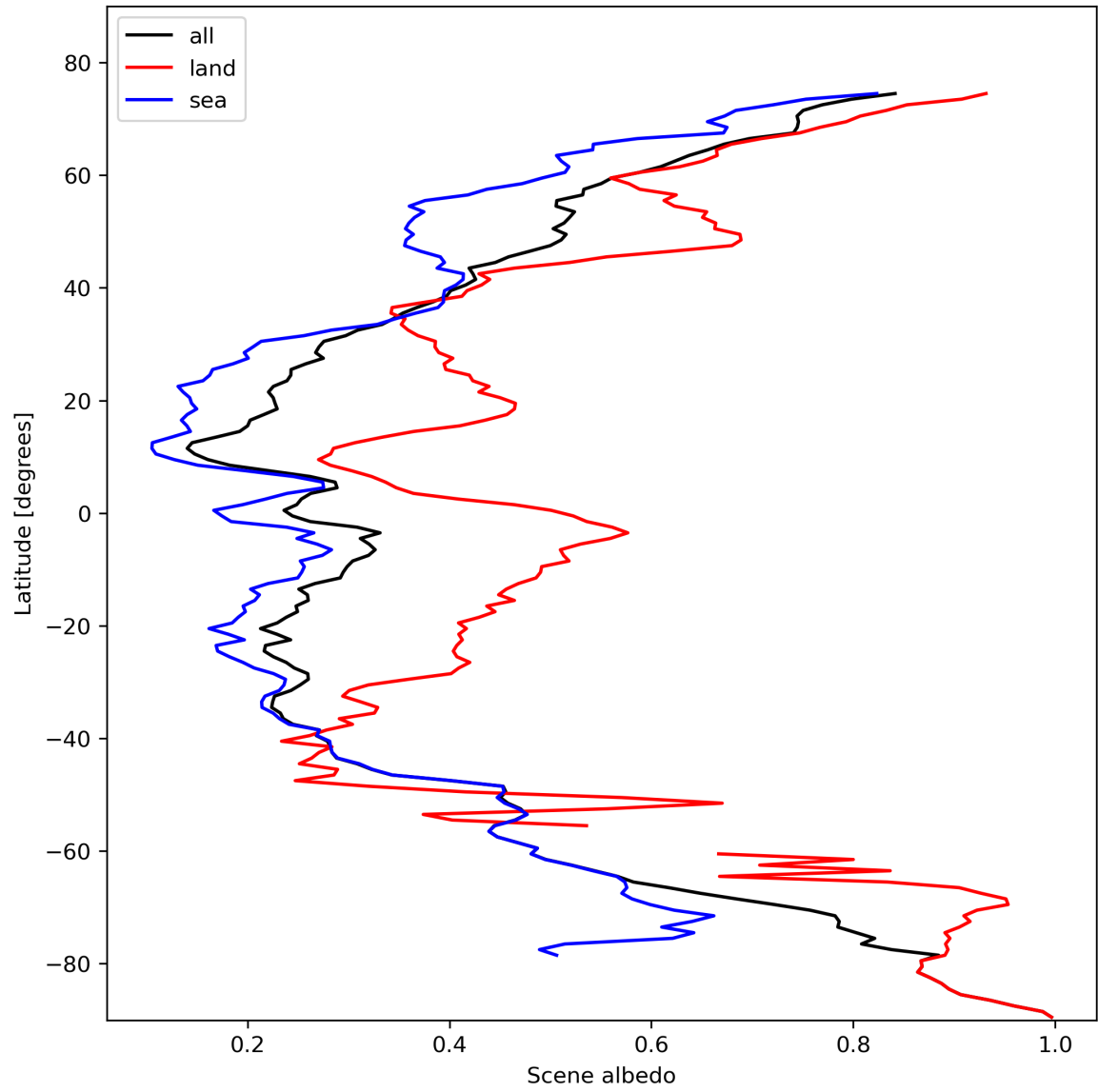
Figure 17: Zonal average of “Scene albedo” for 2024-02-12 to 2024-02-14.
