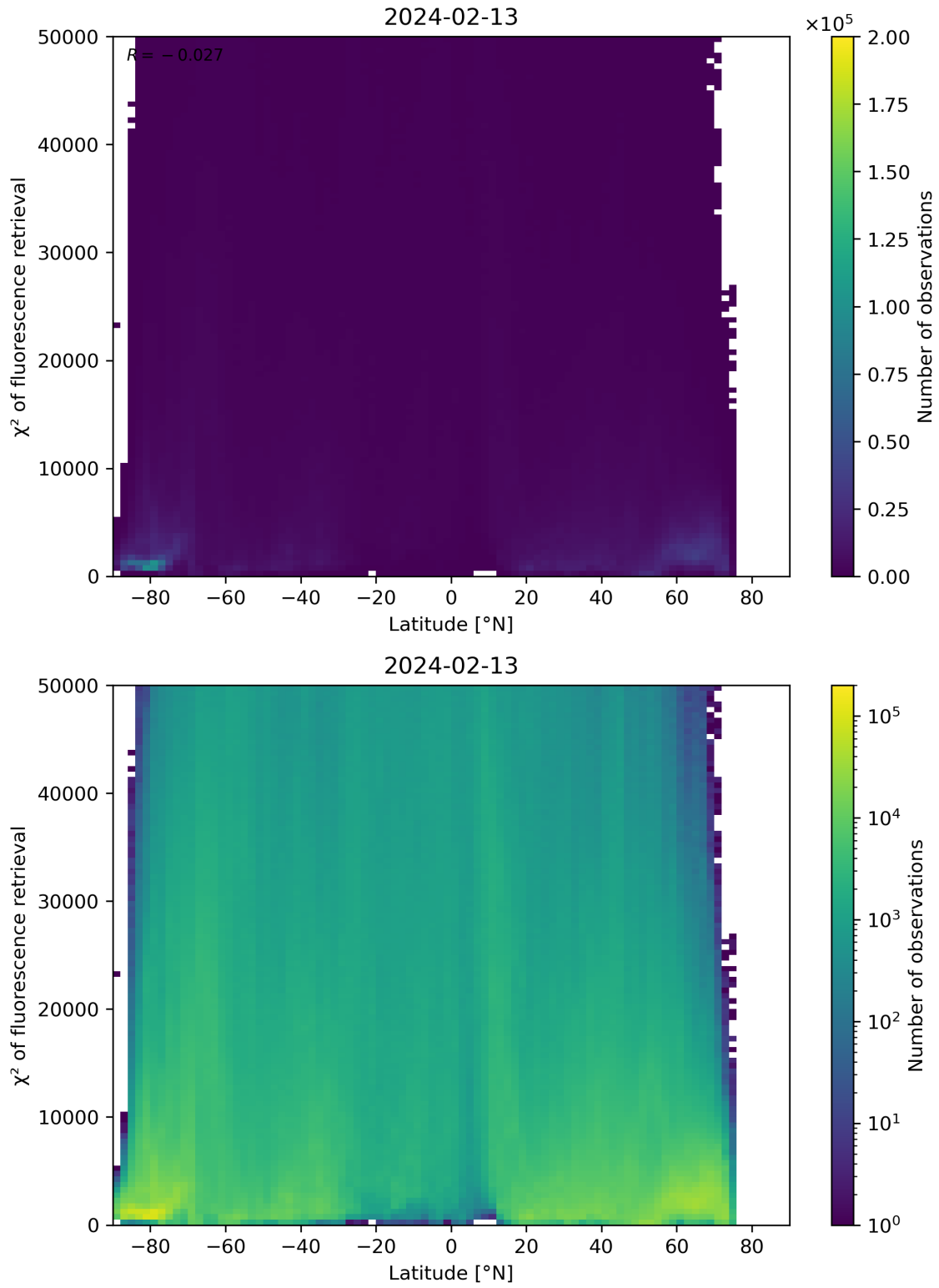
Figure 89: Scatter density plot of “Latitude” against “ \chi^2 of fluorescence retrieval” for 2024-02-12 to 2024-02-14.
