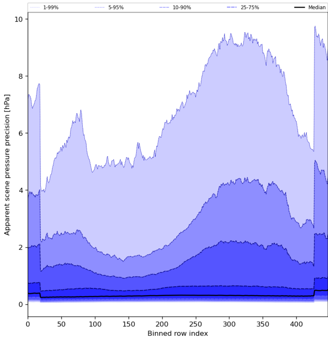
Figure 54: Along track statistics of “Apparent scene pressure precision” for 2024-02-12 to 2024-02-14
