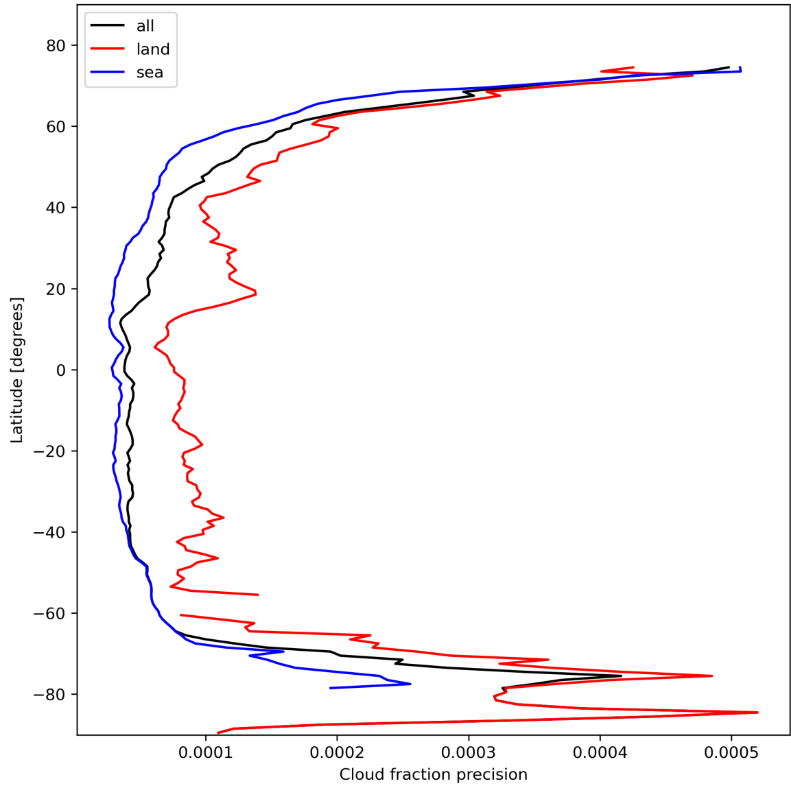
Figure 16: Zonal average of “Cloud fraction precision” for 2024-02-12 to 2024-02-14.
