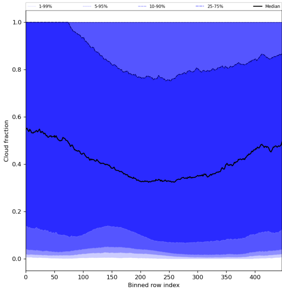
Figure 49: Along track statistics of “Cloud fraction” for 2024-02-12 to 2024-02-14
