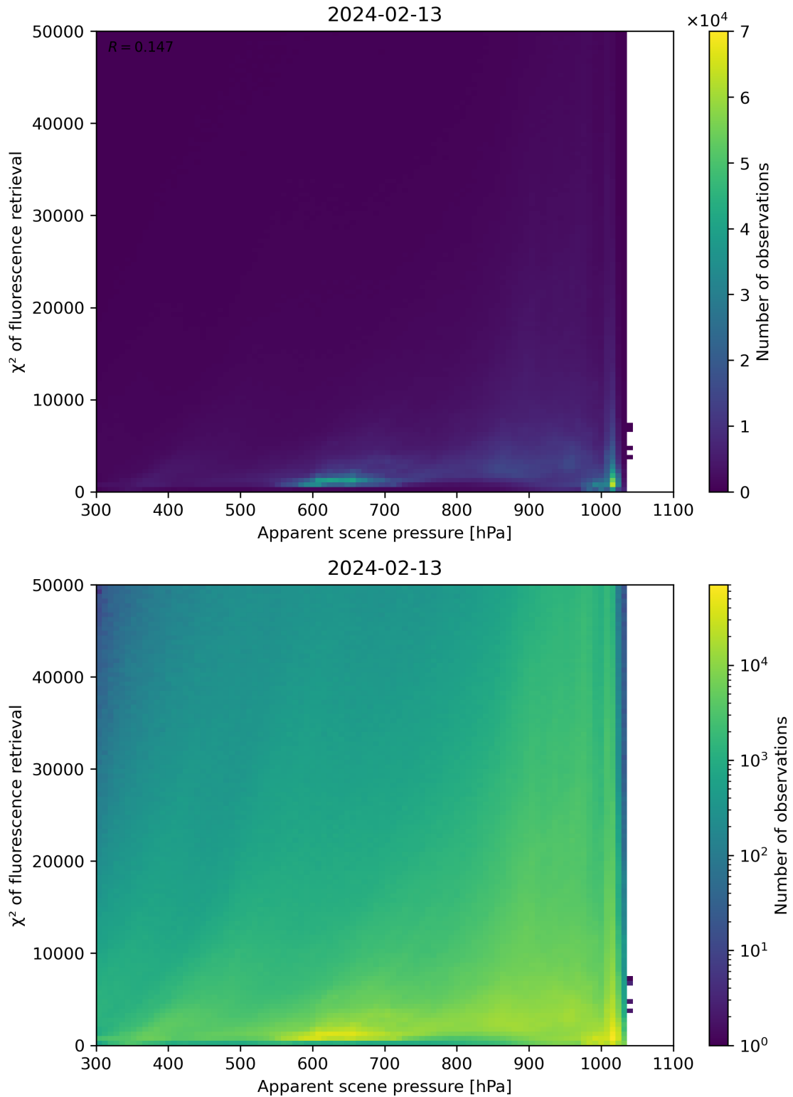
Figure 63: Scatter density plot of “Apparent scene pressure” against “ \chi^2 of fluorescence retrieval” for 2024-02-12 to 2024-02-14.
