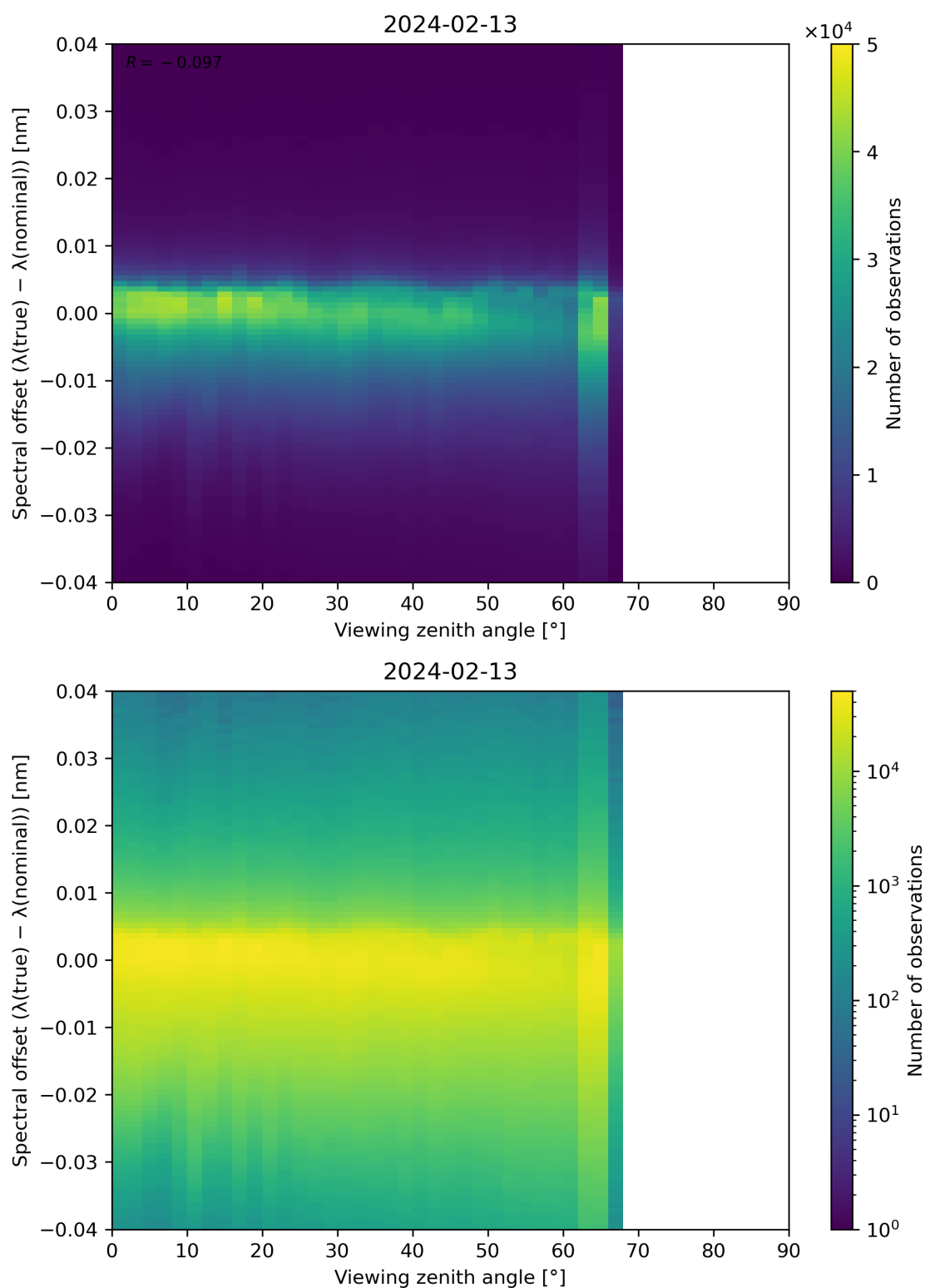
Figure 128: Scatter density plot of “Viewing zenith angle” against “Spectral offset ( \lambda(\text{true}) - \lambda(\text{nominal}) )” for 2024-02-12 to 2024-02-14.
