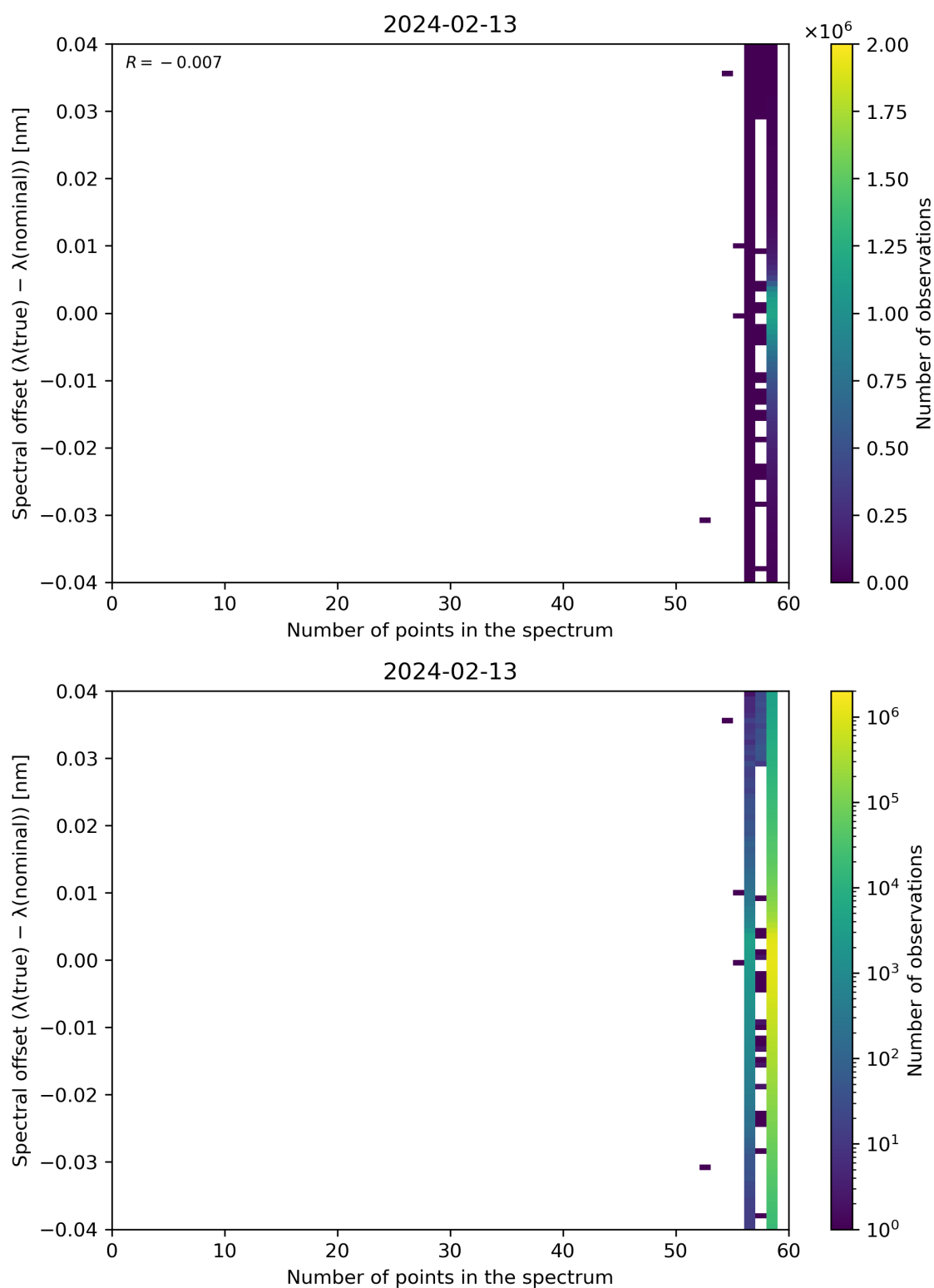
Figure 101: Scatter density plot of “Number of points in the spectrum” against “Spectral offset ( \lambda(\text{true}) - \lambda(\text{nominal}) )” for 2024-02-12 to 2024-02-14.
