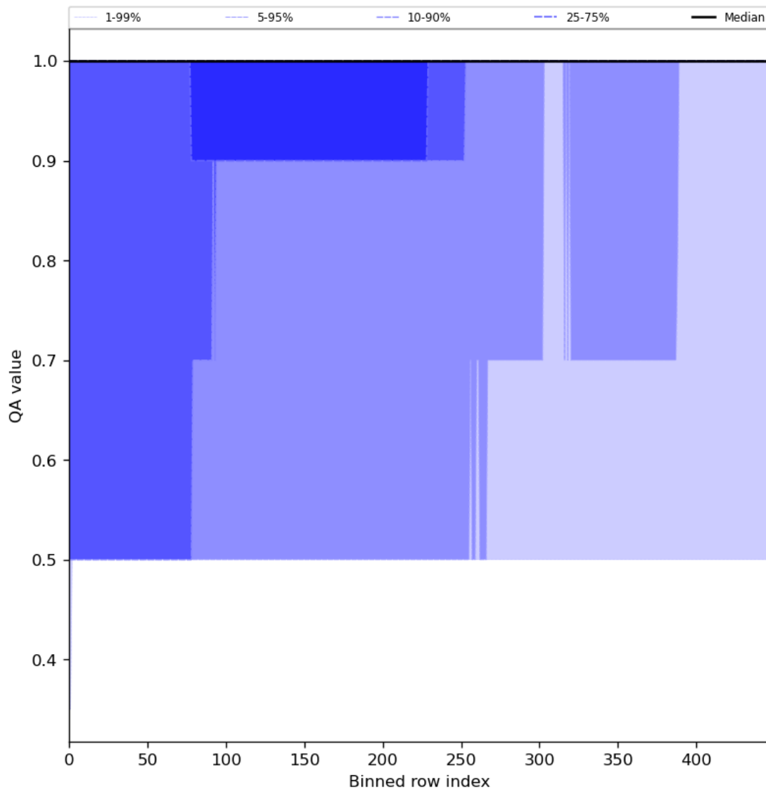
Figure 46: Along track statistics of “QA value” for 2024-02-12 to 2024-02-14
