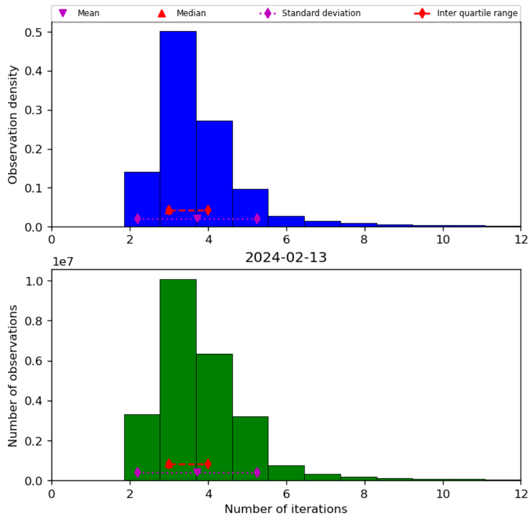
Figure 39: Histogram of “Number of iterations” for 2024-02-12 to 2024-02-14
