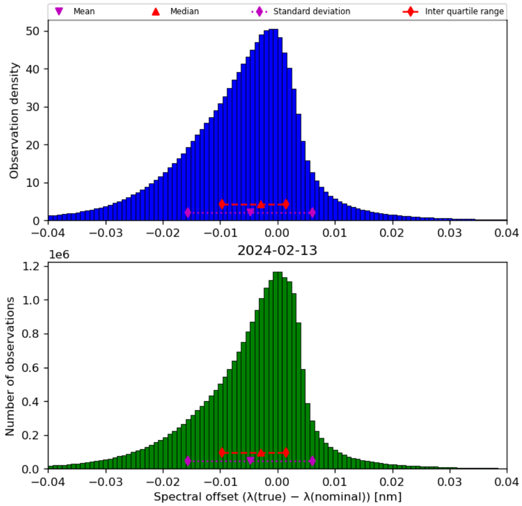
Figure 45: Histogram of “Spectral offset ( \lambda(\text{true}) - \lambda(\text{nominal}) )” for 2024-02-12 to 2024-02-14
