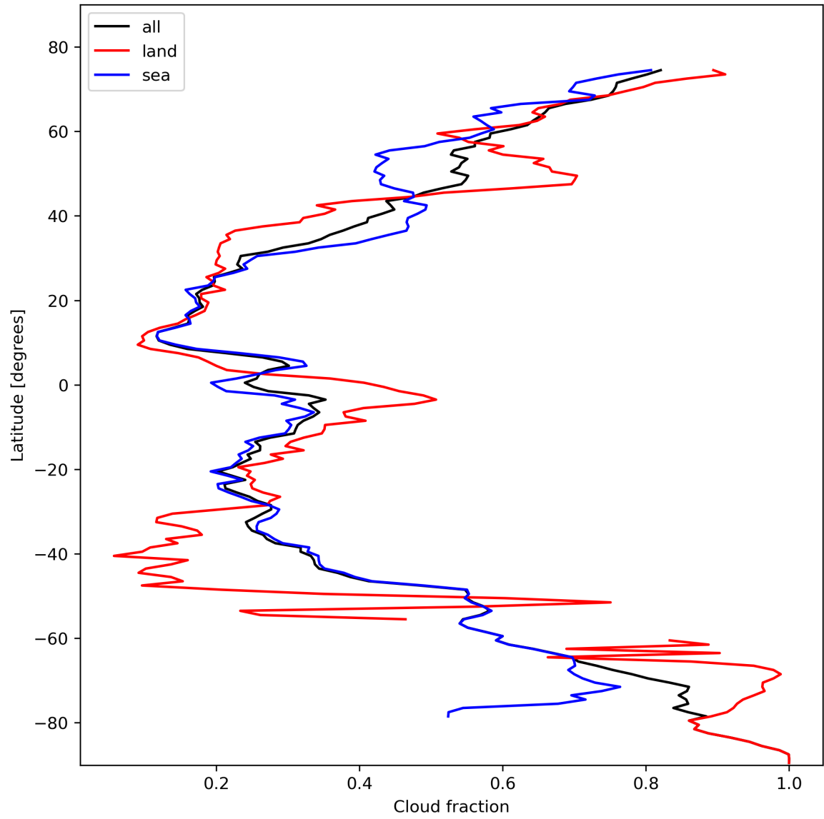
Figure 15: Zonal average of “Cloud fraction” for 2024-02-12 to 2024-02-14.
