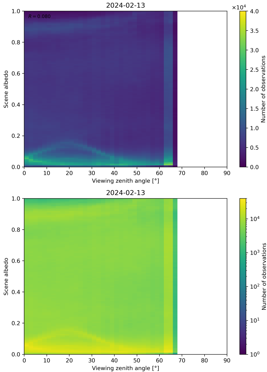
Figure 126: Scatter density plot of “Viewing zenith angle” against “Scene albedo” for 2024-02-12 to 2024-02-14.
