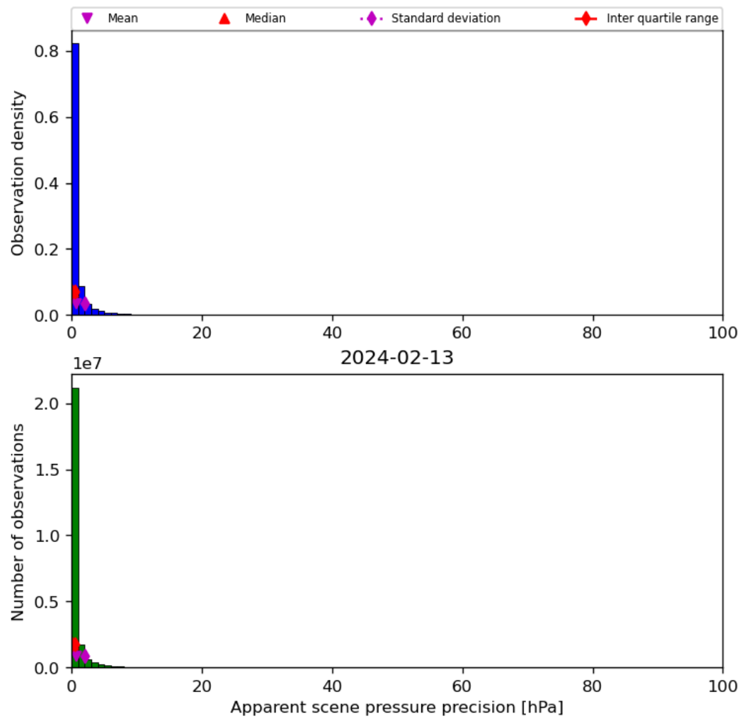
Figure 37: Histogram of “Apparent scene pressure precision” for 2024-02-12 to 2024-02-14
