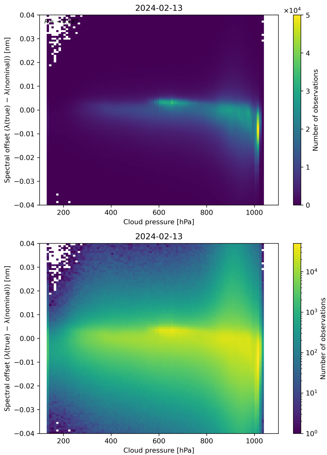
Figure 84: Scatter density plot of “Cloud pressure” against “Spectral offset ( \lambda(\text{true}) - \lambda(\text{nominal}) )” for 2024-02-12 to 2024-02-14.
