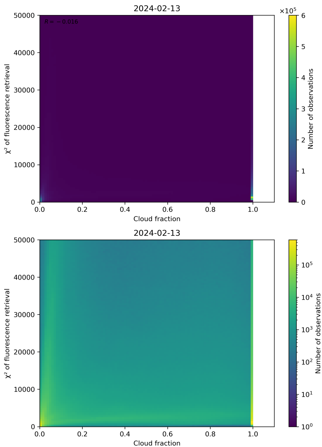
Figure 71: Scatter density plot of “Cloud fraction” against “ \chi^2 of fluorescence retrieval” for 2024-02-12 to 2024-02-14.
