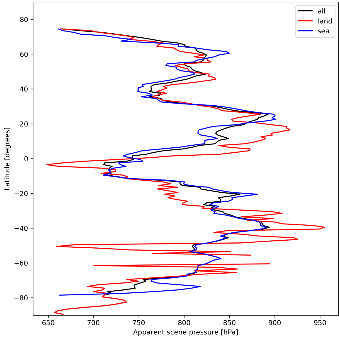
Figure 19: Zonal average of “Apparent scene pressure” for 2024-02-12 to 2024-02-14.
