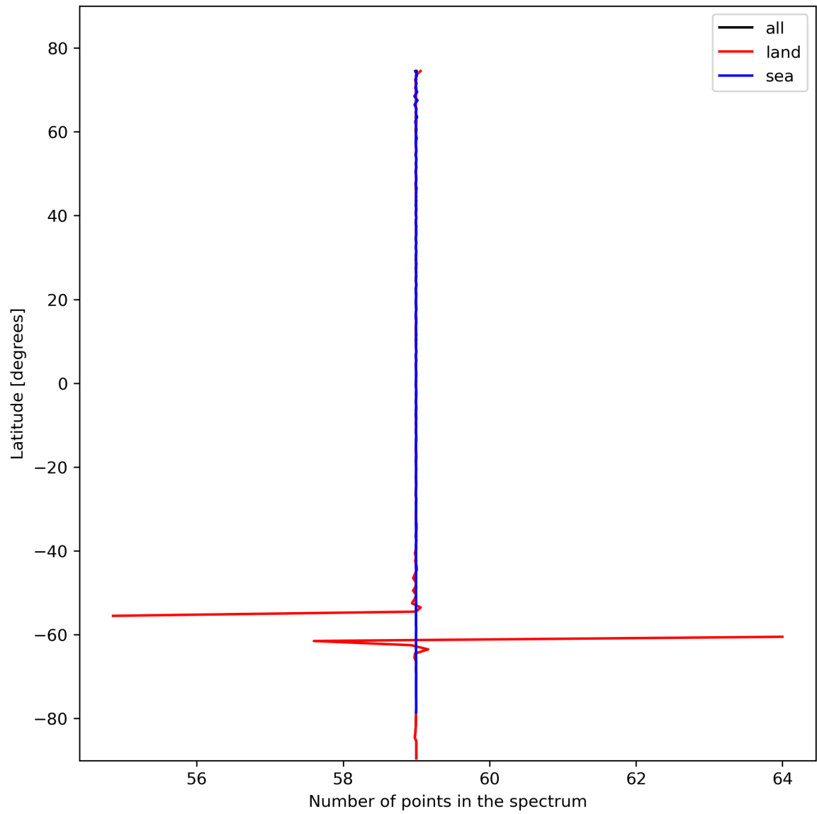
Figure 27: Zonal average of “Number of points in the spectrum” for 2024-02-12 to 2024-02-14.
