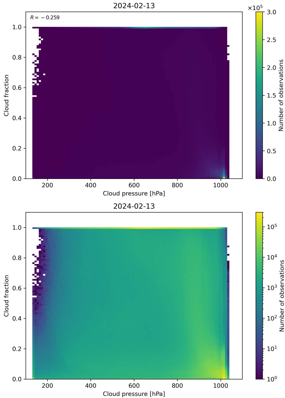
Figure 79: Scatter density plot of “Cloud pressure” against “Cloud fraction” for 2024-02-12 to 2024-02-14.
