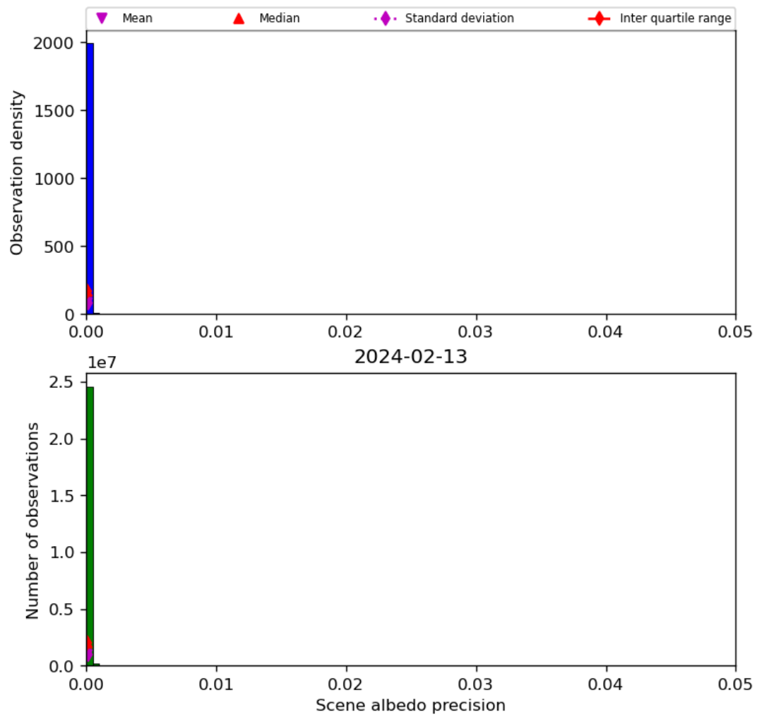
Figure 35: Histogram of “Scene albedo precision” for 2024-02-12 to 2024-02-14
