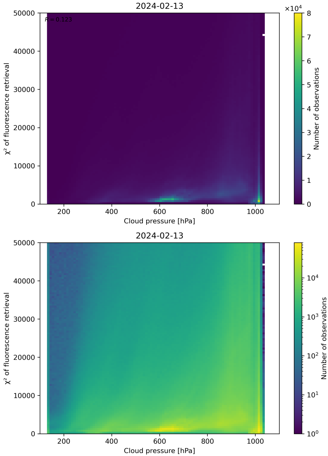
Figure 78: Scatter density plot of “Cloud pressure” against “ \chi^2 of fluorescence retrieval” for 2024-02-12 to 2024-02-14.
