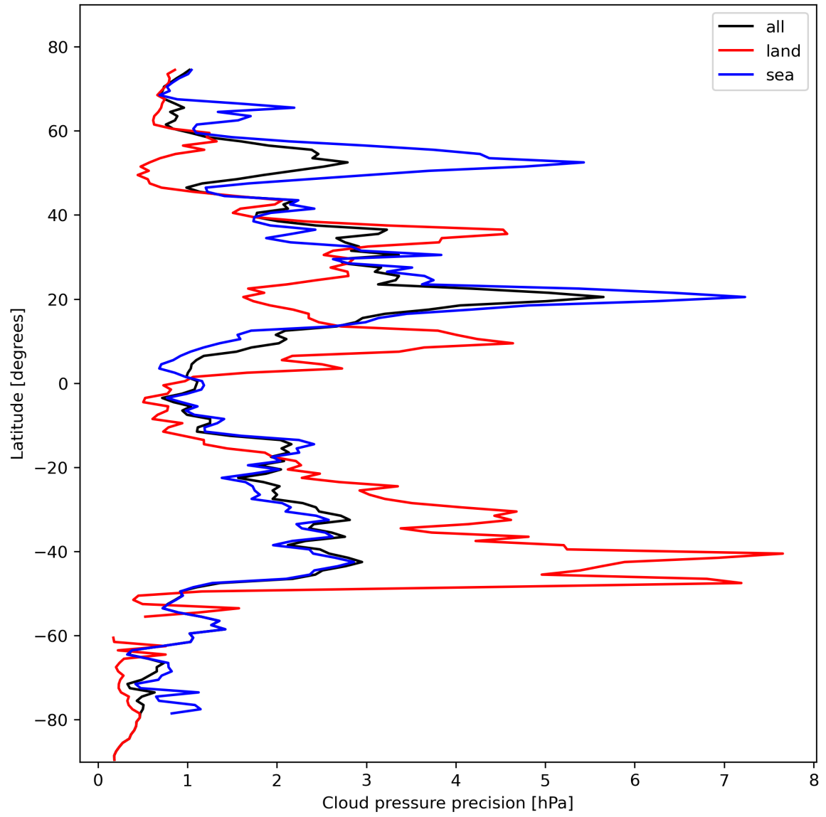
Figure 14: Zonal average of “Cloud pressure precision” for 2024-02-12 to 2024-02-14.
