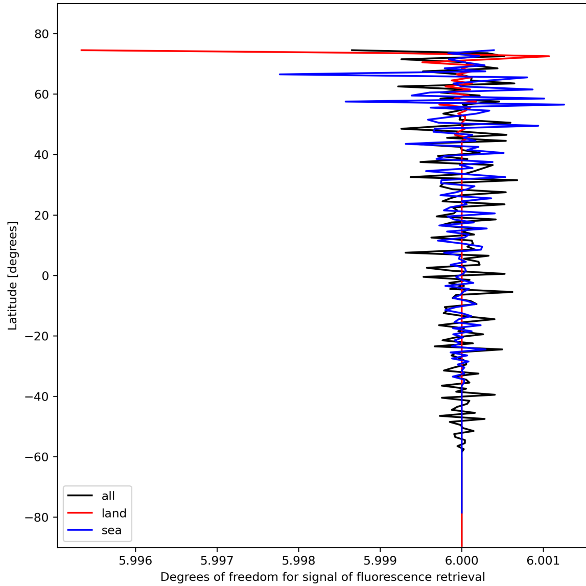
Figure 26: Zonal average of “Degrees of freedom for signal of fluorescence retrieval” for 2024-02-12 to 2024-02-14.
