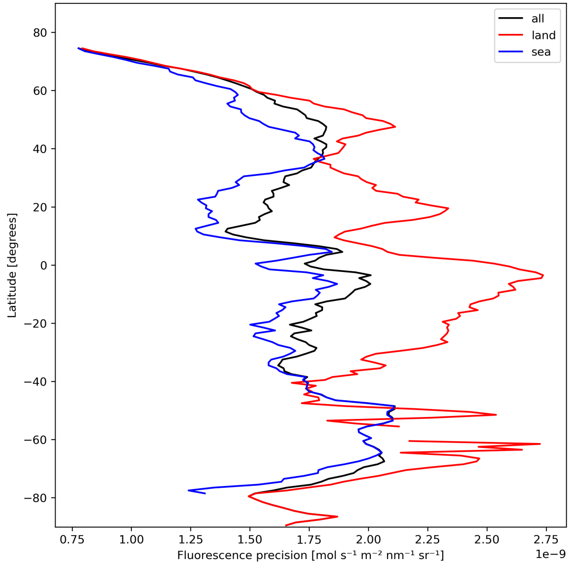
Figure 24: Zonal average of “Fluorescence precision” for 2024-02-12 to 2024-02-14.
