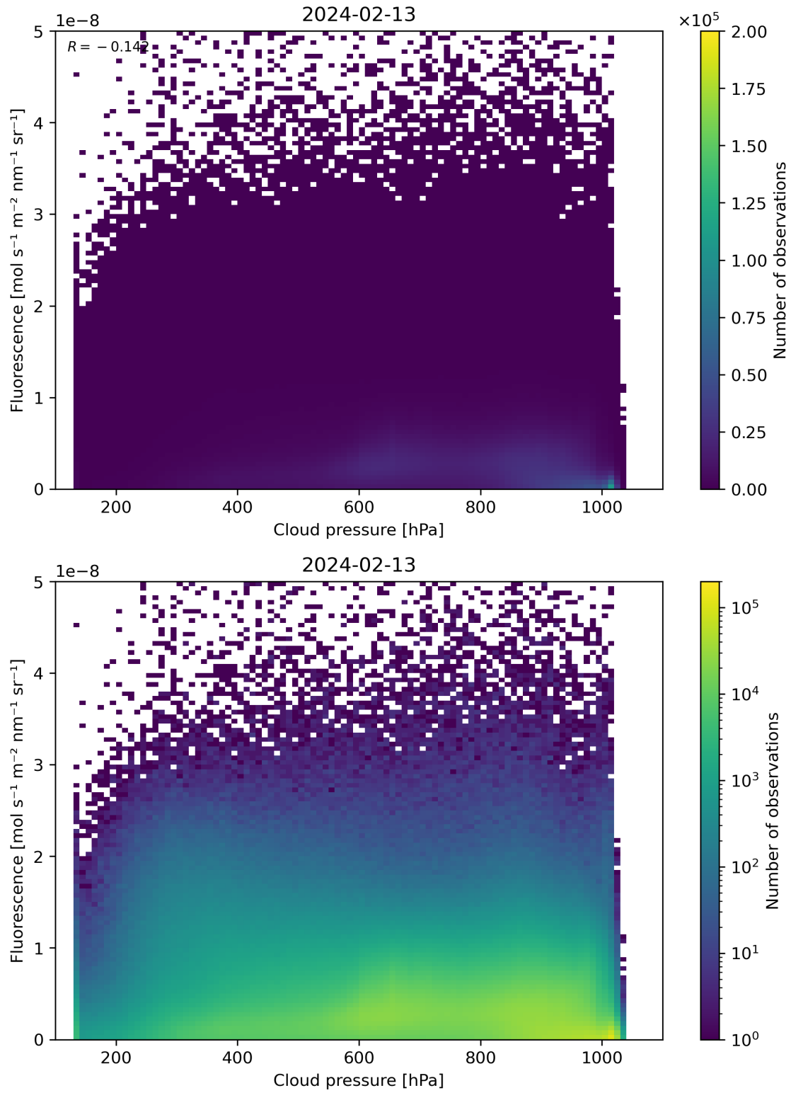
Figure 80: Scatter density plot of “Cloud pressure” against “Fluorescence” for 2024-02-12 to 2024-02-14.
