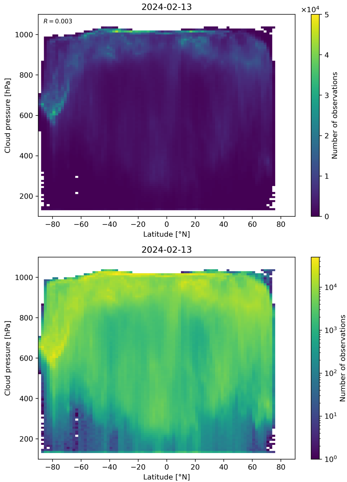
Figure 91: Scatter density plot of “Latitude” against “Cloud pressure” for 2024-02-12 to 2024-02-14.
