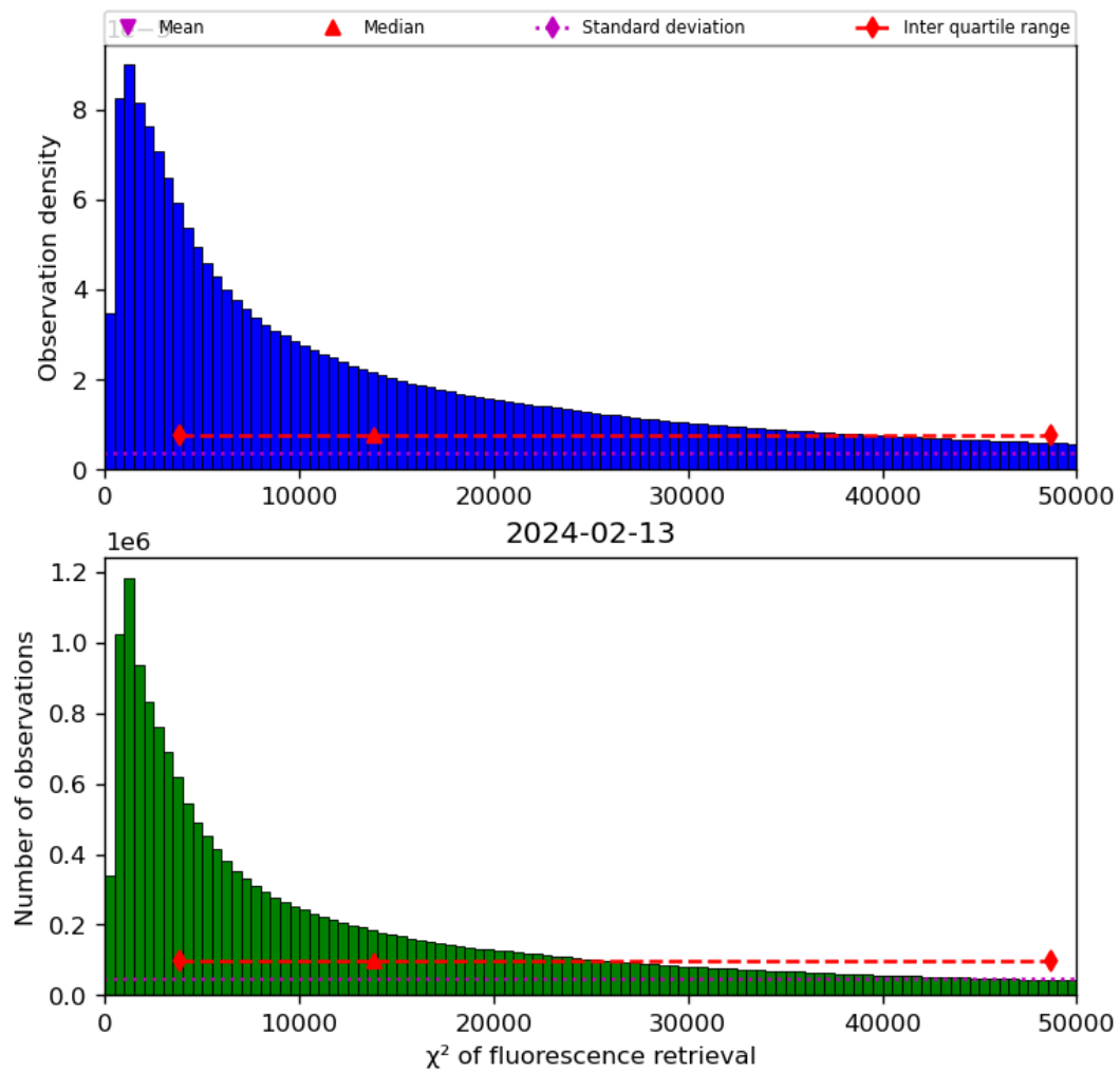
Figure 42: Histogram of “ \chi^2 of fluorescence retrieval” for 2024-02-12 to 2024-02-14
