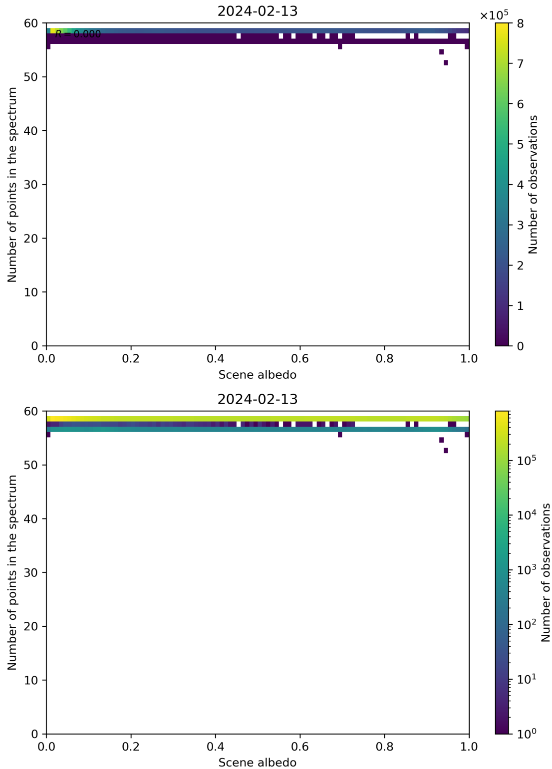
Figure 106: Scatter density plot of “Scene albedo” against “Number of points in the spectrum” for 2024-02-12 to 2024-02-14.
