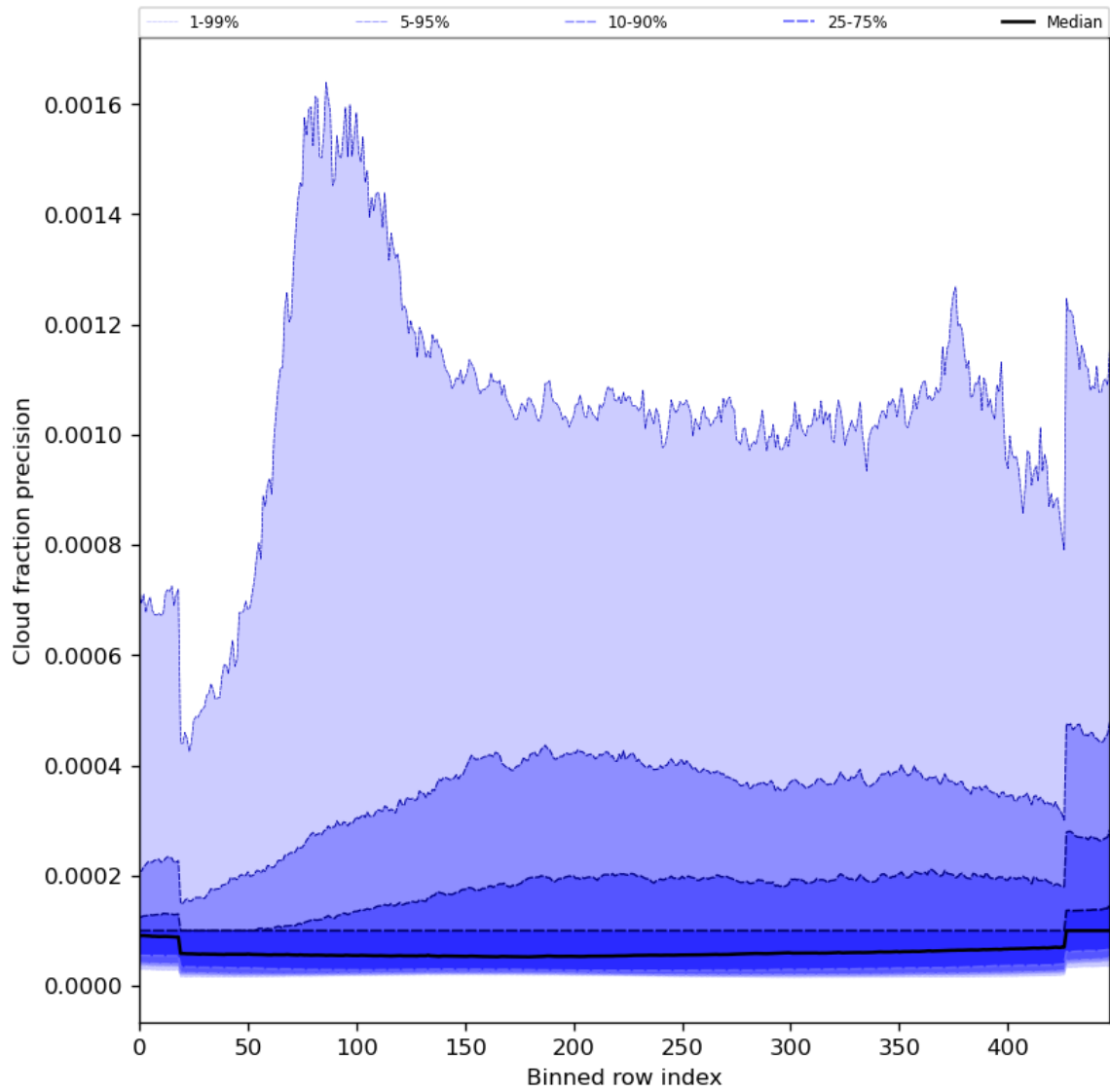
Figure 50: Along track statistics of “Cloud fraction precision” for 2024-02-12 to 2024-02-14
