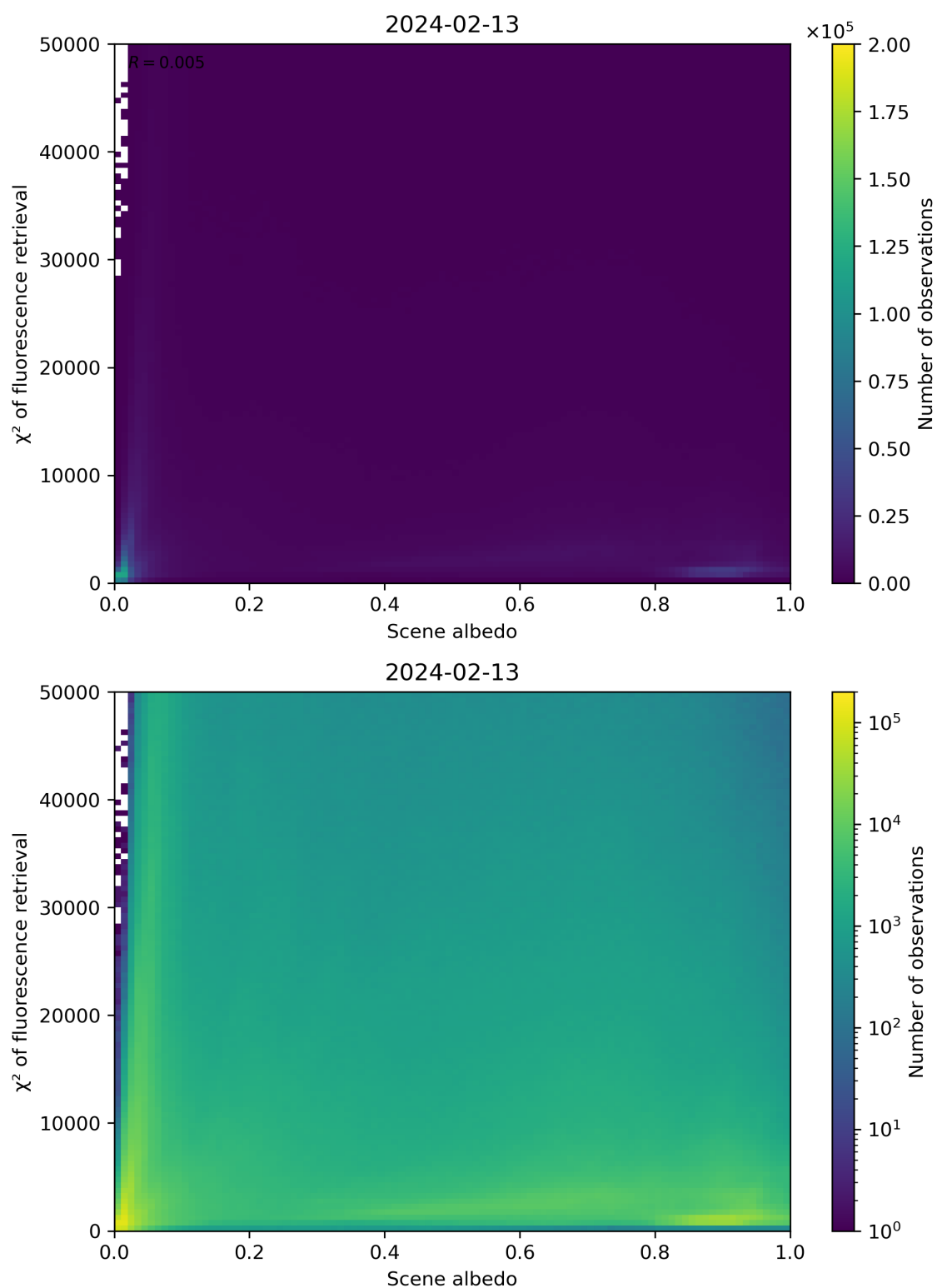
Figure 103: Scatter density plot of “Scene albedo” against “ \chi^2 of fluorescence retrieval” for 2024-02-12 to 2024-02-14.
