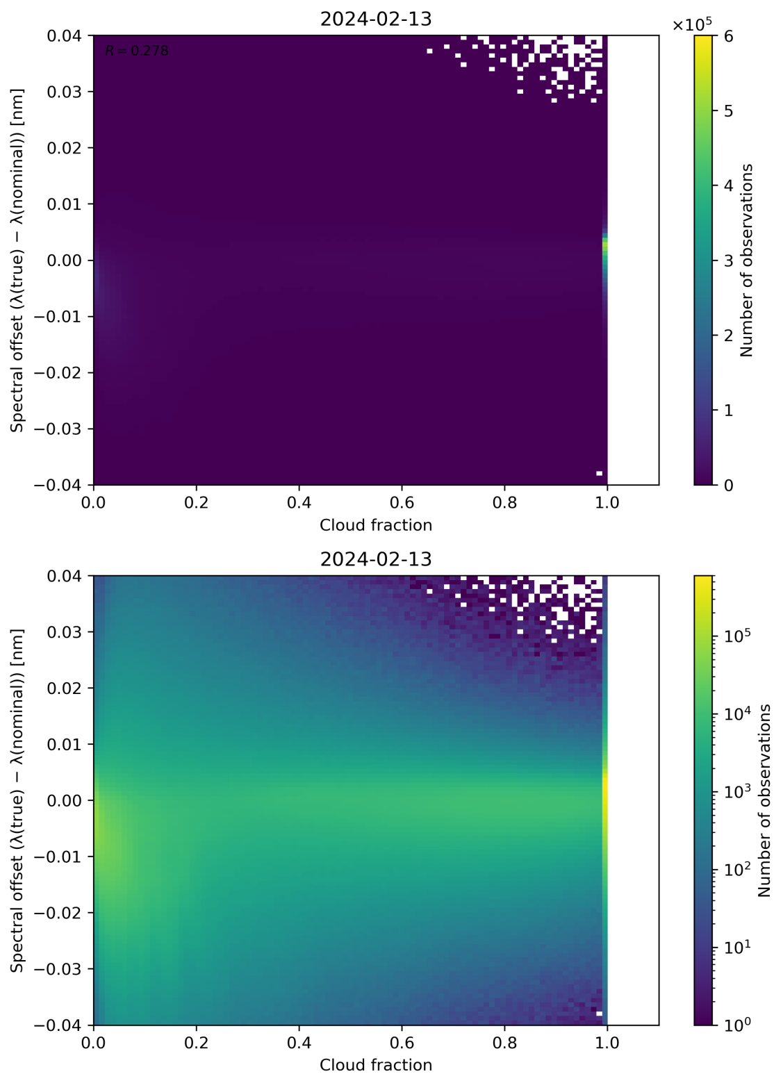
Figure 76: Scatter density plot of “Cloud fraction” against “Spectral offset ( \lambda(\text{true}) - \lambda(\text{nominal}) )” for 2024-02-12 to 2024-02-14.
