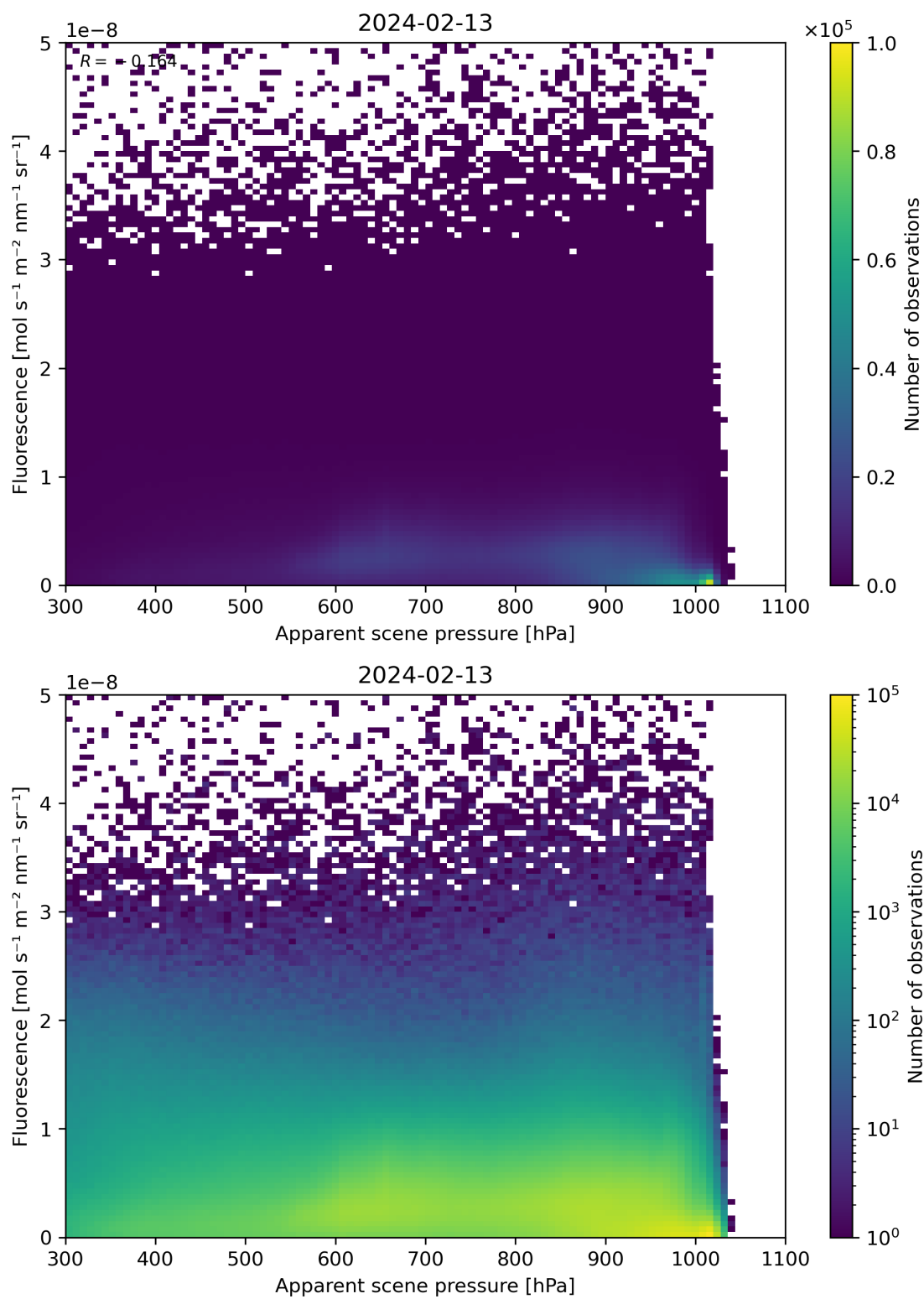
Figure 64: Scatter density plot of “Apparent scene pressure” against “Fluorescence” for 2024-02-12 to 2024-02-14.
