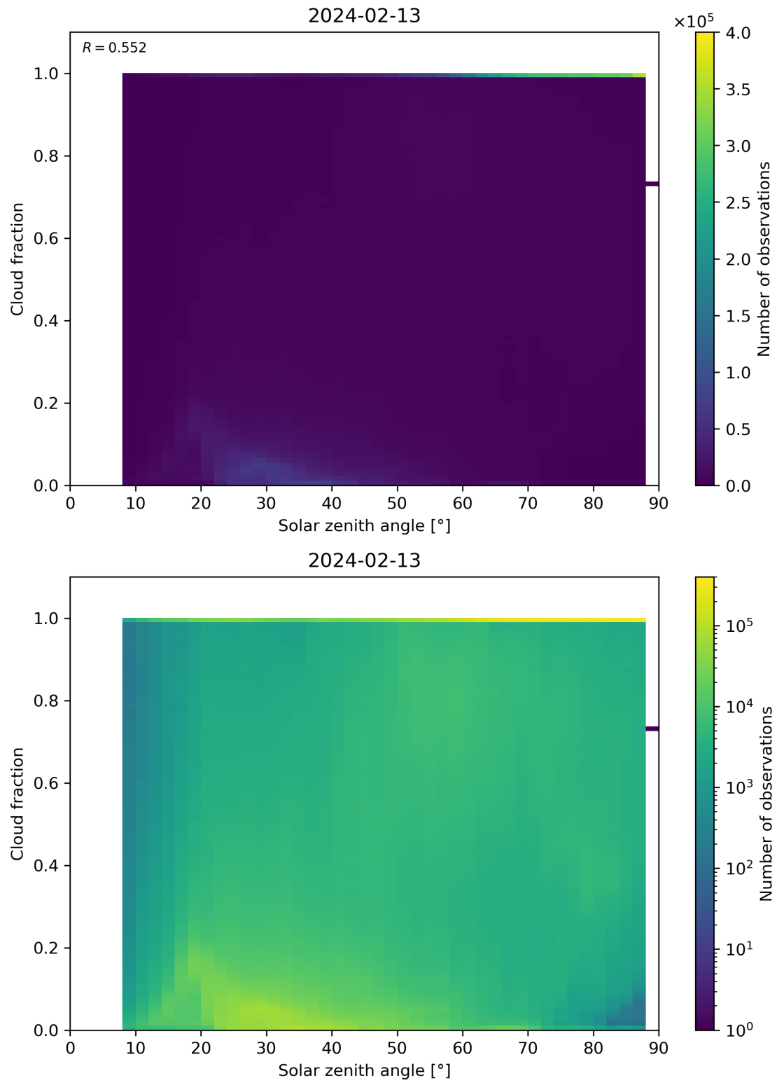
Figure 110: Scatter density plot of “Solar zenith angle” against “Cloud fraction” for 2024-02-12 to 2024-02-14.
