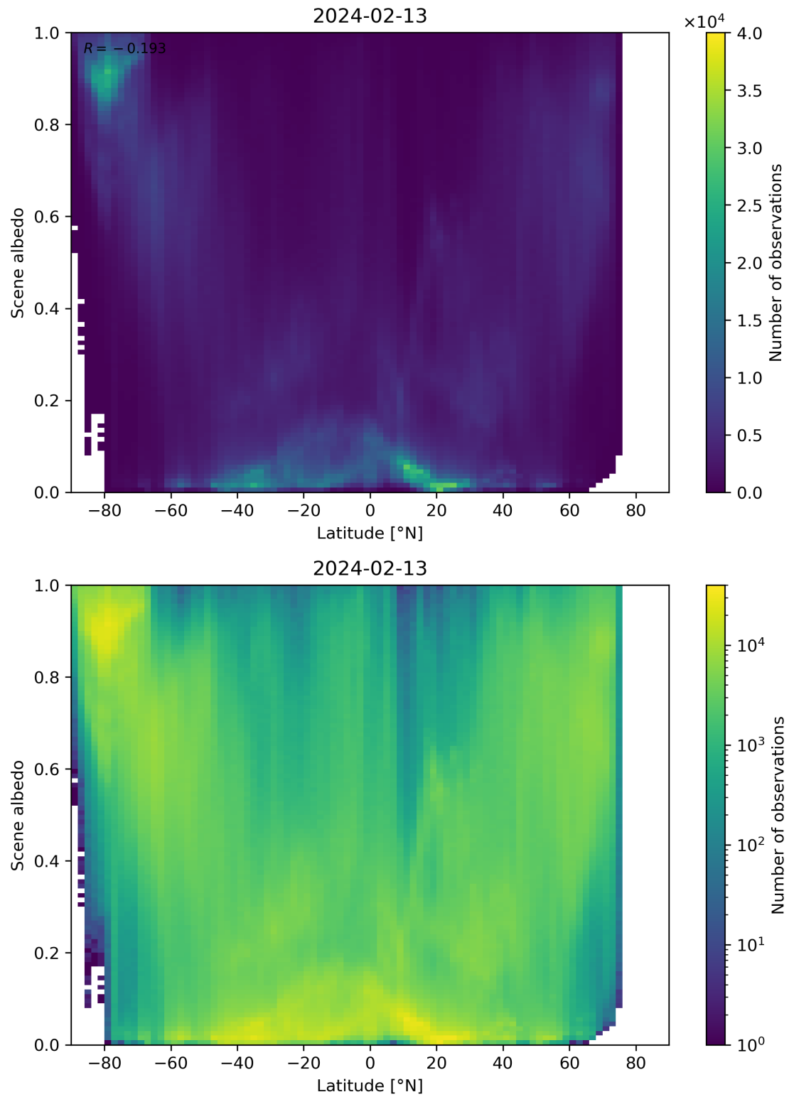
Figure 95: Scatter density plot of “Latitude” against “Scene albedo” for 2024-02-12 to 2024-02-14.
