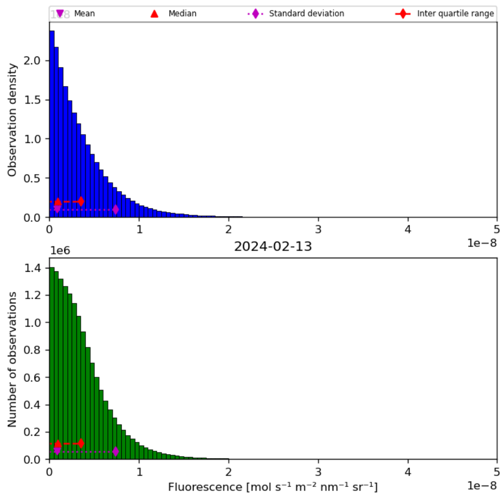
Figure 40: Histogram of “Fluorescence” for 2024-02-12 to 2024-02-14
