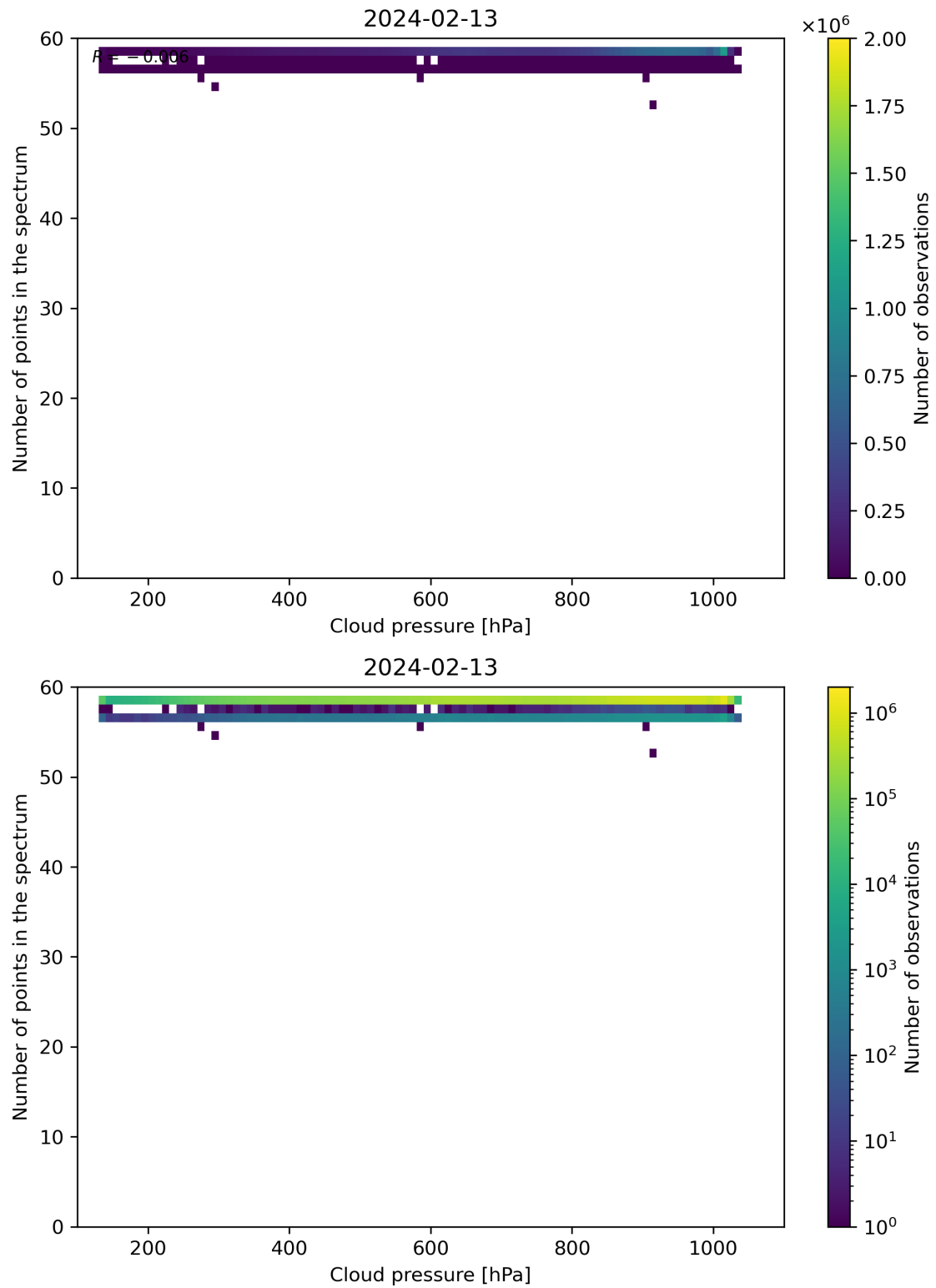
Figure 82: Scatter density plot of “Cloud pressure” against “Number of points in the spectrum” for 2024-02-12 to 2024-02-14.
