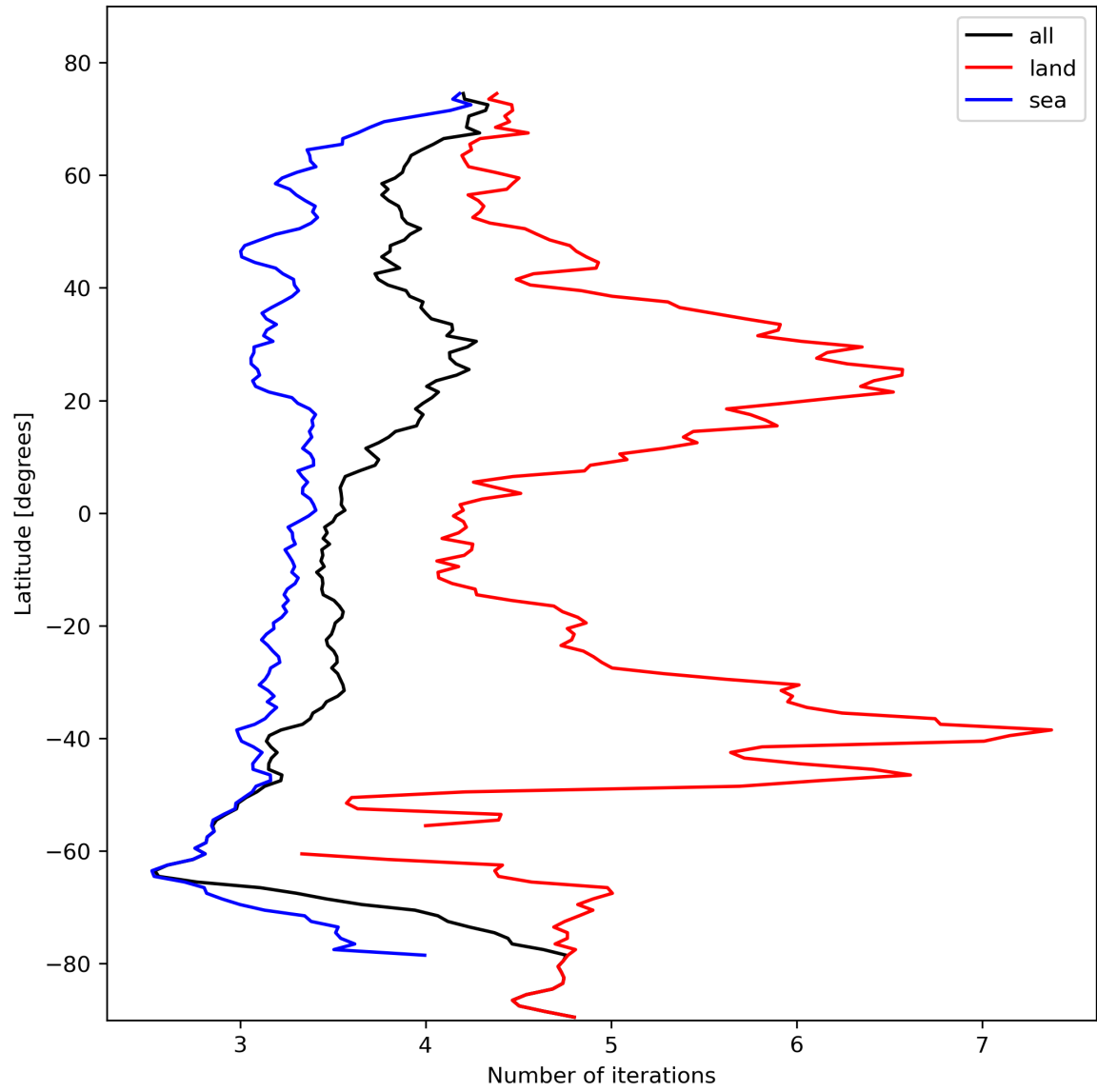
Figure 22: Zonal average of “Number of iterations” for 2024-02-12 to 2024-02-14.
