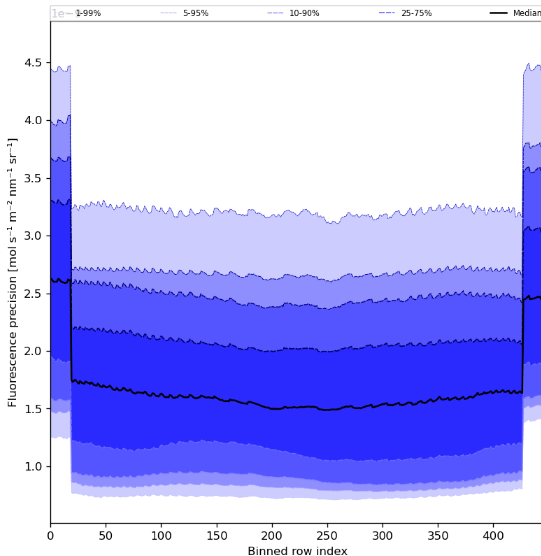
Figure 58: Along track statistics of “Fluorescence precision” for 2024-02-12 to 2024-02-14
