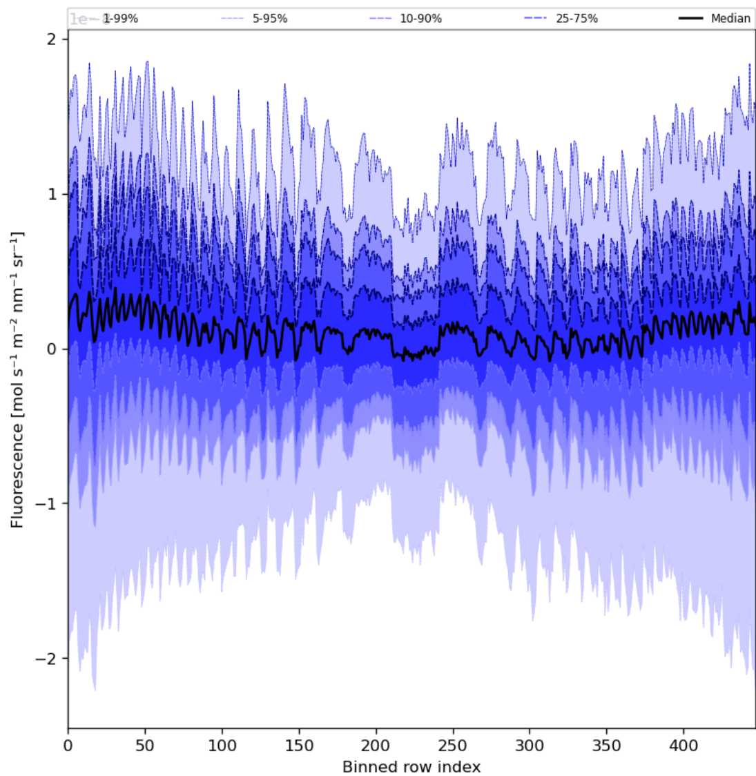
Figure 57: Along track statistics of “Fluorescence” for 2024-02-12 to 2024-02-14
