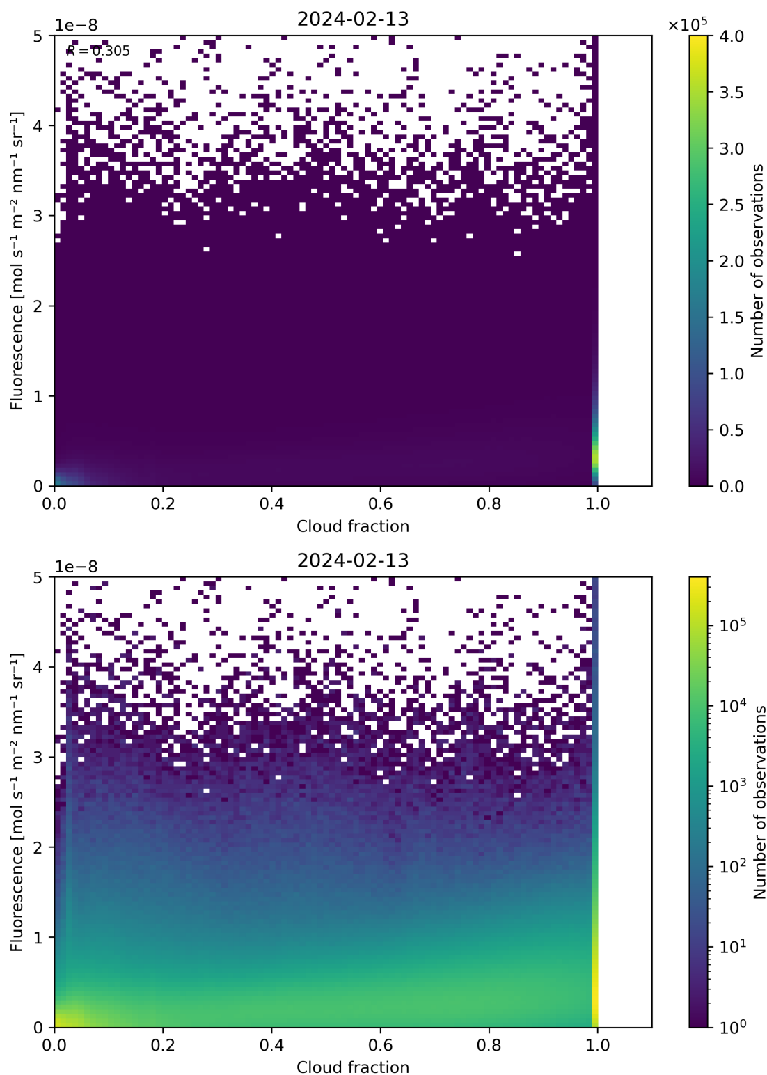
Figure 72: Scatter density plot of “Cloud fraction” against “Fluorescence” for 2024-02-12 to 2024-02-14.
