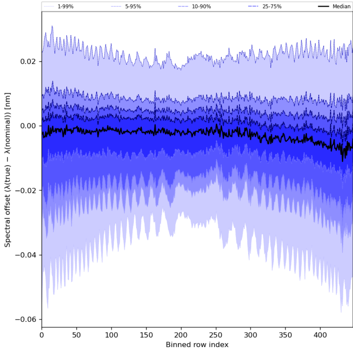
Figure 62: Along track statistics of “Spectral offset ( \lambda(\text{true}) - \lambda(\text{nominal}) )” for 2024-02-12 to 2024-02-14
