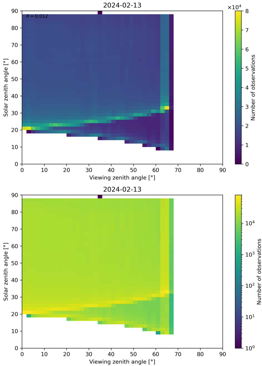
Figure 127: Scatter density plot of “Viewing zenith angle” against “Solar zenith angle” for 2024-02-12 to 2024-02-14.
