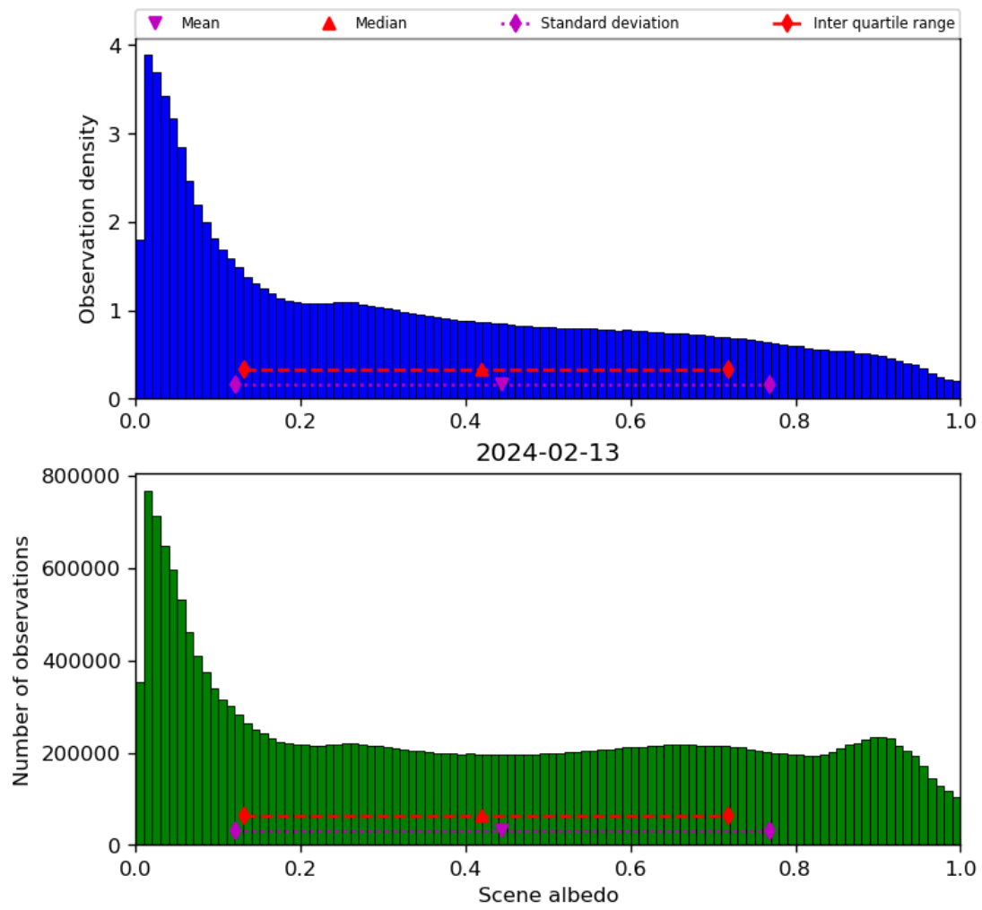
Figure 34: Histogram of “Scene albedo” for 2024-02-12 to 2024-02-14
