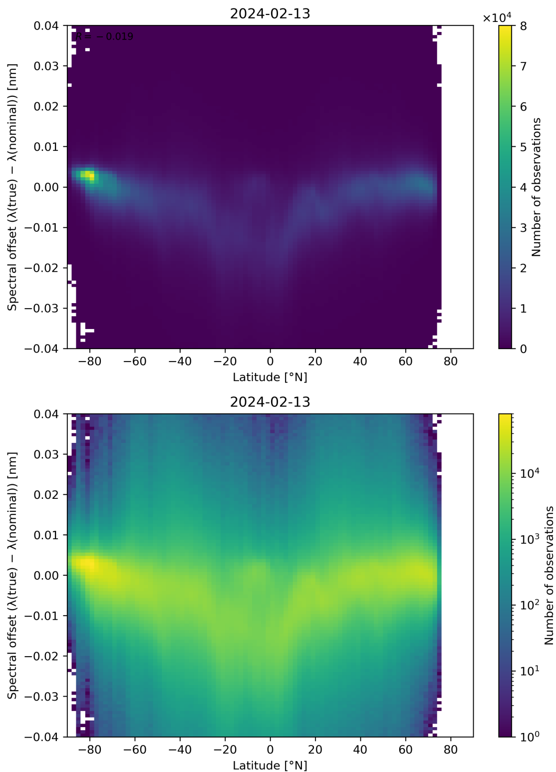
Figure 96: Scatter density plot of “Latitude” against “Spectral offset ( \lambda(\text{true}) - \lambda(\text{nominal}) )” for 2024-02-12 to 2024-02-14.
