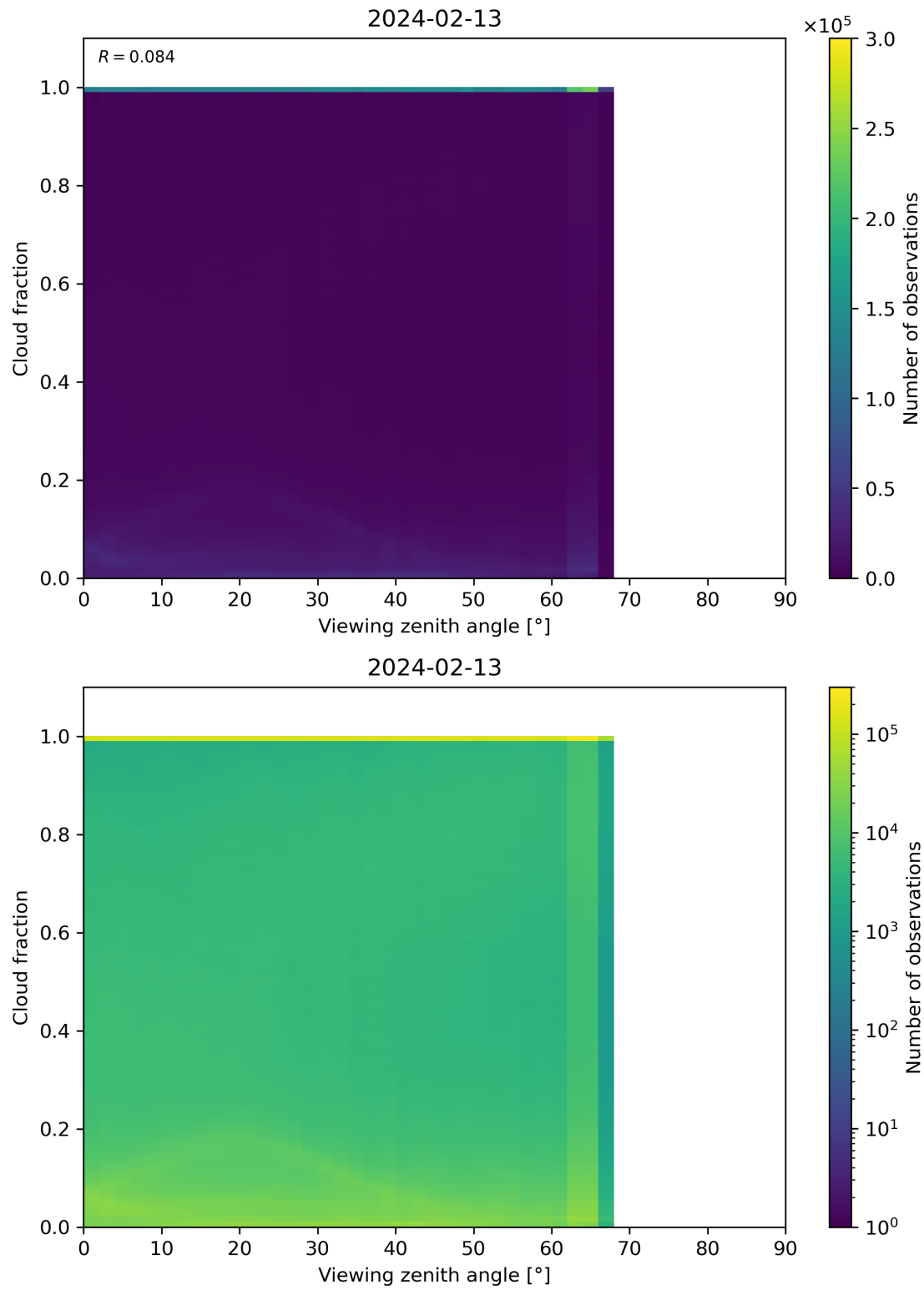
Figure 120: Scatter density plot of “Viewing zenith angle” against “Cloud fraction” for 2024-02-12 to 2024-02-14.
