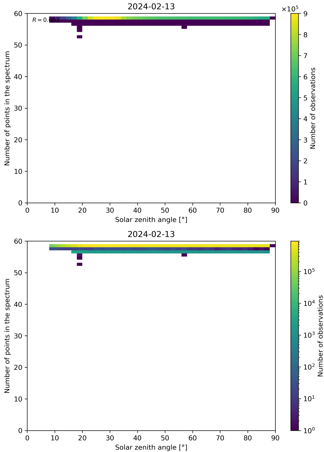
Figure 115: Scatter density plot of “Solar zenith angle” against “Number of points in the spectrum” for 2024-02-12 to 2024-02-14.
