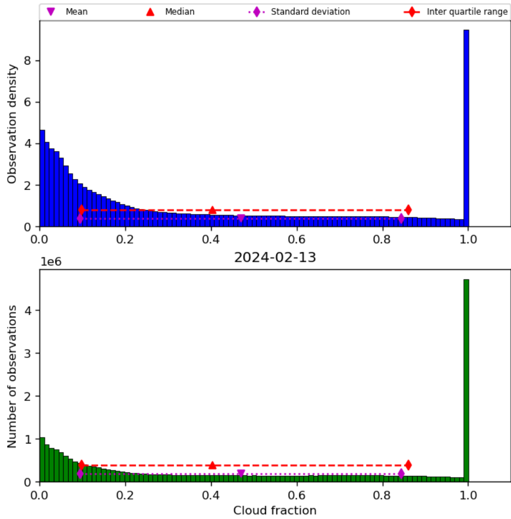
Figure 32: Histogram of “Cloud fraction” for 2024-02-12 to 2024-02-14
