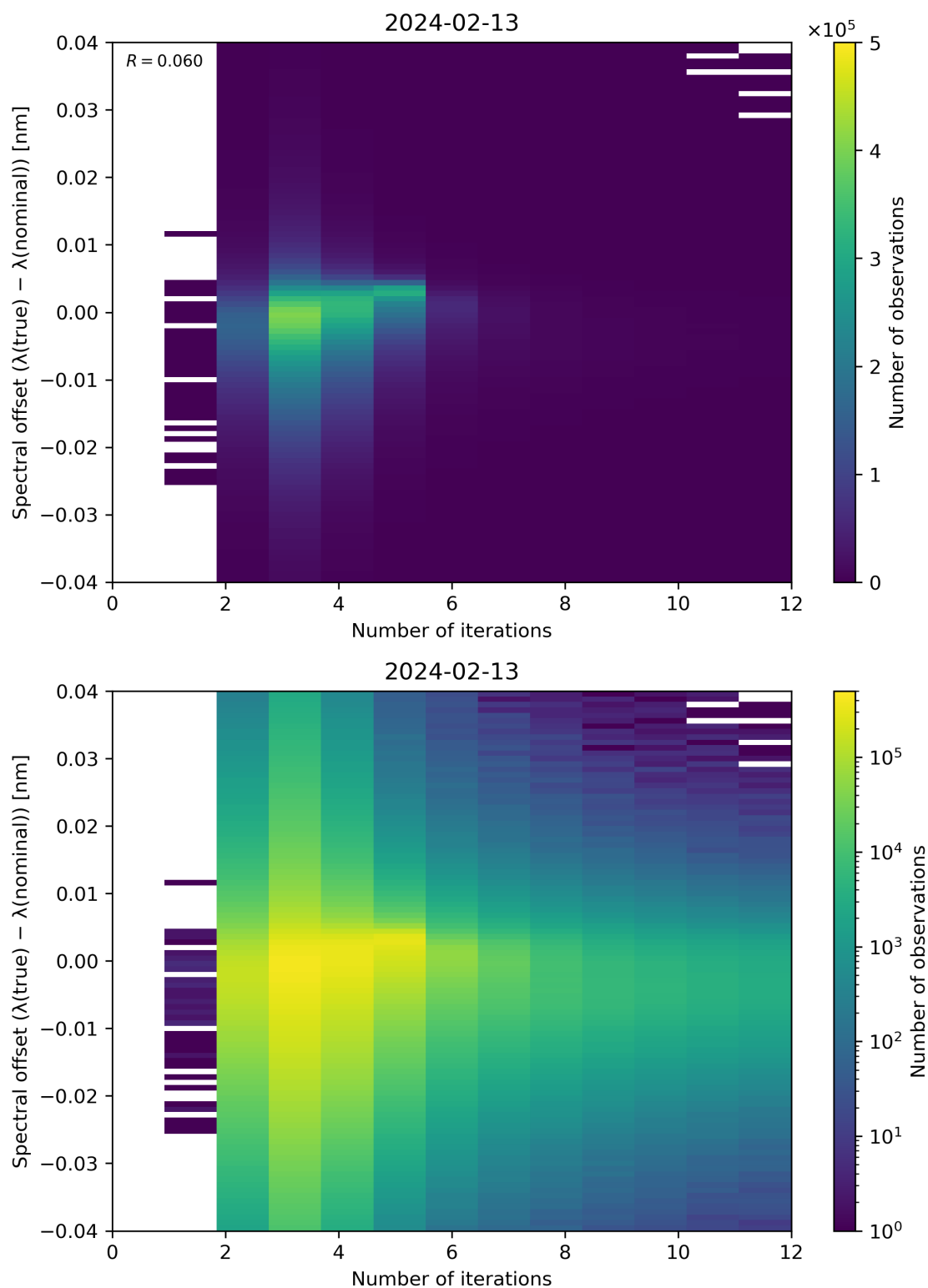
Figure 100: Scatter density plot of “Number of iterations” against “Spectral offset ( \lambda(\text{true}) - \lambda(\text{nominal}) )” for 2024-02-12 to 2024-02-14.
