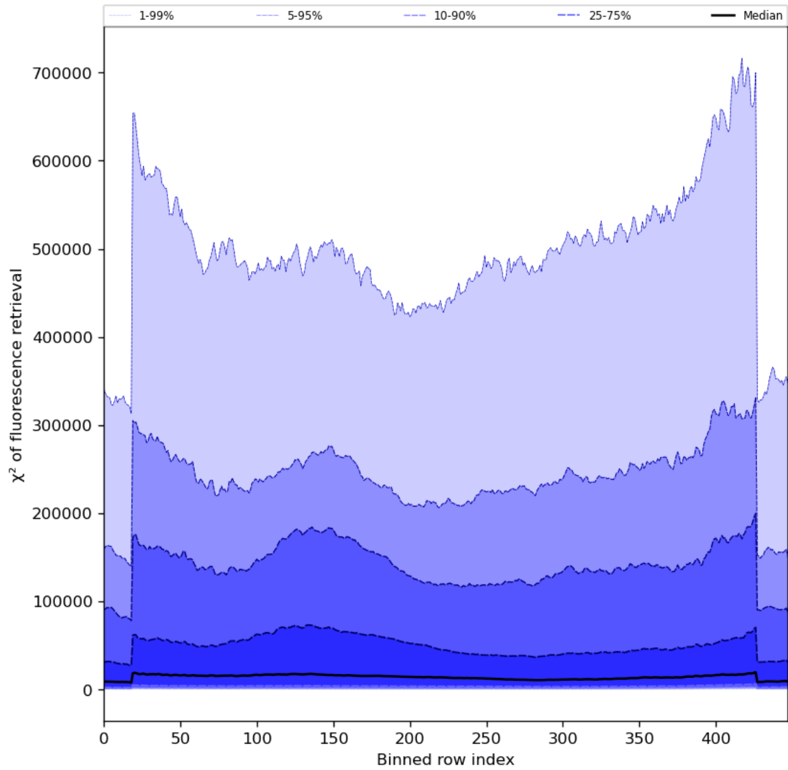
Figure 59: Along track statistics of " \chi^2 of fluorescence retrieval" for 2024-02-12 to 2024-02-14
