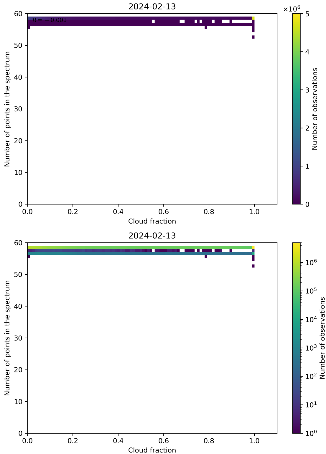
Figure 74: Scatter density plot of “Cloud fraction” against “Number of points in the spectrum” for 2024-02-12 to 2024-02-14.
