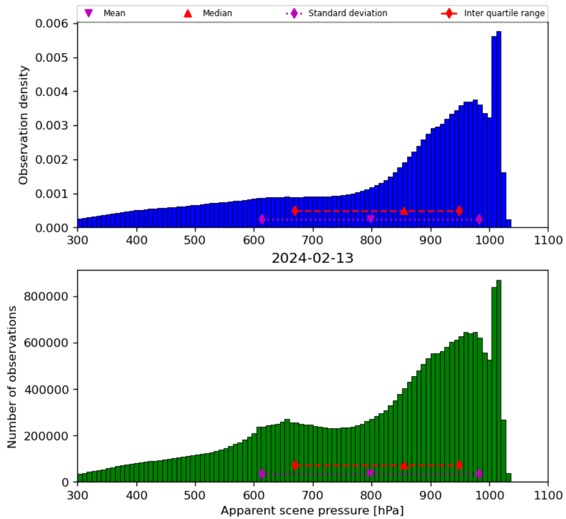
Figure 36: Histogram of “Apparent scene pressure” for 2024-02-12 to 2024-02-14
