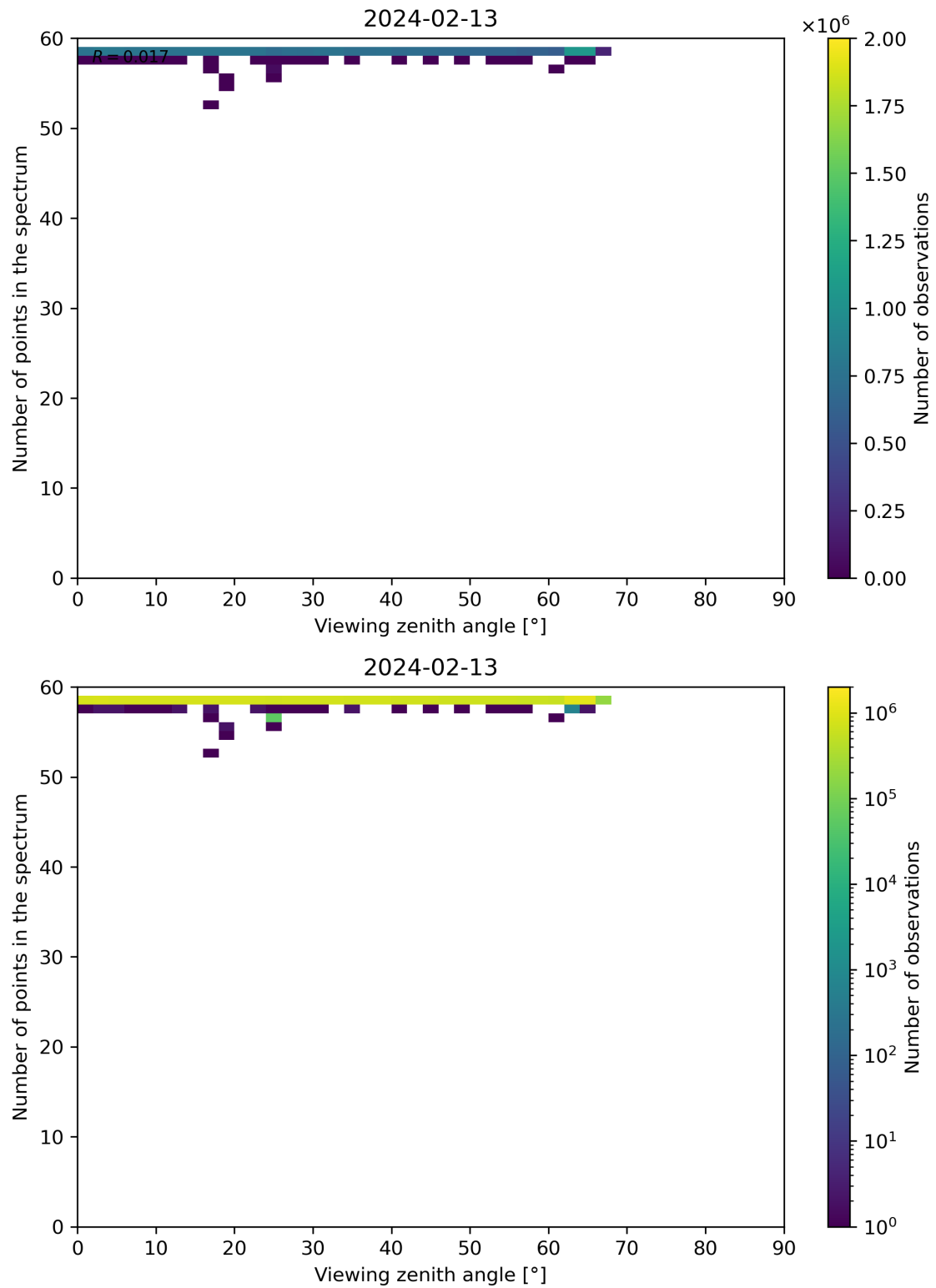
Figure 125: Scatter density plot of “Viewing zenith angle” against “Number of points in the spectrum” for 2024-02-12 to 2024-02-14.
