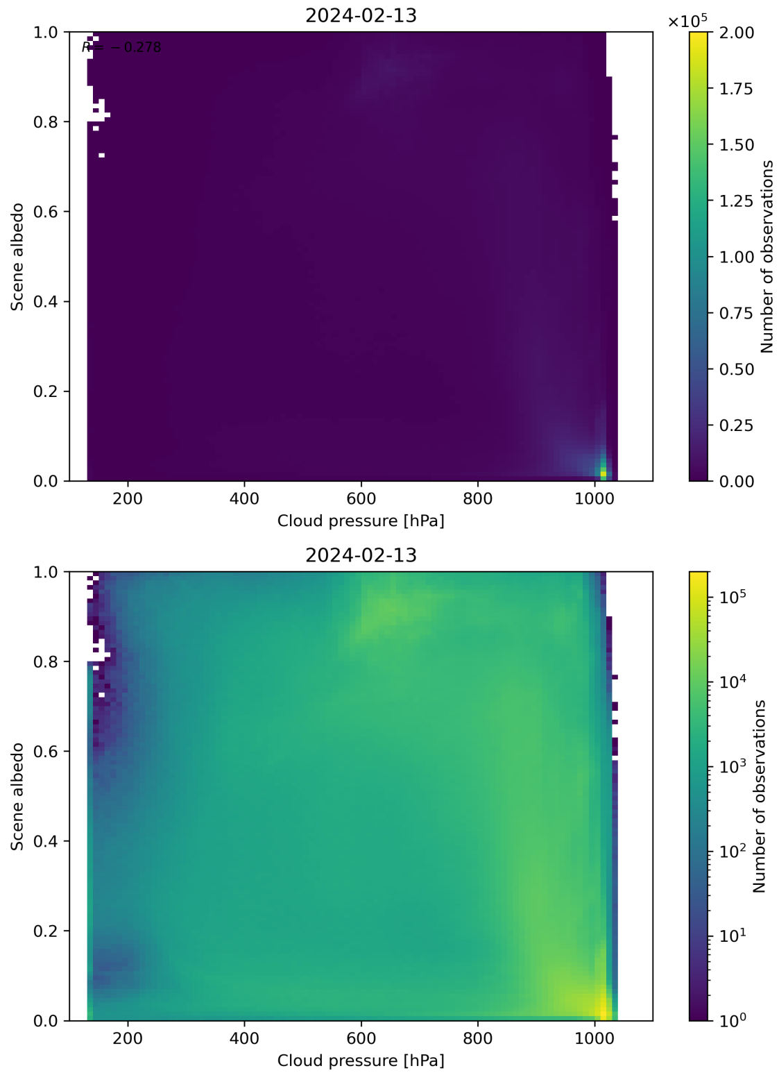
Figure 83: Scatter density plot of “Cloud pressure” against “Scene albedo” for 2024-02-12 to 2024-02-14.
