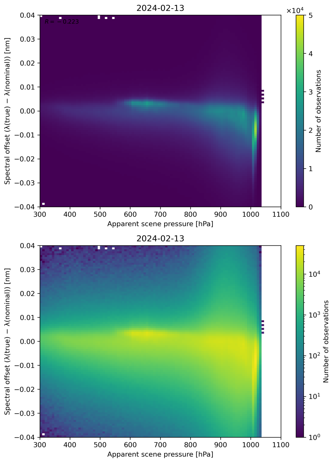
Figure 67: Scatter density plot of “Apparent scene pressure” against “Spectral offset ( \lambda(\text{true}) - \lambda(\text{nominal}) )” for 2024-02-12 to 2024-02-14.
