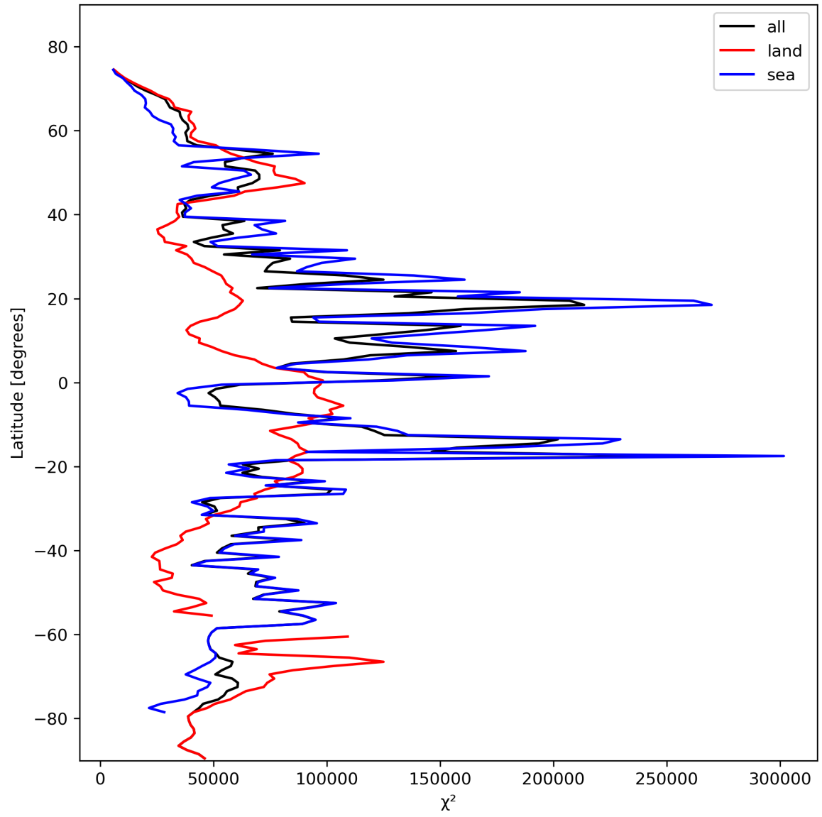
Figure 21: Zonal average of “ \chi^2 ” for 2024-02-12 to 2024-02-14.
