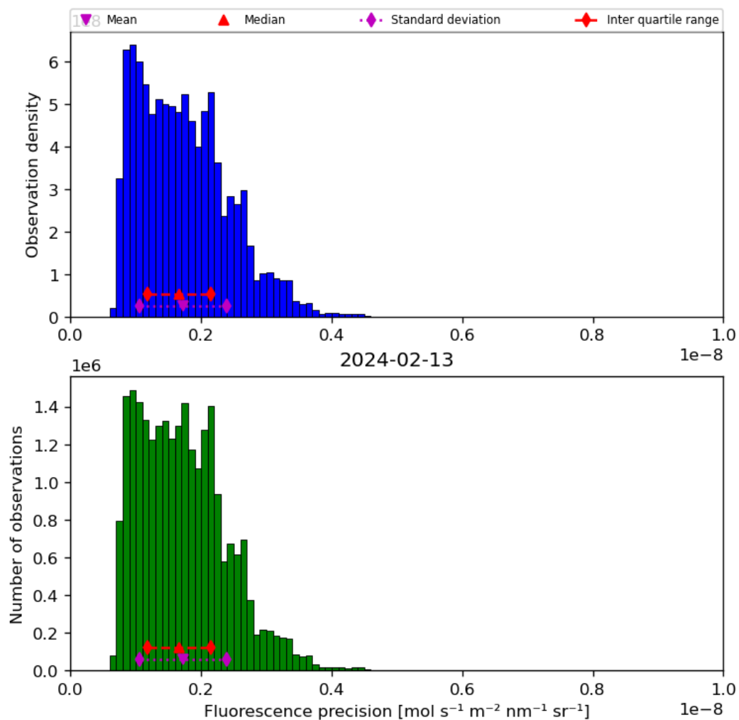
Figure 41: Histogram of “Fluorescence precision” for 2024-02-12 to 2024-02-14
