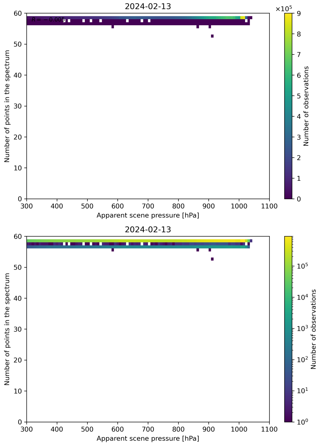
Figure 66: Scatter density plot of “Apparent scene pressure” against “Number of points in the spectrum” for 2024-02-12 to 2024-02-14.
