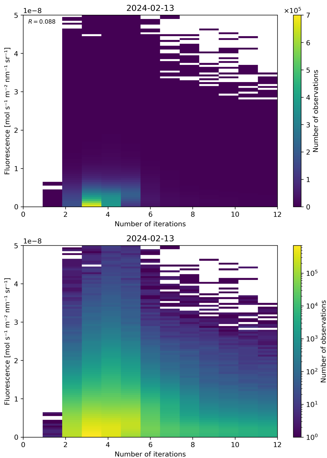
Figure 98: Scatter density plot of “Number of iterations” against “Fluorescence” for 2024-02-12 to 2024-02-14.
