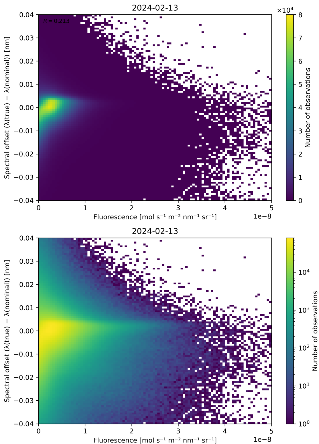
Figure 87: Scatter density plot of “Fluorescence” against “Spectral offset ( \lambda(\text{true}) - \lambda(\text{nominal}) )” for 2024-02-12 to 2024-02-14.
