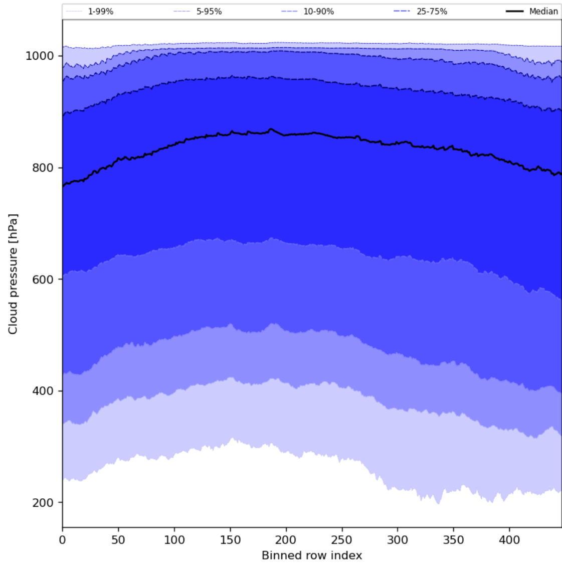
Figure 47: Along track statistics of “Cloud pressure” for 2024-02-12 to 2024-02-14
