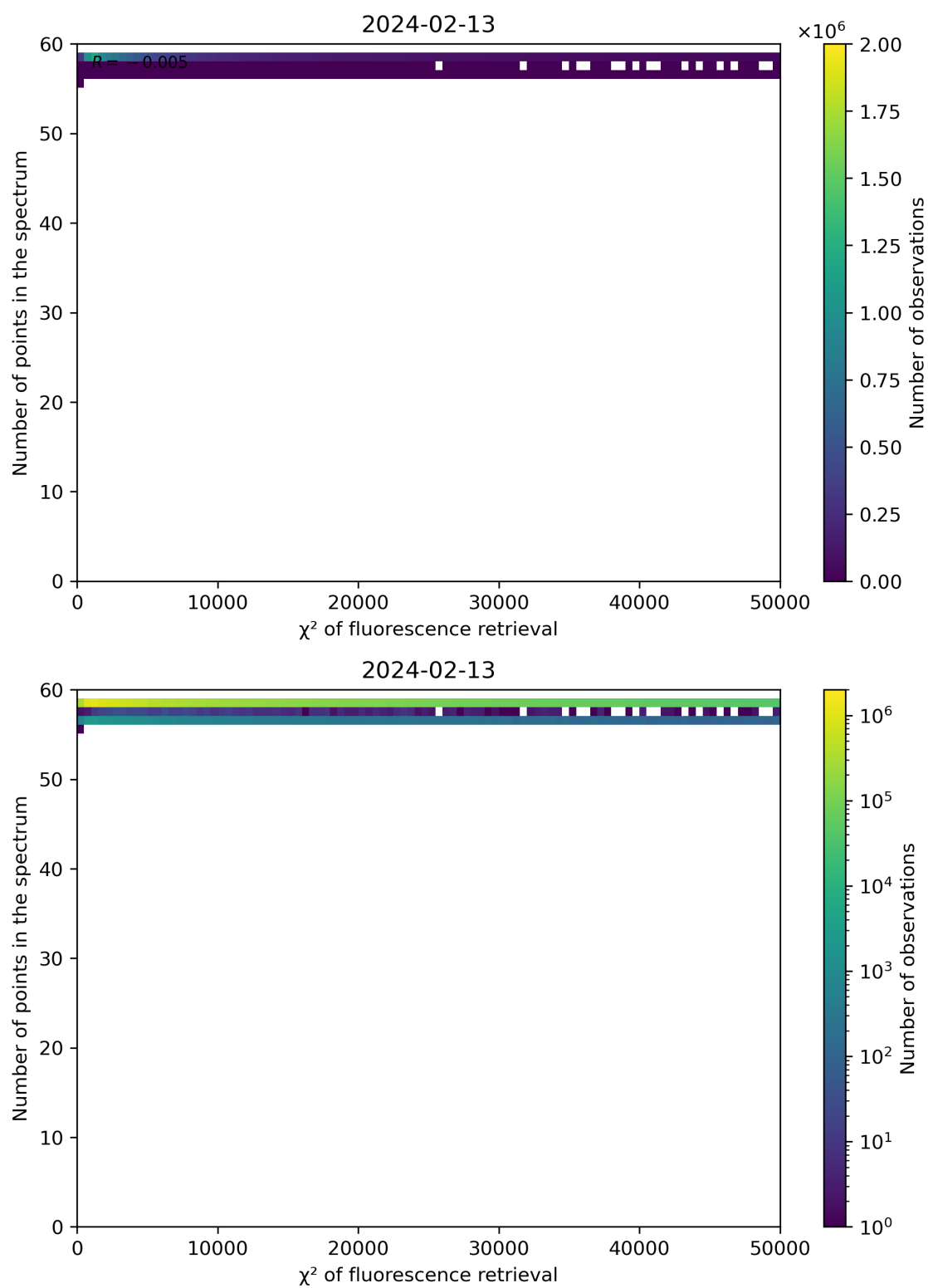
Figure 68: Scatter density plot of " \chi^2 of fluorescence retrieval" against "Number of points in the spectrum" for 2024-02-12 to 2024-02-14.
