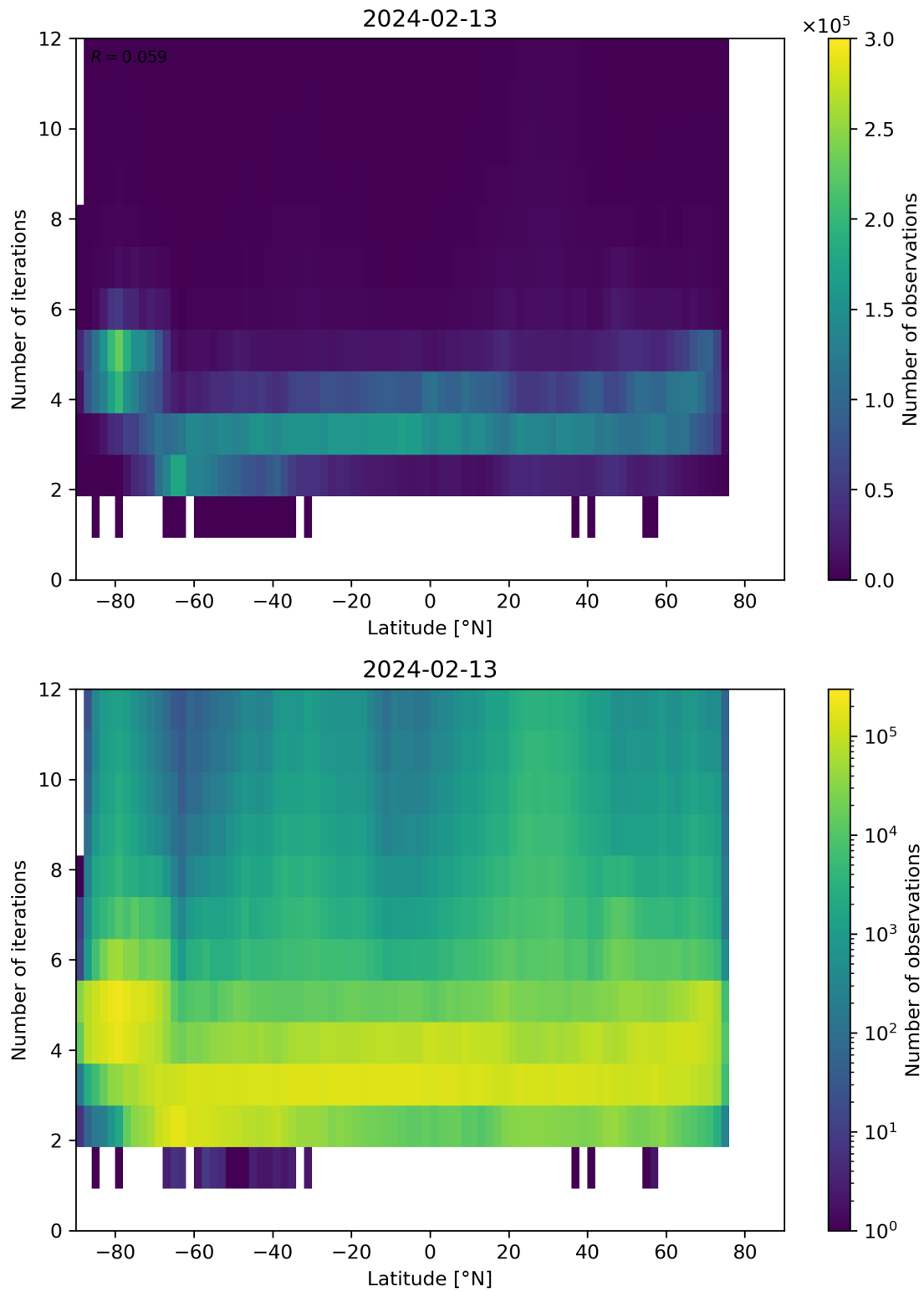
Figure 93: Scatter density plot of “Latitude” against “Number of iterations” for 2024-02-12 to 2024-02-14.
