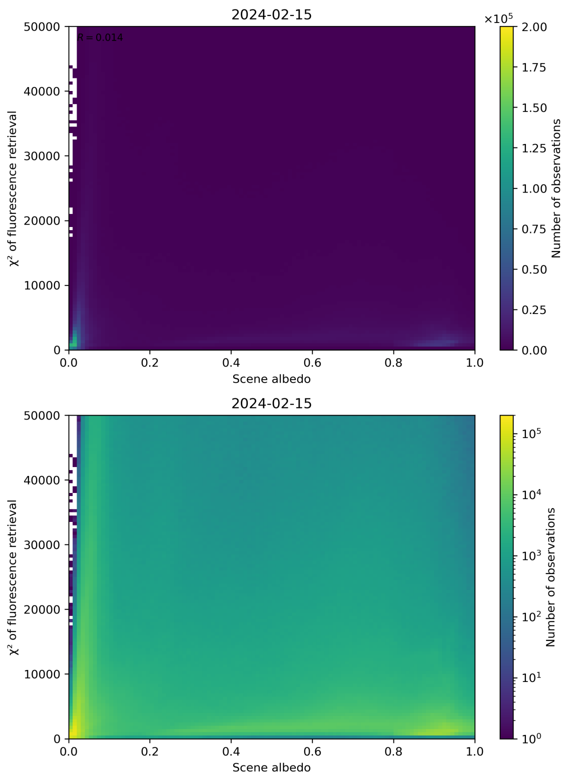
Figure 103: Scatter density plot of “Scene albedo” against “ \chi^2 of fluorescence retrieval” for 2024-02-14 to 2024-02-16.
