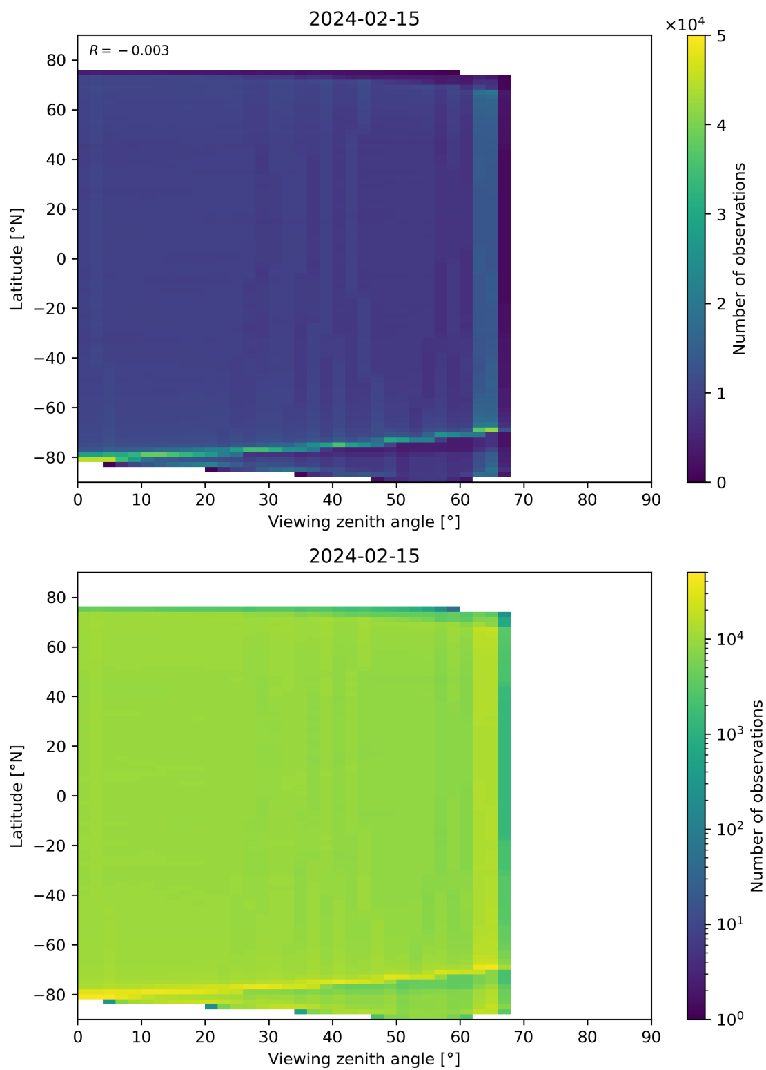
Figure 123: Scatter density plot of “Viewing zenith angle” against “Latitude” for 2024-02-14 to 2024-02-16.
