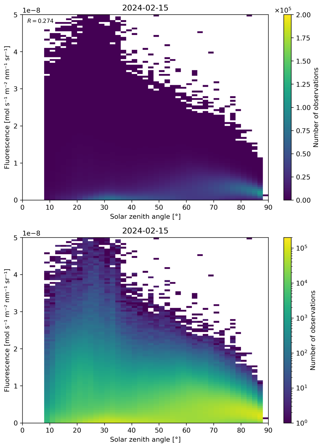
Figure 112: Scatter density plot of “Solar zenith angle” against “Fluorescence” for 2024-02-14 to 2024-02-16.
