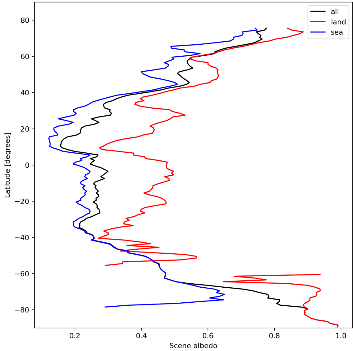
Figure 17: Zonal average of “Scene albedo” for 2024-02-14 to 2024-02-16.
