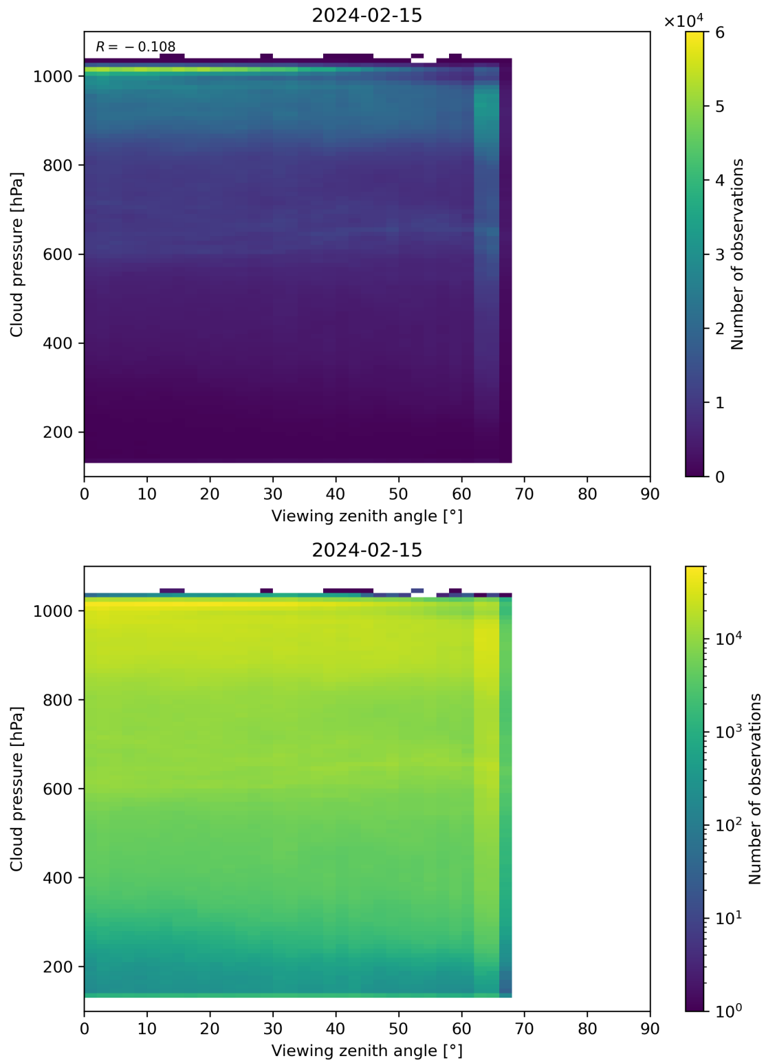
Figure 121: Scatter density plot of “Viewing zenith angle” against “Cloud pressure” for 2024-02-14 to 2024-02-16.
