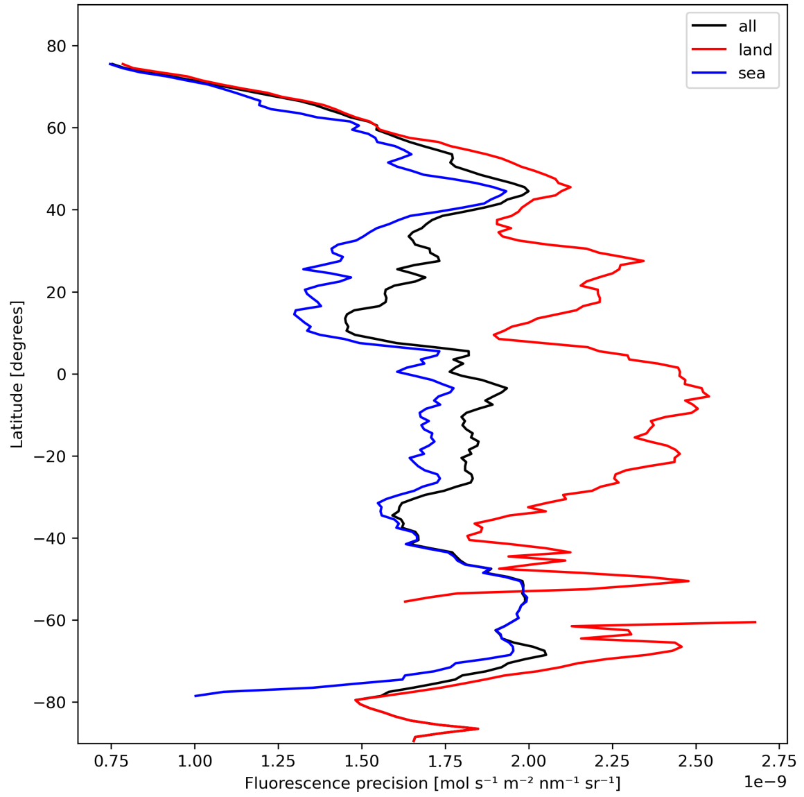
Figure 24: Zonal average of “Fluorescence precision” for 2024-02-14 to 2024-02-16.
