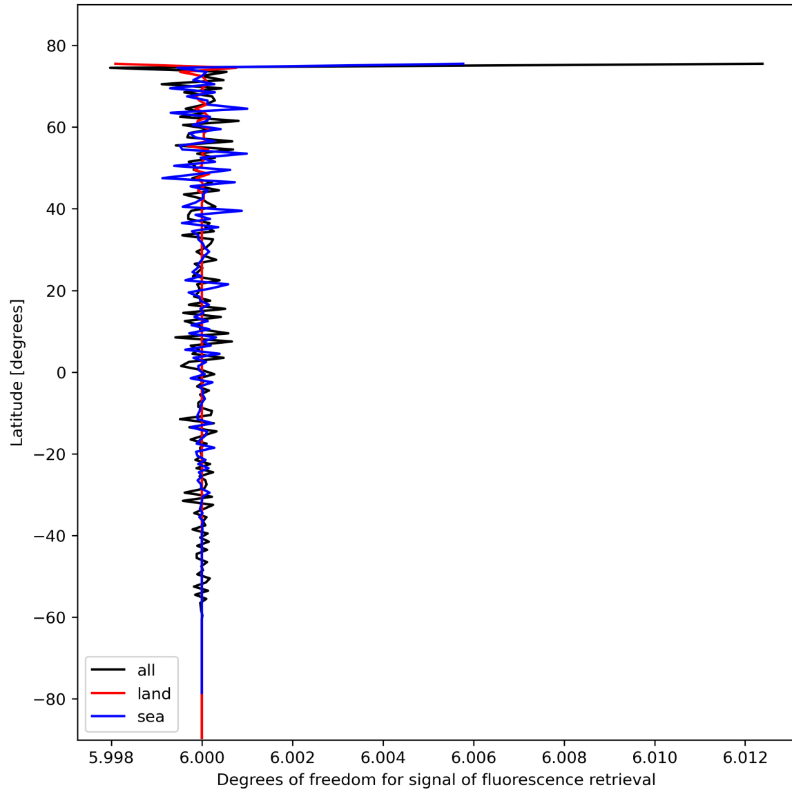
Figure 26: Zonal average of “Degrees of freedom for signal of fluorescence retrieval” for 2024-02-14 to 2024-02-16.
