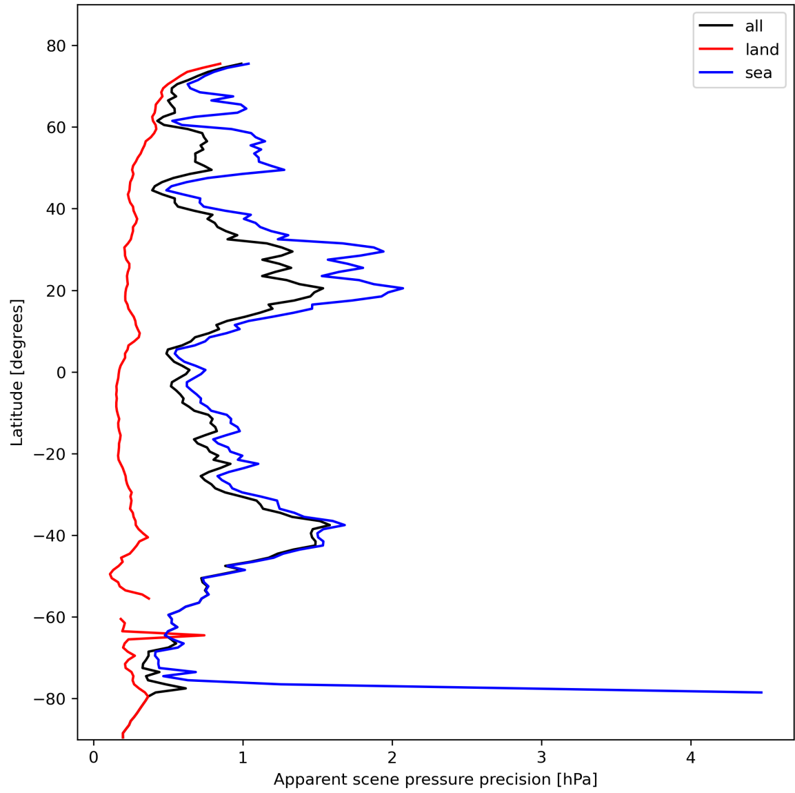
Figure 20: Zonal average of “Apparent scene pressure precision” for 2024-02-14 to 2024-02-16.
