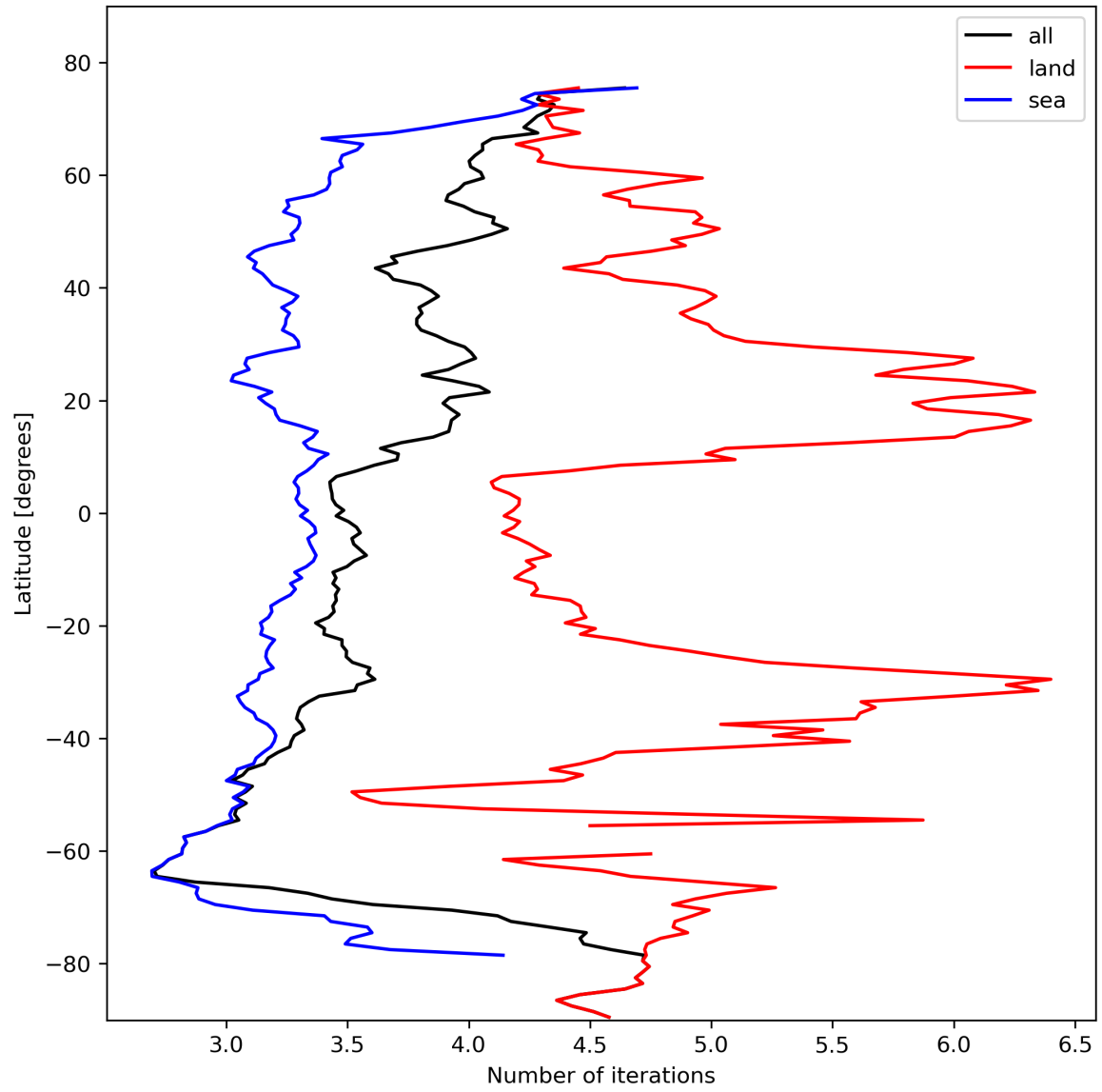
Figure 22: Zonal average of “Number of iterations” for 2024-02-14 to 2024-02-16.
