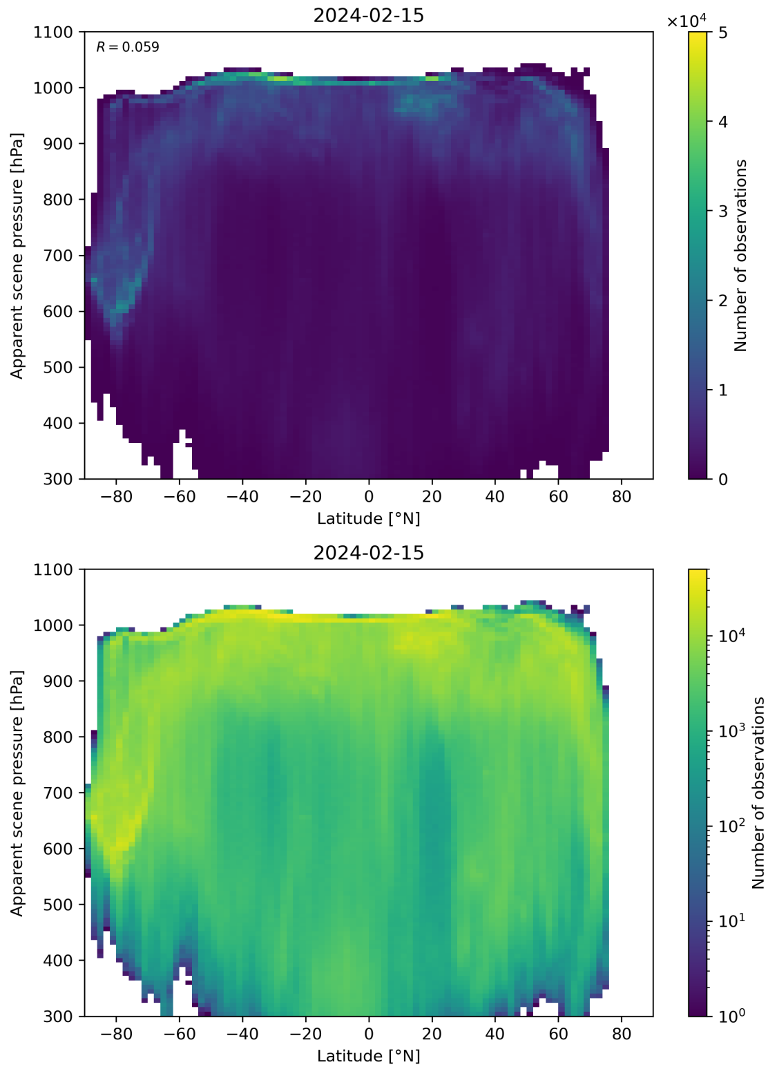
Figure 88: Scatter density plot of “Latitude” against “Apparent scene pressure” for 2024-02-14 to 2024-02-16.
