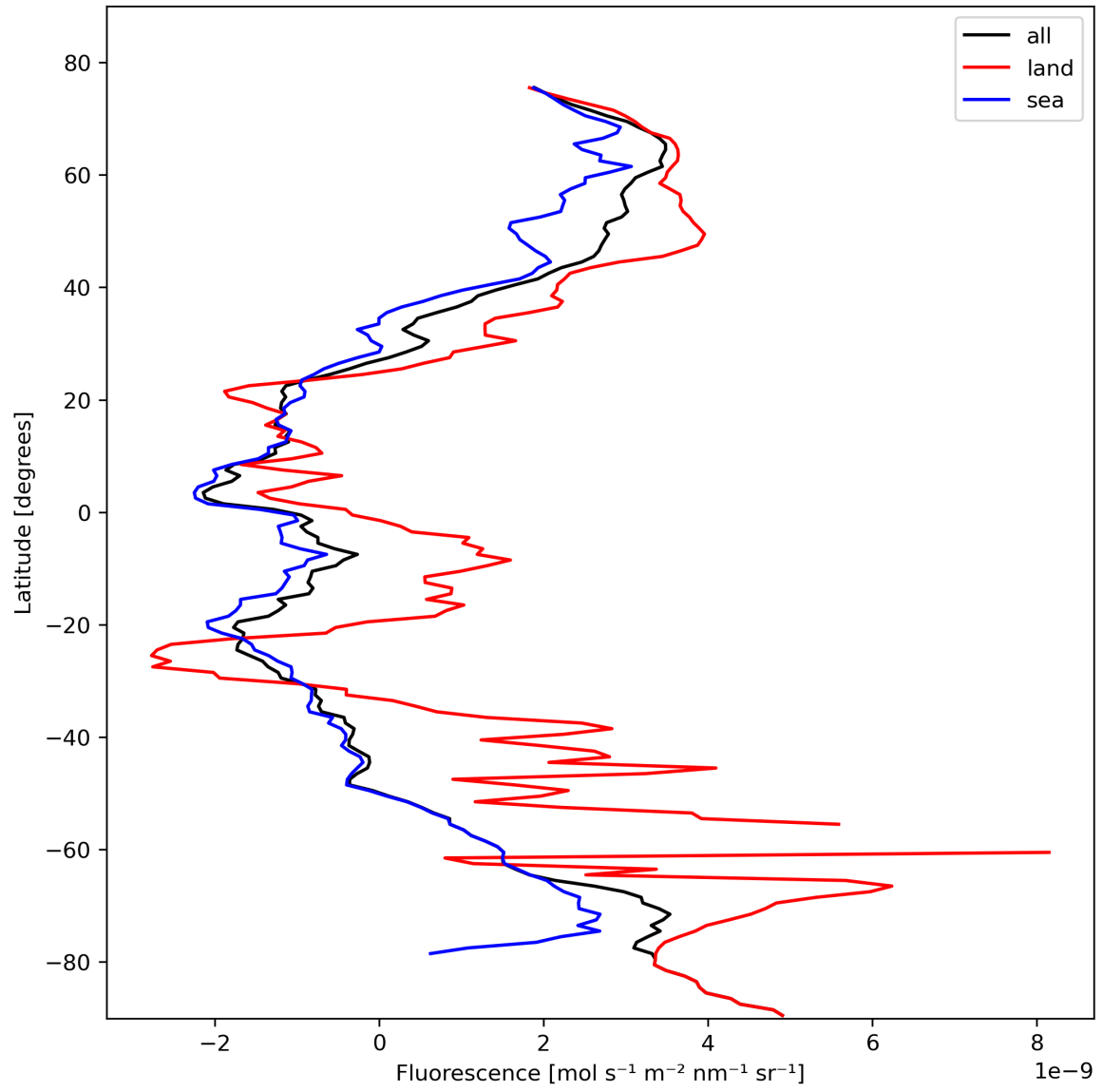
Figure 23: Zonal average of “Fluorescence” for 2024-02-14 to 2024-02-16.
