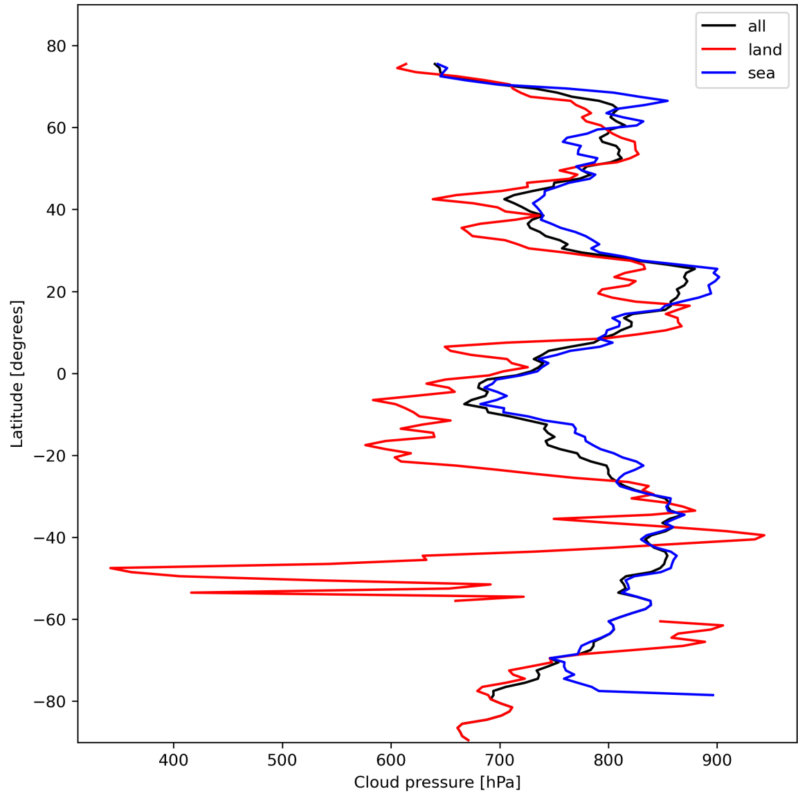
Figure 13: Zonal average of “Cloud pressure” for 2024-02-14 to 2024-02-16.
