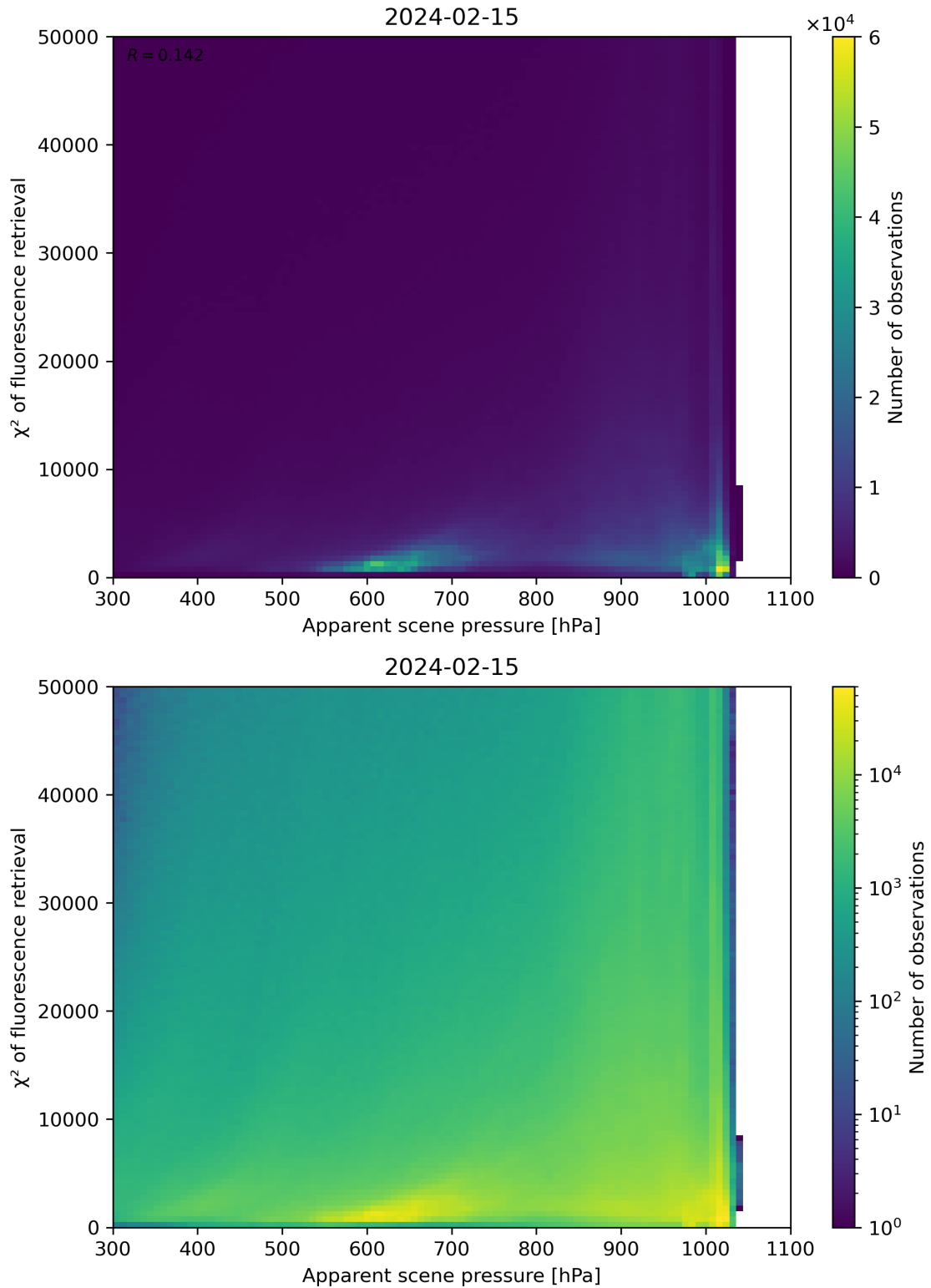
Figure 63: Scatter density plot of “Apparent scene pressure” against “ \chi^2 of fluorescence retrieval” for 2024-02-14 to 2024-02-16.
