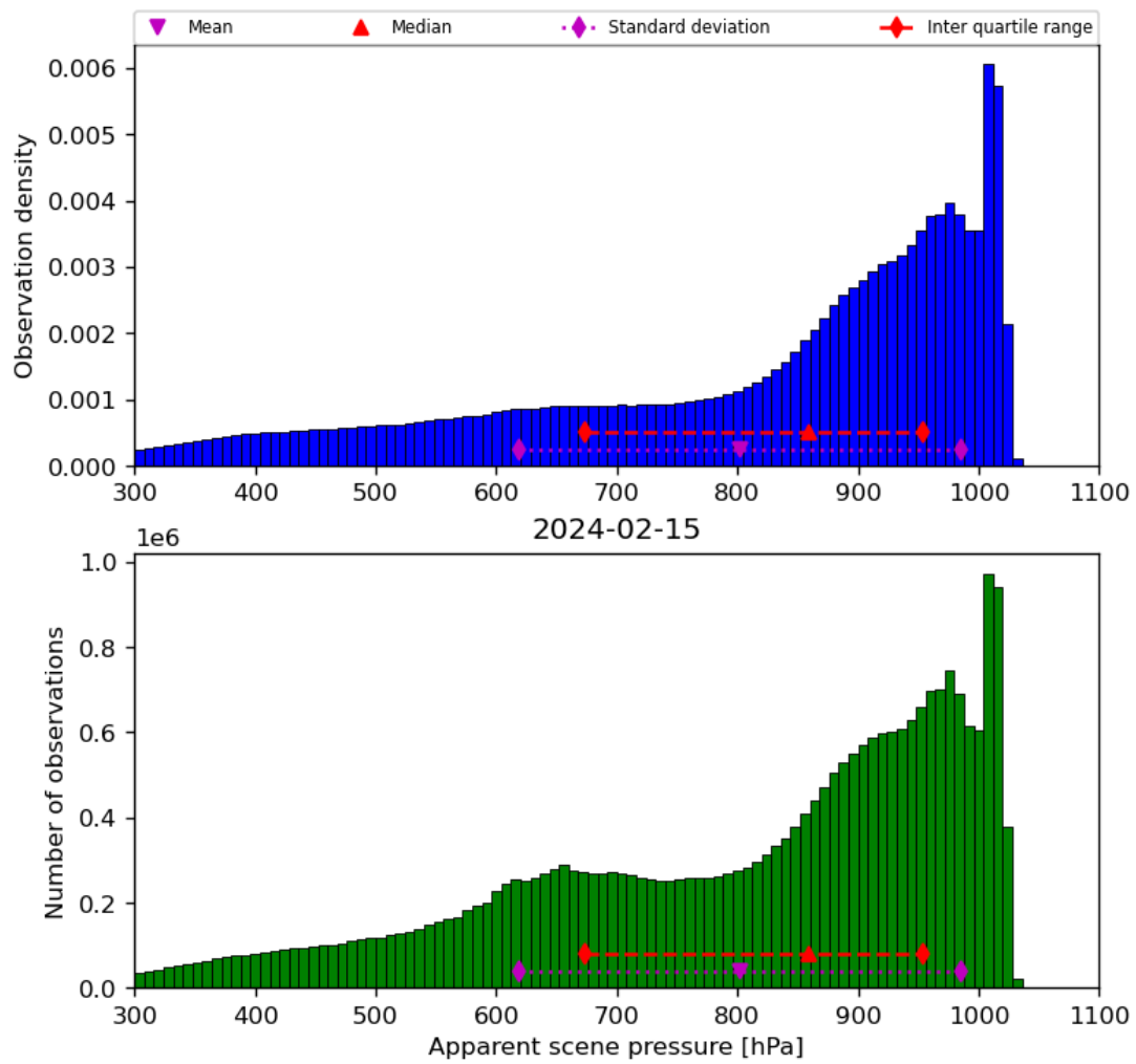
Figure 36: Histogram of “Apparent scene pressure” for 2024-02-14 to 2024-02-16
