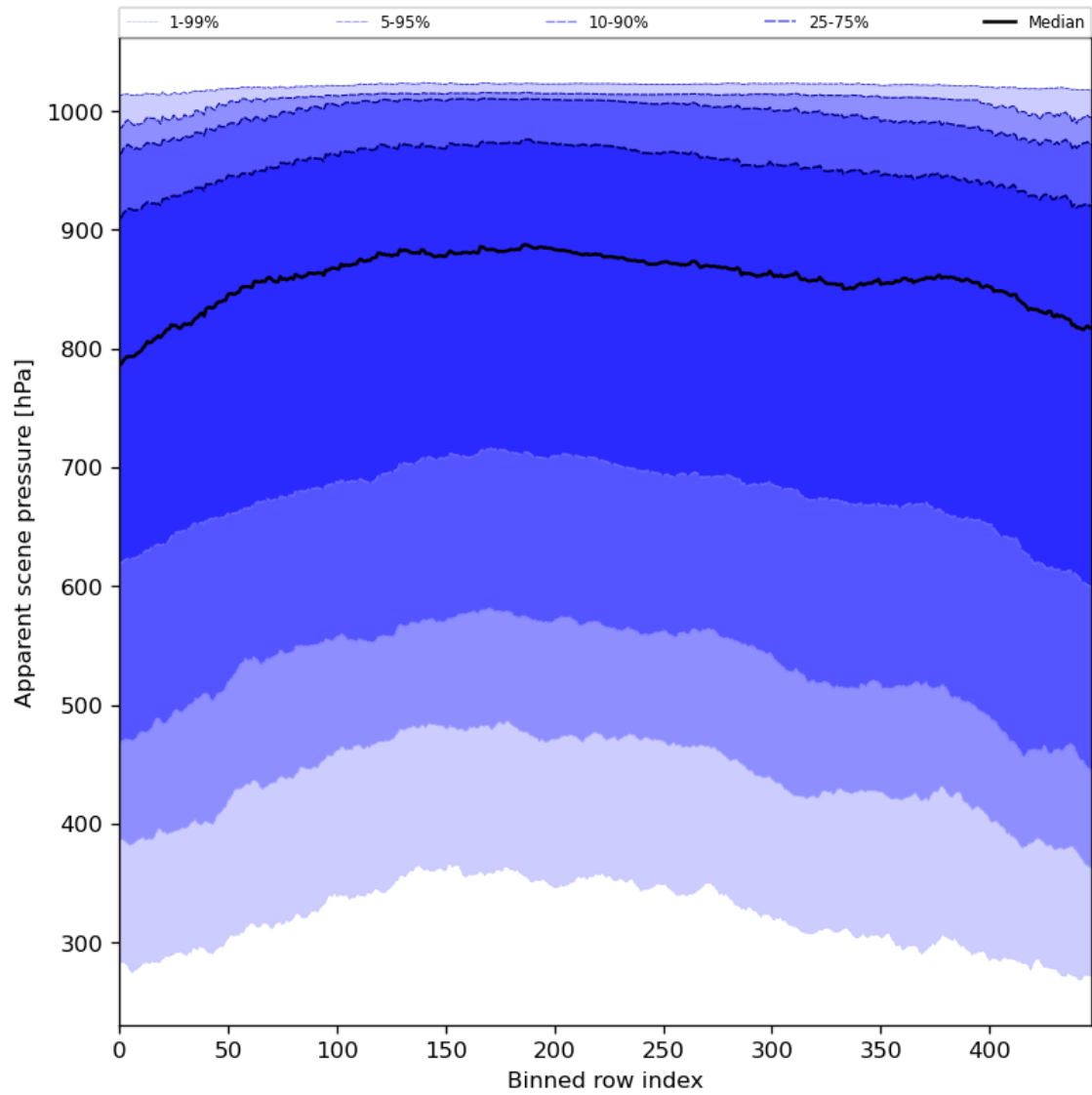
Figure 53: Along track statistics of “Apparent scene pressure” for 2024-02-14 to 2024-02-16
