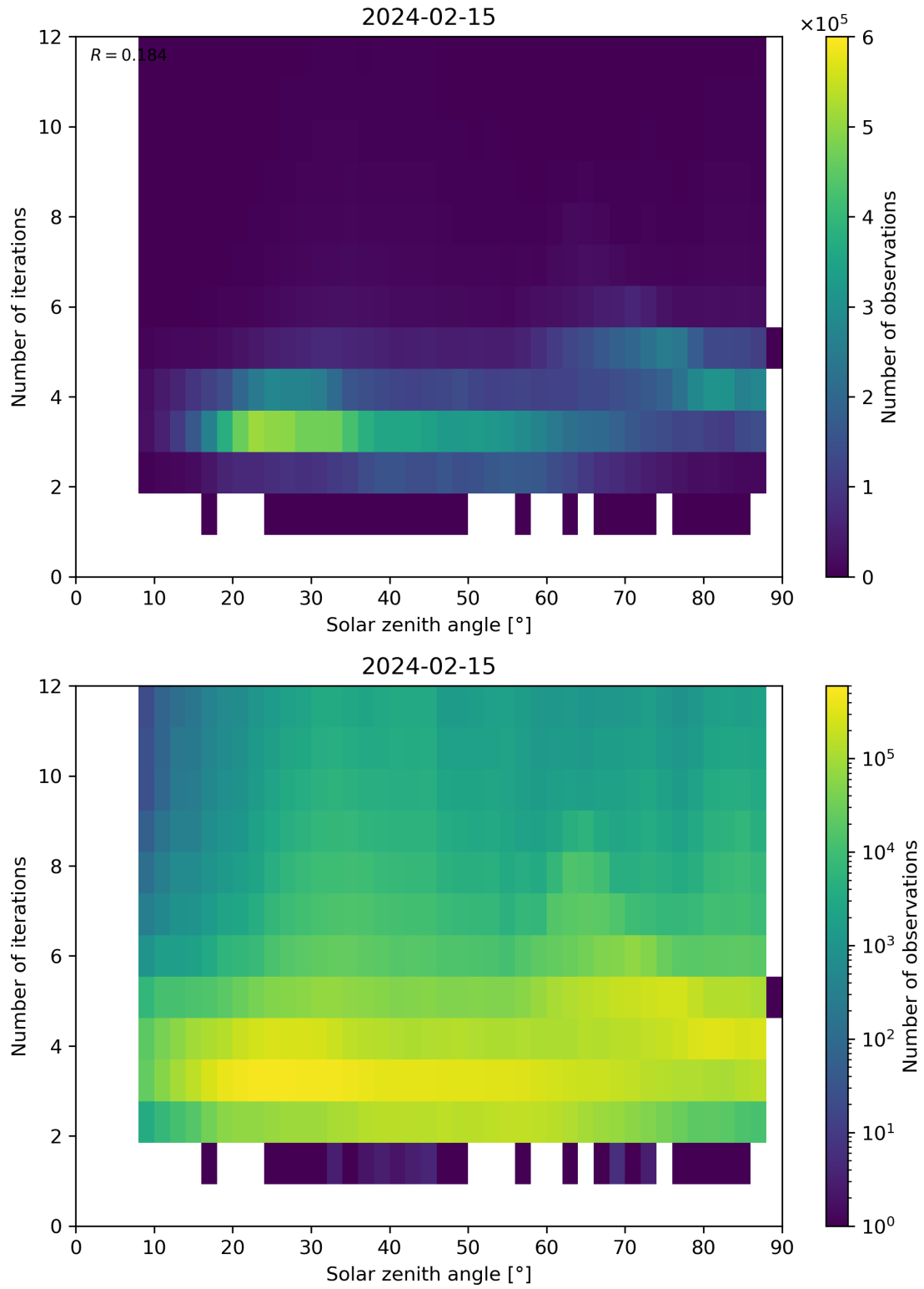
Figure 114: Scatter density plot of “Solar zenith angle” against “Number of iterations” for 2024-02-14 to 2024-02-16.
