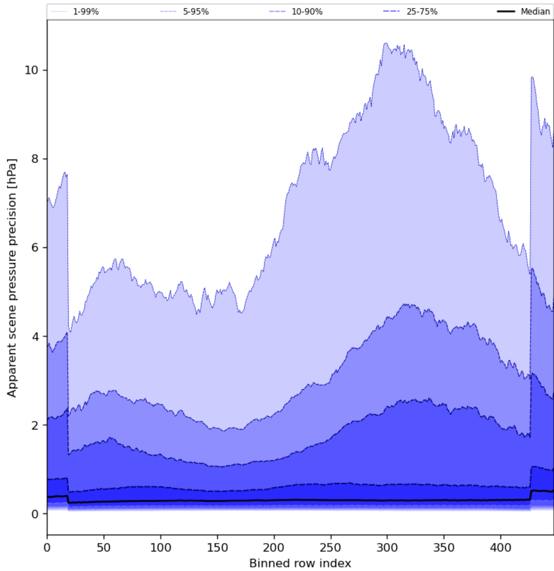
Figure 54: Along track statistics of “Apparent scene pressure precision” for 2024-02-14 to 2024-02-16
