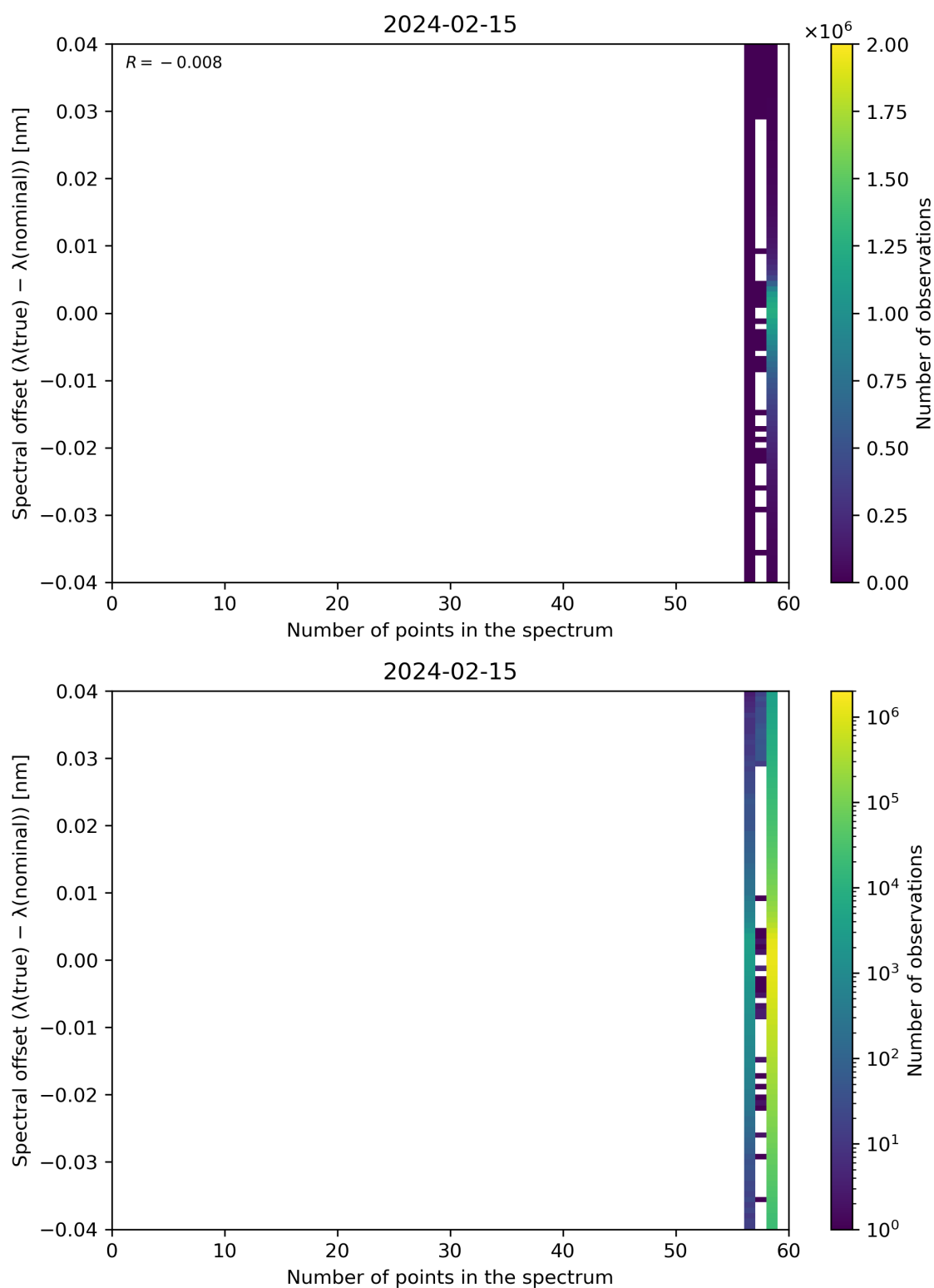
Figure 101: Scatter density plot of “Number of points in the spectrum” against “Spectral offset ( \lambda(\text{true}) - \lambda(\text{nominal}) )” for 2024-02-14 to 2024-02-16.
