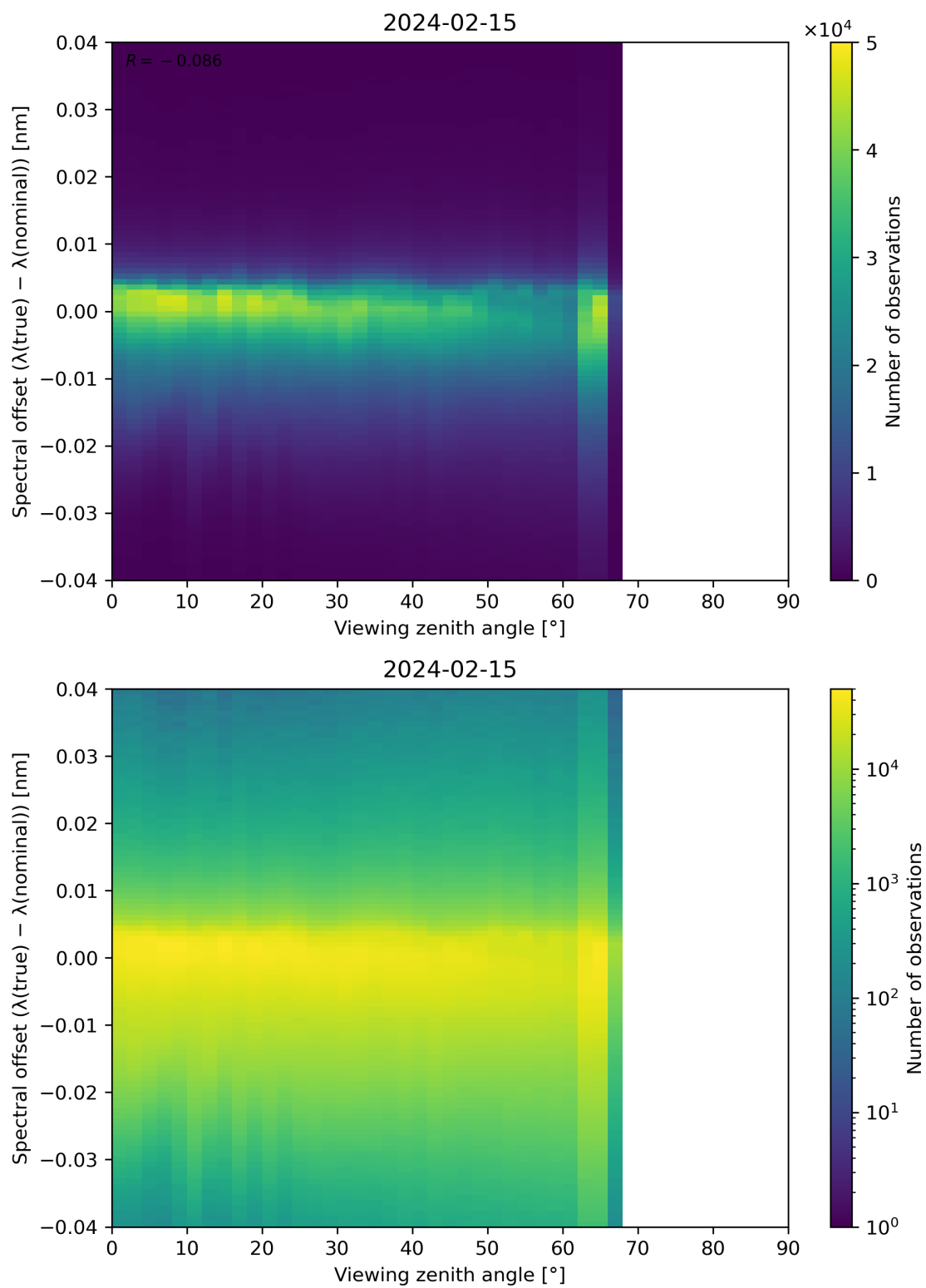
Figure 128: Scatter density plot of “Viewing zenith angle” against “Spectral offset ( \lambda(\text{true}) - \lambda(\text{nominal}) )” for 2024-02-14 to 2024-02-16.
