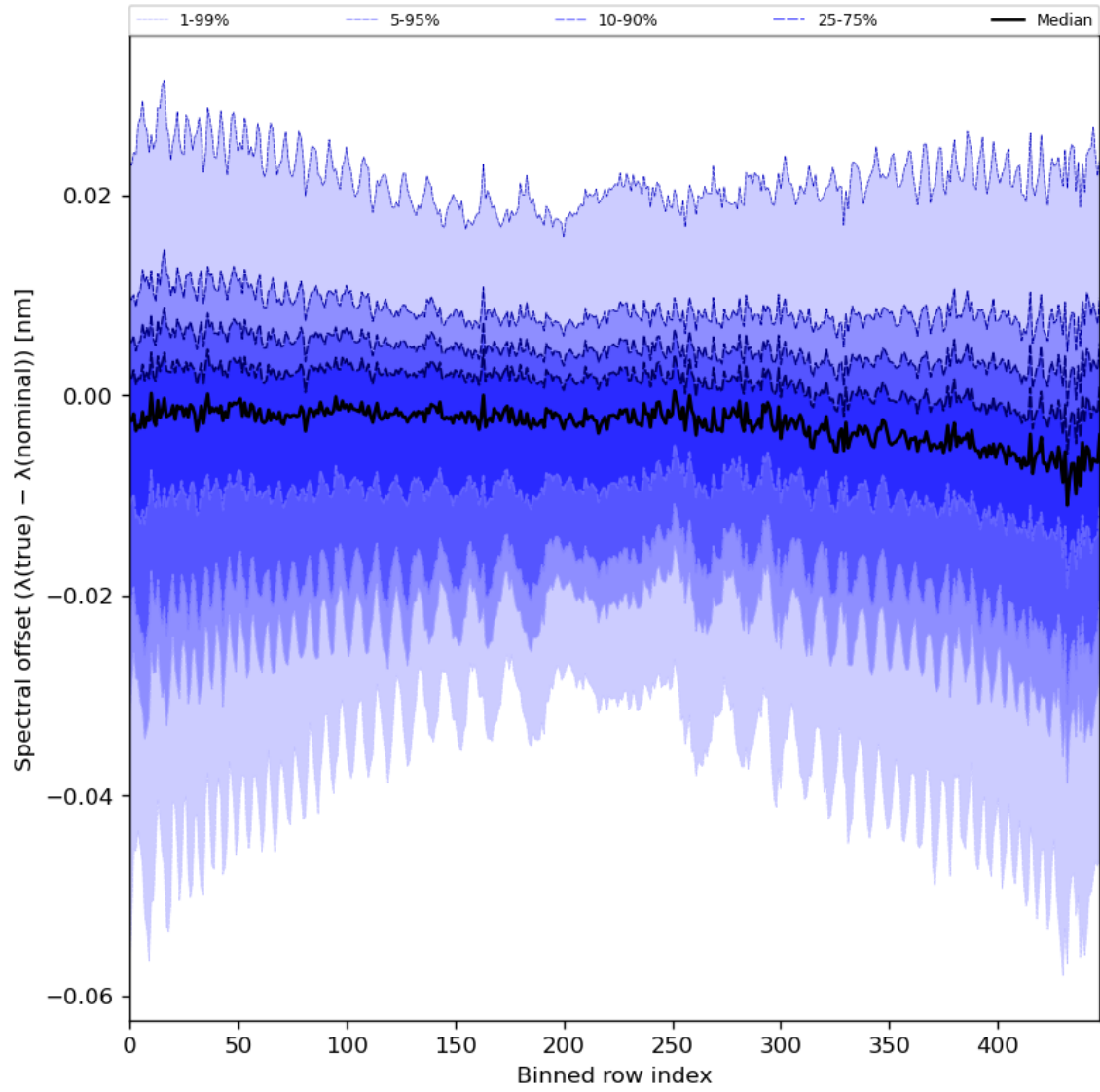
Figure 62: Along track statistics of “Spectral offset ( \lambda(\text{true}) - \lambda(\text{nominal}) )” for 2024-02-14 to 2024-02-16
