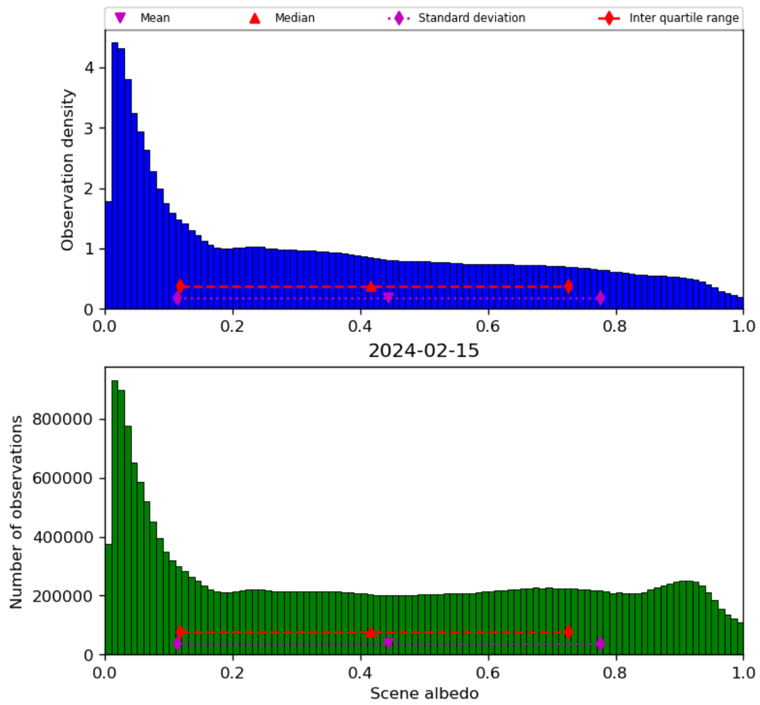
Figure 34: Histogram of “Scene albedo” for 2024-02-14 to 2024-02-16
