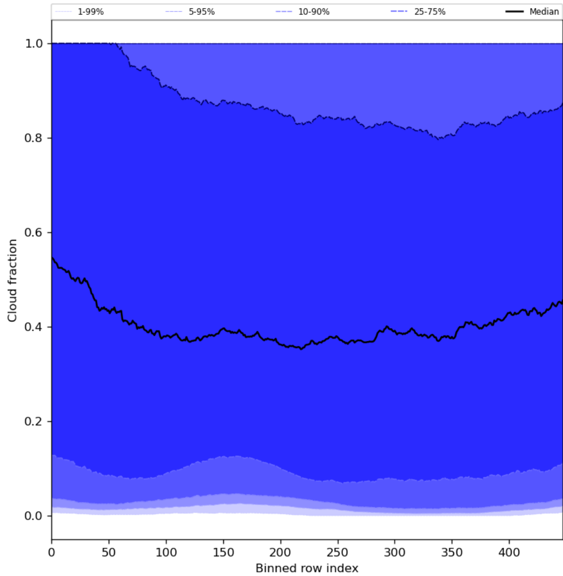
Figure 49: Along track statistics of “Cloud fraction” for 2024-02-14 to 2024-02-16
