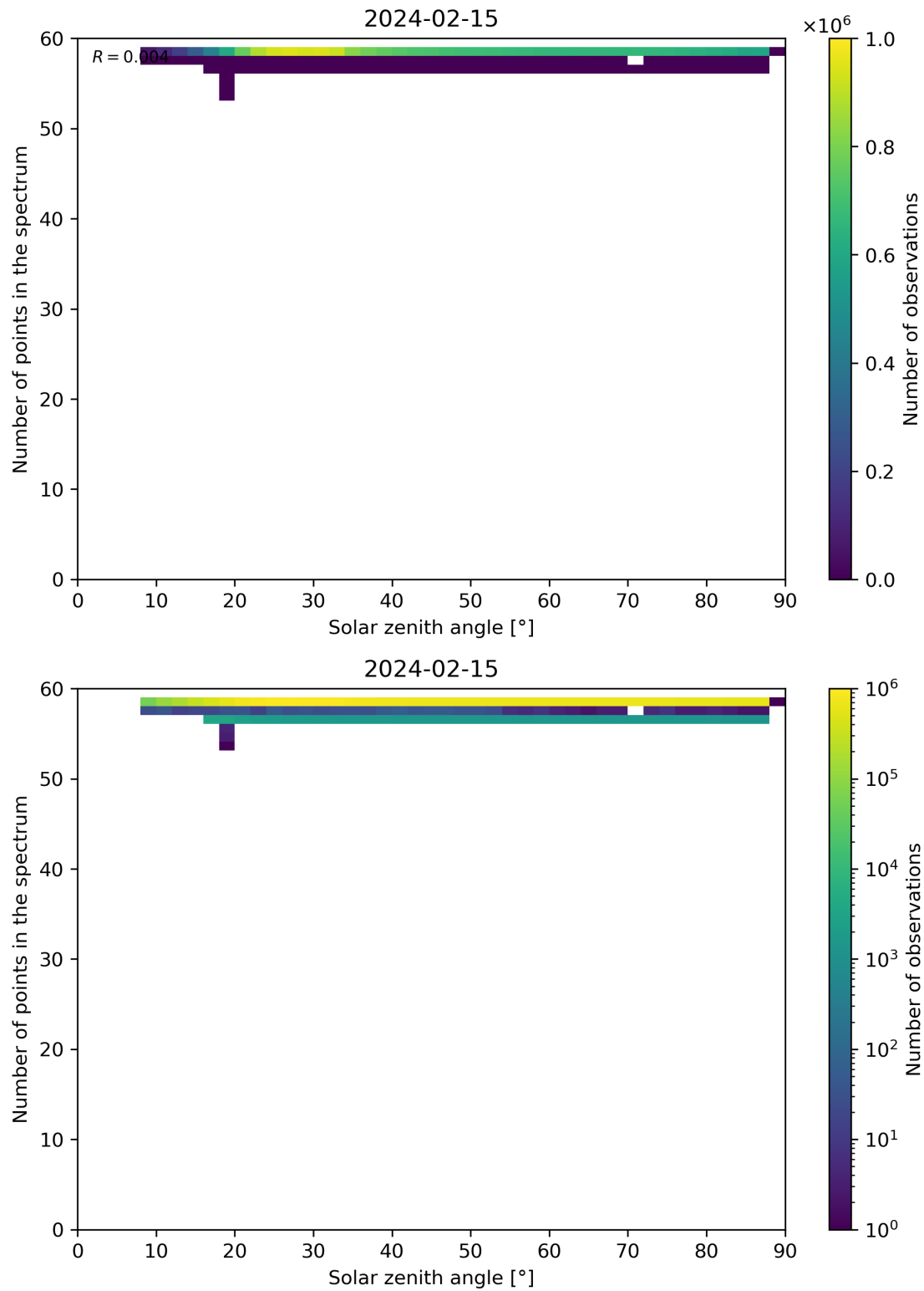
Figure 115: Scatter density plot of “Solar zenith angle” against “Number of points in the spectrum” for 2024-02-14 to 2024-02-16.
