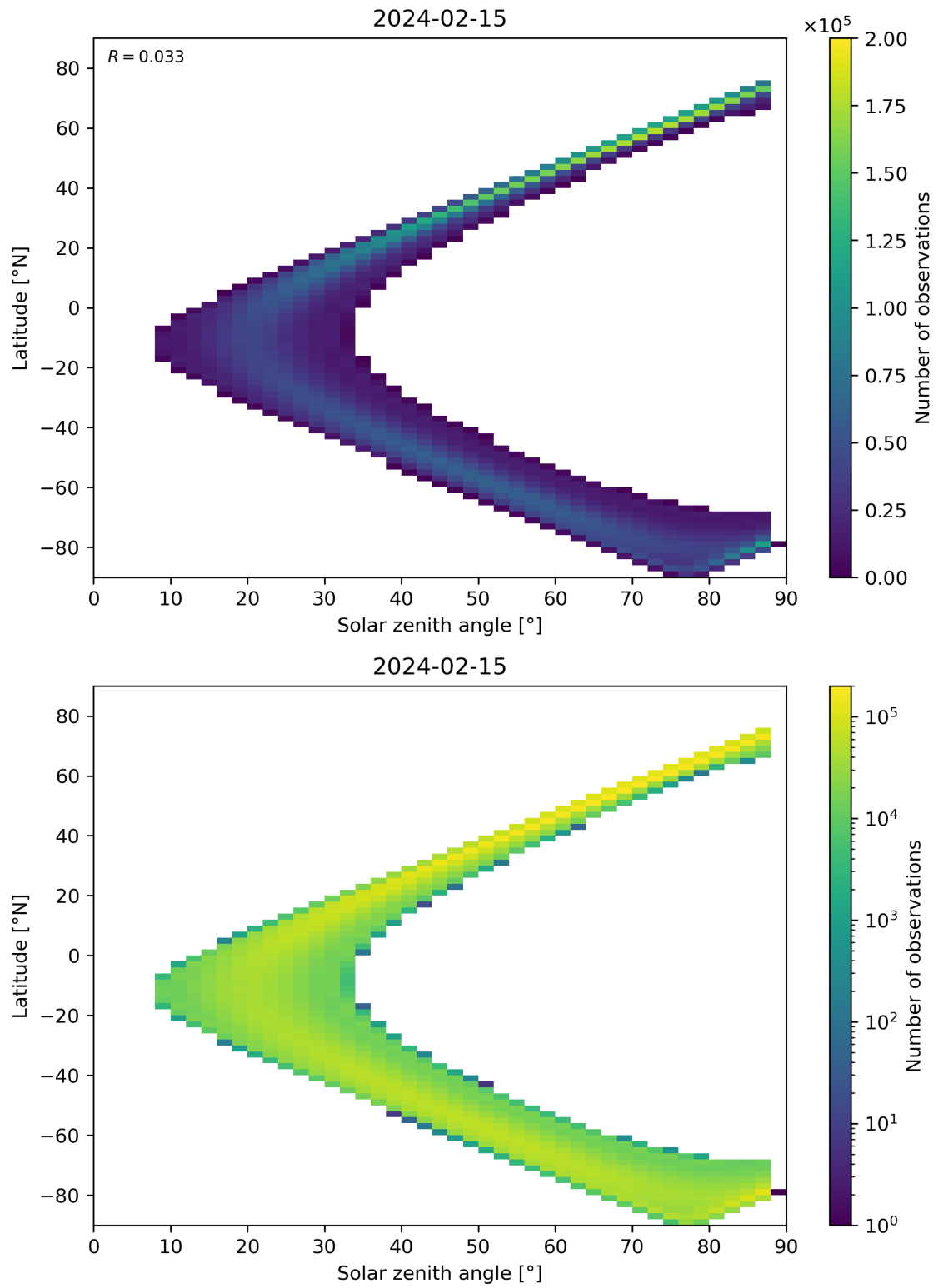
Figure 113: Scatter density plot of “Solar zenith angle” against “Latitude” for 2024-02-14 to 2024-02-16.
