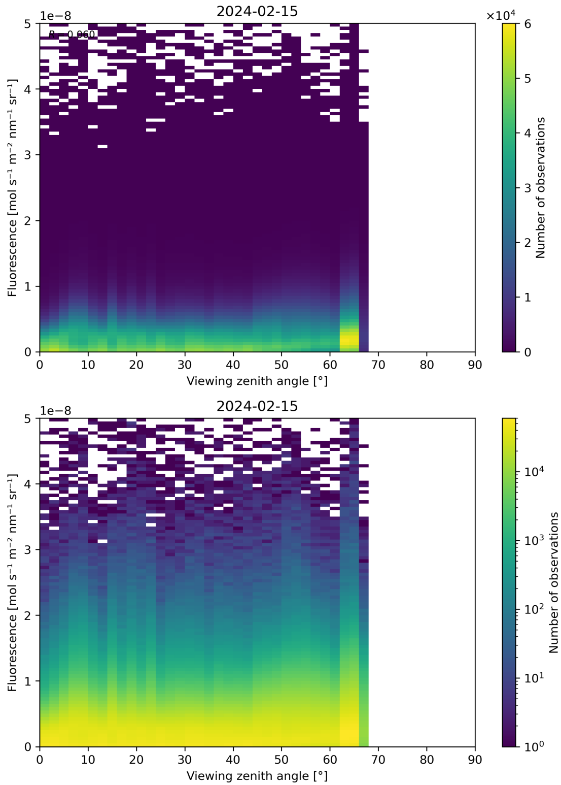
Figure 122: Scatter density plot of “Viewing zenith angle” against “Fluorescence” for 2024-02-14 to 2024-02-16.
