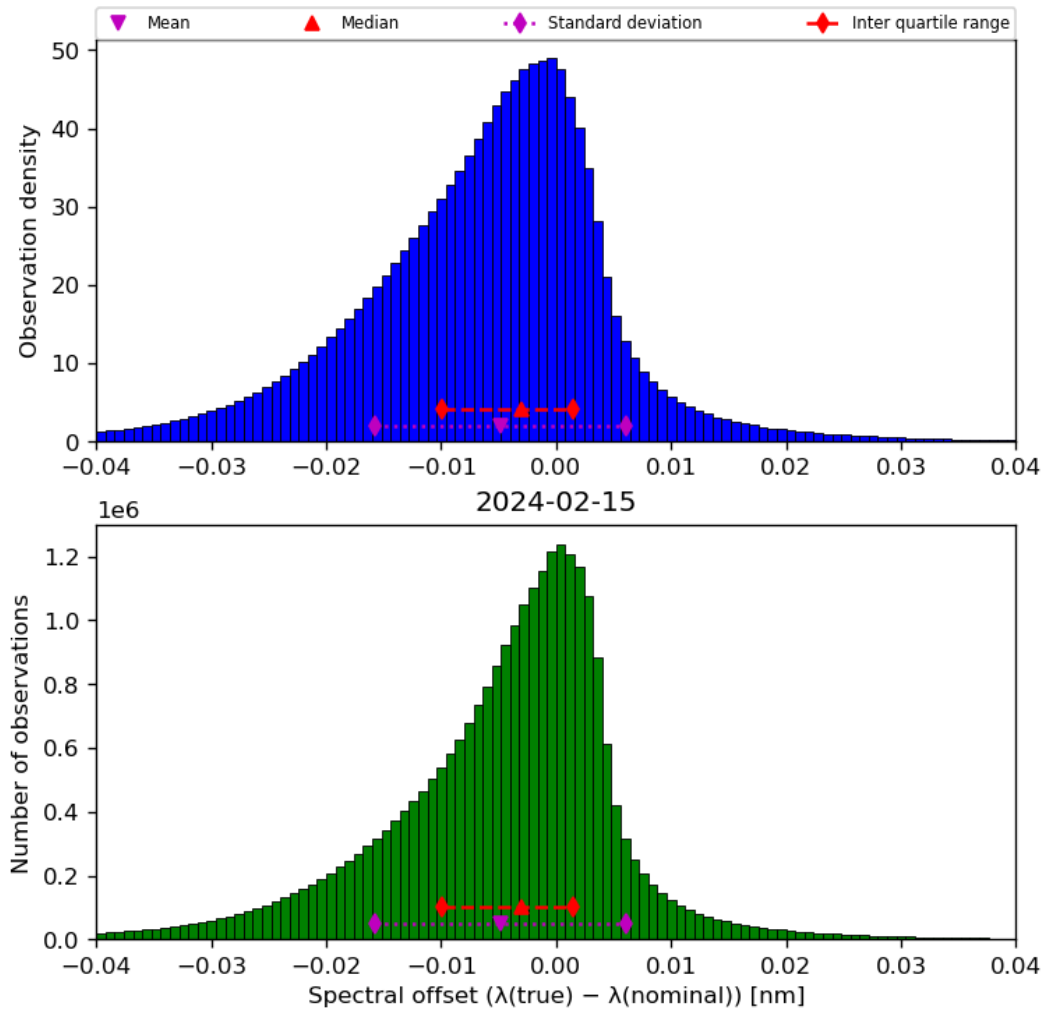
Figure 45: Histogram of “Spectral offset ( \lambda(\text{true}) - \lambda(\text{nominal}) )” for 2024-02-14 to 2024-02-16
