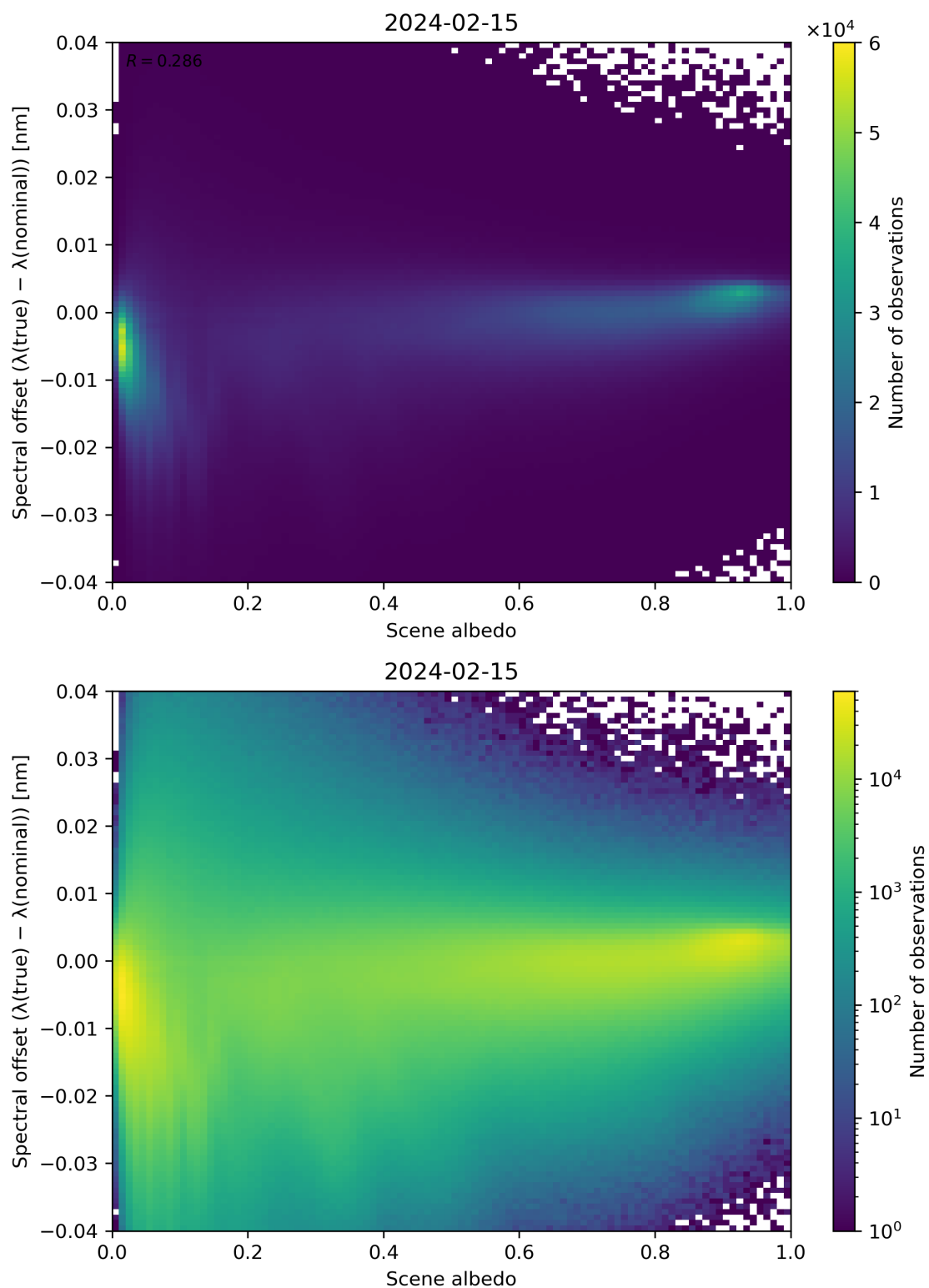
Figure 107: Scatter density plot of “Scene albedo” against “Spectral offset ( \lambda(\text{true}) - \lambda(\text{nominal}) )” for 2024-02-14 to 2024-02-16.
