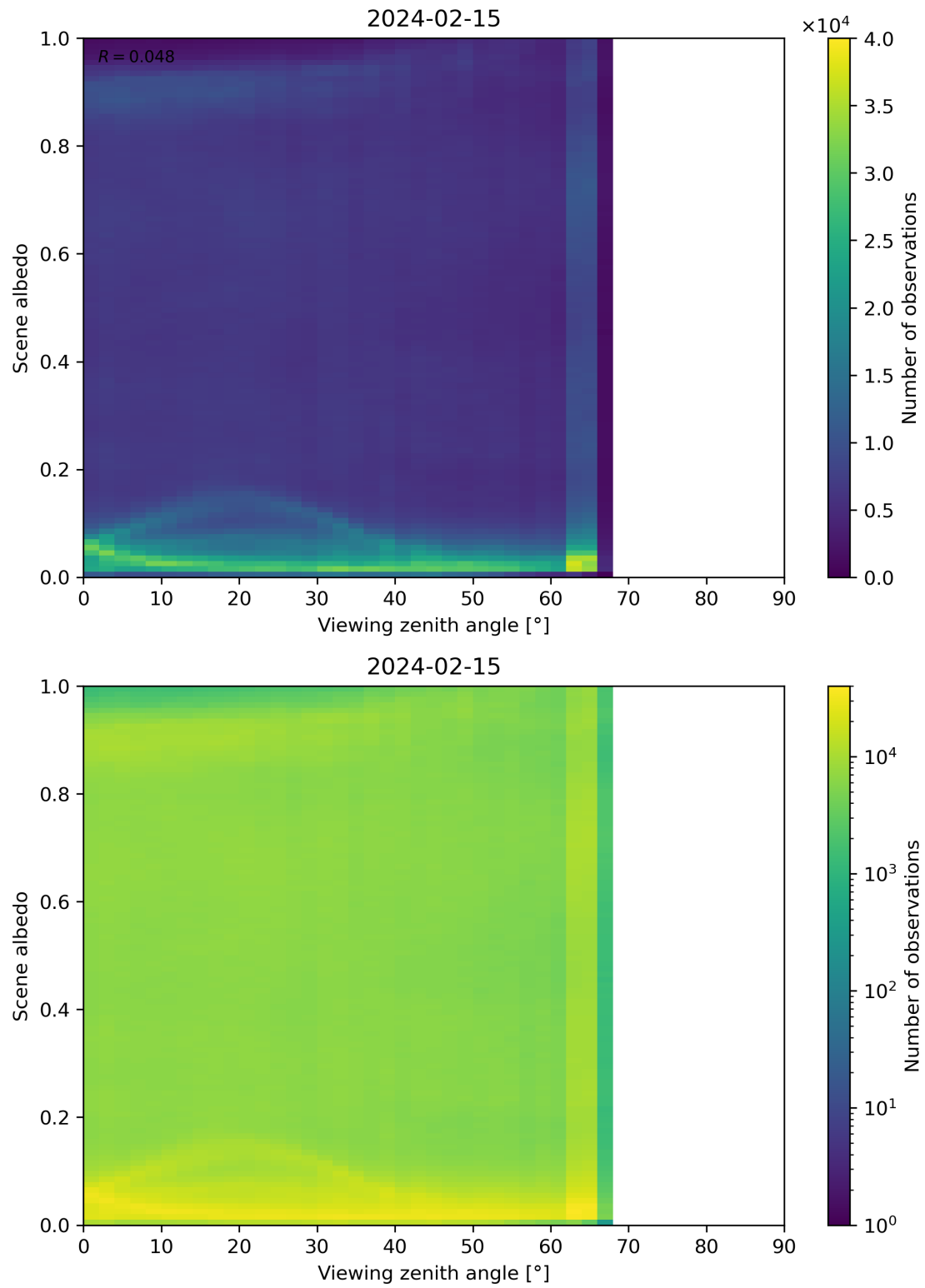
Figure 126: Scatter density plot of “Viewing zenith angle” against “Scene albedo” for 2024-02-14 to 2024-02-16.
