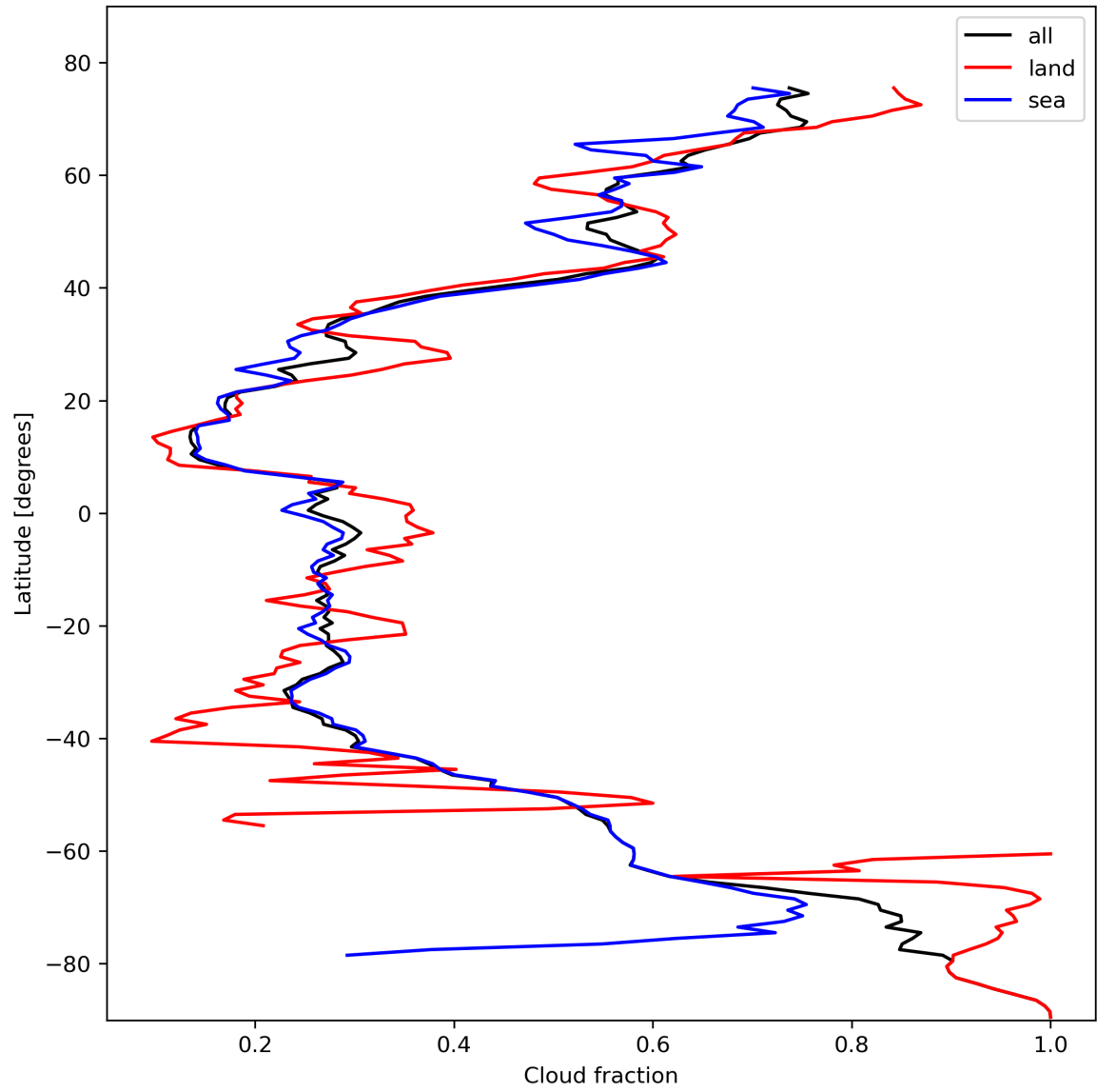
Figure 15: Zonal average of “Cloud fraction” for 2024-02-14 to 2024-02-16.
