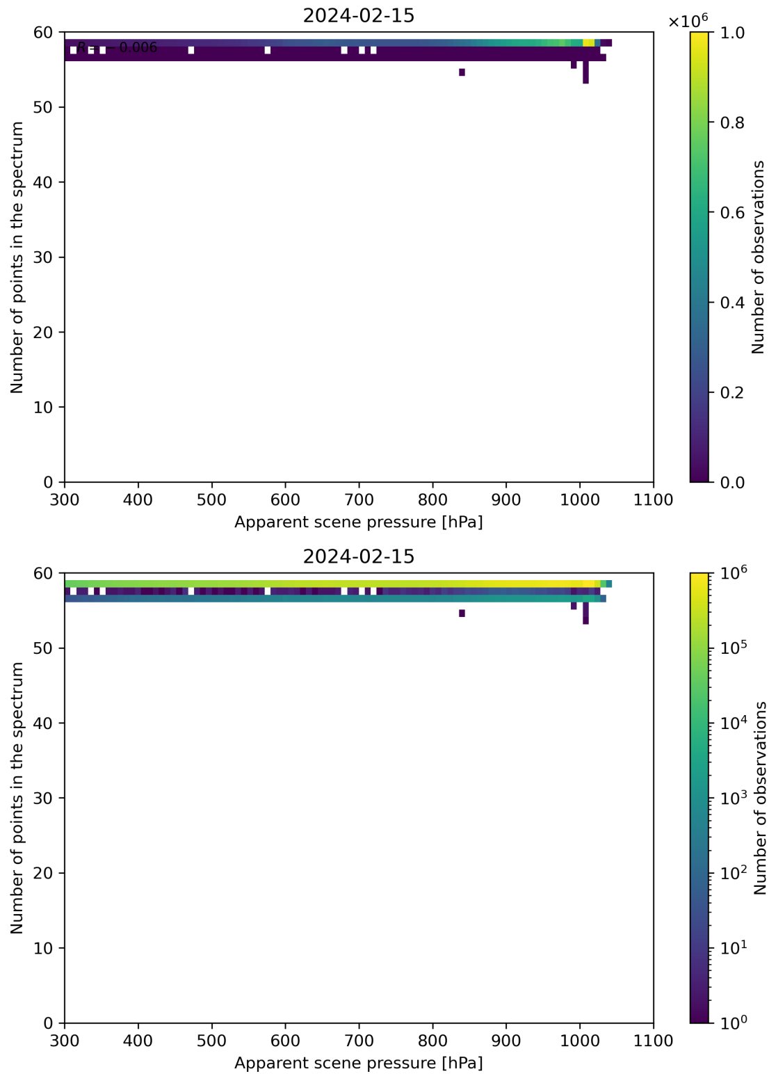
Figure 66: Scatter density plot of “Apparent scene pressure” against “Number of points in the spectrum” for 2024-02-14 to 2024-02-16.
