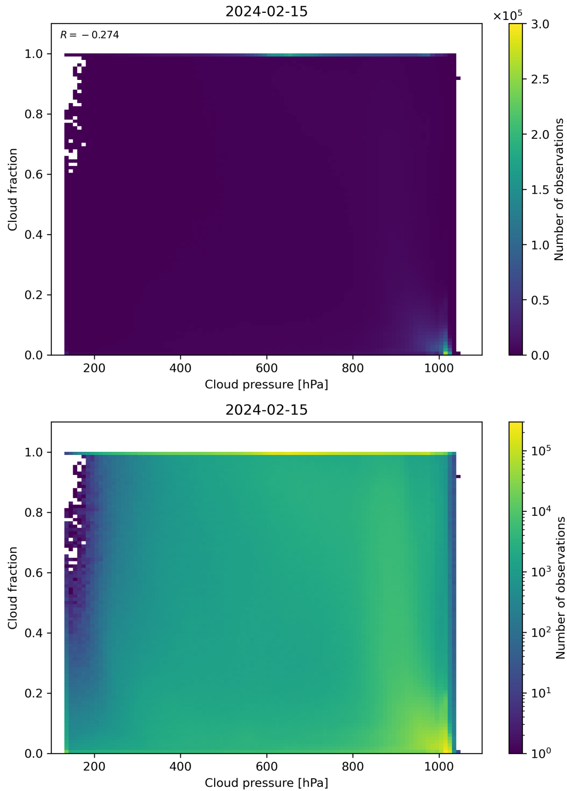
Figure 79: Scatter density plot of “Cloud pressure” against “Cloud fraction” for 2024-02-14 to 2024-02-16.
