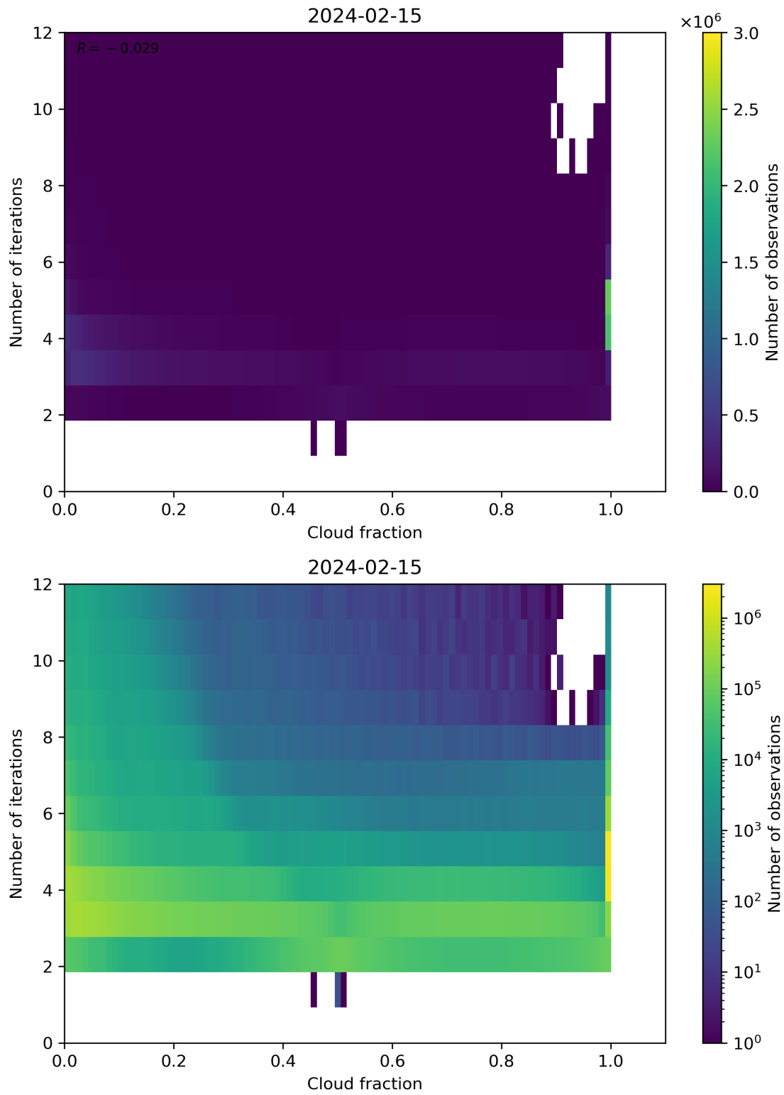
Figure 73: Scatter density plot of “Cloud fraction” against “Number of iterations” for 2024-02-14 to 2024-02-16.
