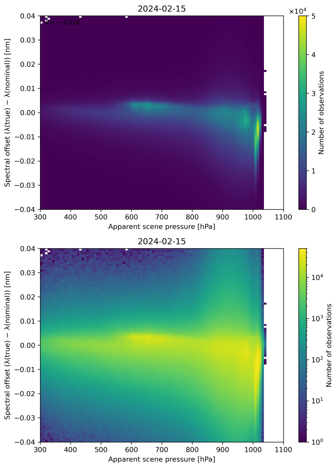
Figure 67: Scatter density plot of “Apparent scene pressure” against “Spectral offset ( \lambda(\text{true}) - \lambda(\text{nominal}) )” for 2024-02-14 to 2024-02-16.
