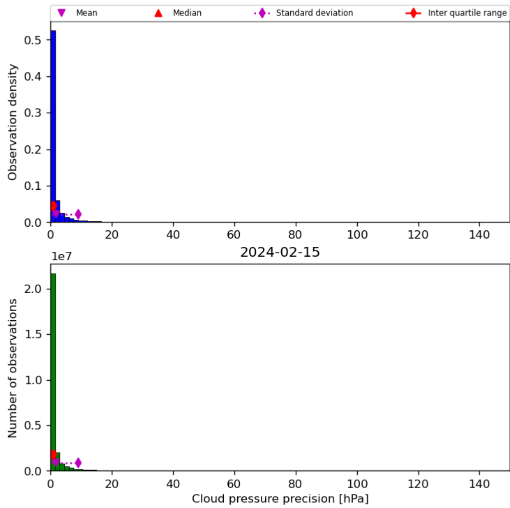
Figure 31: Histogram of “Cloud pressure precision” for 2024-02-14 to 2024-02-16
