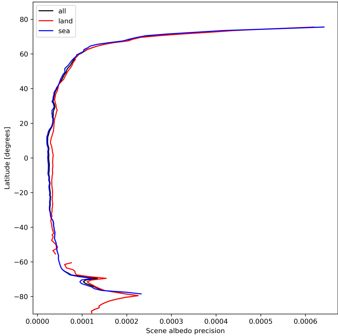
Figure 18: Zonal average of "Scene albedo precision" for 2024-02-14 to 2024-02-16.
