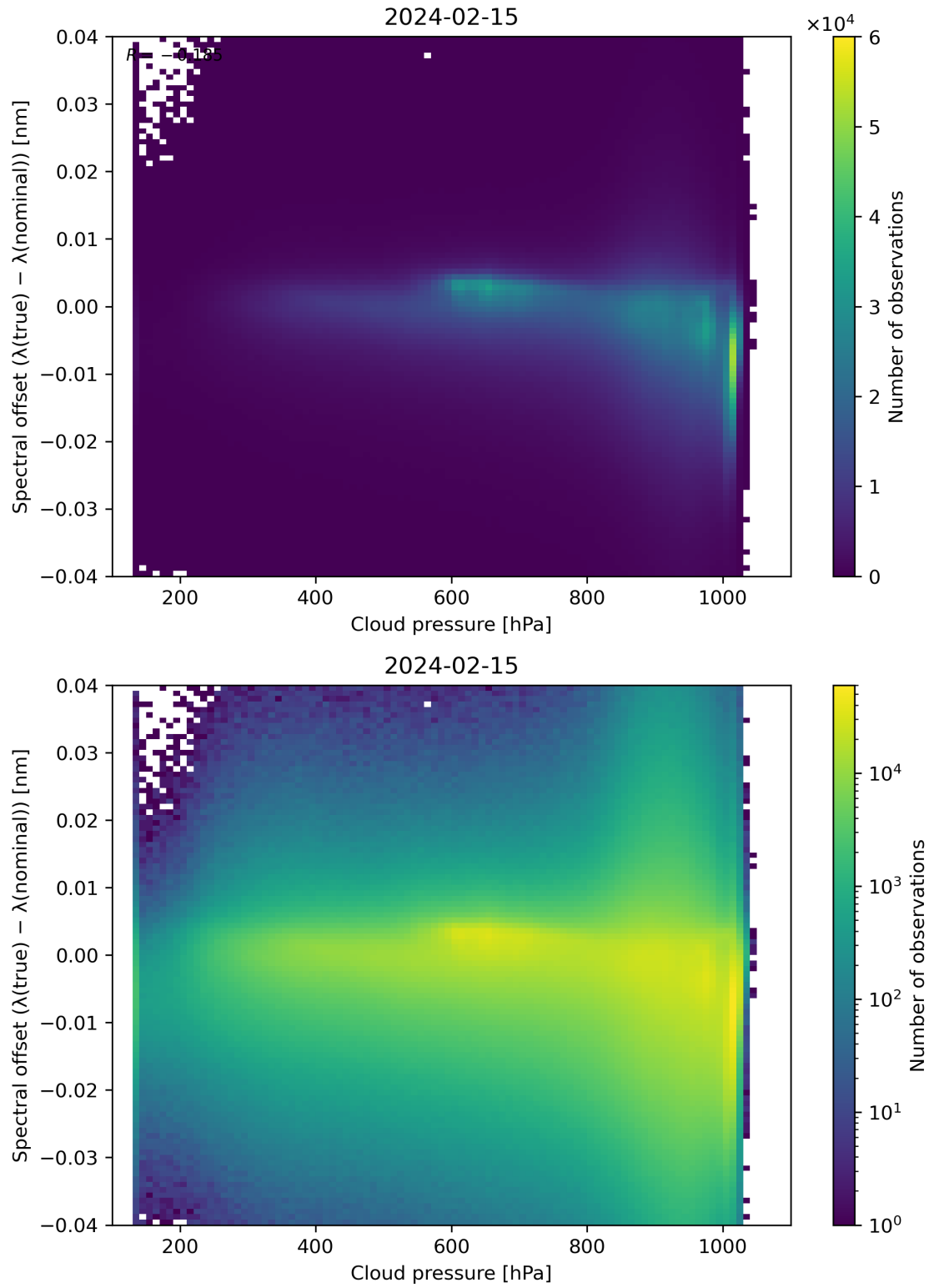
Figure 84: Scatter density plot of “Cloud pressure” against “Spectral offset ( \lambda(\text{true}) - \lambda(\text{nominal}) )” for 2024-02-14 to 2024-02-16.
