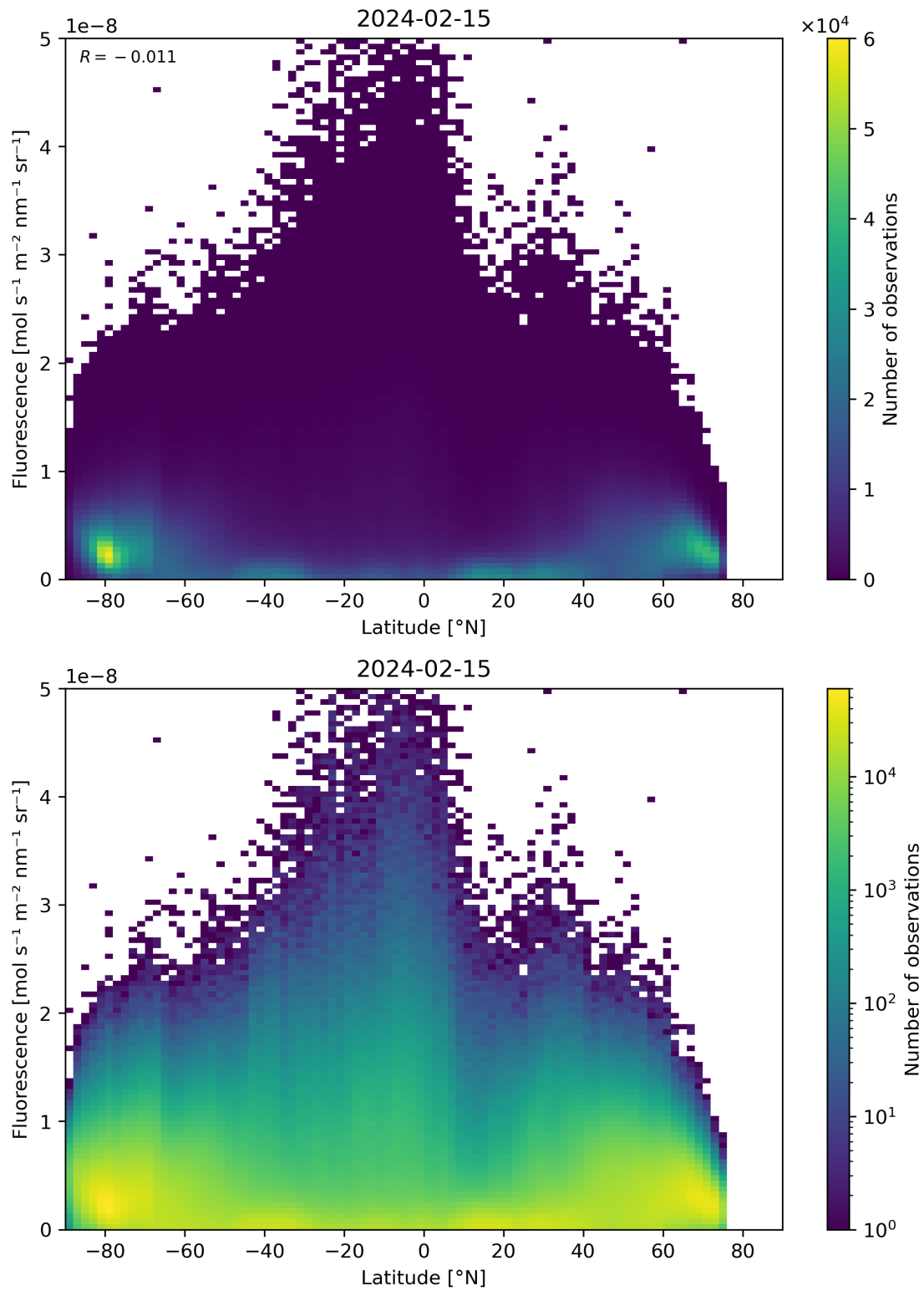
Figure 92: Scatter density plot of “Latitude” against “Fluorescence” for 2024-02-14 to 2024-02-16.
