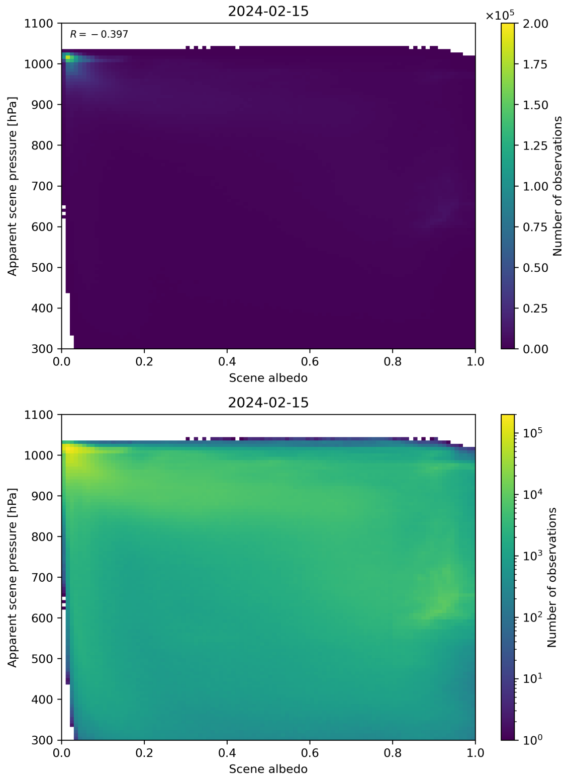
Figure 102: Scatter density plot of “Scene albedo” against “Apparent scene pressure” for 2024-02-14 to 2024-02-16.
