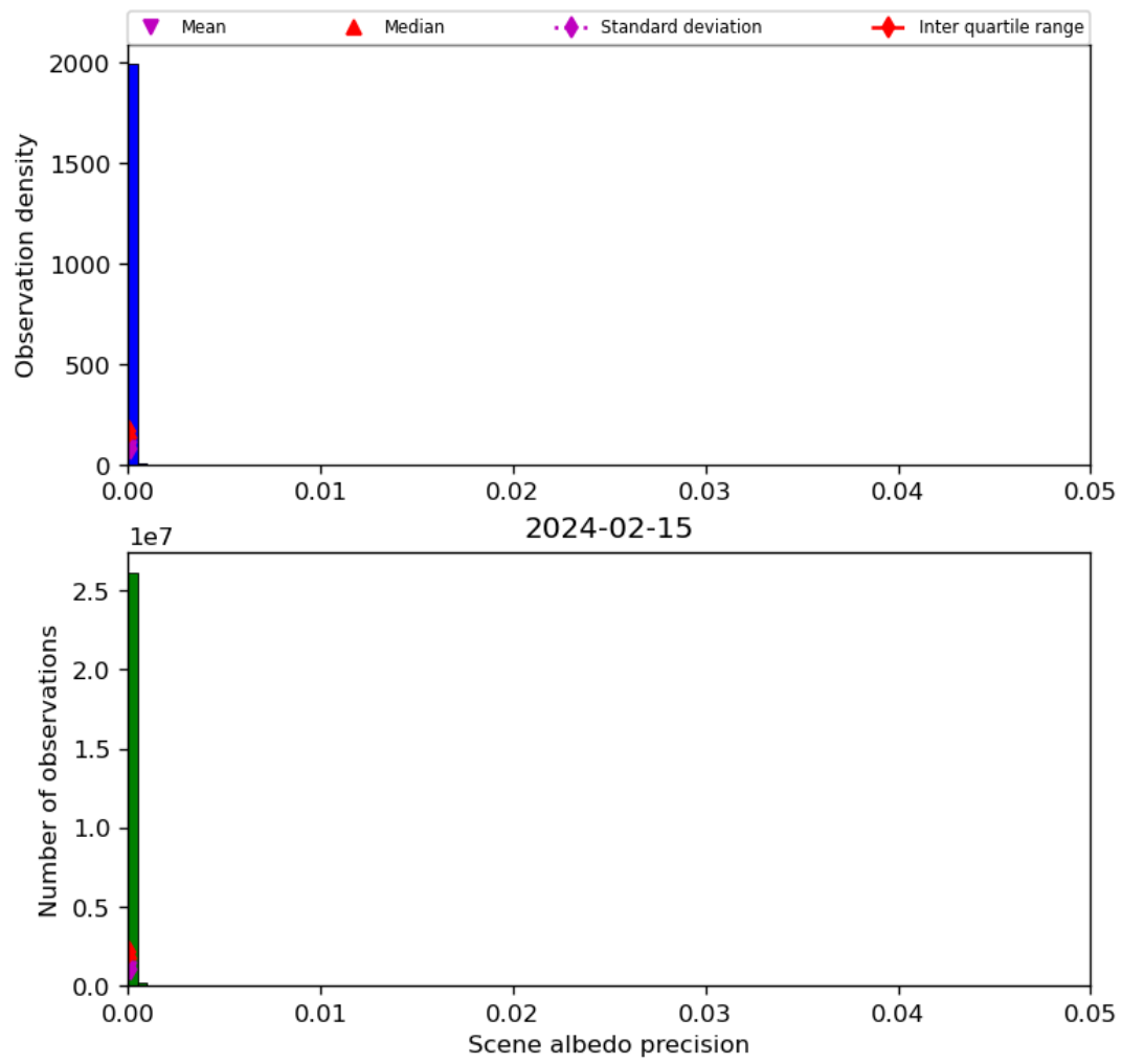
Figure 35: Histogram of “Scene albedo precision” for 2024-02-14 to 2024-02-16
