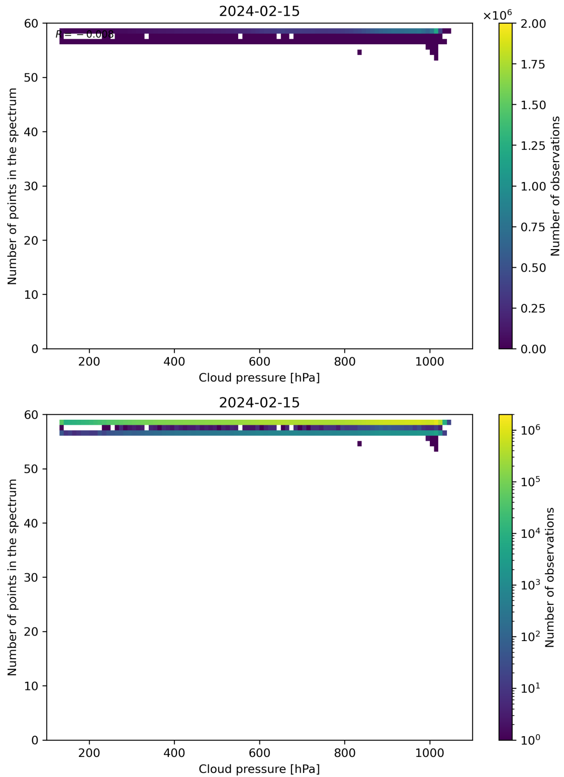
Figure 82: Scatter density plot of “Cloud pressure” against “Number of points in the spectrum” for 2024-02-14 to 2024-02-16.
