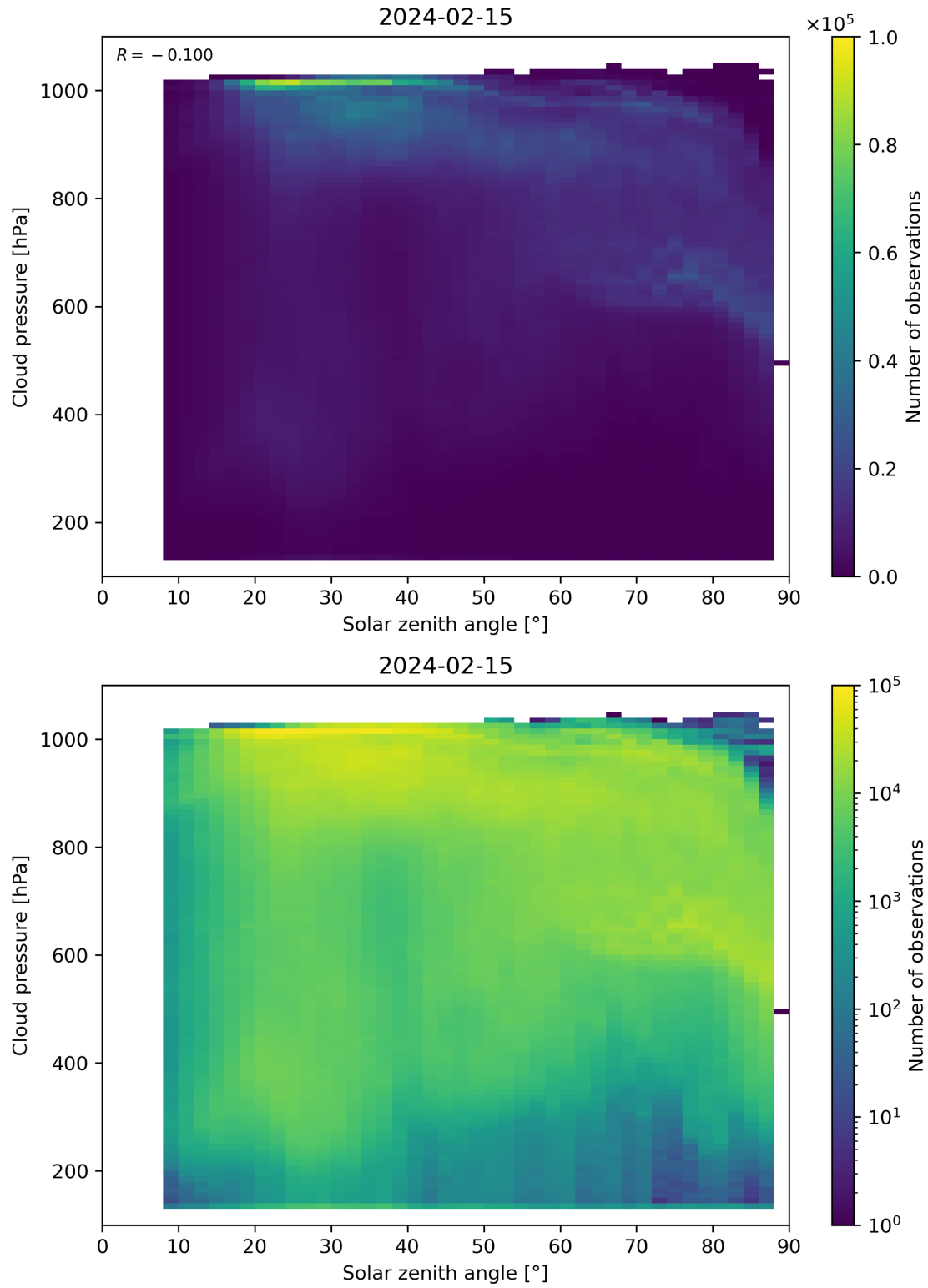
Figure 111: Scatter density plot of “Solar zenith angle” against “Cloud pressure” for 2024-02-14 to 2024-02-16.
