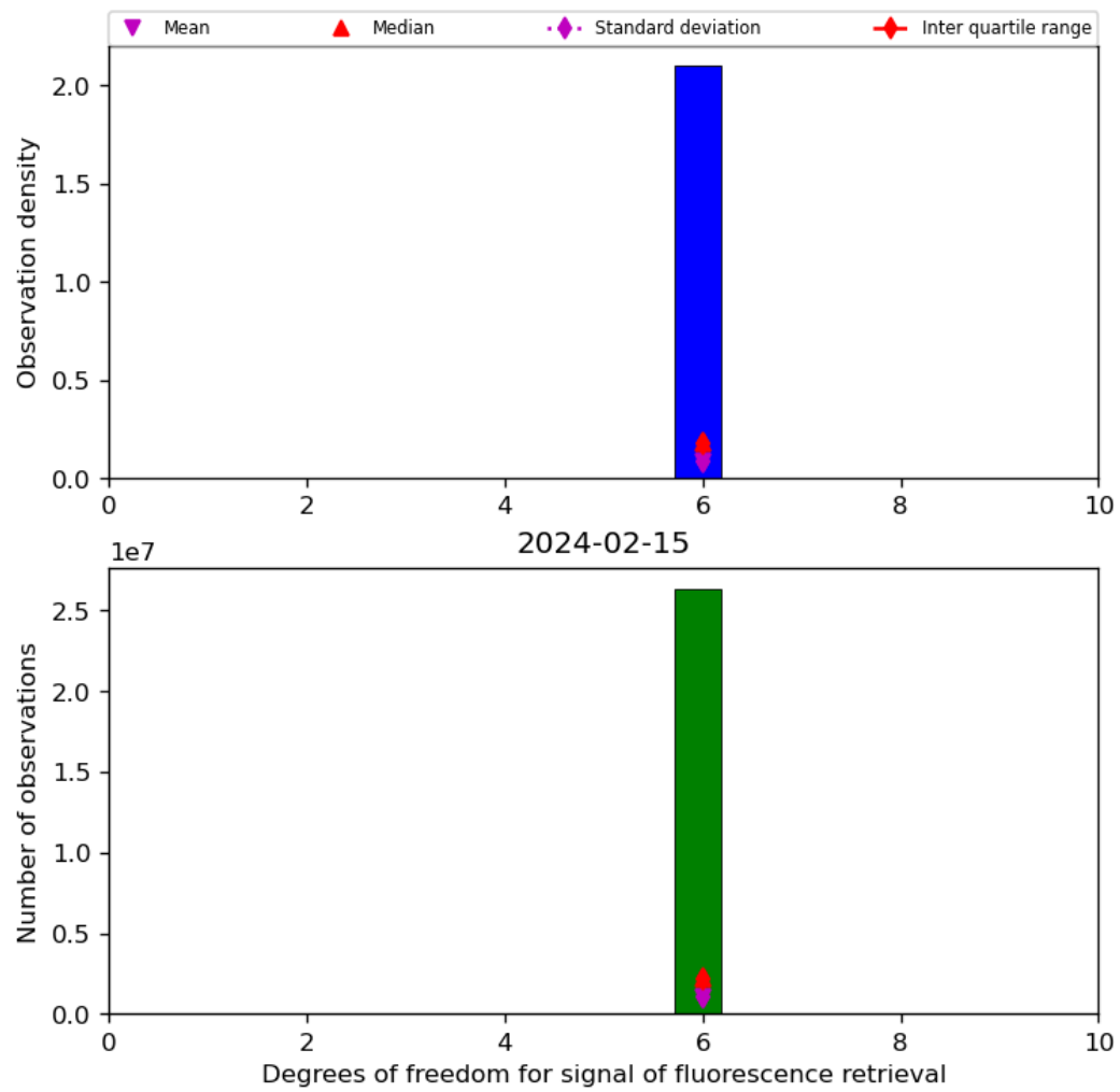
Figure 43: Histogram of "Degrees of freedom for signal of fluorescence retrieval" for 2024-02-14 to 2024-02-16
