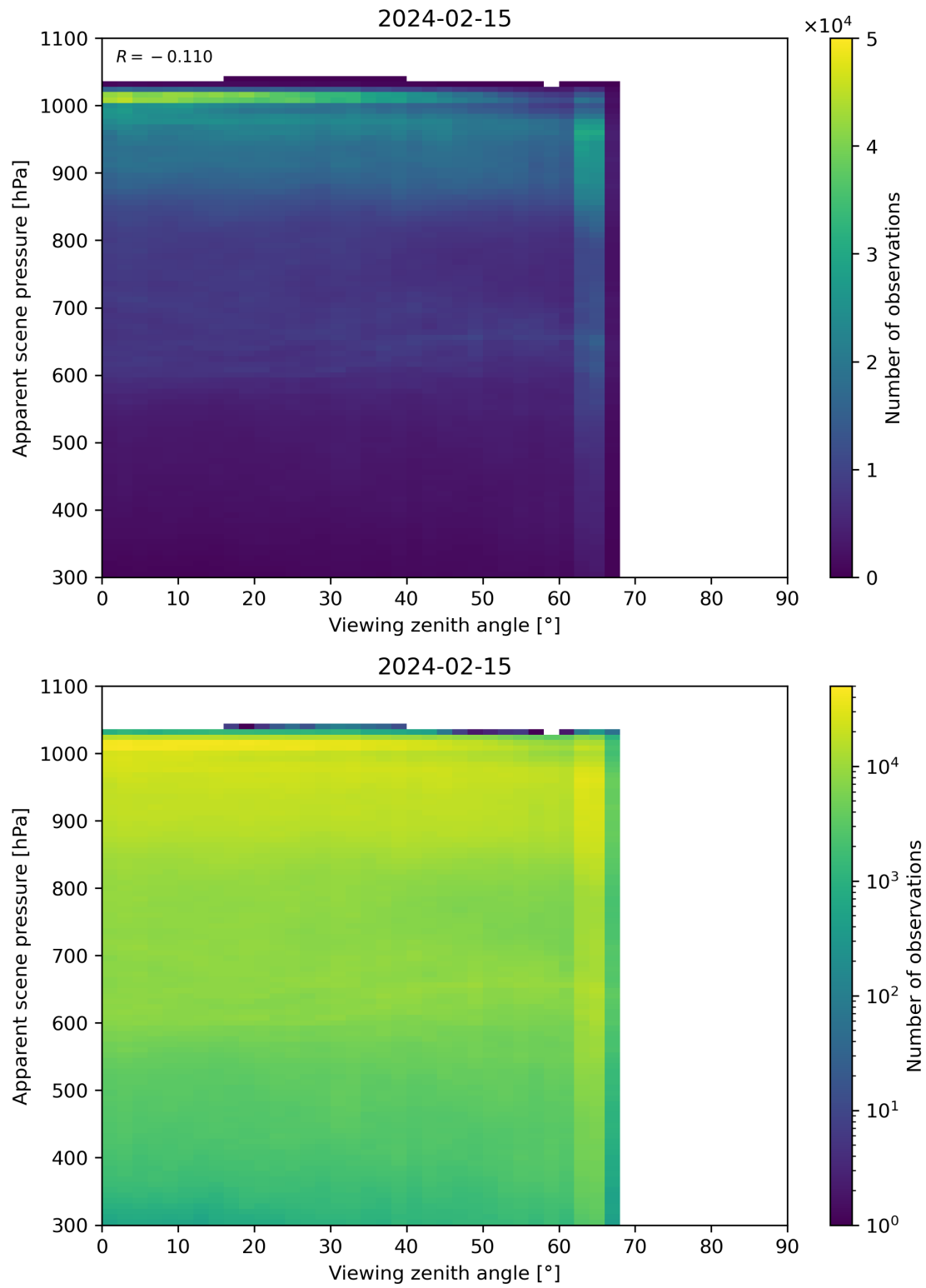
Figure 118: Scatter density plot of “Viewing zenith angle” against “Apparent scene pressure” for 2024-02-14 to 2024-02-16.
