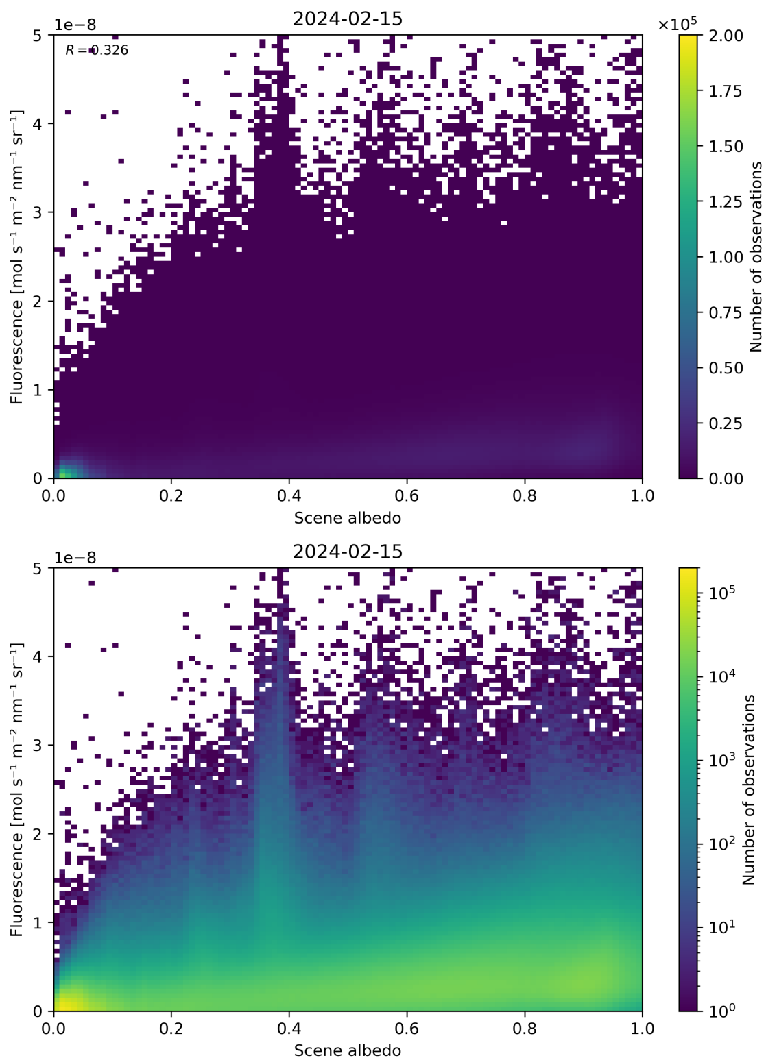
Figure 104: Scatter density plot of “Scene albedo” against “Fluorescence” for 2024-02-14 to 2024-02-16.
