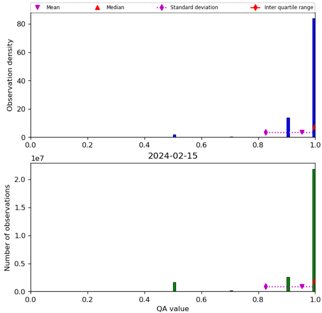
Figure 29: Histogram of “QA value” for 2024-02-14 to 2024-02-16
