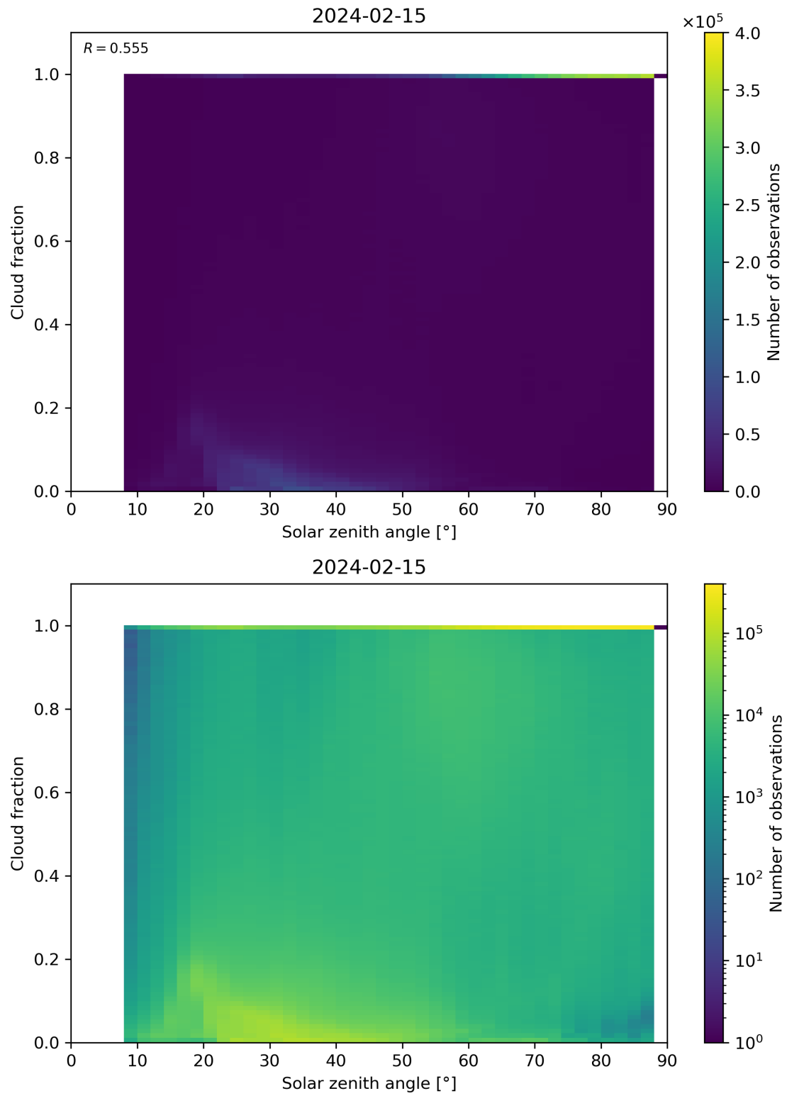
Figure 110: Scatter density plot of “Solar zenith angle” against “Cloud fraction” for 2024-02-14 to 2024-02-16.
