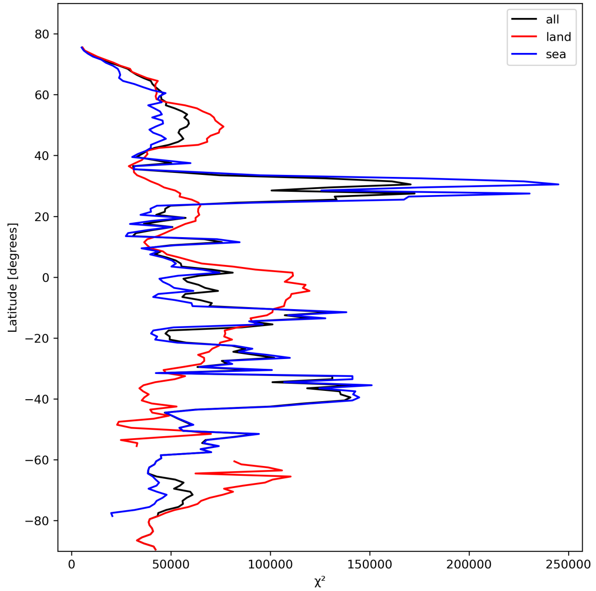
Figure 21: Zonal average of “ \chi^2 ” for 2024-02-14 to 2024-02-16.
