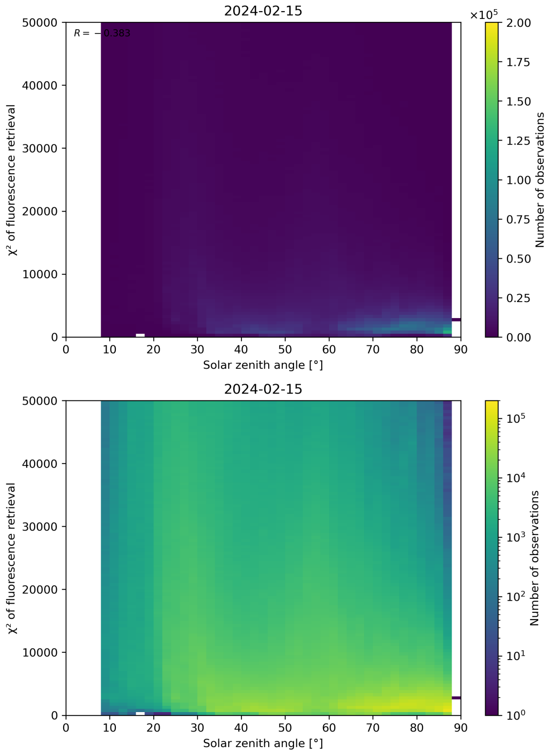
Figure 109: Scatter density plot of “Solar zenith angle” against “ \chi^2 of fluorescence retrieval” for 2024-02-14 to 2024-02-16.
