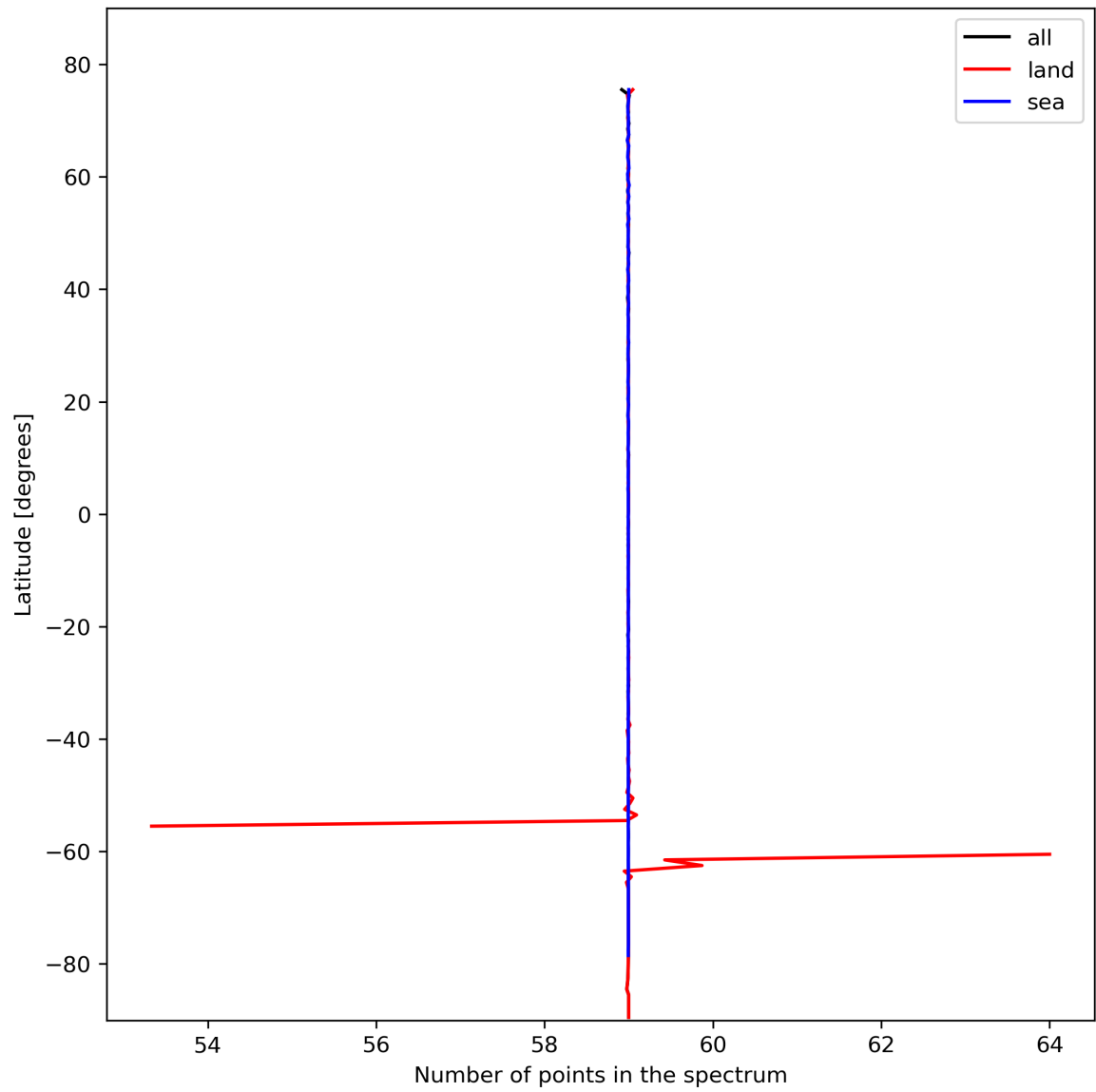
Figure 27: Zonal average of “Number of points in the spectrum” for 2024-02-14 to 2024-02-16.
