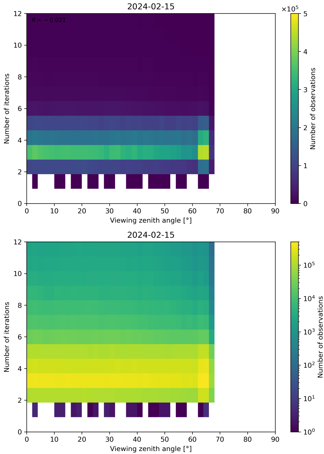
Figure 124: Scatter density plot of “Viewing zenith angle” against “Number of iterations” for 2024-02-14 to 2024-02-16.
