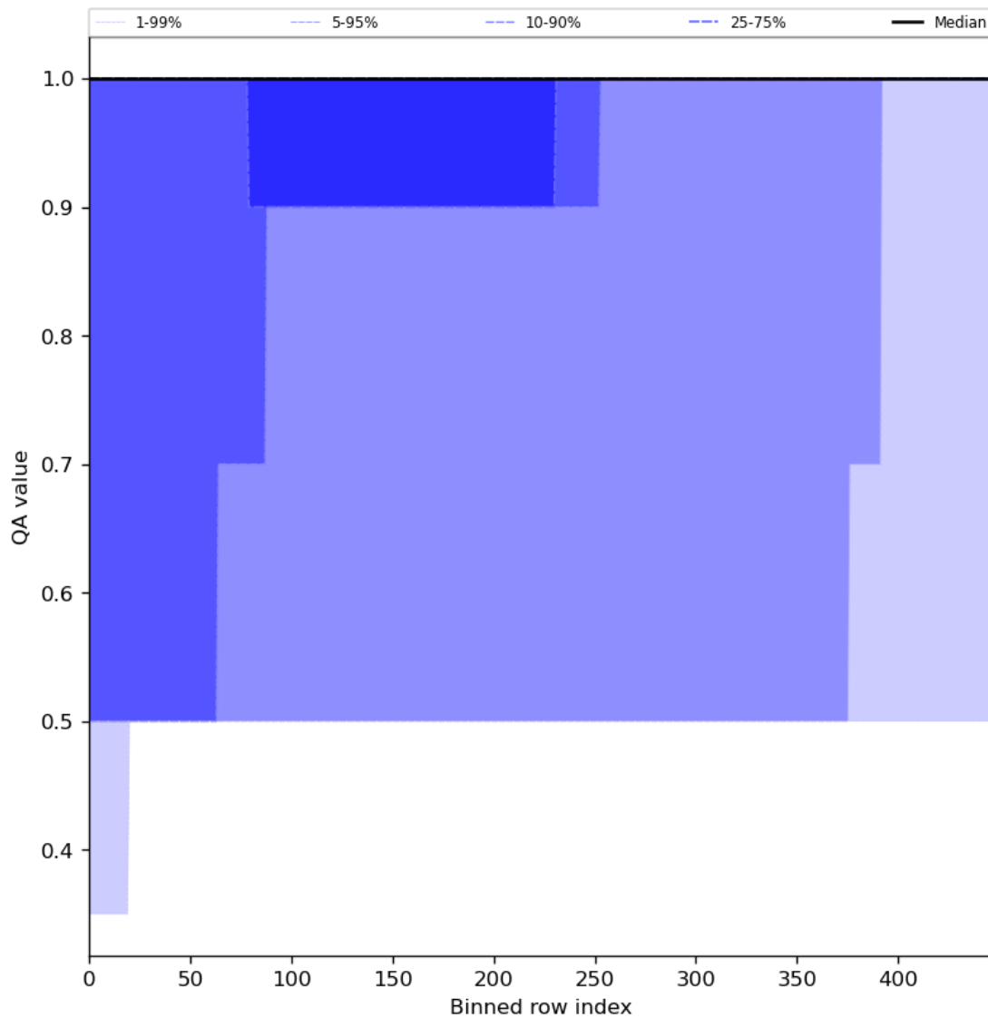
Figure 46: Along track statistics of “QA value” for 2024-02-14 to 2024-02-16
