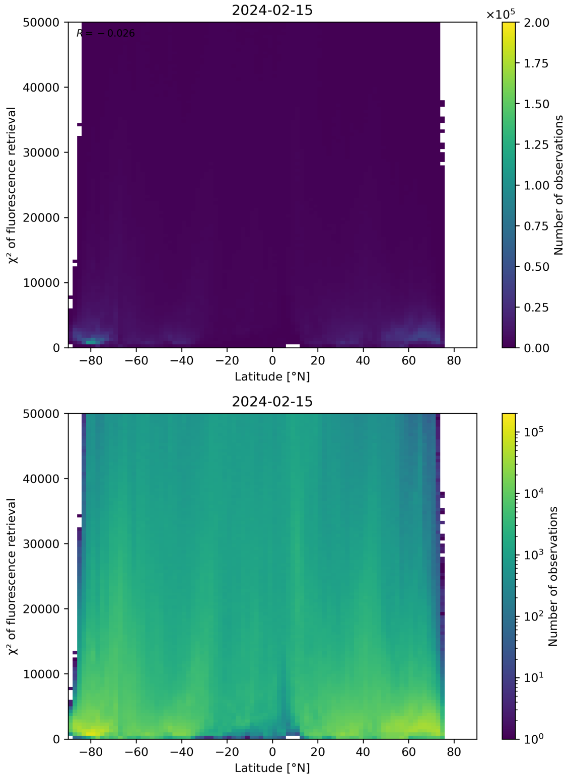
Figure 89: Scatter density plot of “Latitude” against “ \chi^2 of fluorescence retrieval” for 2024-02-14 to 2024-02-16.
