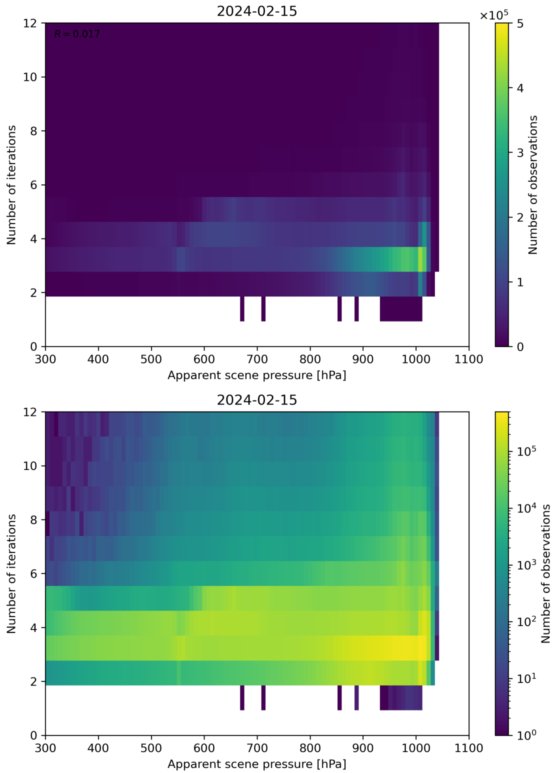
Figure 65: Scatter density plot of “Apparent scene pressure” against “Number of iterations” for 2024-02-14 to 2024-02-16.
