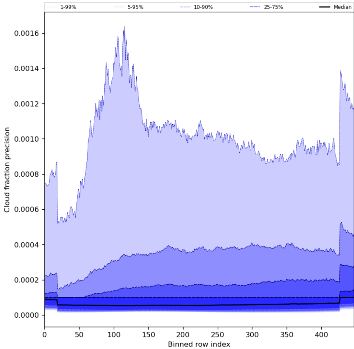
Figure 50: Along track statistics of “Cloud fraction precision” for 2024-02-14 to 2024-02-16
