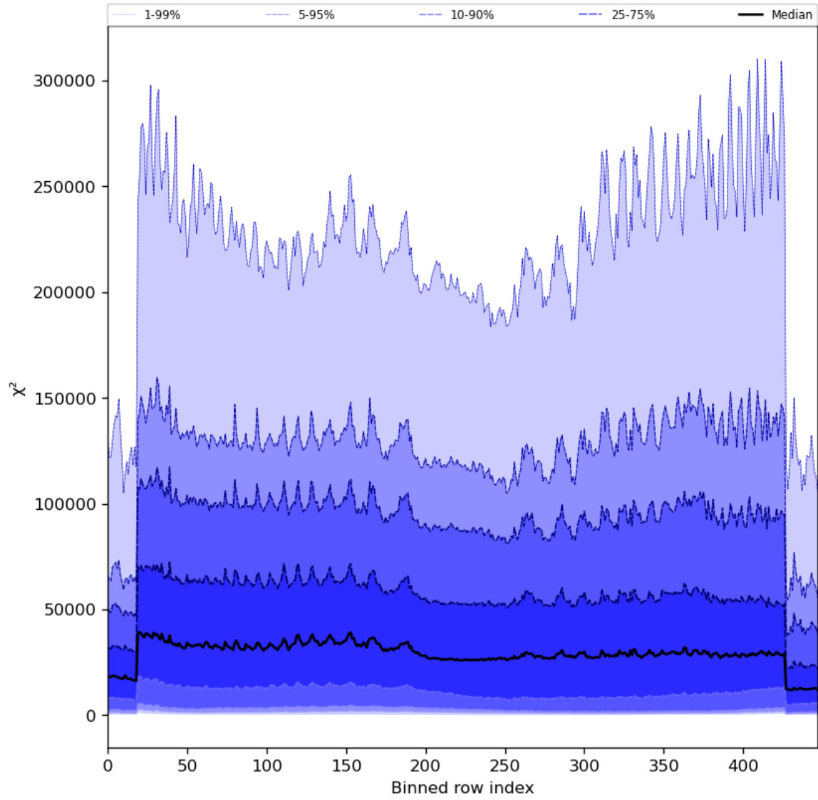
Figure 55: Along track statistics of “ \chi^2 ” for 2024-02-14 to 2024-02-16
