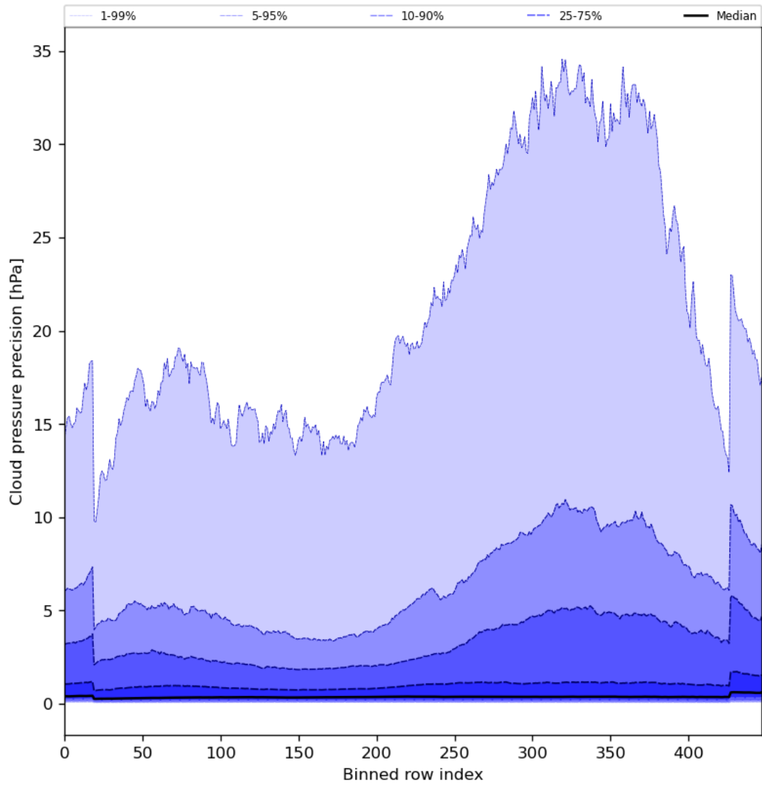
Figure 48: Along track statistics of “Cloud pressure precision” for 2024-02-14 to 2024-02-16
