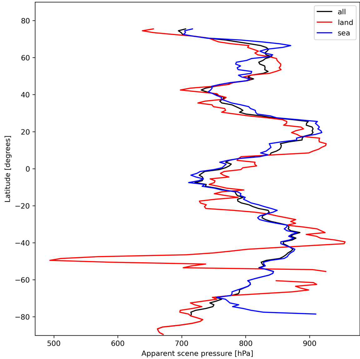
Figure 19: Zonal average of “Apparent scene pressure” for 2024-02-14 to 2024-02-16.
