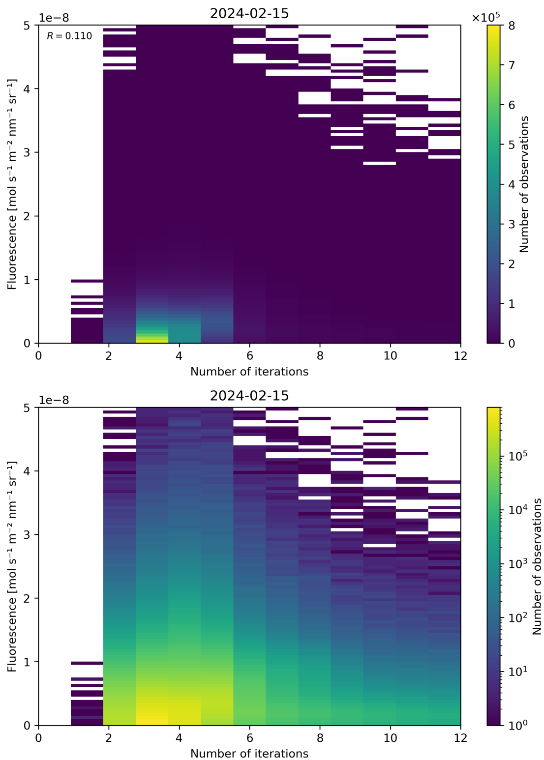
Figure 98: Scatter density plot of “Number of iterations” against “Fluorescence” for 2024-02-14 to 2024-02-16.
