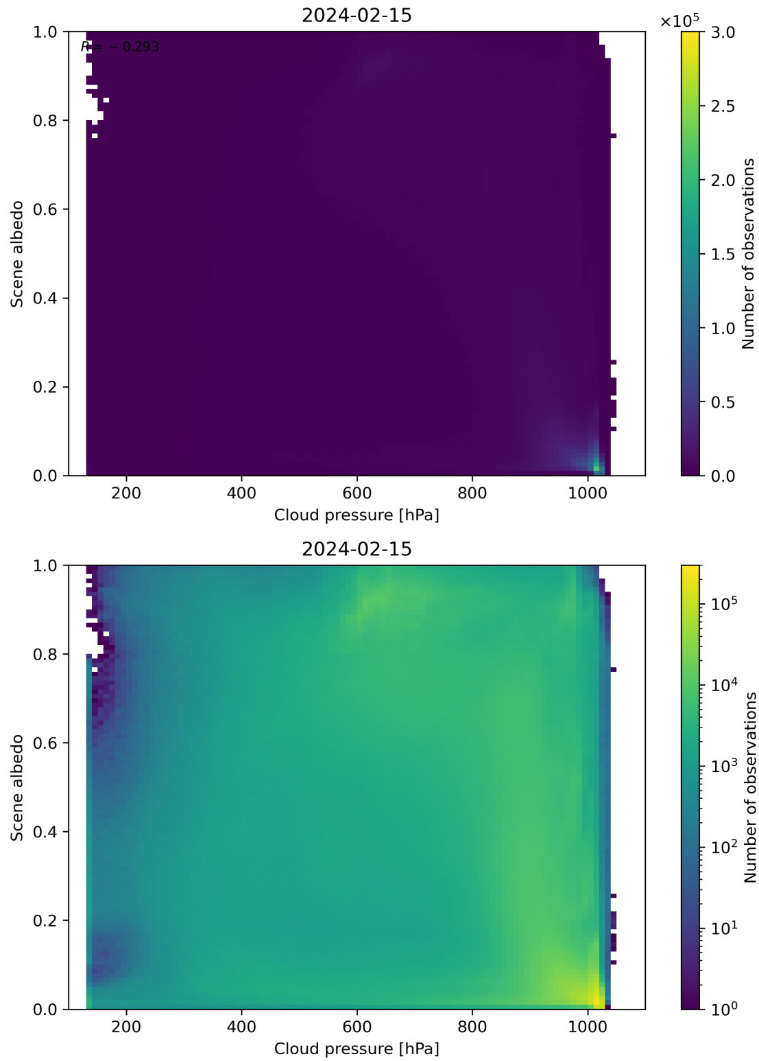
Figure 83: Scatter density plot of “Cloud pressure” against “Scene albedo” for 2024-02-14 to 2024-02-16.
