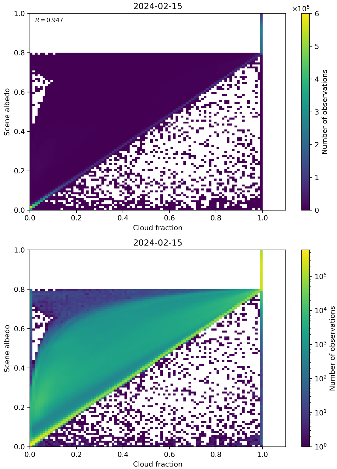
Figure 75: Scatter density plot of “Cloud fraction” against “Scene albedo” for 2024-02-14 to 2024-02-16.
