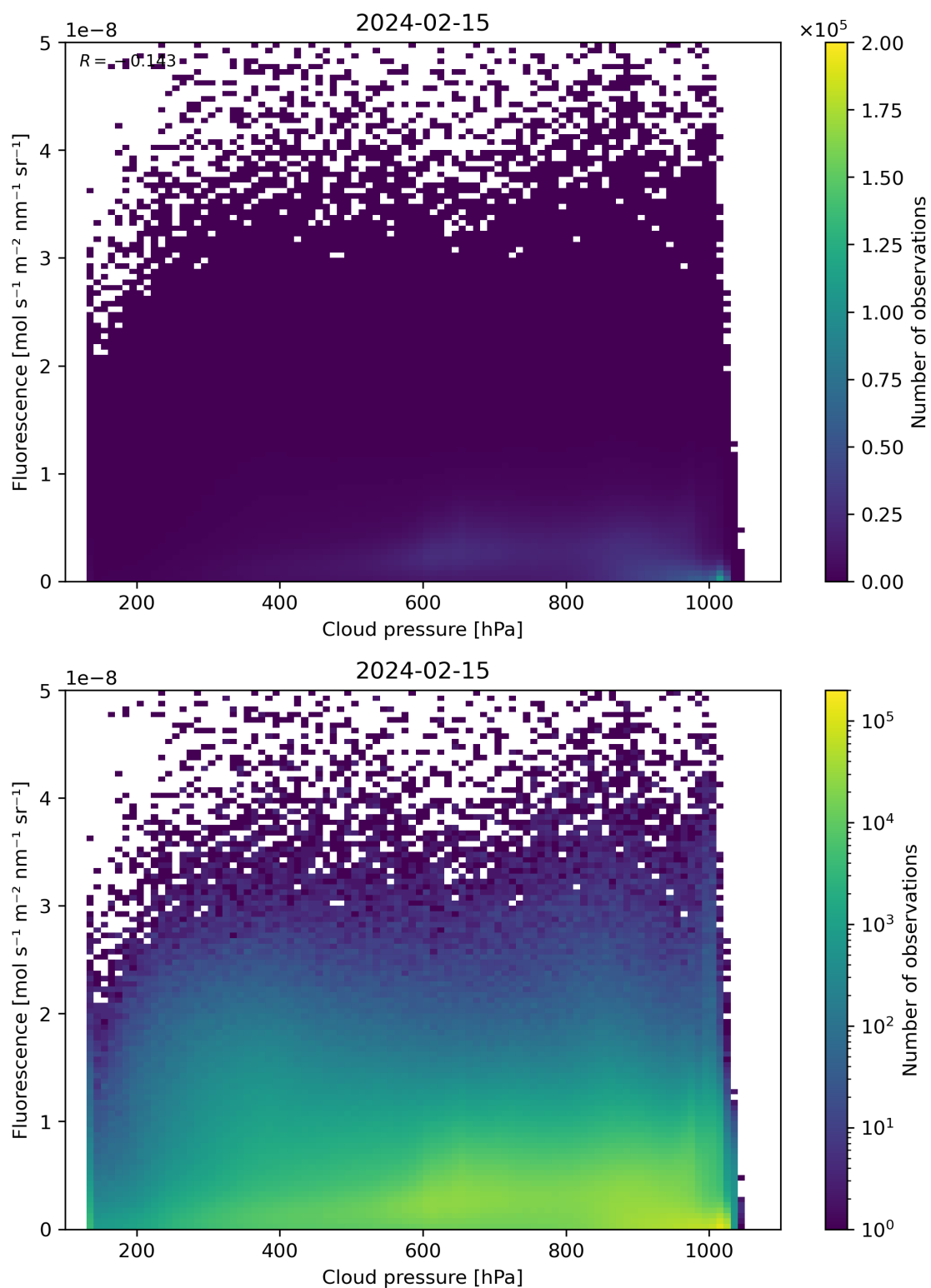
Figure 80: Scatter density plot of “Cloud pressure” against “Fluorescence” for 2024-02-14 to 2024-02-16.
