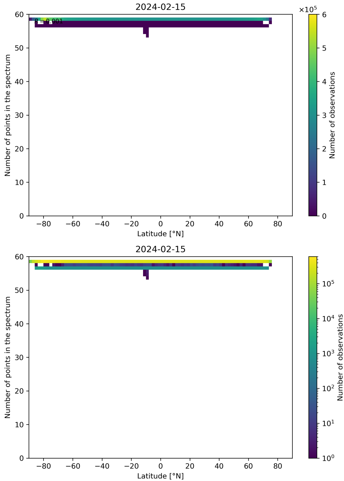
Figure 94: Scatter density plot of “Latitude” against “Number of points in the spectrum” for 2024-02-14 to 2024-02-16.
