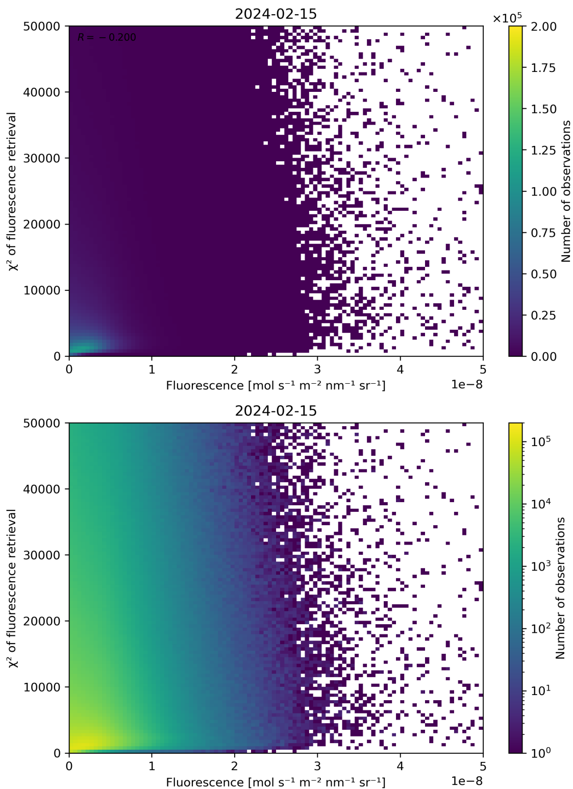
Figure 85: Scatter density plot of “Fluorescence” against “ \chi^2 of fluorescence retrieval” for 2024-02-14 to 2024-02-16.
