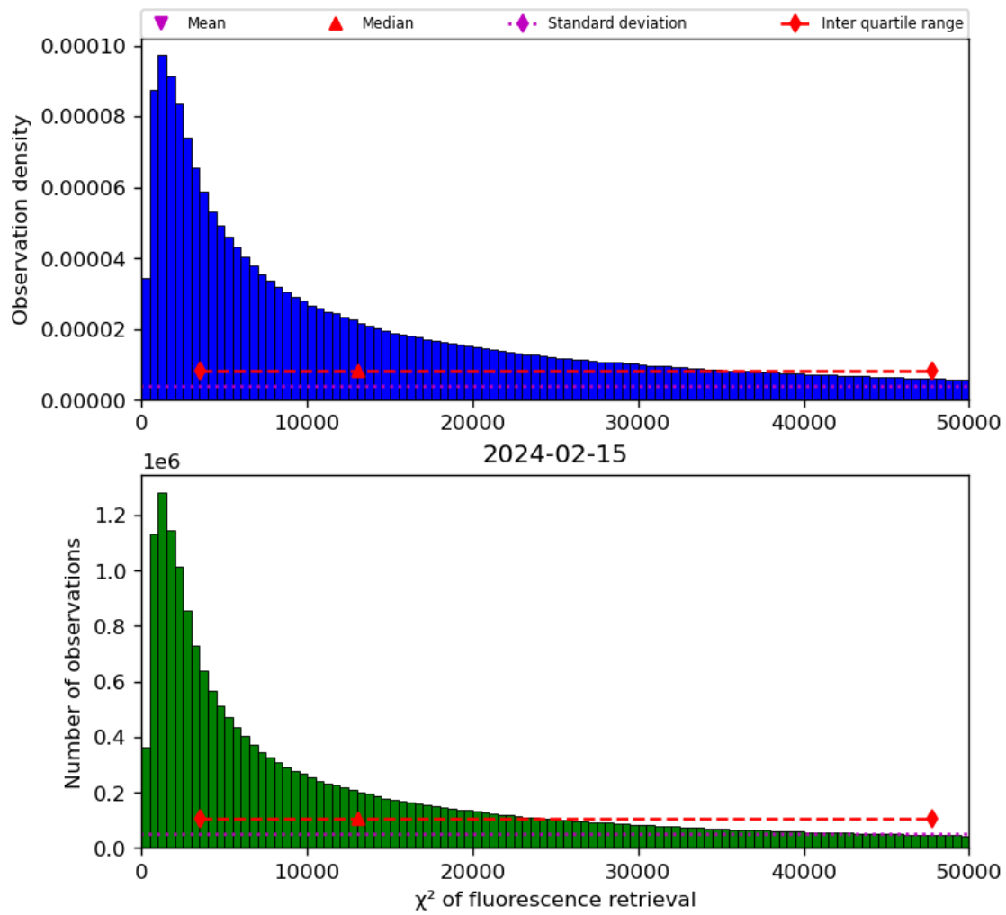
Figure 42: Histogram of “ \chi^2 of fluorescence retrieval” for 2024-02-14 to 2024-02-16
