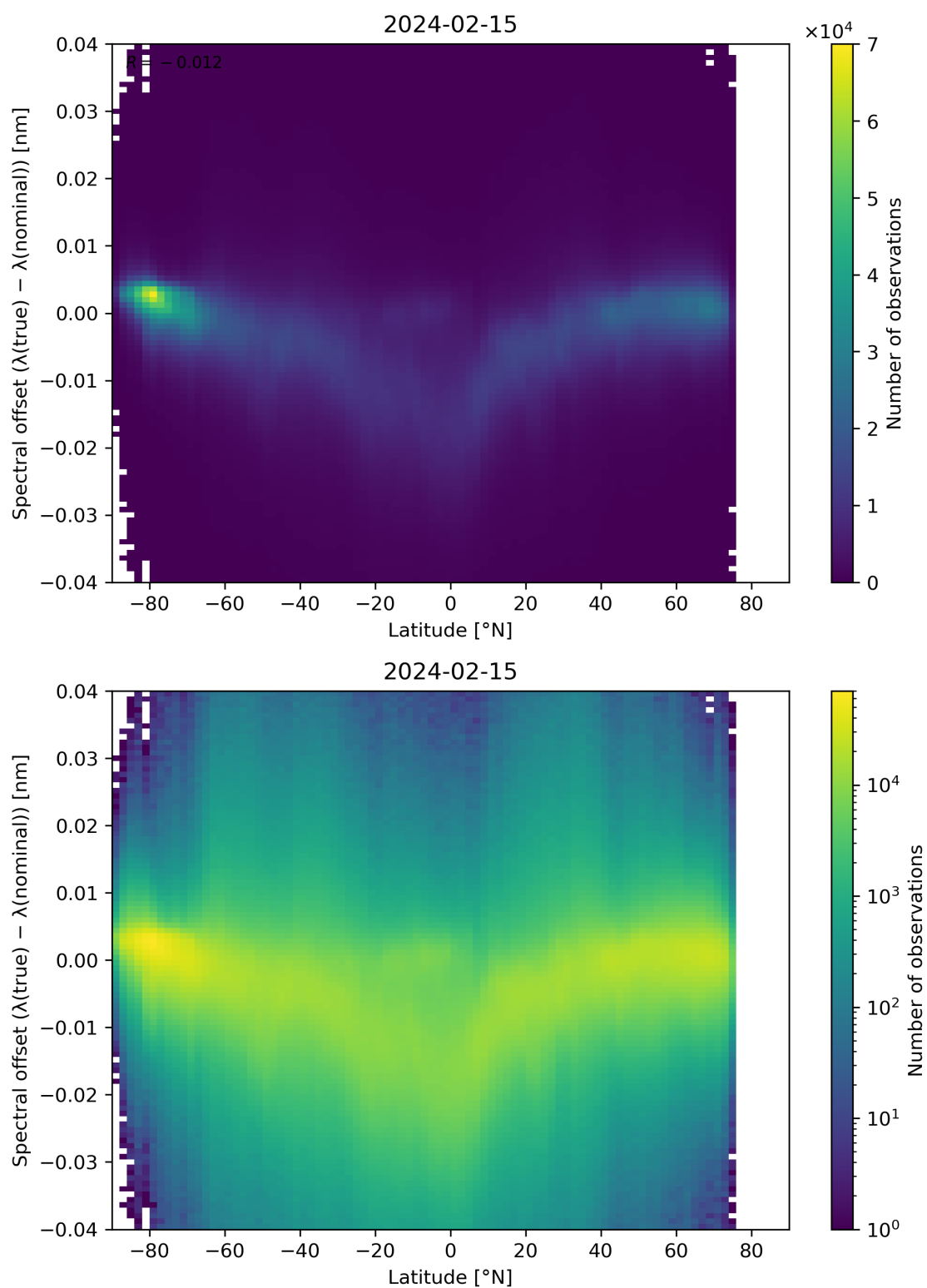
Figure 96: Scatter density plot of “Latitude” against “Spectral offset ( \lambda(\text{true}) - \lambda(\text{nominal}) )” for 2024-02-14 to 2024-02-16.
