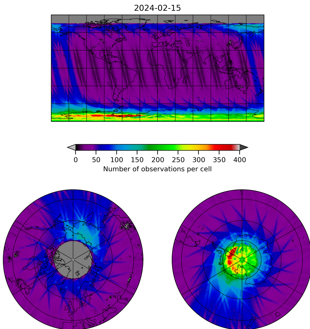
Figure 11: Map of the number of observations for 2024-02-14 to 2024-02-16
