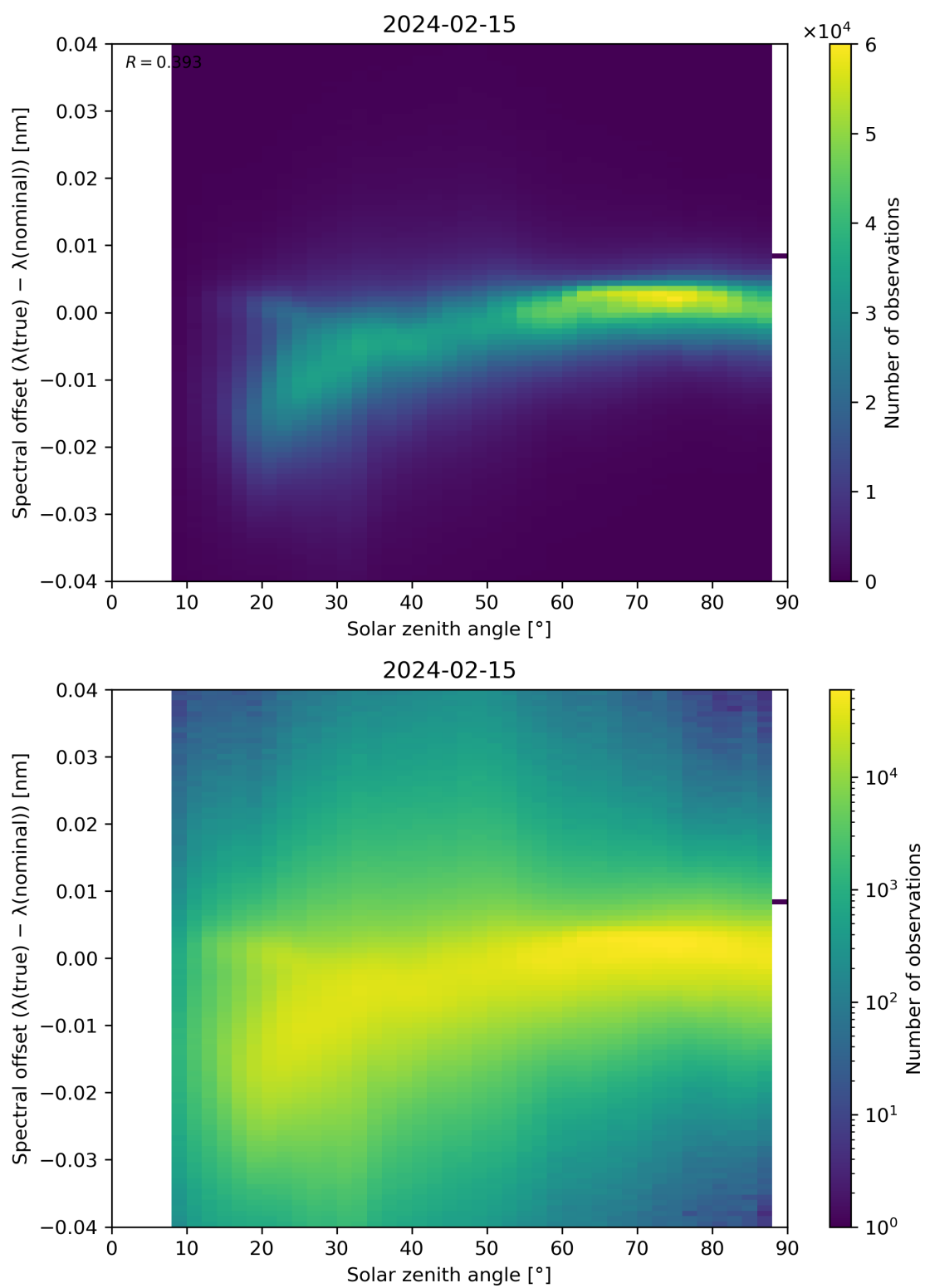
Figure 117: Scatter density plot of “Solar zenith angle” against “Spectral offset ( \lambda(\text{true}) - \lambda(\text{nominal}) )” for 2024-02-14 to 2024-02-16.
