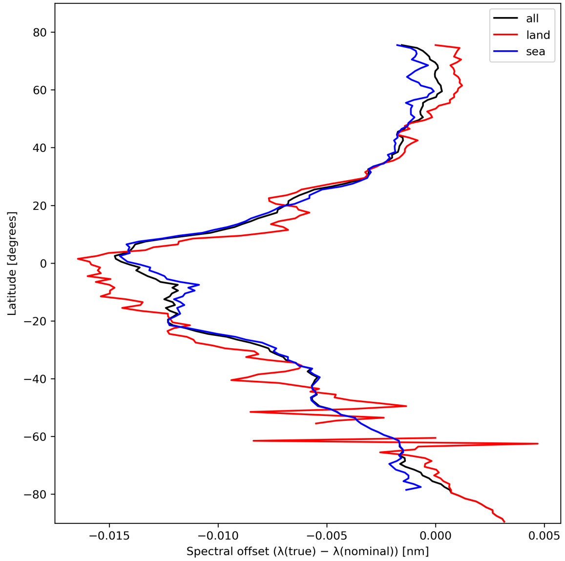
Figure 28: Zonal average of “Spectral offset ( \lambda(\text{true}) - \lambda(\text{nominal}) )” for 2024-02-14 to 2024-02-16.
