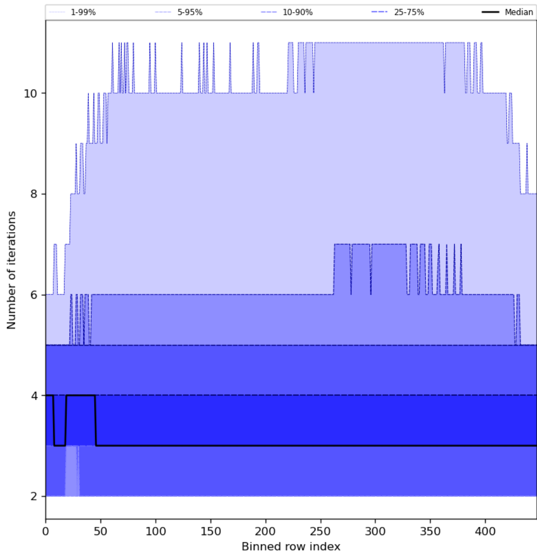
Figure 56: Along track statistics of “Number of iterations” for 2024-02-14 to 2024-02-16
