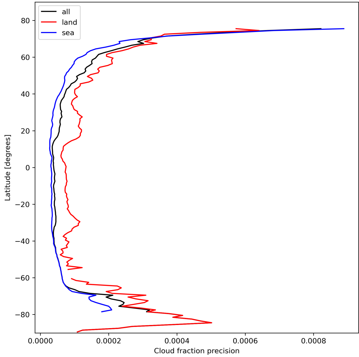
Figure 16: Zonal average of “Cloud fraction precision” for 2024-02-14 to 2024-02-16.
