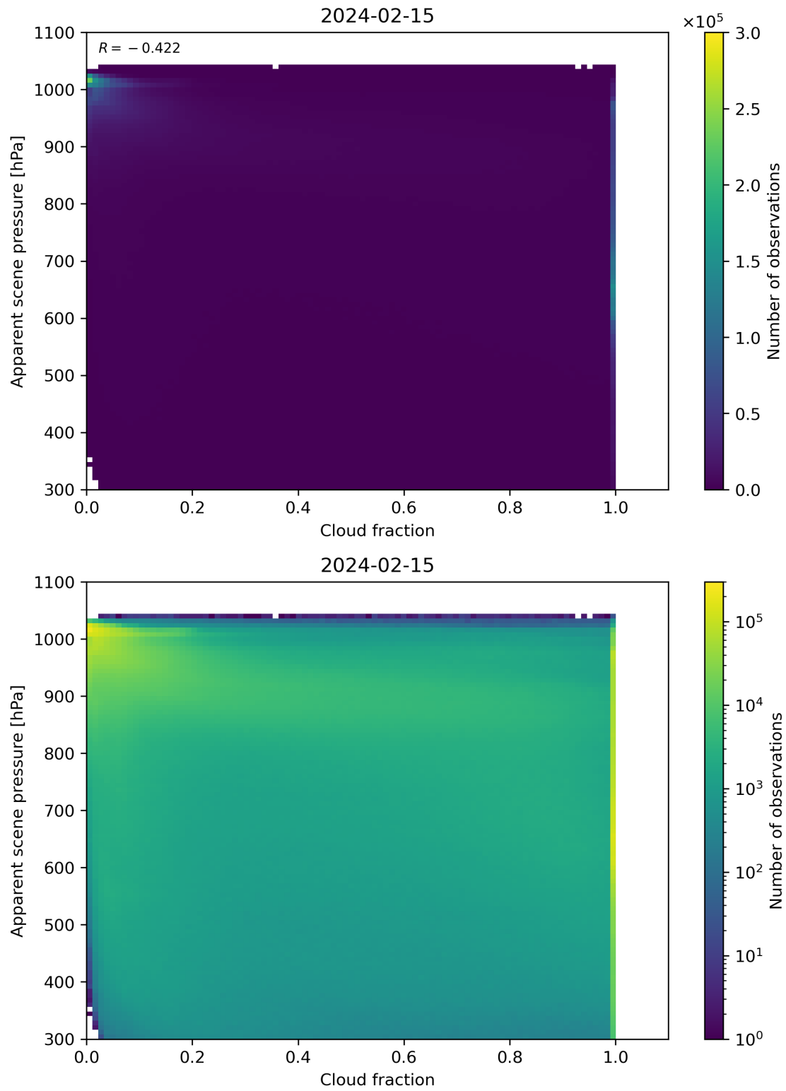
Figure 70: Scatter density plot of “Cloud fraction” against “Apparent scene pressure” for 2024-02-14 to 2024-02-16.
