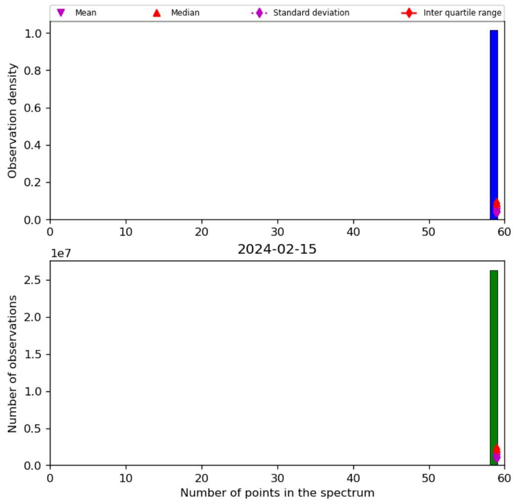
Figure 44: Histogram of “Number of points in the spectrum” for 2024-02-14 to 2024-02-16
