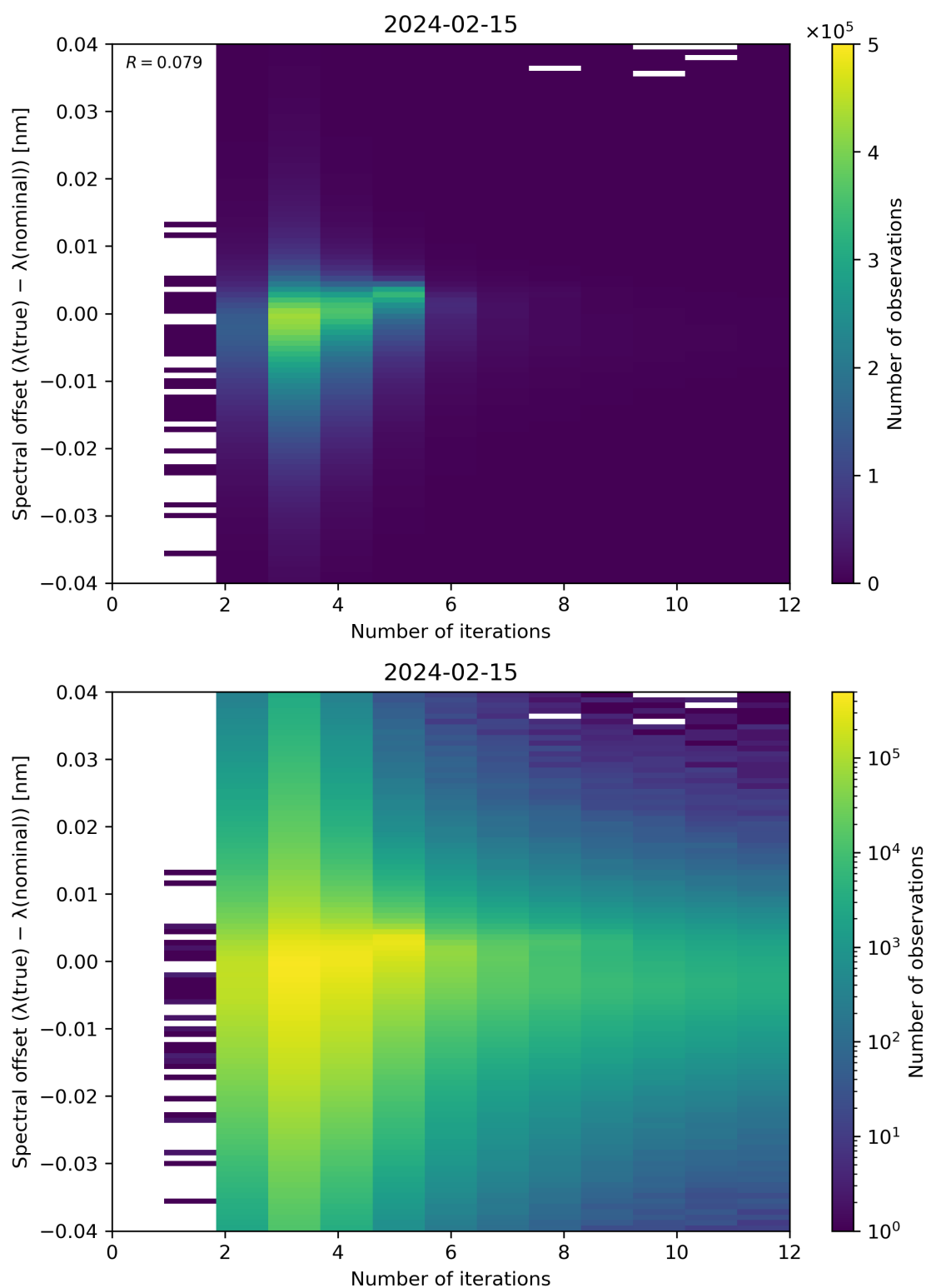
Figure 100: Scatter density plot of “Number of iterations” against “Spectral offset ( \lambda(\text{true}) - \lambda(\text{nominal}) )” for 2024-02-14 to 2024-02-16.
