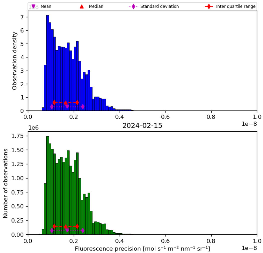
Figure 41: Histogram of “Fluorescence precision” for 2024-02-14 to 2024-02-16
