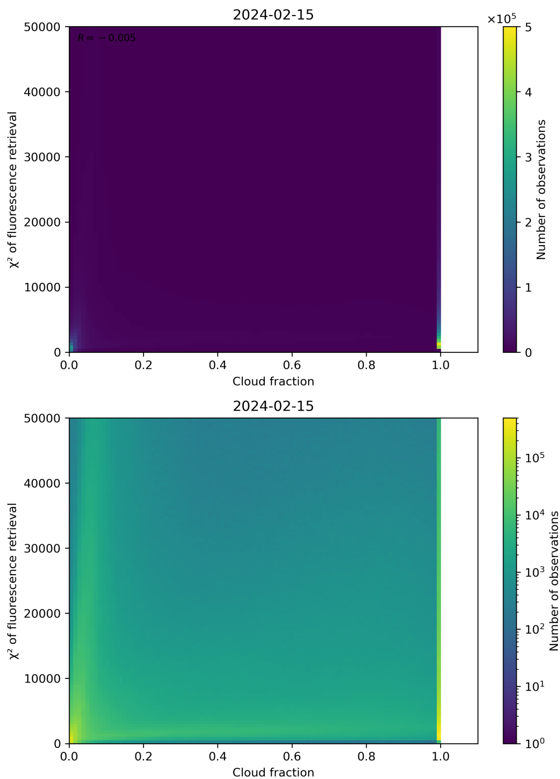
Figure 71: Scatter density plot of “Cloud fraction” against “ \chi^2 of fluorescence retrieval” for 2024-02-14 to 2024-02-16.
