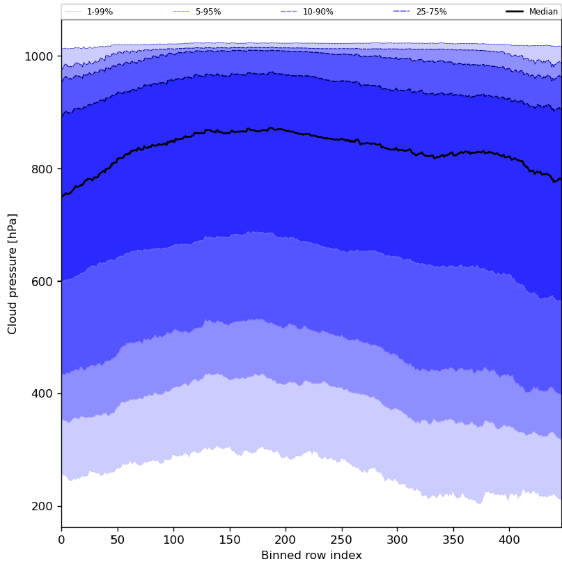
Figure 47: Along track statistics of “Cloud pressure” for 2024-02-14 to 2024-02-16
