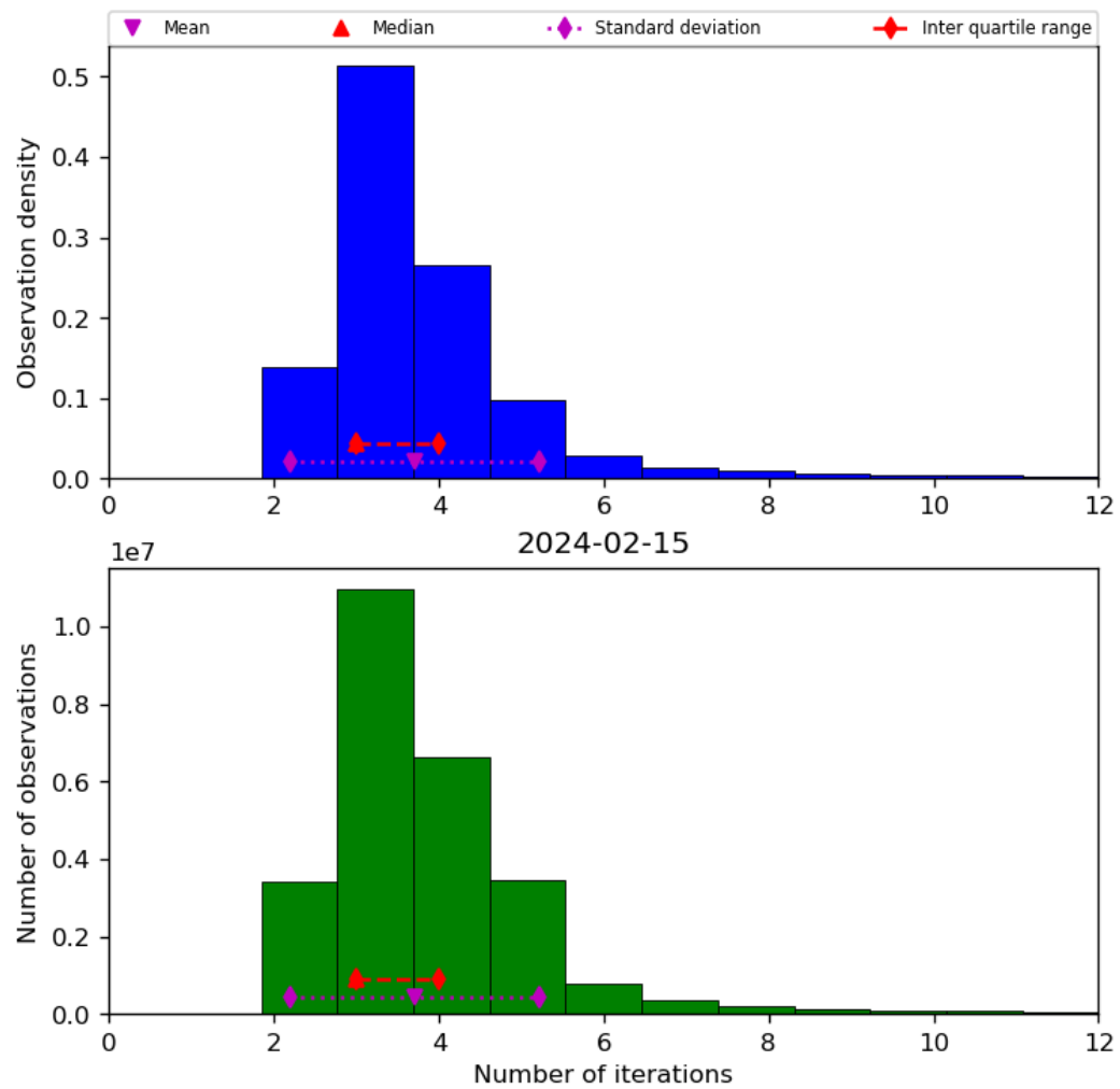
Figure 39: Histogram of “Number of iterations” for 2024-02-14 to 2024-02-16
