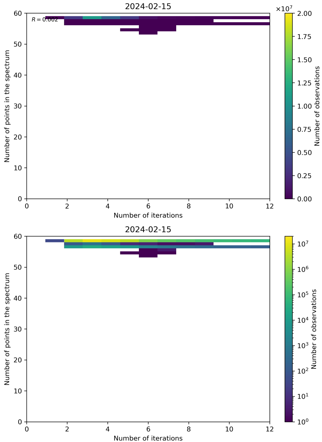
Figure 99: Scatter density plot of “Number of iterations” against “Number of points in the spectrum” for 2024-02-14 to 2024-02-16.
