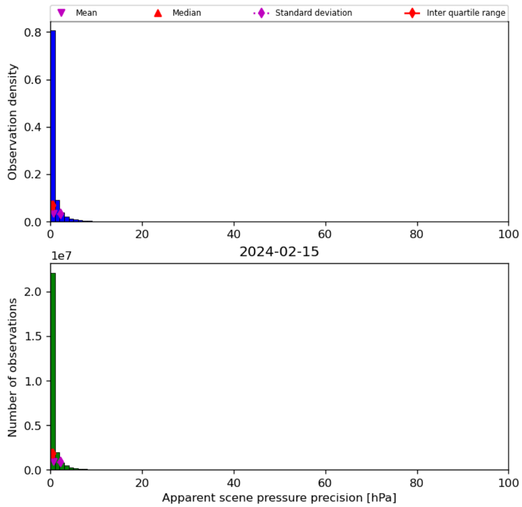
Figure 37: Histogram of “Apparent scene pressure precision” for 2024-02-14 to 2024-02-16
