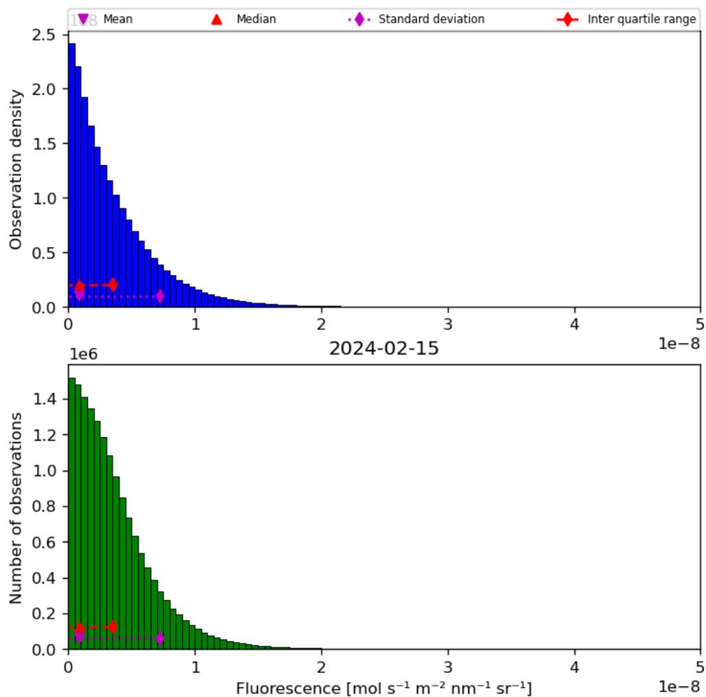
Figure 40: Histogram of “Fluorescence” for 2024-02-14 to 2024-02-16
