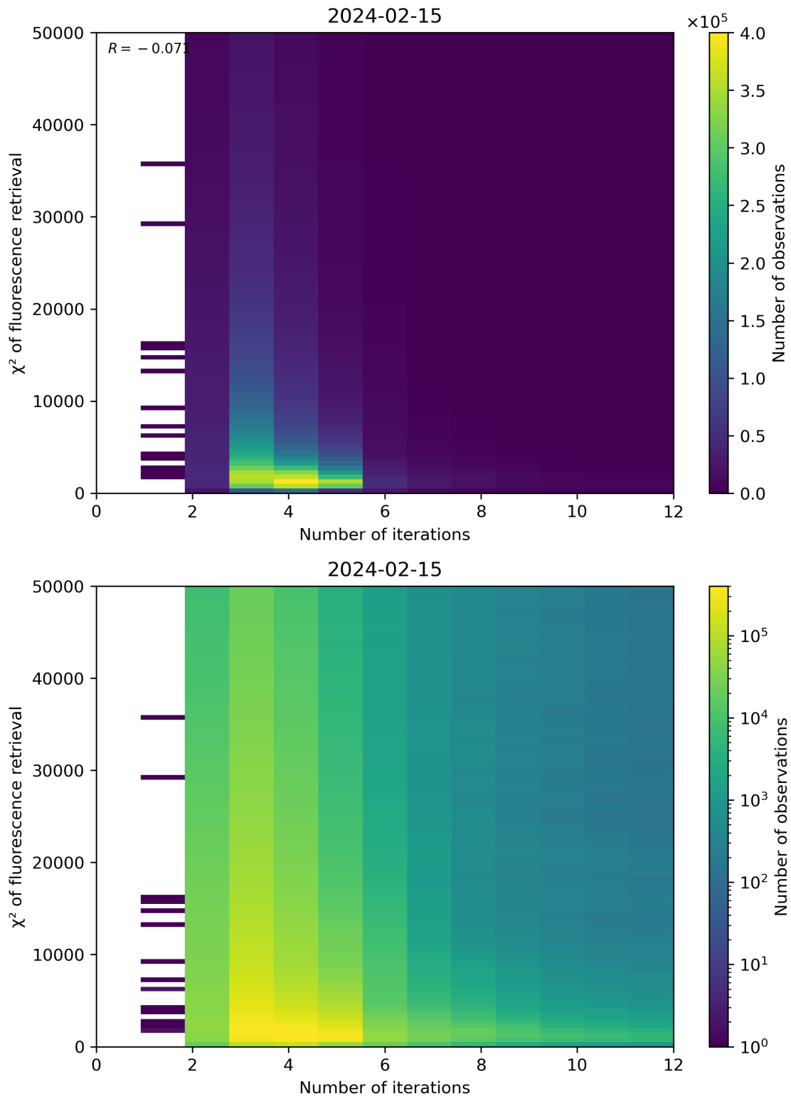
Figure 97: Scatter density plot of “Number of iterations” against “ \chi^2 of fluorescence retrieval” for 2024-02-14 to 2024-02-16.
