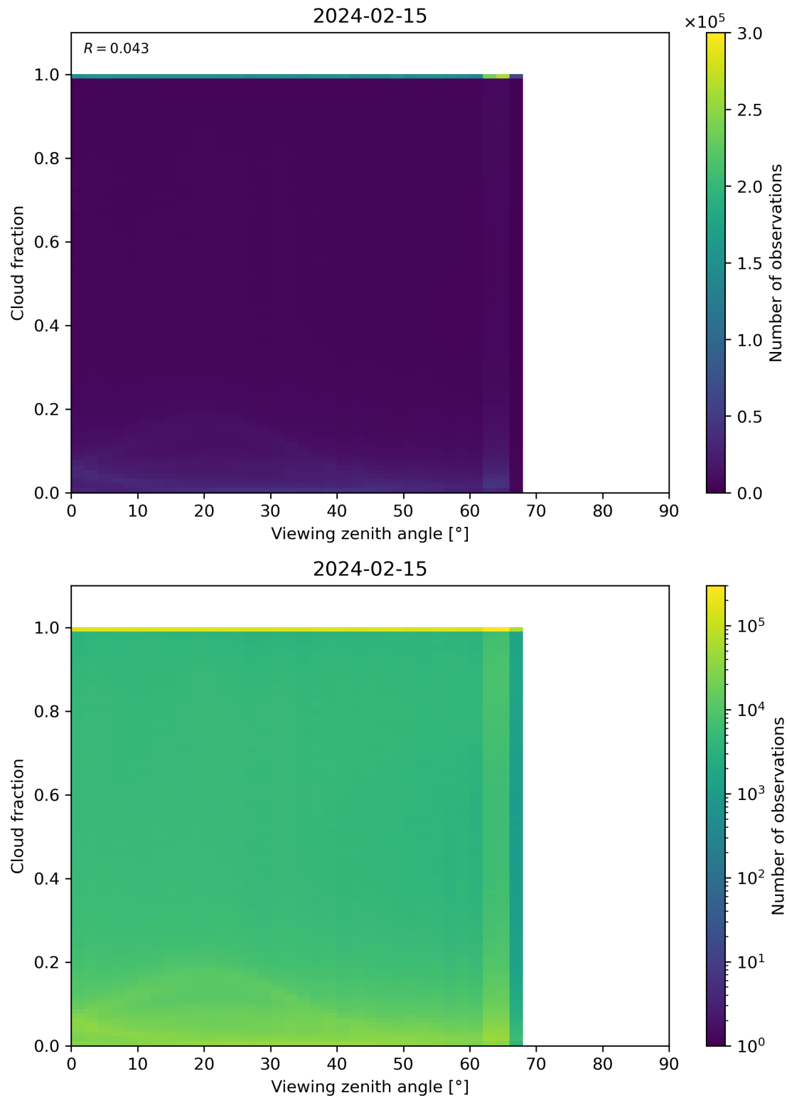
Figure 120: Scatter density plot of “Viewing zenith angle” against “Cloud fraction” for 2024-02-14 to 2024-02-16.
