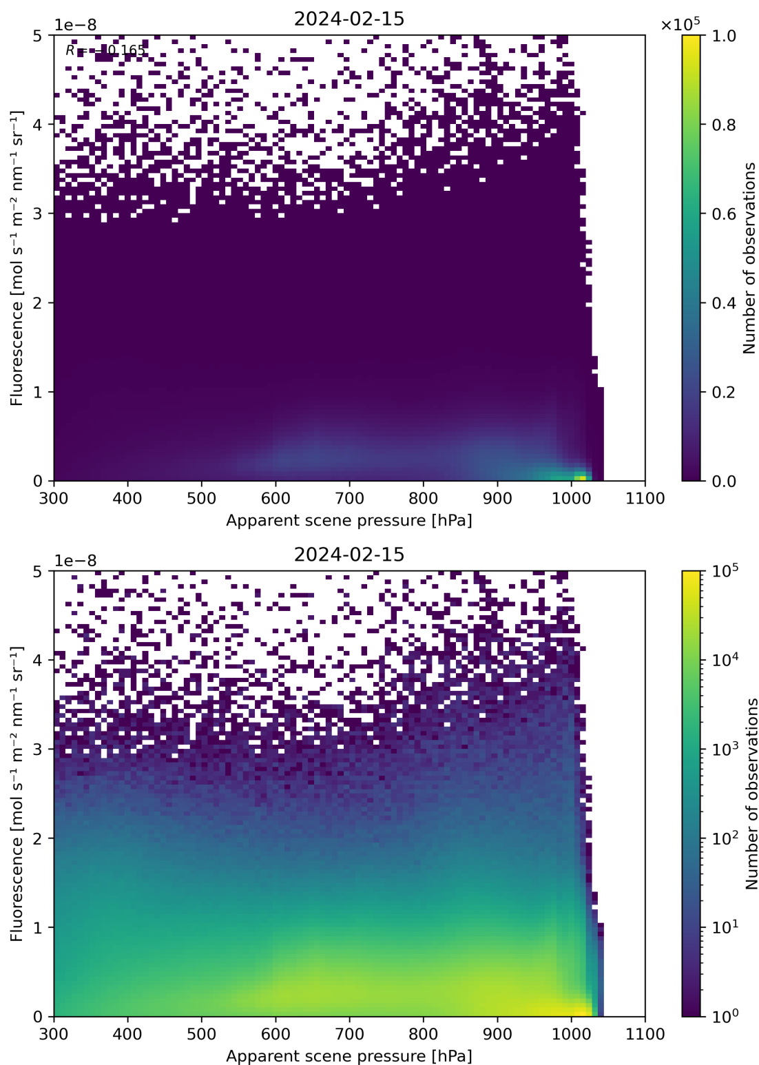
Figure 64: Scatter density plot of “Apparent scene pressure” against “Fluorescence” for 2024-02-14 to 2024-02-16.
