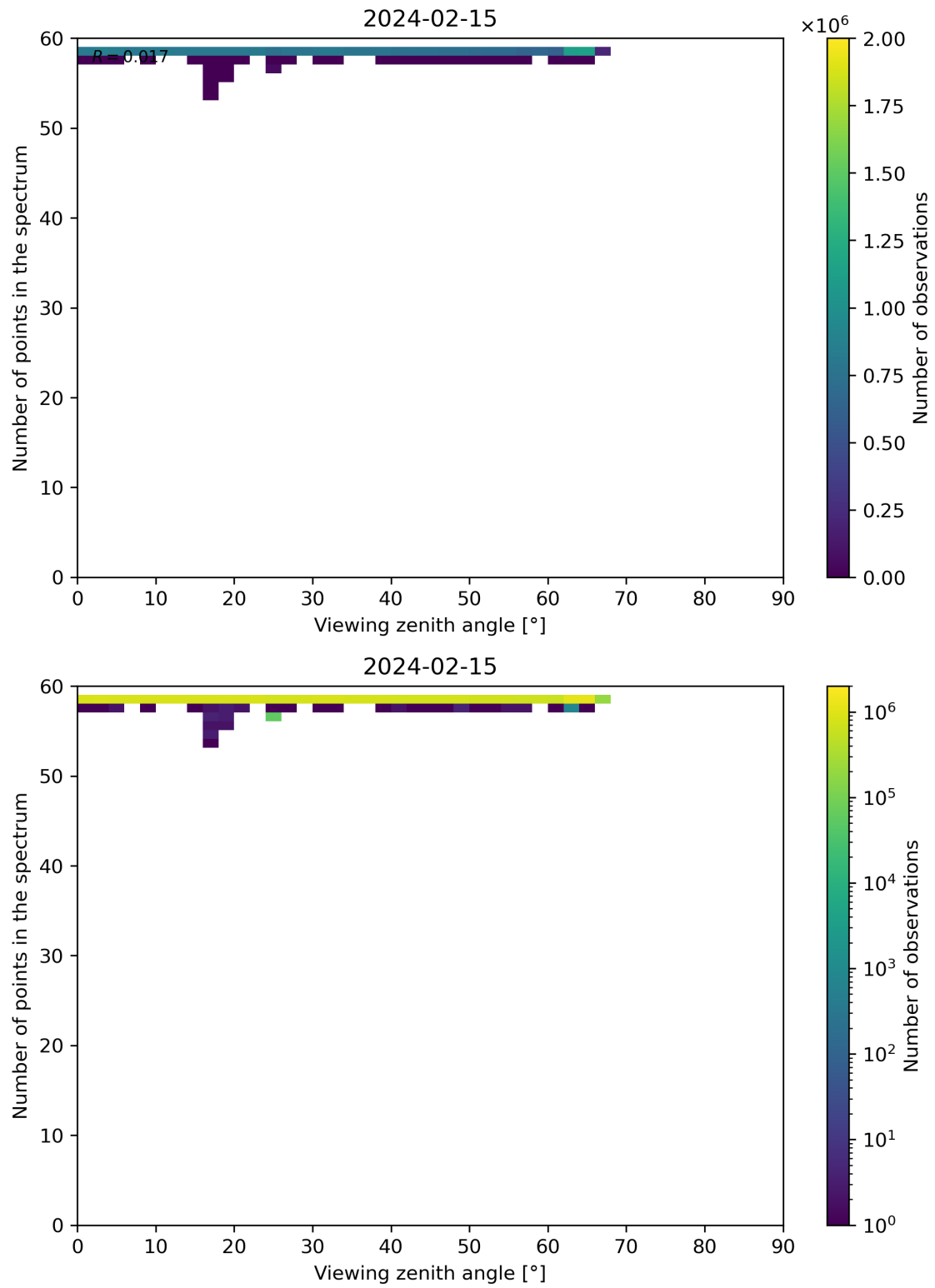
Figure 125: Scatter density plot of “Viewing zenith angle” against “Number of points in the spectrum” for 2024-02-14 to 2024-02-16.
