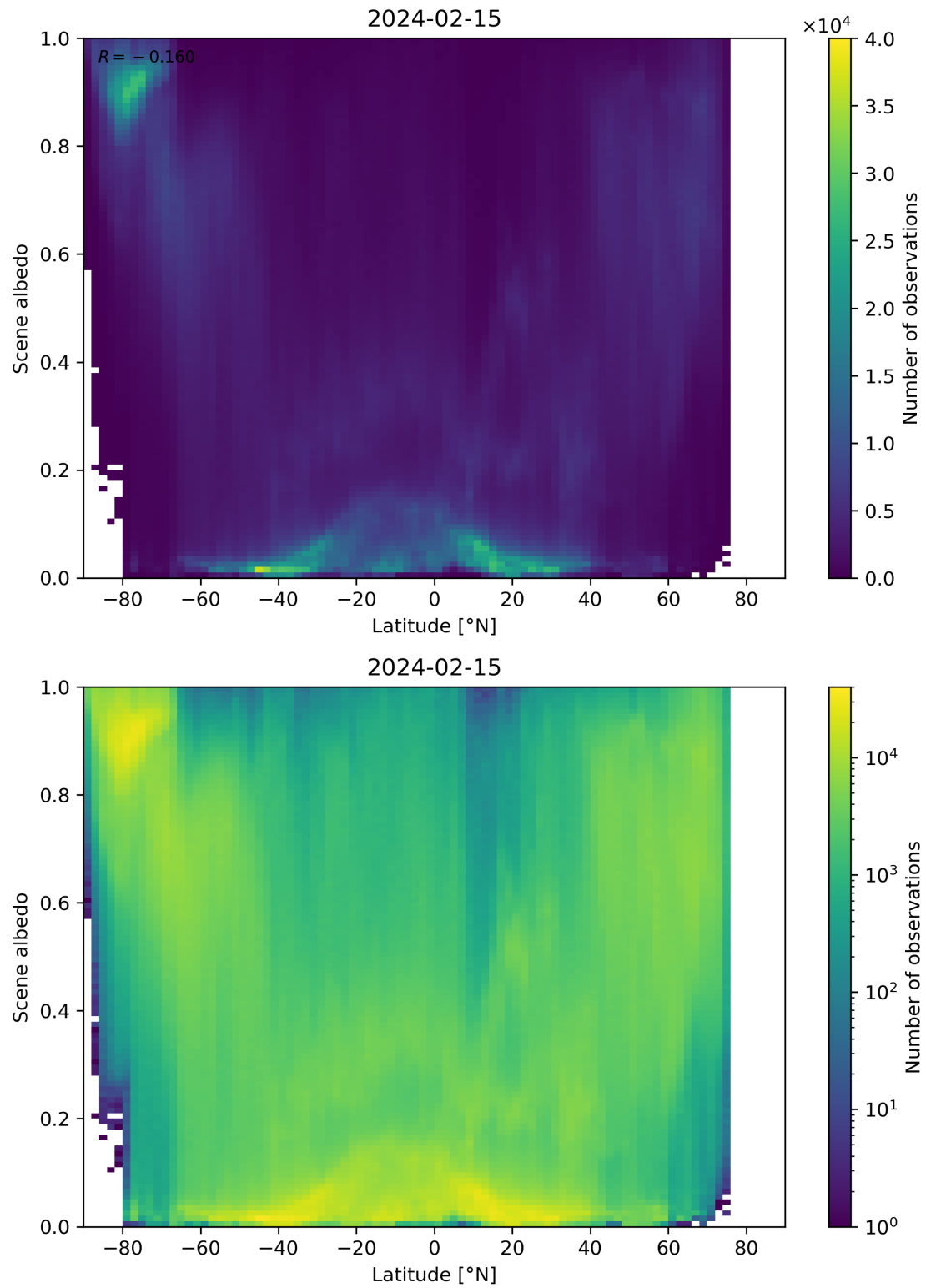
Figure 95: Scatter density plot of “Latitude” against “Scene albedo” for 2024-02-14 to 2024-02-16.
