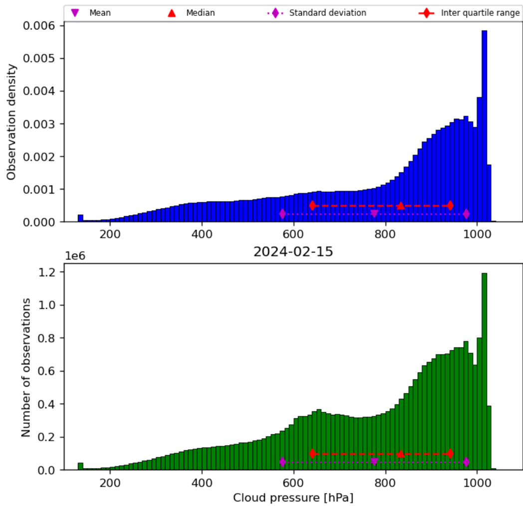
Figure 30: Histogram of “Cloud pressure” for 2024-02-14 to 2024-02-16
