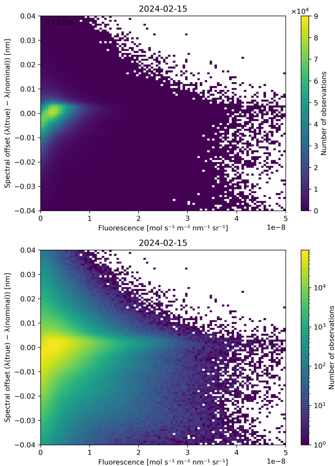
Figure 87: Scatter density plot of “Fluorescence” against “Spectral offset ( \lambda(\text{true}) - \lambda(\text{nominal}) )” for 2024-02-14 to 2024-02-16.
