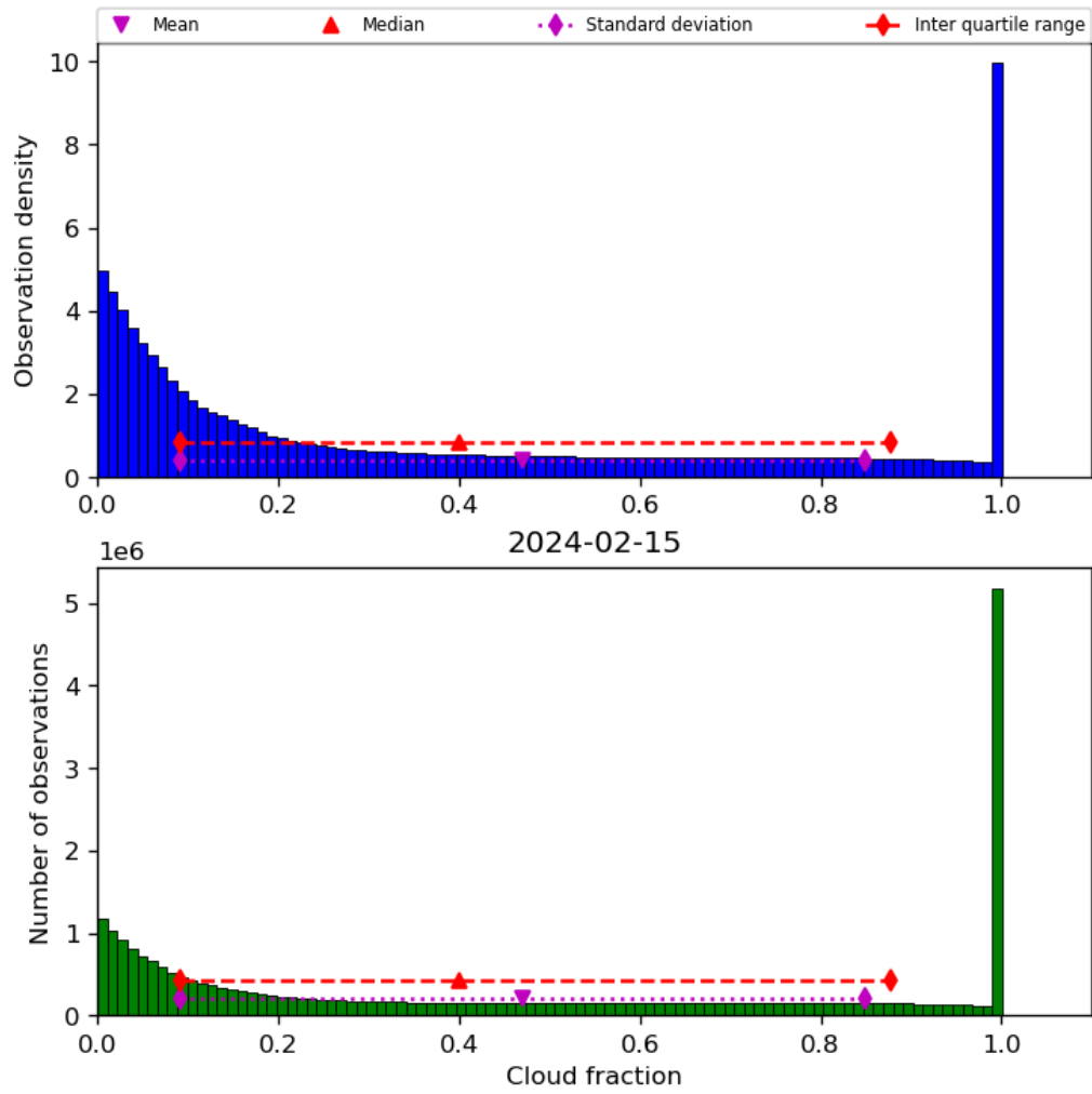
Figure 32: Histogram of “Cloud fraction” for 2024-02-14 to 2024-02-16
