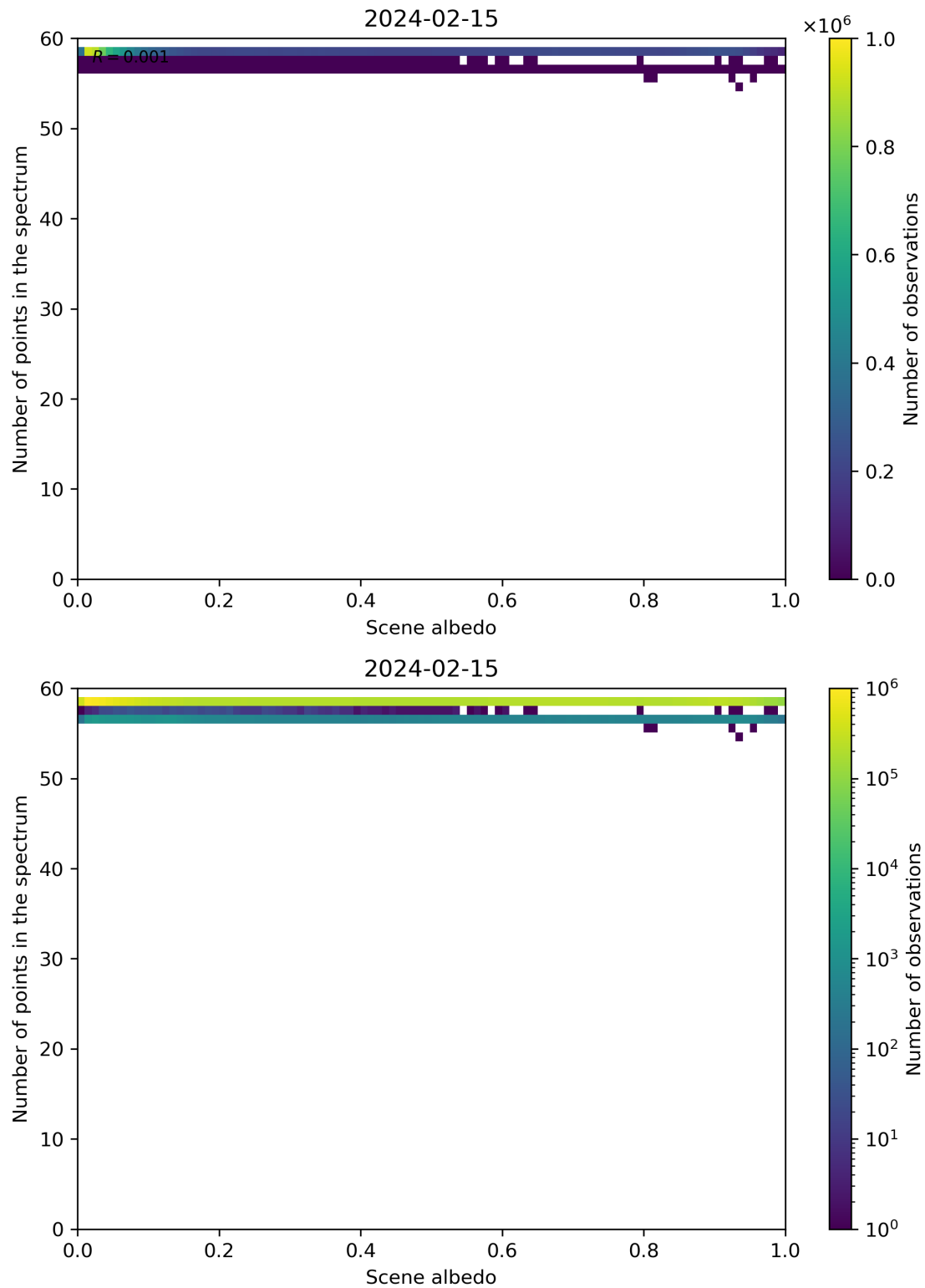
Figure 106: Scatter density plot of “Scene albedo” against “Number of points in the spectrum” for 2024-02-14 to 2024-02-16.
