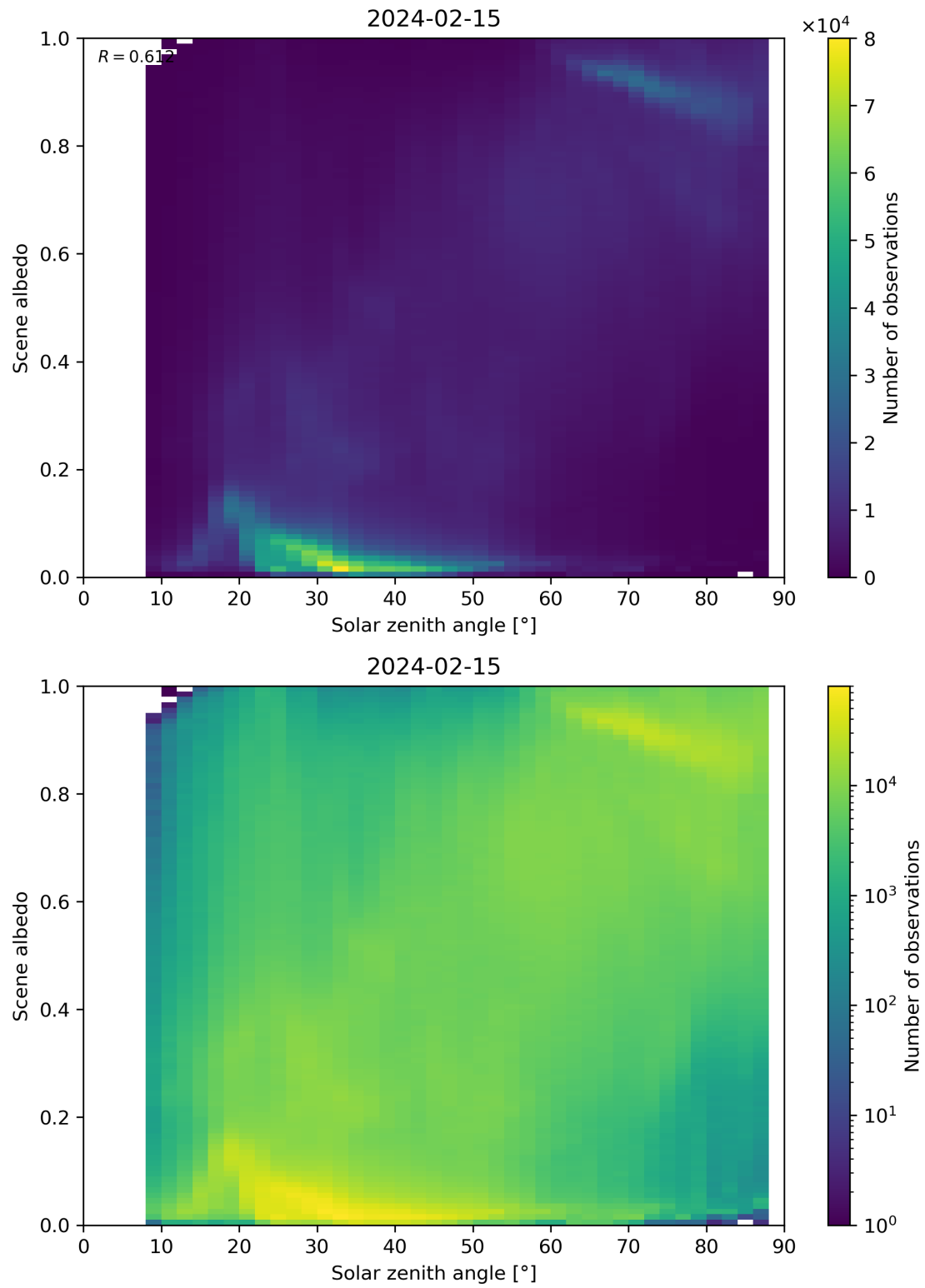
Figure 116: Scatter density plot of “Solar zenith angle” against “Scene albedo” for 2024-02-14 to 2024-02-16.
