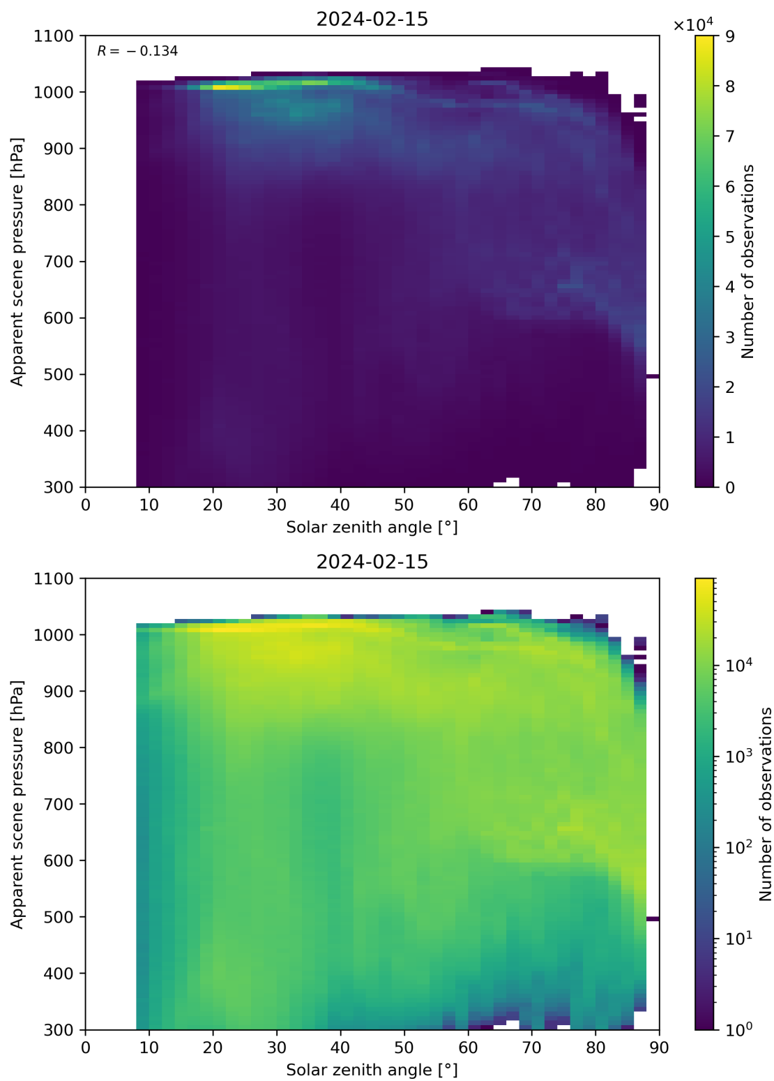
Figure 108: Scatter density plot of “Solar zenith angle” against “Apparent scene pressure” for 2024-02-14 to 2024-02-16.
