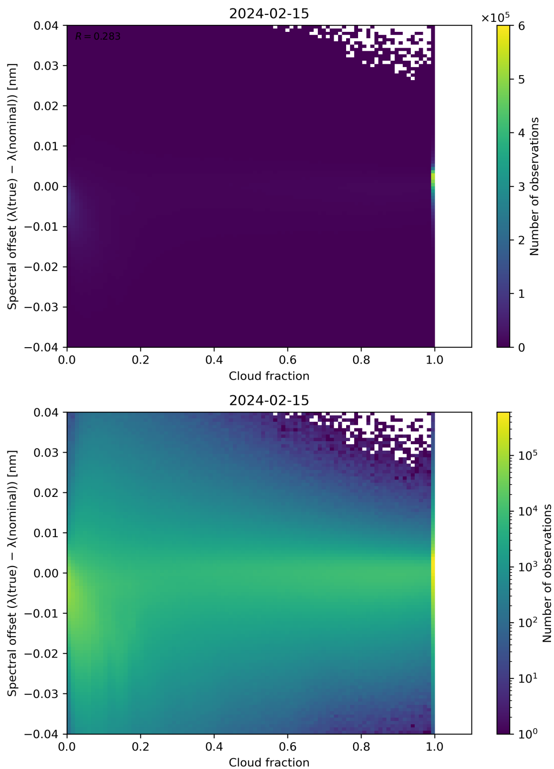
Figure 76: Scatter density plot of “Cloud fraction” against “Spectral offset ( \lambda(\text{true}) - \lambda(\text{nominal}) )” for 2024-02-14 to 2024-02-16.
