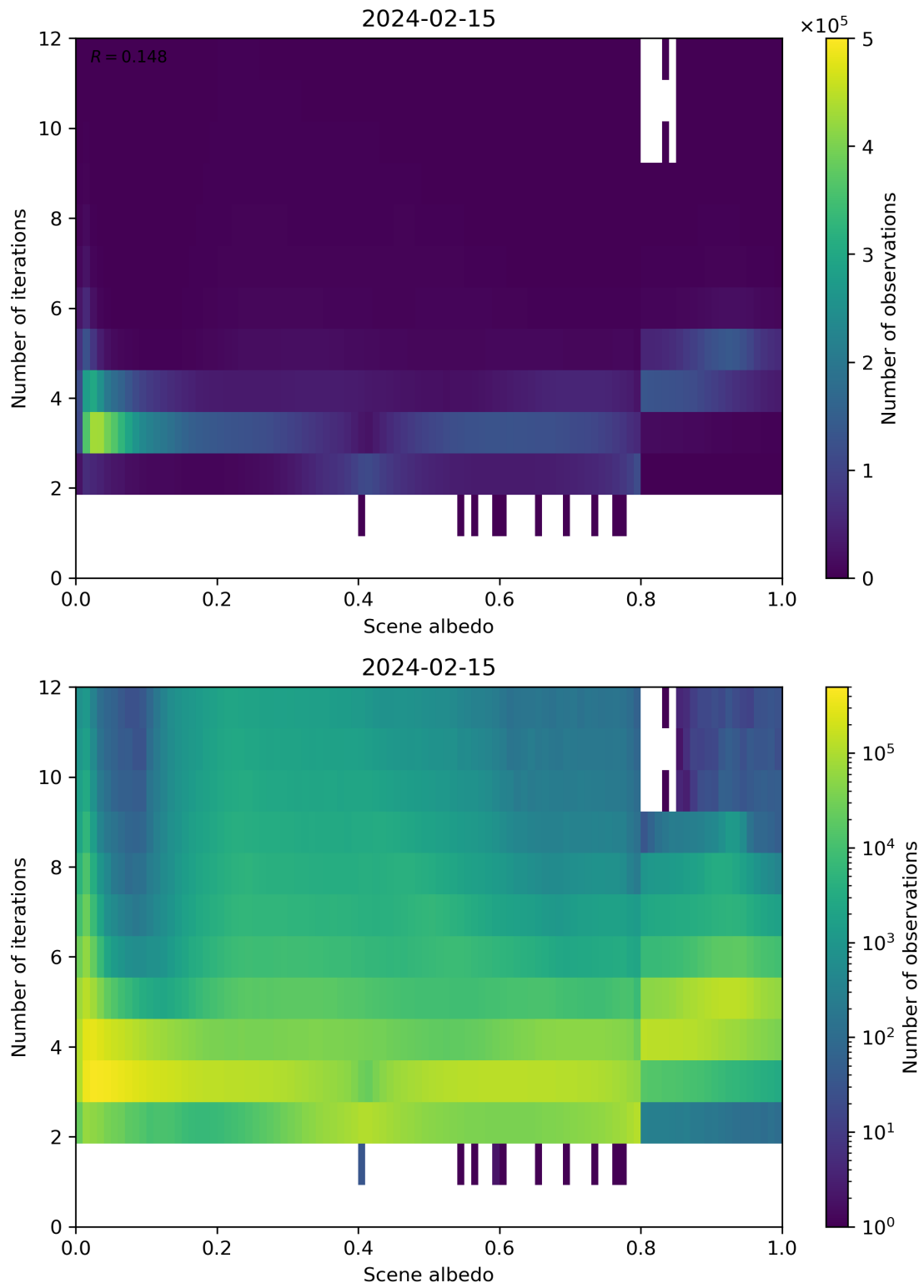
Figure 105: Scatter density plot of “Scene albedo” against “Number of iterations” for 2024-02-14 to 2024-02-16.
