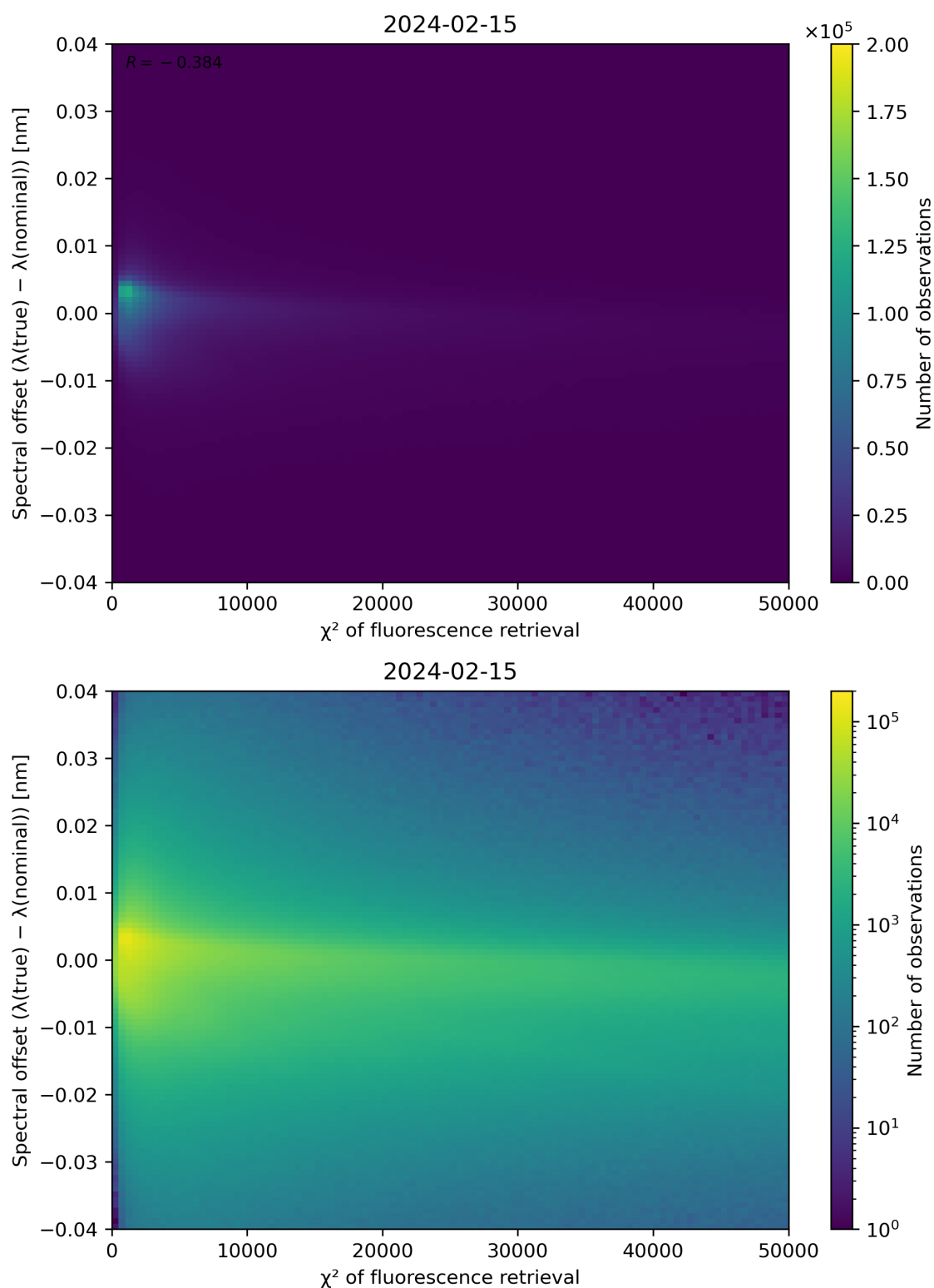
Figure 69: Scatter density plot of " \chi^2 of fluorescence retrieval" against "Spectral offset ( \lambda(\text{true}) - \lambda(\text{nominal}) )" for 2024-02-14 to 2024-02-16.
