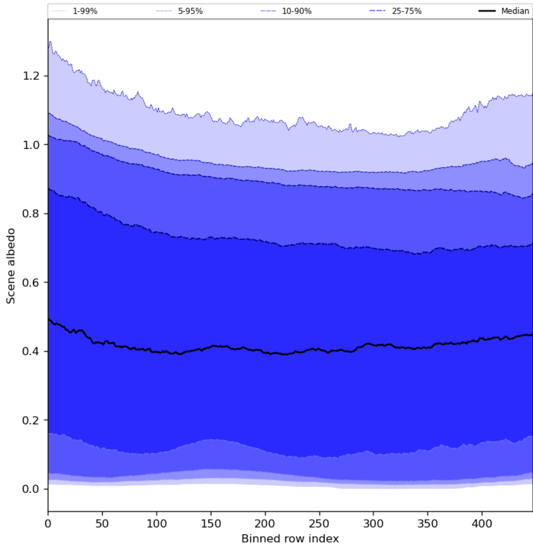
Figure 51: Along track statistics of “Scene albedo” for 2024-02-14 to 2024-02-16
