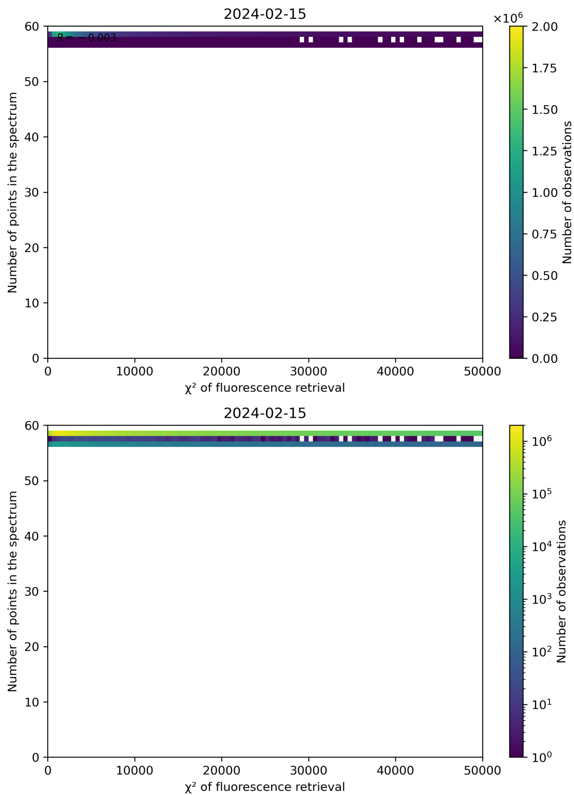
Figure 68: Scatter density plot of " \chi^2 of fluorescence retrieval" against "Number of points in the spectrum" for 2024-02-14 to 2024-02-16.
