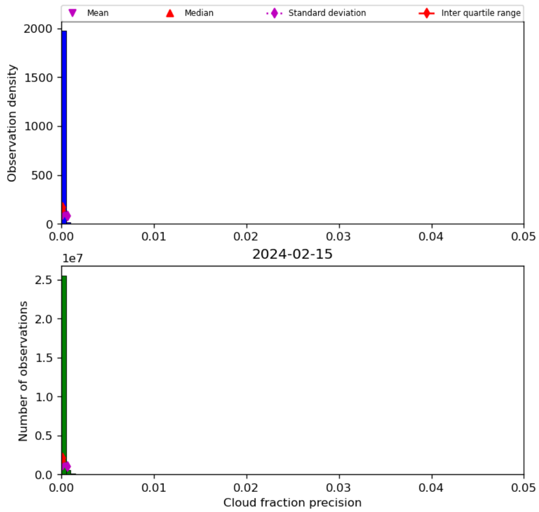
Figure 33: Histogram of “Cloud fraction precision” for 2024-02-14 to 2024-02-16
