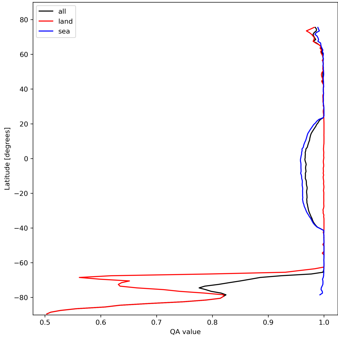
Figure 12: Zonal average of “QA value” for 2024-02-14 to 2024-02-16.
