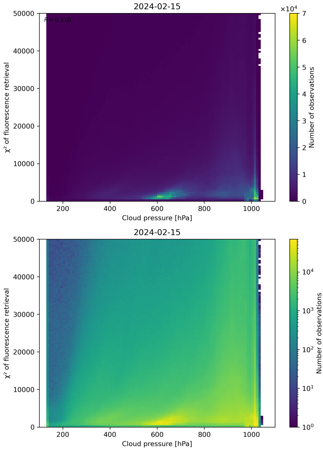
Figure 78: Scatter density plot of “Cloud pressure” against “ \chi^2 of fluorescence retrieval” for 2024-02-14 to 2024-02-16.
