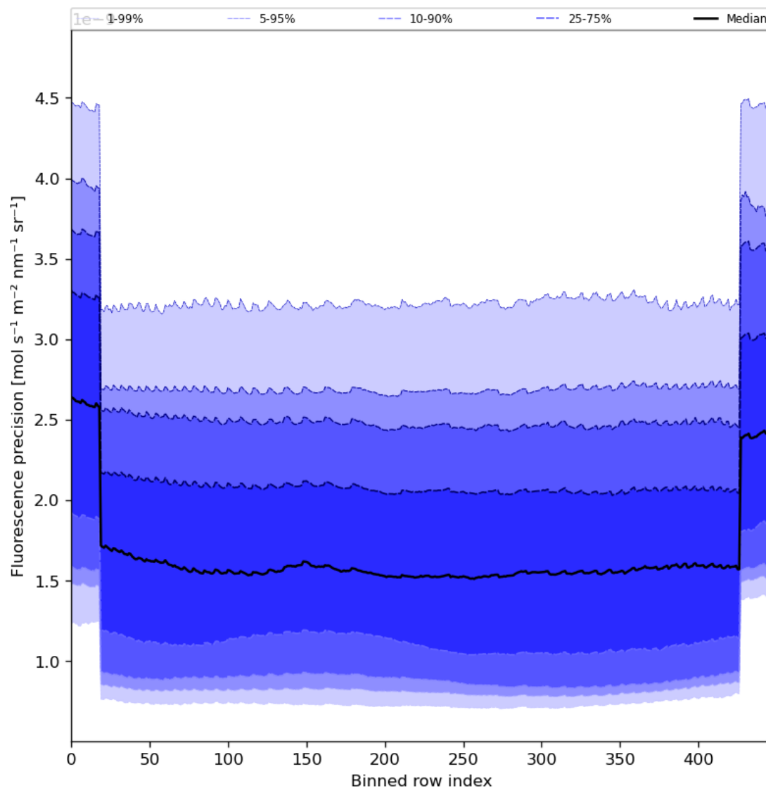
Figure 58: Along track statistics of “Fluorescence precision” for 2024-02-14 to 2024-02-16
