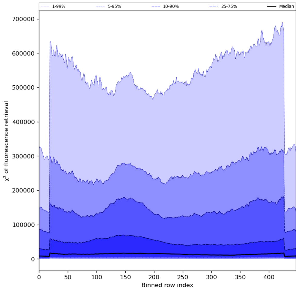
Figure 59: Along track statistics of “ \chi^2 of fluorescence retrieval” for 2024-02-14 to 2024-02-16
