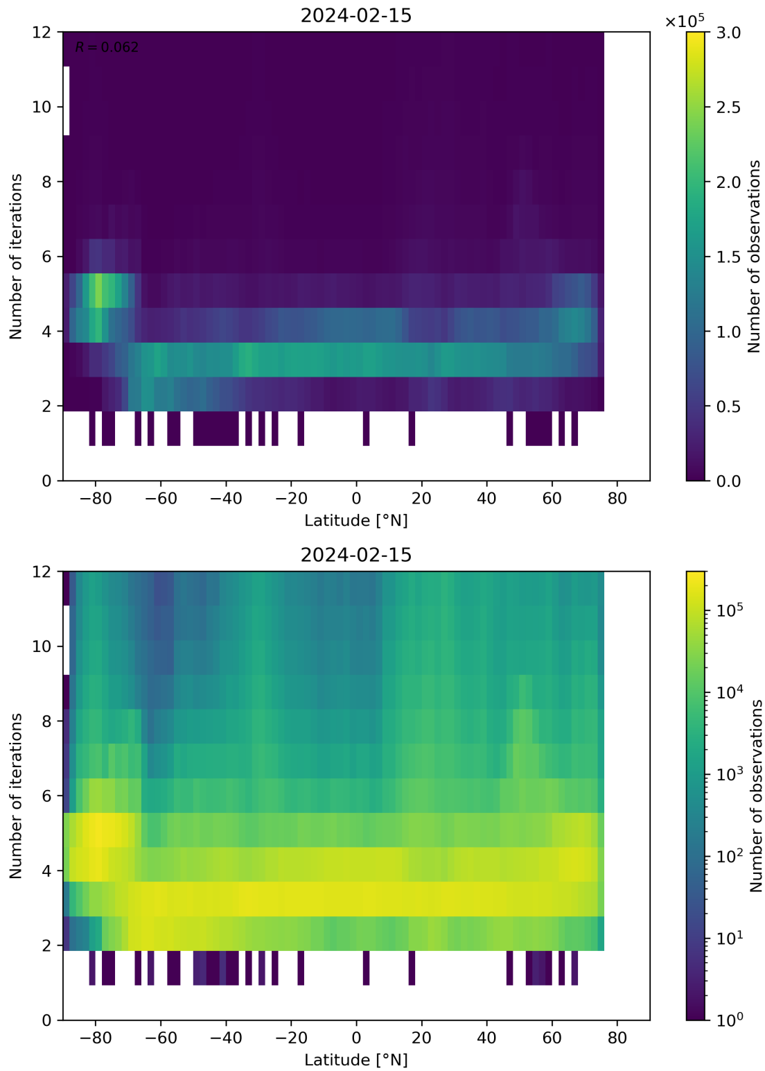
Figure 93: Scatter density plot of “Latitude” against “Number of iterations” for 2024-02-14 to 2024-02-16.
