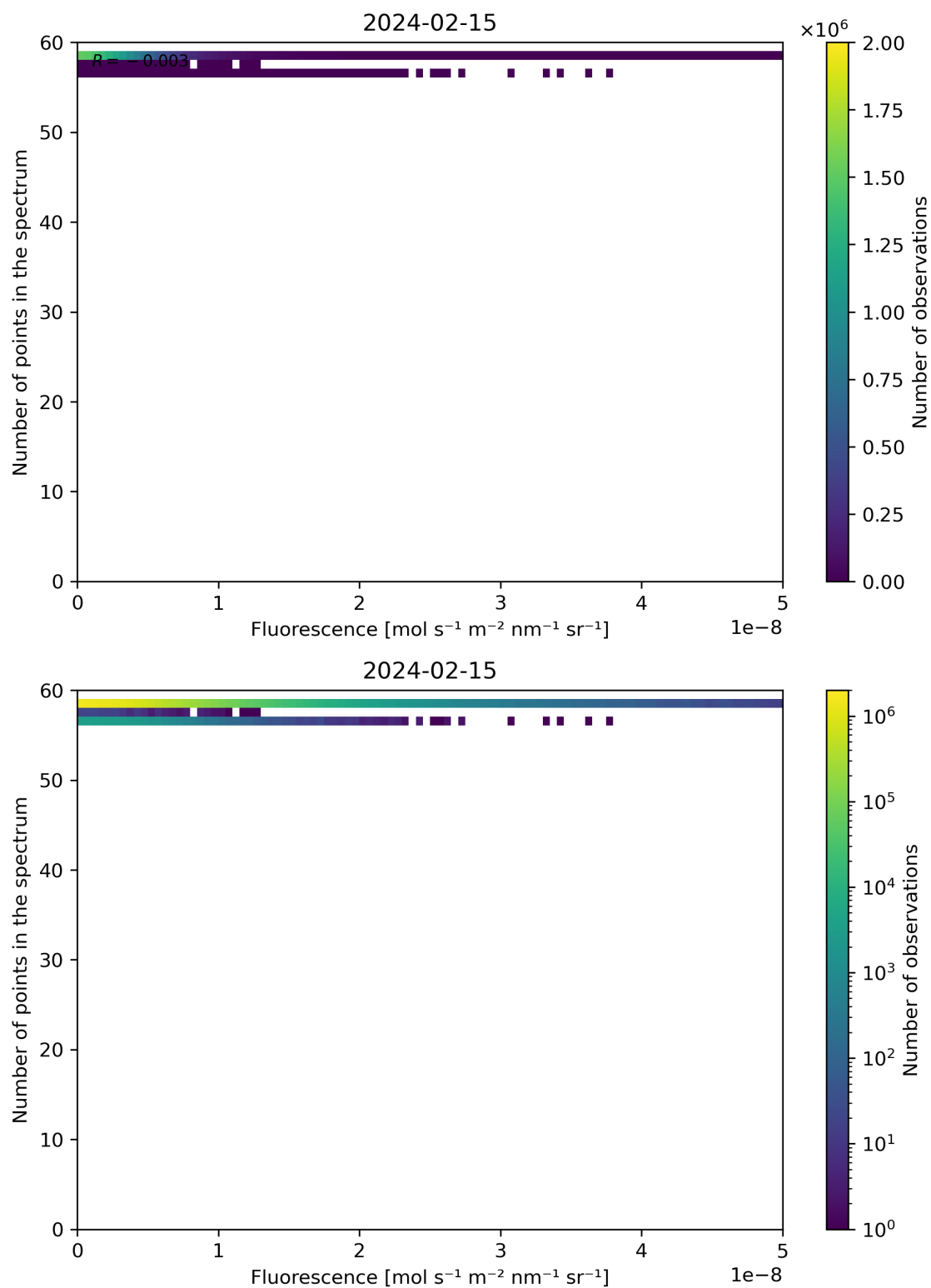
Figure 86: Scatter density plot of “Fluorescence” against “Number of points in the spectrum” for 2024-02-14 to 2024-02-16.
