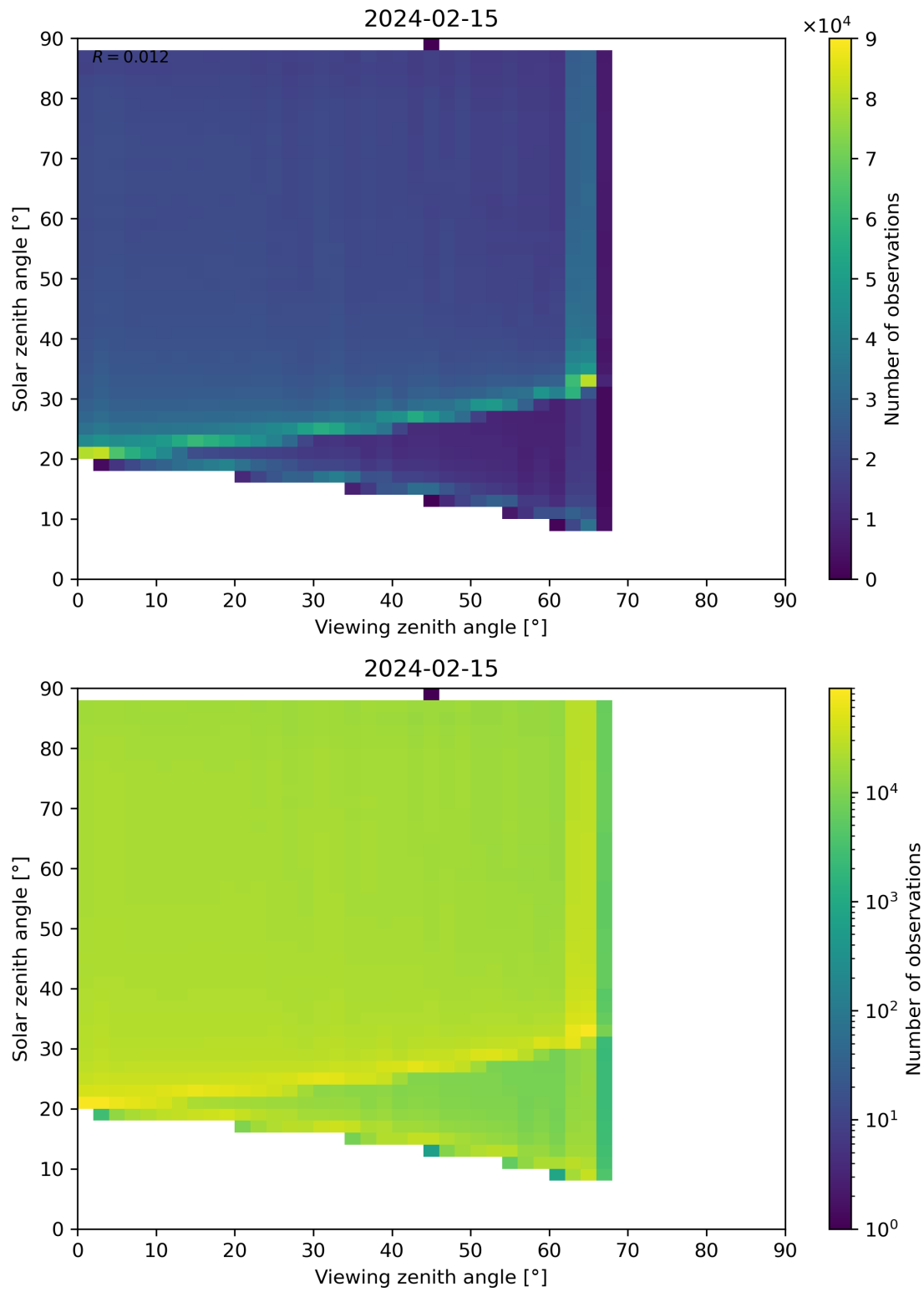
Figure 127: Scatter density plot of “Viewing zenith angle” against “Solar zenith angle” for 2024-02-14 to 2024-02-16.
