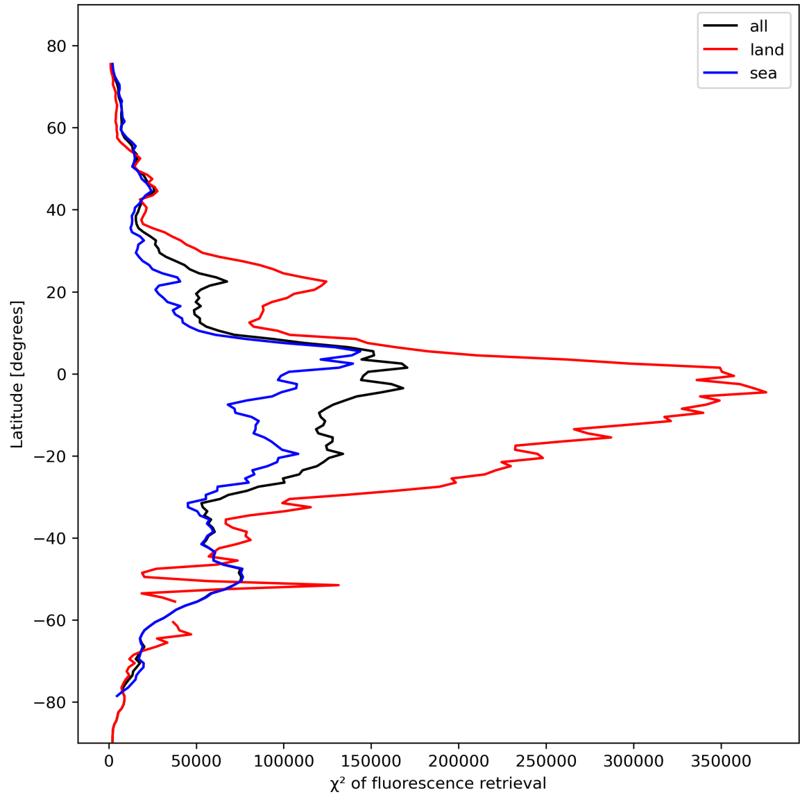
Figure 25: Zonal average of “ \chi^2 of fluorescence retrieval” for 2024-02-14 to 2024-02-16.
