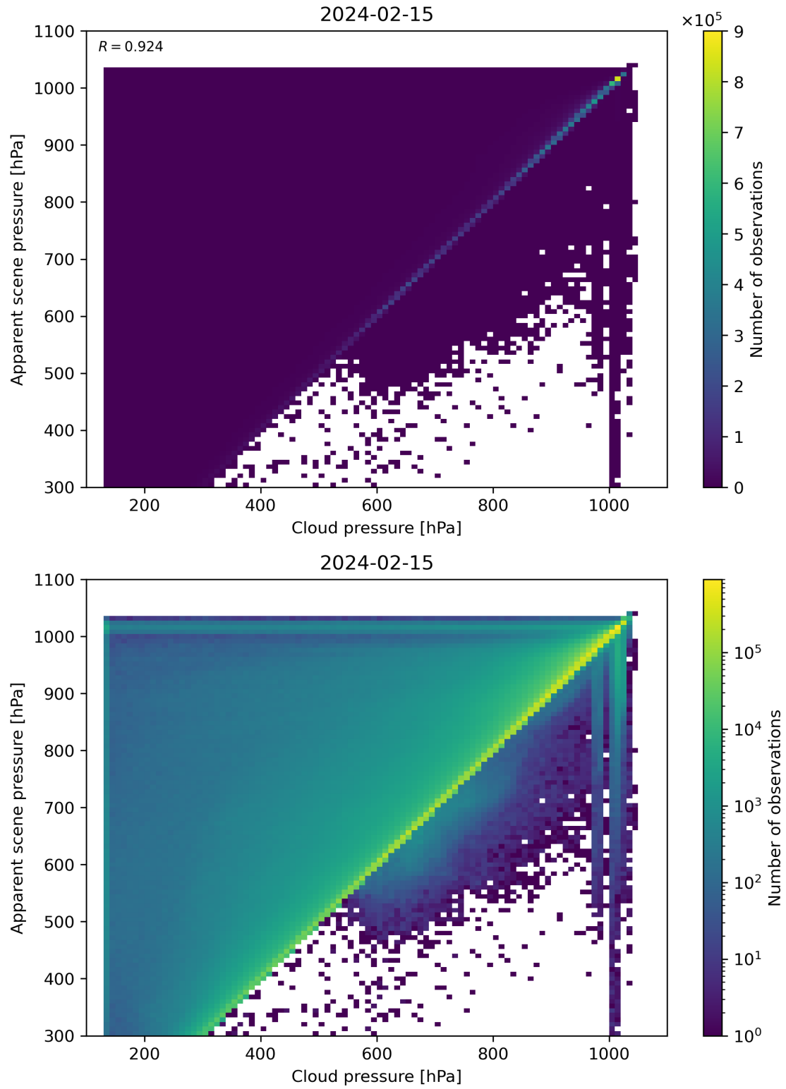
Figure 77: Scatter density plot of “Cloud pressure” against “Apparent scene pressure” for 2024-02-14 to 2024-02-16.
