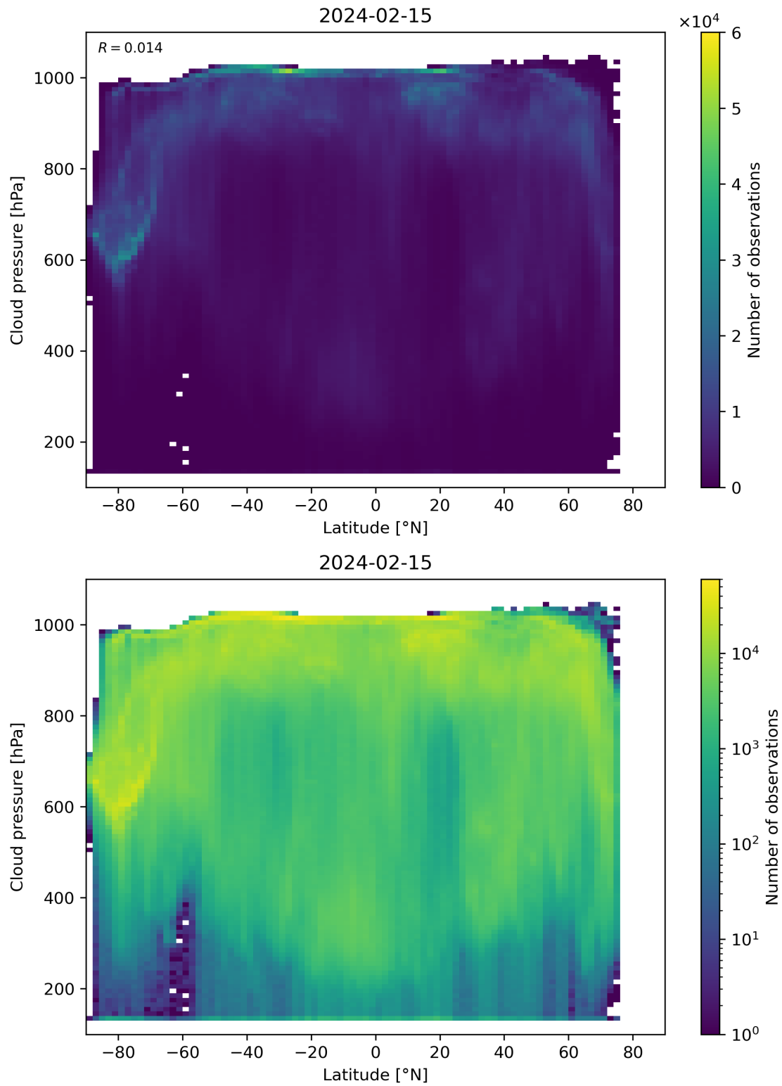
Figure 91: Scatter density plot of “Latitude” against “Cloud pressure” for 2024-02-14 to 2024-02-16.
