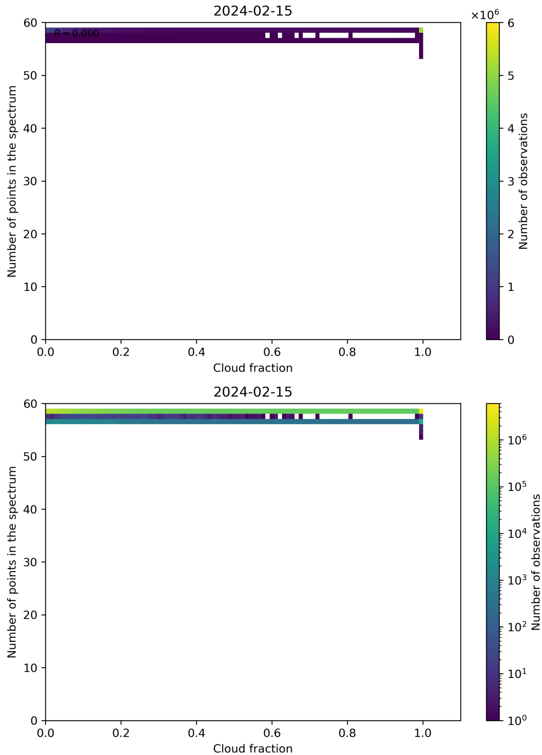
Figure 74: Scatter density plot of “Cloud fraction” against “Number of points in the spectrum” for 2024-02-14 to 2024-02-16.
