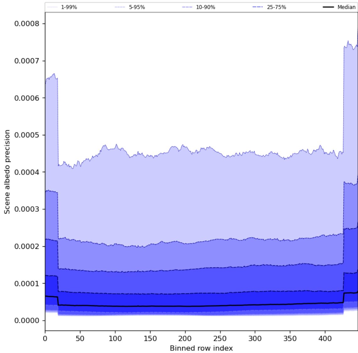
Figure 52: Along track statistics of “Scene albedo precision” for 2024-02-14 to 2024-02-16
