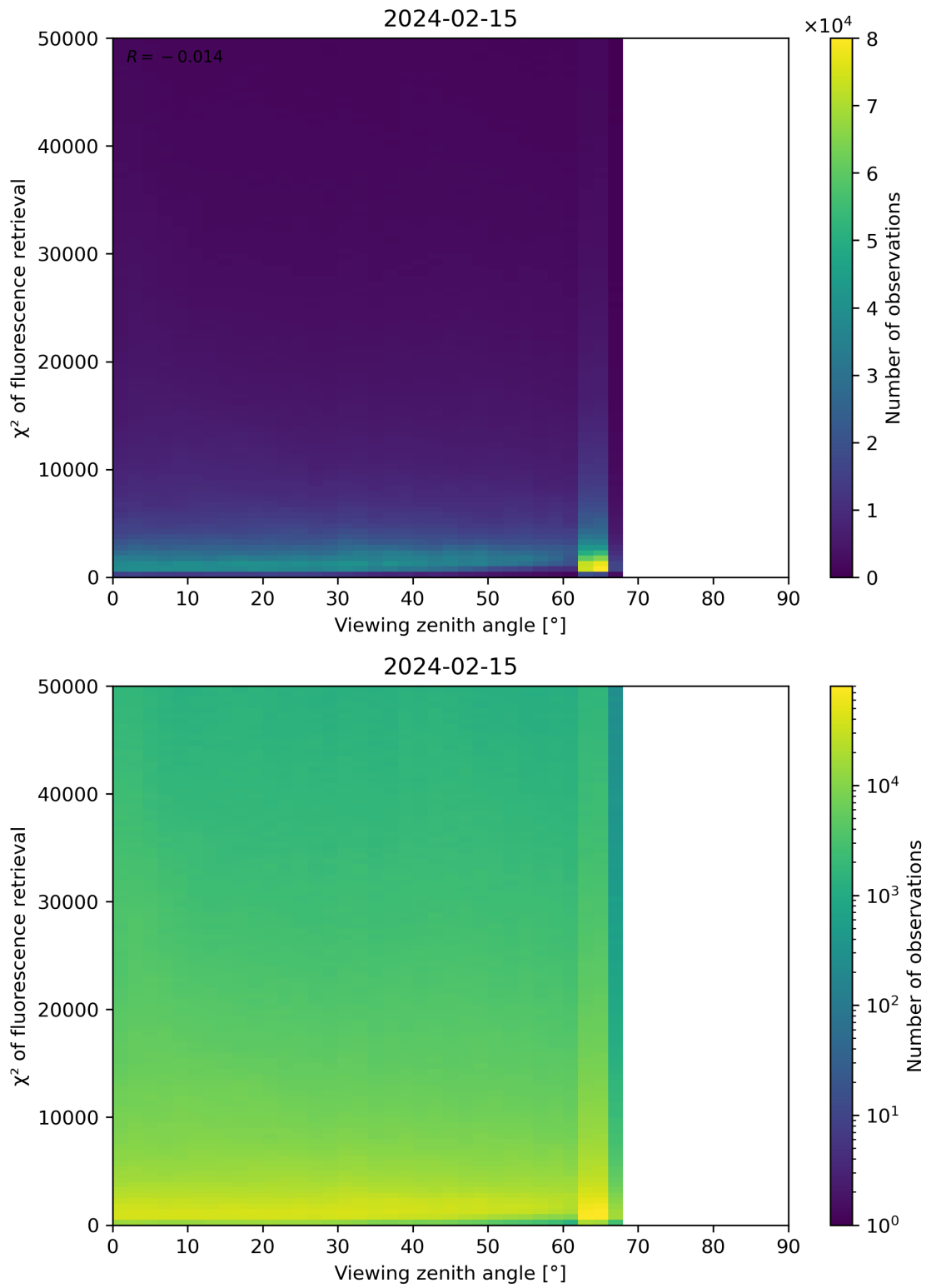
Figure 119: Scatter density plot of “Viewing zenith angle” against “ \chi^2 of fluorescence retrieval” for 2024-02-14 to 2024-02-16.
