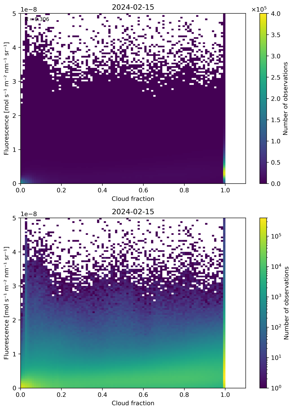
Figure 72: Scatter density plot of “Cloud fraction” against “Fluorescence” for 2024-02-14 to 2024-02-16.
