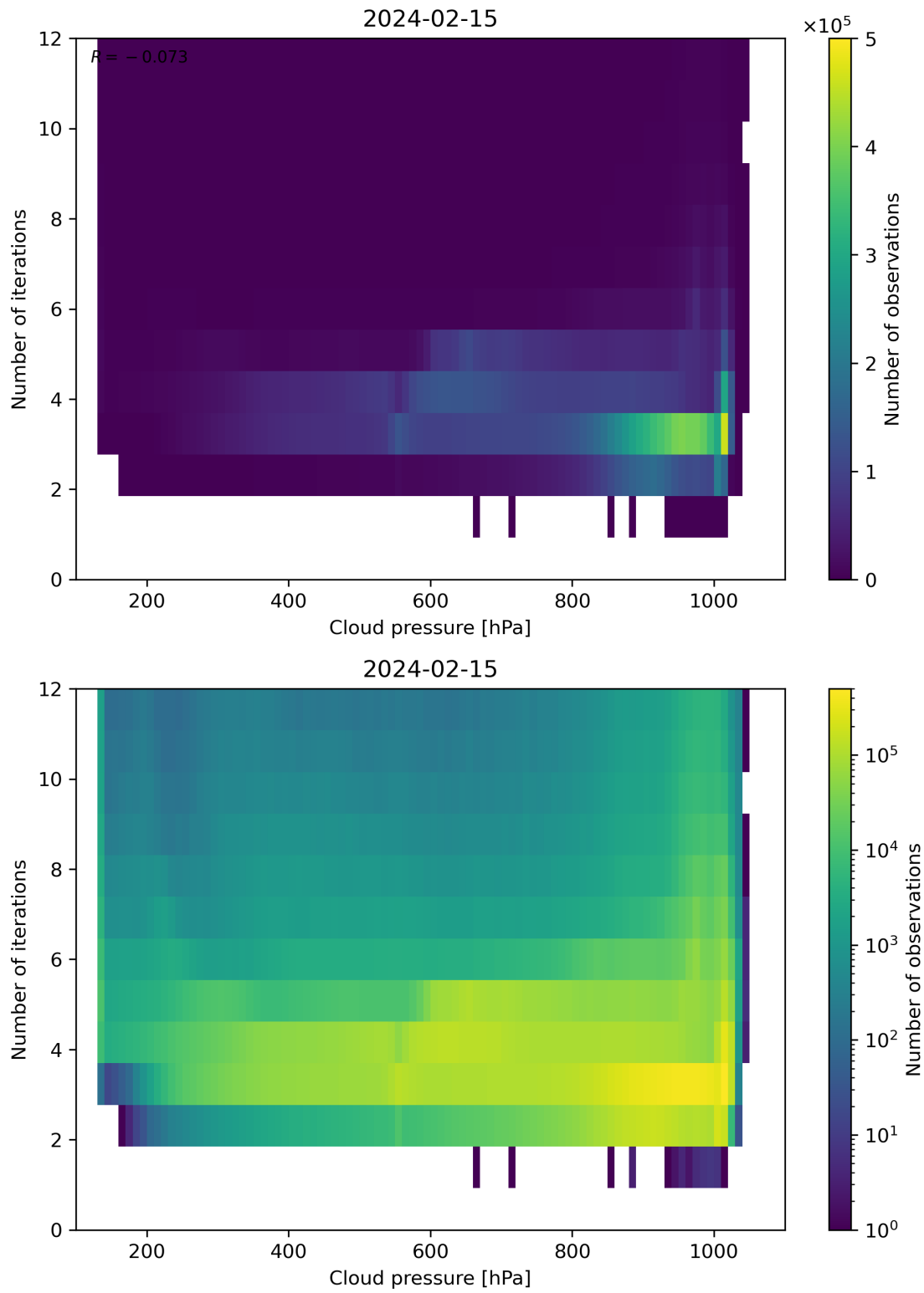
Figure 81: Scatter density plot of “Cloud pressure” against “Number of iterations” for 2024-02-14 to 2024-02-16.
