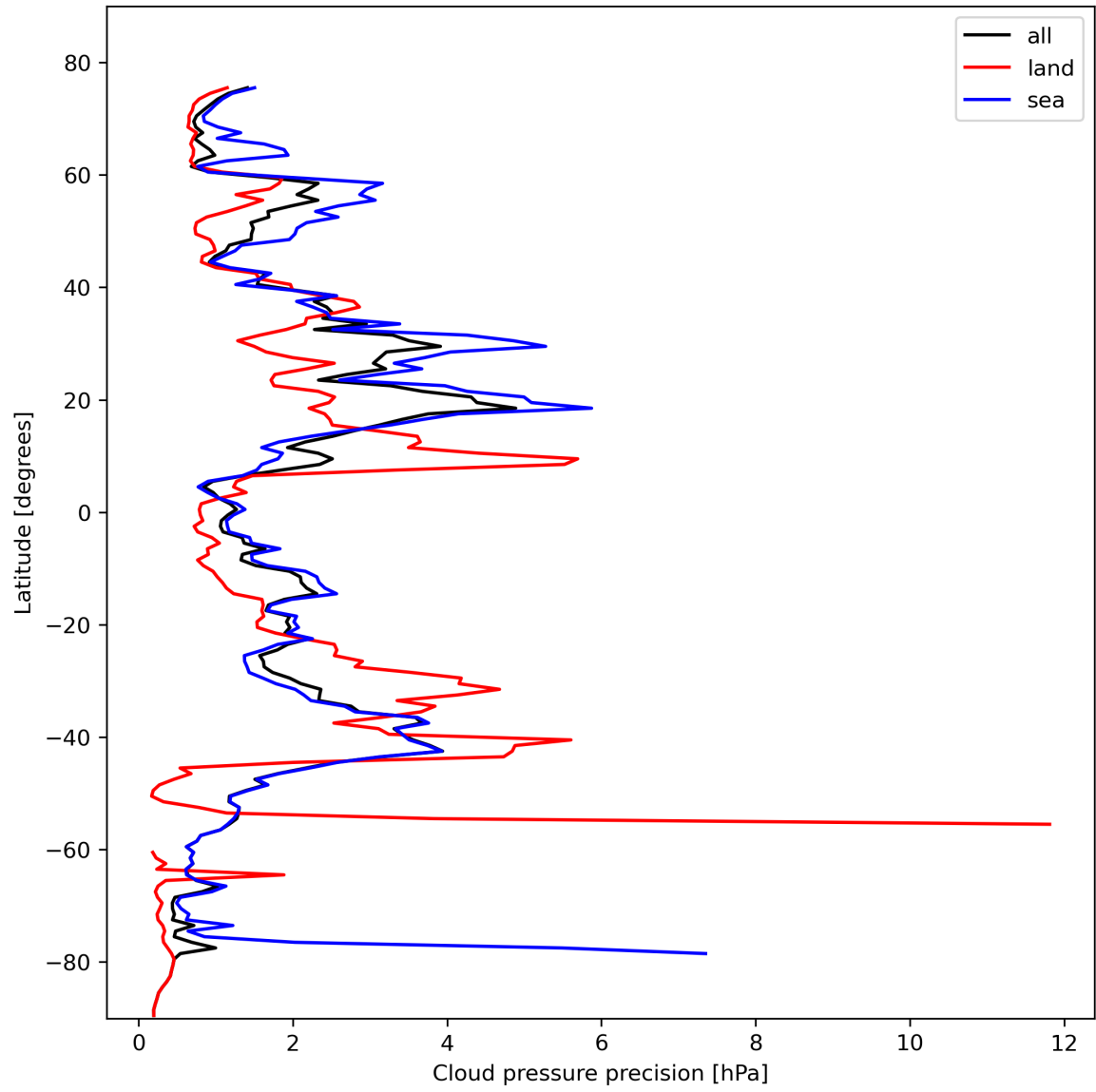
Figure 14: Zonal average of “Cloud pressure precision” for 2024-02-14 to 2024-02-16.
