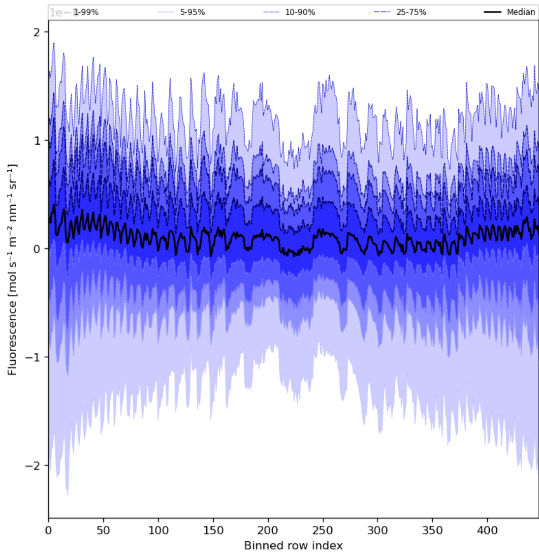
Figure 57: Along track statistics of “Fluorescence” for 2024-02-14 to 2024-02-16
