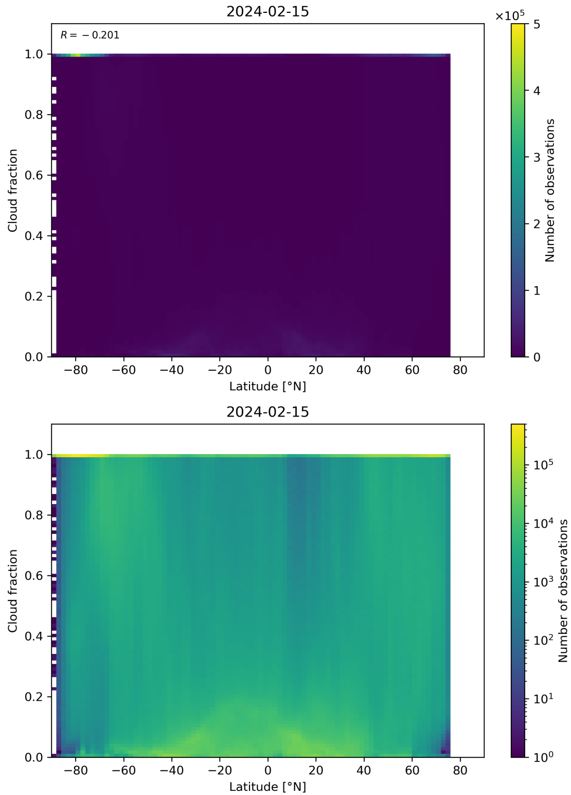
Figure 90: Scatter density plot of “Latitude” against “Cloud fraction” for 2024-02-14 to 2024-02-16.
