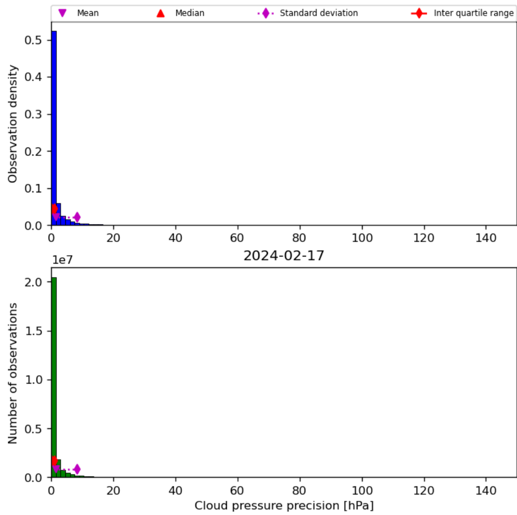
Figure 31: Histogram of “Cloud pressure precision” for 2024-02-17 to 2024-02-18
