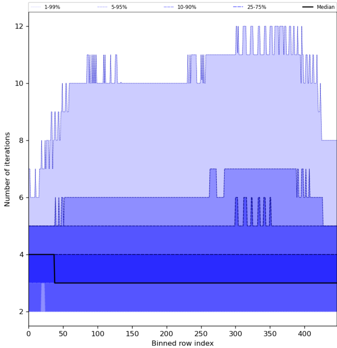
Figure 56: Along track statistics of “Number of iterations” for 2024-02-17 to 2024-02-18
