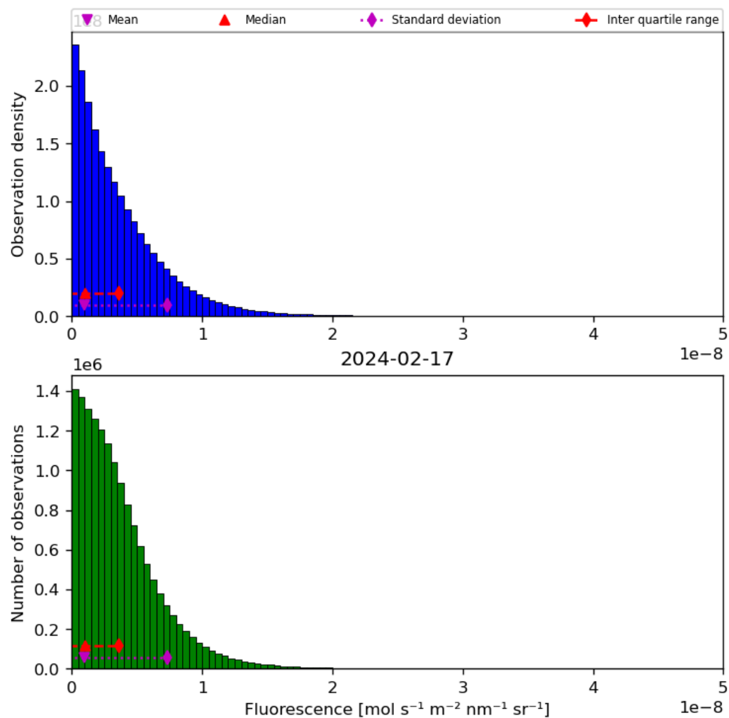
Figure 40: Histogram of “Fluorescence” for 2024-02-17 to 2024-02-18
