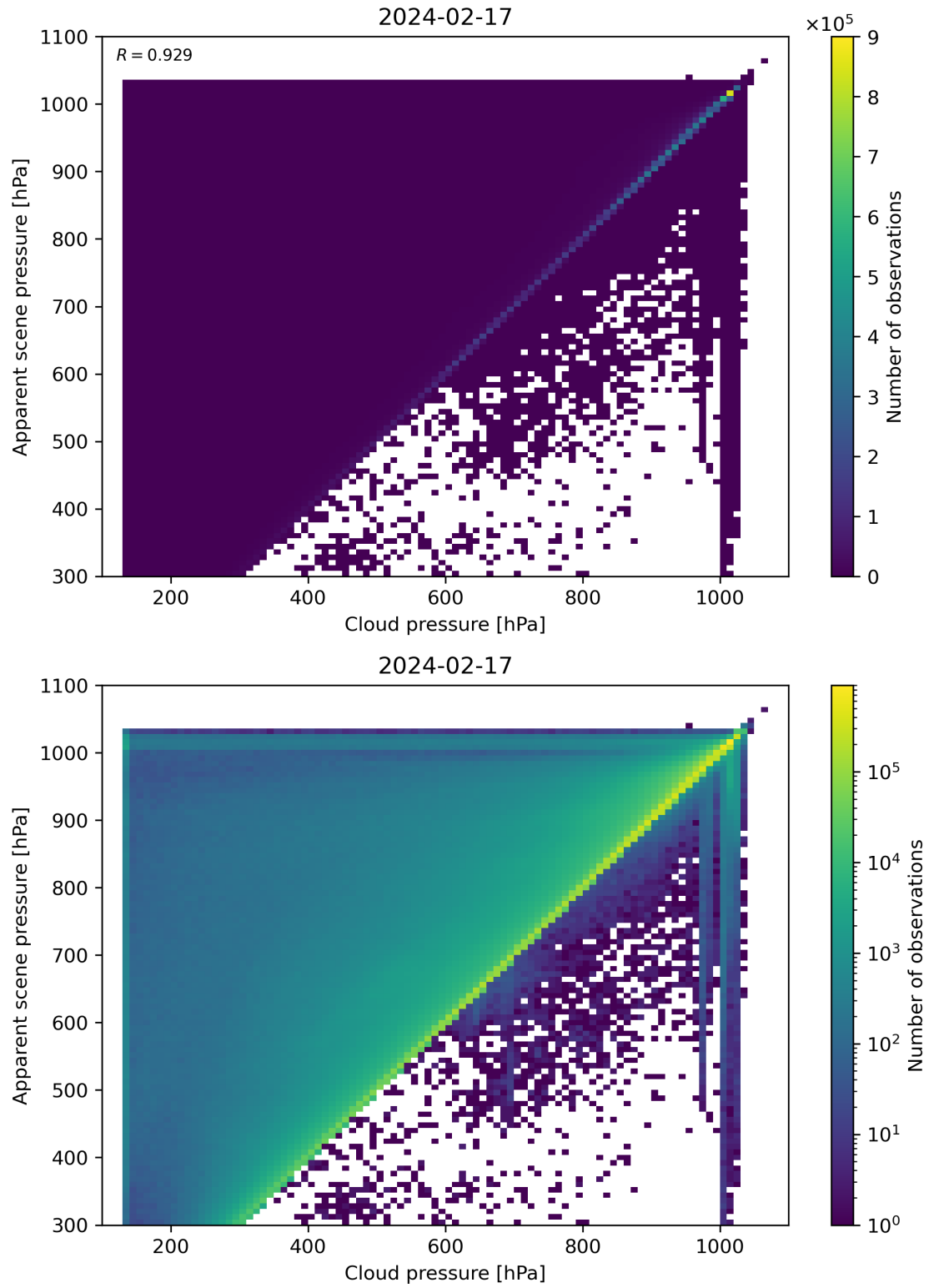
Figure 77: Scatter density plot of “Cloud pressure” against “Apparent scene pressure” for 2024-02-17 to 2024-02-18.
