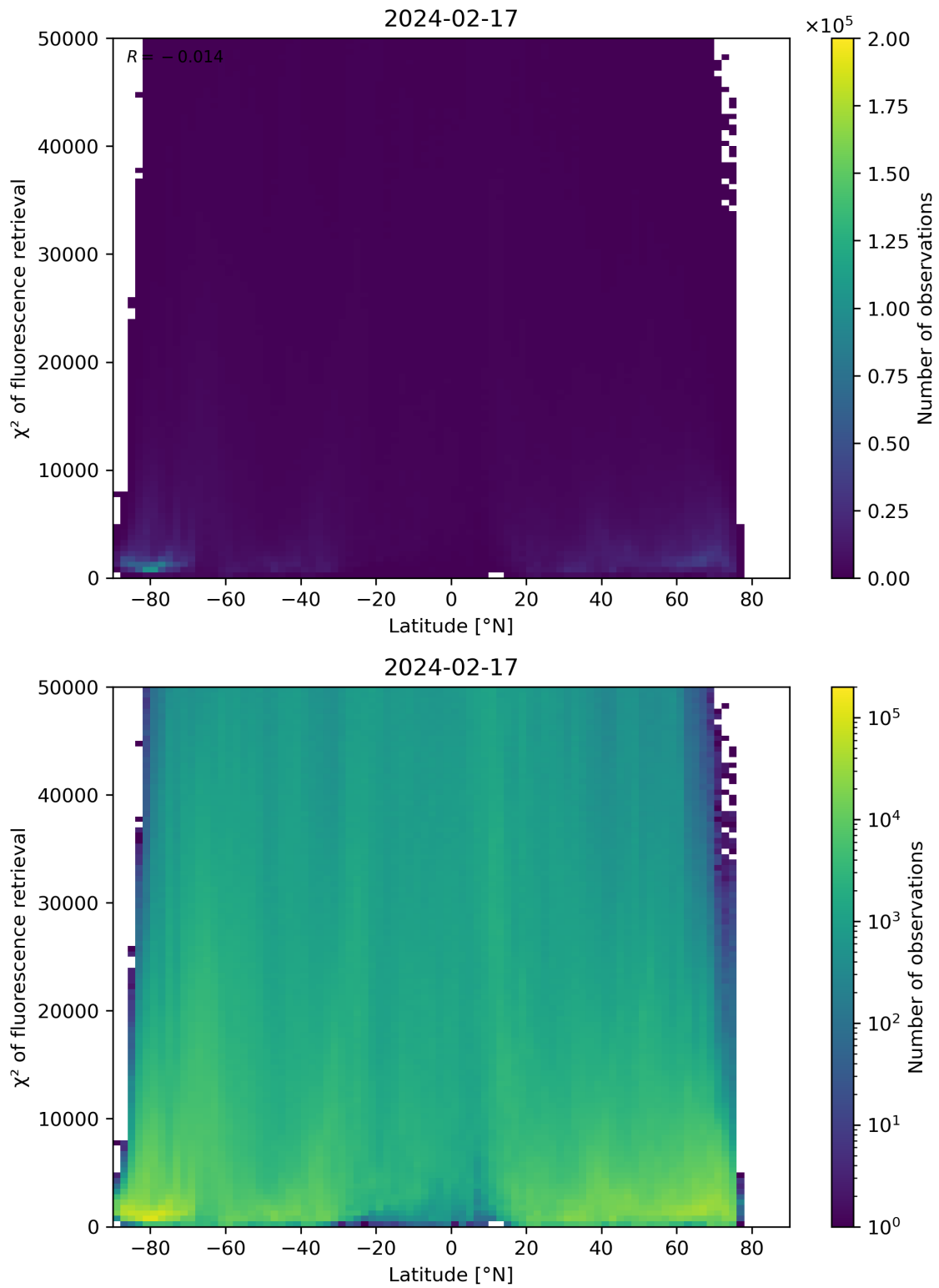
Figure 89: Scatter density plot of “Latitude” against “ \chi^2 of fluorescence retrieval” for 2024-02-17 to 2024-02-18.
