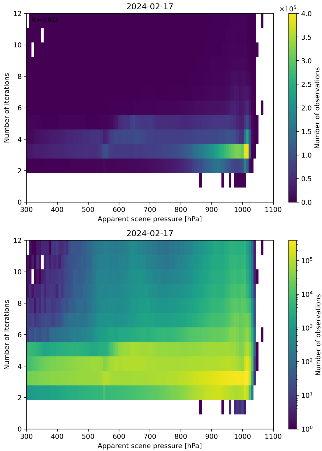
Figure 65: Scatter density plot of “Apparent scene pressure” against “Number of iterations” for 2024-02-17 to 2024-02-18.
