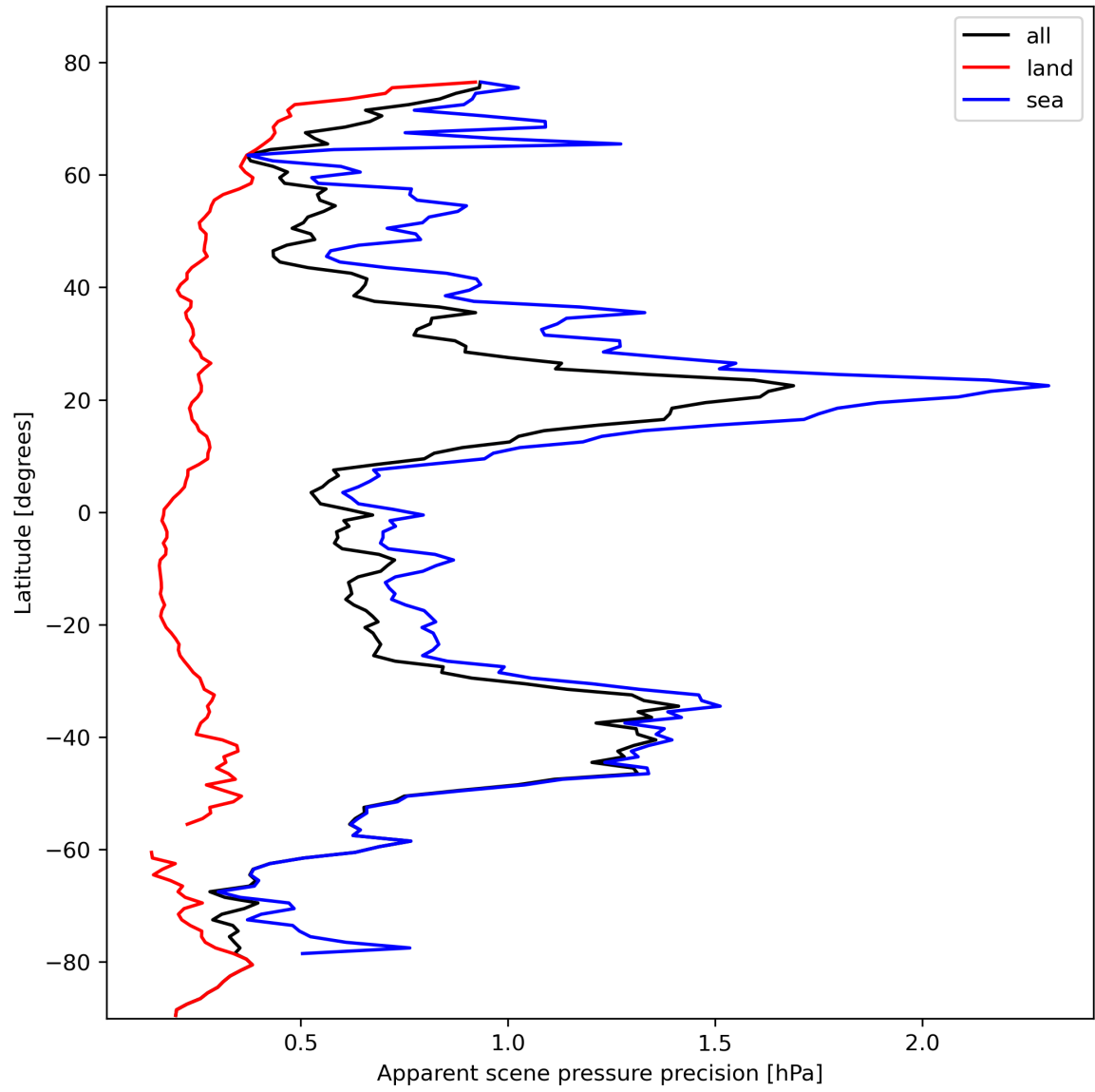
Figure 20: Zonal average of “Apparent scene pressure precision” for 2024-02-17 to 2024-02-18.
