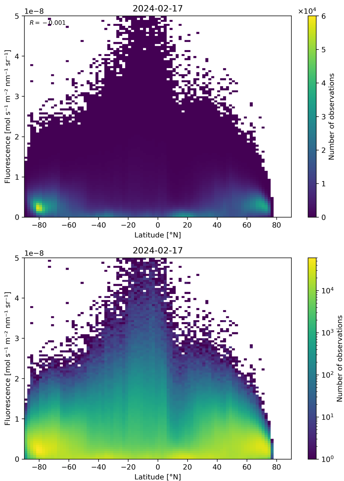
Figure 92: Scatter density plot of “Latitude” against “Fluorescence” for 2024-02-17 to 2024-02-18.
