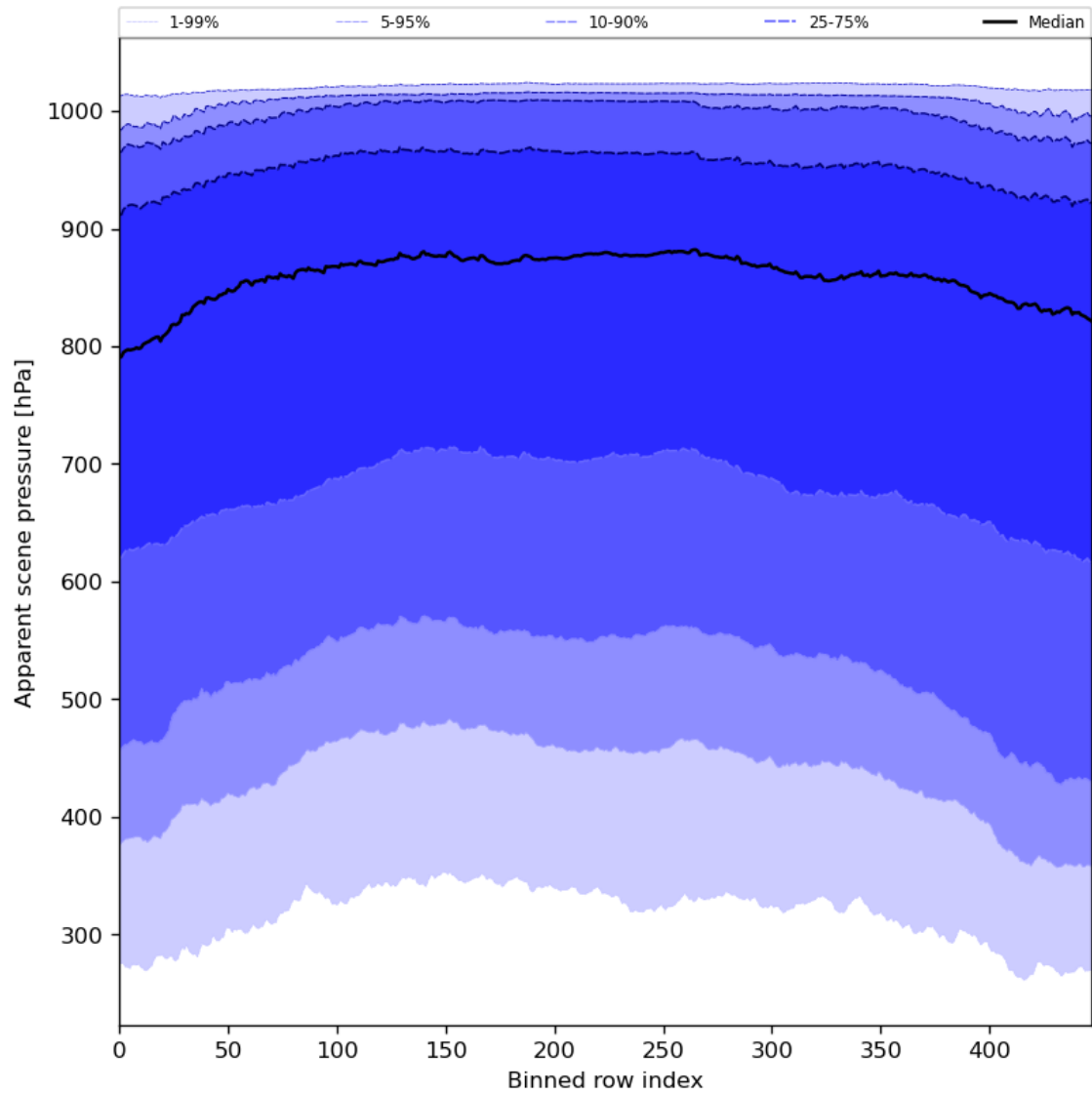
Figure 53: Along track statistics of “Apparent scene pressure” for 2024-02-17 to 2024-02-18
