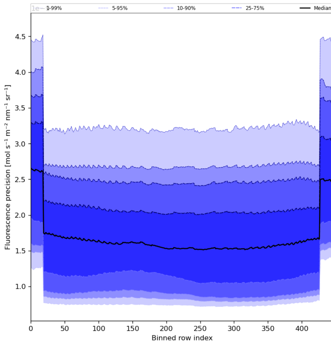
Figure 58: Along track statistics of “Fluorescence precision” for 2024-02-17 to 2024-02-18
