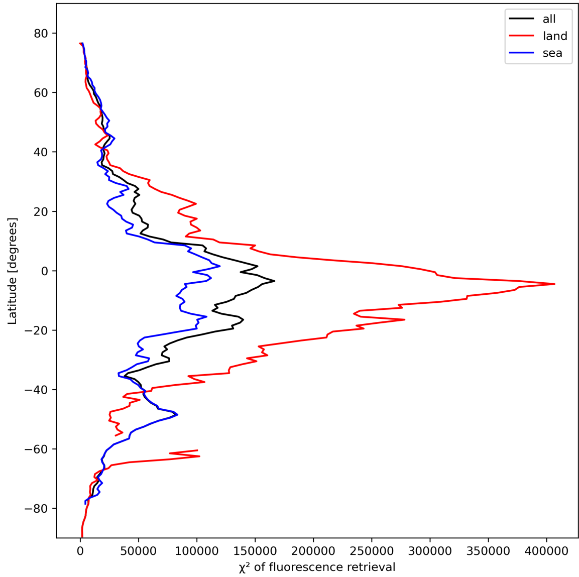
Figure 25: Zonal average of “ \chi^2 of fluorescence retrieval” for 2024-02-17 to 2024-02-18.
