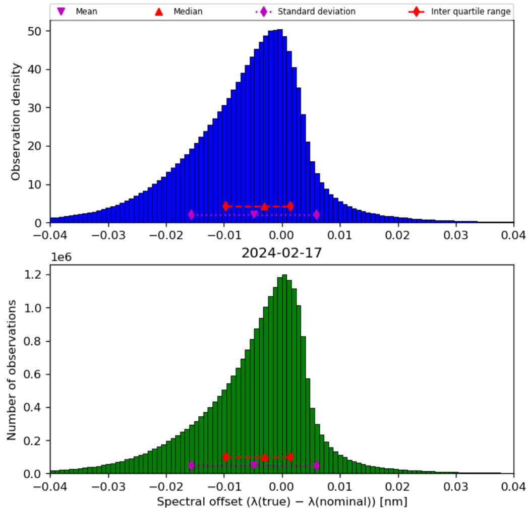
Figure 45: Histogram of “Spectral offset ( \lambda(\text{true}) - \lambda(\text{nominal}) )” for 2024-02-17 to 2024-02-18
