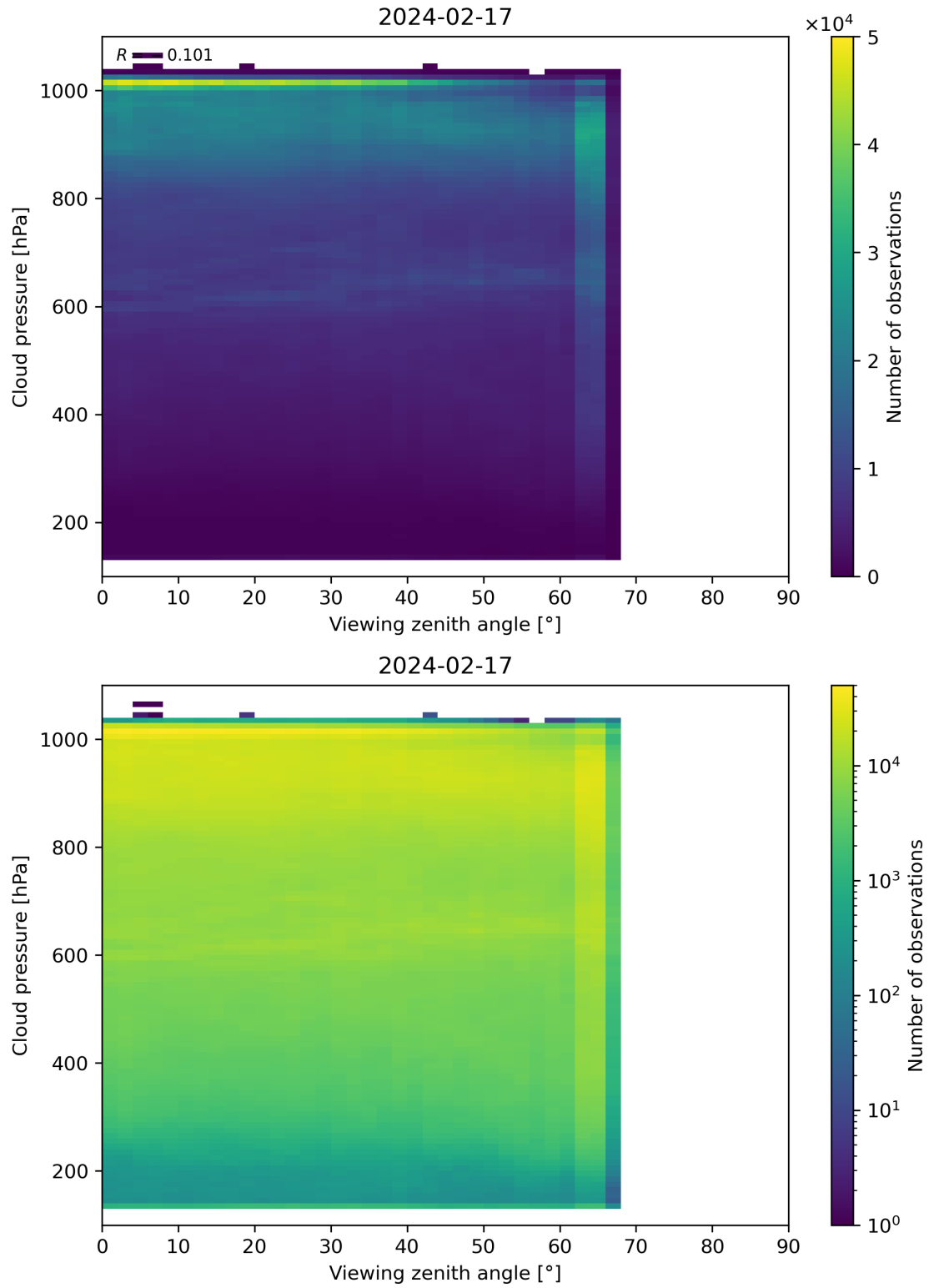
Figure 121: Scatter density plot of “Viewing zenith angle” against “Cloud pressure” for 2024-02-17 to 2024-02-18.
