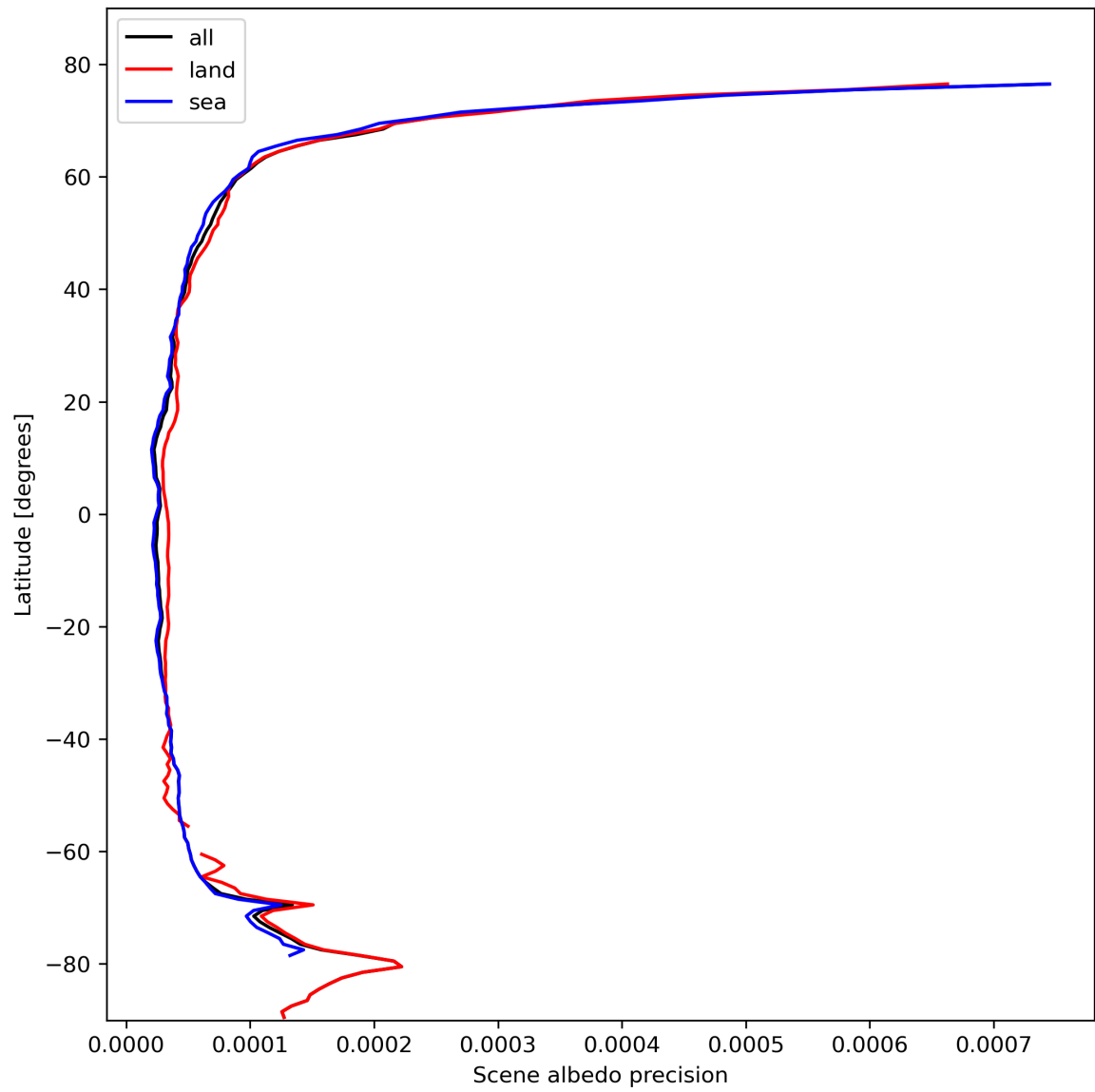
Figure 18: Zonal average of “Scene albedo precision” for 2024-02-17 to 2024-02-18.
