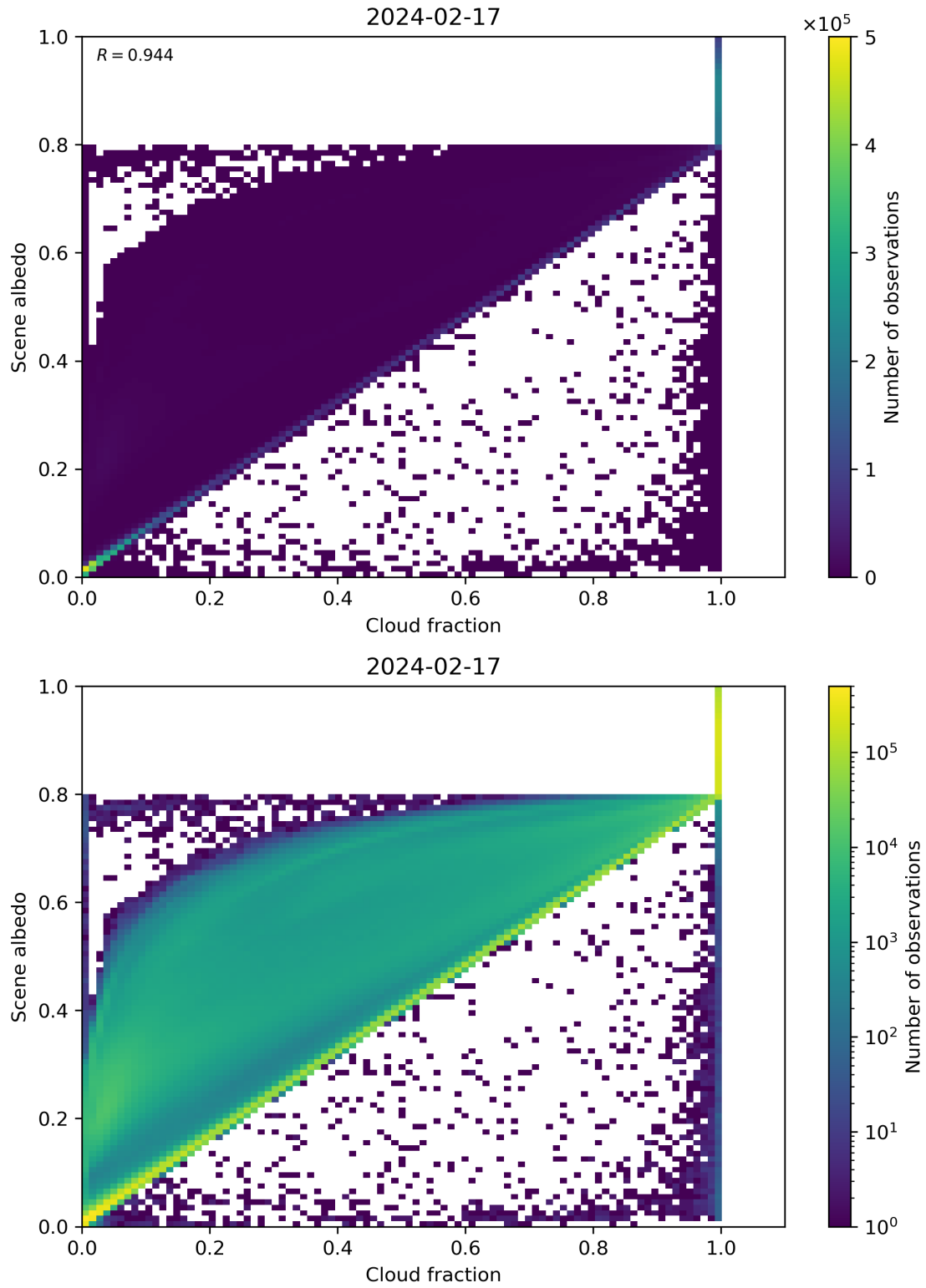
Figure 75: Scatter density plot of “Cloud fraction” against “Scene albedo” for 2024-02-17 to 2024-02-18.
