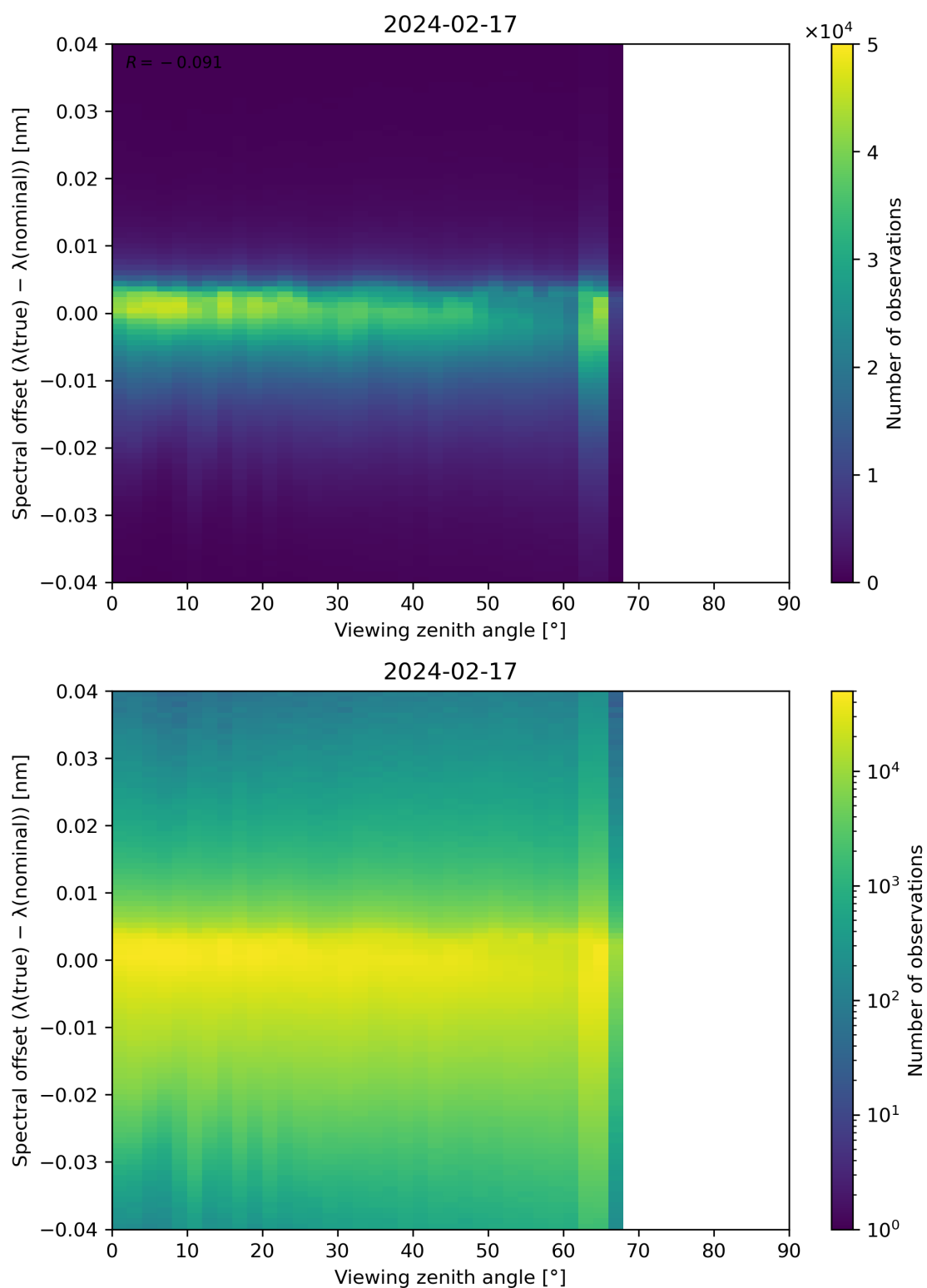
Figure 128: Scatter density plot of “Viewing zenith angle” against “Spectral offset ( \lambda(\text{true}) - \lambda(\text{nominal}) )” for 2024-02-17 to 2024-02-18.
