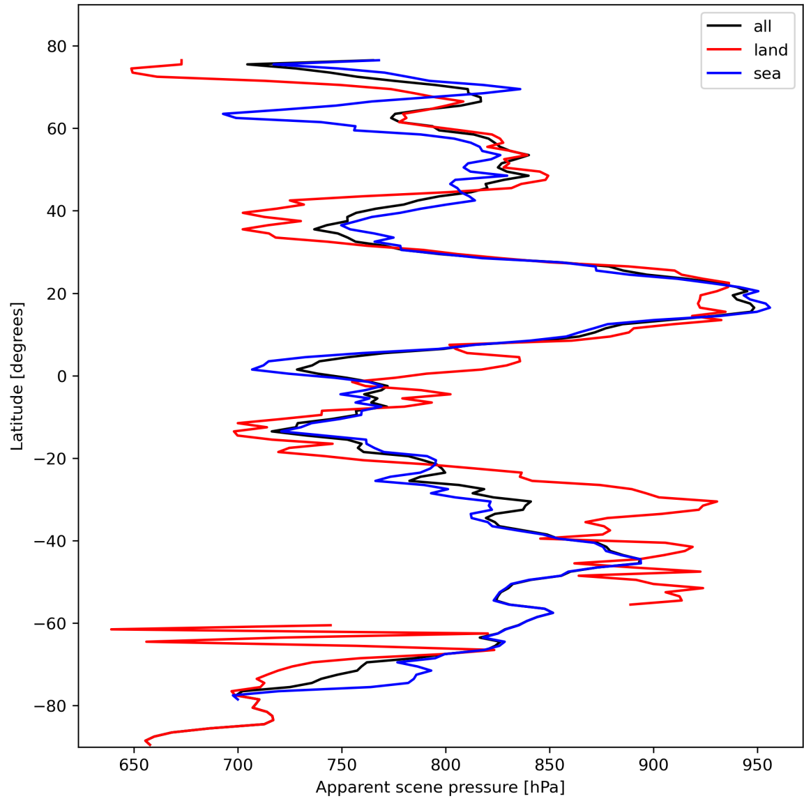
Figure 19: Zonal average of “Apparent scene pressure” for 2024-02-17 to 2024-02-18.
