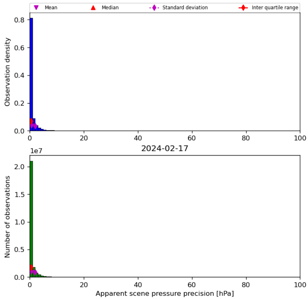
Figure 37: Histogram of “Apparent scene pressure precision” for 2024-02-17 to 2024-02-18
