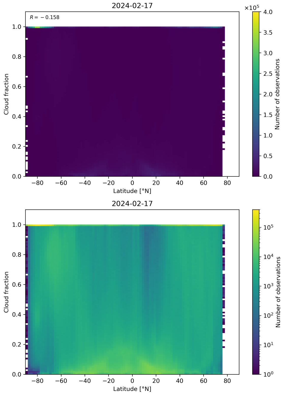
Figure 90: Scatter density plot of “Latitude” against “Cloud fraction” for 2024-02-17 to 2024-02-18.
