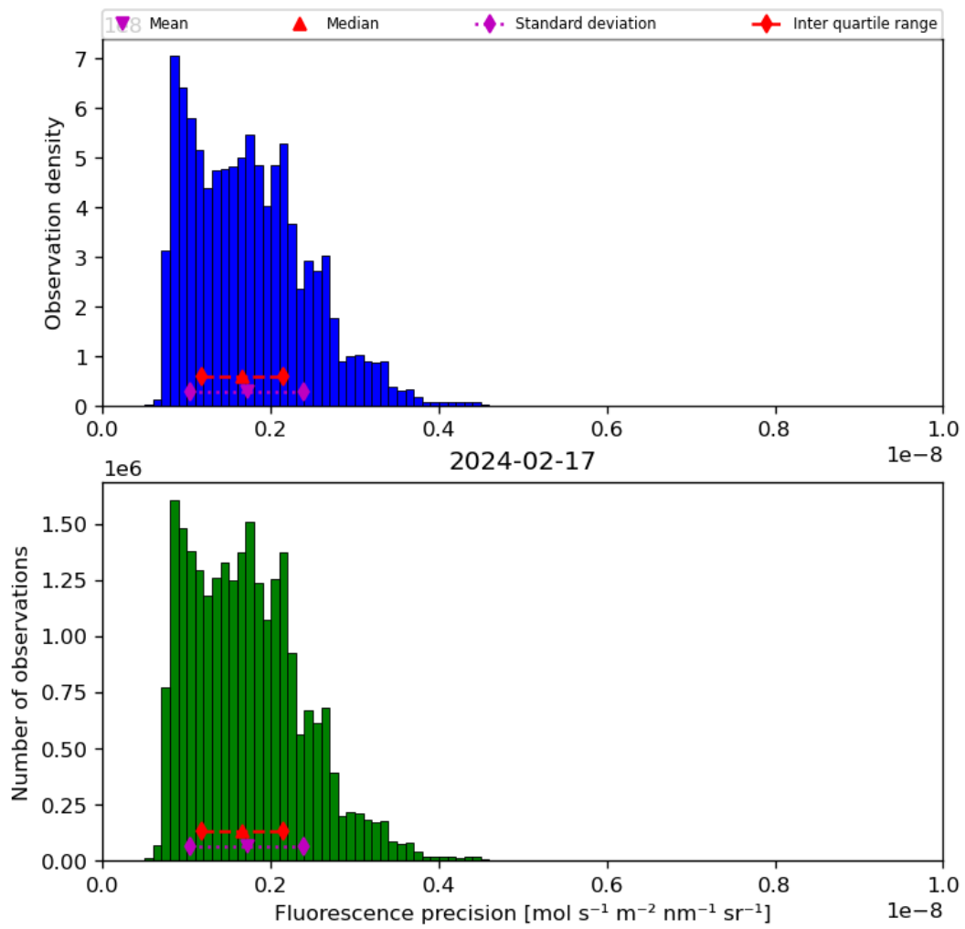
Figure 41: Histogram of “Fluorescence precision” for 2024-02-17 to 2024-02-18
