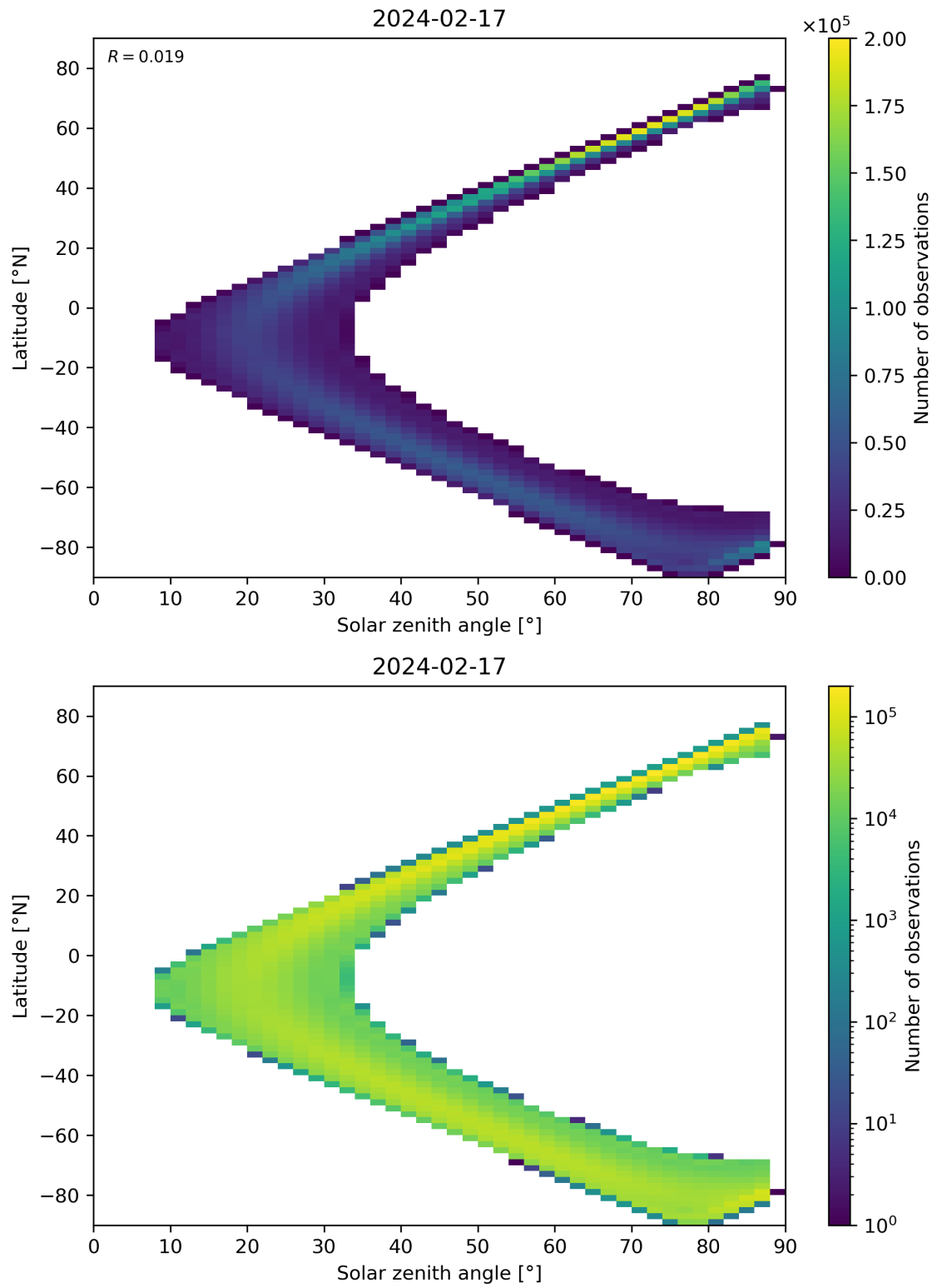
Figure 113: Scatter density plot of “Solar zenith angle” against “Latitude” for 2024-02-17 to 2024-02-18.
