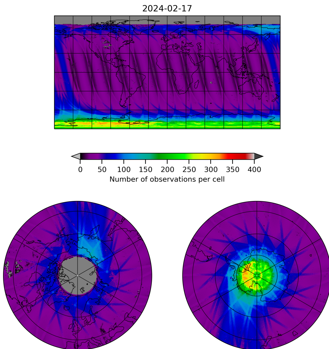
Figure 11: Map of the number of observations for 2024-02-17 to 2024-02-18
