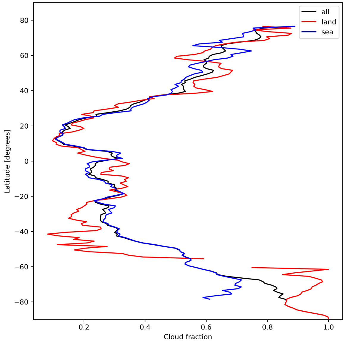
Figure 15: Zonal average of “Cloud fraction” for 2024-02-17 to 2024-02-18.
