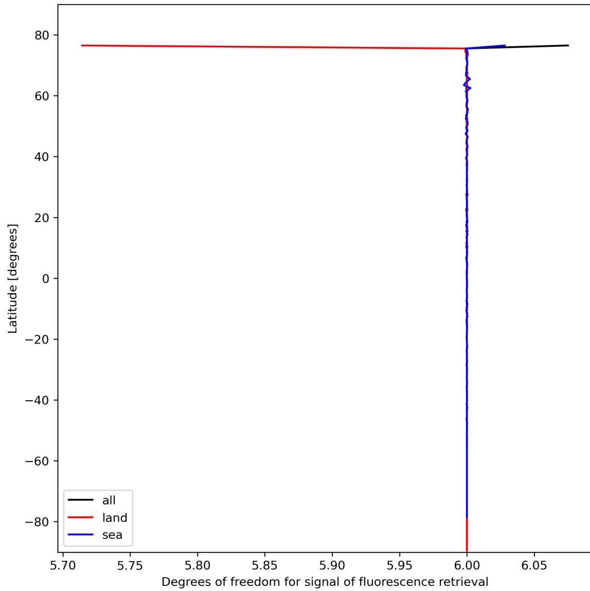
Figure 26: Zonal average of “Degrees of freedom for signal of fluorescence retrieval” for 2024-02-17 to 2024-02-18.
