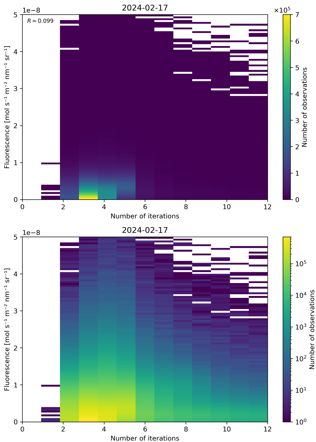
Figure 98: Scatter density plot of “Number of iterations” against “Fluorescence” for 2024-02-17 to 2024-02-18.
