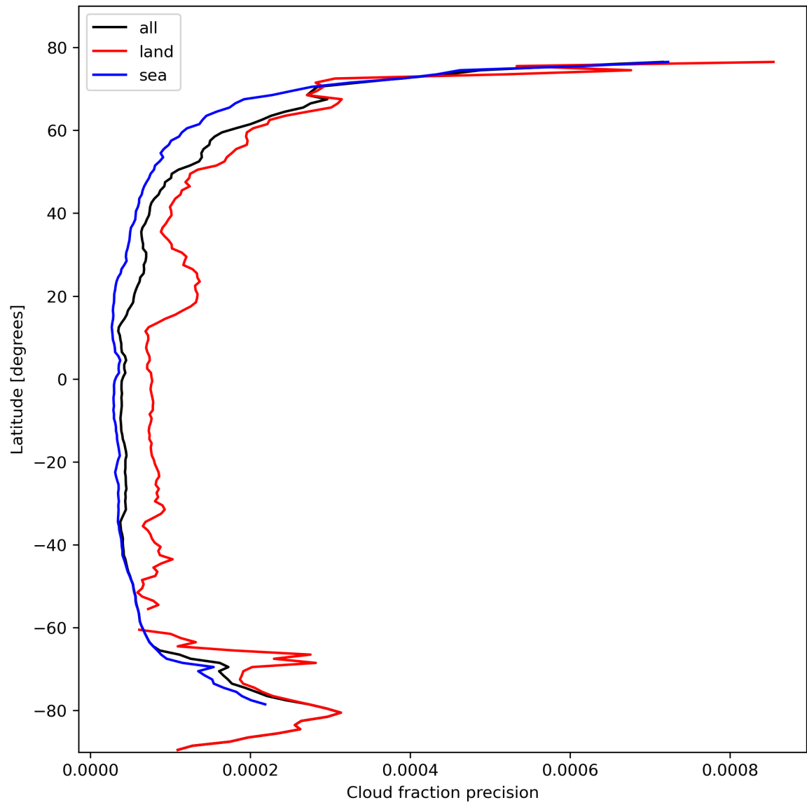
Figure 16: Zonal average of “Cloud fraction precision” for 2024-02-17 to 2024-02-18.
