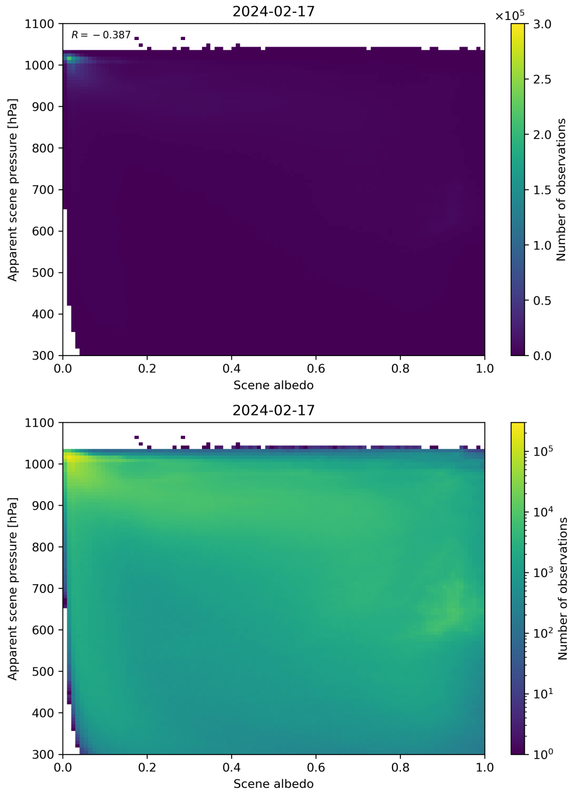
Figure 102: Scatter density plot of “Scene albedo” against “Apparent scene pressure” for 2024-02-17 to 2024-02-18.
