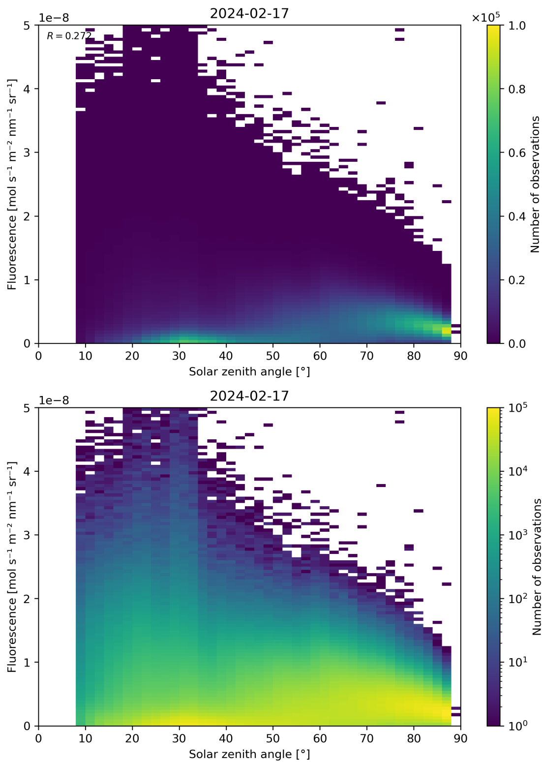
Figure 112: Scatter density plot of “Solar zenith angle” against “Fluorescence” for 2024-02-17 to 2024-02-18.
