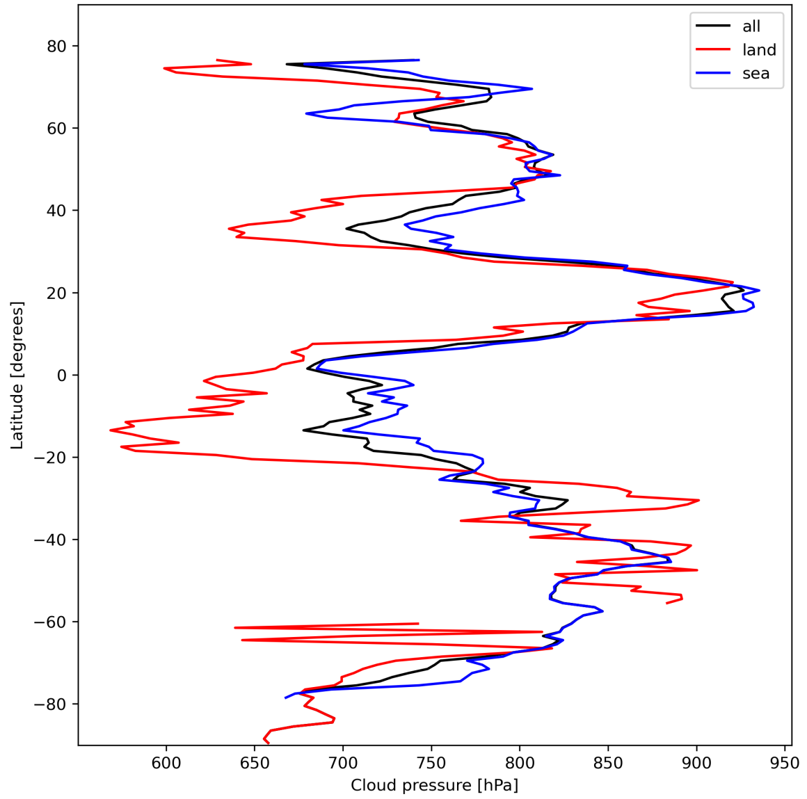
Figure 13: Zonal average of “Cloud pressure” for 2024-02-17 to 2024-02-18.
