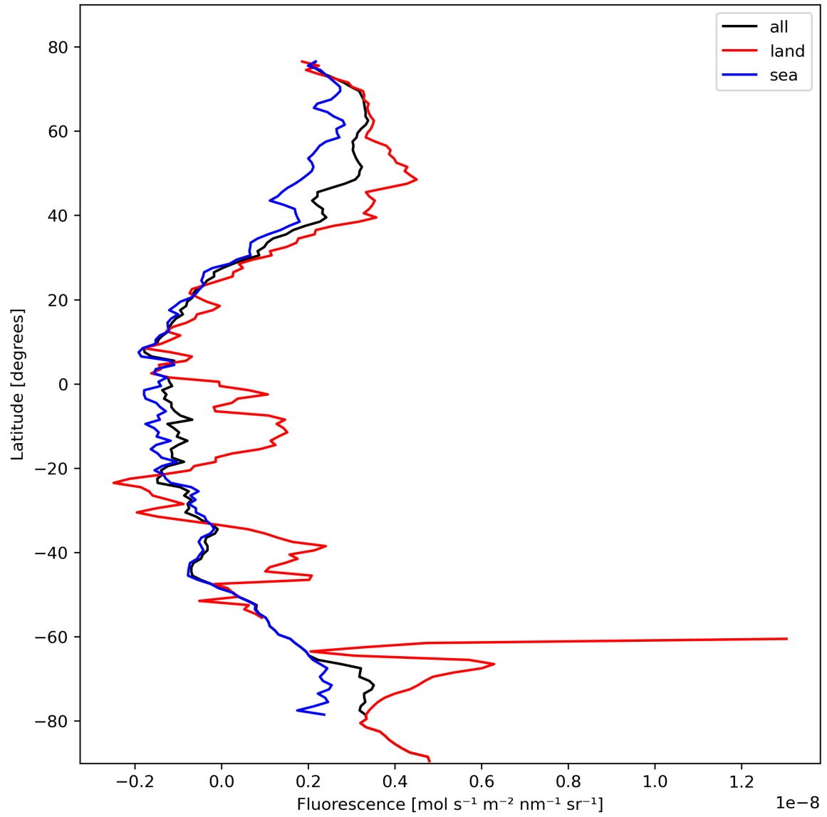
Figure 23: Zonal average of “Fluorescence” for 2024-02-17 to 2024-02-18.
