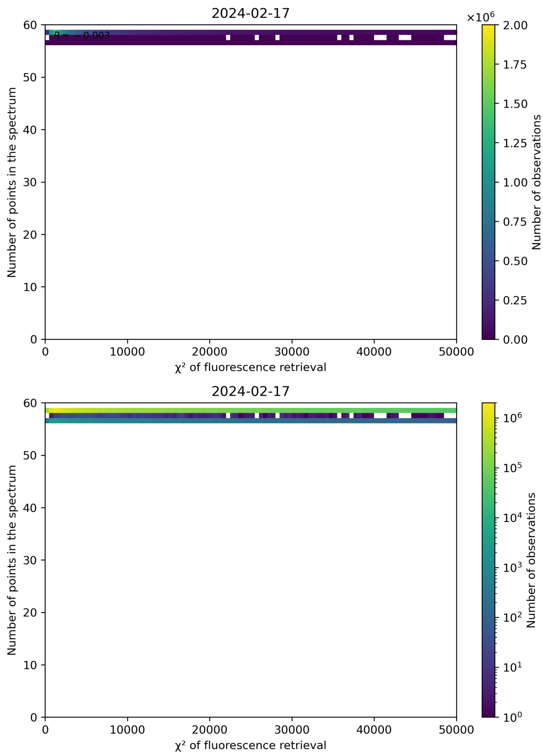
Figure 68: Scatter density plot of " \chi^2 of fluorescence retrieval" against "Number of points in the spectrum" for 2024-02-17 to 2024-02-18.
