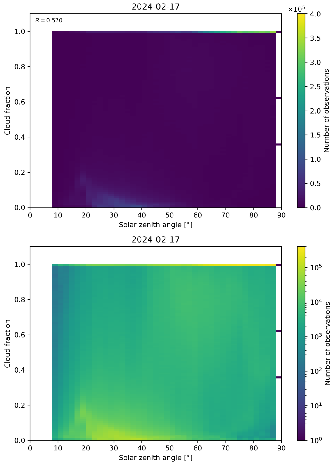
Figure 110: Scatter density plot of “Solar zenith angle” against “Cloud fraction” for 2024-02-17 to 2024-02-18.
