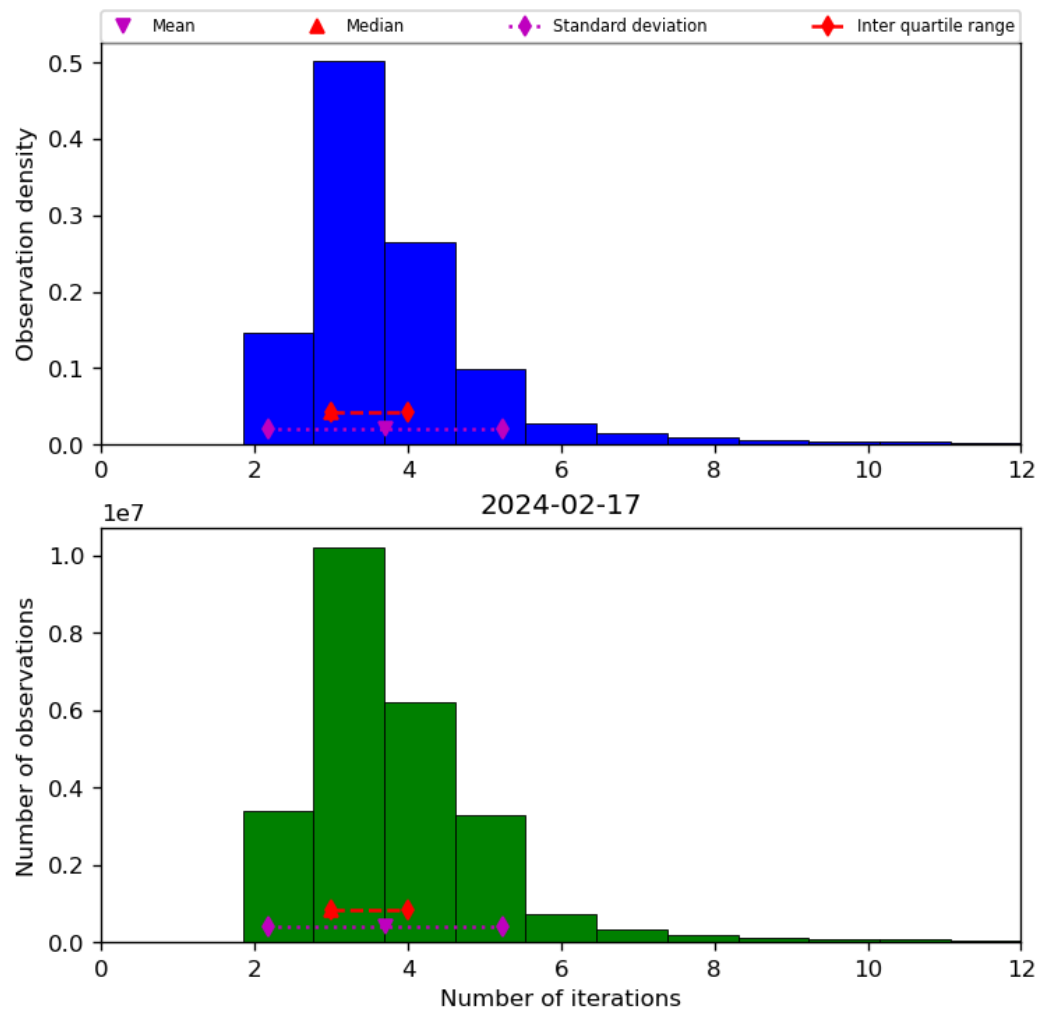
Figure 39: Histogram of “Number of iterations” for 2024-02-17 to 2024-02-18
