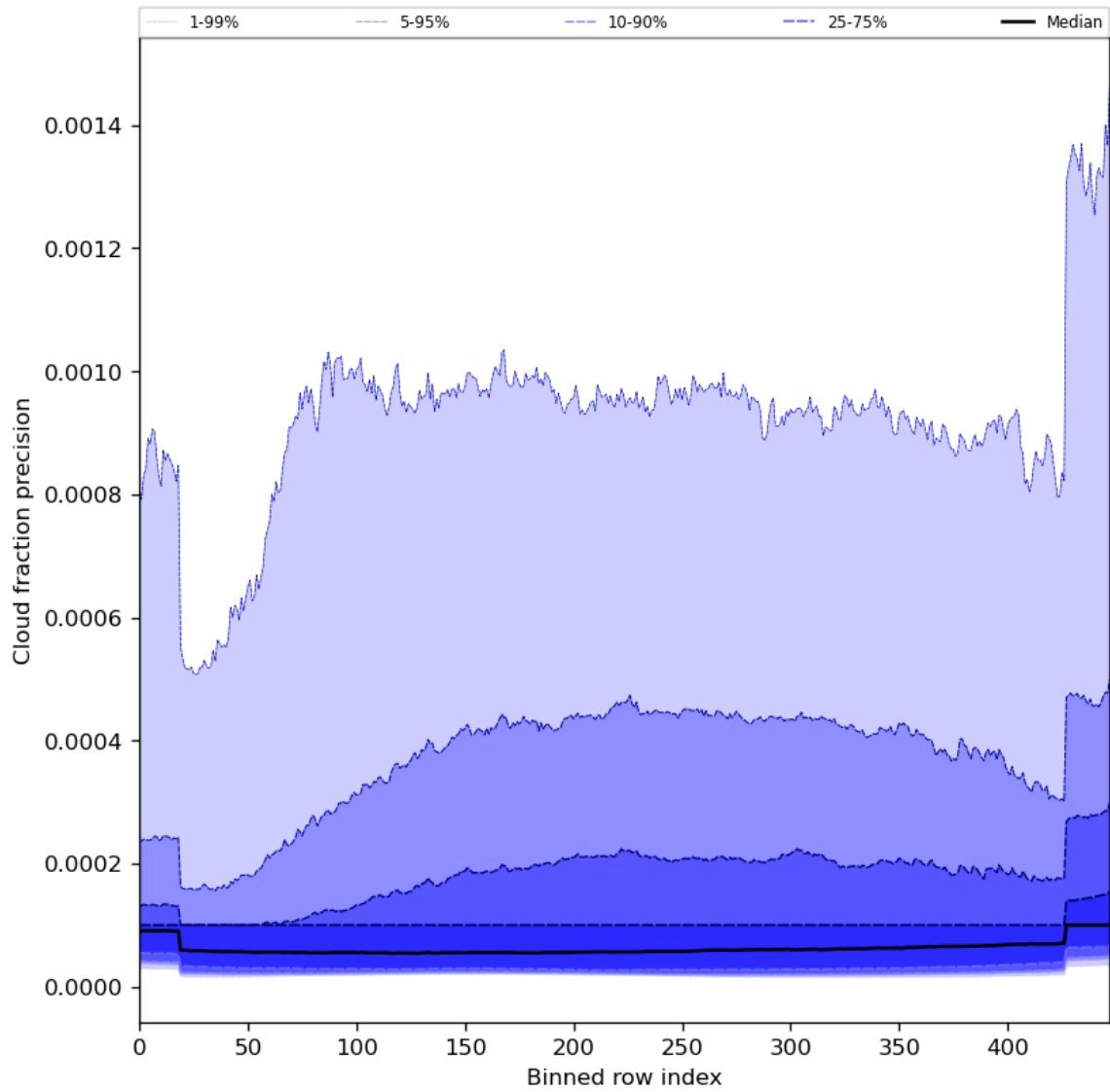
Figure 50: Along track statistics of “Cloud fraction precision” for 2024-02-17 to 2024-02-18
