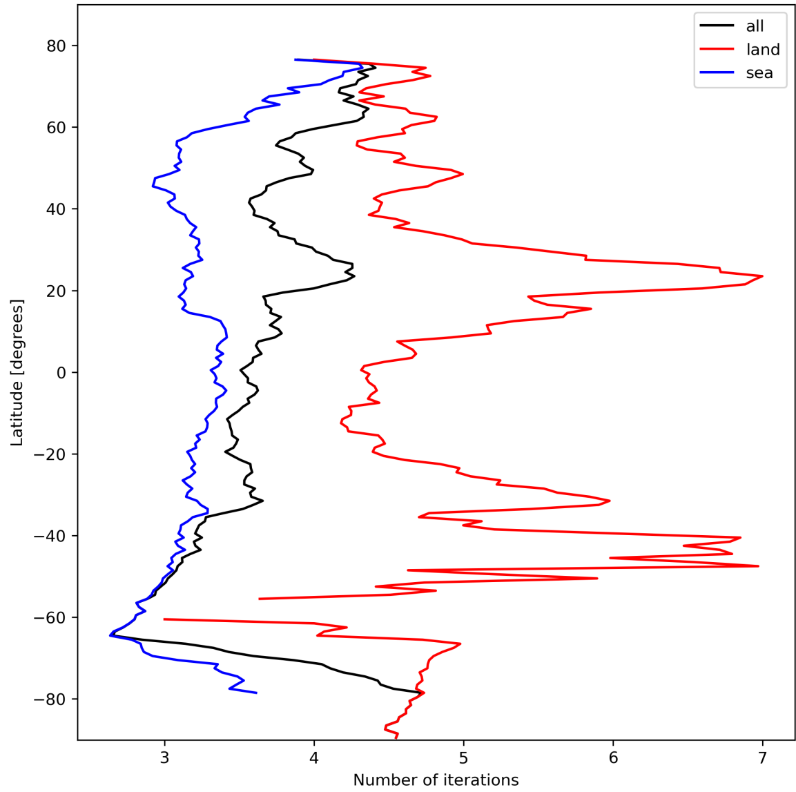
Figure 22: Zonal average of “Number of iterations” for 2024-02-17 to 2024-02-18.
