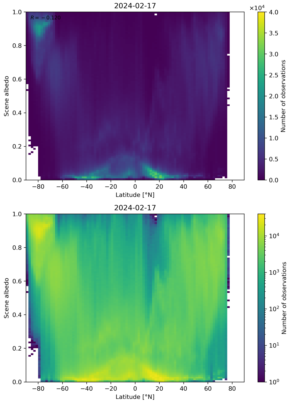
Figure 95: Scatter density plot of “Latitude” against “Scene albedo” for 2024-02-17 to 2024-02-18.
