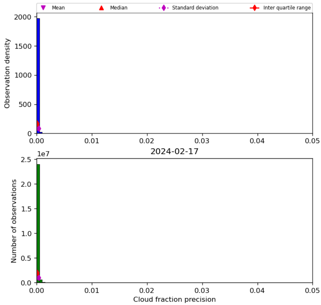
Figure 33: Histogram of “Cloud fraction precision” for 2024-02-17 to 2024-02-18
