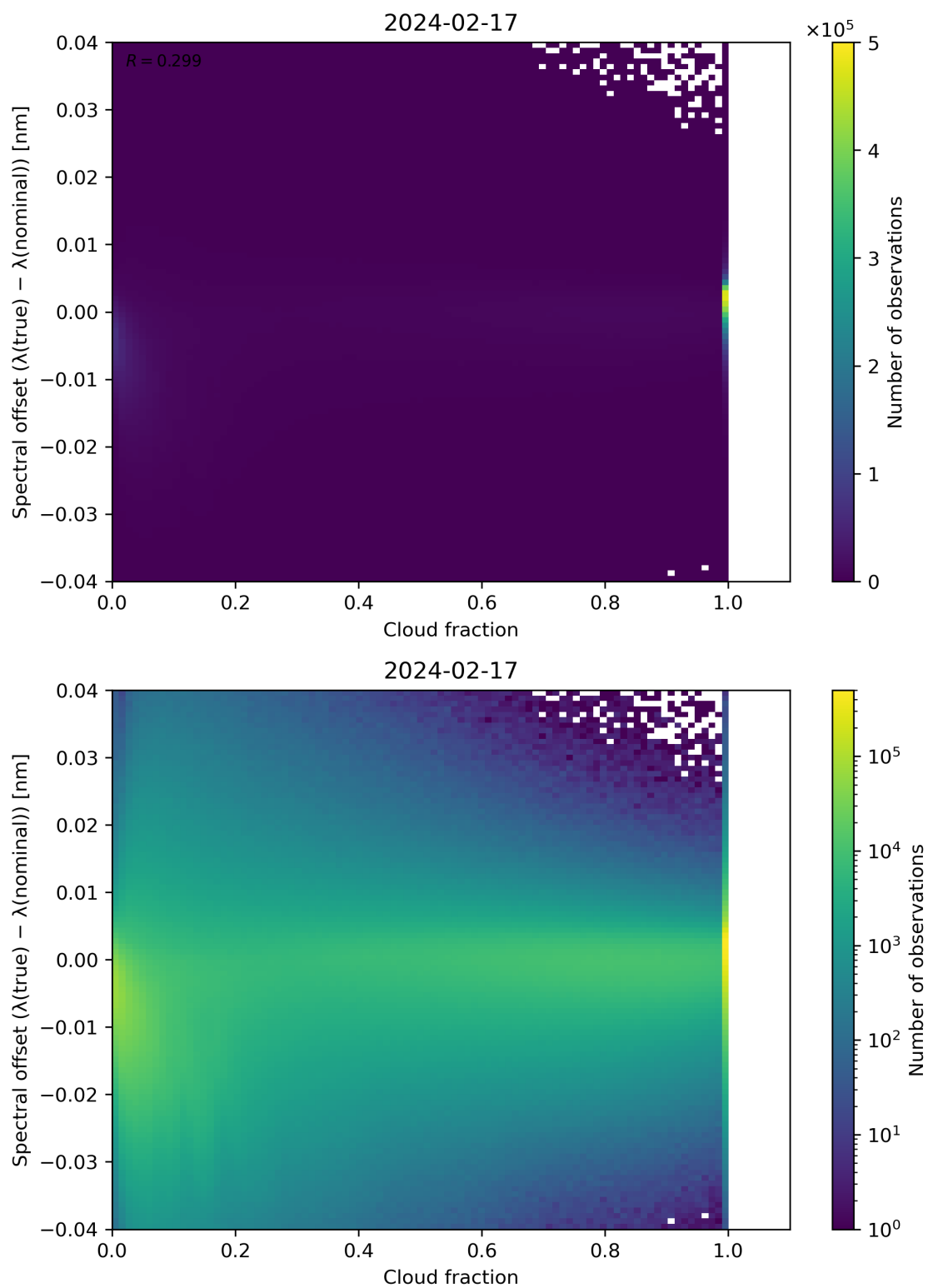
Figure 76: Scatter density plot of “Cloud fraction” against “Spectral offset ( \lambda(\text{true}) - \lambda(\text{nominal}) )” for 2024-02-17 to 2024-02-18.
