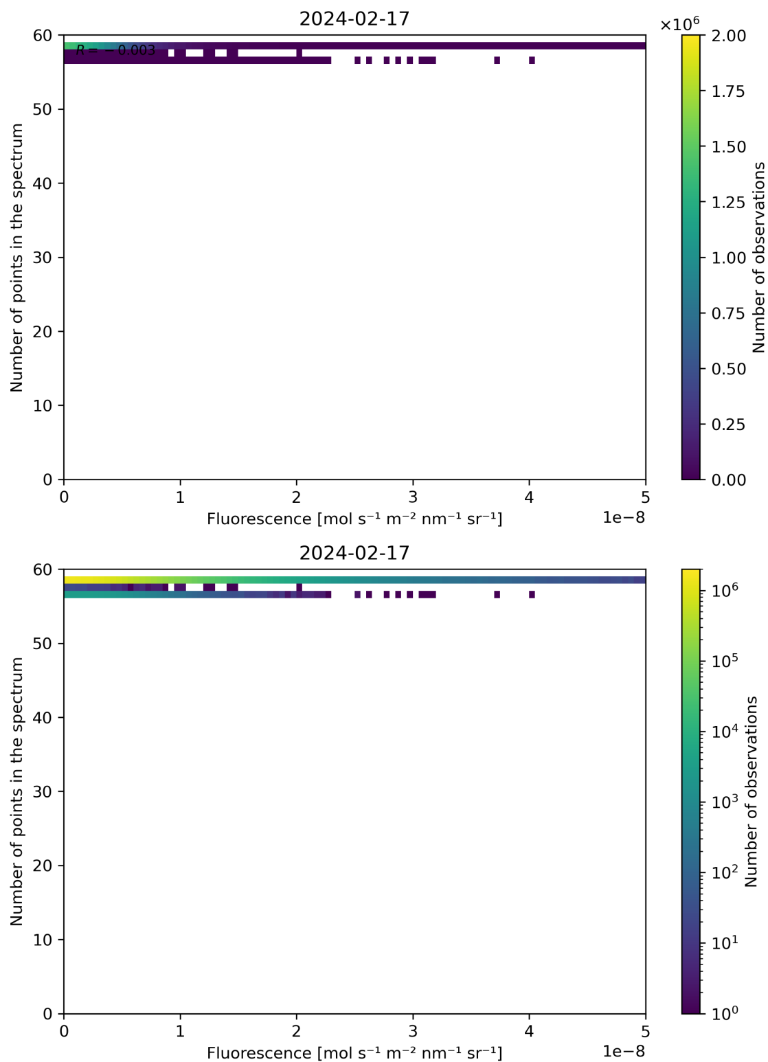
Figure 86: Scatter density plot of “Fluorescence” against “Number of points in the spectrum” for 2024-02-17 to 2024-02-18.
