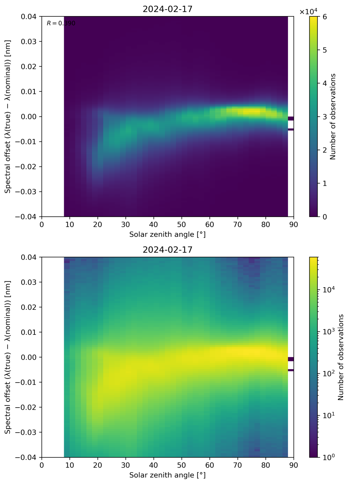
Figure 117: Scatter density plot of “Solar zenith angle” against “Spectral offset ( \lambda(\text{true}) - \lambda(\text{nominal}) )” for 2024-02-17 to 2024-02-18.
