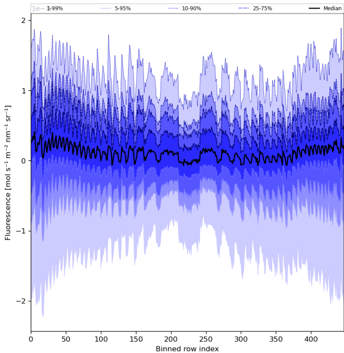
Figure 57: Along track statistics of “Fluorescence” for 2024-02-17 to 2024-02-18
