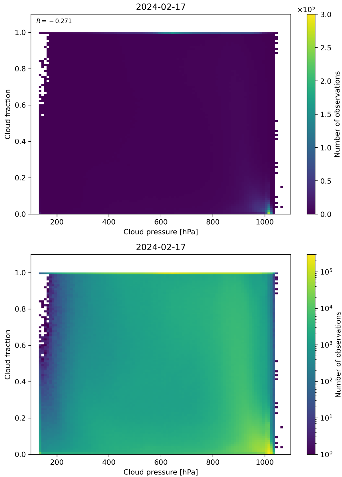
Figure 79: Scatter density plot of “Cloud pressure” against “Cloud fraction” for 2024-02-17 to 2024-02-18.
