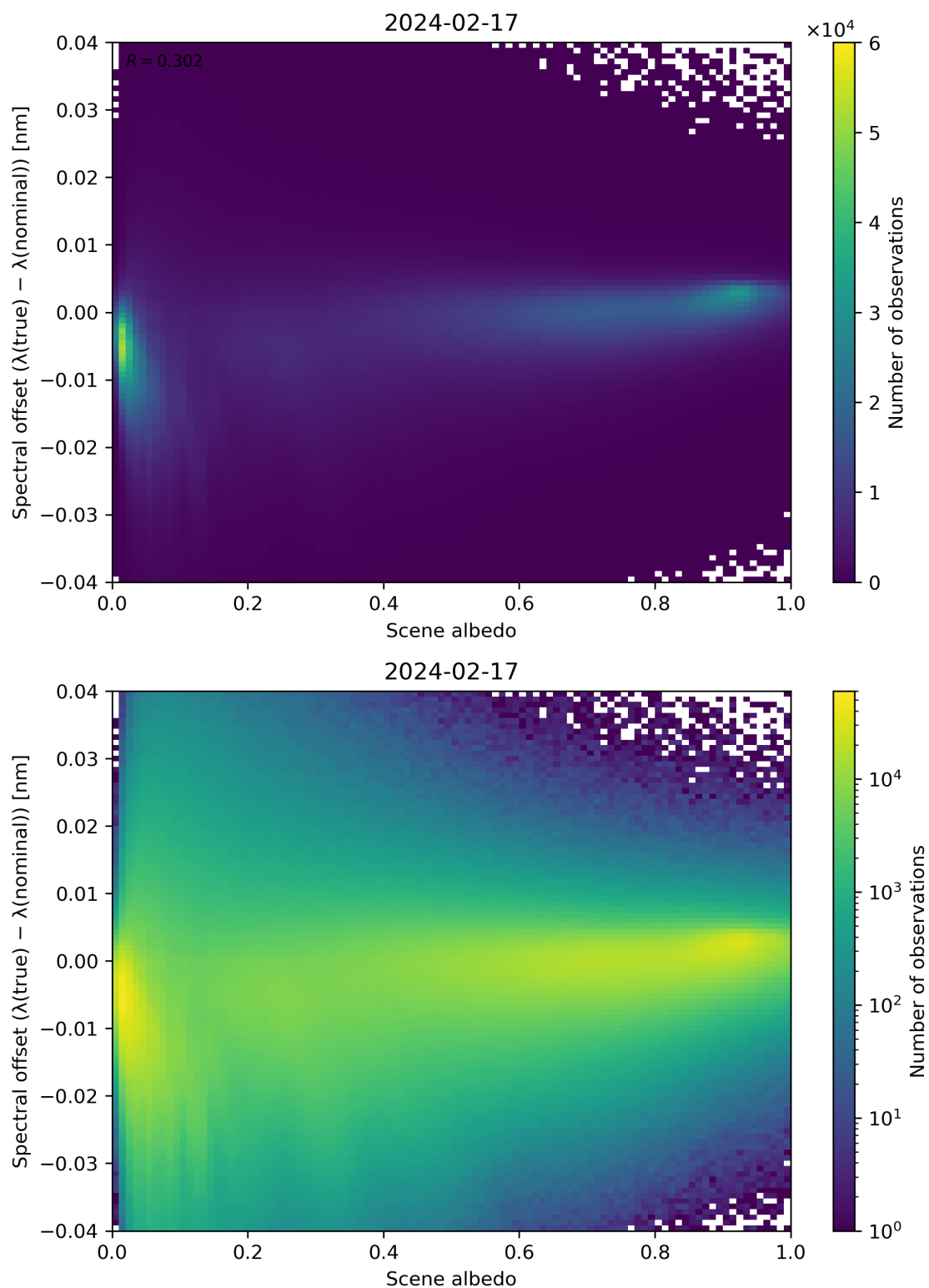
Figure 107: Scatter density plot of “Scene albedo” against “Spectral offset ( \lambda(\text{true}) - \lambda(\text{nominal}) )” for 2024-02-17 to 2024-02-18.
