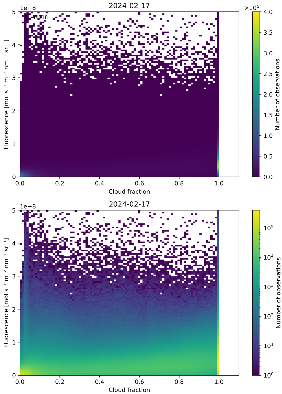
Figure 72: Scatter density plot of “Cloud fraction” against “Fluorescence” for 2024-02-17 to 2024-02-18.
