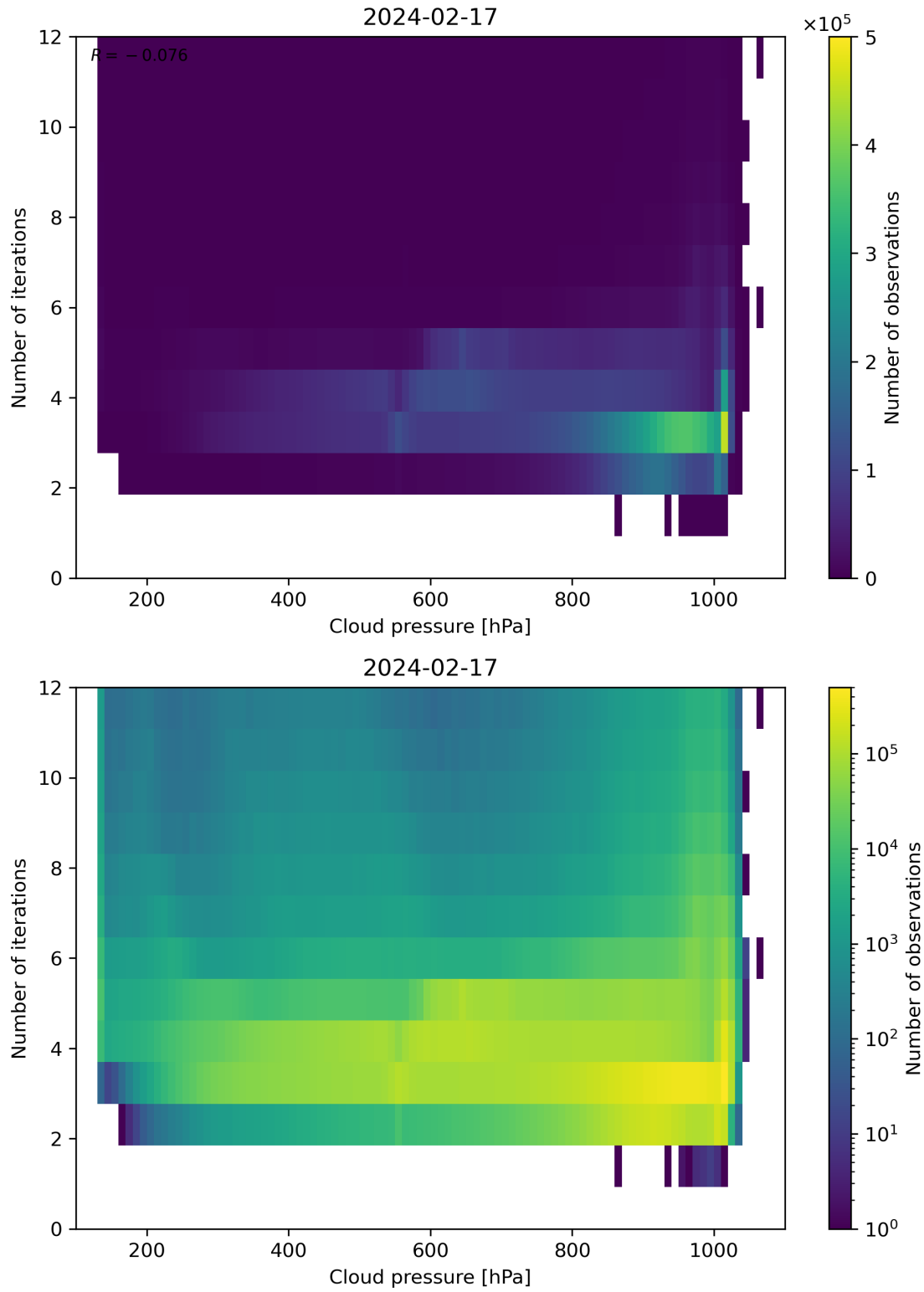
Figure 81: Scatter density plot of “Cloud pressure” against “Number of iterations” for 2024-02-17 to 2024-02-18.
