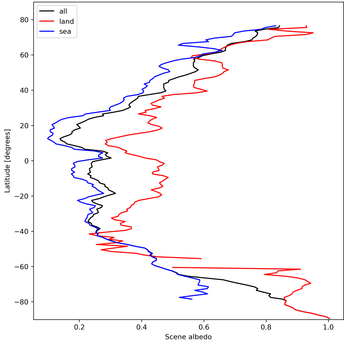
Figure 17: Zonal average of “Scene albedo” for 2024-02-17 to 2024-02-18.
