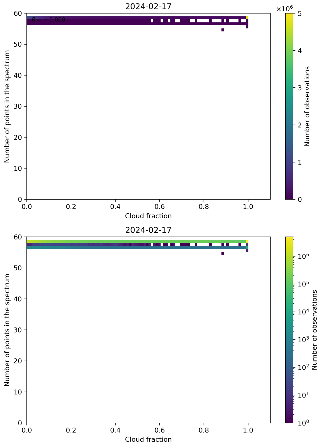
Figure 74: Scatter density plot of “Cloud fraction” against “Number of points in the spectrum” for 2024-02-17 to 2024-02-18.
