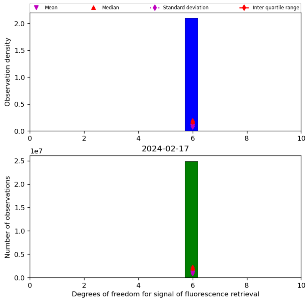
Figure 43: Histogram of “Degrees of freedom for signal of fluorescence retrieval” for 2024-02-17 to 2024-02-18
