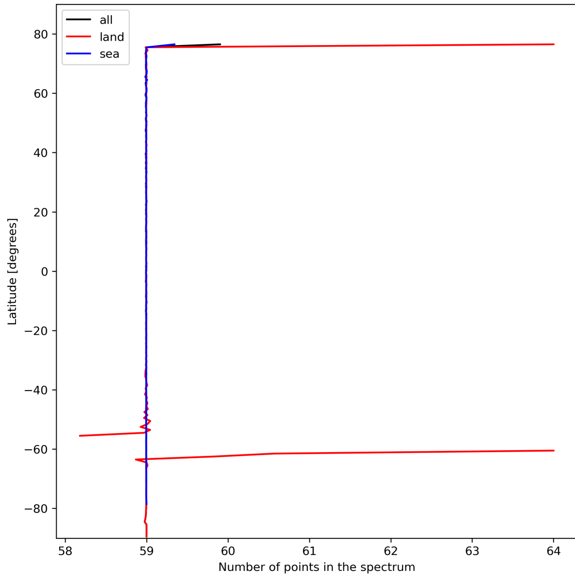
Figure 27: Zonal average of “Number of points in the spectrum” for 2024-02-17 to 2024-02-18.
