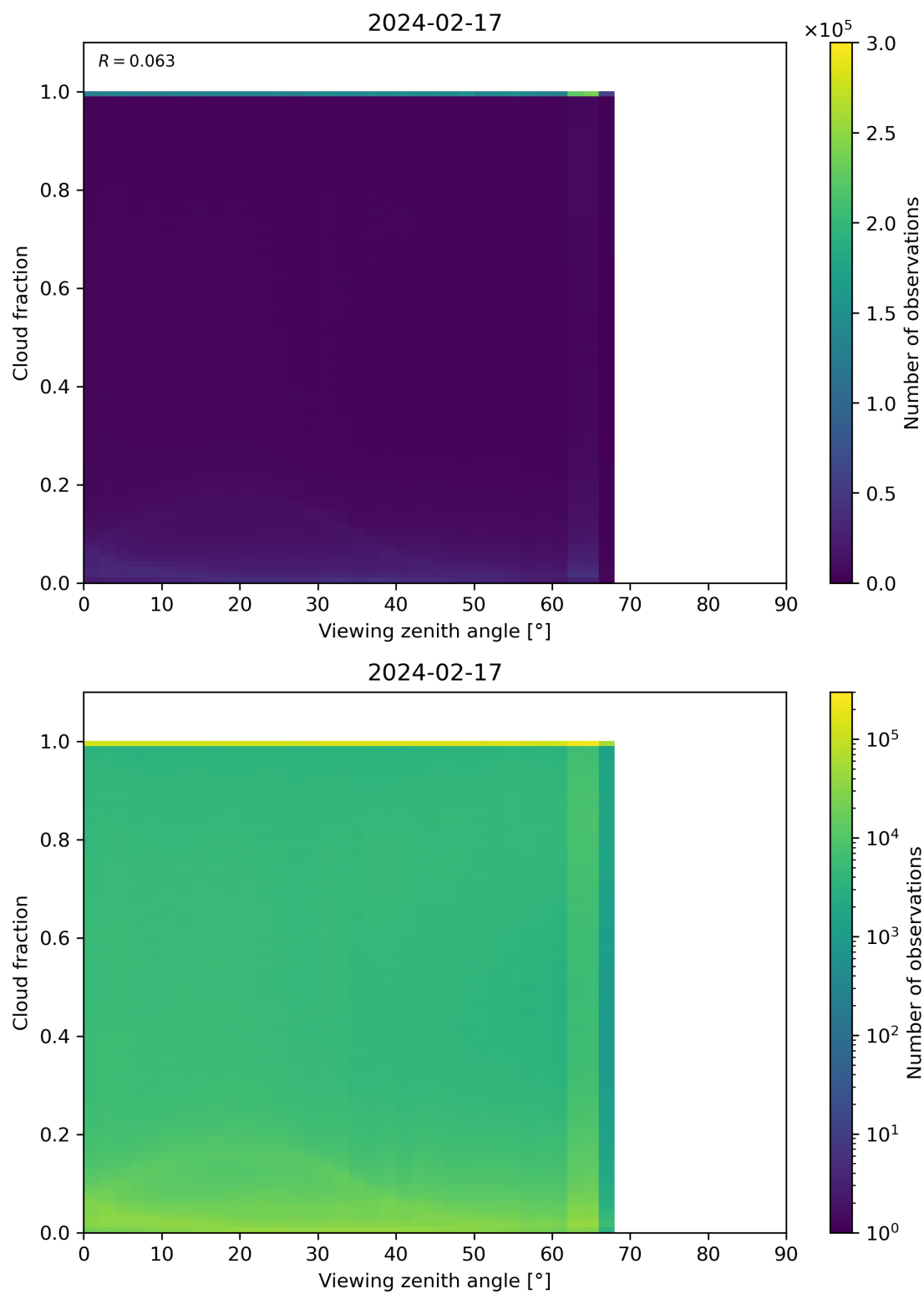
Figure 120: Scatter density plot of “Viewing zenith angle” against “Cloud fraction” for 2024-02-17 to 2024-02-18.
