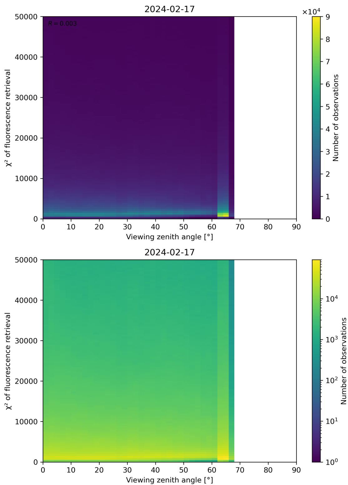
Figure 119: Scatter density plot of “Viewing zenith angle” against “ \chi^2 of fluorescence retrieval” for 2024-02-17 to 2024-02-18.
