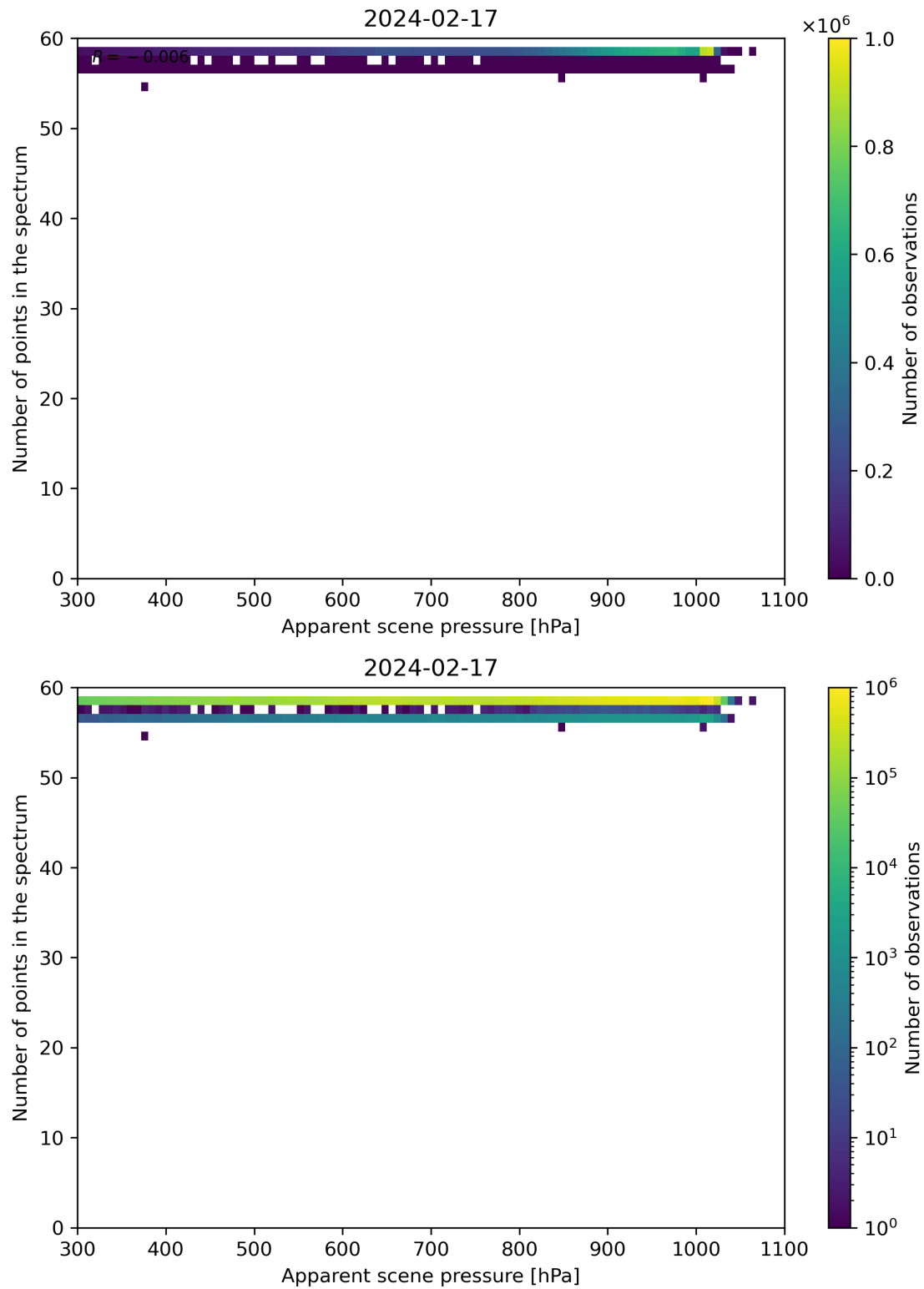
Figure 66: Scatter density plot of “Apparent scene pressure” against “Number of points in the spectrum” for 2024-02-17 to 2024-02-18.
