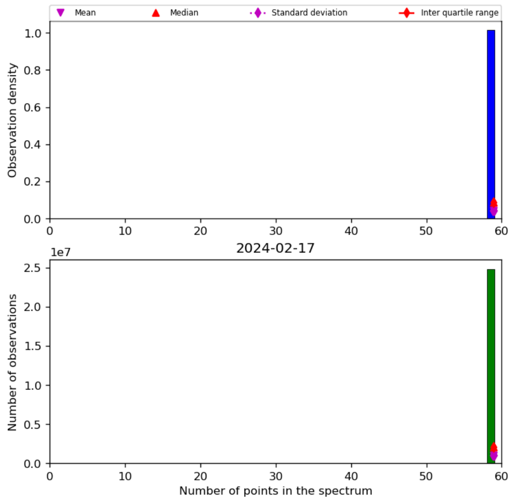
Figure 44: Histogram of “Number of points in the spectrum” for 2024-02-17 to 2024-02-18
