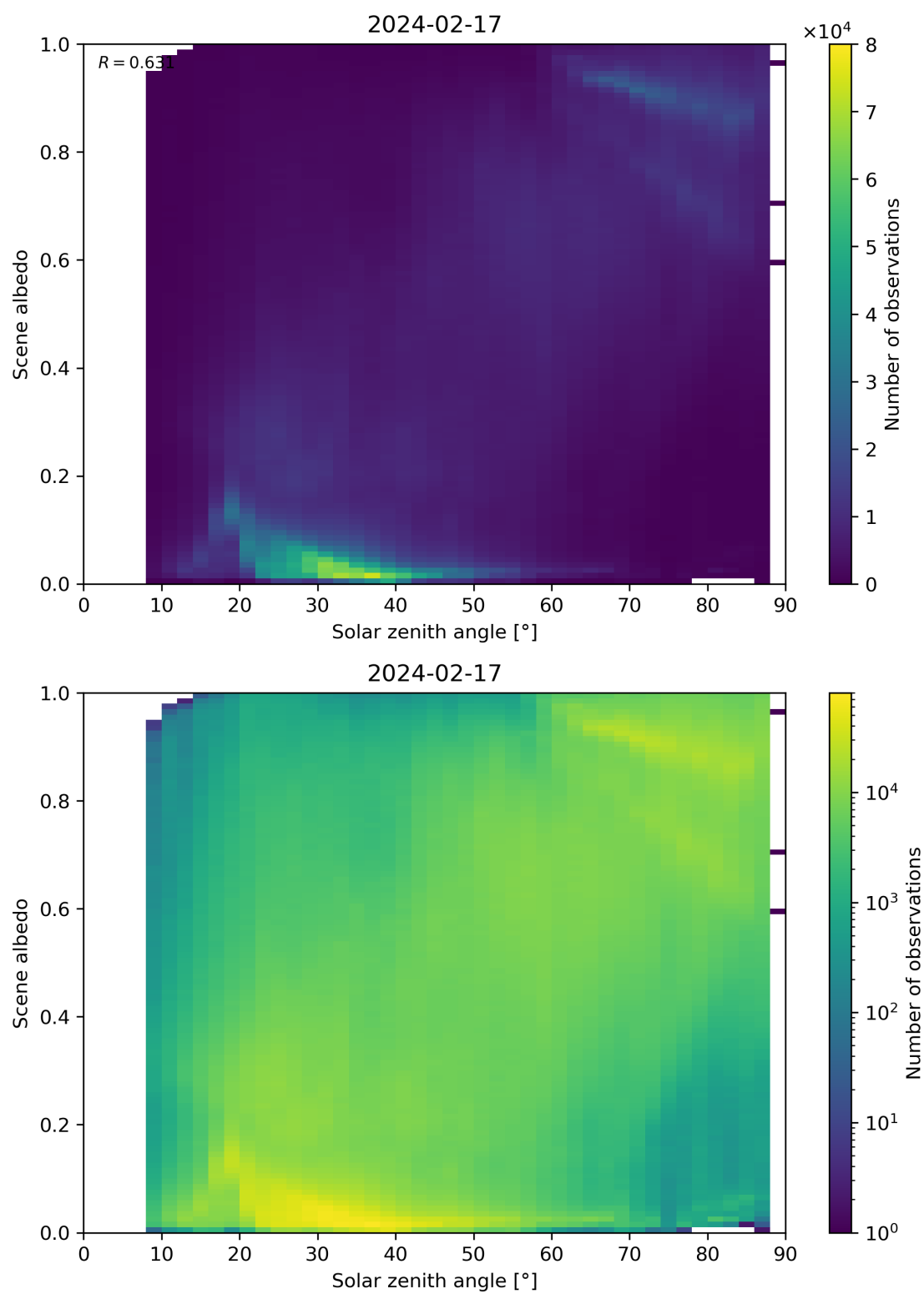
Figure 116: Scatter density plot of “Solar zenith angle” against “Scene albedo” for 2024-02-17 to 2024-02-18.
