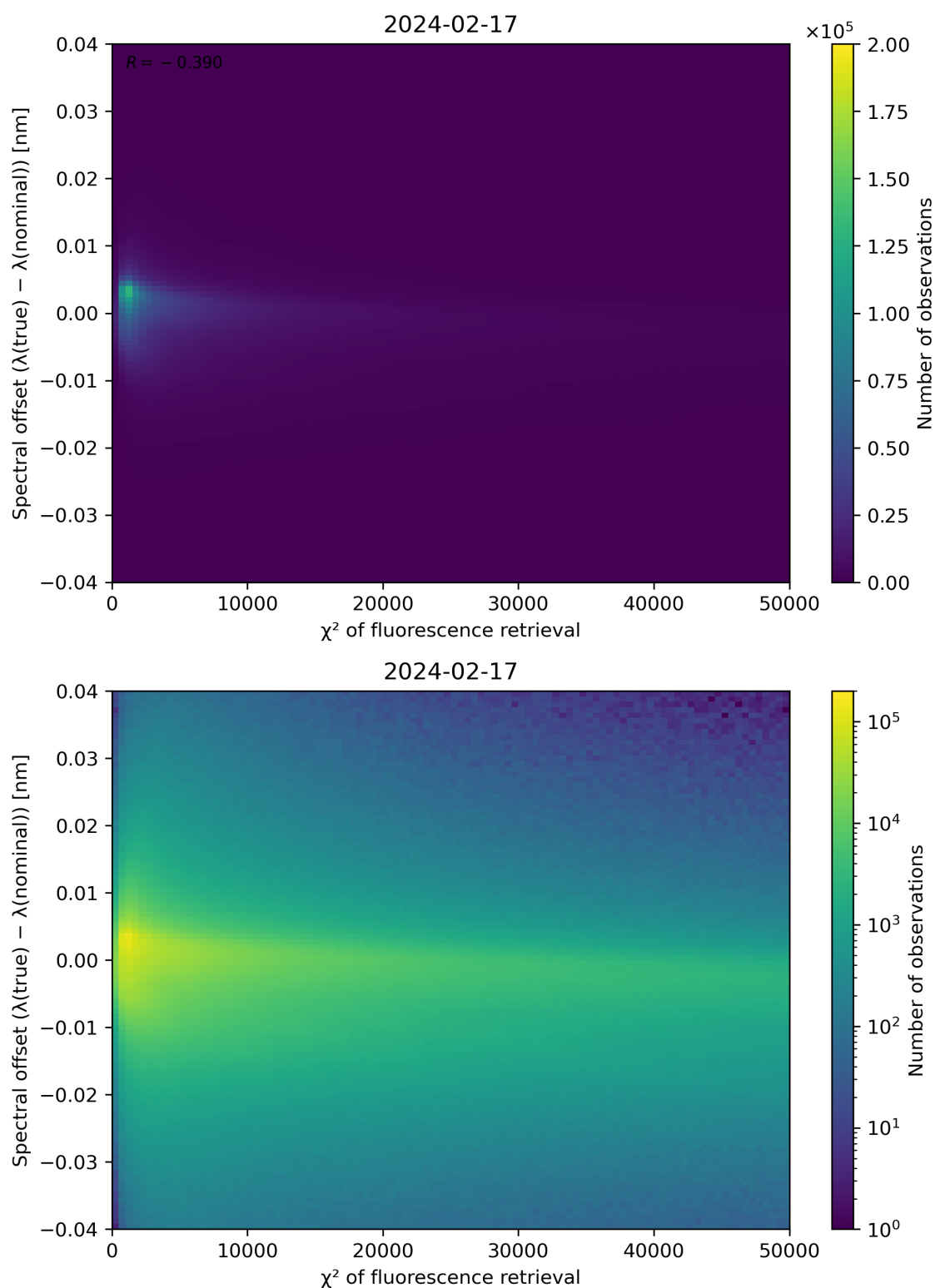
Figure 69: Scatter density plot of " \chi^2 of fluorescence retrieval" against "Spectral offset ( \lambda(\text{true}) - \lambda(\text{nominal})) " for 2024-02-17 to 2024-02-18.
