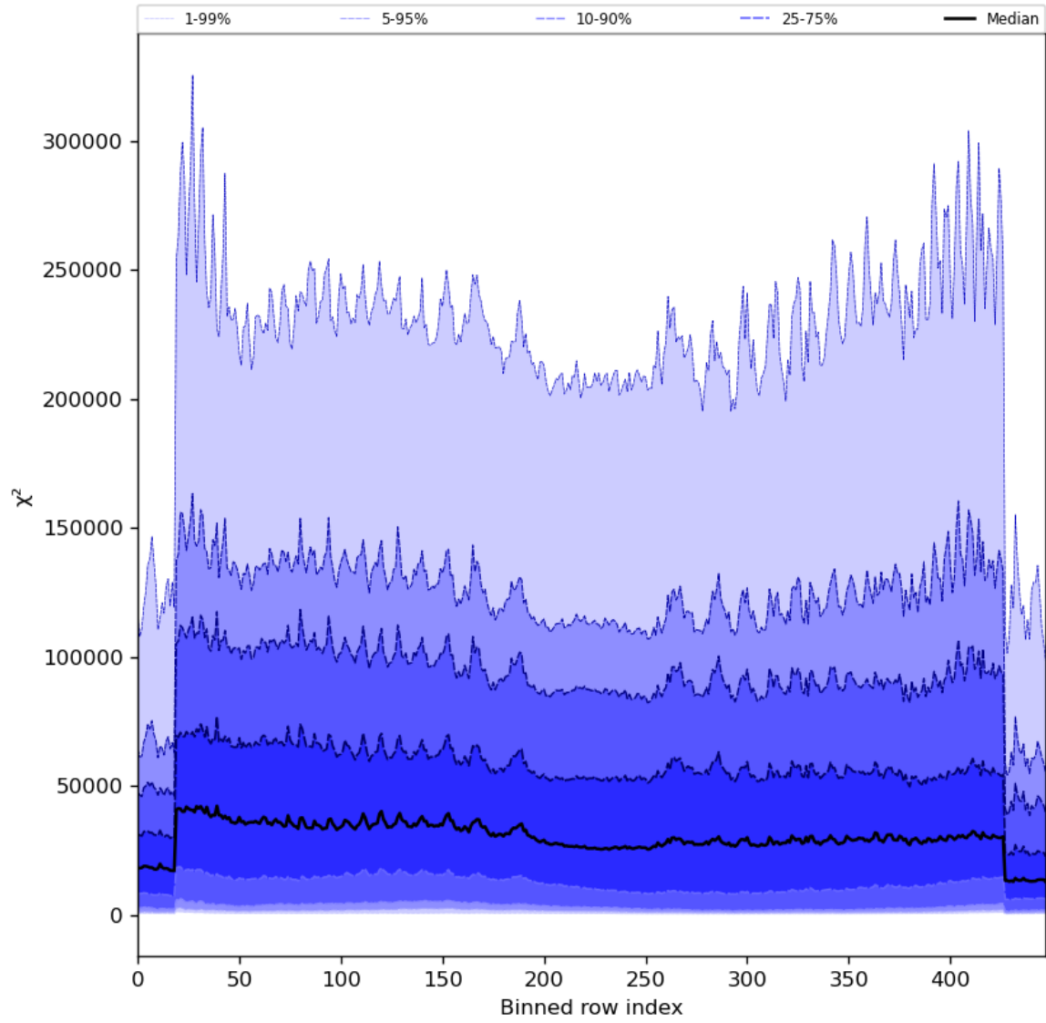
Figure 55: Along track statistics of “ \chi^2 ” for 2024-02-17 to 2024-02-18
