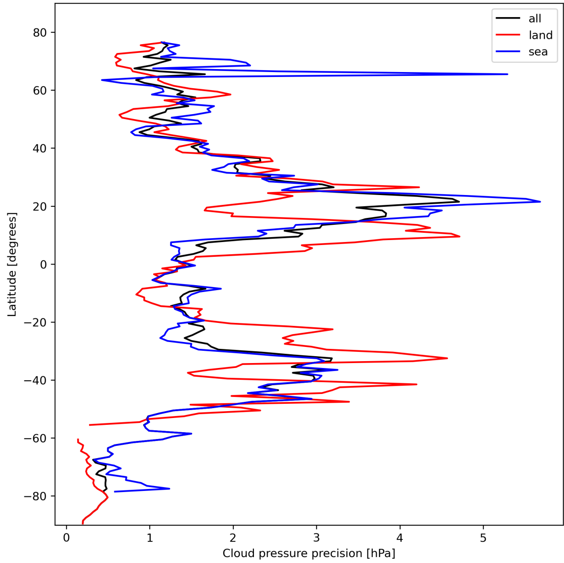
Figure 14: Zonal average of “Cloud pressure precision” for 2024-02-17 to 2024-02-18.
