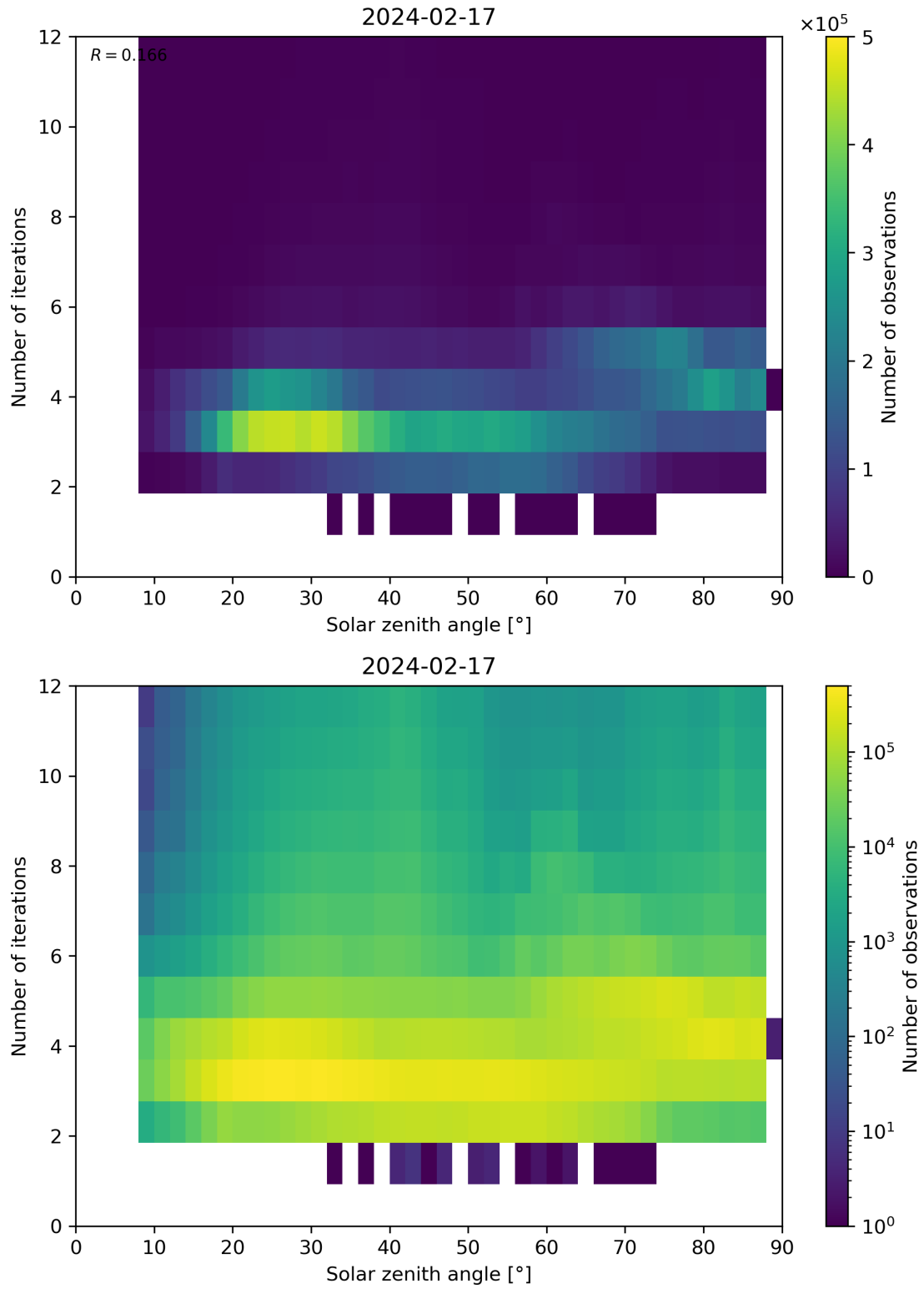
Figure 114: Scatter density plot of “Solar zenith angle” against “Number of iterations” for 2024-02-17 to 2024-02-18.
