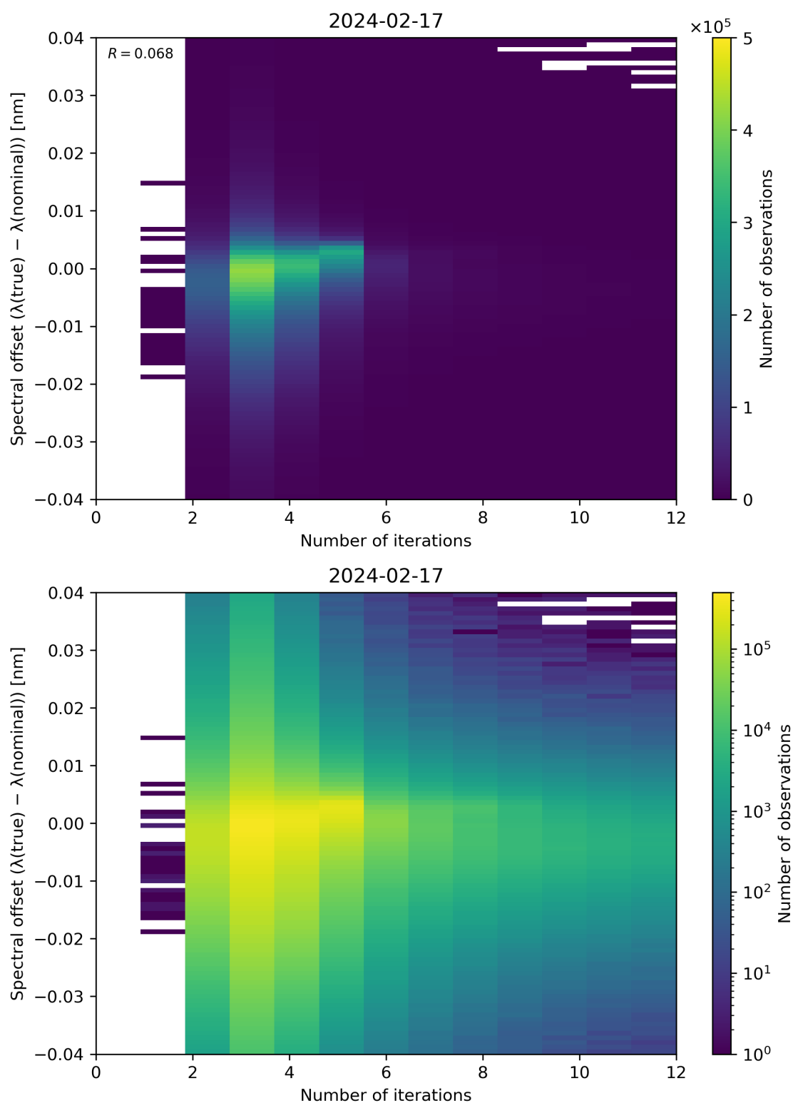
Figure 100: Scatter density plot of “Number of iterations” against “Spectral offset ( \lambda(\text{true}) - \lambda(\text{nominal}) )” for 2024-02-17 to 2024-02-18.
