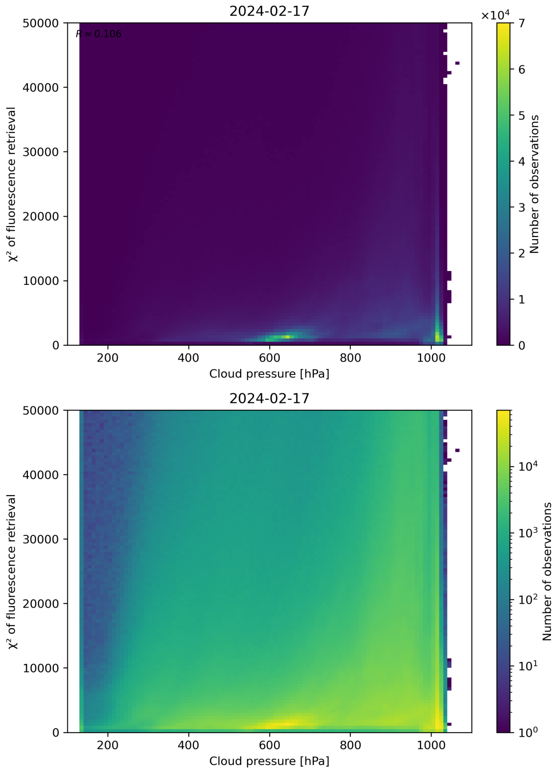
Figure 78: Scatter density plot of “Cloud pressure” against “ \chi^2 of fluorescence retrieval” for 2024-02-17 to 2024-02-18.
