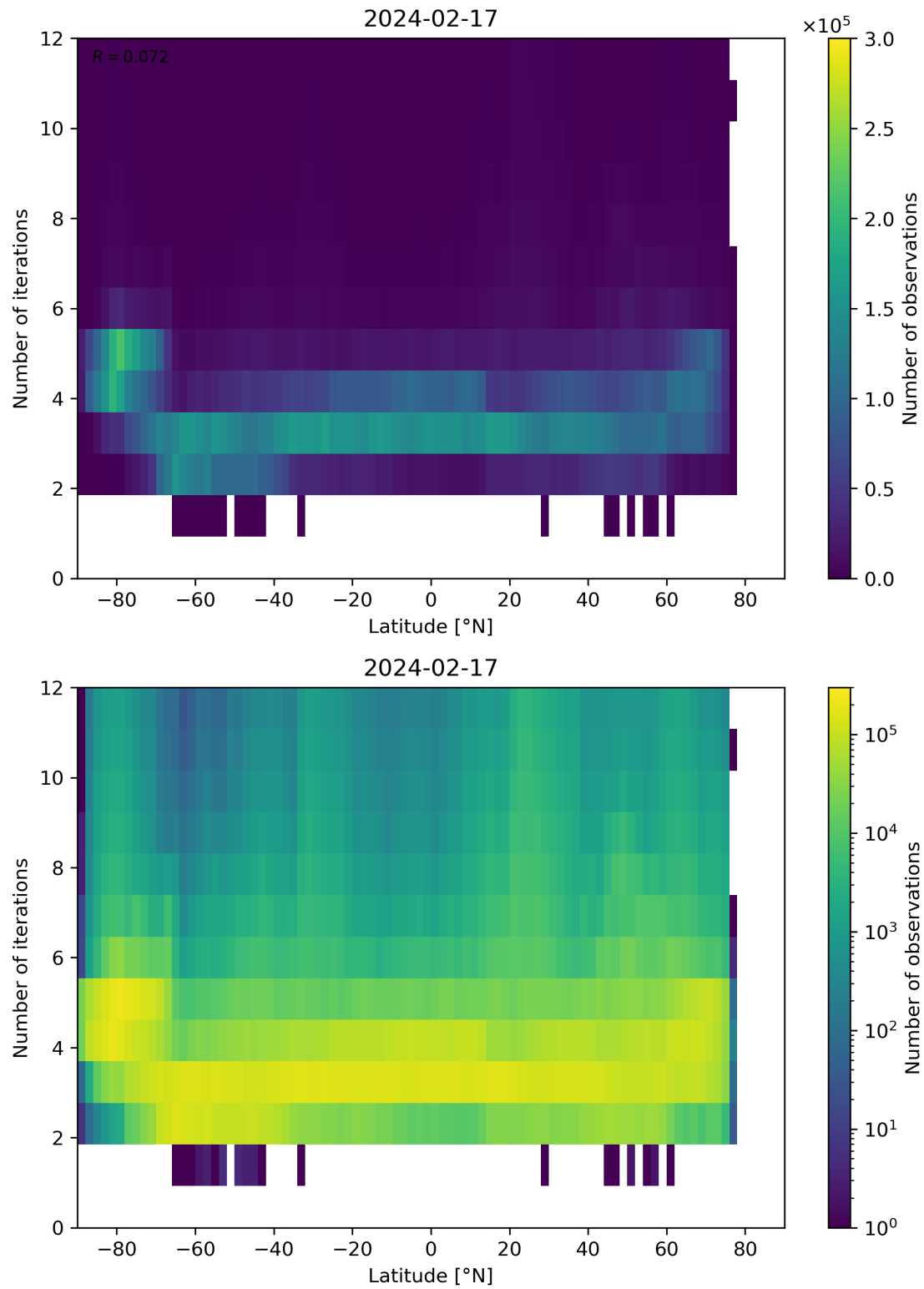
Figure 93: Scatter density plot of “Latitude” against “Number of iterations” for 2024-02-17 to 2024-02-18.
