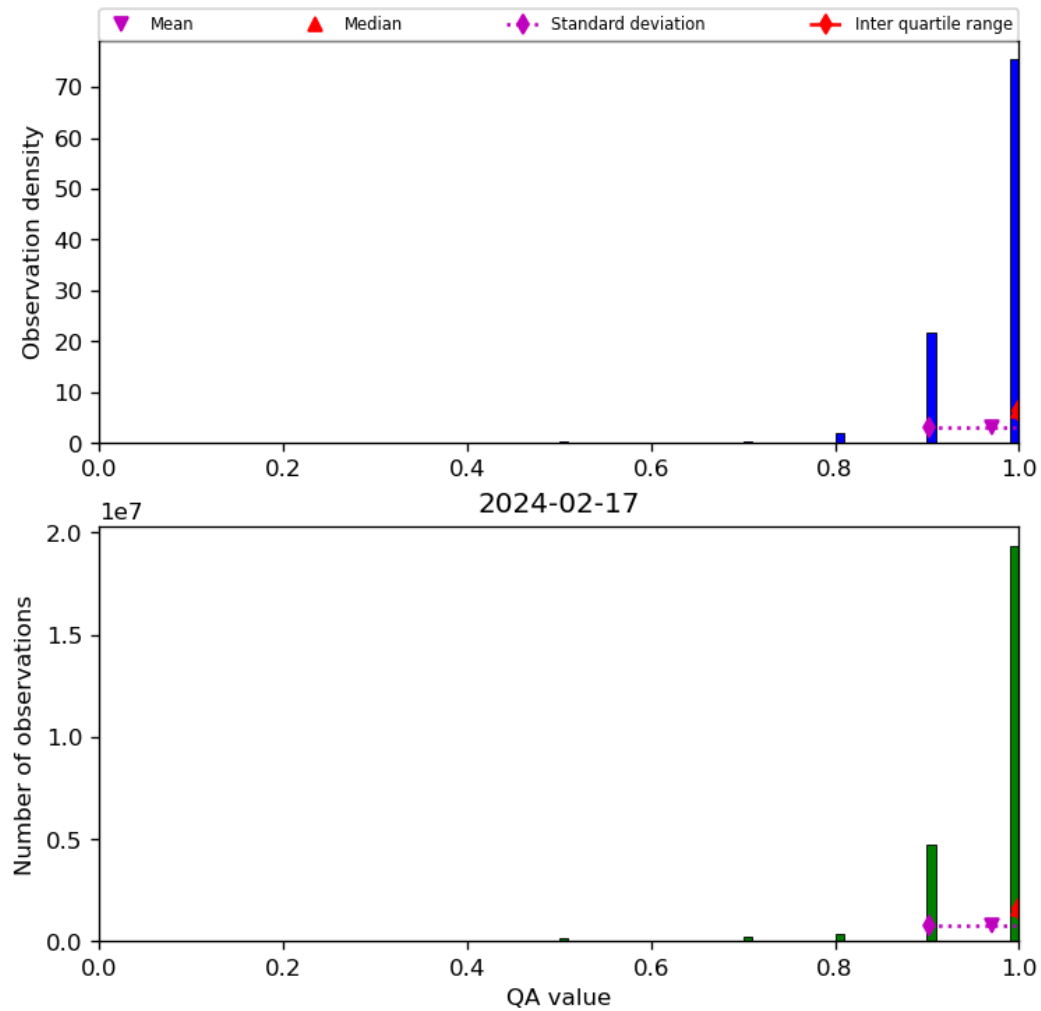
Figure 29: Histogram of “QA value” for 2024-02-17 to 2024-02-18
