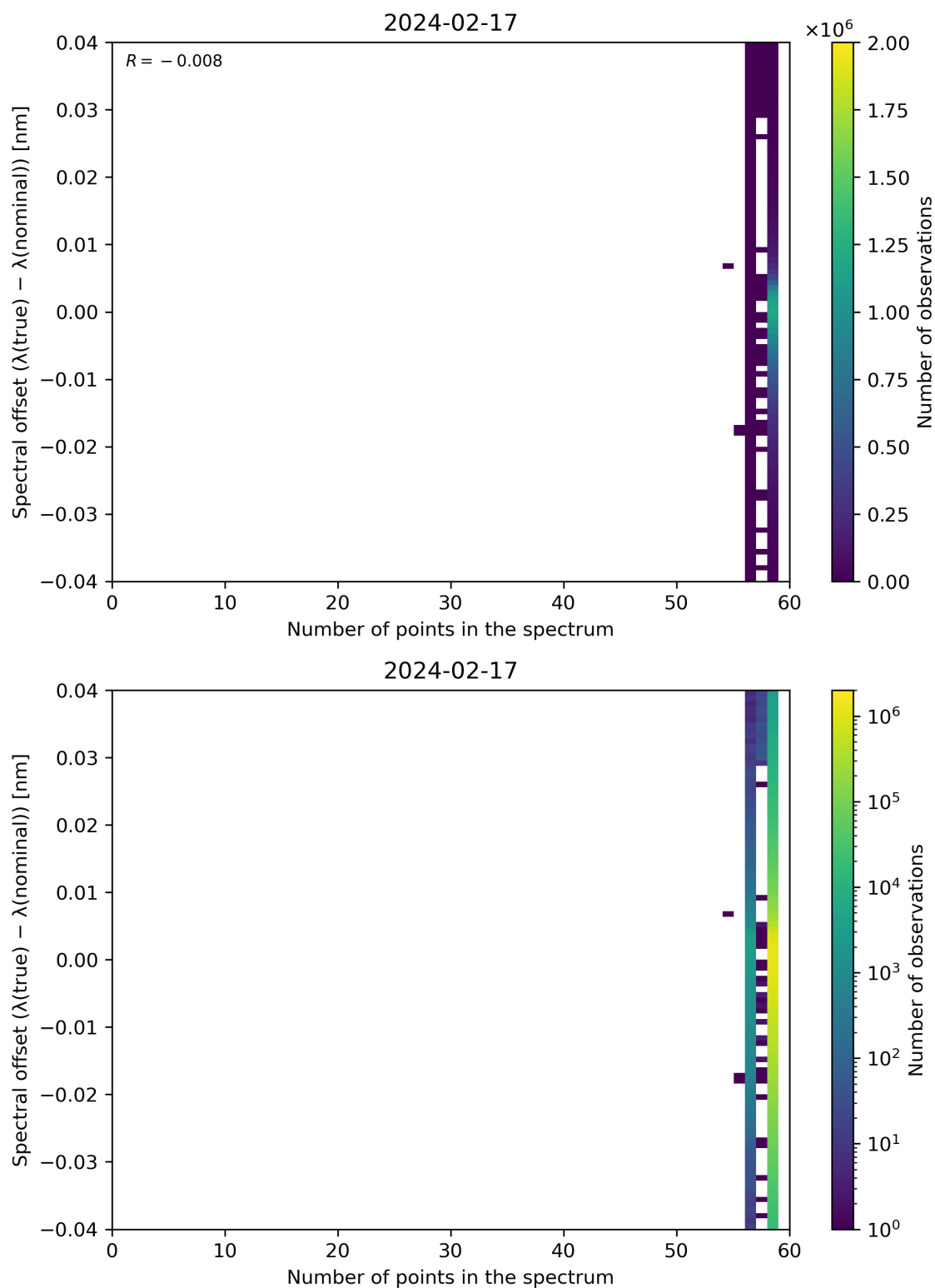
Figure 101: Scatter density plot of “Number of points in the spectrum” against “Spectral offset ( \lambda(\text{true}) - \lambda(\text{nominal}) )” for 2024-02-17 to 2024-02-18.
