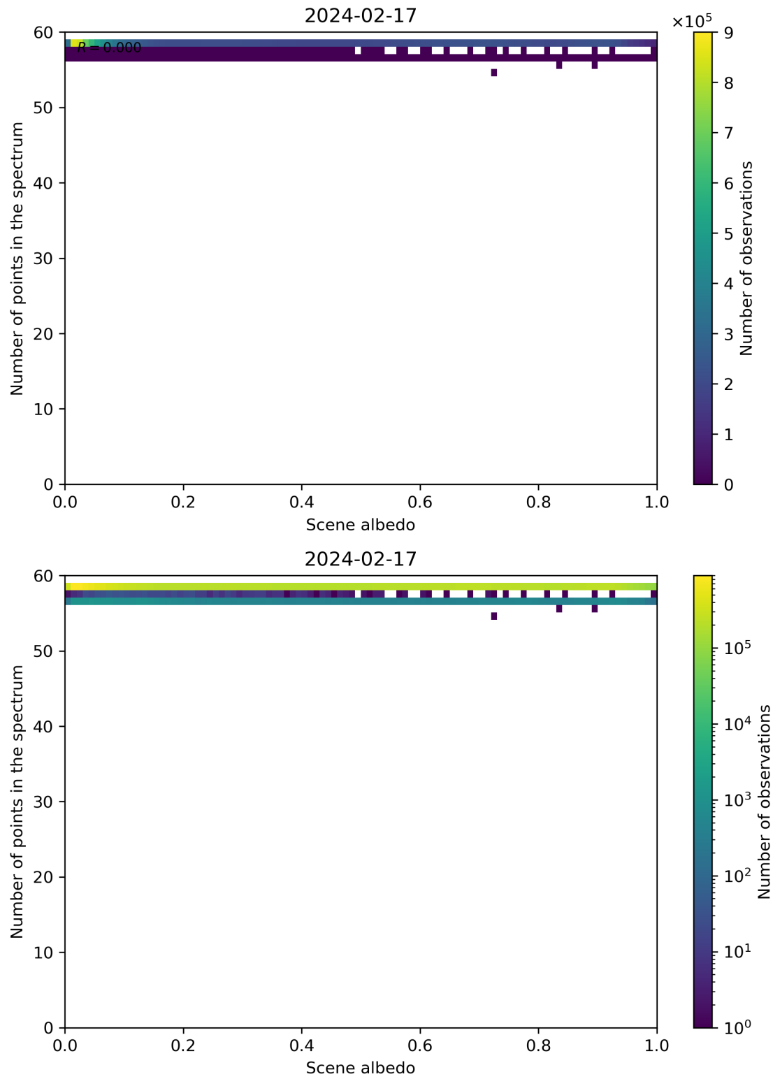
Figure 106: Scatter density plot of “Scene albedo” against “Number of points in the spectrum” for 2024-02-17 to 2024-02-18.
