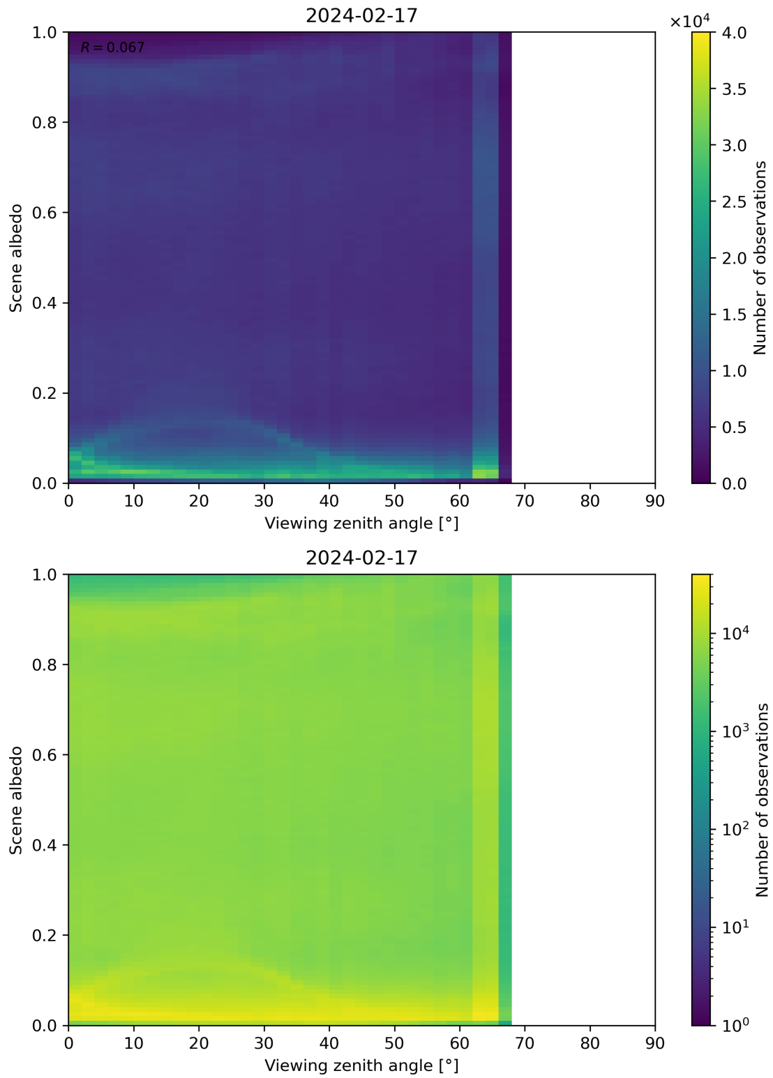
Figure 126: Scatter density plot of “Viewing zenith angle” against “Scene albedo” for 2024-02-17 to 2024-02-18.
