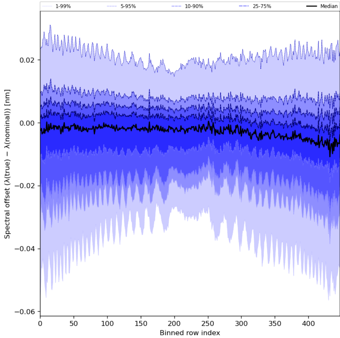
Figure 62: Along track statistics of “Spectral offset ( \lambda(\text{true}) - \lambda(\text{nominal}) )” for 2024-02-17 to 2024-02-18
