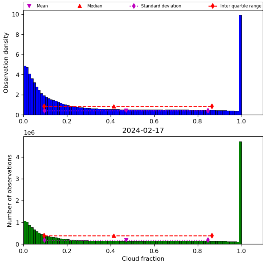
Figure 32: Histogram of “Cloud fraction” for 2024-02-17 to 2024-02-18
