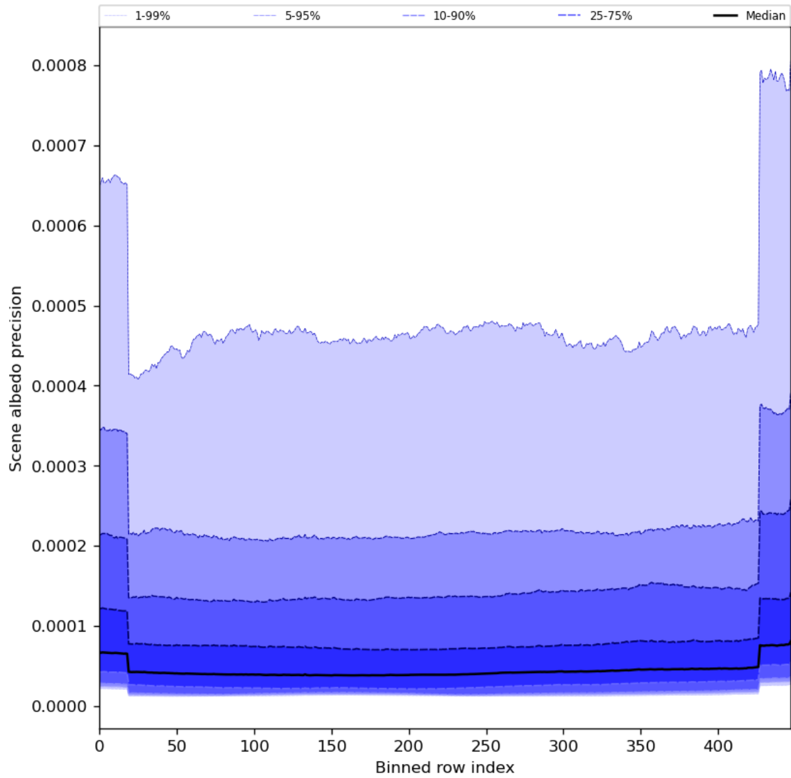
Figure 52: Along track statistics of “Scene albedo precision” for 2024-02-17 to 2024-02-18
