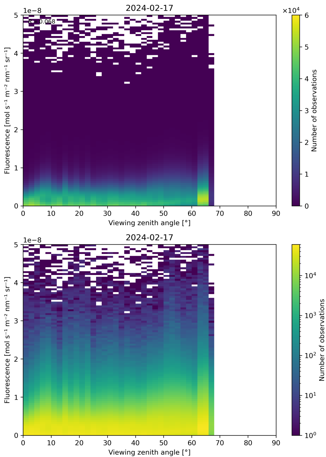
Figure 122: Scatter density plot of “Viewing zenith angle” against “Fluorescence” for 2024-02-17 to 2024-02-18.
