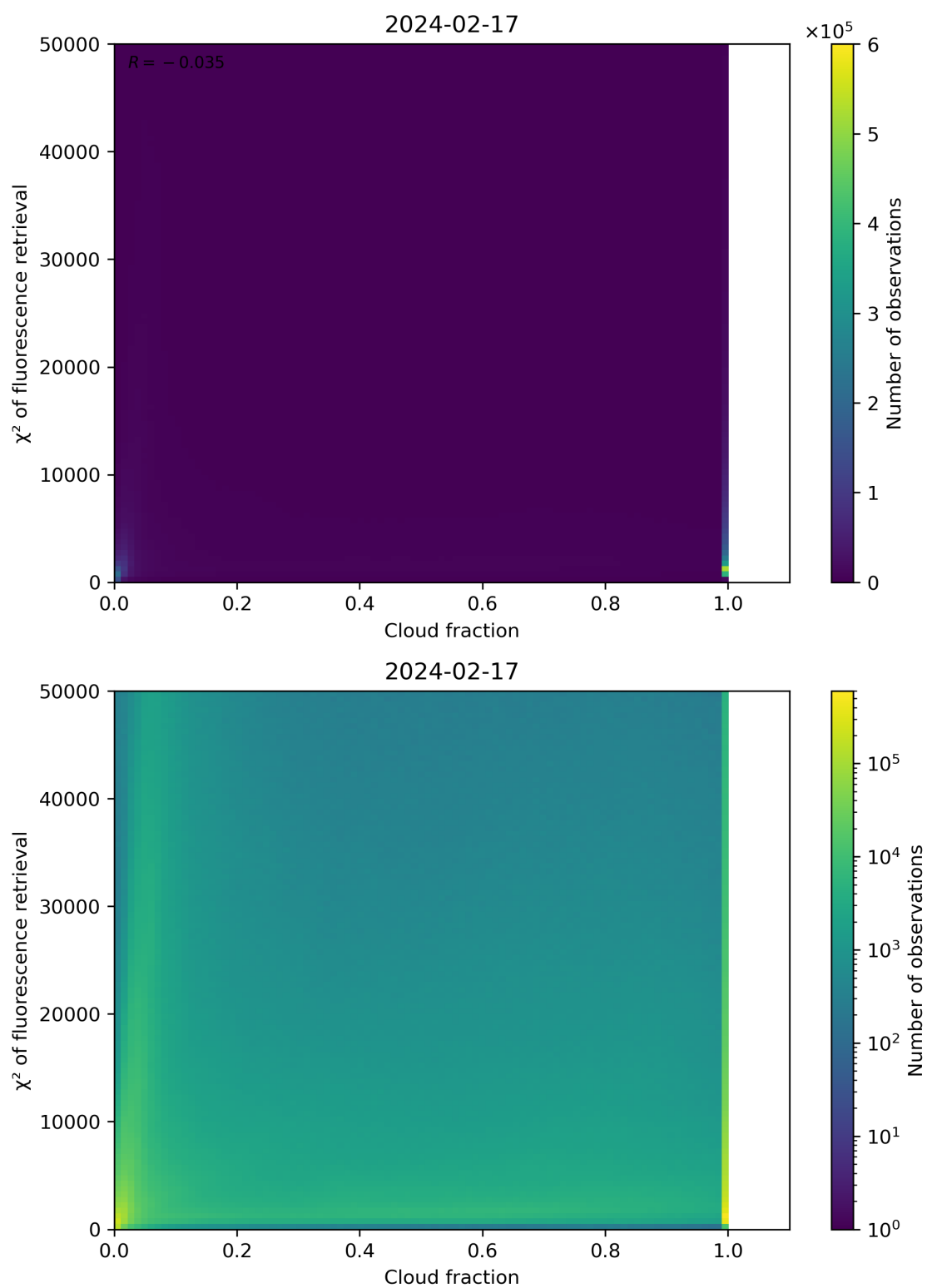
Figure 71: Scatter density plot of “Cloud fraction” against “ \chi^2 of fluorescence retrieval” for 2024-02-17 to 2024-02-18.
