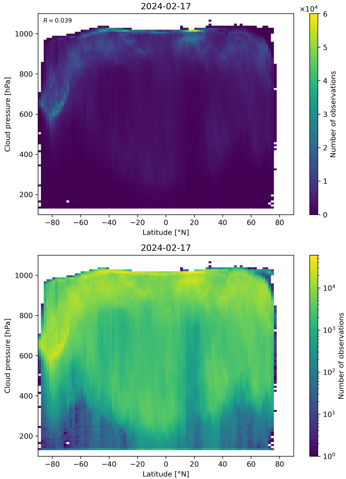
Figure 91: Scatter density plot of “Latitude” against “Cloud pressure” for 2024-02-17 to 2024-02-18.
