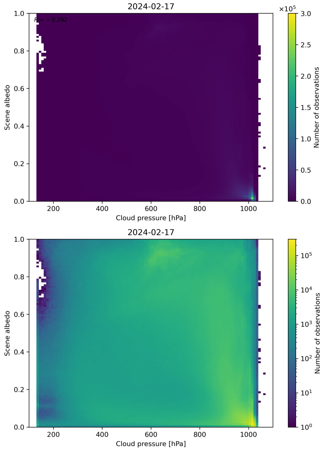
Figure 83: Scatter density plot of “Cloud pressure” against “Scene albedo” for 2024-02-17 to 2024-02-18.
