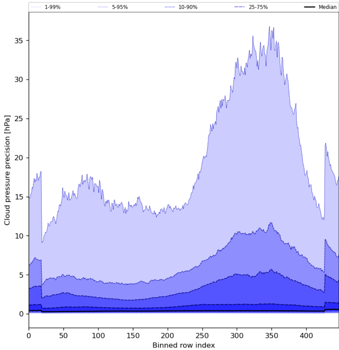
Figure 48: Along track statistics of “Cloud pressure precision” for 2024-02-17 to 2024-02-18
