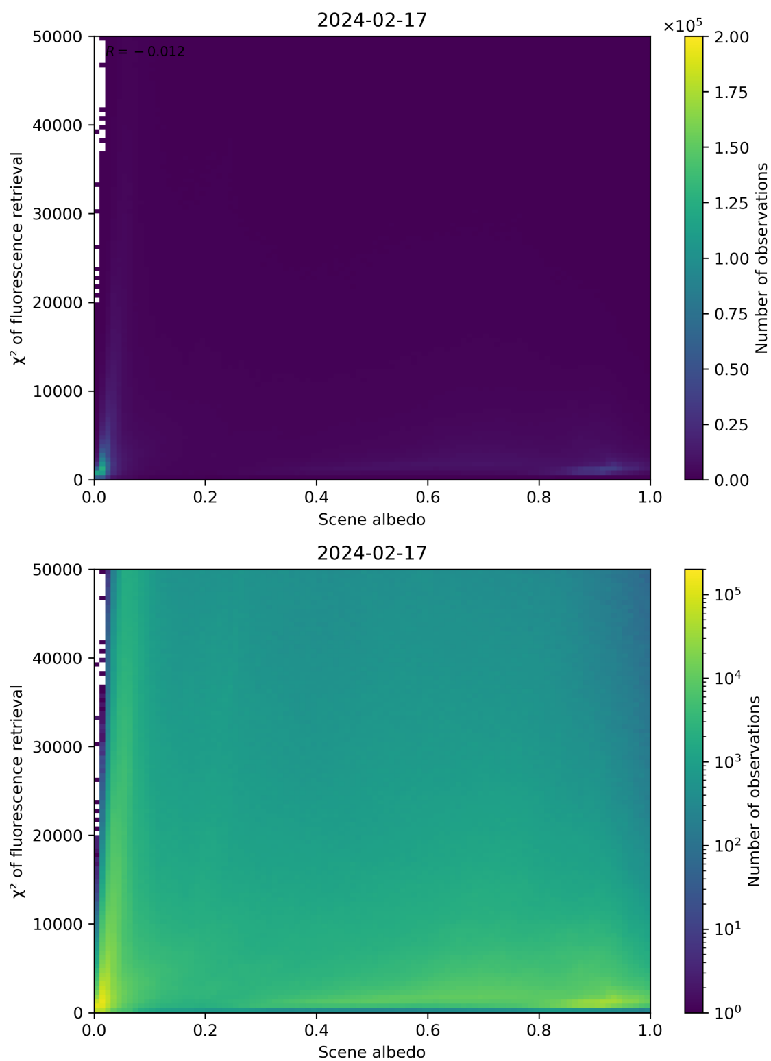
Figure 103: Scatter density plot of “Scene albedo” against “ \chi^2 of fluorescence retrieval” for 2024-02-17 to 2024-02-18.
