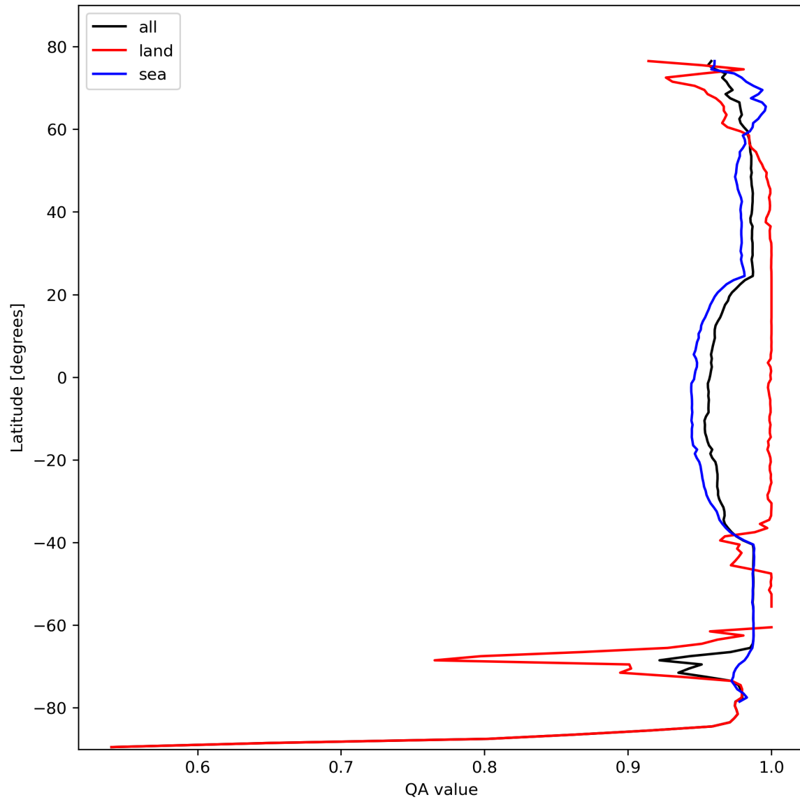
Figure 12: Zonal average of “QA value” for 2024-02-17 to 2024-02-18.
