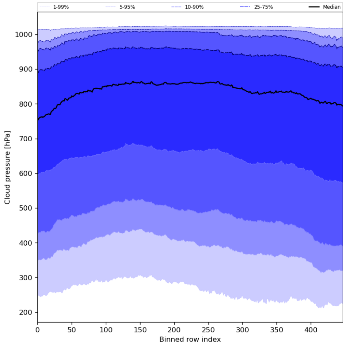
Figure 47: Along track statistics of “Cloud pressure” for 2024-02-17 to 2024-02-18
