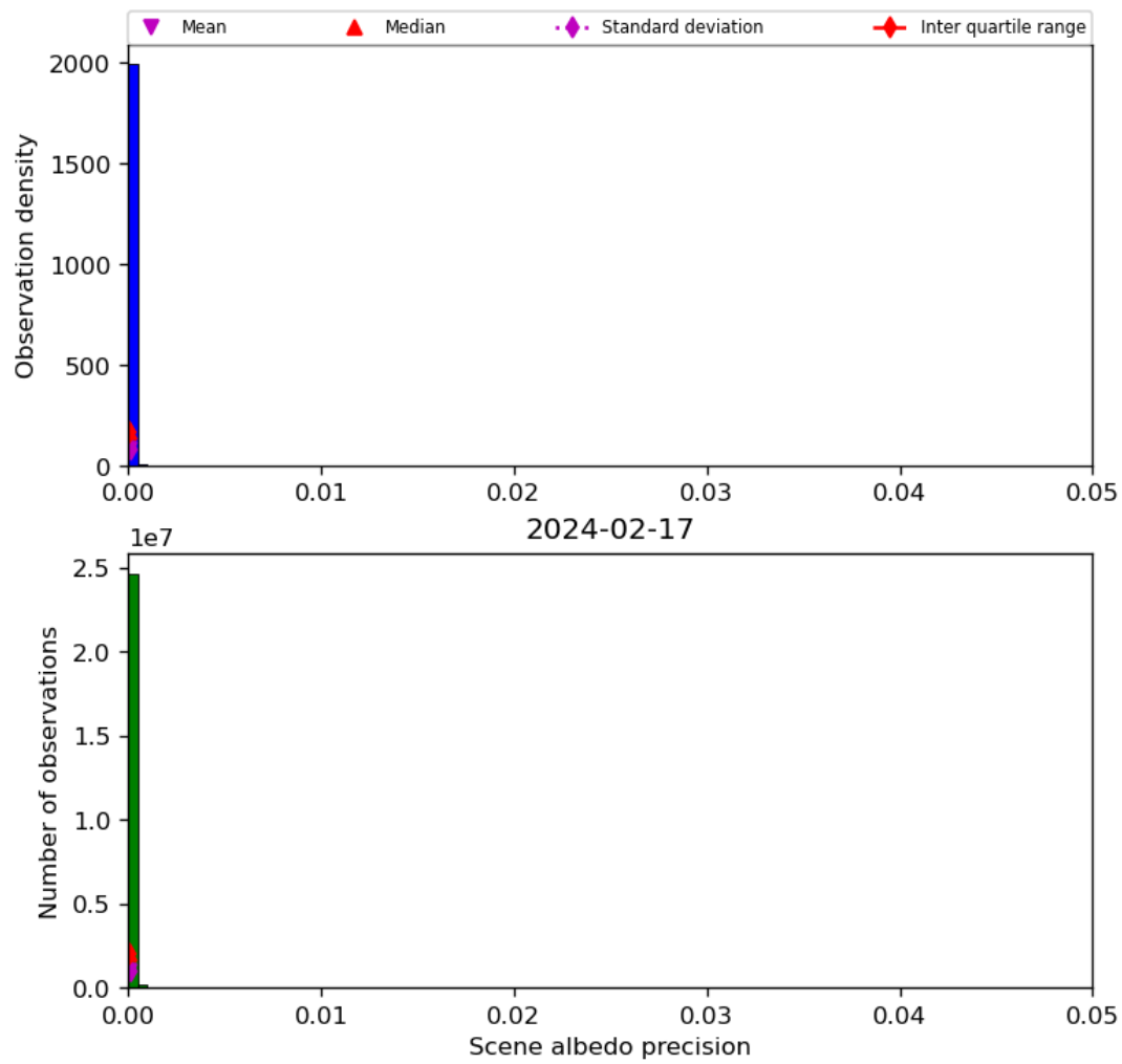
Figure 35: Histogram of “Scene albedo precision” for 2024-02-17 to 2024-02-18
