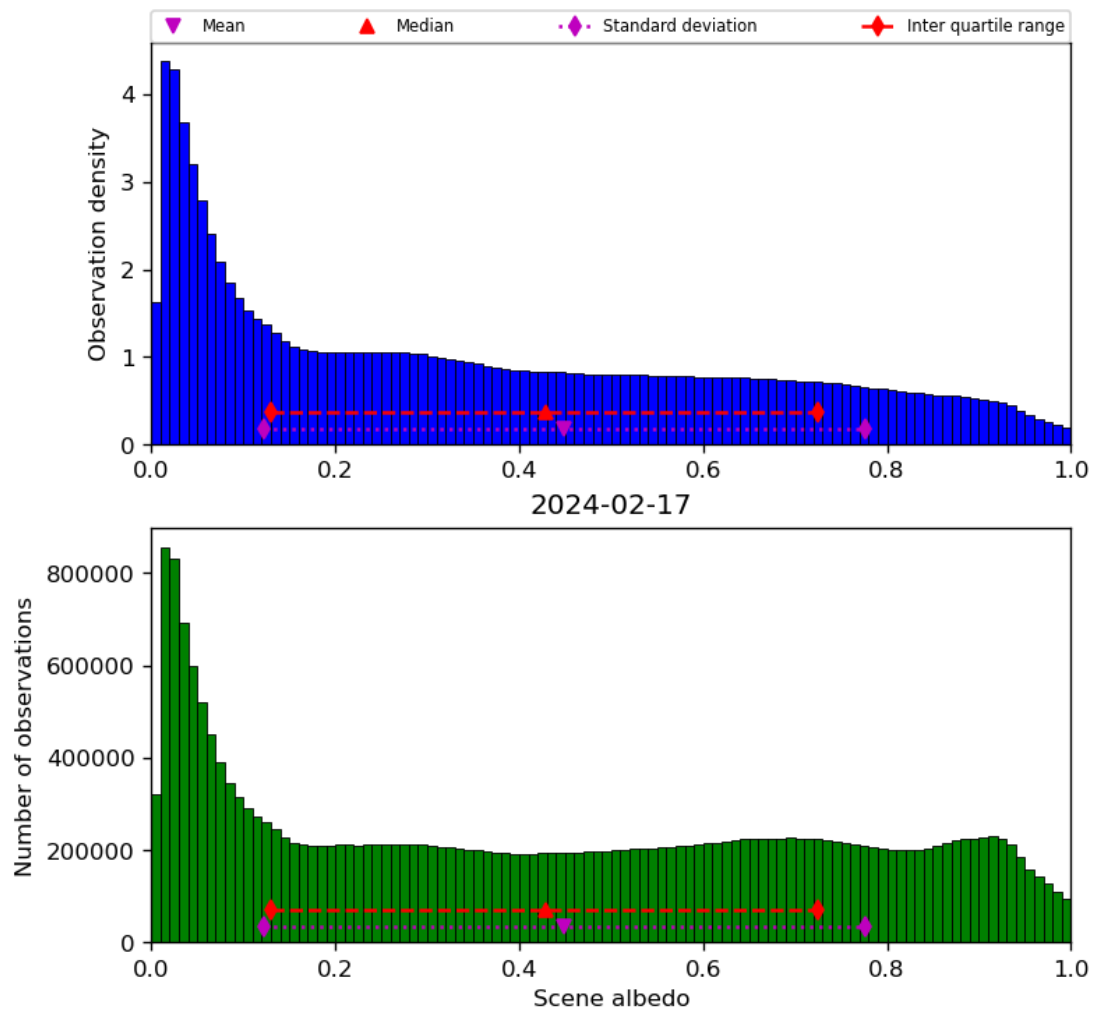
Figure 34: Histogram of “Scene albedo” for 2024-02-17 to 2024-02-18
