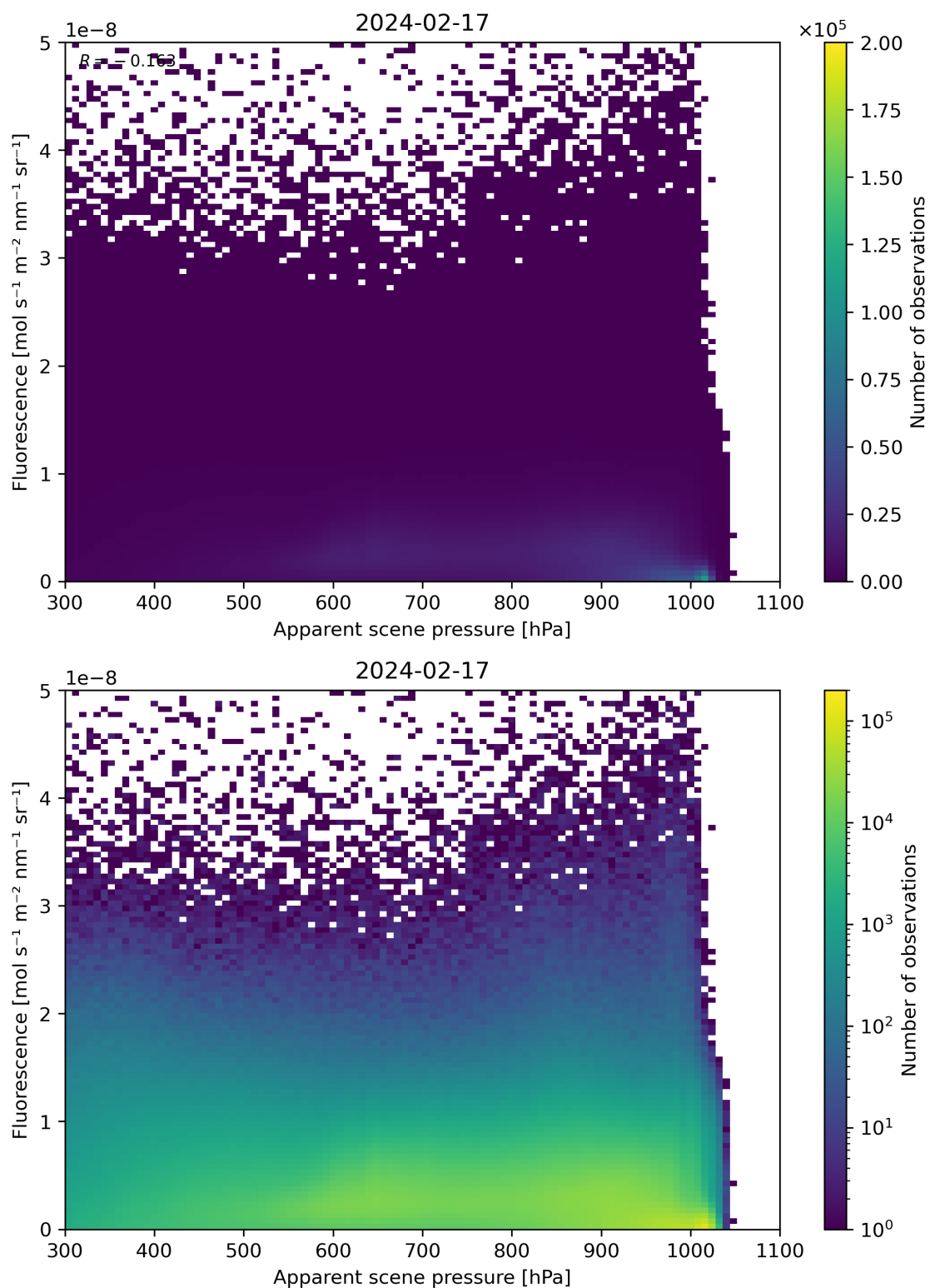
Figure 64: Scatter density plot of “Apparent scene pressure” against “Fluorescence” for 2024-02-17 to 2024-02-18.
