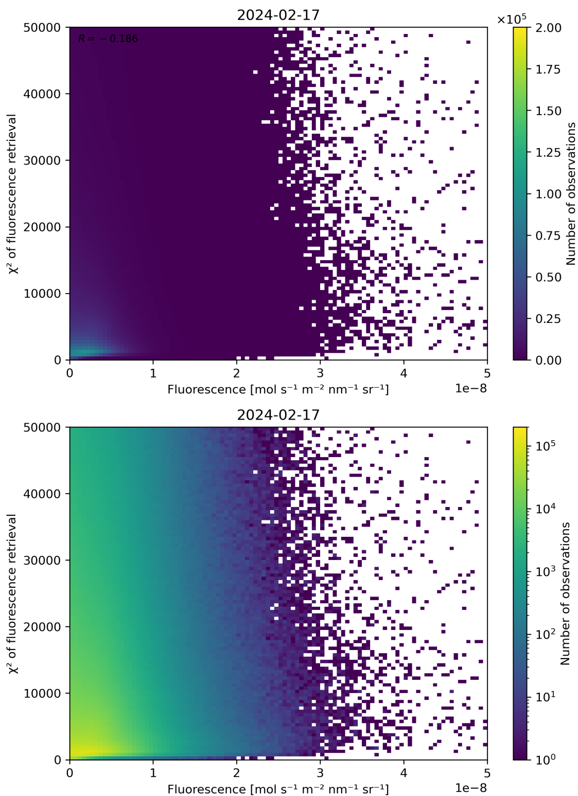
Figure 85: Scatter density plot of “Fluorescence” against “ \chi^2 of fluorescence retrieval” for 2024-02-17 to 2024-02-18.
