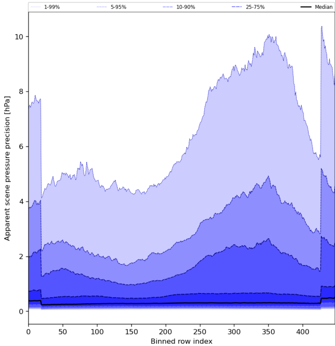
Figure 54: Along track statistics of “Apparent scene pressure precision” for 2024-02-17 to 2024-02-18
