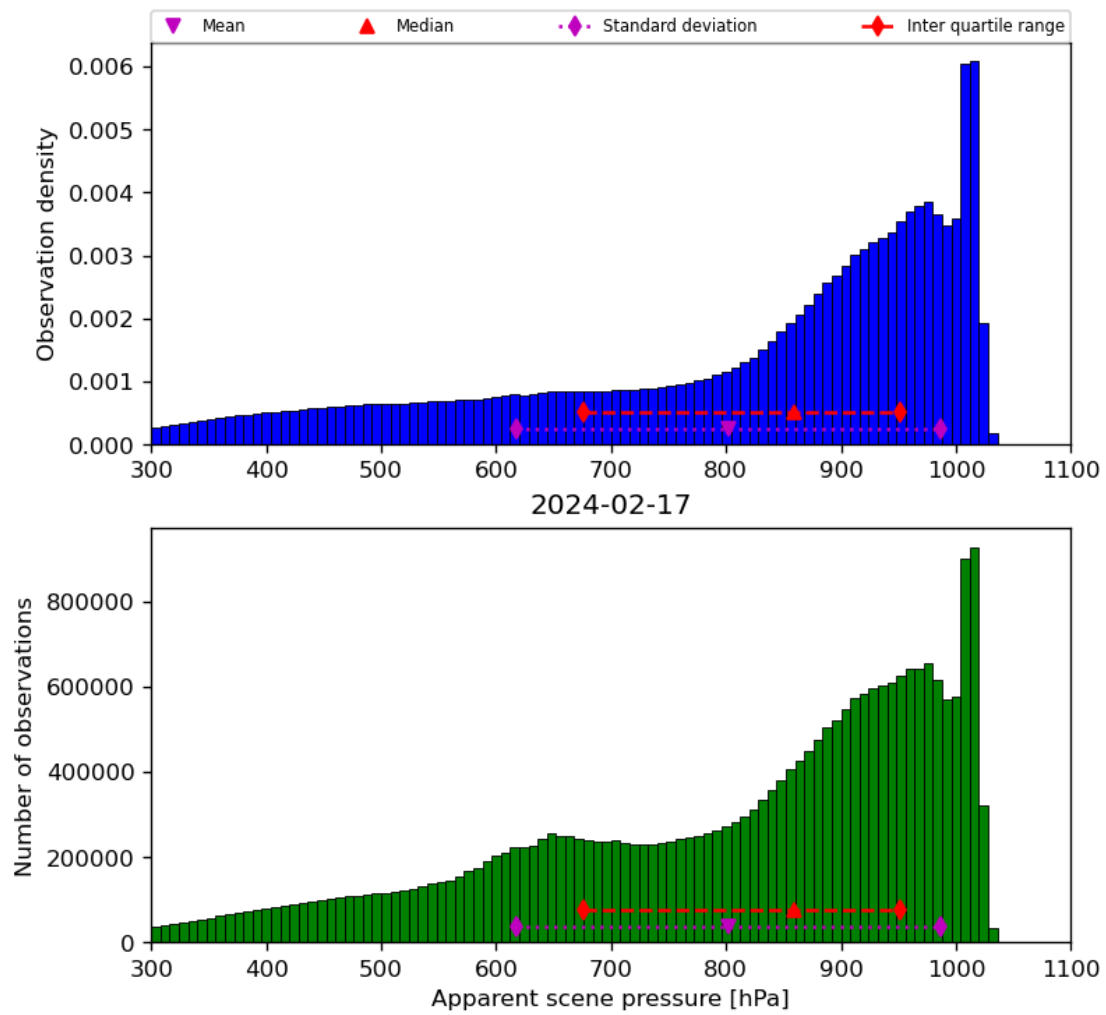
Figure 36: Histogram of “Apparent scene pressure” for 2024-02-17 to 2024-02-18
