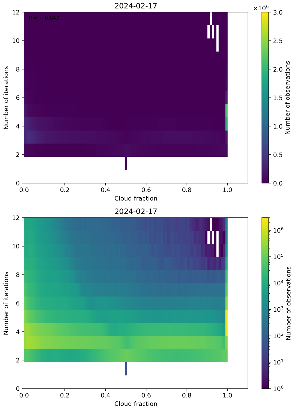
Figure 73: Scatter density plot of “Cloud fraction” against “Number of iterations” for 2024-02-17 to 2024-02-18.
