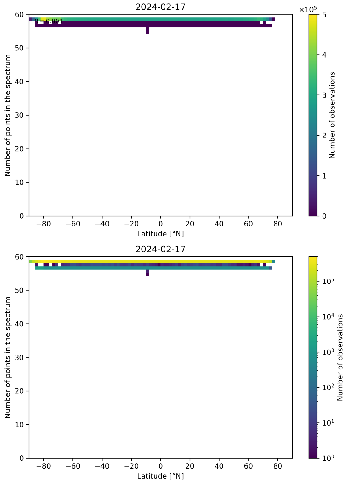
Figure 94: Scatter density plot of “Latitude” against “Number of points in the spectrum” for 2024-02-17 to 2024-02-18.
