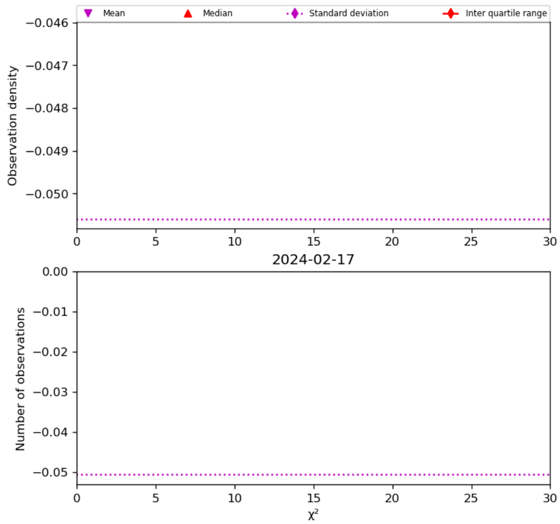
Figure 38: Histogram of “ \chi^2 ” for 2024-02-17 to 2024-02-18
