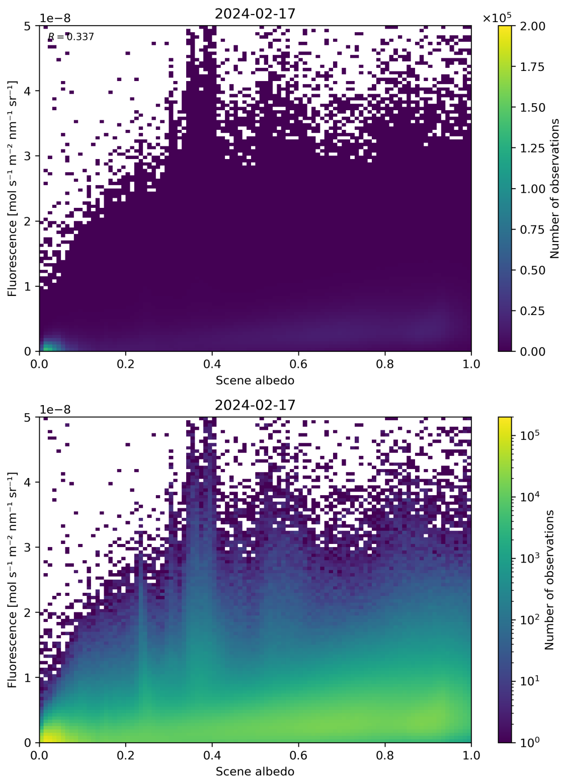
Figure 104: Scatter density plot of “Scene albedo” against “Fluorescence” for 2024-02-17 to 2024-02-18.
