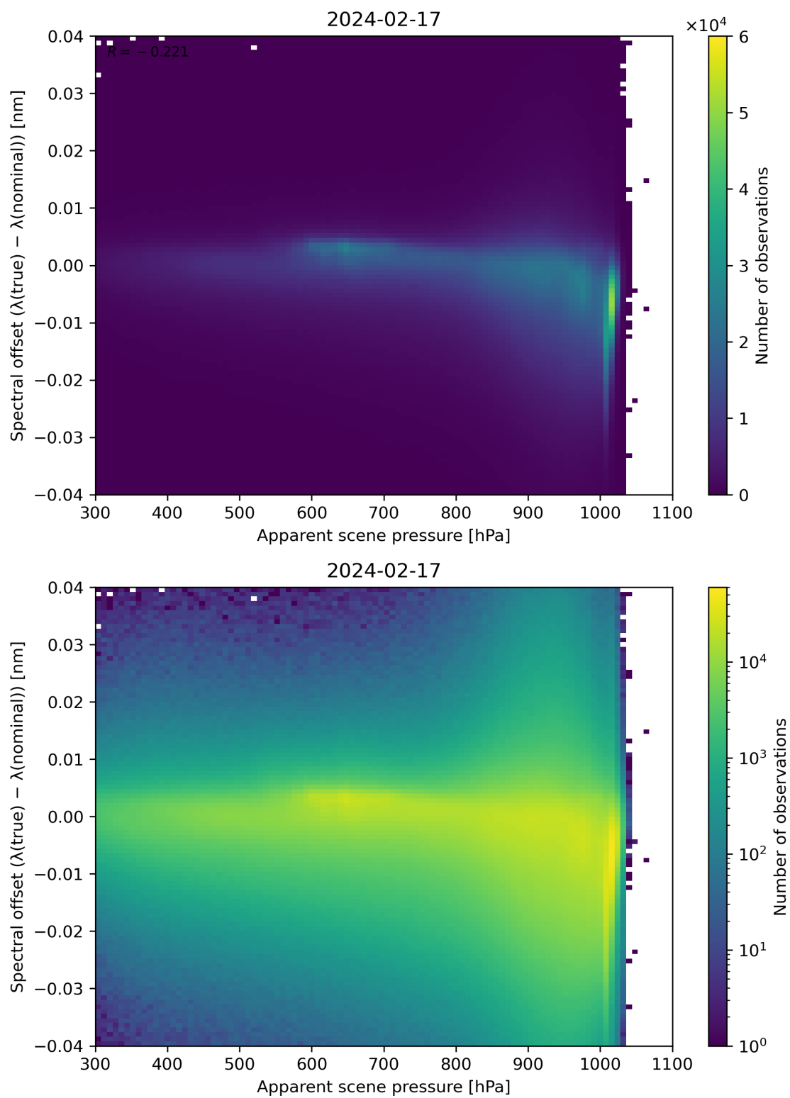
Figure 67: Scatter density plot of “Apparent scene pressure” against “Spectral offset ( \lambda(\text{true}) - \lambda(\text{nominal}) )” for 2024-02-17 to 2024-02-18.
