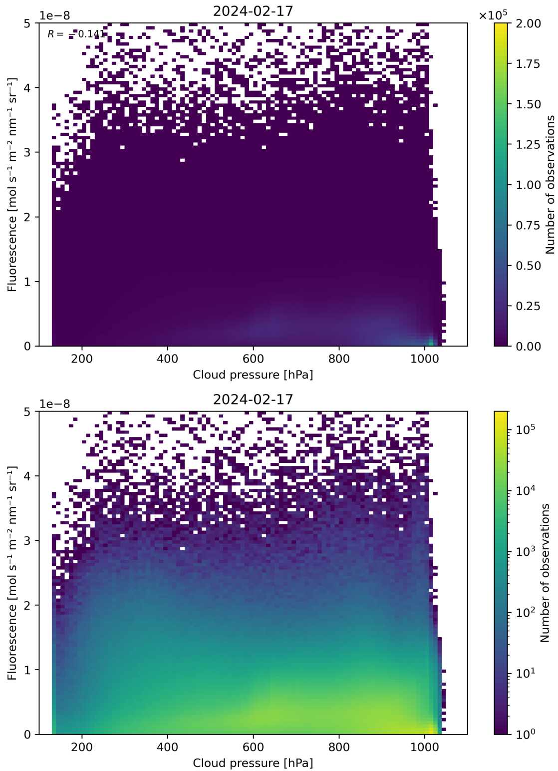
Figure 80: Scatter density plot of “Cloud pressure” against “Fluorescence” for 2024-02-17 to 2024-02-18.
