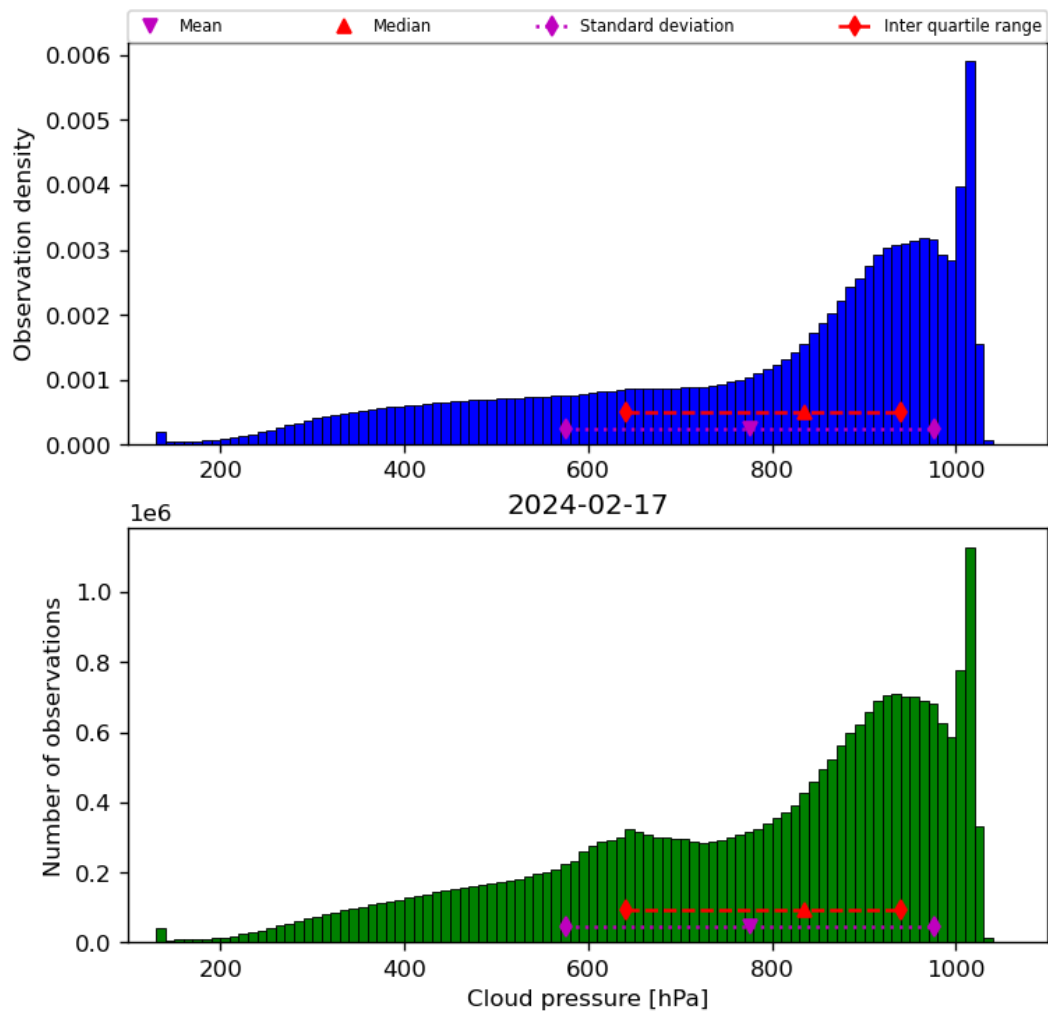
Figure 30: Histogram of “Cloud pressure” for 2024-02-17 to 2024-02-18
