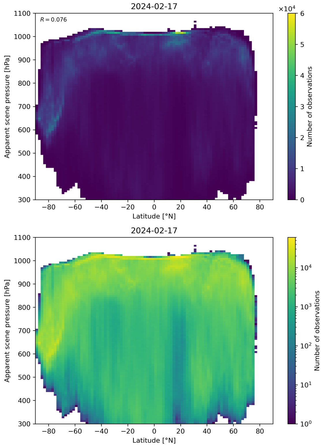
Figure 88: Scatter density plot of “Latitude” against “Apparent scene pressure” for 2024-02-17 to 2024-02-18.
