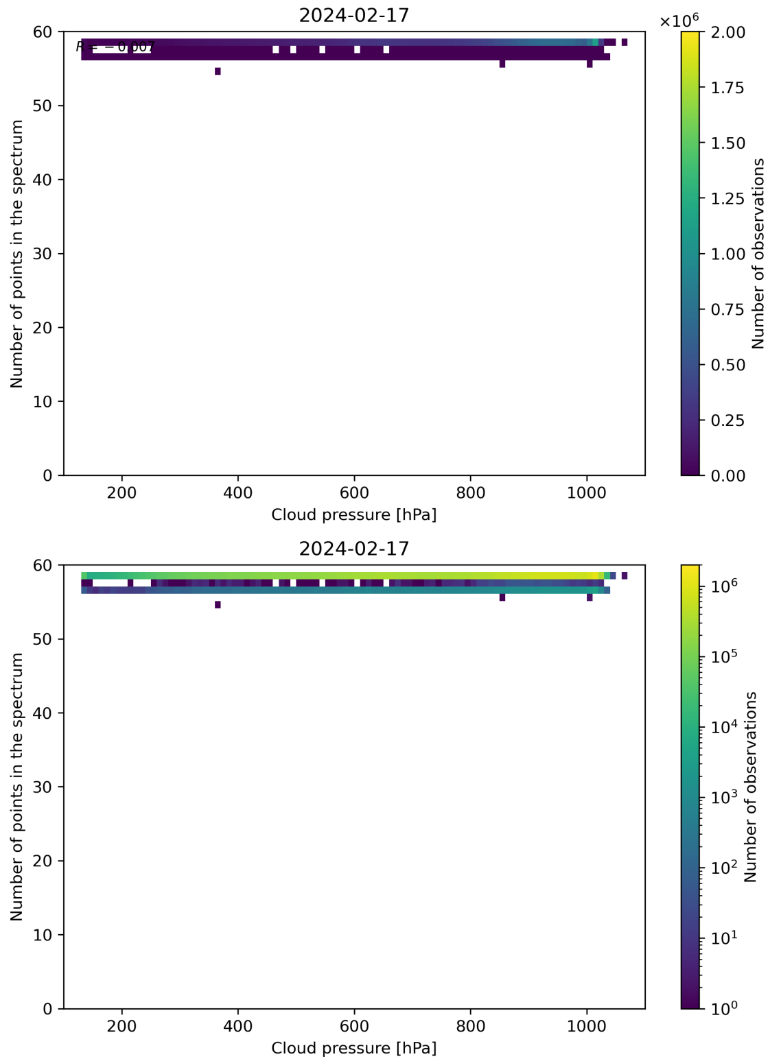
Figure 82: Scatter density plot of “Cloud pressure” against “Number of points in the spectrum” for 2024-02-17 to 2024-02-18.
