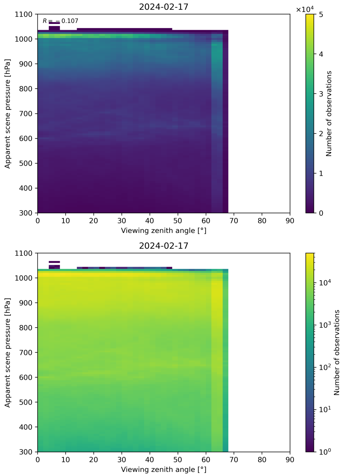
Figure 118: Scatter density plot of “Viewing zenith angle” against “Apparent scene pressure” for 2024-02-17 to 2024-02-18.
