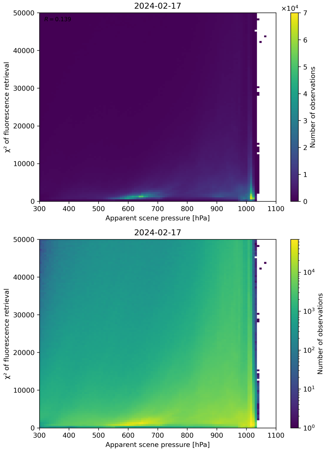
Figure 63: Scatter density plot of “Apparent scene pressure” against “ \chi^2 of fluorescence retrieval” for 2024-02-17 to 2024-02-18.
