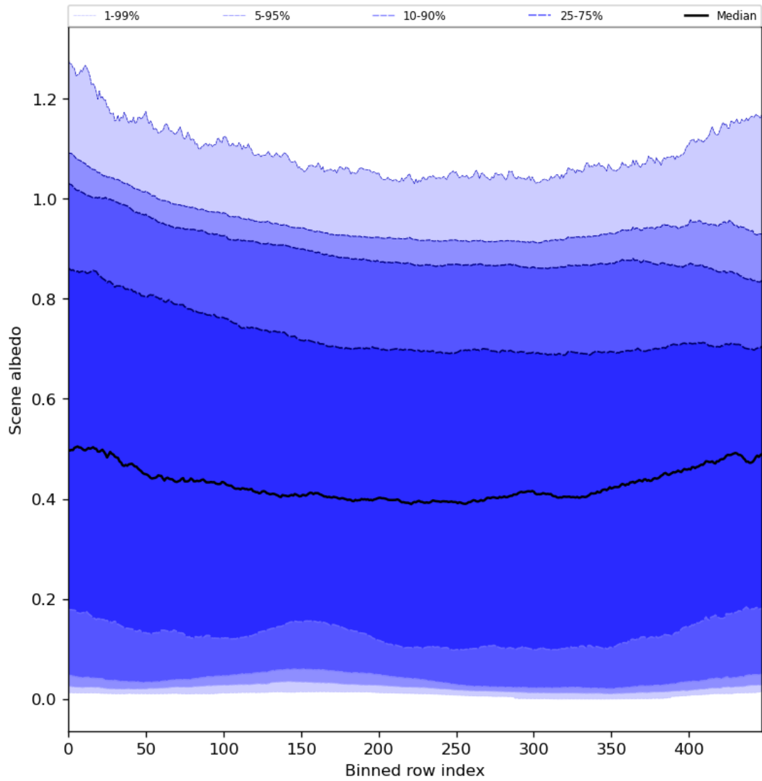
Figure 51: Along track statistics of “Scene albedo” for 2024-02-17 to 2024-02-18
