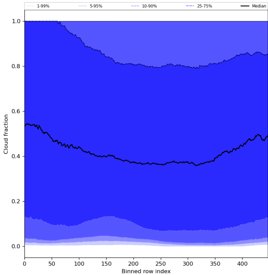
Figure 49: Along track statistics of “Cloud fraction” for 2024-02-17 to 2024-02-18
