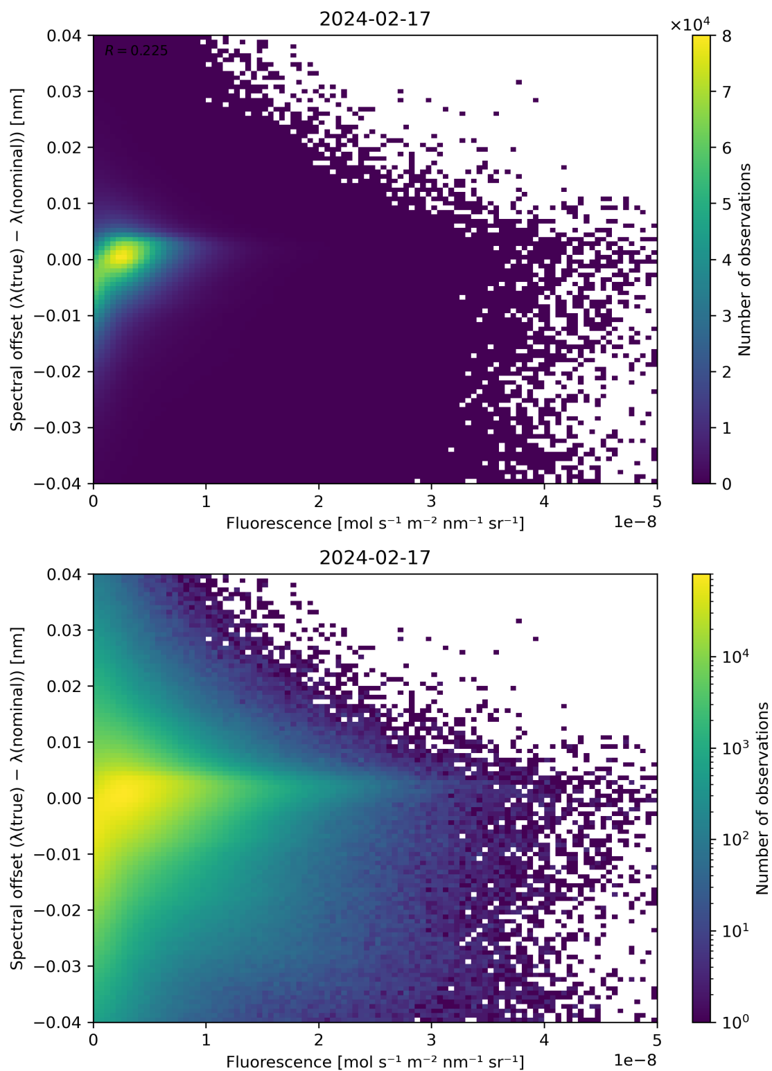
Figure 87: Scatter density plot of “Fluorescence” against “Spectral offset ( \lambda(\text{true}) - \lambda(\text{nominal}) )” for 2024-02-17 to 2024-02-18.
