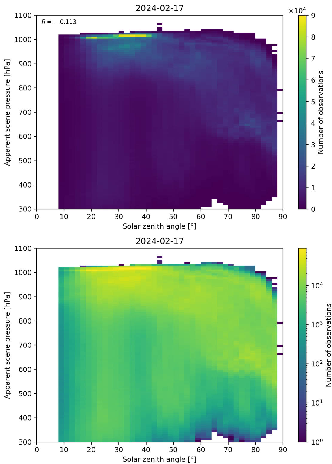
Figure 108: Scatter density plot of “Solar zenith angle” against “Apparent scene pressure” for 2024-02-17 to 2024-02-18.
