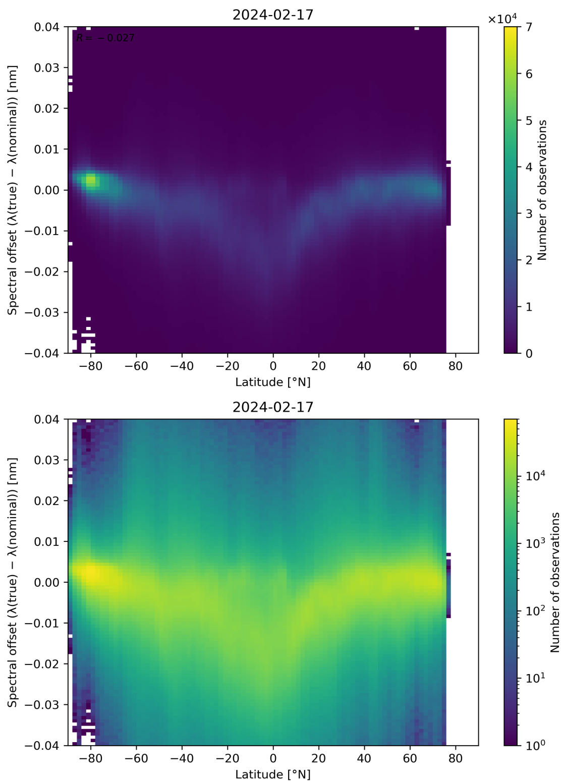
Figure 96: Scatter density plot of “Latitude” against “Spectral offset ( \lambda(\text{true}) - \lambda(\text{nominal}) )” for 2024-02-17 to 2024-02-18.
