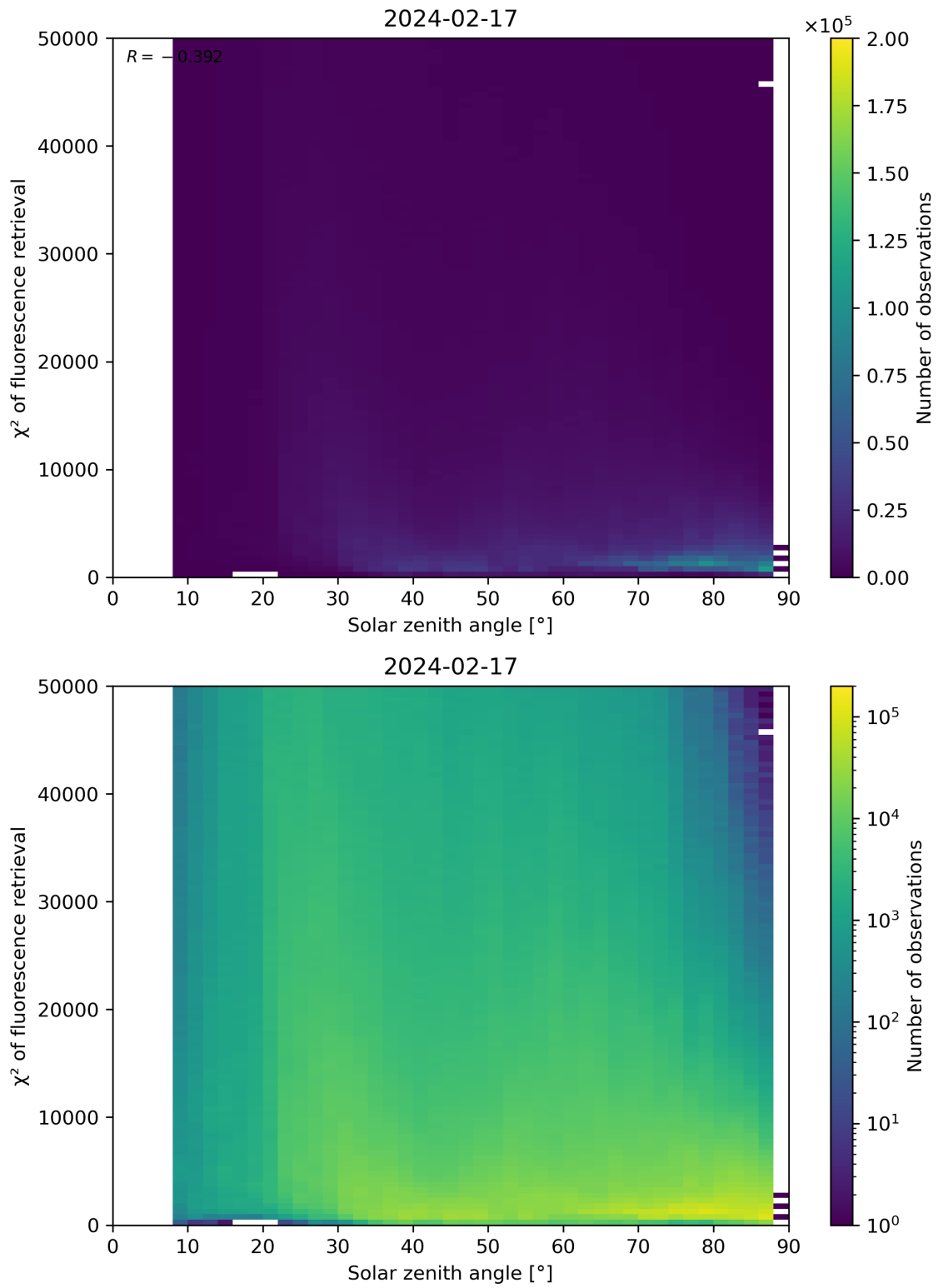
Figure 109: Scatter density plot of “Solar zenith angle” against “ \chi^2 of fluorescence retrieval” for 2024-02-17 to 2024-02-18.
