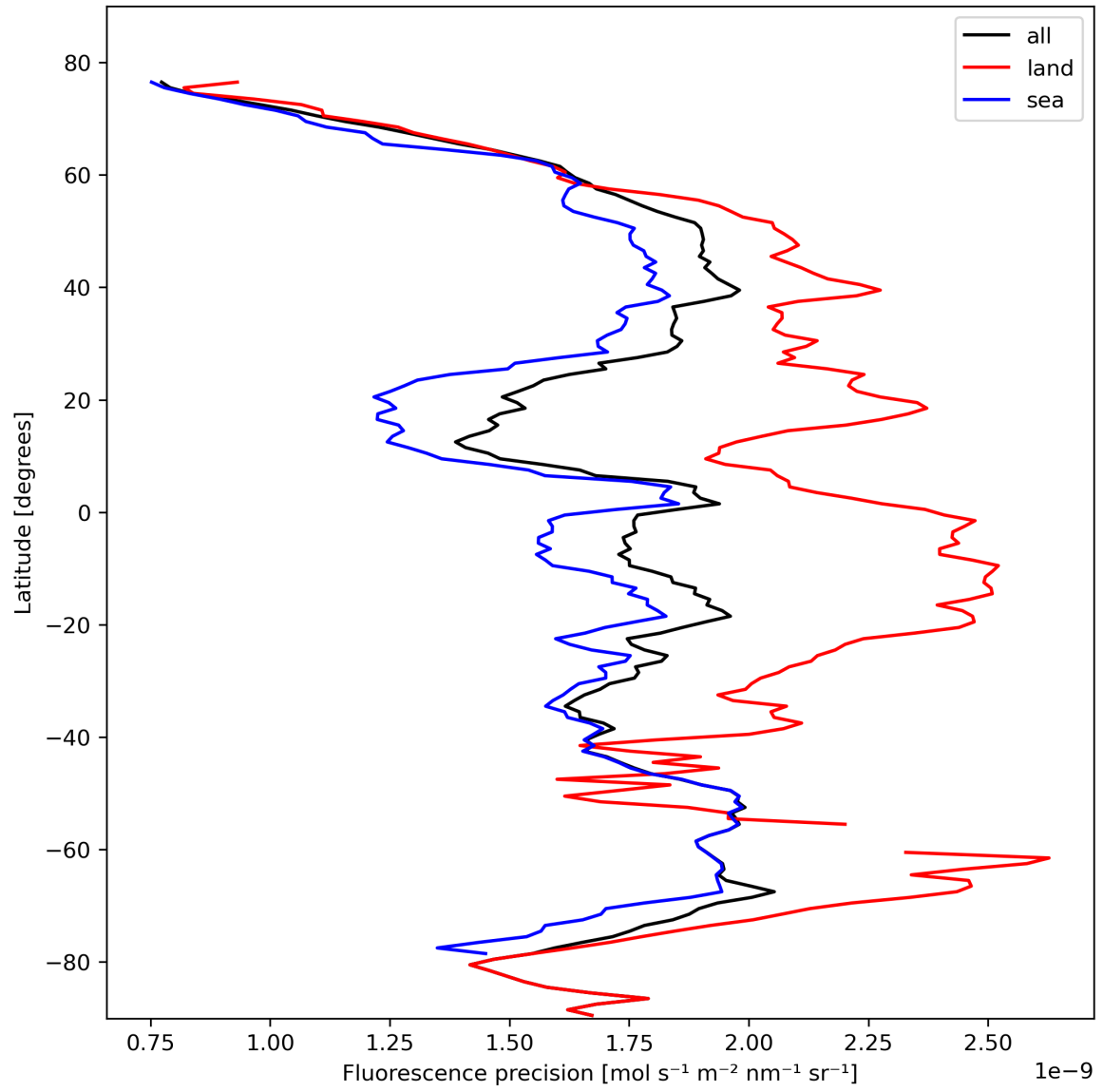
Figure 24: Zonal average of “Fluorescence precision” for 2024-02-17 to 2024-02-18.
