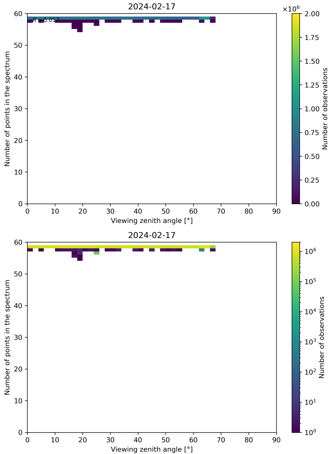
Figure 125: Scatter density plot of “Viewing zenith angle” against “Number of points in the spectrum” for 2024-02-17 to 2024-02-18.
