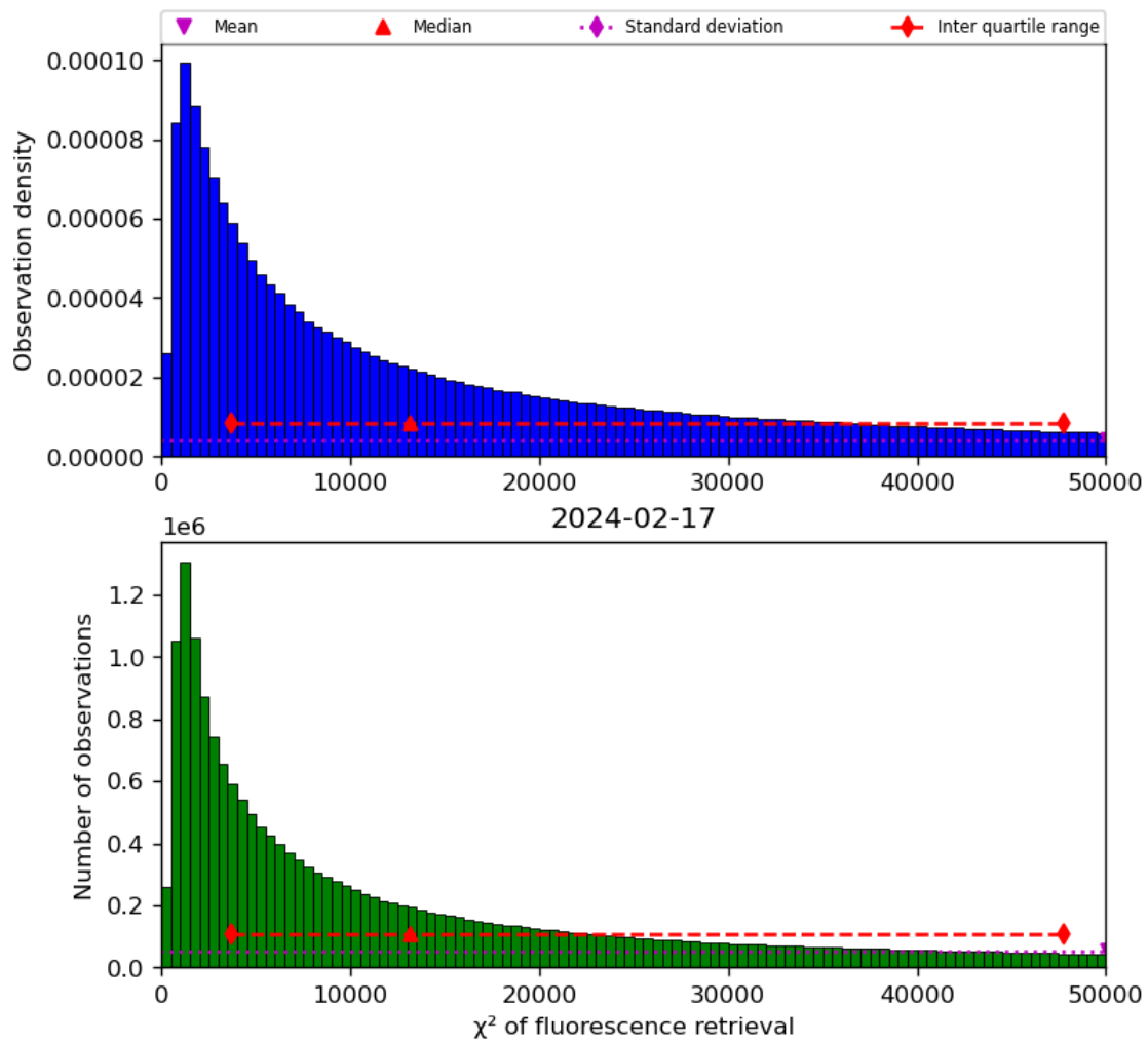
Figure 42: Histogram of “ \chi^2 of fluorescence retrieval” for 2024-02-17 to 2024-02-18
