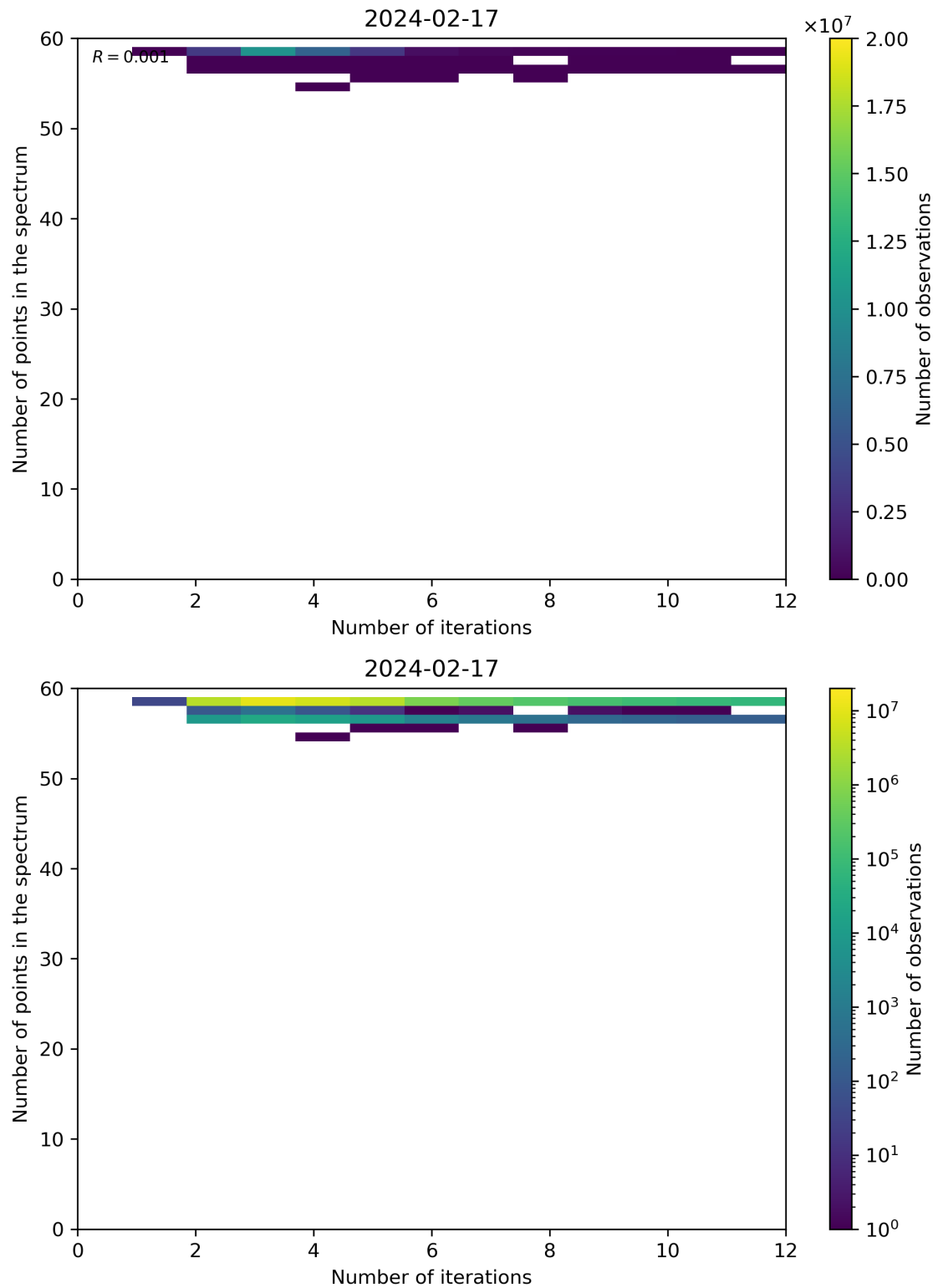
Figure 99: Scatter density plot of “Number of iterations” against “Number of points in the spectrum” for 2024-02-17 to 2024-02-18.
