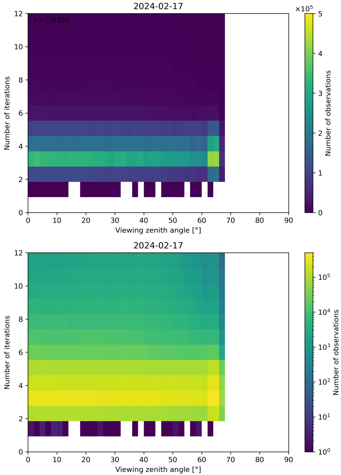
Figure 124: Scatter density plot of “Viewing zenith angle” against “Number of iterations” for 2024-02-17 to 2024-02-18.
