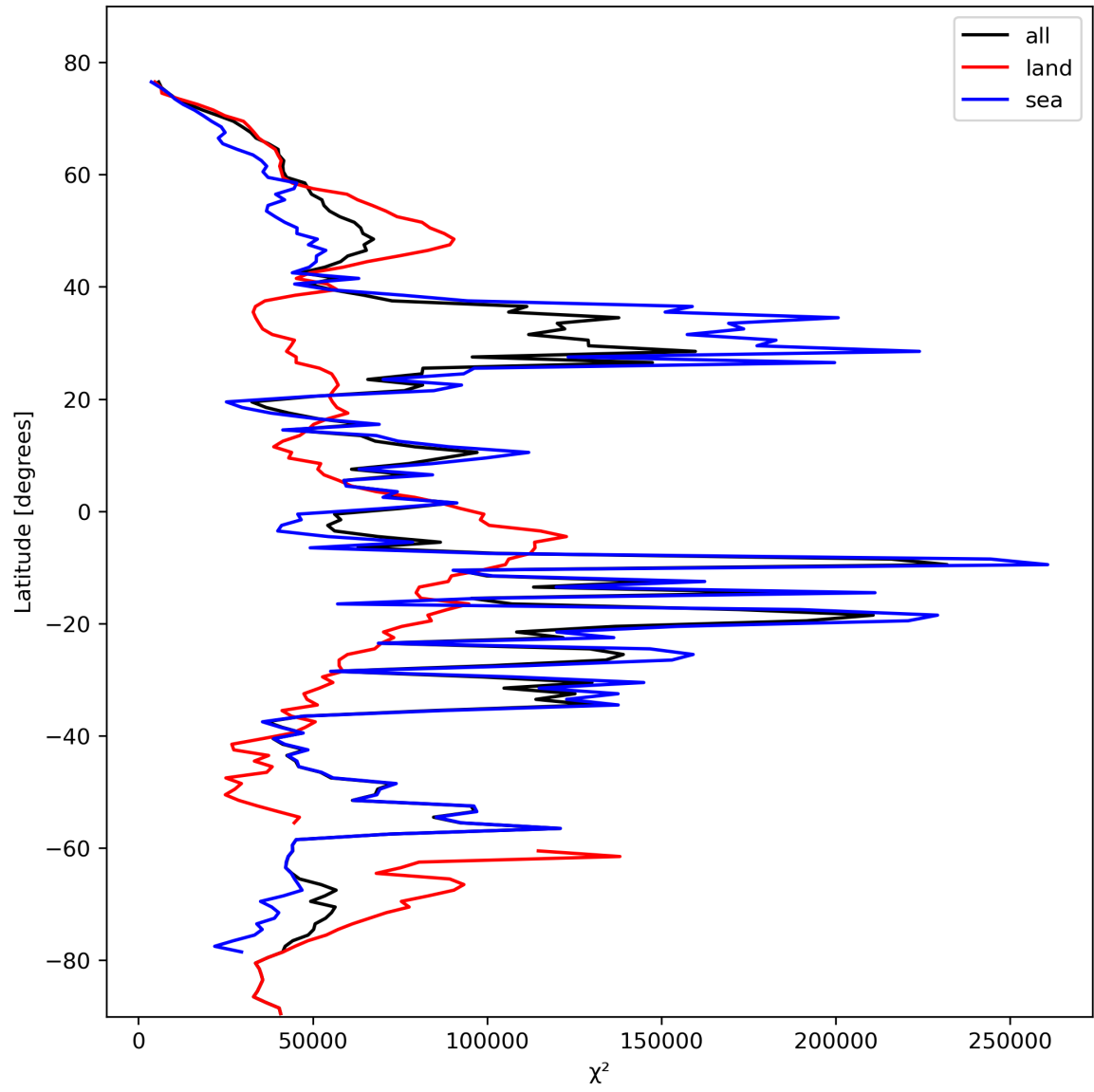
Figure 21: Zonal average of “ \chi^2 ” for 2024-02-17 to 2024-02-18.
