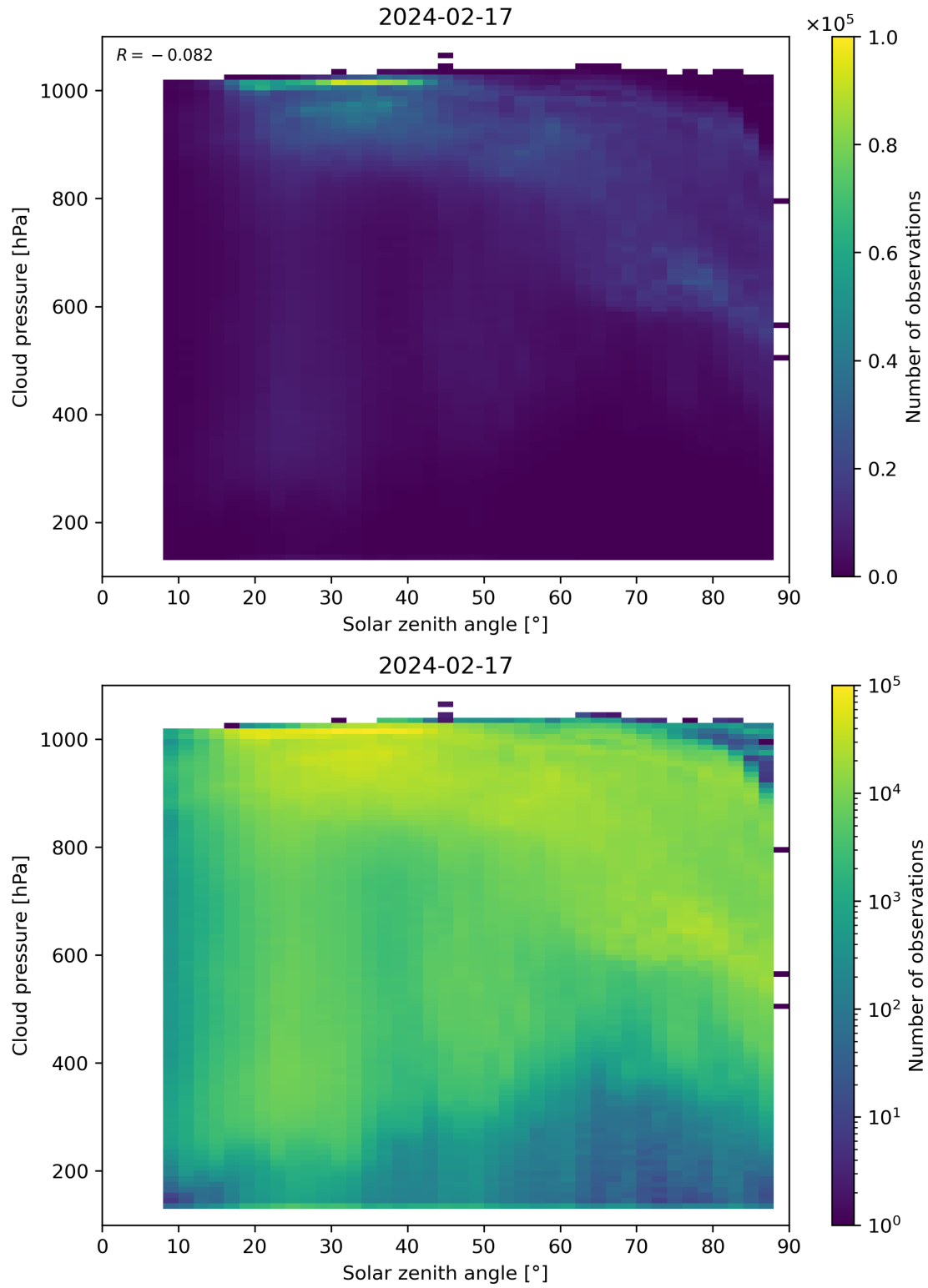
Figure 111: Scatter density plot of “Solar zenith angle” against “Cloud pressure” for 2024-02-17 to 2024-02-18.
