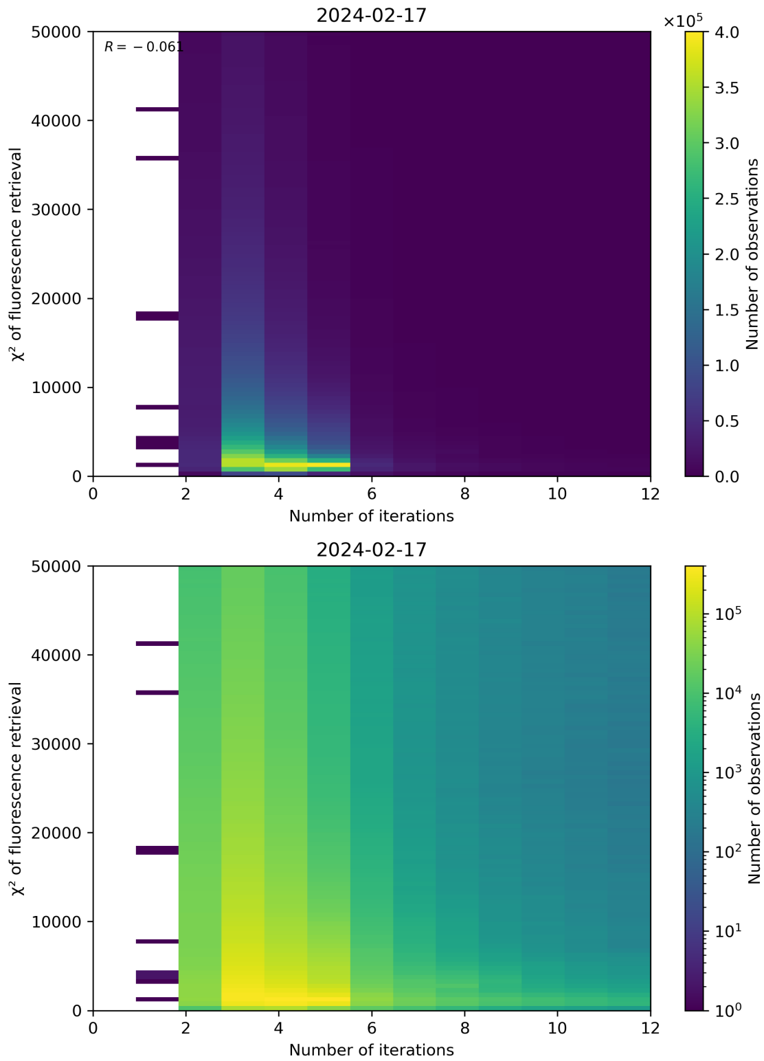
Figure 97: Scatter density plot of “Number of iterations” against “ \chi^2 of fluorescence retrieval” for 2024-02-17 to 2024-02-18.
