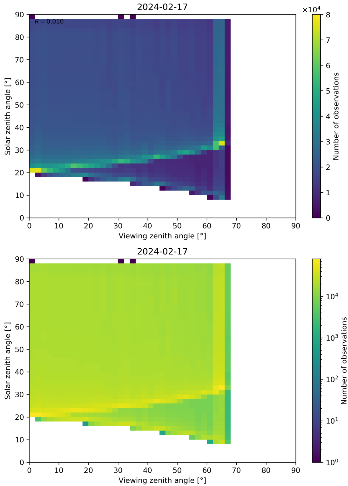
Figure 127: Scatter density plot of “Viewing zenith angle” against “Solar zenith angle” for 2024-02-17 to 2024-02-18.
