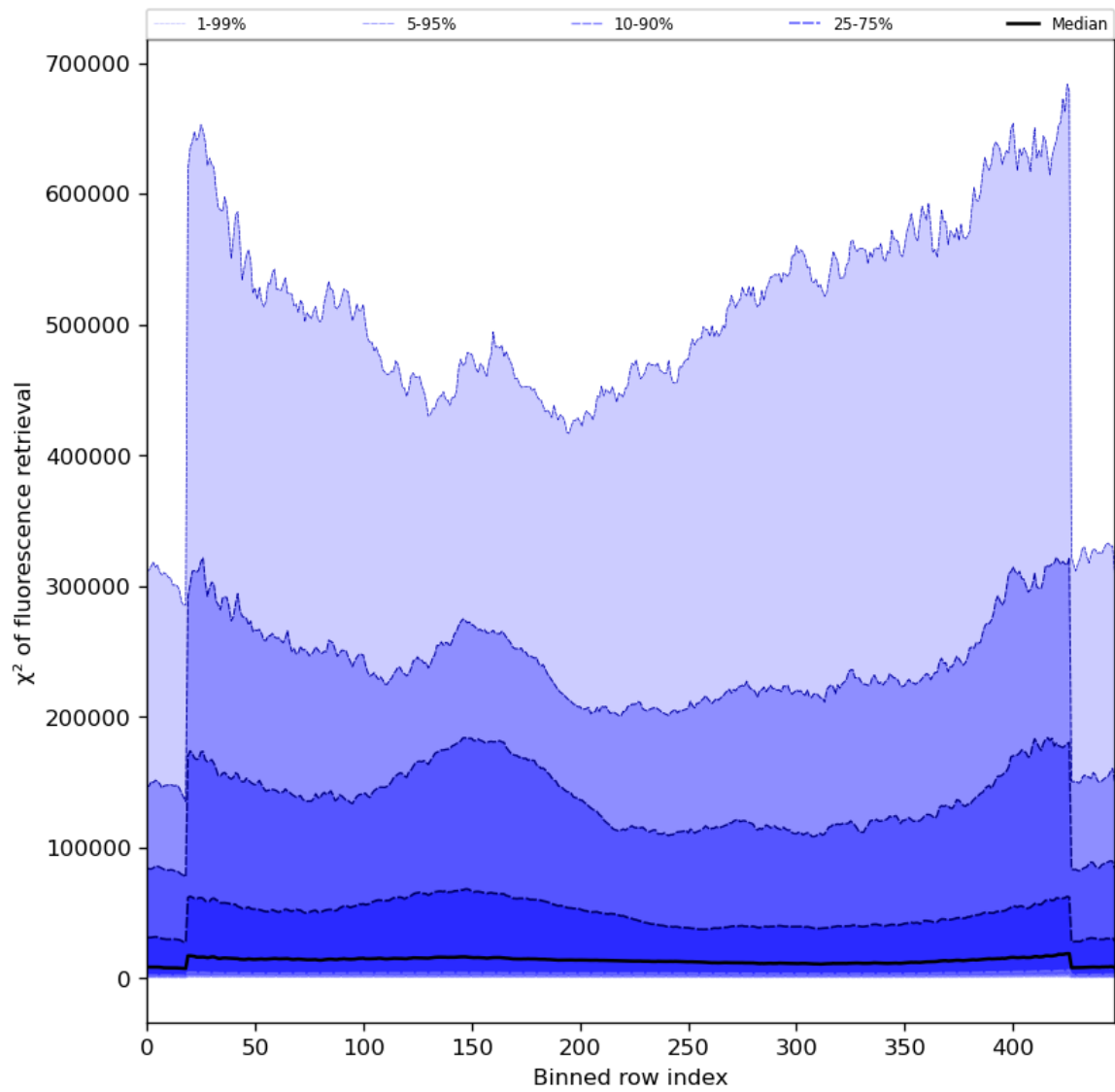
Figure 59: Along track statistics of “ \chi^2 of fluorescence retrieval” for 2024-02-17 to 2024-02-18
