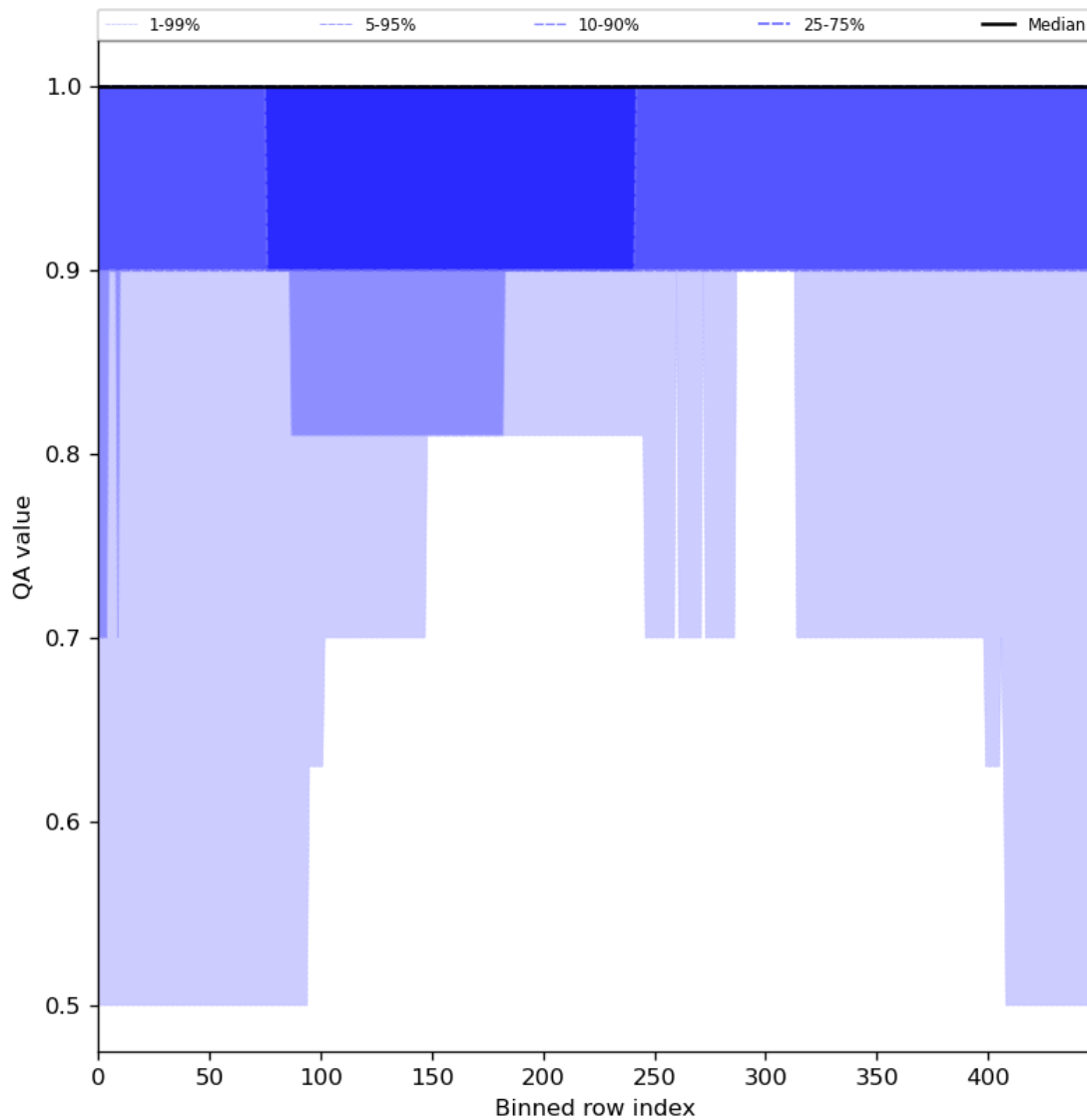
Figure 46: Along track statistics of “QA value” for 2024-02-17 to 2024-02-18
