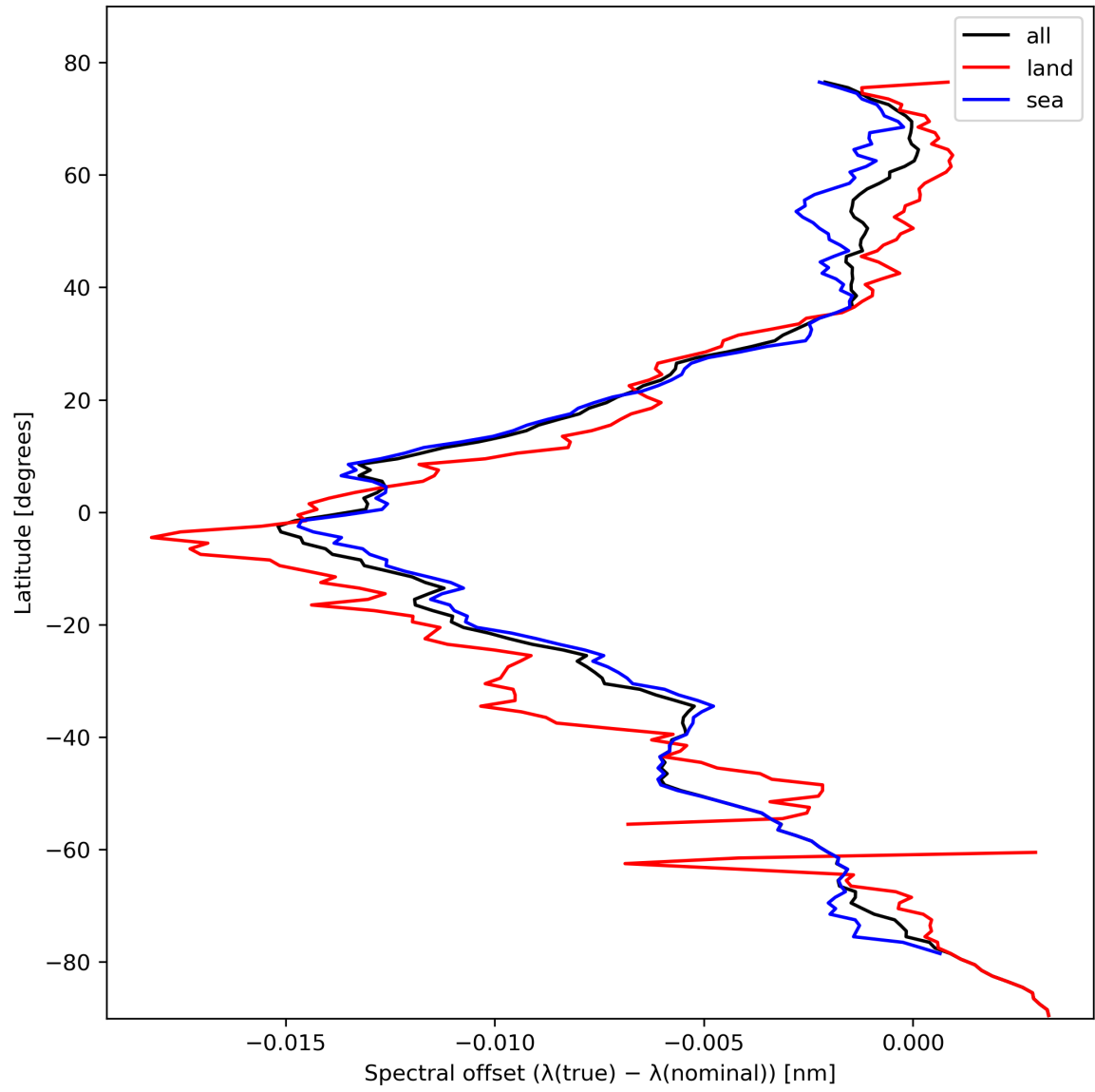
Figure 28: Zonal average of “Spectral offset ( \lambda(\text{true}) - \lambda(\text{nominal}) )” for 2024-02-17 to 2024-02-18.
