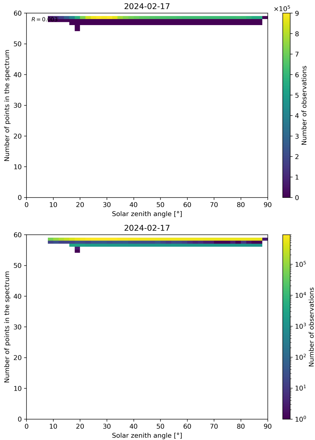
Figure 115: Scatter density plot of “Solar zenith angle” against “Number of points in the spectrum” for 2024-02-17 to 2024-02-18.
