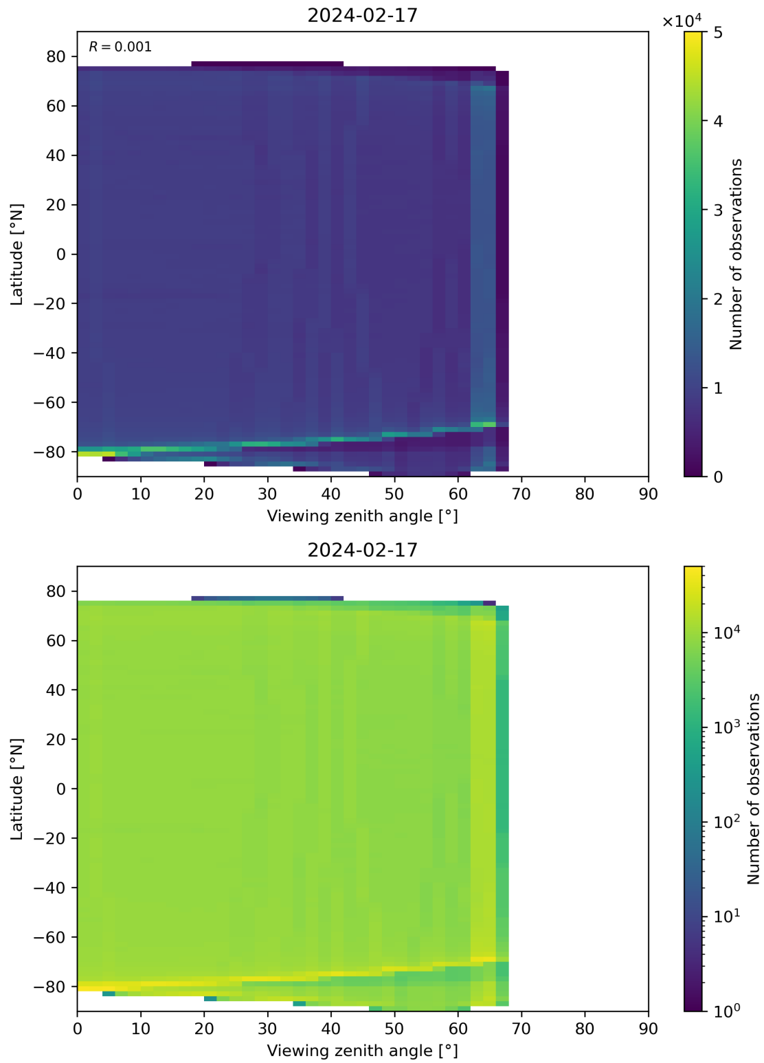
Figure 123: Scatter density plot of “Viewing zenith angle” against “Latitude” for 2024-02-17 to 2024-02-18.
