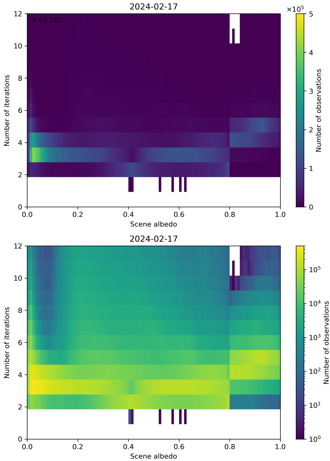
Figure 105: Scatter density plot of “Scene albedo” against “Number of iterations” for 2024-02-17 to 2024-02-18.
