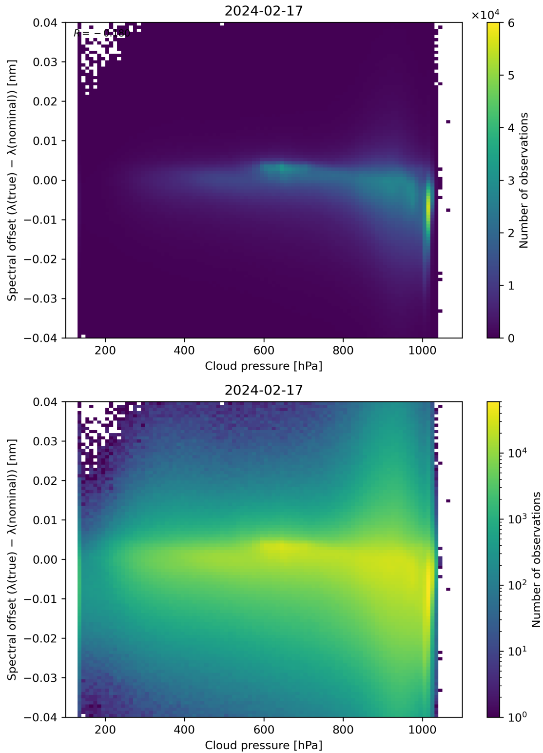
Figure 84: Scatter density plot of “Cloud pressure” against “Spectral offset ( \lambda(\text{true}) - \lambda(\text{nominal}) )” for 2024-02-17 to 2024-02-18.
