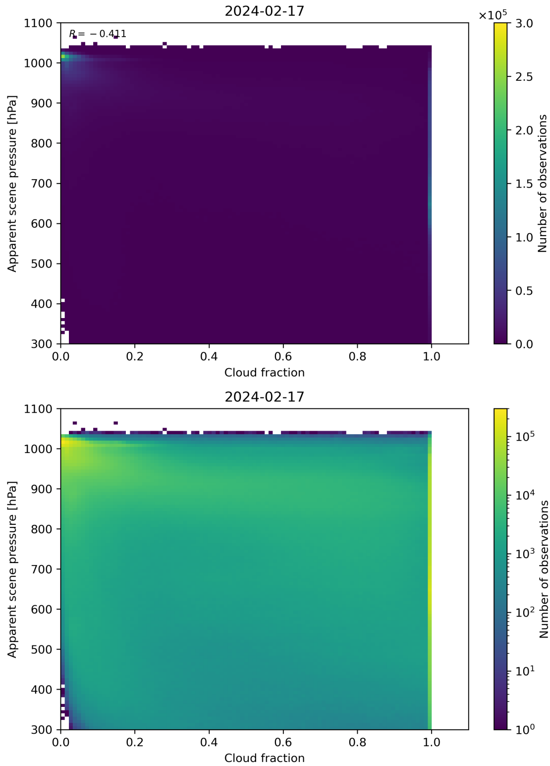
Figure 70: Scatter density plot of “Cloud fraction” against “Apparent scene pressure” for 2024-02-17 to 2024-02-18.
