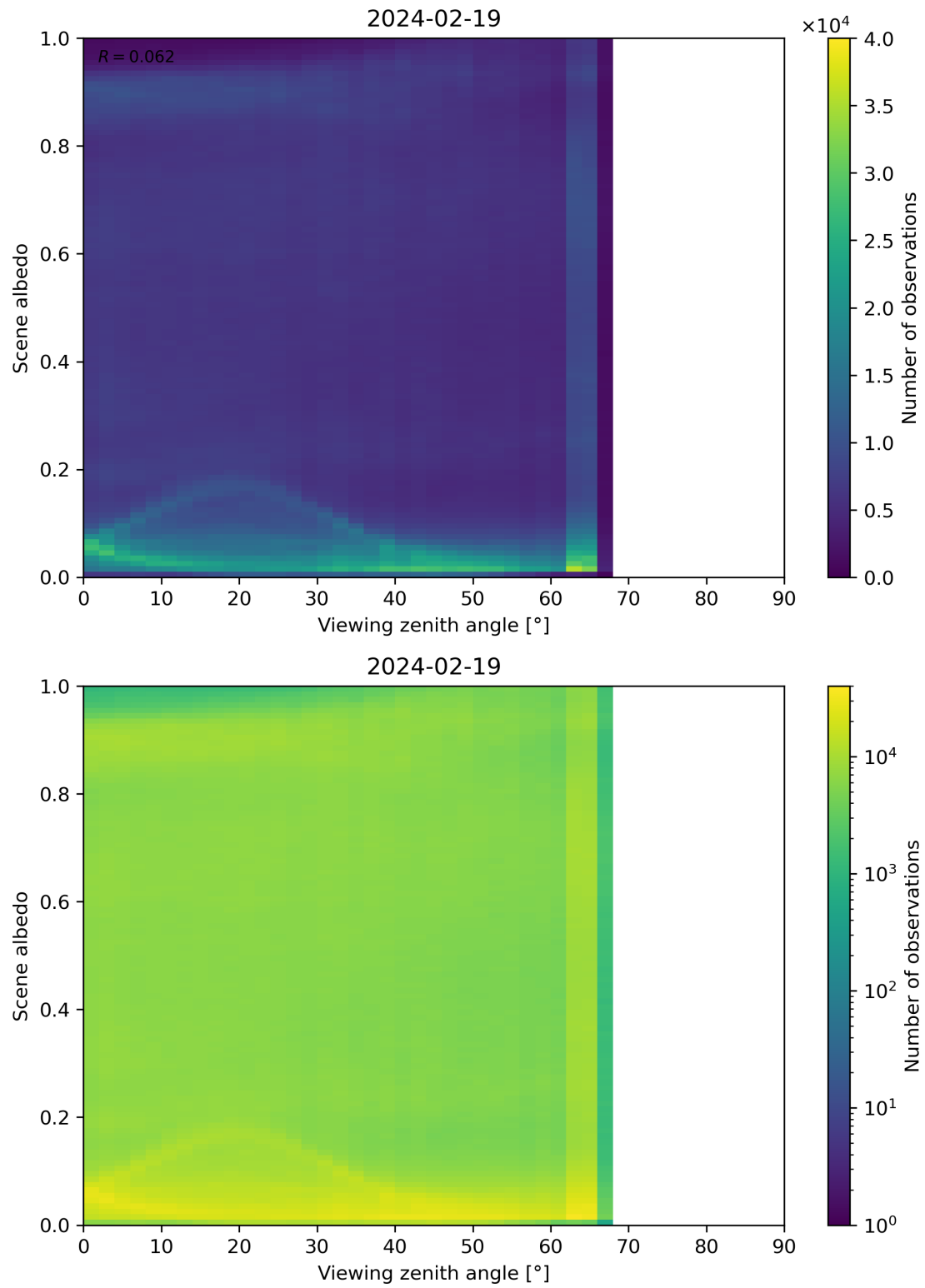
Figure 126: Scatter density plot of “Viewing zenith angle” against “Scene albedo” for 2024-02-18 to 2024-02-20.
