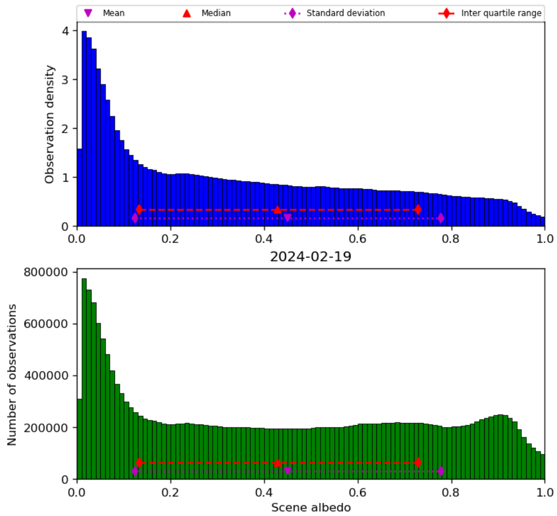
Figure 34: Histogram of “Scene albedo” for 2024-02-18 to 2024-02-20
