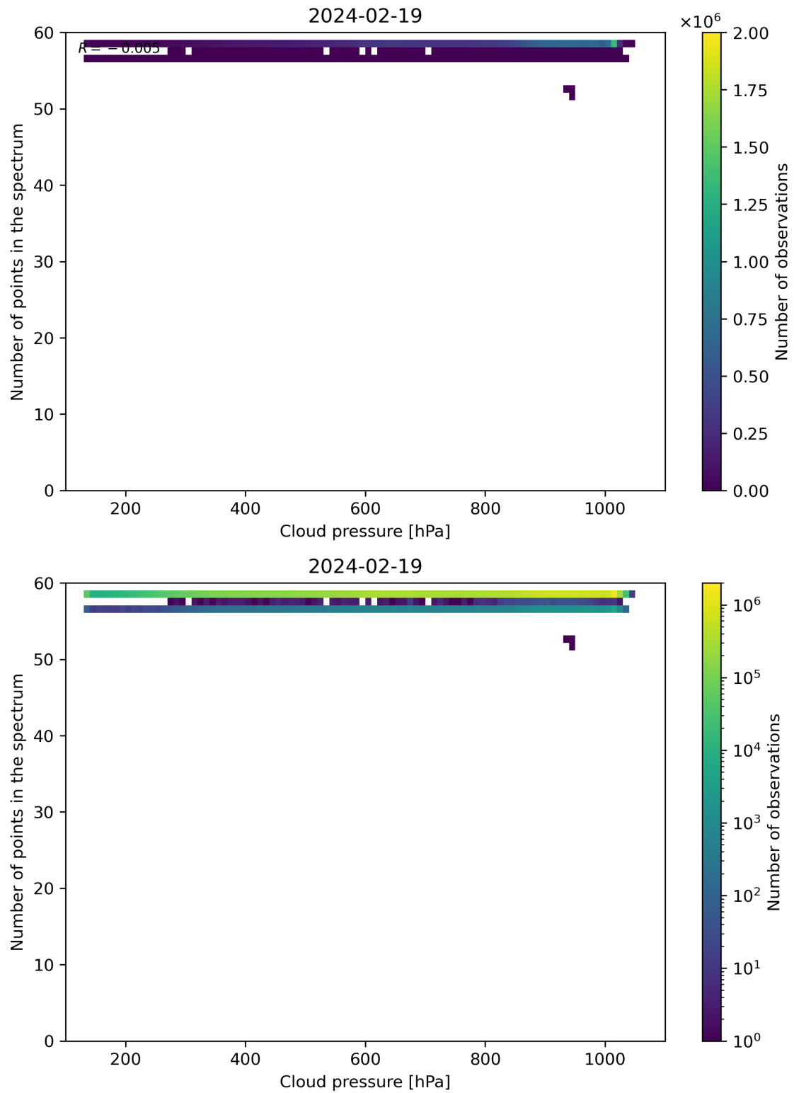
Figure 82: Scatter density plot of “Cloud pressure” against “Number of points in the spectrum” for 2024-02-18 to 2024-02-20.
