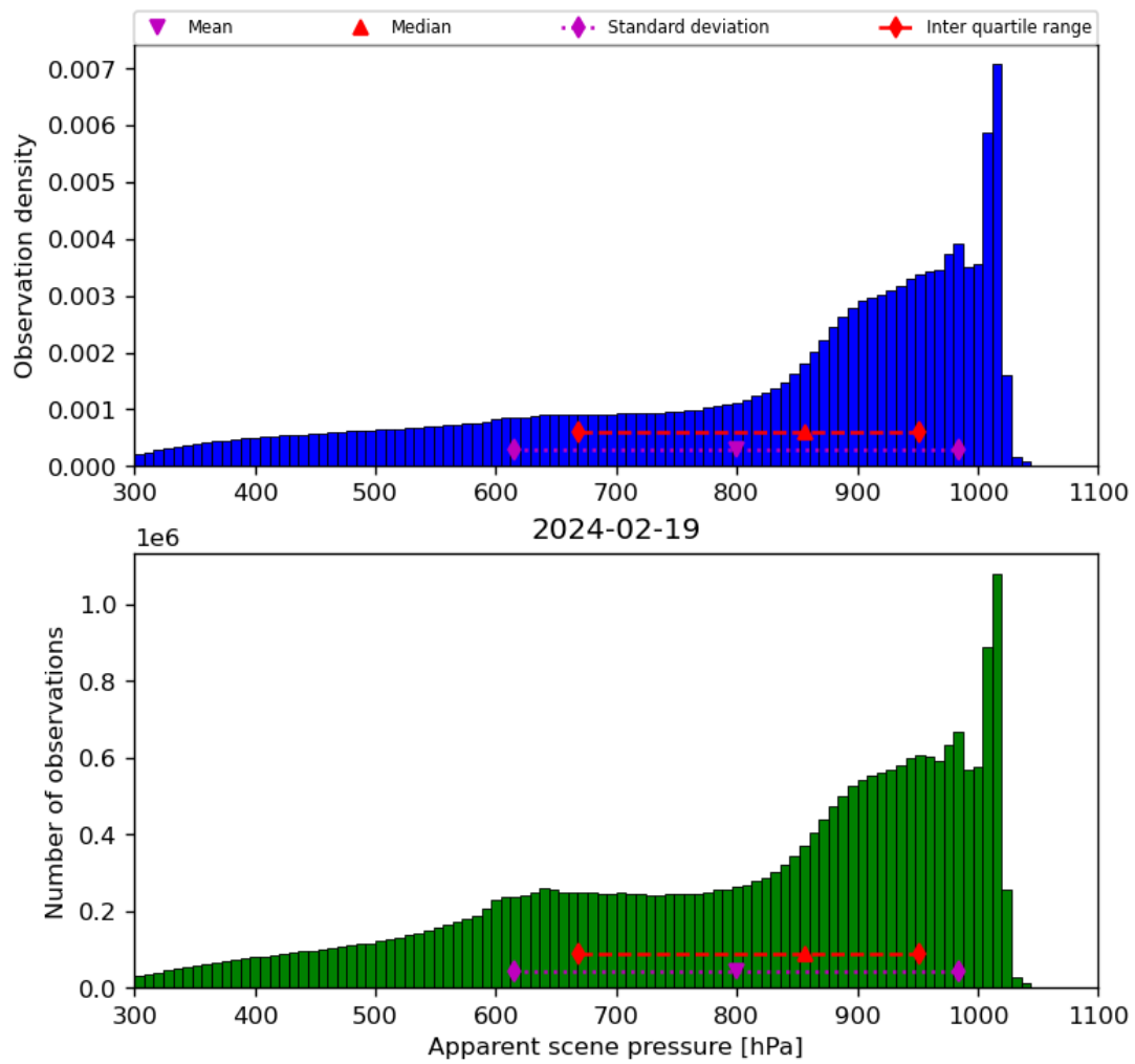
Figure 36: Histogram of “Apparent scene pressure” for 2024-02-18 to 2024-02-20
