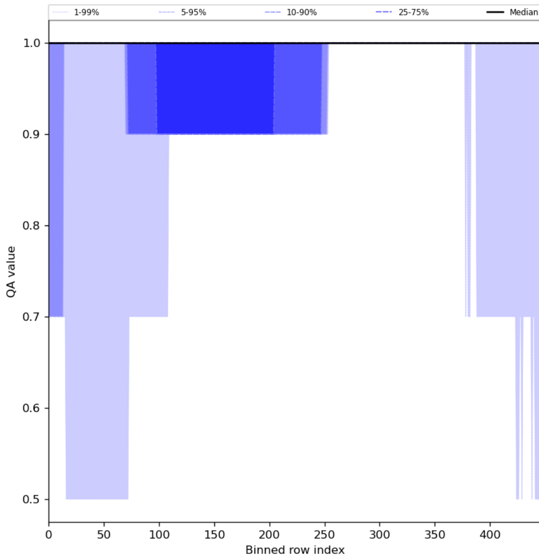
Figure 46: Along track statistics of “QA value” for 2024-02-18 to 2024-02-20
