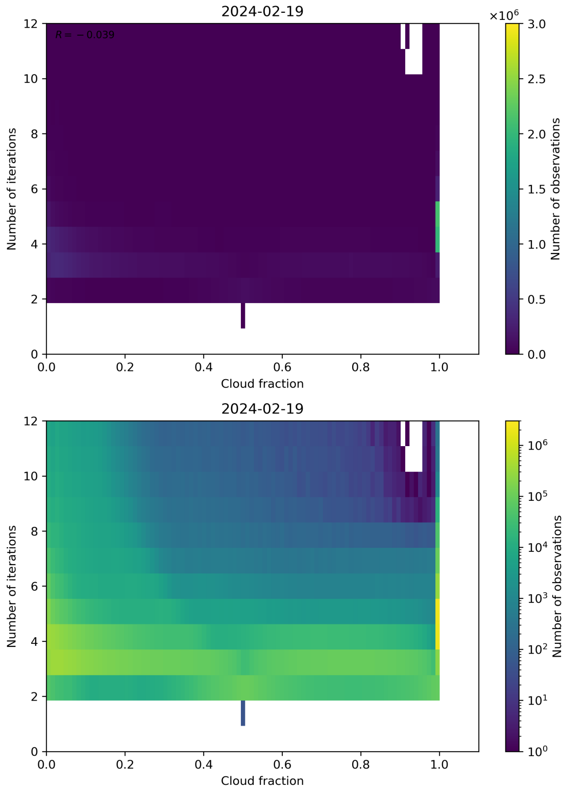
Figure 73: Scatter density plot of “Cloud fraction” against “Number of iterations” for 2024-02-18 to 2024-02-20.
