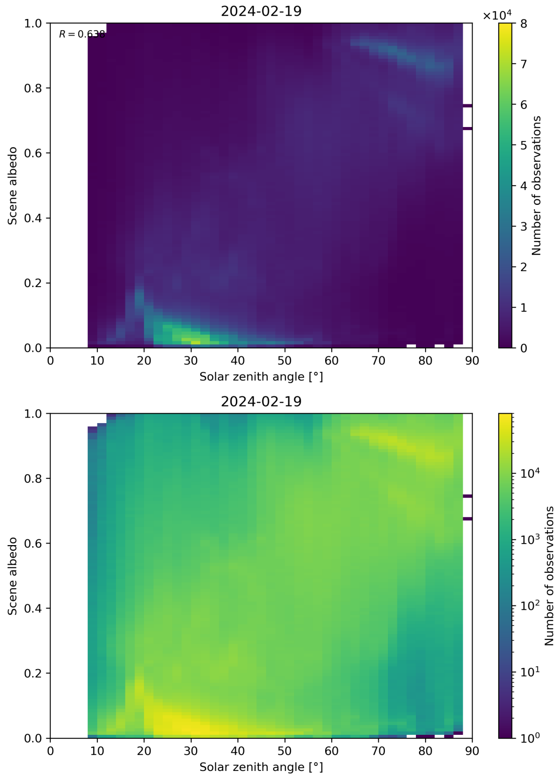
Figure 116: Scatter density plot of “Solar zenith angle” against “Scene albedo” for 2024-02-18 to 2024-02-20.
