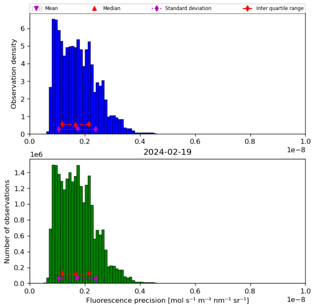
Figure 41: Histogram of “Fluorescence precision” for 2024-02-18 to 2024-02-20
