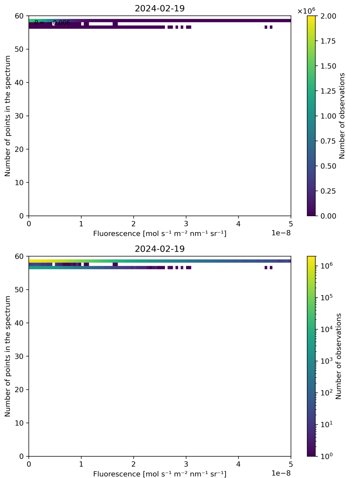
Figure 86: Scatter density plot of “Fluorescence” against “Number of points in the spectrum” for 2024-02-18 to 2024-02-20.
