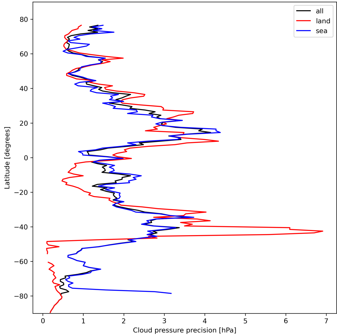
Figure 14: Zonal average of “Cloud pressure precision” for 2024-02-18 to 2024-02-20.
