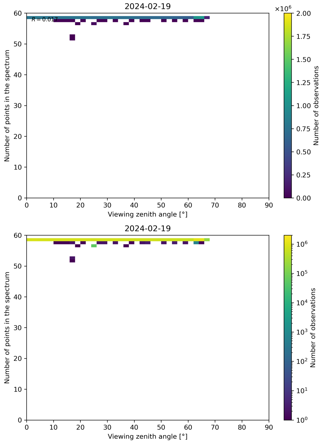
Figure 125: Scatter density plot of “Viewing zenith angle” against “Number of points in the spectrum” for 2024-02-18 to 2024-02-20.
