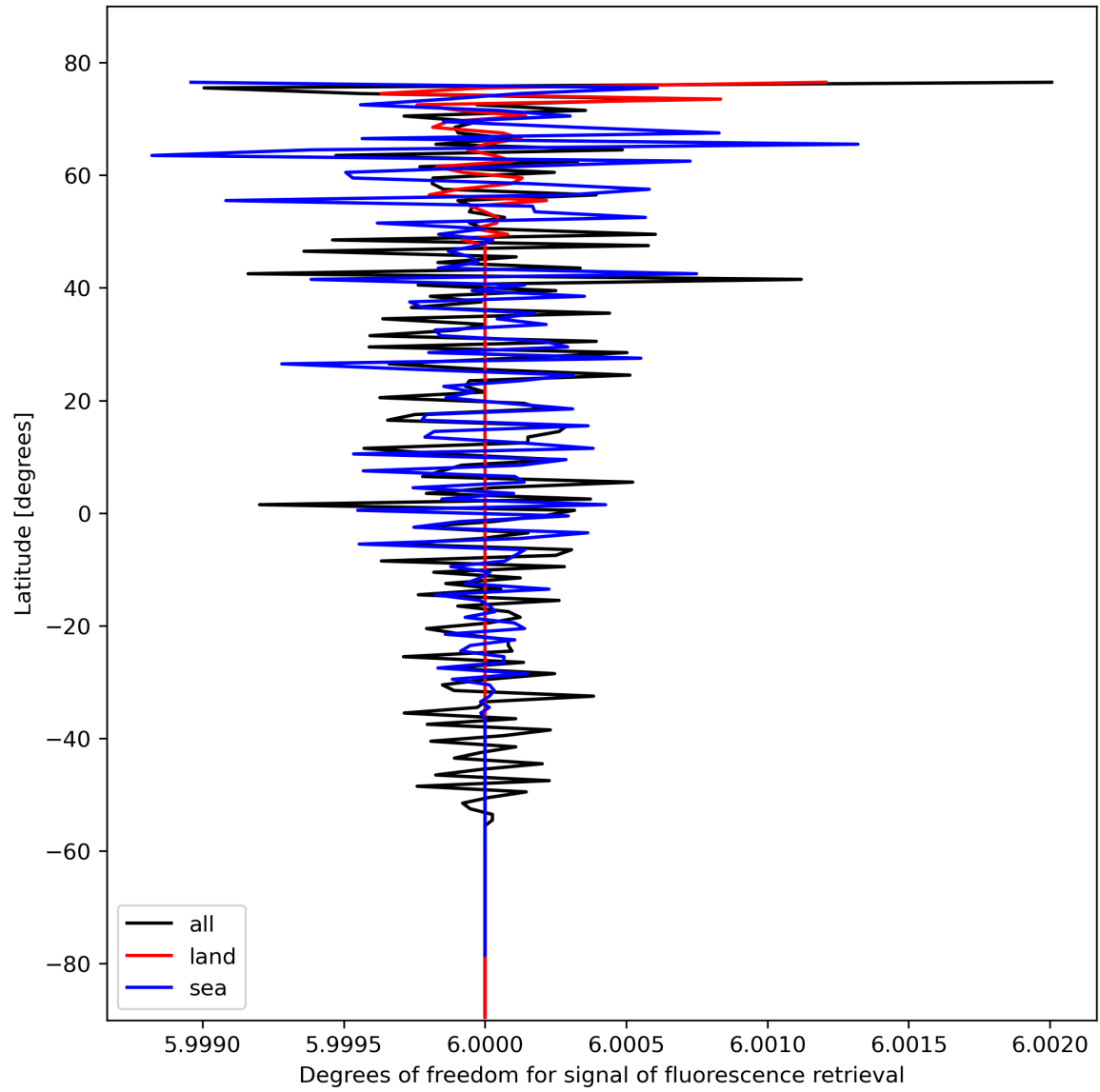
Figure 26: Zonal average of “Degrees of freedom for signal of fluorescence retrieval” for 2024-02-18 to 2024-02-20.
