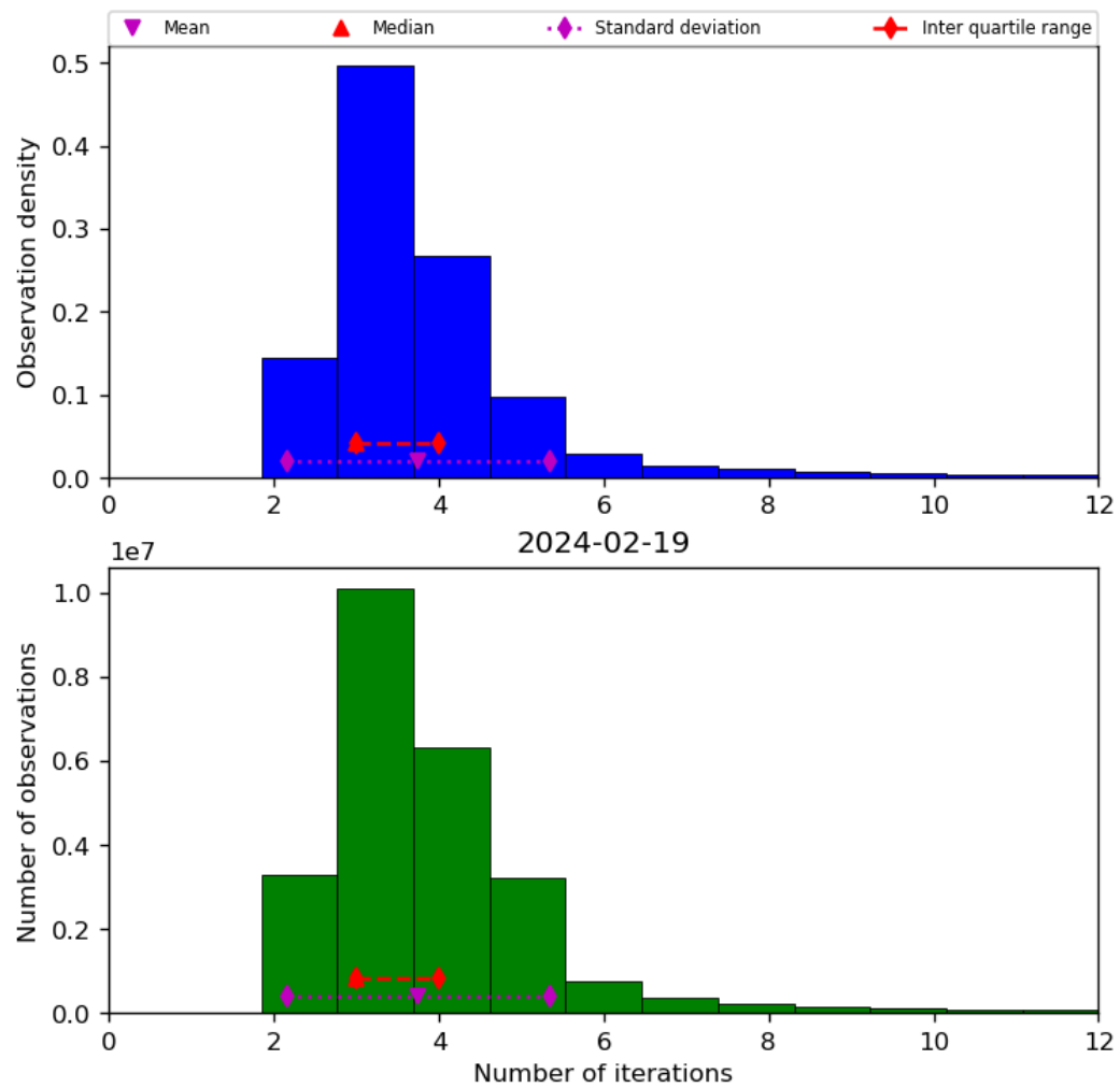
Figure 39: Histogram of “Number of iterations” for 2024-02-18 to 2024-02-20
