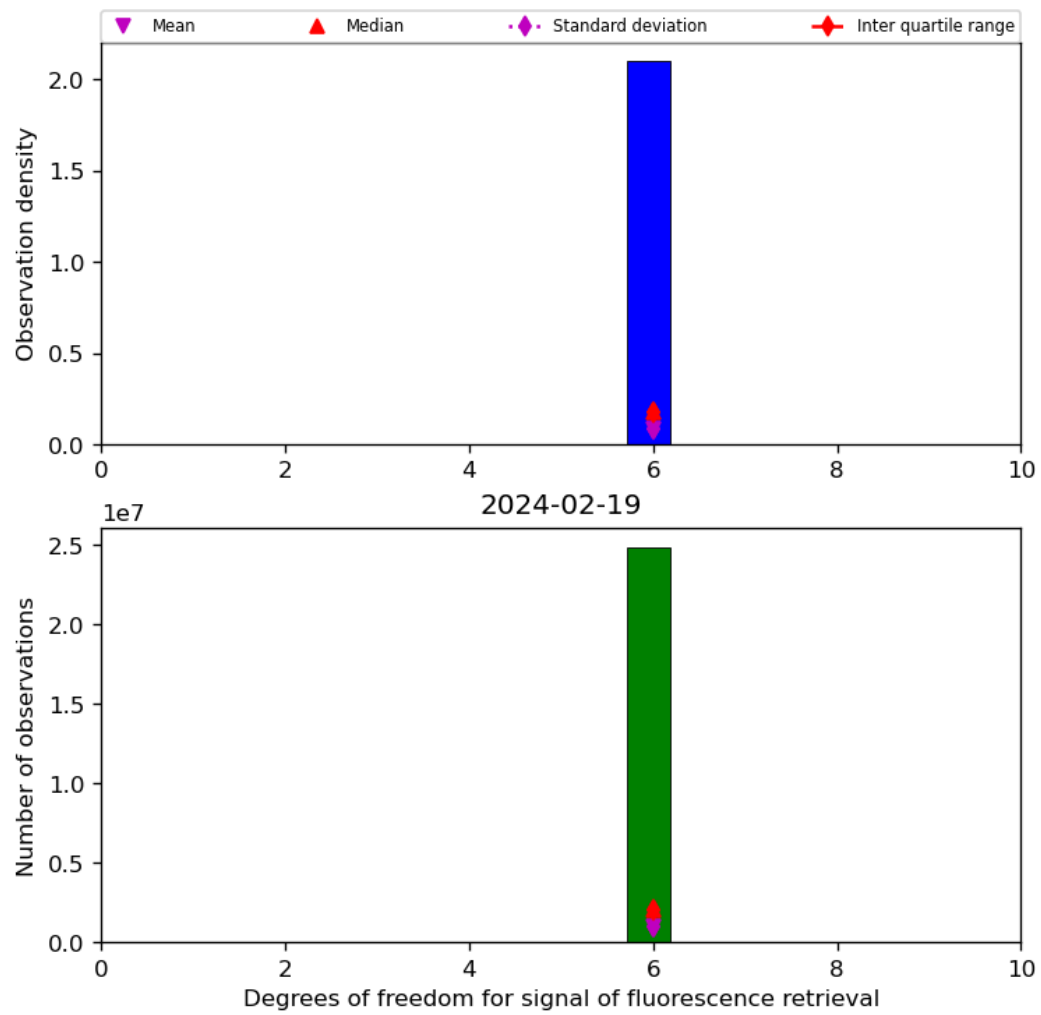
Figure 43: Histogram of “Degrees of freedom for signal of fluorescence retrieval” for 2024-02-18 to 2024-02-20
