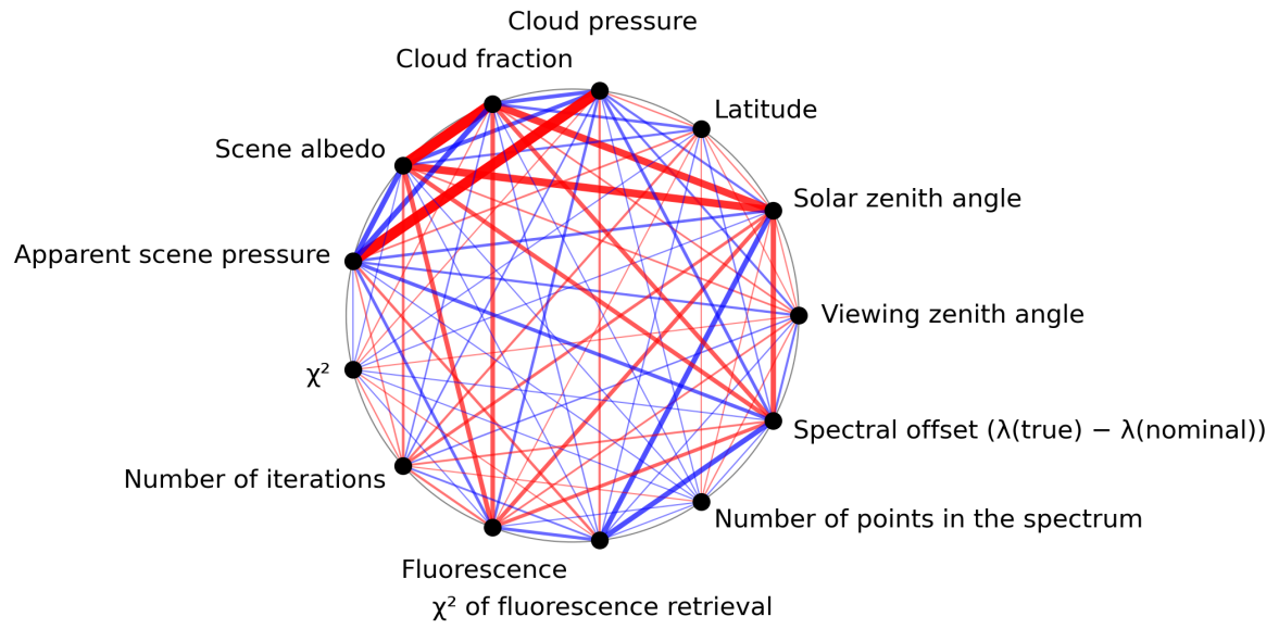
Figure 1: Map of correlation graph for 2024-02-18 to 2024-02-20.
