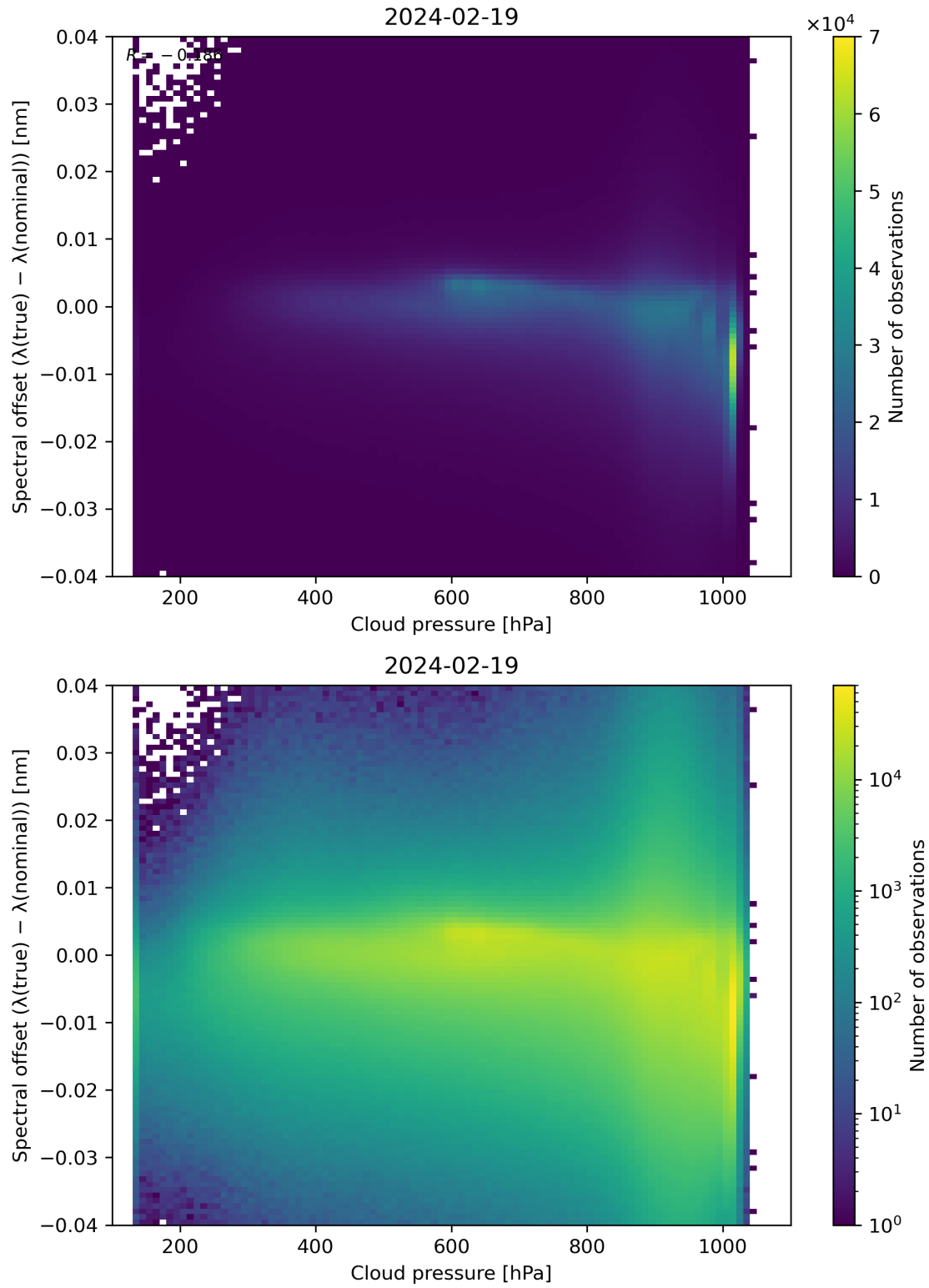
Figure 84: Scatter density plot of “Cloud pressure” against “Spectral offset ( \lambda(\text{true}) - \lambda(\text{nominal}) )” for 2024-02-18 to 2024-02-20.
