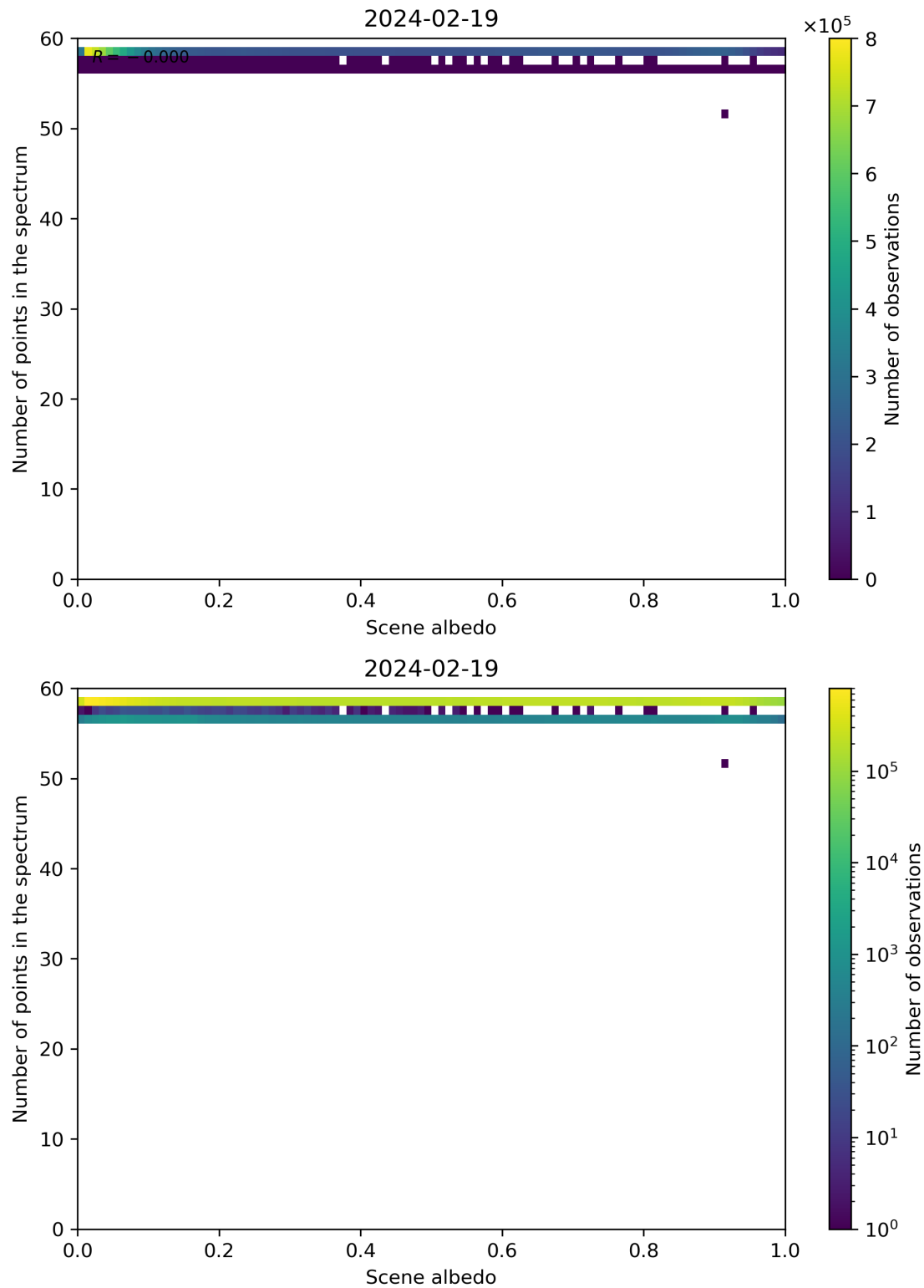
Figure 106: Scatter density plot of “Scene albedo” against “Number of points in the spectrum” for 2024-02-18 to 2024-02-20.
