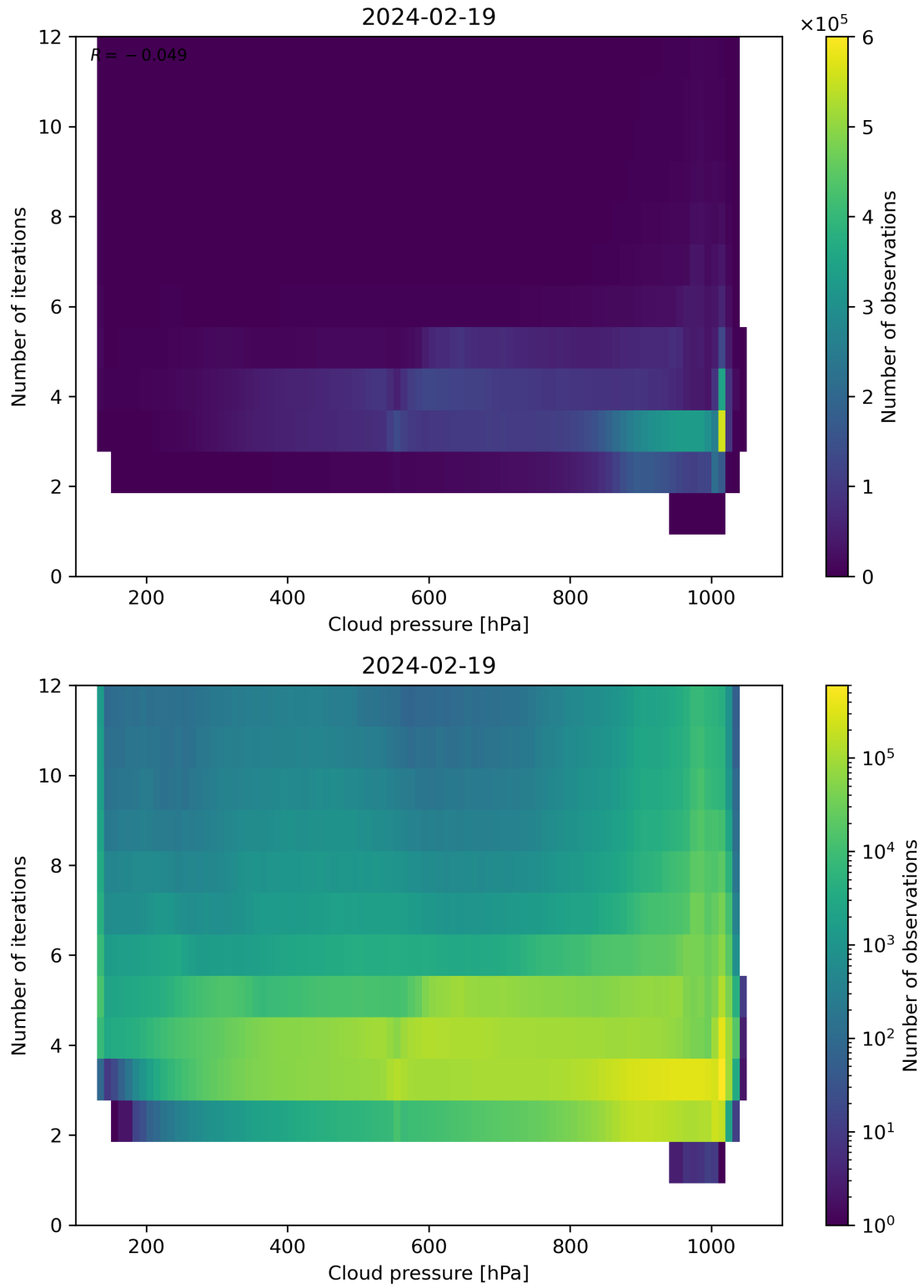
Figure 81: Scatter density plot of “Cloud pressure” against “Number of iterations” for 2024-02-18 to 2024-02-20.
