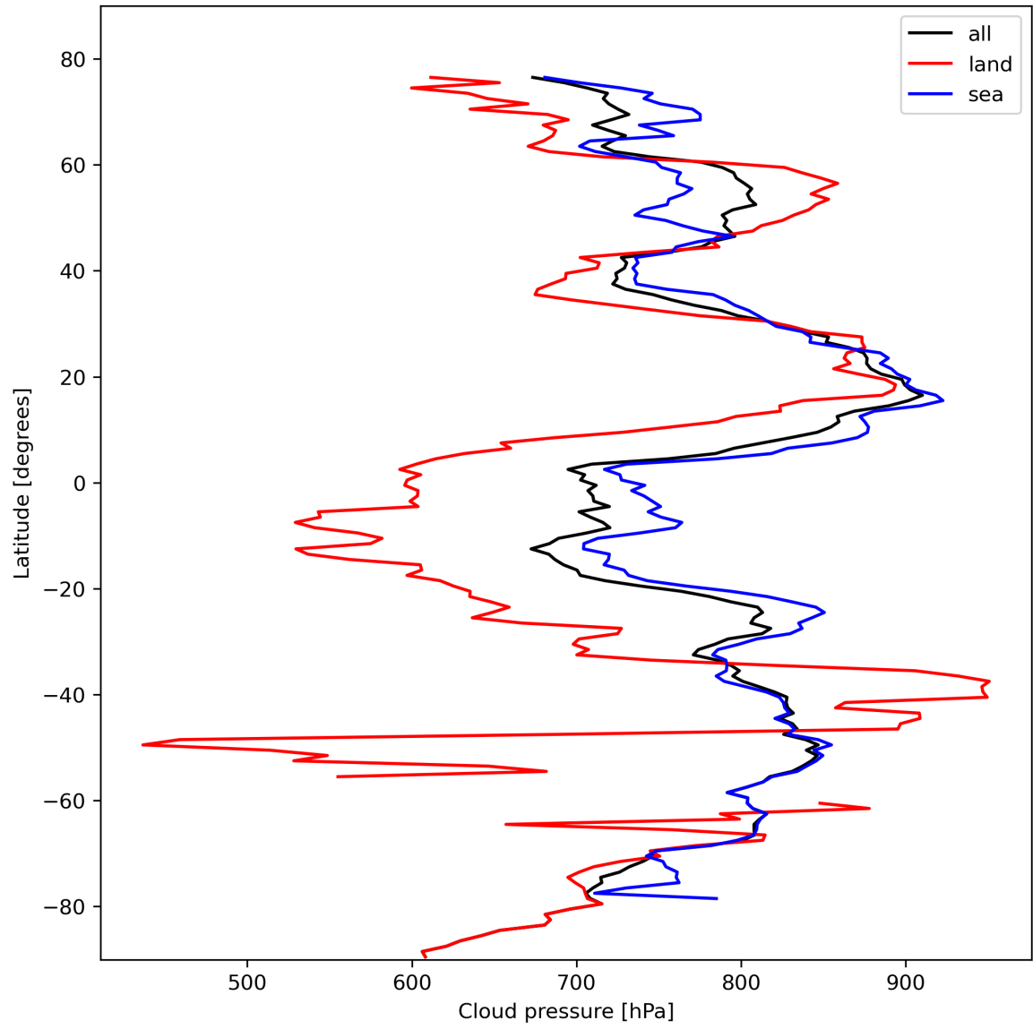
Figure 13: Zonal average of “Cloud pressure” for 2024-02-18 to 2024-02-20.
