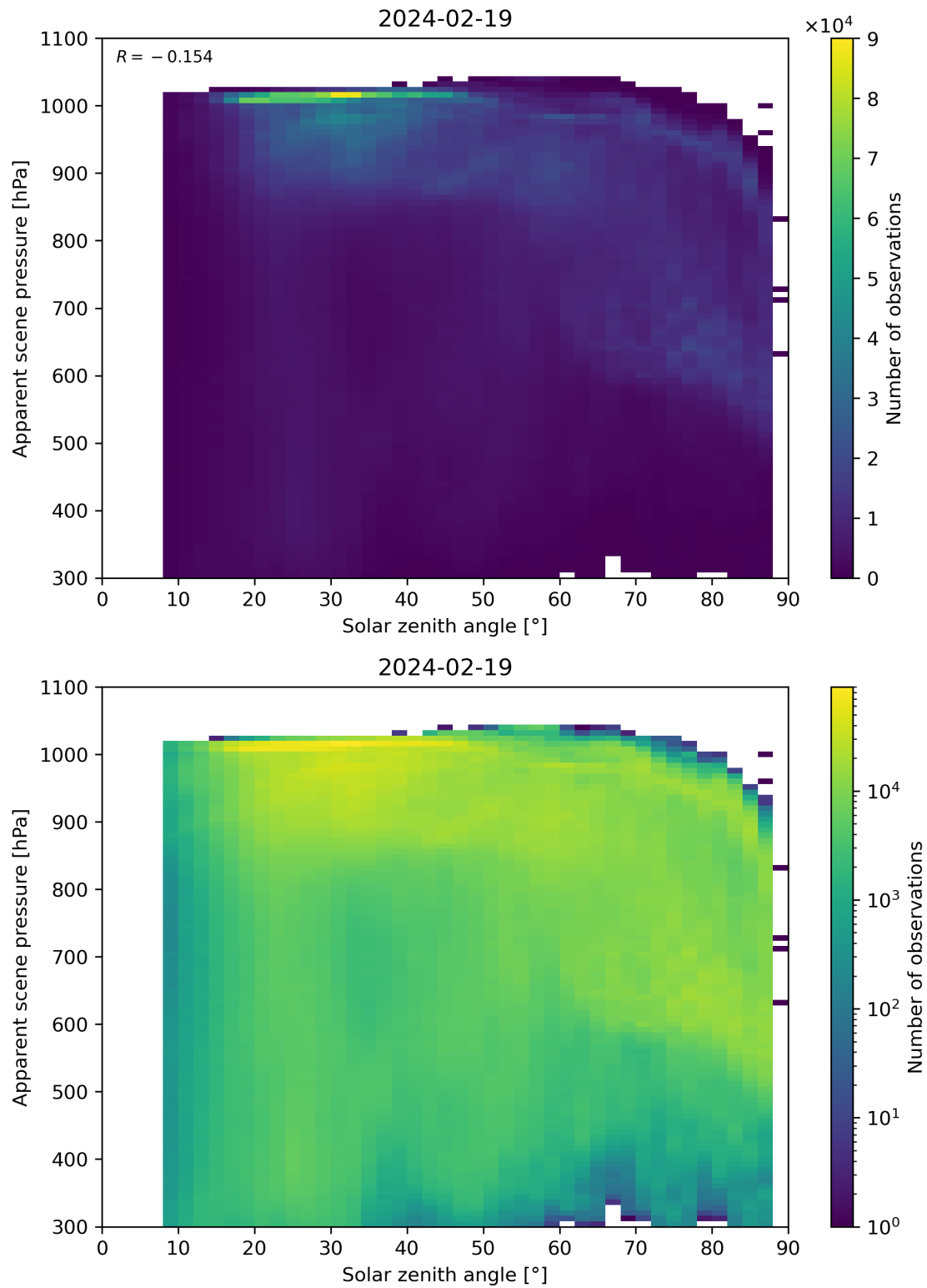
Figure 108: Scatter density plot of “Solar zenith angle” against “Apparent scene pressure” for 2024-02-18 to 2024-02-20.
