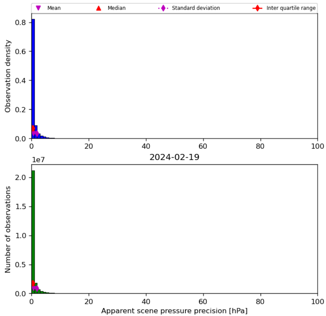
Figure 37: Histogram of “Apparent scene pressure precision” for 2024-02-18 to 2024-02-20
