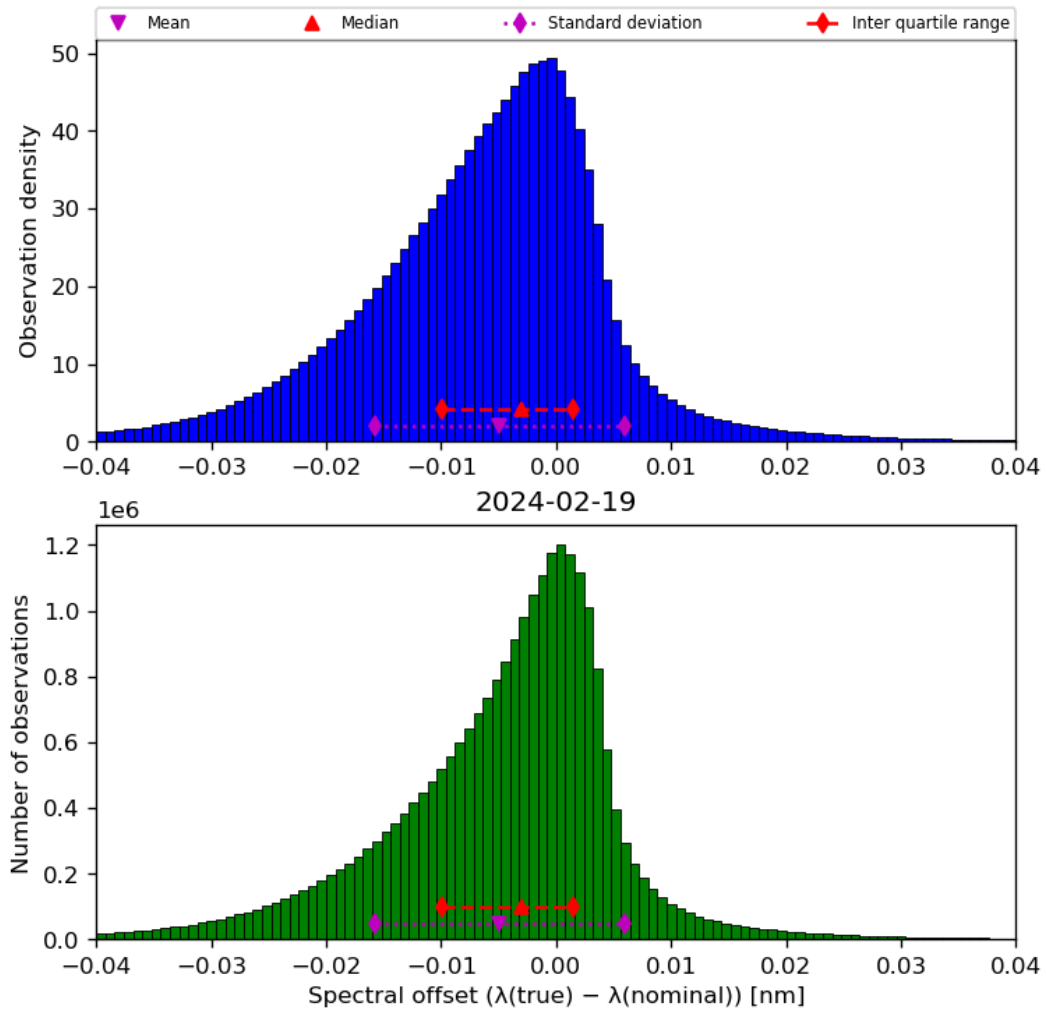
Figure 45: Histogram of “Spectral offset ( \lambda(\text{true}) - \lambda(\text{nominal}) )” for 2024-02-18 to 2024-02-20
