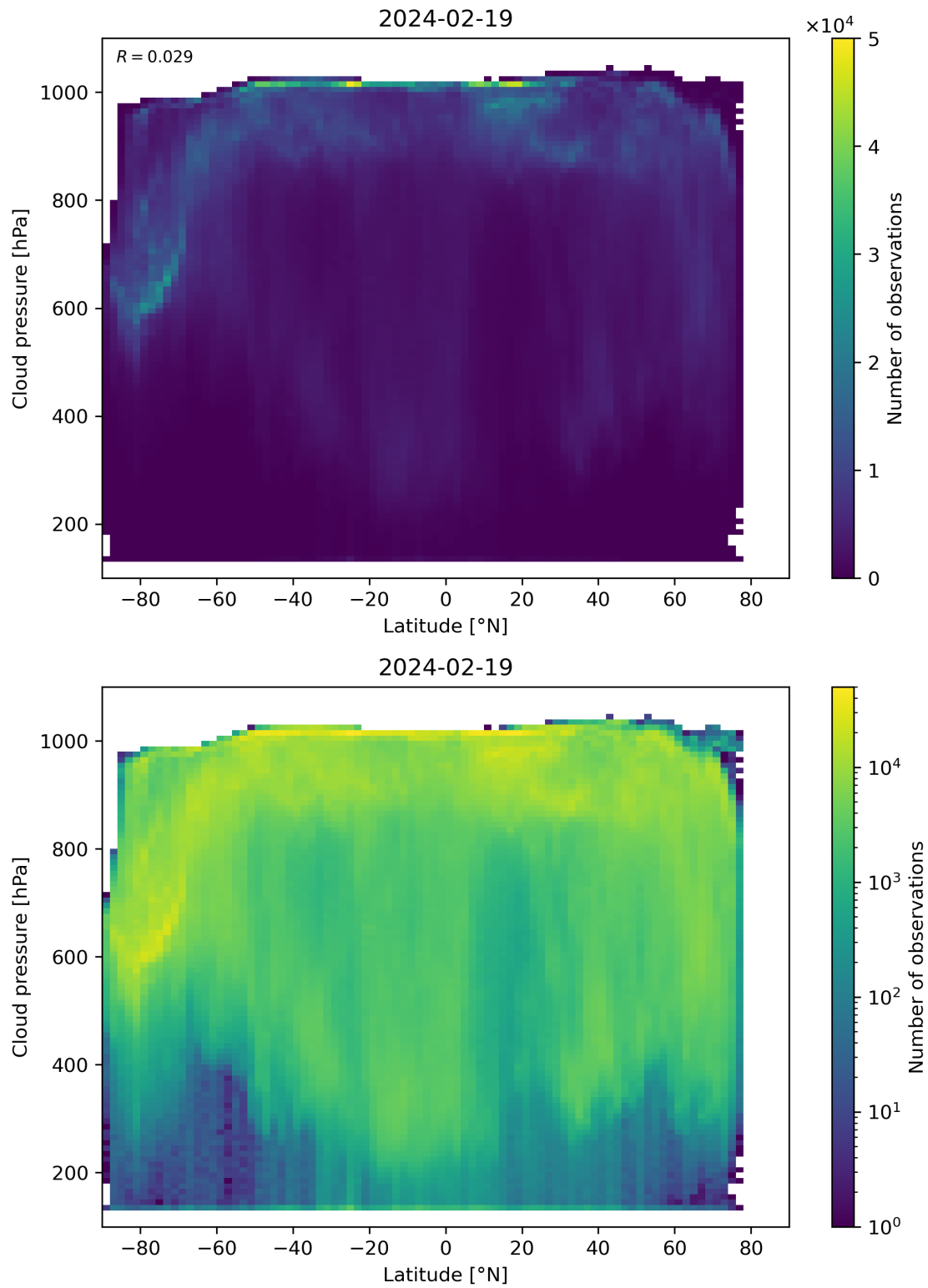
Figure 91: Scatter density plot of “Latitude” against “Cloud pressure” for 2024-02-18 to 2024-02-20.
