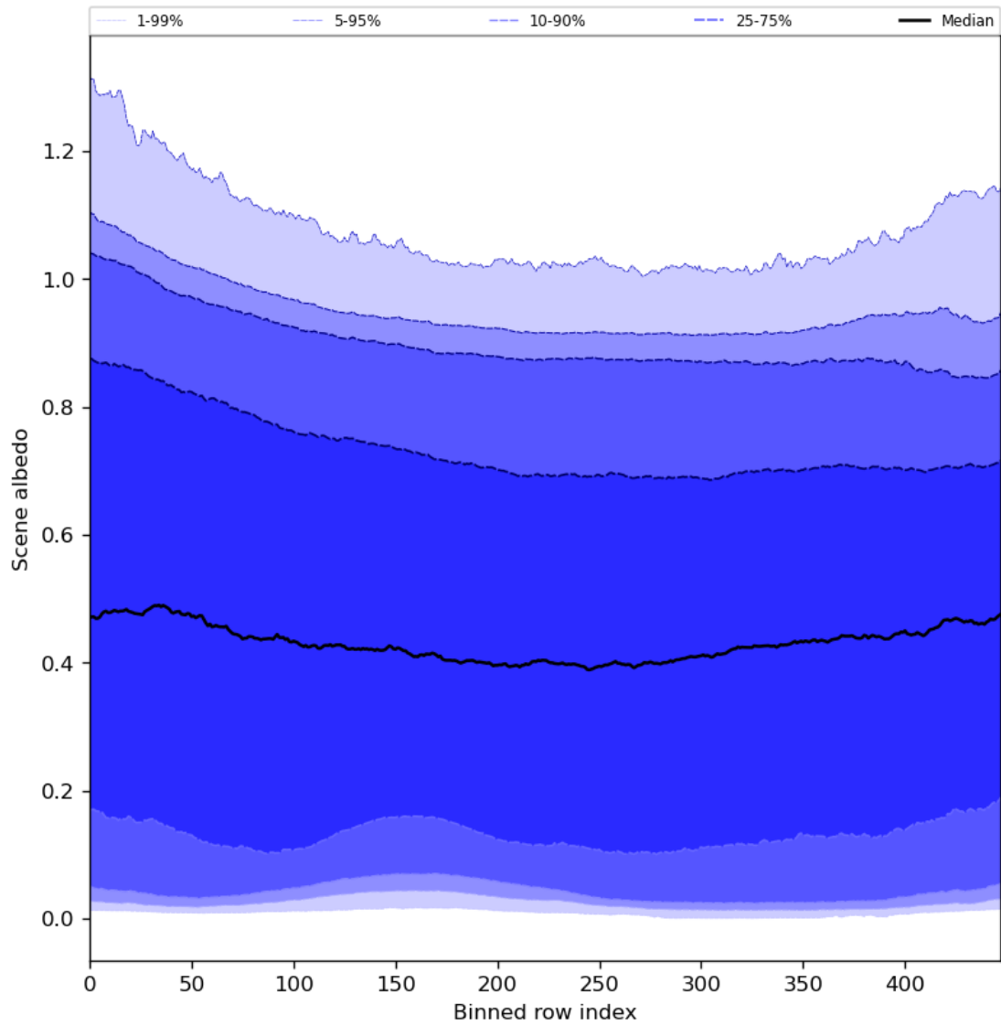
Figure 51: Along track statistics of “Scene albedo” for 2024-02-18 to 2024-02-20
