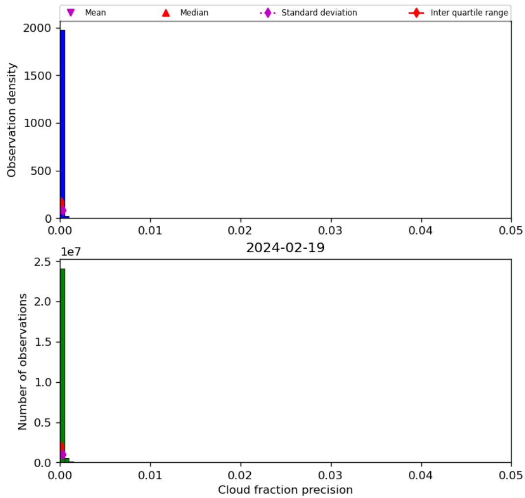
Figure 33: Histogram of “Cloud fraction precision” for 2024-02-18 to 2024-02-20
