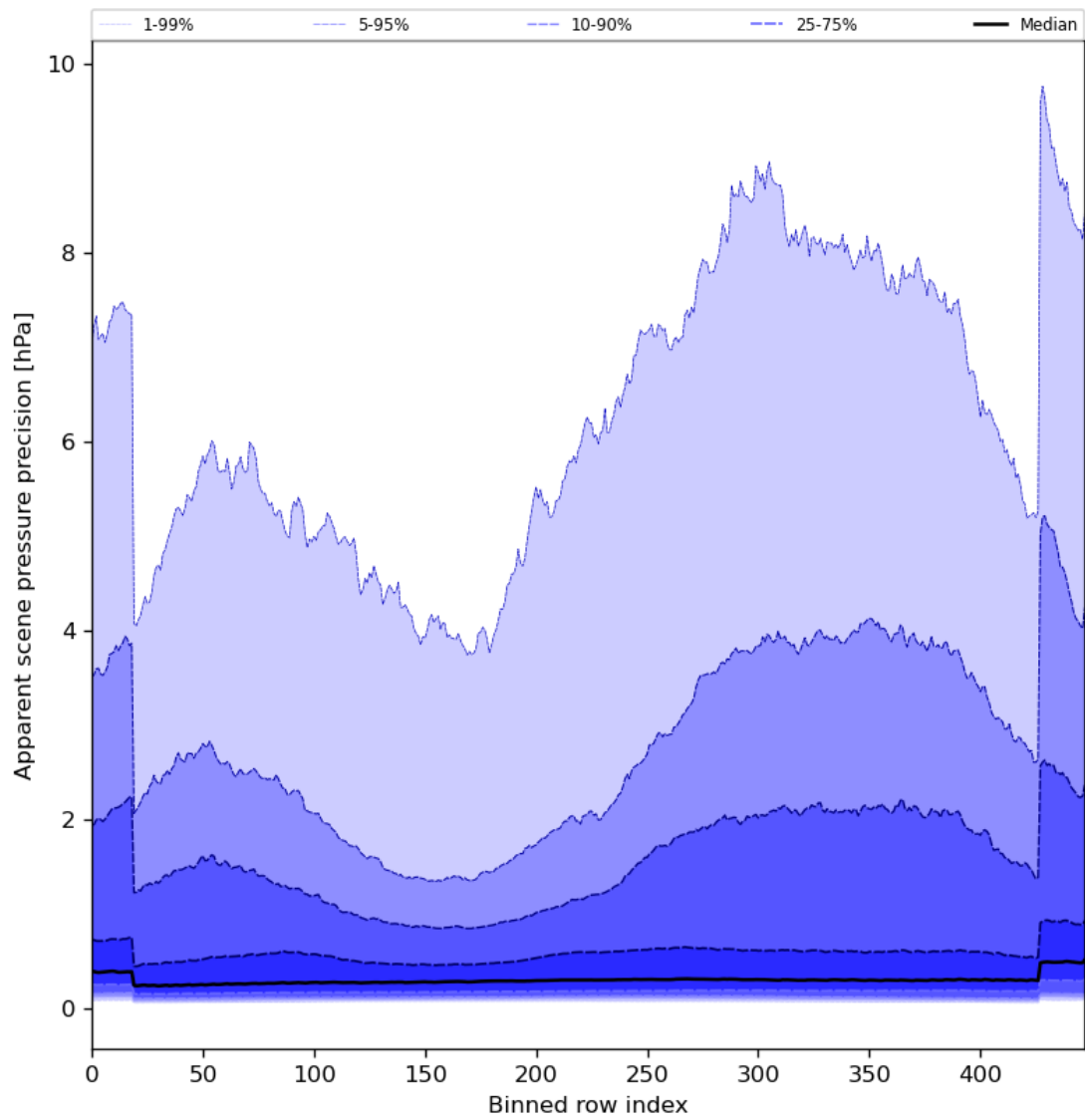
Figure 54: Along track statistics of “Apparent scene pressure precision” for 2024-02-18 to 2024-02-20
