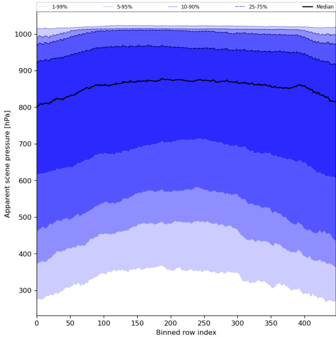
Figure 53: Along track statistics of “Apparent scene pressure” for 2024-02-18 to 2024-02-20
