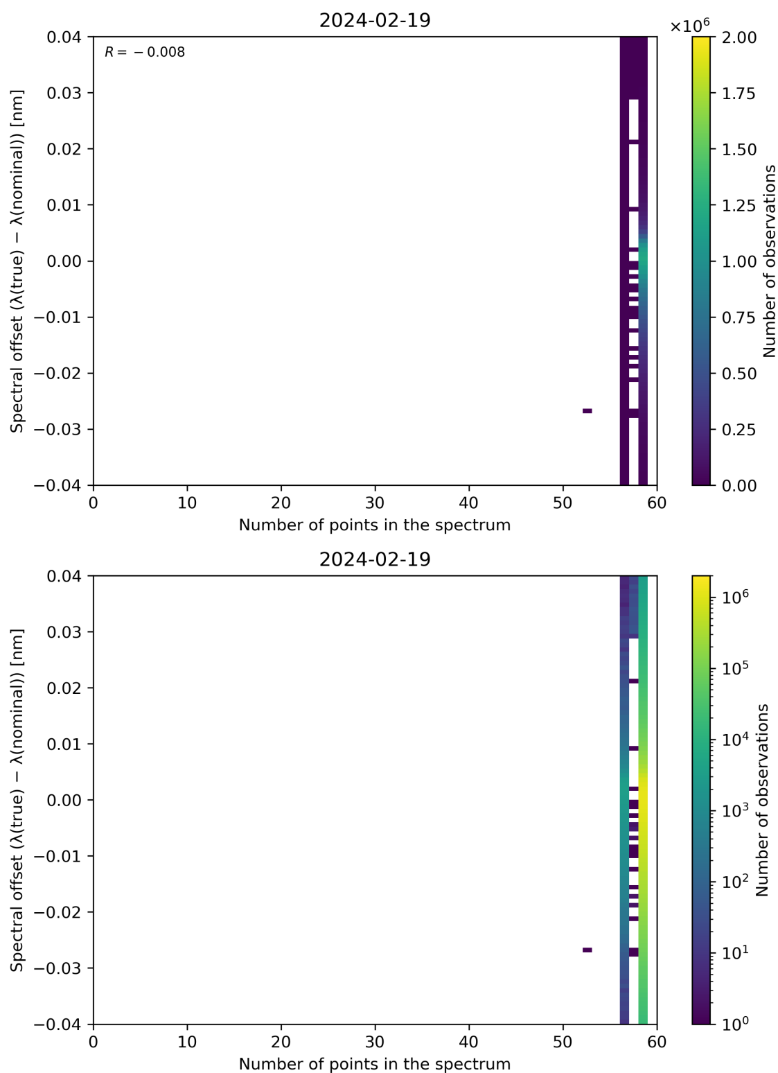
Figure 101: Scatter density plot of “Number of points in the spectrum” against “Spectral offset ( \lambda(\text{true}) - \lambda(\text{nominal}) )” for 2024-02-18 to 2024-02-20.
