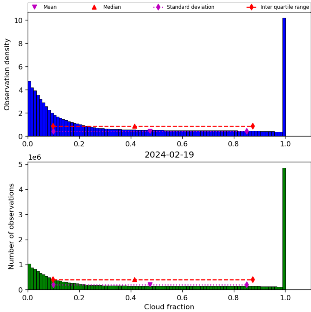
Figure 32: Histogram of “Cloud fraction” for 2024-02-18 to 2024-02-20
