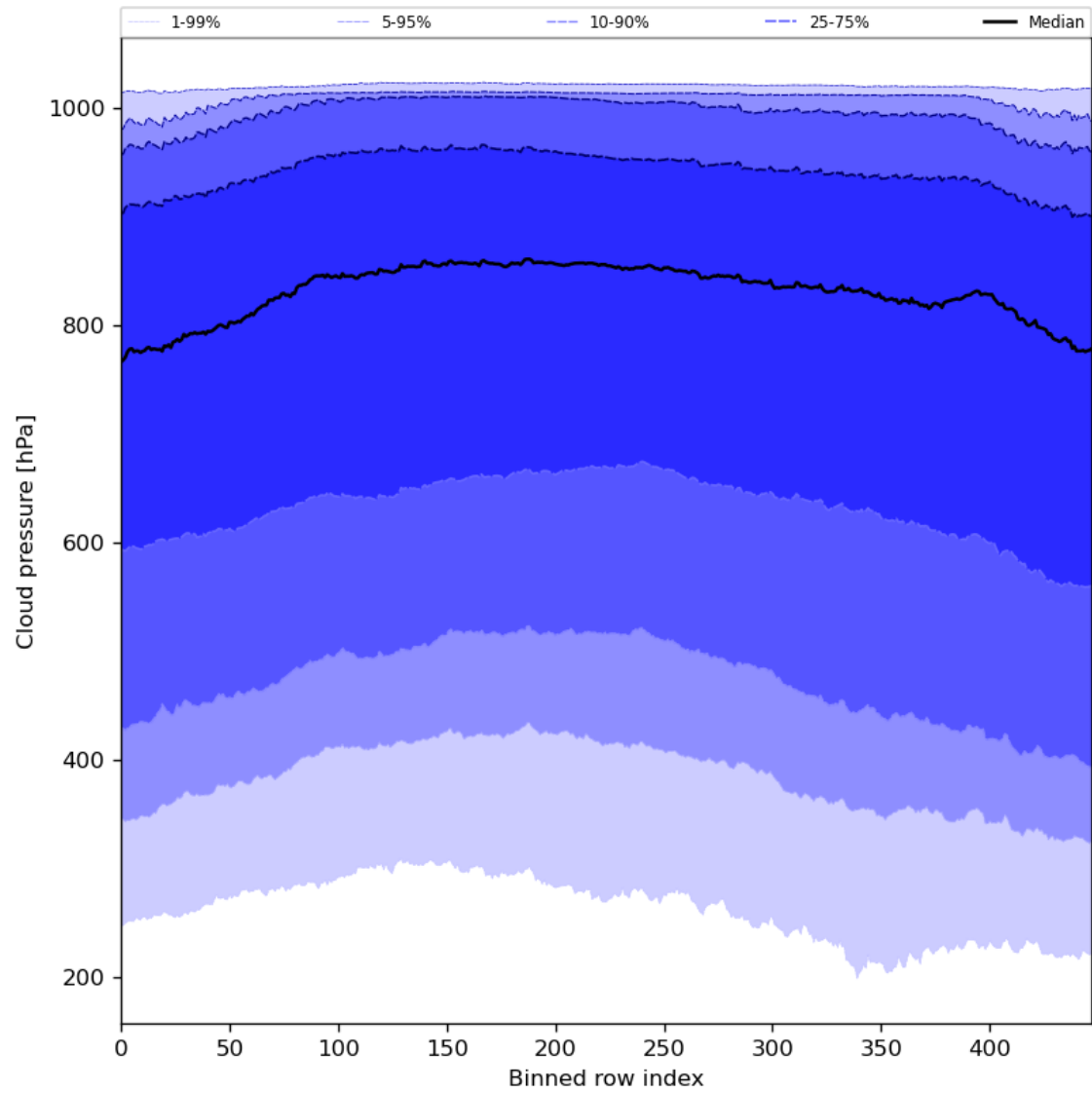
Figure 47: Along track statistics of “Cloud pressure” for 2024-02-18 to 2024-02-20
