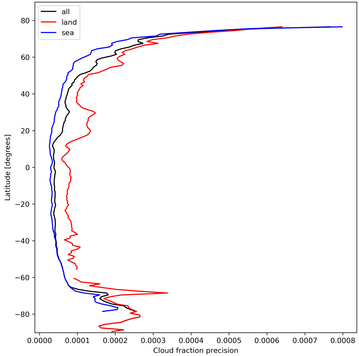
Figure 16: Zonal average of “Cloud fraction precision” for 2024-02-18 to 2024-02-20.
