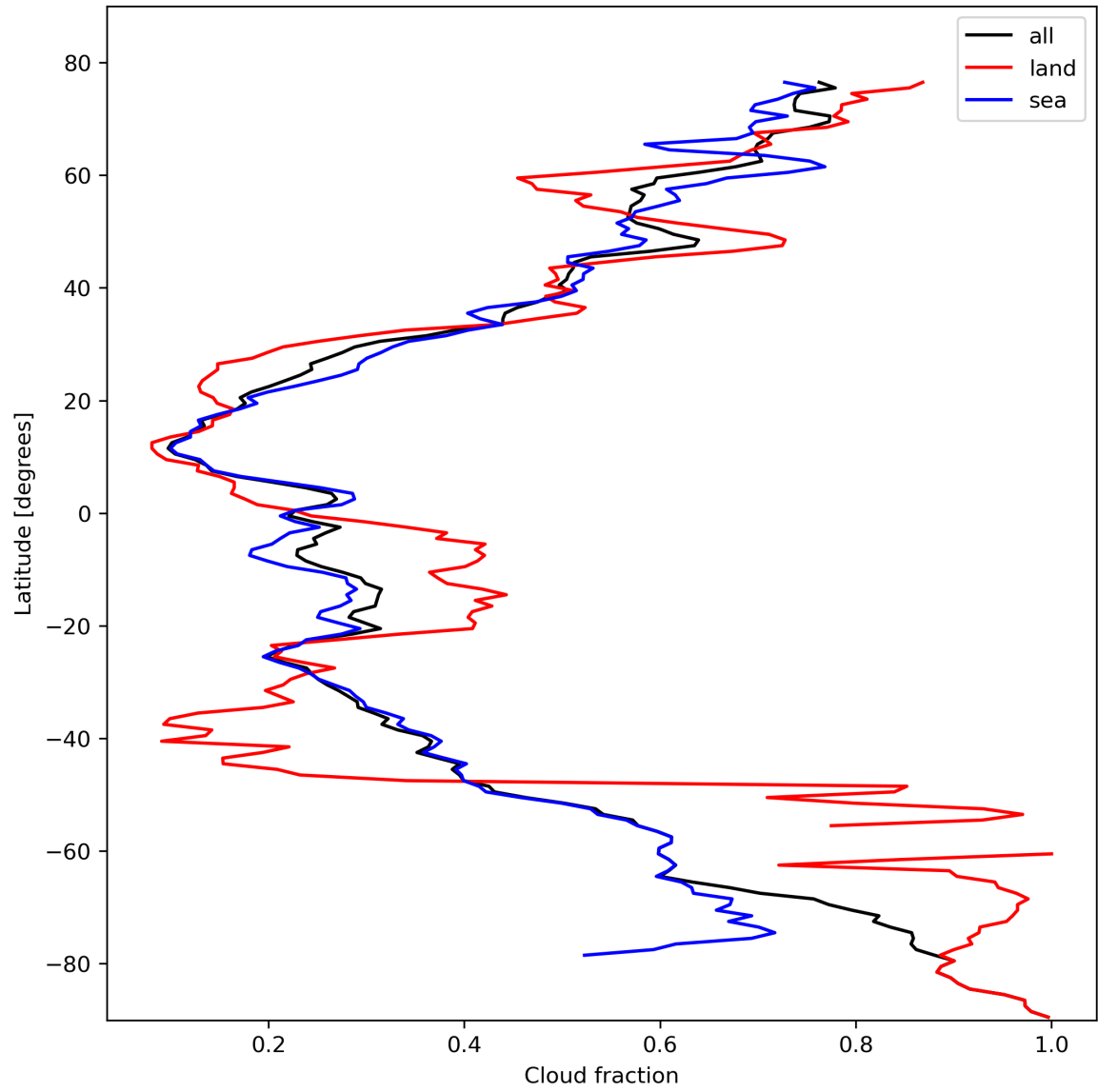
Figure 15: Zonal average of “Cloud fraction” for 2024-02-18 to 2024-02-20.
