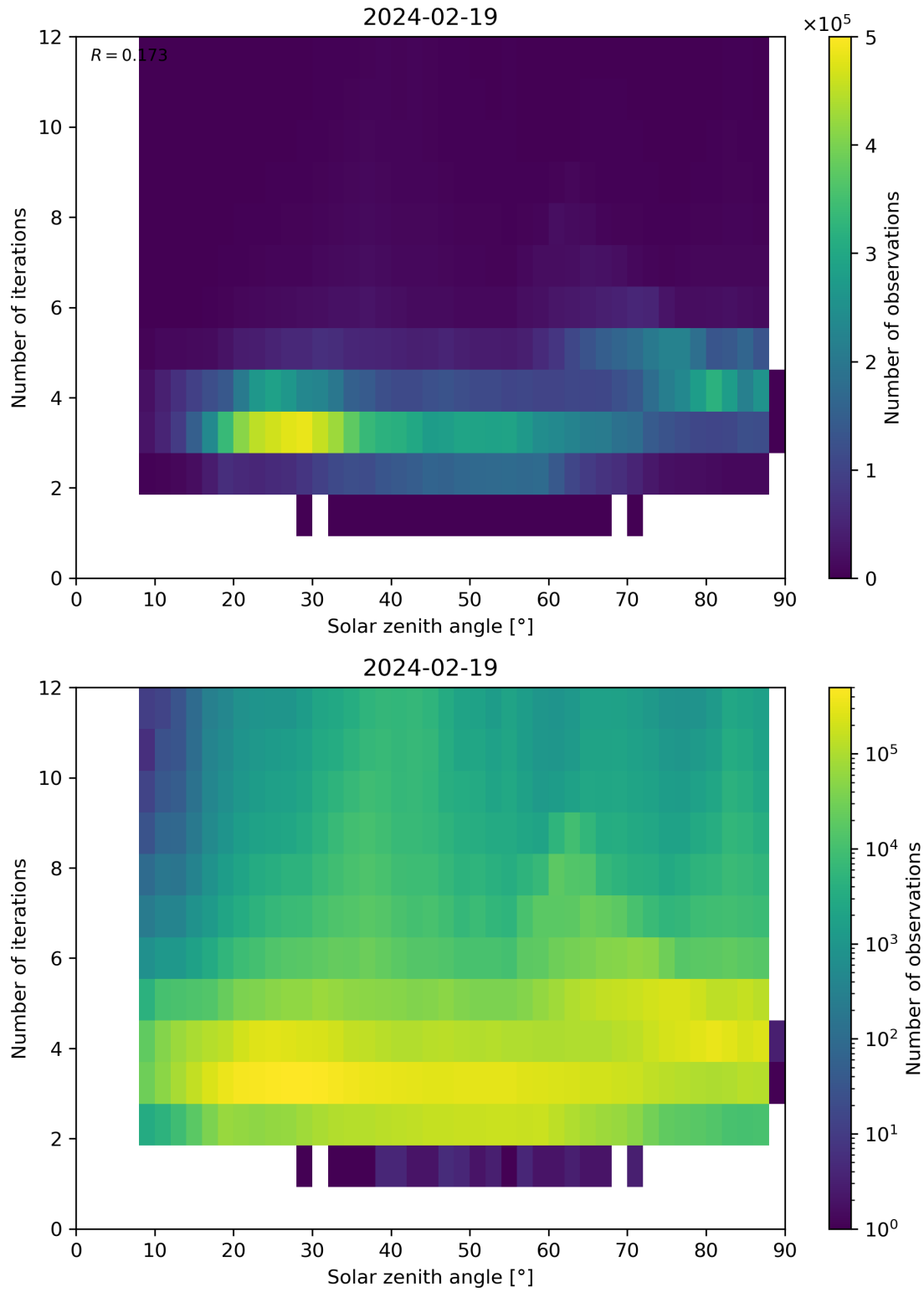
Figure 114: Scatter density plot of “Solar zenith angle” against “Number of iterations” for 2024-02-18 to 2024-02-20.
