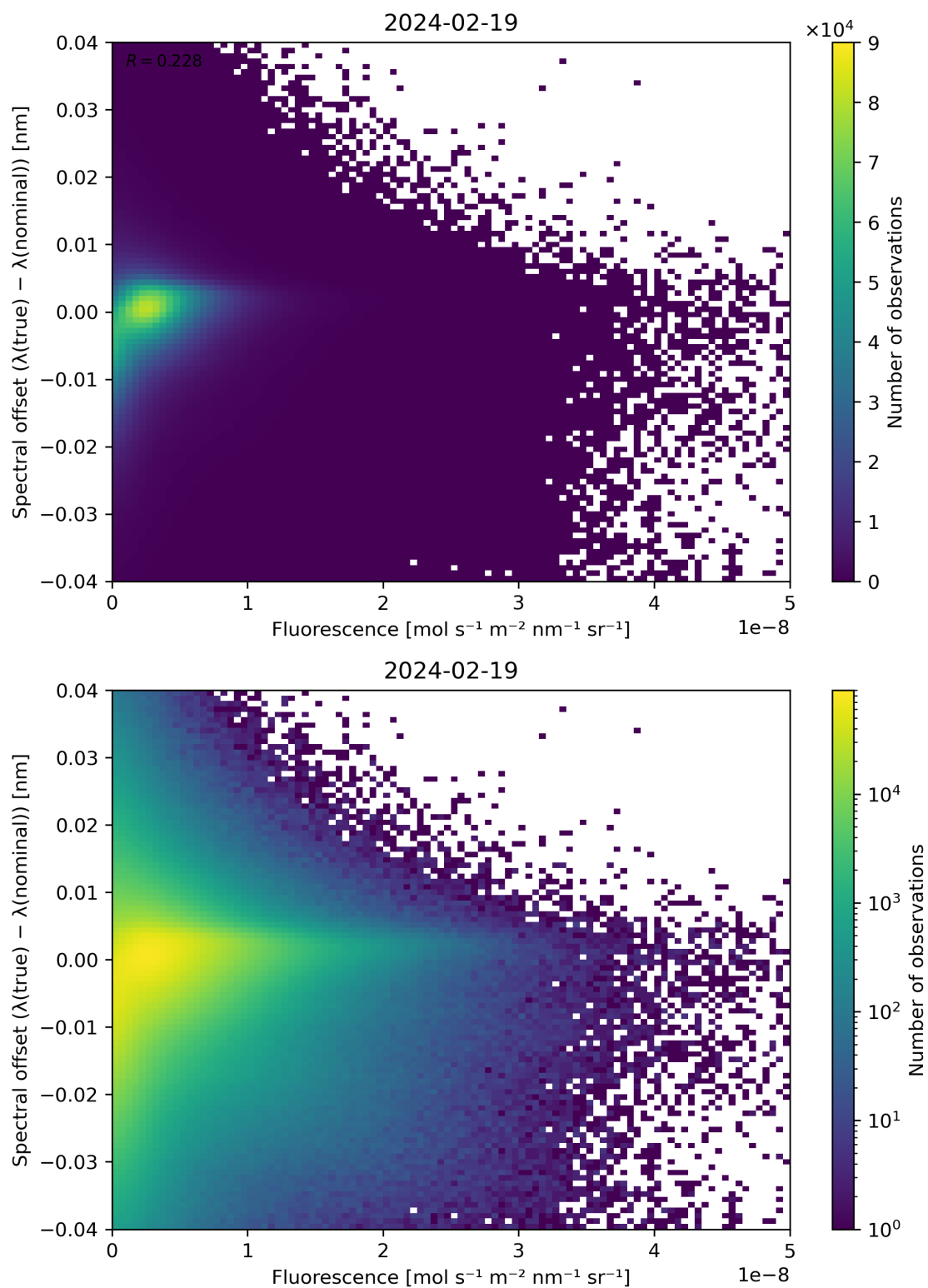
Figure 87: Scatter density plot of “Fluorescence” against “Spectral offset ( \lambda(\text{true}) - \lambda(\text{nominal}) )” for 2024-02-18 to 2024-02-20.
