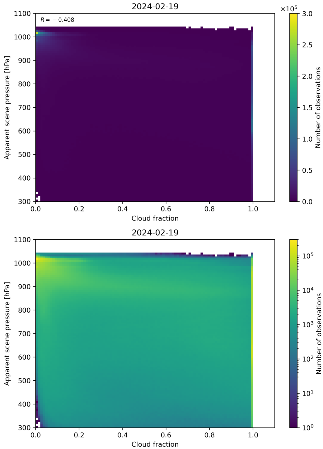
Figure 70: Scatter density plot of “Cloud fraction” against “Apparent scene pressure” for 2024-02-18 to 2024-02-20.
