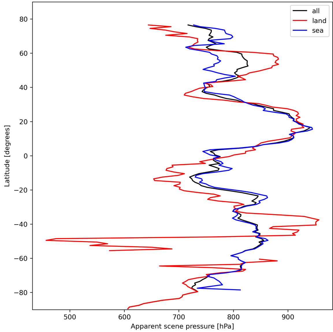
Figure 19: Zonal average of “Apparent scene pressure” for 2024-02-18 to 2024-02-20.
