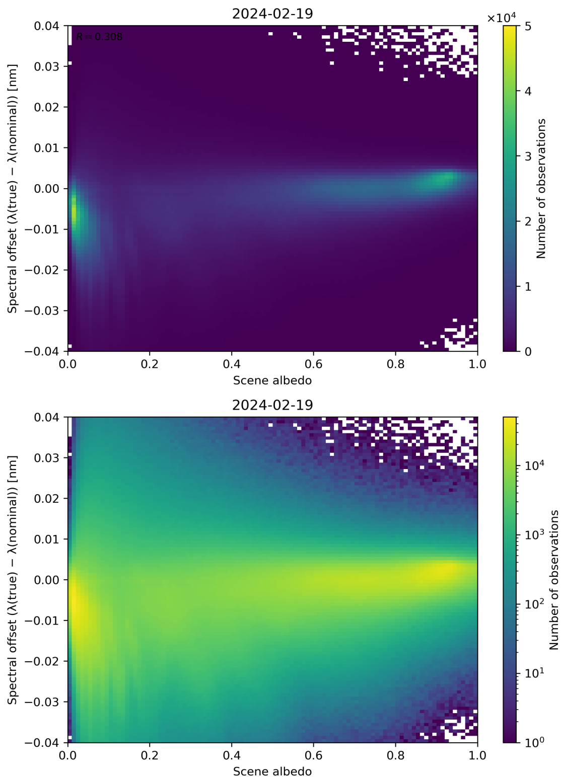
Figure 107: Scatter density plot of “Scene albedo” against “Spectral offset ( \lambda(\text{true}) - \lambda(\text{nominal}) )” for 2024-02-18 to 2024-02-20.
