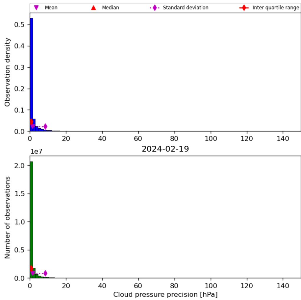
Figure 31: Histogram of “Cloud pressure precision” for 2024-02-18 to 2024-02-20
