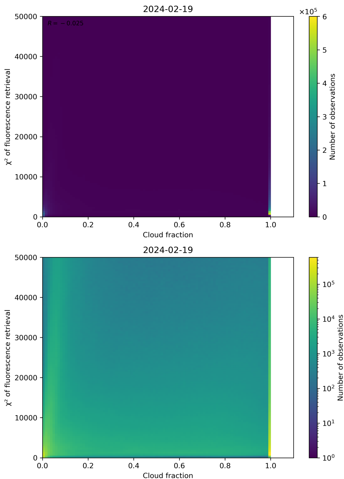
Figure 71: Scatter density plot of “Cloud fraction” against “ \chi^2 of fluorescence retrieval” for 2024-02-18 to 2024-02-20.
