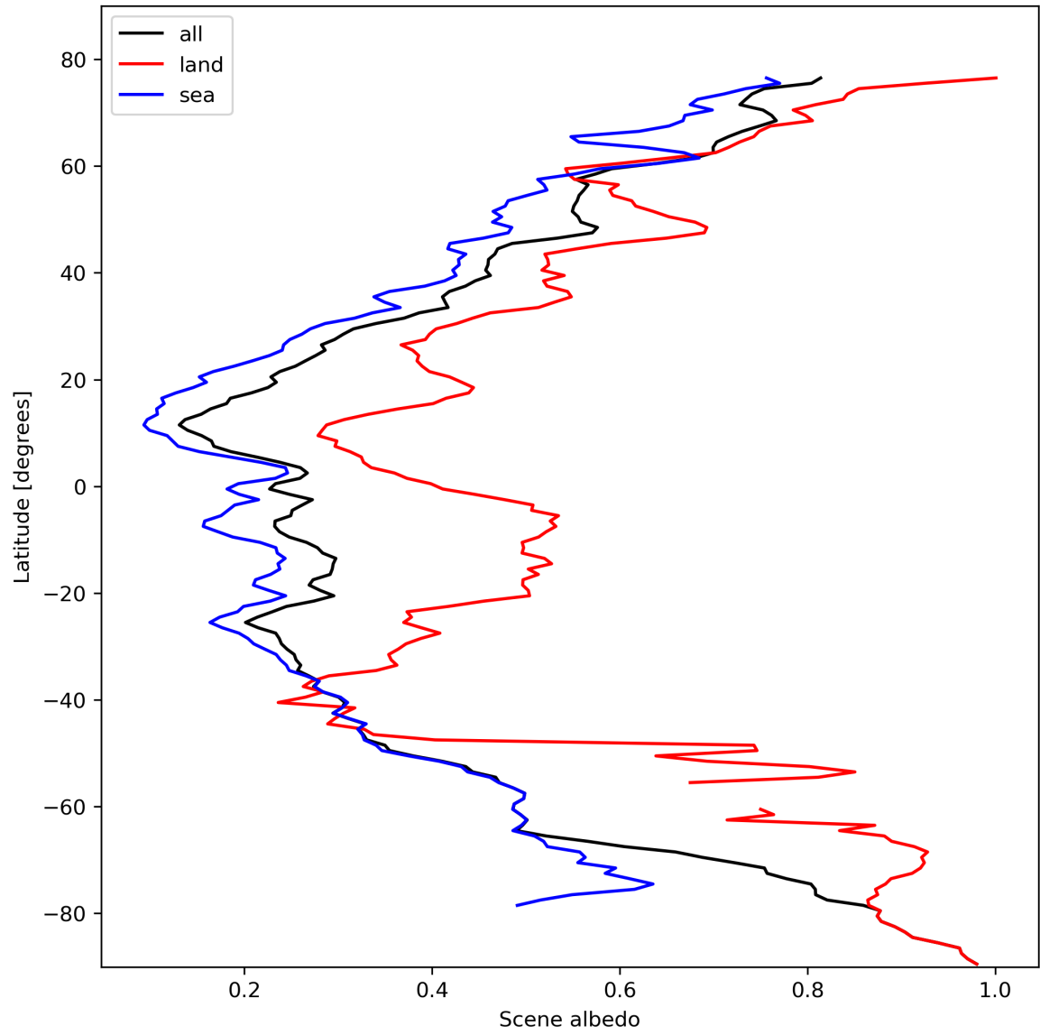
Figure 17: Zonal average of “Scene albedo” for 2024-02-18 to 2024-02-20.
