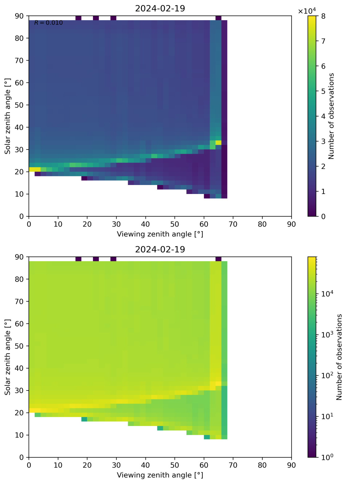
Figure 127: Scatter density plot of “Viewing zenith angle” against “Solar zenith angle” for 2024-02-18 to 2024-02-20.
