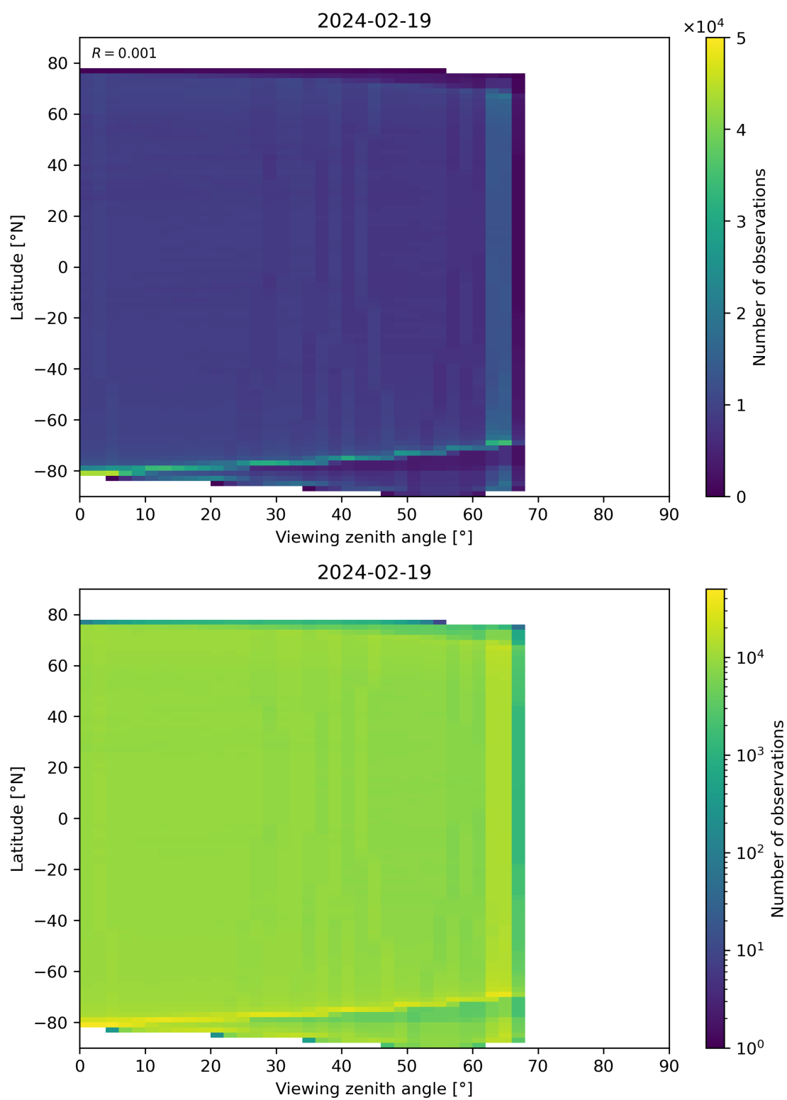
Figure 123: Scatter density plot of “Viewing zenith angle” against “Latitude” for 2024-02-18 to 2024-02-20.
