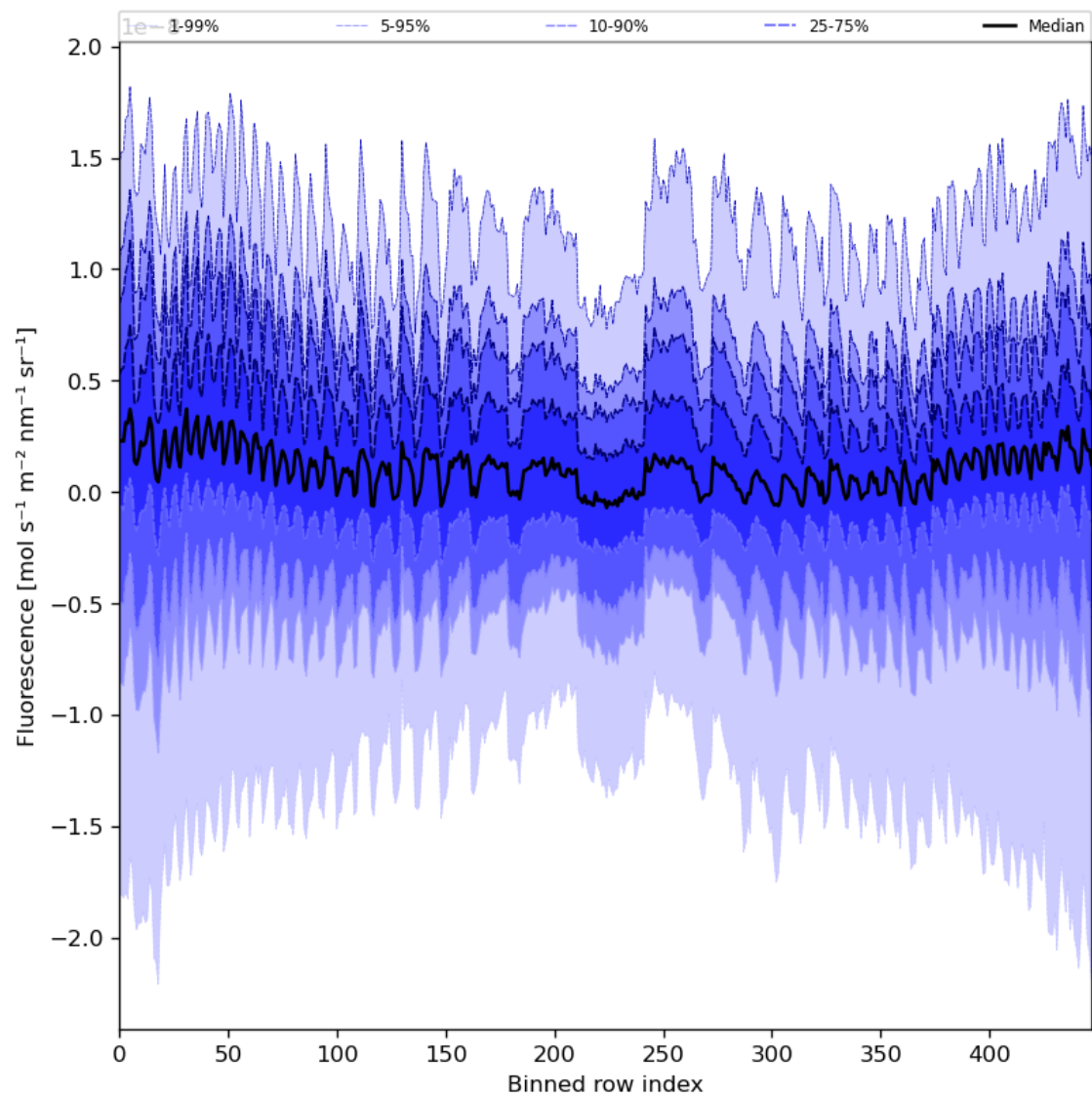
Figure 57: Along track statistics of “Fluorescence” for 2024-02-18 to 2024-02-20
