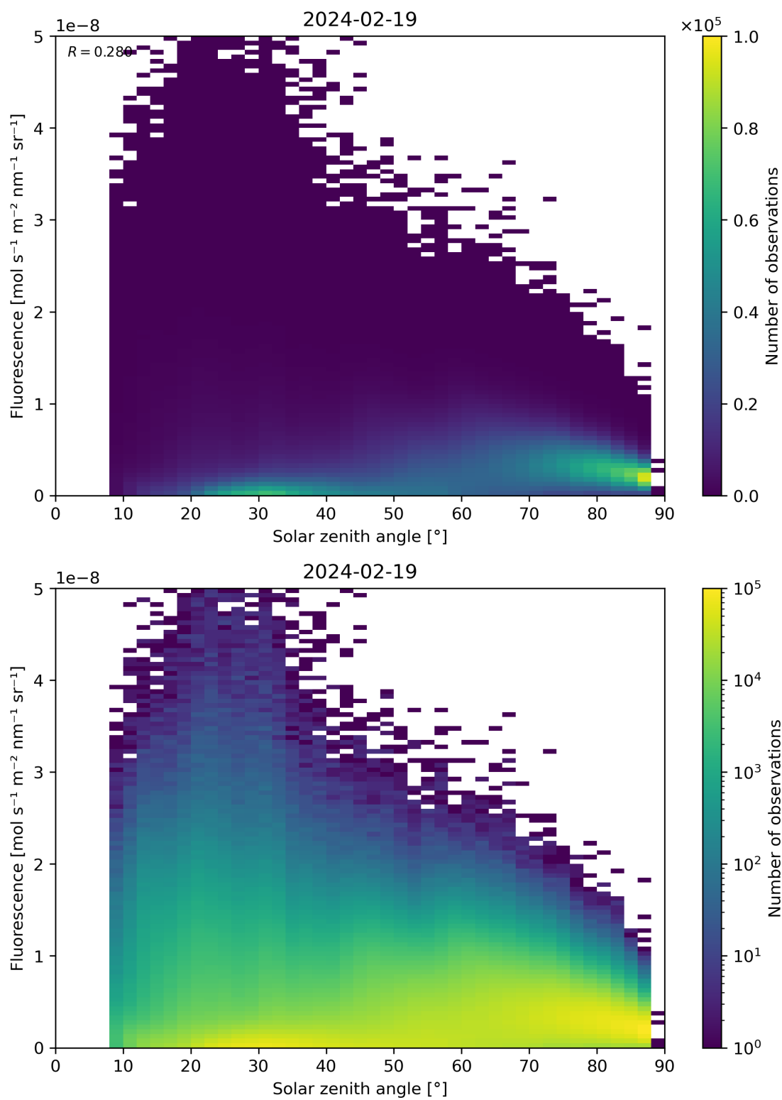
Figure 112: Scatter density plot of “Solar zenith angle” against “Fluorescence” for 2024-02-18 to 2024-02-20.
