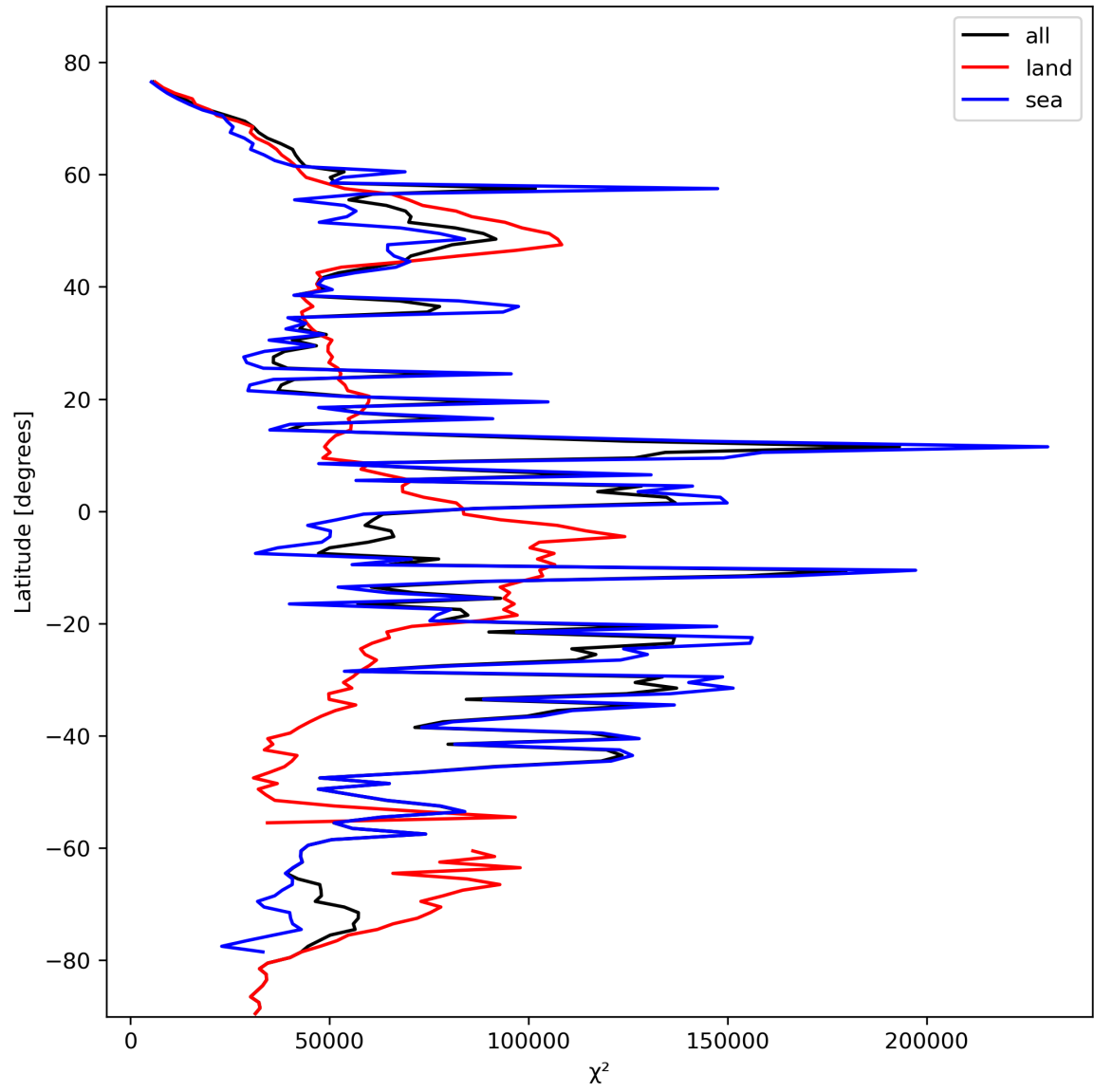
Figure 21: Zonal average of “ \chi^2 ” for 2024-02-18 to 2024-02-20.
