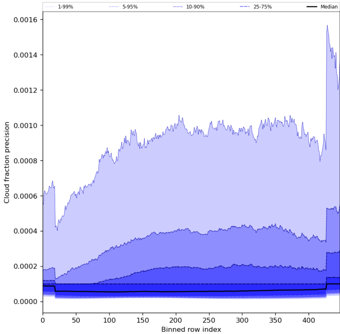
Figure 50: Along track statistics of “Cloud fraction precision” for 2024-02-18 to 2024-02-20
