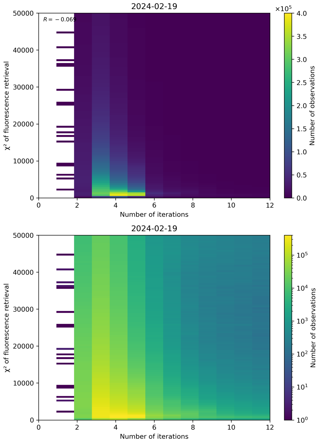
Figure 97: Scatter density plot of “Number of iterations” against “ \chi^2 of fluorescence retrieval” for 2024-02-18 to 2024-02-20.
