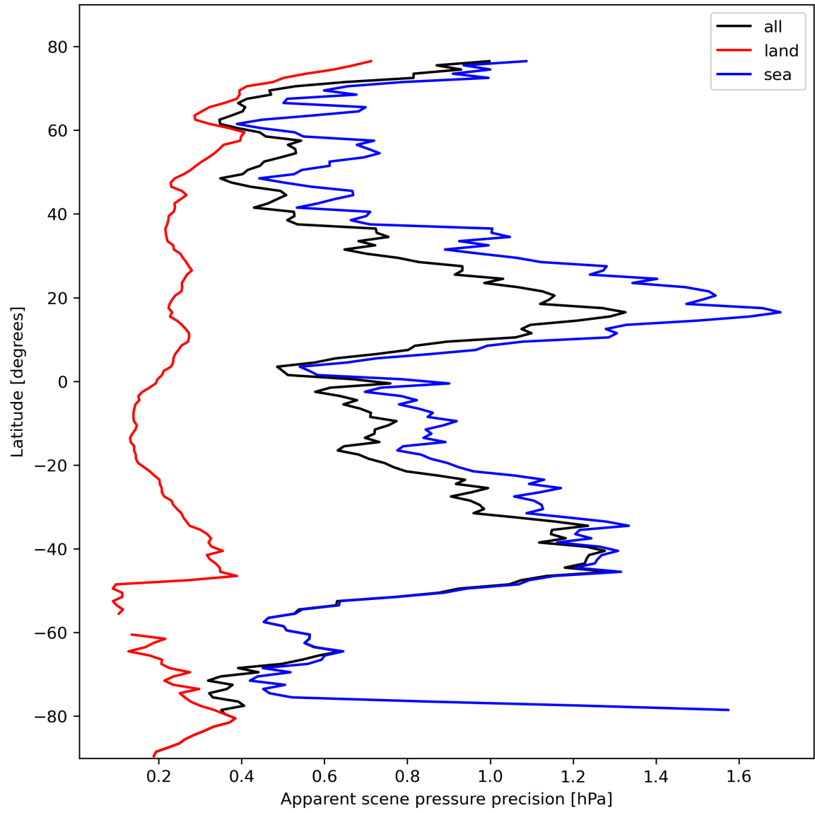
Figure 20: Zonal average of “Apparent scene pressure precision” for 2024-02-18 to 2024-02-20.
