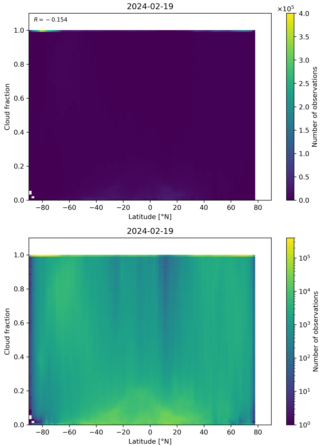
Figure 90: Scatter density plot of “Latitude” against “Cloud fraction” for 2024-02-18 to 2024-02-20.
