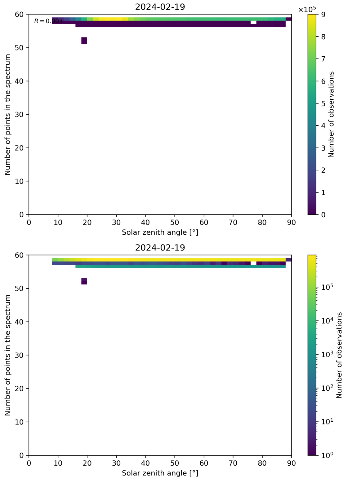
Figure 115: Scatter density plot of “Solar zenith angle” against “Number of points in the spectrum” for 2024-02-18 to 2024-02-20.
