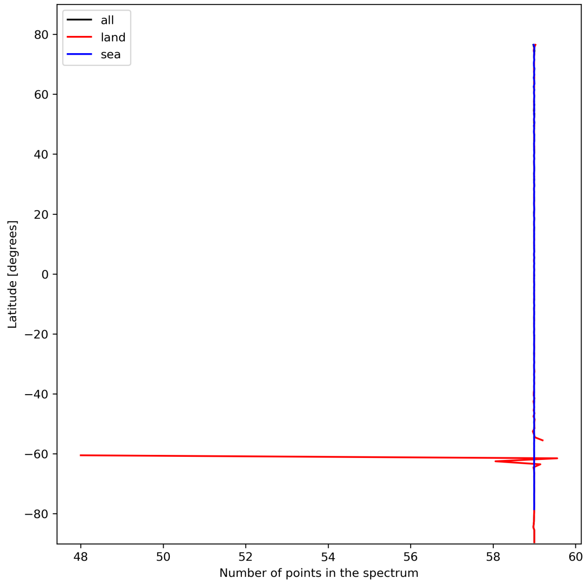
Figure 27: Zonal average of “Number of points in the spectrum” for 2024-02-18 to 2024-02-20.
