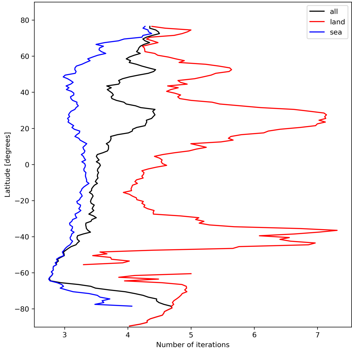
Figure 22: Zonal average of “Number of iterations” for 2024-02-18 to 2024-02-20.
