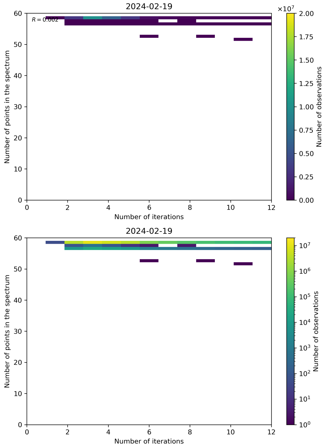
Figure 99: Scatter density plot of “Number of iterations” against “Number of points in the spectrum” for 2024-02-18 to 2024-02-20.
