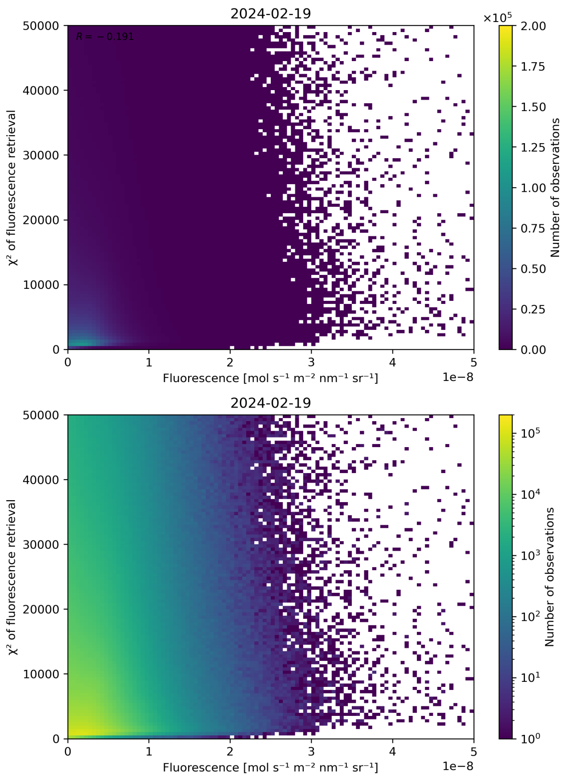
Figure 85: Scatter density plot of “Fluorescence” against “ \chi^2 of fluorescence retrieval” for 2024-02-18 to 2024-02-20.
