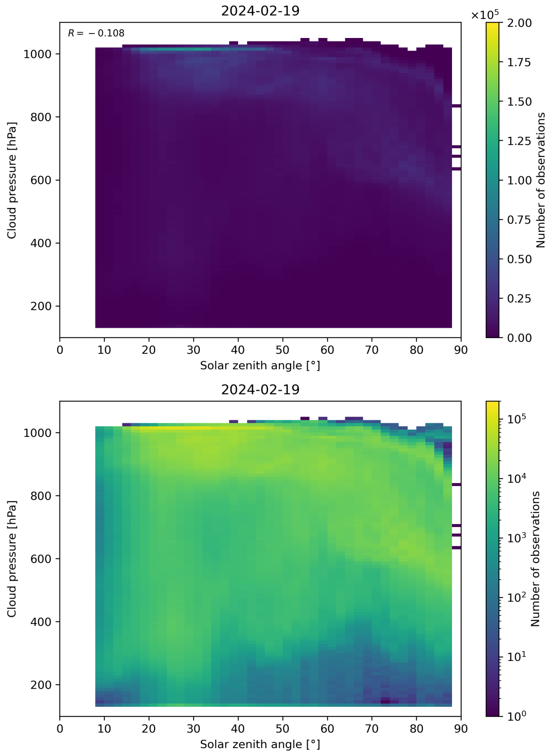
Figure 111: Scatter density plot of “Solar zenith angle” against “Cloud pressure” for 2024-02-18 to 2024-02-20.
