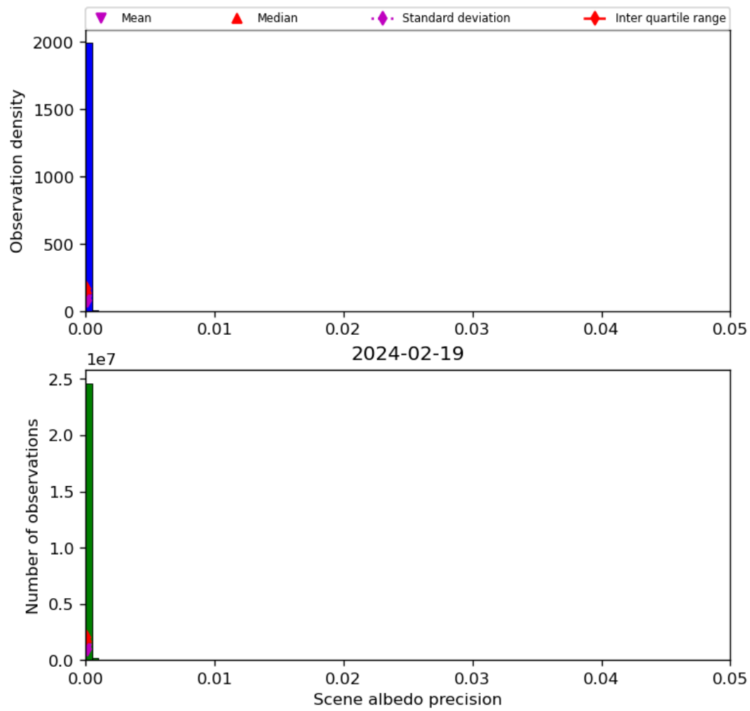
Figure 35: Histogram of “Scene albedo precision” for 2024-02-18 to 2024-02-20
