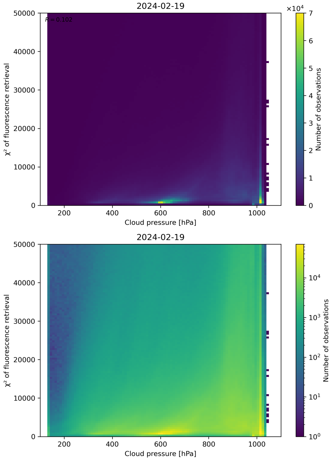
Figure 78: Scatter density plot of “Cloud pressure” against “ \chi^2 of fluorescence retrieval” for 2024-02-18 to 2024-02-20.
