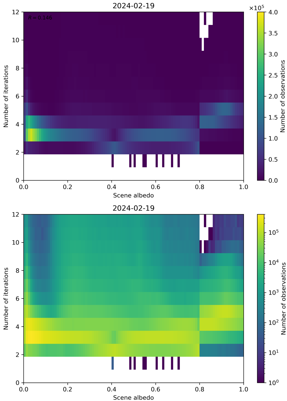
Figure 105: Scatter density plot of “Scene albedo” against “Number of iterations” for 2024-02-18 to 2024-02-20.
