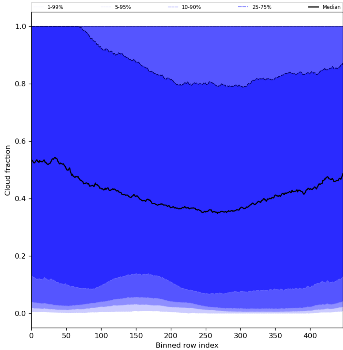
Figure 49: Along track statistics of “Cloud fraction” for 2024-02-18 to 2024-02-20
