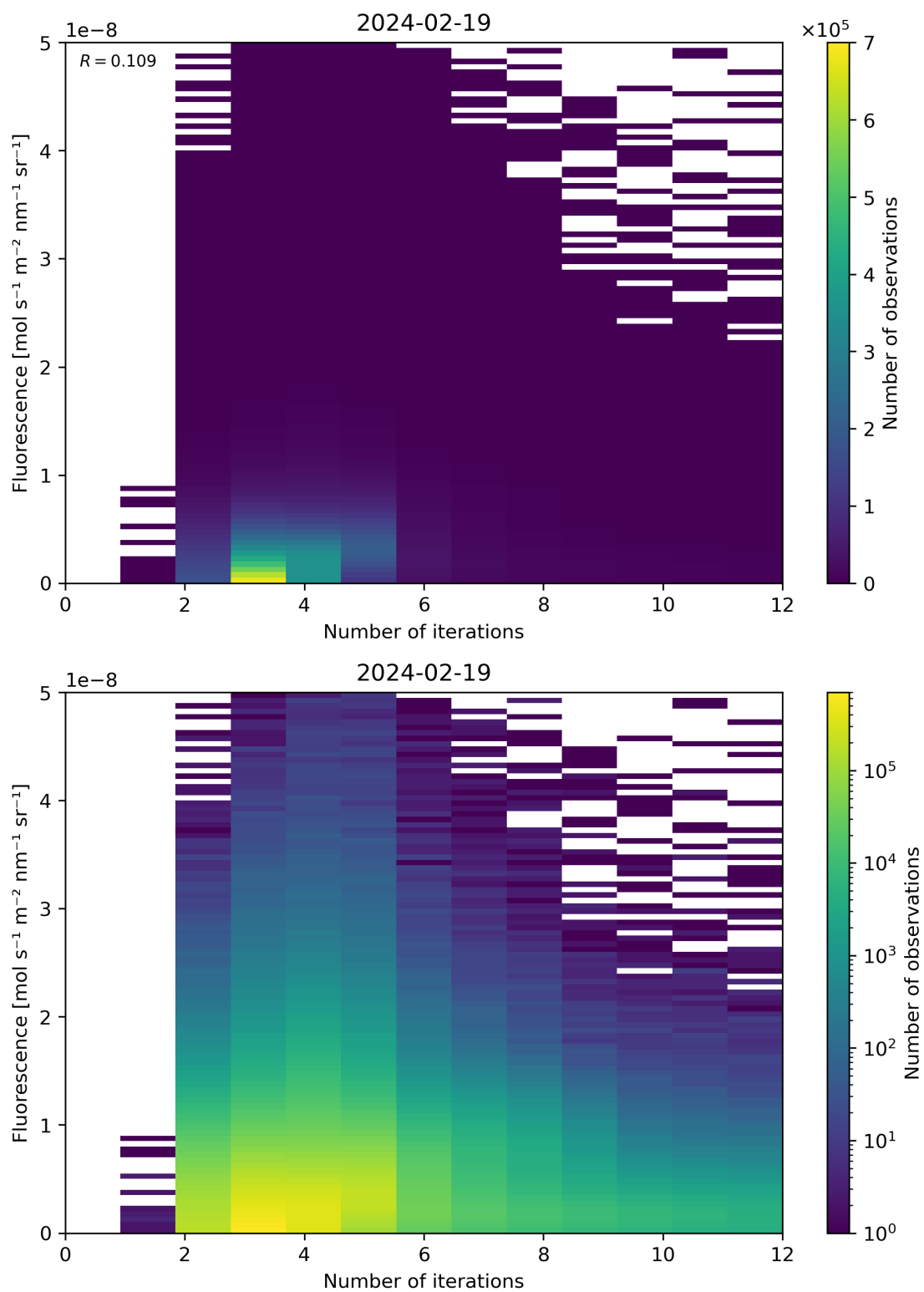
Figure 98: Scatter density plot of “Number of iterations” against “Fluorescence” for 2024-02-18 to 2024-02-20.
