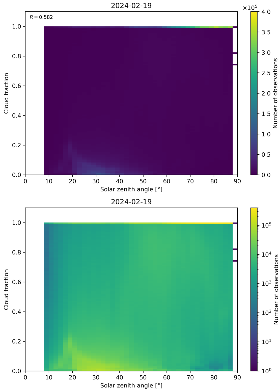
Figure 110: Scatter density plot of “Solar zenith angle” against “Cloud fraction” for 2024-02-18 to 2024-02-20.
