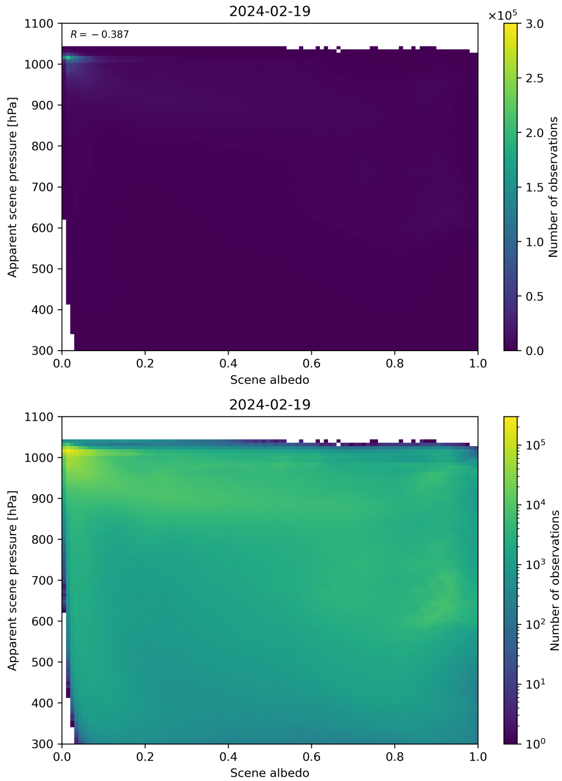
Figure 102: Scatter density plot of “Scene albedo” against “Apparent scene pressure” for 2024-02-18 to 2024-02-20.
