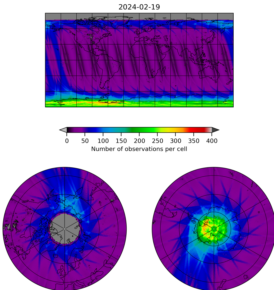
Figure 11: Map of the number of observations for 2024-02-18 to 2024-02-20
