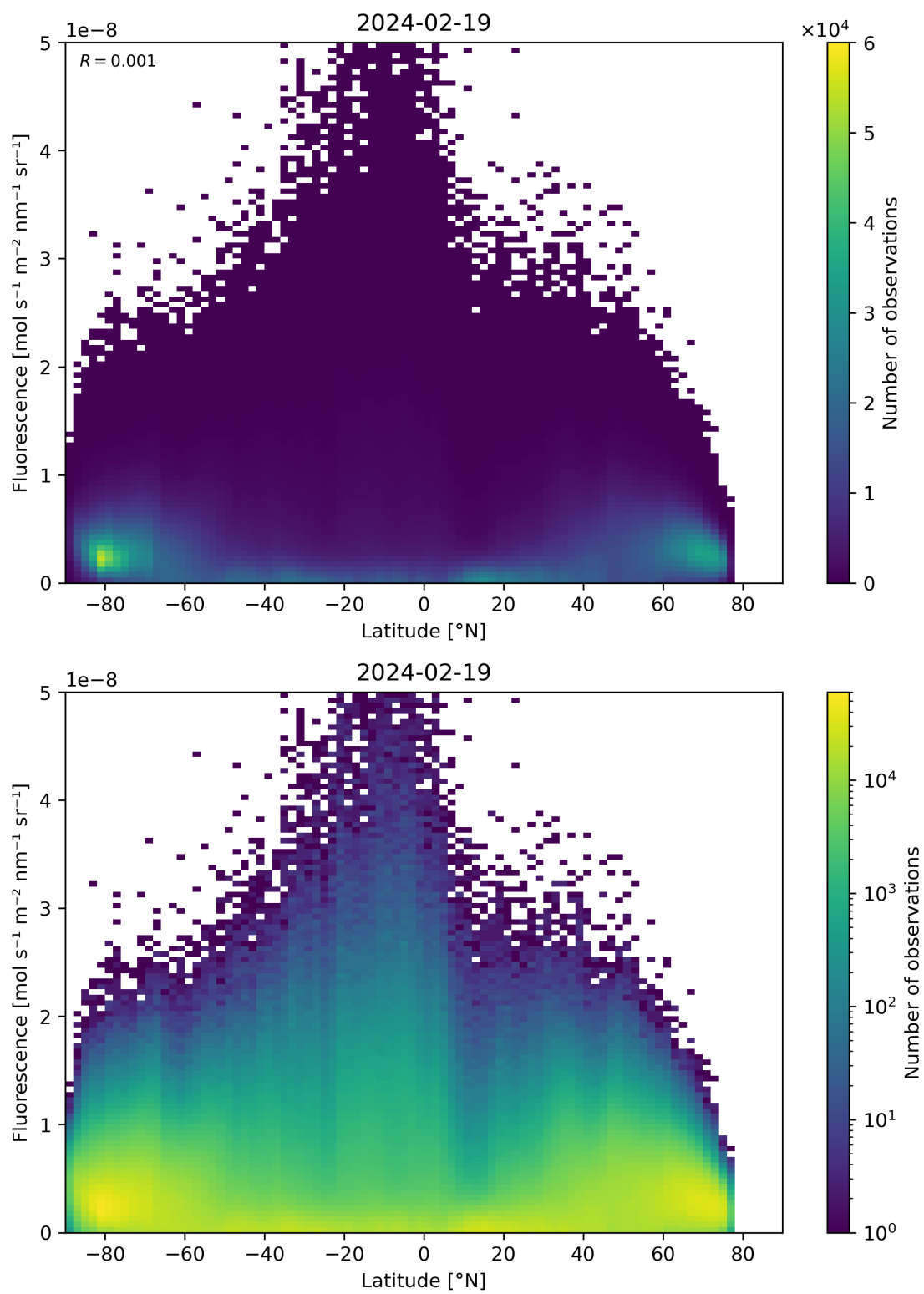
Figure 92: Scatter density plot of “Latitude” against “Fluorescence” for 2024-02-18 to 2024-02-20.
