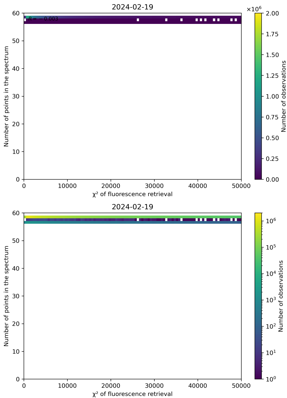
Figure 68: Scatter density plot of " \chi^2 of fluorescence retrieval" against "Number of points in the spectrum" for 2024-02-18 to 2024-02-20.
