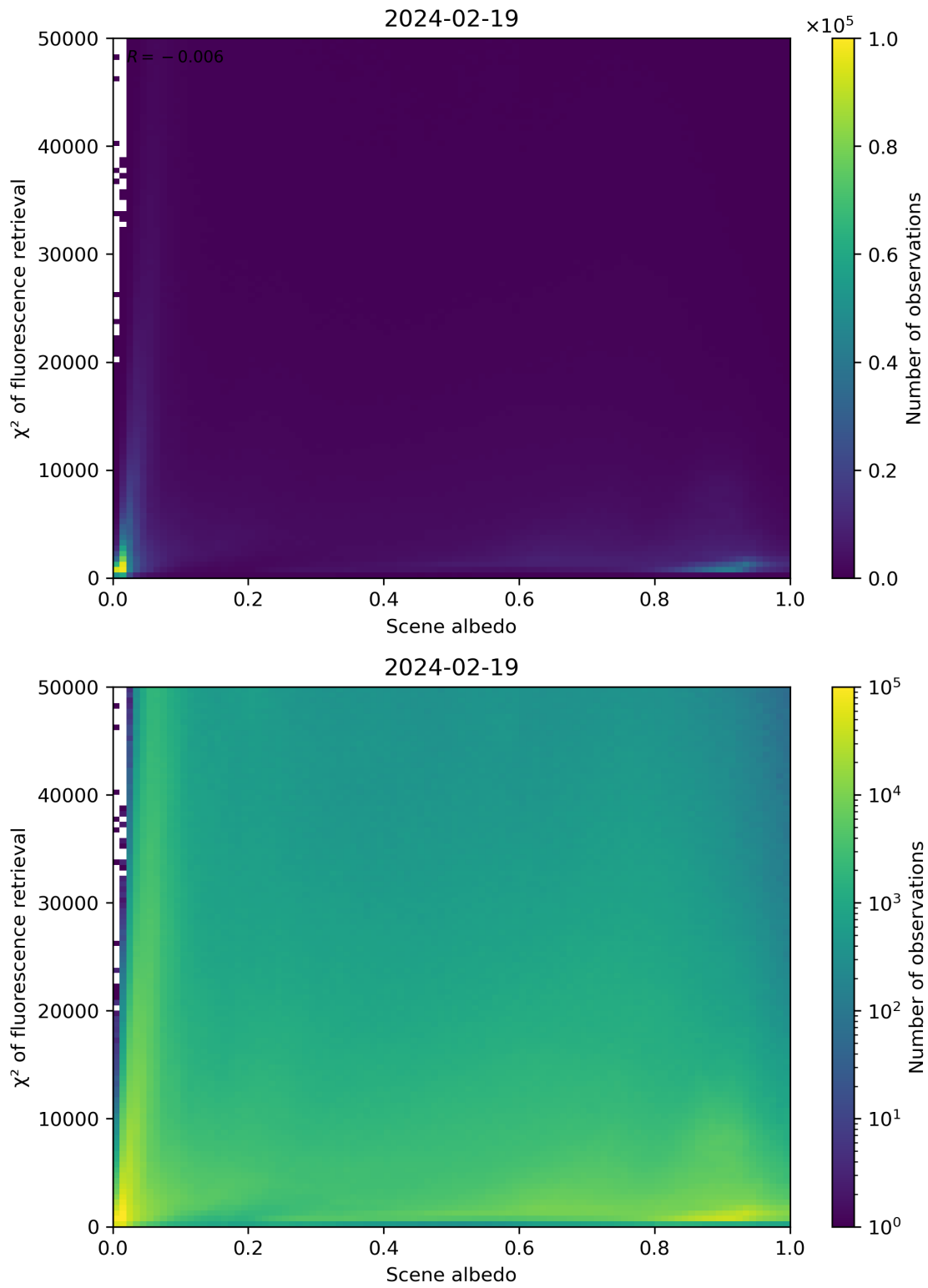
Figure 103: Scatter density plot of “Scene albedo” against “ \chi^2 of fluorescence retrieval” for 2024-02-18 to 2024-02-20.
