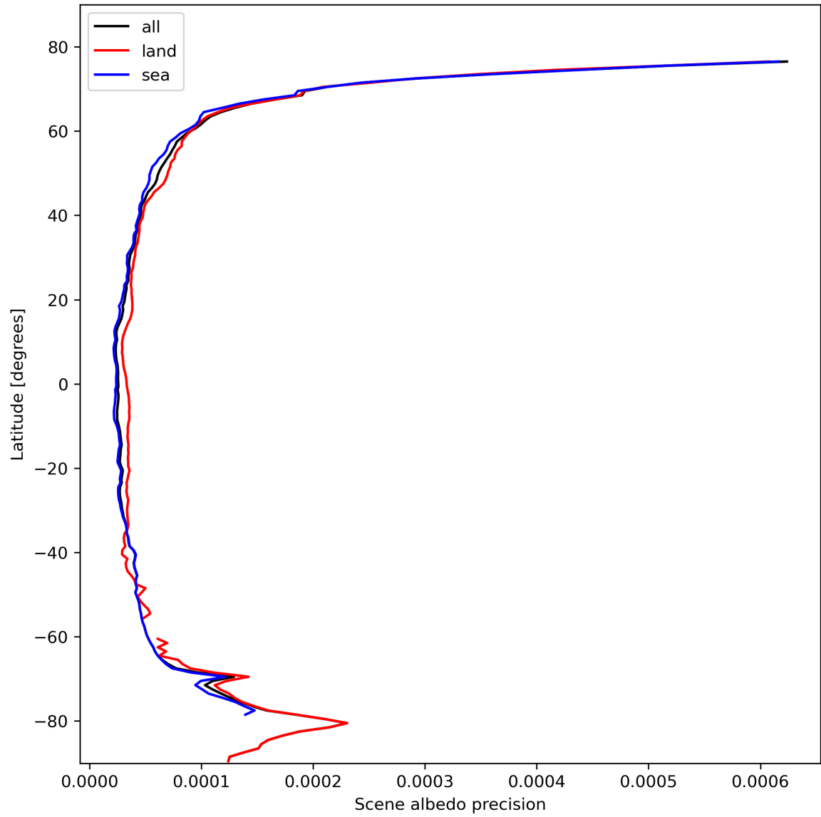
Figure 18: Zonal average of “Scene albedo precision” for 2024-02-18 to 2024-02-20.
