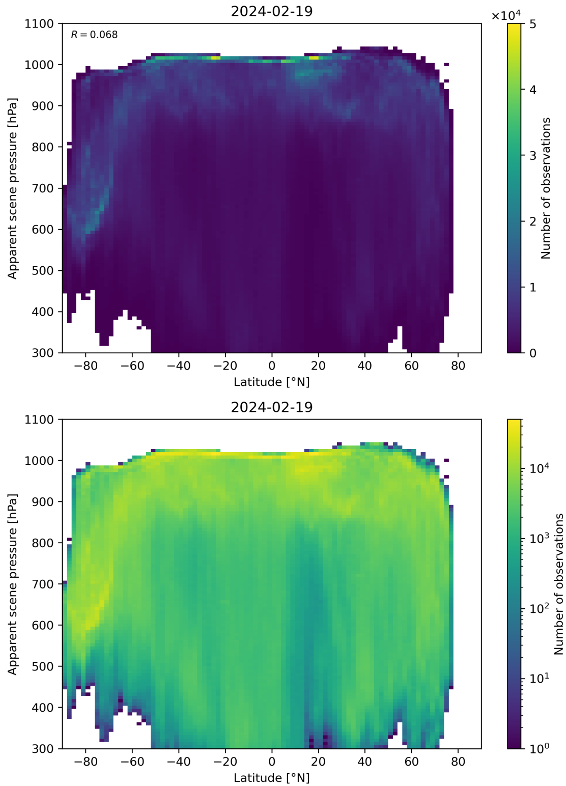
Figure 88: Scatter density plot of “Latitude” against “Apparent scene pressure” for 2024-02-18 to 2024-02-20.
