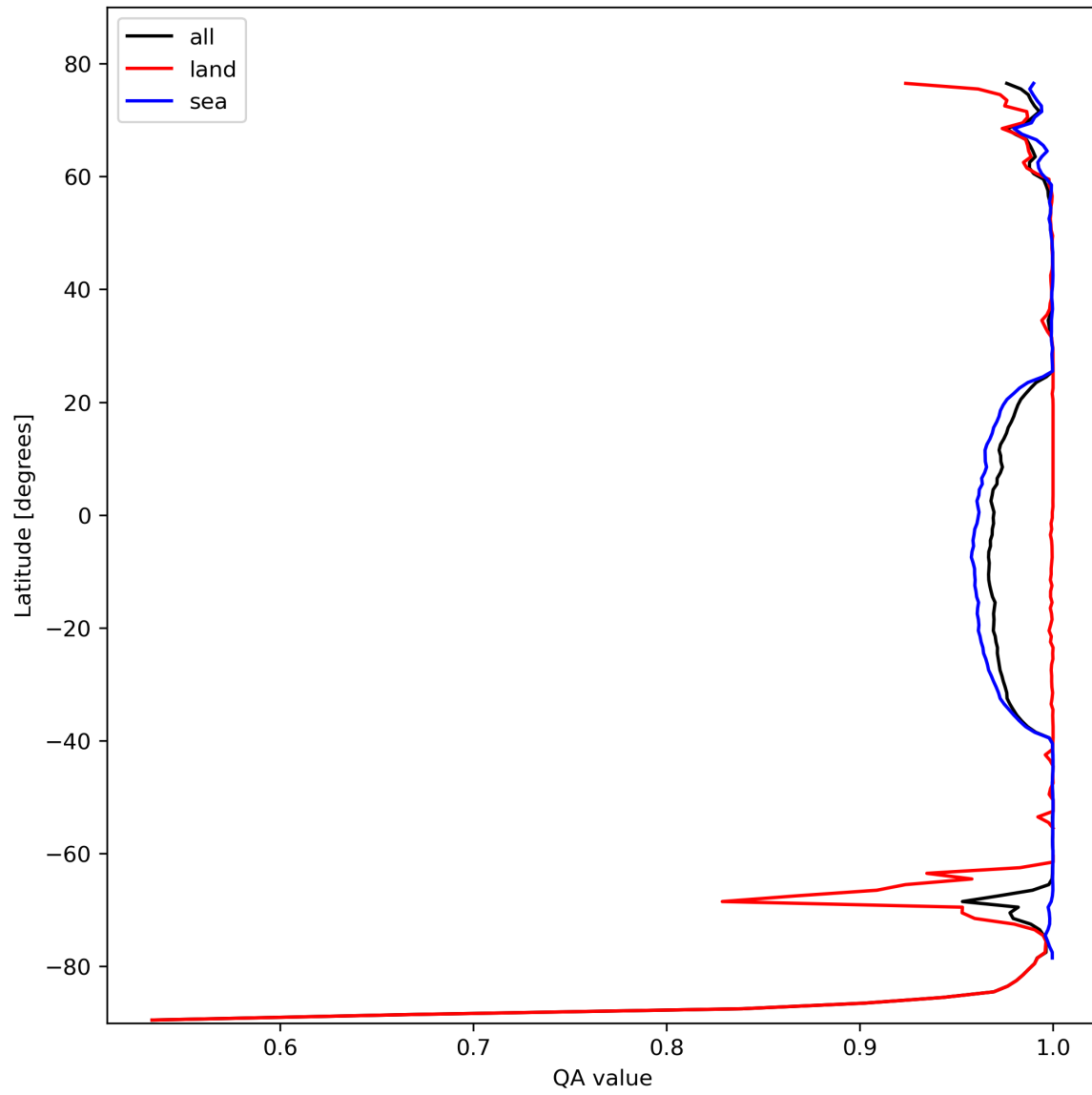
Figure 12: Zonal average of “QA value” for 2024-02-18 to 2024-02-20.
