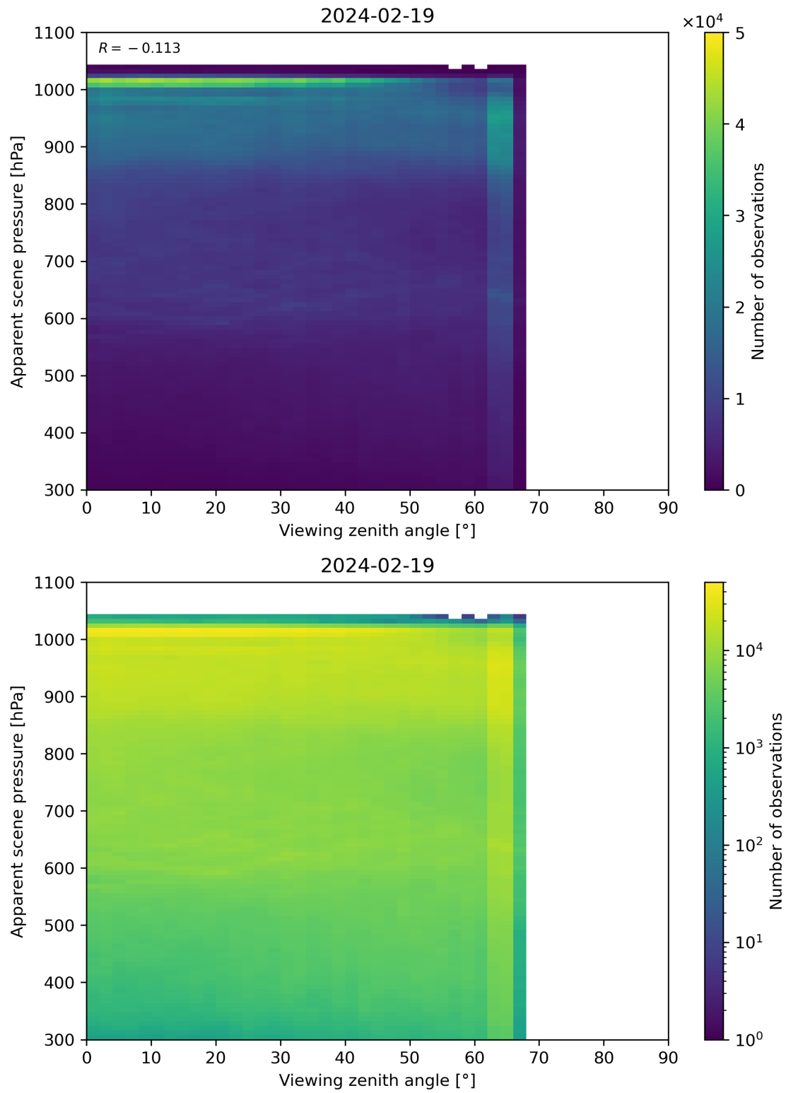
Figure 118: Scatter density plot of “Viewing zenith angle” against “Apparent scene pressure” for 2024-02-18 to 2024-02-20.
