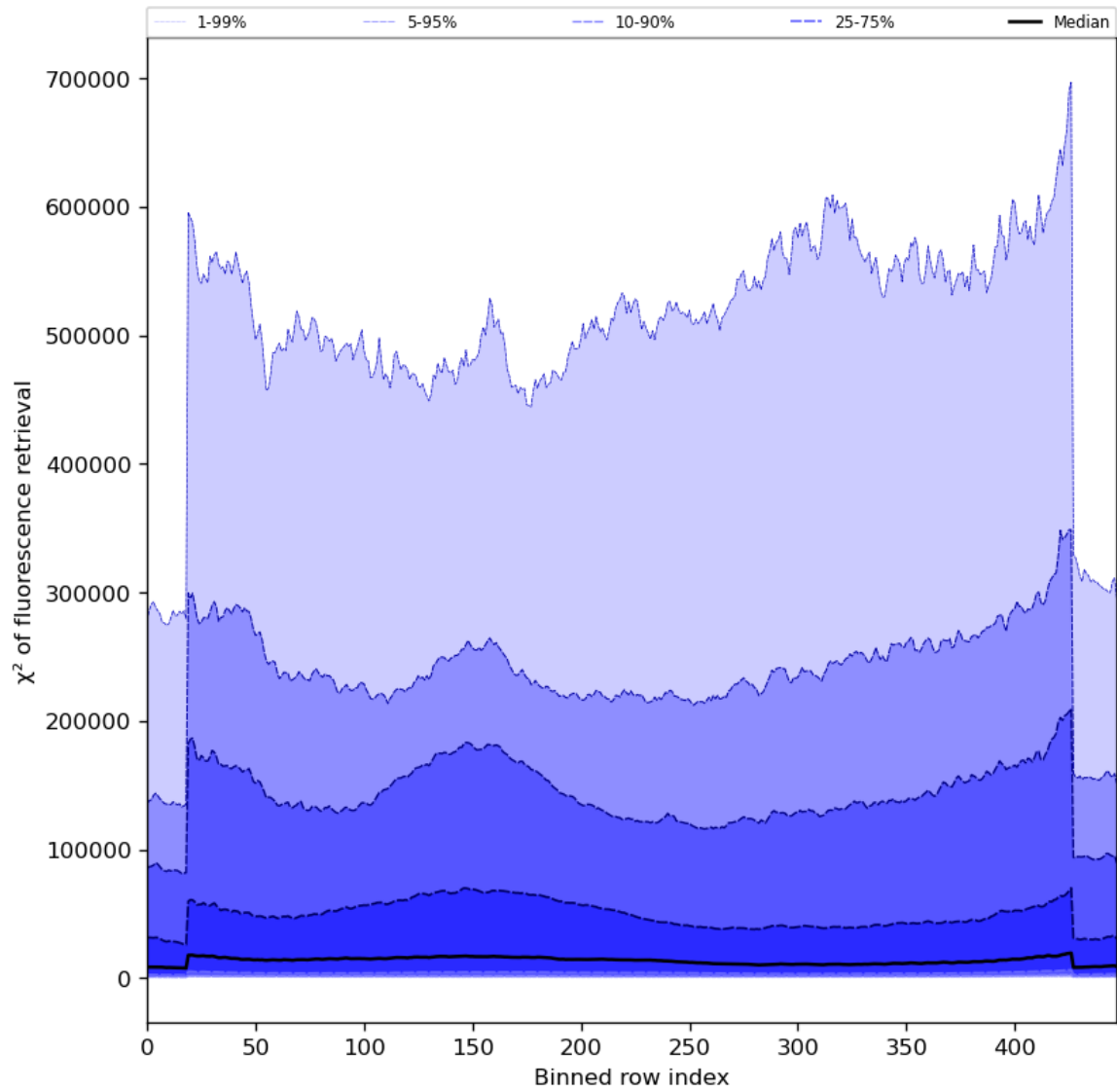
Figure 59: Along track statistics of “ \chi^2 of fluorescence retrieval” for 2024-02-18 to 2024-02-20
