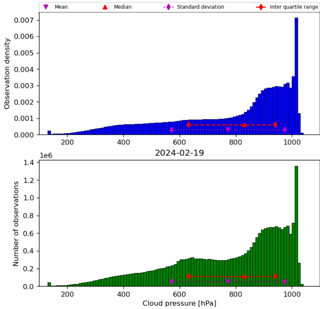
Figure 30: Histogram of “Cloud pressure” for 2024-02-18 to 2024-02-20
