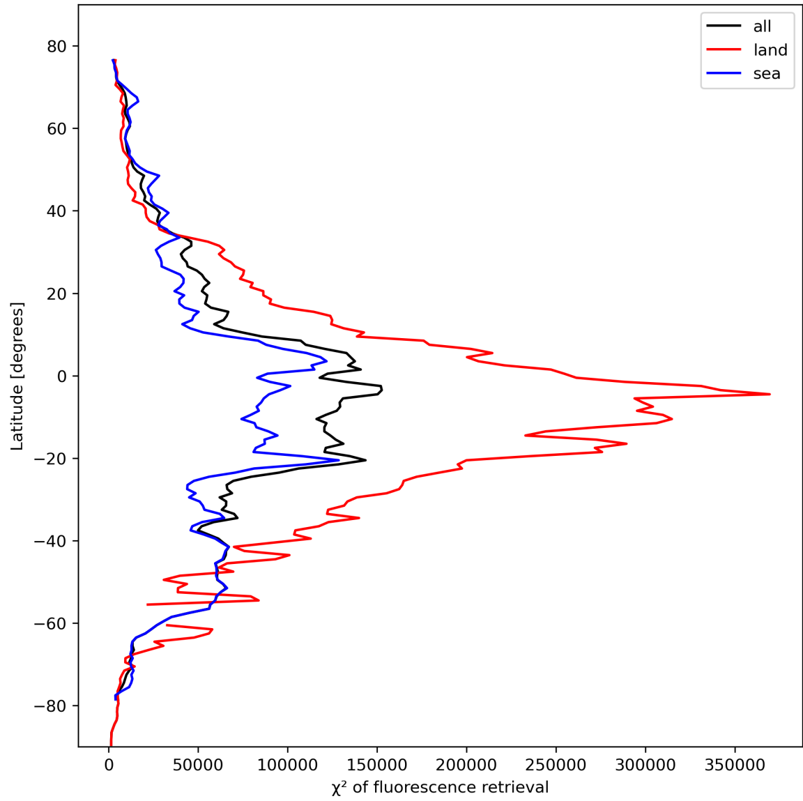
Figure 25: Zonal average of “ \chi^2 of fluorescence retrieval” for 2024-02-18 to 2024-02-20.
