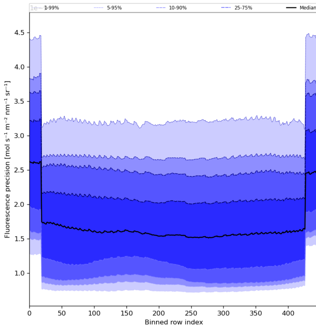
Figure 58: Along track statistics of “Fluorescence precision” for 2024-02-18 to 2024-02-20
