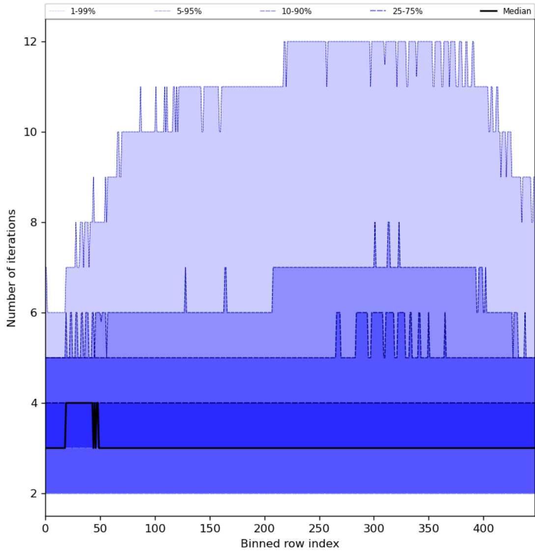
Figure 56: Along track statistics of “Number of iterations” for 2024-02-18 to 2024-02-20
