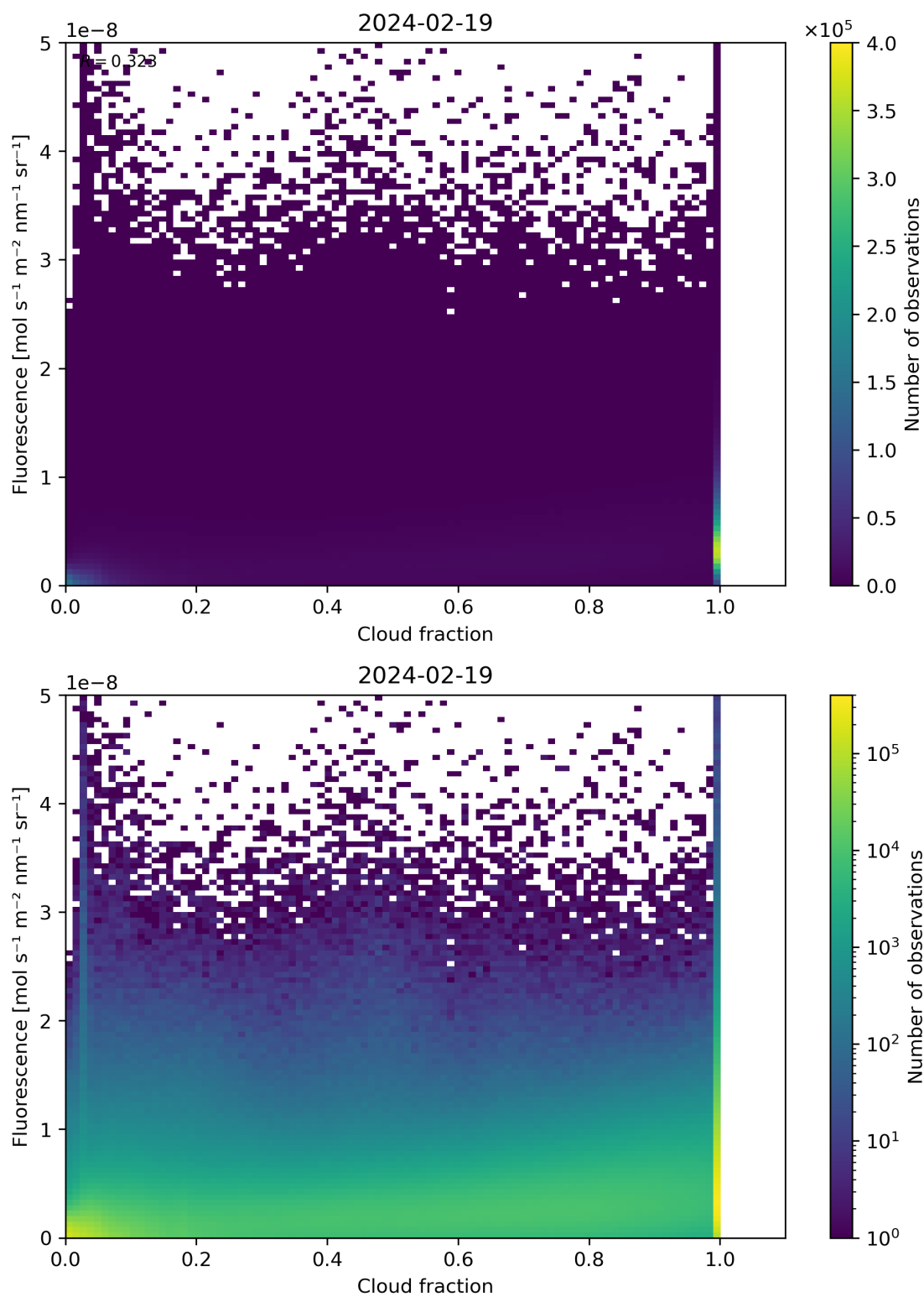
Figure 72: Scatter density plot of “Cloud fraction” against “Fluorescence” for 2024-02-18 to 2024-02-20.
