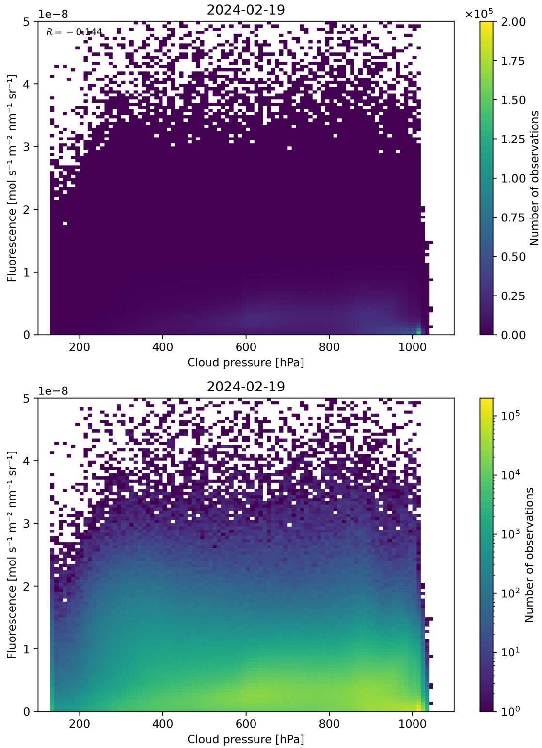
Figure 80: Scatter density plot of “Cloud pressure” against “Fluorescence” for 2024-02-18 to 2024-02-20.
