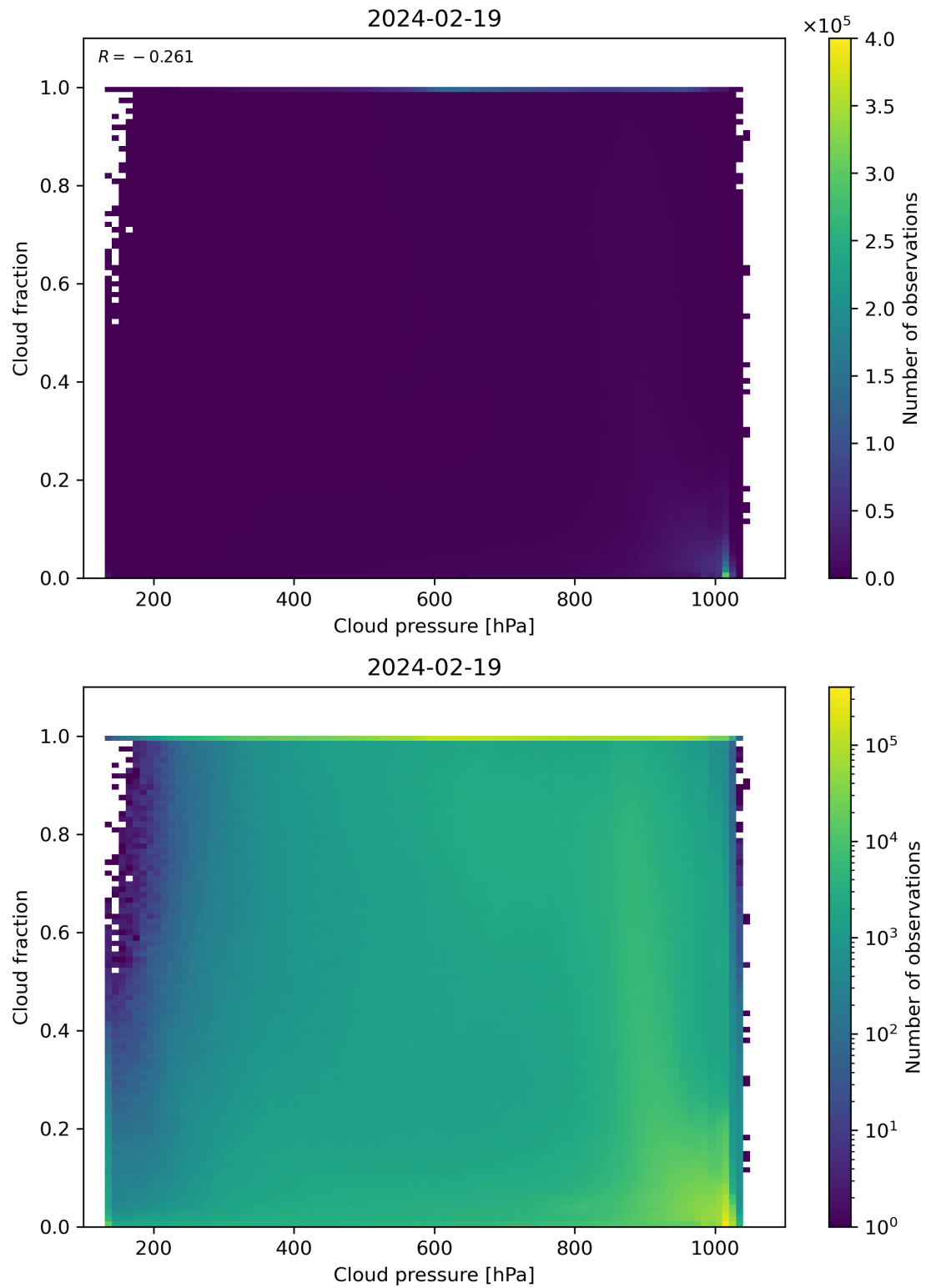
Figure 79: Scatter density plot of “Cloud pressure” against “Cloud fraction” for 2024-02-18 to 2024-02-20.
