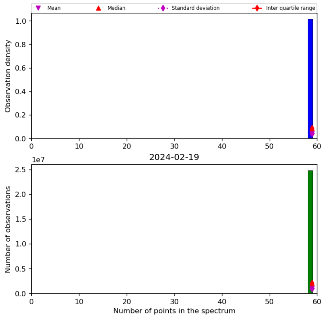
Figure 44: Histogram of “Number of points in the spectrum” for 2024-02-18 to 2024-02-20
