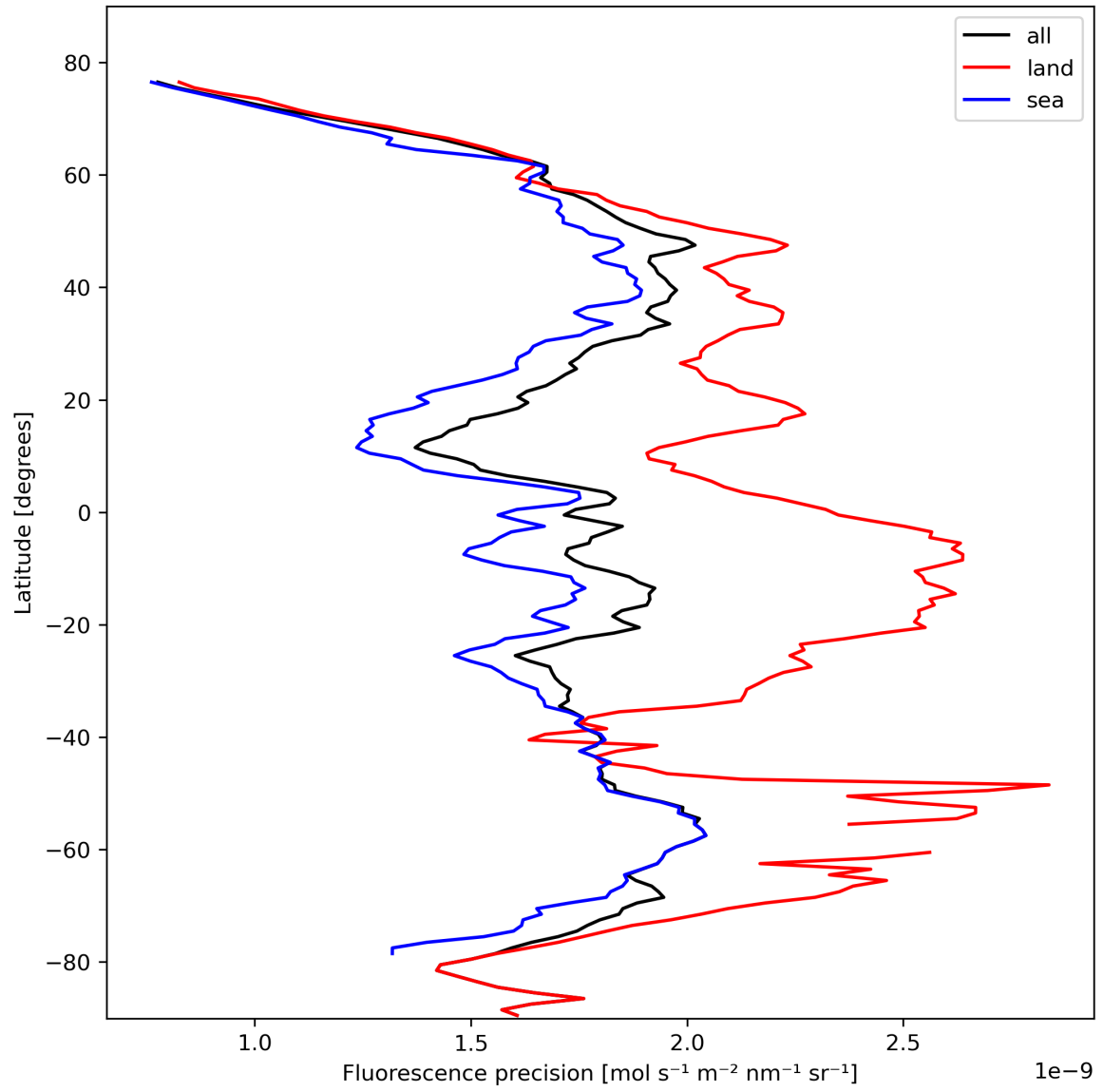
Figure 24: Zonal average of “Fluorescence precision” for 2024-02-18 to 2024-02-20.
