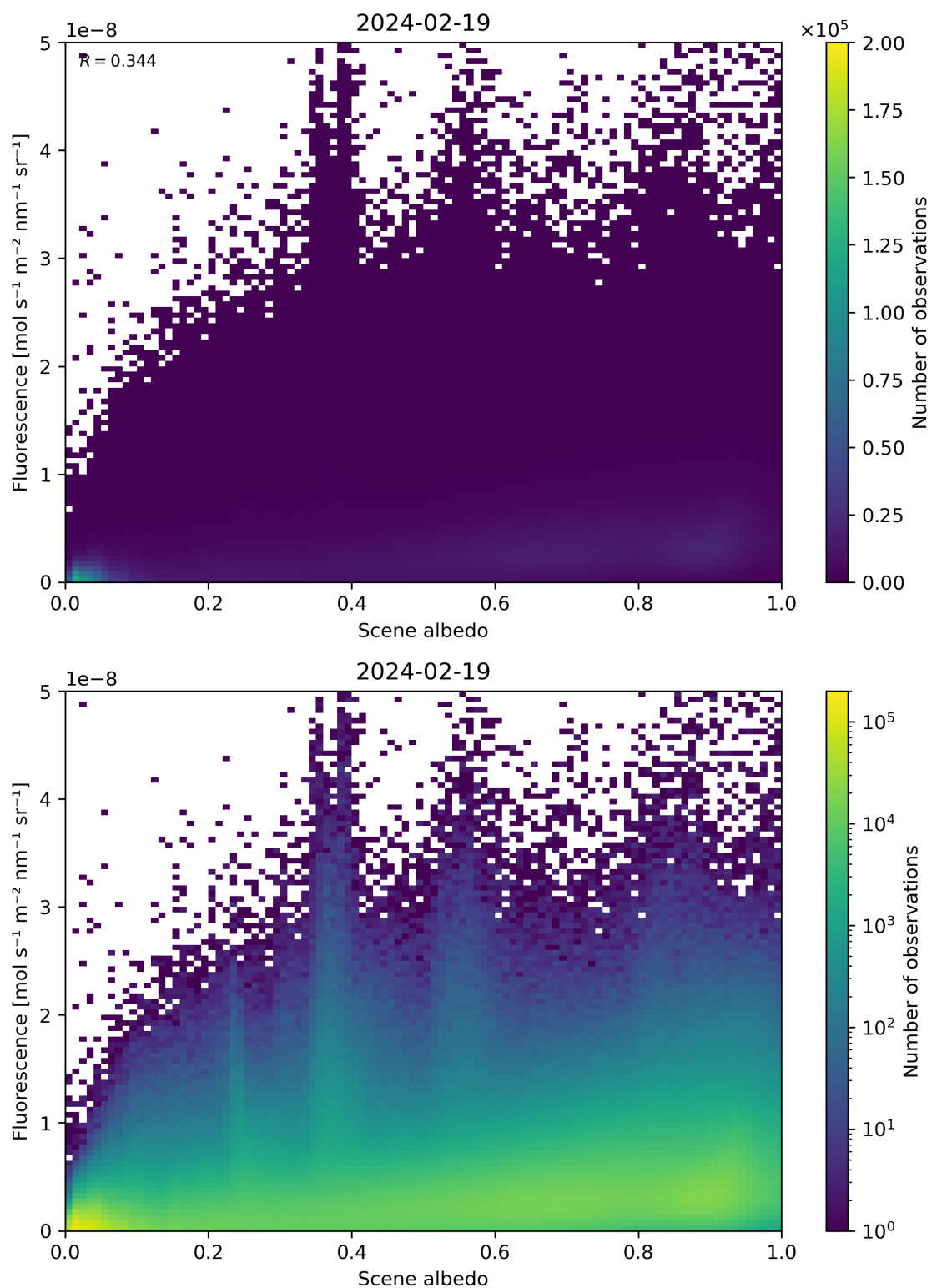
Figure 104: Scatter density plot of “Scene albedo” against “Fluorescence” for 2024-02-18 to 2024-02-20.
