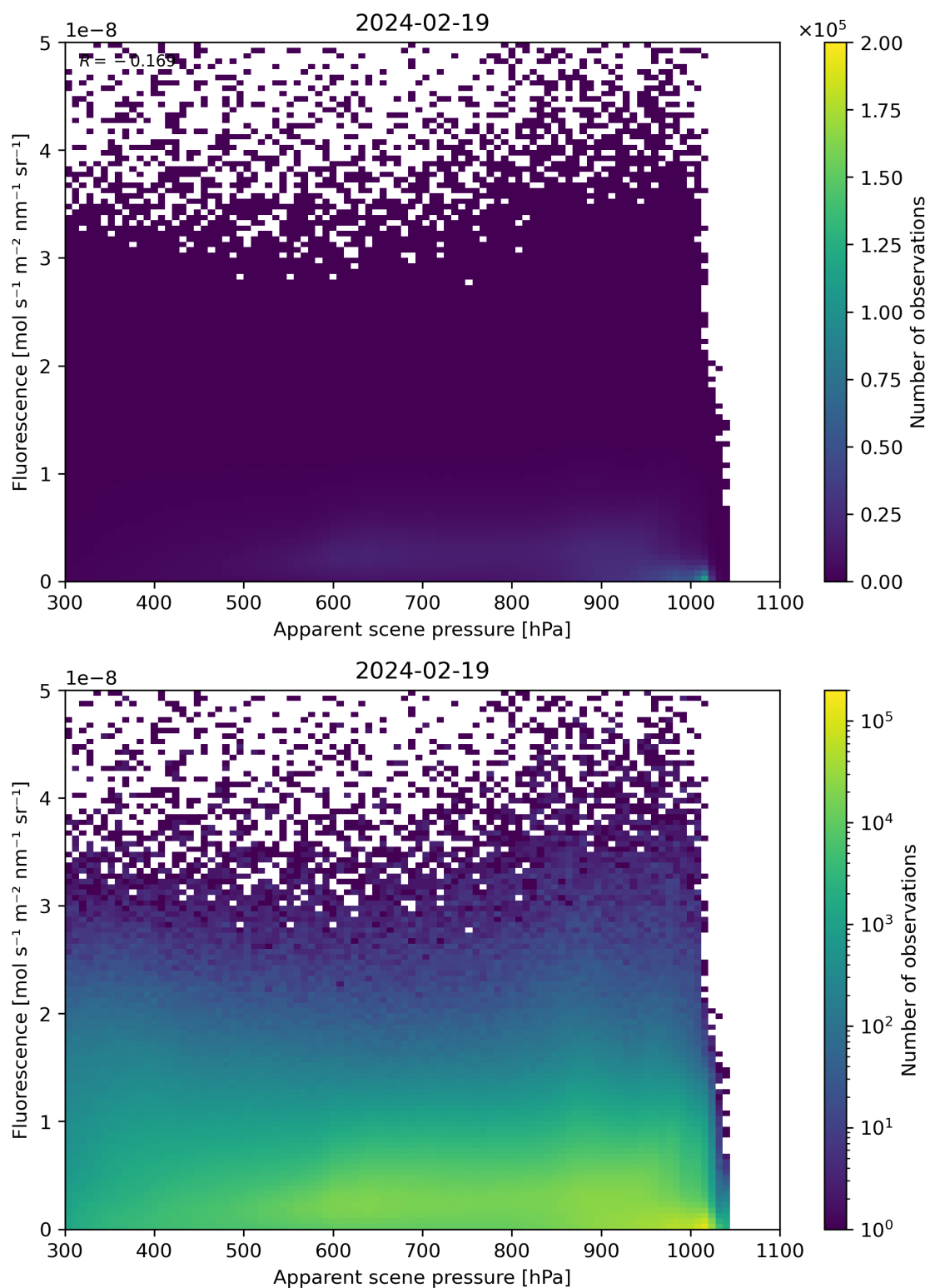
Figure 64: Scatter density plot of “Apparent scene pressure” against “Fluorescence” for 2024-02-18 to 2024-02-20.
