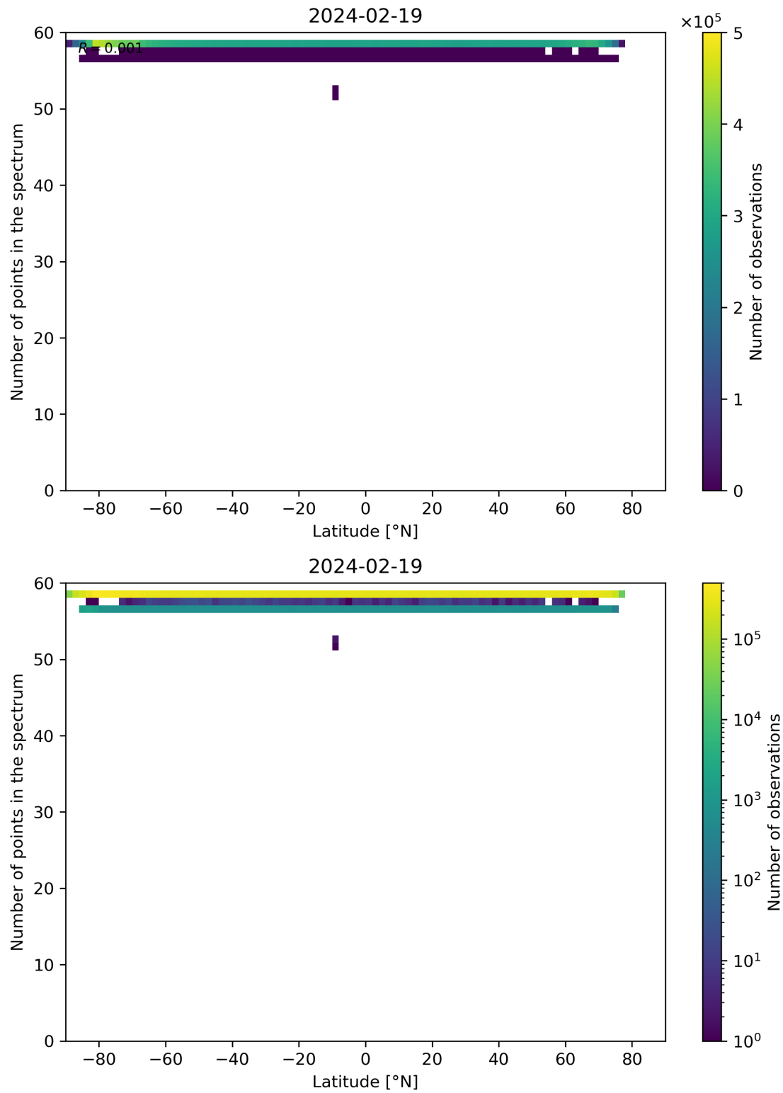
Figure 94: Scatter density plot of “Latitude” against “Number of points in the spectrum” for 2024-02-18 to 2024-02-20.
