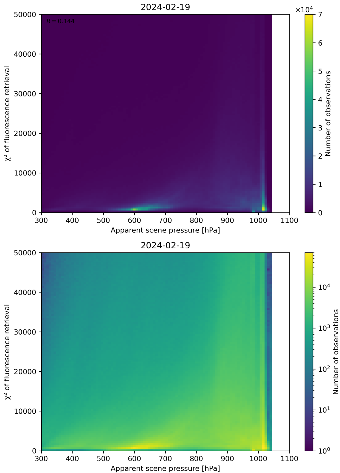
Figure 63: Scatter density plot of “Apparent scene pressure” against “ \chi^2 of fluorescence retrieval” for 2024-02-18 to 2024-02-20.
