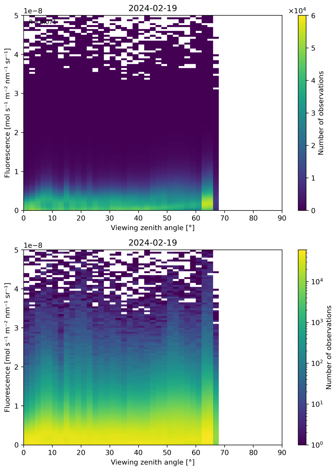
Figure 122: Scatter density plot of “Viewing zenith angle” against “Fluorescence” for 2024-02-18 to 2024-02-20.
