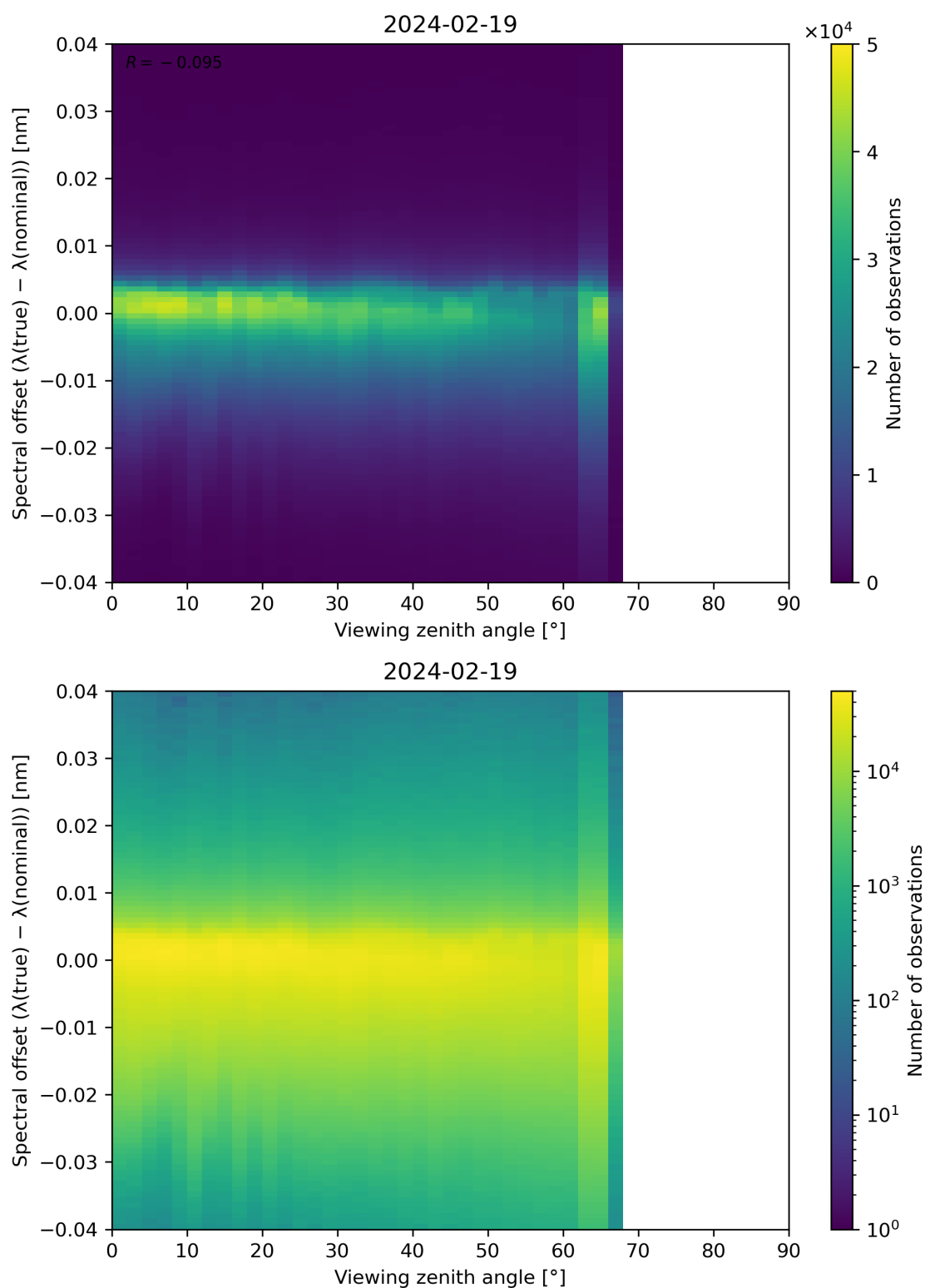
Figure 128: Scatter density plot of “Viewing zenith angle” against “Spectral offset ( \lambda(\text{true}) - \lambda(\text{nominal}) )” for 2024-02-18 to 2024-02-20.
