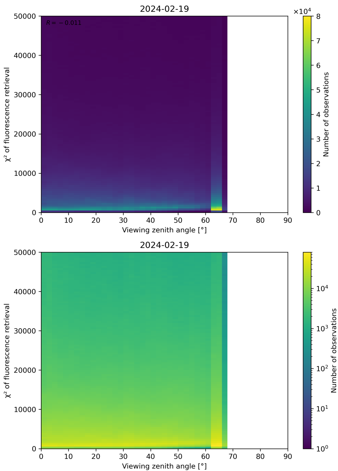
Figure 119: Scatter density plot of “Viewing zenith angle” against “ \chi^2 of fluorescence retrieval” for 2024-02-18 to 2024-02-20.
