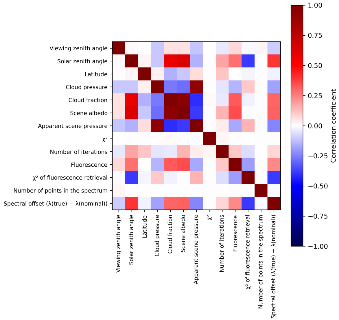
Figure 2: Map of correlation matrix for 2024-02-18 to 2024-02-20.
