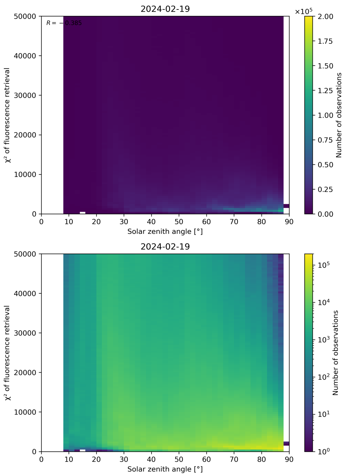
Figure 109: Scatter density plot of “Solar zenith angle” against “ \chi^2 of fluorescence retrieval” for 2024-02-18 to 2024-02-20.
