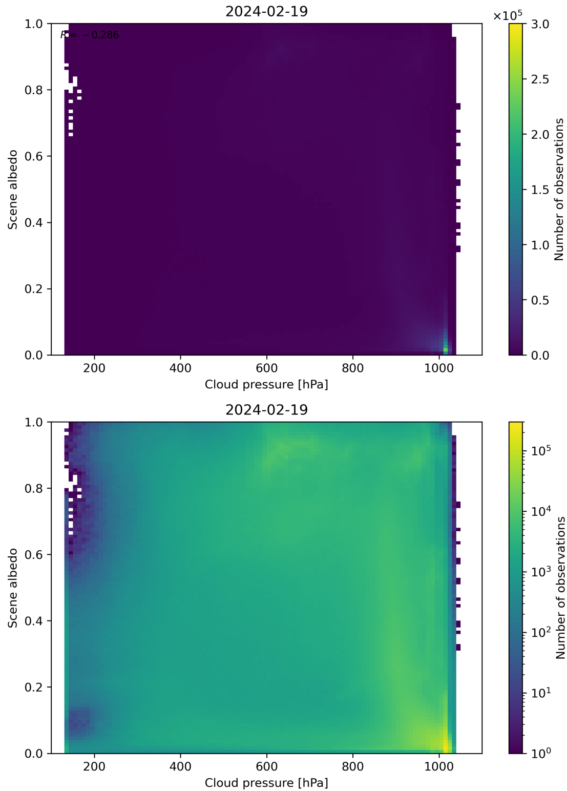
Figure 83: Scatter density plot of “Cloud pressure” against “Scene albedo” for 2024-02-18 to 2024-02-20.
