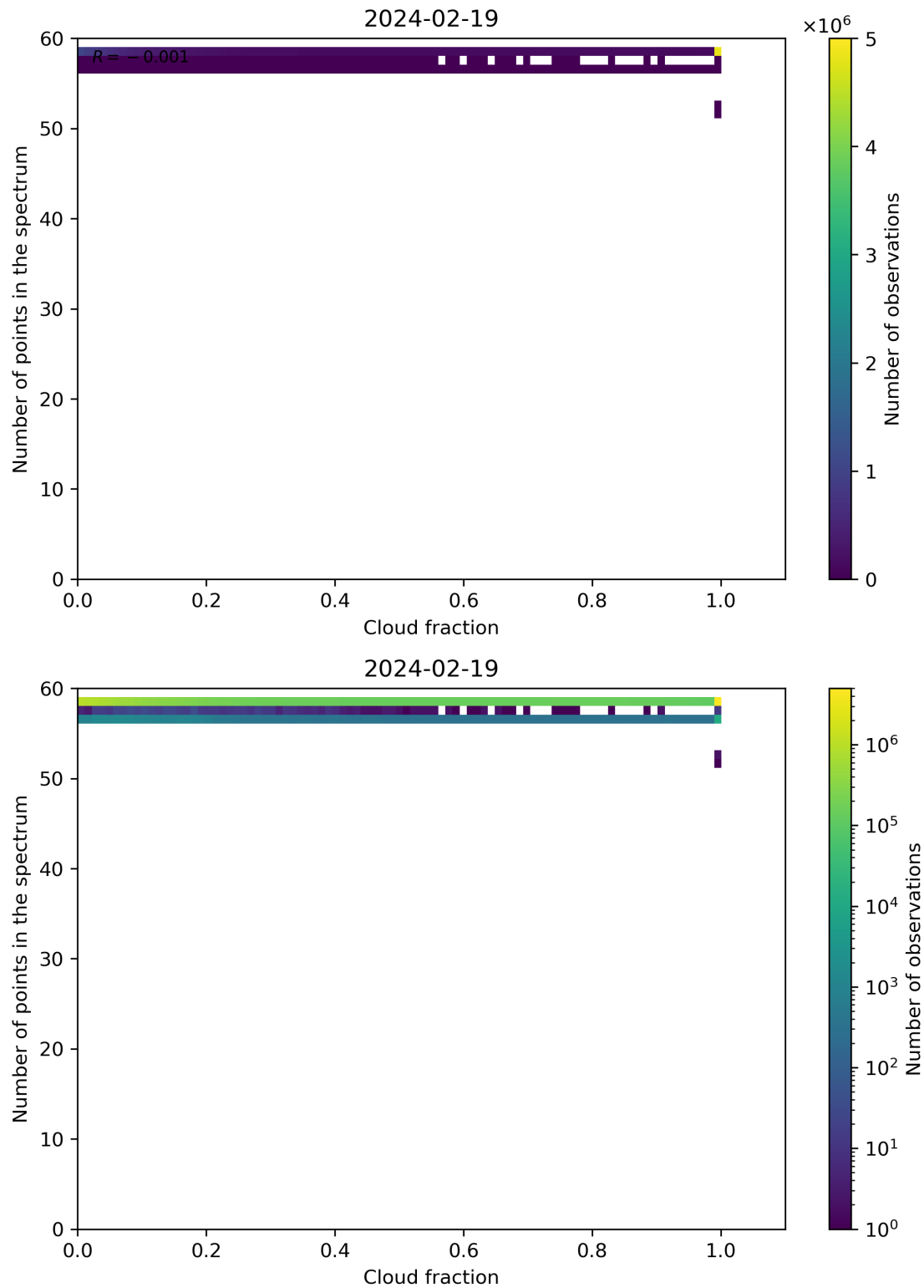
Figure 74: Scatter density plot of “Cloud fraction” against “Number of points in the spectrum” for 2024-02-18 to 2024-02-20.
