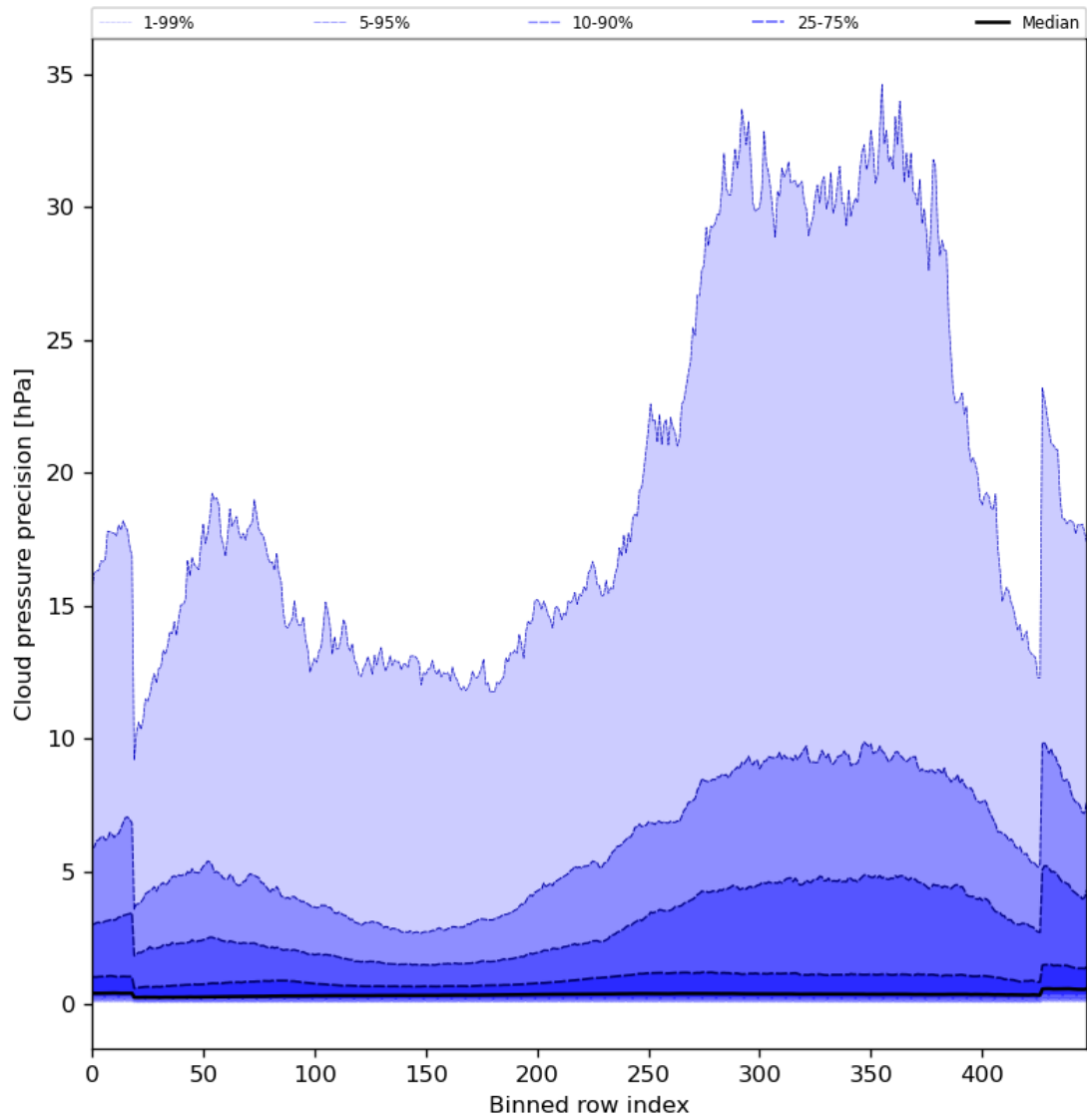
Figure 48: Along track statistics of “Cloud pressure precision” for 2024-02-18 to 2024-02-20
