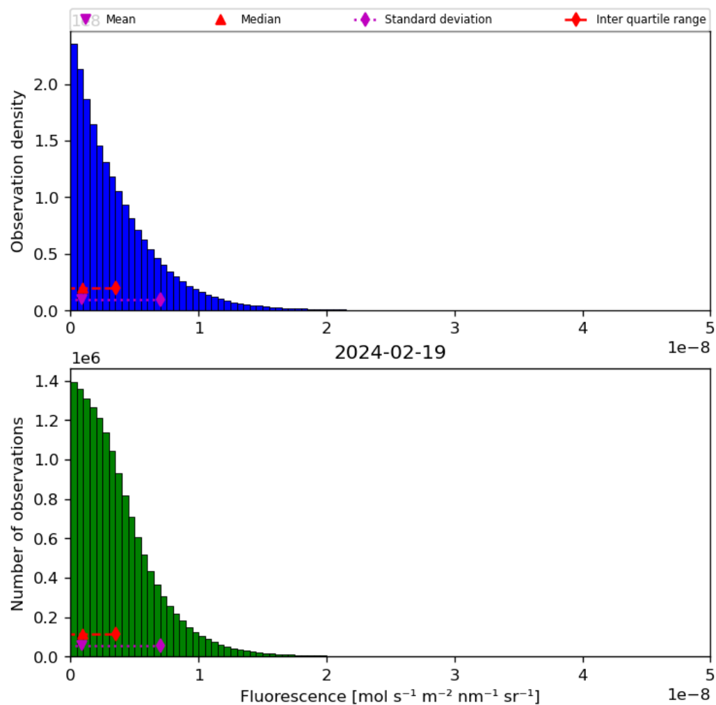
Figure 40: Histogram of “Fluorescence” for 2024-02-18 to 2024-02-20
