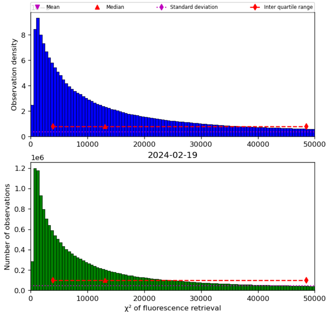
Figure 42: Histogram of “ \chi^2 of fluorescence retrieval” for 2024-02-18 to 2024-02-20
