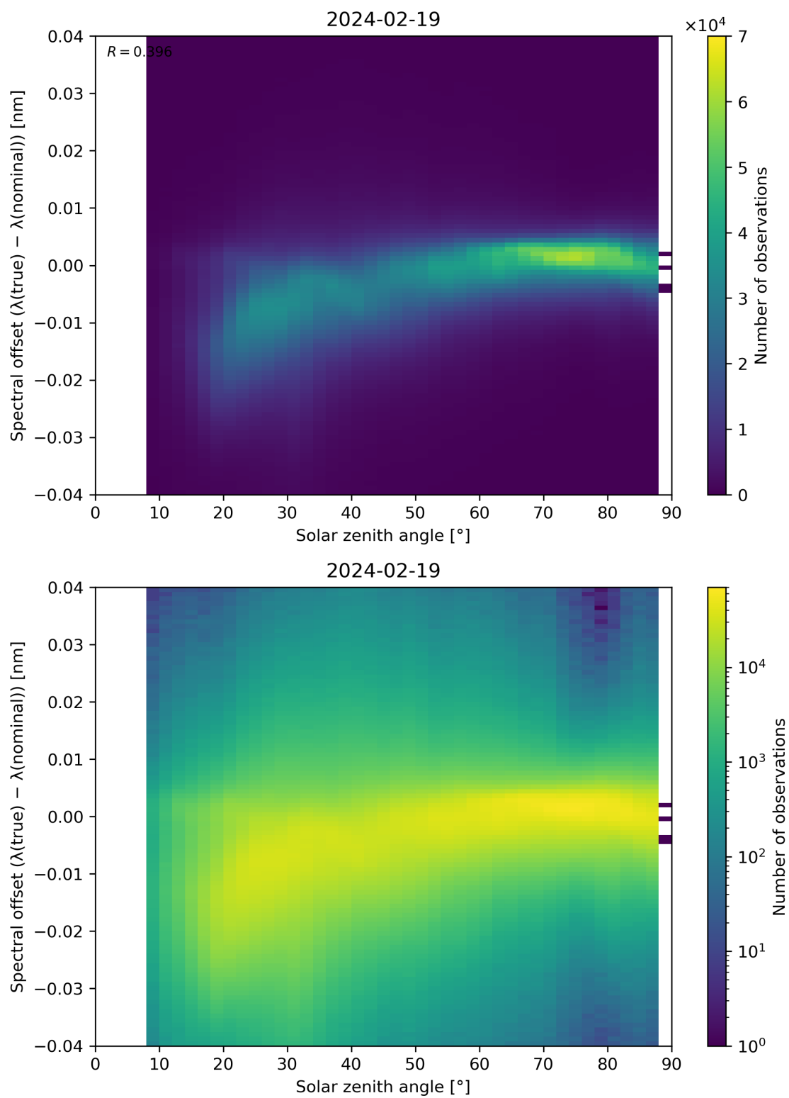
Figure 117: Scatter density plot of “Solar zenith angle” against “Spectral offset ( \lambda(\text{true}) - \lambda(\text{nominal}) )” for 2024-02-18 to 2024-02-20.
