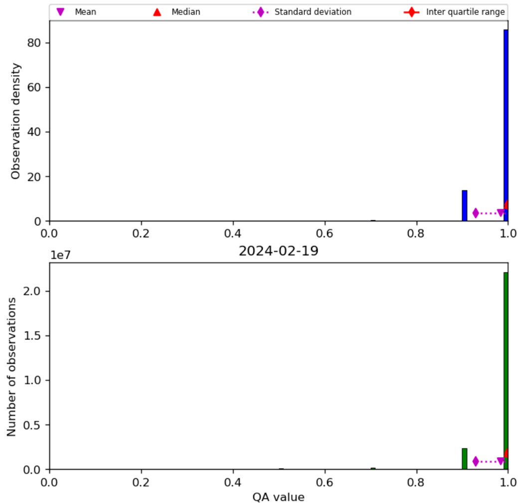
Figure 29: Histogram of “QA value” for 2024-02-18 to 2024-02-20
