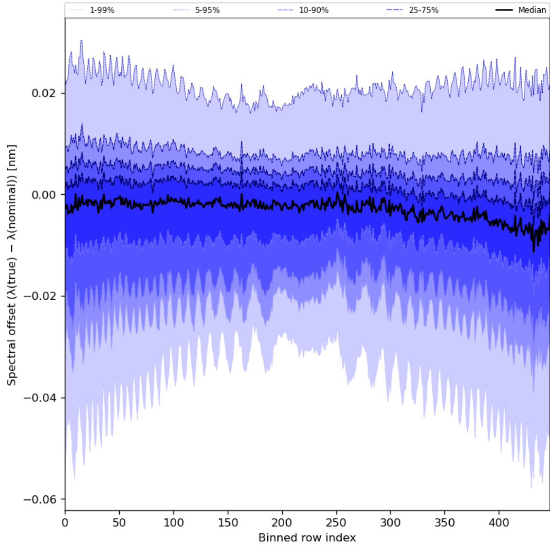
Figure 62: Along track statistics of “Spectral offset ( \lambda(\text{true}) - \lambda(\text{nominal}) )” for 2024-02-18 to 2024-02-20
