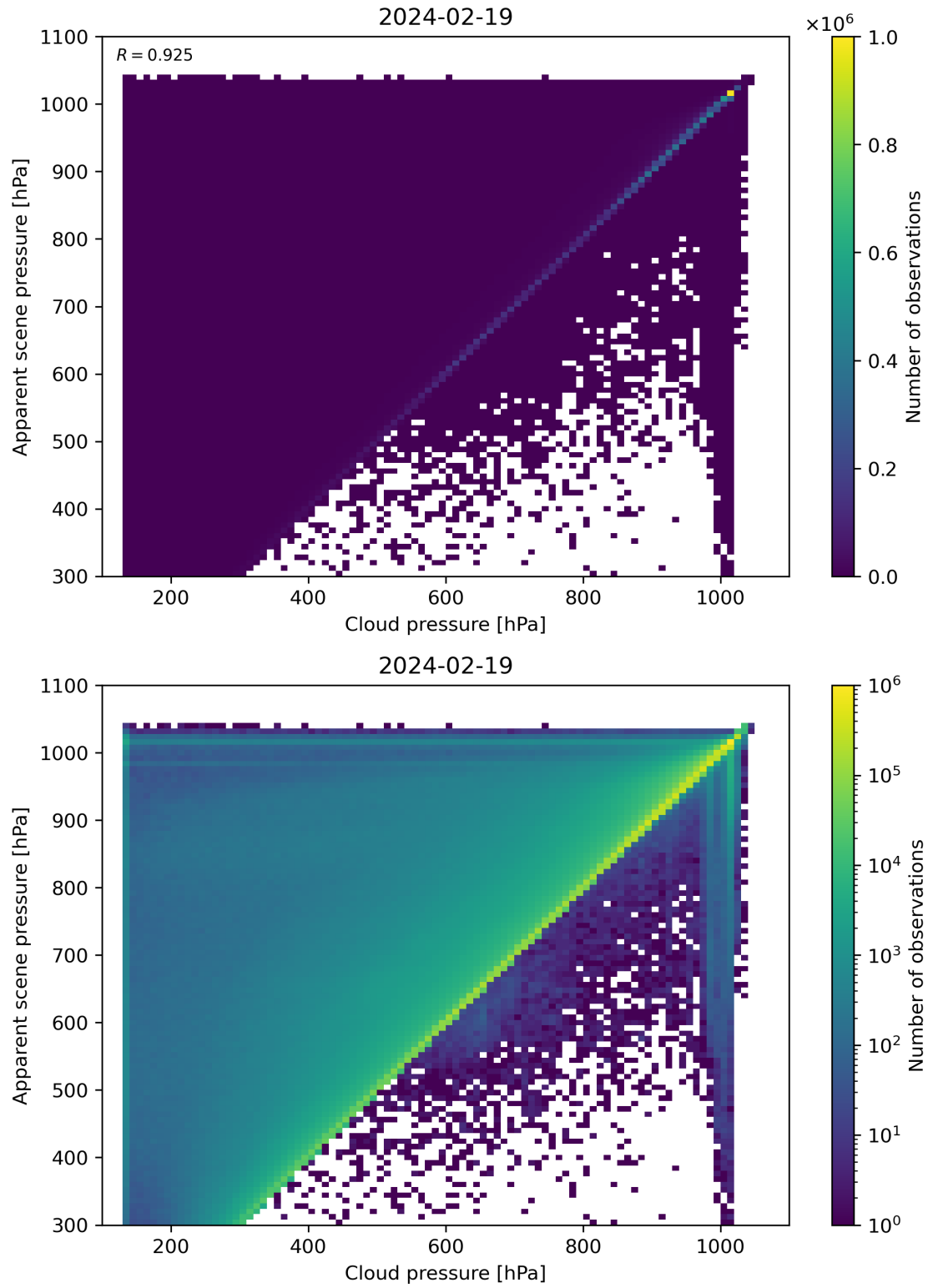
Figure 77: Scatter density plot of “Cloud pressure” against “Apparent scene pressure” for 2024-02-18 to 2024-02-20.
