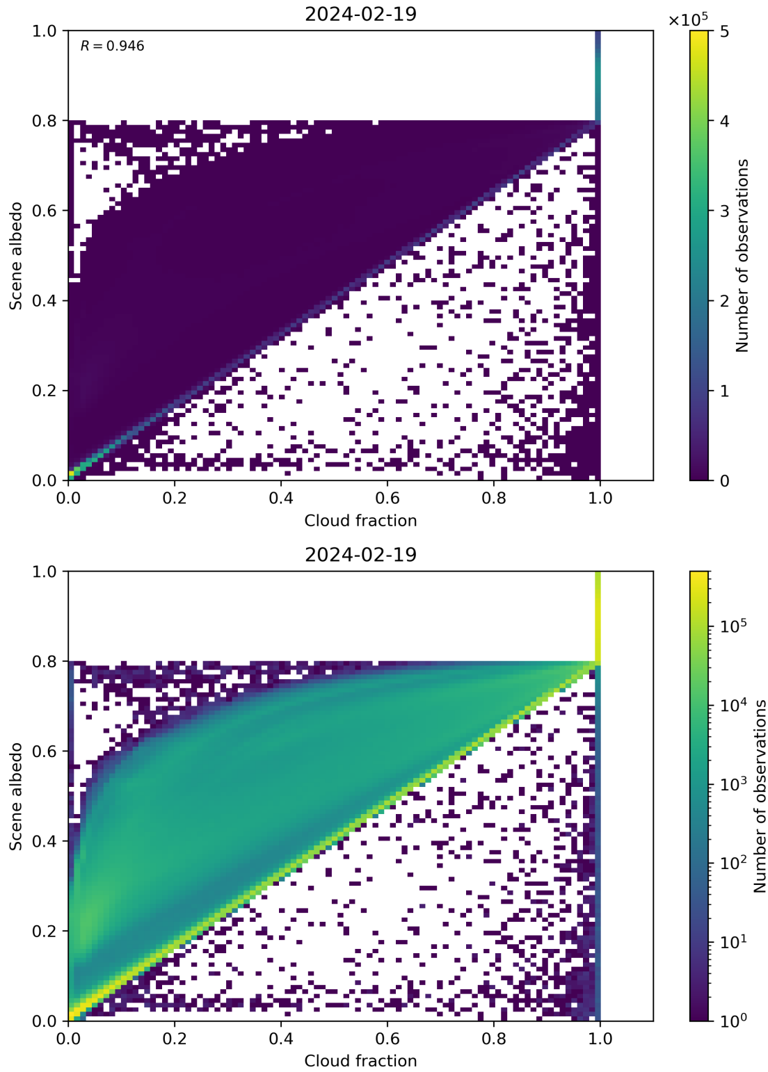
Figure 75: Scatter density plot of “Cloud fraction” against “Scene albedo” for 2024-02-18 to 2024-02-20.
