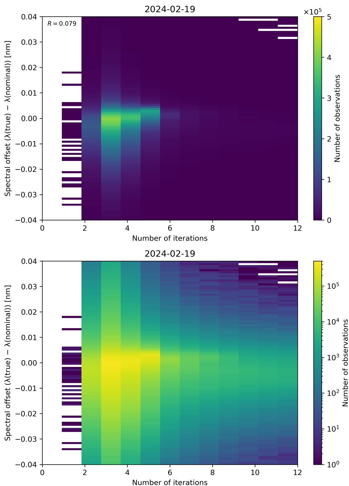
Figure 100: Scatter density plot of “Number of iterations” against “Spectral offset ( \lambda(\text{true}) - \lambda(\text{nominal}) )” for 2024-02-18 to 2024-02-20.
