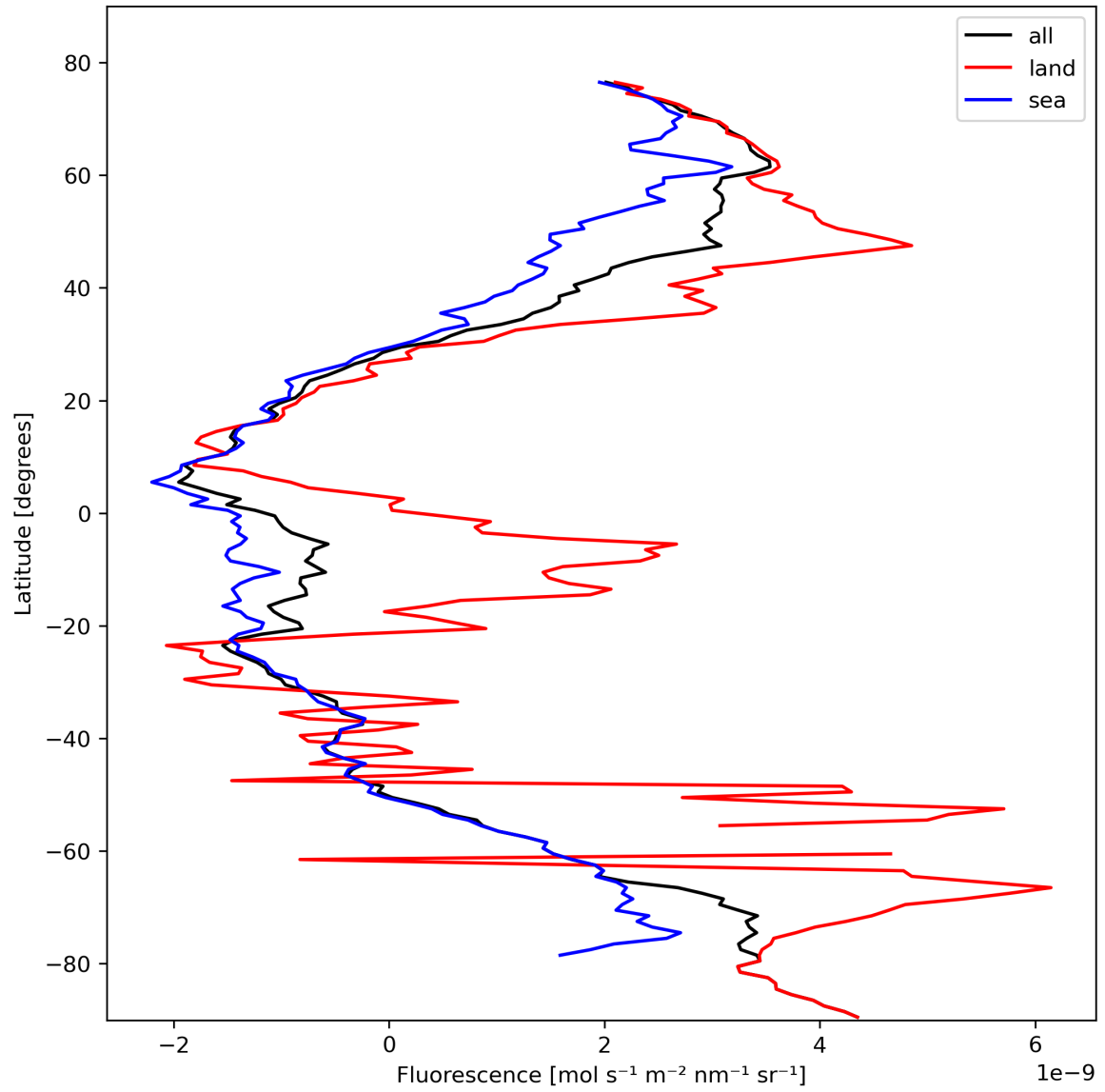
Figure 23: Zonal average of “Fluorescence” for 2024-02-18 to 2024-02-20.
