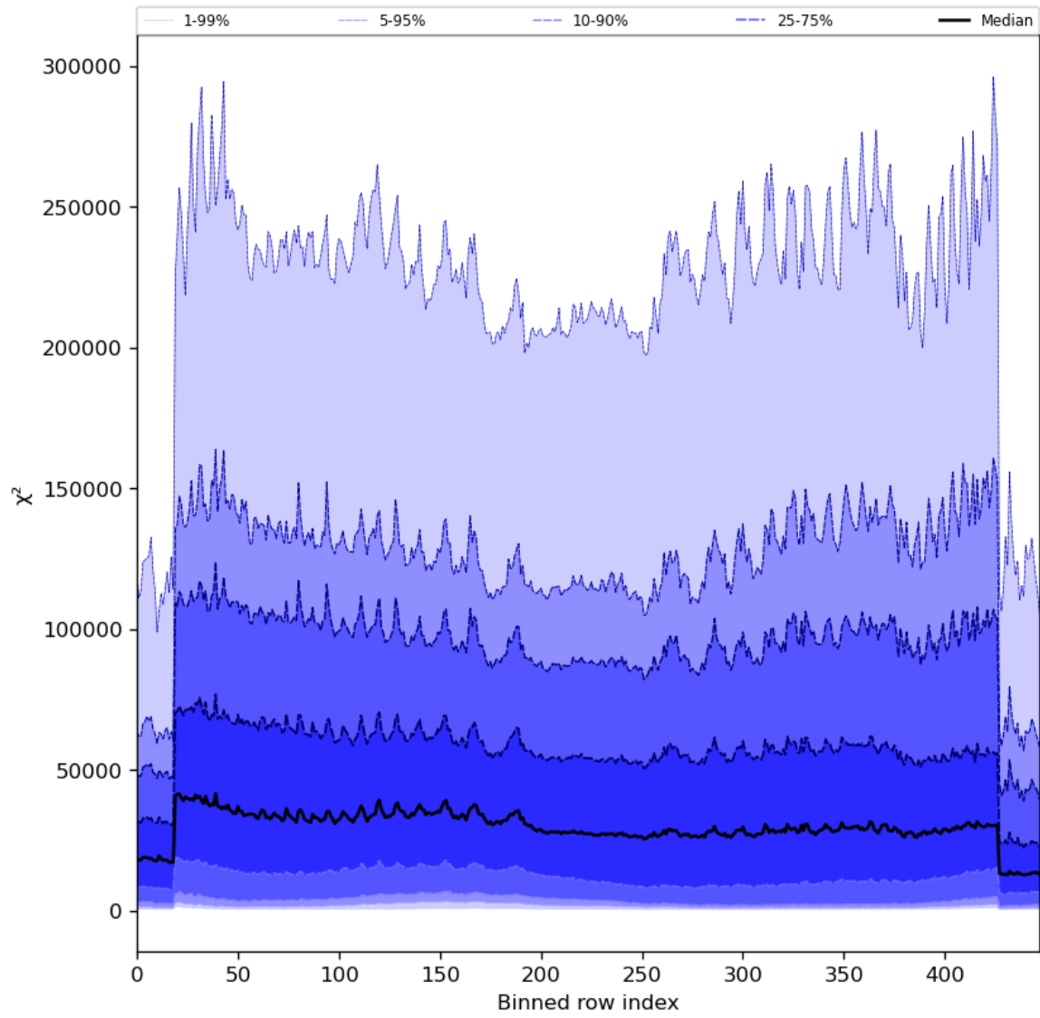
Figure 55: Along track statistics of “ \chi^2 ” for 2024-02-18 to 2024-02-20
