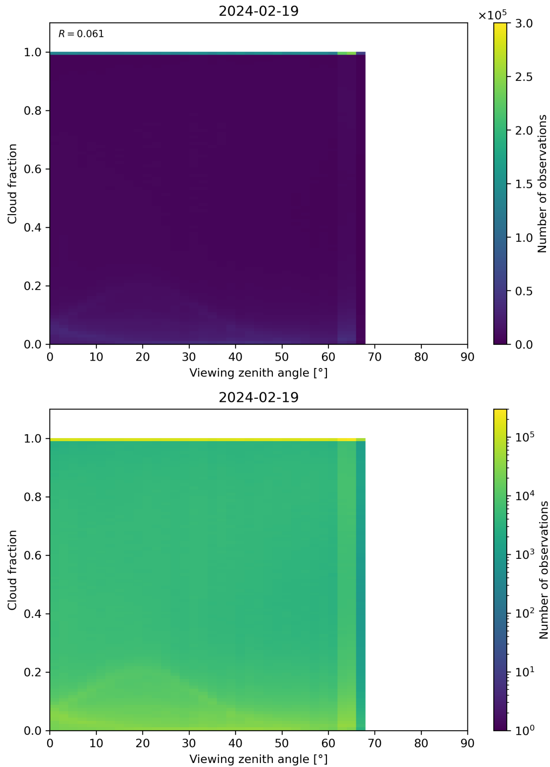
Figure 120: Scatter density plot of “Viewing zenith angle” against “Cloud fraction” for 2024-02-18 to 2024-02-20.
