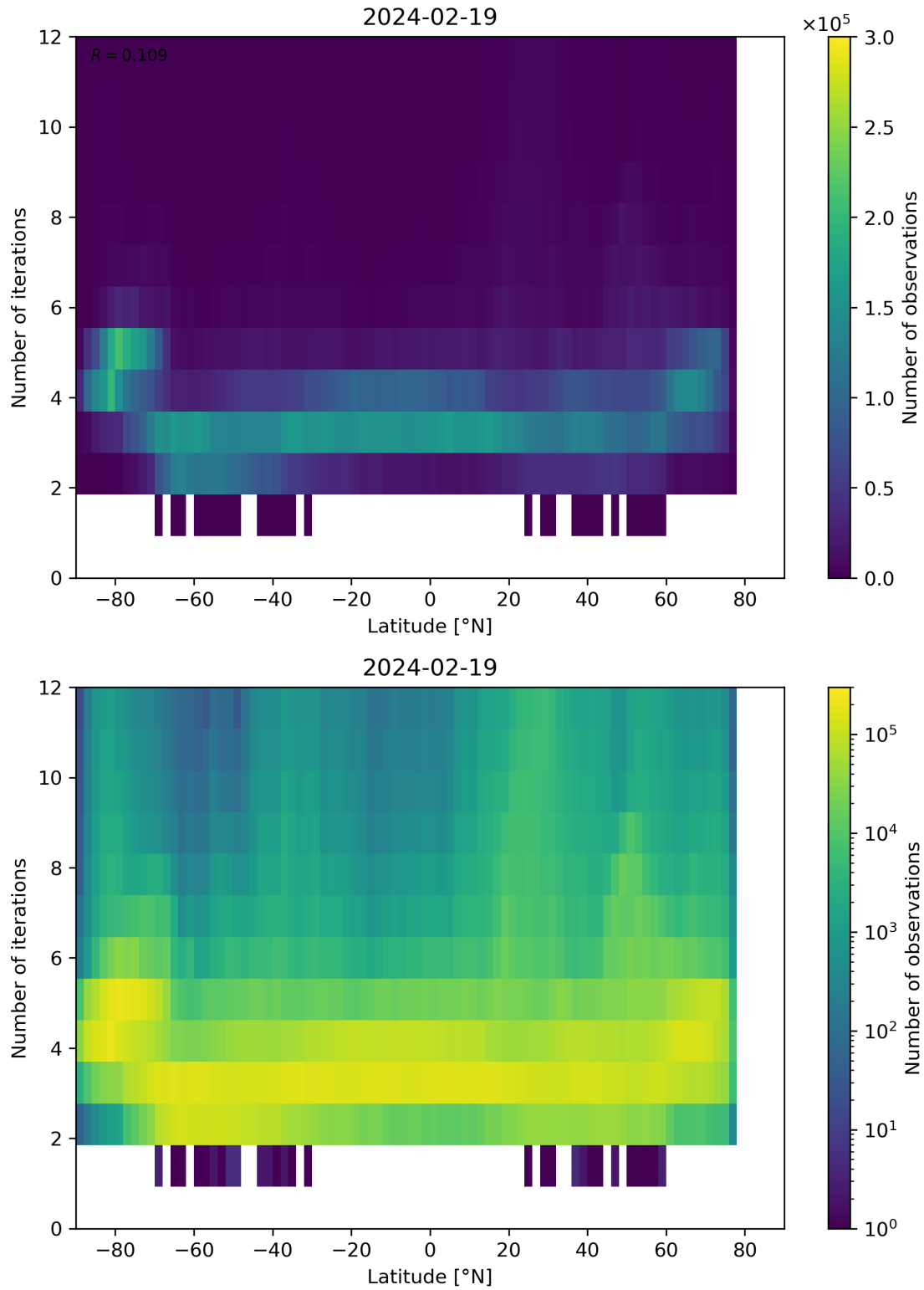
Figure 93: Scatter density plot of “Latitude” against “Number of iterations” for 2024-02-18 to 2024-02-20.
