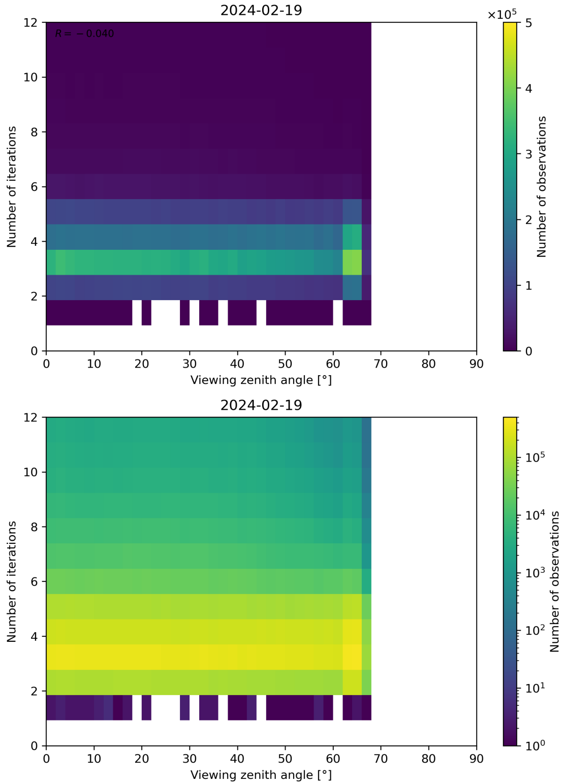
Figure 124: Scatter density plot of “Viewing zenith angle” against “Number of iterations” for 2024-02-18 to 2024-02-20.
