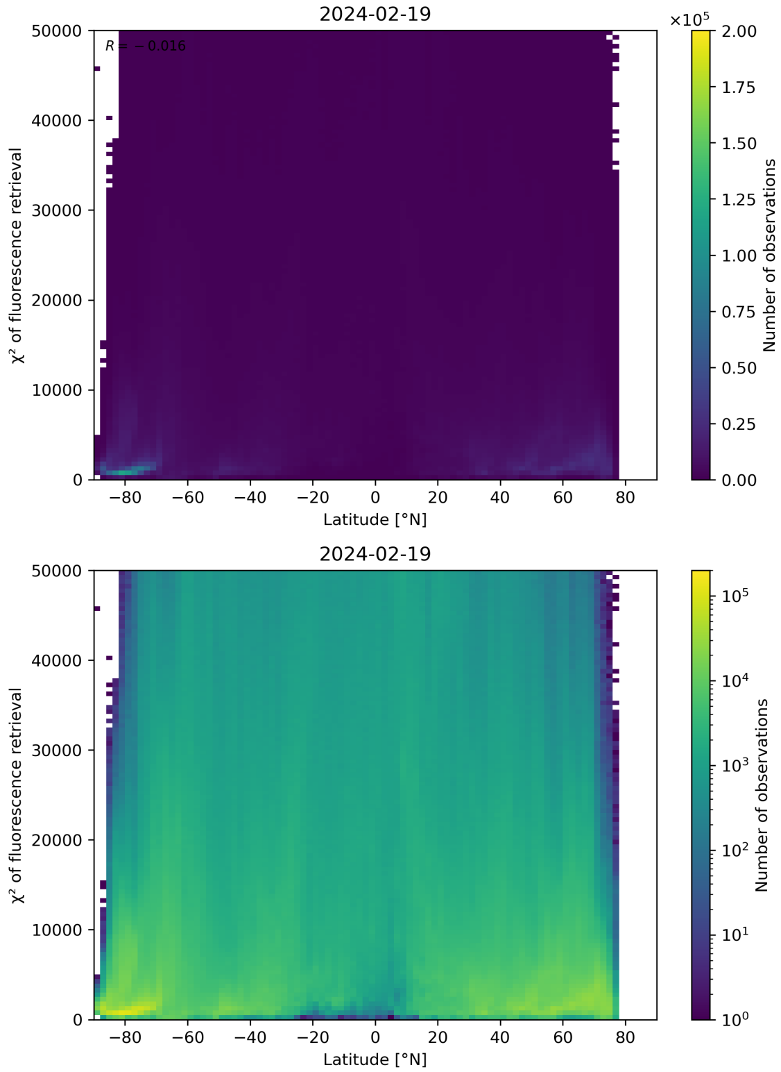
Figure 89: Scatter density plot of “Latitude” against “ \chi^2 of fluorescence retrieval” for 2024-02-18 to 2024-02-20.
