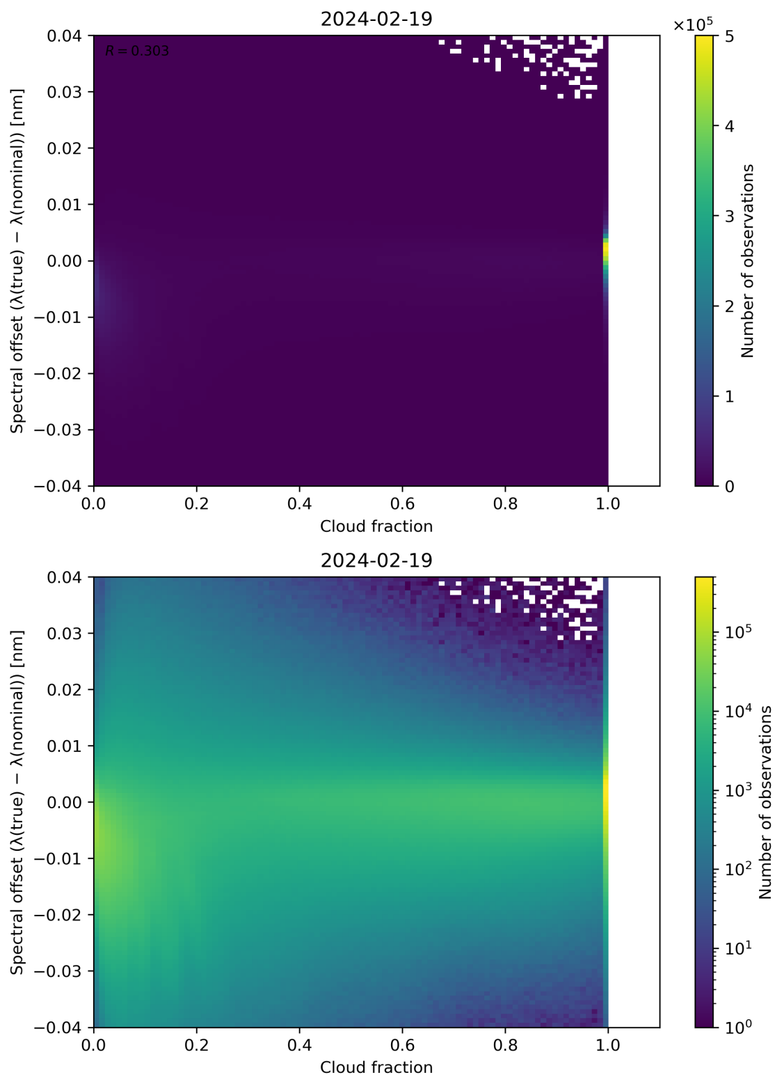
Figure 76: Scatter density plot of “Cloud fraction” against “Spectral offset ( \lambda(\text{true}) - \lambda(\text{nominal}) )” for 2024-02-18 to 2024-02-20.
