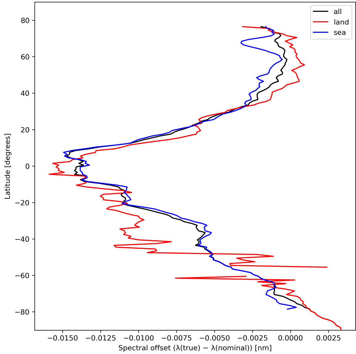
Figure 28: Zonal average of “Spectral offset ( \lambda(\text{true}) - \lambda(\text{nominal}) )” for 2024-02-18 to 2024-02-20.
