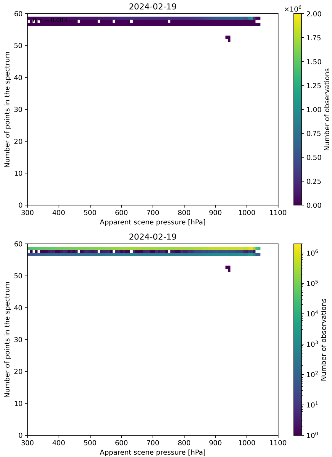
Figure 66: Scatter density plot of “Apparent scene pressure” against “Number of points in the spectrum” for 2024-02-18 to 2024-02-20.
