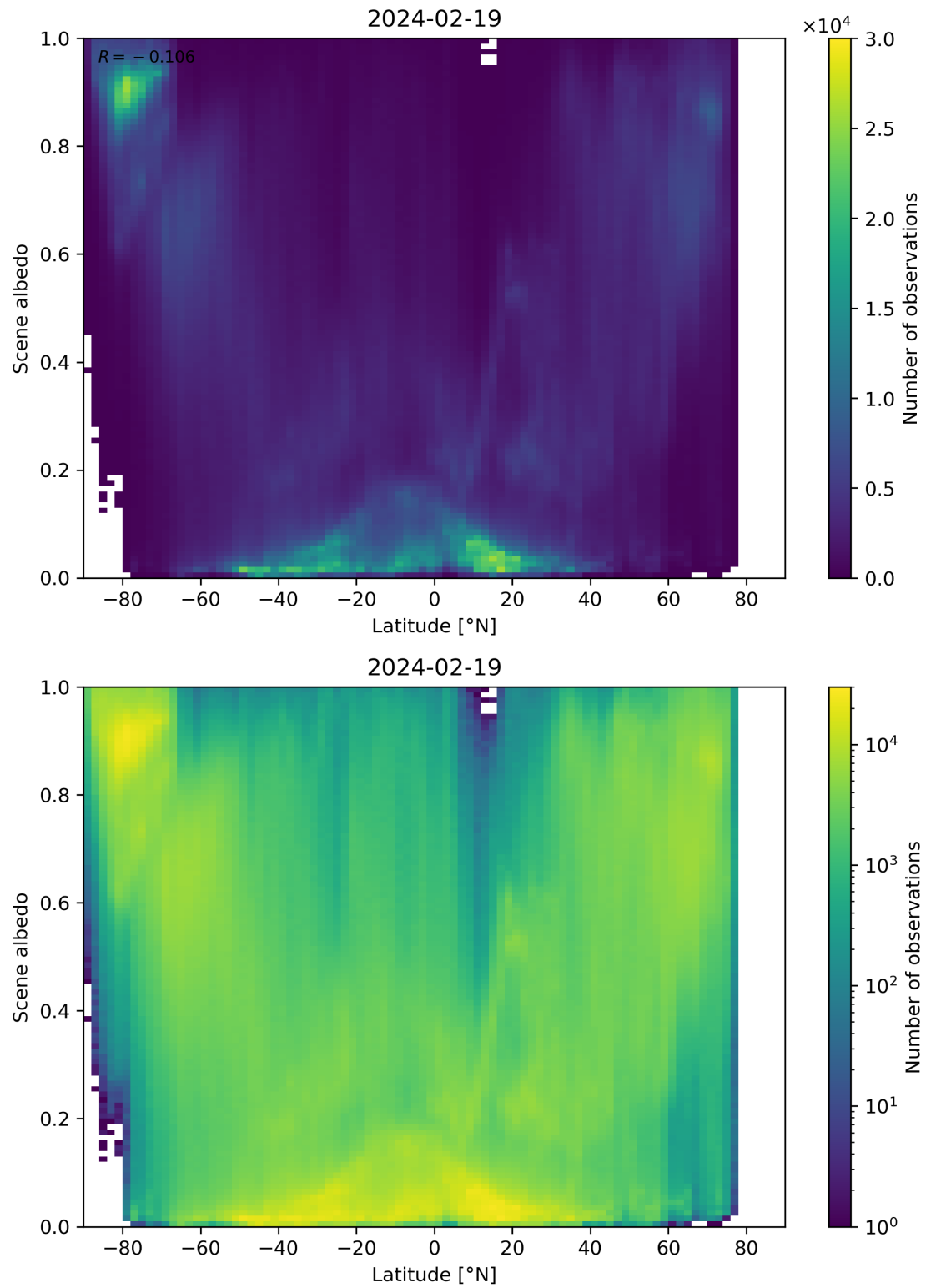
Figure 95: Scatter density plot of “Latitude” against “Scene albedo” for 2024-02-18 to 2024-02-20.
