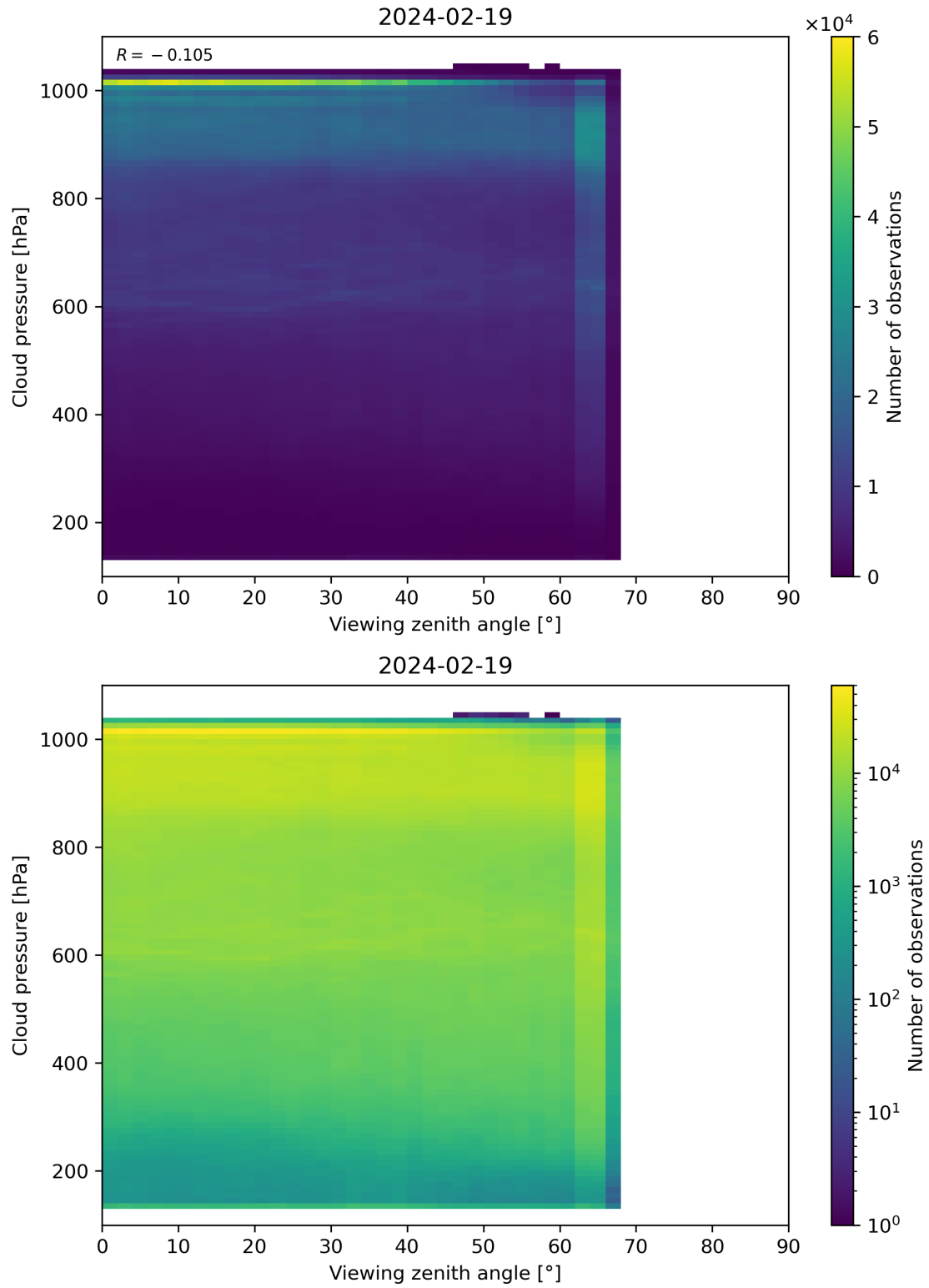
Figure 121: Scatter density plot of “Viewing zenith angle” against “Cloud pressure” for 2024-02-18 to 2024-02-20.
