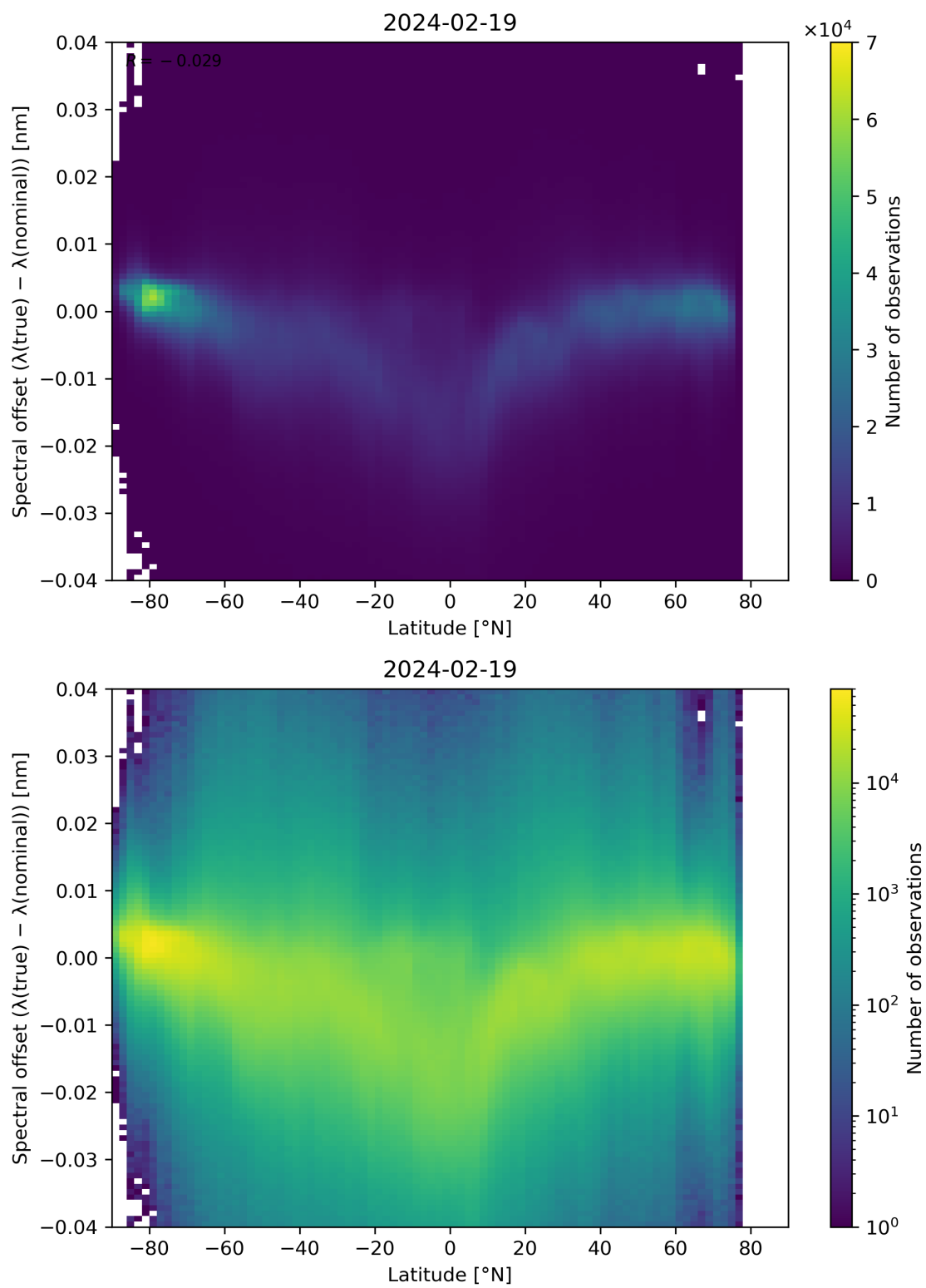
Figure 96: Scatter density plot of “Latitude” against “Spectral offset ( \lambda(\text{true}) - \lambda(\text{nominal}) )” for 2024-02-18 to 2024-02-20.
