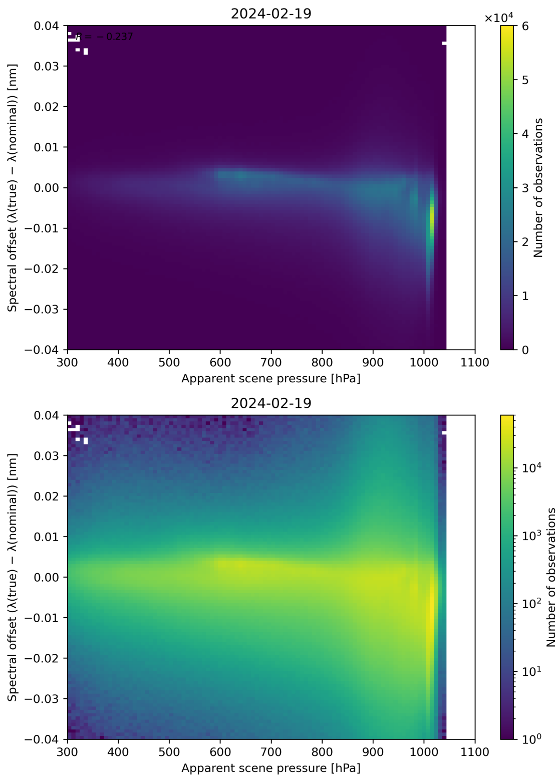
Figure 67: Scatter density plot of “Apparent scene pressure” against “Spectral offset ( \lambda(\text{true}) - \lambda(\text{nominal}) )” for 2024-02-18 to 2024-02-20.
