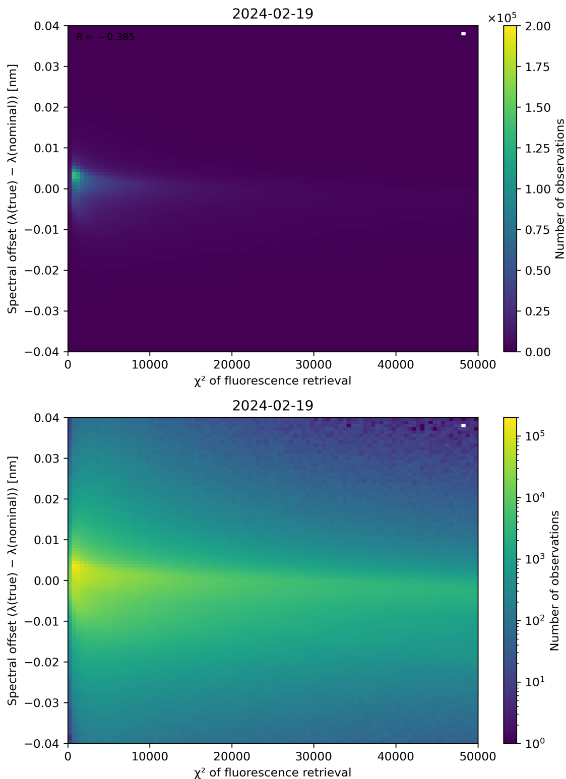
Figure 69: Scatter density plot of " \chi^2 of fluorescence retrieval" against "Spectral offset ( \lambda(\text{true}) - \lambda(\text{nominal}) )" for 2024-02-18 to 2024-02-20.
