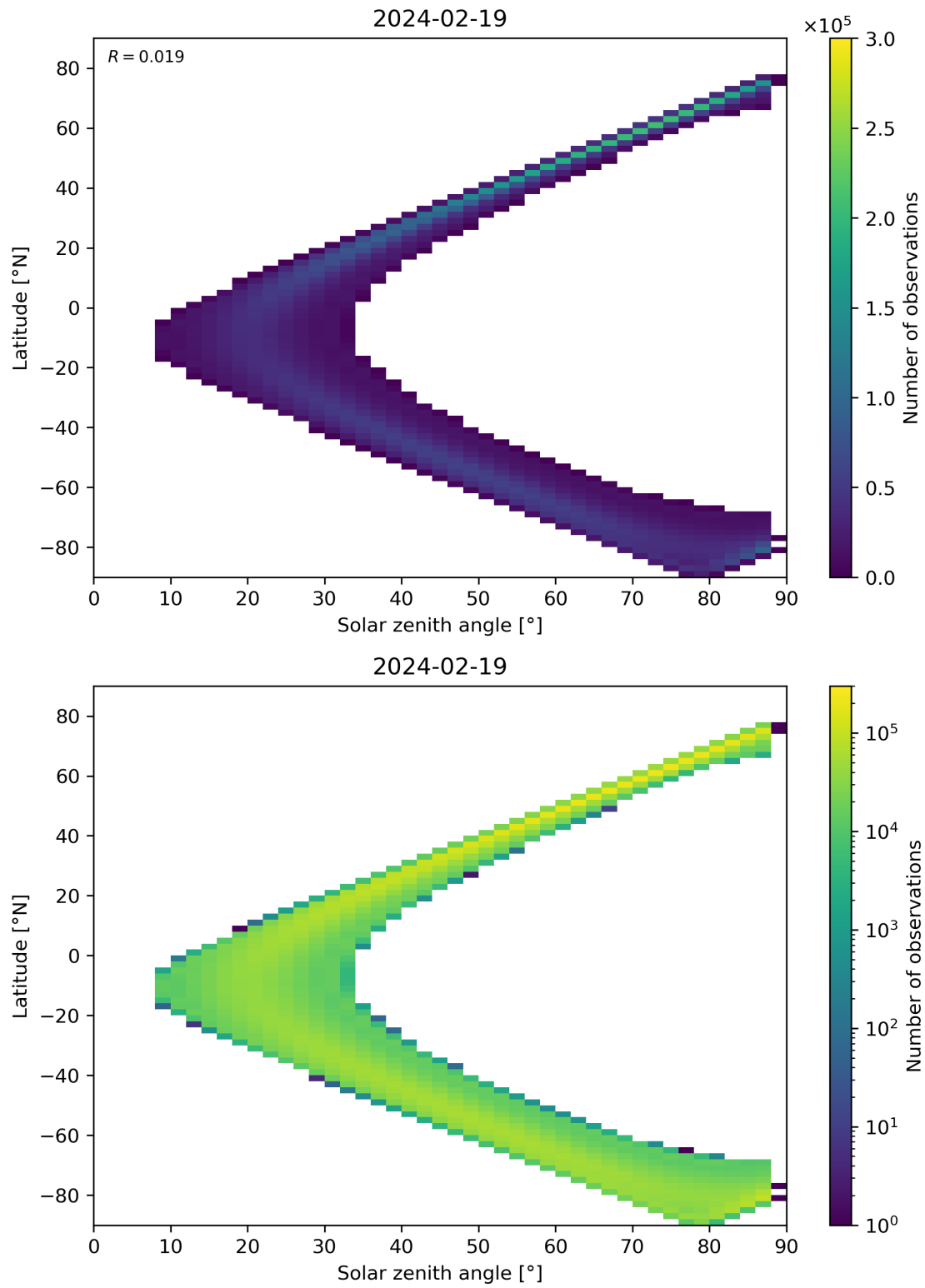
Figure 113: Scatter density plot of “Solar zenith angle” against “Latitude” for 2024-02-18 to 2024-02-20.
