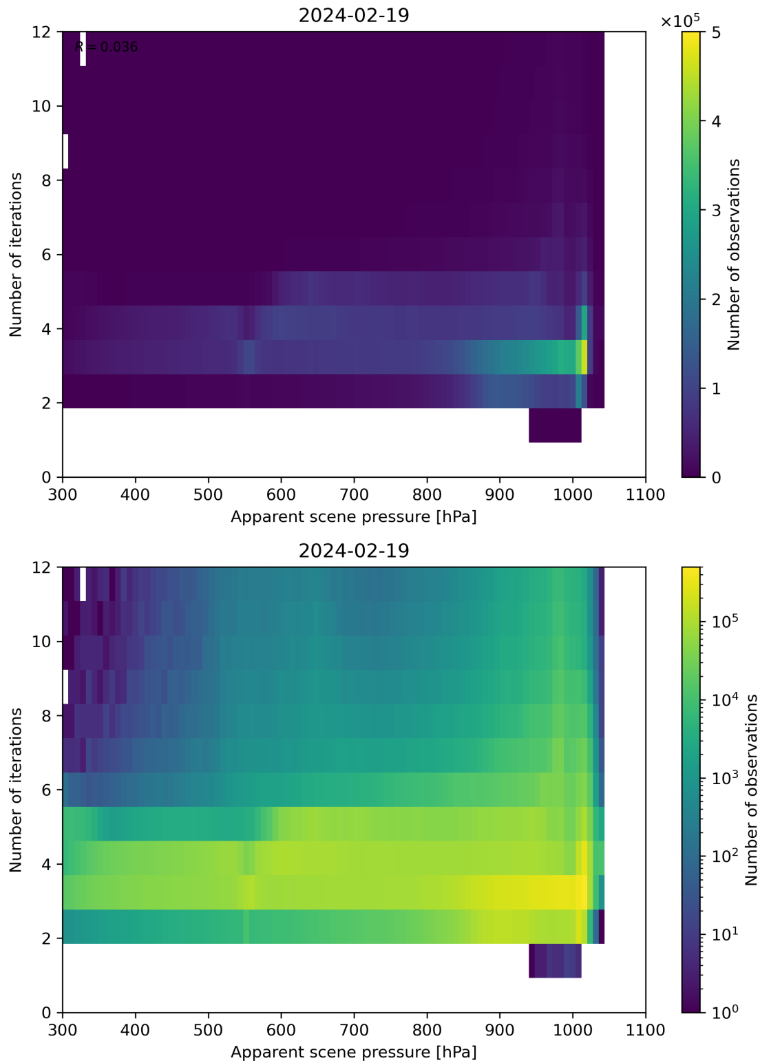
Figure 65: Scatter density plot of “Apparent scene pressure” against “Number of iterations” for 2024-02-18 to 2024-02-20.
