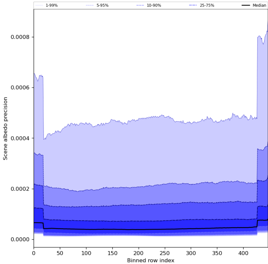
Figure 52: Along track statistics of “Scene albedo precision” for 2024-02-18 to 2024-02-20
