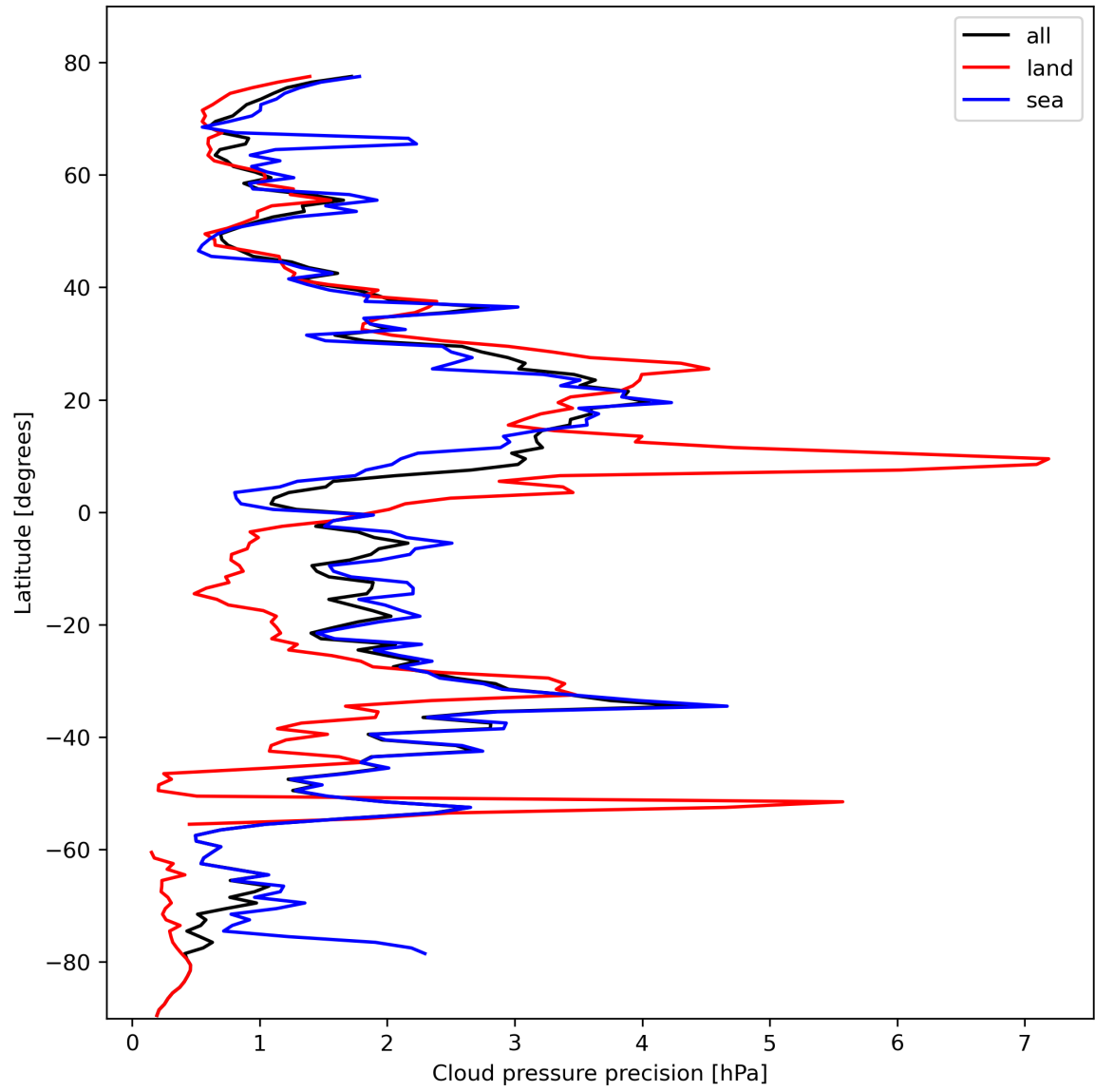
Figure 14: Zonal average of “Cloud pressure precision” for 2024-02-19 to 2024-02-21.
