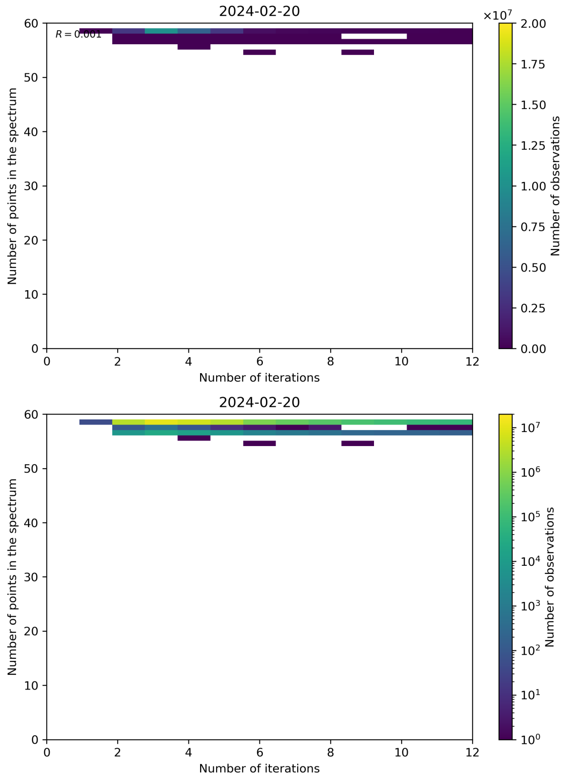
Figure 99: Scatter density plot of “Number of iterations” against “Number of points in the spectrum” for 2024-02-19 to 2024-02-21.
