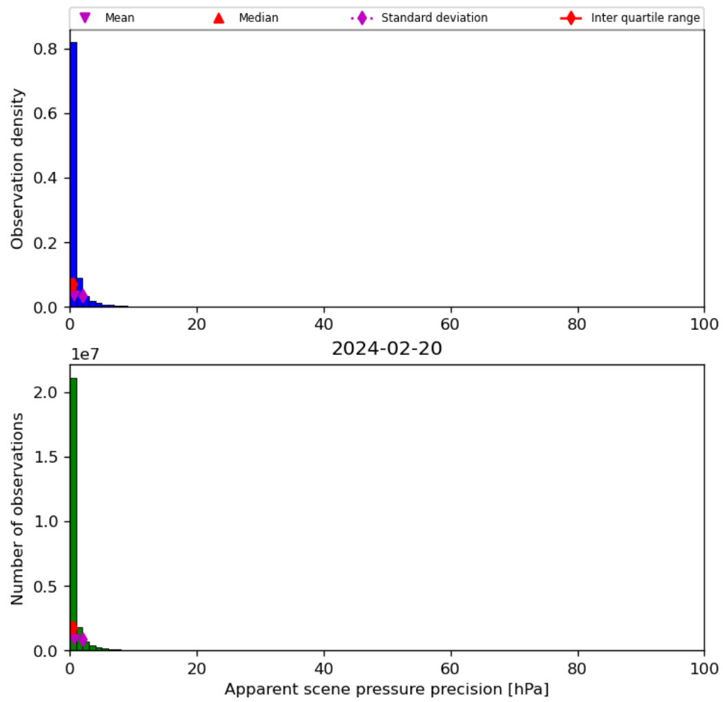
Figure 37: Histogram of “Apparent scene pressure precision” for 2024-02-19 to 2024-02-21
