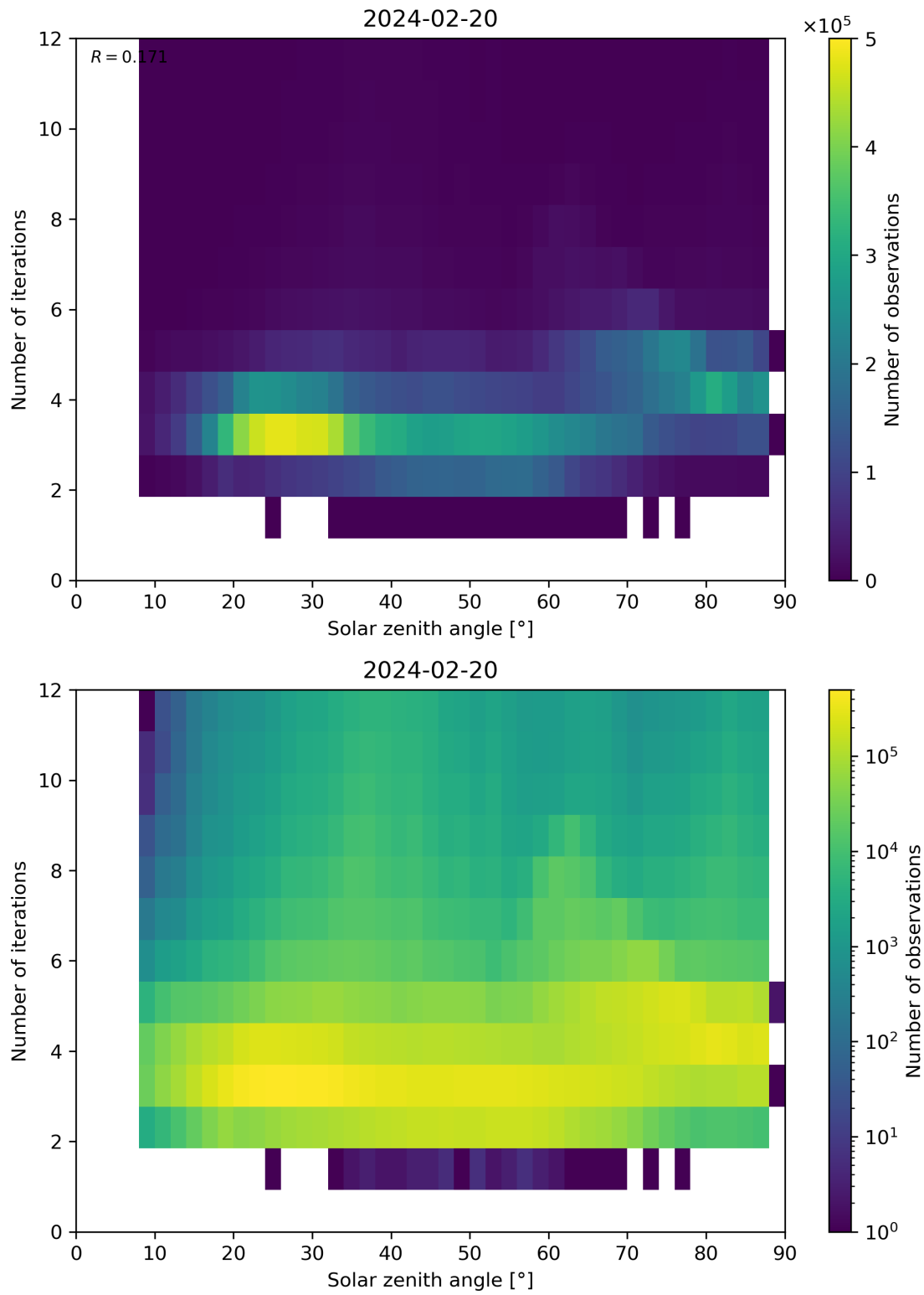
Figure 114: Scatter density plot of “Solar zenith angle” against “Number of iterations” for 2024-02-19 to 2024-02-21.
