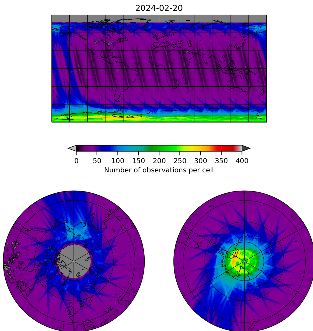
Figure 11: Map of the number of observations for 2024-02-19 to 2024-02-21
