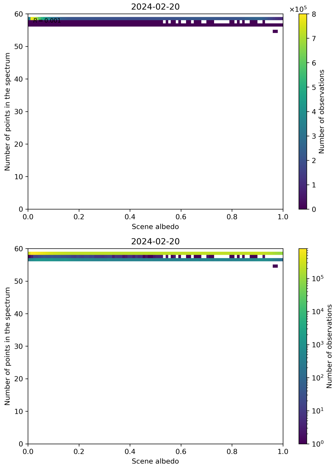
Figure 106: Scatter density plot of “Scene albedo” against “Number of points in the spectrum” for 2024-02-19 to 2024-02-21.
