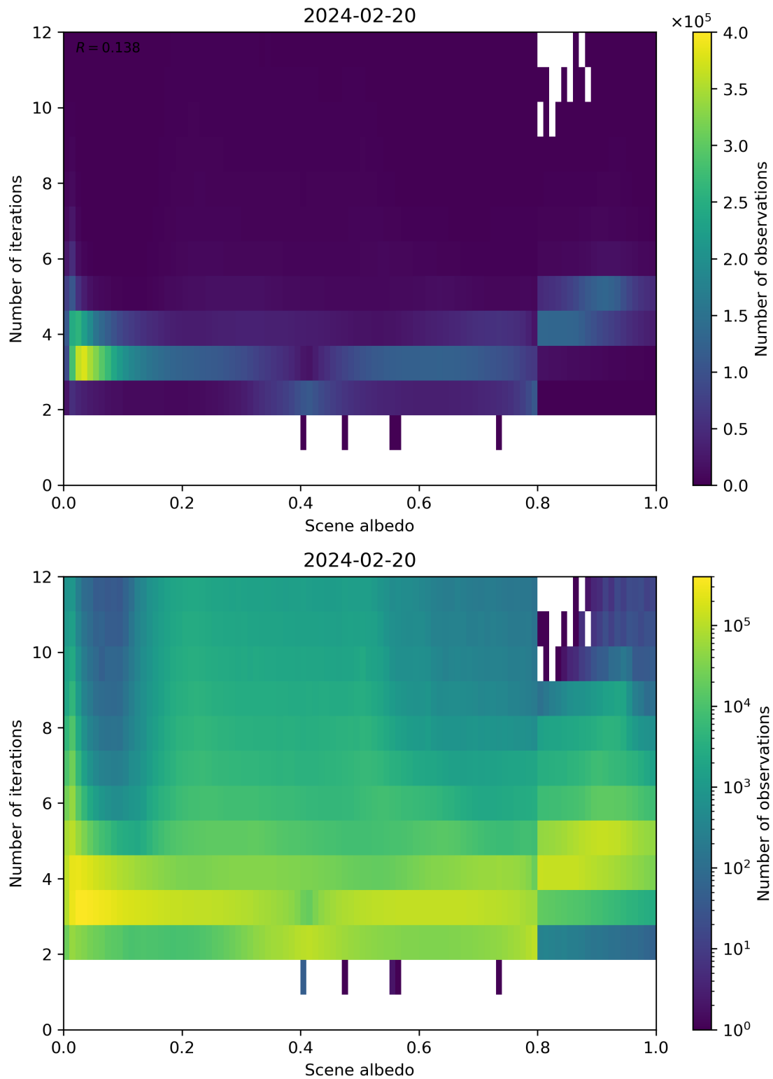
Figure 105: Scatter density plot of “Scene albedo” against “Number of iterations” for 2024-02-19 to 2024-02-21.
