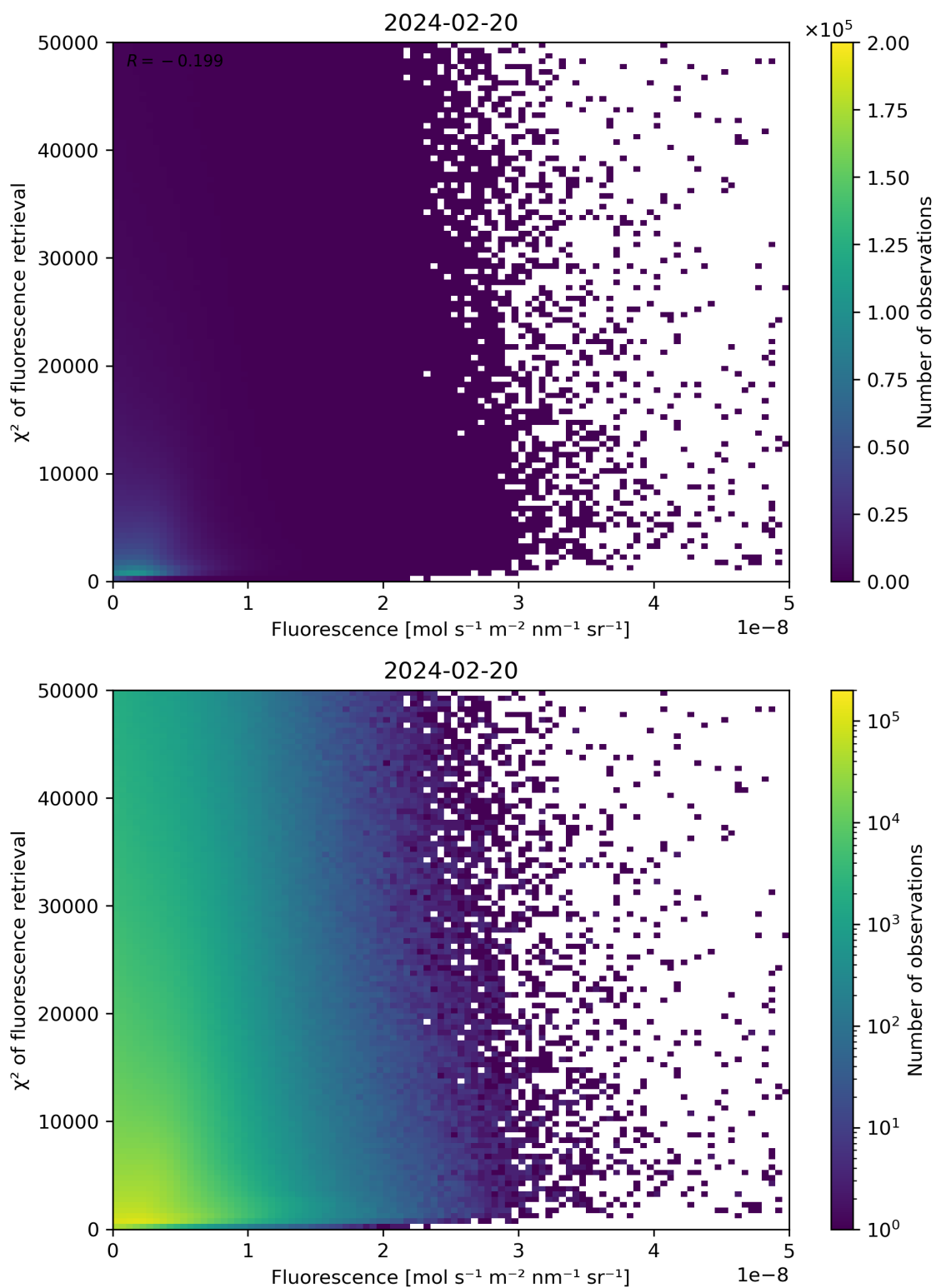
Figure 85: Scatter density plot of “Fluorescence” against “ \chi^2 of fluorescence retrieval” for 2024-02-19 to 2024-02-21.
