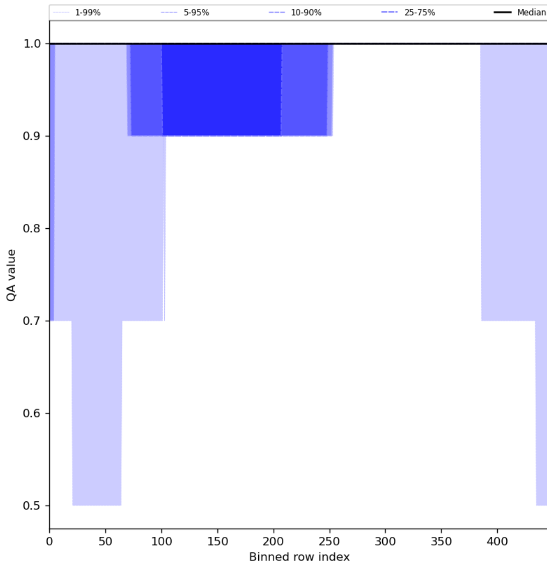
Figure 46: Along track statistics of “QA value” for 2024-02-19 to 2024-02-21
