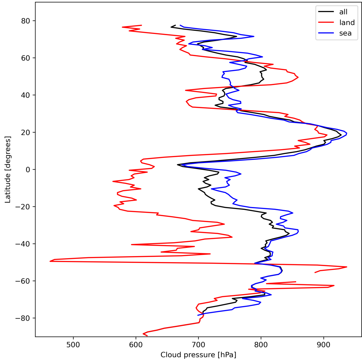
Figure 13: Zonal average of “Cloud pressure” for 2024-02-19 to 2024-02-21.
