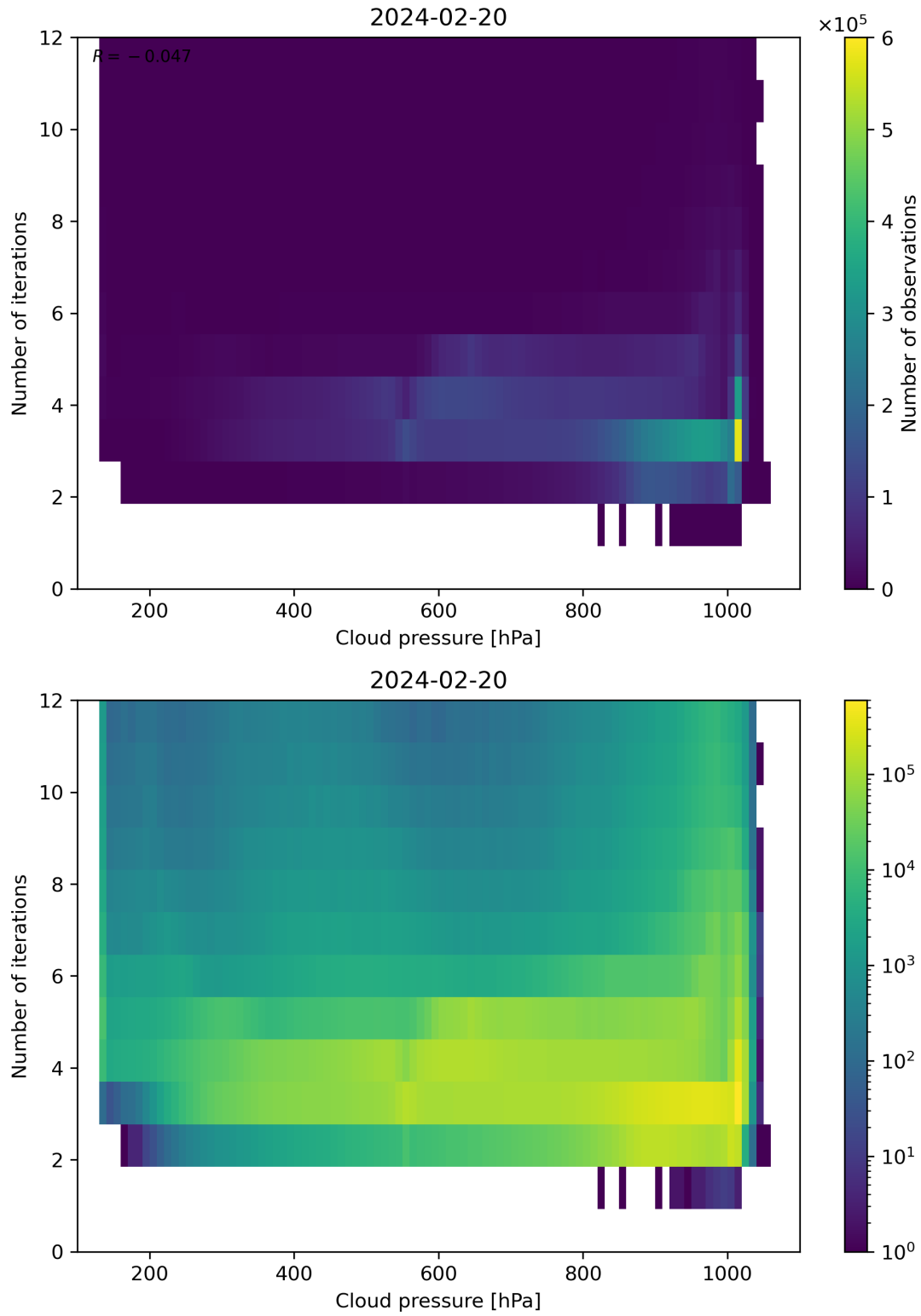
Figure 81: Scatter density plot of “Cloud pressure” against “Number of iterations” for 2024-02-19 to 2024-02-21.
