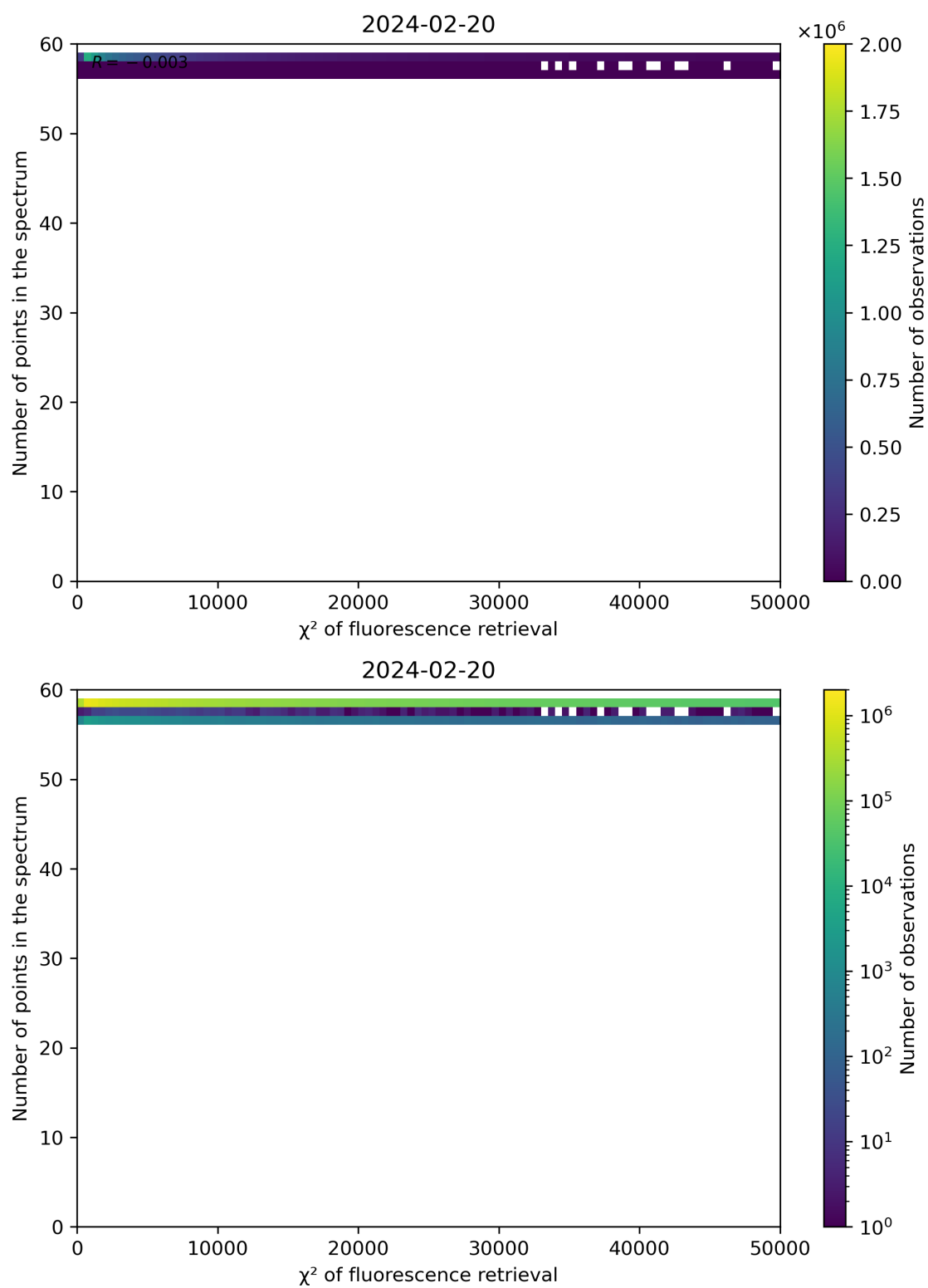
Figure 68: Scatter density plot of " \chi^2 of fluorescence retrieval" against "Number of points in the spectrum" for 2024-02-19 to 2024-02-21.
