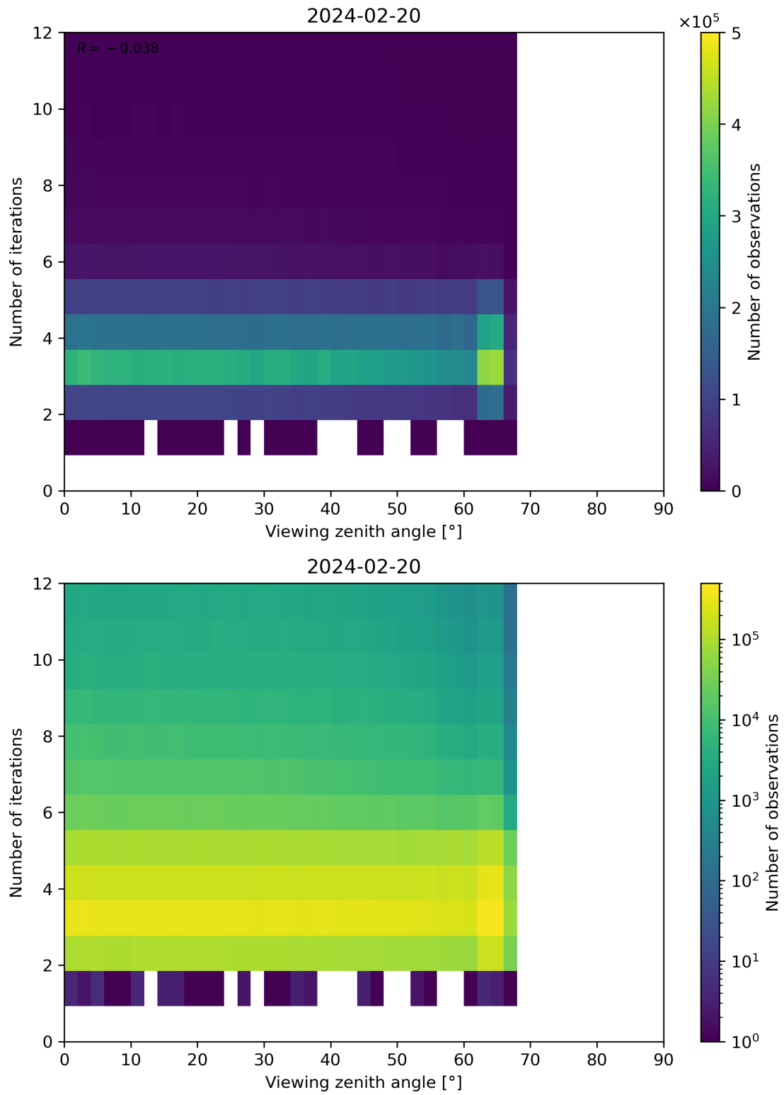
Figure 124: Scatter density plot of “Viewing zenith angle” against “Number of iterations” for 2024-02-19 to 2024-02-21.
