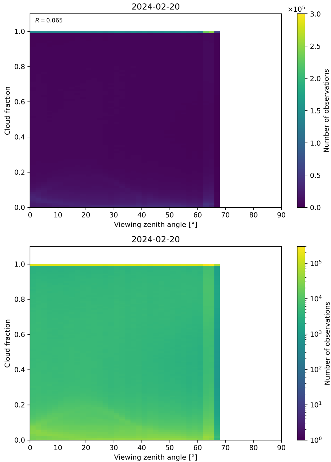
Figure 120: Scatter density plot of “Viewing zenith angle” against “Cloud fraction” for 2024-02-19 to 2024-02-21.
