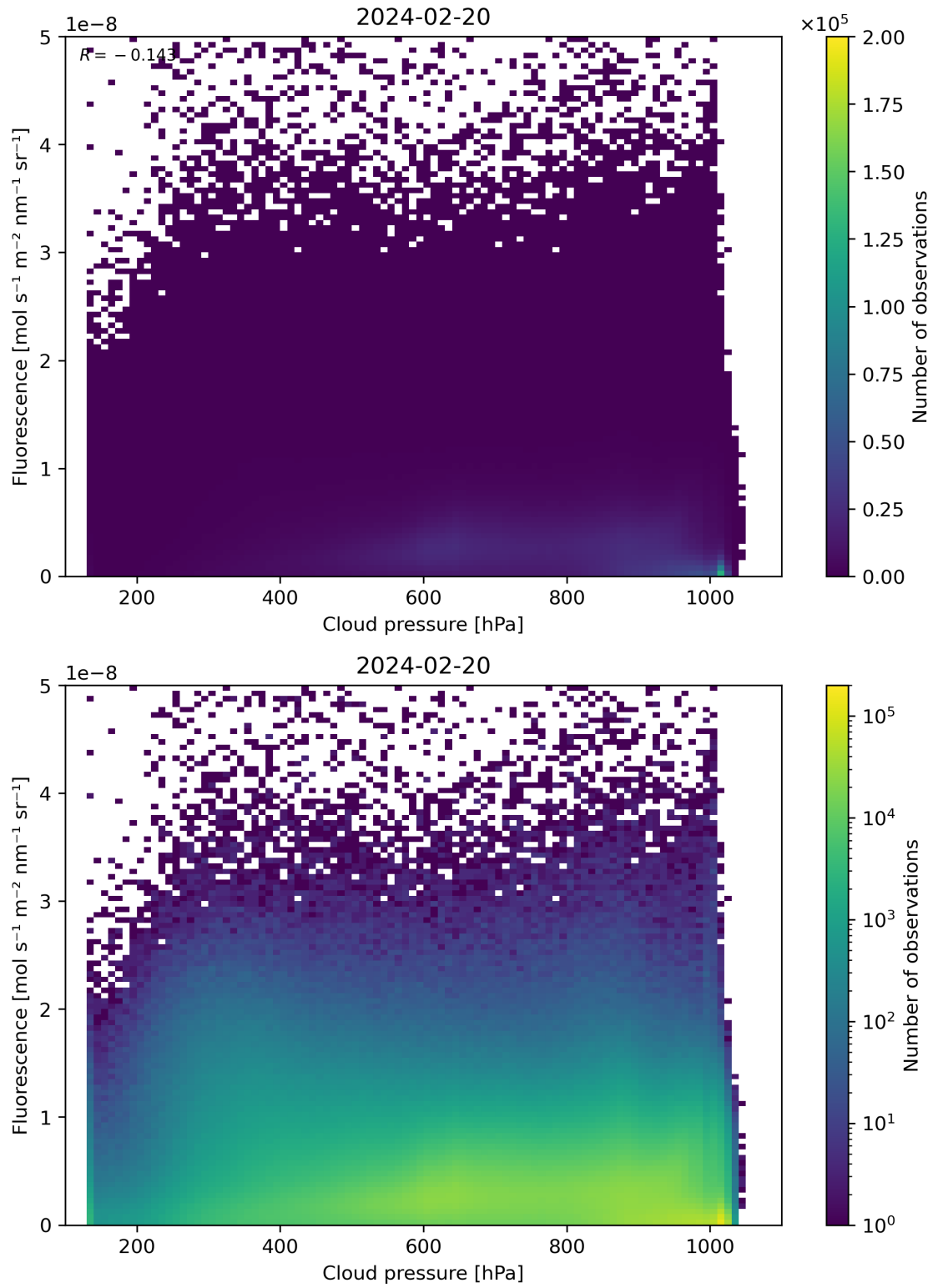
Figure 80: Scatter density plot of “Cloud pressure” against “Fluorescence” for 2024-02-19 to 2024-02-21.
