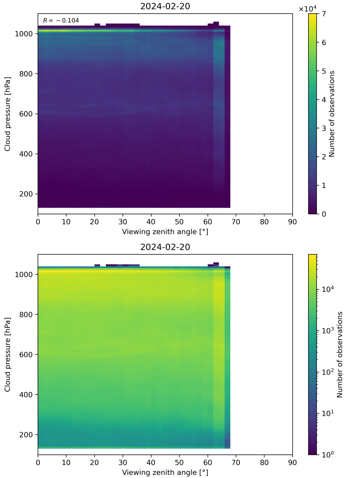
Figure 121: Scatter density plot of “Viewing zenith angle” against “Cloud pressure” for 2024-02-19 to 2024-02-21.
