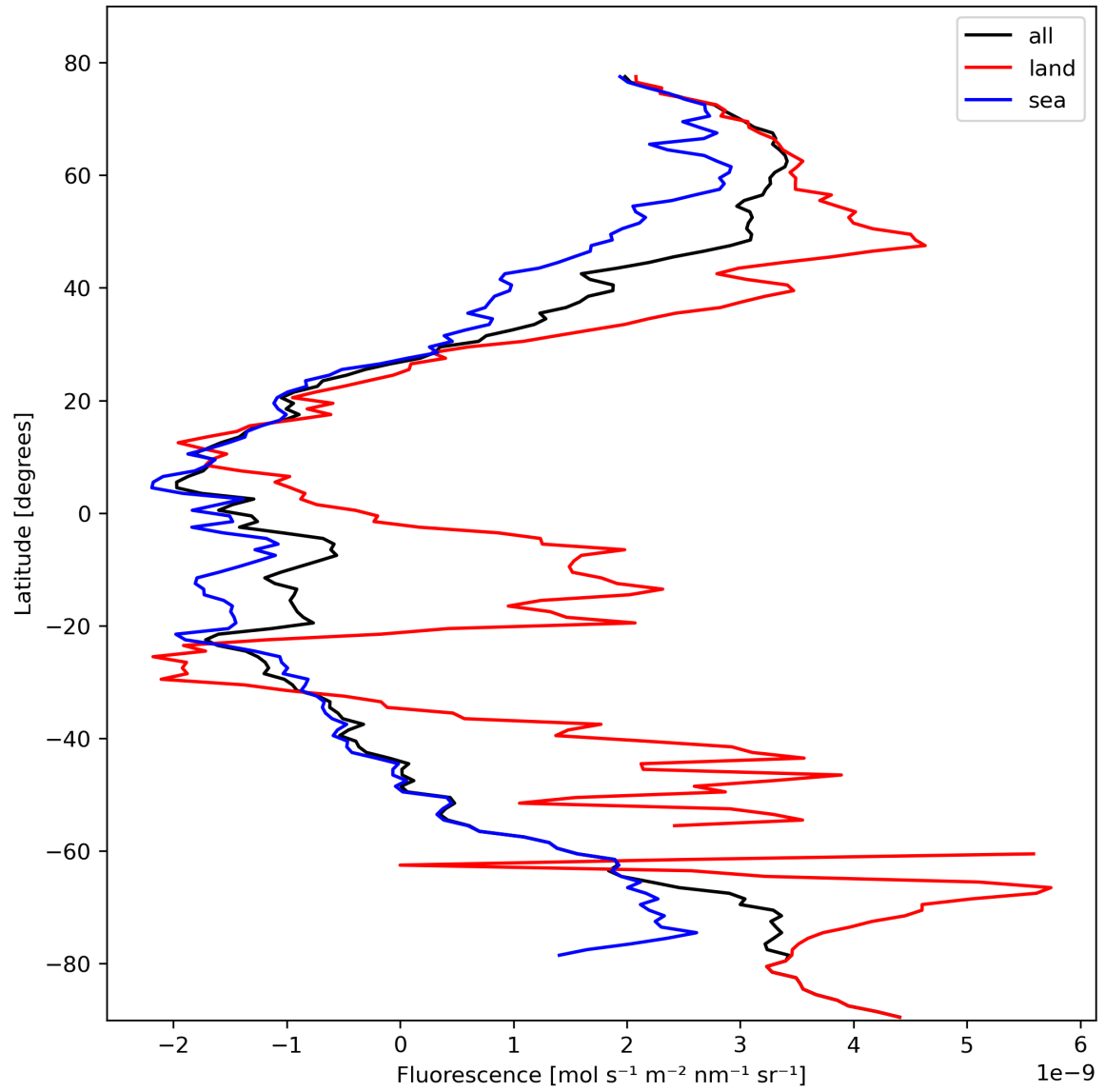
Figure 23: Zonal average of “Fluorescence” for 2024-02-19 to 2024-02-21.
