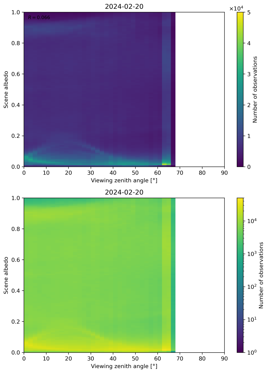
Figure 126: Scatter density plot of “Viewing zenith angle” against “Scene albedo” for 2024-02-19 to 2024-02-21.
