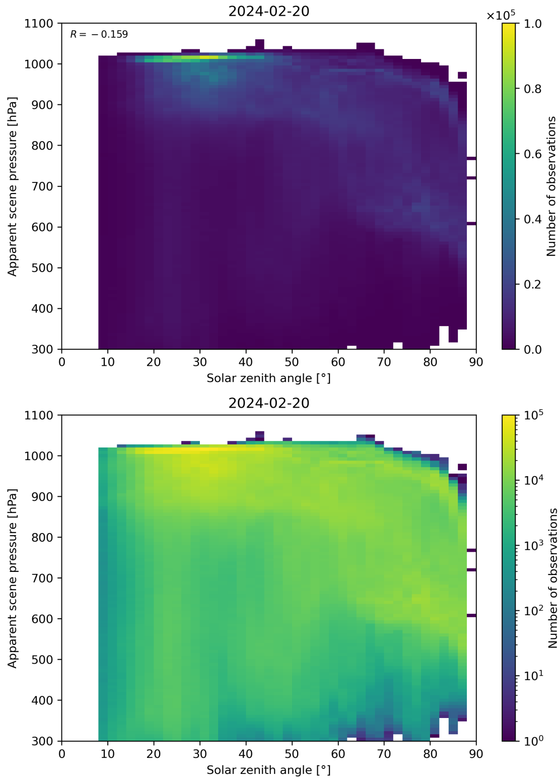
Figure 108: Scatter density plot of “Solar zenith angle” against “Apparent scene pressure” for 2024-02-19 to 2024-02-21.
