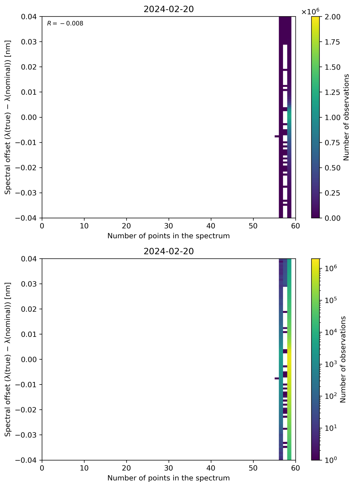
Figure 101: Scatter density plot of “Number of points in the spectrum” against “Spectral offset ( \lambda(\text{true}) - \lambda(\text{nominal}) )” for 2024-02-19 to 2024-02-21.
