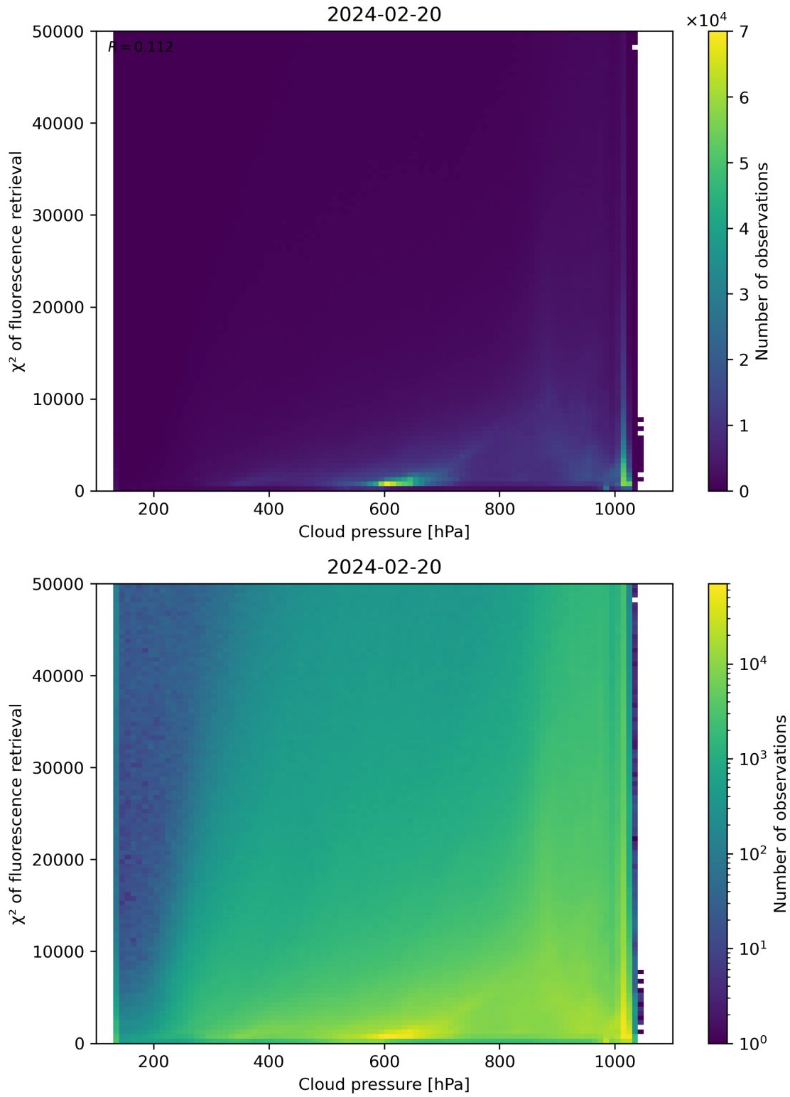
Figure 78: Scatter density plot of “Cloud pressure” against “ \chi^2 of fluorescence retrieval” for 2024-02-19 to 2024-02-21.
