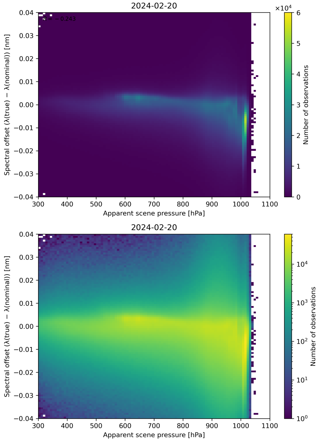
Figure 67: Scatter density plot of “Apparent scene pressure” against “Spectral offset ( \lambda(\text{true}) - \lambda(\text{nominal}) )” for 2024-02-19 to 2024-02-21.
