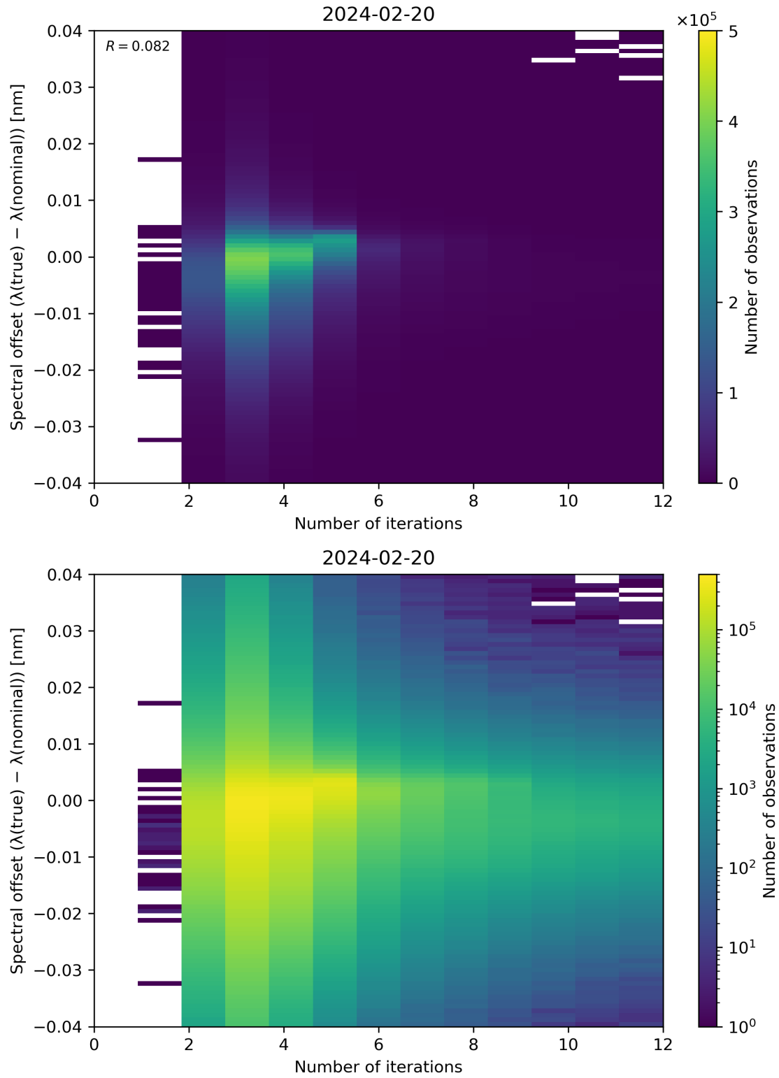
Figure 100: Scatter density plot of “Number of iterations” against “Spectral offset ( \lambda(\text{true}) - \lambda(\text{nominal}) )” for 2024-02-19 to 2024-02-21.
