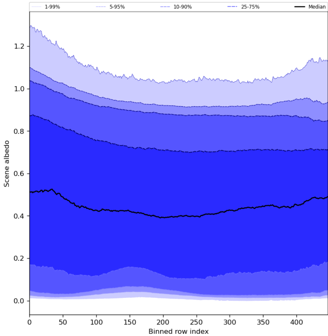
Figure 51: Along track statistics of “Scene albedo” for 2024-02-19 to 2024-02-21
