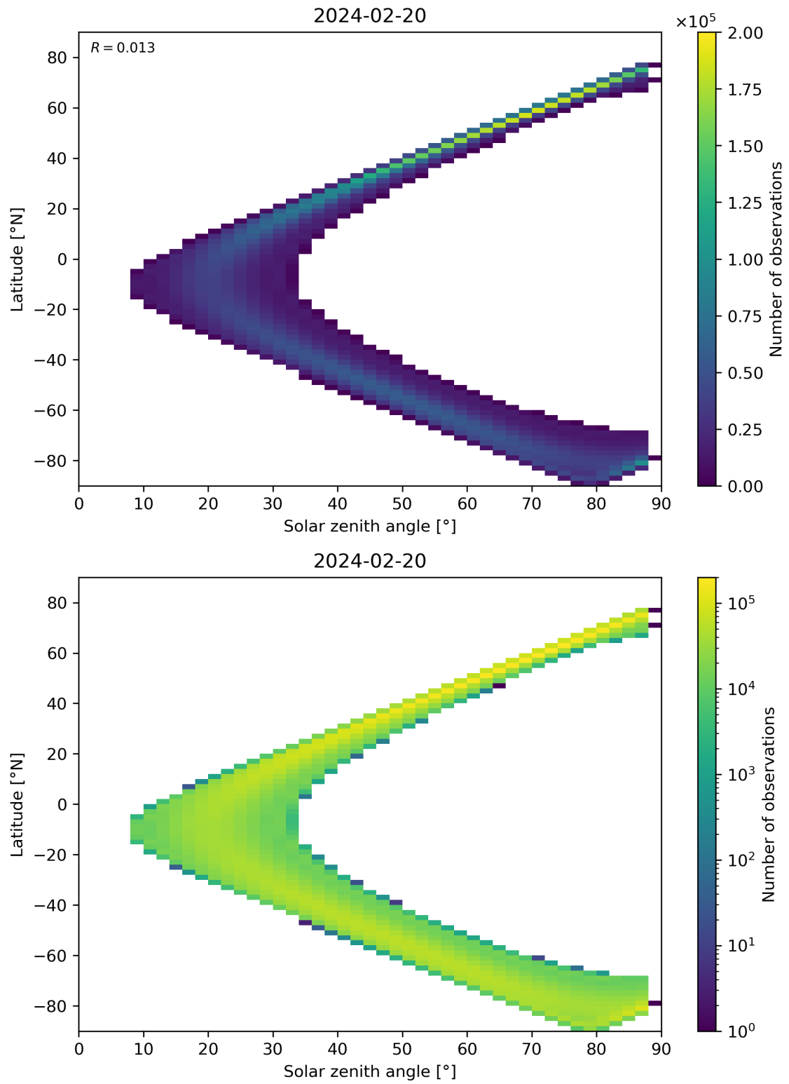
Figure 113: Scatter density plot of “Solar zenith angle” against “Latitude” for 2024-02-19 to 2024-02-21.
