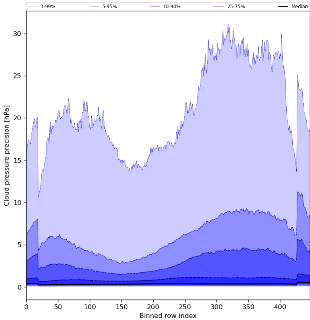
Figure 48: Along track statistics of “Cloud pressure precision” for 2024-02-19 to 2024-02-21
