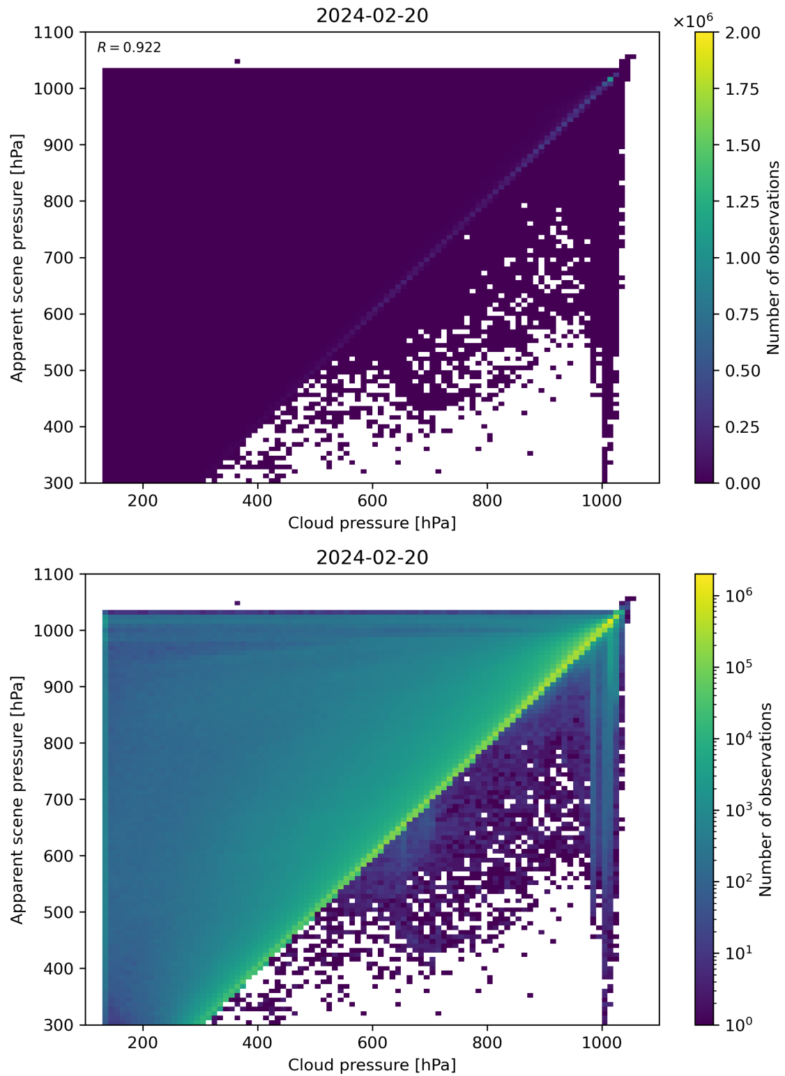
Figure 77: Scatter density plot of “Cloud pressure” against “Apparent scene pressure” for 2024-02-19 to 2024-02-21.
