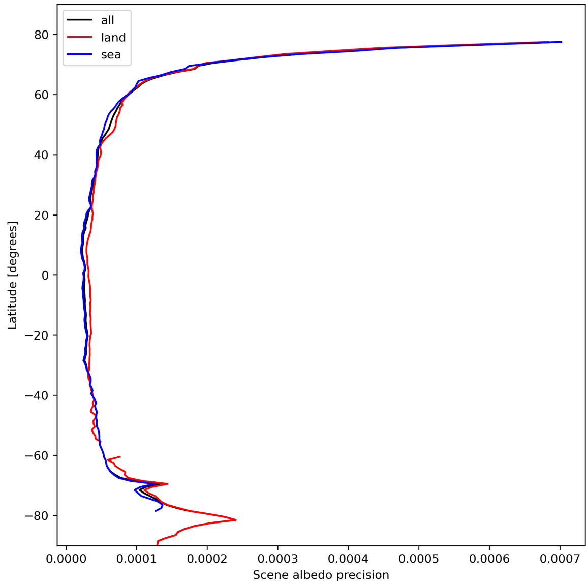
Figure 18: Zonal average of “Scene albedo precision” for 2024-02-19 to 2024-02-21.
