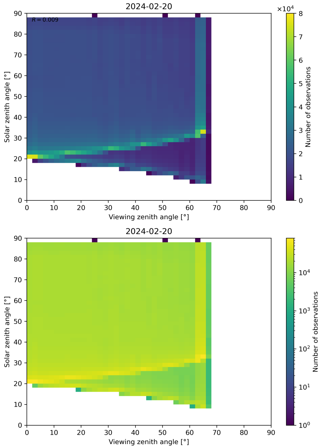
Figure 127: Scatter density plot of “Viewing zenith angle” against “Solar zenith angle” for 2024-02-19 to 2024-02-21.
