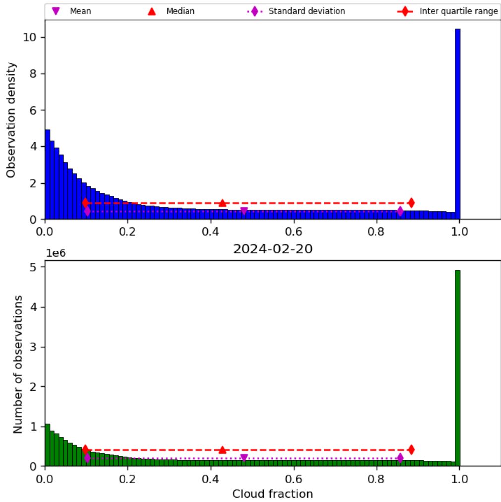
Figure 32: Histogram of “Cloud fraction” for 2024-02-19 to 2024-02-21
