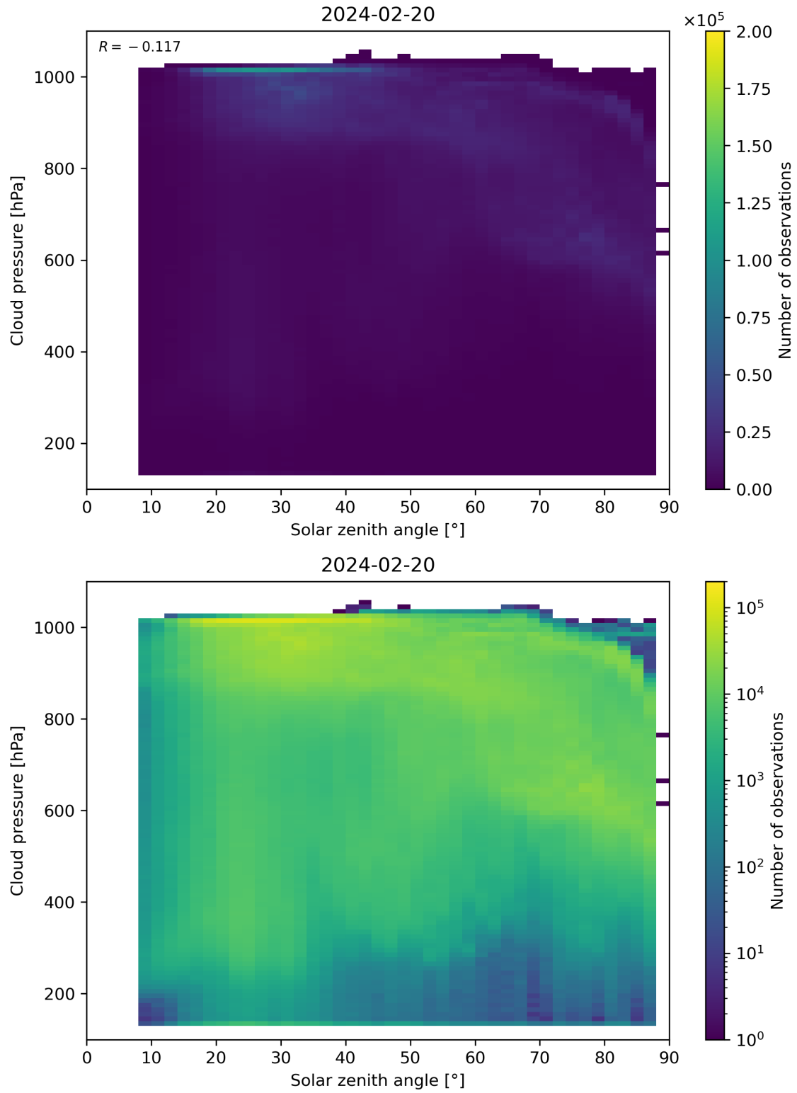
Figure 111: Scatter density plot of “Solar zenith angle” against “Cloud pressure” for 2024-02-19 to 2024-02-21.
