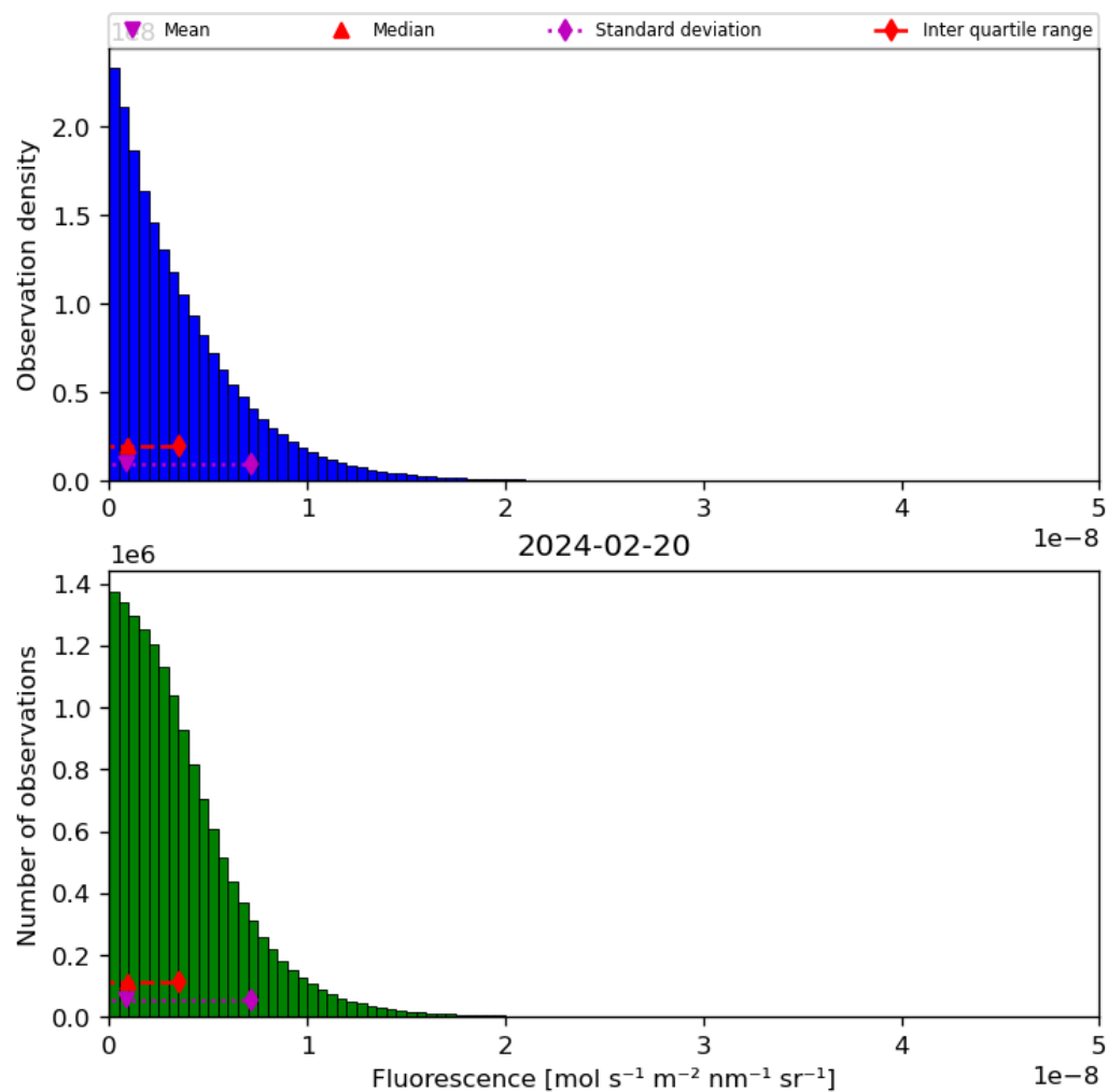
Figure 40: Histogram of “Fluorescence” for 2024-02-19 to 2024-02-21
