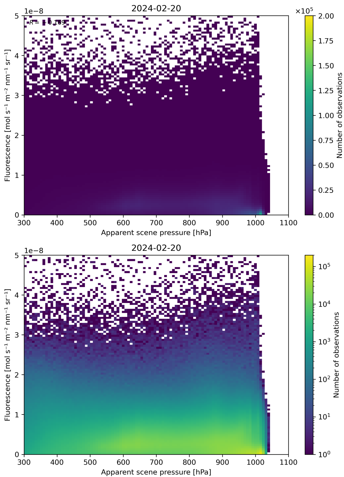
Figure 64: Scatter density plot of “Apparent scene pressure” against “Fluorescence” for 2024-02-19 to 2024-02-21.
