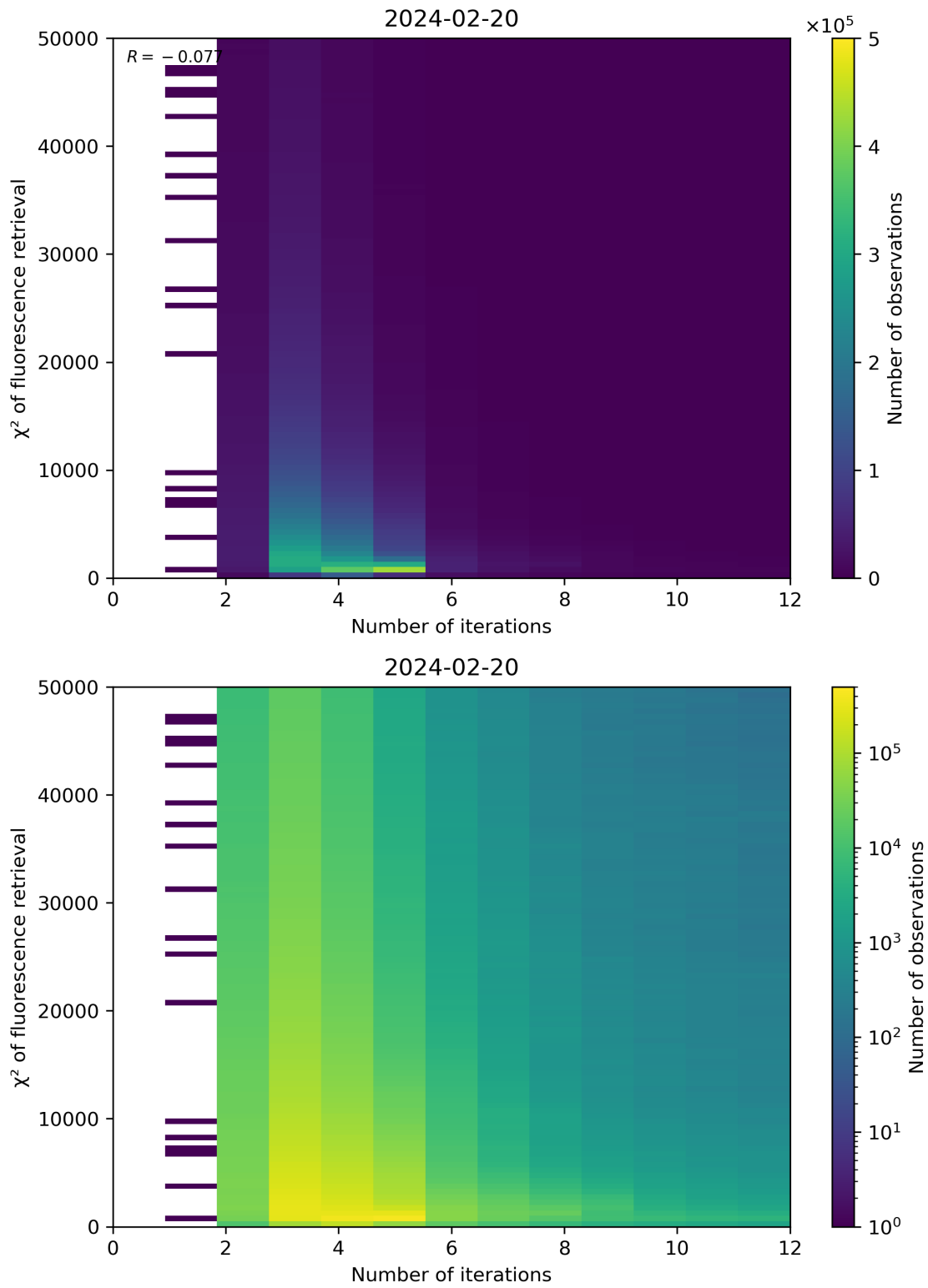
Figure 97: Scatter density plot of “Number of iterations” against “ \chi^2 of fluorescence retrieval” for 2024-02-19 to 2024-02-21.
