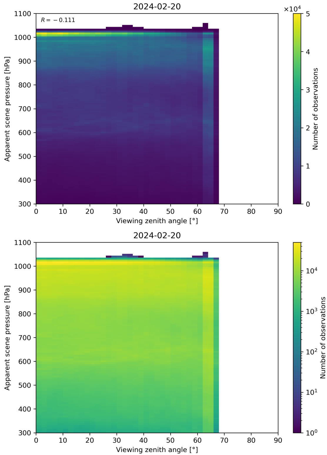
Figure 118: Scatter density plot of “Viewing zenith angle” against “Apparent scene pressure” for 2024-02-19 to 2024-02-21.
