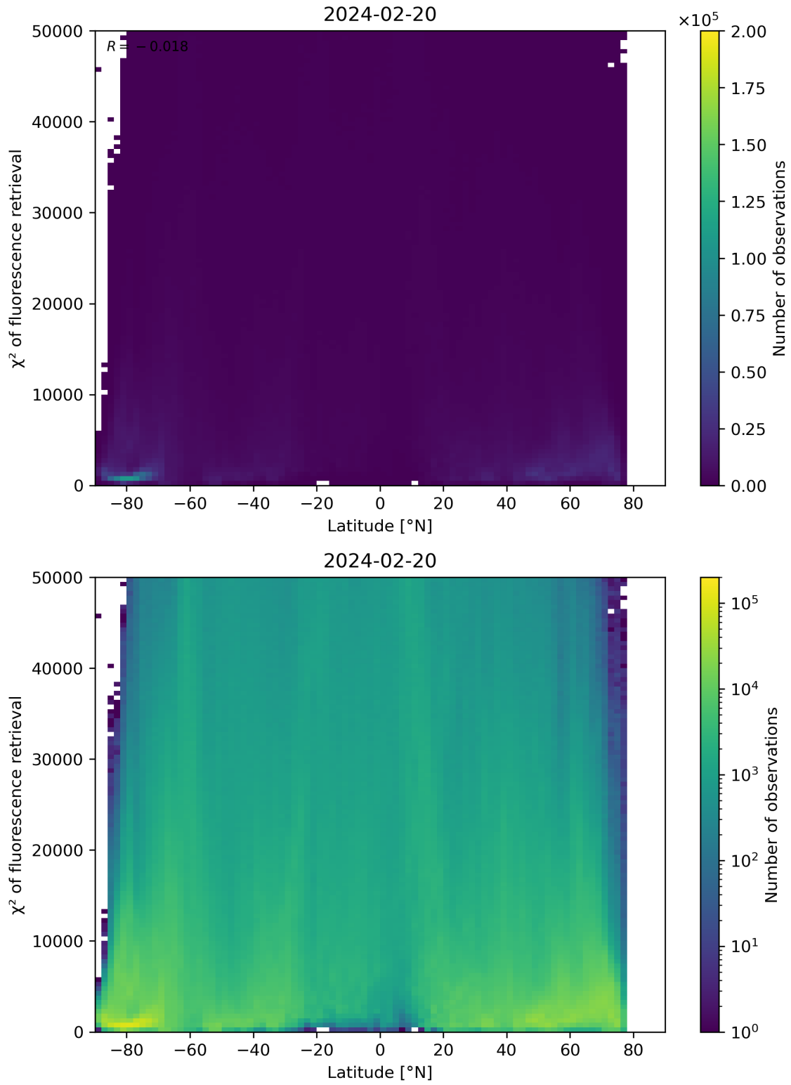
Figure 89: Scatter density plot of “Latitude” against “ \chi^2 of fluorescence retrieval” for 2024-02-19 to 2024-02-21.
