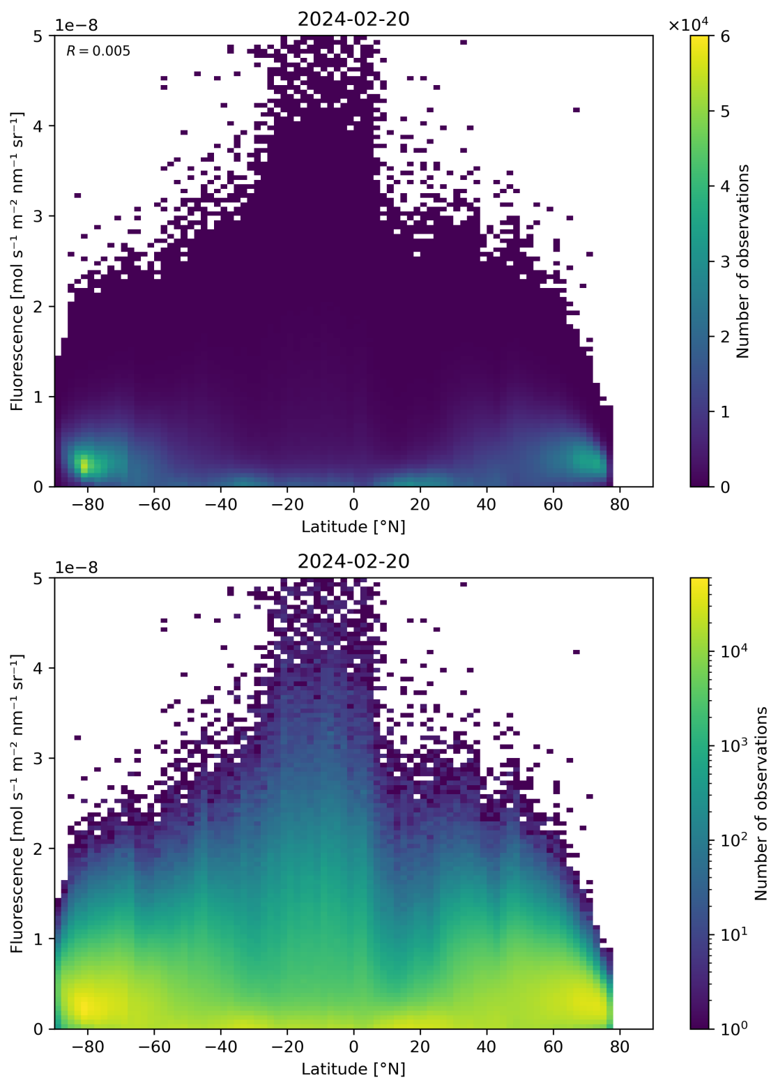
Figure 92: Scatter density plot of “Latitude” against “Fluorescence” for 2024-02-19 to 2024-02-21.
