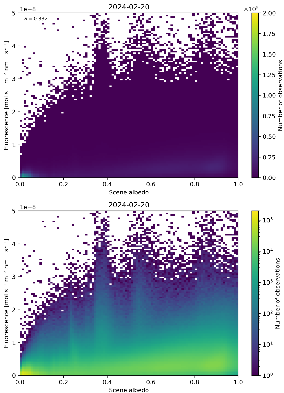
Figure 104: Scatter density plot of “Scene albedo” against “Fluorescence” for 2024-02-19 to 2024-02-21.
