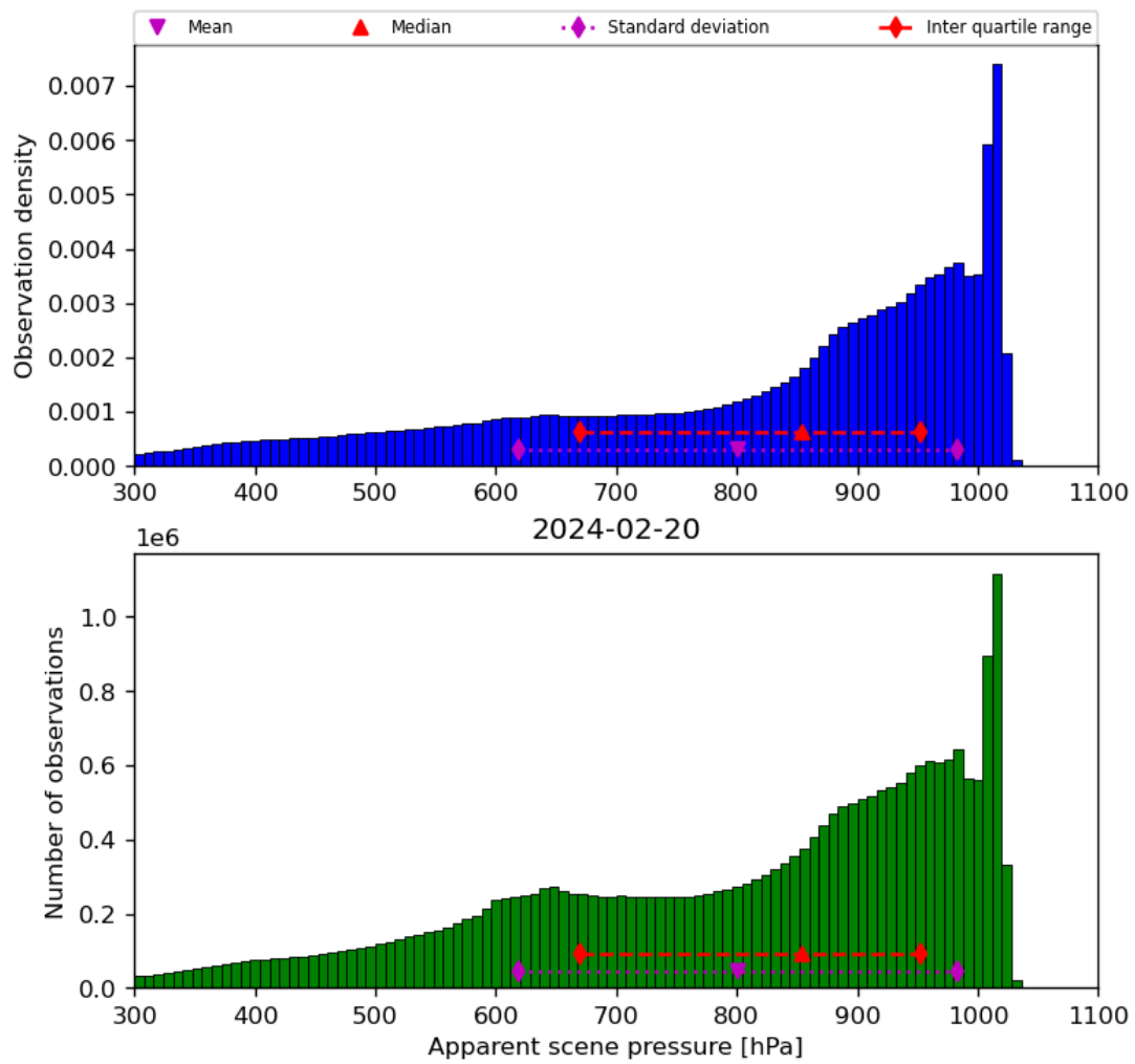
Figure 36: Histogram of “Apparent scene pressure” for 2024-02-19 to 2024-02-21
