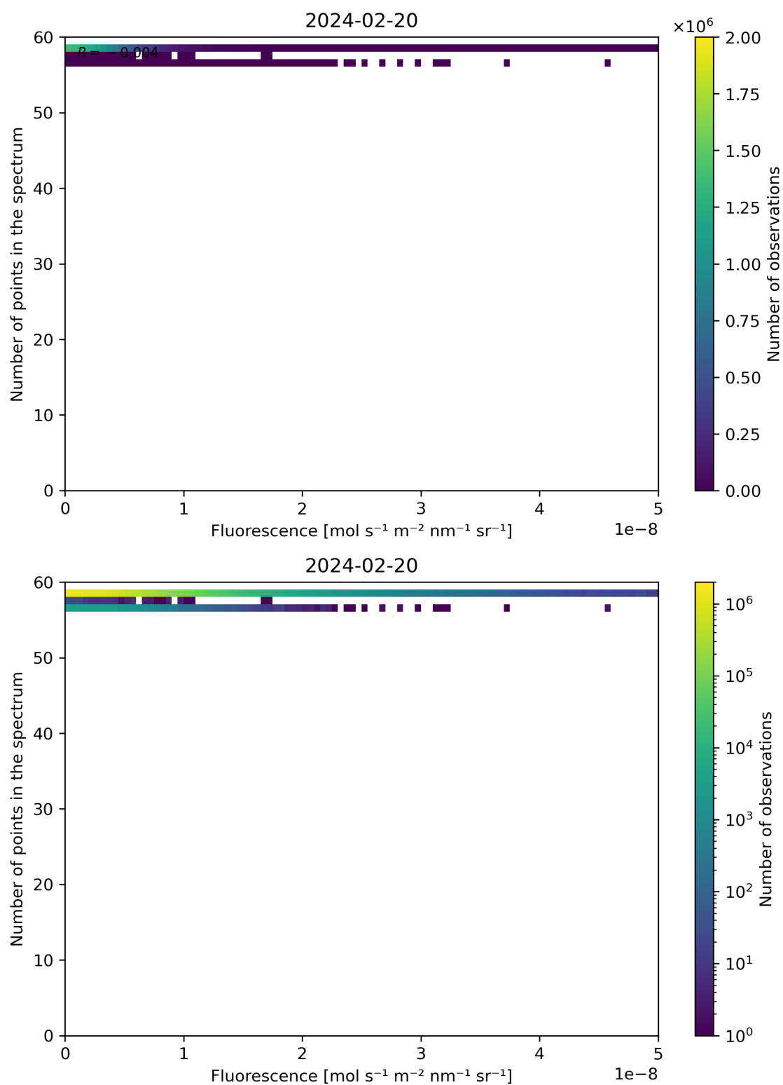
Figure 86: Scatter density plot of “Fluorescence” against “Number of points in the spectrum” for 2024-02-19 to 2024-02-21.
