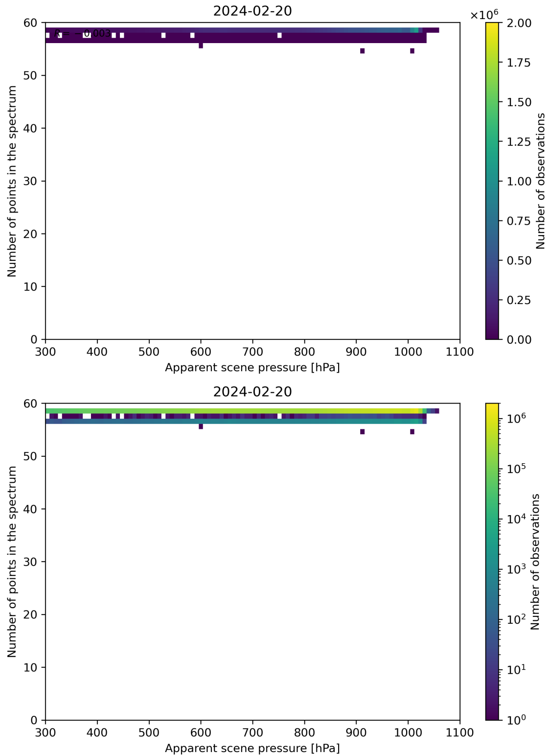
Figure 66: Scatter density plot of “Apparent scene pressure” against “Number of points in the spectrum” for 2024-02-19 to 2024-02-21.
