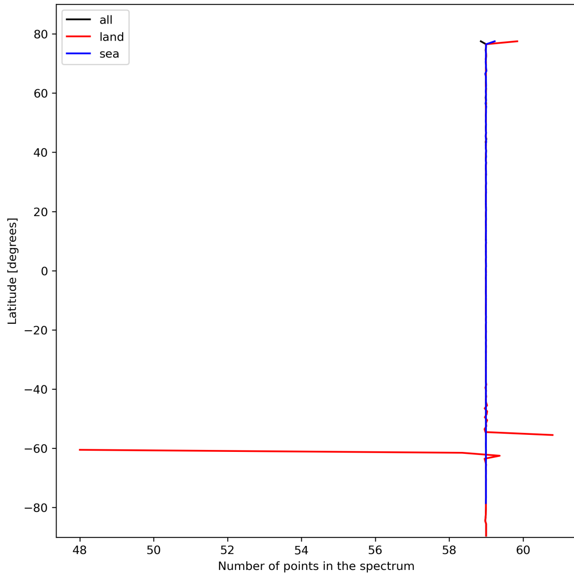
Figure 27: Zonal average of “Number of points in the spectrum” for 2024-02-19 to 2024-02-21.
