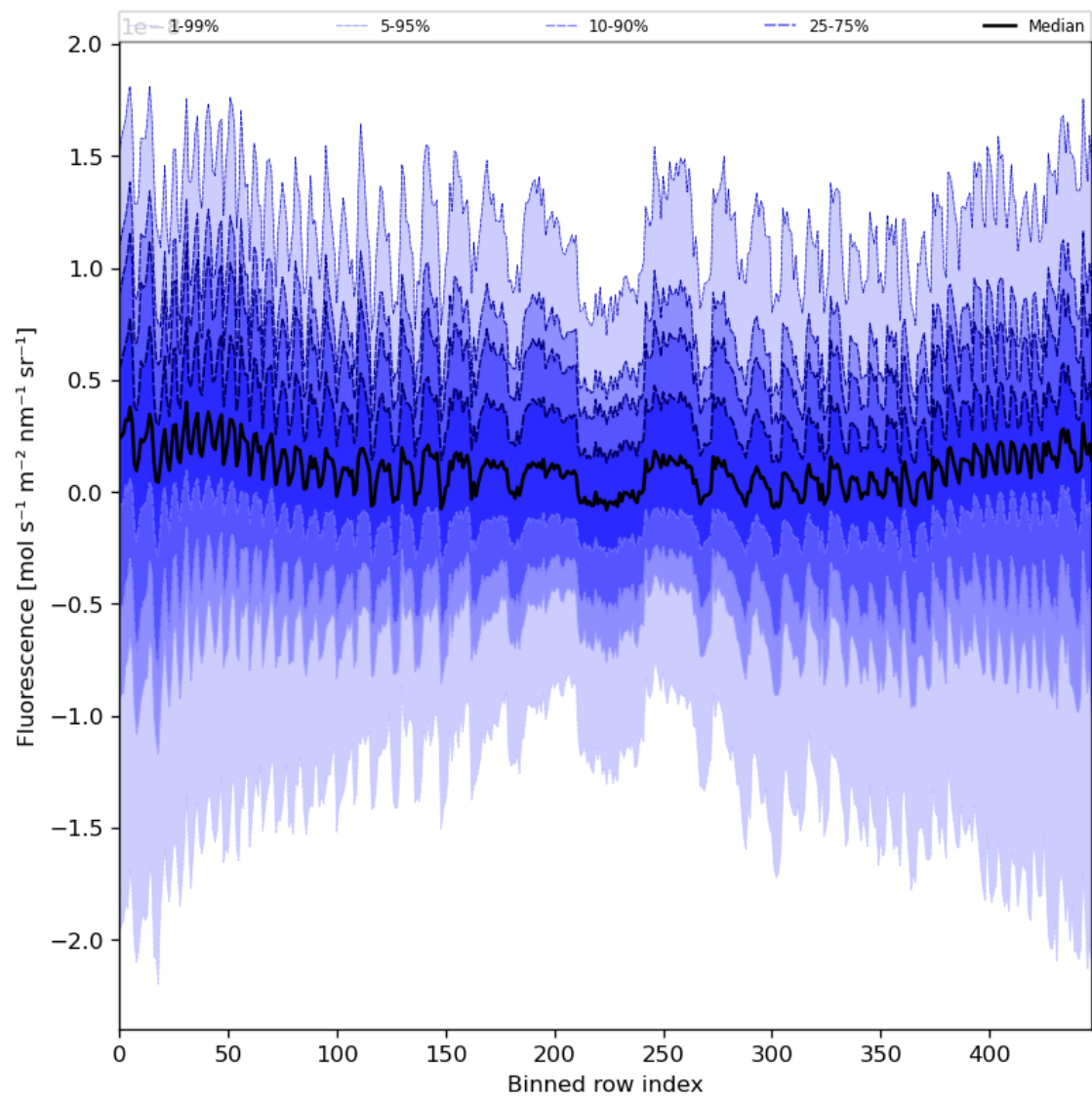
Figure 57: Along track statistics of “Fluorescence” for 2024-02-19 to 2024-02-21
