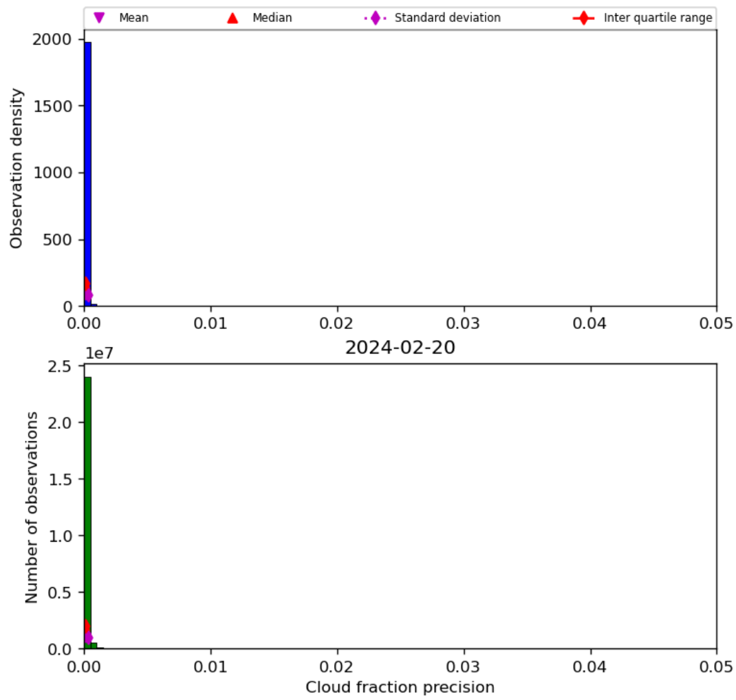
Figure 33: Histogram of “Cloud fraction precision” for 2024-02-19 to 2024-02-21
