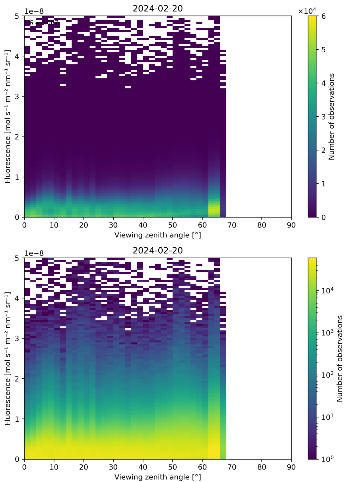
Figure 122: Scatter density plot of “Viewing zenith angle” against “Fluorescence” for 2024-02-19 to 2024-02-21.
