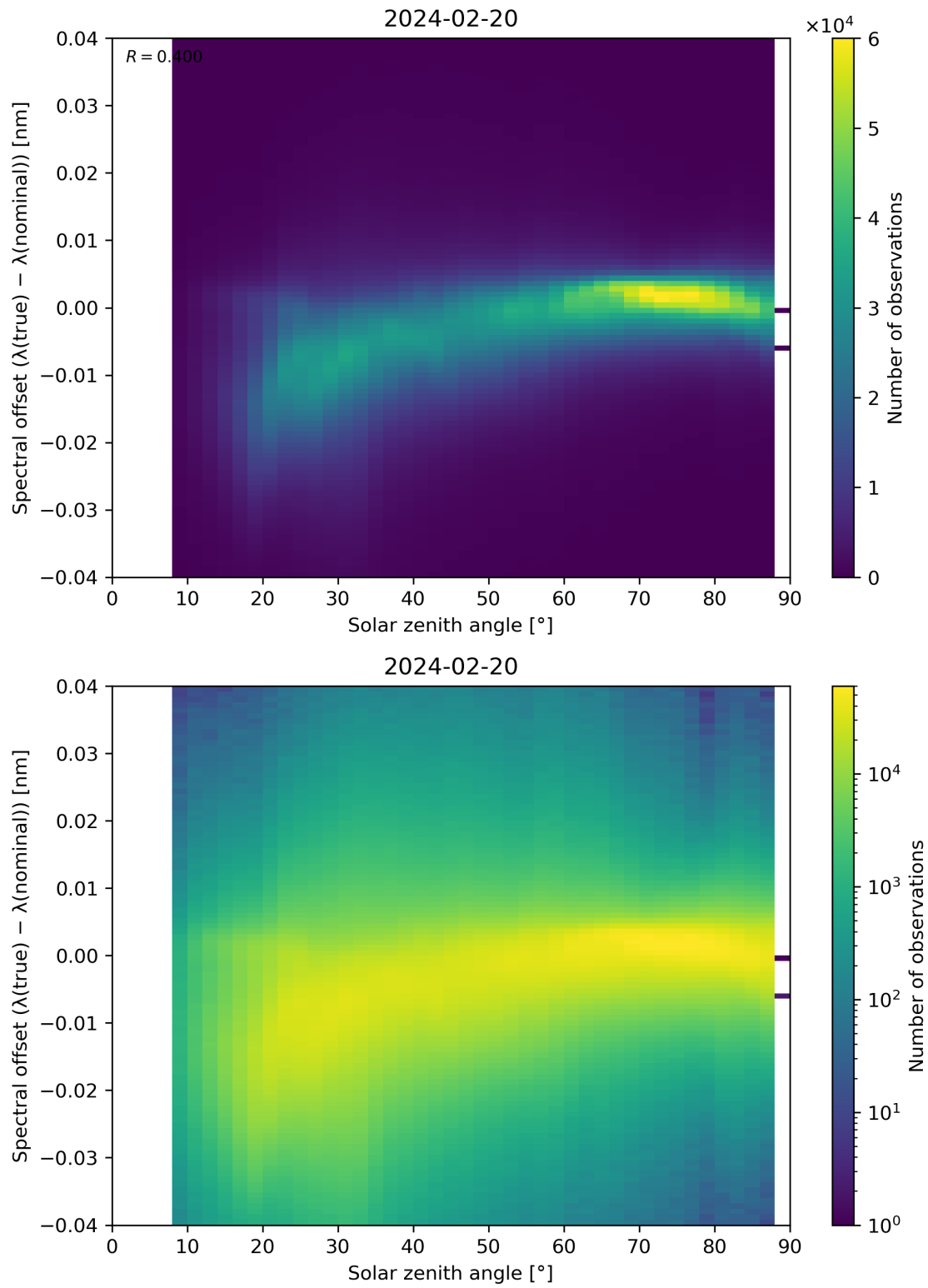
Figure 117: Scatter density plot of “Solar zenith angle” against “Spectral offset ( \lambda(\text{true}) - \lambda(\text{nominal}) )” for 2024-02-19 to 2024-02-21.
