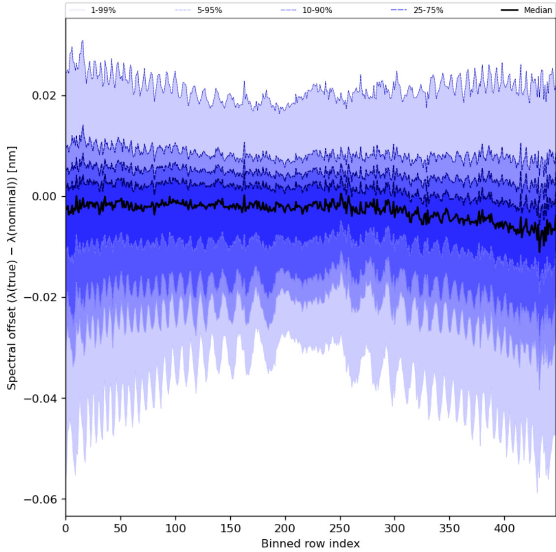
Figure 62: Along track statistics of “Spectral offset ( \lambda(\text{true}) - \lambda(\text{nominal}) )” for 2024-02-19 to 2024-02-21
