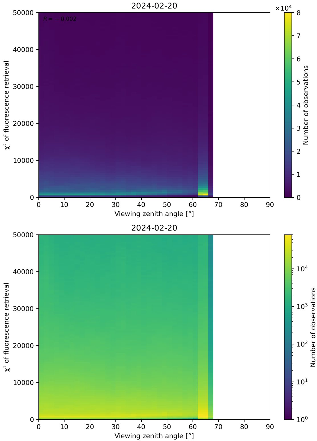
Figure 119: Scatter density plot of “Viewing zenith angle” against “ \chi^2 of fluorescence retrieval” for 2024-02-19 to 2024-02-21.
