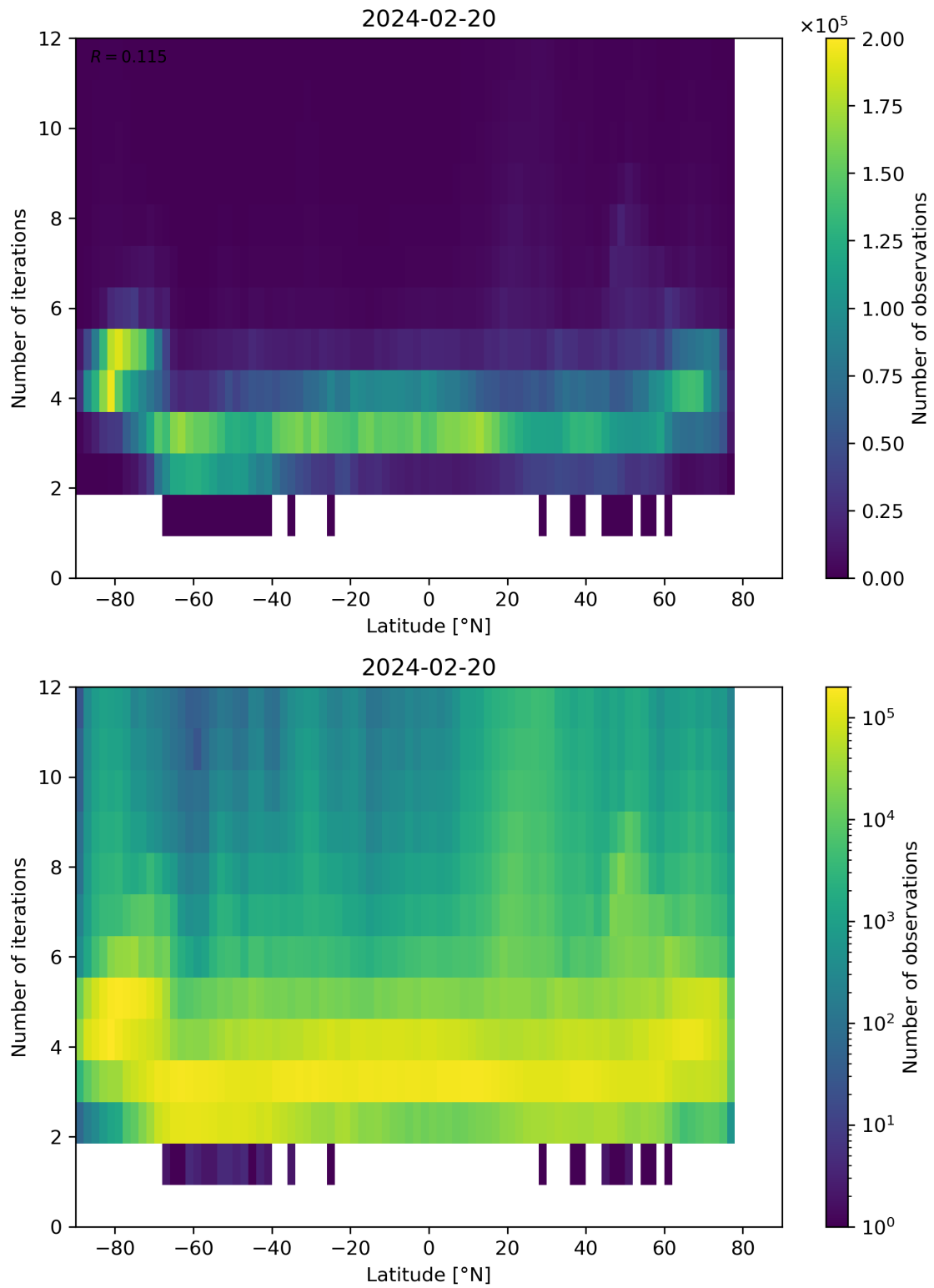
Figure 93: Scatter density plot of “Latitude” against “Number of iterations” for 2024-02-19 to 2024-02-21.
