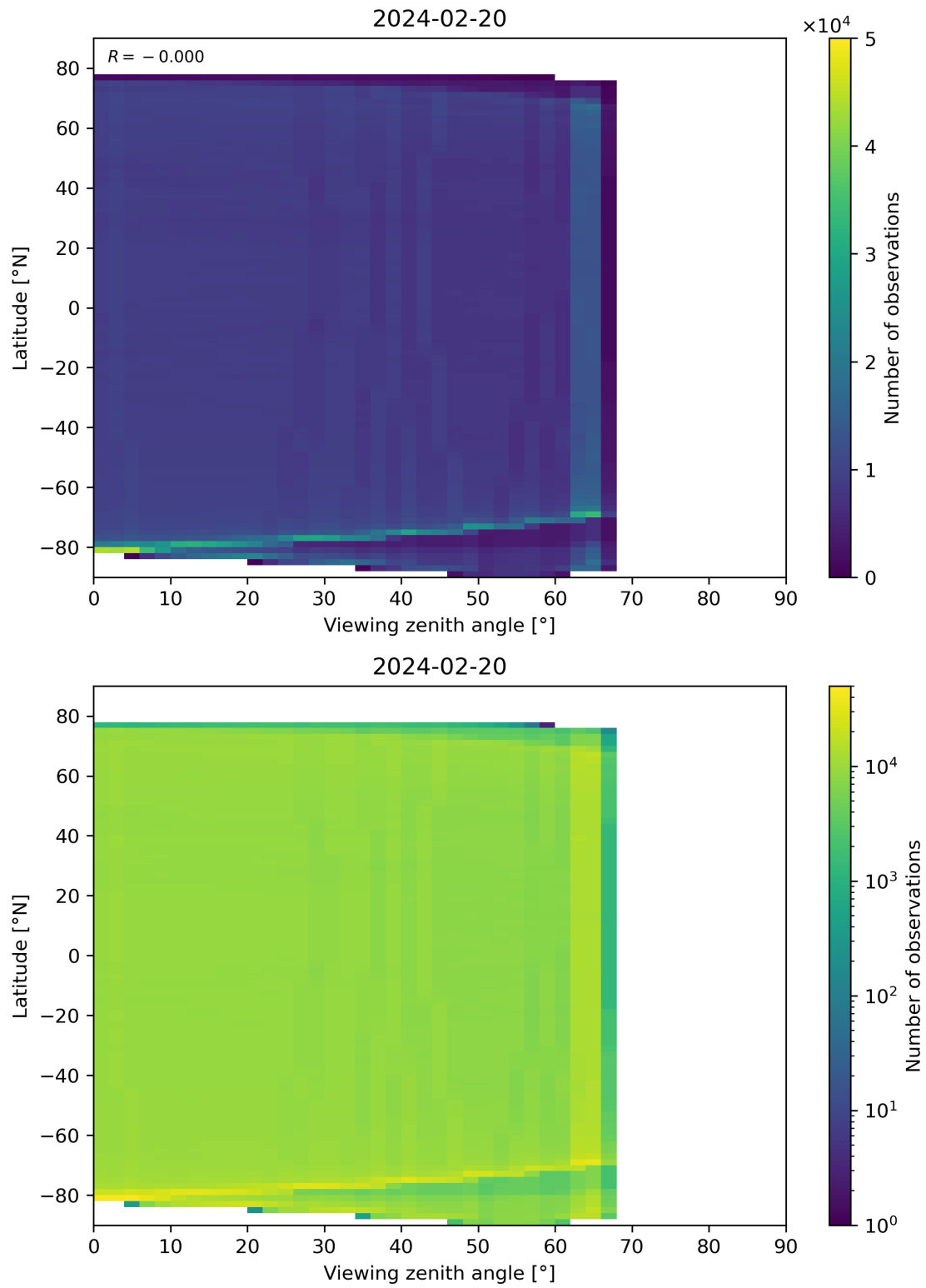
Figure 123: Scatter density plot of “Viewing zenith angle” against “Latitude” for 2024-02-19 to 2024-02-21.
