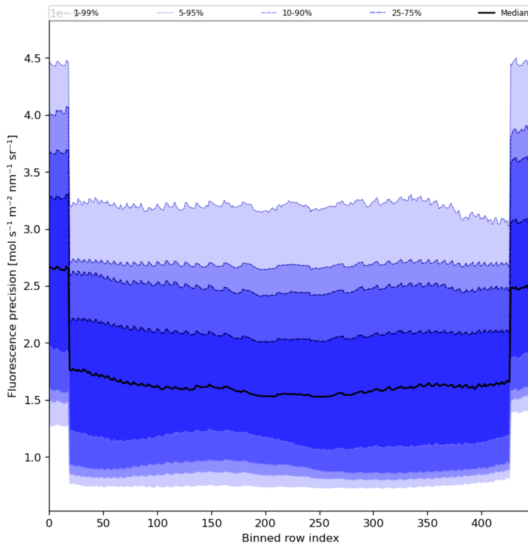
Figure 58: Along track statistics of “Fluorescence precision” for 2024-02-19 to 2024-02-21
