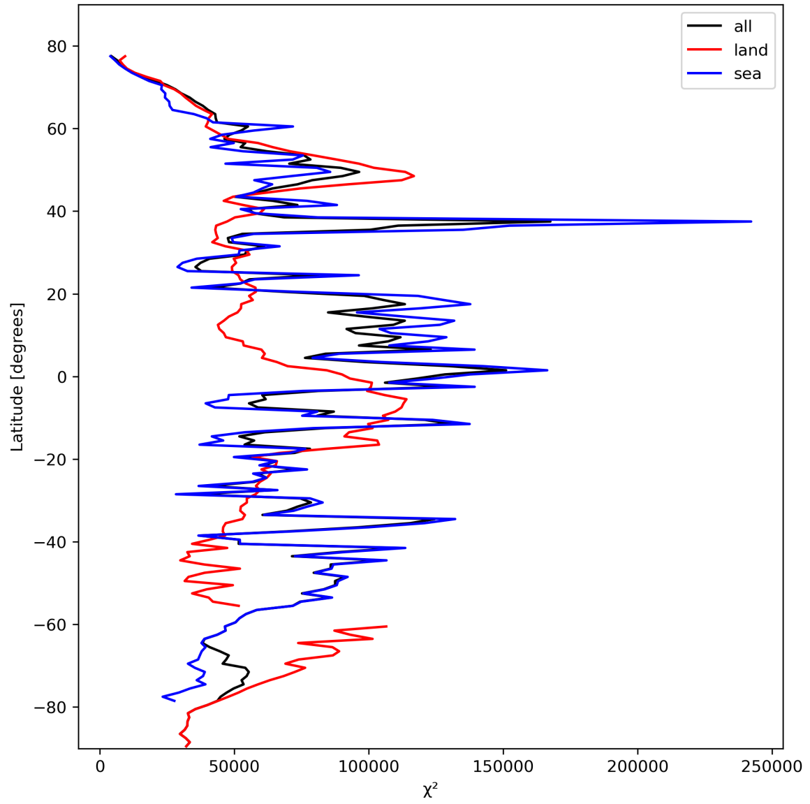
Figure 21: Zonal average of “ \chi^2 ” for 2024-02-19 to 2024-02-21.
