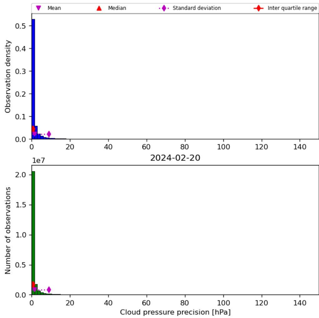
Figure 31: Histogram of “Cloud pressure precision” for 2024-02-19 to 2024-02-21
