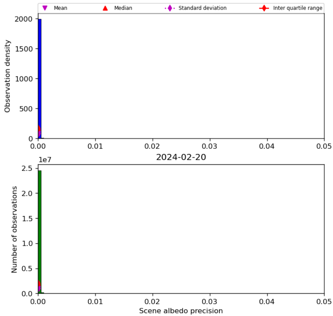
Figure 35: Histogram of “Scene albedo precision” for 2024-02-19 to 2024-02-21
