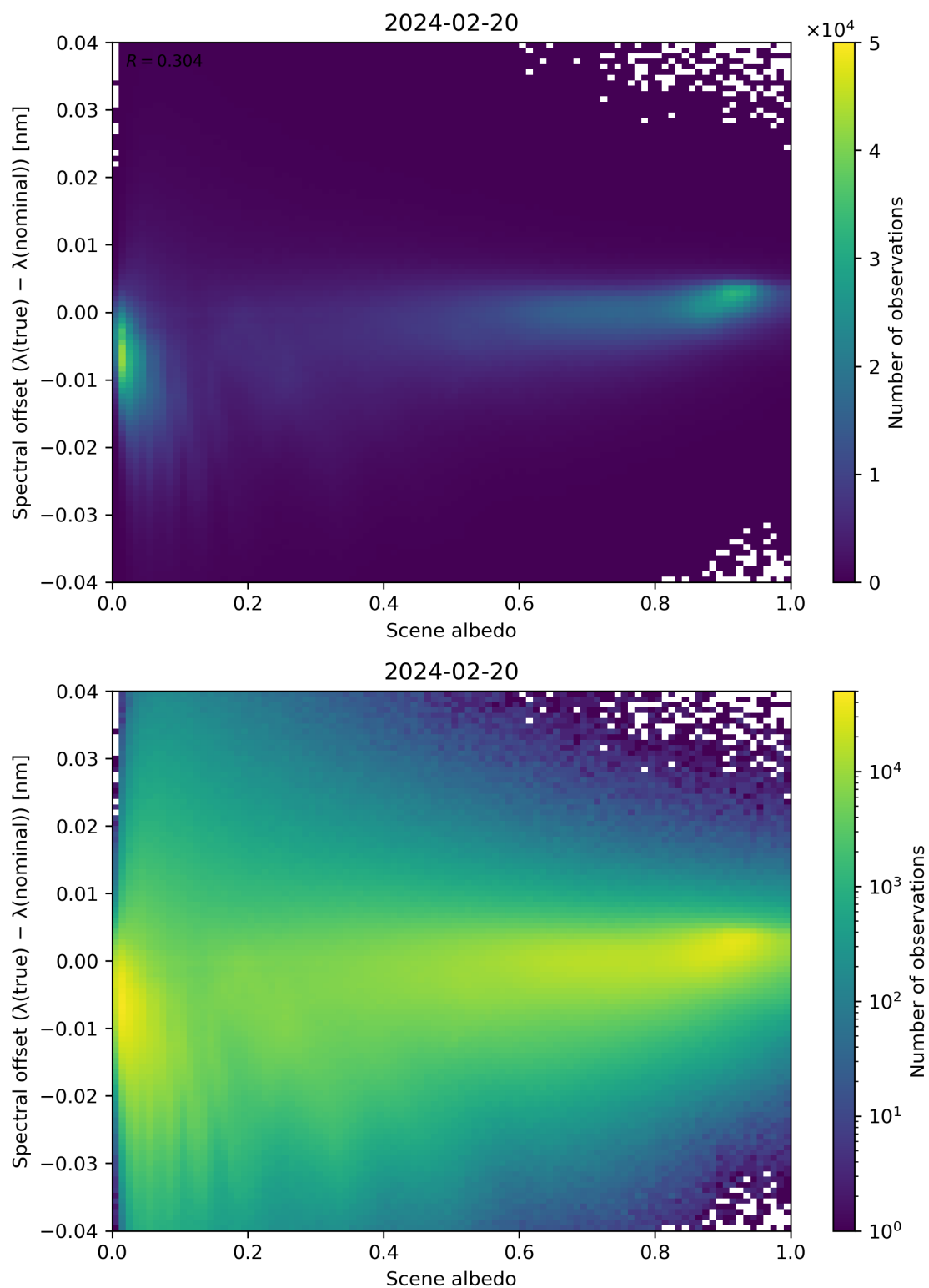
Figure 107: Scatter density plot of “Scene albedo” against “Spectral offset ( \lambda(\text{true}) - \lambda(\text{nominal}) )” for 2024-02-19 to 2024-02-21.
