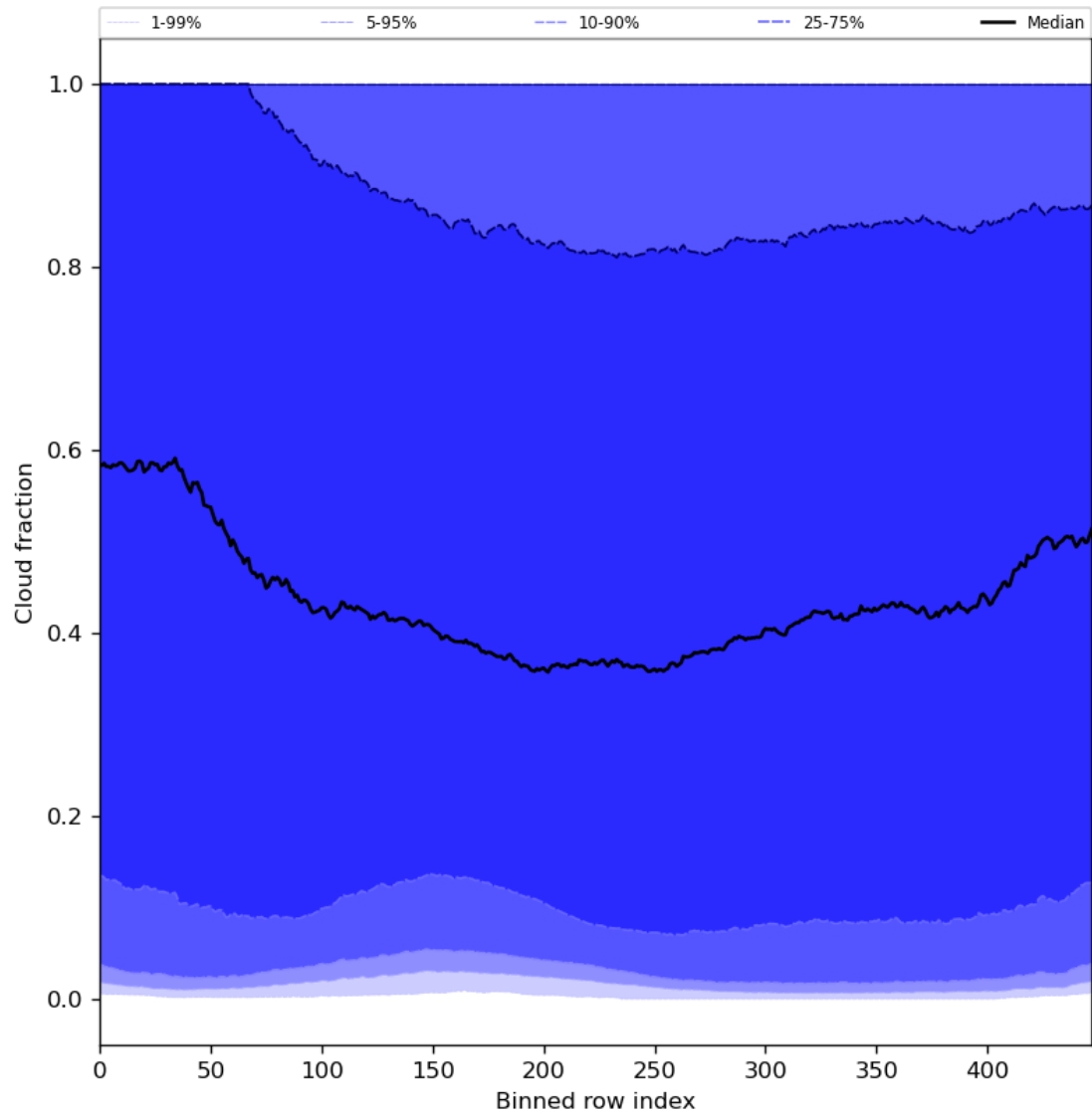
Figure 49: Along track statistics of “Cloud fraction” for 2024-02-19 to 2024-02-21
