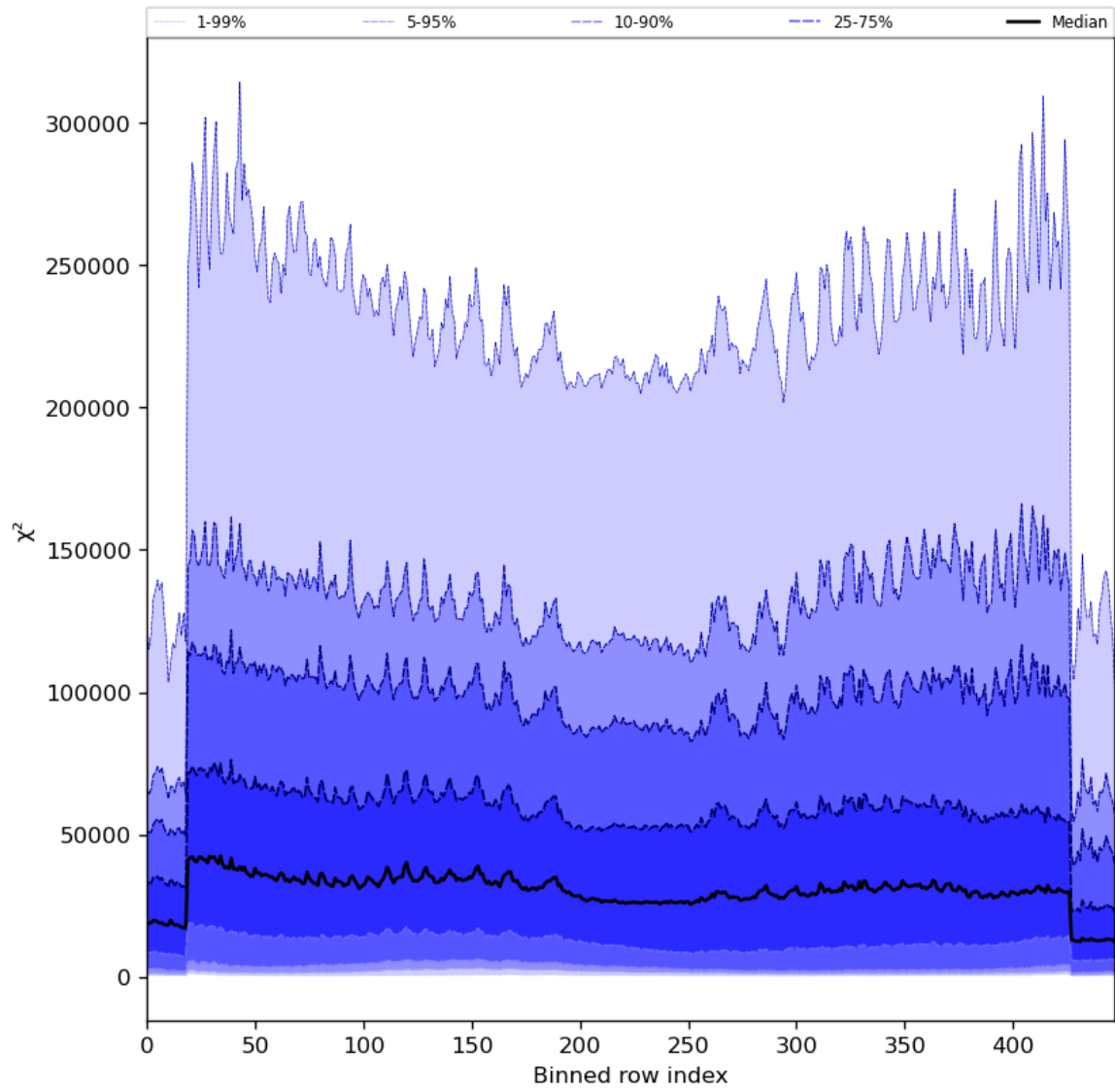
Figure 55: Along track statistics of “ \chi^2 ” for 2024-02-19 to 2024-02-21
