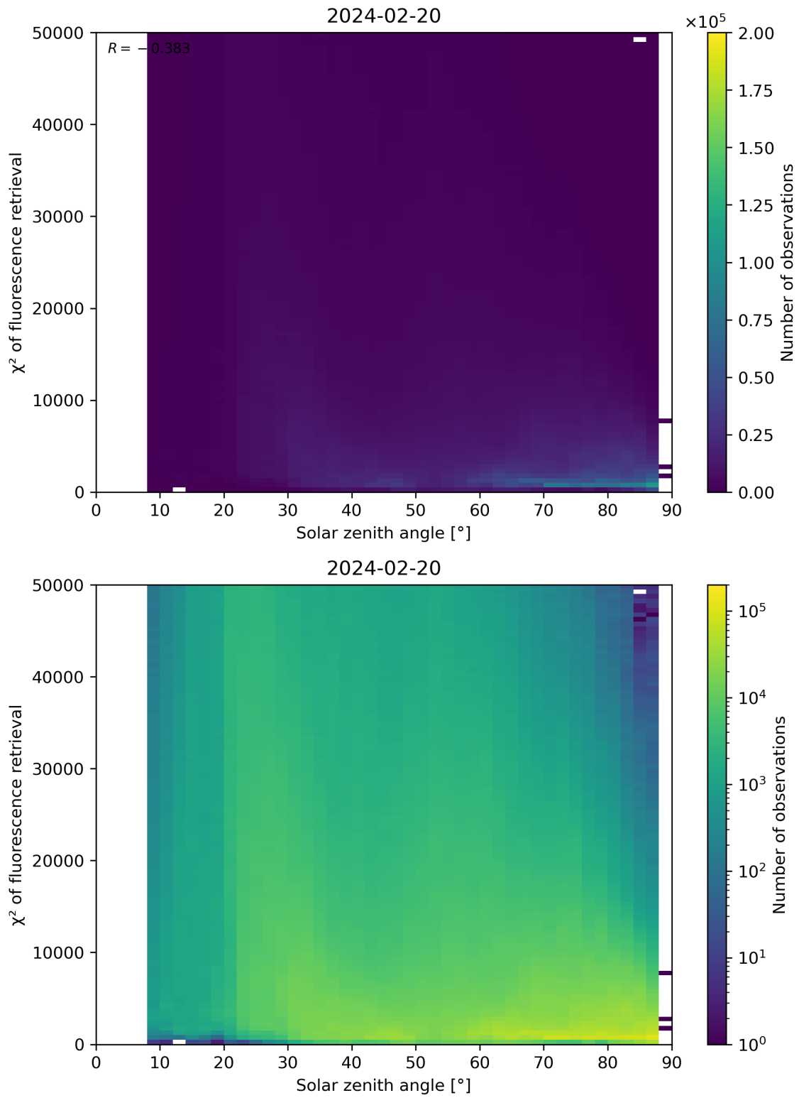
Figure 109: Scatter density plot of “Solar zenith angle” against “ \chi^2 of fluorescence retrieval” for 2024-02-19 to 2024-02-21.
