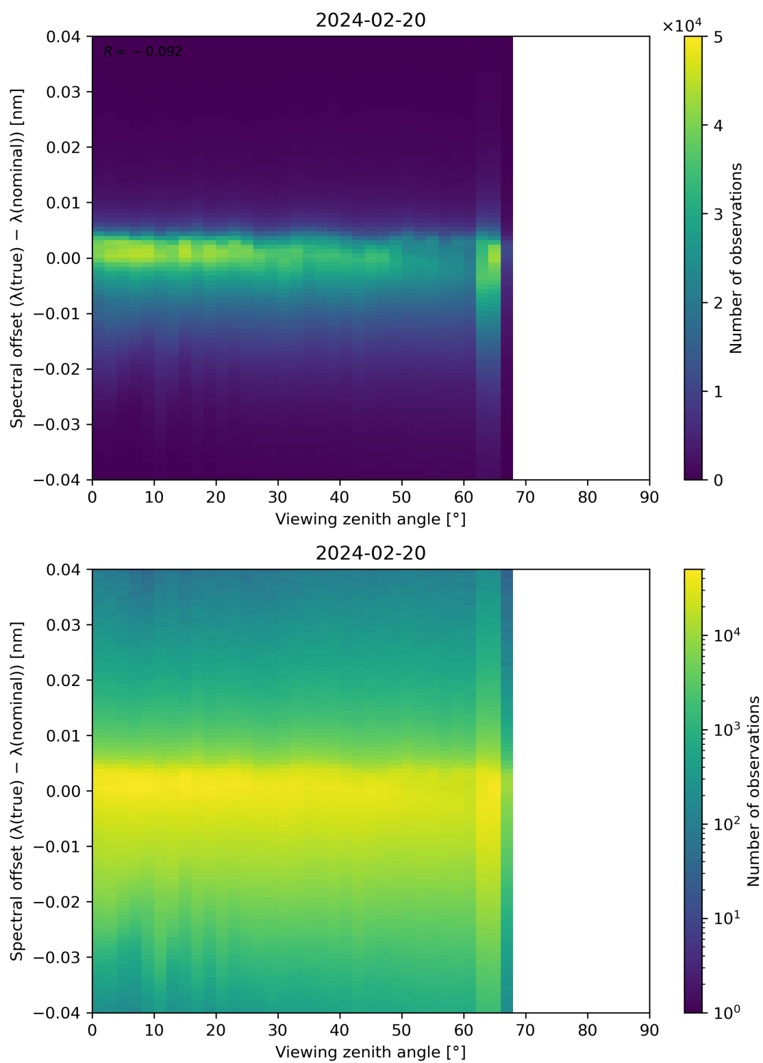
Figure 128: Scatter density plot of “Viewing zenith angle” against “Spectral offset ( \lambda(\text{true}) - \lambda(\text{nominal}) )” for 2024-02-19 to 2024-02-21.
