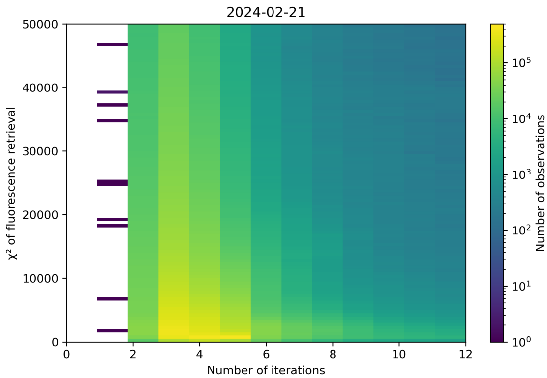
Figure 97: Scatter density plot of “Number of iterations” against “ \chi^2 of fluorescence retrieval” for 2024-02-20 to 2024-02-22.
