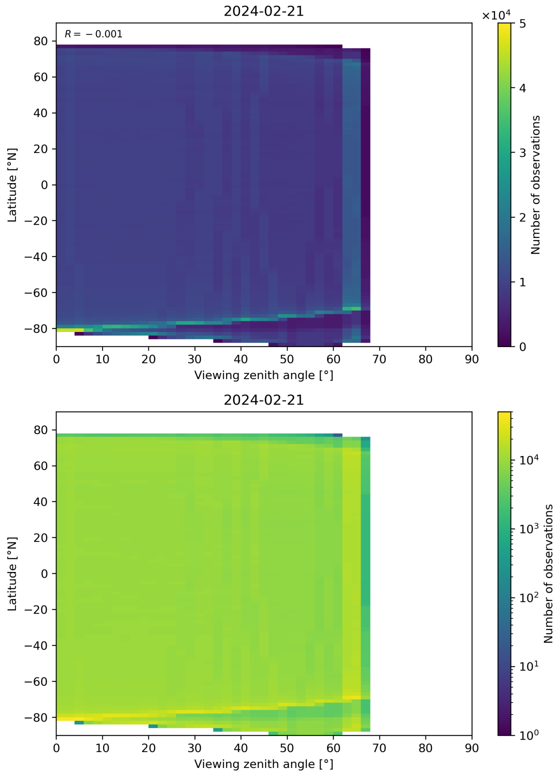
Figure 123: Scatter density plot of “Viewing zenith angle” against “Latitude” for 2024-02-20 to 2024-02-22.
