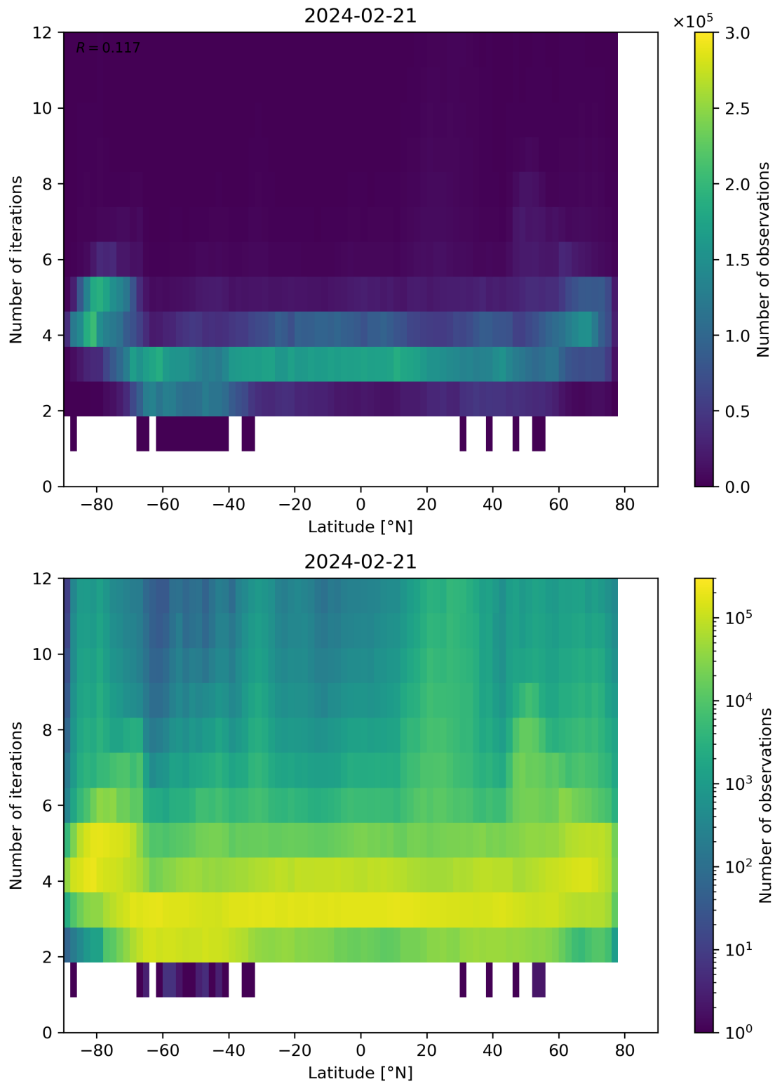
Figure 93: Scatter density plot of “Latitude” against “Number of iterations” for 2024-02-20 to 2024-02-22.
