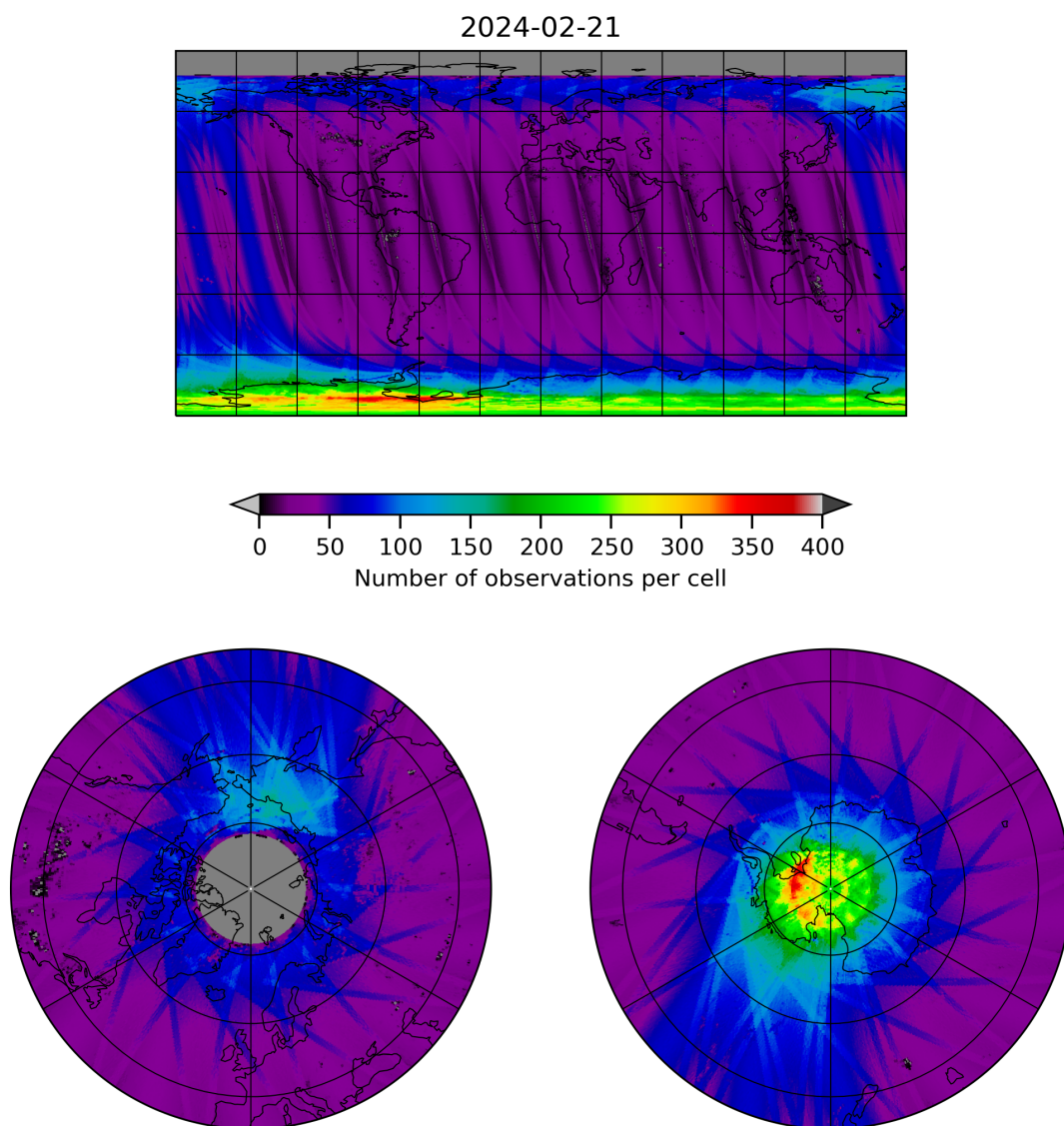
Figure 11: Map of the number of observations for 2024-02-20 to 2024-02-22
