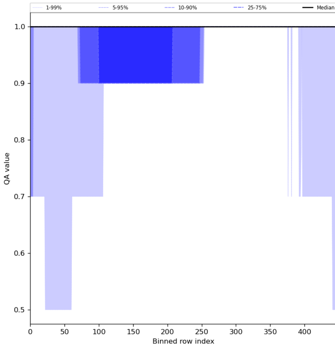
Figure 46: Along track statistics of “QA value” for 2024-02-20 to 2024-02-22
