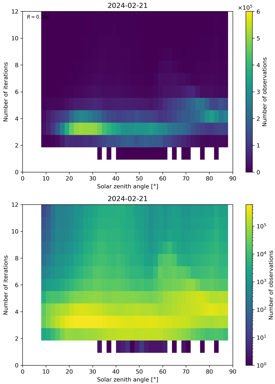
Figure 114: Scatter density plot of “Solar zenith angle” against “Number of iterations” for 2024-02-20 to 2024-02-22.
