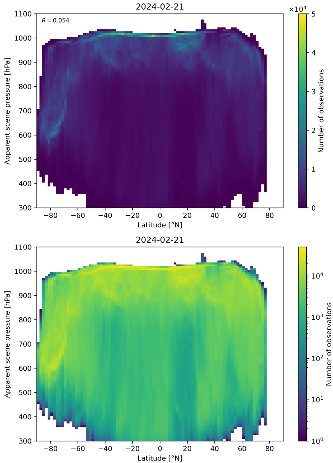
Figure 88: Scatter density plot of “Latitude” against “Apparent scene pressure” for 2024-02-20 to 2024-02-22.
