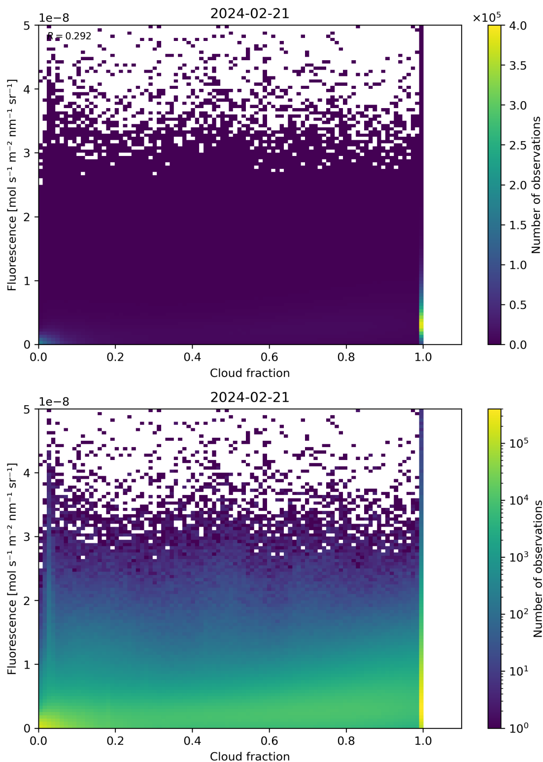
Figure 72: Scatter density plot of “Cloud fraction” against “Fluorescence” for 2024-02-20 to 2024-02-22.
