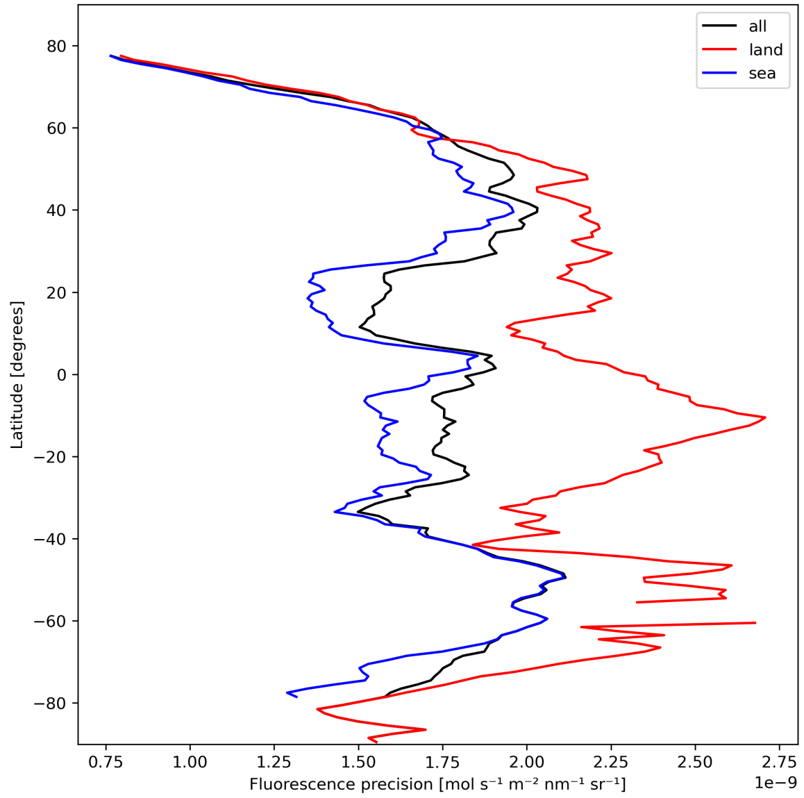
Figure 24: Zonal average of “Fluorescence precision” for 2024-02-20 to 2024-02-22.
