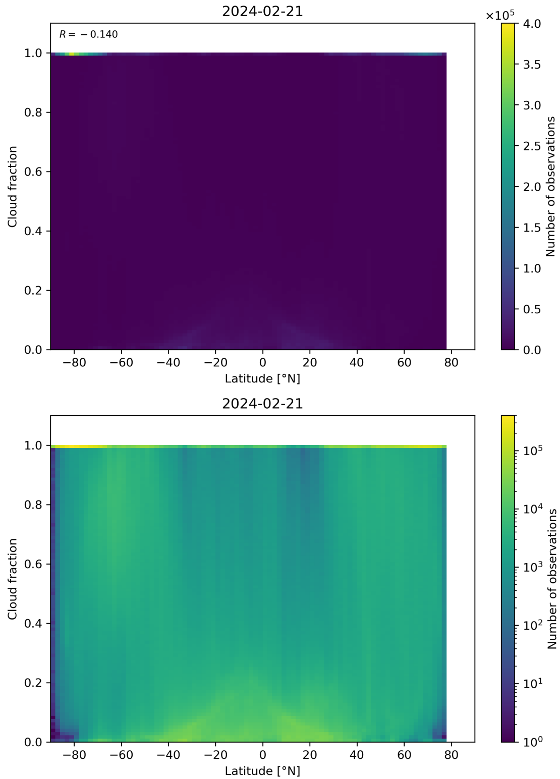
Figure 90: Scatter density plot of “Latitude” against “Cloud fraction” for 2024-02-20 to 2024-02-22.
