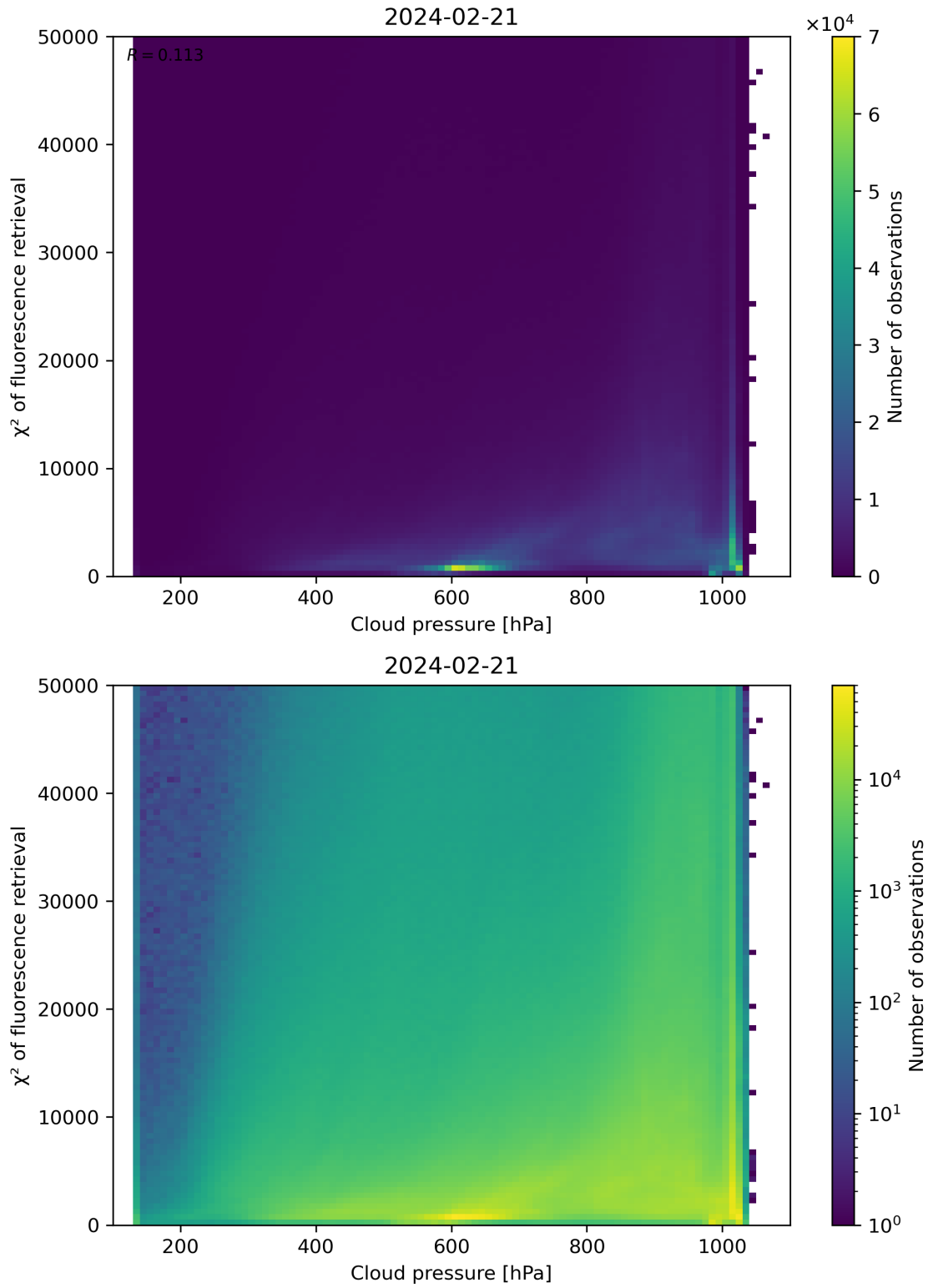
Figure 78: Scatter density plot of “Cloud pressure” against “ \chi^2 of fluorescence retrieval” for 2024-02-20 to 2024-02-22.
