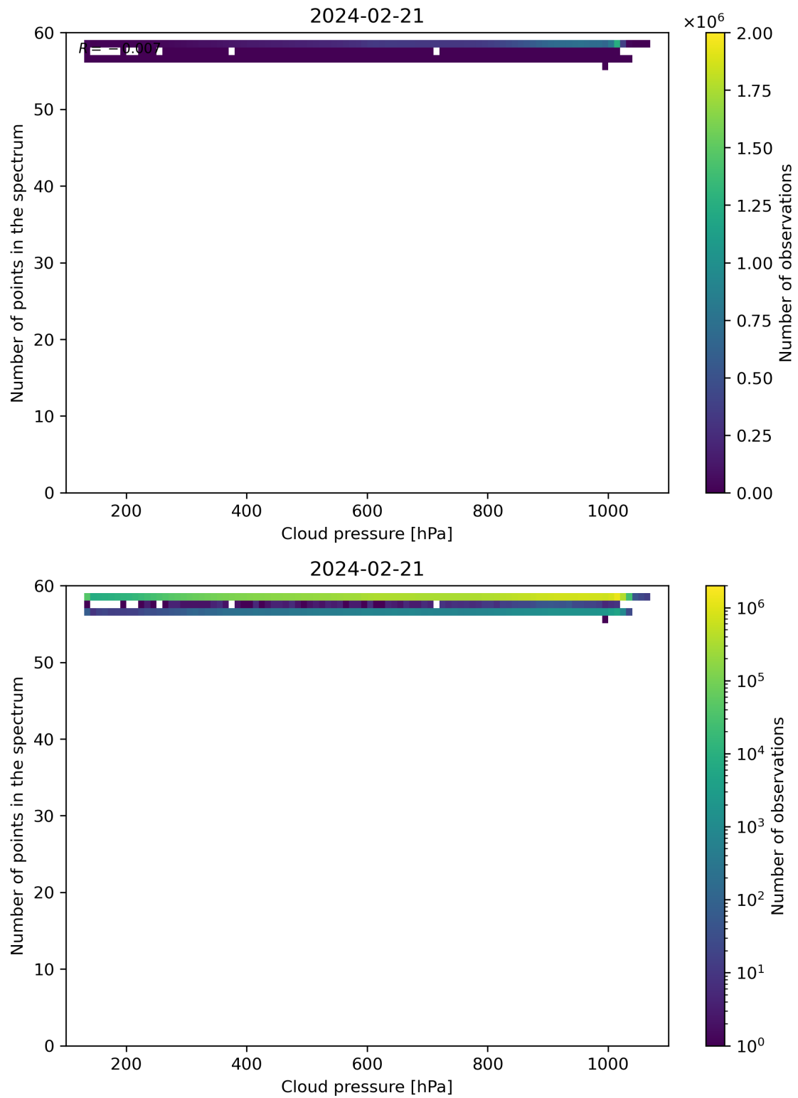
Figure 82: Scatter density plot of “Cloud pressure” against “Number of points in the spectrum” for 2024-02-20 to 2024-02-22.
