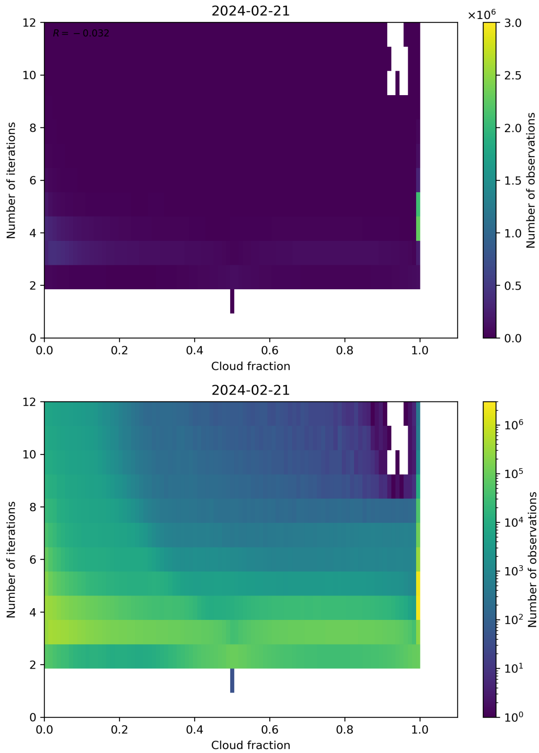
Figure 73: Scatter density plot of “Cloud fraction” against “Number of iterations” for 2024-02-20 to 2024-02-22.
