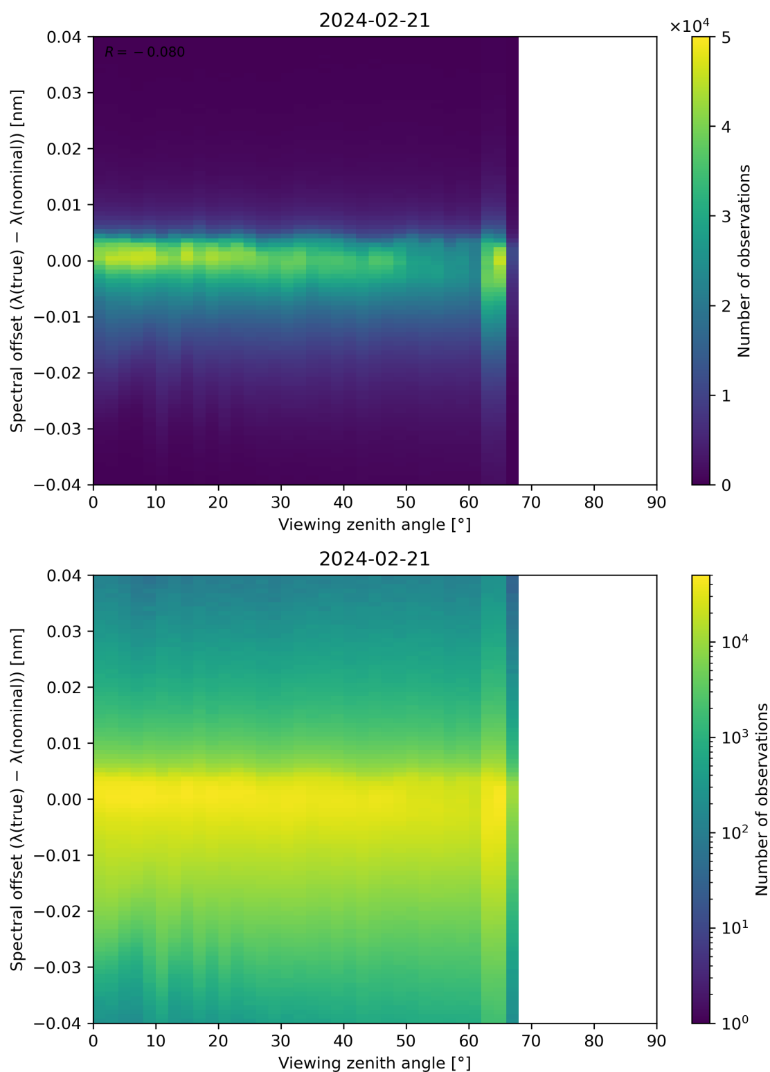
Figure 128: Scatter density plot of “Viewing zenith angle” against “Spectral offset ( \lambda(\text{true}) - \lambda(\text{nominal}) )” for 2024-02-20 to 2024-02-22.
