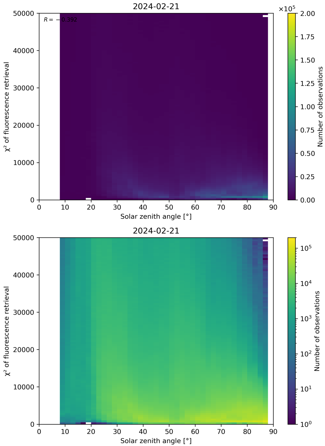
Figure 109: Scatter density plot of “Solar zenith angle” against “ \chi^2 of fluorescence retrieval” for 2024-02-20 to 2024-02-22.
