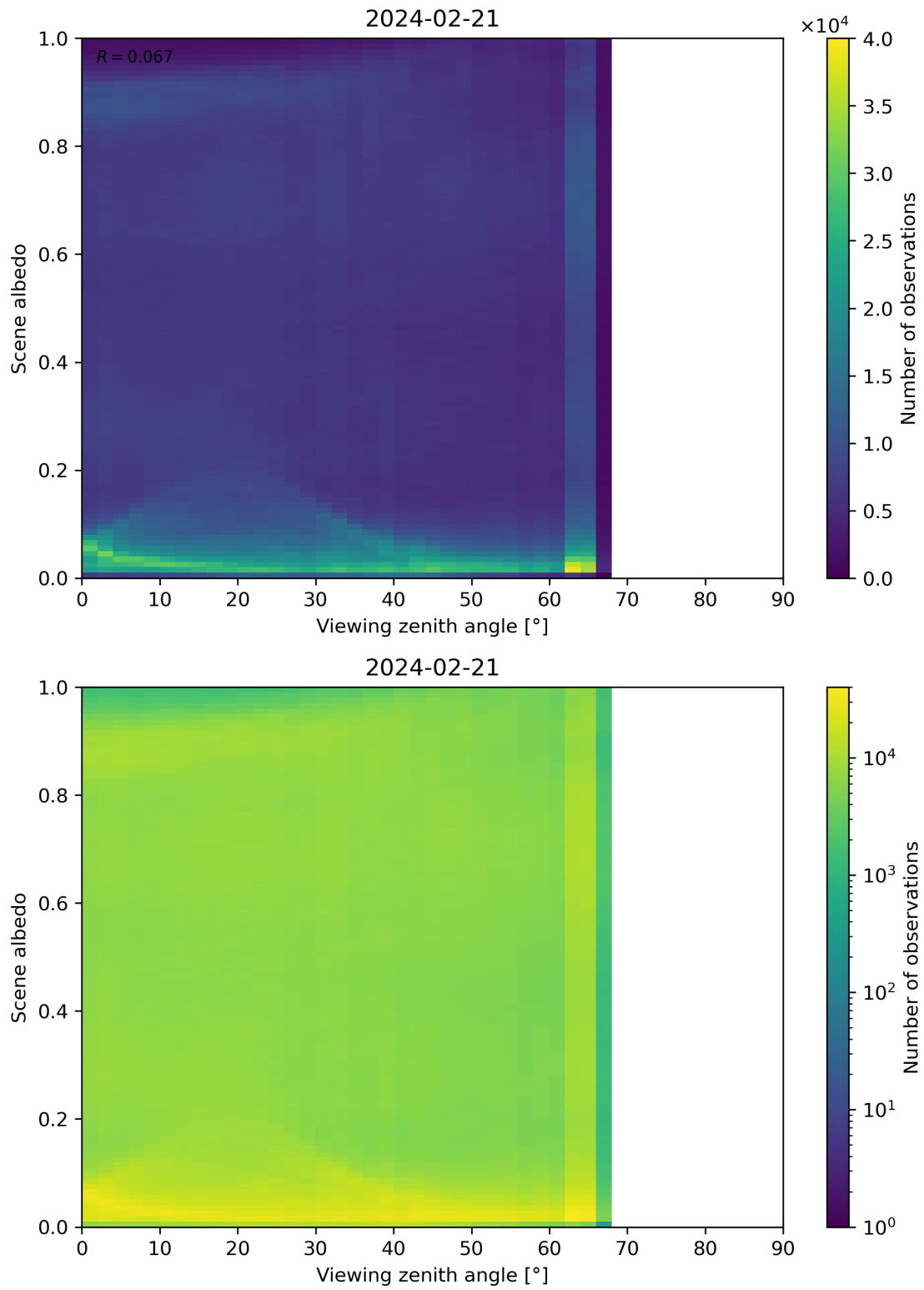
Figure 126: Scatter density plot of “Viewing zenith angle” against “Scene albedo” for 2024-02-20 to 2024-02-22.
