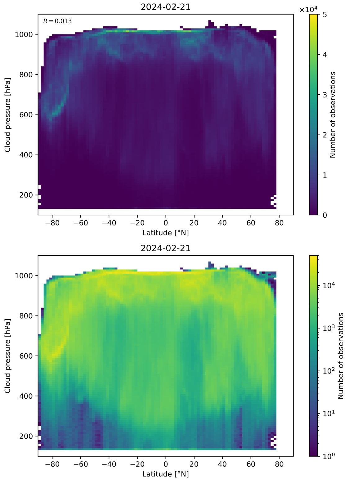
Figure 91: Scatter density plot of “Latitude” against “Cloud pressure” for 2024-02-20 to 2024-02-22.
