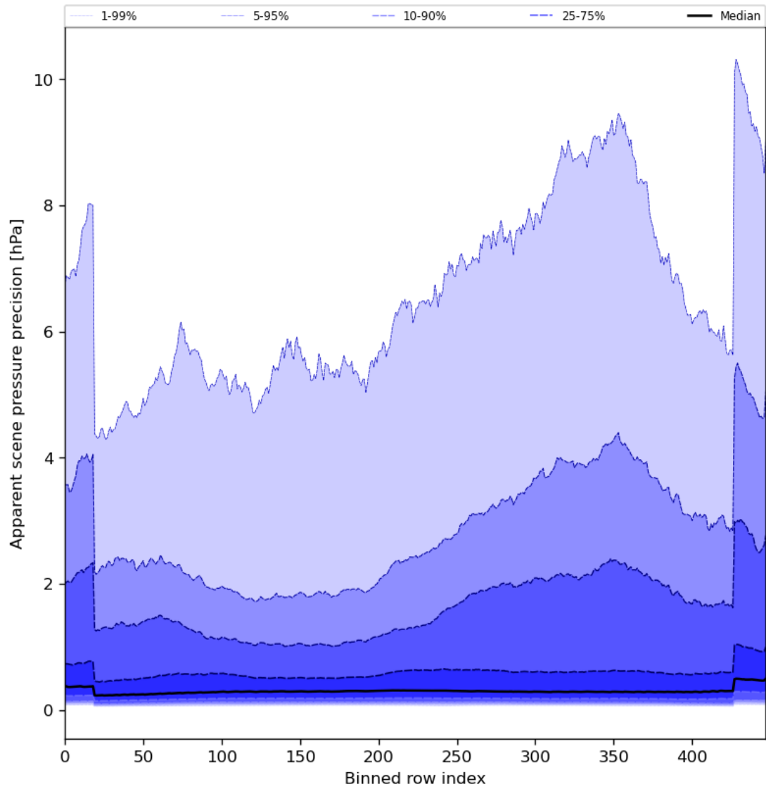
Figure 54: Along track statistics of “Apparent scene pressure precision” for 2024-02-20 to 2024-02-22
