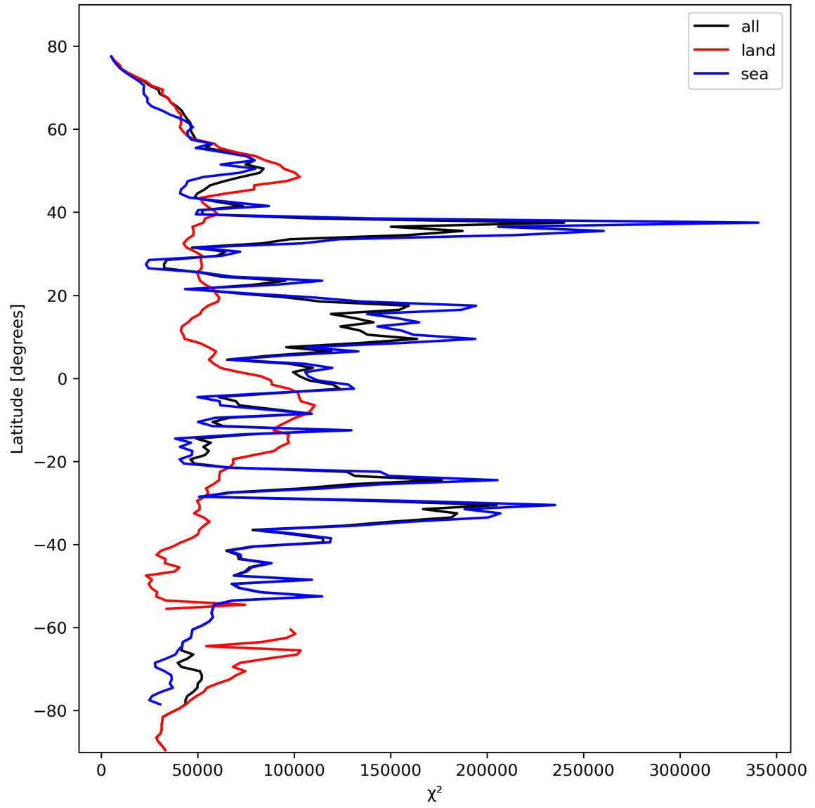
Figure 21: Zonal average of “ \chi^2 ” for 2024-02-20 to 2024-02-22.
