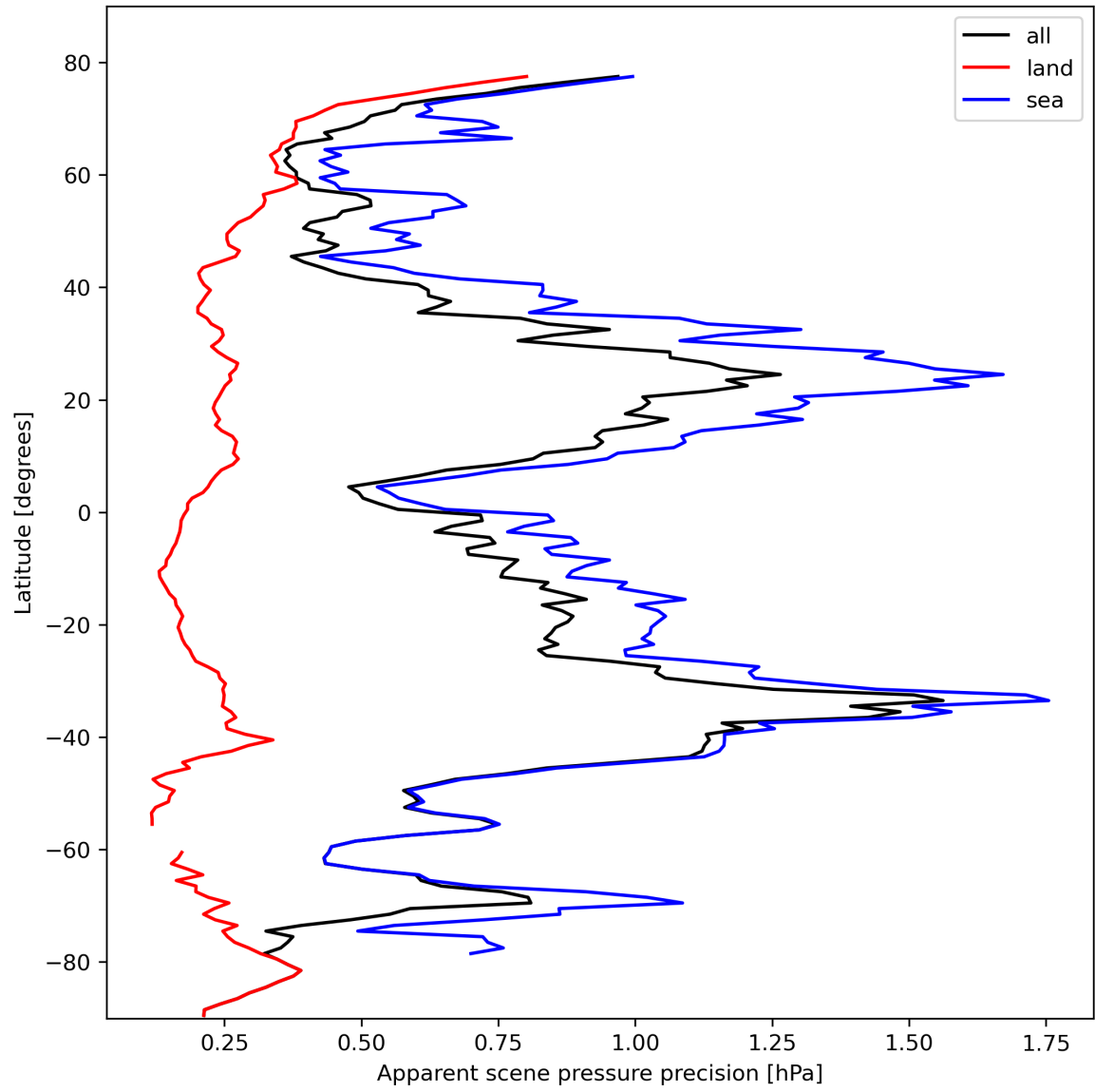
Figure 20: Zonal average of “Apparent scene pressure precision” for 2024-02-20 to 2024-02-22.
