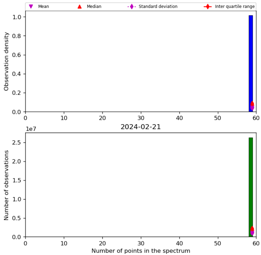
Figure 44: Histogram of “Number of points in the spectrum” for 2024-02-20 to 2024-02-22
