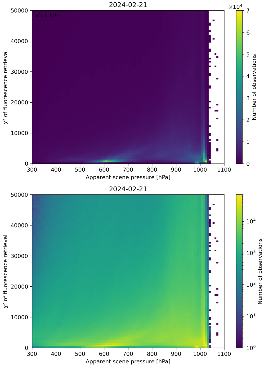
Figure 63: Scatter density plot of “Apparent scene pressure” against “ \chi^2 of fluorescence retrieval” for 2024-02-20 to 2024-02-22.
