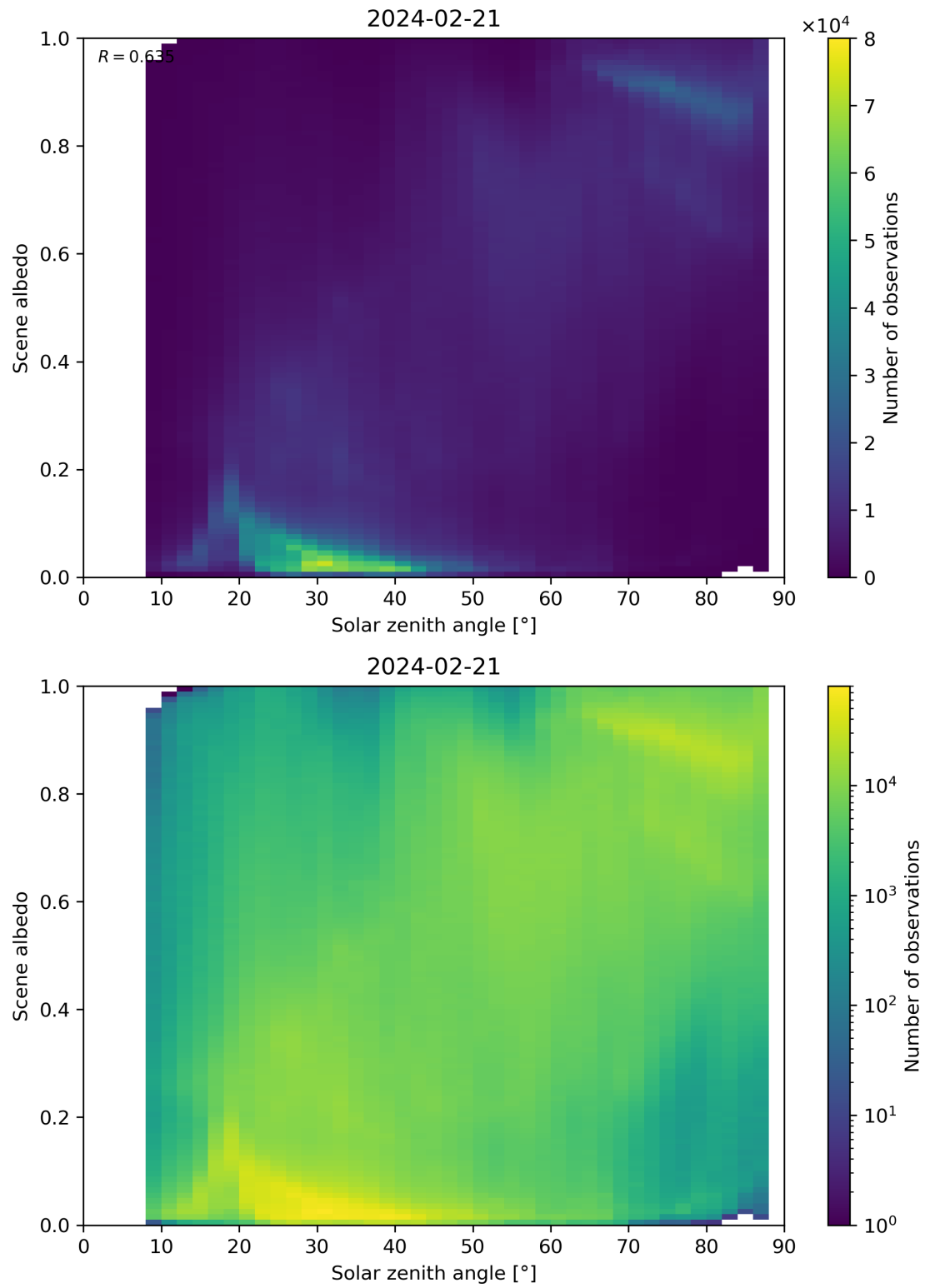
Figure 116: Scatter density plot of “Solar zenith angle” against “Scene albedo” for 2024-02-20 to 2024-02-22.
