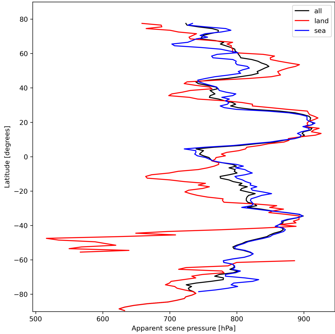
Figure 19: Zonal average of “Apparent scene pressure” for 2024-02-20 to 2024-02-22.
