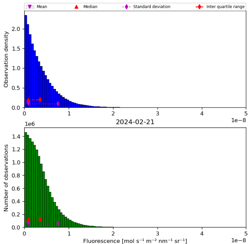
Figure 40: Histogram of “Fluorescence” for 2024-02-20 to 2024-02-22
