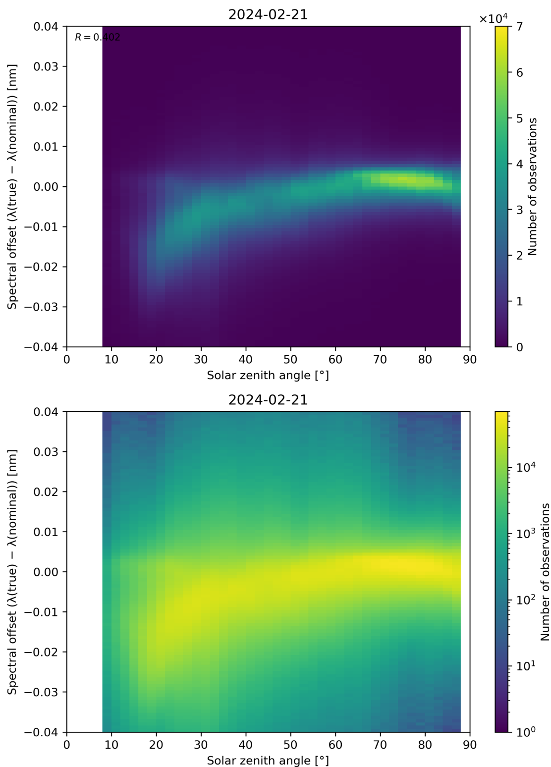
Figure 117: Scatter density plot of “Solar zenith angle” against “Spectral offset ( \lambda(\text{true}) - \lambda(\text{nominal}) )” for 2024-02-20 to 2024-02-22.
