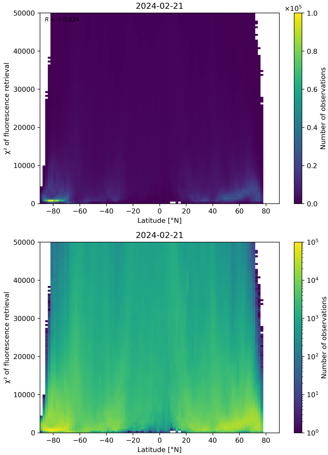
Figure 89: Scatter density plot of “Latitude” against “ \chi^2 of fluorescence retrieval” for 2024-02-20 to 2024-02-22.
