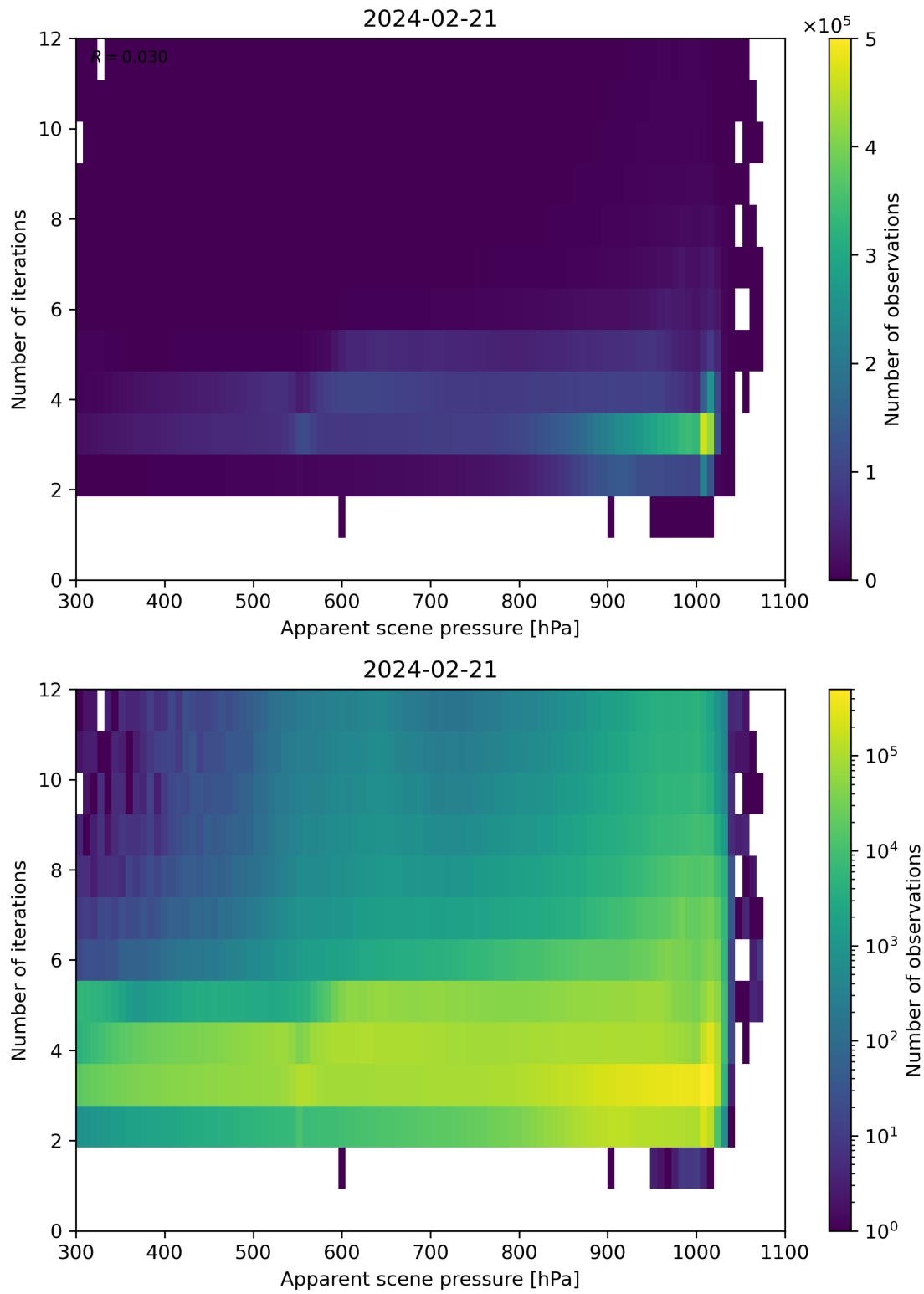
Figure 65: Scatter density plot of “Apparent scene pressure” against “Number of iterations” for 2024-02-20 to 2024-02-22.
