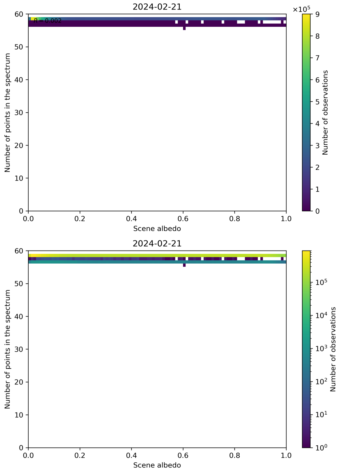
Figure 106: Scatter density plot of “Scene albedo” against “Number of points in the spectrum” for 2024-02-20 to 2024-02-22.
