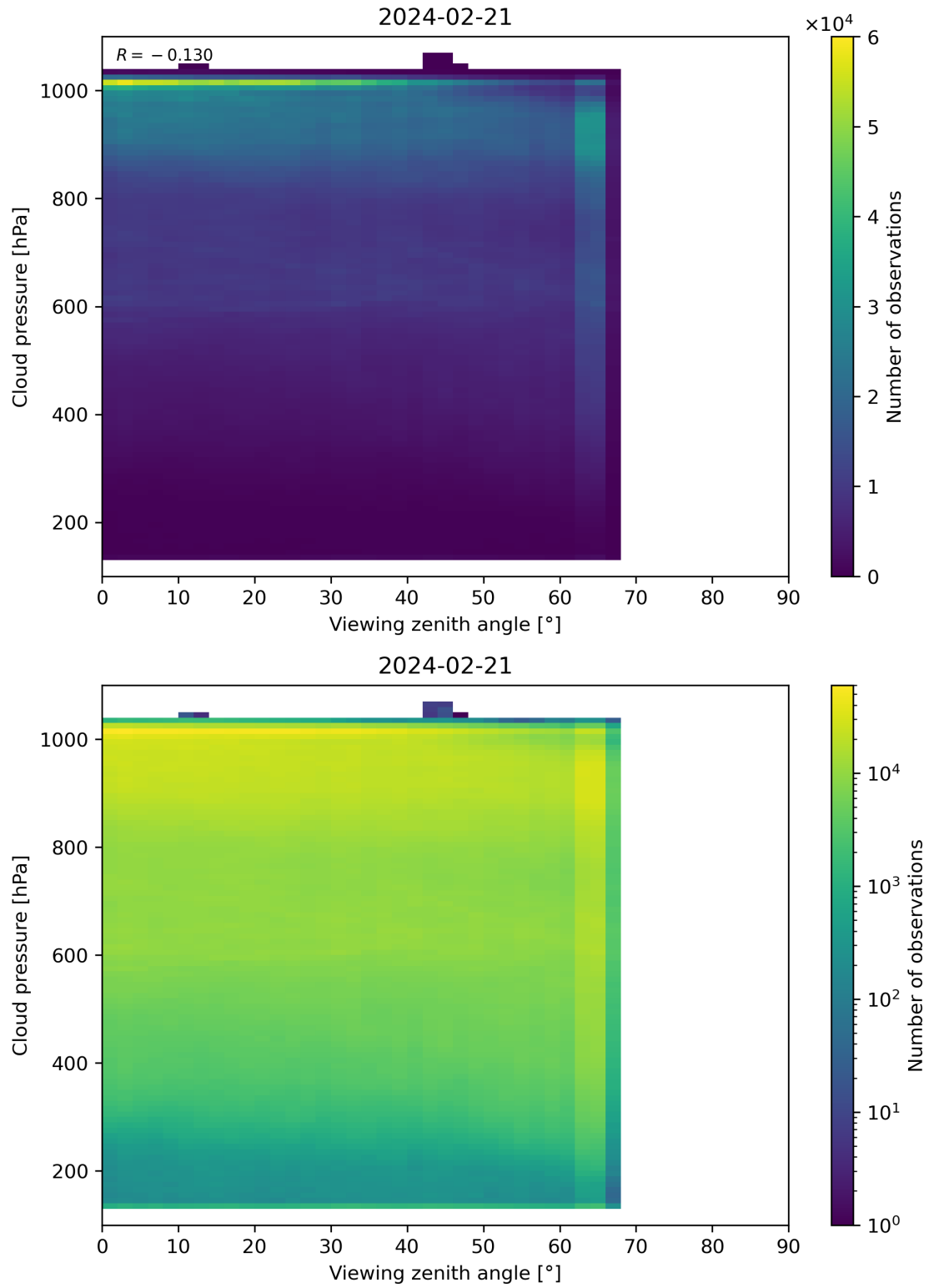
Figure 121: Scatter density plot of “Viewing zenith angle” against “Cloud pressure” for 2024-02-20 to 2024-02-22.
