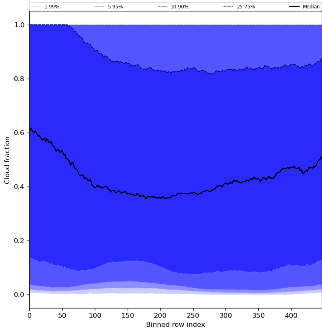
Figure 49: Along track statistics of “Cloud fraction” for 2024-02-20 to 2024-02-22
