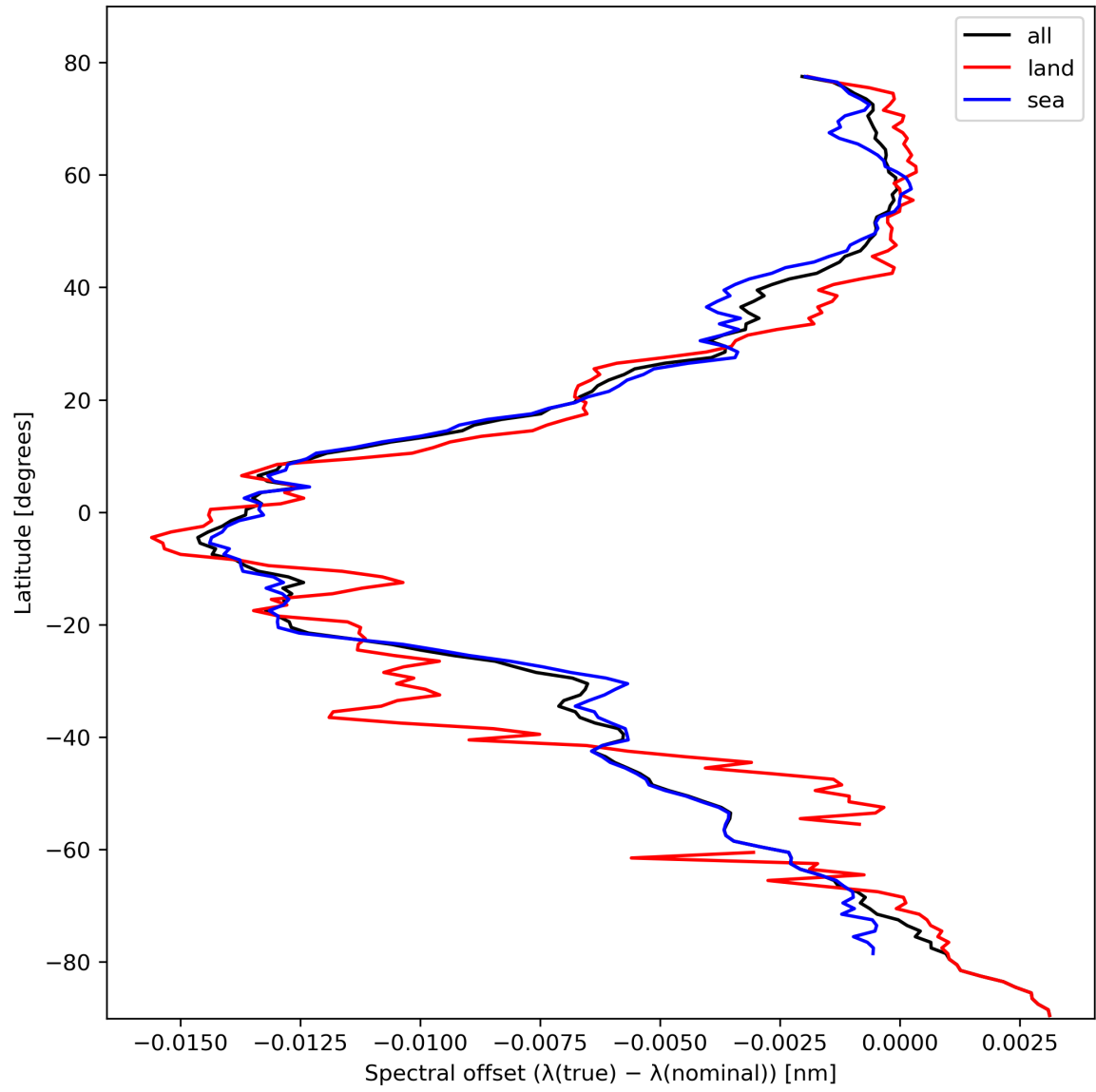
Figure 28: Zonal average of “Spectral offset ( \lambda(\text{true}) - \lambda(\text{nominal}) )” for 2024-02-20 to 2024-02-22.
