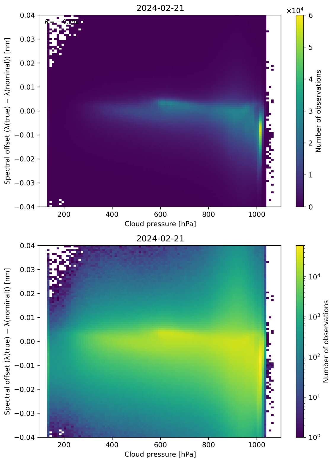
Figure 84: Scatter density plot of “Cloud pressure” against “Spectral offset ( \lambda(\text{true}) - \lambda(\text{nominal}) )” for 2024-02-20 to 2024-02-22.
