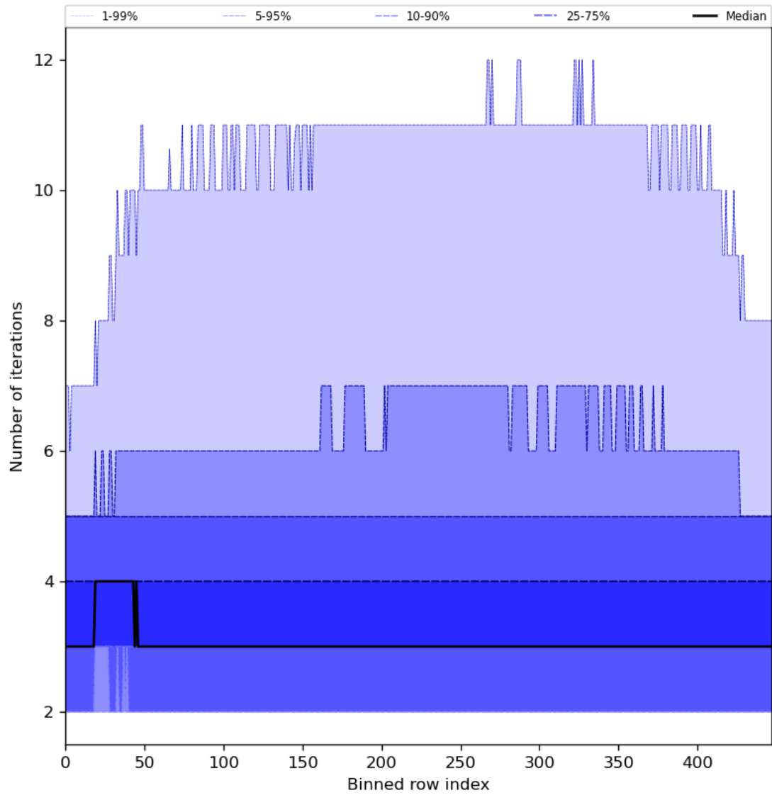
Figure 56: Along track statistics of “Number of iterations” for 2024-02-20 to 2024-02-22
