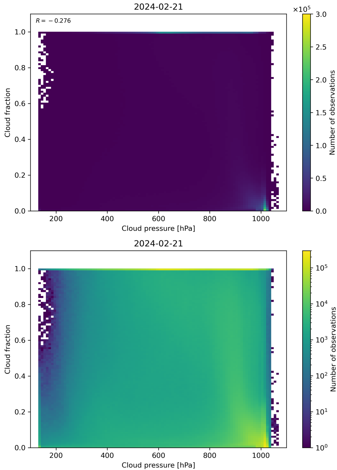
Figure 79: Scatter density plot of “Cloud pressure” against “Cloud fraction” for 2024-02-20 to 2024-02-22.
