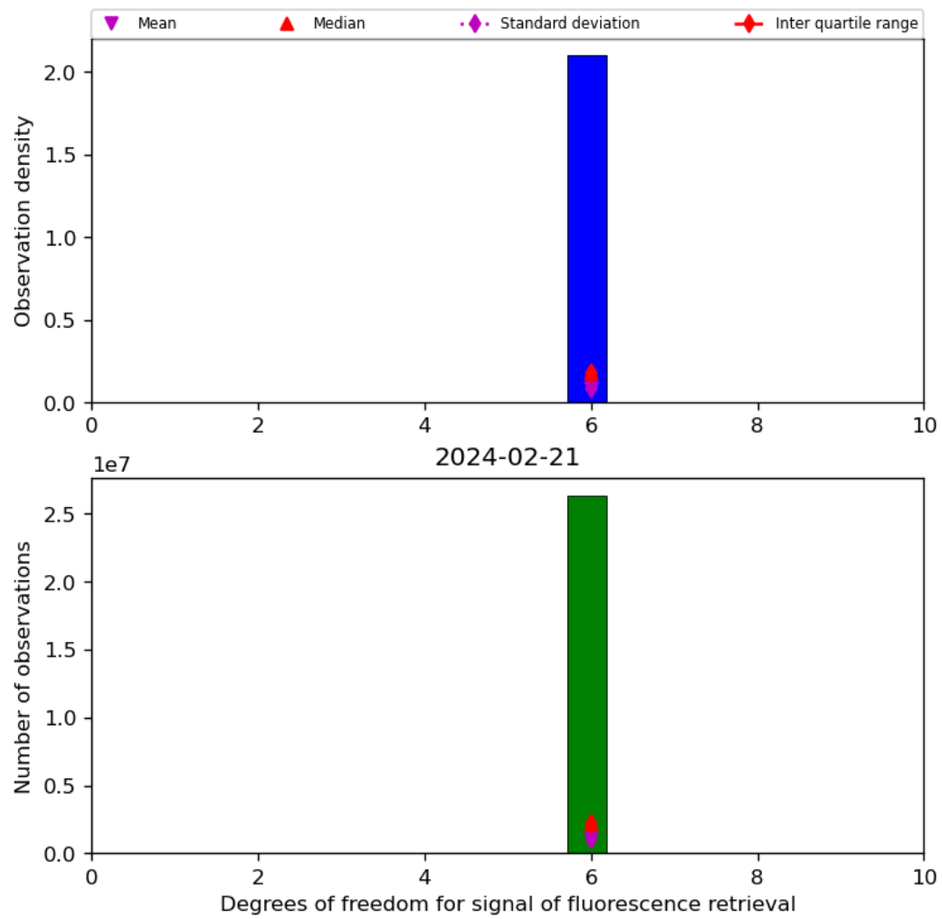
Figure 43: Histogram of “Degrees of freedom for signal of fluorescence retrieval” for 2024-02-20 to 2024-02-22
