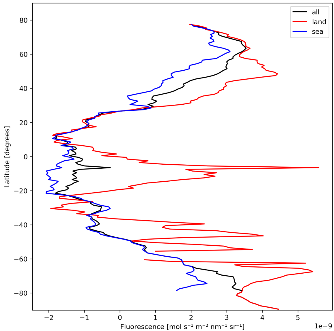
Figure 23: Zonal average of “Fluorescence” for 2024-02-20 to 2024-02-22.
