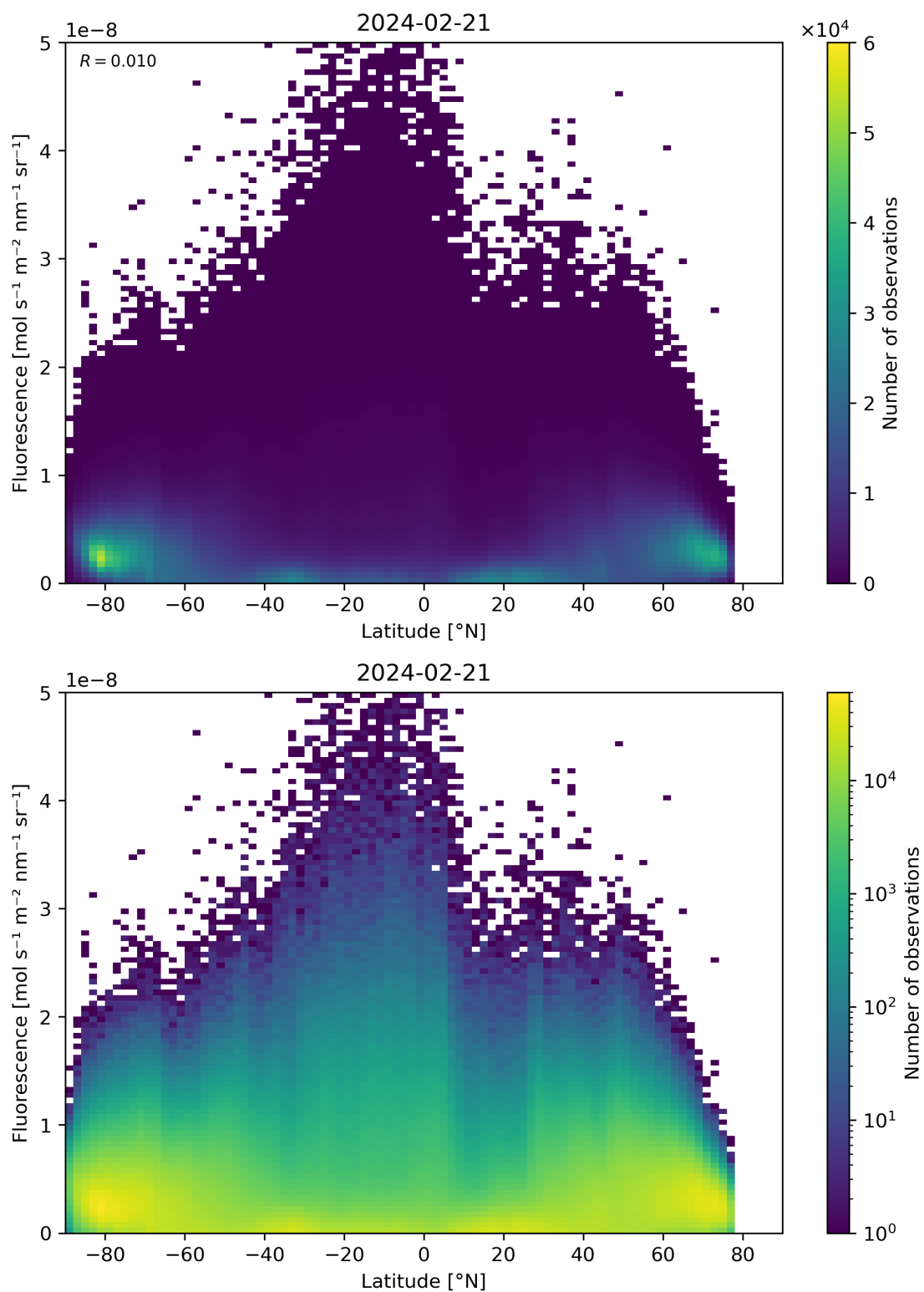
Figure 92: Scatter density plot of “Latitude” against “Fluorescence” for 2024-02-20 to 2024-02-22.
