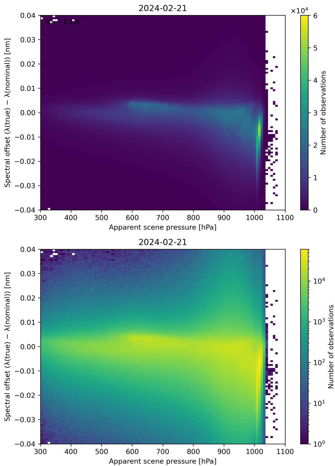
Figure 67: Scatter density plot of “Apparent scene pressure” against “Spectral offset ( \lambda(\text{true}) - \lambda(\text{nominal}) )” for 2024-02-20 to 2024-02-22.
