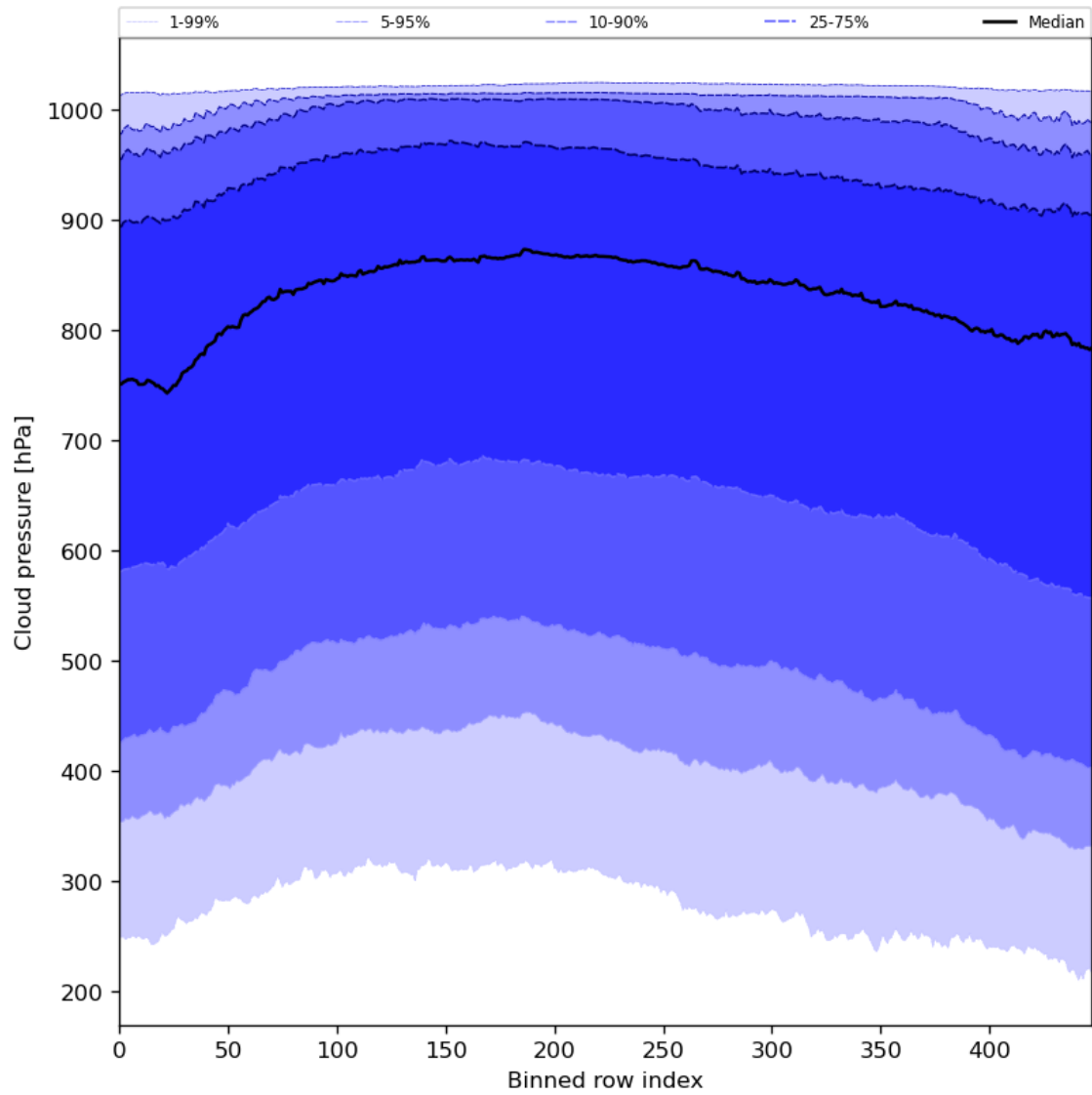
Figure 47: Along track statistics of “Cloud pressure” for 2024-02-20 to 2024-02-22
