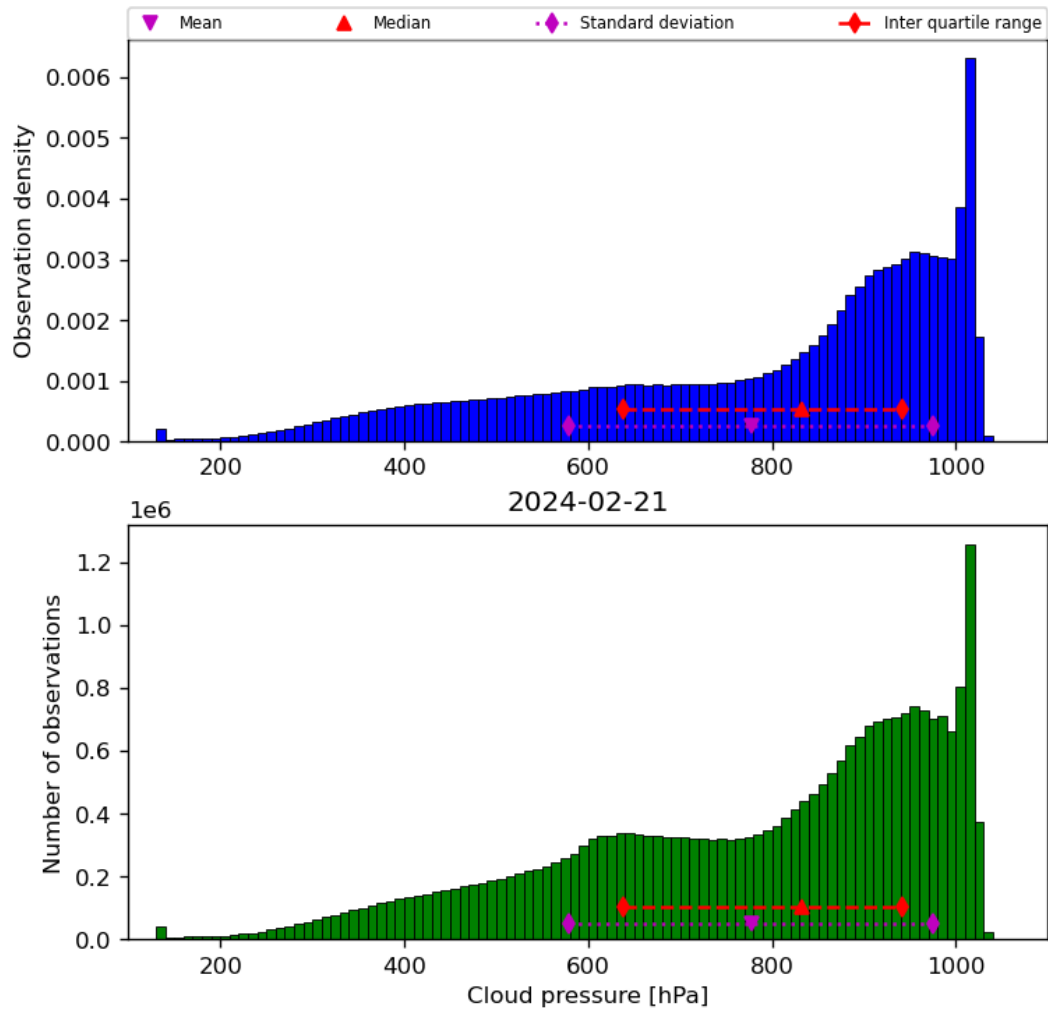
Figure 30: Histogram of “Cloud pressure” for 2024-02-20 to 2024-02-22
