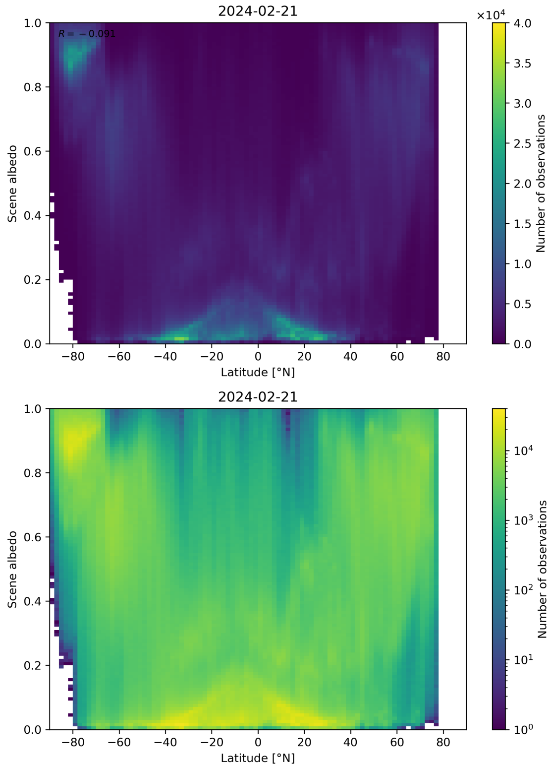
Figure 95: Scatter density plot of “Latitude” against “Scene albedo” for 2024-02-20 to 2024-02-22.
