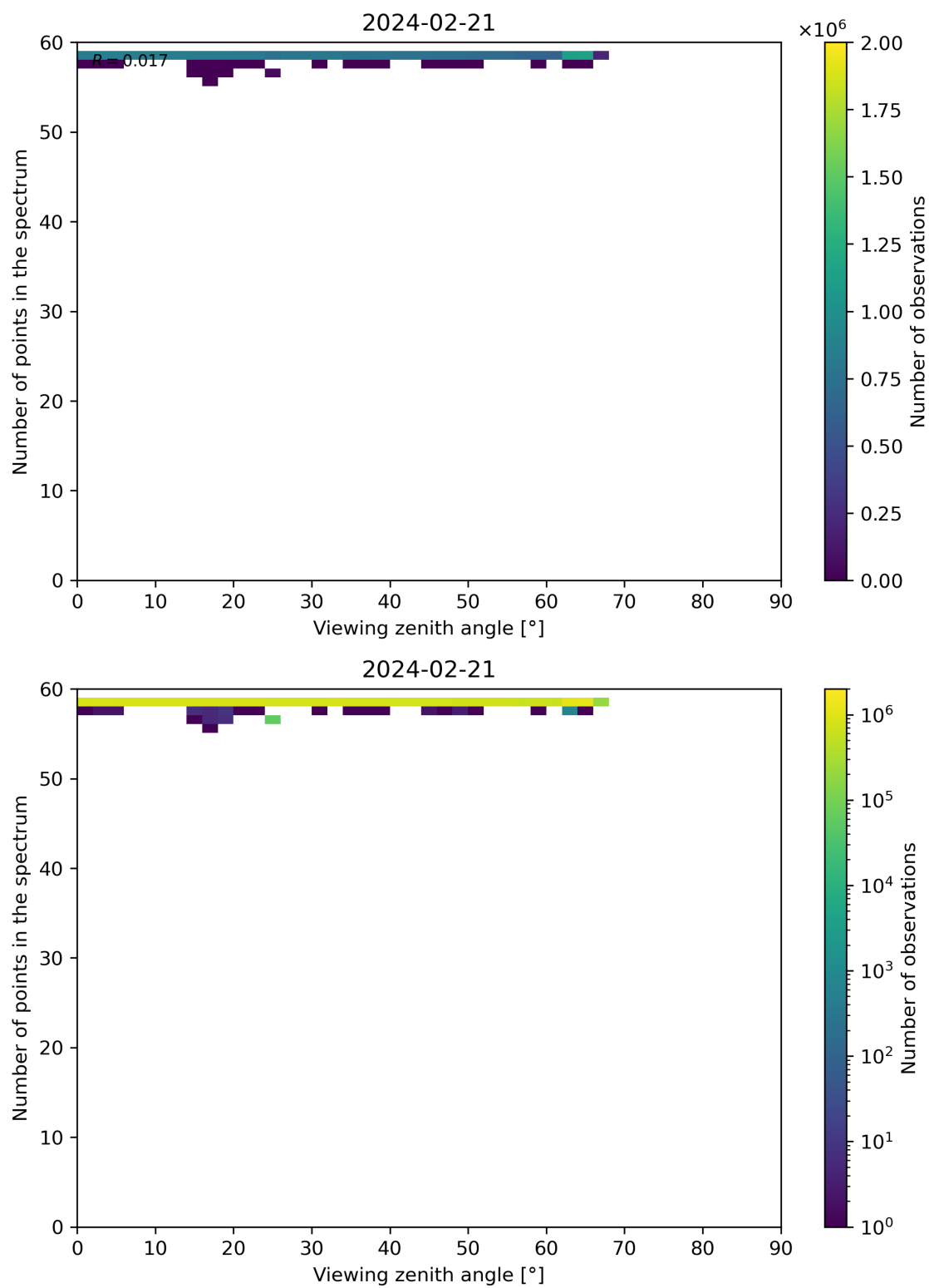
Figure 125: Scatter density plot of “Viewing zenith angle” against “Number of points in the spectrum” for 2024-02-20 to 2024-02-22.
