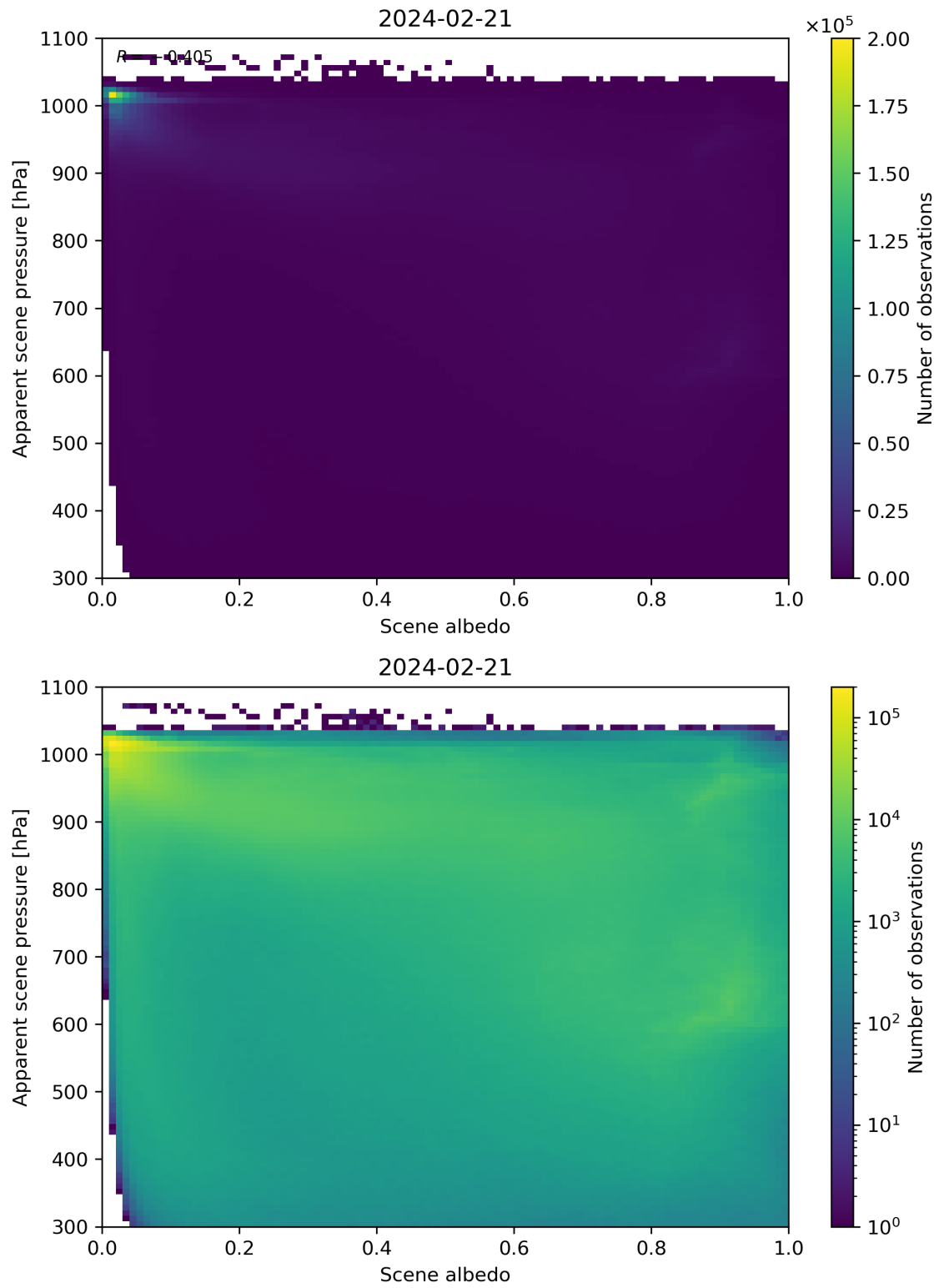
Figure 102: Scatter density plot of “Scene albedo” against “Apparent scene pressure” for 2024-02-20 to 2024-02-22.
