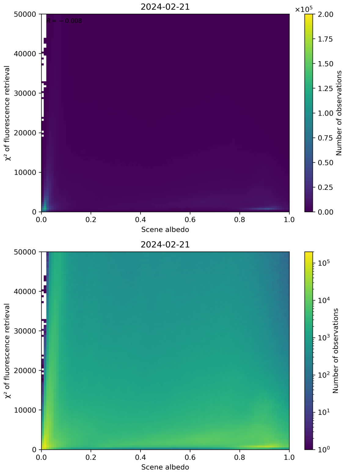
Figure 103: Scatter density plot of “Scene albedo” against “ \chi^2 of fluorescence retrieval” for 2024-02-20 to 2024-02-22.
