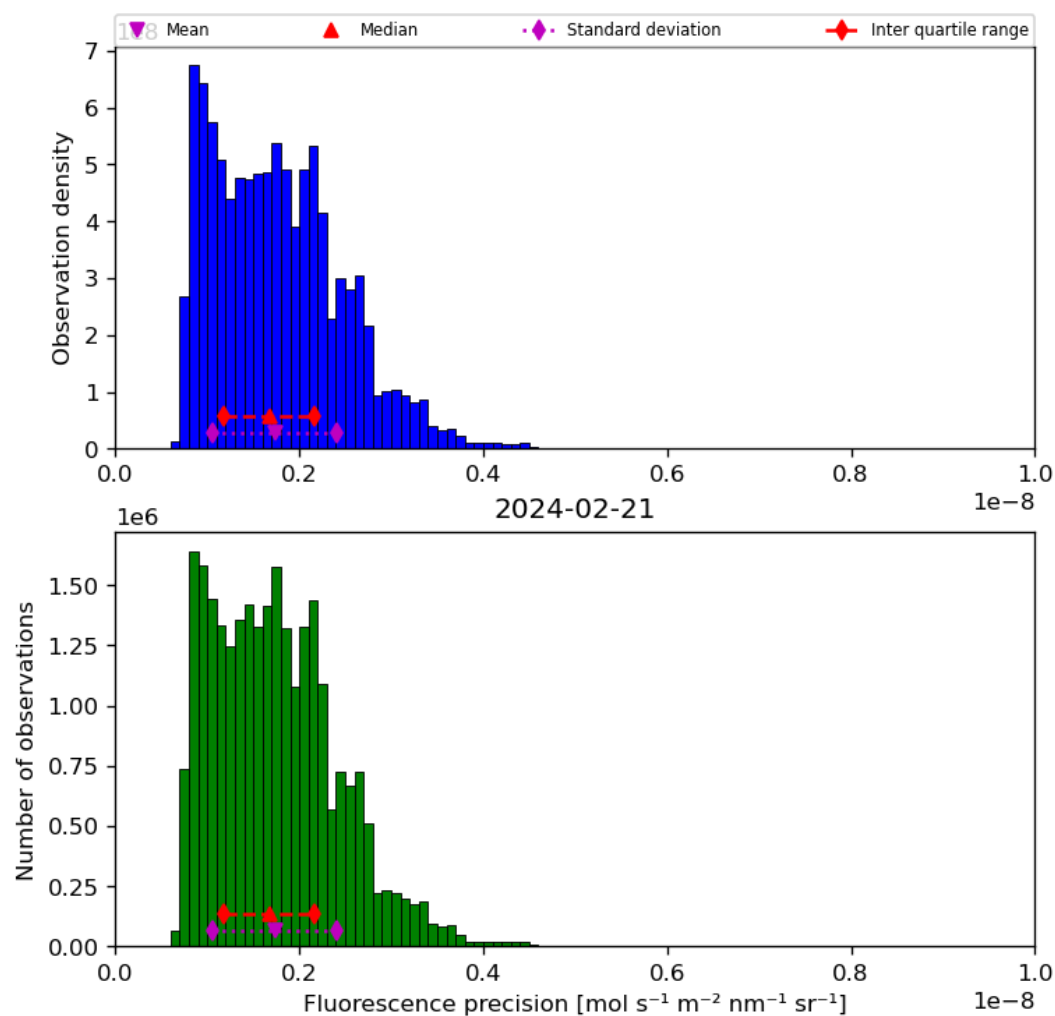
Figure 41: Histogram of “Fluorescence precision” for 2024-02-20 to 2024-02-22
