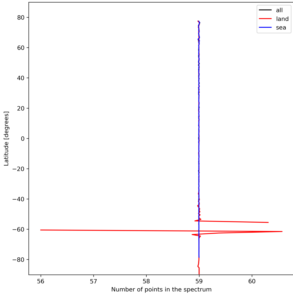
Figure 27: Zonal average of “Number of points in the spectrum” for 2024-02-20 to 2024-02-22.
