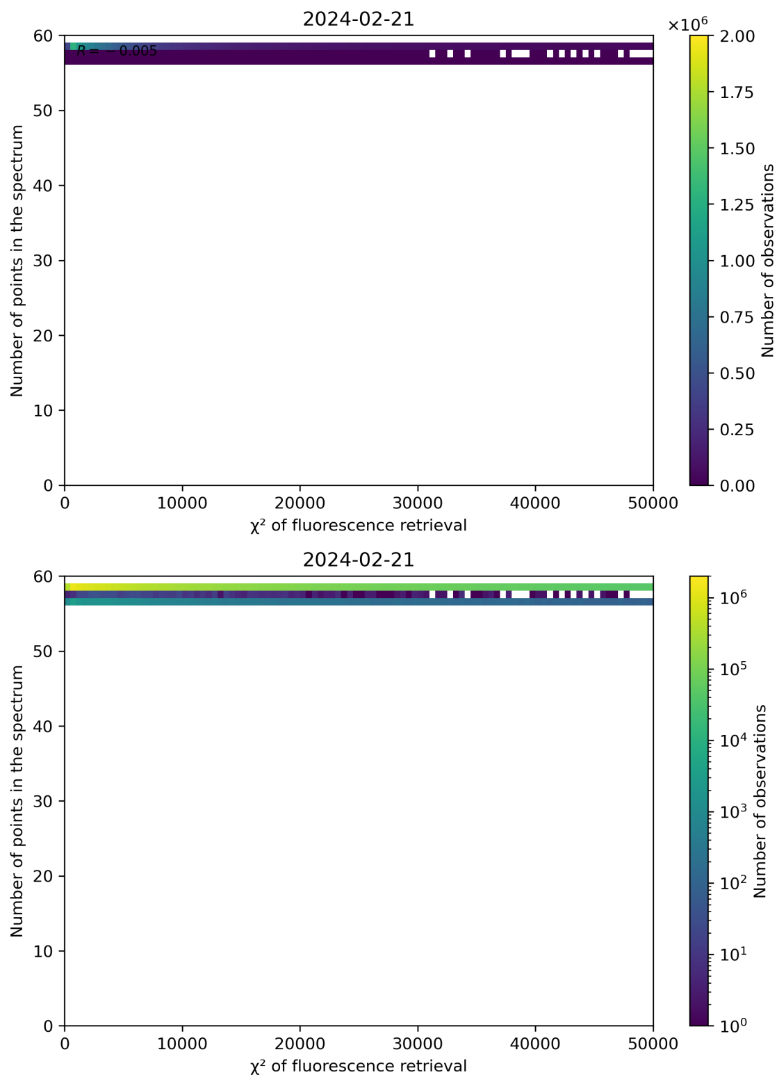
Figure 68: Scatter density plot of " \chi^2 of fluorescence retrieval" against "Number of points in the spectrum" for 2024-02-20 to 2024-02-22.
