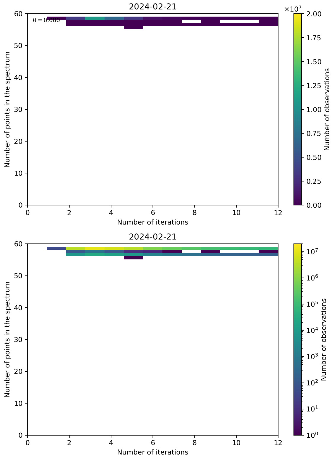
Figure 99: Scatter density plot of “Number of iterations” against “Number of points in the spectrum” for 2024-02-20 to 2024-02-22.
