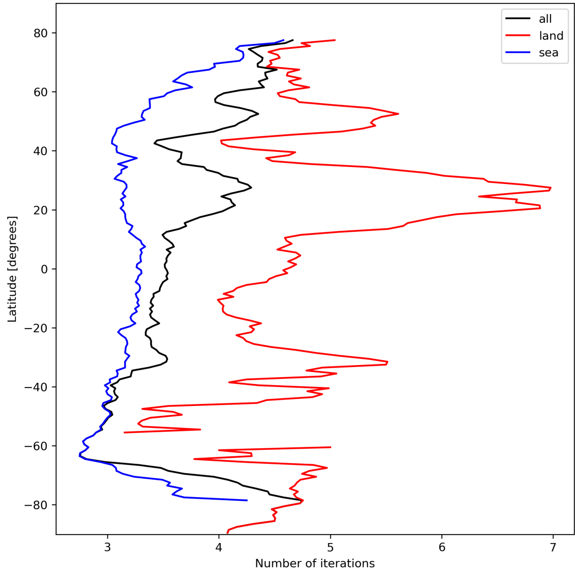
Figure 22: Zonal average of “Number of iterations” for 2024-02-20 to 2024-02-22.
