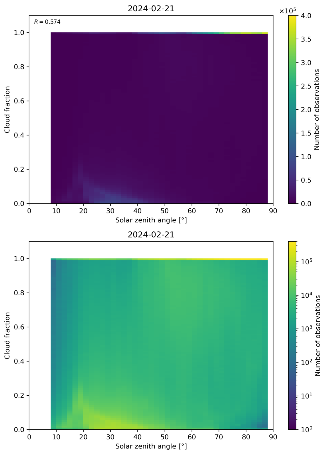
Figure 110: Scatter density plot of “Solar zenith angle” against “Cloud fraction” for 2024-02-20 to 2024-02-22.
