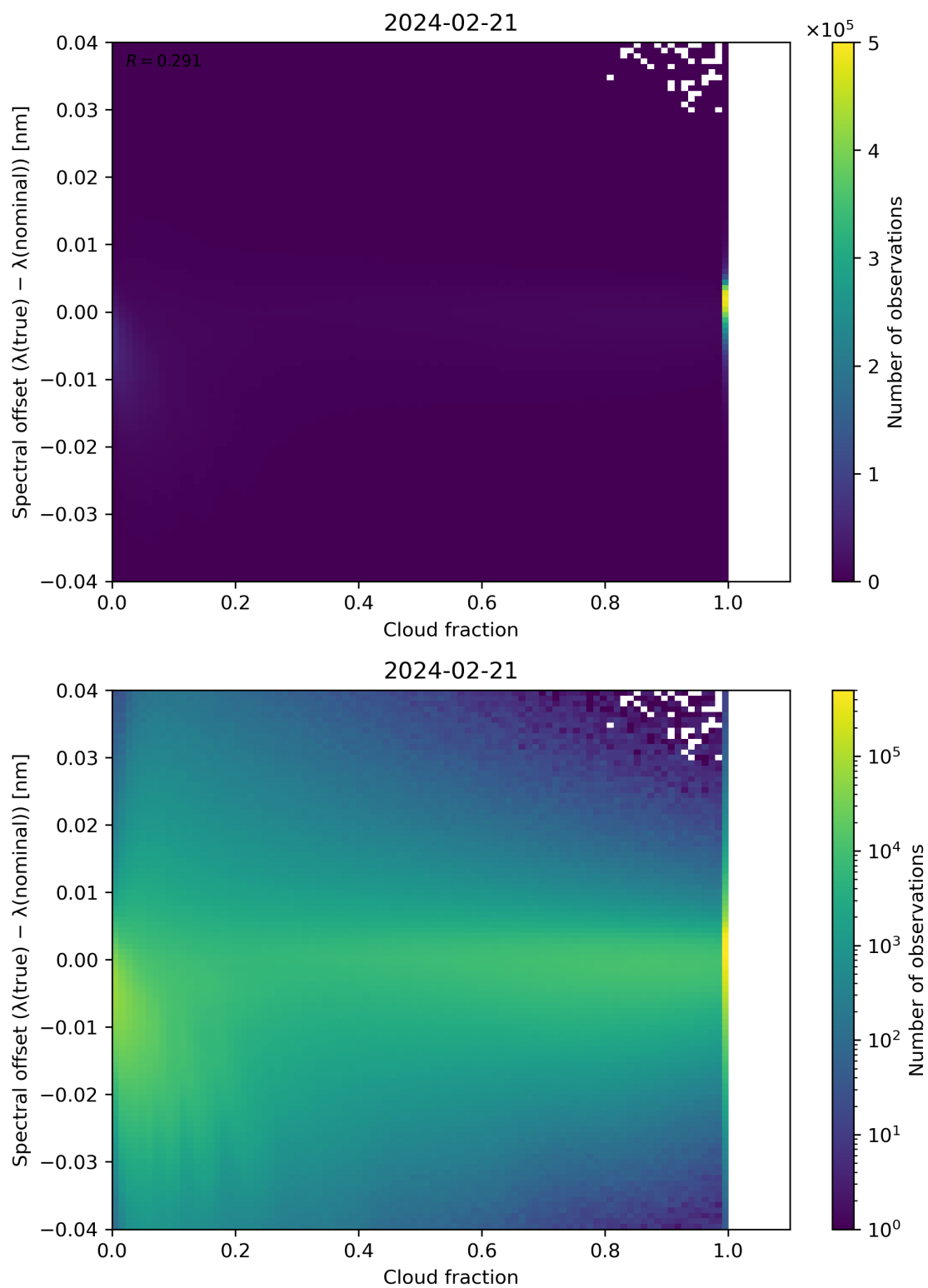
Figure 76: Scatter density plot of “Cloud fraction” against “Spectral offset ( \lambda(\text{true}) - \lambda(\text{nominal}) )” for 2024-02-20 to 2024-02-22.
