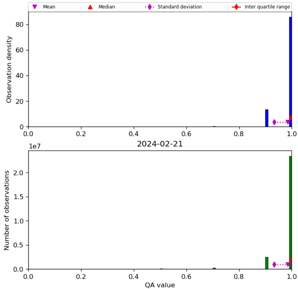
Figure 29: Histogram of “QA value” for 2024-02-20 to 2024-02-22
