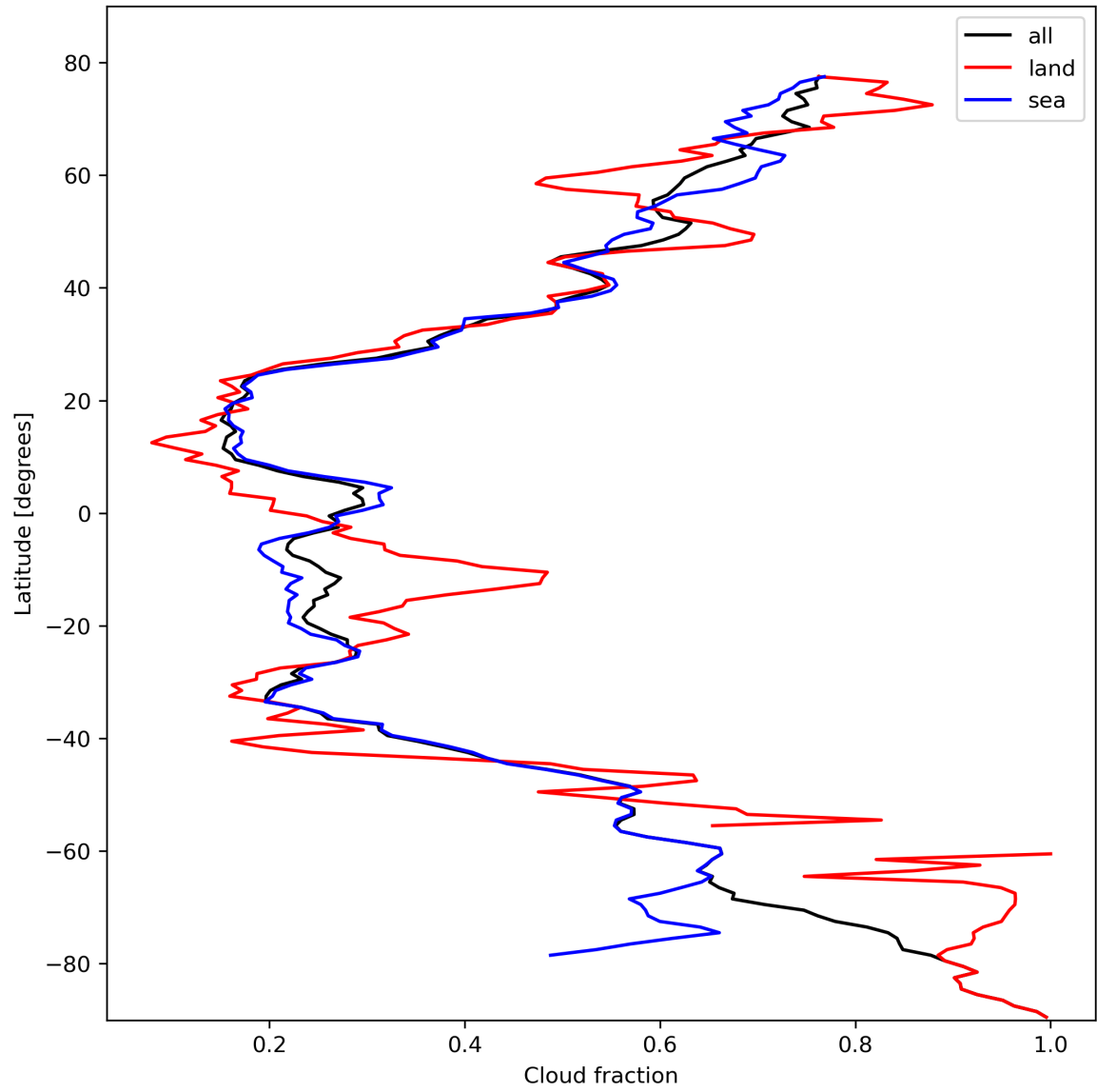
Figure 15: Zonal average of “Cloud fraction” for 2024-02-20 to 2024-02-22.
