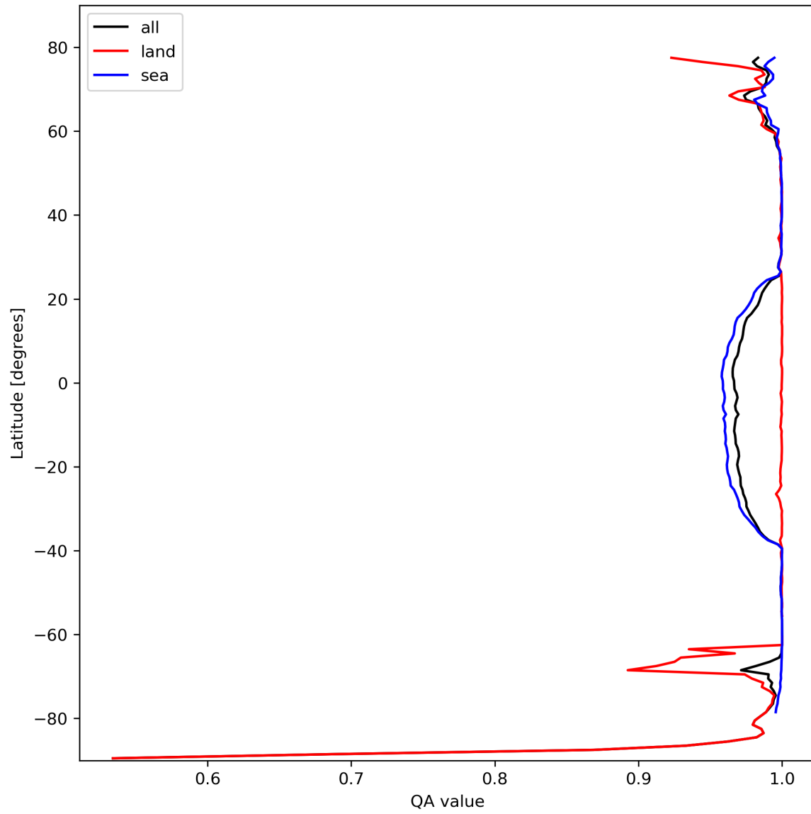
Figure 12: Zonal average of “QA value” for 2024-02-20 to 2024-02-22.
