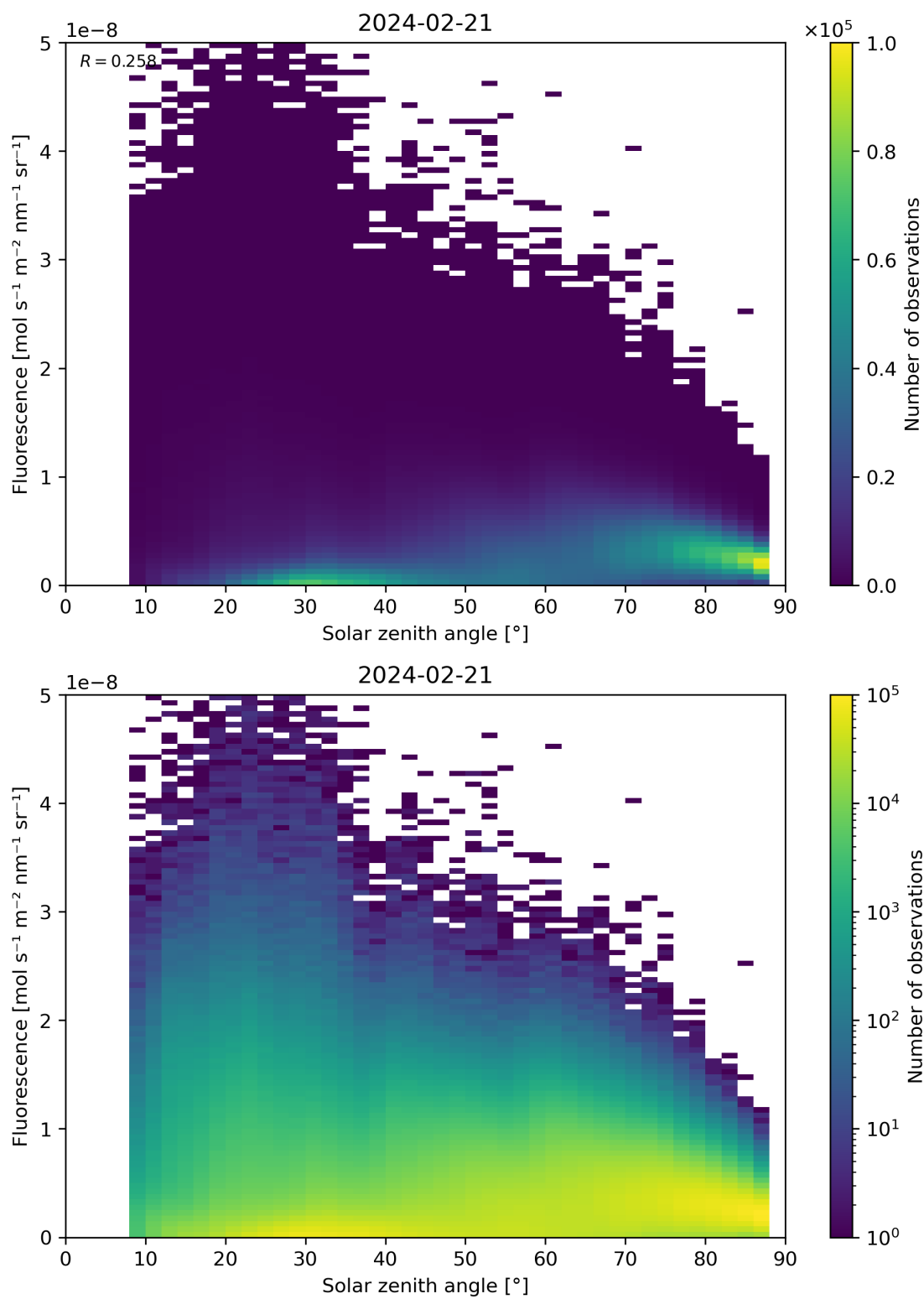
Figure 112: Scatter density plot of “Solar zenith angle” against “Fluorescence” for 2024-02-20 to 2024-02-22.
