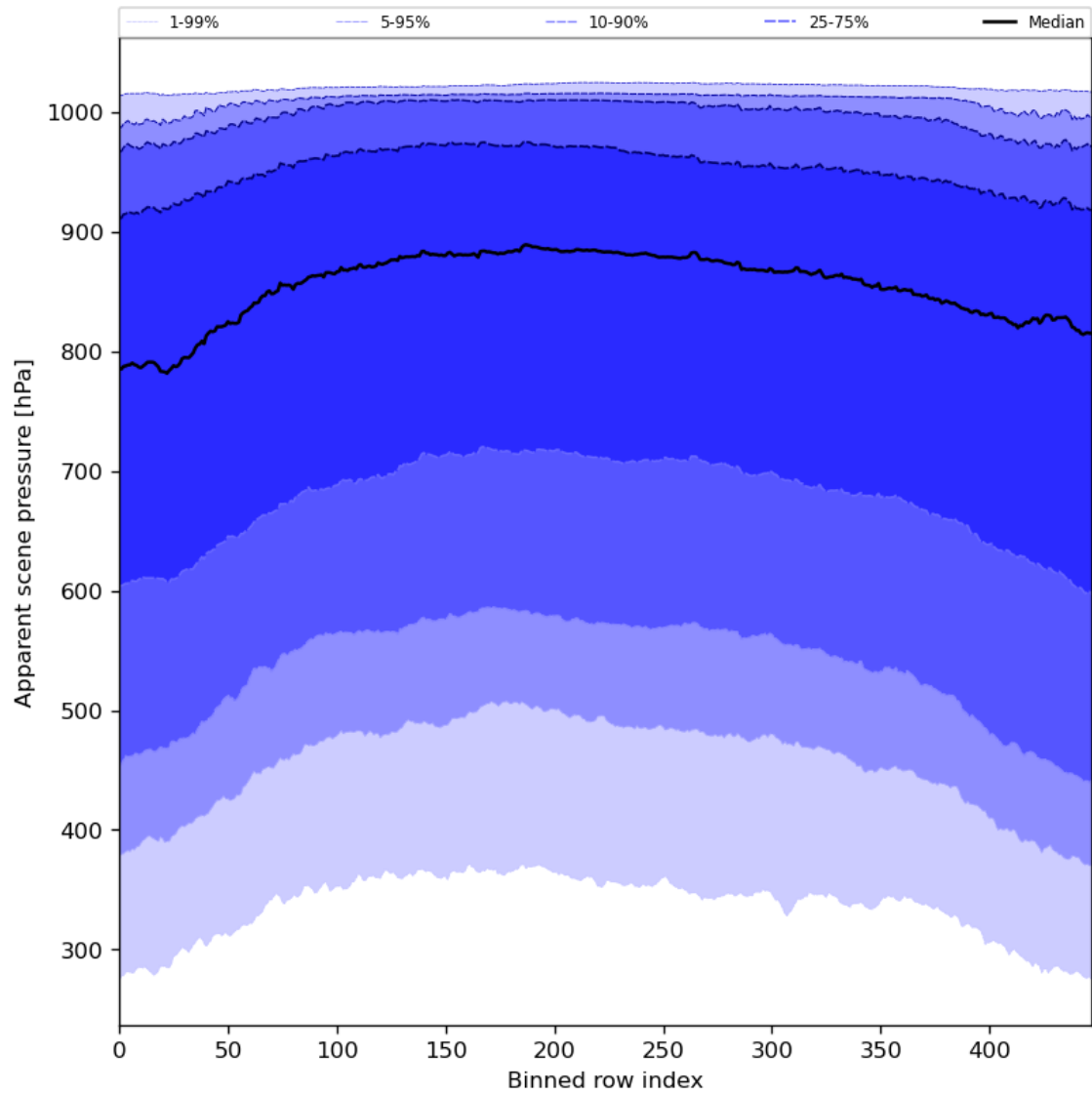
Figure 53: Along track statistics of “Apparent scene pressure” for 2024-02-20 to 2024-02-22
