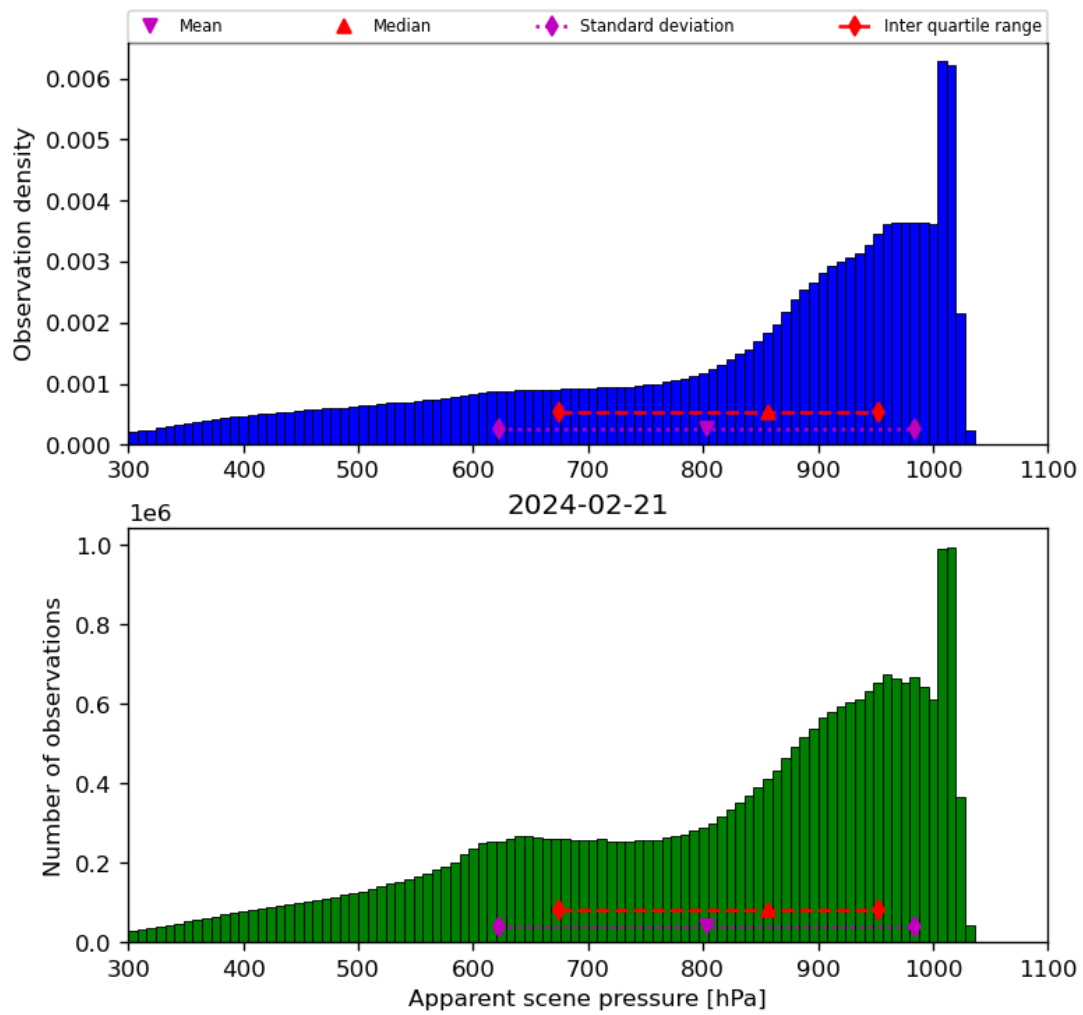
Figure 36: Histogram of “Apparent scene pressure” for 2024-02-20 to 2024-02-22
