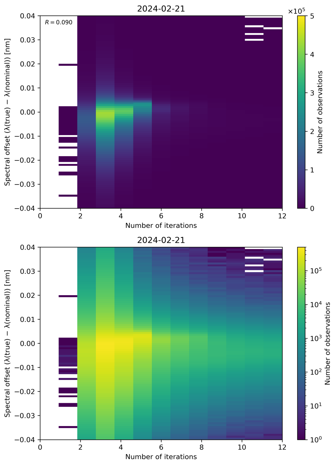
Figure 100: Scatter density plot of “Number of iterations” against “Spectral offset ( \lambda(\text{true}) - \lambda(\text{nominal}) )” for 2024-02-20 to 2024-02-22.
