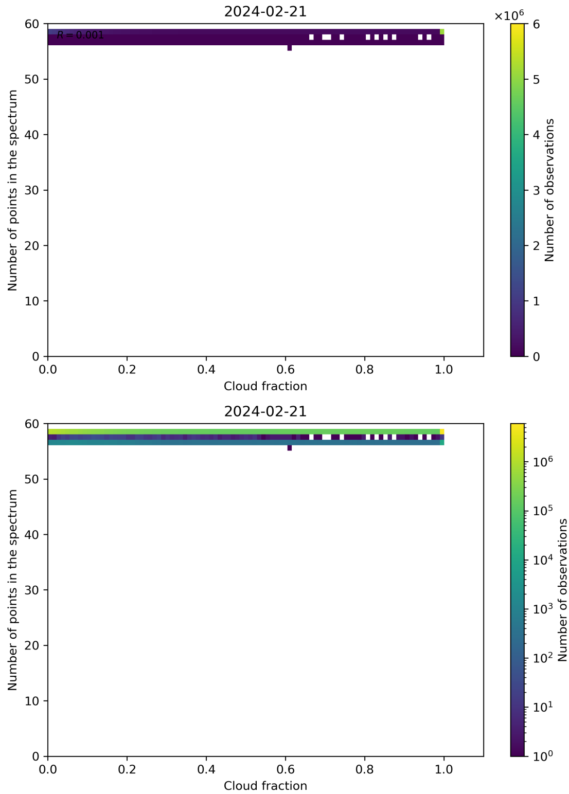
Figure 74: Scatter density plot of “Cloud fraction” against “Number of points in the spectrum” for 2024-02-20 to 2024-02-22.
