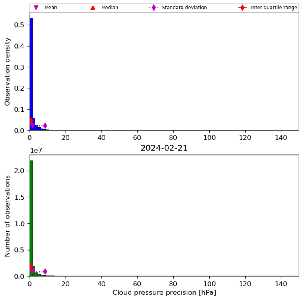
Figure 31: Histogram of “Cloud pressure precision” for 2024-02-20 to 2024-02-22
