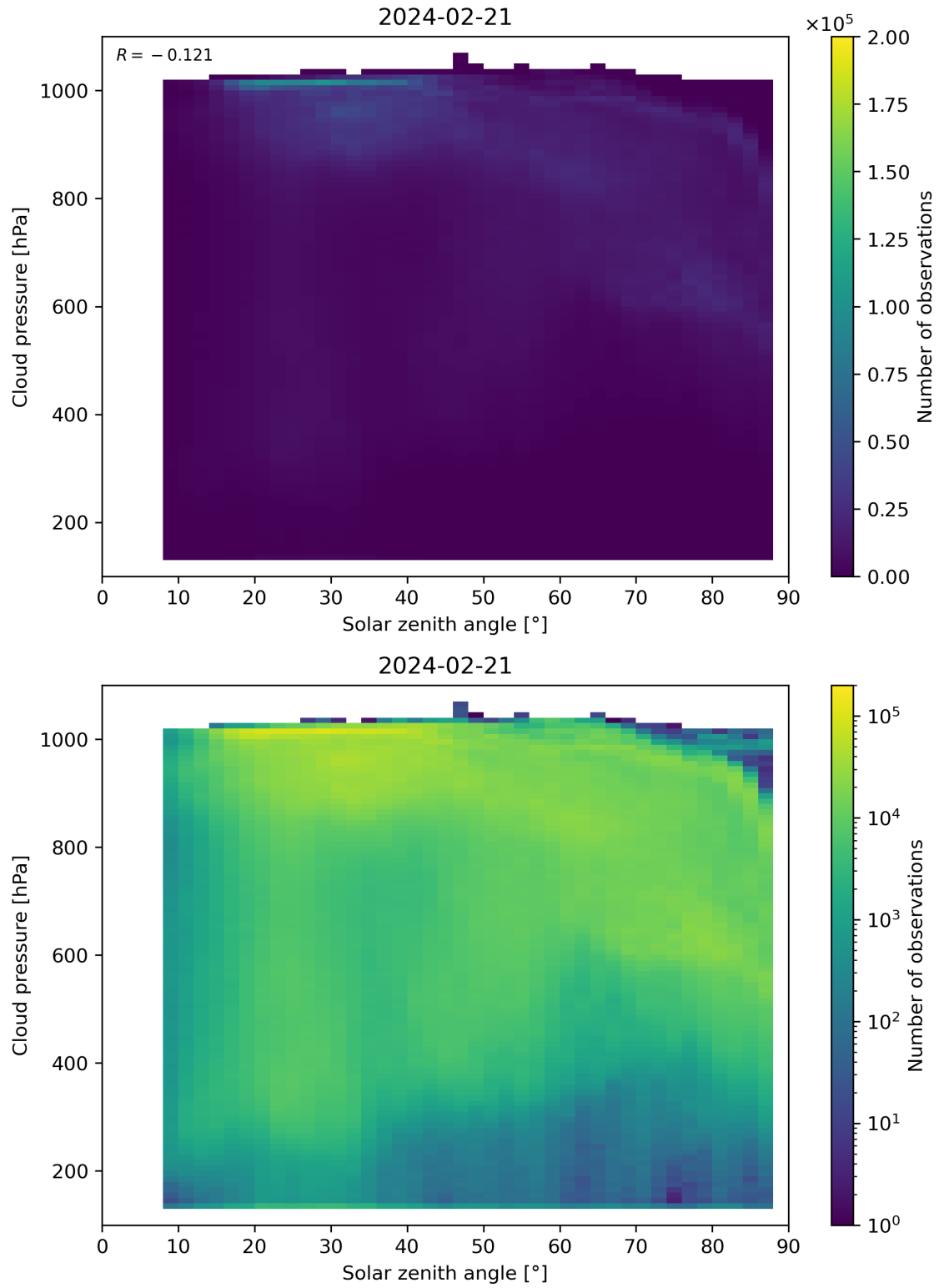
Figure 111: Scatter density plot of “Solar zenith angle” against “Cloud pressure” for 2024-02-20 to 2024-02-22.
