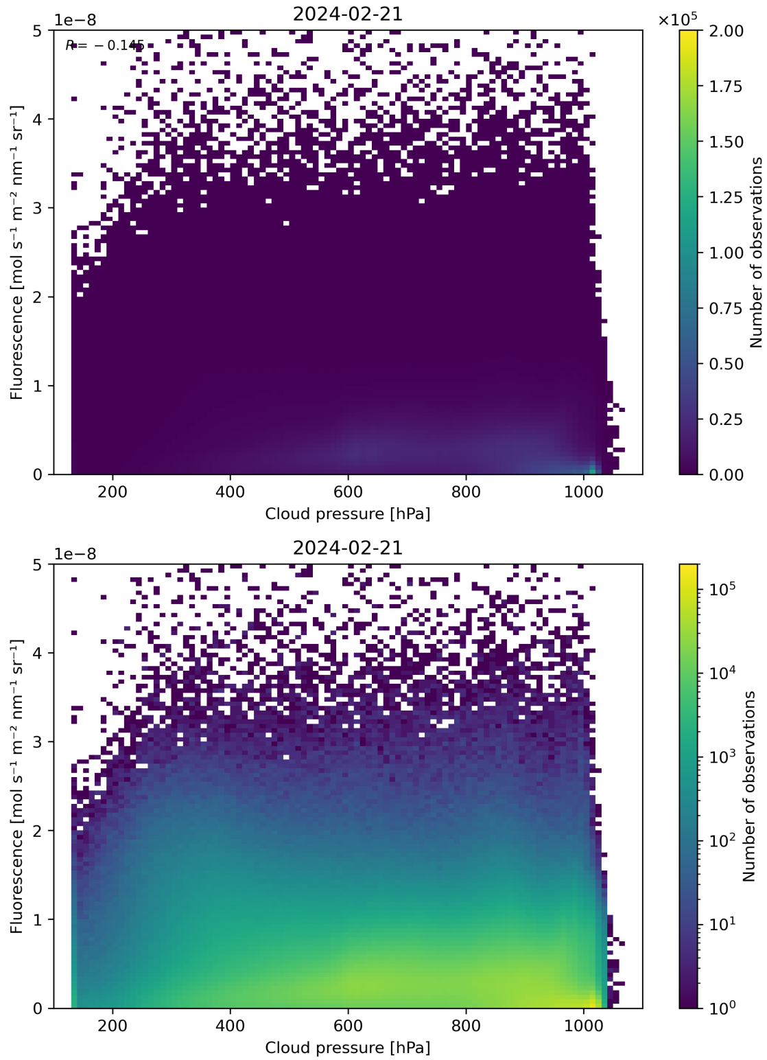
Figure 80: Scatter density plot of “Cloud pressure” against “Fluorescence” for 2024-02-20 to 2024-02-22.
