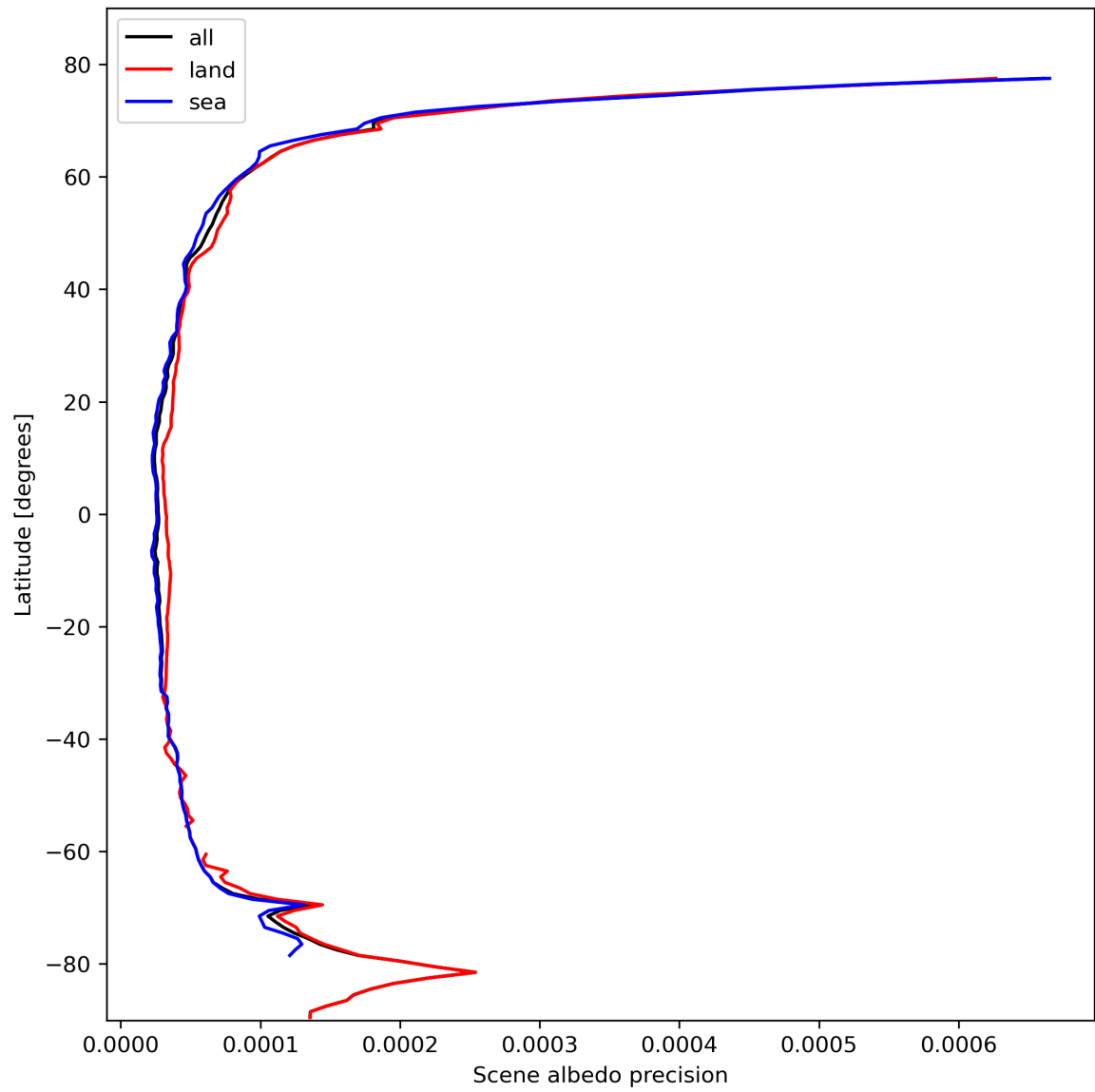
Figure 18: Zonal average of “Scene albedo precision” for 2024-02-20 to 2024-02-22.
