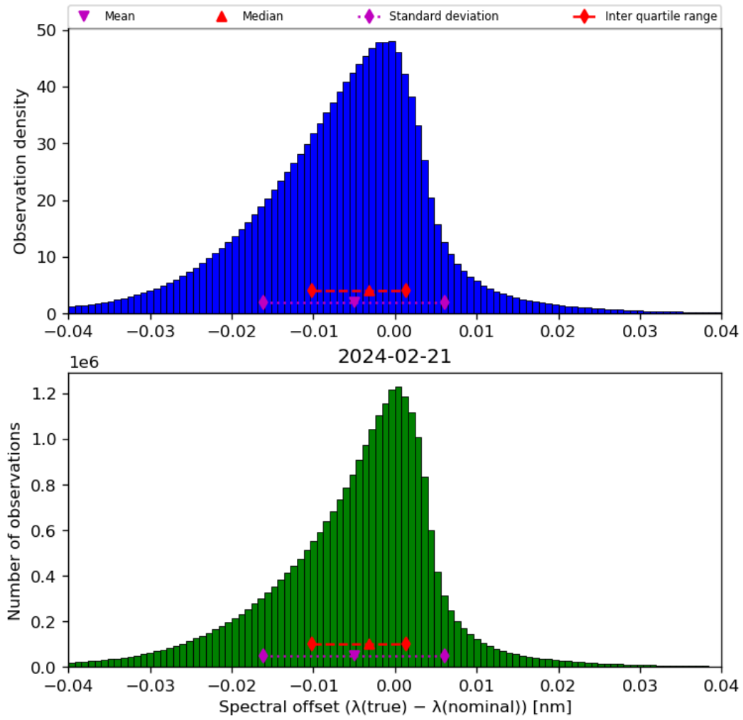
Figure 45: Histogram of “Spectral offset ( \lambda(\text{true}) - \lambda(\text{nominal}) )” for 2024-02-20 to 2024-02-22
