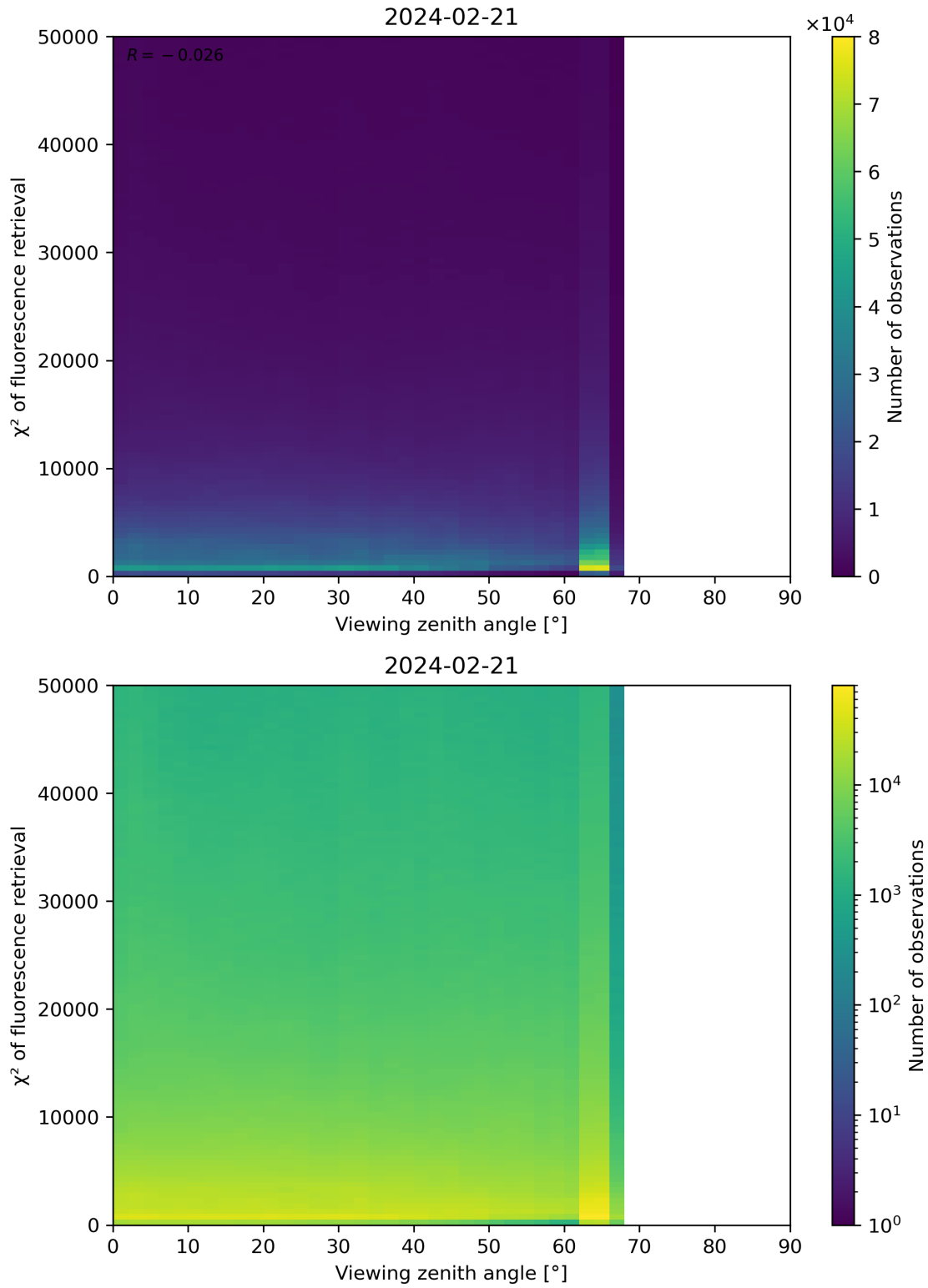
Figure 119: Scatter density plot of “Viewing zenith angle” against “ \chi^2 of fluorescence retrieval” for 2024-02-20 to 2024-02-22.
