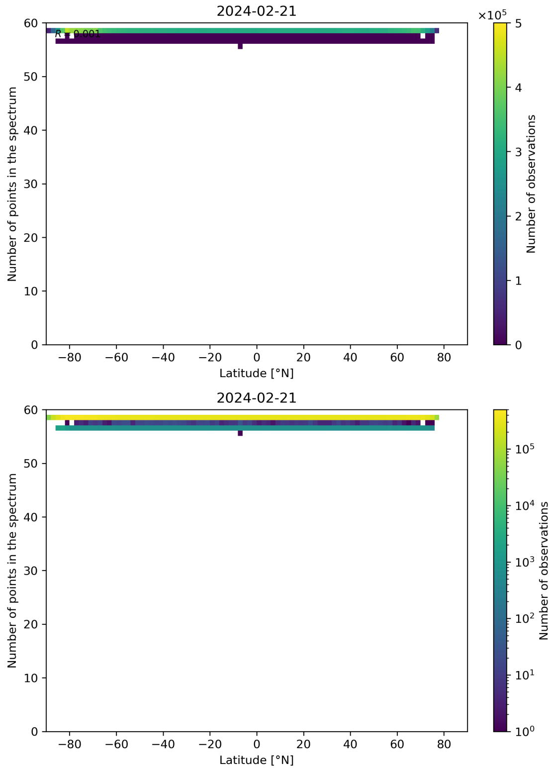
Figure 94: Scatter density plot of “Latitude” against “Number of points in the spectrum” for 2024-02-20 to 2024-02-22.
