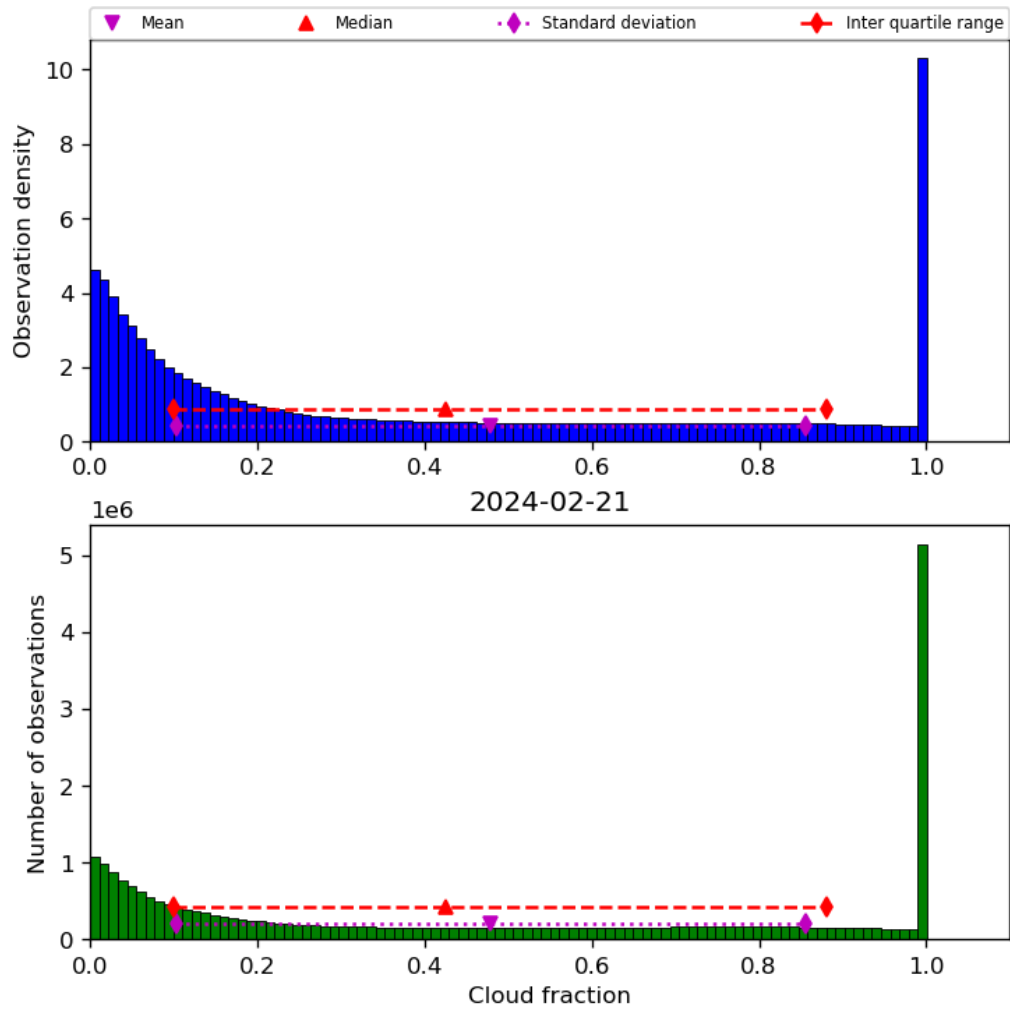
Figure 32: Histogram of “Cloud fraction” for 2024-02-20 to 2024-02-22
