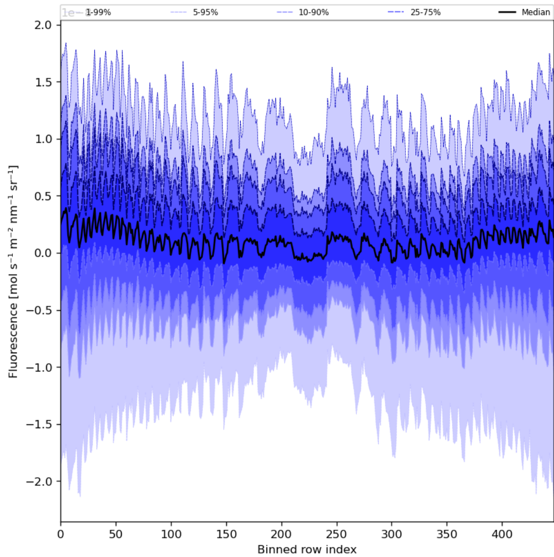
Figure 57: Along track statistics of “Fluorescence” for 2024-02-20 to 2024-02-22
