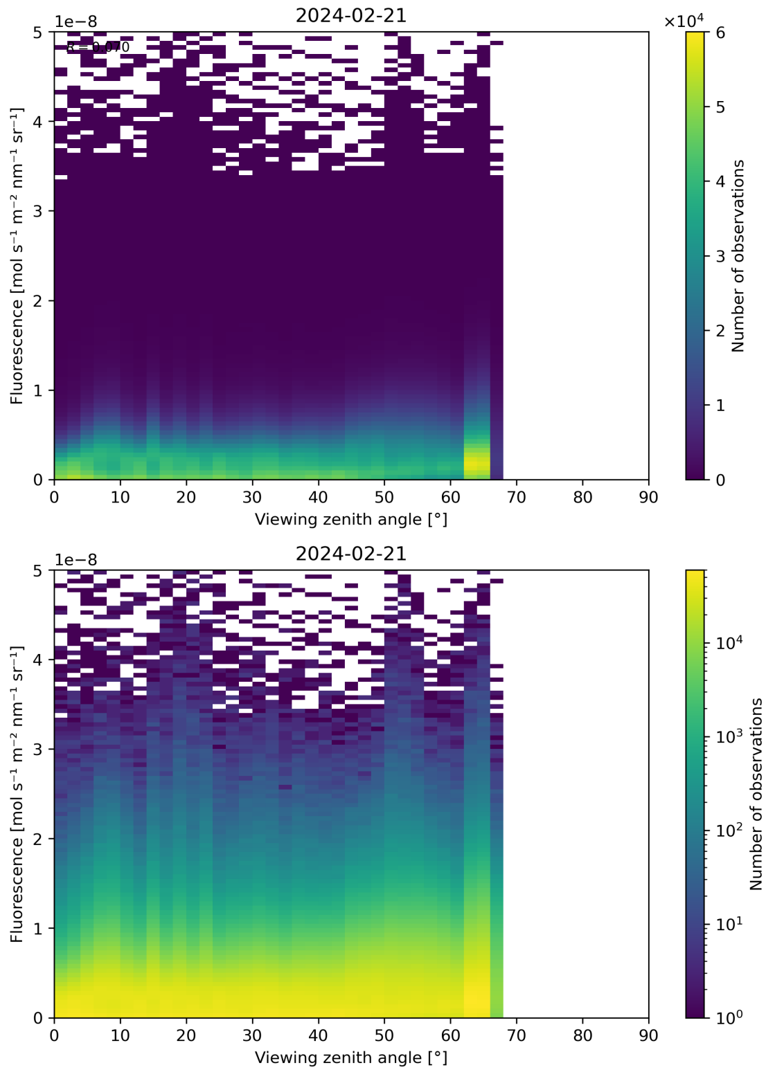
Figure 122: Scatter density plot of “Viewing zenith angle” against “Fluorescence” for 2024-02-20 to 2024-02-22.
