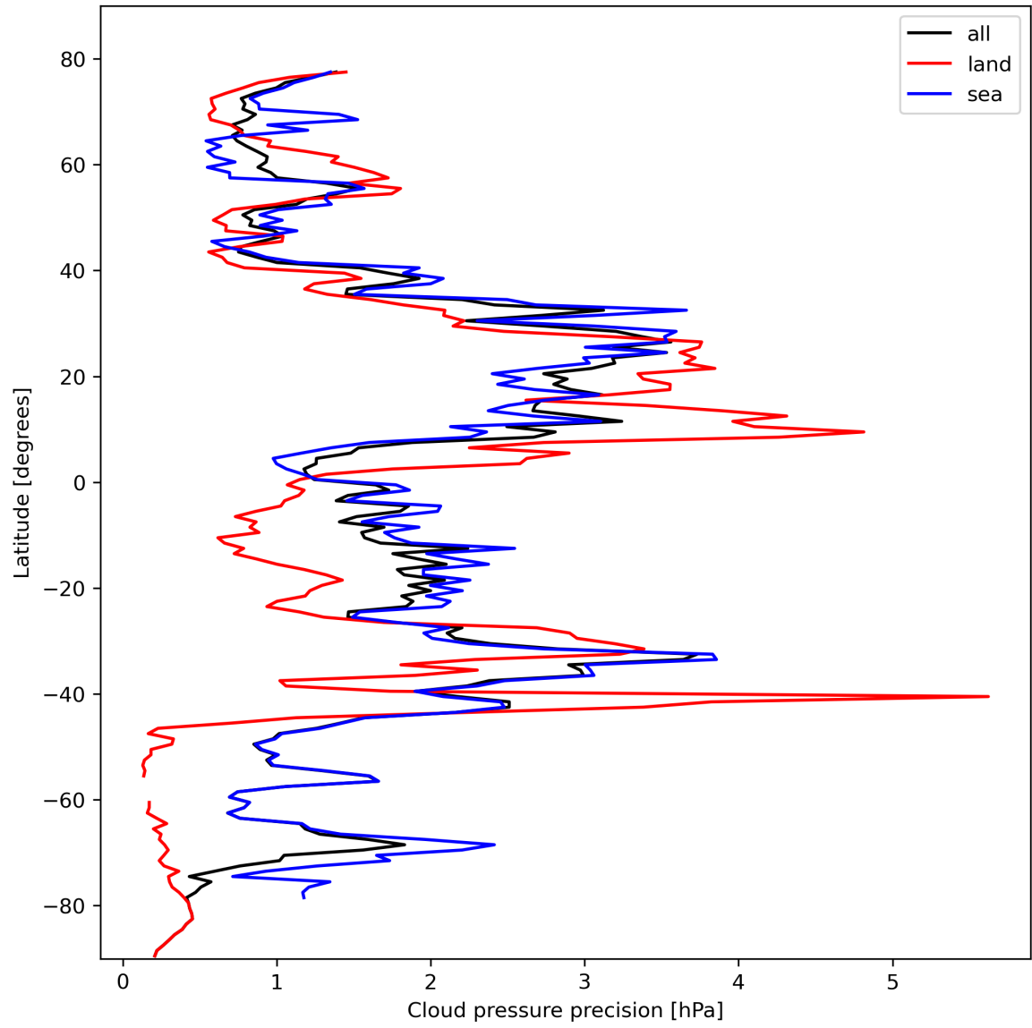
Figure 14: Zonal average of “Cloud pressure precision” for 2024-02-20 to 2024-02-22.
