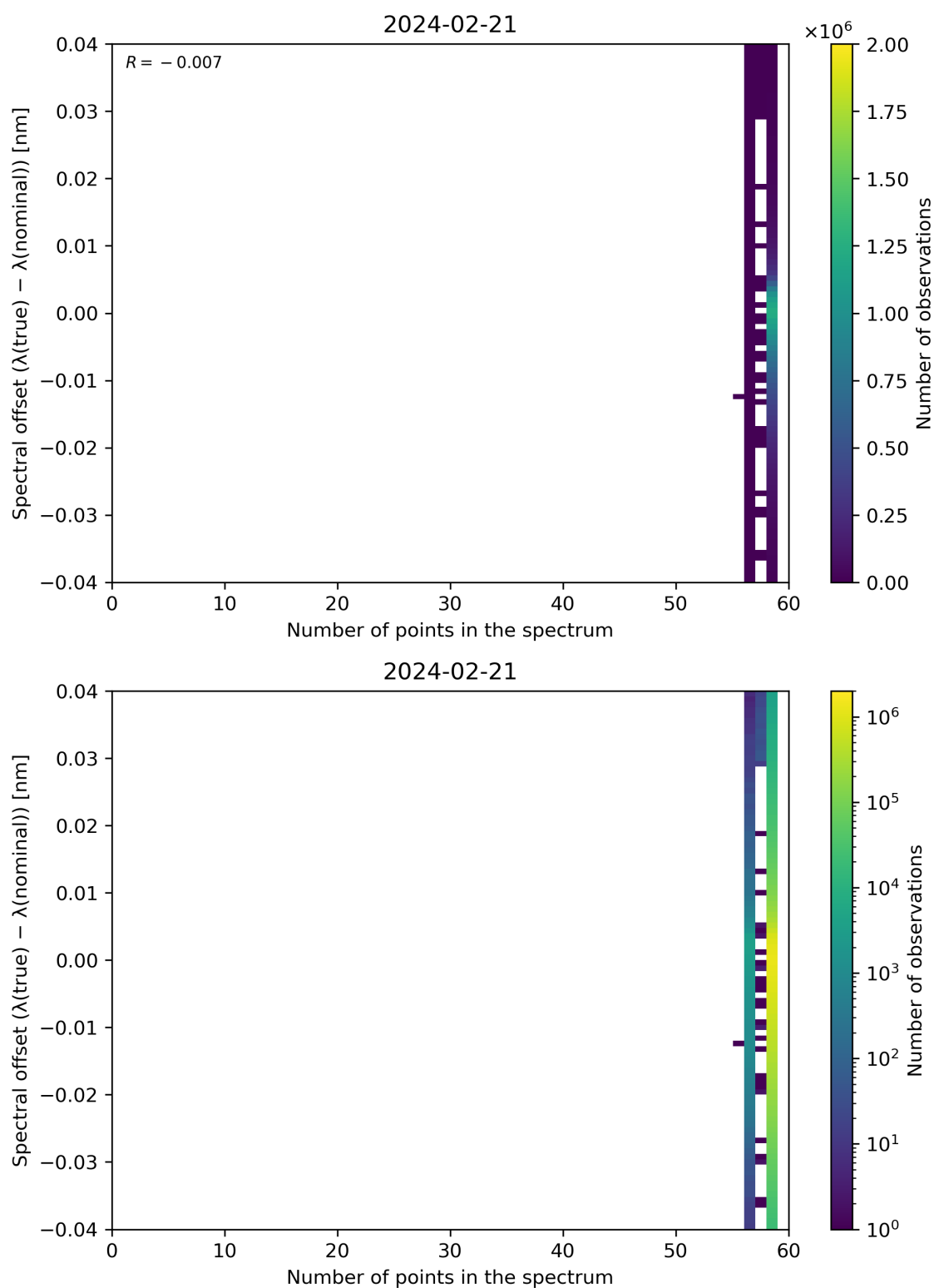
Figure 101: Scatter density plot of “Number of points in the spectrum” against “Spectral offset ( \lambda(\text{true}) - \lambda(\text{nominal}) )” for 2024-02-20 to 2024-02-22.
