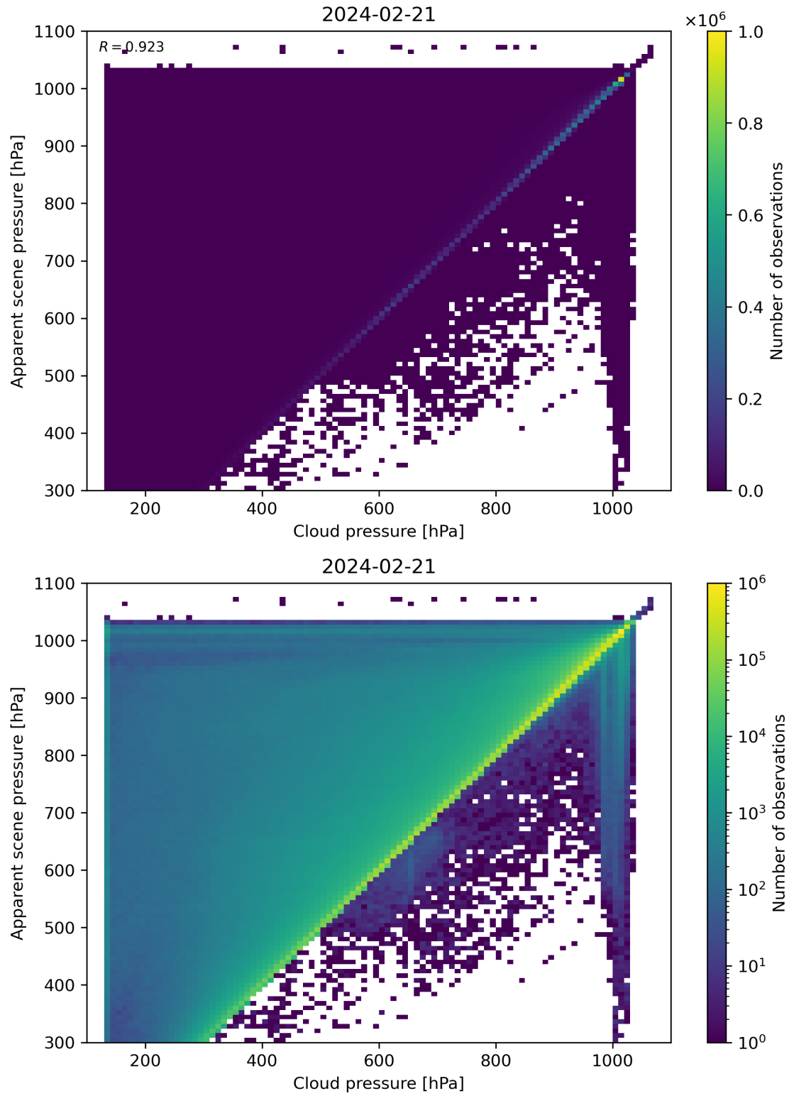
Figure 77: Scatter density plot of “Cloud pressure” against “Apparent scene pressure” for 2024-02-20 to 2024-02-22.
