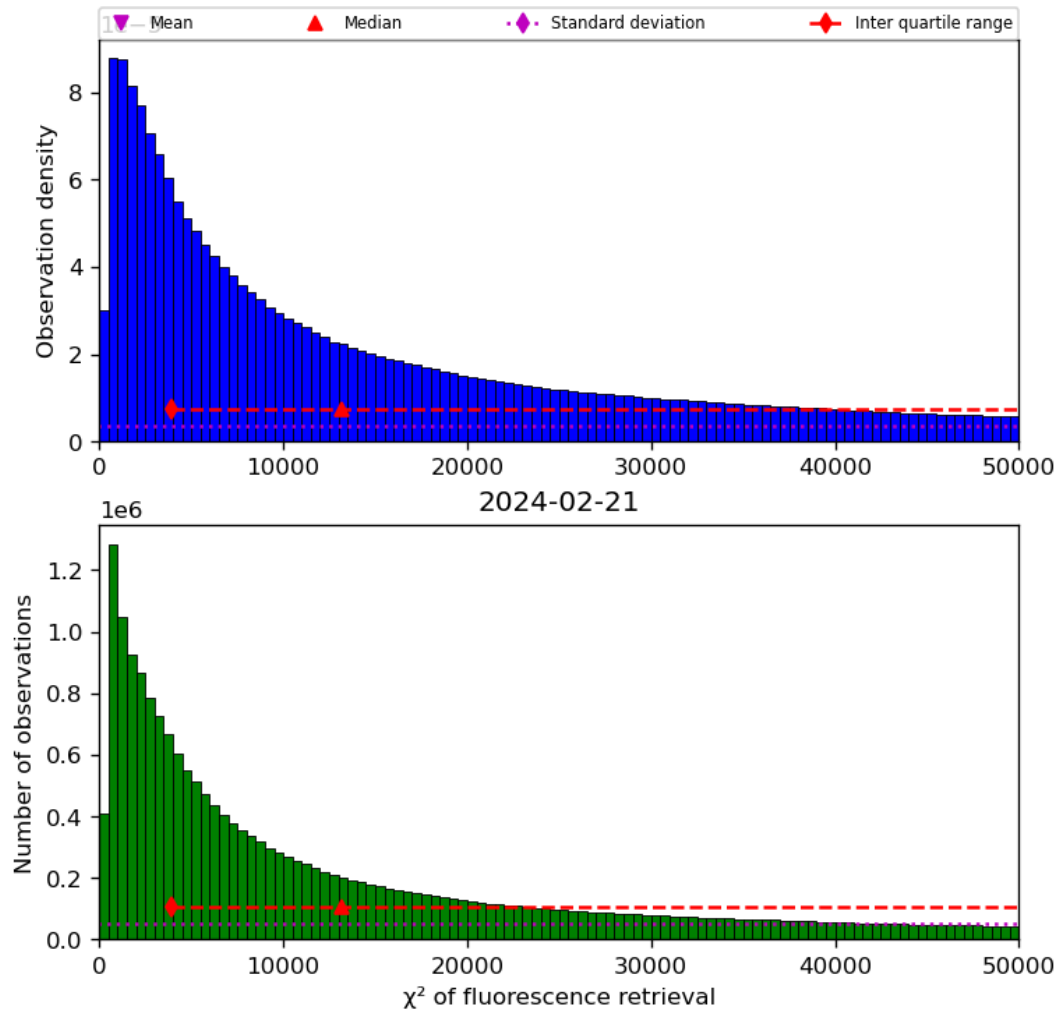
Figure 42: Histogram of “ \chi^2 of fluorescence retrieval” for 2024-02-20 to 2024-02-22
