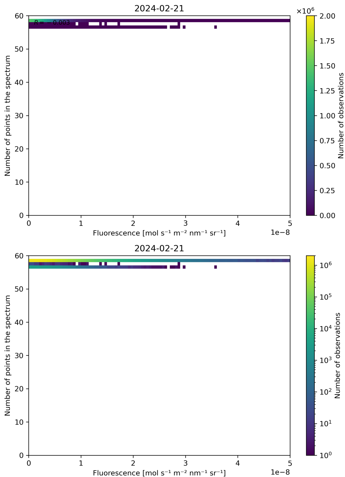
Figure 86: Scatter density plot of “Fluorescence” against “Number of points in the spectrum” for 2024-02-20 to 2024-02-22.
