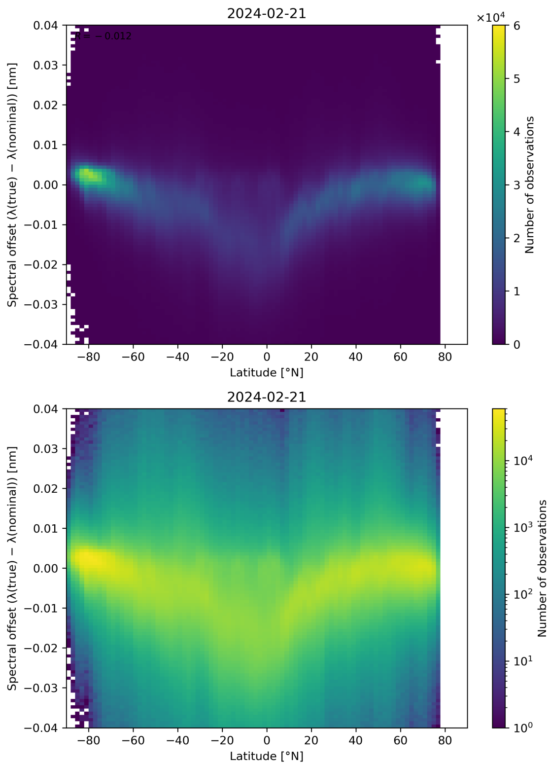
Figure 96: Scatter density plot of “Latitude” against “Spectral offset ( \lambda(\text{true}) - \lambda(\text{nominal}) )” for 2024-02-20 to 2024-02-22.
