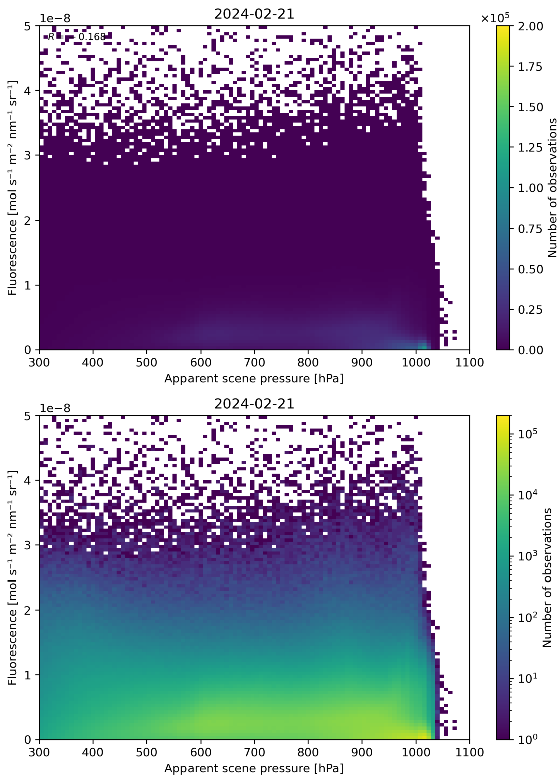
Figure 64: Scatter density plot of “Apparent scene pressure” against “Fluorescence” for 2024-02-20 to 2024-02-22.
