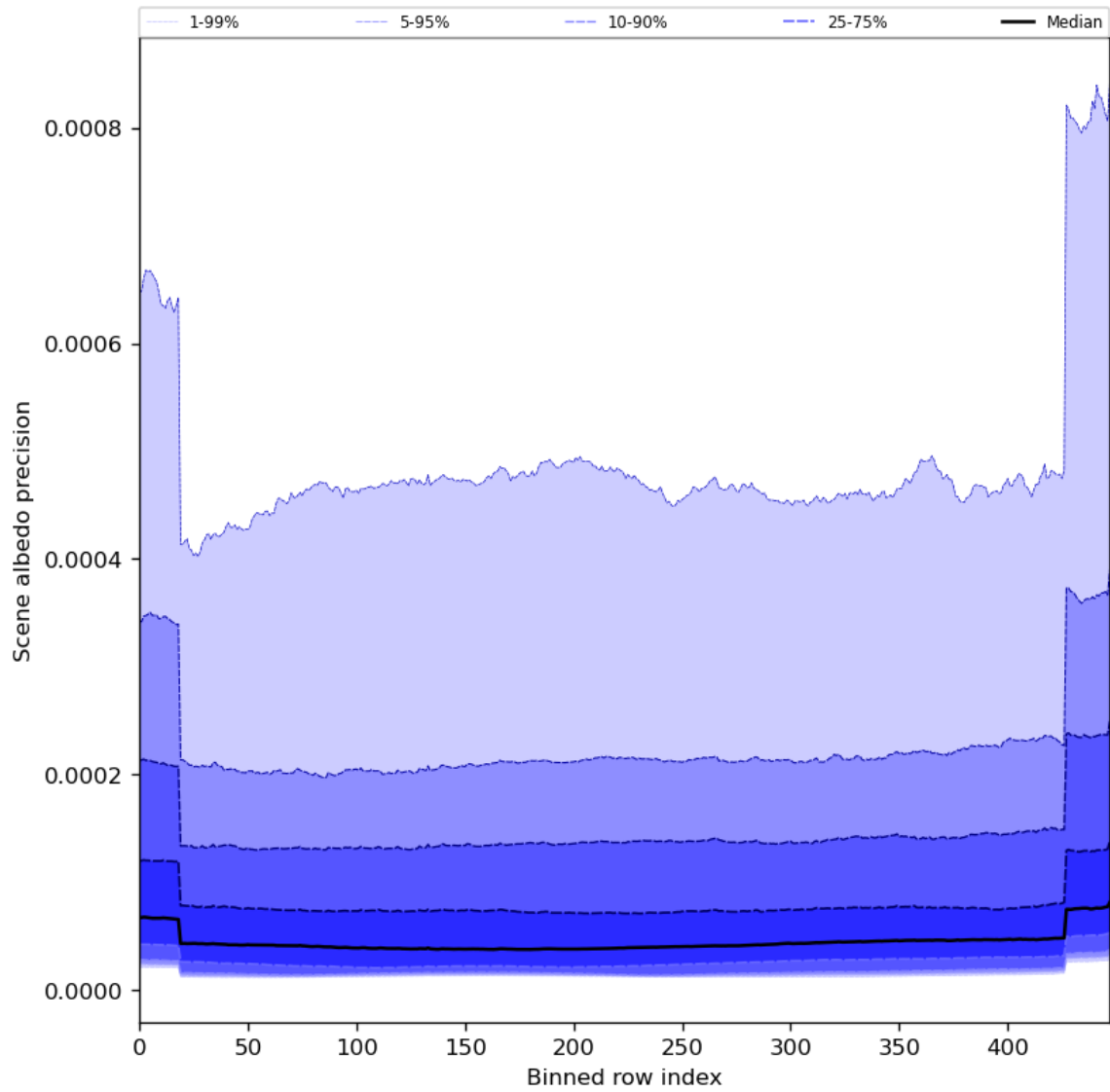
Figure 52: Along track statistics of “Scene albedo precision” for 2024-02-20 to 2024-02-22
