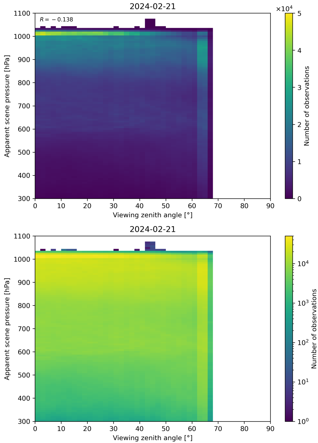
Figure 118: Scatter density plot of “Viewing zenith angle” against “Apparent scene pressure” for 2024-02-20 to 2024-02-22.
