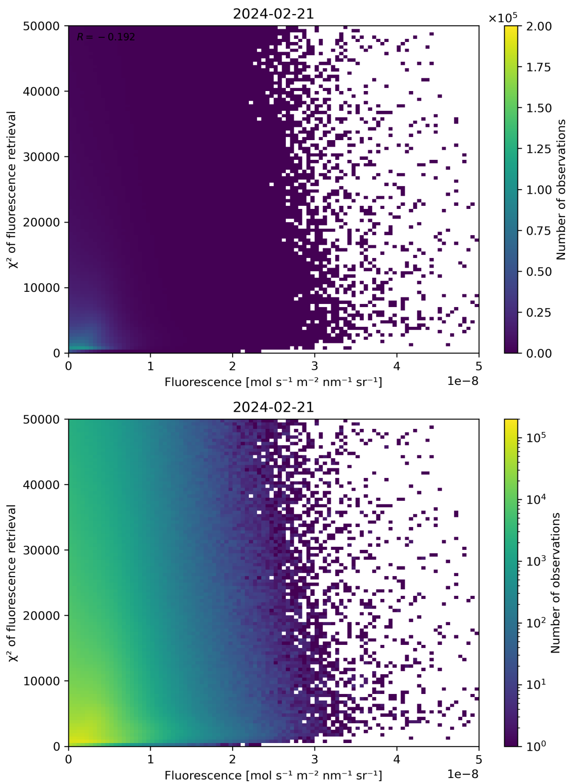
Figure 85: Scatter density plot of “Fluorescence” against “ \chi^2 of fluorescence retrieval” for 2024-02-20 to 2024-02-22.
