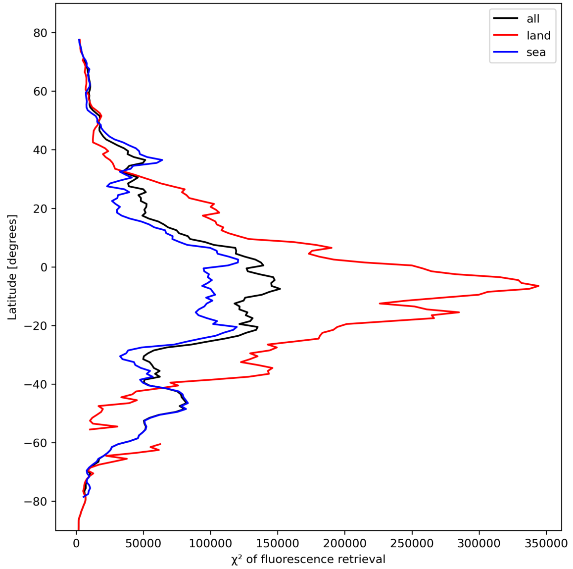
Figure 25: Zonal average of “ \chi^2 of fluorescence retrieval” for 2024-02-20 to 2024-02-22.
