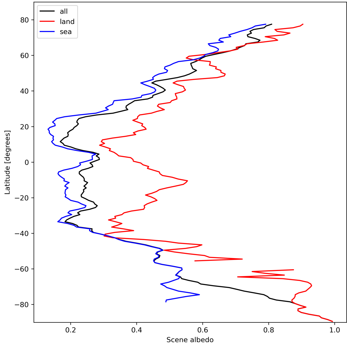
Figure 17: Zonal average of “Scene albedo” for 2024-02-20 to 2024-02-22.
