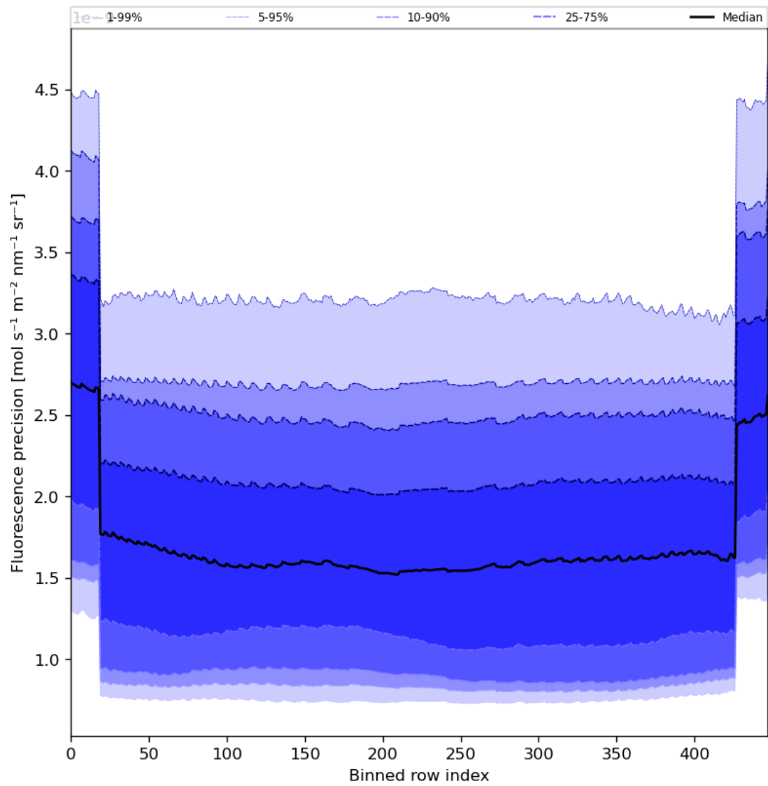
Figure 58: Along track statistics of “Fluorescence precision” for 2024-02-20 to 2024-02-22
