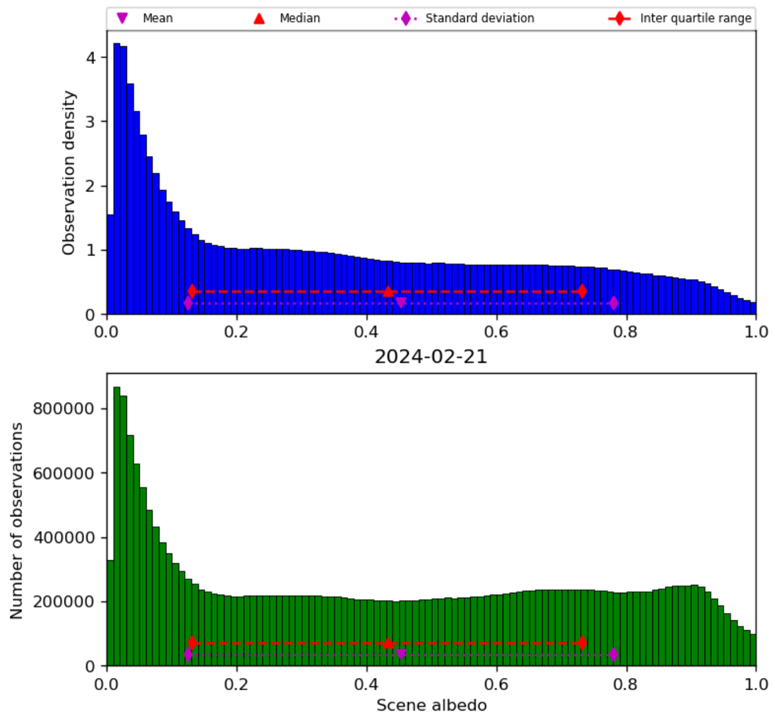
Figure 34: Histogram of “Scene albedo” for 2024-02-20 to 2024-02-22
