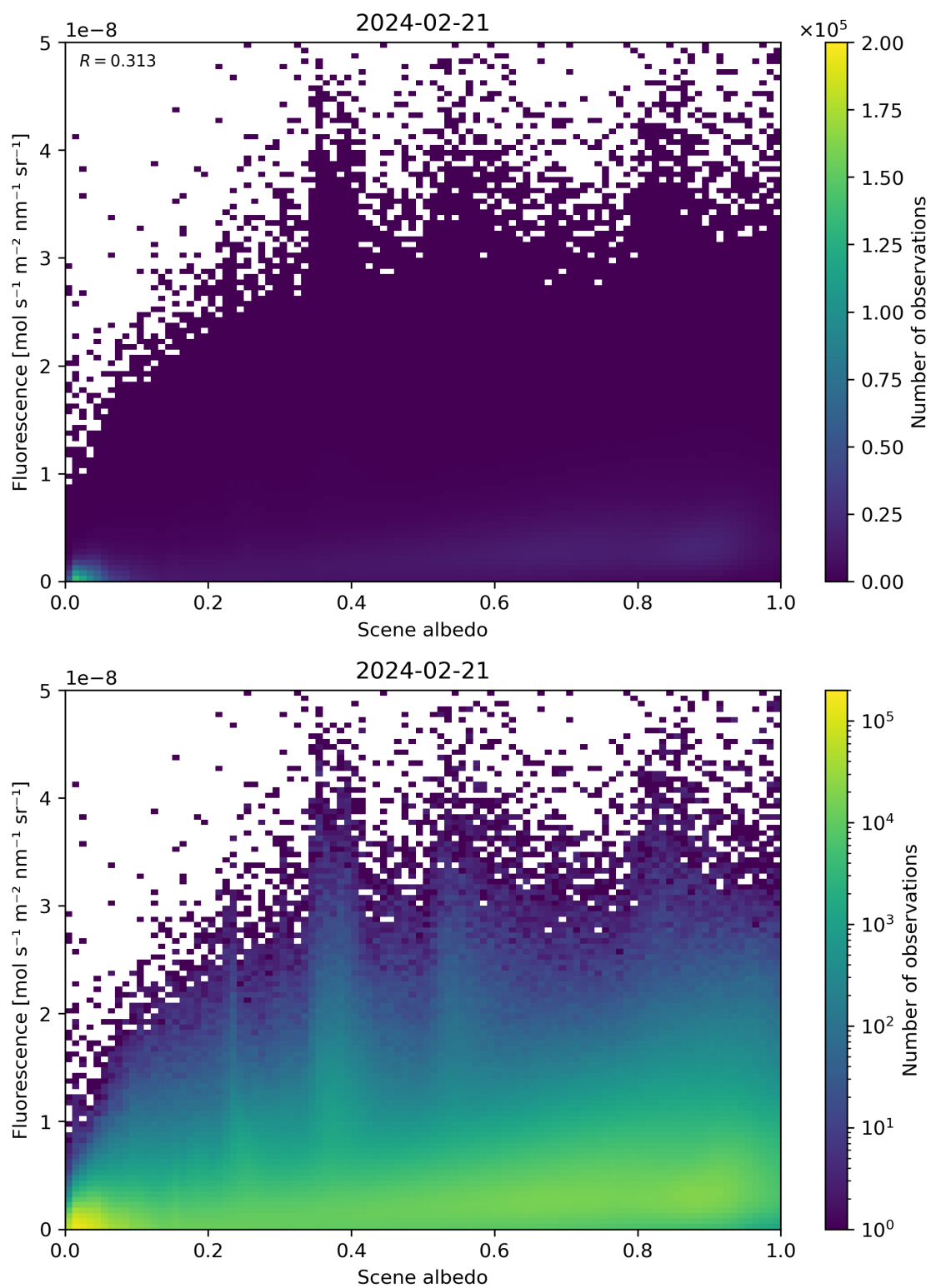
Figure 104: Scatter density plot of “Scene albedo” against “Fluorescence” for 2024-02-20 to 2024-02-22.
