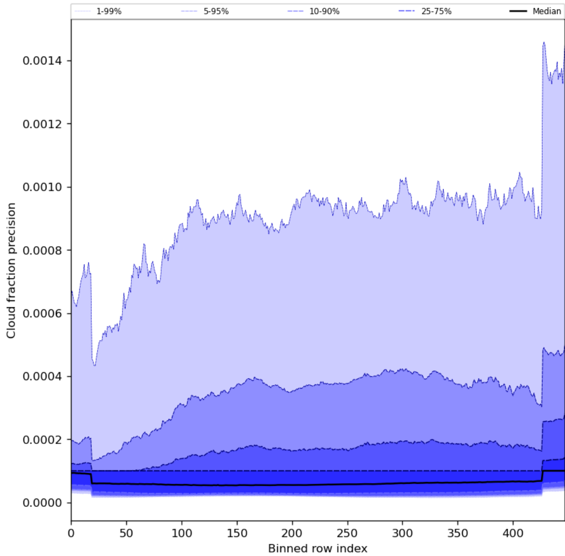
Figure 50: Along track statistics of “Cloud fraction precision” for 2024-02-20 to 2024-02-22
