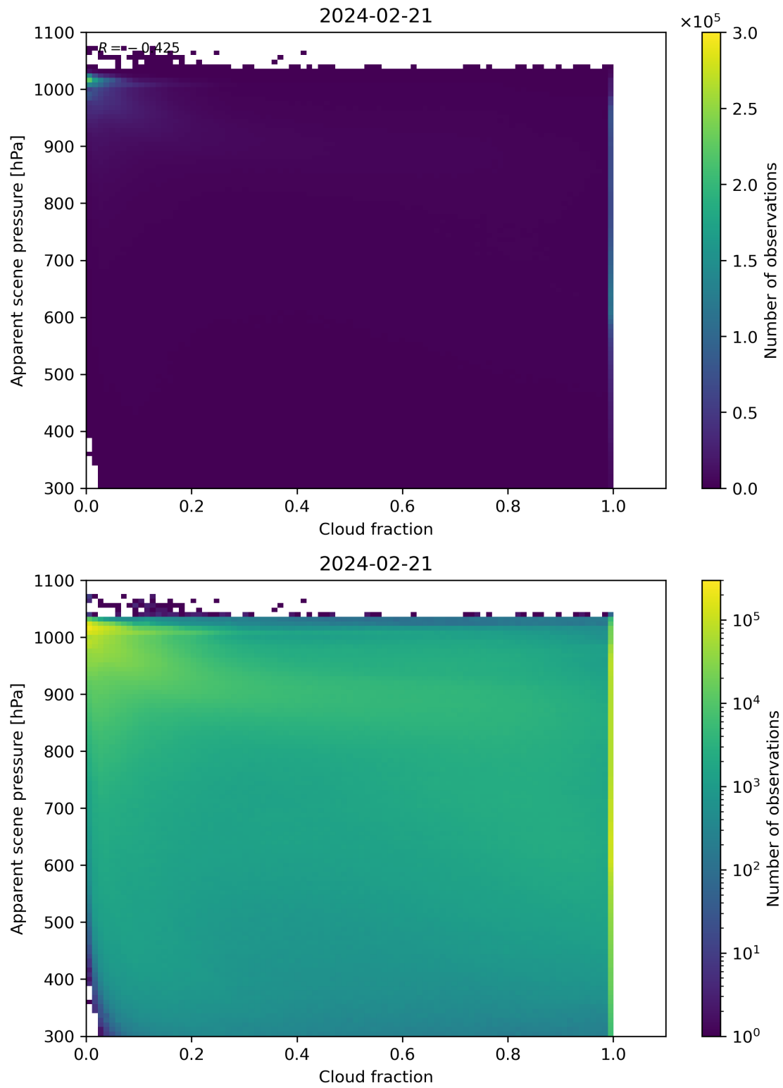
Figure 70: Scatter density plot of “Cloud fraction” against “Apparent scene pressure” for 2024-02-20 to 2024-02-22.
