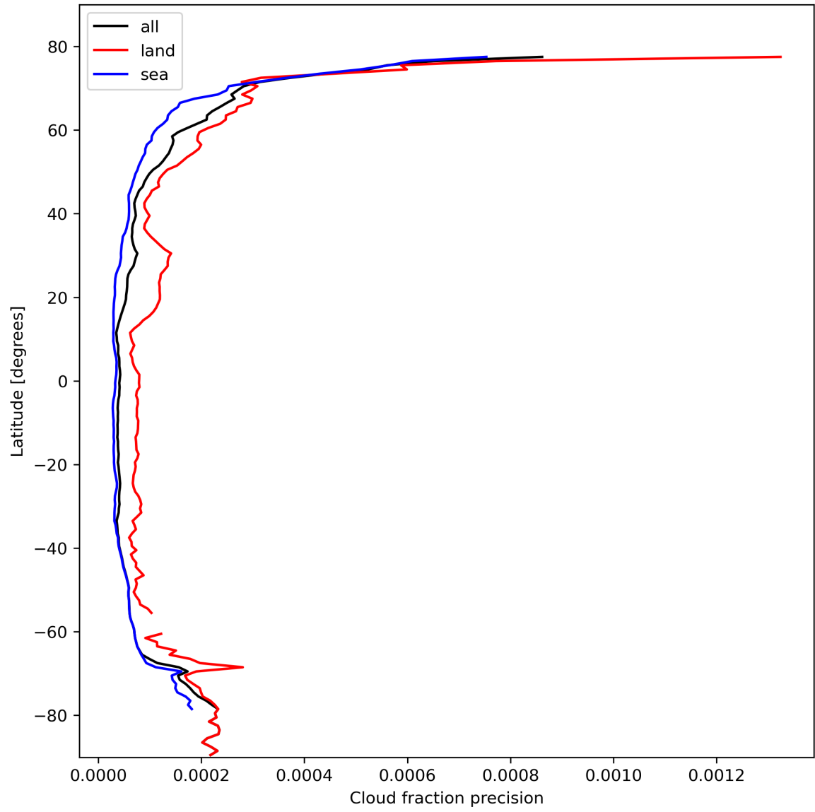
Figure 16: Zonal average of “Cloud fraction precision” for 2024-02-20 to 2024-02-22.
