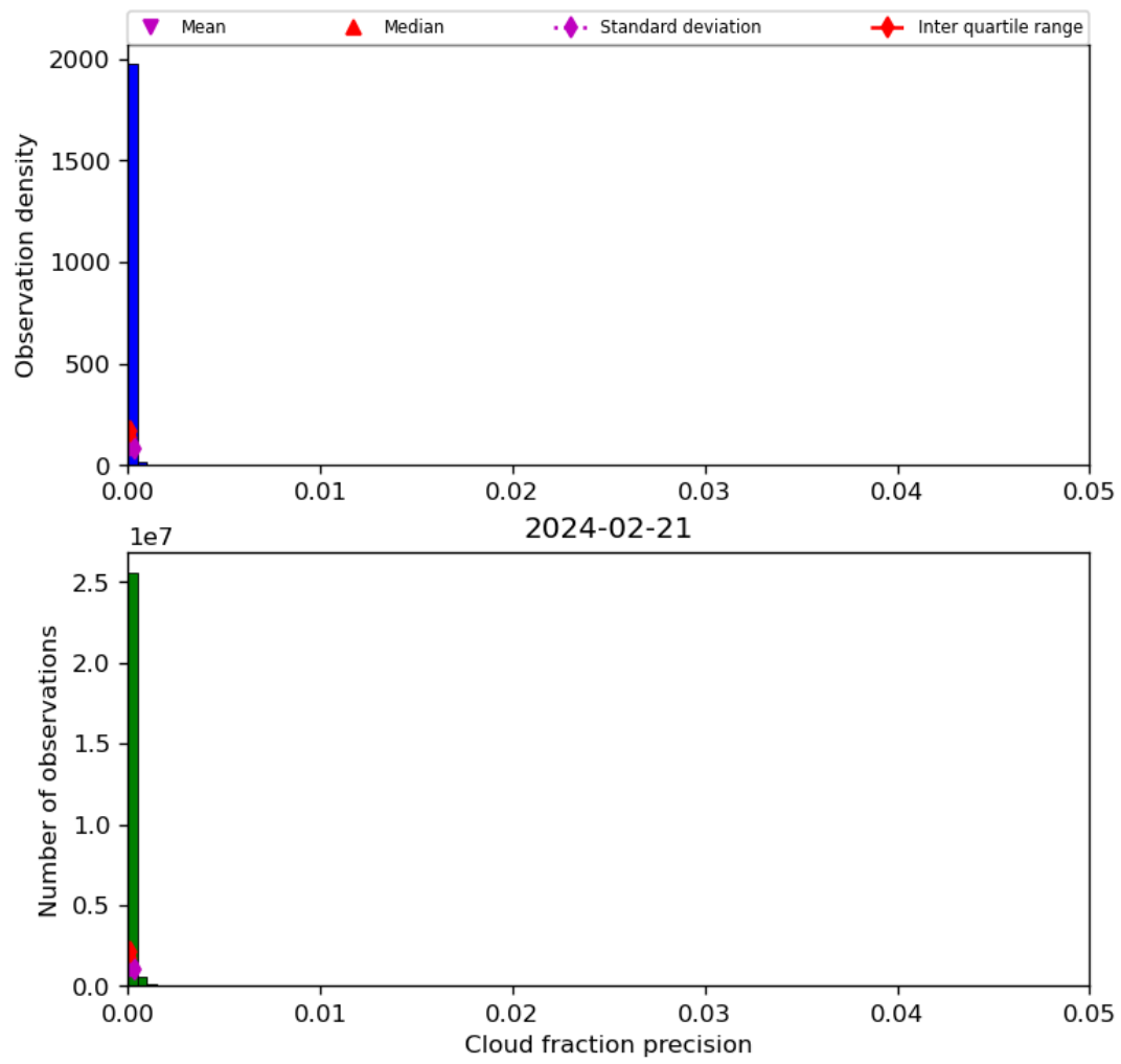
Figure 33: Histogram of “Cloud fraction precision” for 2024-02-20 to 2024-02-22
