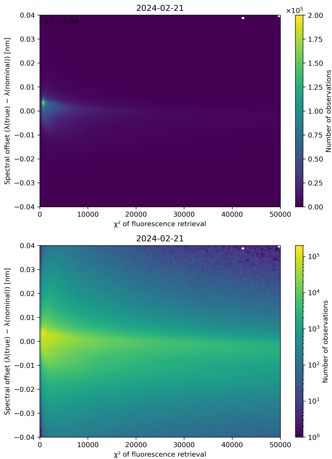
Figure 69: Scatter density plot of “ \chi^2 of fluorescence retrieval” against “Spectral offset ( \lambda(\text{true}) - \lambda(\text{nominal}) )” for 2024-02-20 to 2024-02-22.
