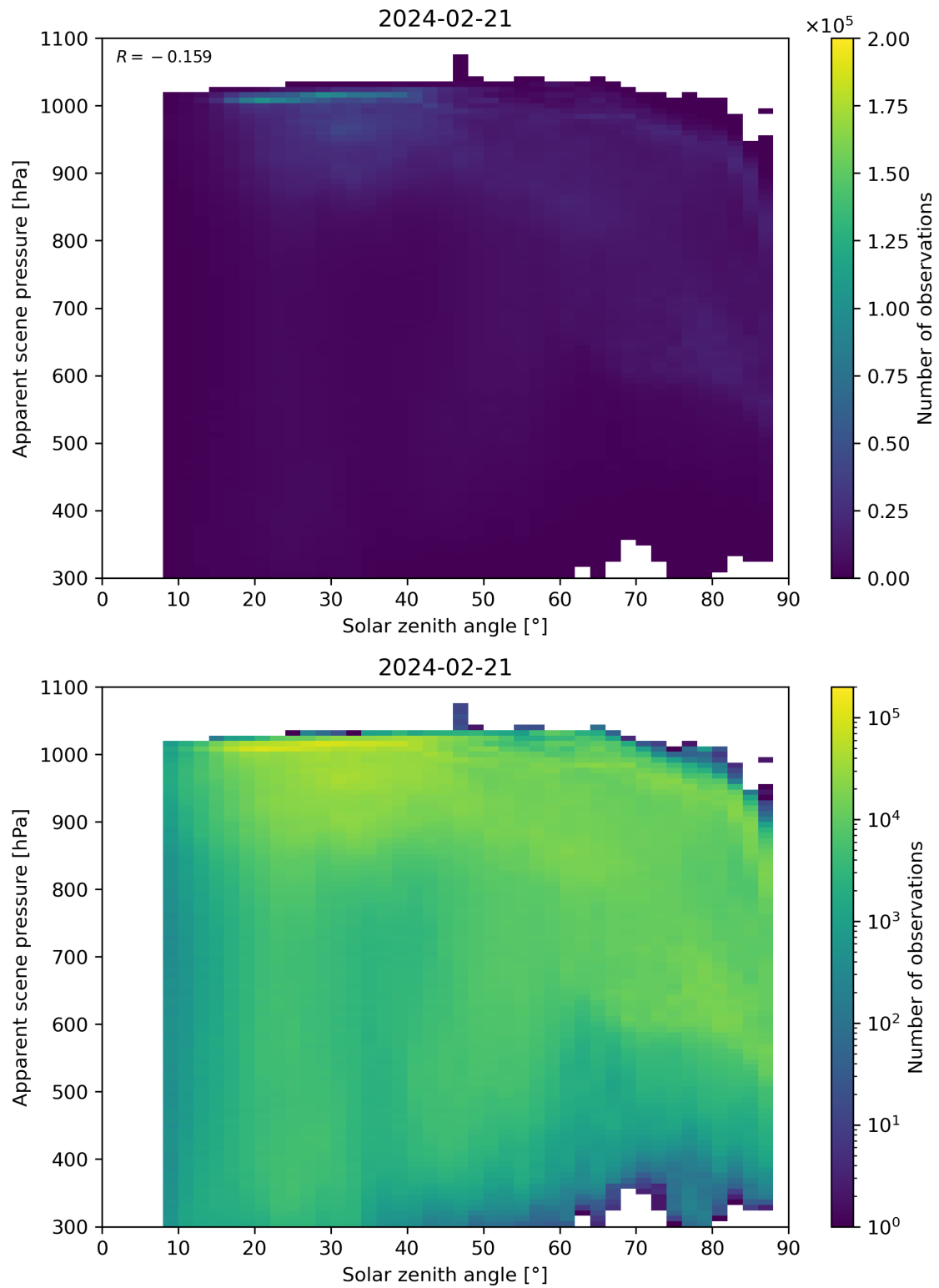
Figure 108: Scatter density plot of “Solar zenith angle” against “Apparent scene pressure” for 2024-02-20 to 2024-02-22.
