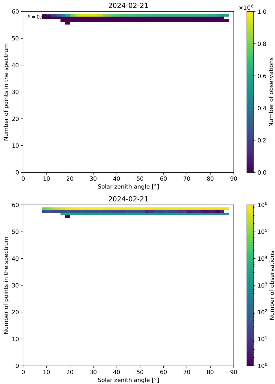
Figure 115: Scatter density plot of “Solar zenith angle” against “Number of points in the spectrum” for 2024-02-20 to 2024-02-22.
