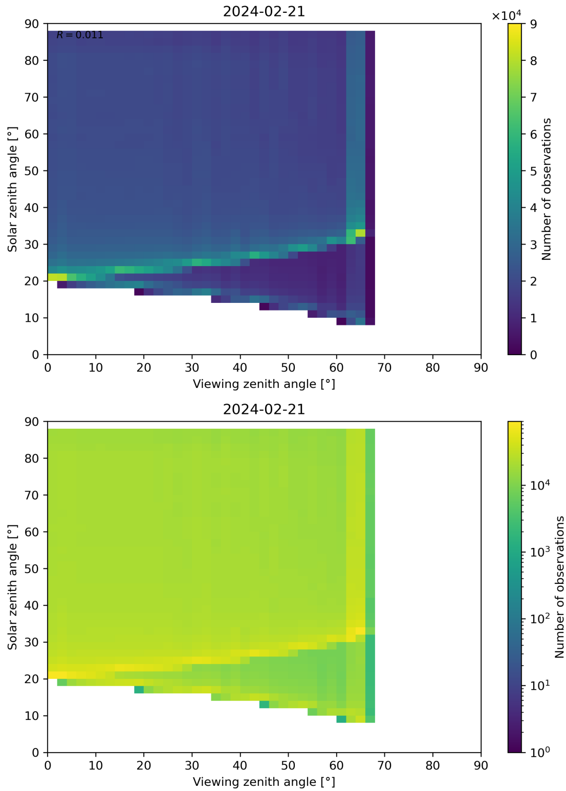
Figure 127: Scatter density plot of “Viewing zenith angle” against “Solar zenith angle” for 2024-02-20 to 2024-02-22.
