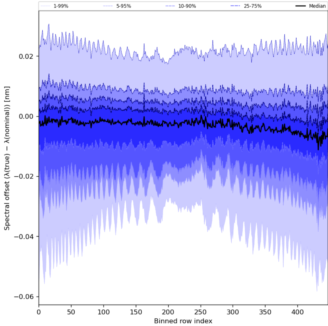
Figure 62: Along track statistics of “Spectral offset ( \lambda(\text{true}) - \lambda(\text{nominal}) )” for 2024-02-20 to 2024-02-22
