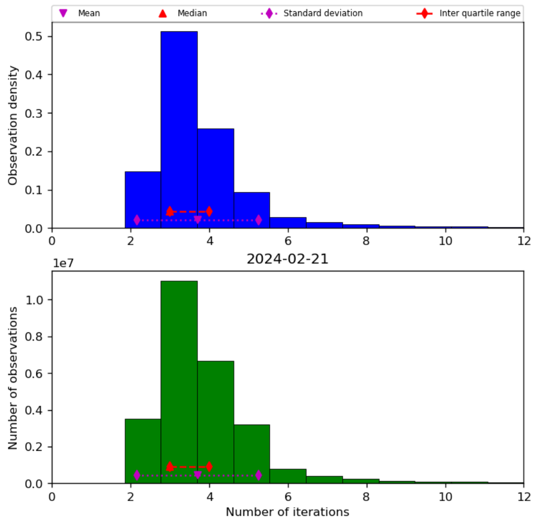
Figure 39: Histogram of “Number of iterations” for 2024-02-20 to 2024-02-22
