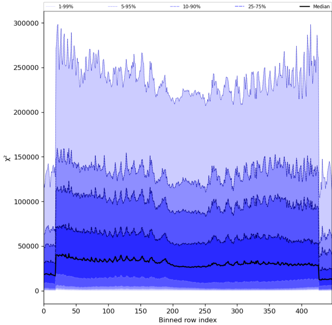
Figure 55: Along track statistics of “ \chi^2 ” for 2024-02-20 to 2024-02-22
