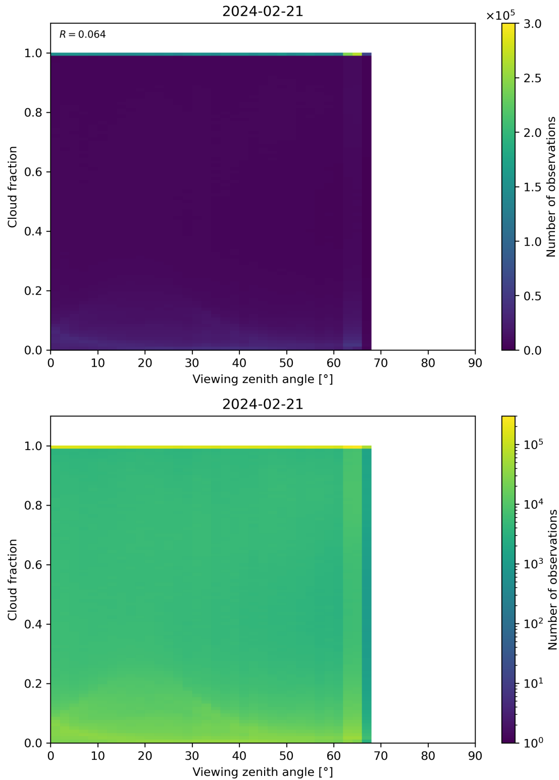
Figure 120: Scatter density plot of “Viewing zenith angle” against “Cloud fraction” for 2024-02-20 to 2024-02-22.
