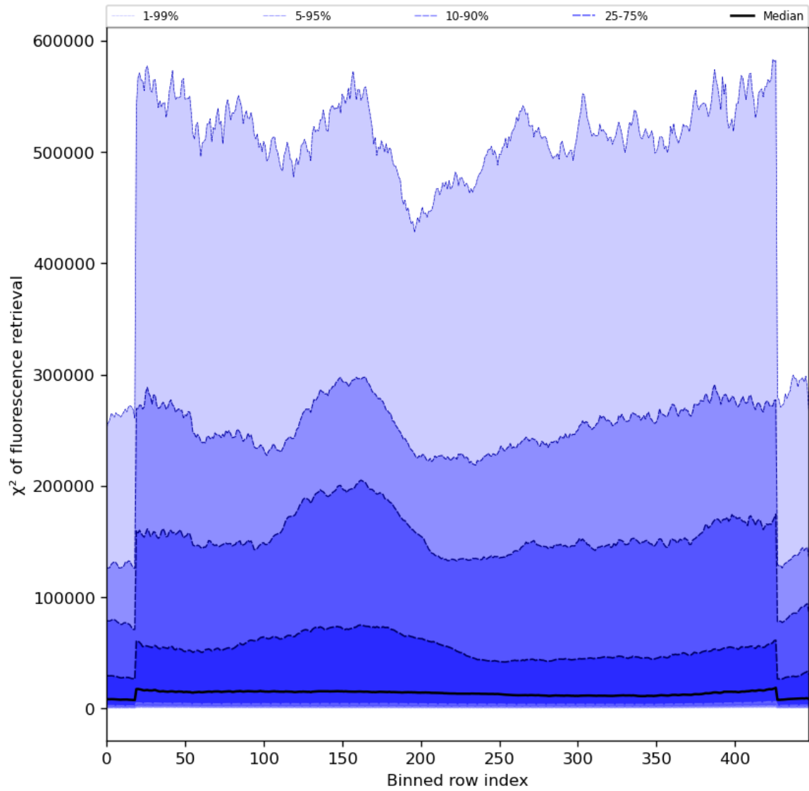
Figure 59: Along track statistics of “ \chi^2 of fluorescence retrieval” for 2024-02-20 to 2024-02-22
