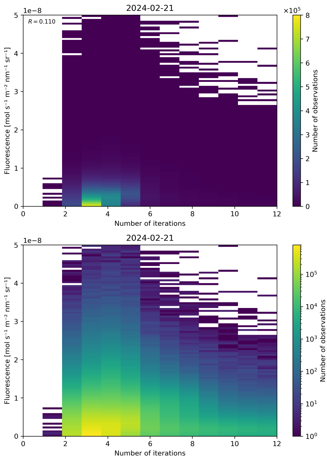
Figure 98: Scatter density plot of “Number of iterations” against “Fluorescence” for 2024-02-20 to 2024-02-22.
