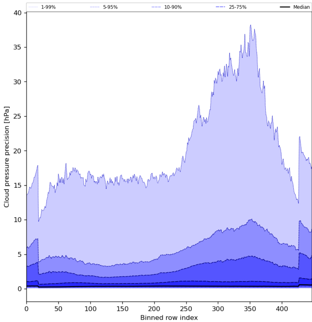
Figure 48: Along track statistics of “Cloud pressure precision” for 2024-02-20 to 2024-02-22
