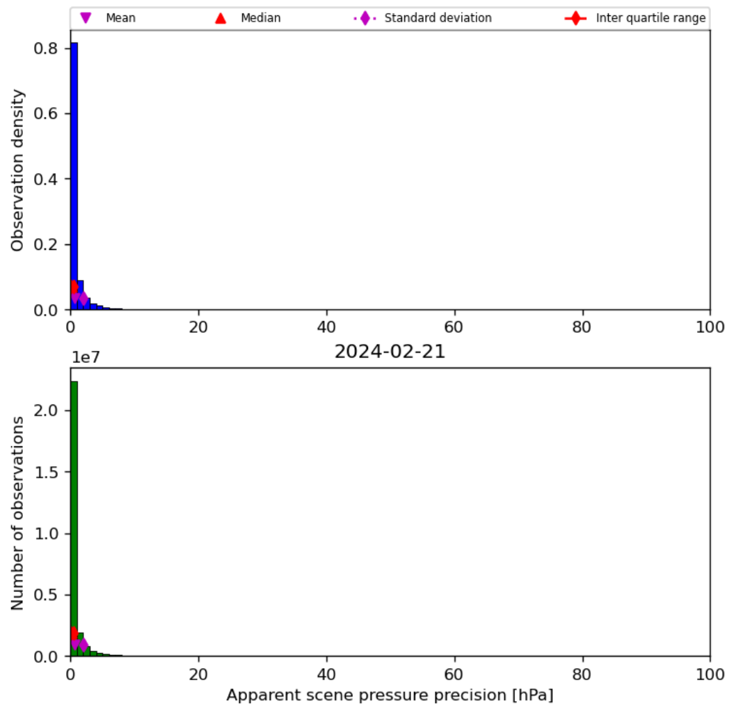
Figure 37: Histogram of “Apparent scene pressure precision” for 2024-02-20 to 2024-02-22
