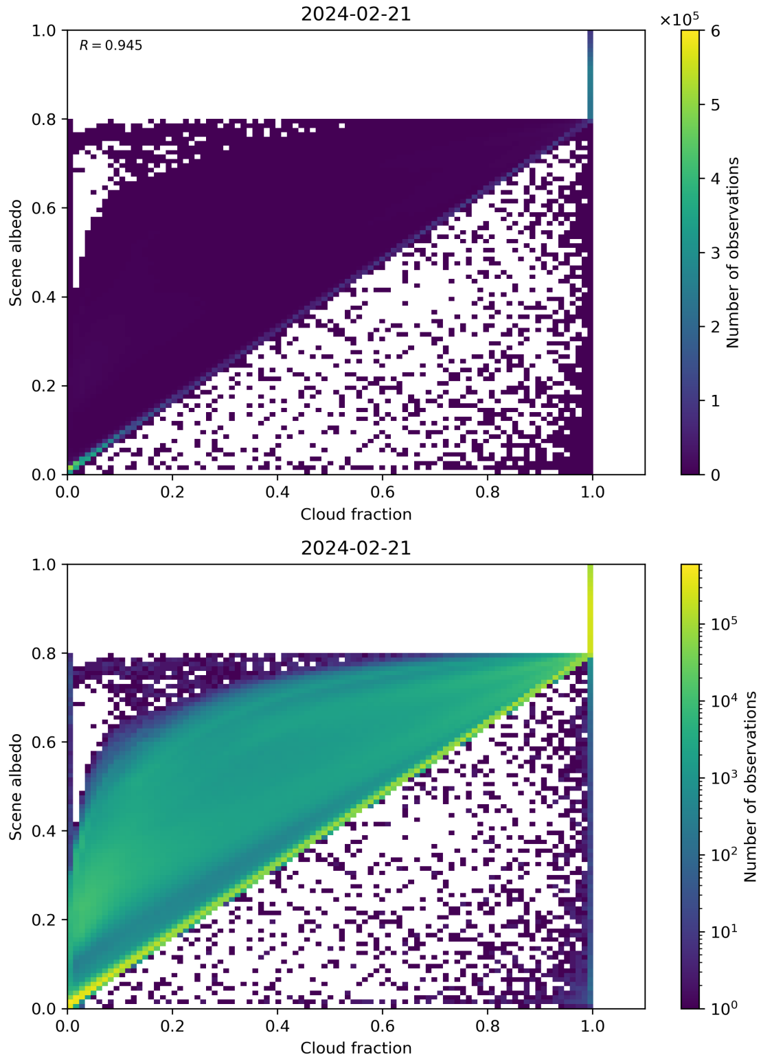
Figure 75: Scatter density plot of “Cloud fraction” against “Scene albedo” for 2024-02-20 to 2024-02-22.
