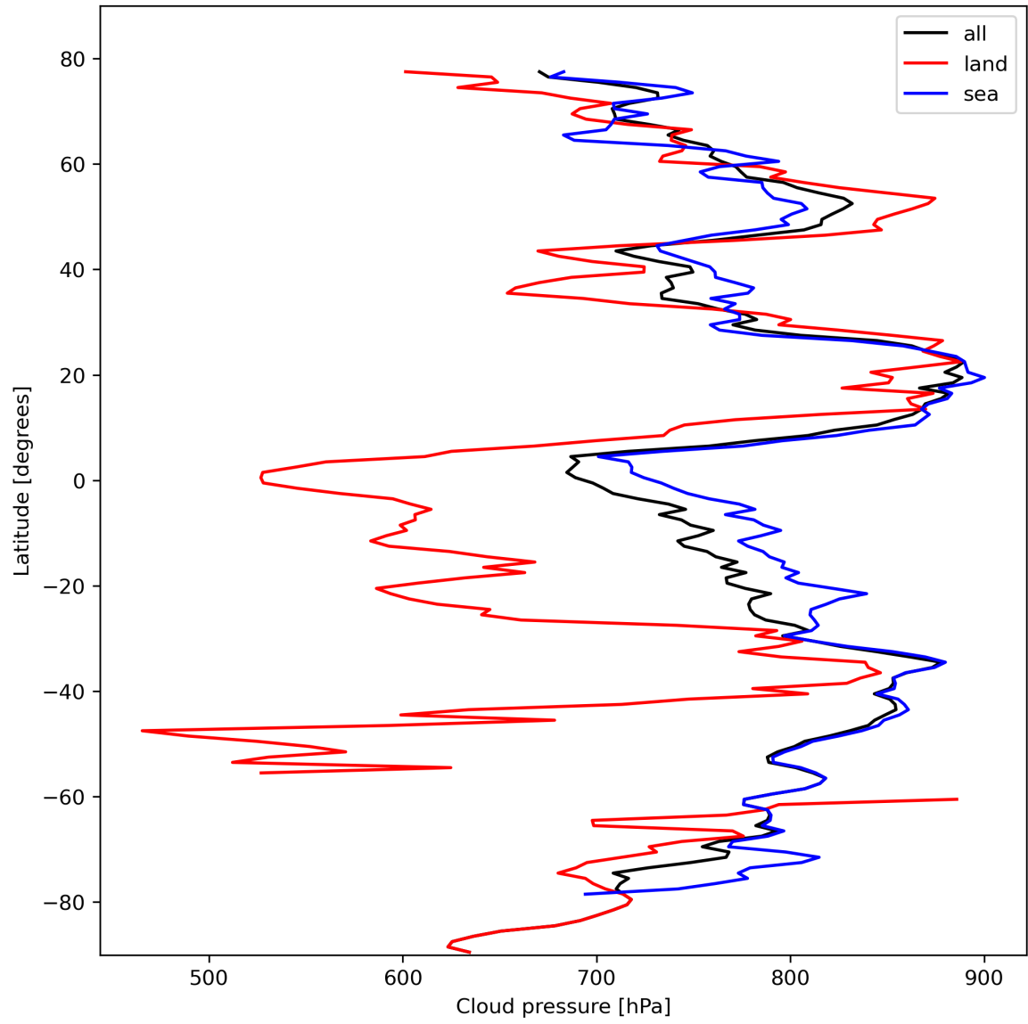
Figure 13: Zonal average of “Cloud pressure” for 2024-02-20 to 2024-02-22.
