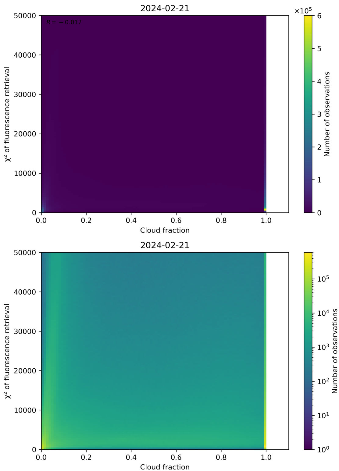
Figure 71: Scatter density plot of “Cloud fraction” against “ \chi^2 of fluorescence retrieval” for 2024-02-20 to 2024-02-22.
