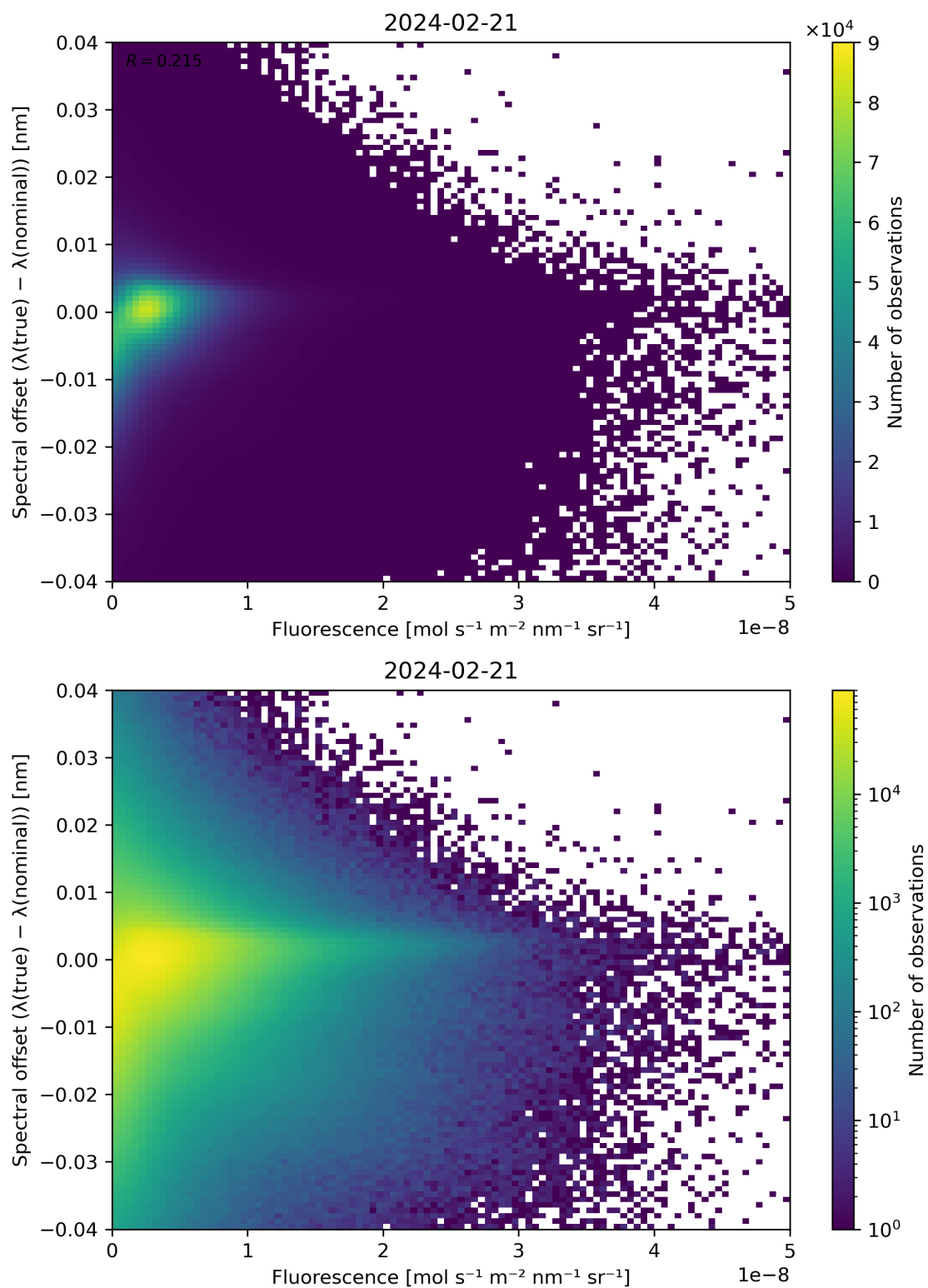
Figure 87: Scatter density plot of “Fluorescence” against “Spectral offset ( \lambda(\text{true}) - \lambda(\text{nominal}) )” for 2024-02-20 to 2024-02-22.
