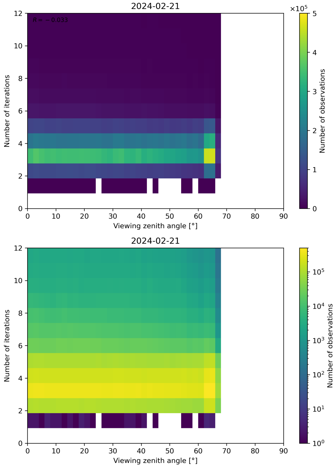
Figure 124: Scatter density plot of “Viewing zenith angle” against “Number of iterations” for 2024-02-20 to 2024-02-22.
