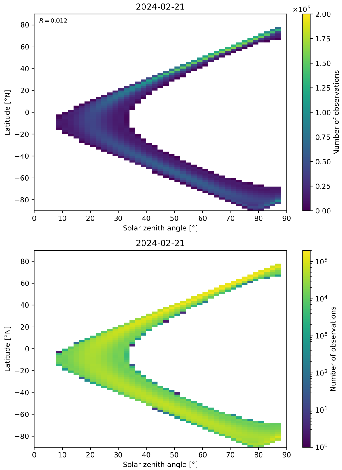
Figure 113: Scatter density plot of “Solar zenith angle” against “Latitude” for 2024-02-20 to 2024-02-22.
