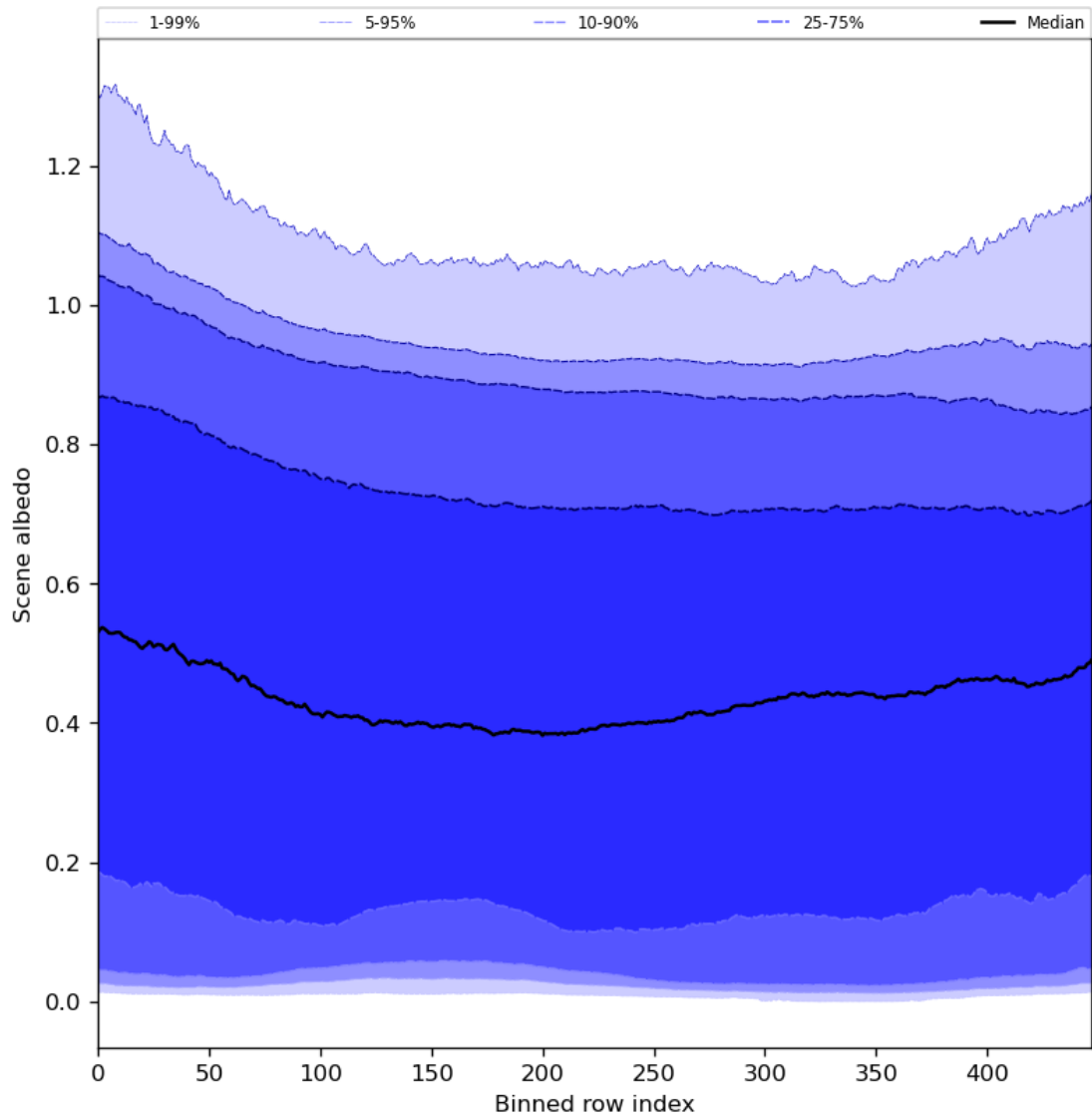
Figure 51: Along track statistics of “Scene albedo” for 2024-02-20 to 2024-02-22
