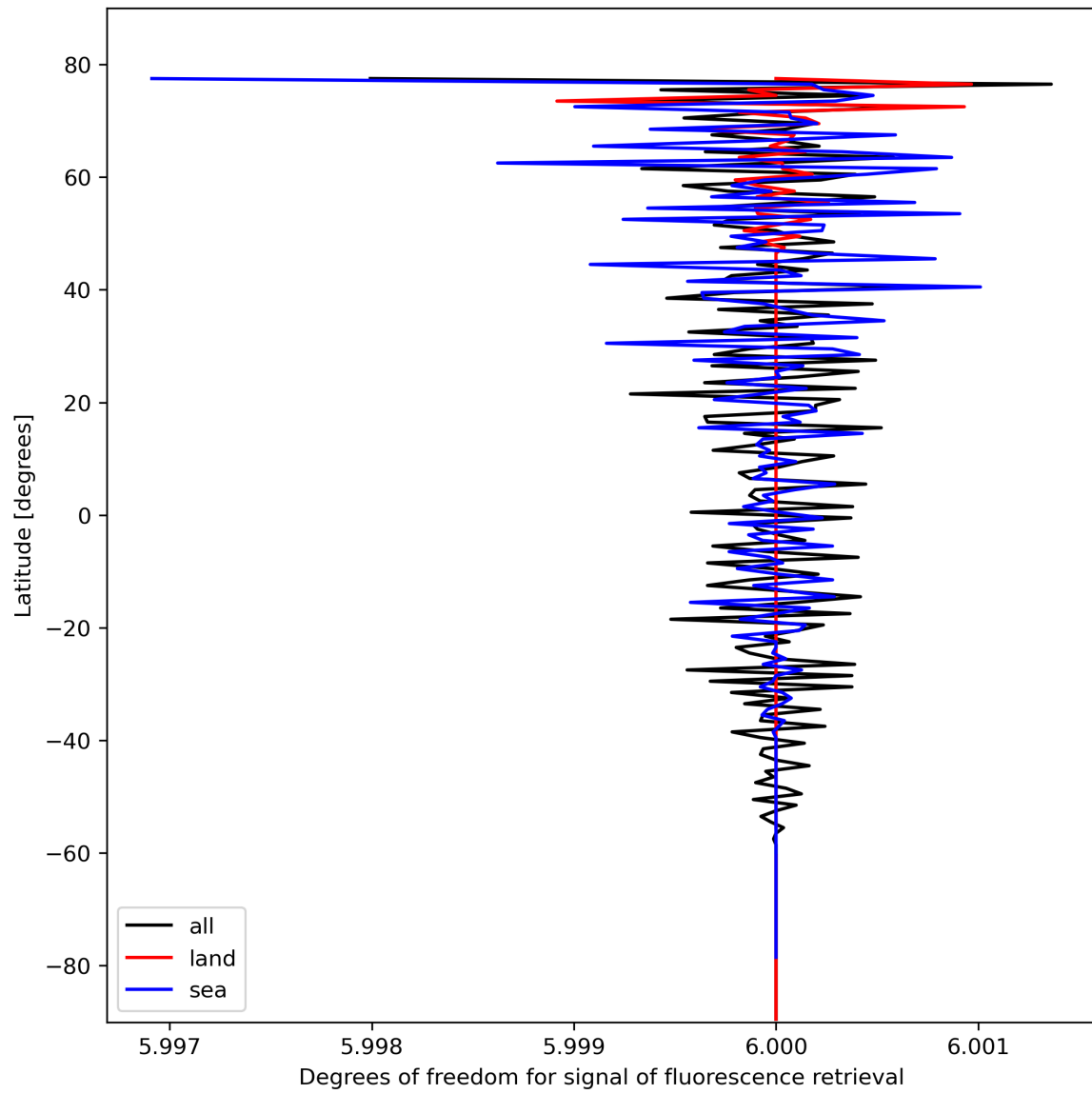
Figure 26: Zonal average of “Degrees of freedom for signal of fluorescence retrieval” for 2024-02-20 to 2024-02-22.
