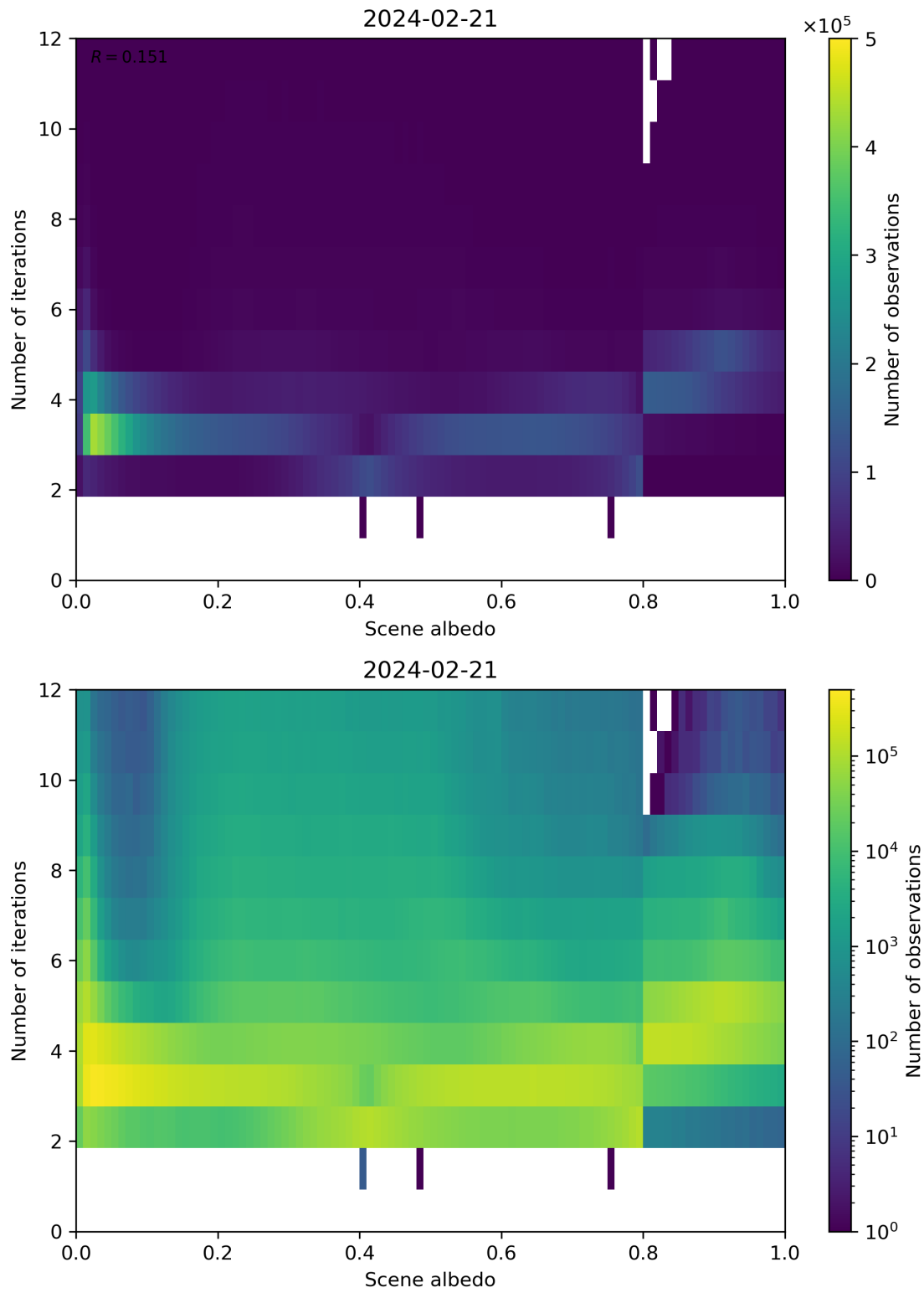
Figure 105: Scatter density plot of “Scene albedo” against “Number of iterations” for 2024-02-20 to 2024-02-22.
