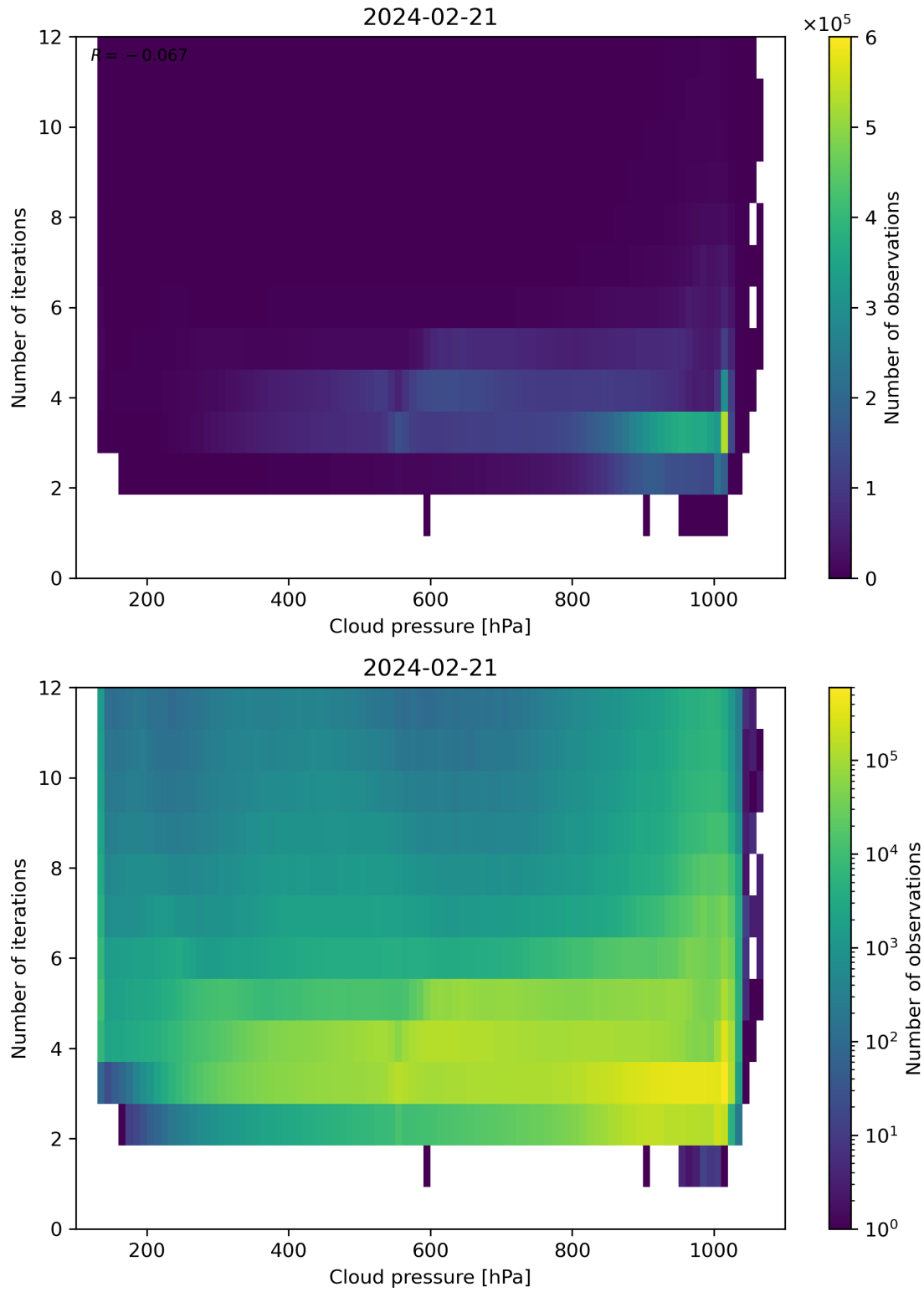
Figure 81: Scatter density plot of “Cloud pressure” against “Number of iterations” for 2024-02-20 to 2024-02-22.
