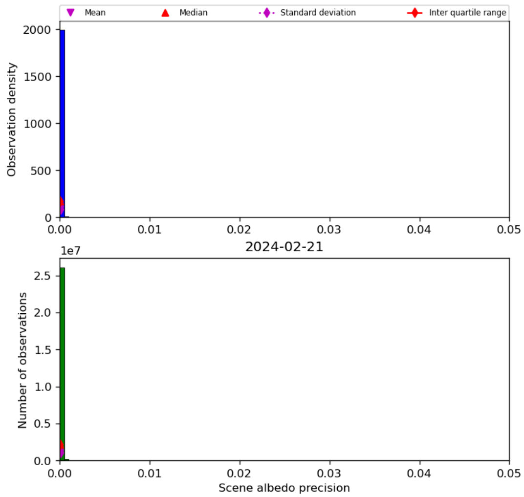
Figure 35: Histogram of “Scene albedo precision” for 2024-02-20 to 2024-02-22
