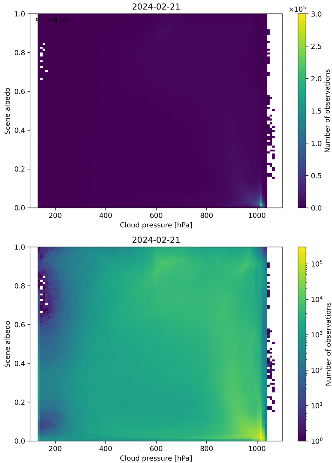
Figure 83: Scatter density plot of “Cloud pressure” against “Scene albedo” for 2024-02-20 to 2024-02-22.
