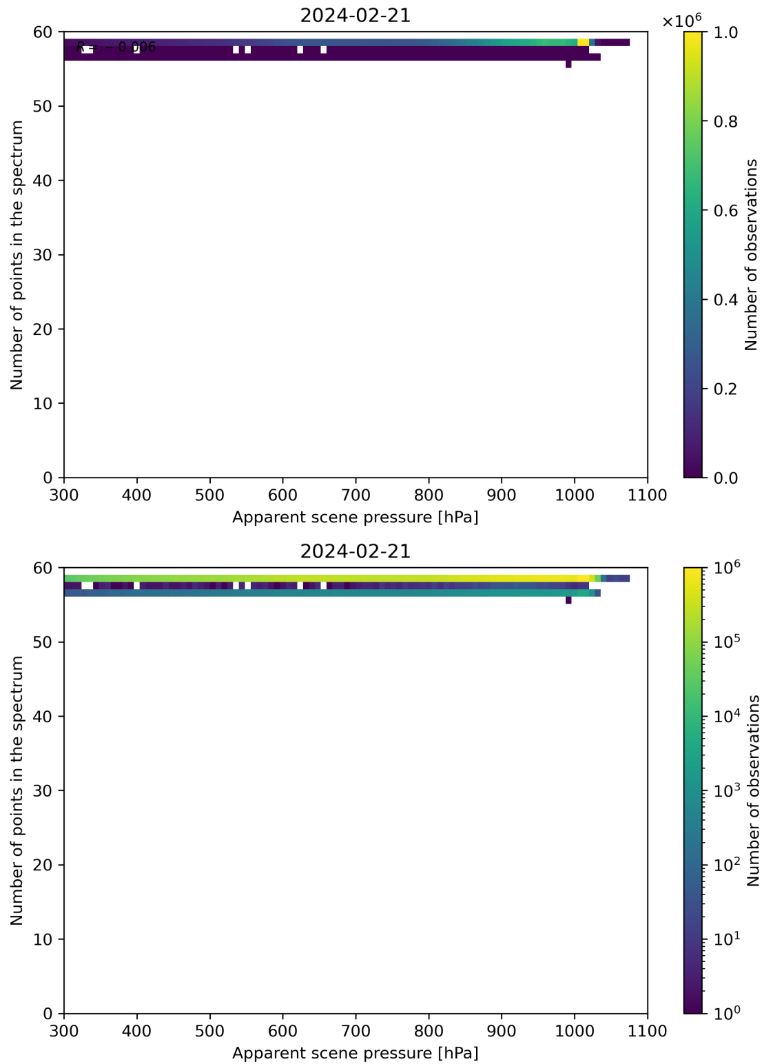
Figure 66: Scatter density plot of “Apparent scene pressure” against “Number of points in the spectrum” for 2024-02-20 to 2024-02-22.
