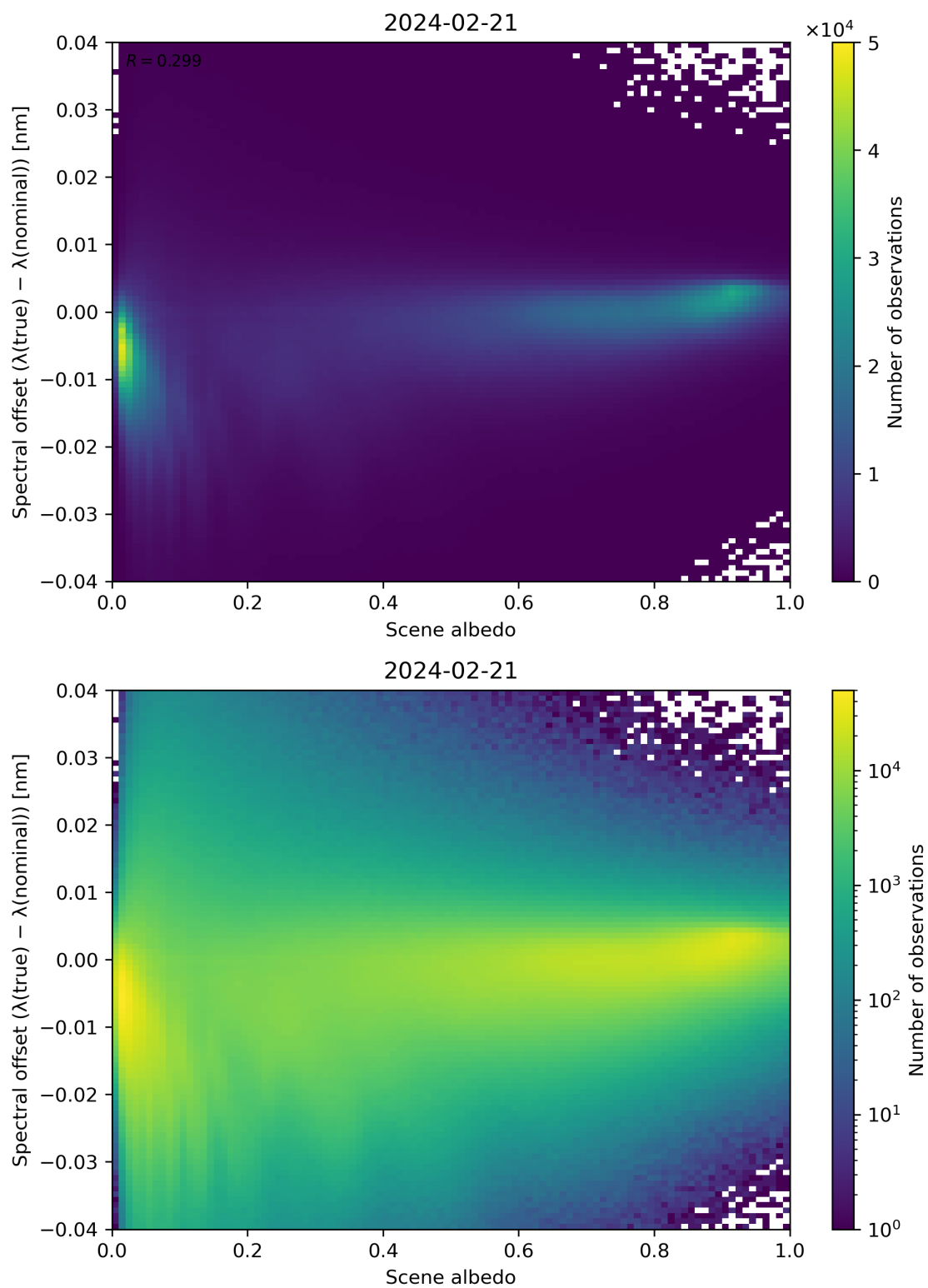
Figure 107: Scatter density plot of “Scene albedo” against “Spectral offset ( \lambda(\text{true}) - \lambda(\text{nominal}) )” for 2024-02-20 to 2024-02-22.
