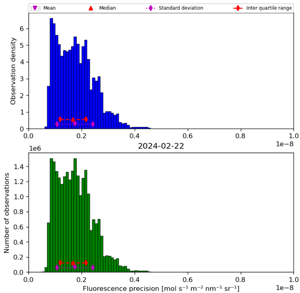
Figure 41: Histogram of “Fluorescence precision” for 2024-02-22 to 2024-02-23
