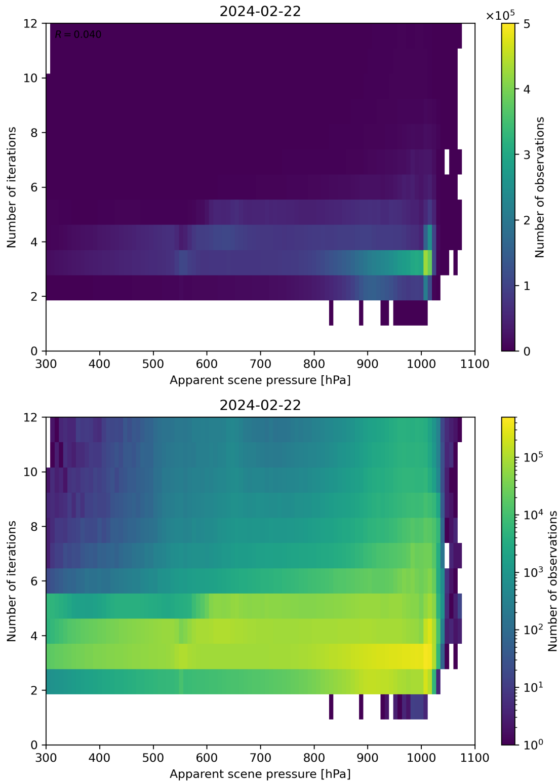
Figure 65: Scatter density plot of “Apparent scene pressure” against “Number of iterations” for 2024-02-22 to 2024-02-23.
