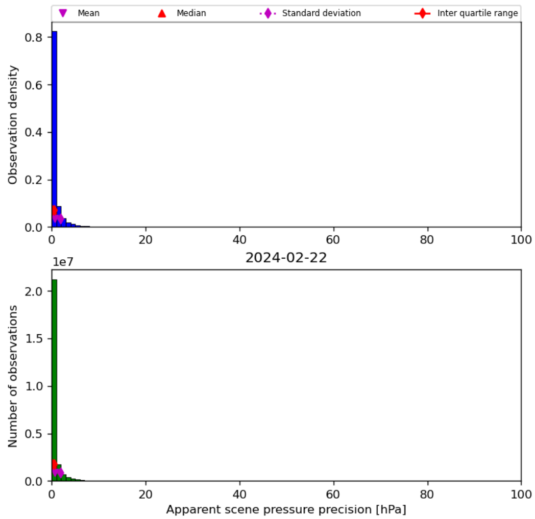
Figure 37: Histogram of “Apparent scene pressure precision” for 2024-02-22 to 2024-02-23
