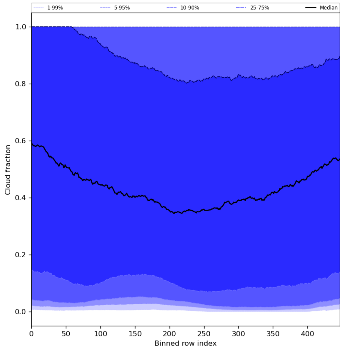
Figure 49: Along track statistics of “Cloud fraction” for 2024-02-22 to 2024-02-23
