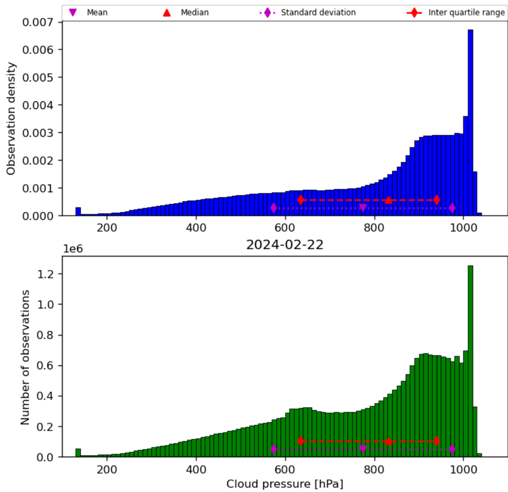
Figure 30: Histogram of “Cloud pressure” for 2024-02-22 to 2024-02-23
