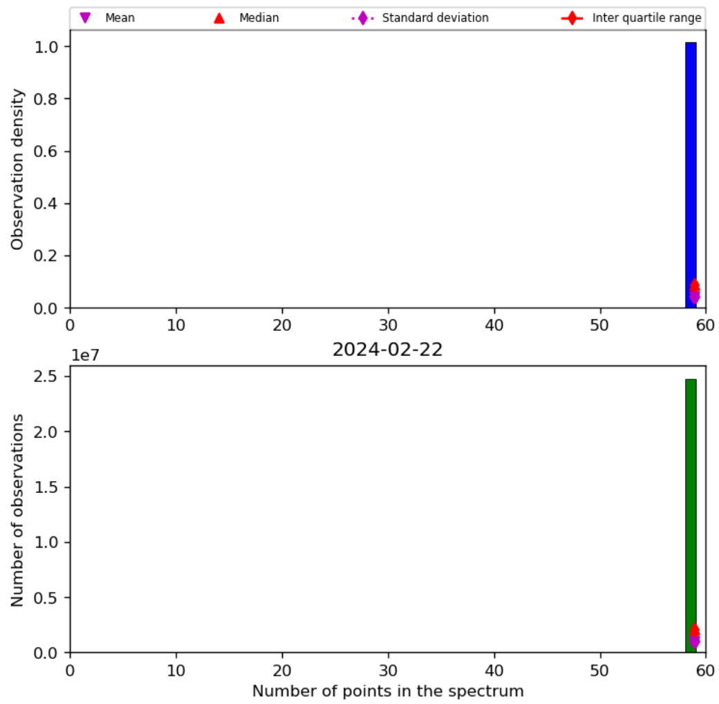
Figure 44: Histogram of "Number of points in the spectrum" for 2024-02-22 to 2024-02-23
