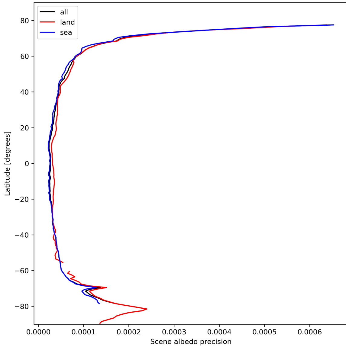
Figure 18: Zonal average of “Scene albedo precision” for 2024-02-22 to 2024-02-23.
