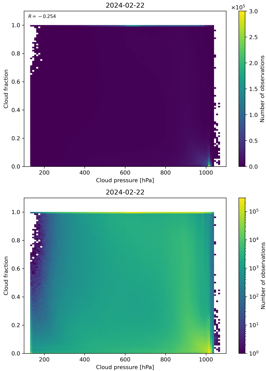
Figure 79: Scatter density plot of “Cloud pressure” against “Cloud fraction” for 2024-02-22 to 2024-02-23.
