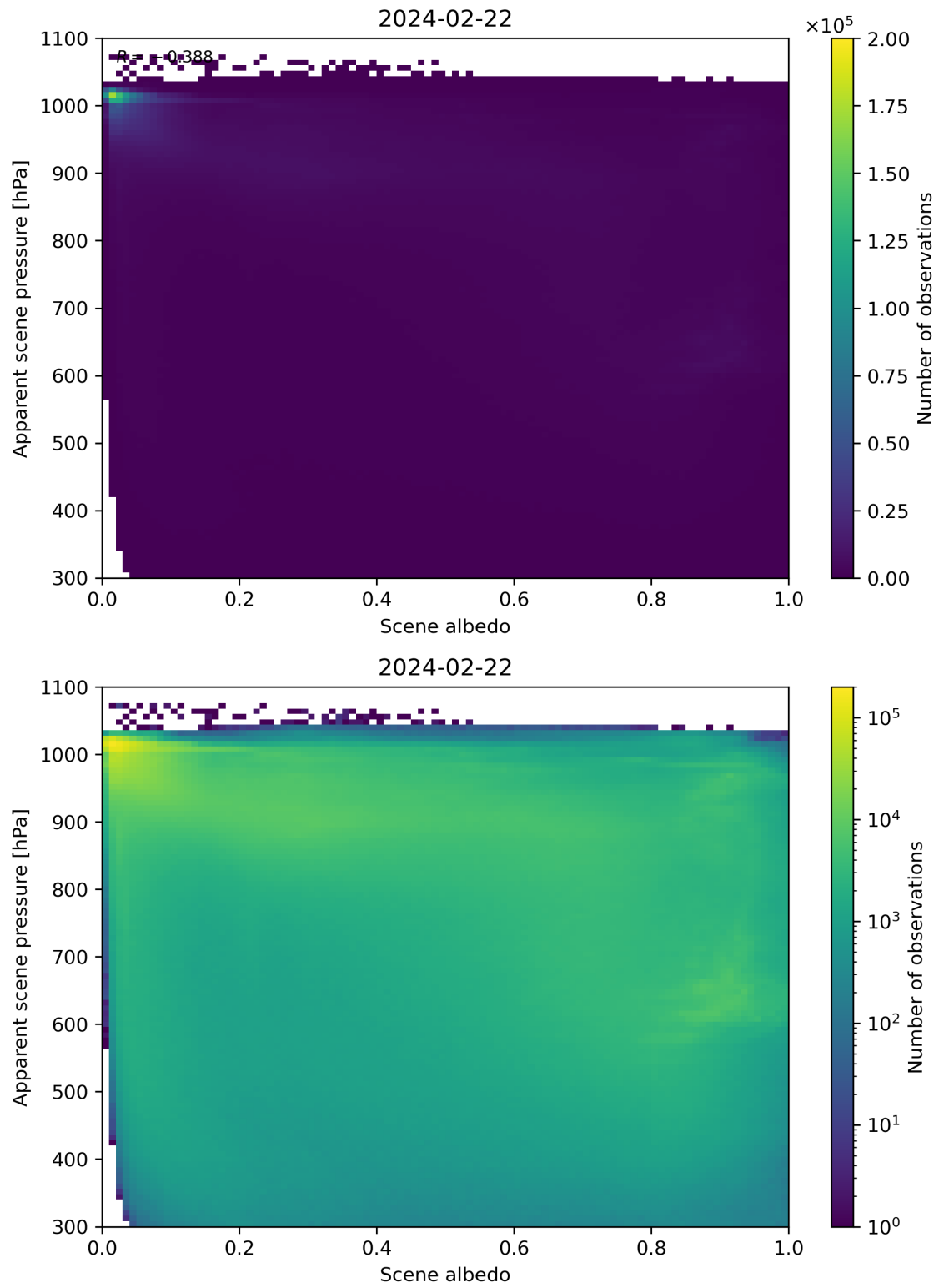
Figure 102: Scatter density plot of “Scene albedo” against “Apparent scene pressure” for 2024-02-22 to 2024-02-23.
