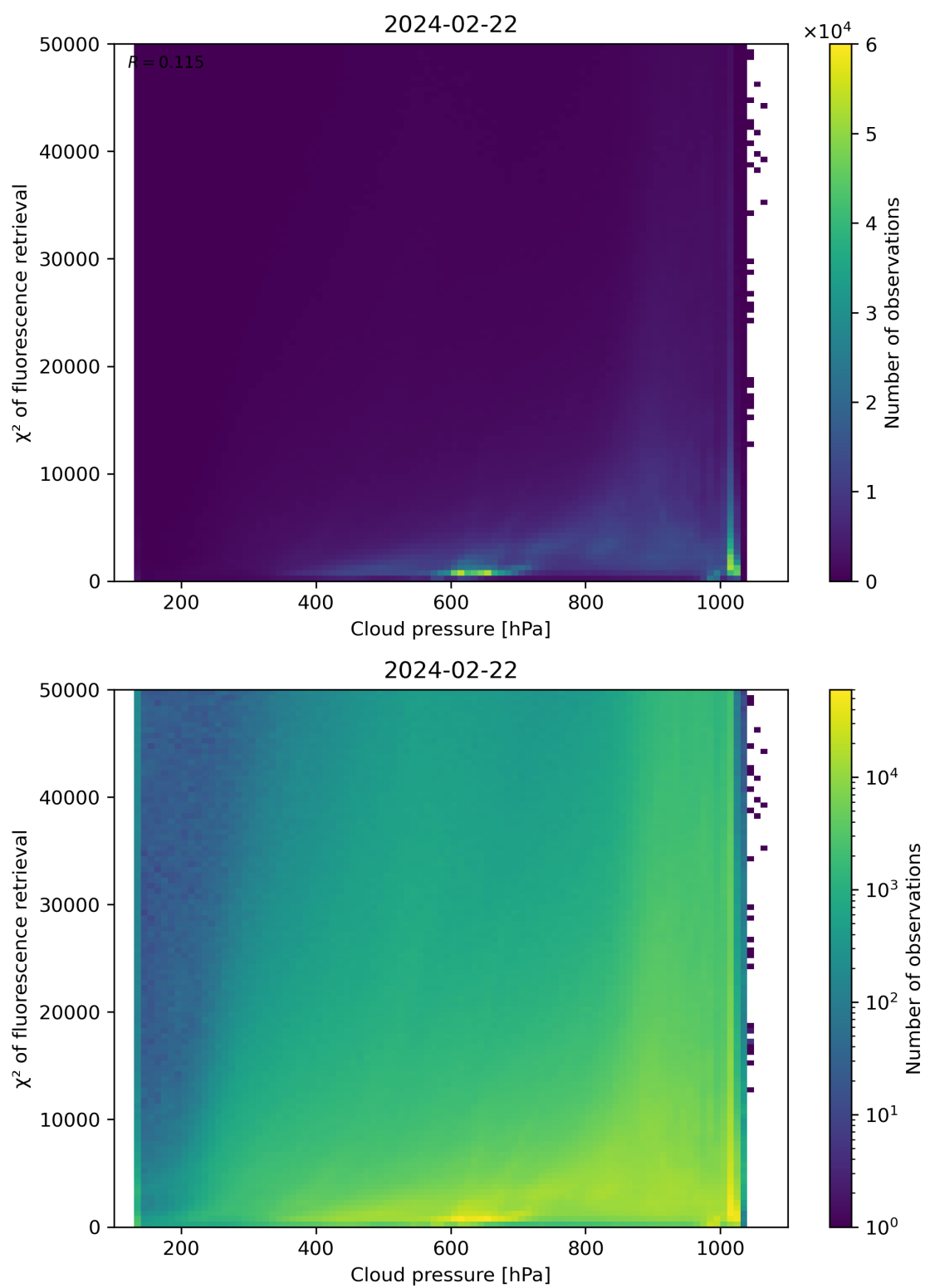
Figure 78: Scatter density plot of “Cloud pressure” against “ \chi^2 of fluorescence retrieval” for 2024-02-22 to 2024-02-23.
