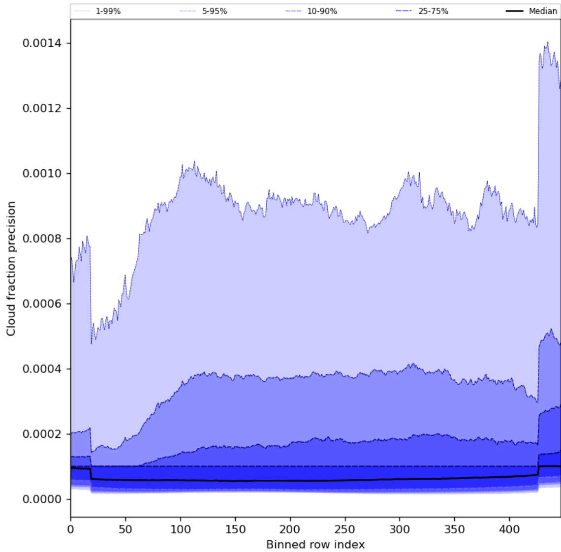
Figure 50: Along track statistics of “Cloud fraction precision” for 2024-02-22 to 2024-02-23
