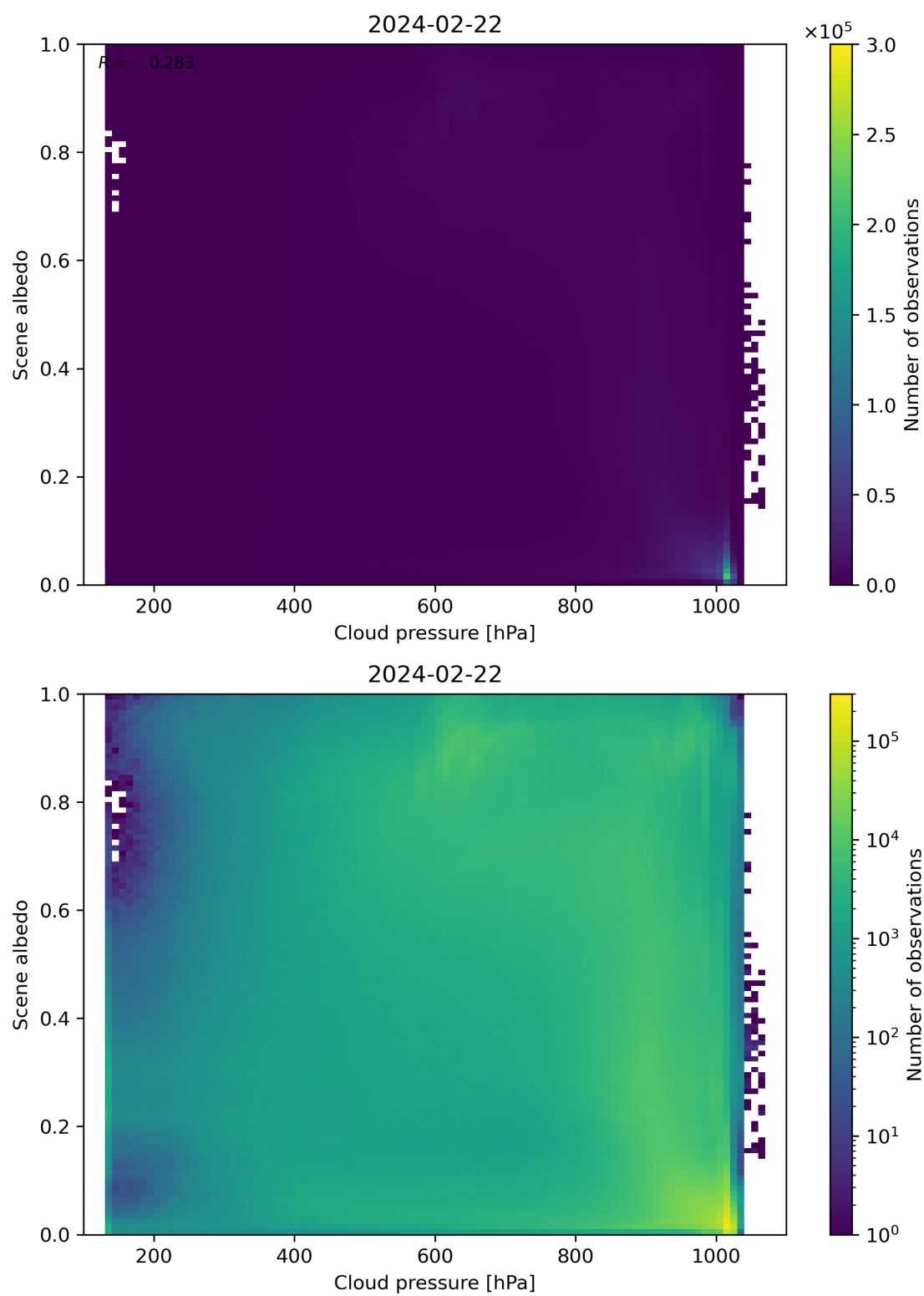
Figure 83: Scatter density plot of “Cloud pressure” against “Scene albedo” for 2024-02-22 to 2024-02-23.
