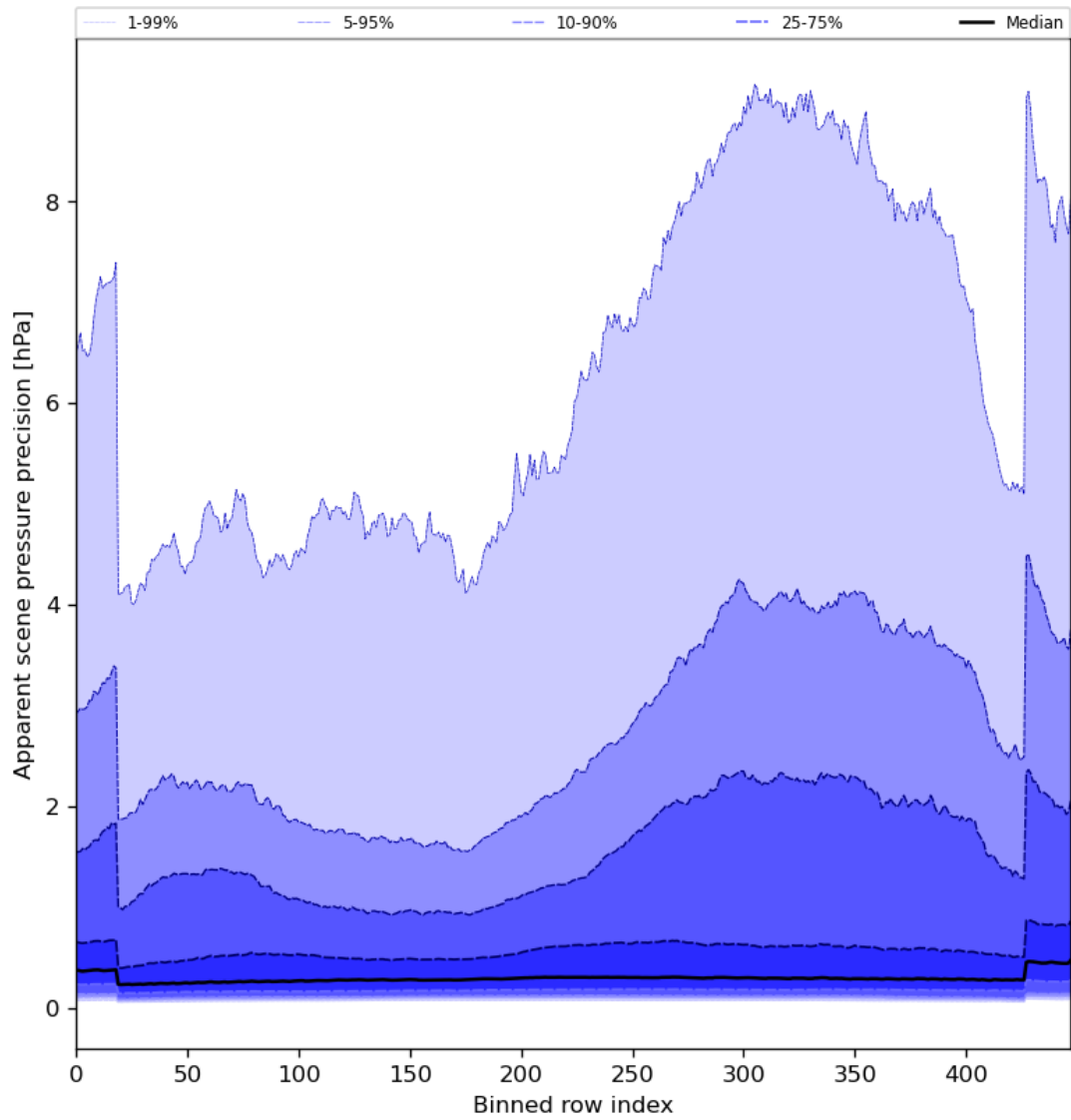
Figure 54: Along track statistics of “Apparent scene pressure precision” for 2024-02-22 to 2024-02-23
