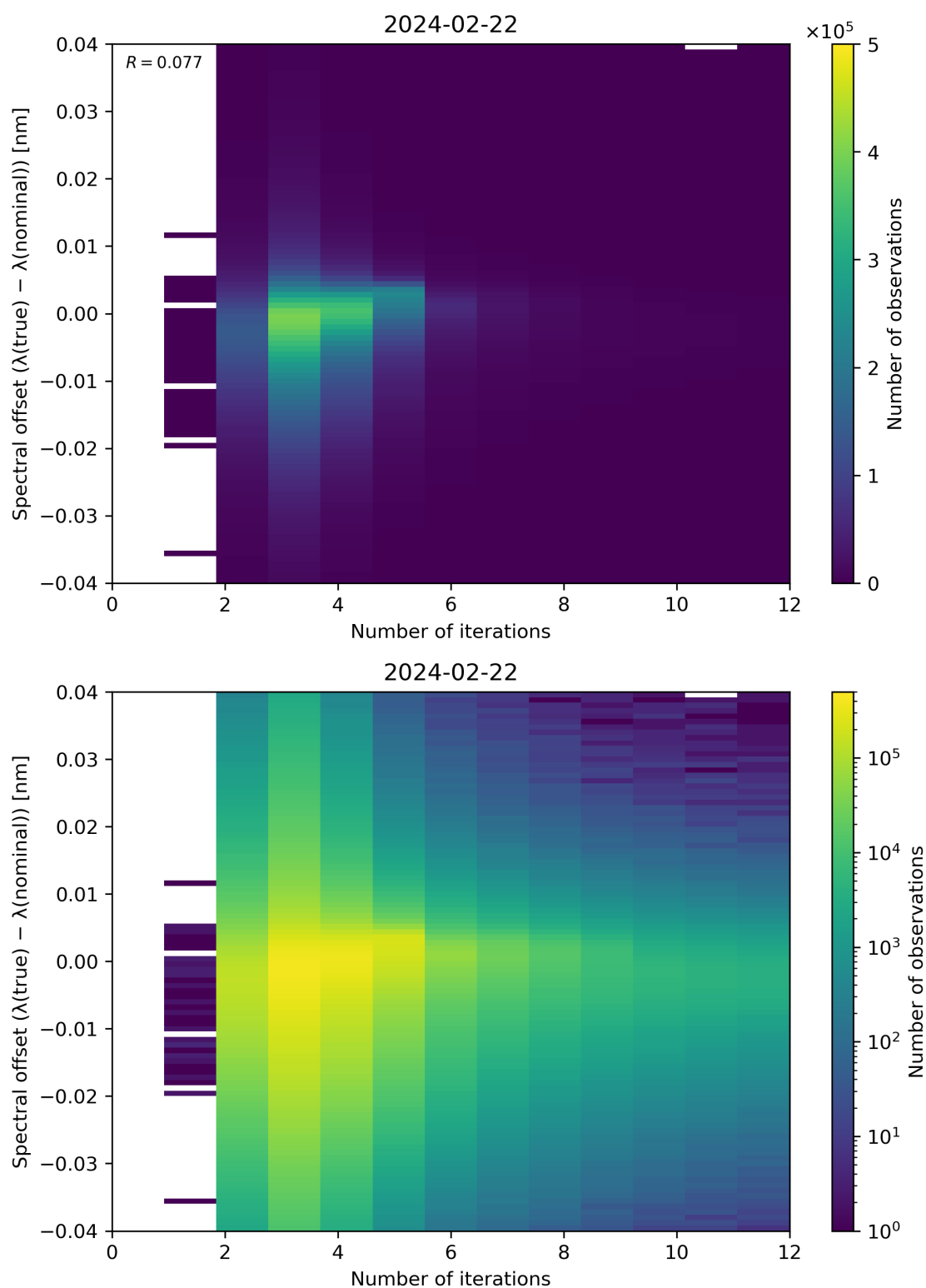
Figure 100: Scatter density plot of “Number of iterations” against “Spectral offset ( \lambda(\text{true}) - \lambda(\text{nominal}) )” for 2024-02-22 to 2024-02-23.
