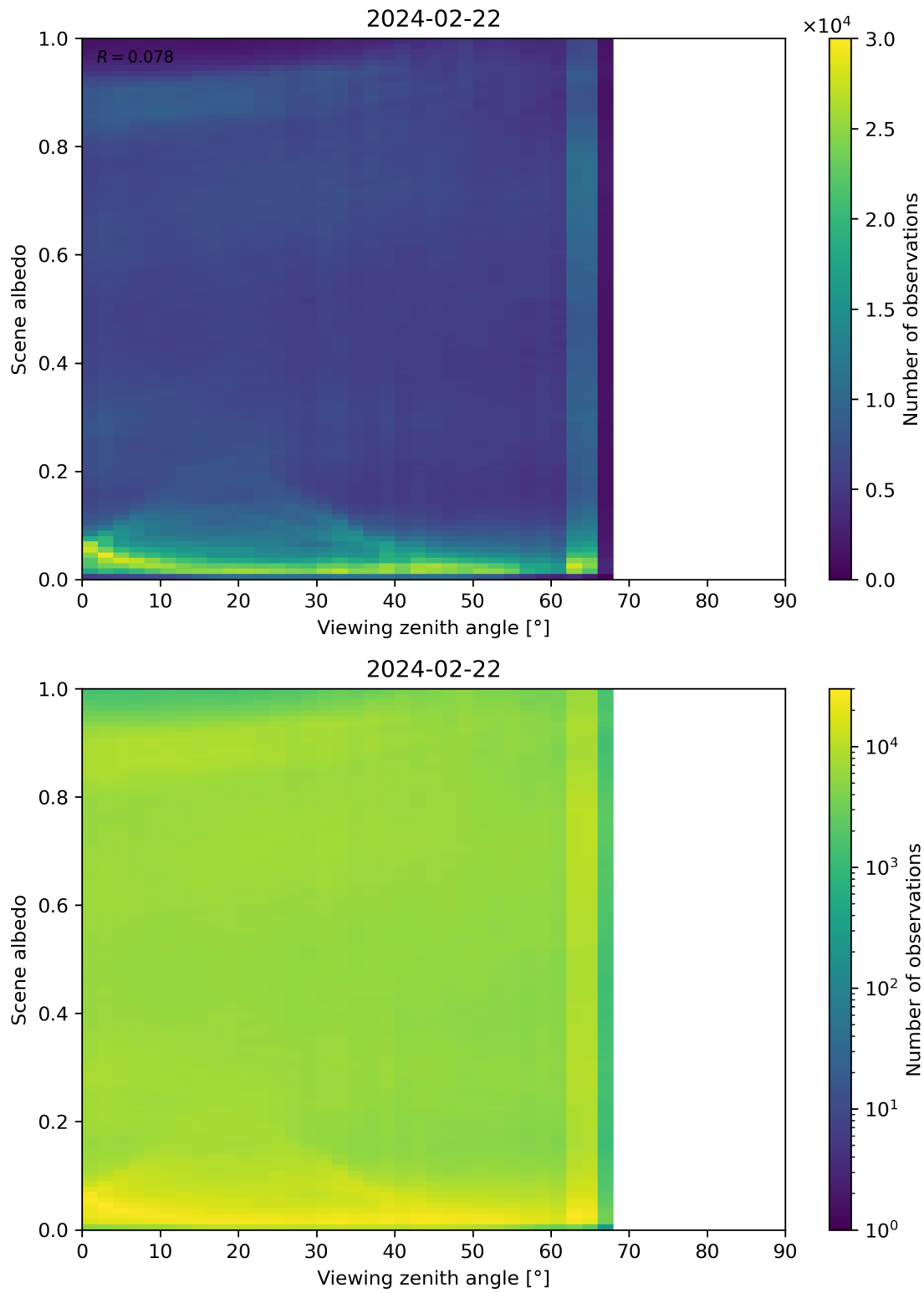
Figure 126: Scatter density plot of “Viewing zenith angle” against “Scene albedo” for 2024-02-22 to 2024-02-23.
