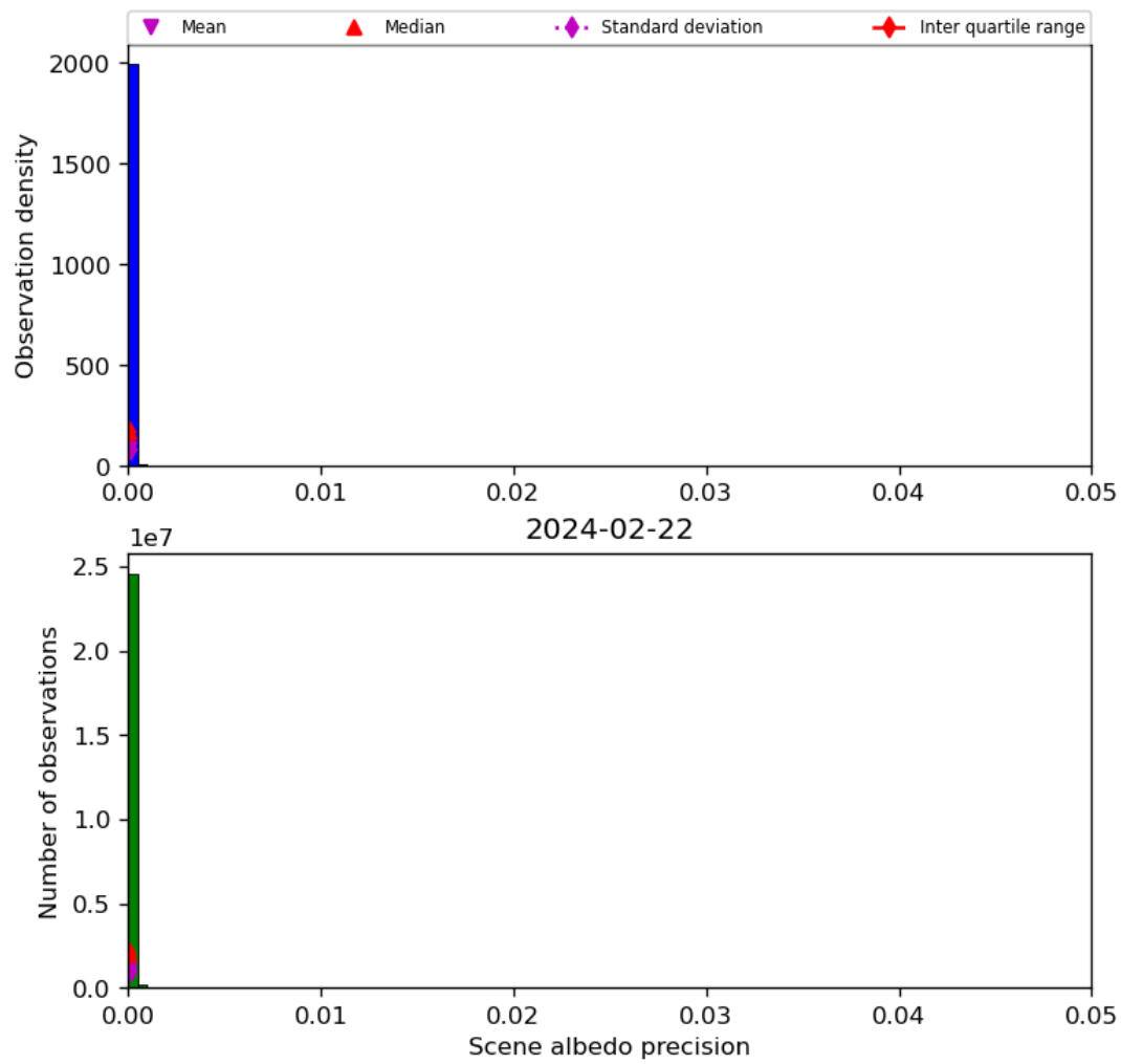
Figure 35: Histogram of “Scene albedo precision” for 2024-02-22 to 2024-02-23
