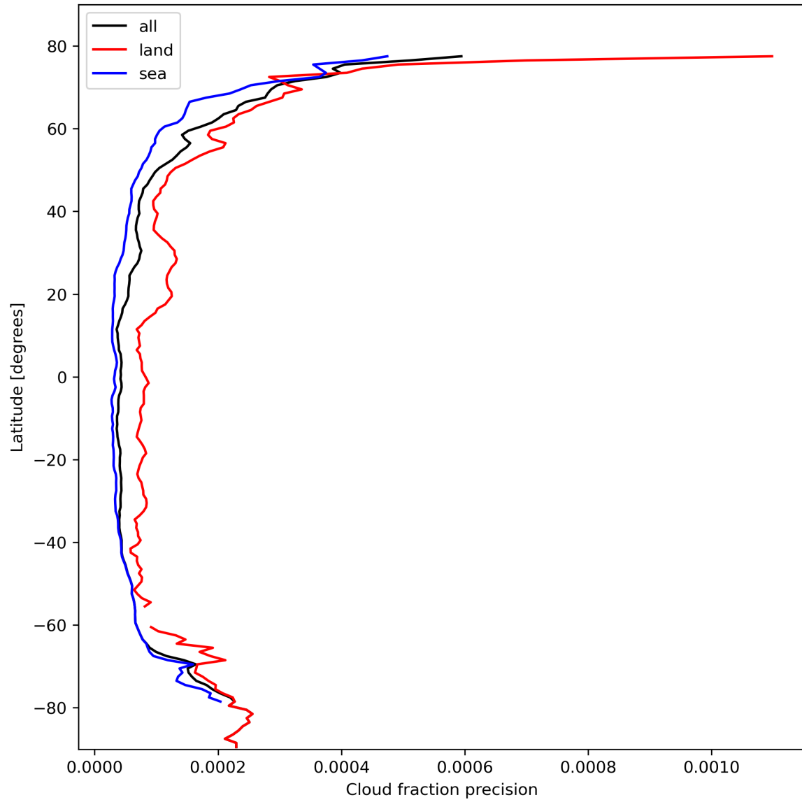
Figure 16: Zonal average of “Cloud fraction precision” for 2024-02-22 to 2024-02-23.
