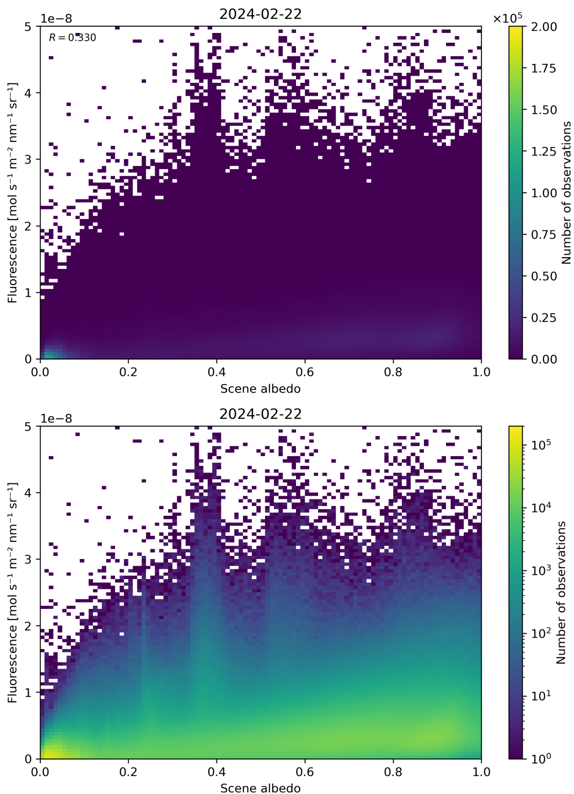
Figure 104: Scatter density plot of “Scene albedo” against “Fluorescence” for 2024-02-22 to 2024-02-23.
