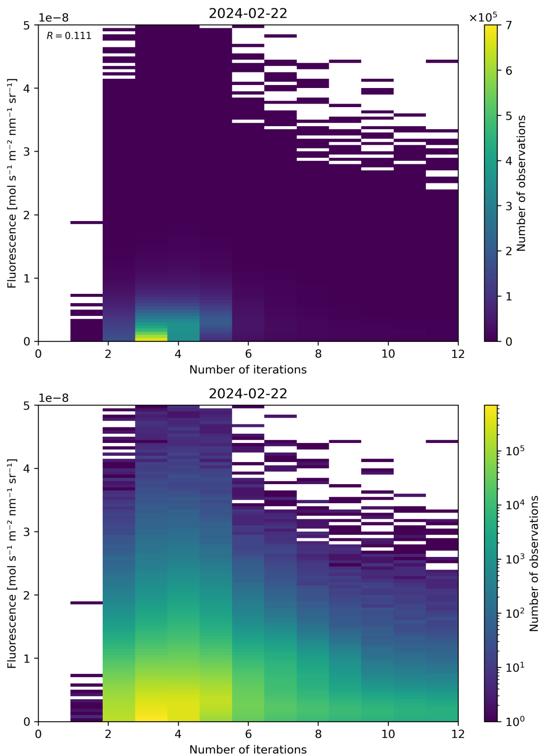
Figure 98: Scatter density plot of “Number of iterations” against “Fluorescence” for 2024-02-22 to 2024-02-23.
