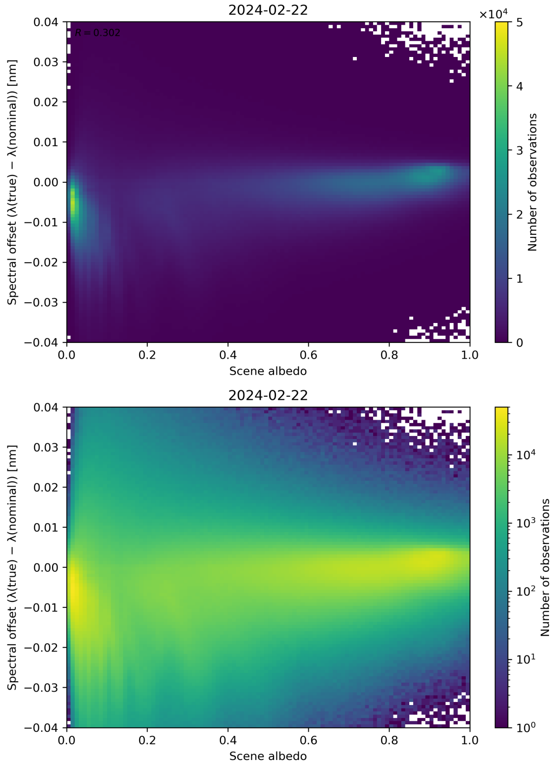
Figure 107: Scatter density plot of “Scene albedo” against “Spectral offset ( \lambda(\text{true}) - \lambda(\text{nominal}) )” for 2024-02-22 to 2024-02-23.
