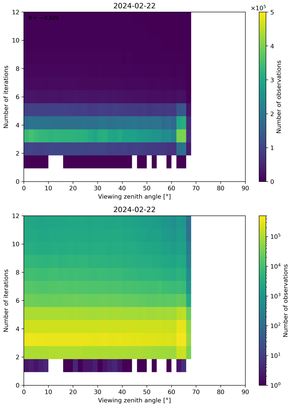
Figure 124: Scatter density plot of “Viewing zenith angle” against “Number of iterations” for 2024-02-22 to 2024-02-23.
