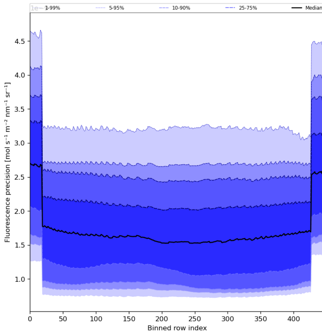
Figure 58: Along track statistics of “Fluorescence precision” for 2024-02-22 to 2024-02-23
