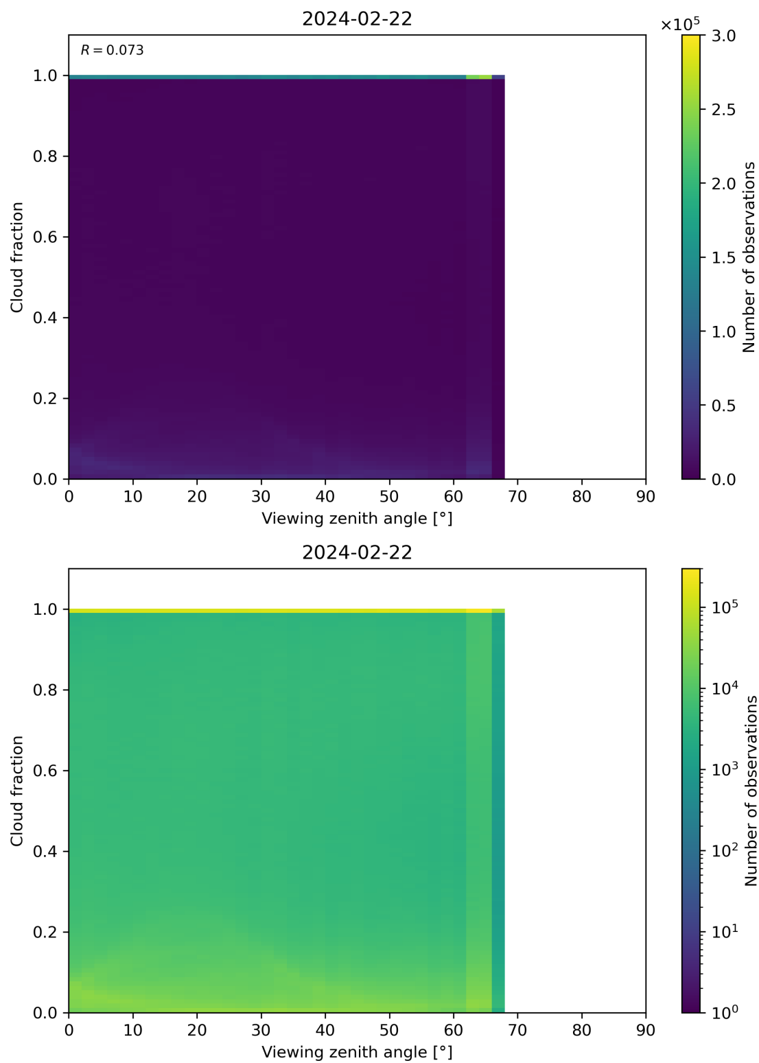
Figure 120: Scatter density plot of “Viewing zenith angle” against “Cloud fraction” for 2024-02-22 to 2024-02-23.
