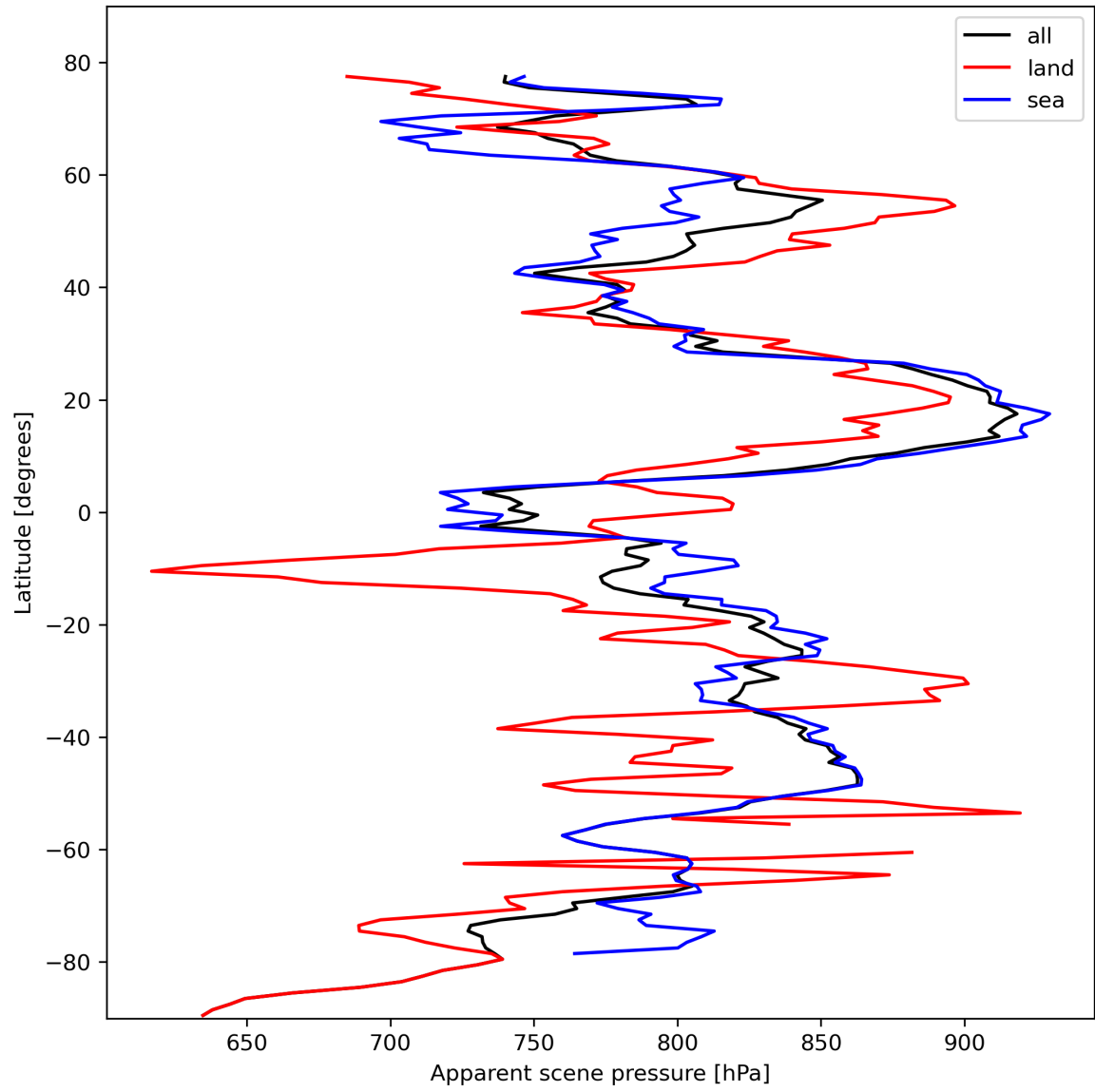
Figure 19: Zonal average of “Apparent scene pressure” for 2024-02-22 to 2024-02-23.
