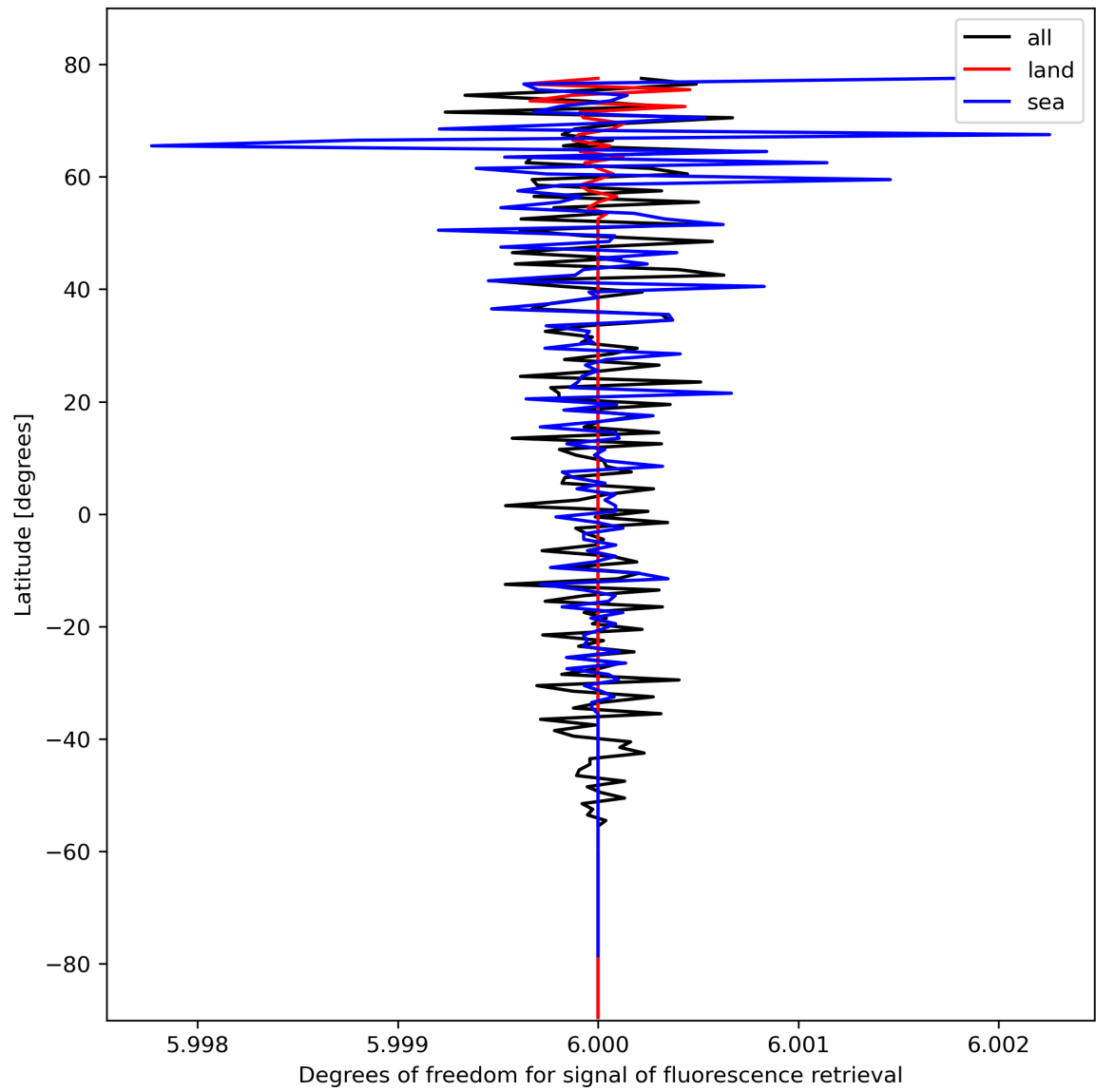
Figure 26: Zonal average of “Degrees of freedom for signal of fluorescence retrieval” for 2024-02-22 to 2024-02-23.
