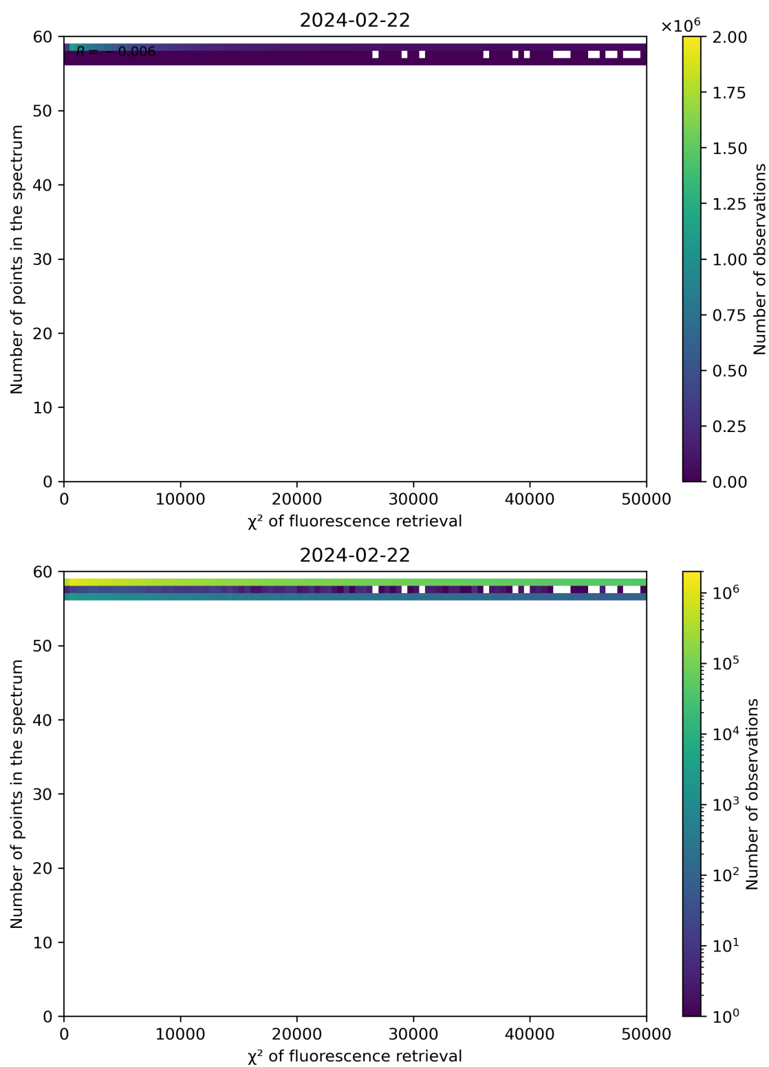
Figure 68: Scatter density plot of “ \chi^2 of fluorescence retrieval” against “Number of points in the spectrum” for 2024-02-22 to 2024-02-23.
