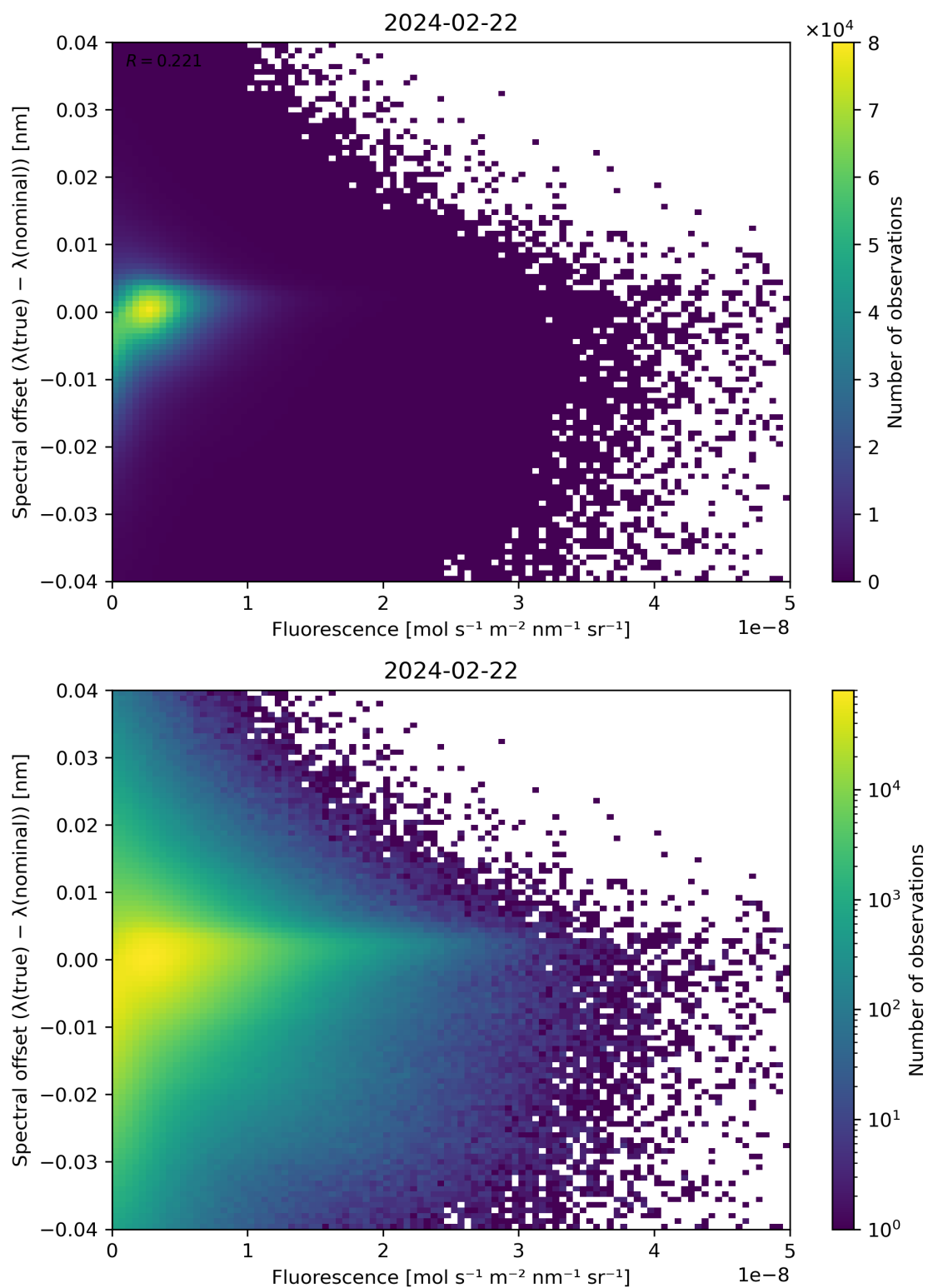
Figure 87: Scatter density plot of “Fluorescence” against “Spectral offset ( \lambda(\text{true}) - \lambda(\text{nominal}) )” for 2024-02-22 to 2024-02-23.
