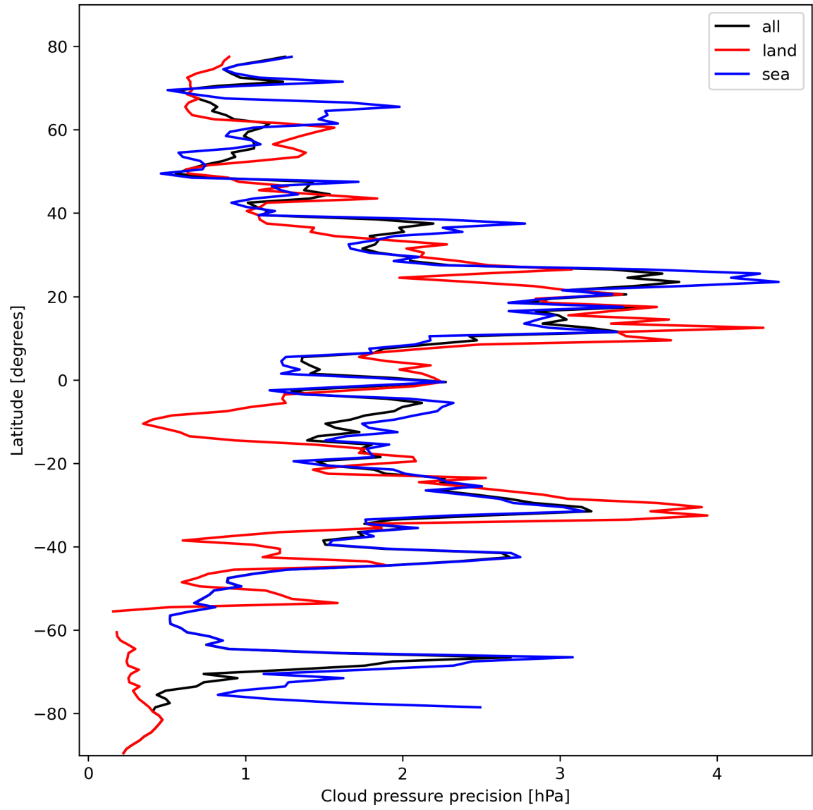
Figure 14: Zonal average of "Cloud pressure precision" for 2024-02-22 to 2024-02-23.
