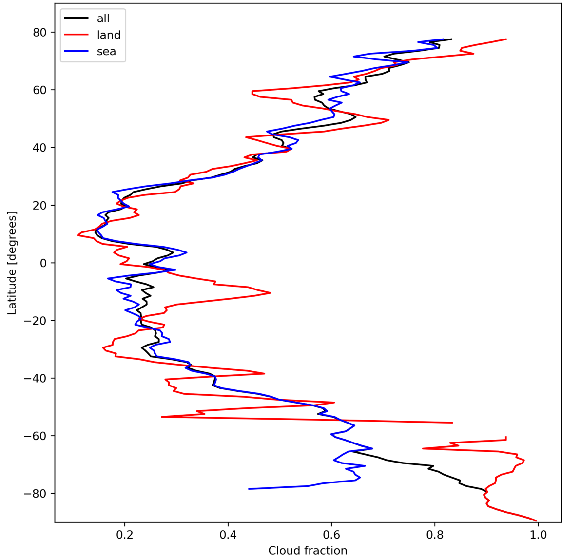
Figure 15: Zonal average of “Cloud fraction” for 2024-02-22 to 2024-02-23.
