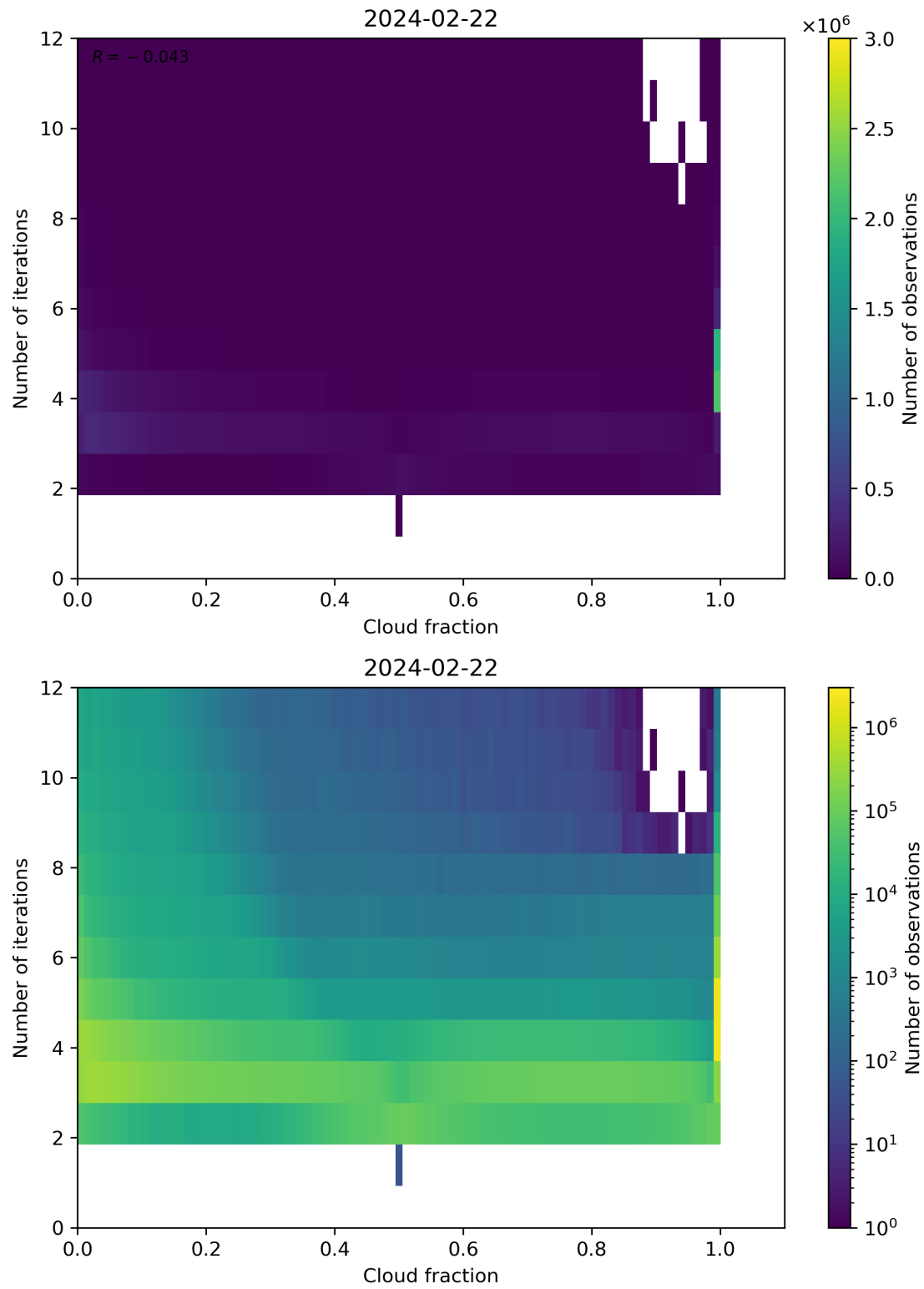
Figure 73: Scatter density plot of “Cloud fraction” against “Number of iterations” for 2024-02-22 to 2024-02-23.
