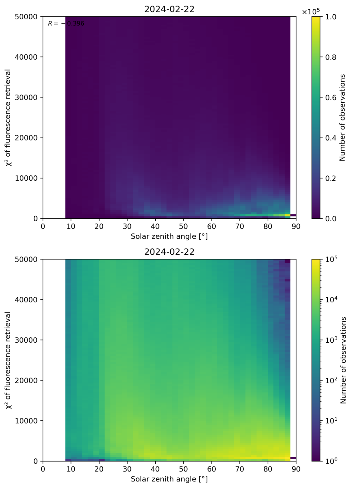
Figure 109: Scatter density plot of “Solar zenith angle” against “ \chi^2 of fluorescence retrieval” for 2024-02-22 to 2024-02-23.
