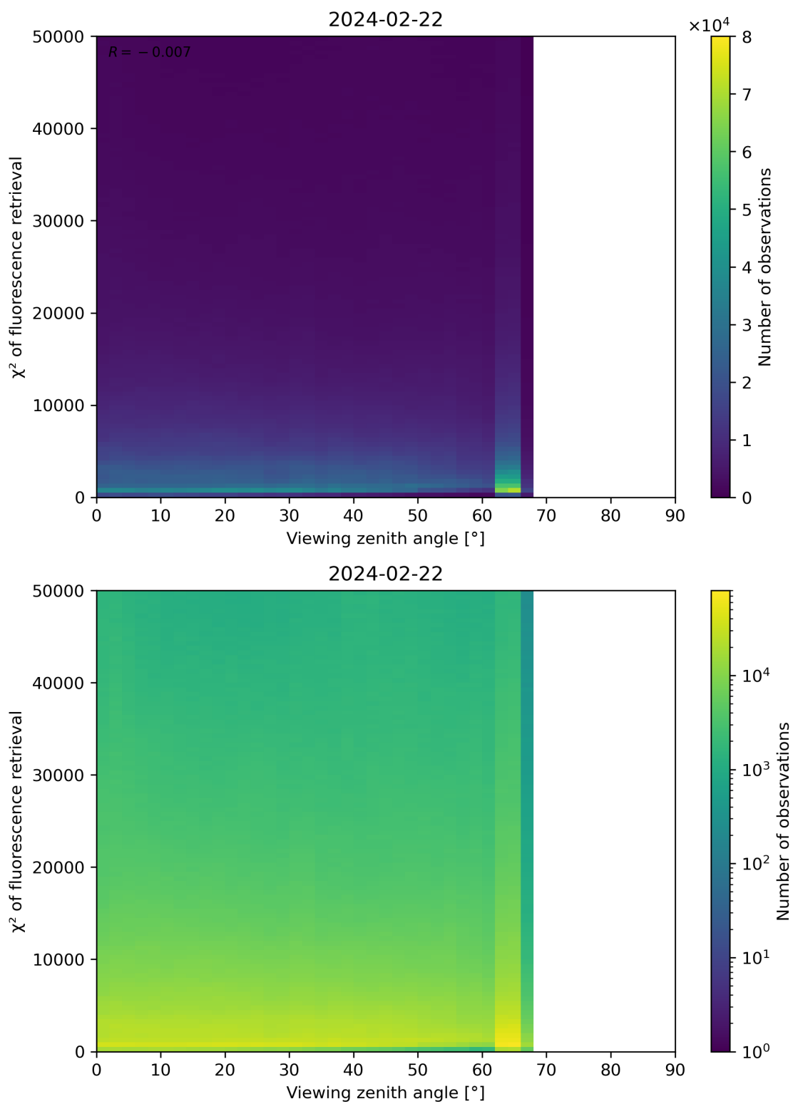
Figure 119: Scatter density plot of “Viewing zenith angle” against “ \chi^2 of fluorescence retrieval” for 2024-02-22 to 2024-02-23.
