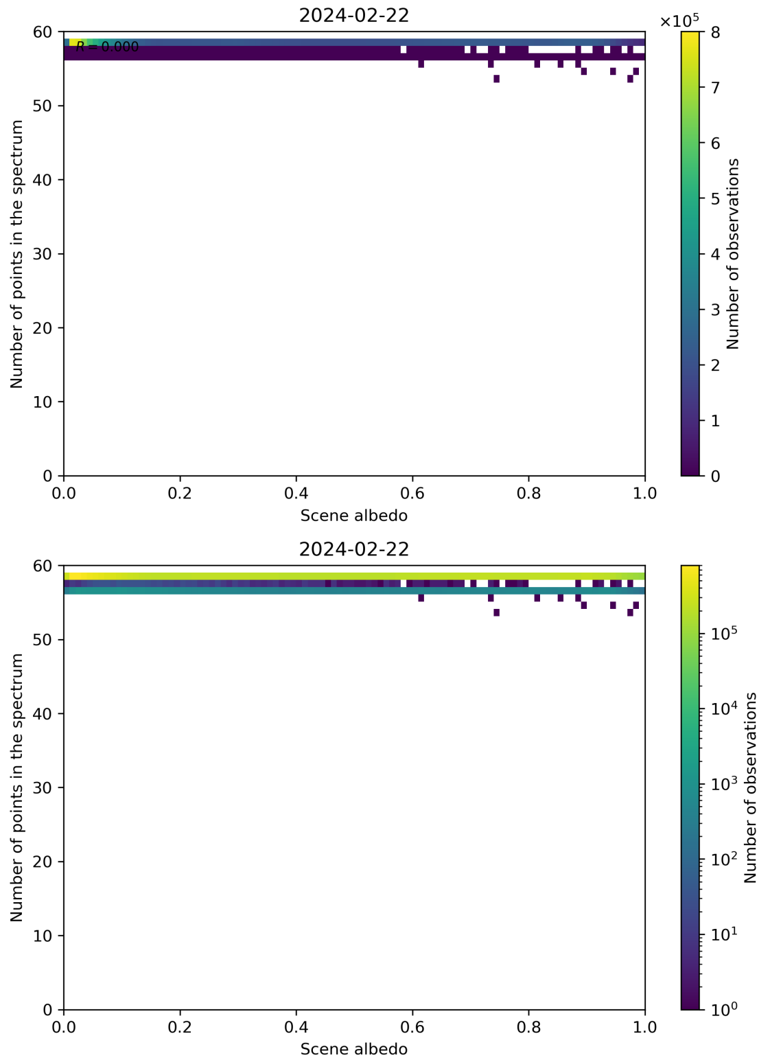
Figure 106: Scatter density plot of “Scene albedo” against “Number of points in the spectrum” for 2024-02-22 to 2024-02-23.
