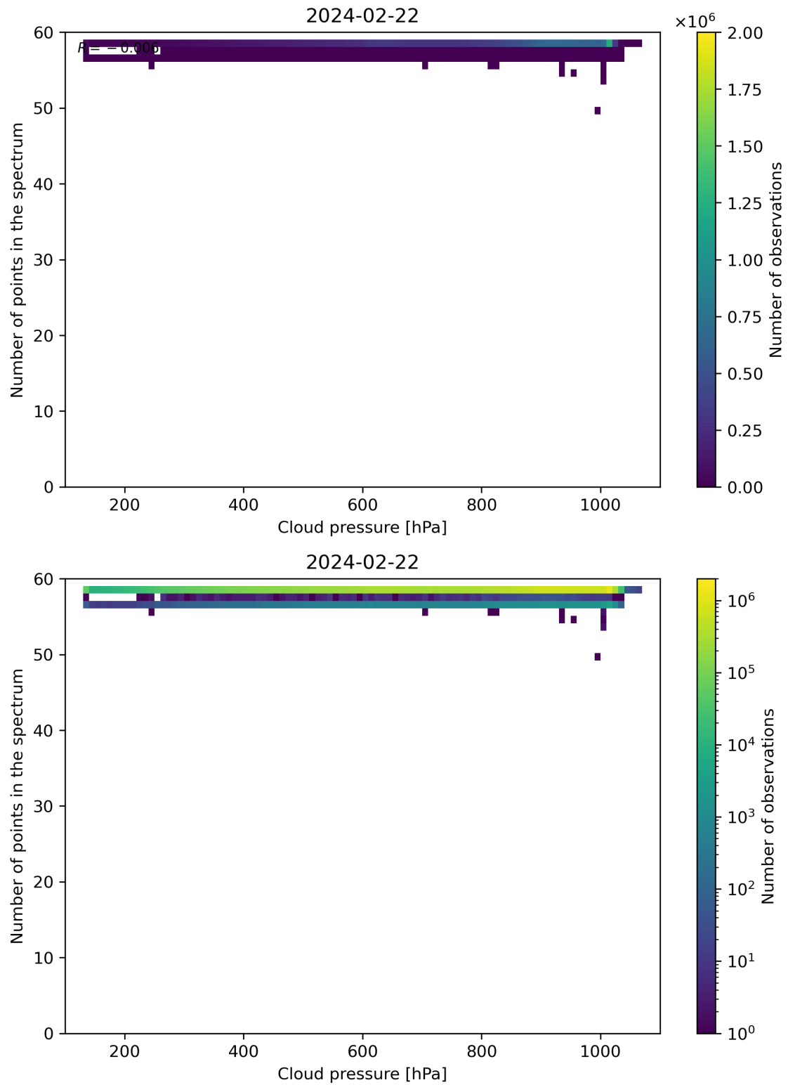
Figure 82: Scatter density plot of “Cloud pressure” against “Number of points in the spectrum” for 2024-02-22 to 2024-02-23.
