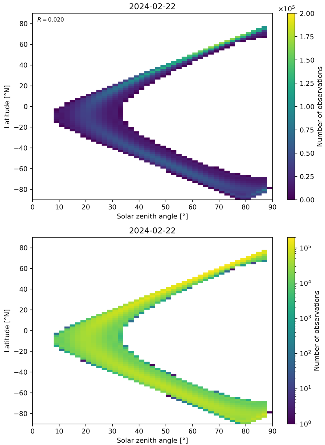
Figure 113: Scatter density plot of “Solar zenith angle” against “Latitude” for 2024-02-22 to 2024-02-23.
