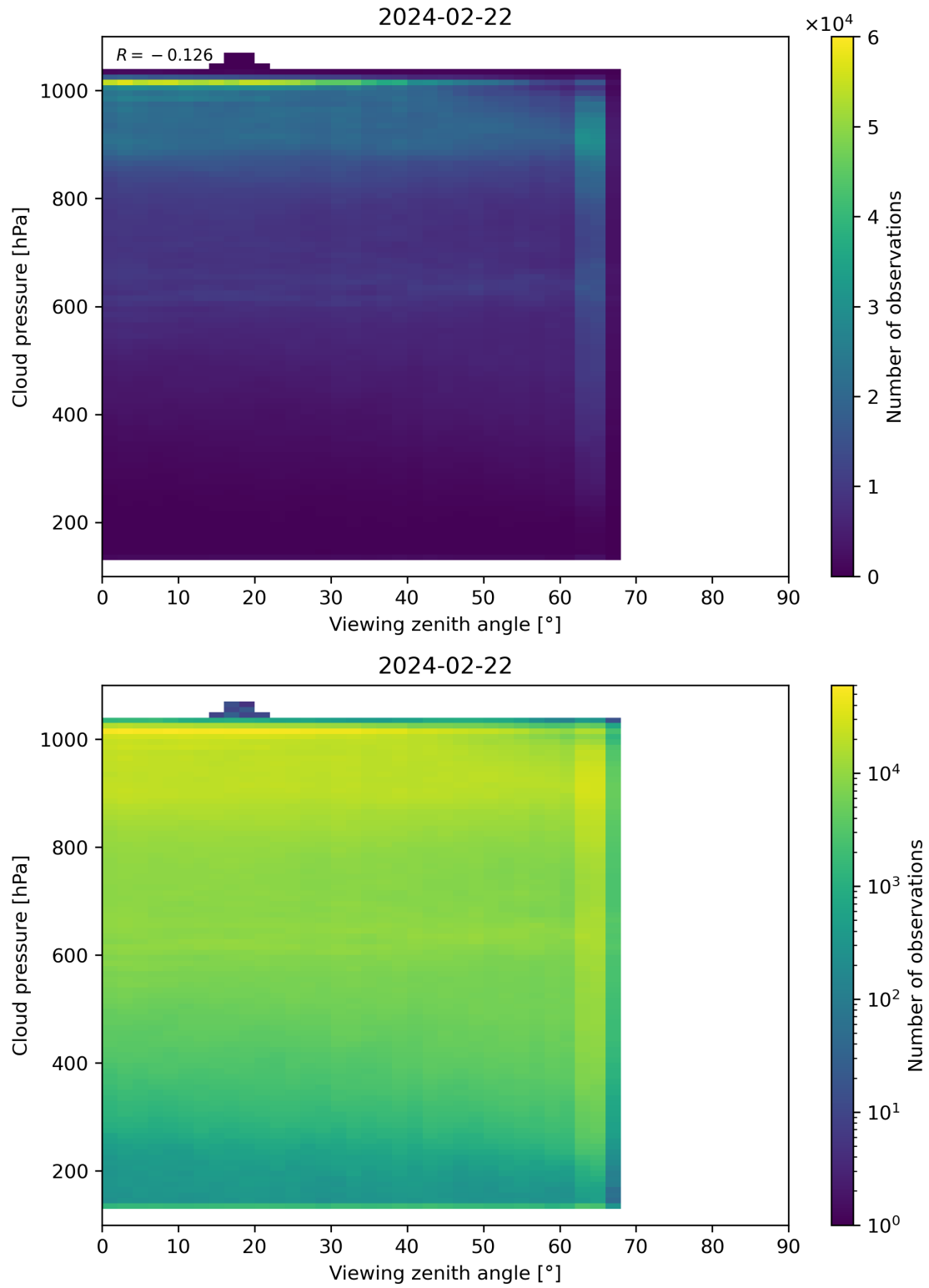
Figure 121: Scatter density plot of “Viewing zenith angle” against “Cloud pressure” for 2024-02-22 to 2024-02-23.
