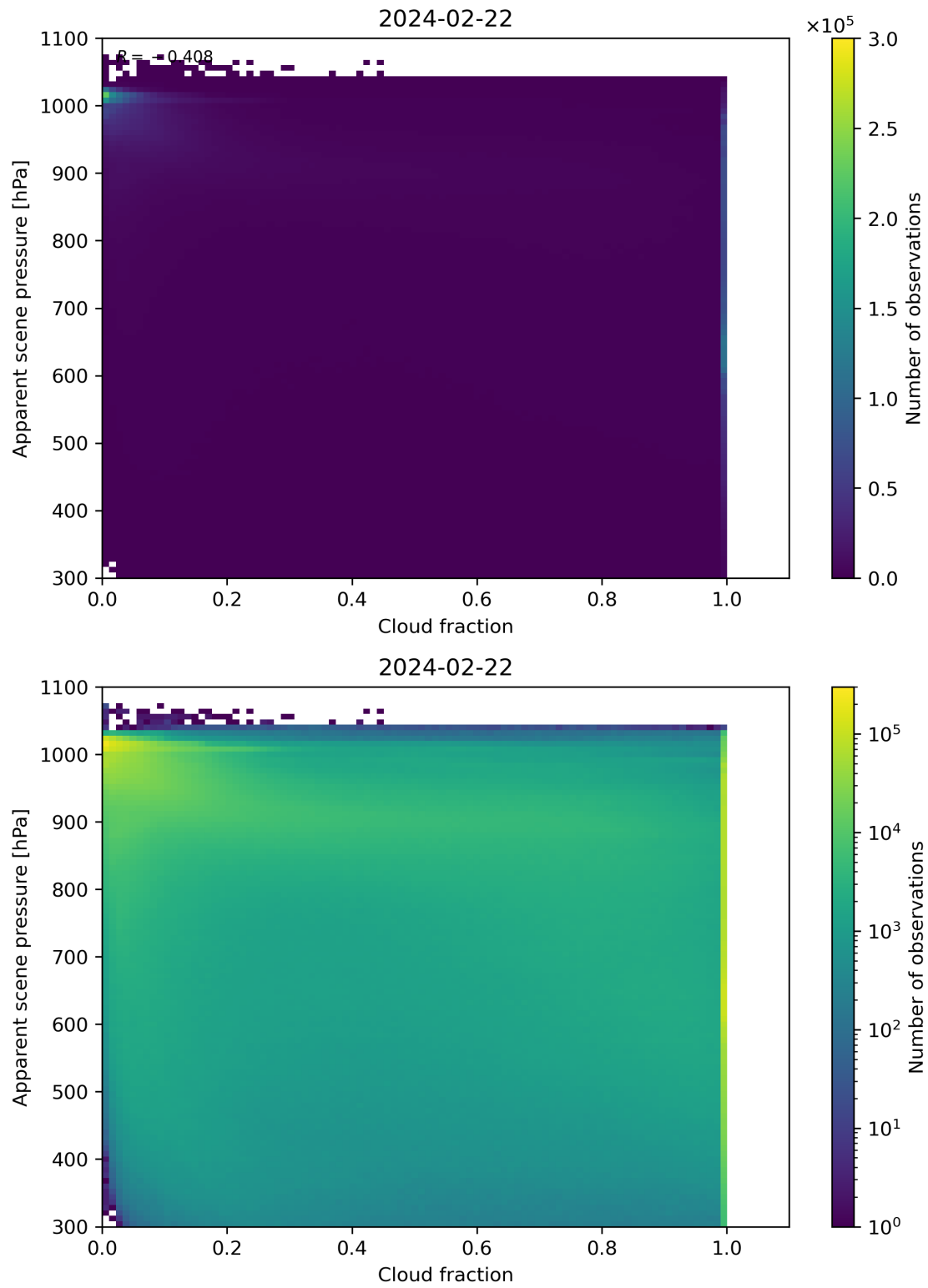
Figure 70: Scatter density plot of “Cloud fraction” against “Apparent scene pressure” for 2024-02-22 to 2024-02-23.
