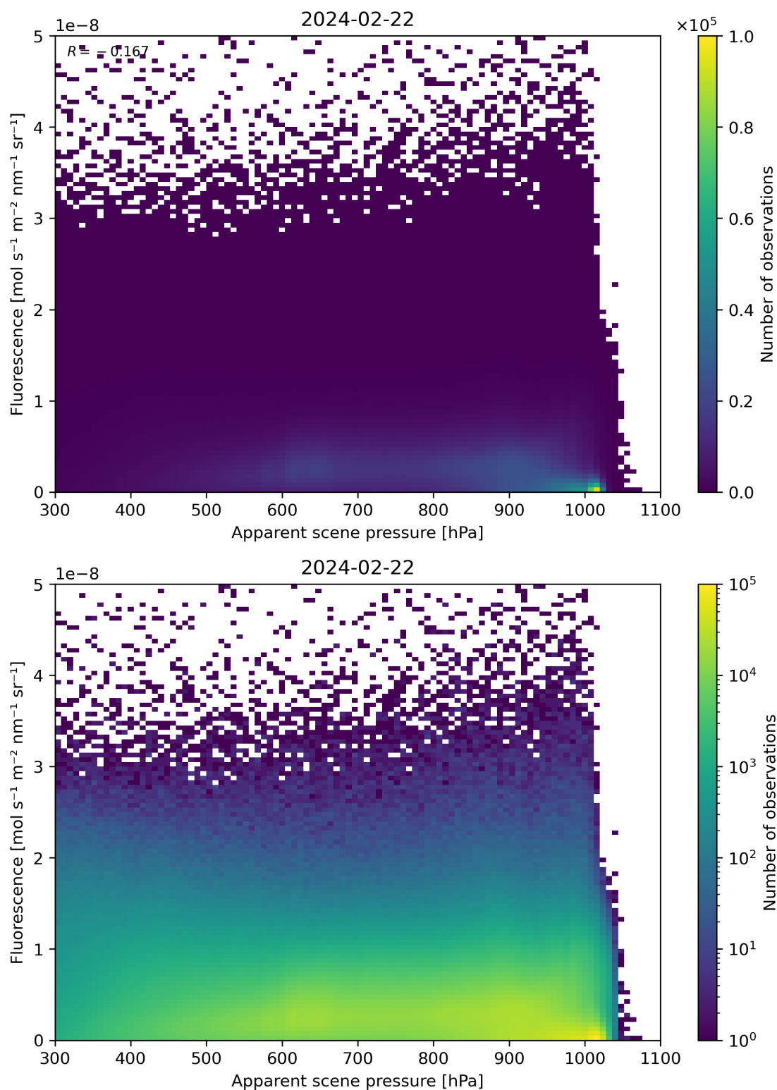
Figure 64: Scatter density plot of “Apparent scene pressure” against “Fluorescence” for 2024-02-22 to 2024-02-23.
