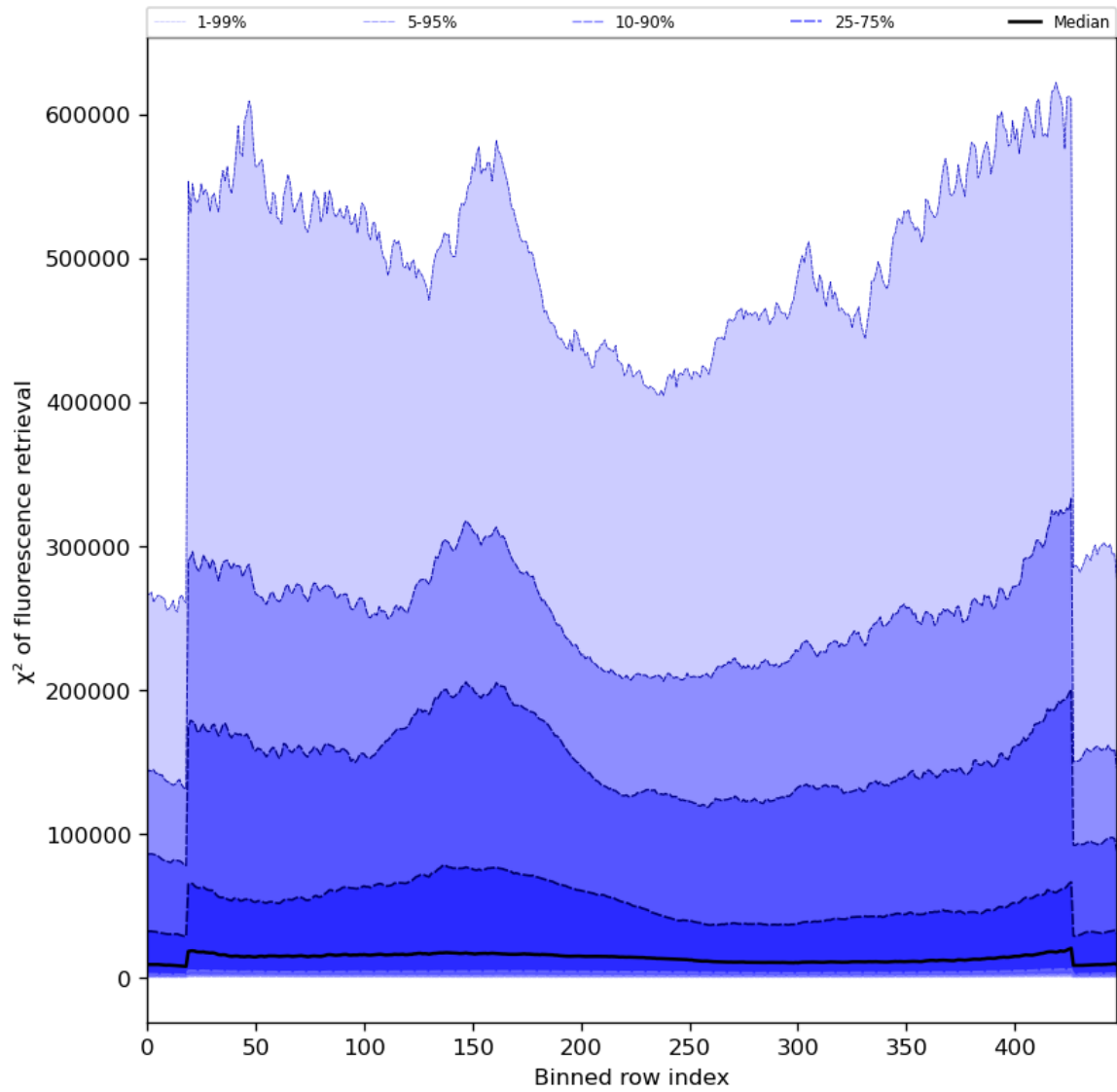
Figure 59: Along track statistics of “ \chi^2 of fluorescence retrieval” for 2024-02-22 to 2024-02-23
