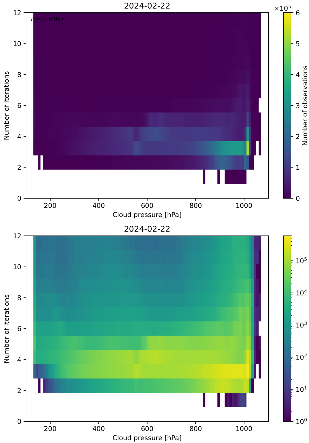
Figure 81: Scatter density plot of “Cloud pressure” against “Number of iterations” for 2024-02-22 to 2024-02-23.
