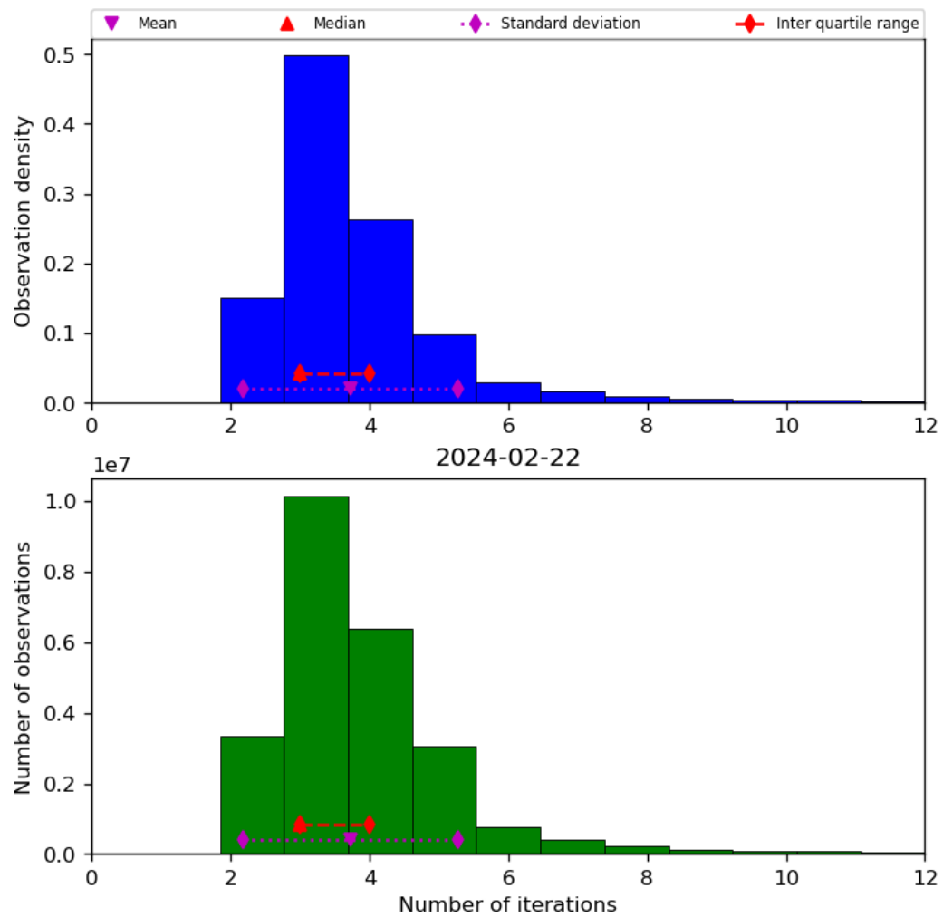
Figure 39: Histogram of “Number of iterations” for 2024-02-22 to 2024-02-23
