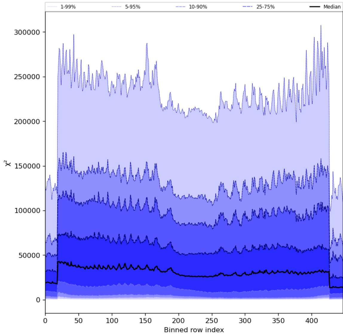
Figure 55: Along track statistics of “ \chi^2 ” for 2024-02-22 to 2024-02-23
