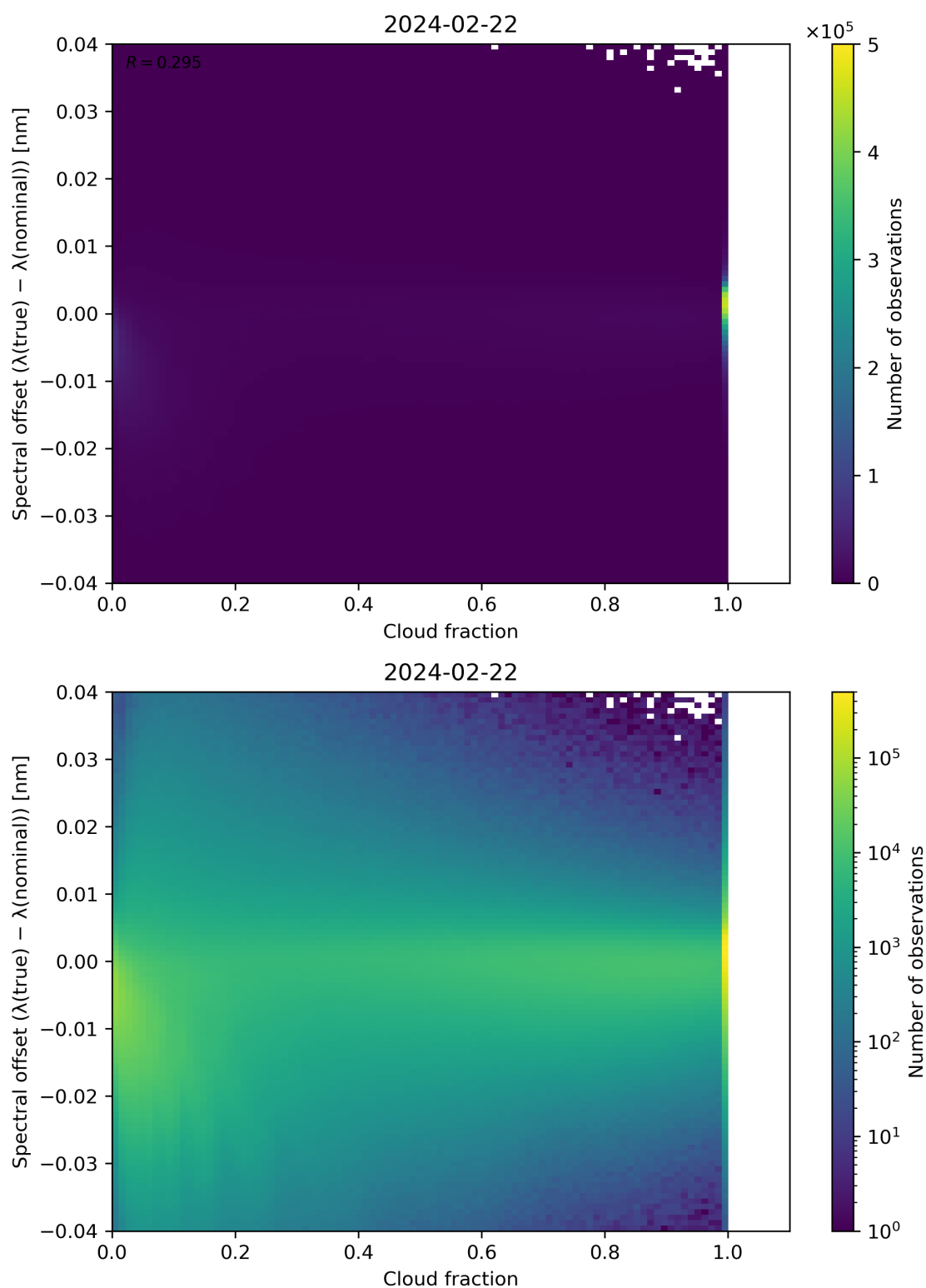
Figure 76: Scatter density plot of “Cloud fraction” against “Spectral offset ( \lambda(\text{true}) - \lambda(\text{nominal}) )” for 2024-02-22 to 2024-02-23.
