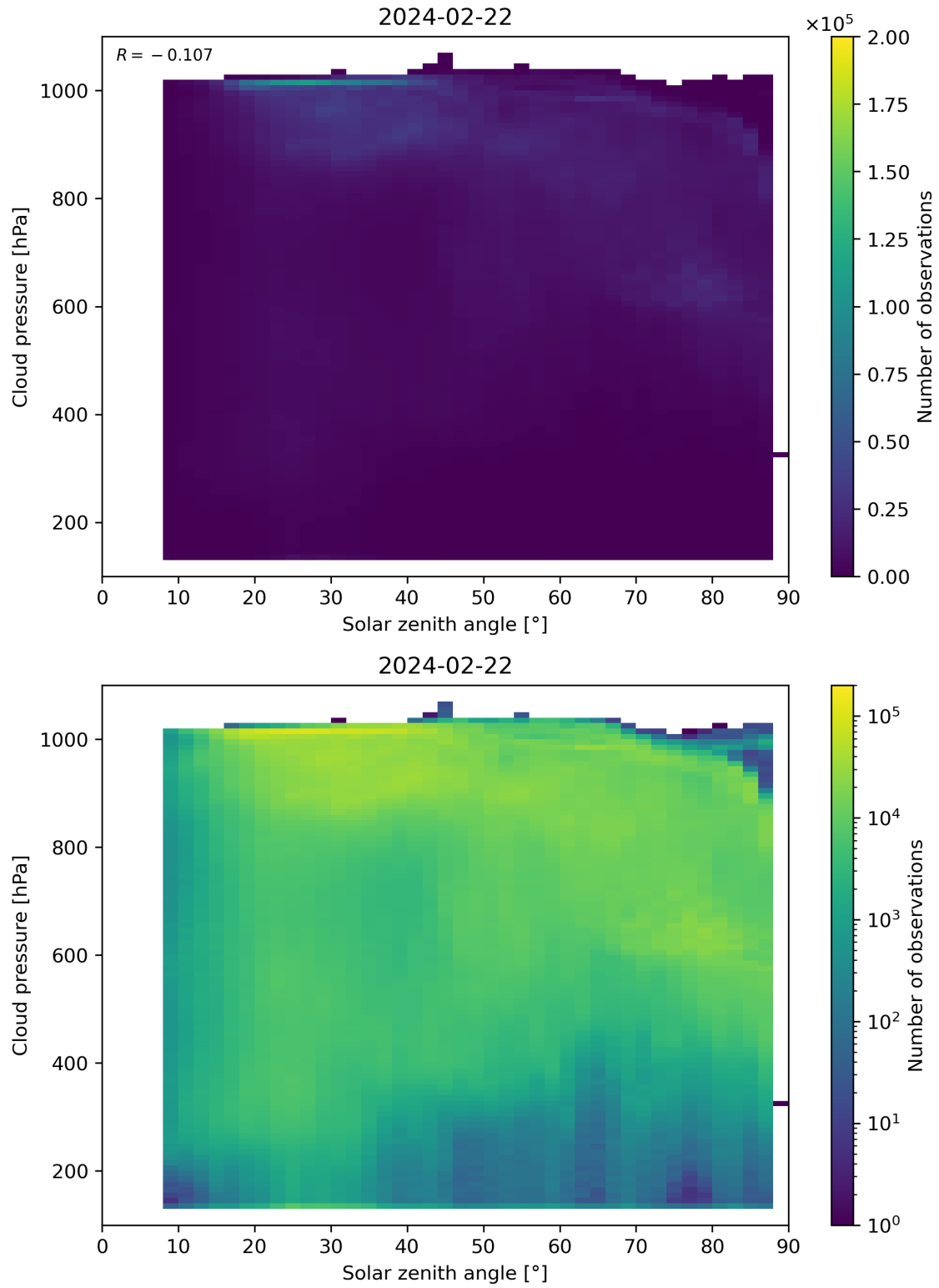
Figure 111: Scatter density plot of “Solar zenith angle” against “Cloud pressure” for 2024-02-22 to 2024-02-23.
