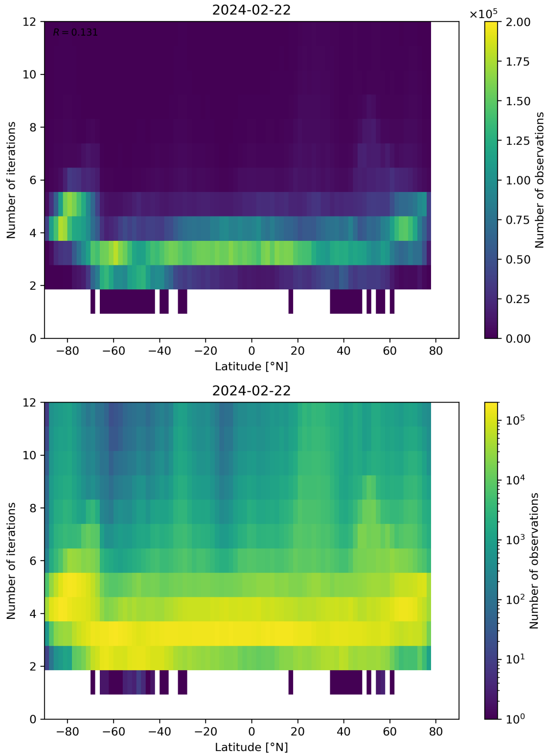
Figure 93: Scatter density plot of “Latitude” against “Number of iterations” for 2024-02-22 to 2024-02-23.
