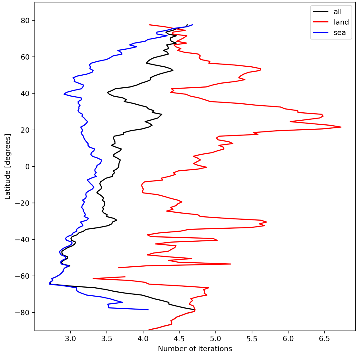
Figure 22: Zonal average of “Number of iterations” for 2024-02-22 to 2024-02-23.
