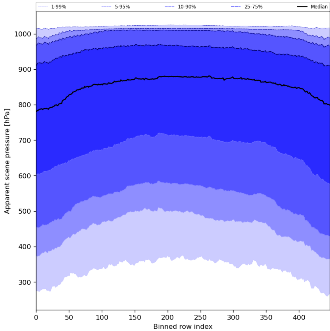
Figure 53: Along track statistics of “Apparent scene pressure” for 2024-02-22 to 2024-02-23
