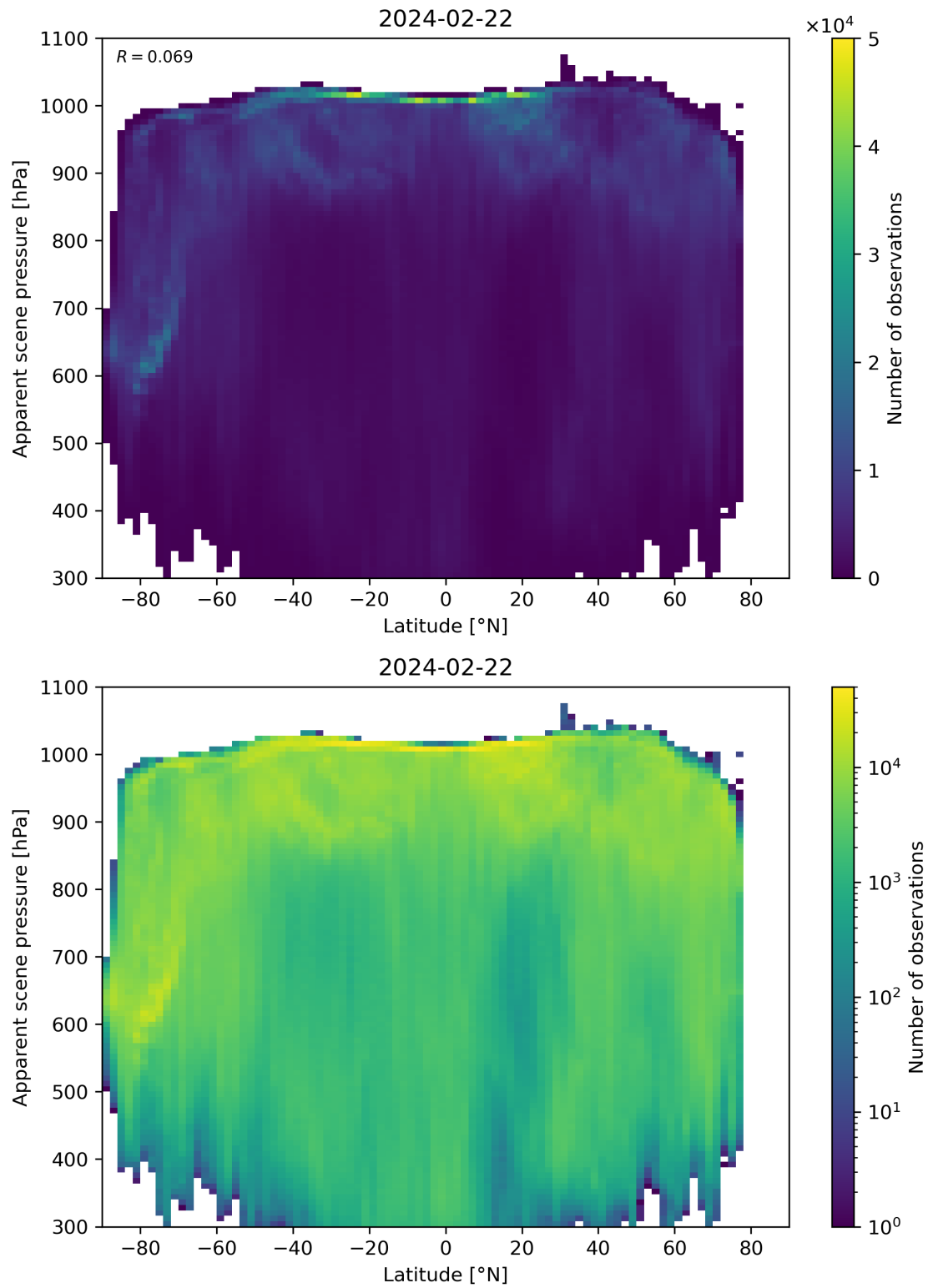
Figure 88: Scatter density plot of “Latitude” against “Apparent scene pressure” for 2024-02-22 to 2024-02-23.
