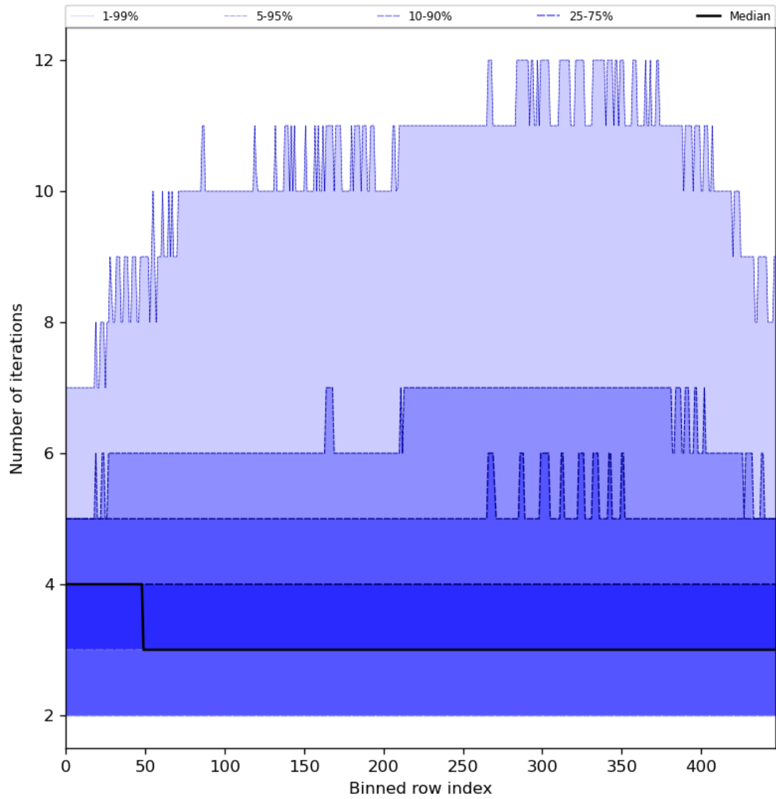
Figure 56: Along track statistics of “Number of iterations” for 2024-02-22 to 2024-02-23
