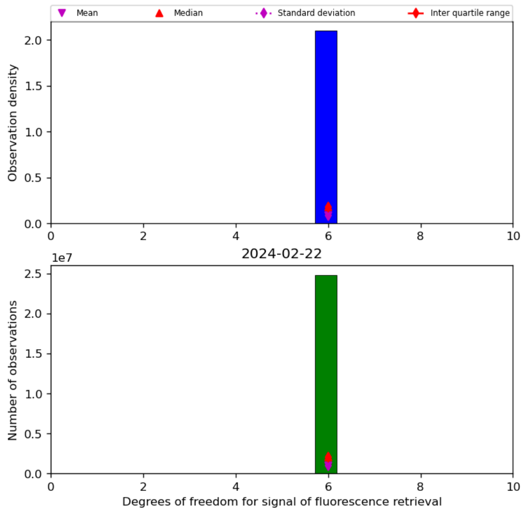
Figure 43: Histogram of “Degrees of freedom for signal of fluorescence retrieval” for 2024-02-22 to 2024-02-23
