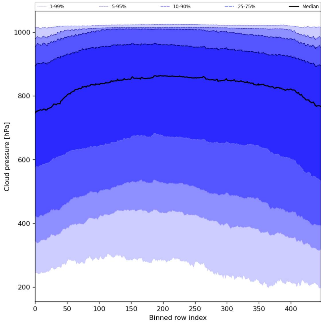
Figure 47: Along track statistics of “Cloud pressure” for 2024-02-22 to 2024-02-23
