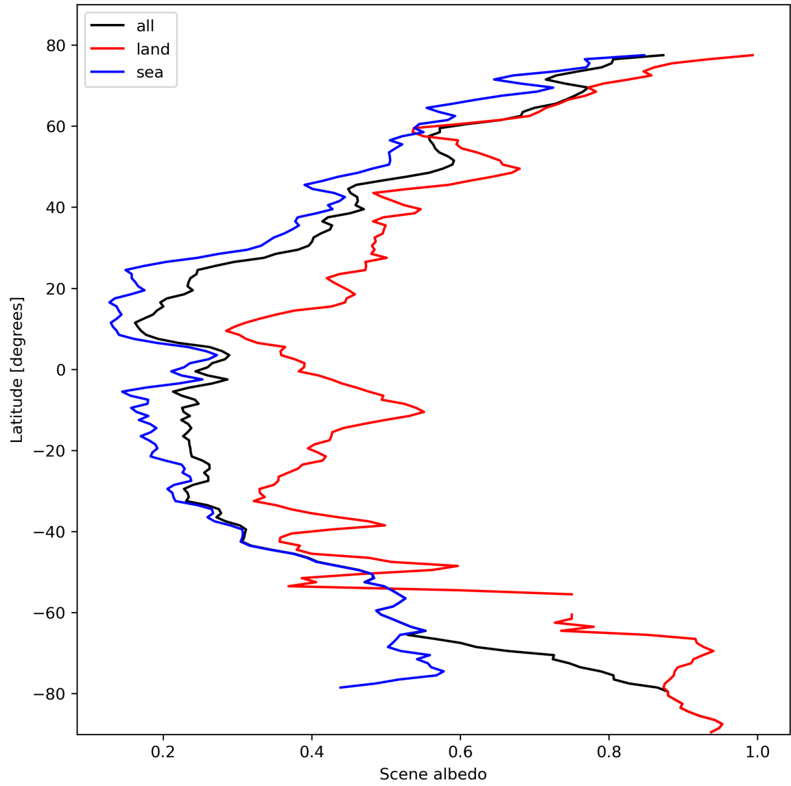
Figure 17: Zonal average of “Scene albedo” for 2024-02-22 to 2024-02-23.
