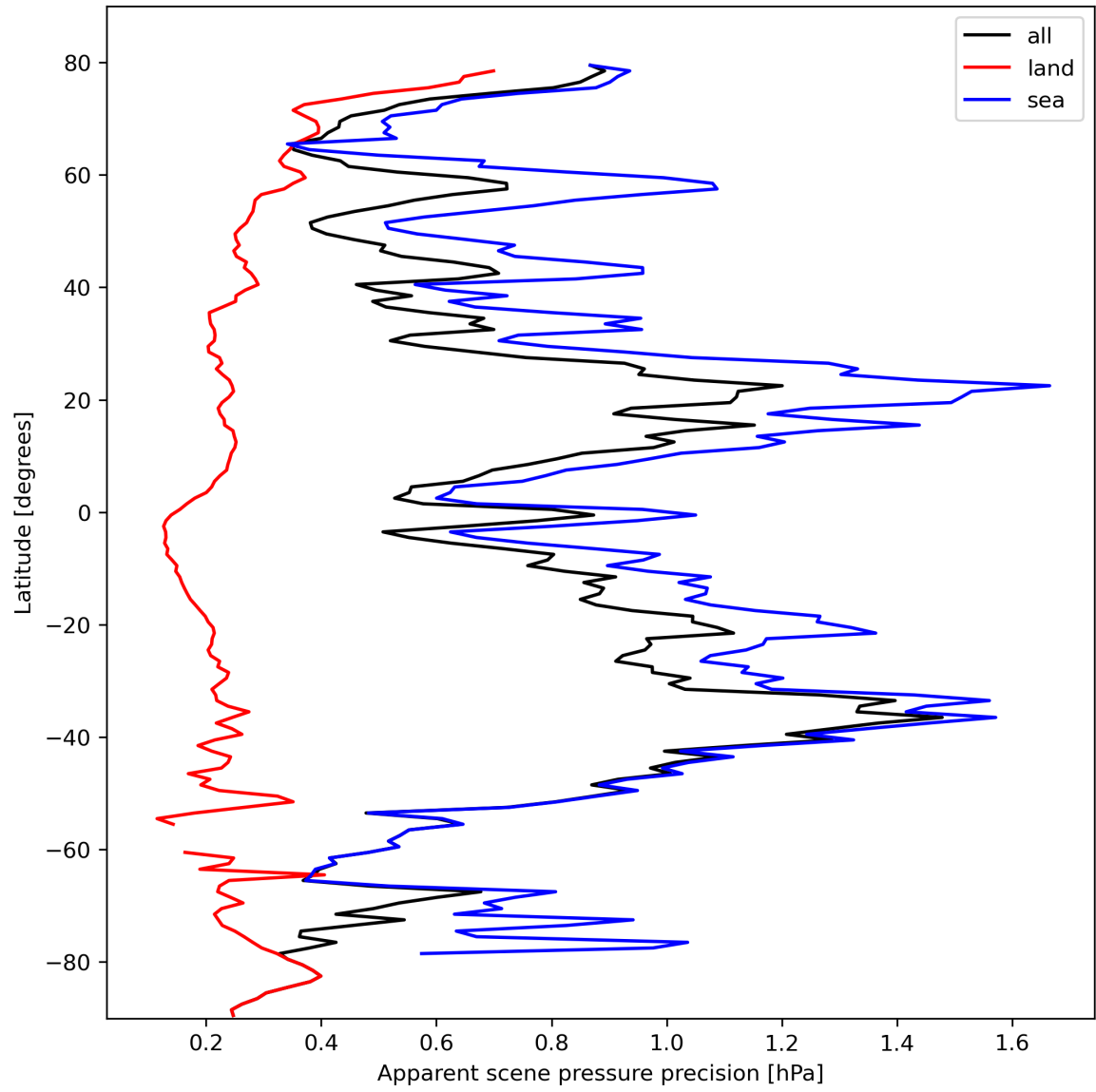
Figure 20: Zonal average of “Apparent scene pressure precision” for 2024-02-24 to 2024-02-26.
