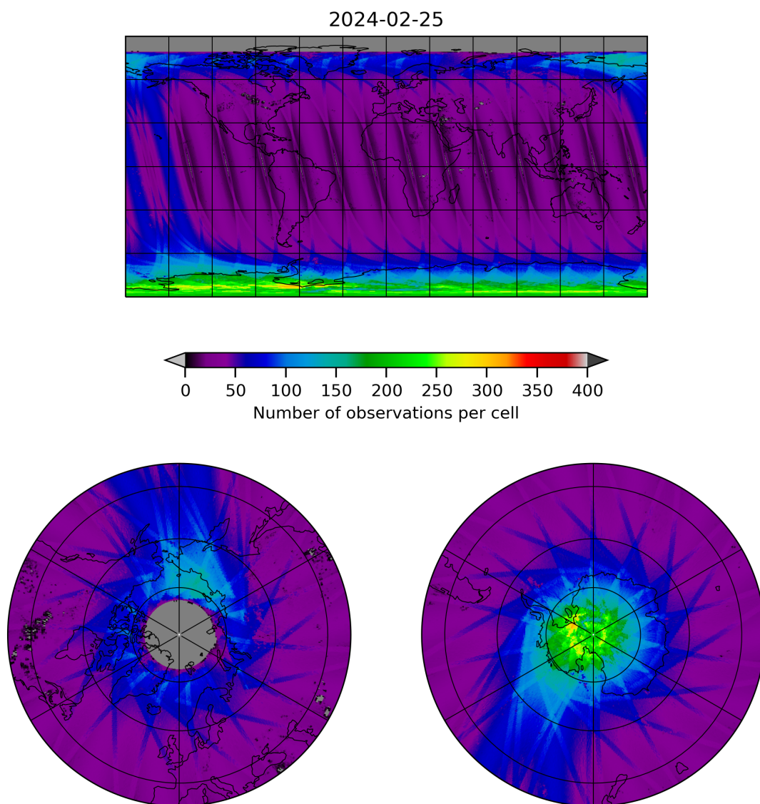
Figure 11: Map of the number of observations for 2024-02-24 to 2024-02-26
