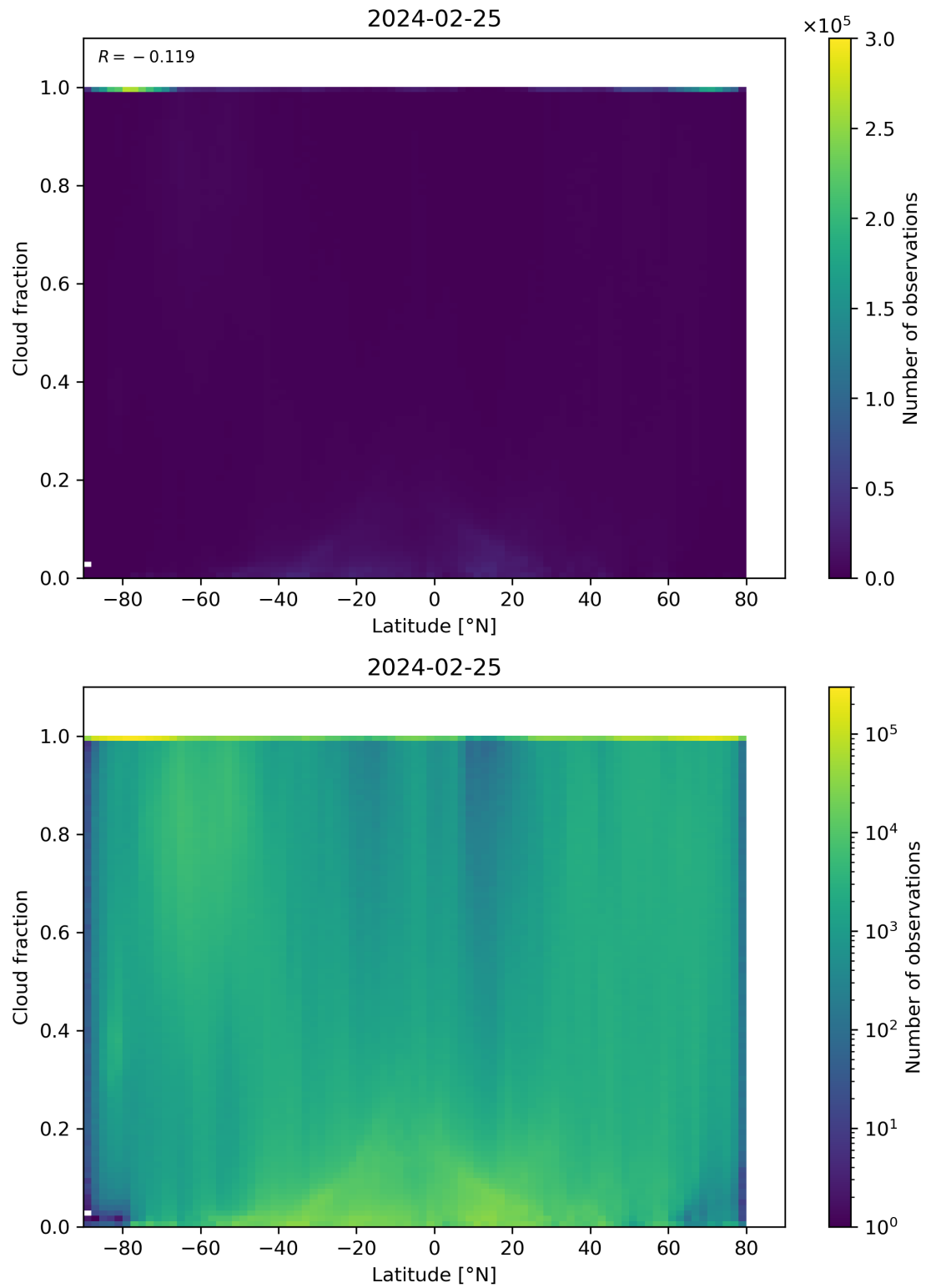
Figure 90: Scatter density plot of “Latitude” against “Cloud fraction” for 2024-02-24 to 2024-02-26.
