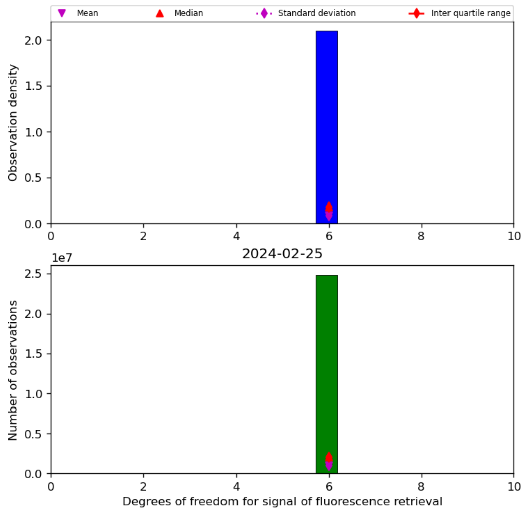
Figure 43: Histogram of “Degrees of freedom for signal of fluorescence retrieval” for 2024-02-24 to 2024-02-26
