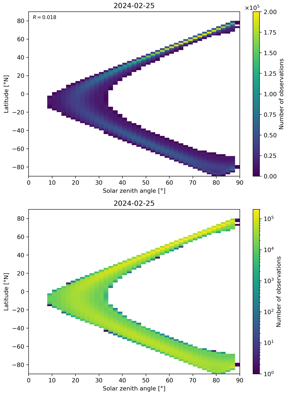
Figure 113: Scatter density plot of “Solar zenith angle” against “Latitude” for 2024-02-24 to 2024-02-26.
