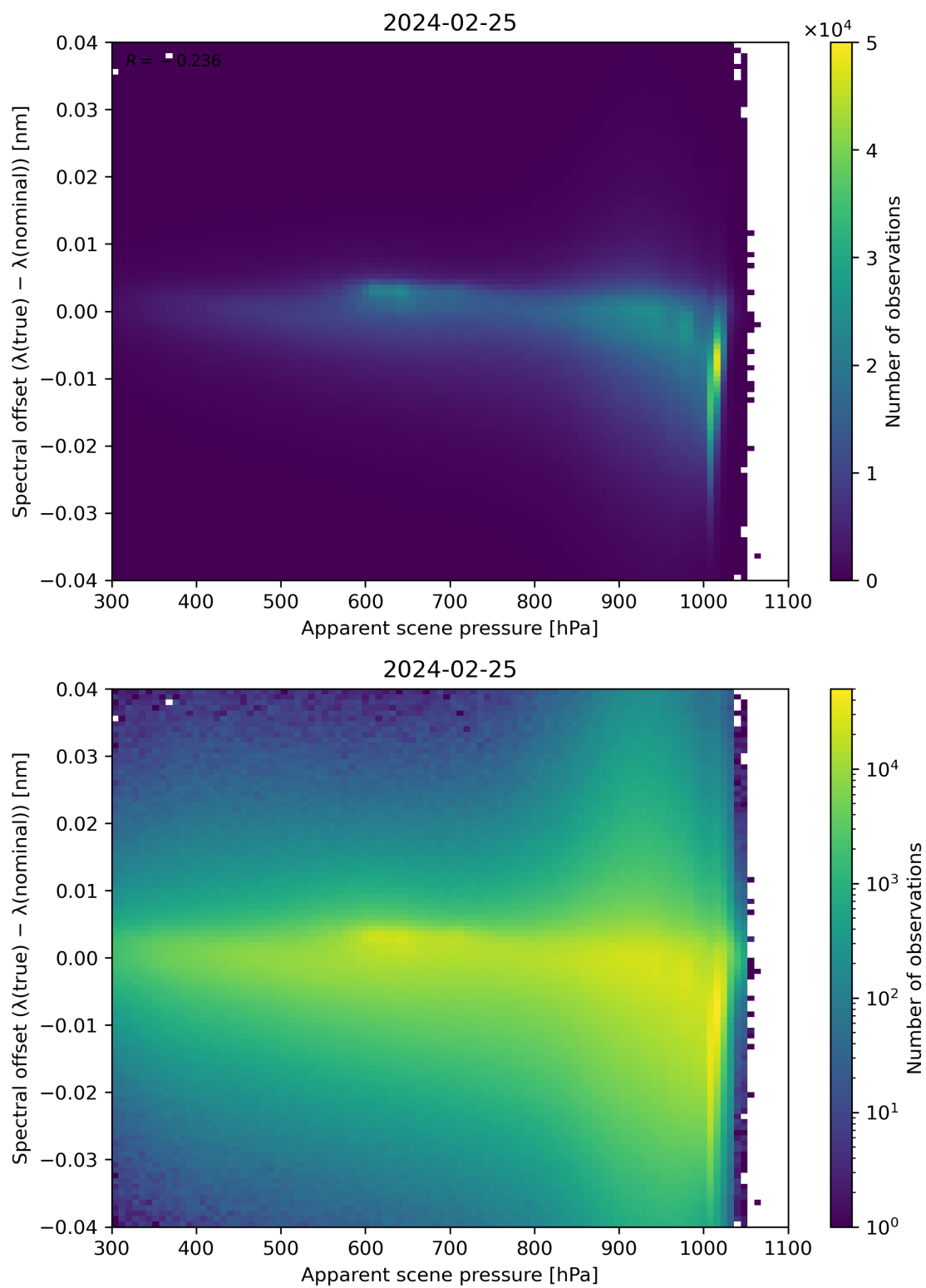
Figure 67: Scatter density plot of “Apparent scene pressure” against “Spectral offset ( \lambda(\text{true}) - \lambda(\text{nominal}) )” for 2024-02-24 to 2024-02-26.
