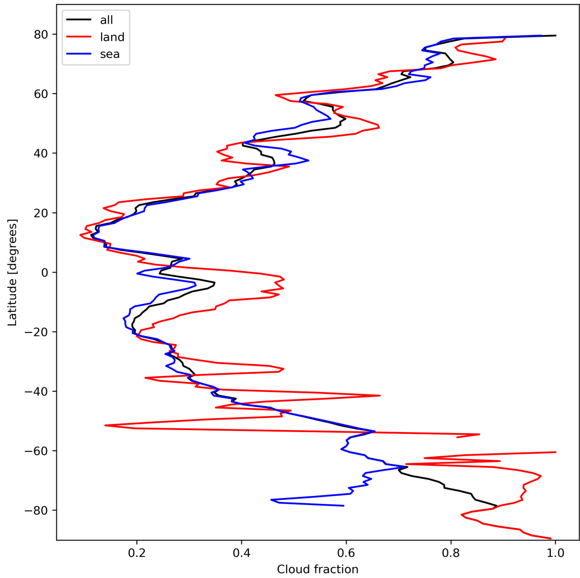
Figure 15: Zonal average of “Cloud fraction” for 2024-02-24 to 2024-02-26.
