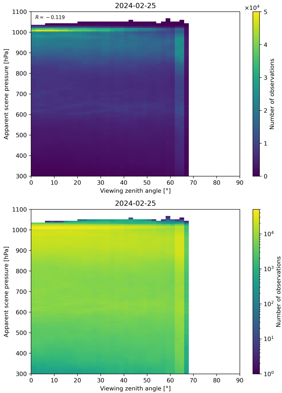
Figure 118: Scatter density plot of “Viewing zenith angle” against “Apparent scene pressure” for 2024-02-24 to 2024-02-26.
