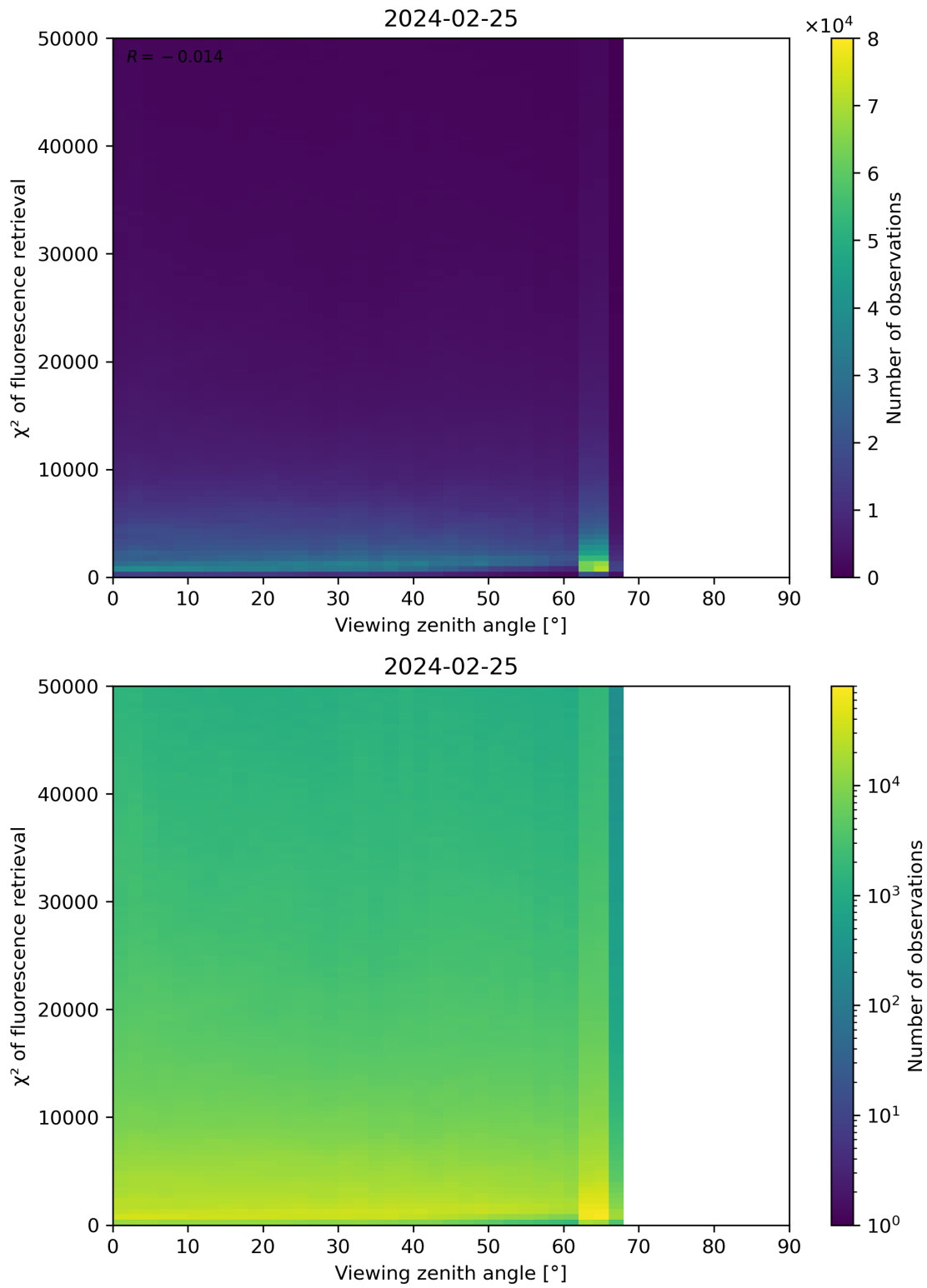
Figure 119: Scatter density plot of “Viewing zenith angle” against “ \chi^2 of fluorescence retrieval” for 2024-02-24 to 2024-02-26.
