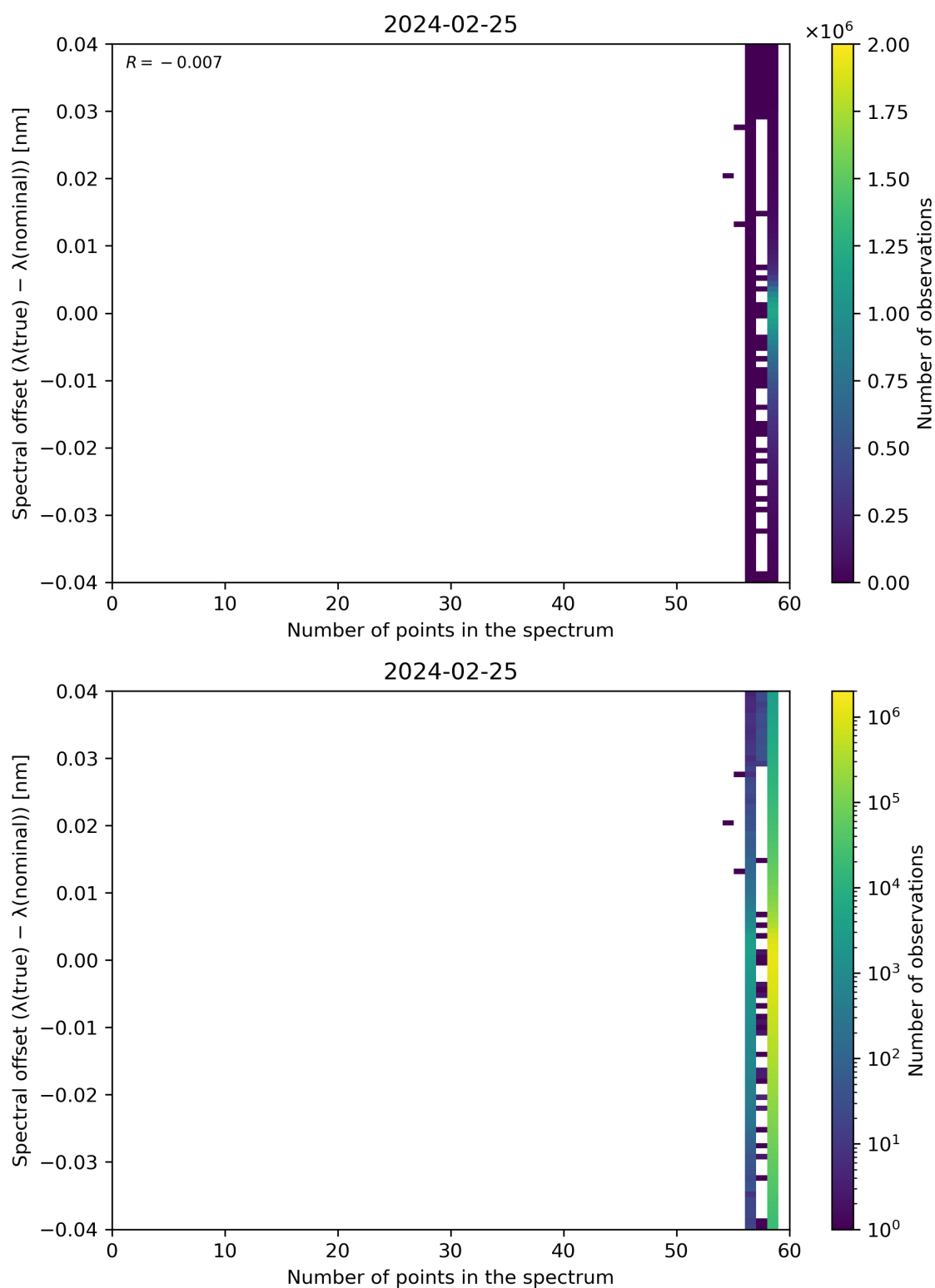
Figure 101: Scatter density plot of “Number of points in the spectrum” against “Spectral offset ( \lambda(\text{true}) - \lambda(\text{nominal}) )” for 2024-02-24 to 2024-02-26.
