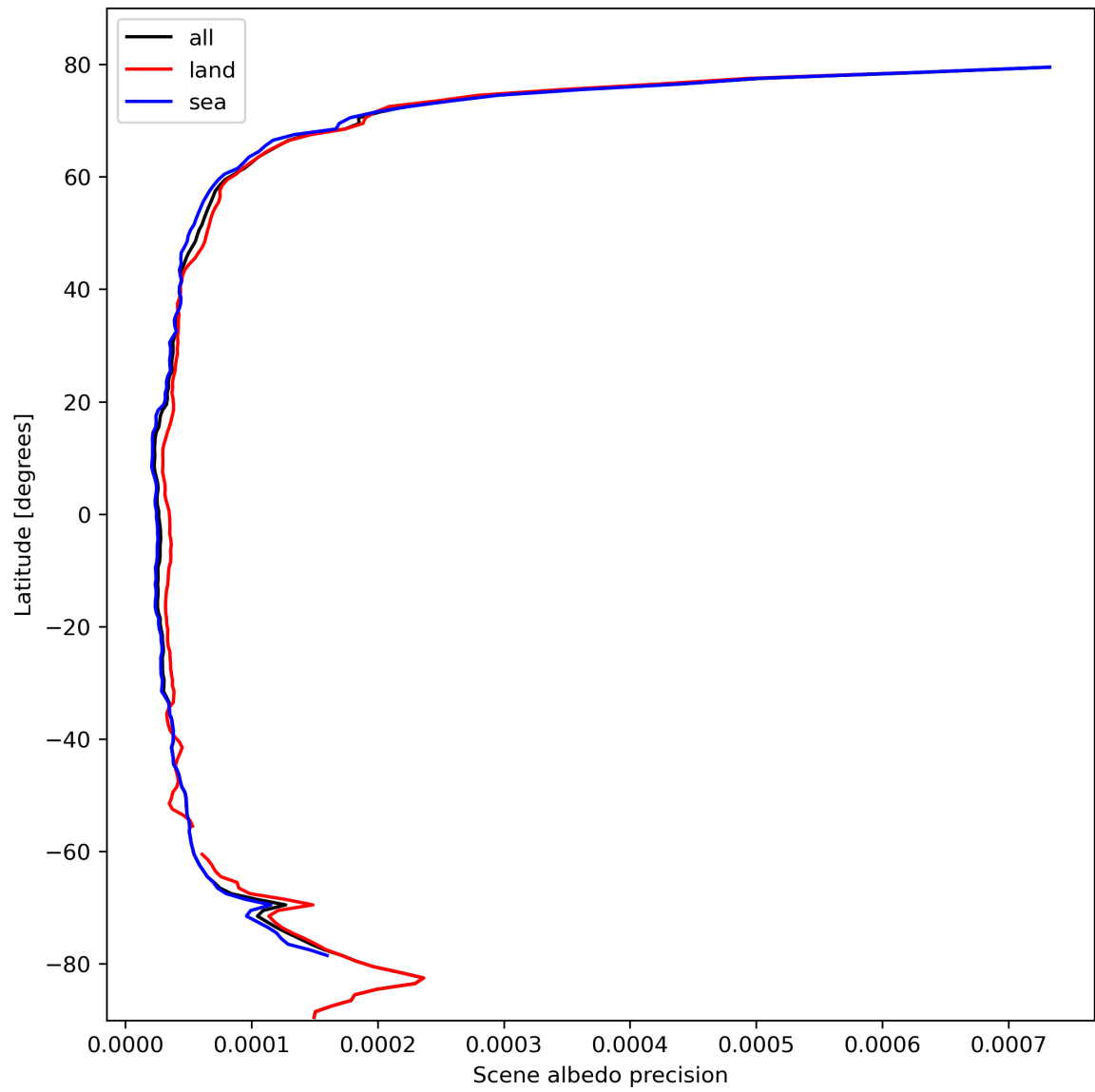
Figure 18: Zonal average of “Scene albedo precision” for 2024-02-24 to 2024-02-26.
