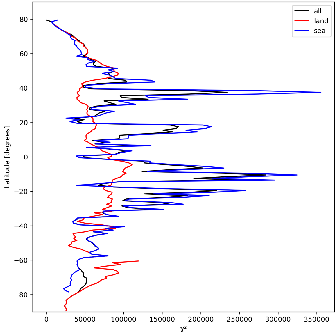
Figure 21: Zonal average of “ \chi^2 ” for 2024-02-24 to 2024-02-26.
