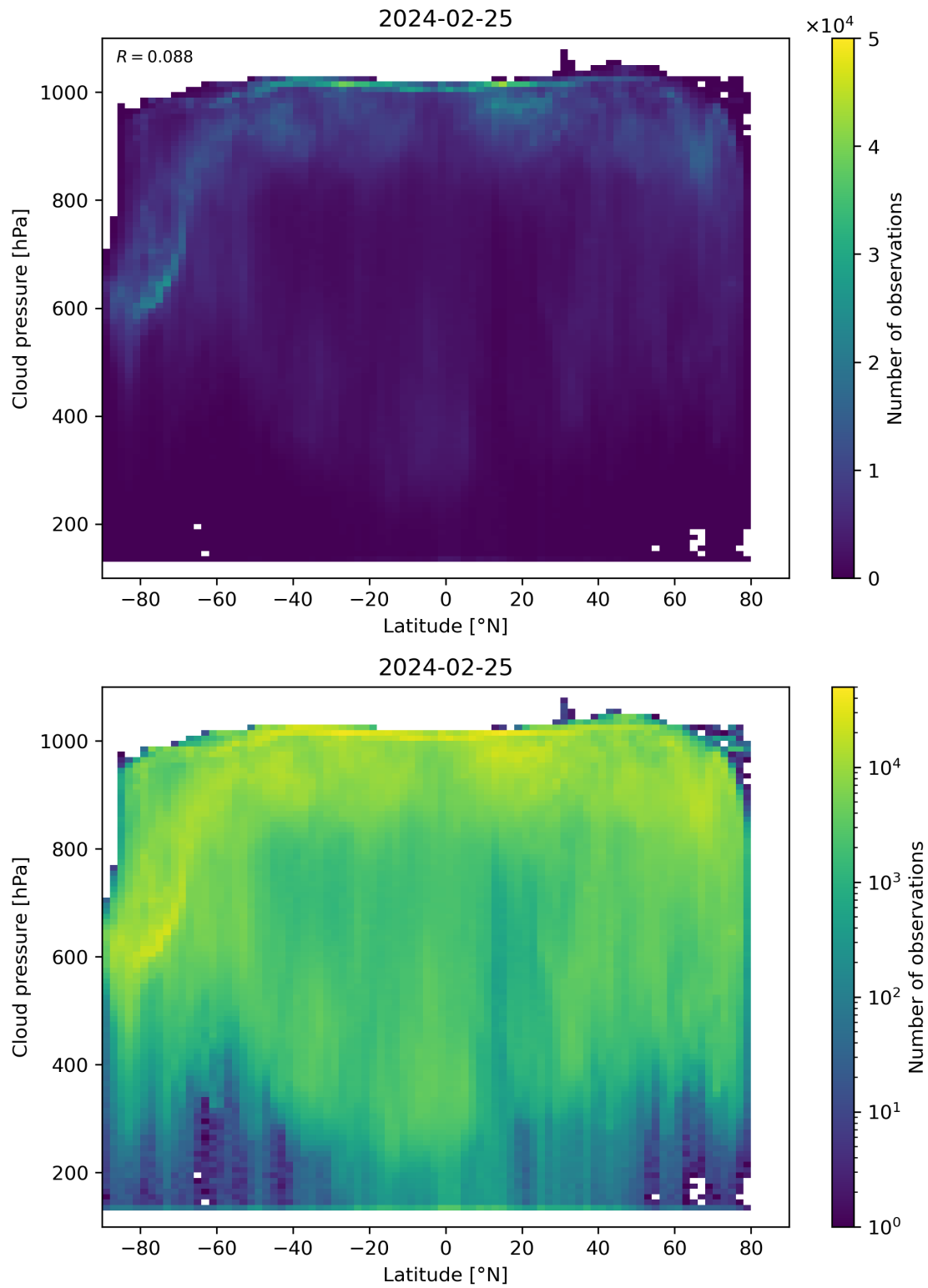
Figure 91: Scatter density plot of “Latitude” against “Cloud pressure” for 2024-02-24 to 2024-02-26.
