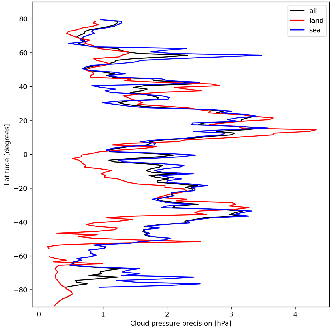
Figure 14: Zonal average of “Cloud pressure precision” for 2024-02-24 to 2024-02-26.
