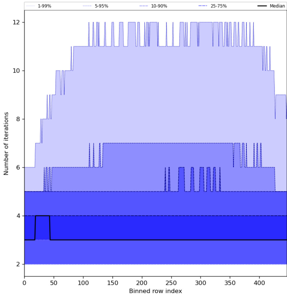
Figure 56: Along track statistics of “Number of iterations” for 2024-02-24 to 2024-02-26
