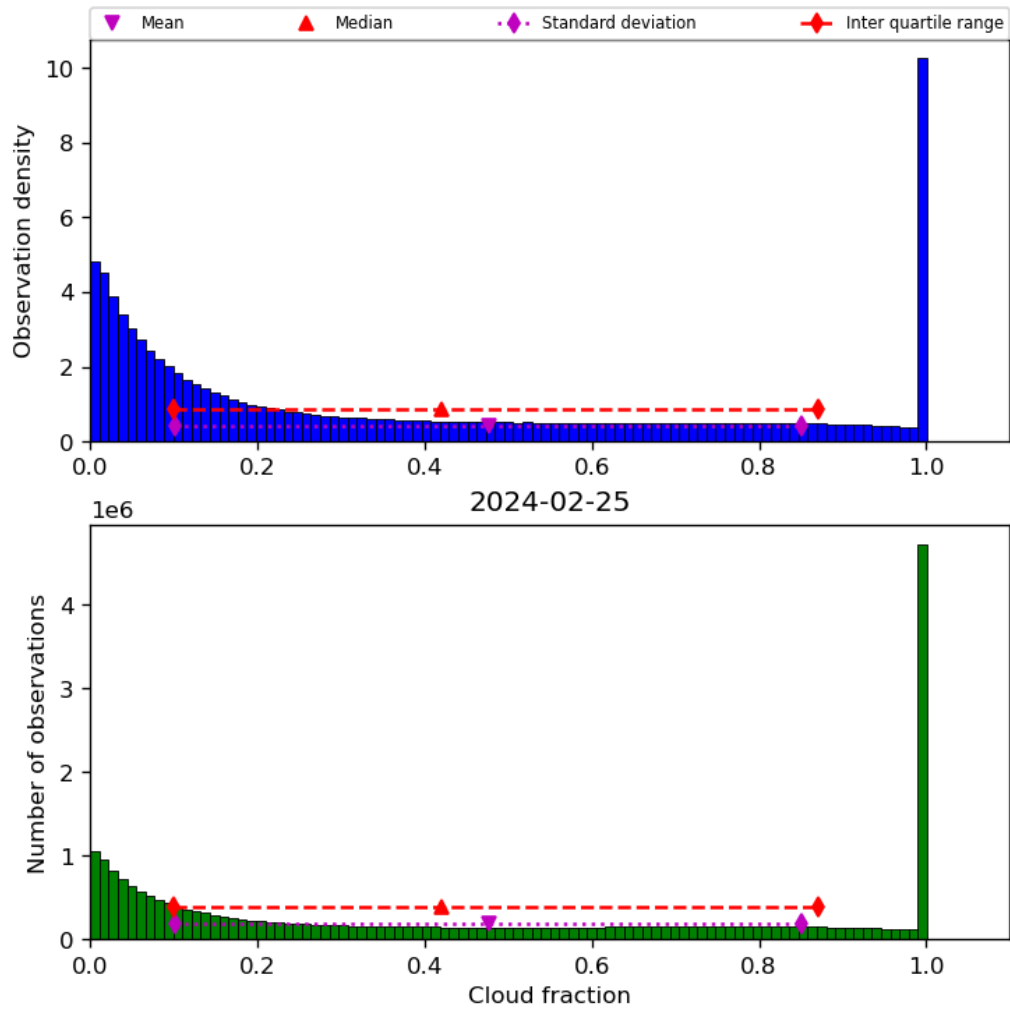
Figure 32: Histogram of “Cloud fraction” for 2024-02-24 to 2024-02-26
