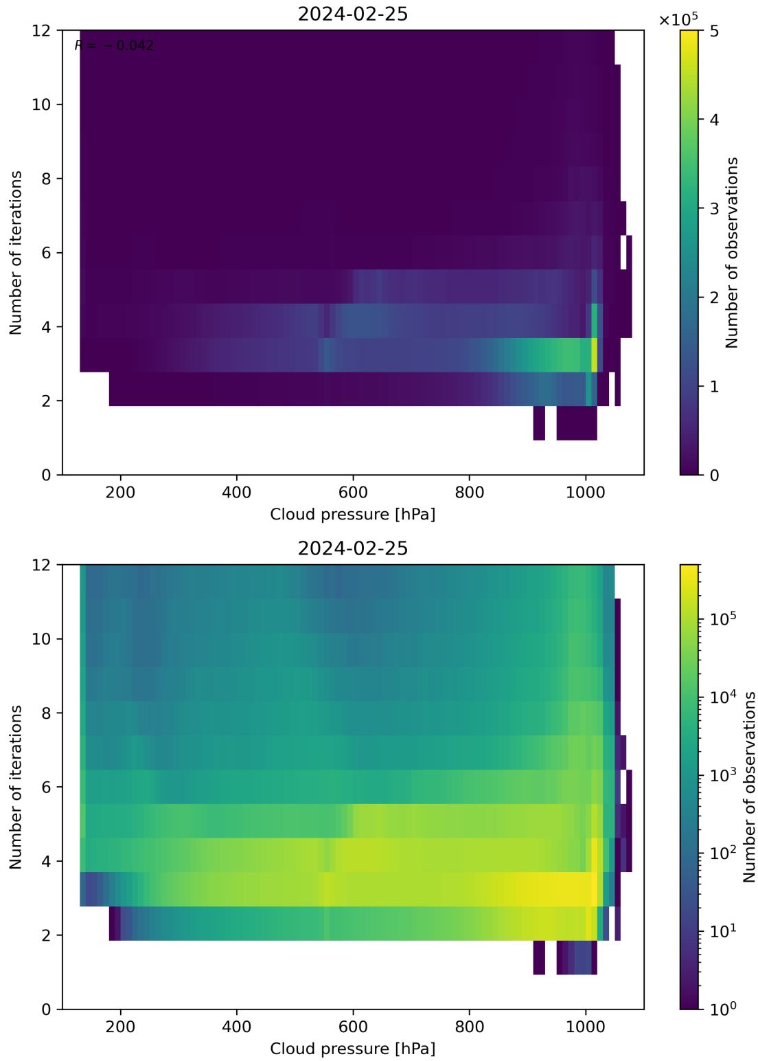
Figure 81: Scatter density plot of “Cloud pressure” against “Number of iterations” for 2024-02-24 to 2024-02-26.
