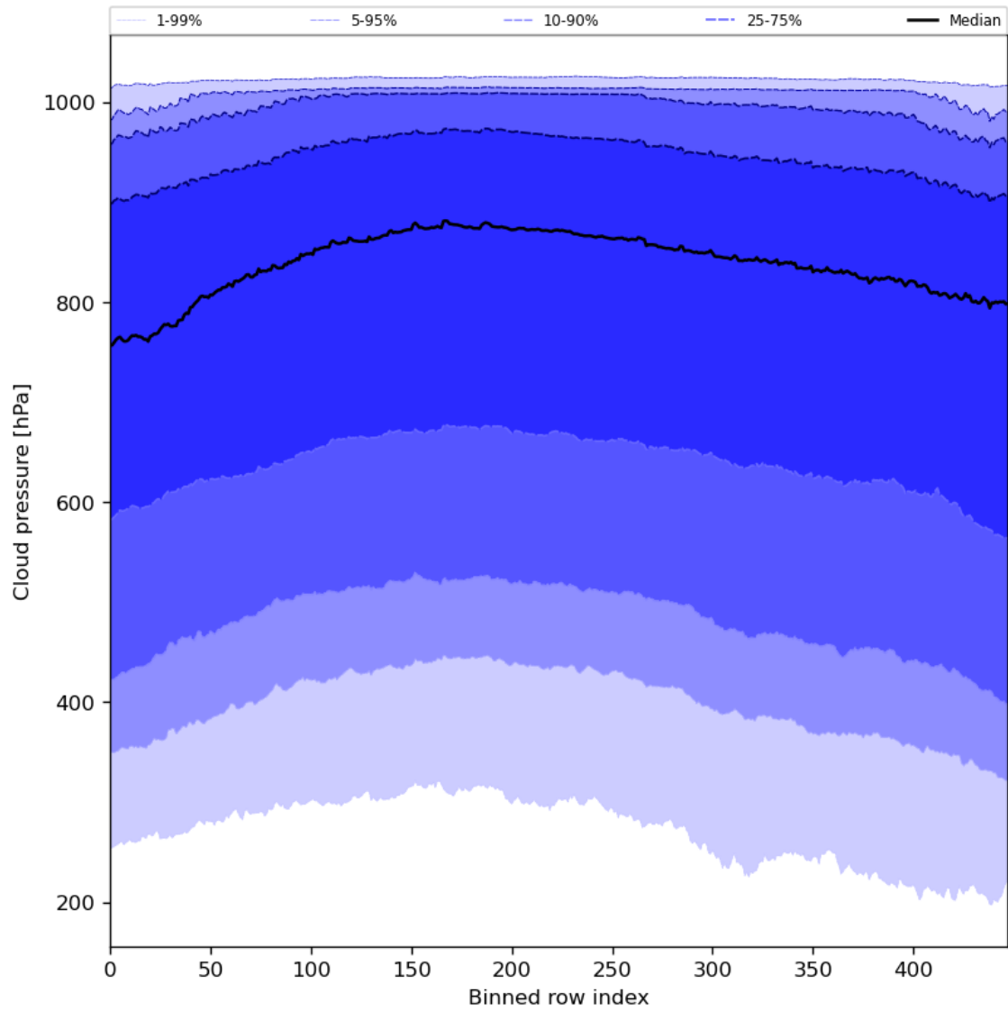
Figure 47: Along track statistics of “Cloud pressure” for 2024-02-24 to 2024-02-26
