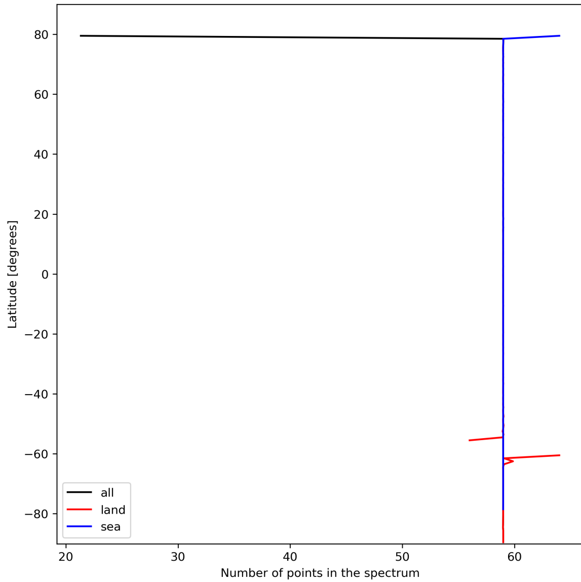
Figure 27: Zonal average of “Number of points in the spectrum” for 2024-02-24 to 2024-02-26.
