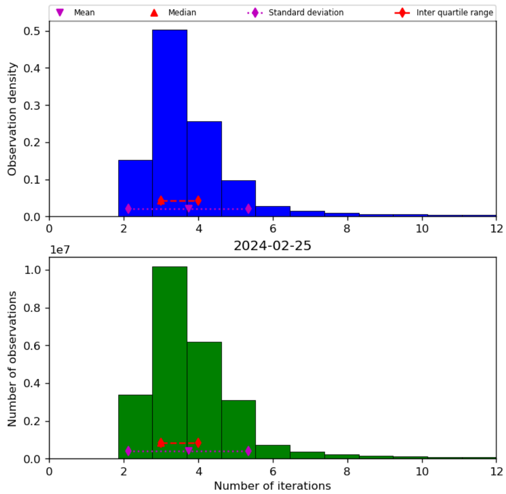
Figure 39: Histogram of “Number of iterations” for 2024-02-24 to 2024-02-26
