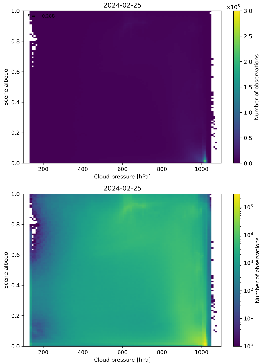
Figure 83: Scatter density plot of “Cloud pressure” against “Scene albedo” for 2024-02-24 to 2024-02-26.
