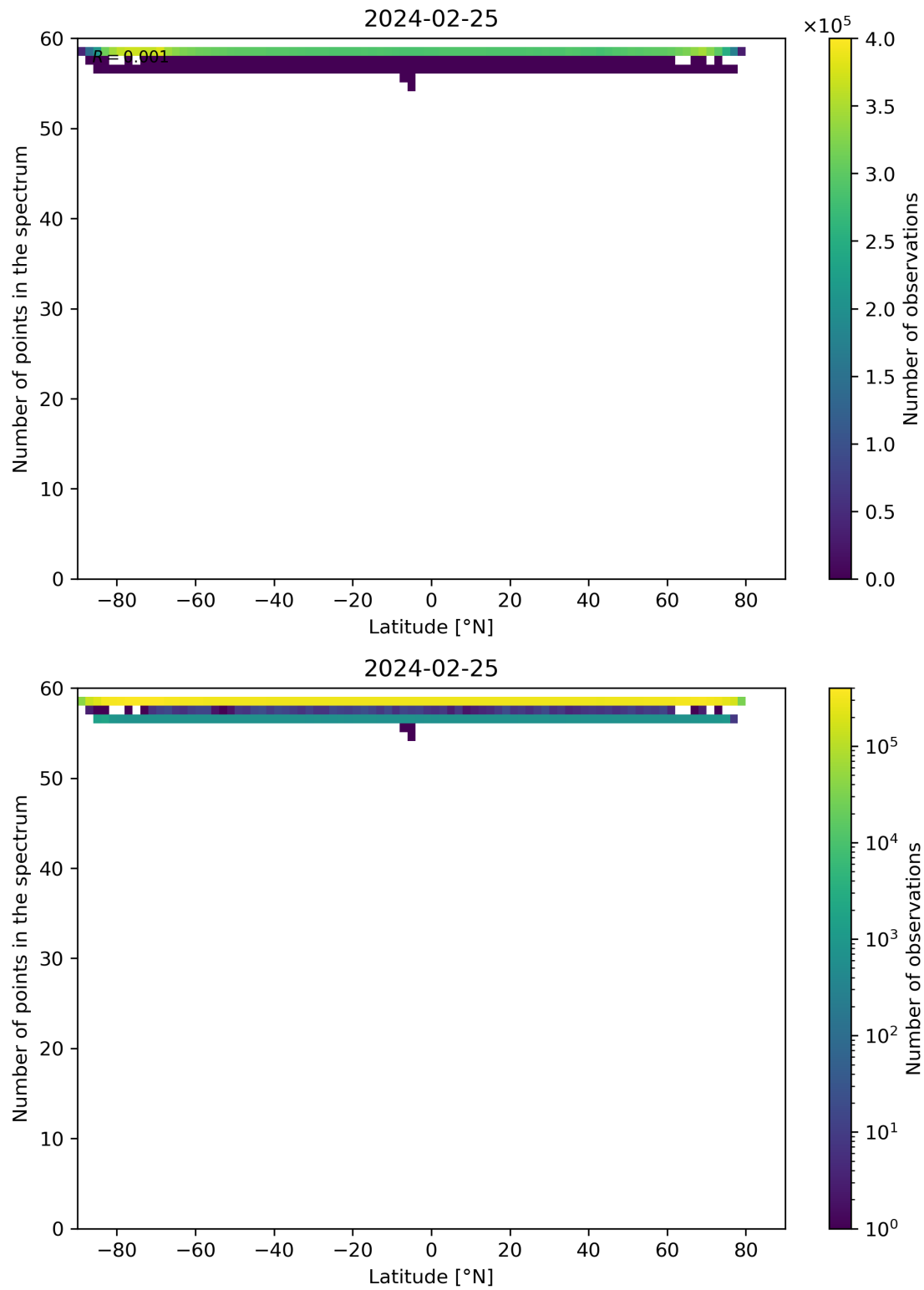
Figure 94: Scatter density plot of “Latitude” against “Number of points in the spectrum” for 2024-02-24 to 2024-02-26.
