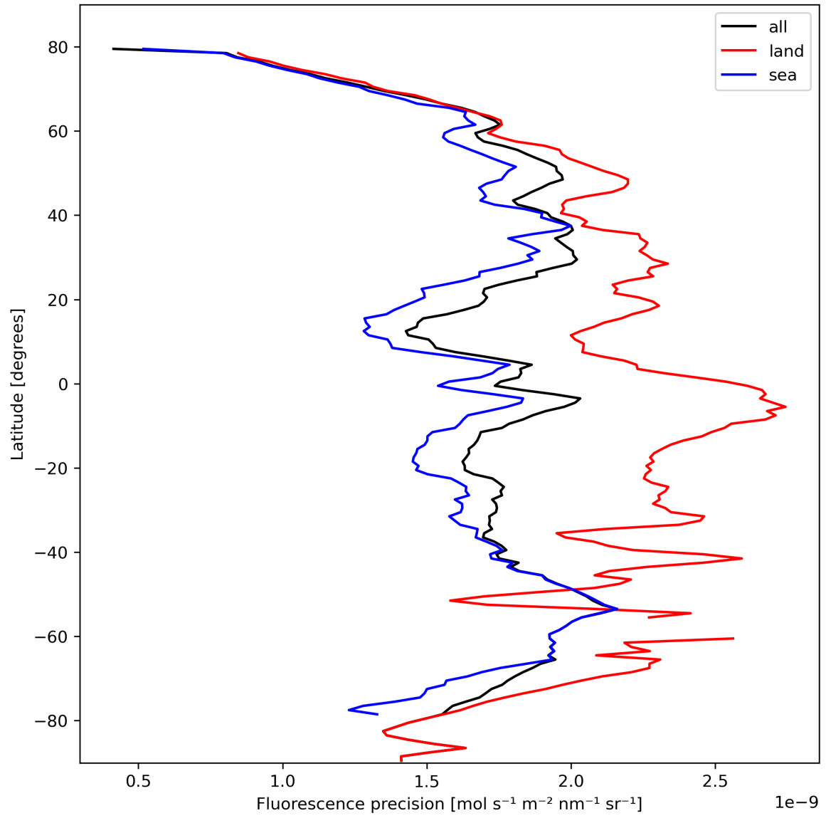
Figure 24: Zonal average of “Fluorescence precision” for 2024-02-24 to 2024-02-26.
