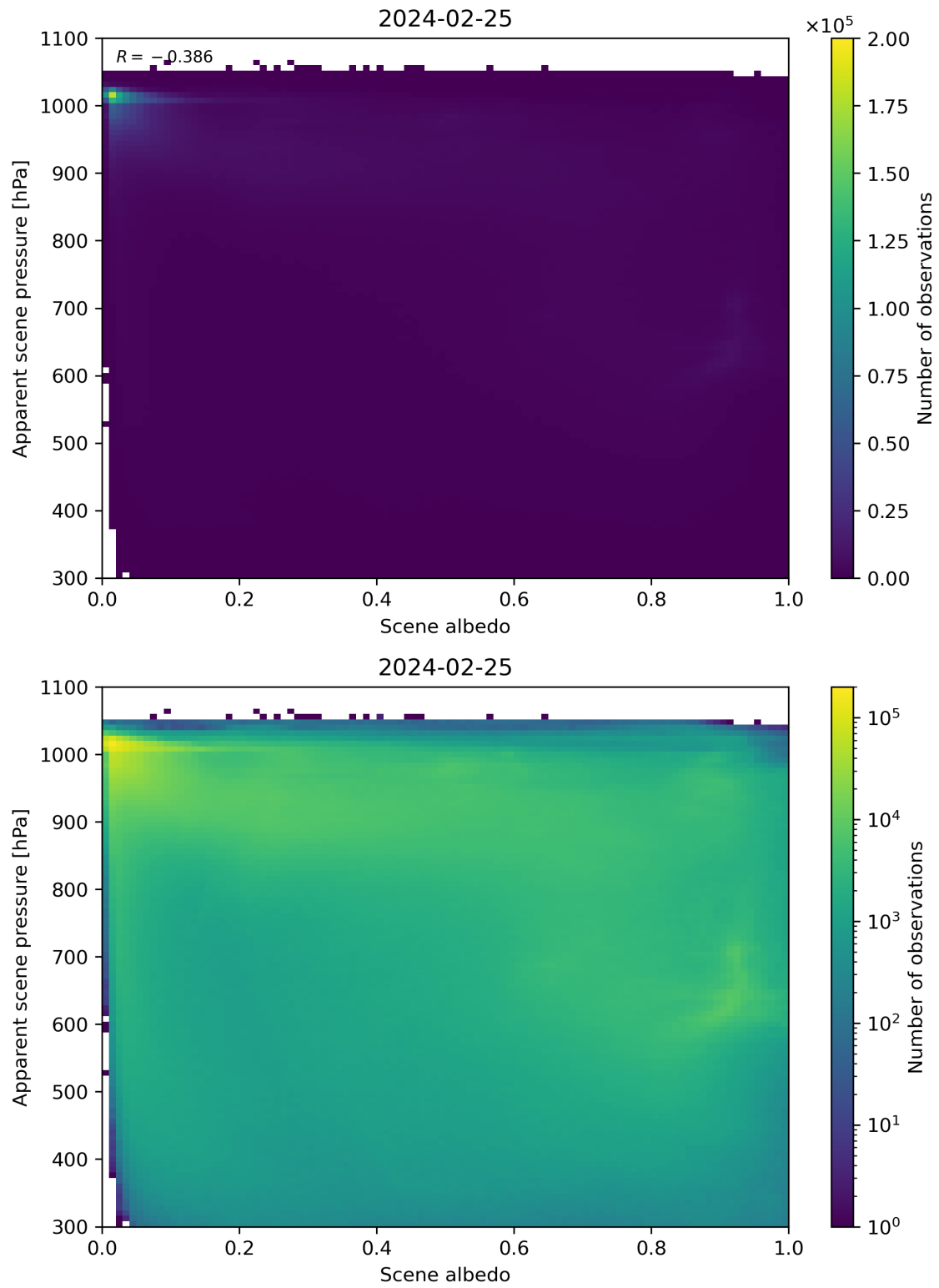
Figure 102: Scatter density plot of “Scene albedo” against “Apparent scene pressure” for 2024-02-24 to 2024-02-26.
