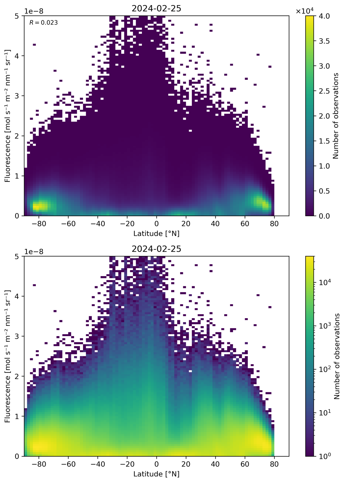
Figure 92: Scatter density plot of “Latitude” against “Fluorescence” for 2024-02-24 to 2024-02-26.
