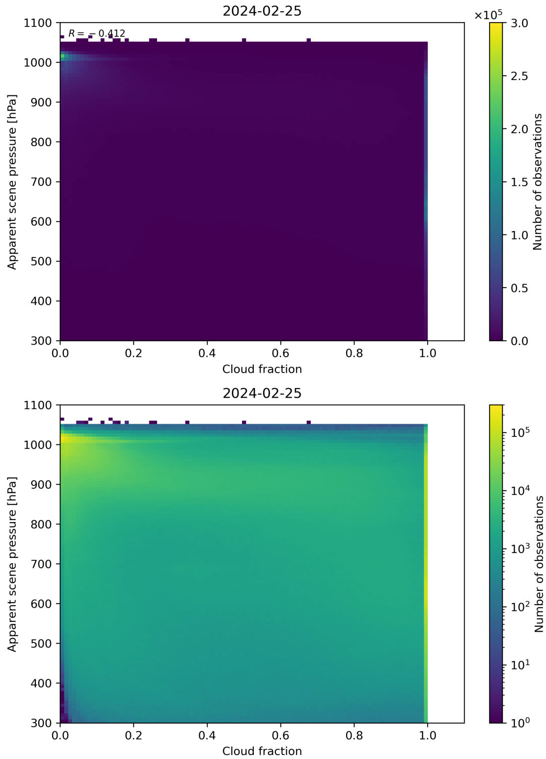
Figure 70: Scatter density plot of “Cloud fraction” against “Apparent scene pressure” for 2024-02-24 to 2024-02-26.
