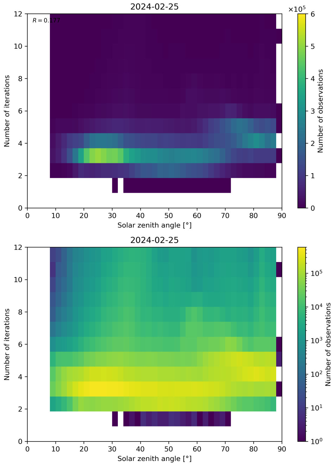
Figure 114: Scatter density plot of “Solar zenith angle” against “Number of iterations” for 2024-02-24 to 2024-02-26.
