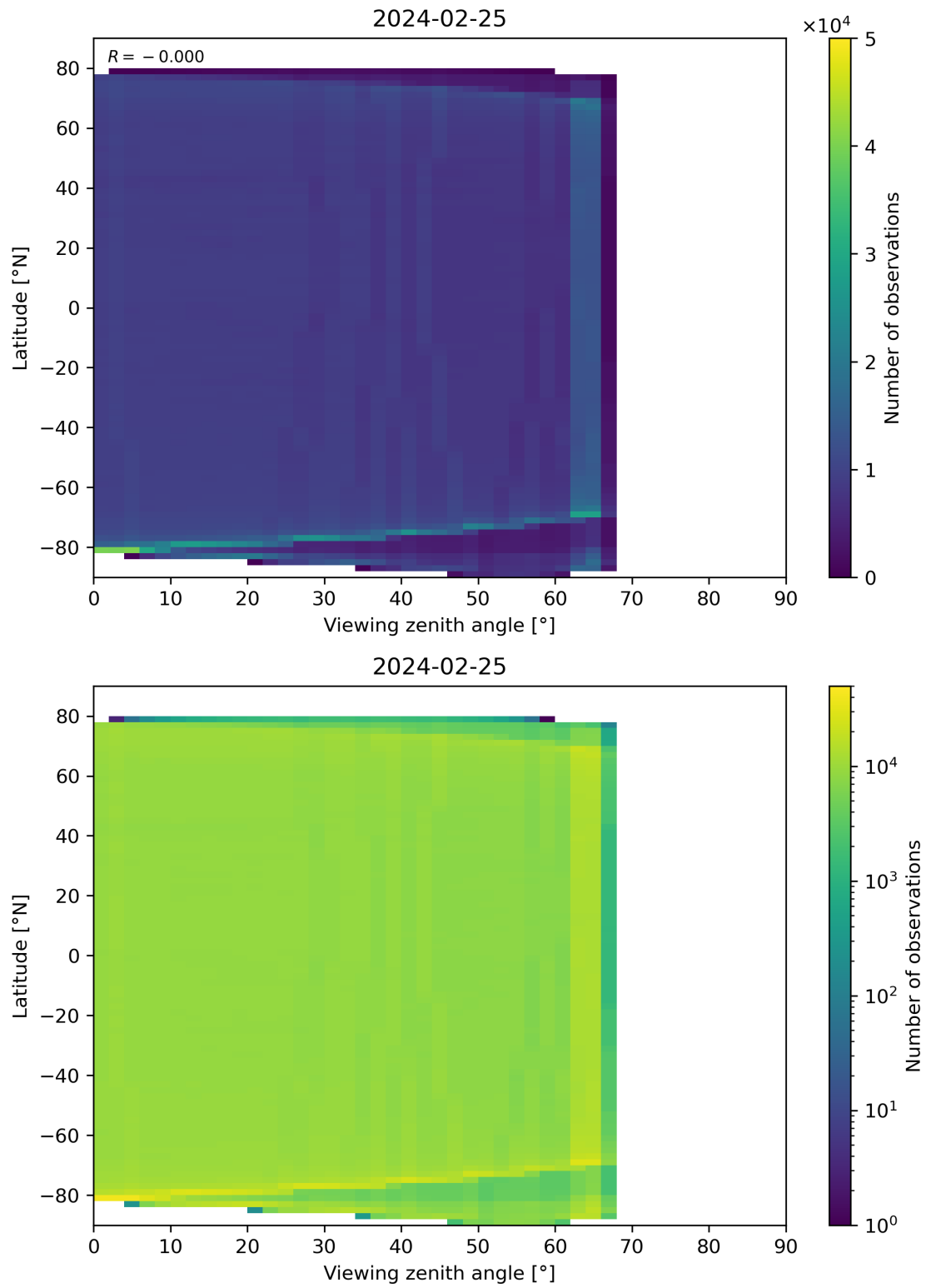
Figure 123: Scatter density plot of “Viewing zenith angle” against “Latitude” for 2024-02-24 to 2024-02-26.
