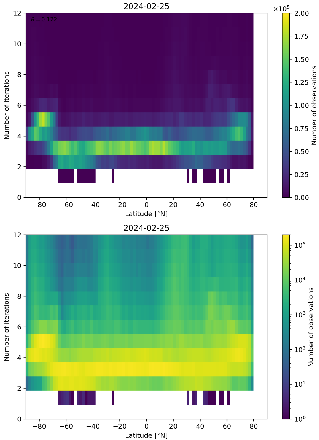
Figure 93: Scatter density plot of “Latitude” against “Number of iterations” for 2024-02-24 to 2024-02-26.
