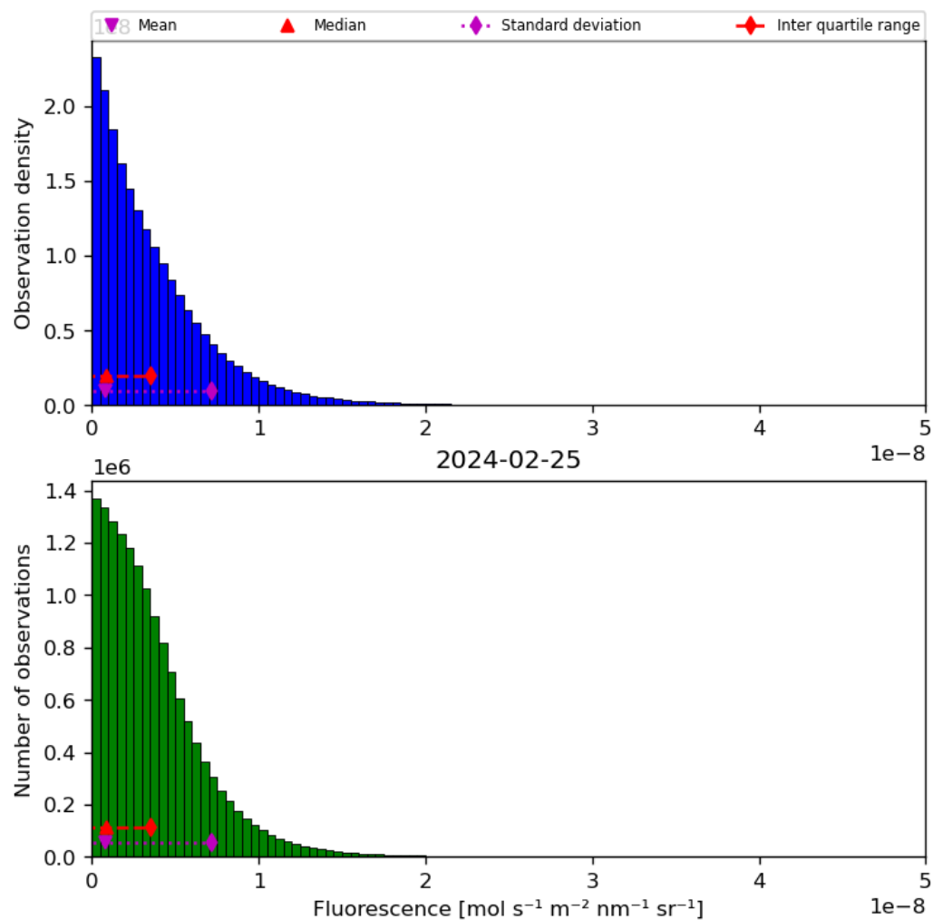
Figure 40: Histogram of “Fluorescence” for 2024-02-24 to 2024-02-26
