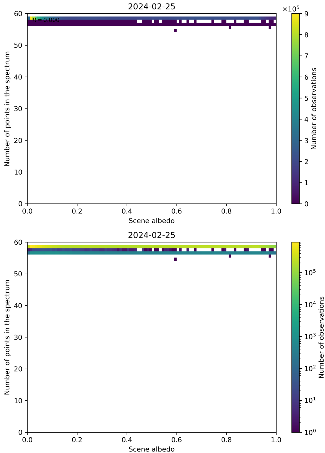
Figure 106: Scatter density plot of “Scene albedo” against “Number of points in the spectrum” for 2024-02-24 to 2024-02-26.
