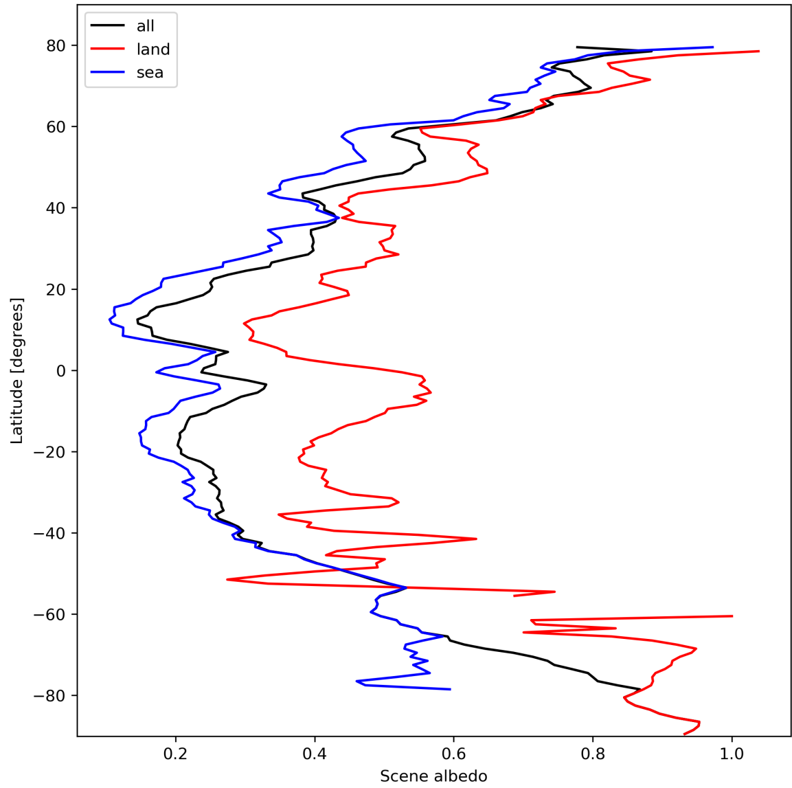
Figure 17: Zonal average of “Scene albedo” for 2024-02-24 to 2024-02-26.
