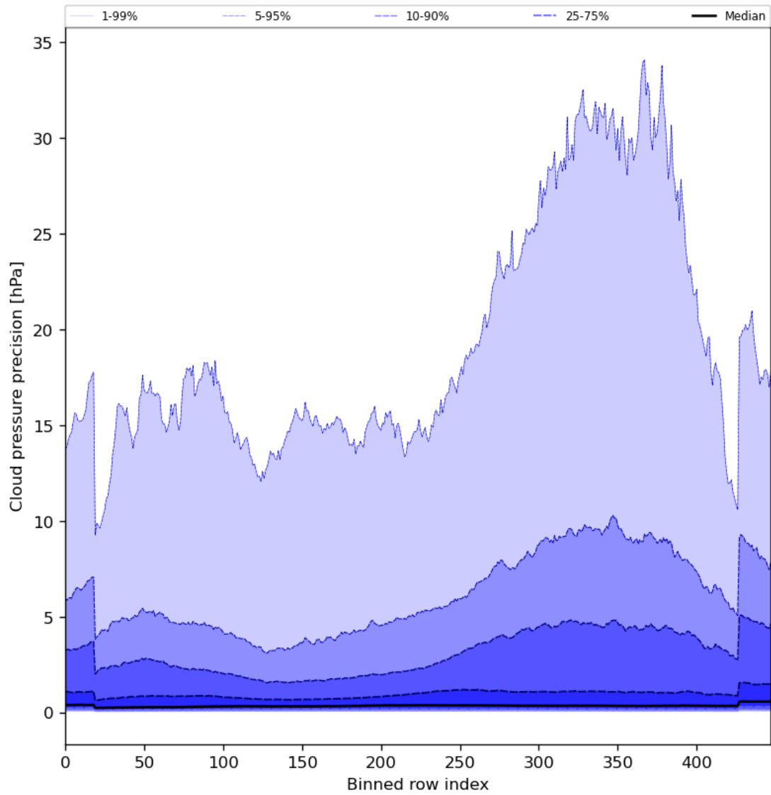
Figure 48: Along track statistics of “Cloud pressure precision” for 2024-02-24 to 2024-02-26
