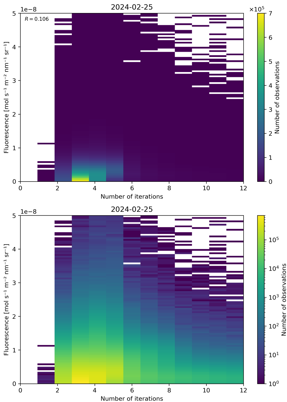
Figure 98: Scatter density plot of “Number of iterations” against “Fluorescence” for 2024-02-24 to 2024-02-26.
