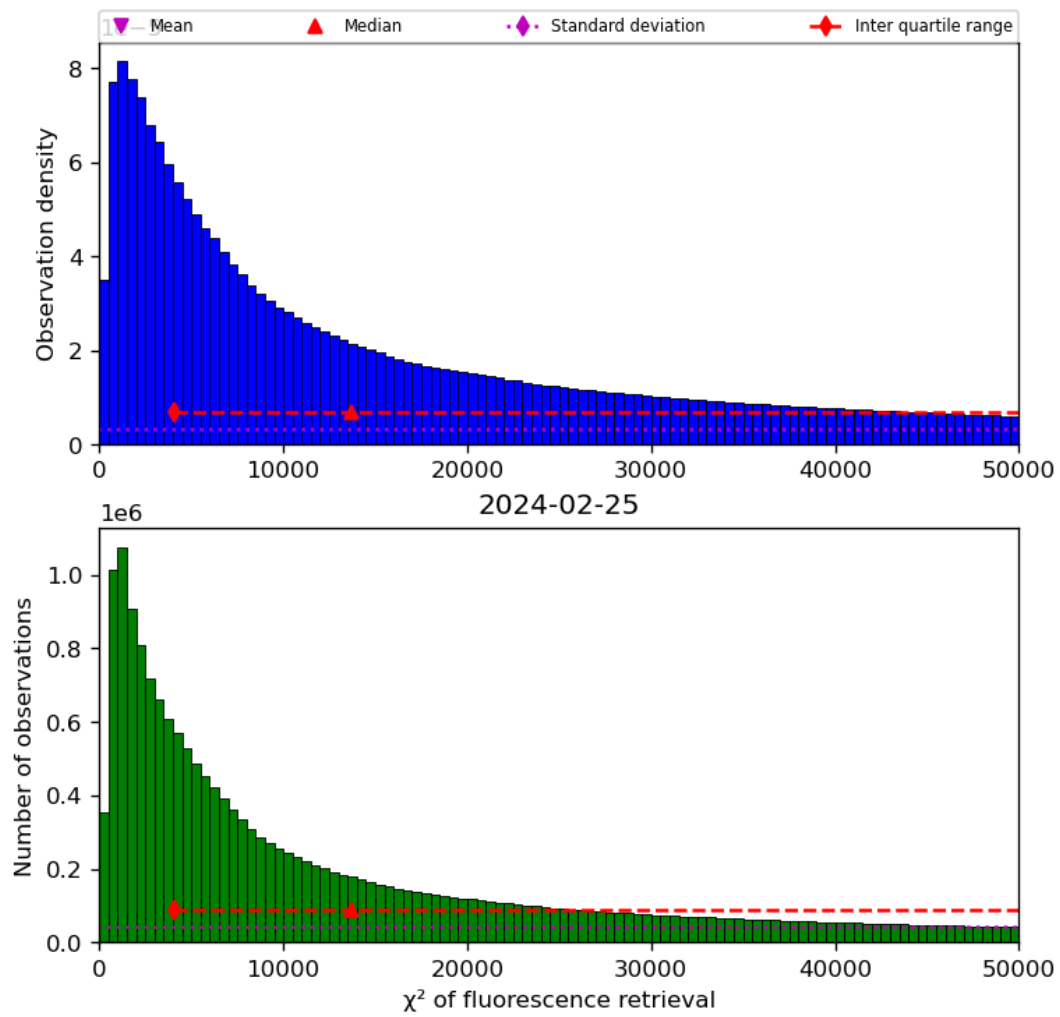
Figure 42: Histogram of “ \chi^2 of fluorescence retrieval” for 2024-02-24 to 2024-02-26
