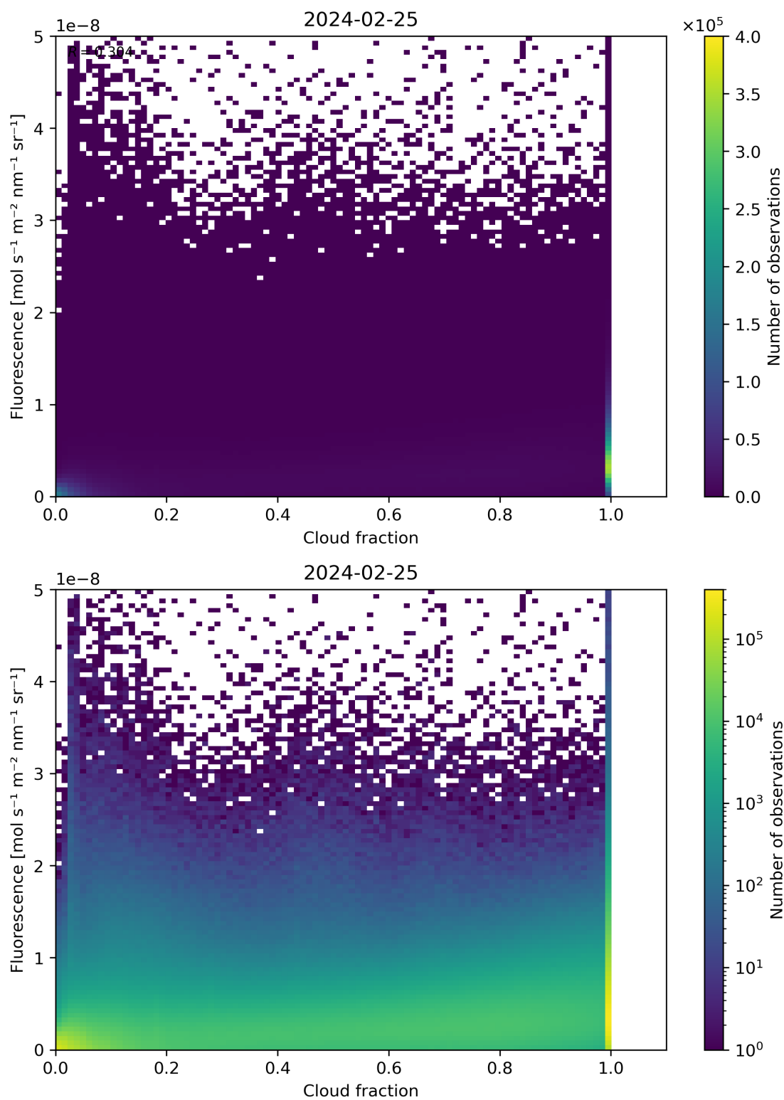
Figure 72: Scatter density plot of “Cloud fraction” against “Fluorescence” for 2024-02-24 to 2024-02-26.
