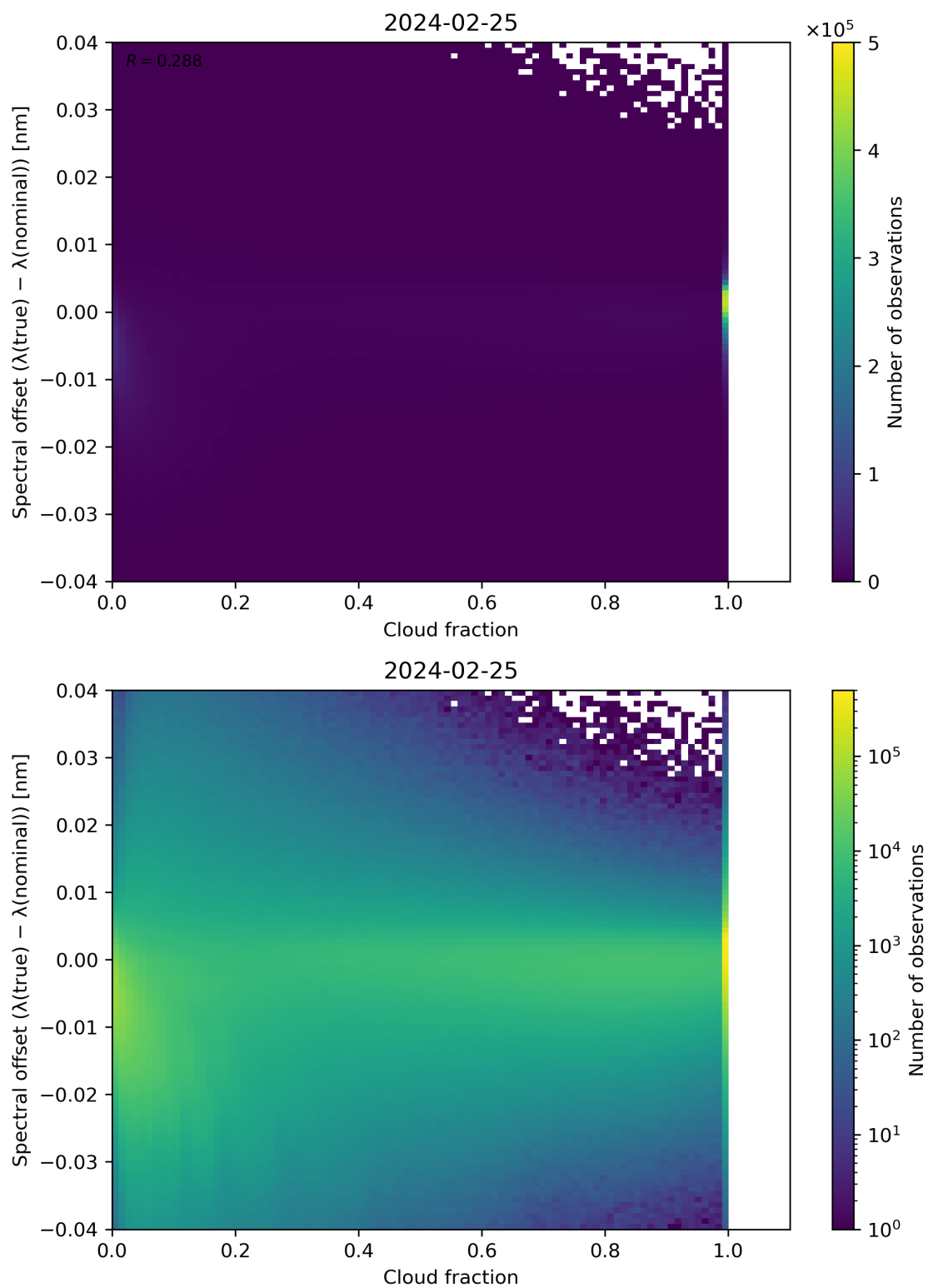
Figure 76: Scatter density plot of “Cloud fraction” against “Spectral offset ( \lambda(\text{true}) - \lambda(\text{nominal}) )” for 2024-02-24 to 2024-02-26.
