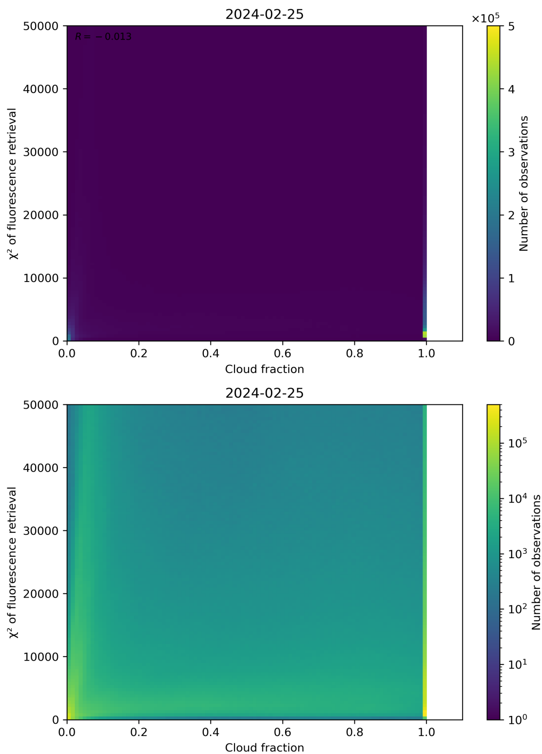
Figure 71: Scatter density plot of “Cloud fraction” against “ \chi^2 of fluorescence retrieval” for 2024-02-24 to 2024-02-26.
