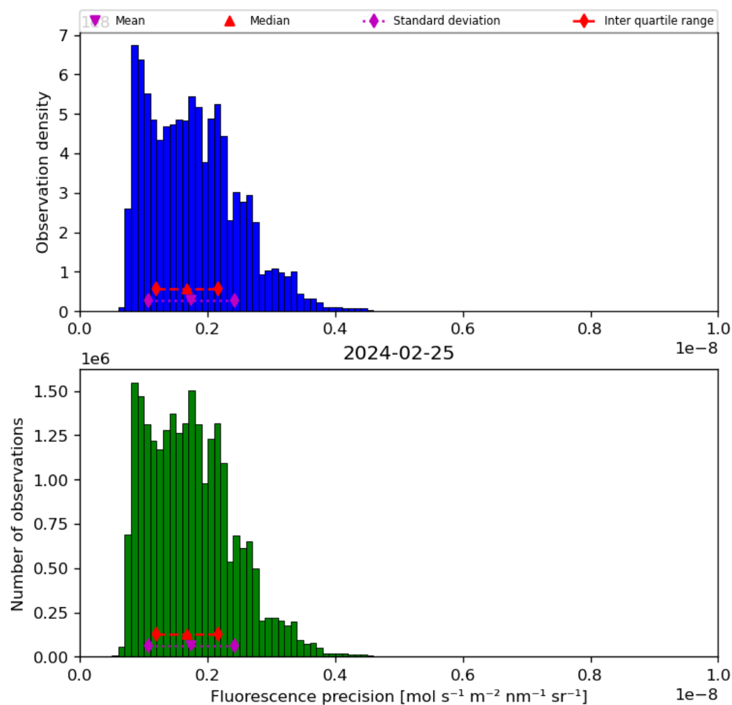
Figure 41: Histogram of “Fluorescence precision” for 2024-02-24 to 2024-02-26
