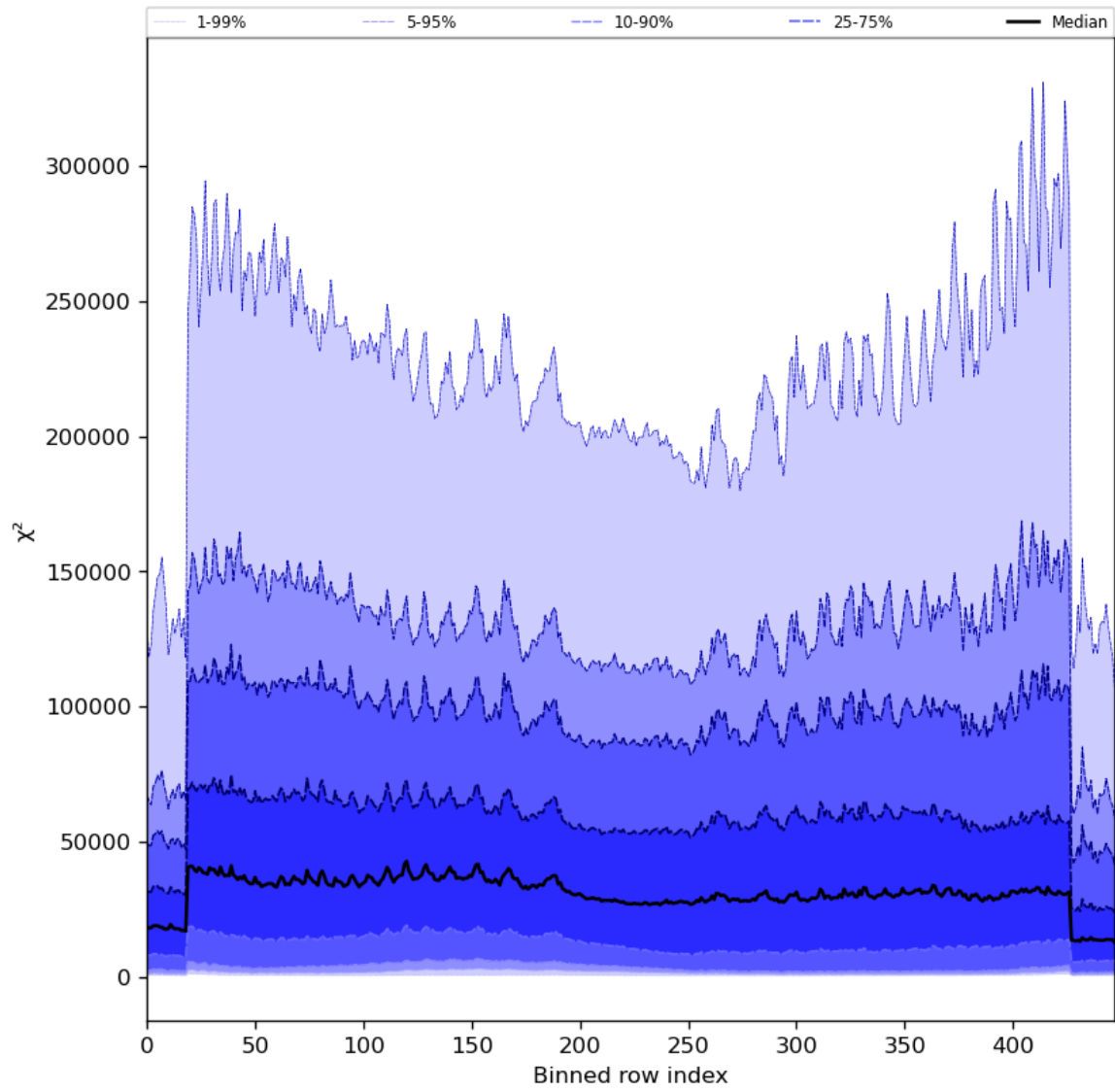
Figure 55: Along track statistics of “ \chi^2 ” for 2024-02-24 to 2024-02-26
