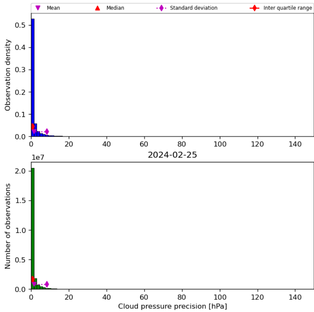
Figure 31: Histogram of “Cloud pressure precision” for 2024-02-24 to 2024-02-26
