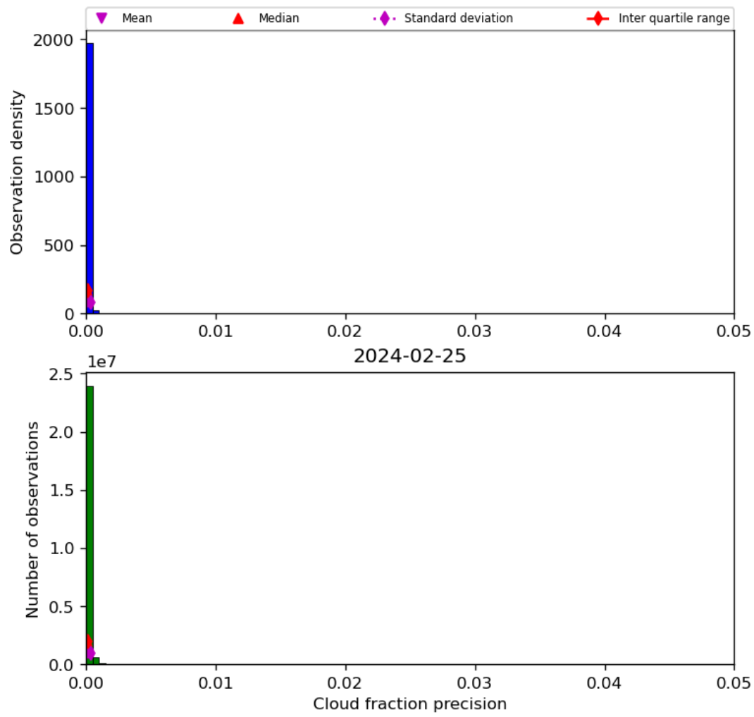
Figure 33: Histogram of “Cloud fraction precision” for 2024-02-24 to 2024-02-26
