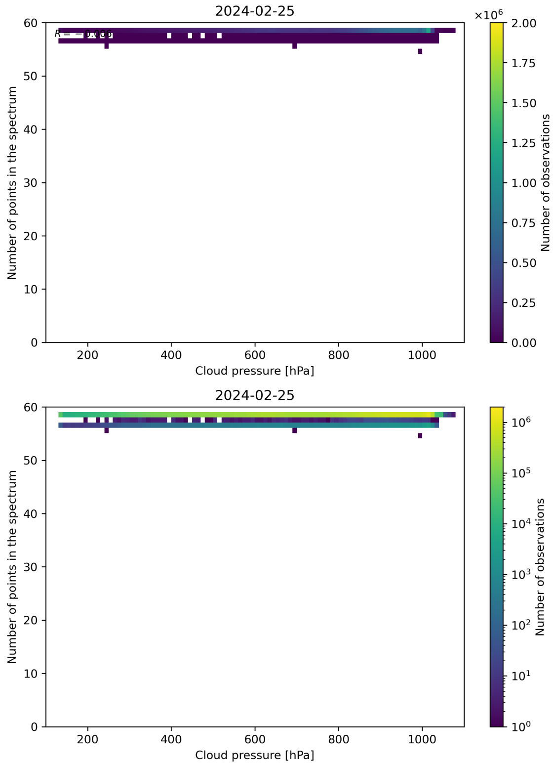
Figure 82: Scatter density plot of “Cloud pressure” against “Number of points in the spectrum” for 2024-02-24 to 2024-02-26.
