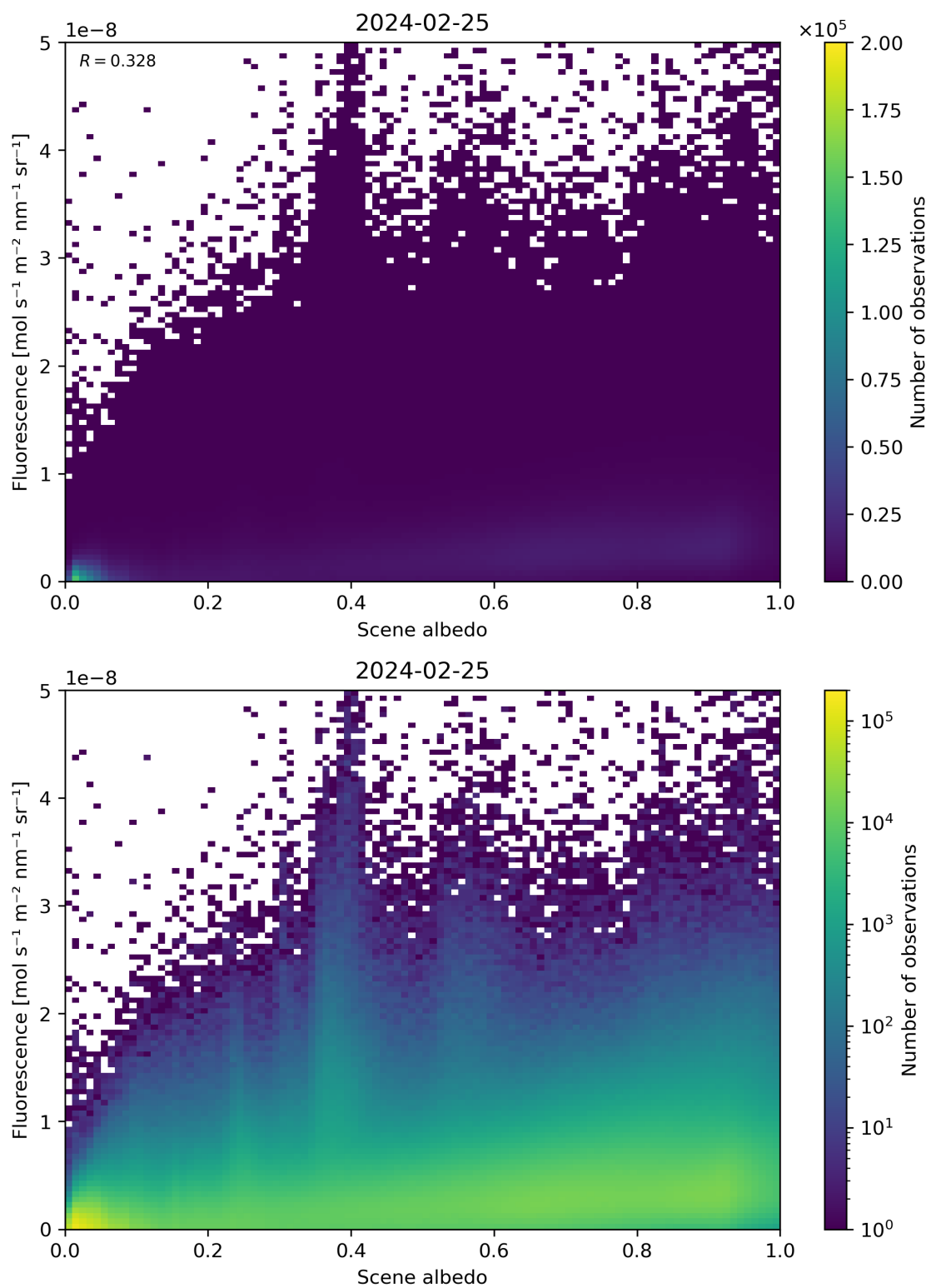
Figure 104: Scatter density plot of “Scene albedo” against “Fluorescence” for 2024-02-24 to 2024-02-26.
