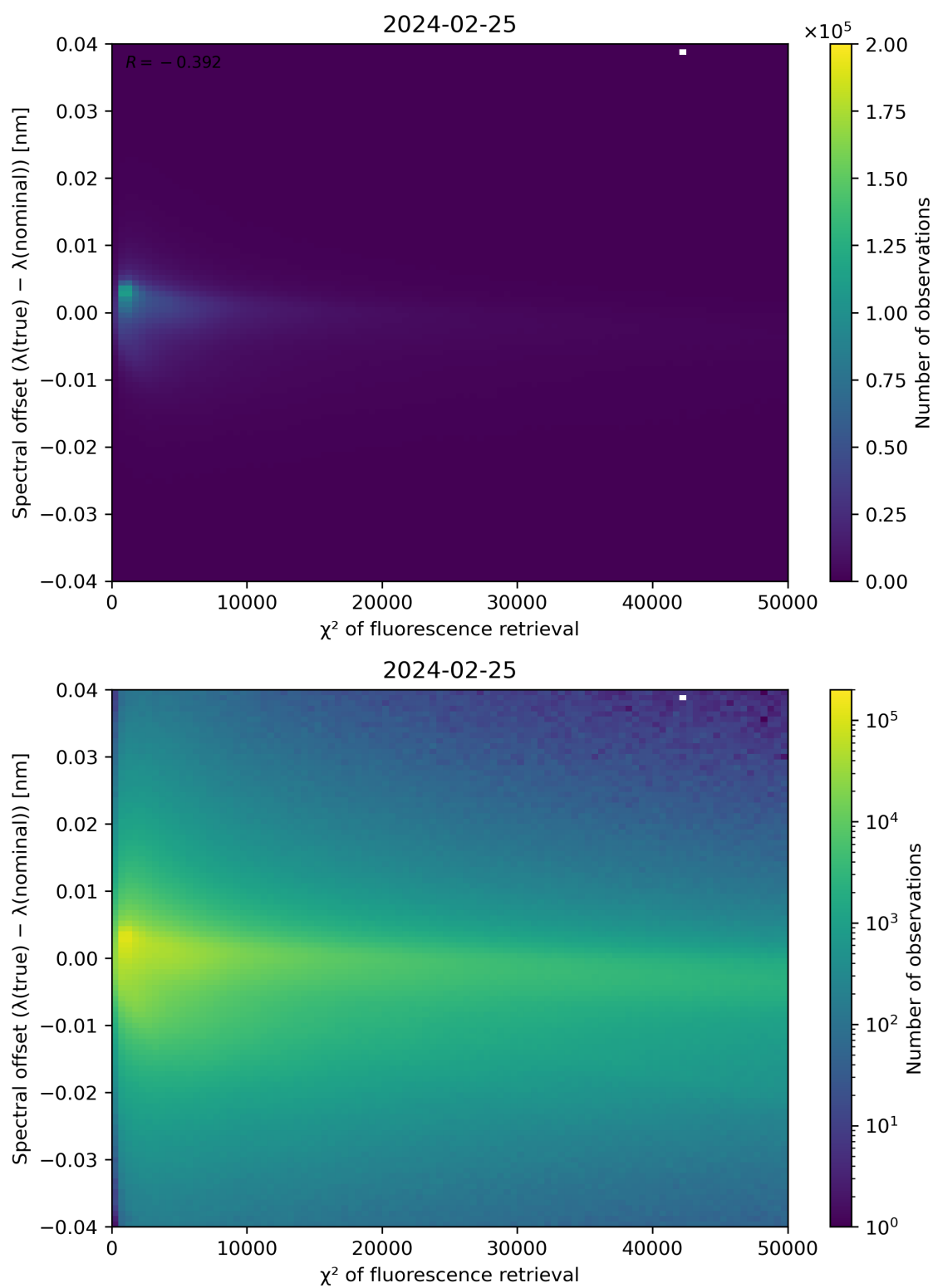
Figure 69: Scatter density plot of " \chi^2 of fluorescence retrieval" against "Spectral offset ( \lambda(\text{true}) - \lambda(\text{nominal})) " for 2024-02-24 to 2024-02-26.
