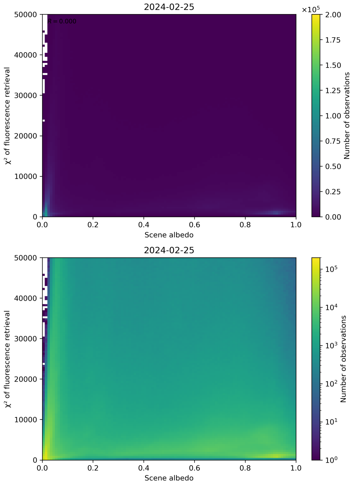
Figure 103: Scatter density plot of “Scene albedo” against “ \chi^2 of fluorescence retrieval” for 2024-02-24 to 2024-02-26.
