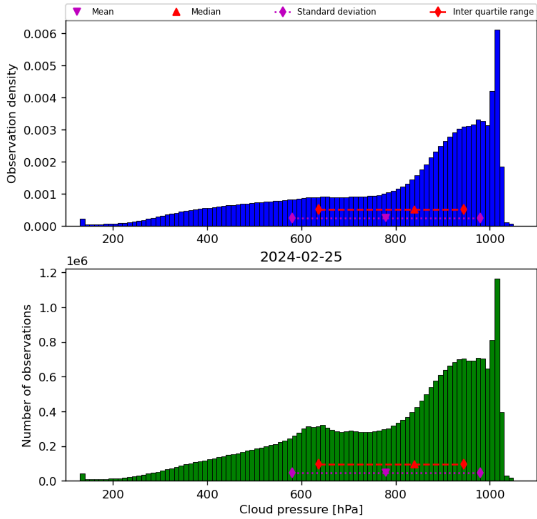
Figure 30: Histogram of “Cloud pressure” for 2024-02-24 to 2024-02-26
