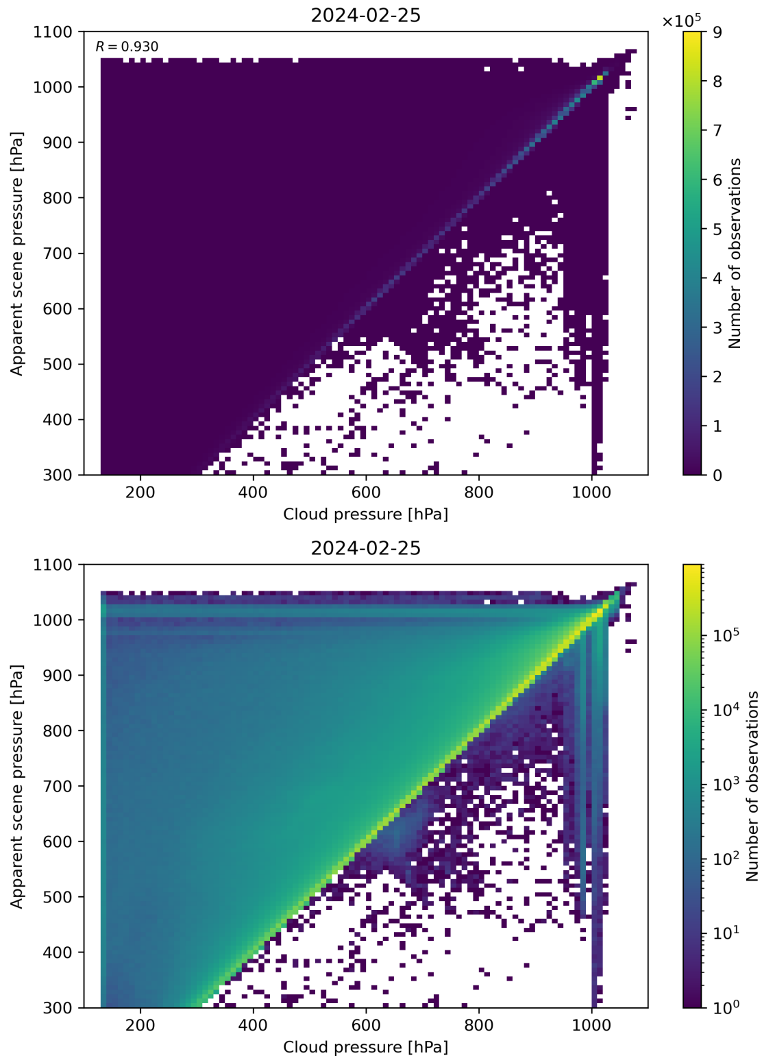
Figure 77: Scatter density plot of “Cloud pressure” against “Apparent scene pressure” for 2024-02-24 to 2024-02-26.
