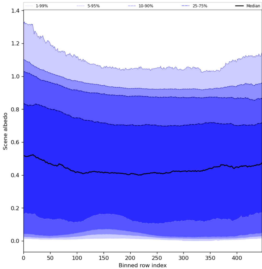
Figure 51: Along track statistics of “Scene albedo” for 2024-02-24 to 2024-02-26
