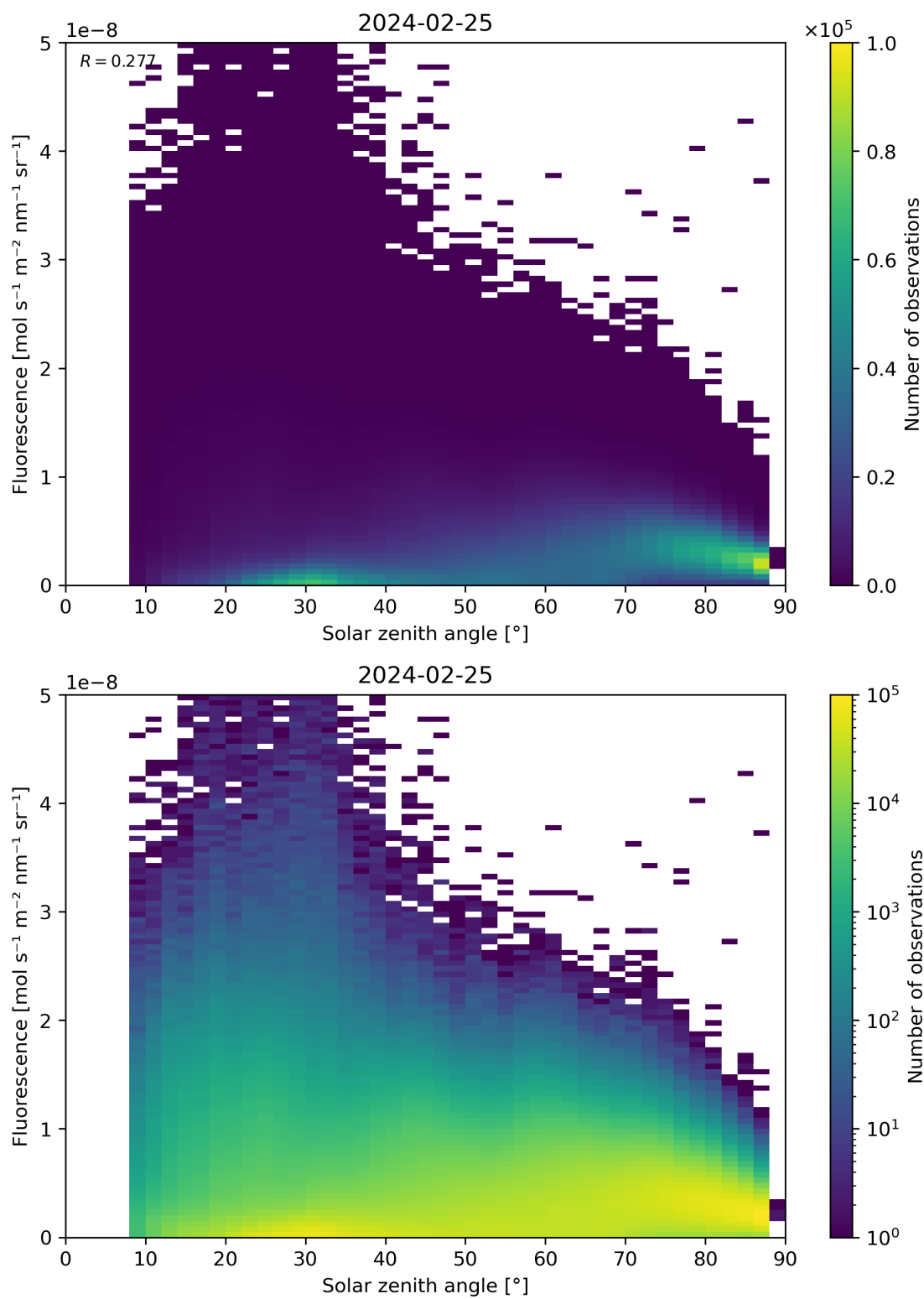
Figure 112: Scatter density plot of “Solar zenith angle” against “Fluorescence” for 2024-02-24 to 2024-02-26.
