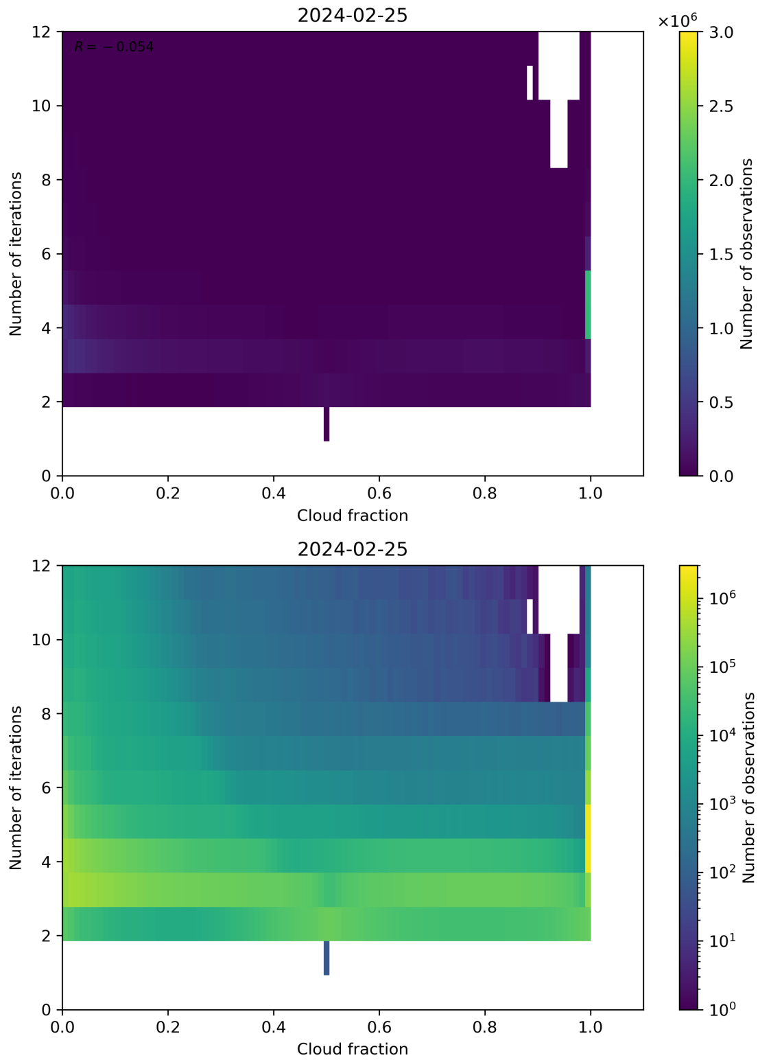
Figure 73: Scatter density plot of “Cloud fraction” against “Number of iterations” for 2024-02-24 to 2024-02-26.
