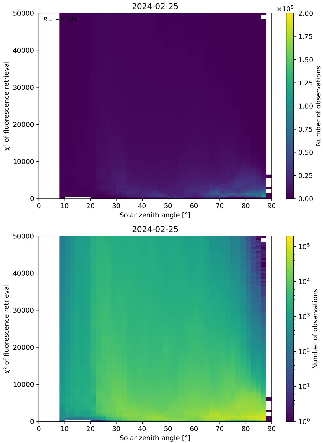
Figure 109: Scatter density plot of “Solar zenith angle” against “ \chi^2 of fluorescence retrieval” for 2024-02-24 to 2024-02-26.
