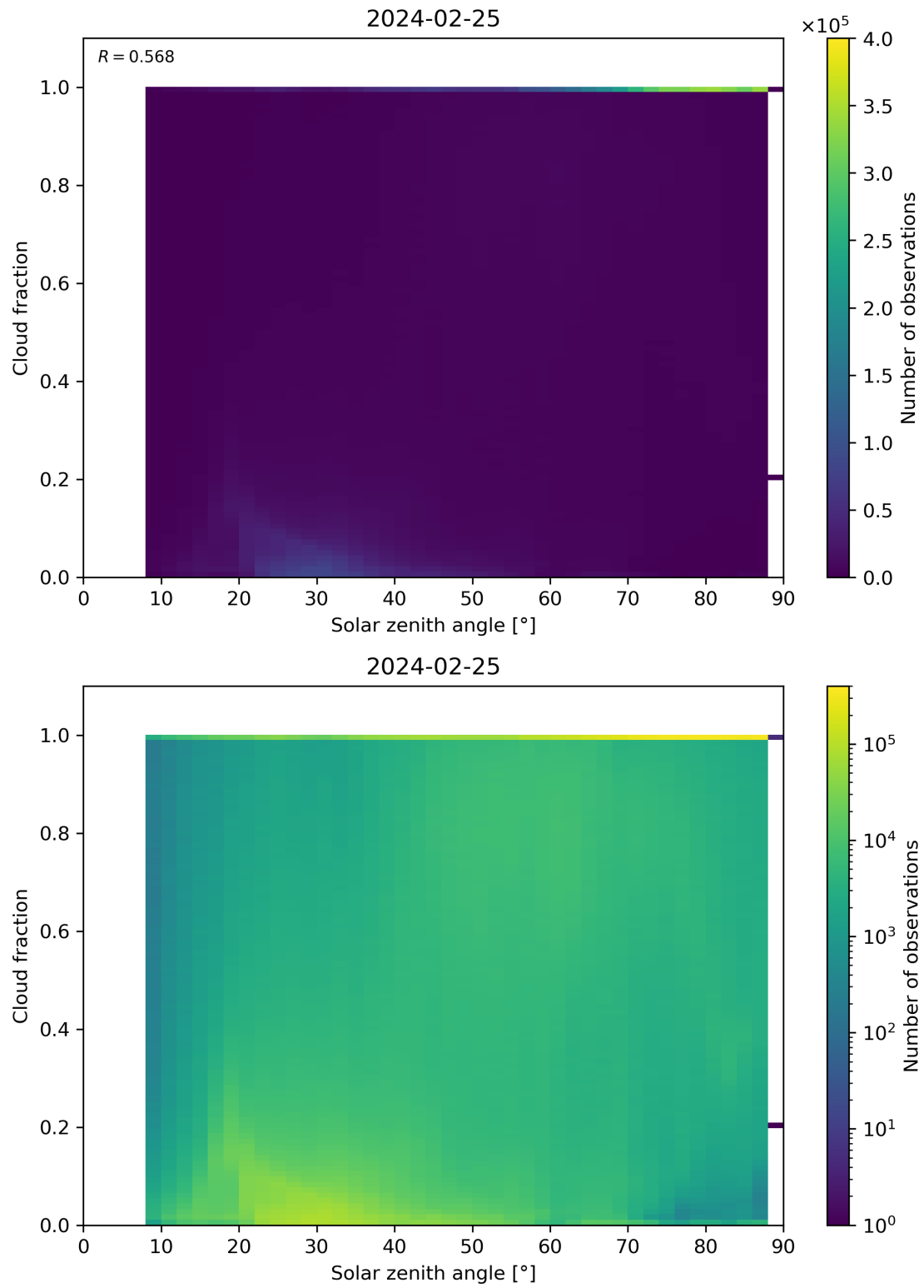
Figure 110: Scatter density plot of “Solar zenith angle” against “Cloud fraction” for 2024-02-24 to 2024-02-26.
