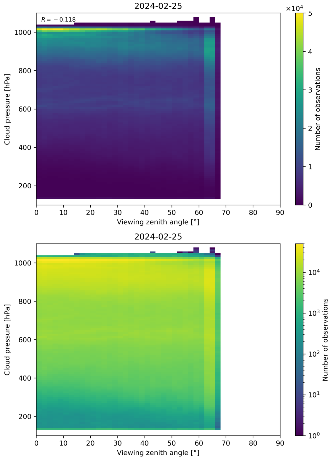
Figure 121: Scatter density plot of “Viewing zenith angle” against “Cloud pressure” for 2024-02-24 to 2024-02-26.
