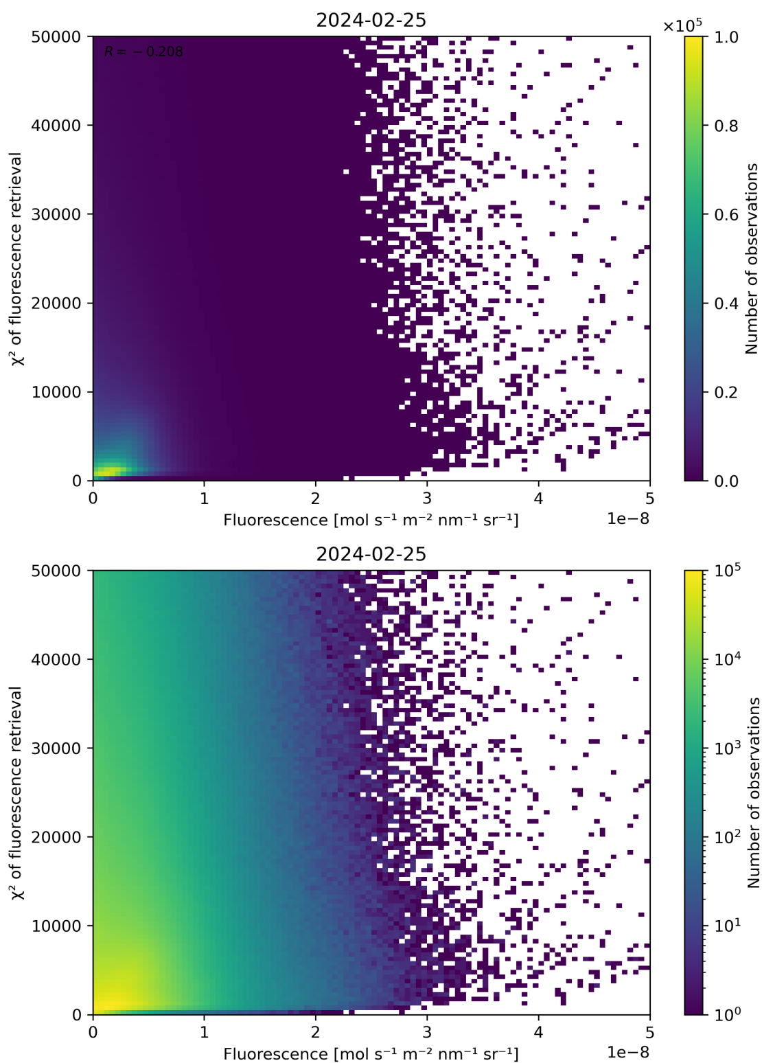
Figure 85: Scatter density plot of “Fluorescence” against “ \chi^2 of fluorescence retrieval” for 2024-02-24 to 2024-02-26.
