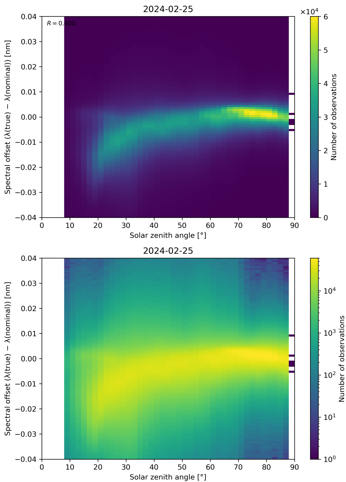
Figure 117: Scatter density plot of “Solar zenith angle” against “Spectral offset ( \lambda(\text{true}) - \lambda(\text{nominal}) )” for 2024-02-24 to 2024-02-26.
