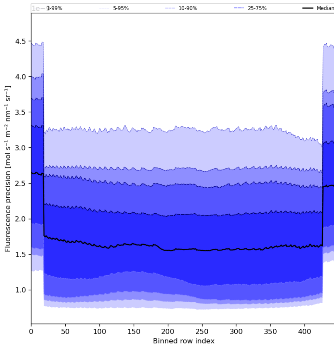
Figure 58: Along track statistics of “Fluorescence precision” for 2024-02-24 to 2024-02-26
