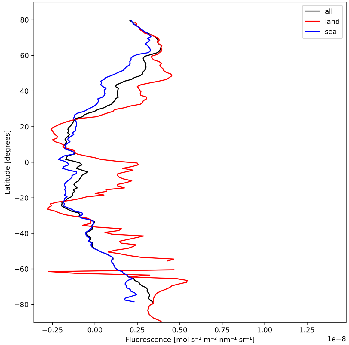
Figure 23: Zonal average of “Fluorescence” for 2024-02-24 to 2024-02-26.
