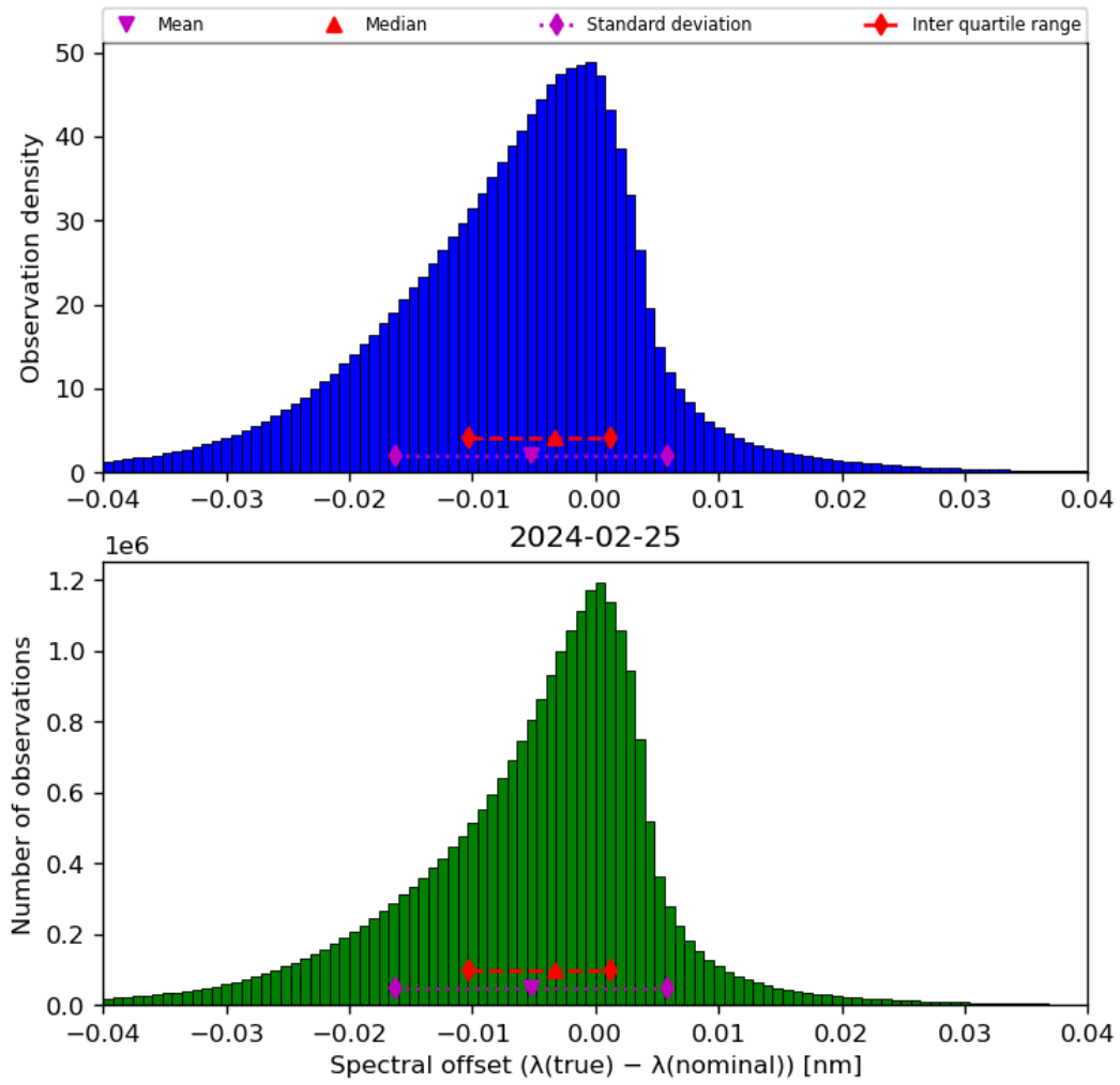
Figure 45: Histogram of “Spectral offset ( \lambda(\text{true}) - \lambda(\text{nominal}) )” for 2024-02-24 to 2024-02-26
