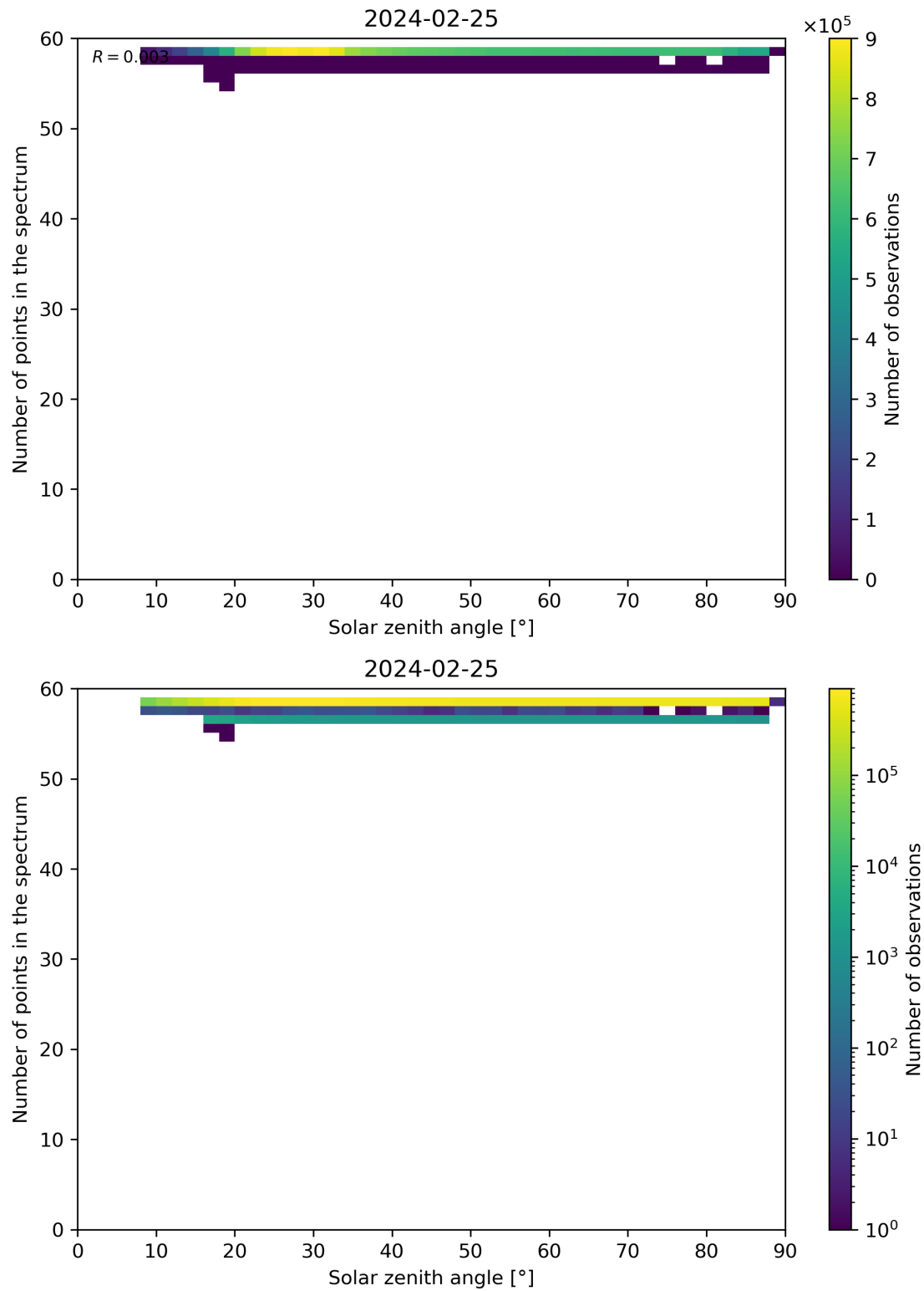
Figure 115: Scatter density plot of “Solar zenith angle” against “Number of points in the spectrum” for 2024-02-24 to 2024-02-26.
