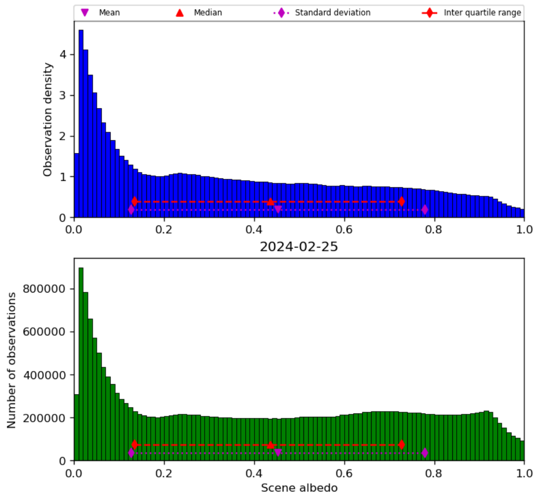
Figure 34: Histogram of “Scene albedo” for 2024-02-24 to 2024-02-26
