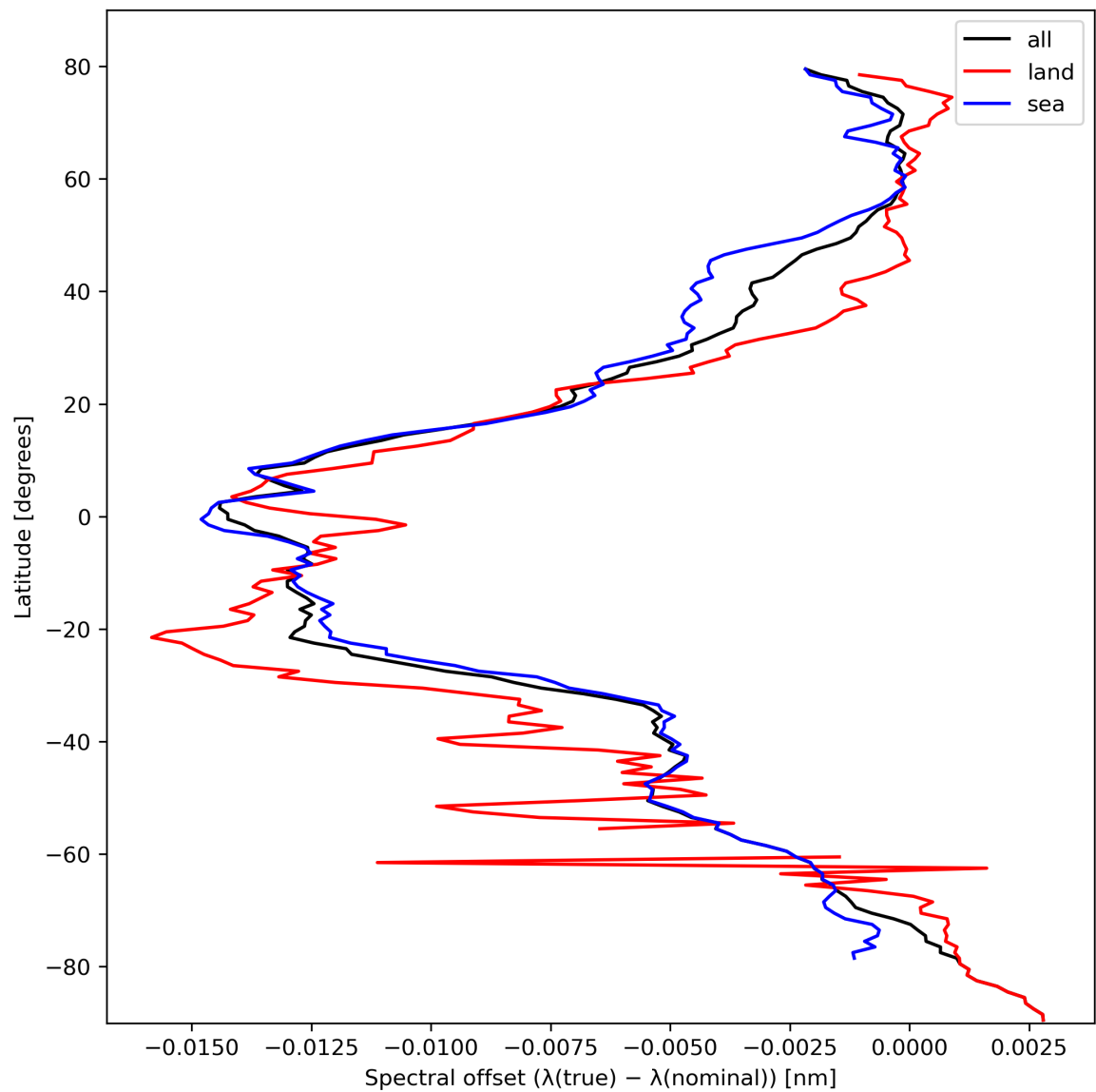
Figure 28: Zonal average of “Spectral offset ( \lambda(\text{true}) - \lambda(\text{nominal}) )” for 2024-02-24 to 2024-02-26.
