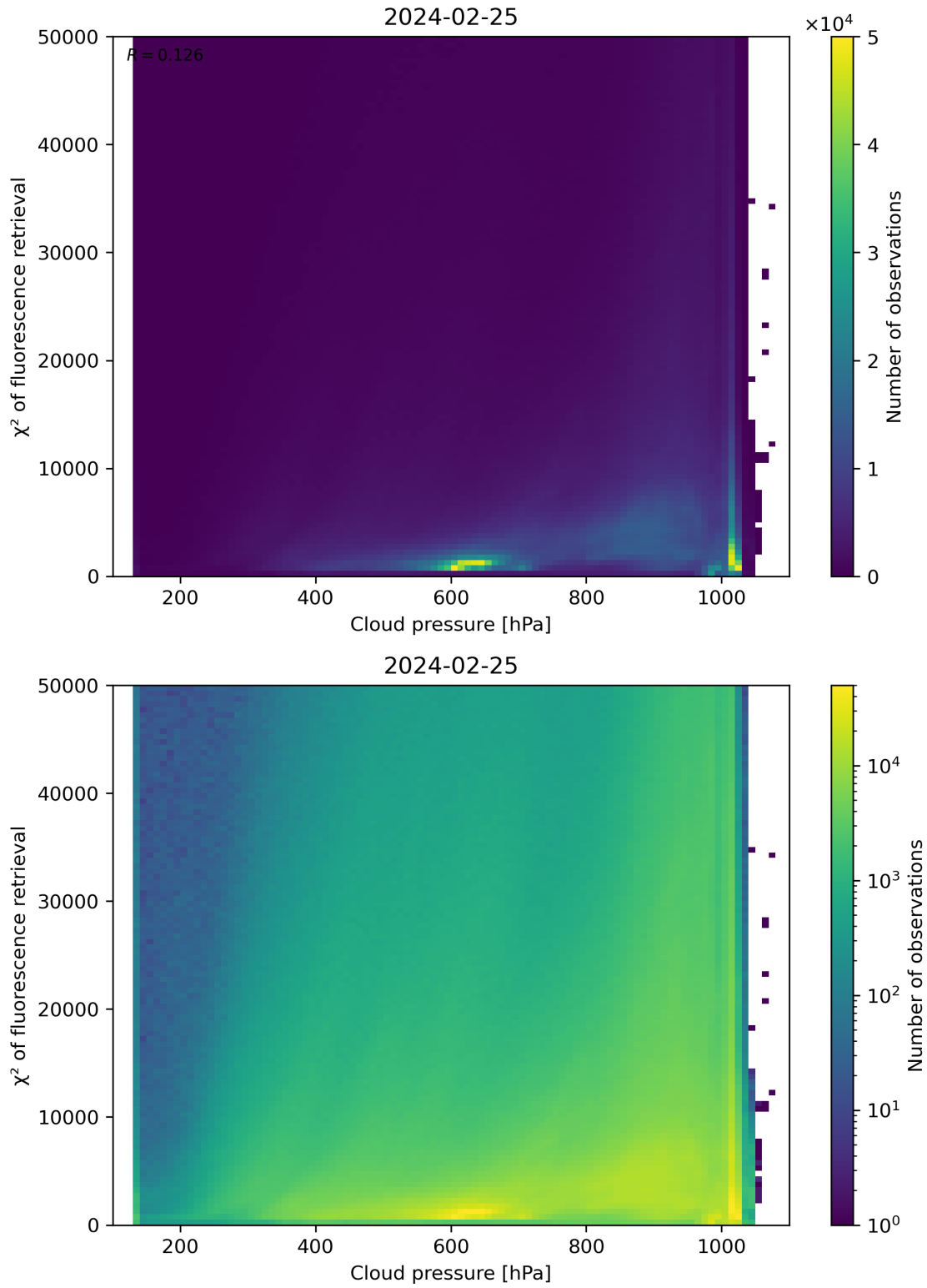
Figure 78: Scatter density plot of “Cloud pressure” against “ \chi^2 of fluorescence retrieval” for 2024-02-24 to 2024-02-26.
