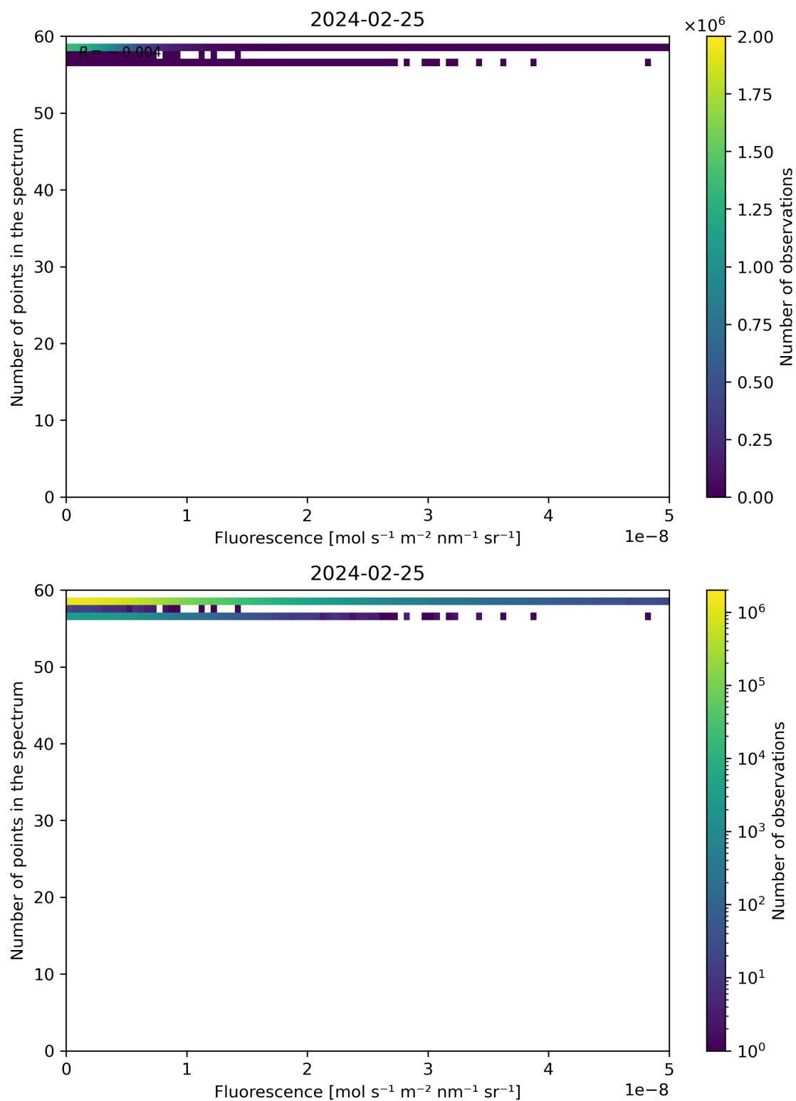
Figure 86: Scatter density plot of “Fluorescence” against “Number of points in the spectrum” for 2024-02-24 to 2024-02-26.
