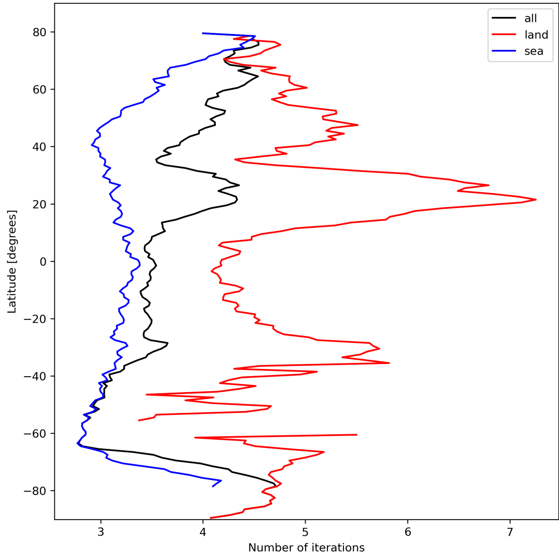
Figure 22: Zonal average of “Number of iterations” for 2024-02-24 to 2024-02-26.
