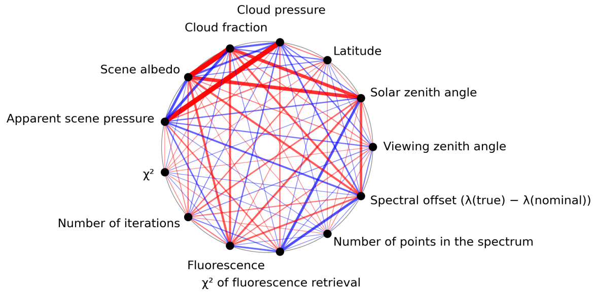
Figure 1: Map of correlation graph for 2024-02-24 to 2024-02-26.
