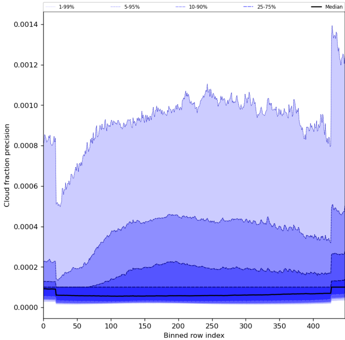
Figure 50: Along track statistics of “Cloud fraction precision” for 2024-02-24 to 2024-02-26
