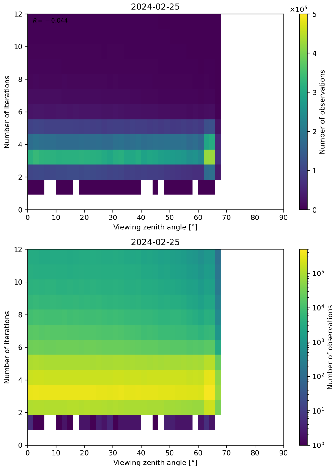
Figure 124: Scatter density plot of “Viewing zenith angle” against “Number of iterations” for 2024-02-24 to 2024-02-26.
