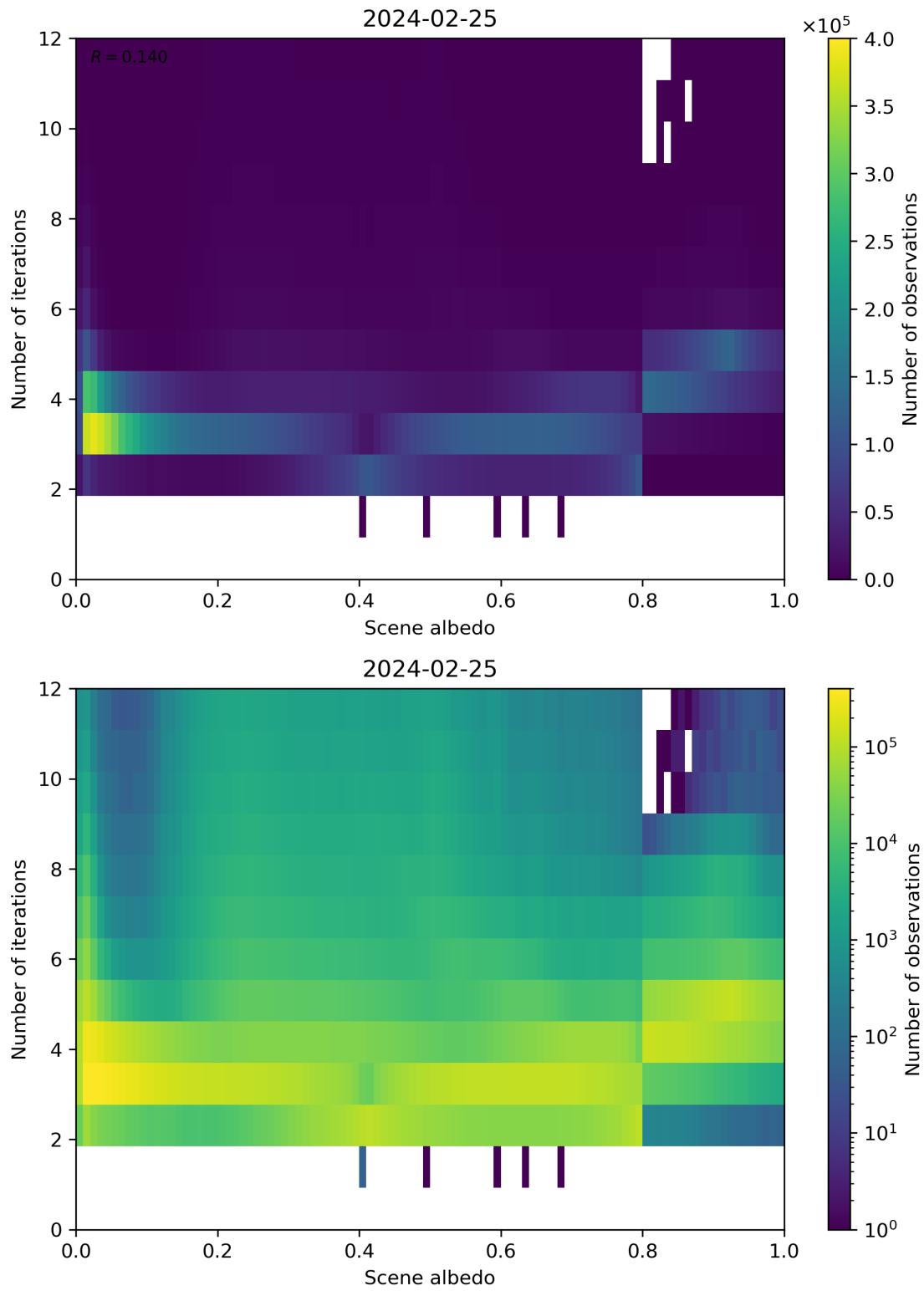
Figure 105: Scatter density plot of “Scene albedo” against “Number of iterations” for 2024-02-24 to 2024-02-26.
