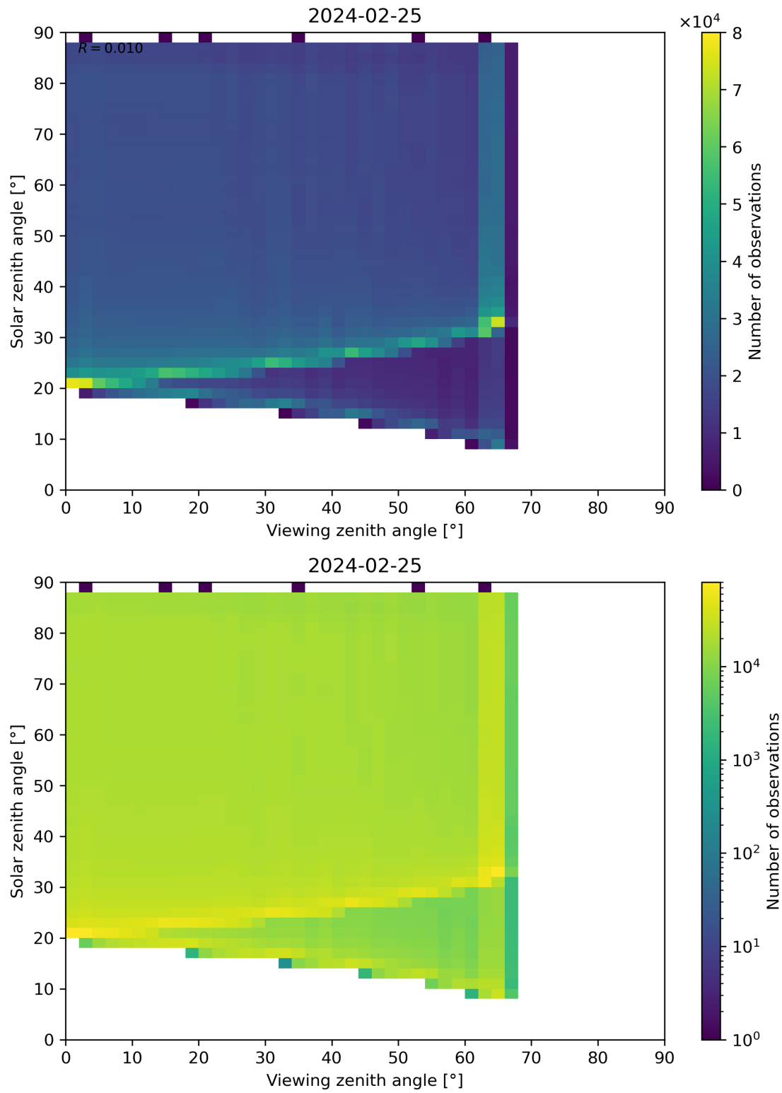
Figure 127: Scatter density plot of “Viewing zenith angle” against “Solar zenith angle” for 2024-02-24 to 2024-02-26.
