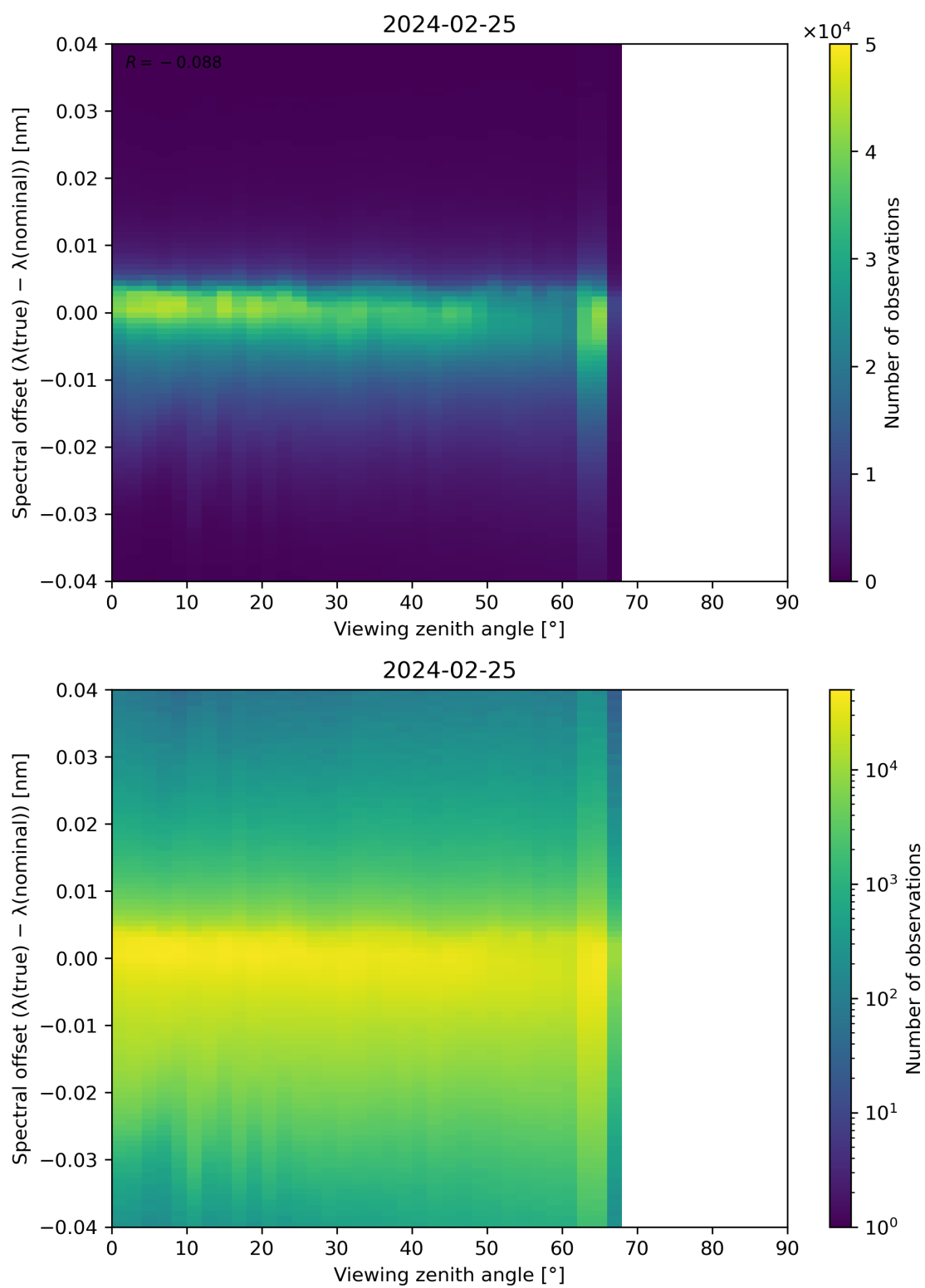
Figure 128: Scatter density plot of “Viewing zenith angle” against “Spectral offset ( \lambda(\text{true}) - \lambda(\text{nominal}) )” for 2024-02-24 to 2024-02-26.
