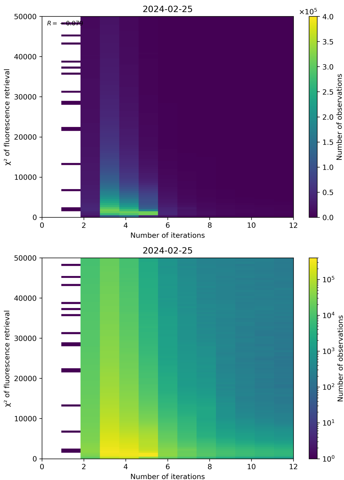
Figure 97: Scatter density plot of “Number of iterations” against “ \chi^2 of fluorescence retrieval” for 2024-02-24 to 2024-02-26.
