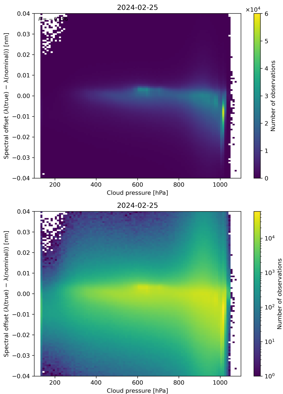
Figure 84: Scatter density plot of “Cloud pressure” against “Spectral offset ( \lambda(\text{true}) - \lambda(\text{nominal}) )” for 2024-02-24 to 2024-02-26.
