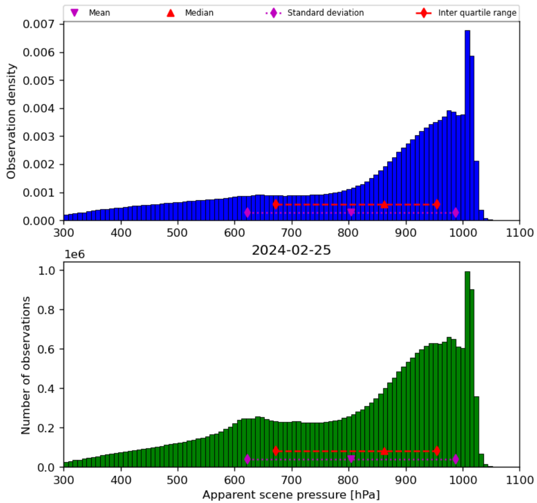
Figure 36: Histogram of “Apparent scene pressure” for 2024-02-24 to 2024-02-26
