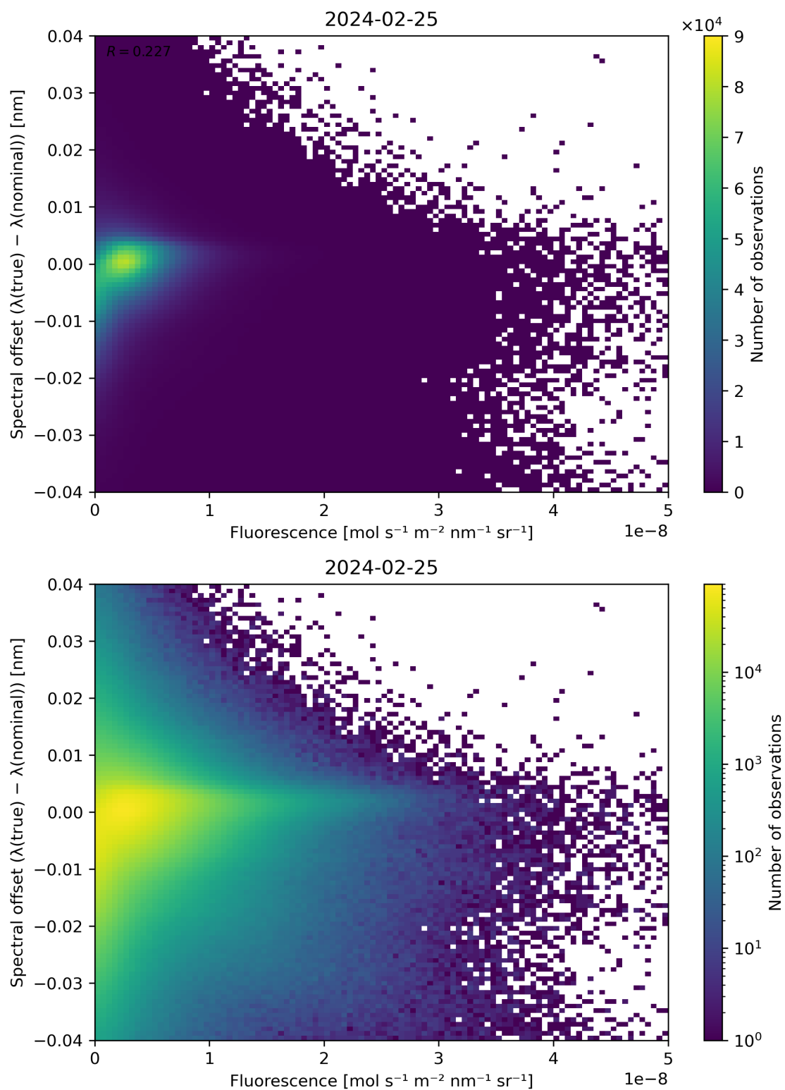
Figure 87: Scatter density plot of “Fluorescence” against “Spectral offset ( \lambda(\text{true}) - \lambda(\text{nominal}) )” for 2024-02-24 to 2024-02-26.
