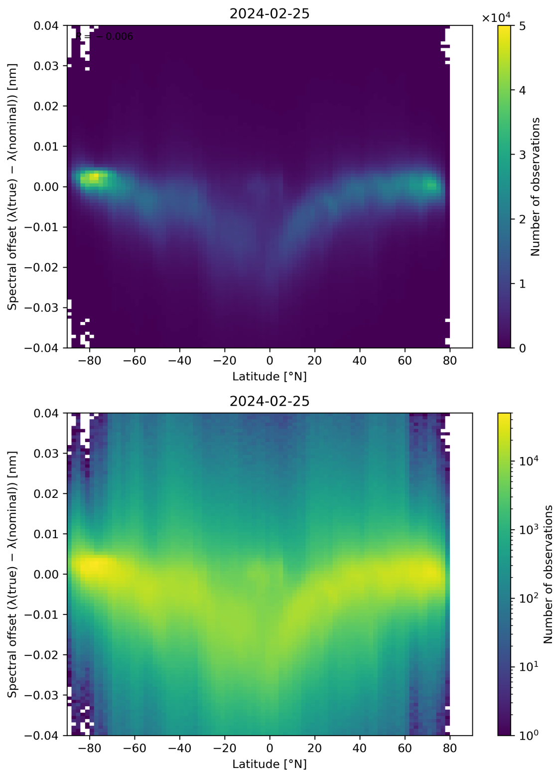
Figure 96: Scatter density plot of “Latitude” against “Spectral offset ( \lambda(\text{true}) - \lambda(\text{nominal}) )” for 2024-02-24 to 2024-02-26.
