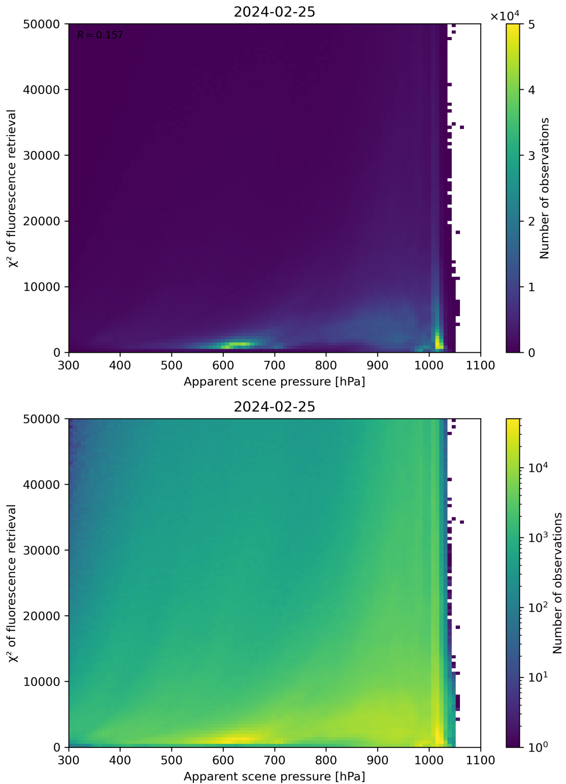
Figure 63: Scatter density plot of “Apparent scene pressure” against “ \chi^2 of fluorescence retrieval” for 2024-02-24 to 2024-02-26.
