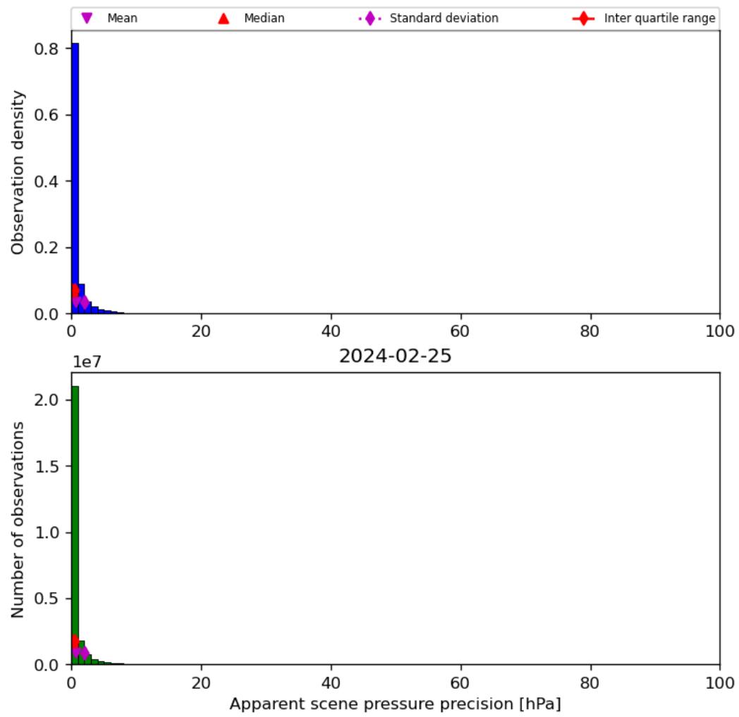
Figure 37: Histogram of “Apparent scene pressure precision” for 2024-02-24 to 2024-02-26
