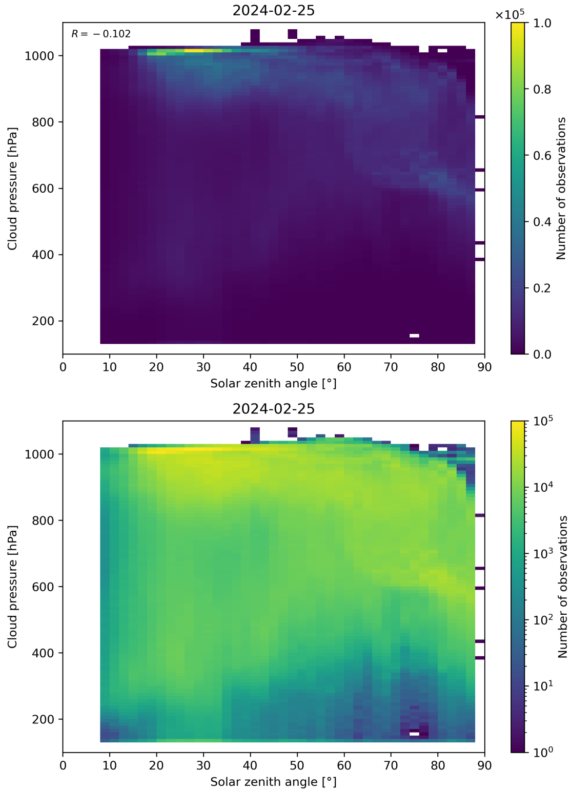
Figure 111: Scatter density plot of “Solar zenith angle” against “Cloud pressure” for 2024-02-24 to 2024-02-26.
