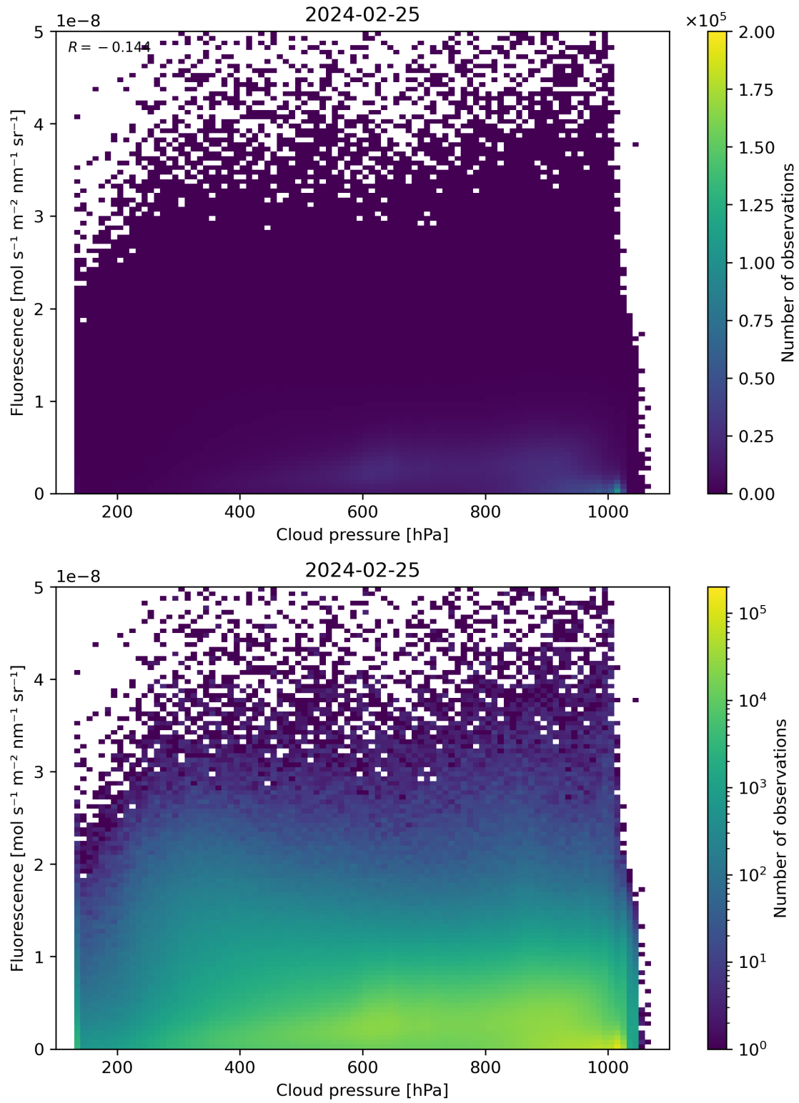
Figure 80: Scatter density plot of “Cloud pressure” against “Fluorescence” for 2024-02-24 to 2024-02-26.
