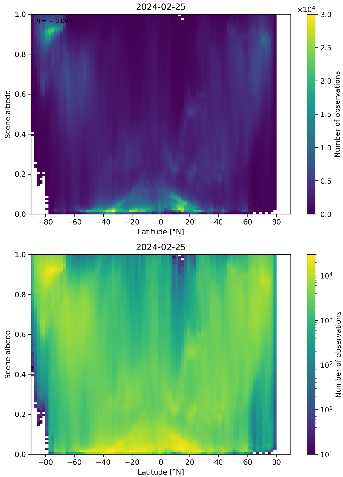
Figure 95: Scatter density plot of “Latitude” against “Scene albedo” for 2024-02-24 to 2024-02-26.
