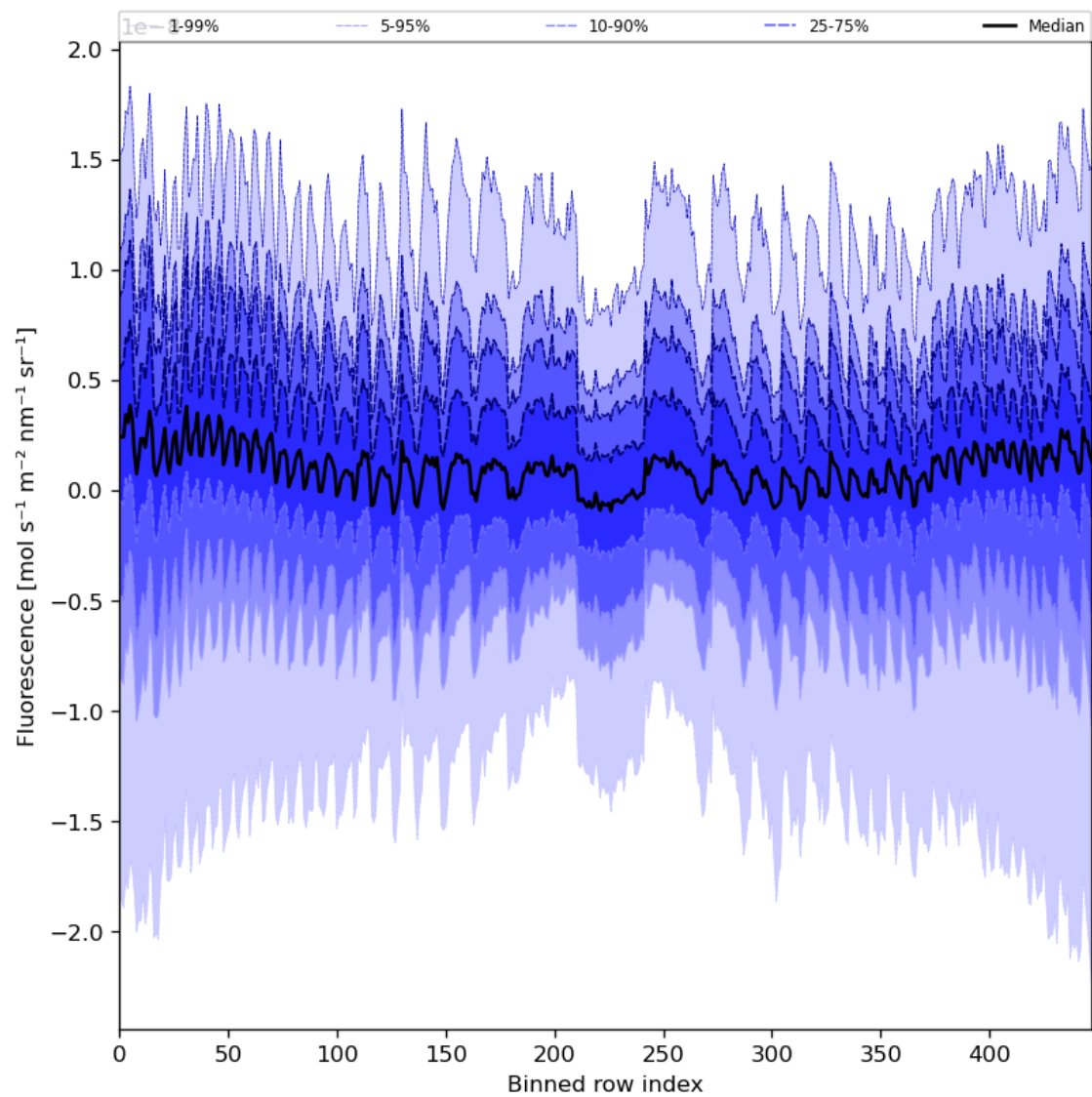
Figure 57: Along track statistics of “Fluorescence” for 2024-02-24 to 2024-02-26
