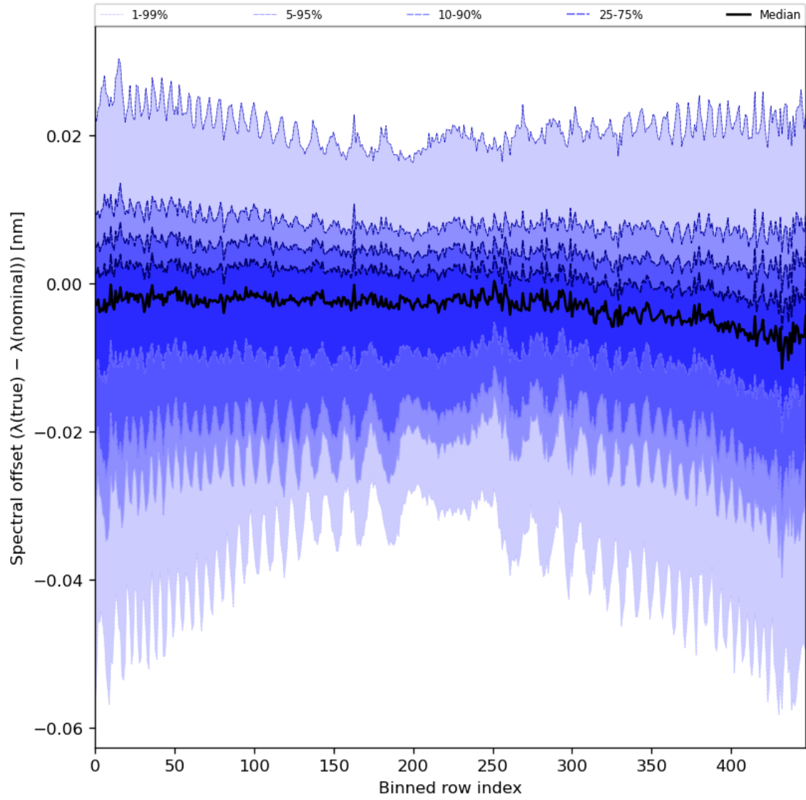
Figure 62: Along track statistics of “Spectral offset ( \lambda(\text{true}) - \lambda(\text{nominal}) )” for 2024-02-24 to 2024-02-26
