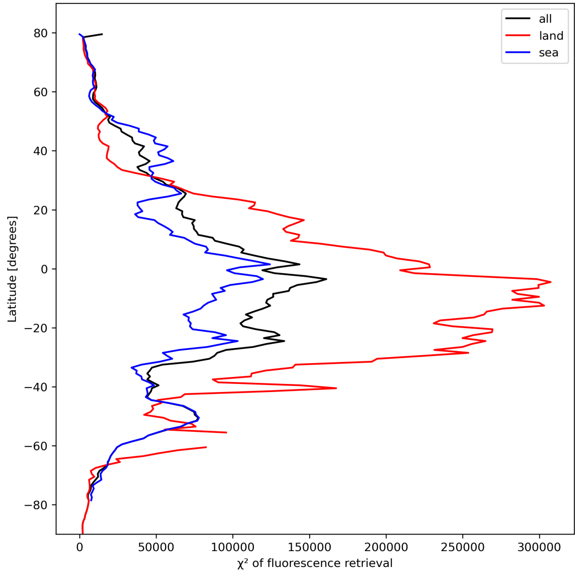
Figure 25: Zonal average of “ \chi^2 of fluorescence retrieval” for 2024-02-24 to 2024-02-26.
