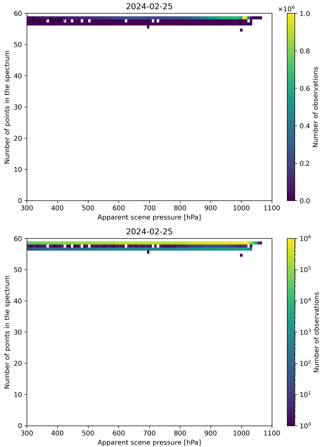
Figure 66: Scatter density plot of “Apparent scene pressure” against “Number of points in the spectrum” for 2024-02-24 to 2024-02-26.
