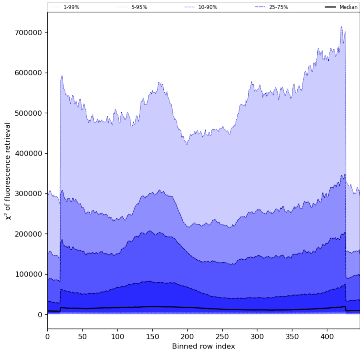
Figure 59: Along track statistics of “ \chi^2 of fluorescence retrieval” for 2024-02-24 to 2024-02-26
