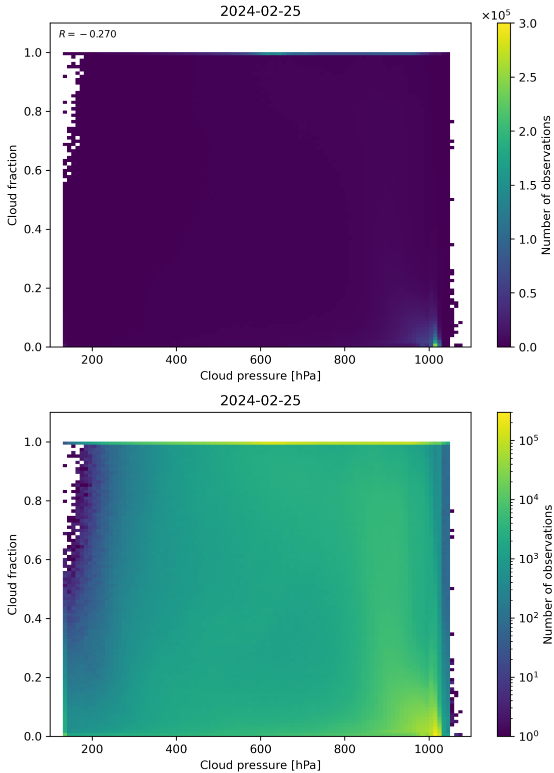
Figure 79: Scatter density plot of “Cloud pressure” against “Cloud fraction” for 2024-02-24 to 2024-02-26.
