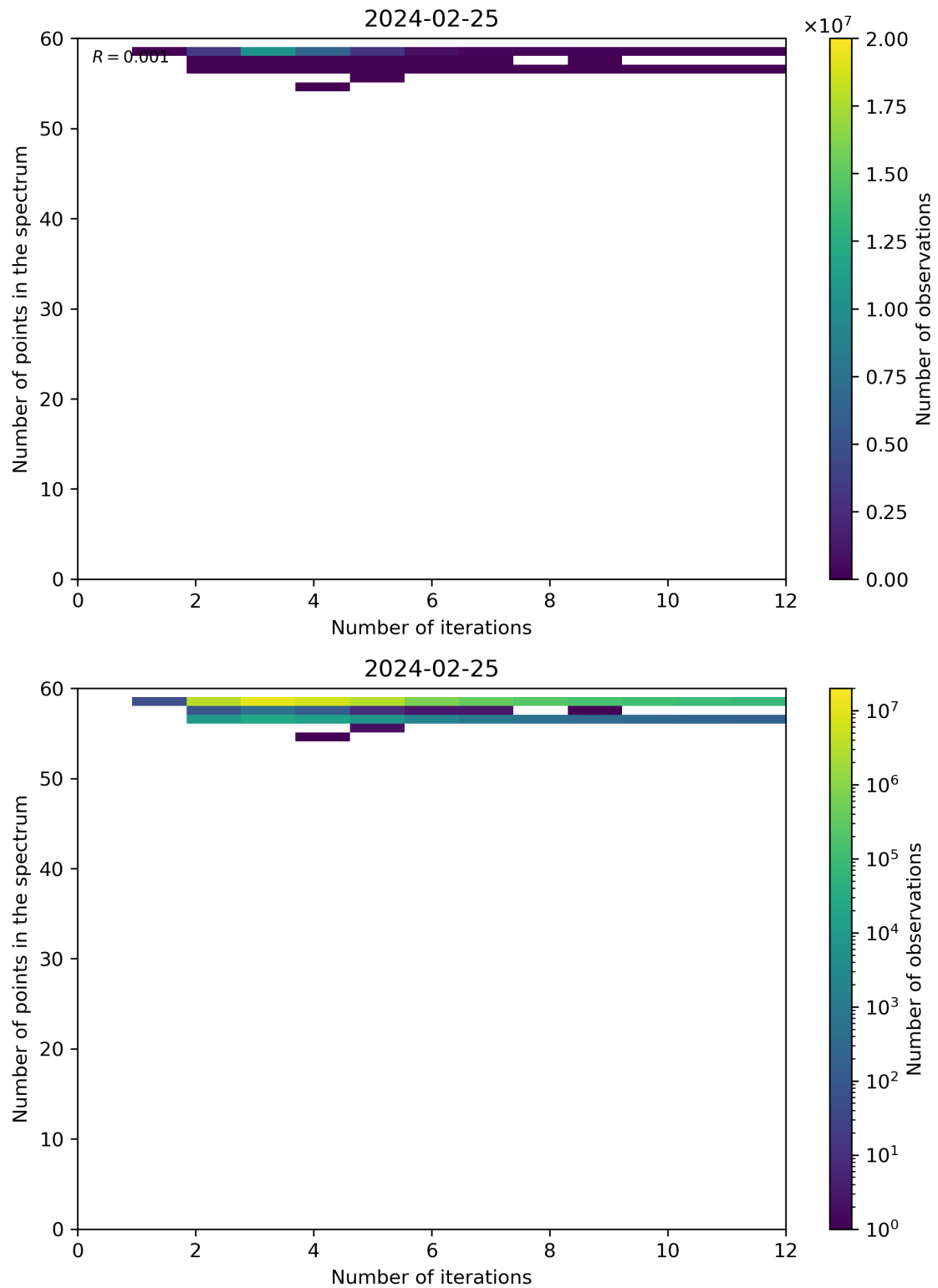
Figure 99: Scatter density plot of “Number of iterations” against “Number of points in the spectrum” for 2024-02-24 to 2024-02-26.
