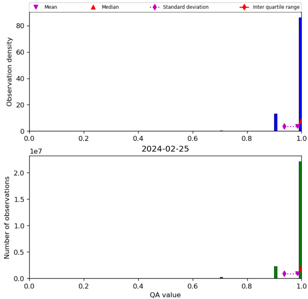
Figure 29: Histogram of “QA value” for 2024-02-24 to 2024-02-26
