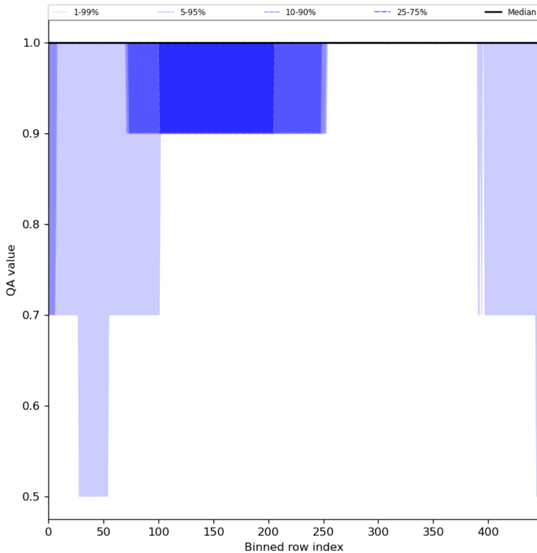
Figure 46: Along track statistics of “QA value” for 2024-02-24 to 2024-02-26
