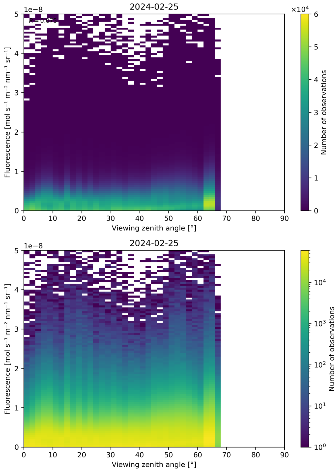
Figure 122: Scatter density plot of “Viewing zenith angle” against “Fluorescence” for 2024-02-24 to 2024-02-26.
