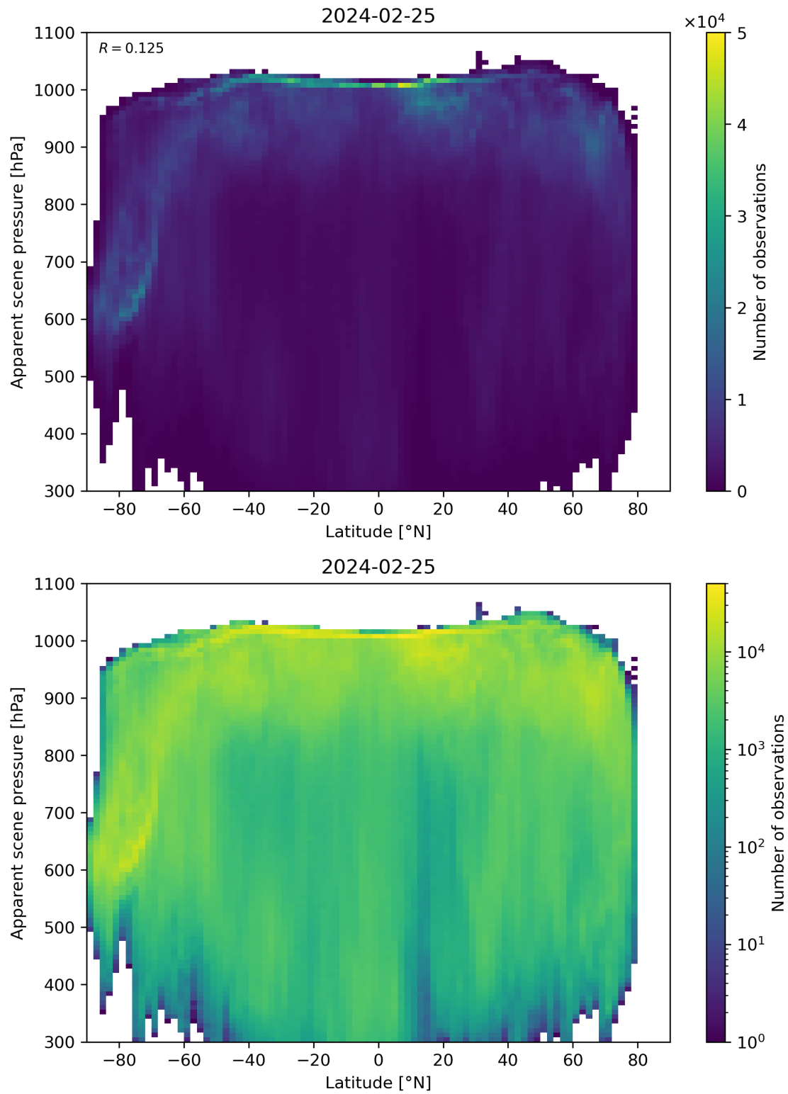
Figure 88: Scatter density plot of “Latitude” against “Apparent scene pressure” for 2024-02-24 to 2024-02-26.
