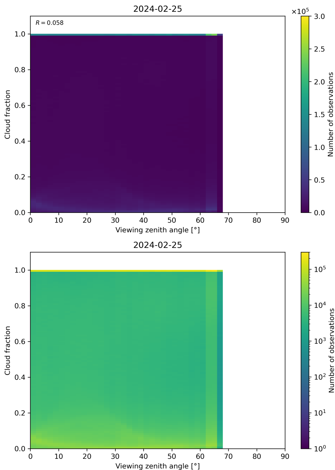
Figure 120: Scatter density plot of “Viewing zenith angle” against “Cloud fraction” for 2024-02-24 to 2024-02-26.
