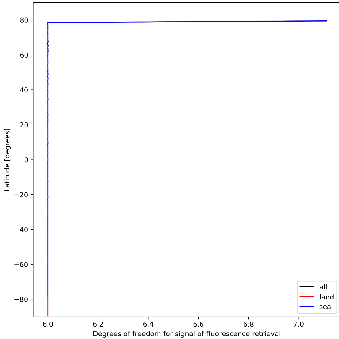
Figure 26: Zonal average of “Degrees of freedom for signal of fluorescence retrieval” for 2024-02-24 to 2024-02-26.
