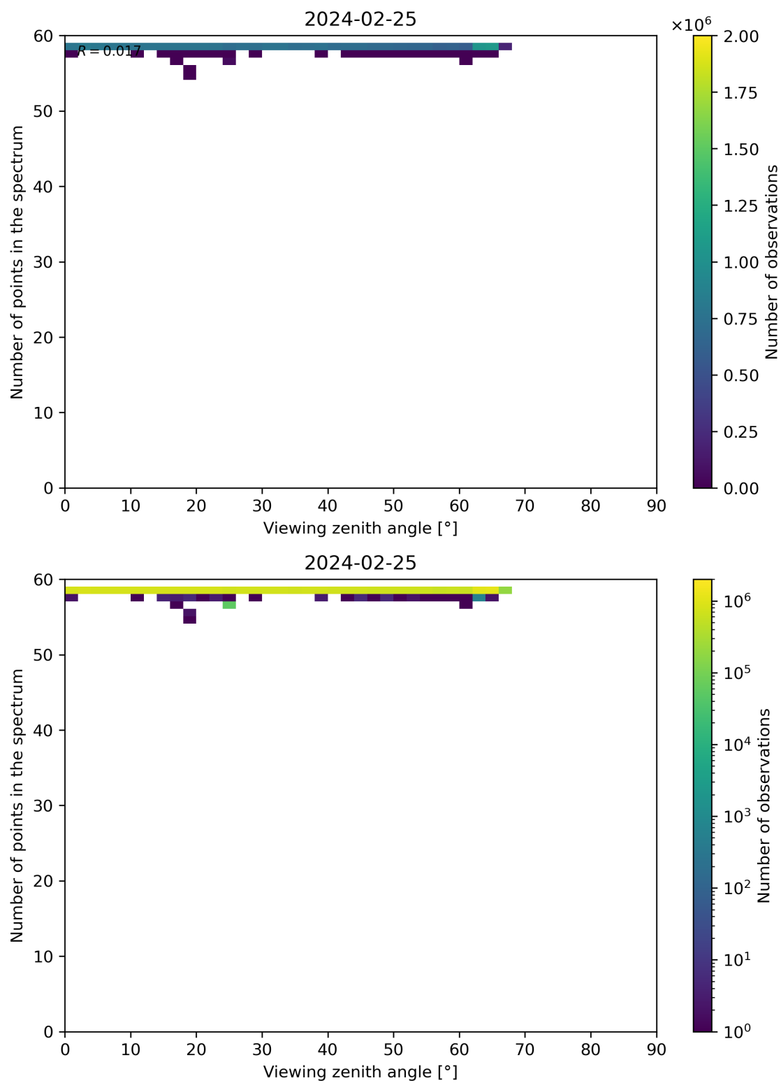
Figure 125: Scatter density plot of “Viewing zenith angle” against “Number of points in the spectrum” for 2024-02-24 to 2024-02-26.
