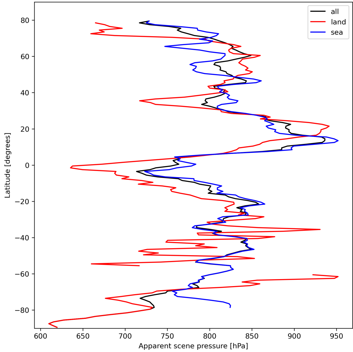
Figure 19: Zonal average of “Apparent scene pressure” for 2024-02-24 to 2024-02-26.
