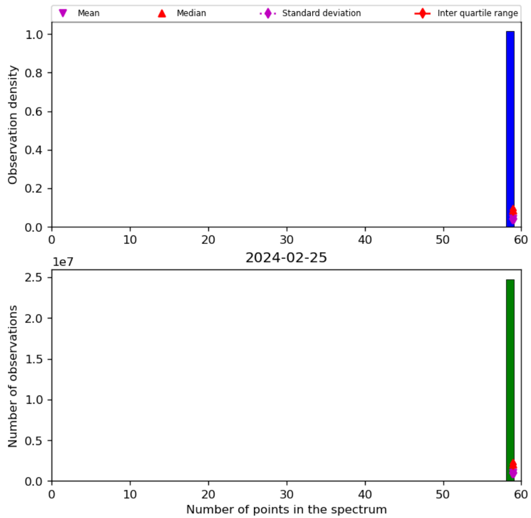
Figure 44: Histogram of “Number of points in the spectrum” for 2024-02-24 to 2024-02-26
