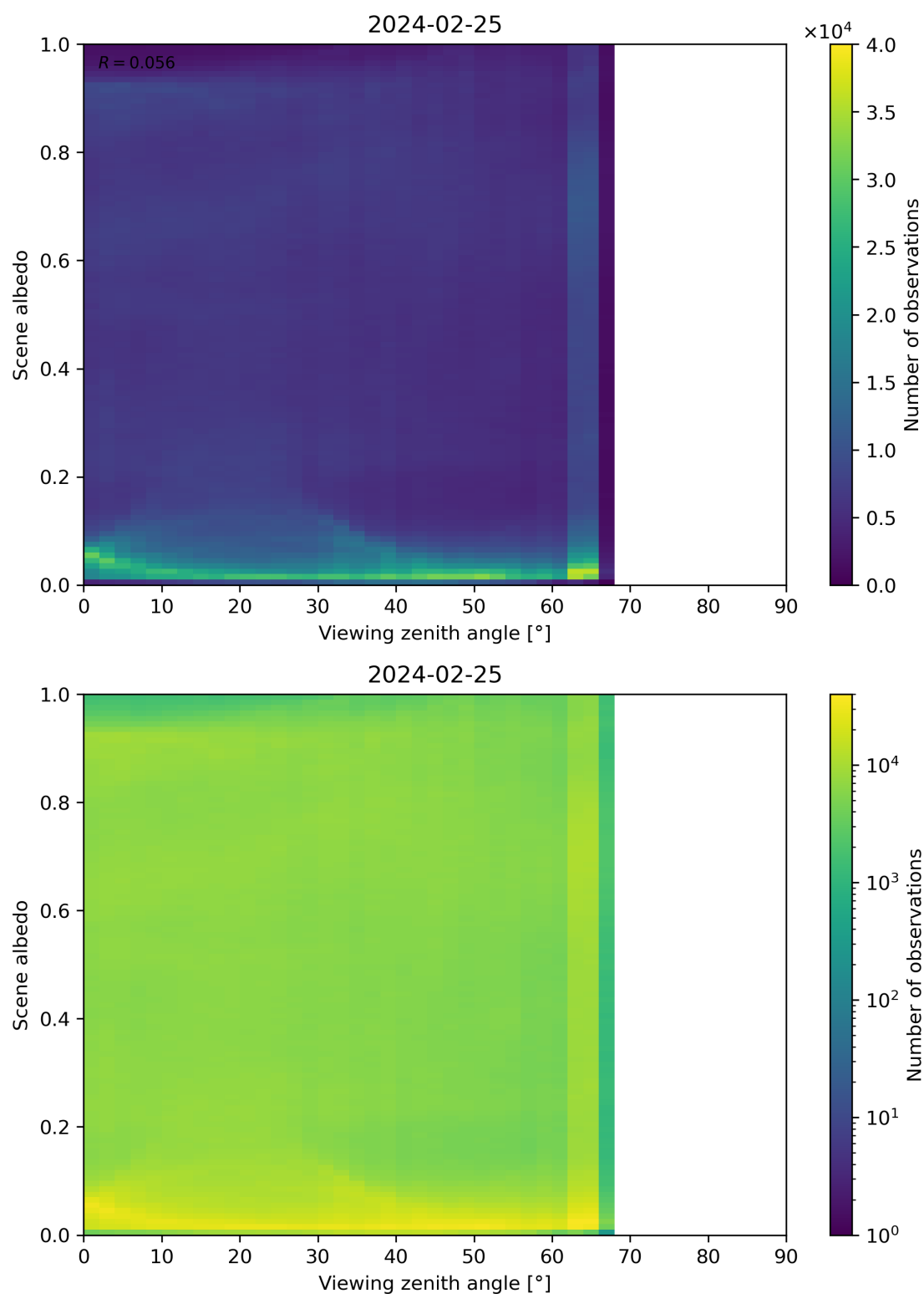
Figure 126: Scatter density plot of “Viewing zenith angle” against “Scene albedo” for 2024-02-24 to 2024-02-26.
