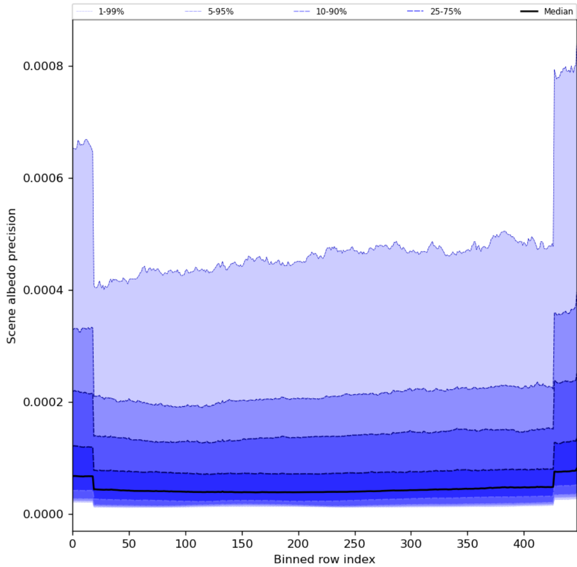
Figure 52: Along track statistics of “Scene albedo precision” for 2024-02-24 to 2024-02-26
