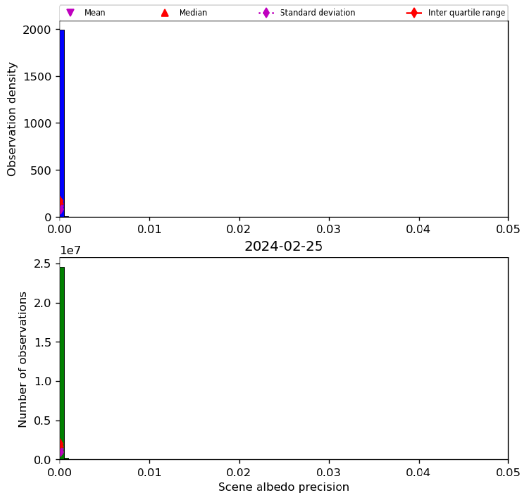
Figure 35: Histogram of “Scene albedo precision” for 2024-02-24 to 2024-02-26
