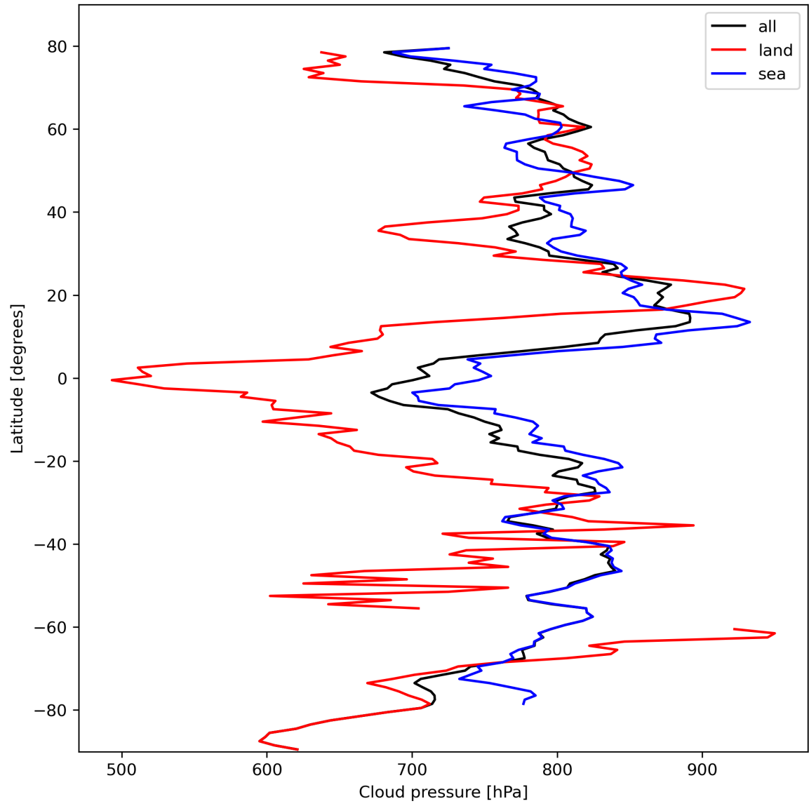
Figure 13: Zonal average of “Cloud pressure” for 2024-02-24 to 2024-02-26.
