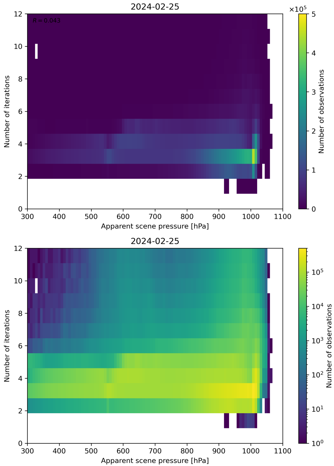
Figure 65: Scatter density plot of “Apparent scene pressure” against “Number of iterations” for 2024-02-24 to 2024-02-26.
