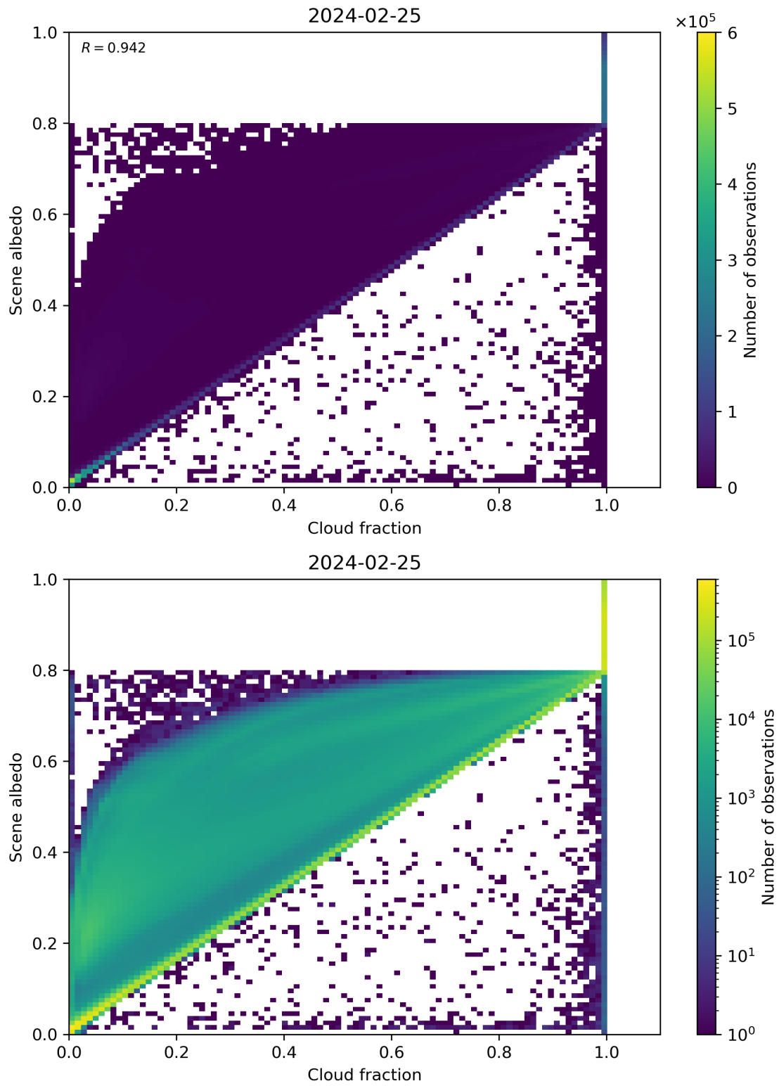
Figure 75: Scatter density plot of “Cloud fraction” against “Scene albedo” for 2024-02-24 to 2024-02-26.
