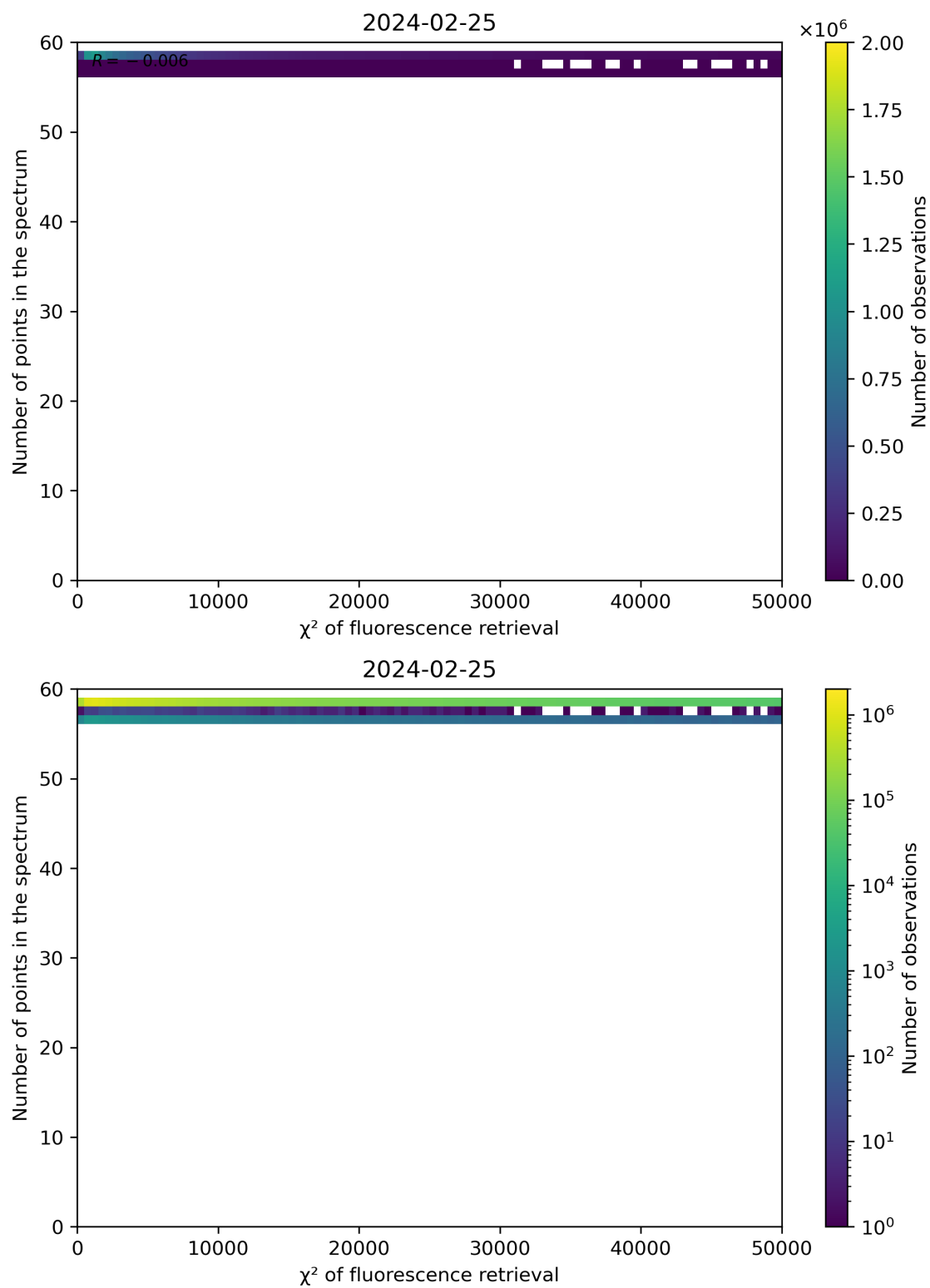
Figure 68: Scatter density plot of " \chi^2 of fluorescence retrieval" against "Number of points in the spectrum" for 2024-02-24 to 2024-02-26.
