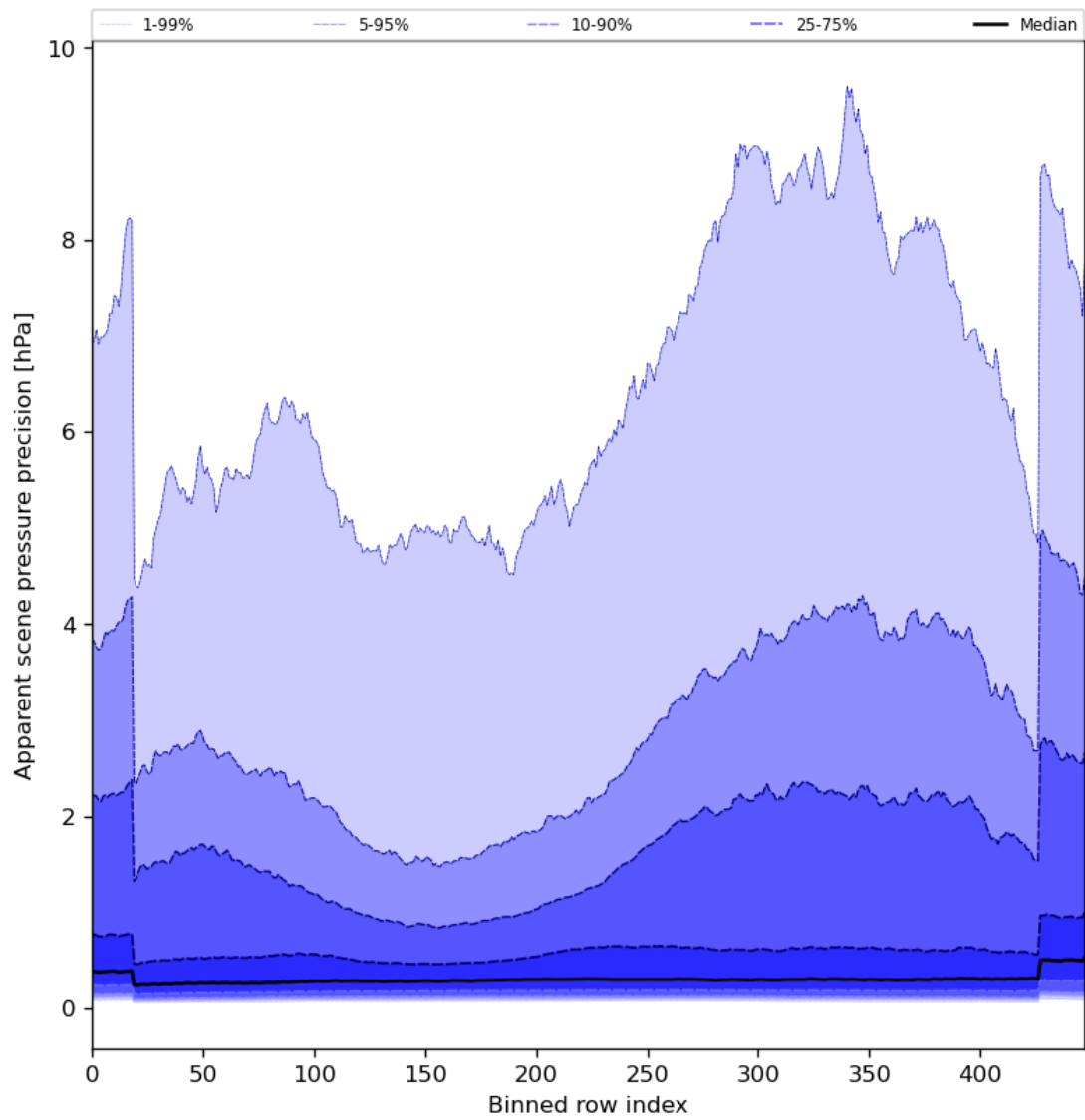
Figure 54: Along track statistics of “Apparent scene pressure precision” for 2024-02-24 to 2024-02-26
