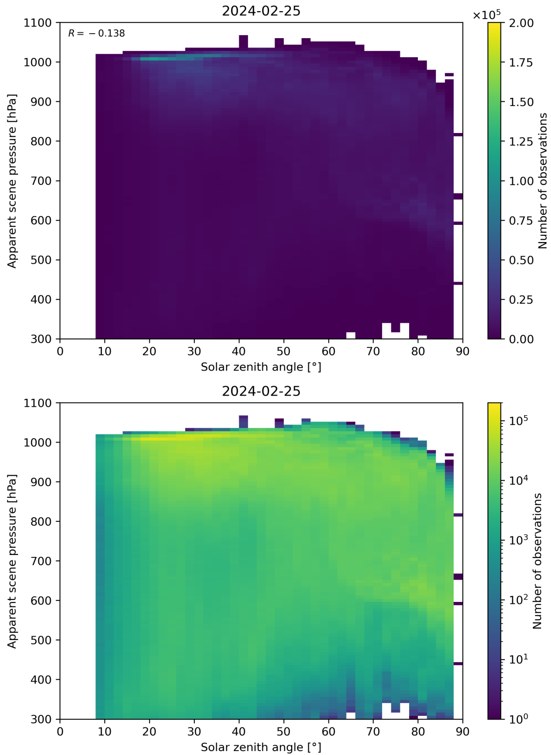
Figure 108: Scatter density plot of “Solar zenith angle” against “Apparent scene pressure” for 2024-02-24 to 2024-02-26.
