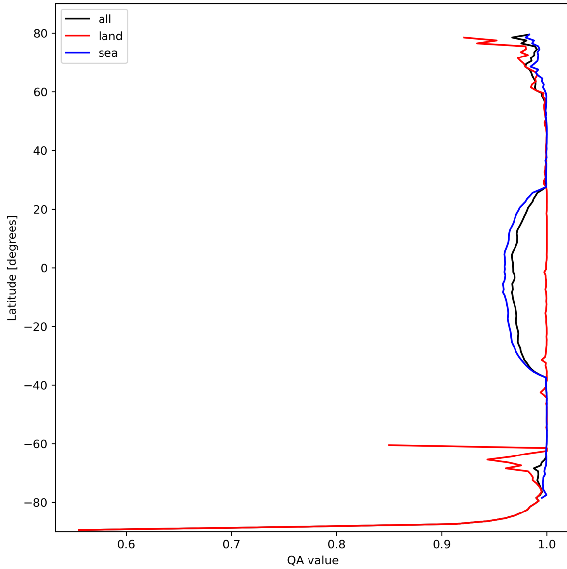
Figure 12: Zonal average of “QA value” for 2024-02-24 to 2024-02-26.
