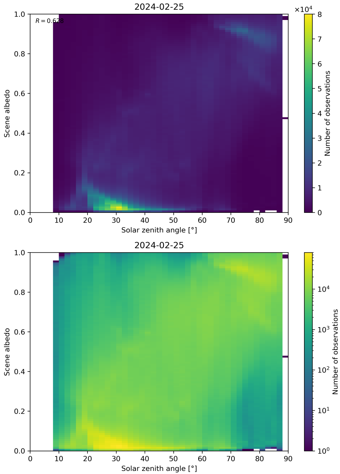
Figure 116: Scatter density plot of “Solar zenith angle” against “Scene albedo” for 2024-02-24 to 2024-02-26.
