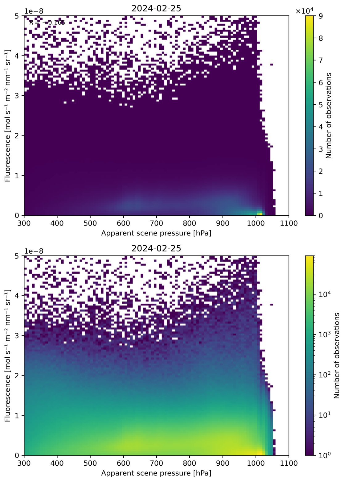
Figure 64: Scatter density plot of “Apparent scene pressure” against “Fluorescence” for 2024-02-24 to 2024-02-26.
