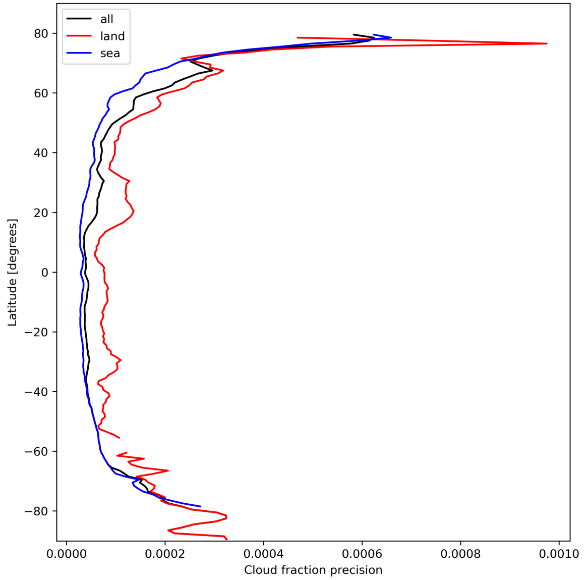
Figure 16: Zonal average of “Cloud fraction precision” for 2024-02-24 to 2024-02-26.
