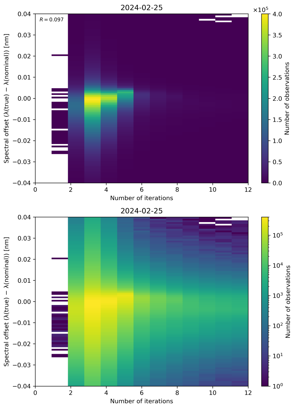
Figure 100: Scatter density plot of “Number of iterations” against “Spectral offset ( \lambda(\text{true}) - \lambda(\text{nominal}) )” for 2024-02-24 to 2024-02-26.
