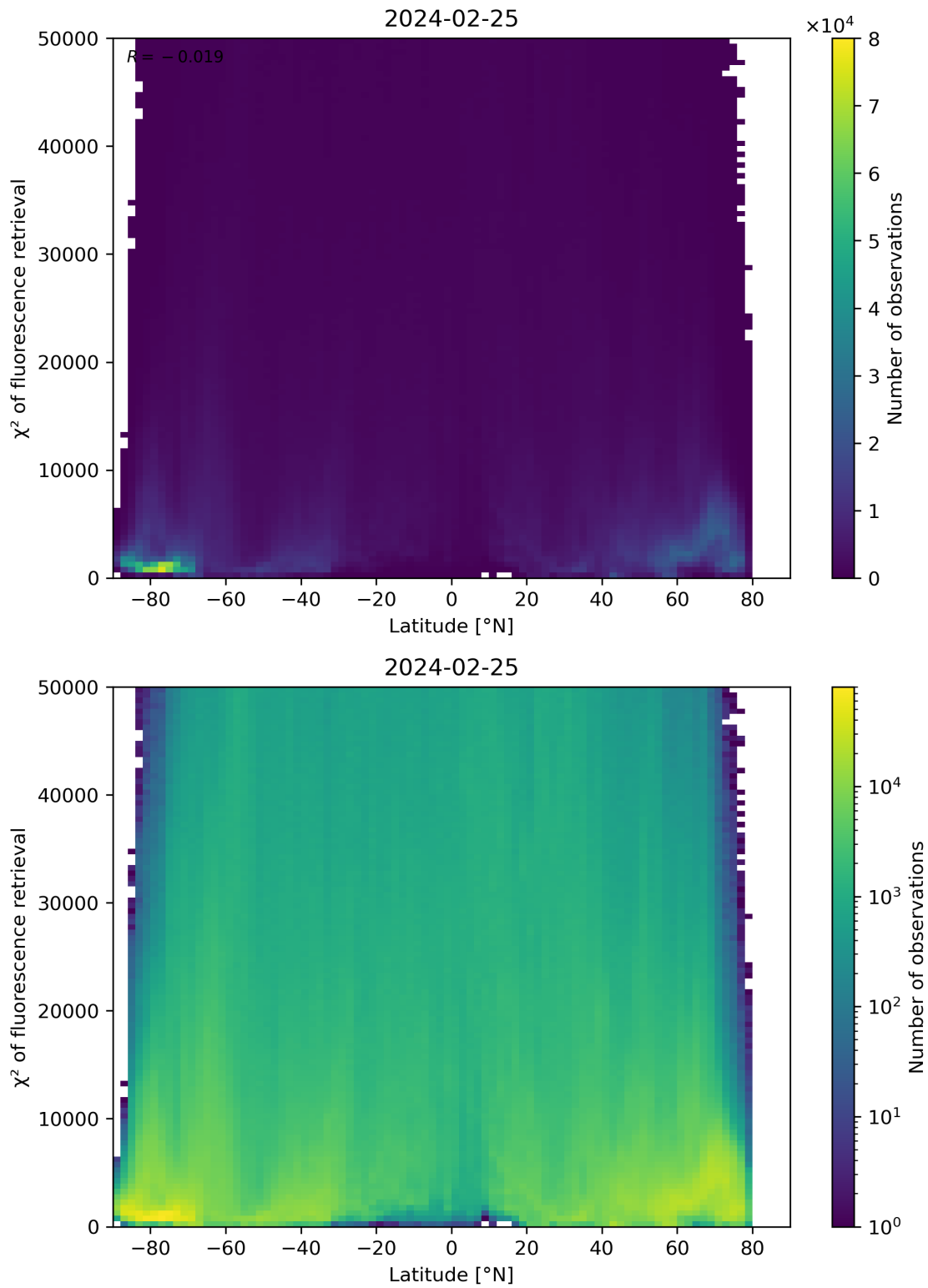
Figure 89: Scatter density plot of “Latitude” against “ \chi^2 of fluorescence retrieval” for 2024-02-24 to 2024-02-26.
