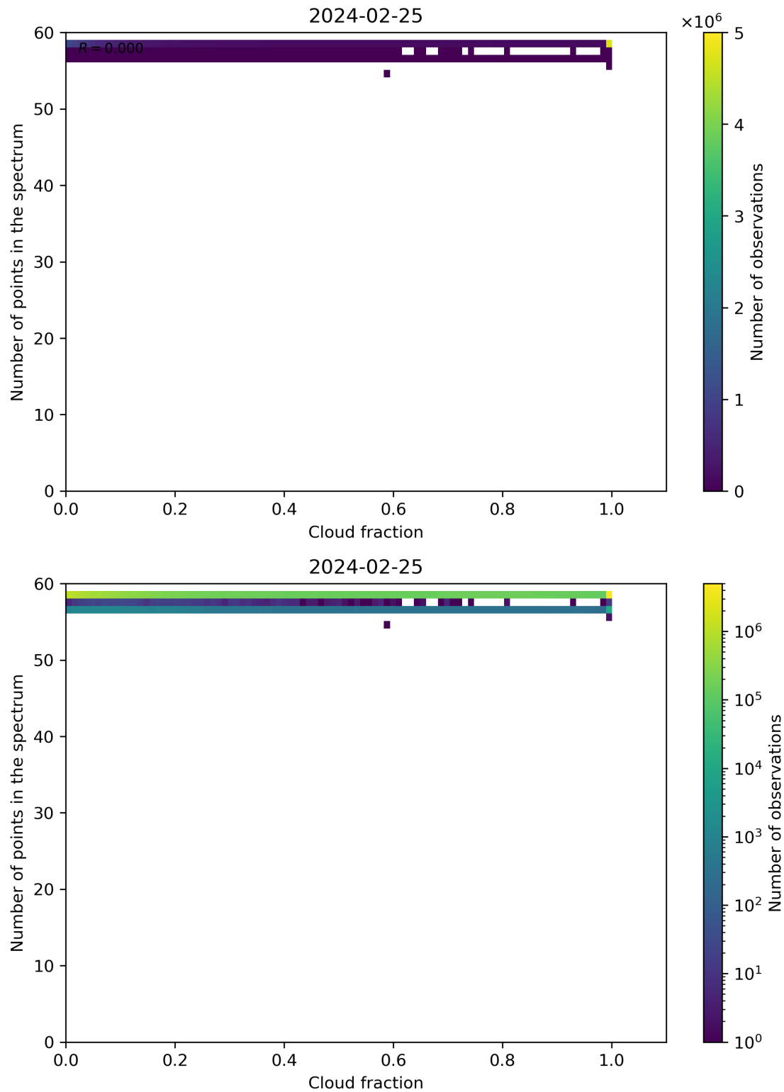
Figure 74: Scatter density plot of “Cloud fraction” against “Number of points in the spectrum” for 2024-02-24 to 2024-02-26.
