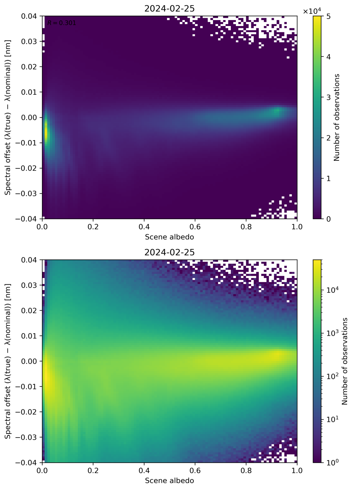
Figure 107: Scatter density plot of “Scene albedo” against “Spectral offset ( \lambda(\text{true}) - \lambda(\text{nominal}) )” for 2024-02-24 to 2024-02-26.
