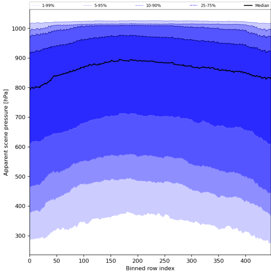
Figure 53: Along track statistics of “Apparent scene pressure” for 2024-02-24 to 2024-02-26
