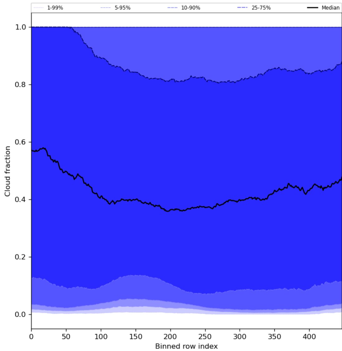
Figure 49: Along track statistics of “Cloud fraction” for 2024-02-24 to 2024-02-26
