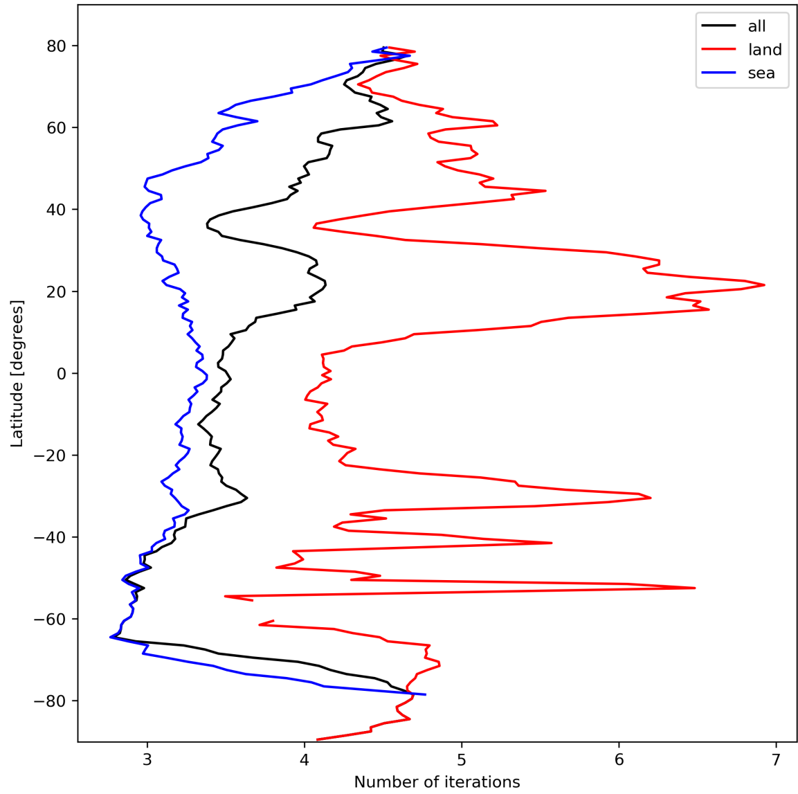
Figure 22: Zonal average of “Number of iterations” for 2024-02-25 to 2024-02-27.
