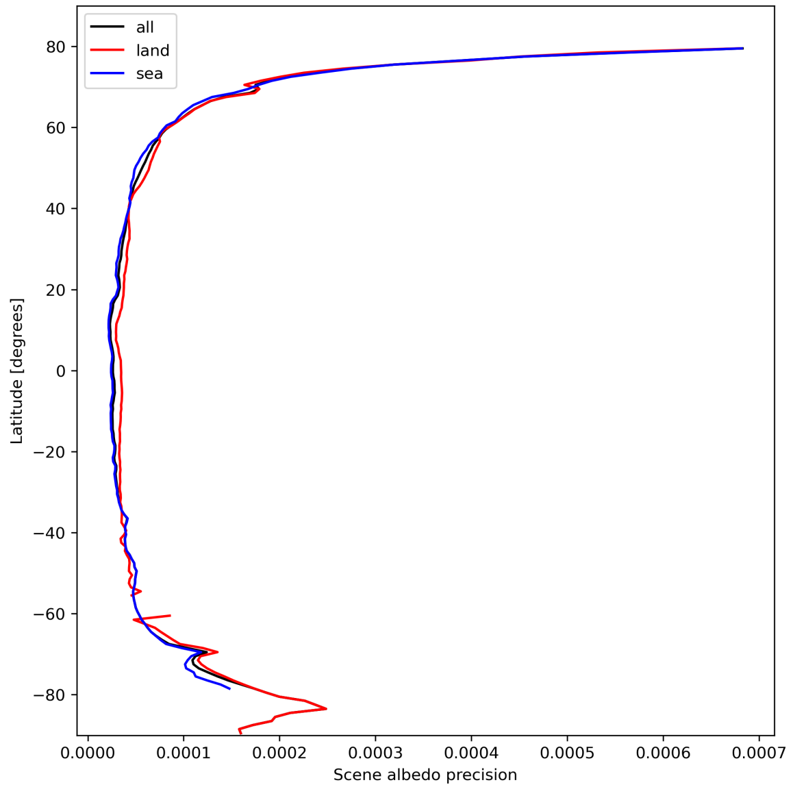
Figure 18: Zonal average of “Scene albedo precision” for 2024-02-25 to 2024-02-27.
