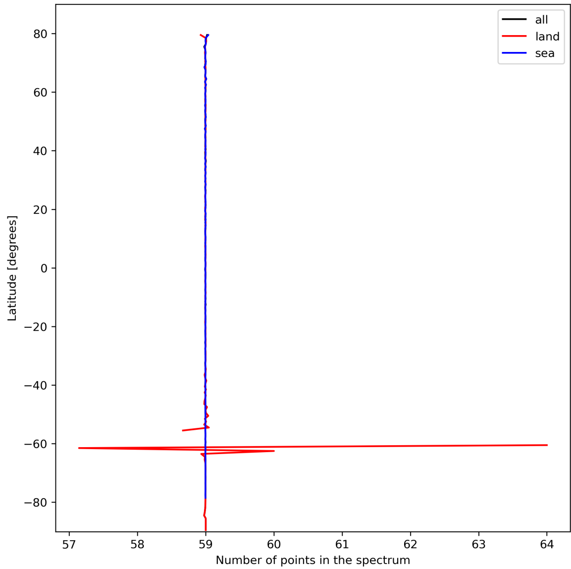
Figure 27: Zonal average of “Number of points in the spectrum” for 2024-02-25 to 2024-02-27.
