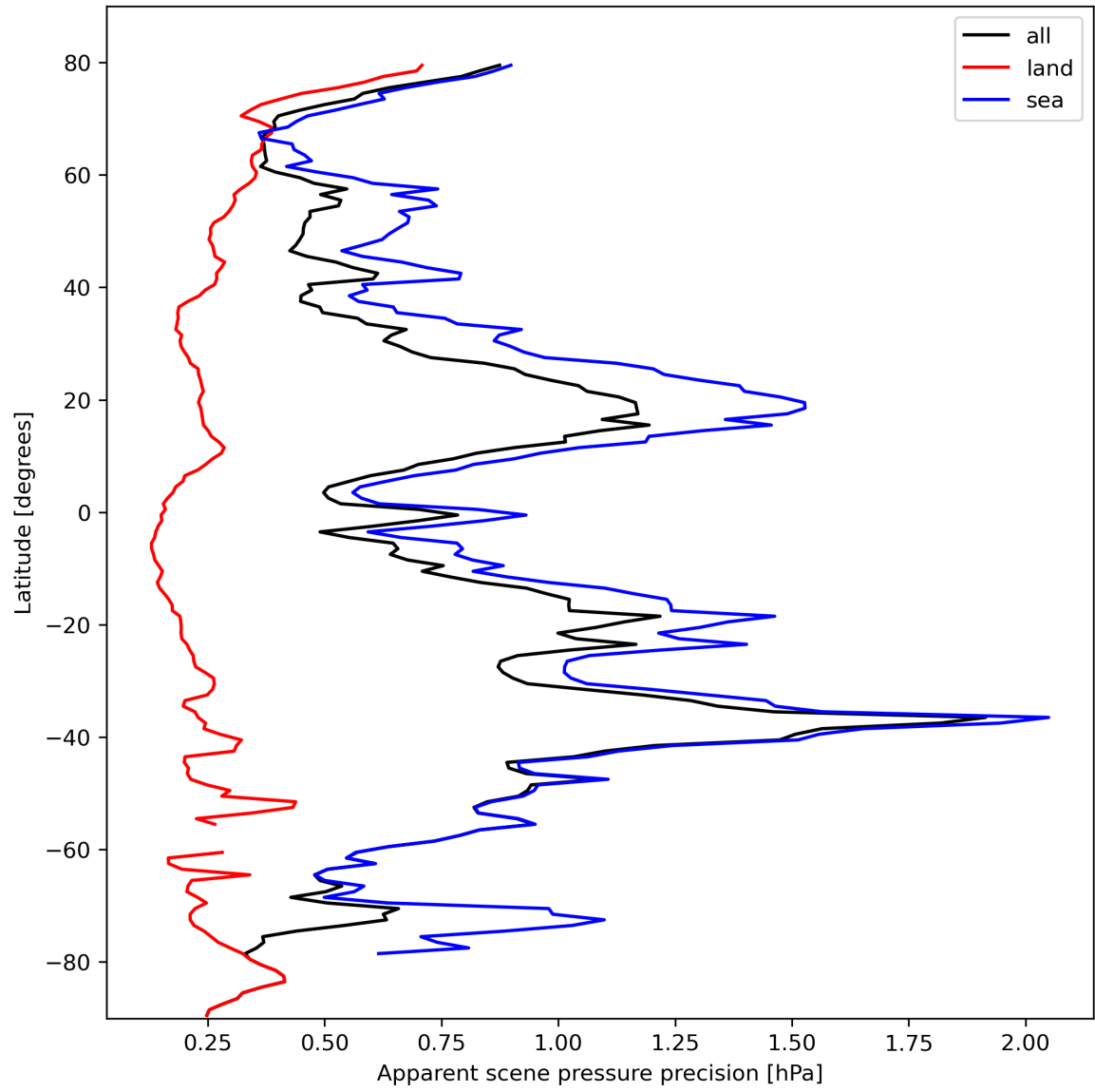
Figure 20: Zonal average of “Apparent scene pressure precision” for 2024-02-25 to 2024-02-27.
