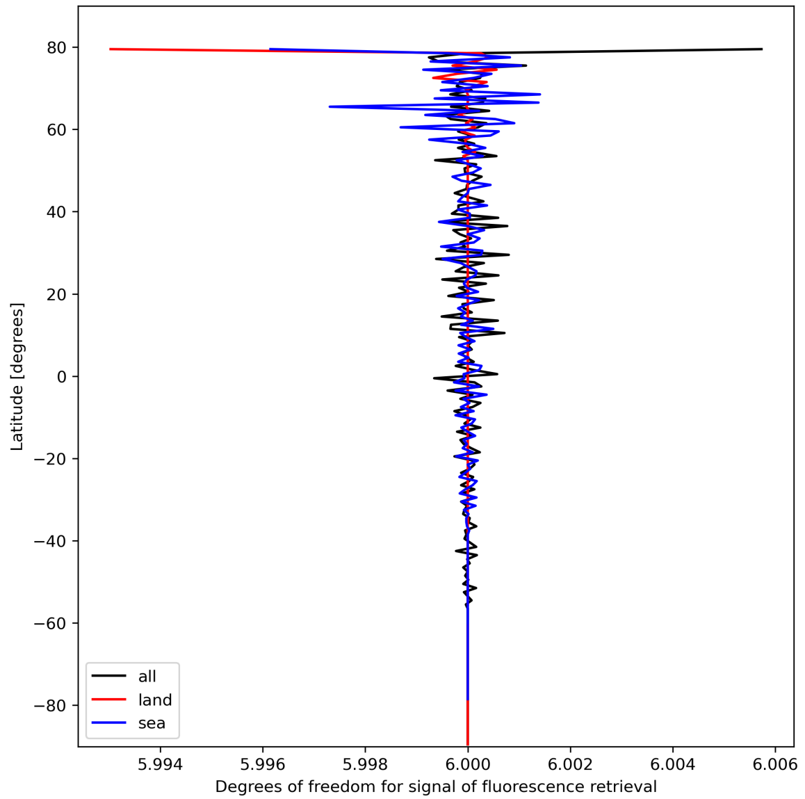
Figure 26: Zonal average of “Degrees of freedom for signal of fluorescence retrieval” for 2024-02-25 to 2024-02-27.
