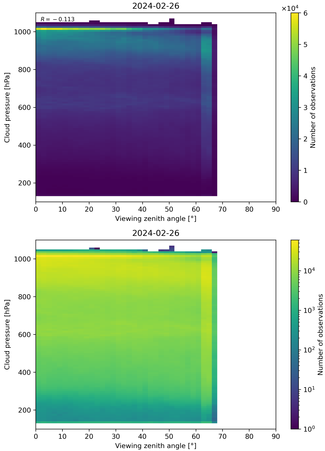
Figure 121: Scatter density plot of “Viewing zenith angle” against “Cloud pressure” for 2024-02-25 to 2024-02-27.
