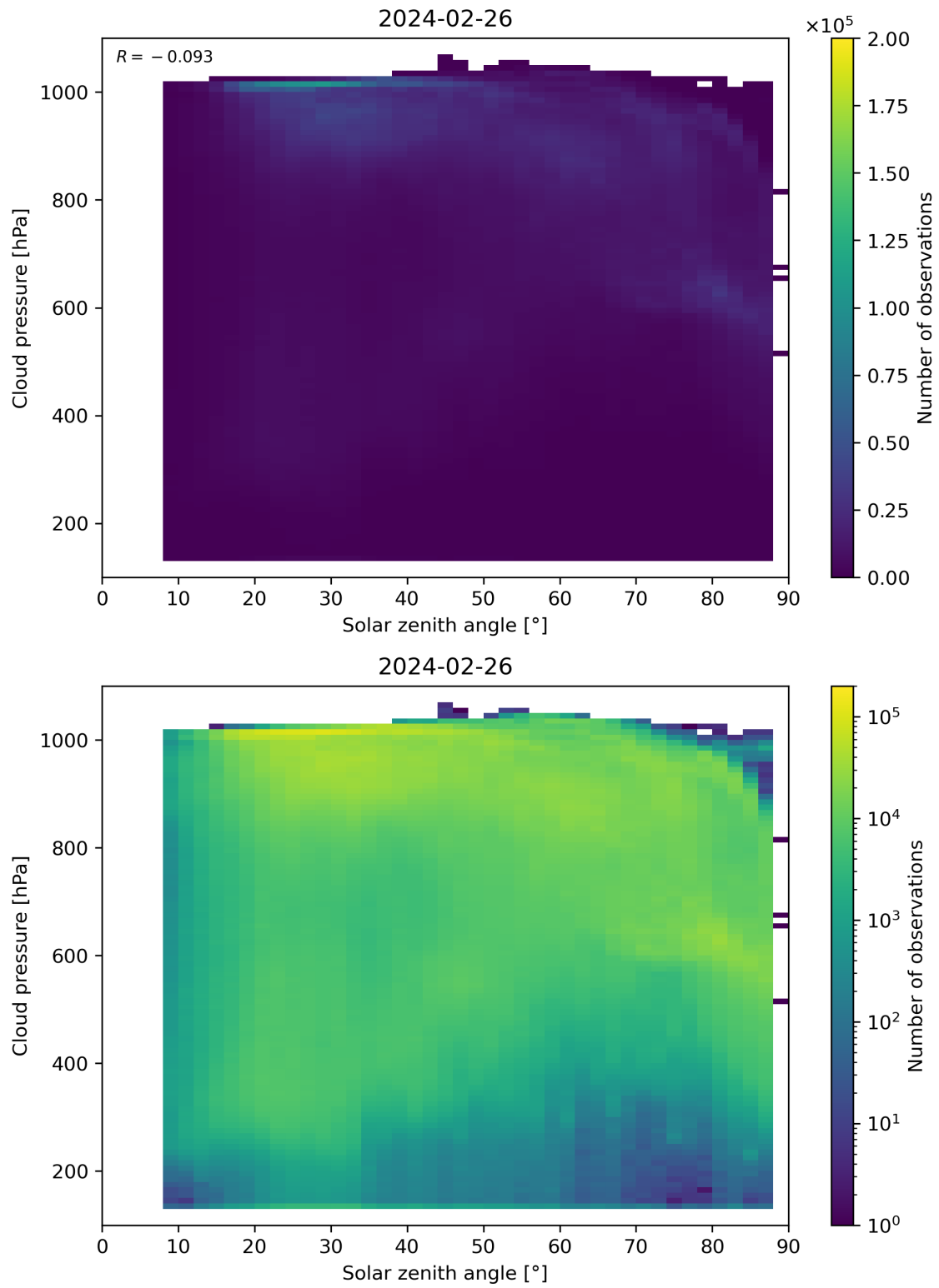
Figure 111: Scatter density plot of “Solar zenith angle” against “Cloud pressure” for 2024-02-25 to 2024-02-27.
