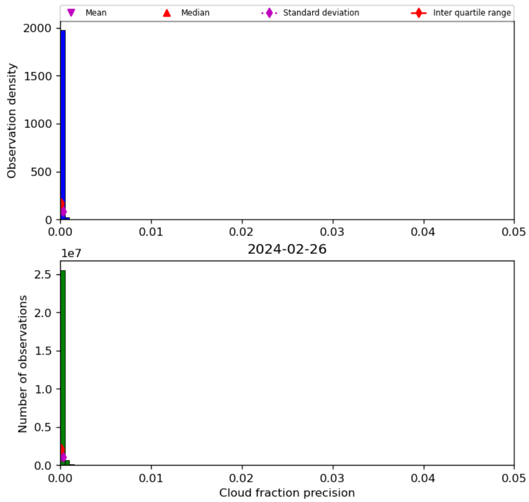
Figure 33: Histogram of “Cloud fraction precision” for 2024-02-25 to 2024-02-27
