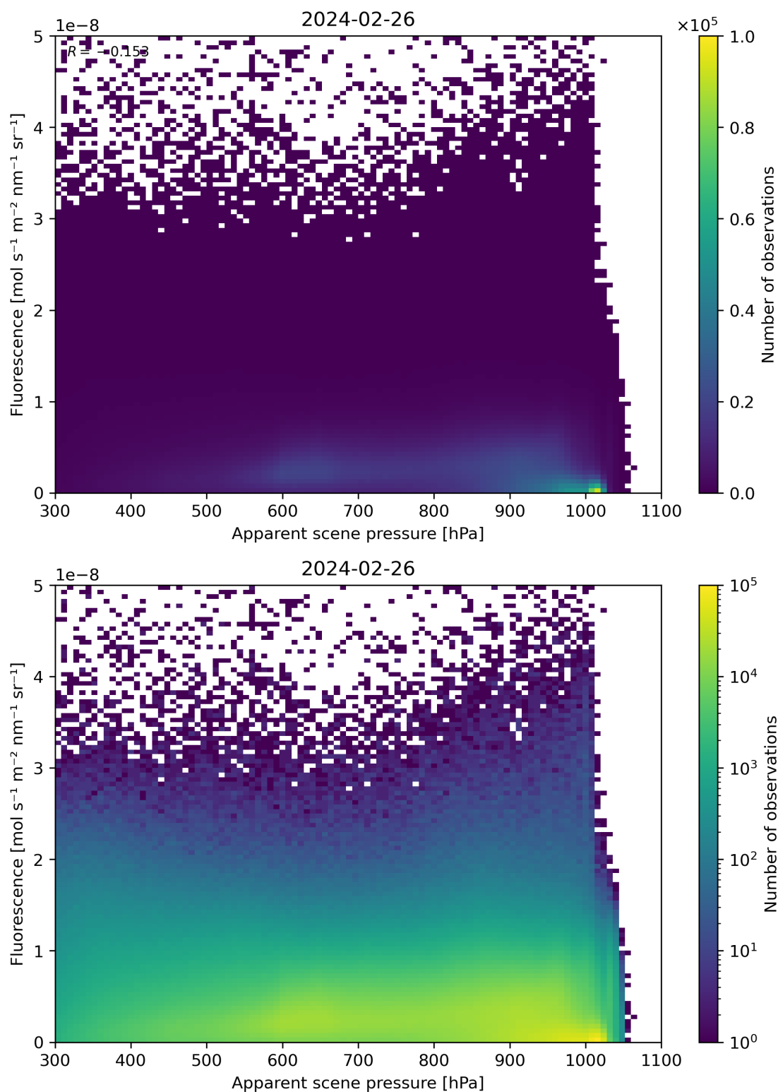
Figure 64: Scatter density plot of “Apparent scene pressure” against “Fluorescence” for 2024-02-25 to 2024-02-27.
