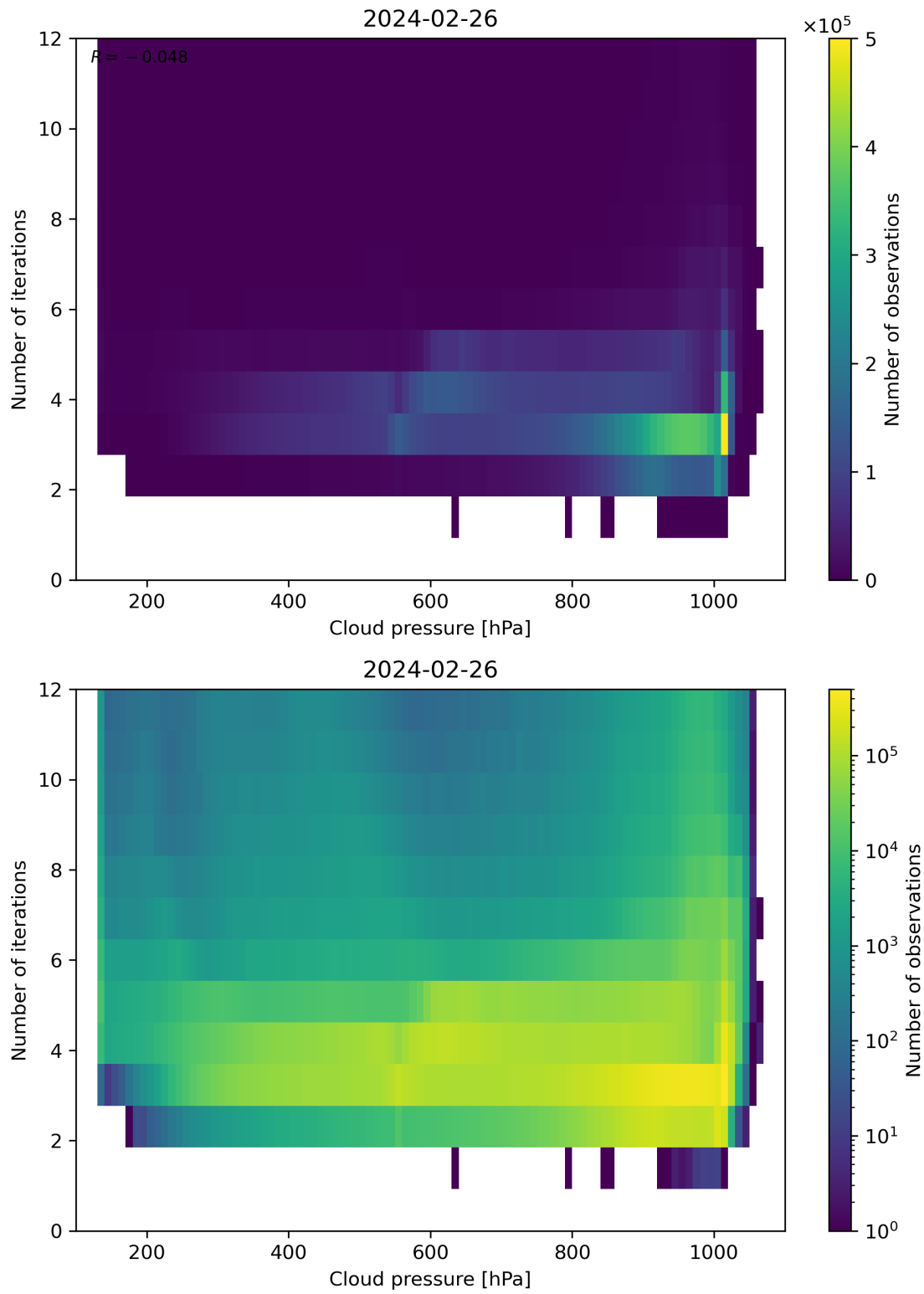
Figure 81: Scatter density plot of “Cloud pressure” against “Number of iterations” for 2024-02-25 to 2024-02-27.
