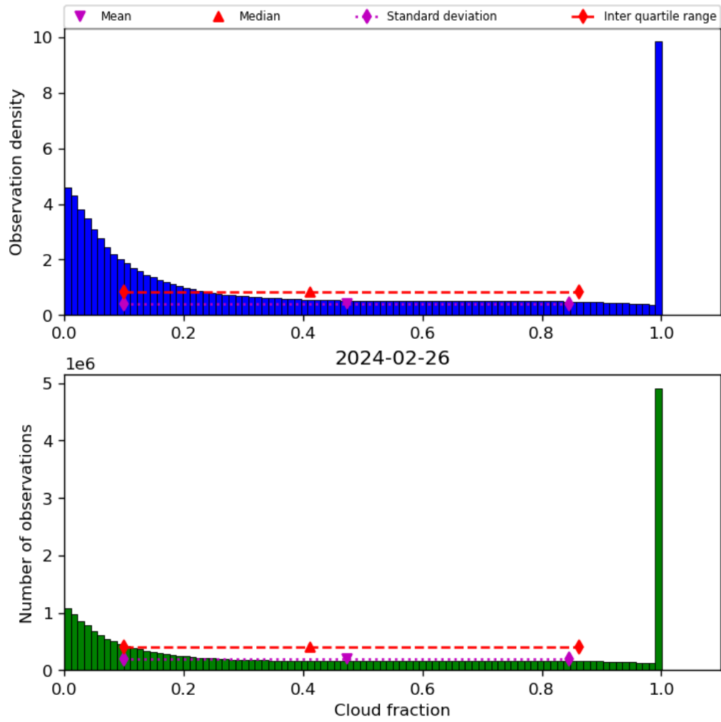
Figure 32: Histogram of “Cloud fraction” for 2024-02-25 to 2024-02-27
