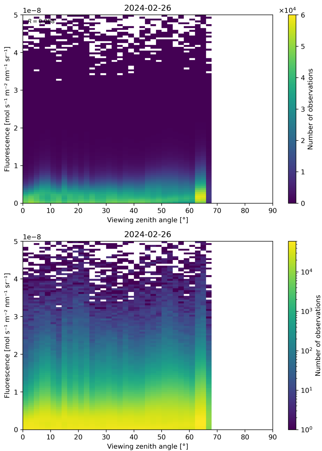
Figure 122: Scatter density plot of “Viewing zenith angle” against “Fluorescence” for 2024-02-25 to 2024-02-27.
