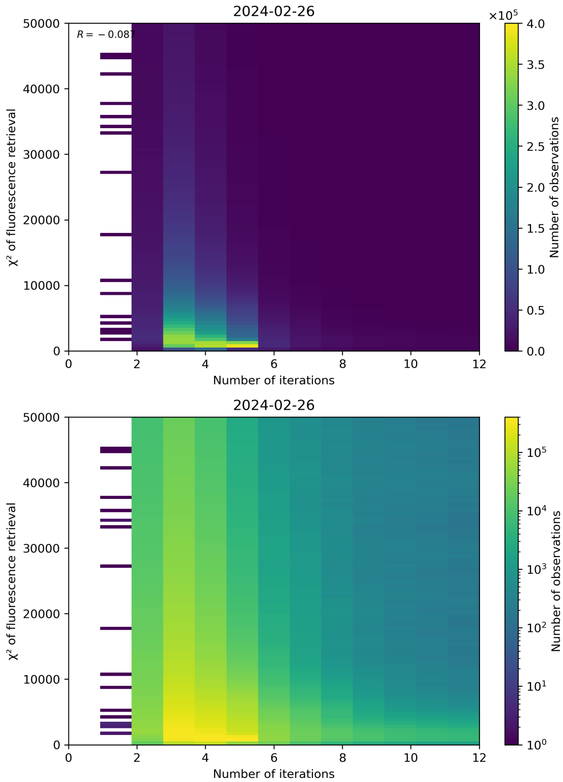
Figure 97: Scatter density plot of “Number of iterations” against “ \chi^2 of fluorescence retrieval” for 2024-02-25 to 2024-02-27.
