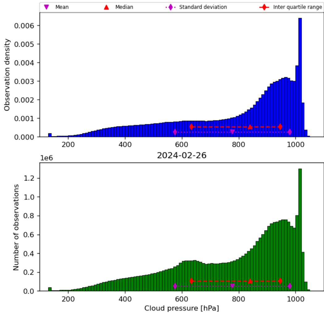
Figure 30: Histogram of “Cloud pressure” for 2024-02-25 to 2024-02-27
