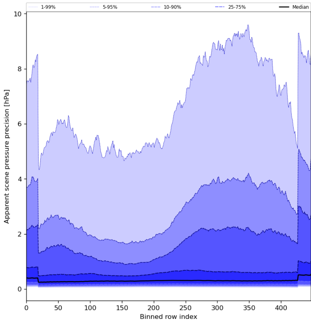
Figure 54: Along track statistics of “Apparent scene pressure precision” for 2024-02-25 to 2024-02-27
