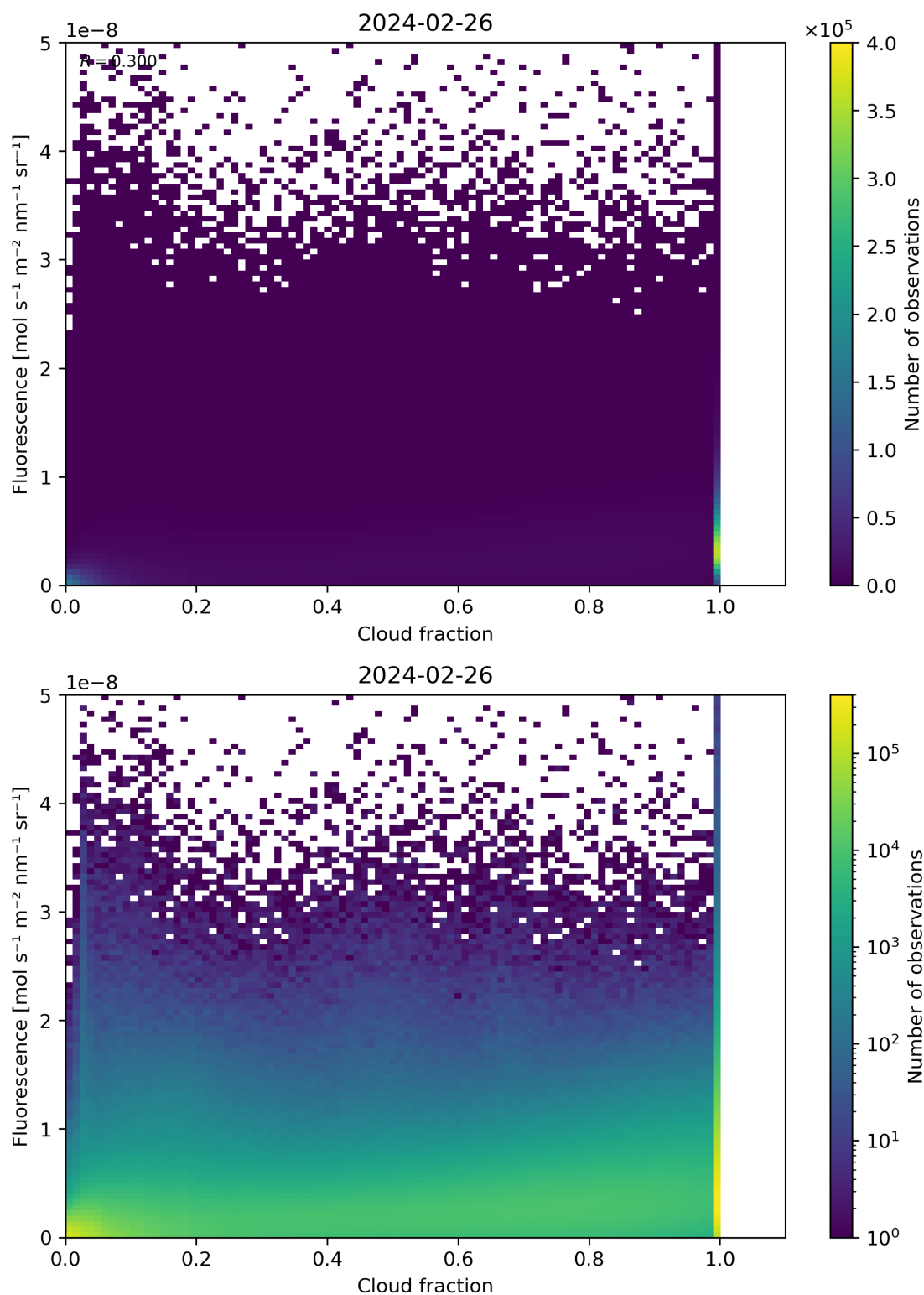
Figure 72: Scatter density plot of “Cloud fraction” against “Fluorescence” for 2024-02-25 to 2024-02-27.
