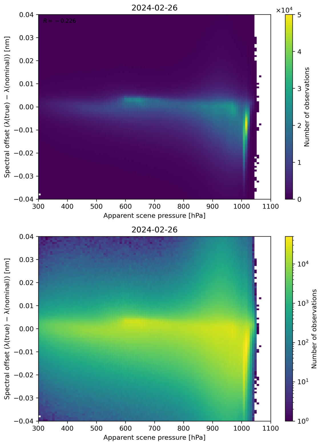
Figure 67: Scatter density plot of “Apparent scene pressure” against “Spectral offset ( \lambda(\text{true}) - \lambda(\text{nominal}) )” for 2024-02-25 to 2024-02-27.
