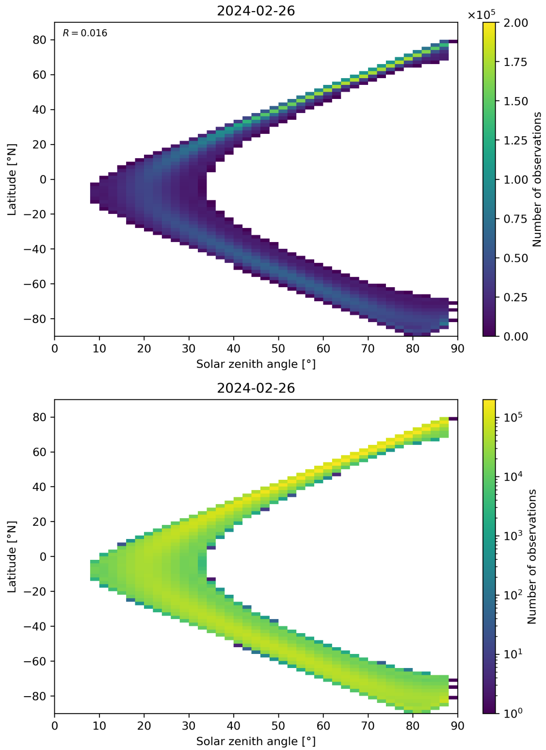
Figure 113: Scatter density plot of “Solar zenith angle” against “Latitude” for 2024-02-25 to 2024-02-27.
