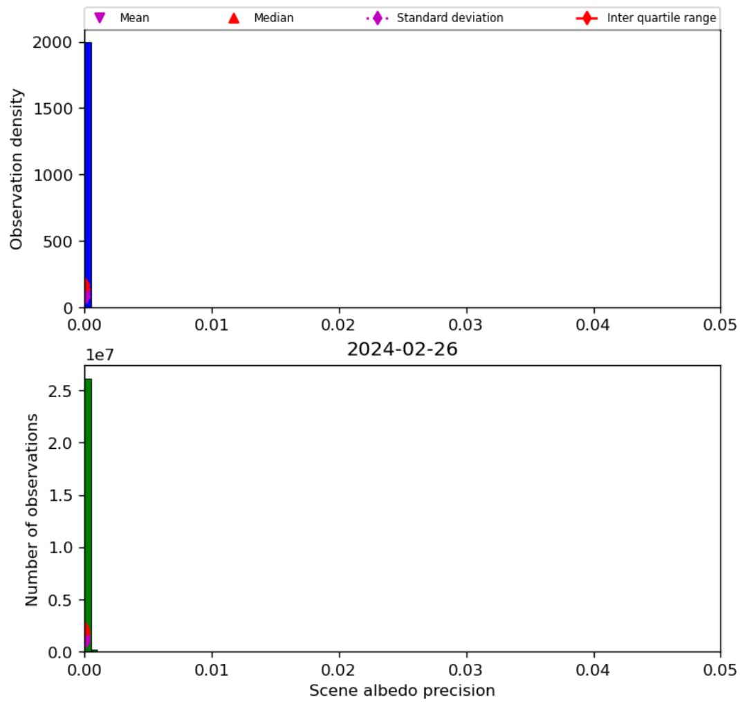
Figure 35: Histogram of “Scene albedo precision” for 2024-02-25 to 2024-02-27
