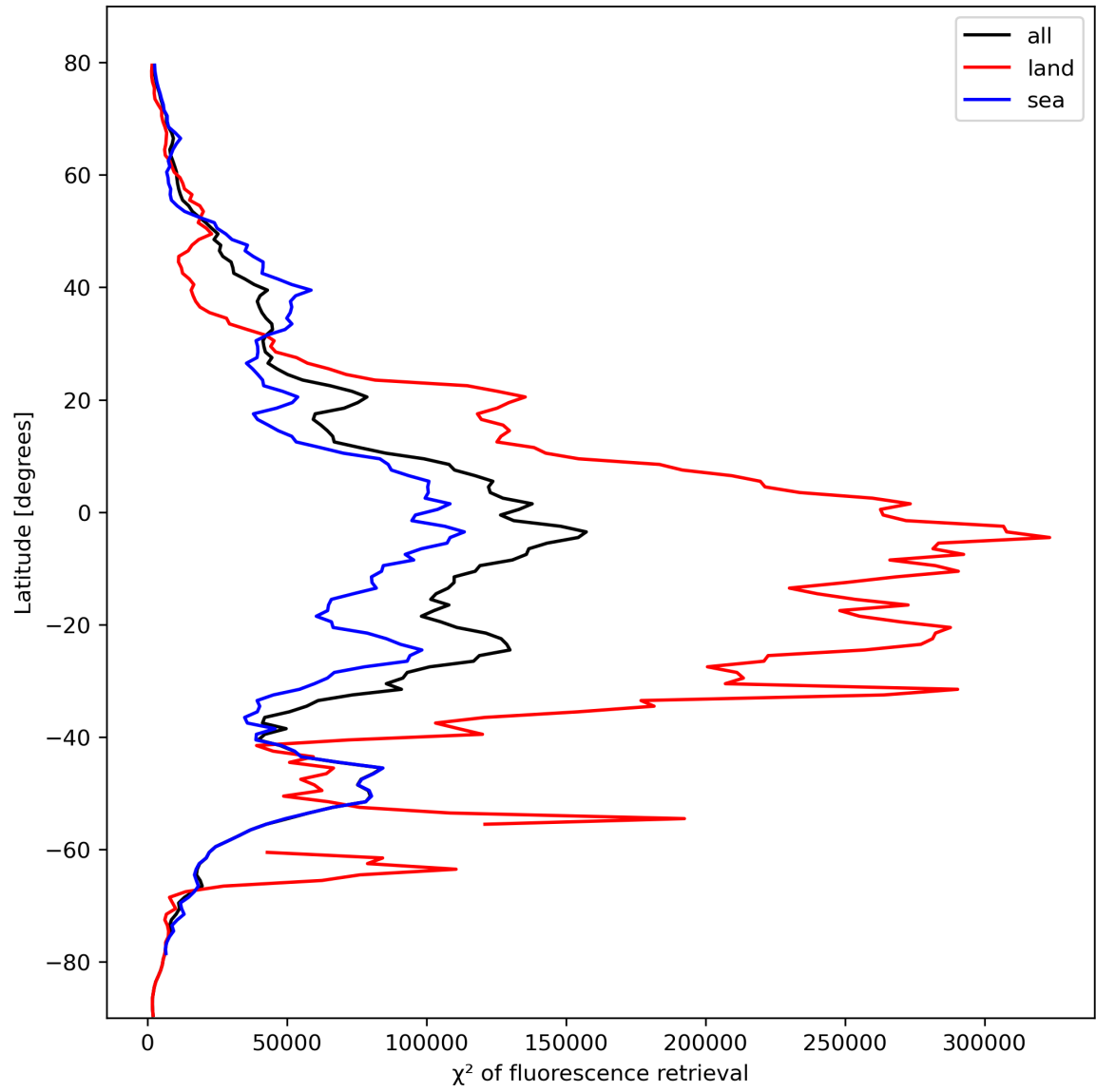
Figure 25: Zonal average of “ \chi^2 of fluorescence retrieval” for 2024-02-25 to 2024-02-27.
