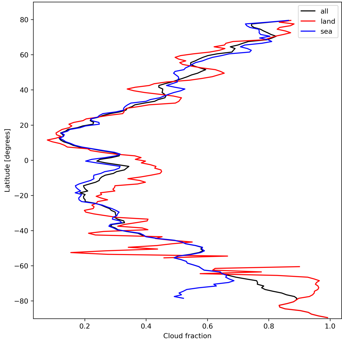
Figure 15: Zonal average of “Cloud fraction” for 2024-02-25 to 2024-02-27.
