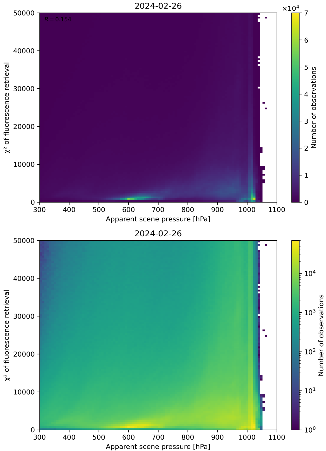
Figure 63: Scatter density plot of “Apparent scene pressure” against “ \chi^2 of fluorescence retrieval” for 2024-02-25 to 2024-02-27.
