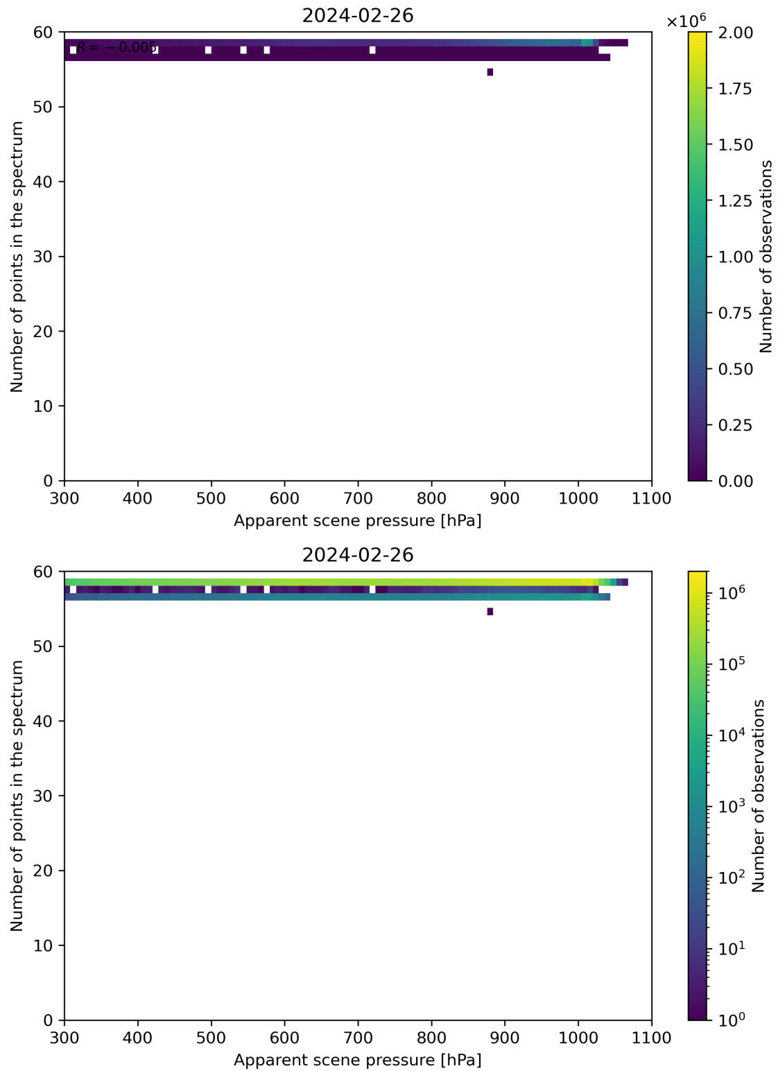
Figure 66: Scatter density plot of “Apparent scene pressure” against “Number of points in the spectrum” for 2024-02-25 to 2024-02-27.
