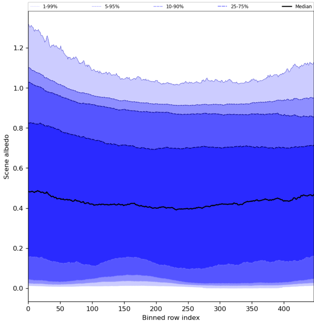
Figure 51: Along track statistics of “Scene albedo” for 2024-02-25 to 2024-02-27
