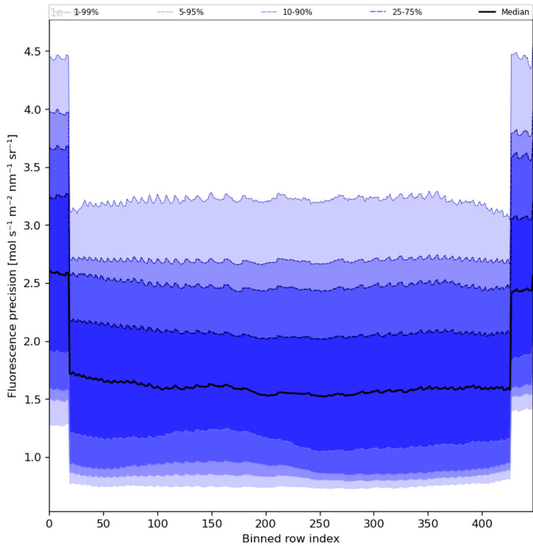
Figure 58: Along track statistics of “Fluorescence precision” for 2024-02-25 to 2024-02-27
