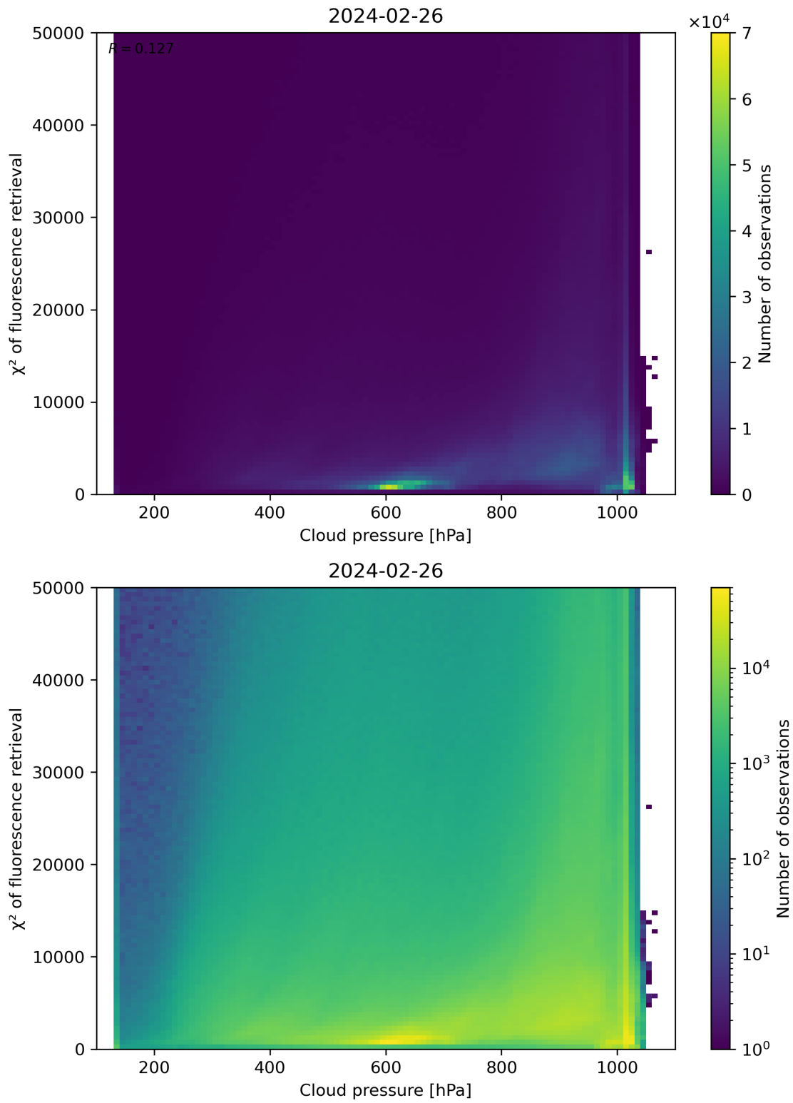
Figure 78: Scatter density plot of “Cloud pressure” against “ \chi^2 of fluorescence retrieval” for 2024-02-25 to 2024-02-27.
