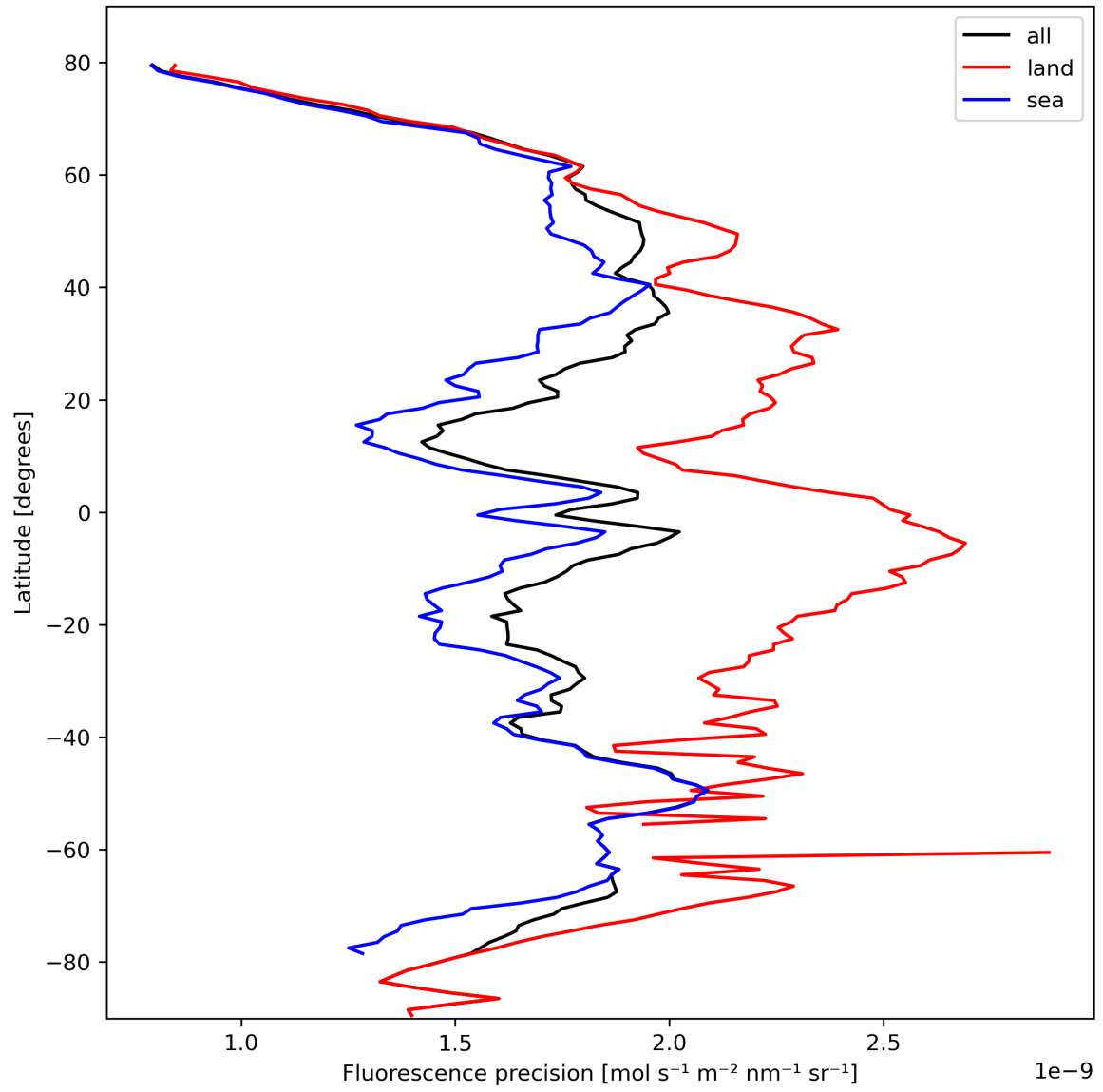
Figure 24: Zonal average of “Fluorescence precision” for 2024-02-25 to 2024-02-27.
