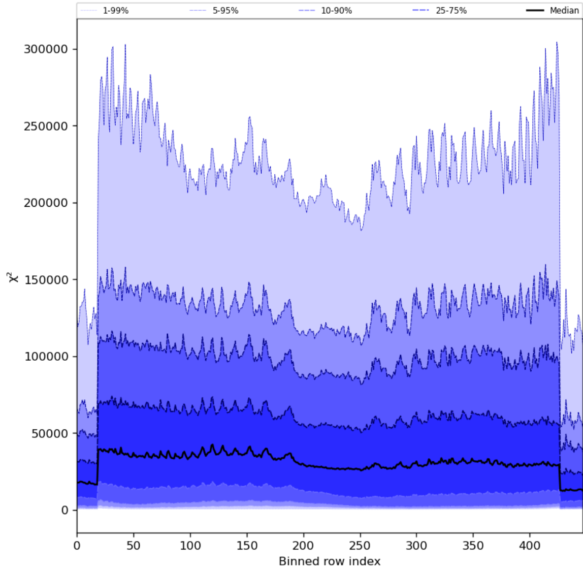
Figure 55: Along track statistics of “ \chi^2 ” for 2024-02-25 to 2024-02-27
