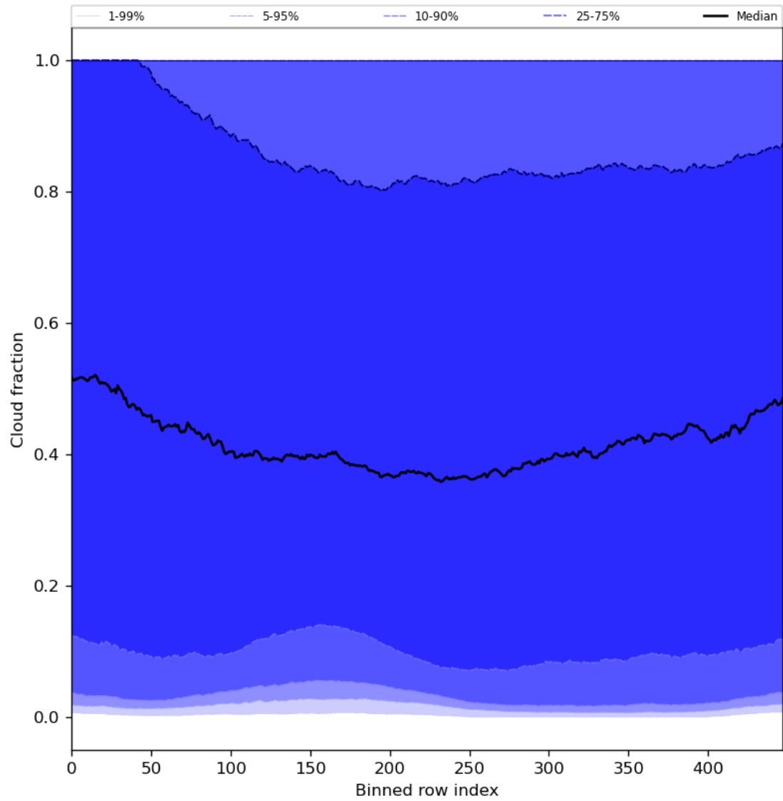
Figure 49: Along track statistics of “Cloud fraction” for 2024-02-25 to 2024-02-27
