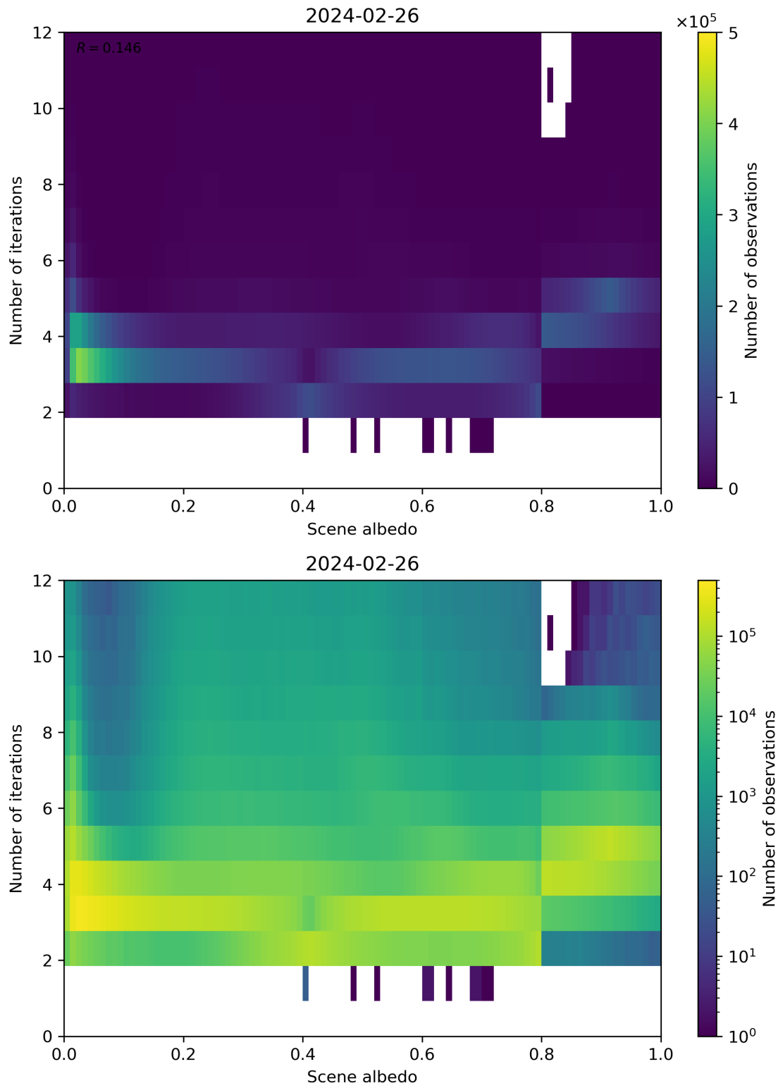
Figure 105: Scatter density plot of “Scene albedo” against “Number of iterations” for 2024-02-25 to 2024-02-27.
