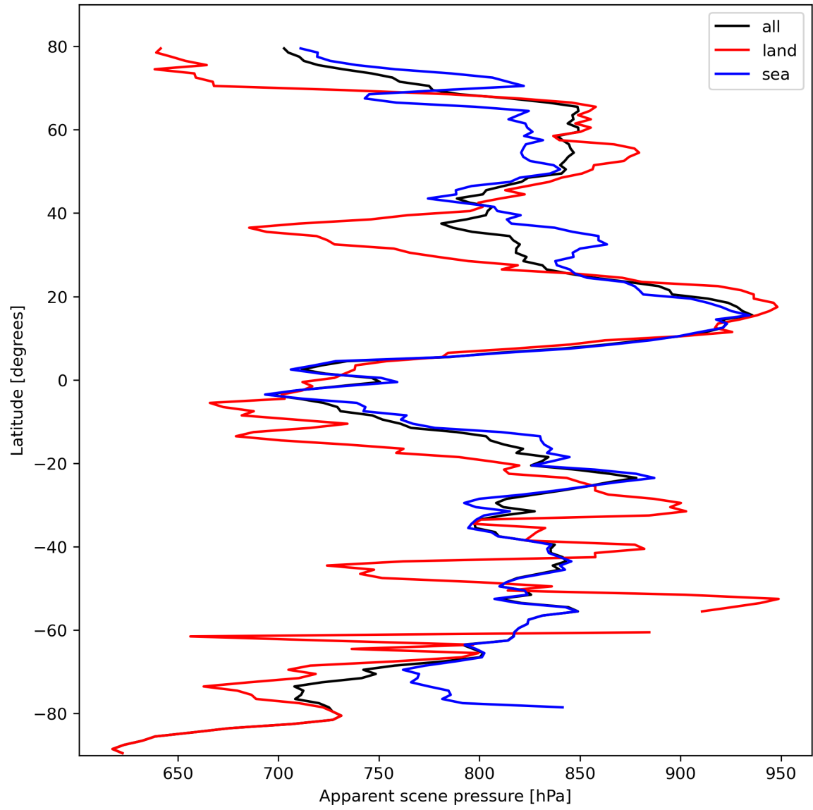
Figure 19: Zonal average of “Apparent scene pressure” for 2024-02-25 to 2024-02-27.
