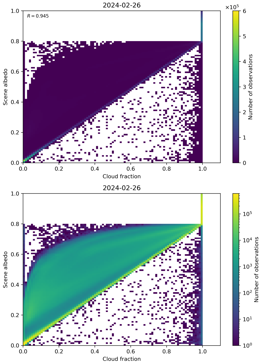
Figure 75: Scatter density plot of “Cloud fraction” against “Scene albedo” for 2024-02-25 to 2024-02-27.
