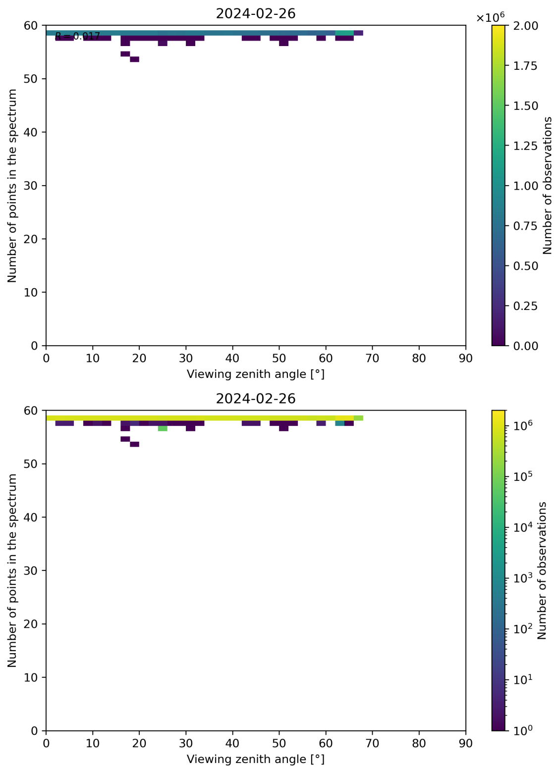
Figure 125: Scatter density plot of “Viewing zenith angle” against “Number of points in the spectrum” for 2024-02-25 to 2024-02-27.
