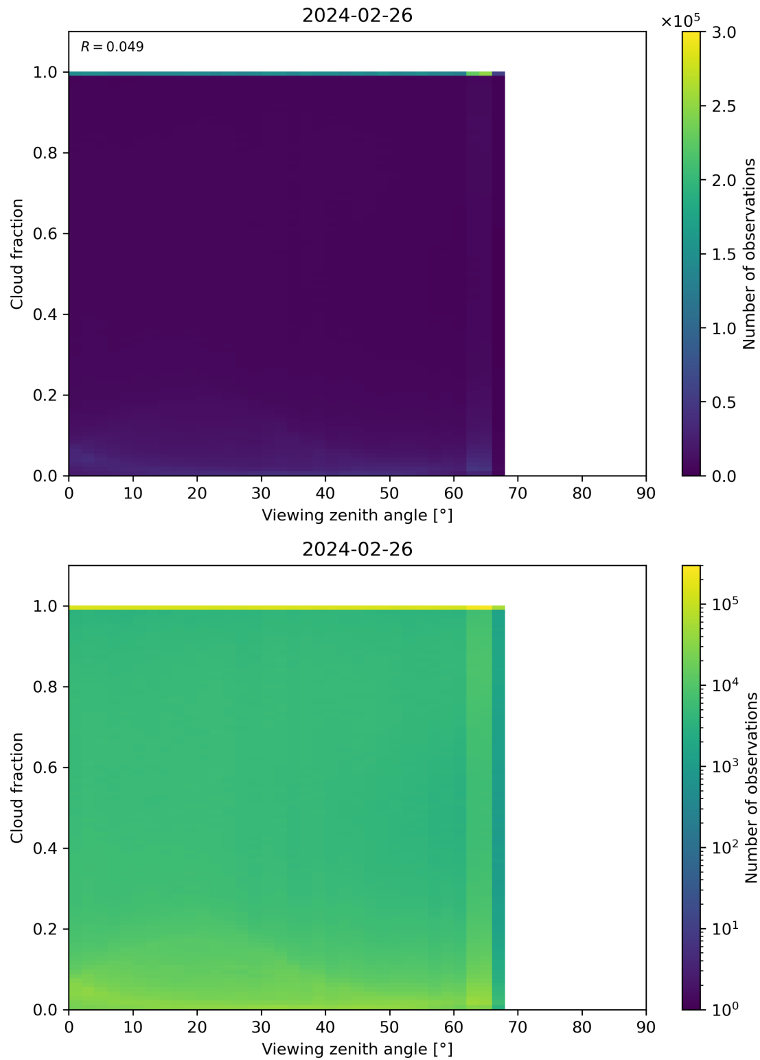
Figure 120: Scatter density plot of “Viewing zenith angle” against “Cloud fraction” for 2024-02-25 to 2024-02-27.
