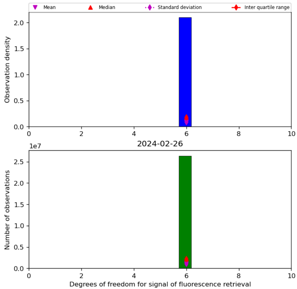
Figure 43: Histogram of “Degrees of freedom for signal of fluorescence retrieval” for 2024-02-25 to 2024-02-27
