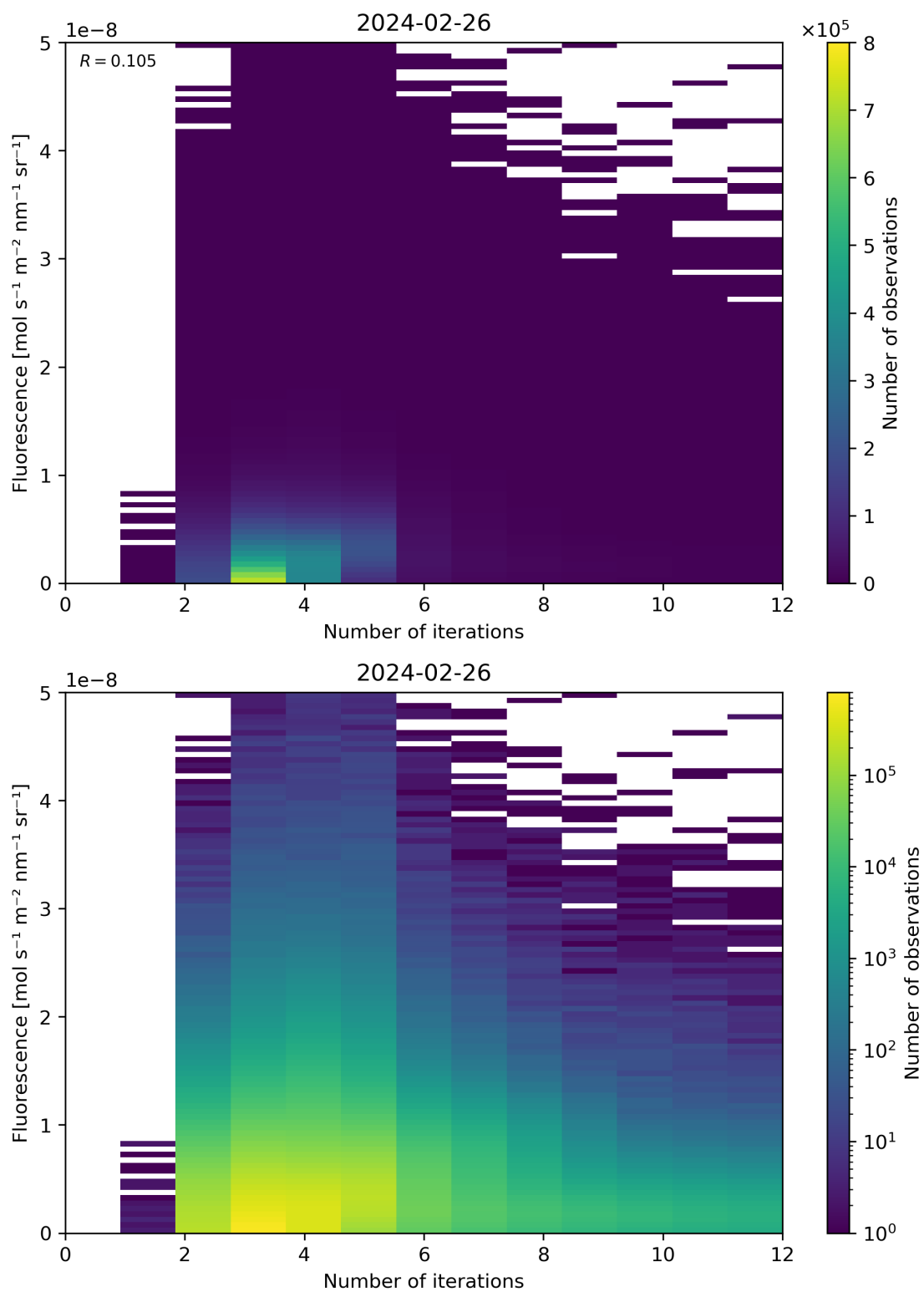
Figure 98: Scatter density plot of “Number of iterations” against “Fluorescence” for 2024-02-25 to 2024-02-27.
