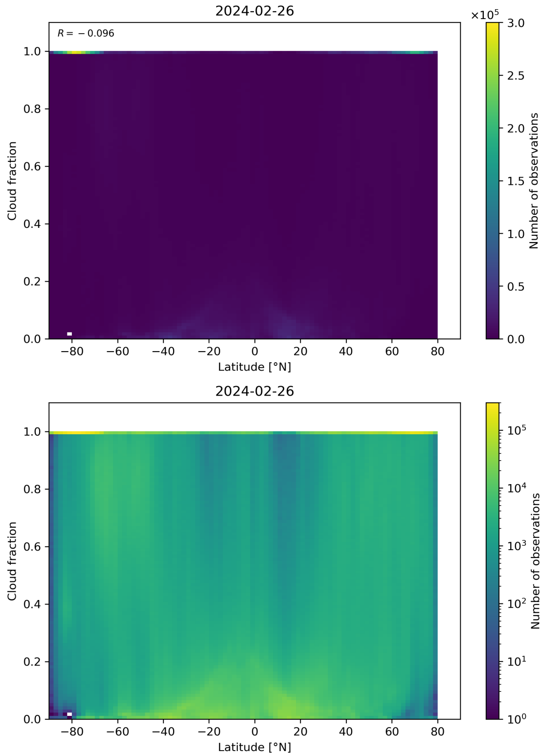
Figure 90: Scatter density plot of “Latitude” against “Cloud fraction” for 2024-02-25 to 2024-02-27.
