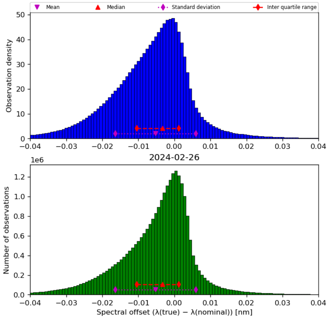
Figure 45: Histogram of “Spectral offset ( \lambda(\text{true}) - \lambda(\text{nominal}) )” for 2024-02-25 to 2024-02-27
