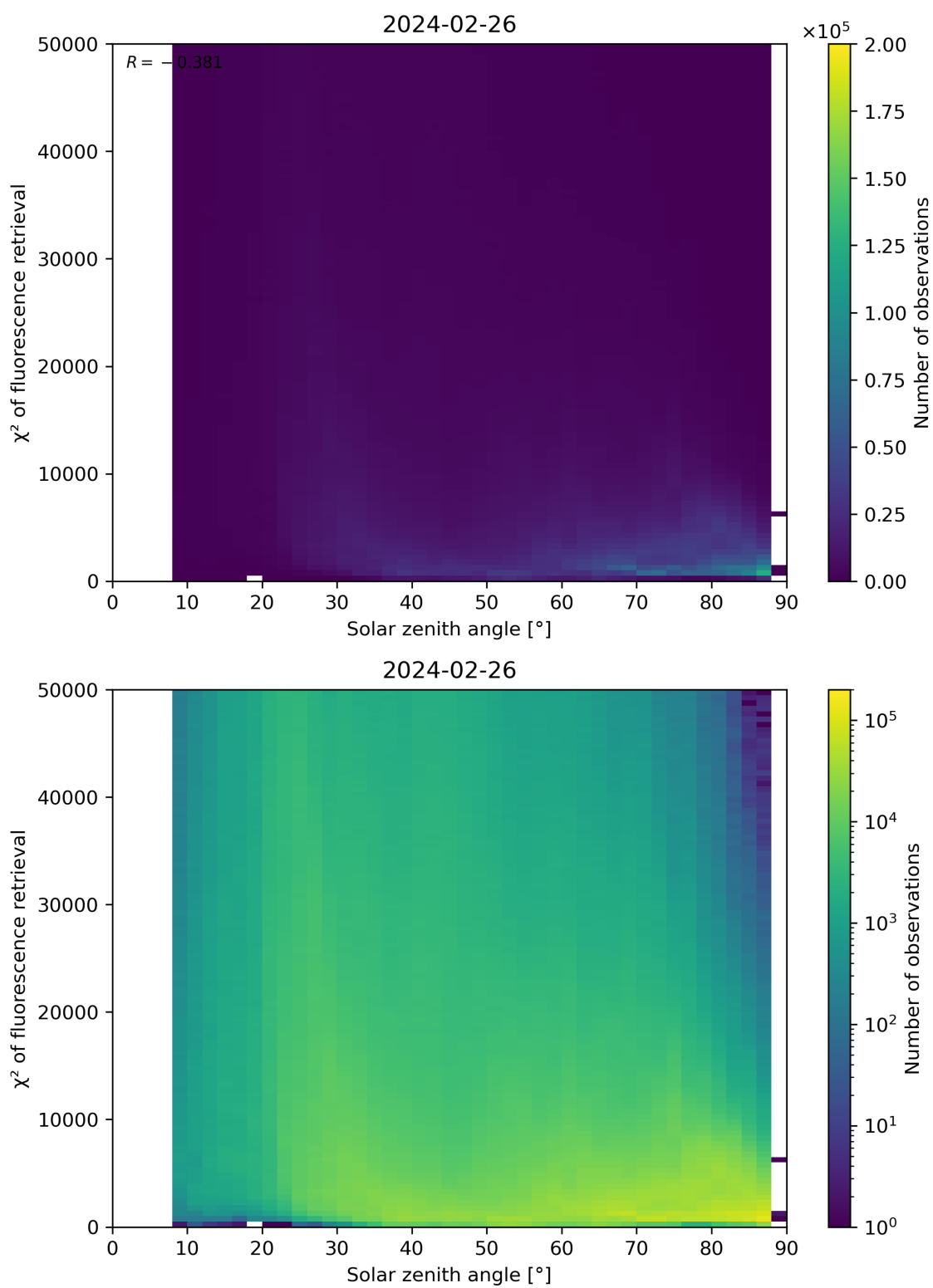
Figure 109: Scatter density plot of “Solar zenith angle” against “ \chi^2 of fluorescence retrieval” for 2024-02-25 to 2024-02-27.
