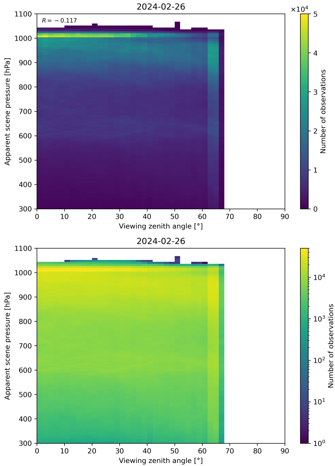
Figure 118: Scatter density plot of “Viewing zenith angle” against “Apparent scene pressure” for 2024-02-25 to 2024-02-27.
