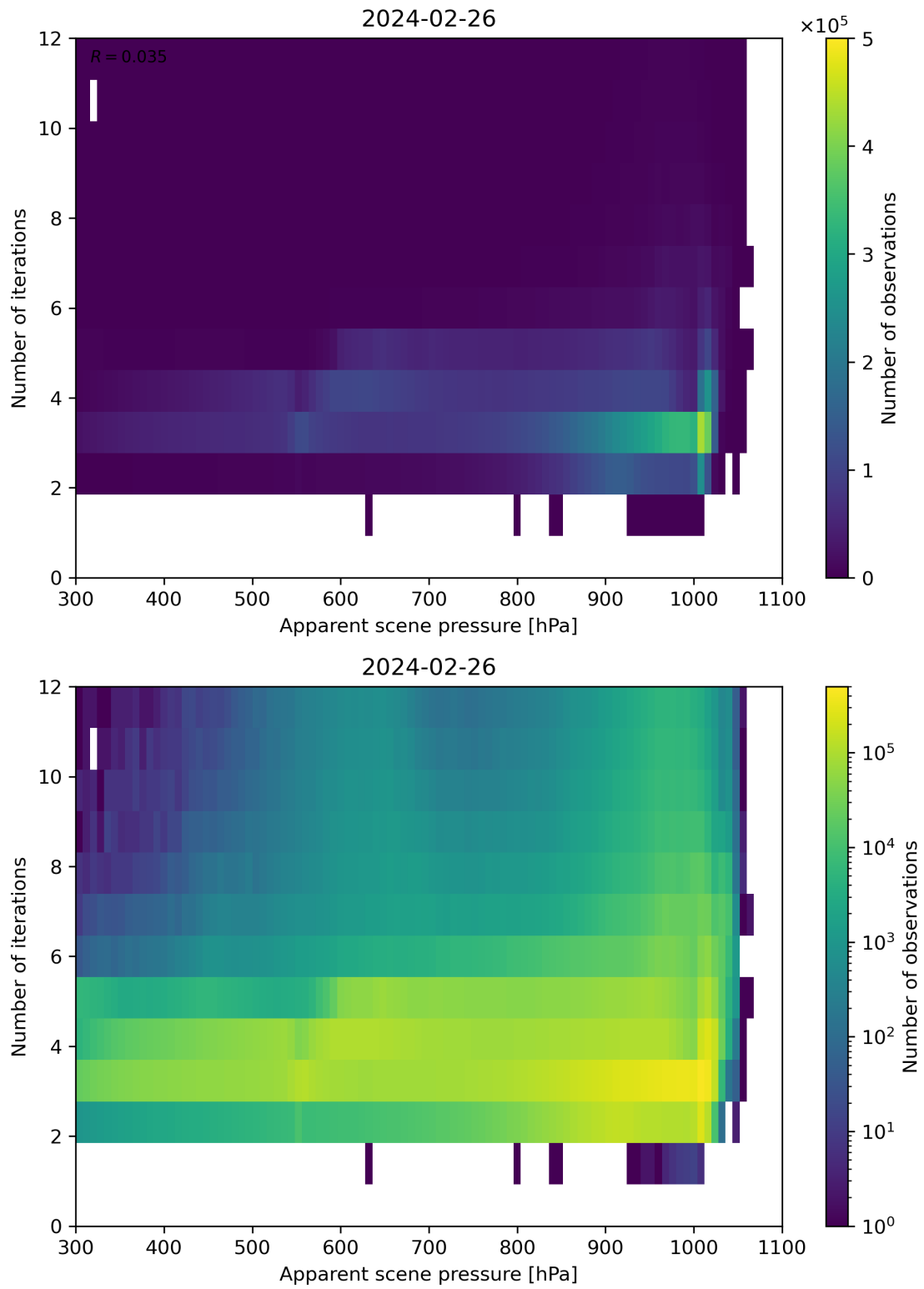
Figure 65: Scatter density plot of “Apparent scene pressure” against “Number of iterations” for 2024-02-25 to 2024-02-27.
