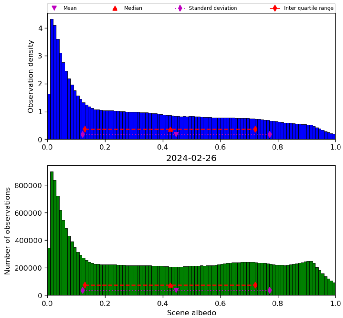
Figure 34: Histogram of “Scene albedo” for 2024-02-25 to 2024-02-27
