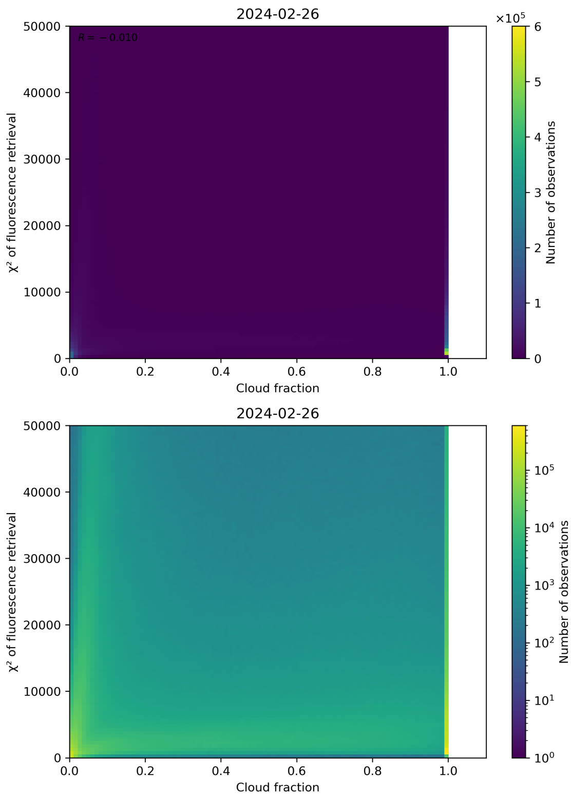
Figure 71: Scatter density plot of “Cloud fraction” against “ \chi^2 of fluorescence retrieval” for 2024-02-25 to 2024-02-27.
