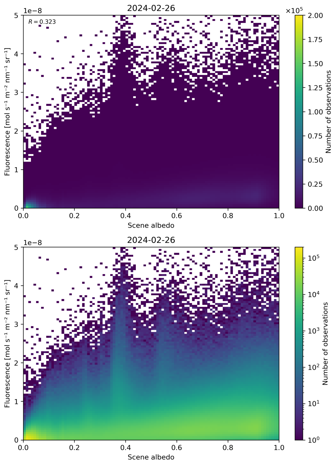
Figure 104: Scatter density plot of “Scene albedo” against “Fluorescence” for 2024-02-25 to 2024-02-27.
