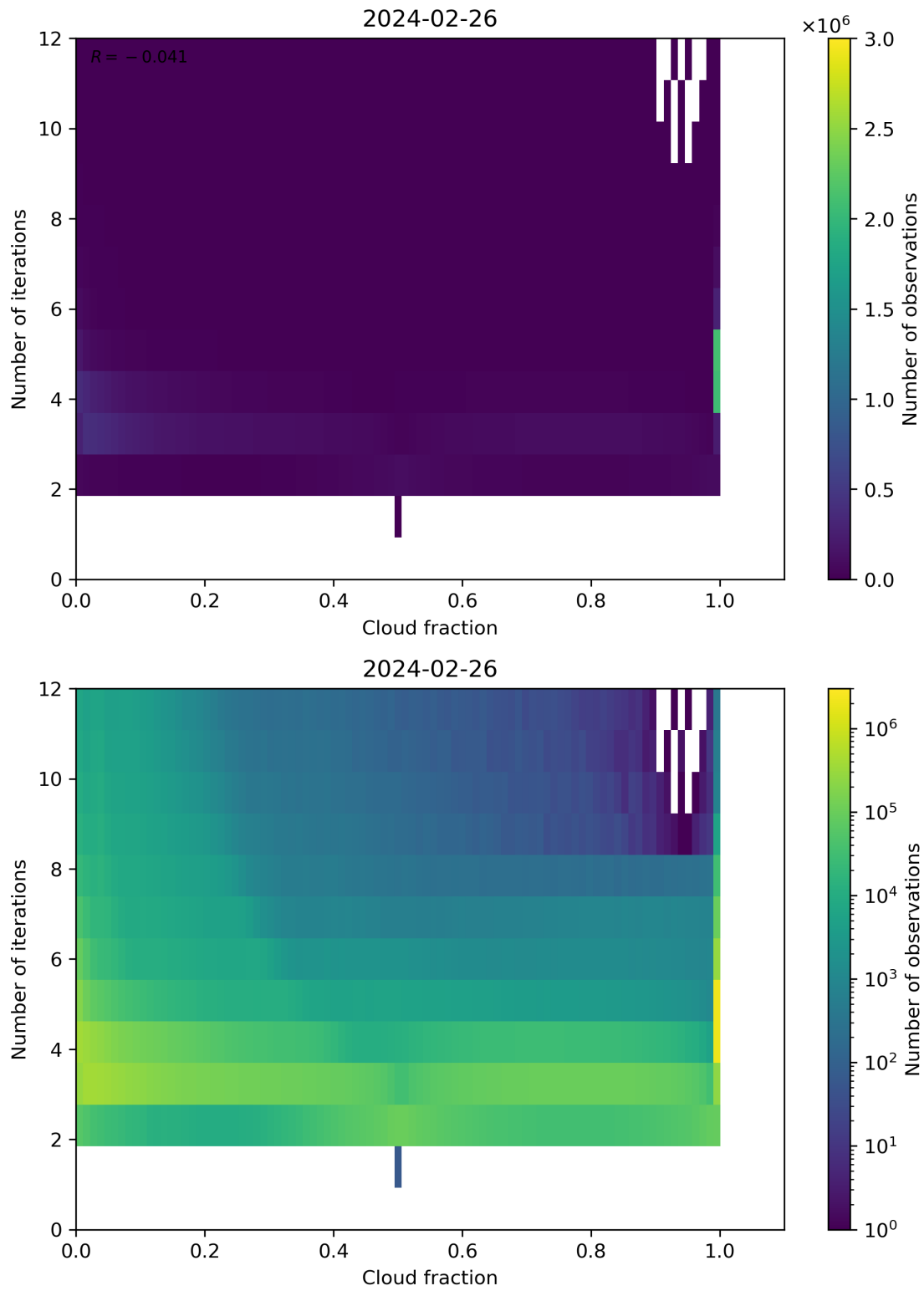
Figure 73: Scatter density plot of “Cloud fraction” against “Number of iterations” for 2024-02-25 to 2024-02-27.
