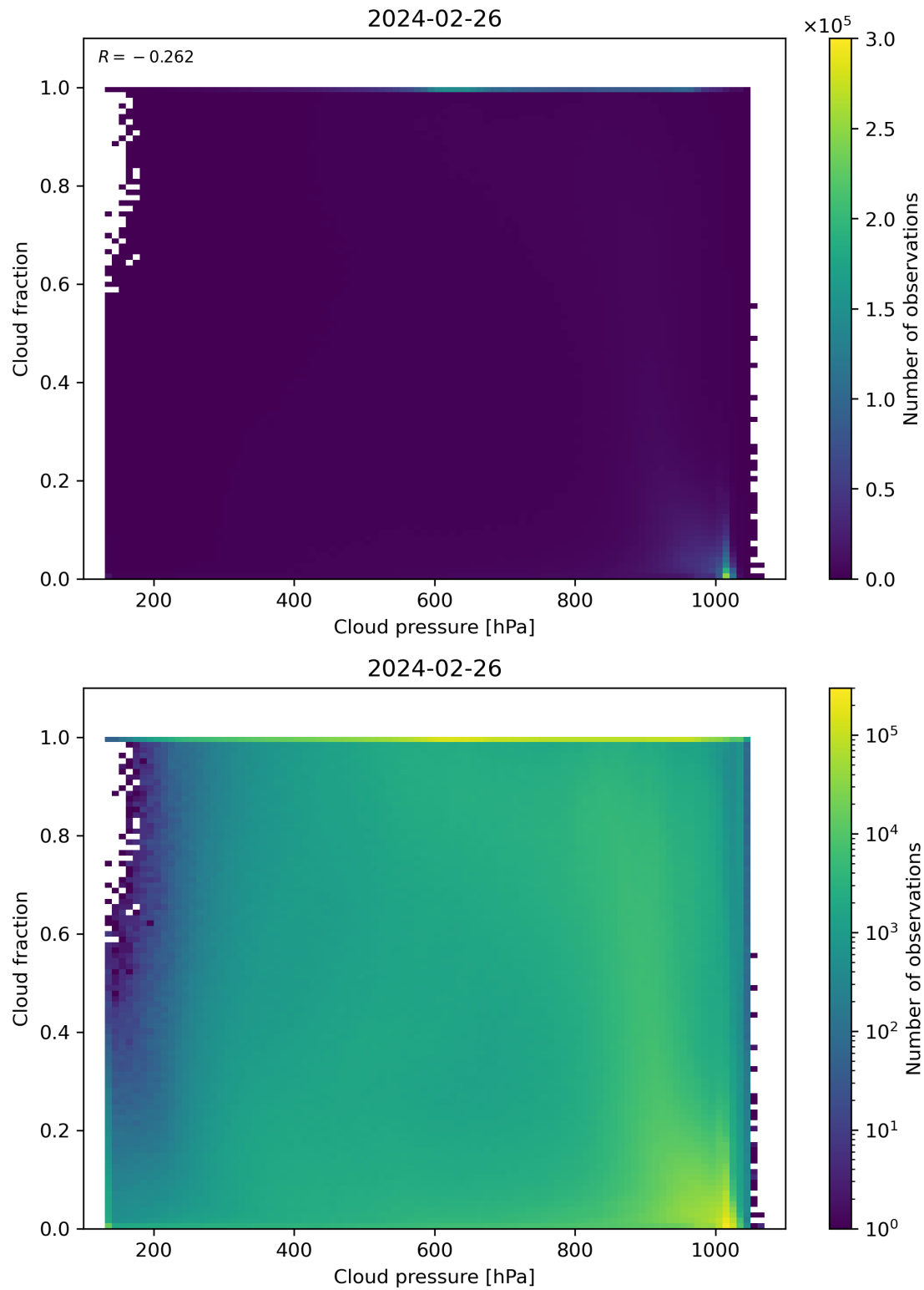
Figure 79: Scatter density plot of “Cloud pressure” against “Cloud fraction” for 2024-02-25 to 2024-02-27.
