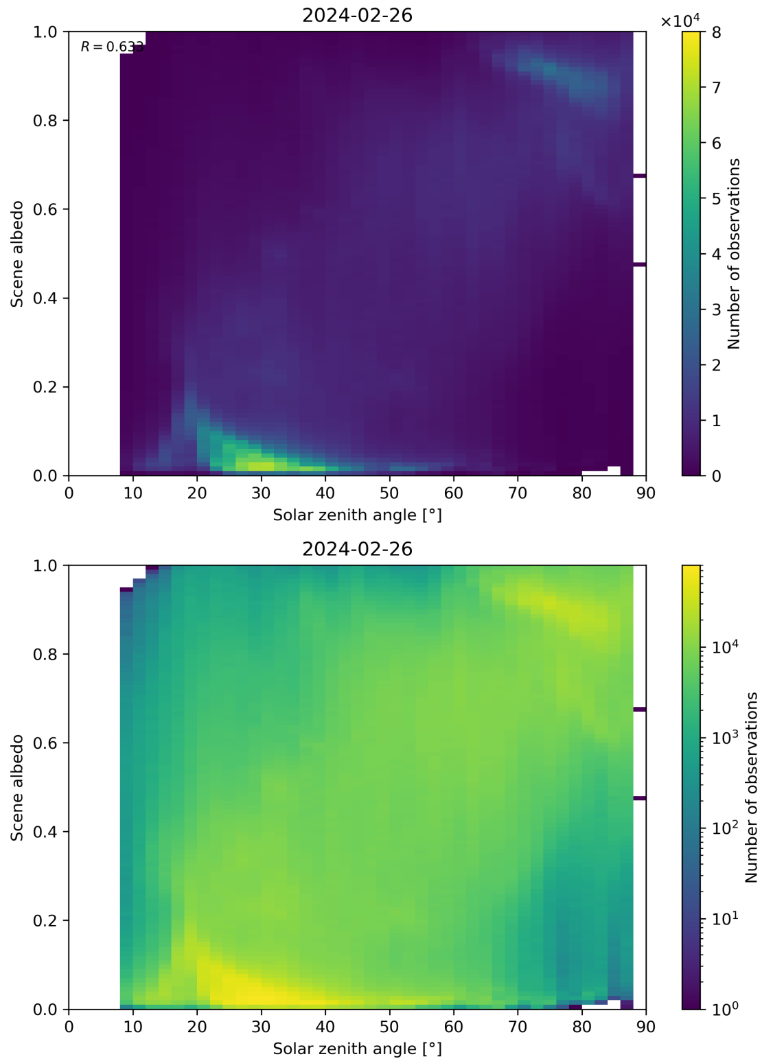
Figure 116: Scatter density plot of “Solar zenith angle” against “Scene albedo” for 2024-02-25 to 2024-02-27.
