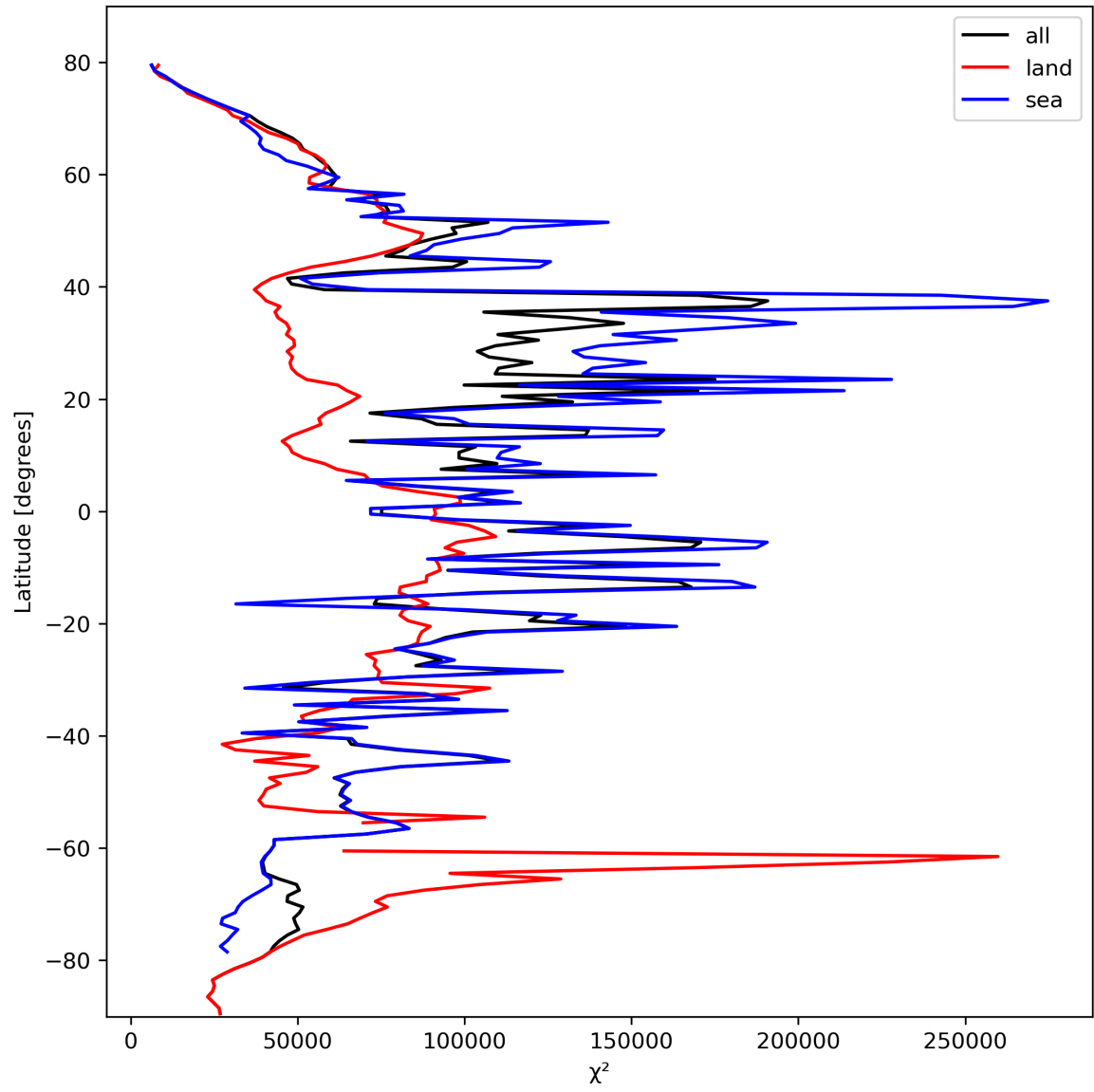
Figure 21: Zonal average of “ \chi^2 ” for 2024-02-25 to 2024-02-27.
