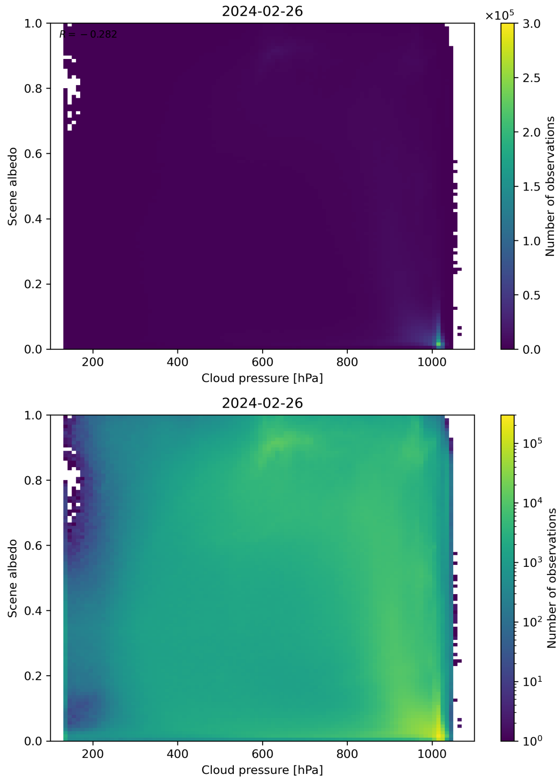
Figure 83: Scatter density plot of “Cloud pressure” against “Scene albedo” for 2024-02-25 to 2024-02-27.
