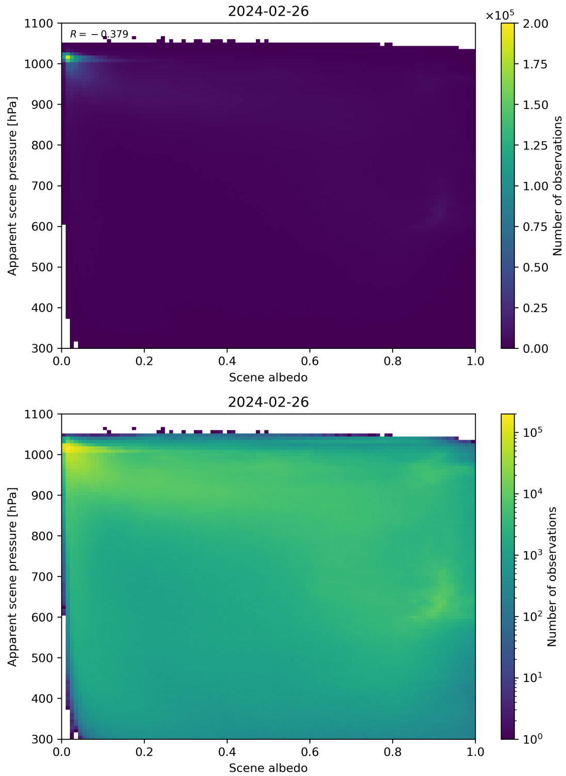
Figure 102: Scatter density plot of “Scene albedo” against “Apparent scene pressure” for 2024-02-25 to 2024-02-27.
