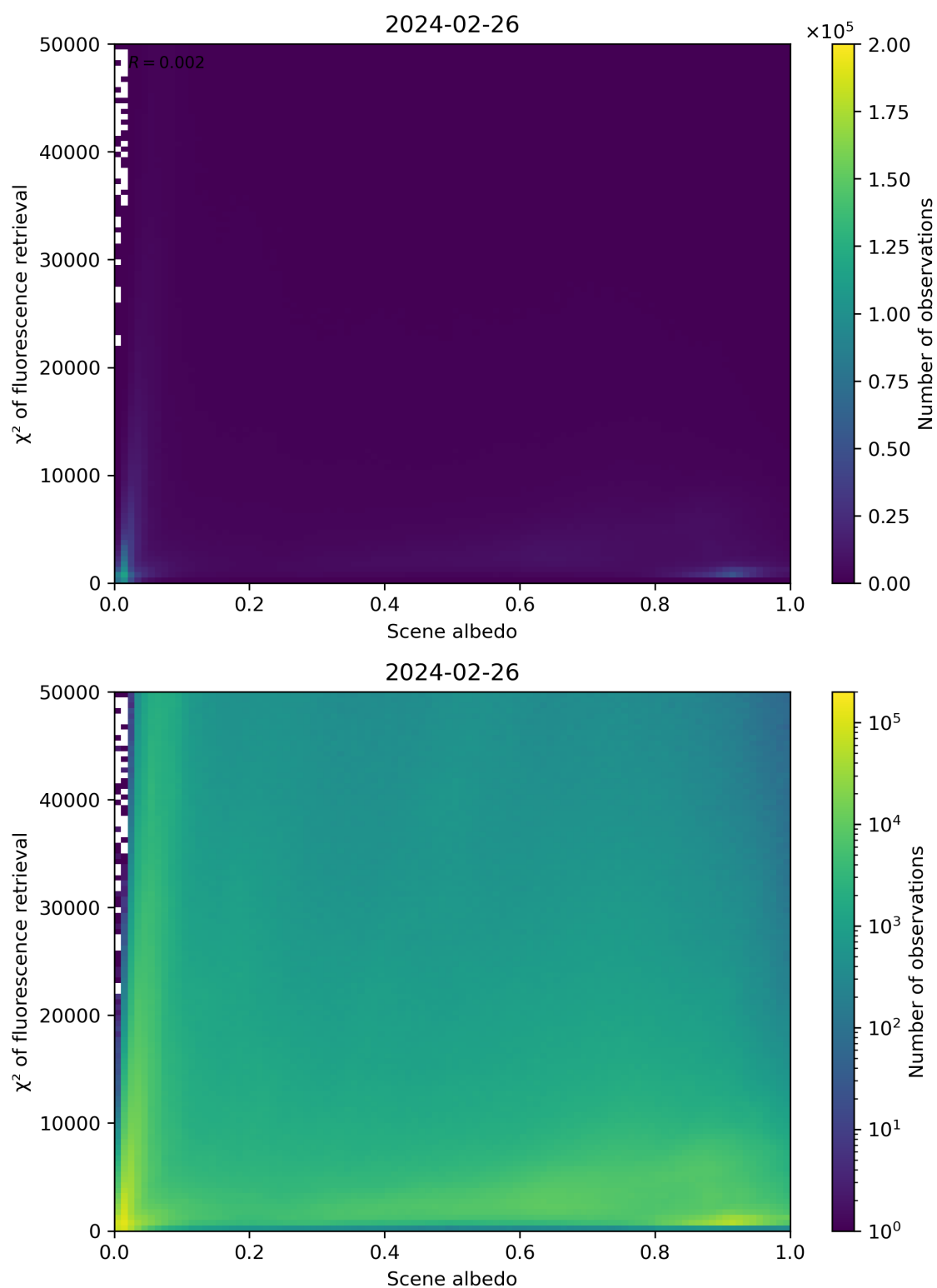
Figure 103: Scatter density plot of “Scene albedo” against “ \chi^2 of fluorescence retrieval” for 2024-02-25 to 2024-02-27.
