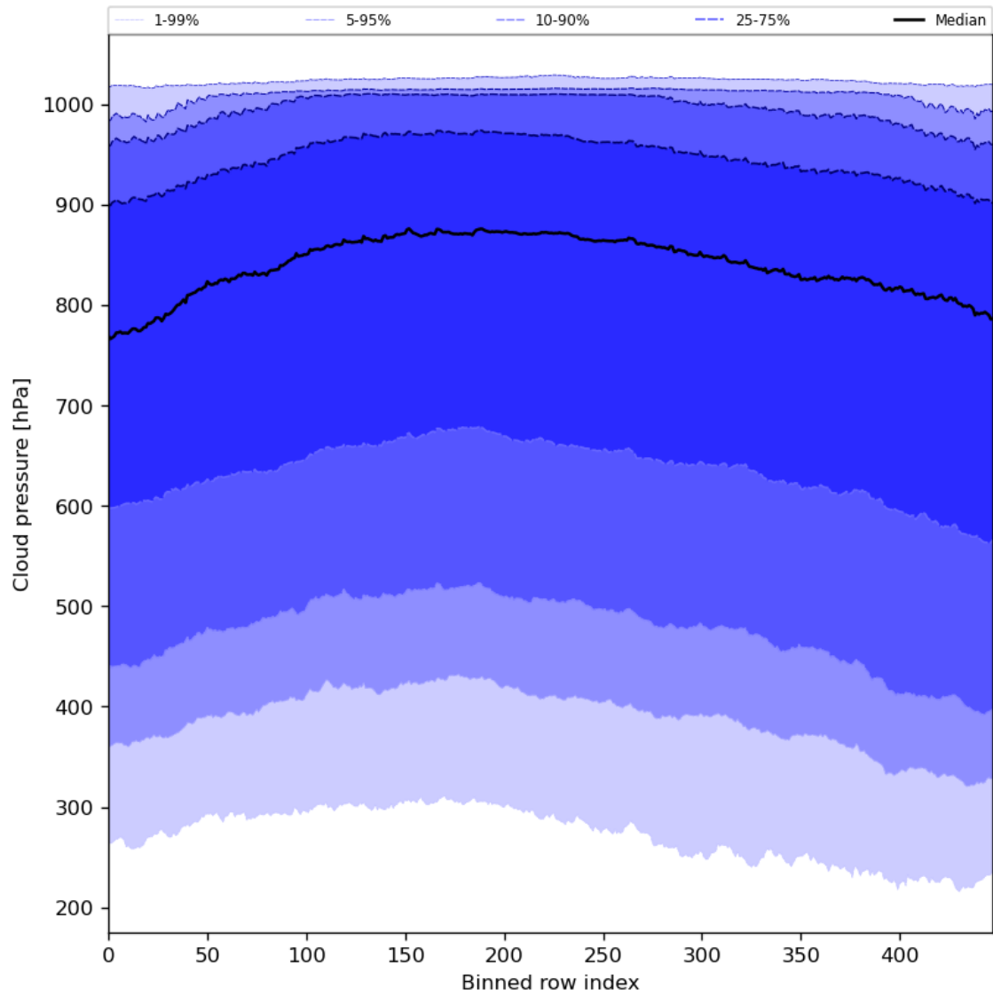
Figure 47: Along track statistics of “Cloud pressure” for 2024-02-25 to 2024-02-27
