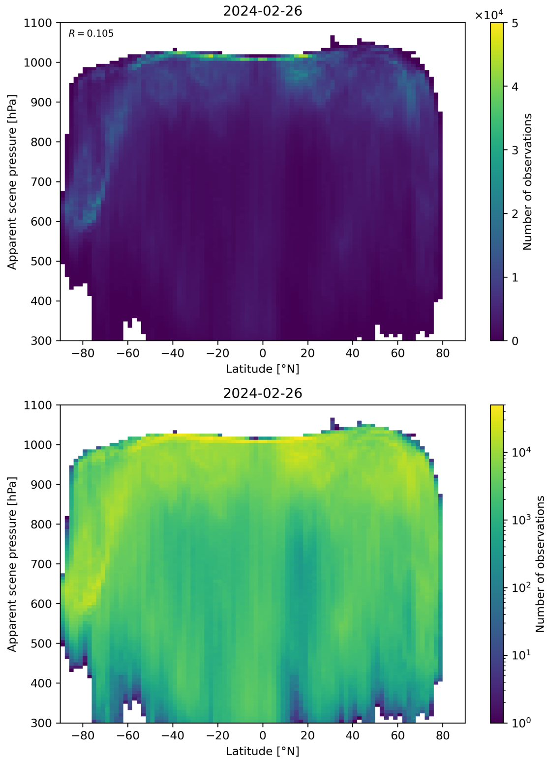
Figure 88: Scatter density plot of “Latitude” against “Apparent scene pressure” for 2024-02-25 to 2024-02-27.
