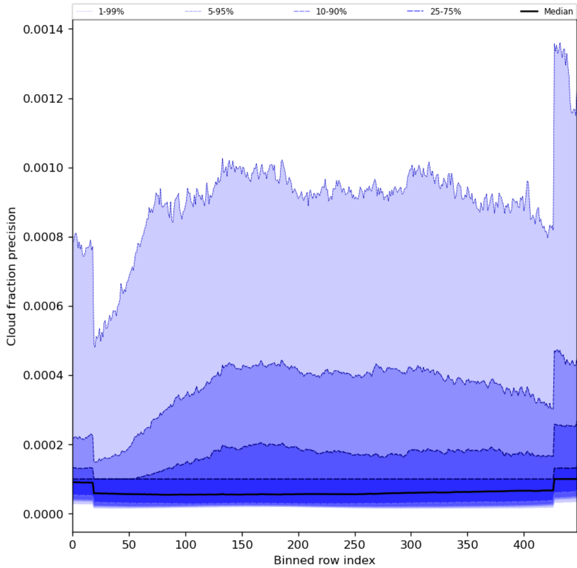
Figure 50: Along track statistics of “Cloud fraction precision” for 2024-02-25 to 2024-02-27
