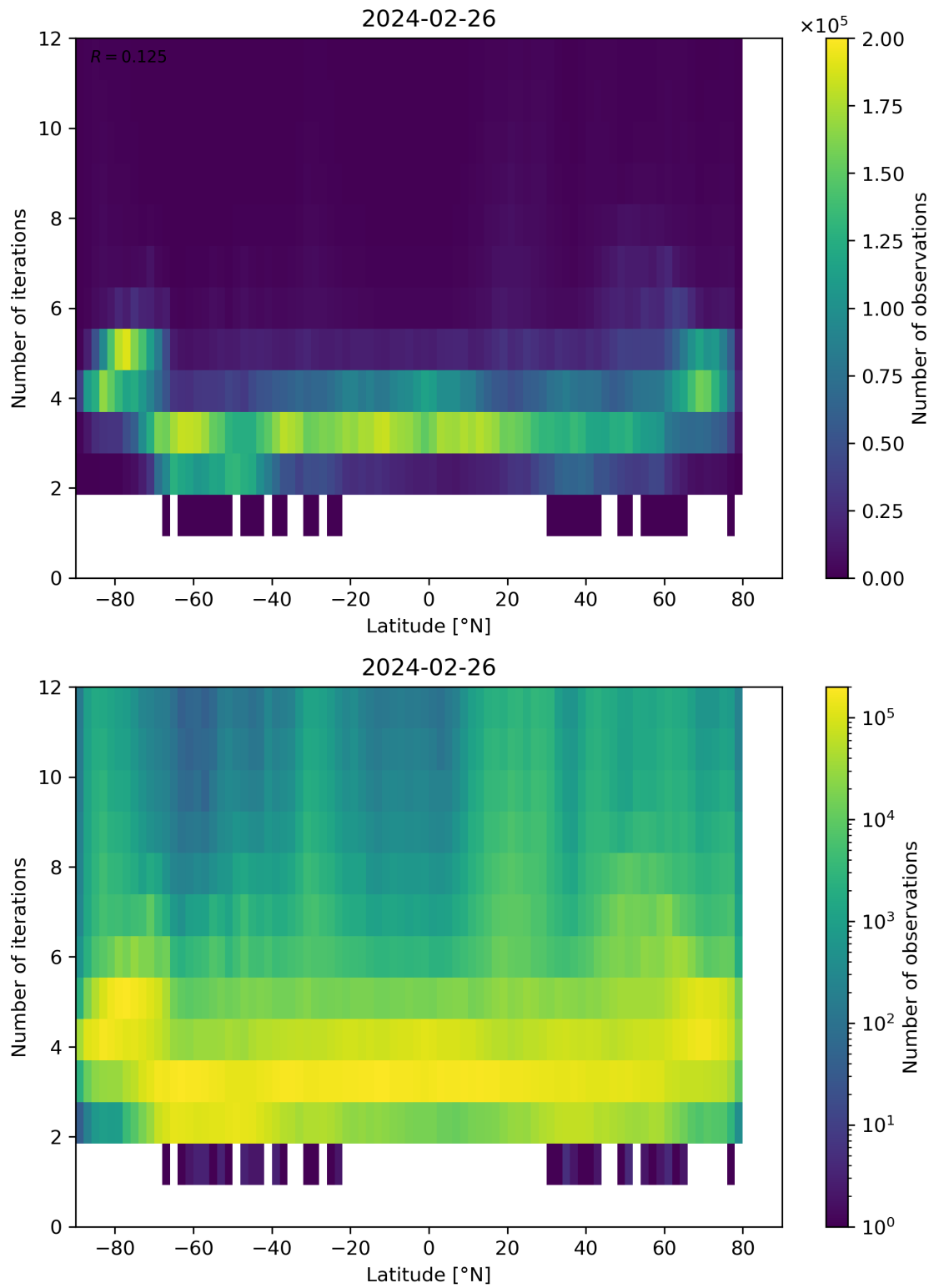
Figure 93: Scatter density plot of “Latitude” against “Number of iterations” for 2024-02-25 to 2024-02-27.
