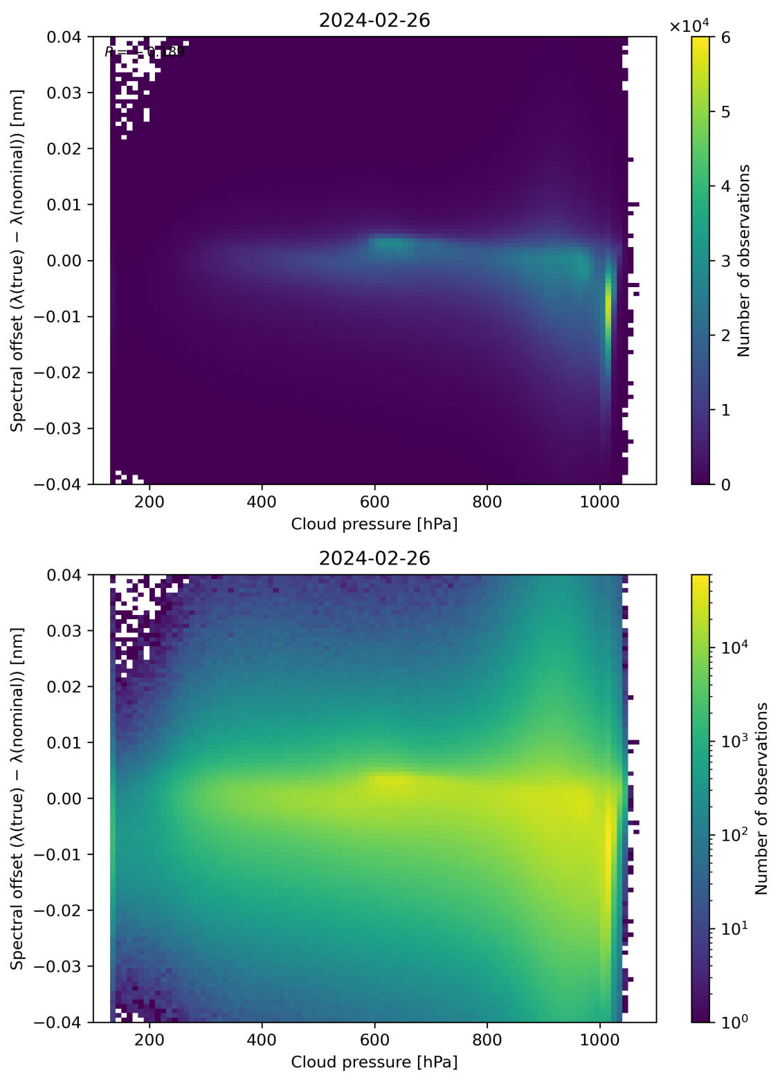
Figure 84: Scatter density plot of “Cloud pressure” against “Spectral offset ( \lambda(\text{true}) - \lambda(\text{nominal}) )” for 2024-02-25 to 2024-02-27.
