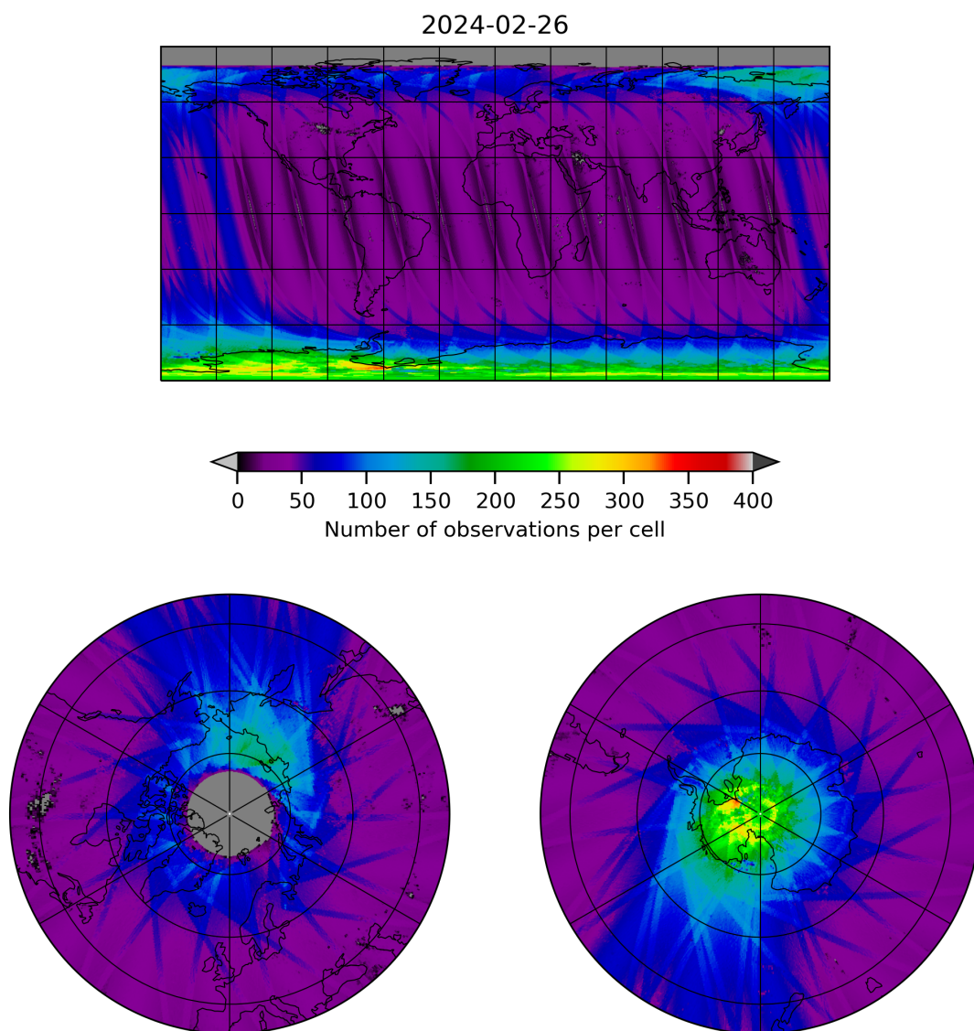
Figure 11: Map of the number of observations for 2024-02-25 to 2024-02-27
