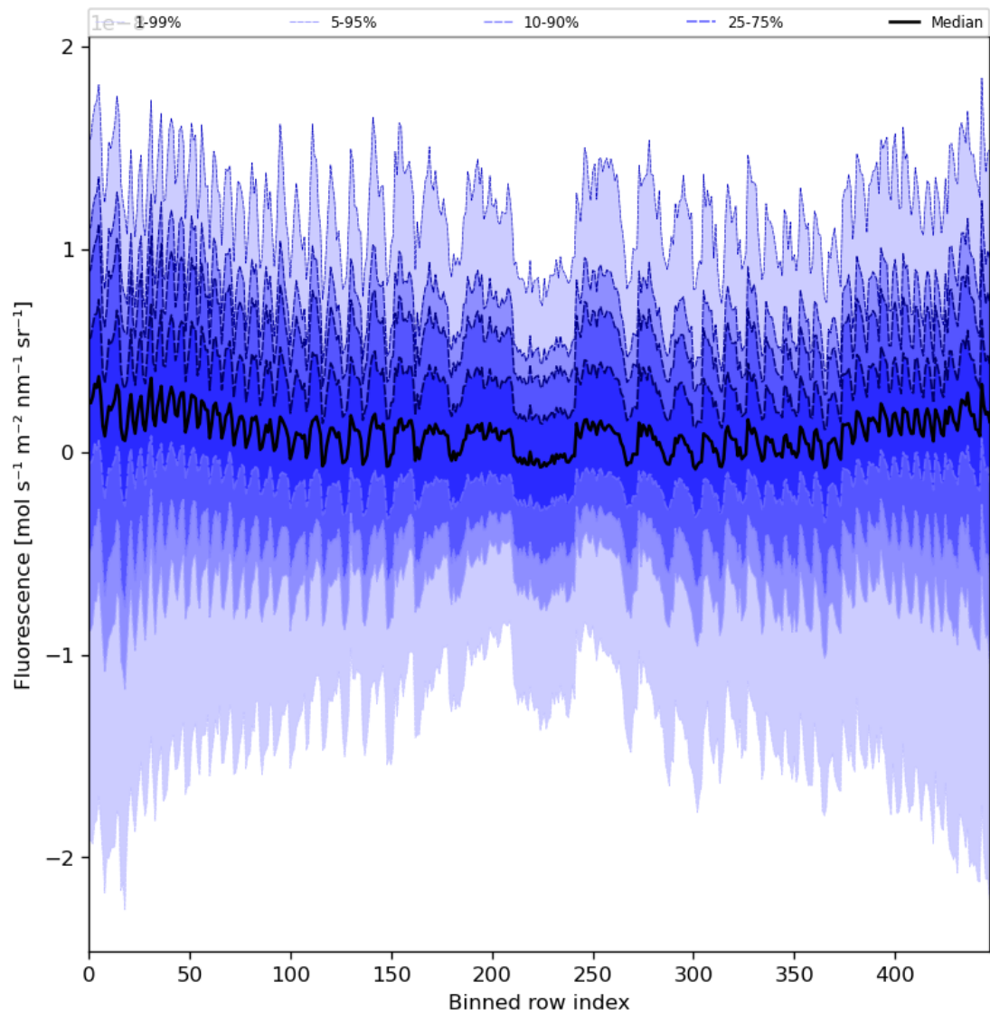
Figure 57: Along track statistics of “Fluorescence” for 2024-02-25 to 2024-02-27
