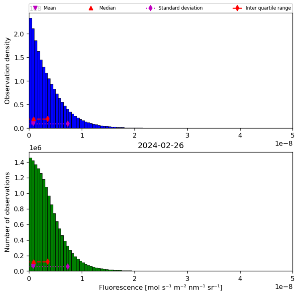
Figure 40: Histogram of “Fluorescence” for 2024-02-25 to 2024-02-27
