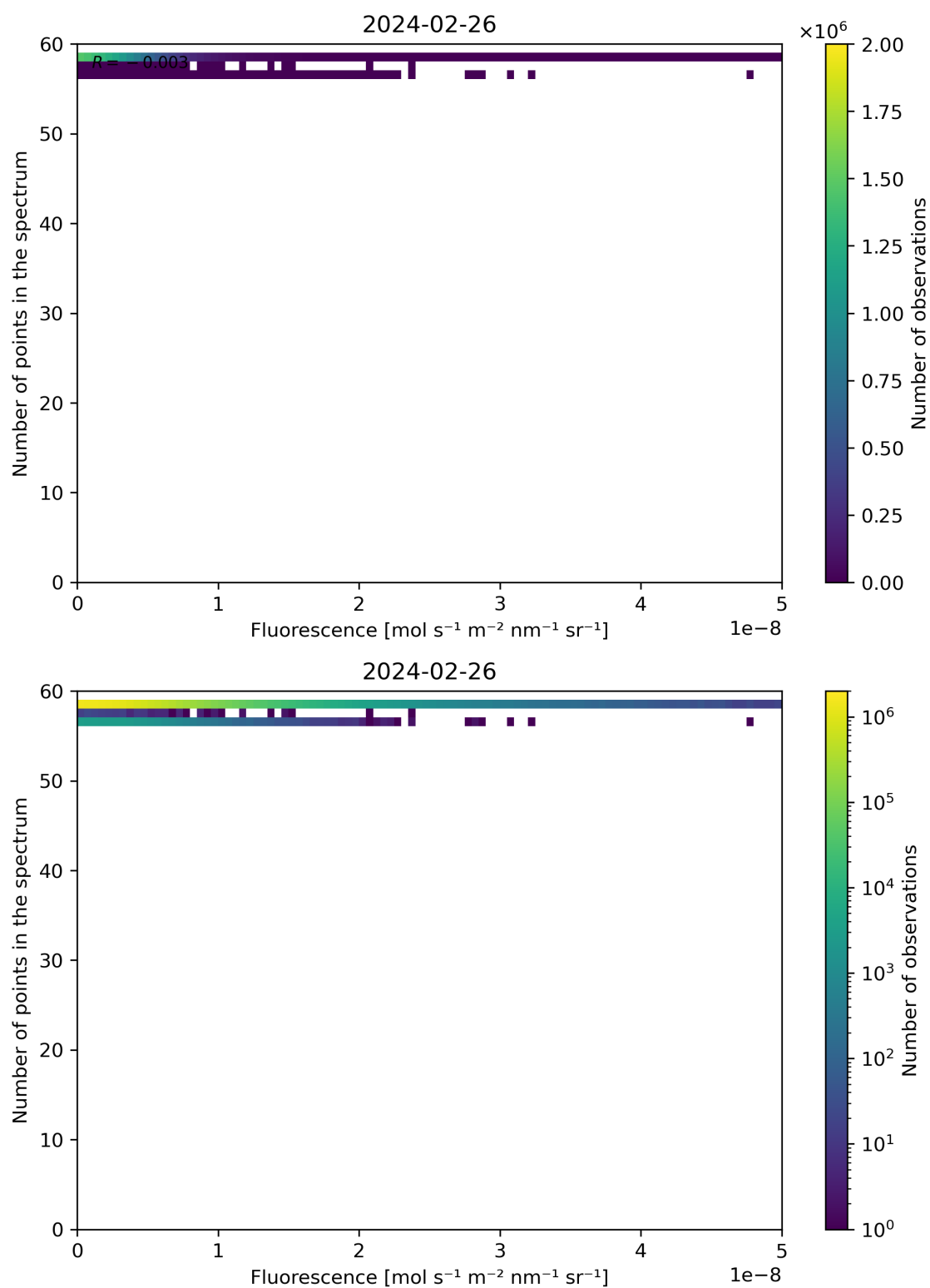
Figure 86: Scatter density plot of “Fluorescence” against “Number of points in the spectrum” for 2024-02-25 to 2024-02-27.
