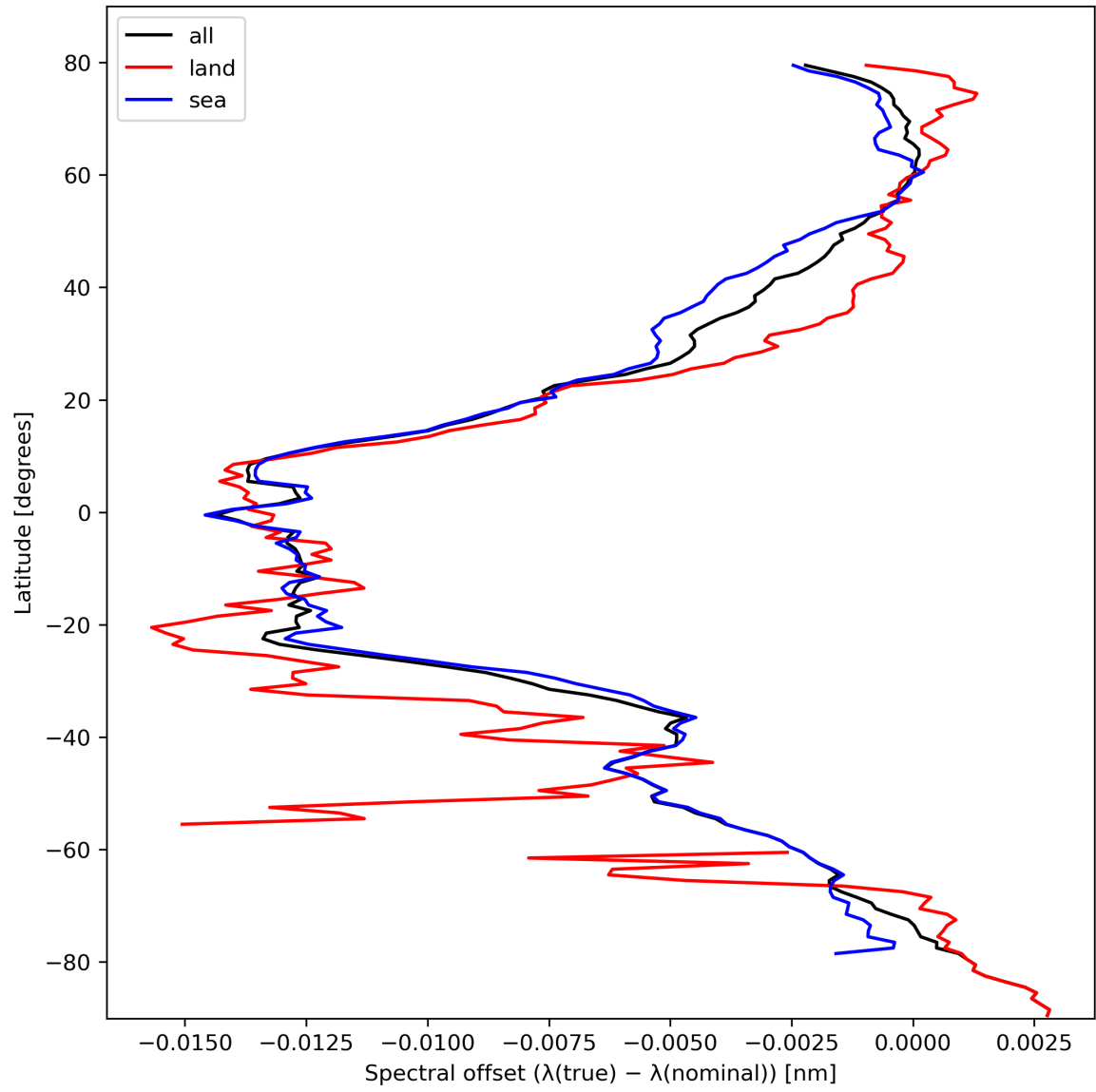
Figure 28: Zonal average of “Spectral offset ( \lambda(\text{true}) - \lambda(\text{nominal}) )” for 2024-02-25 to 2024-02-27.
