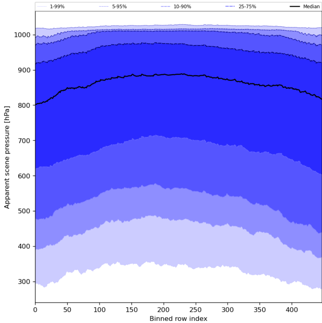
Figure 53: Along track statistics of “Apparent scene pressure” for 2024-02-25 to 2024-02-27
