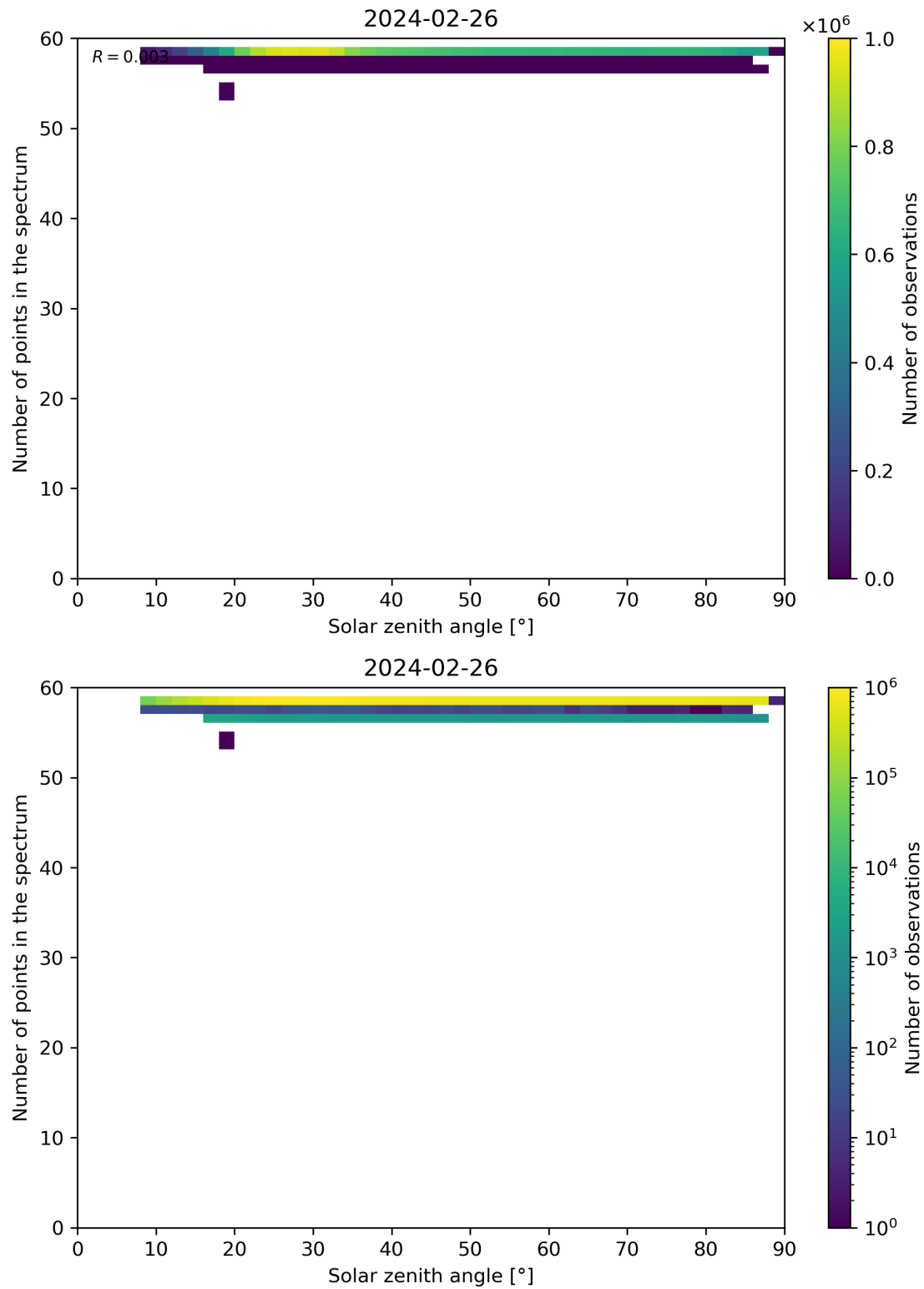
Figure 115: Scatter density plot of “Solar zenith angle” against “Number of points in the spectrum” for 2024-02-25 to 2024-02-27.
