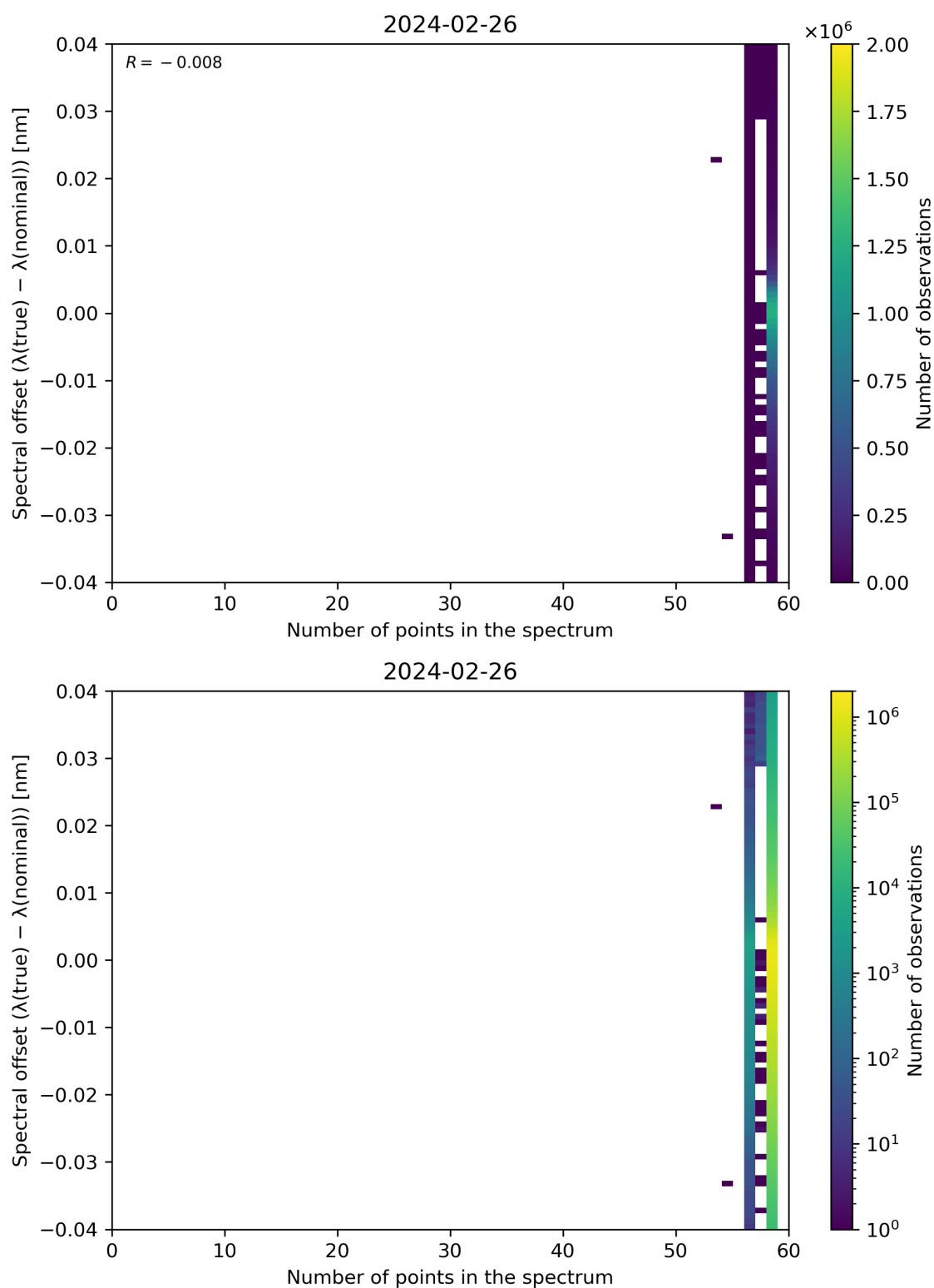
Figure 101: Scatter density plot of “Number of points in the spectrum” against “Spectral offset ( \lambda(\text{true}) - \lambda(\text{nominal}) )” for 2024-02-25 to 2024-02-27.
