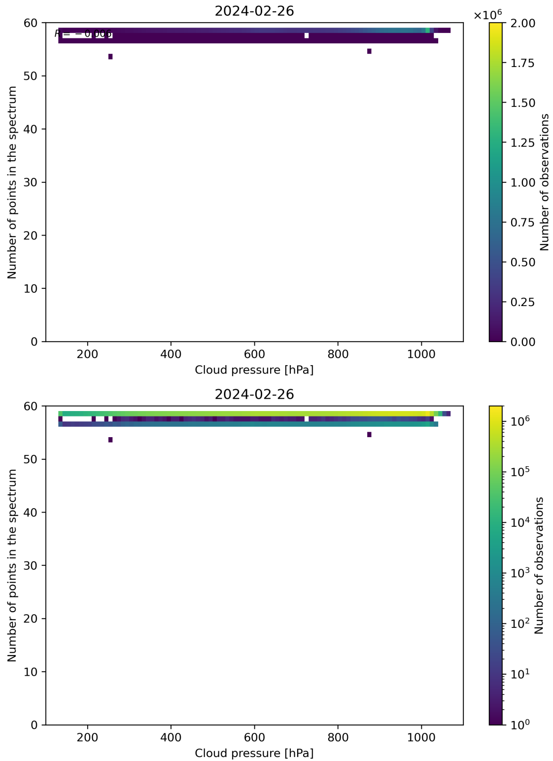
Figure 82: Scatter density plot of “Cloud pressure” against “Number of points in the spectrum” for 2024-02-25 to 2024-02-27.
