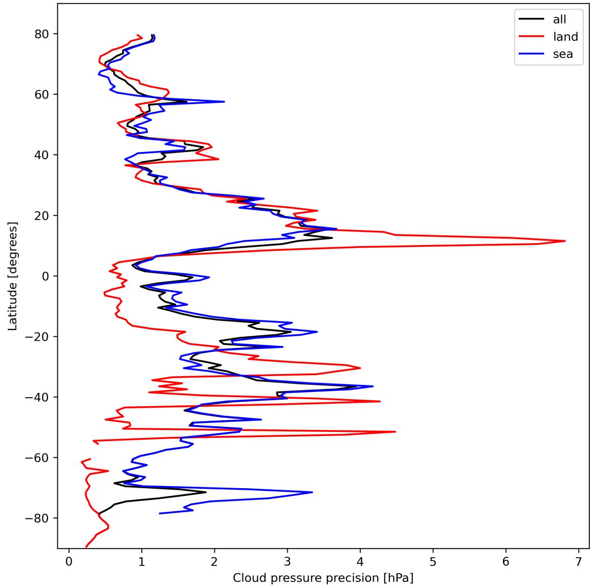
Figure 14: Zonal average of “Cloud pressure precision” for 2024-02-25 to 2024-02-27.
