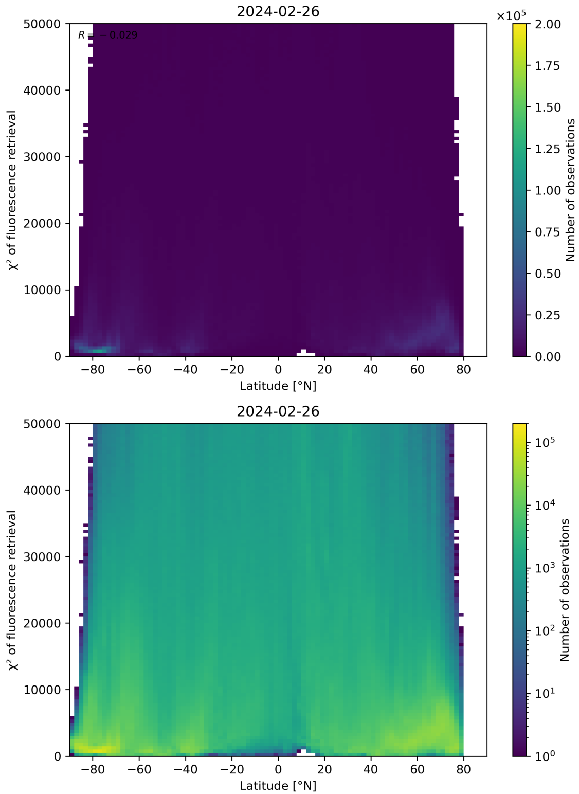
Figure 89: Scatter density plot of “Latitude” against “ \chi^2 of fluorescence retrieval” for 2024-02-25 to 2024-02-27.
