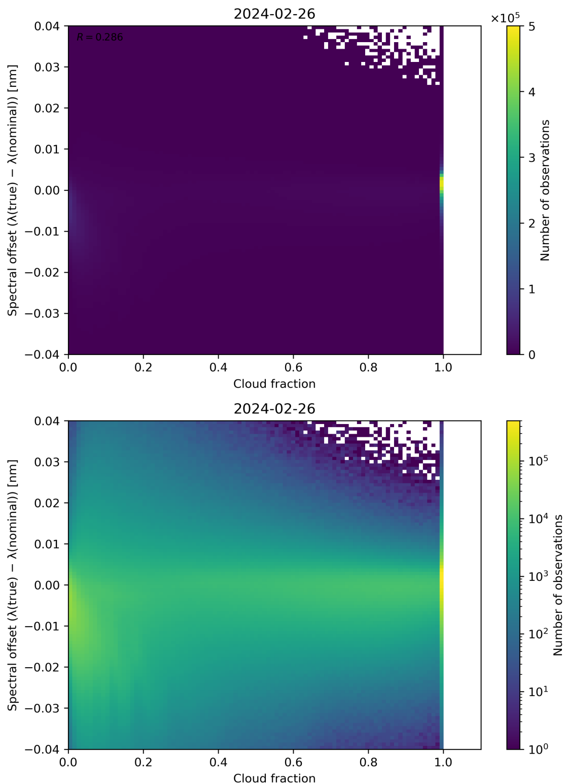
Figure 76: Scatter density plot of “Cloud fraction” against “Spectral offset ( \lambda(\text{true}) - \lambda(\text{nominal}) )” for 2024-02-25 to 2024-02-27.
