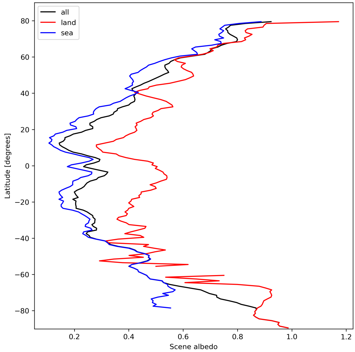
Figure 17: Zonal average of “Scene albedo” for 2024-02-25 to 2024-02-27.
