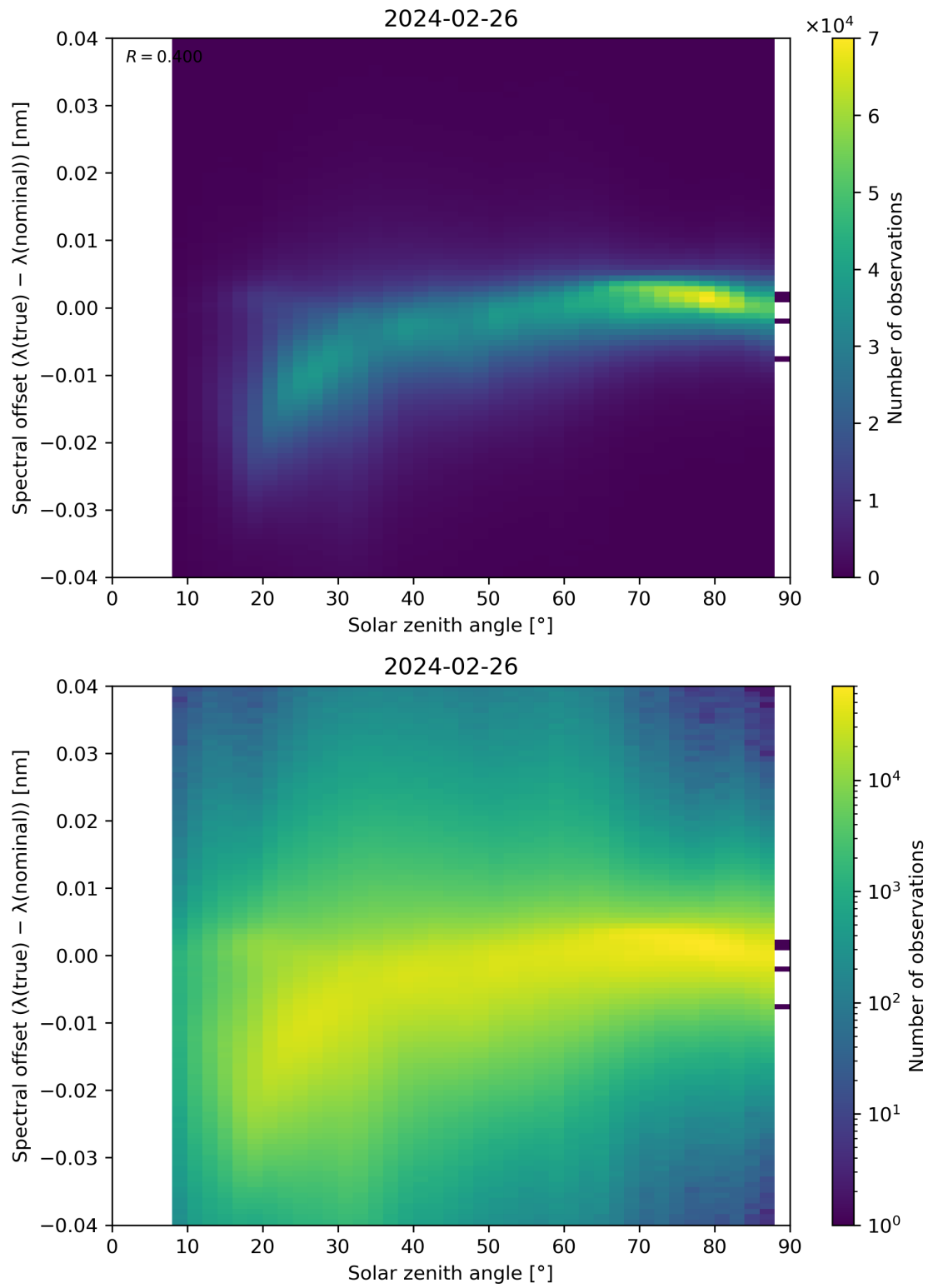
Figure 117: Scatter density plot of “Solar zenith angle” against “Spectral offset ( \lambda(\text{true}) - \lambda(\text{nominal}) )” for 2024-02-25 to 2024-02-27.
