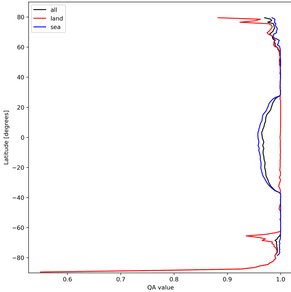
Figure 12: Zonal average of “QA value” for 2024-02-25 to 2024-02-27.
