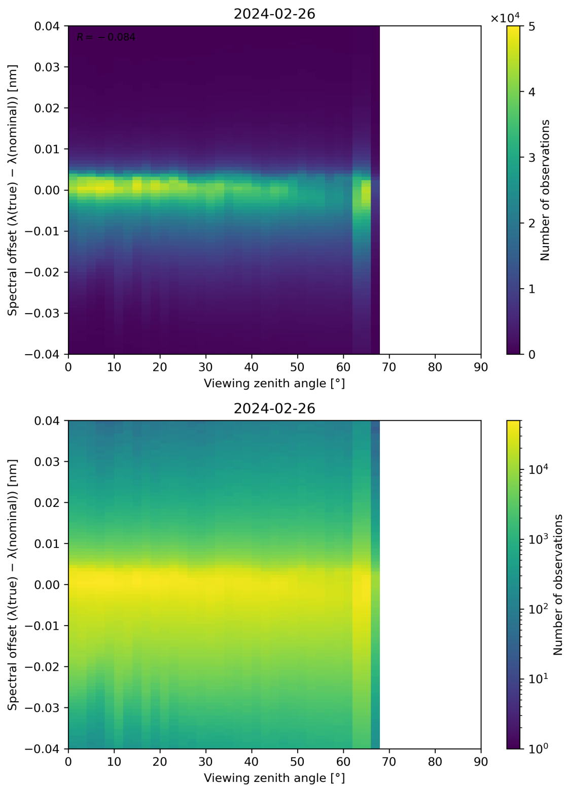
Figure 128: Scatter density plot of “Viewing zenith angle” against “Spectral offset ( \lambda(\text{true}) - \lambda(\text{nominal}) )” for 2024-02-25 to 2024-02-27.
