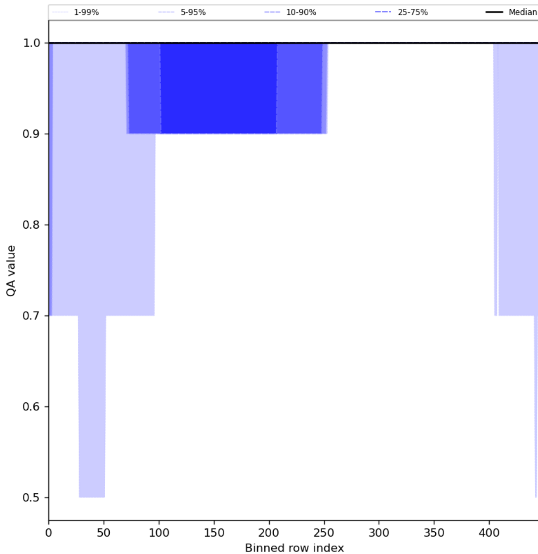
Figure 46: Along track statistics of “QA value” for 2024-02-25 to 2024-02-27
