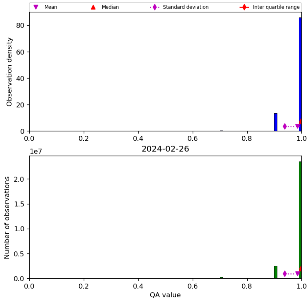
Figure 29: Histogram of “QA value” for 2024-02-25 to 2024-02-27
