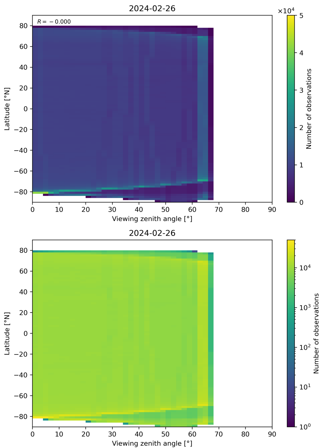
Figure 123: Scatter density plot of “Viewing zenith angle” against “Latitude” for 2024-02-25 to 2024-02-27.
