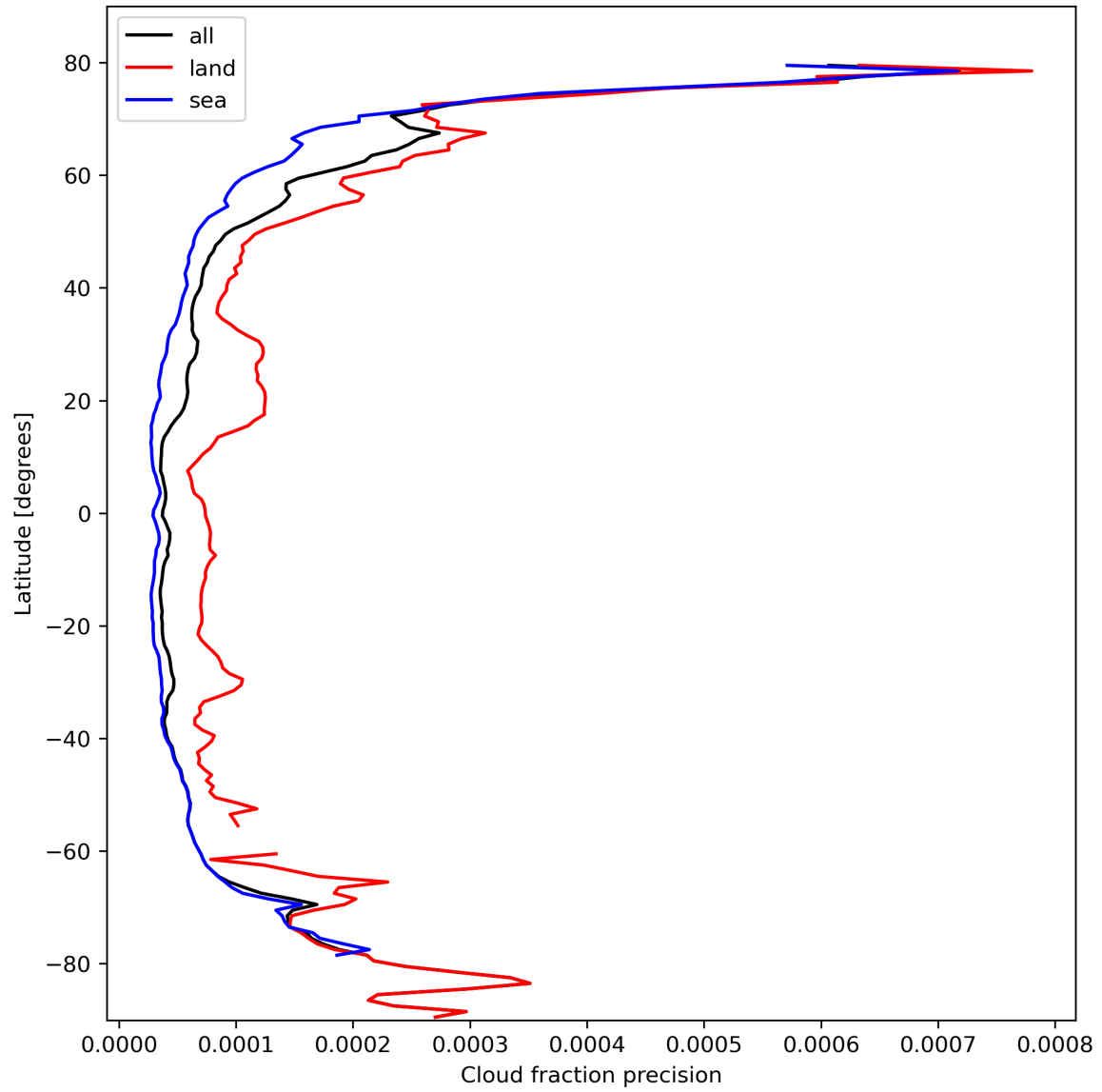
Figure 16: Zonal average of “Cloud fraction precision” for 2024-02-25 to 2024-02-27.
