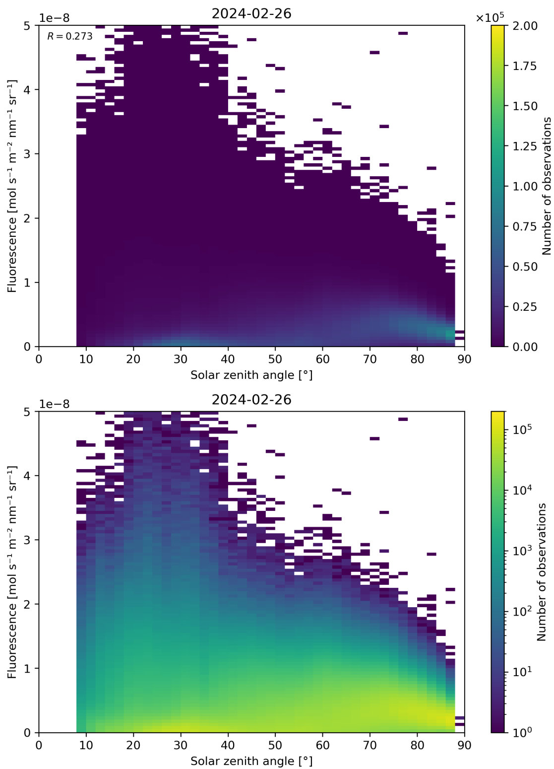
Figure 112: Scatter density plot of “Solar zenith angle” against “Fluorescence” for 2024-02-25 to 2024-02-27.
