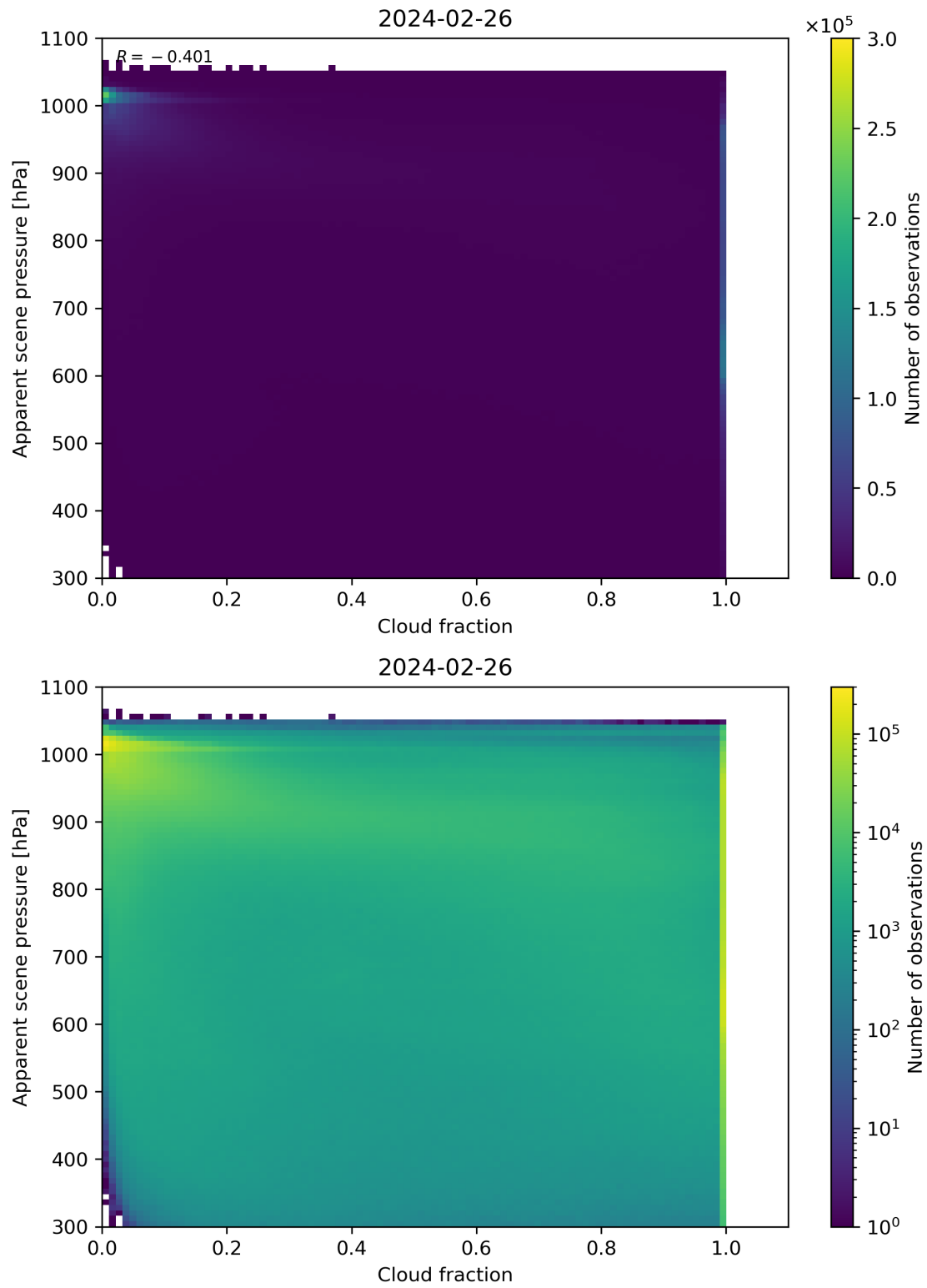
Figure 70: Scatter density plot of “Cloud fraction” against “Apparent scene pressure” for 2024-02-25 to 2024-02-27.
