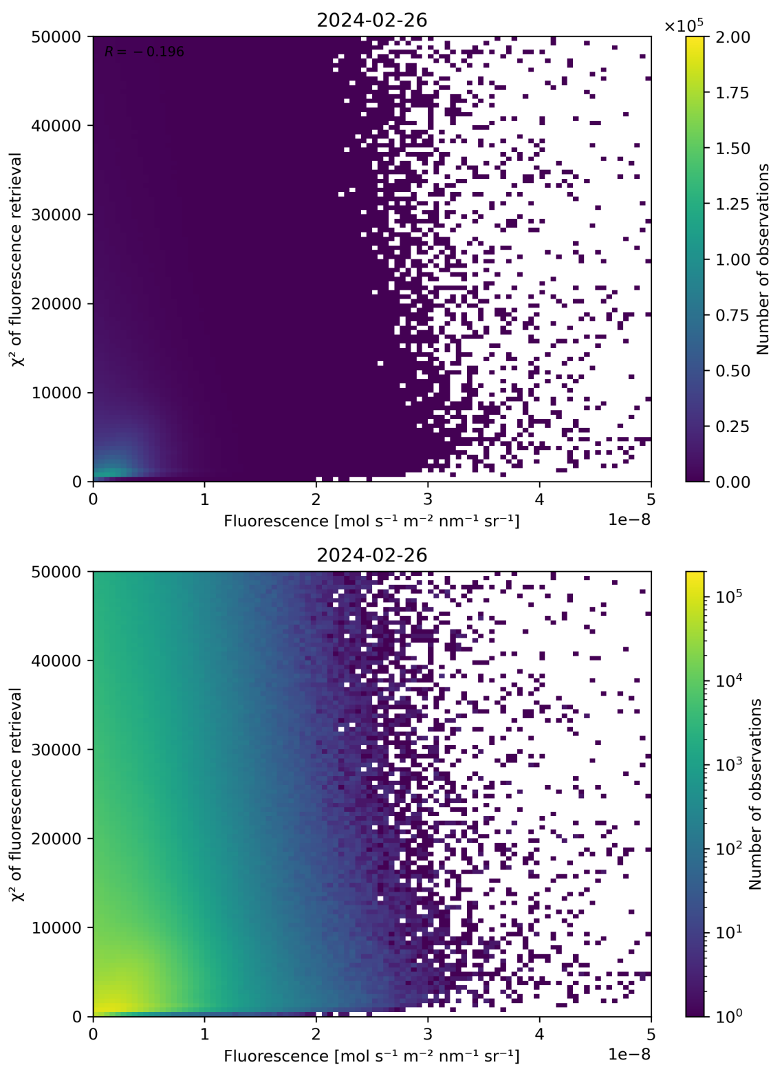
Figure 85: Scatter density plot of “Fluorescence” against “ \chi^2 of fluorescence retrieval” for 2024-02-25 to 2024-02-27.
