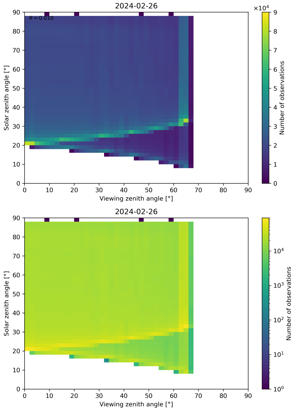
Figure 127: Scatter density plot of “Viewing zenith angle” against “Solar zenith angle” for 2024-02-25 to 2024-02-27.
