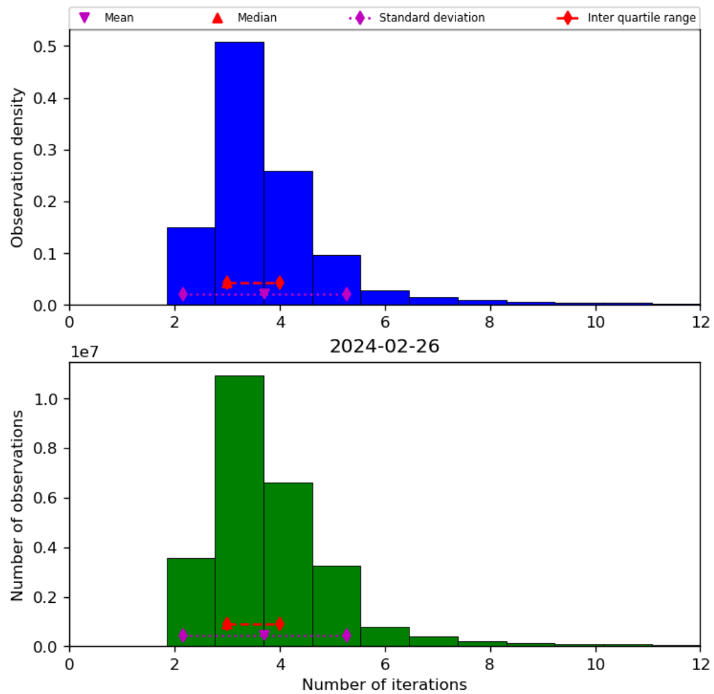
Figure 39: Histogram of “Number of iterations” for 2024-02-25 to 2024-02-27
