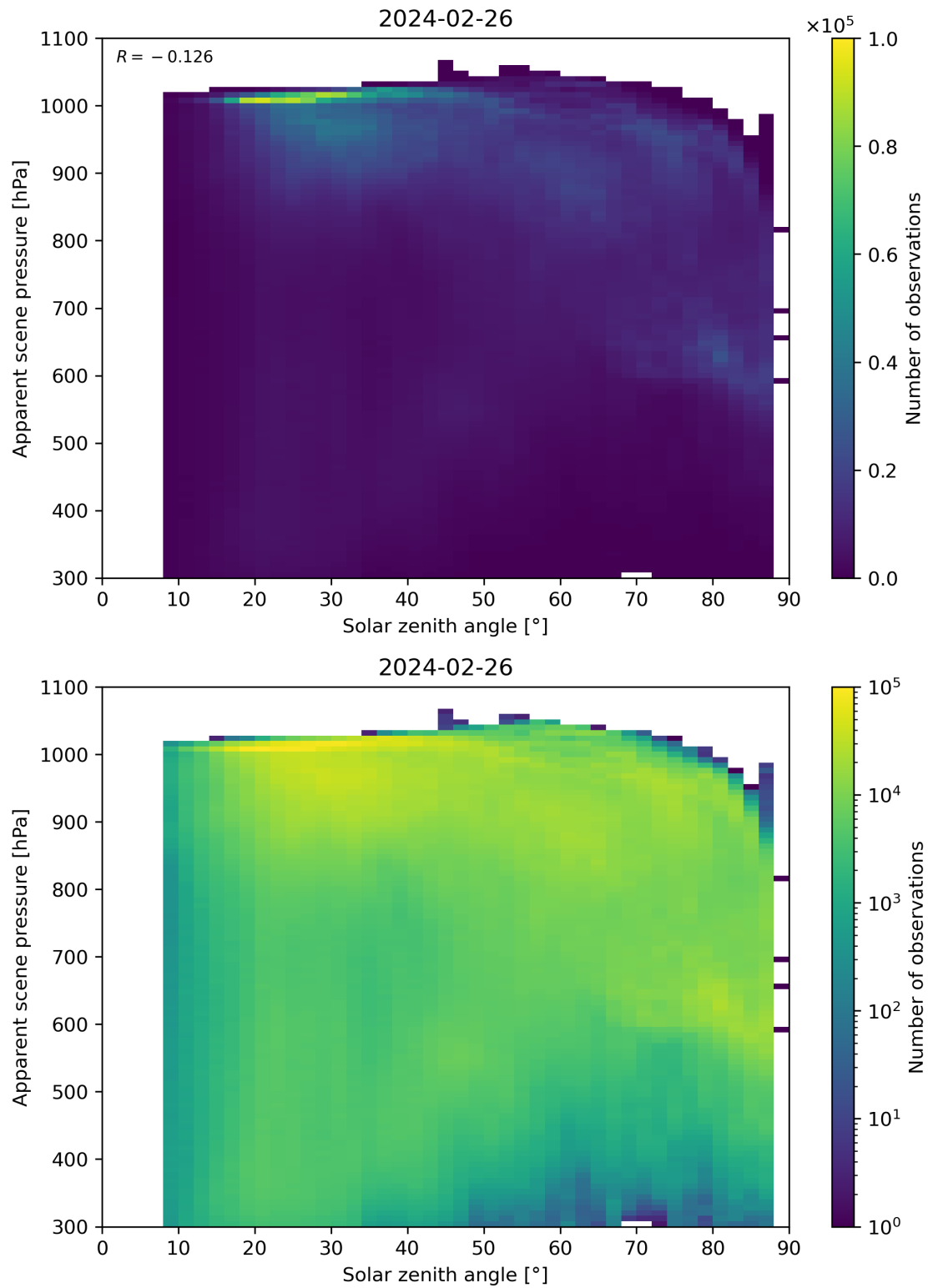
Figure 108: Scatter density plot of “Solar zenith angle” against “Apparent scene pressure” for 2024-02-25 to 2024-02-27.
