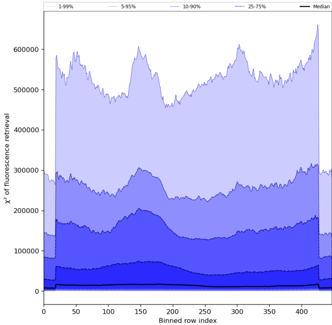
Figure 59: Along track statistics of “ \chi^2 of fluorescence retrieval” for 2024-02-25 to 2024-02-27
