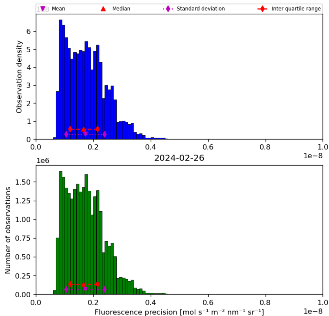
Figure 41: Histogram of “Fluorescence precision” for 2024-02-25 to 2024-02-27
