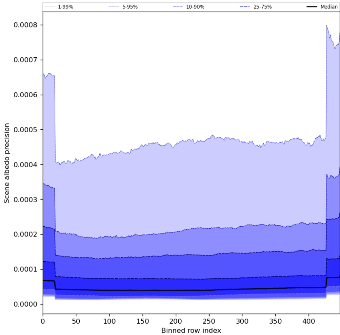
Figure 52: Along track statistics of “Scene albedo precision” for 2024-02-25 to 2024-02-27
