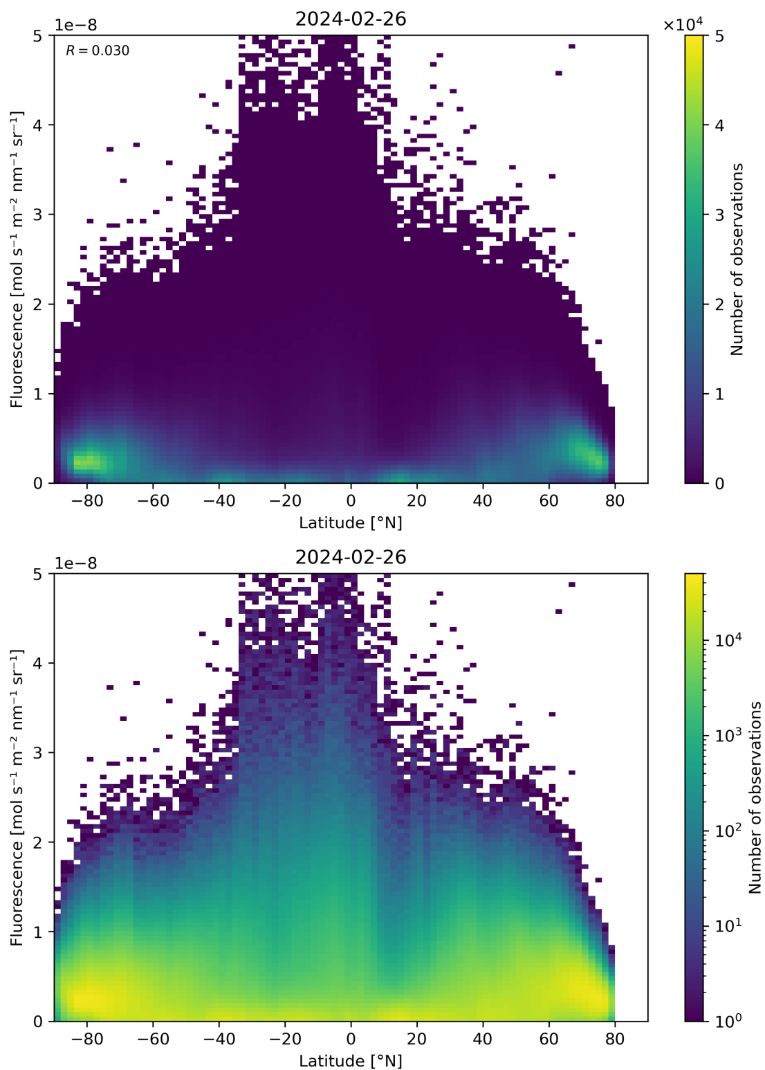
Figure 92: Scatter density plot of “Latitude” against “Fluorescence” for 2024-02-25 to 2024-02-27.
