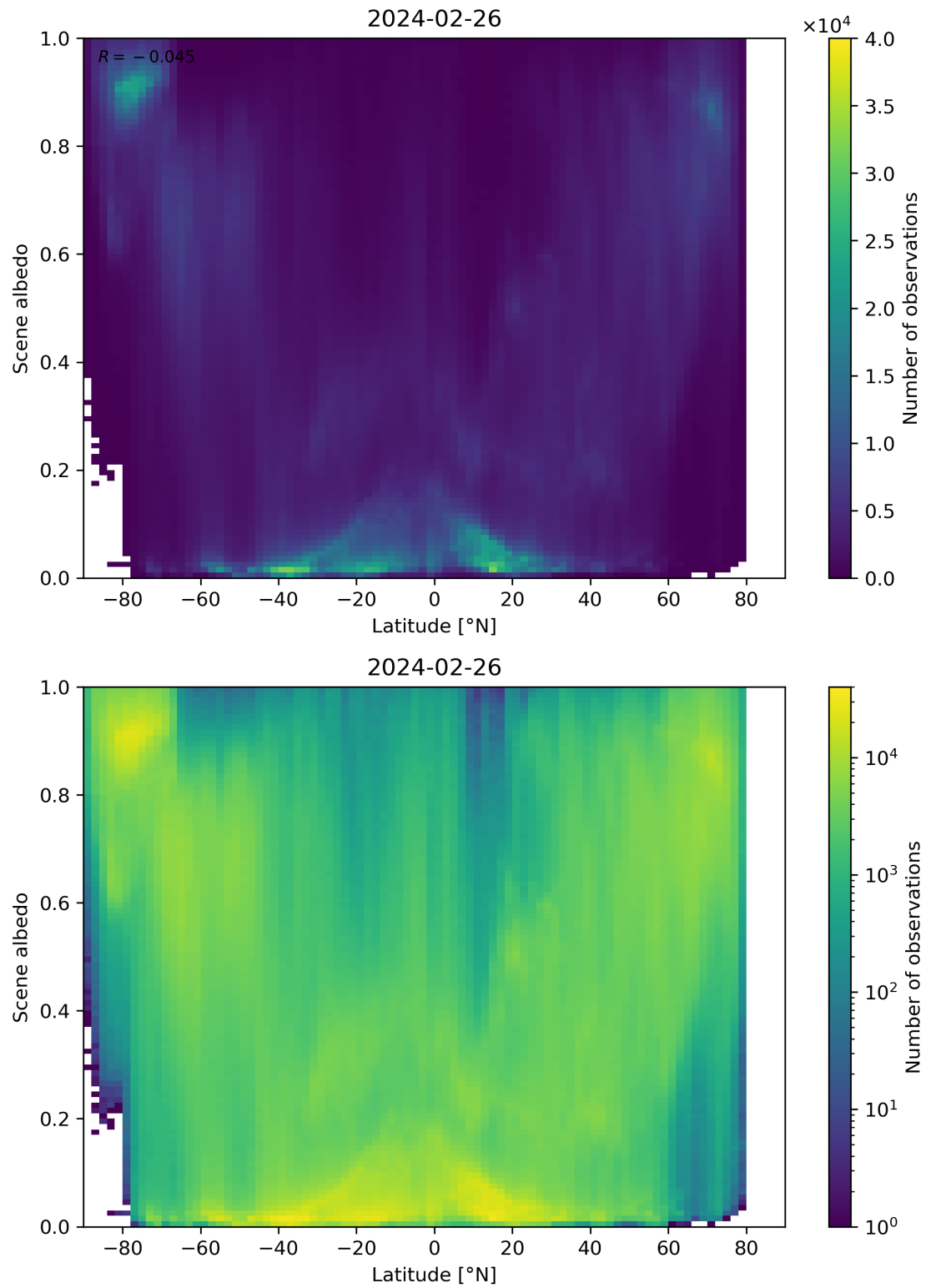
Figure 95: Scatter density plot of “Latitude” against “Scene albedo” for 2024-02-25 to 2024-02-27.
