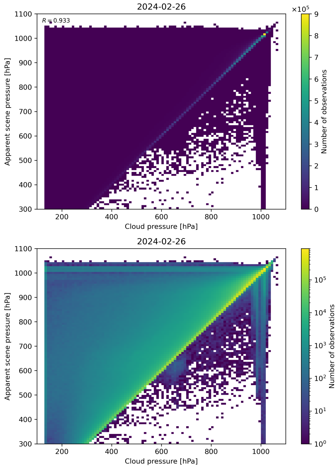
Figure 77: Scatter density plot of “Cloud pressure” against “Apparent scene pressure” for 2024-02-25 to 2024-02-27.
