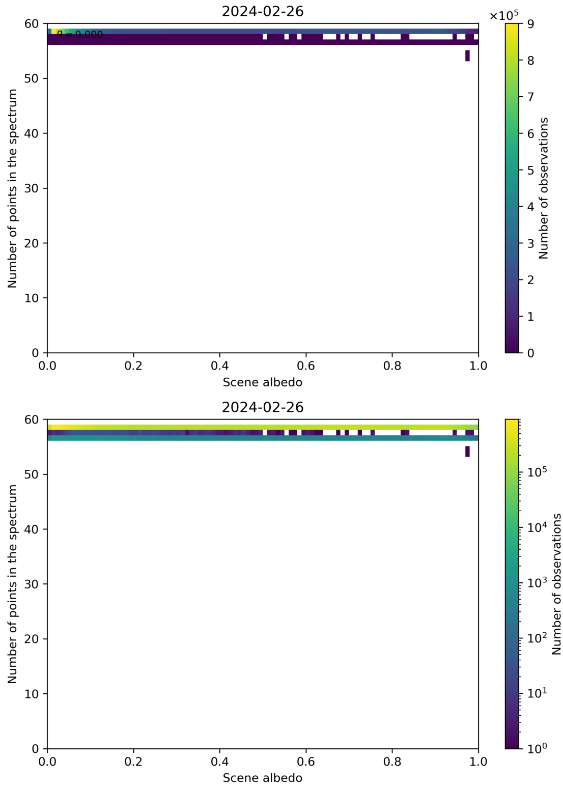
Figure 106: Scatter density plot of “Scene albedo” against “Number of points in the spectrum” for 2024-02-25 to 2024-02-27.
