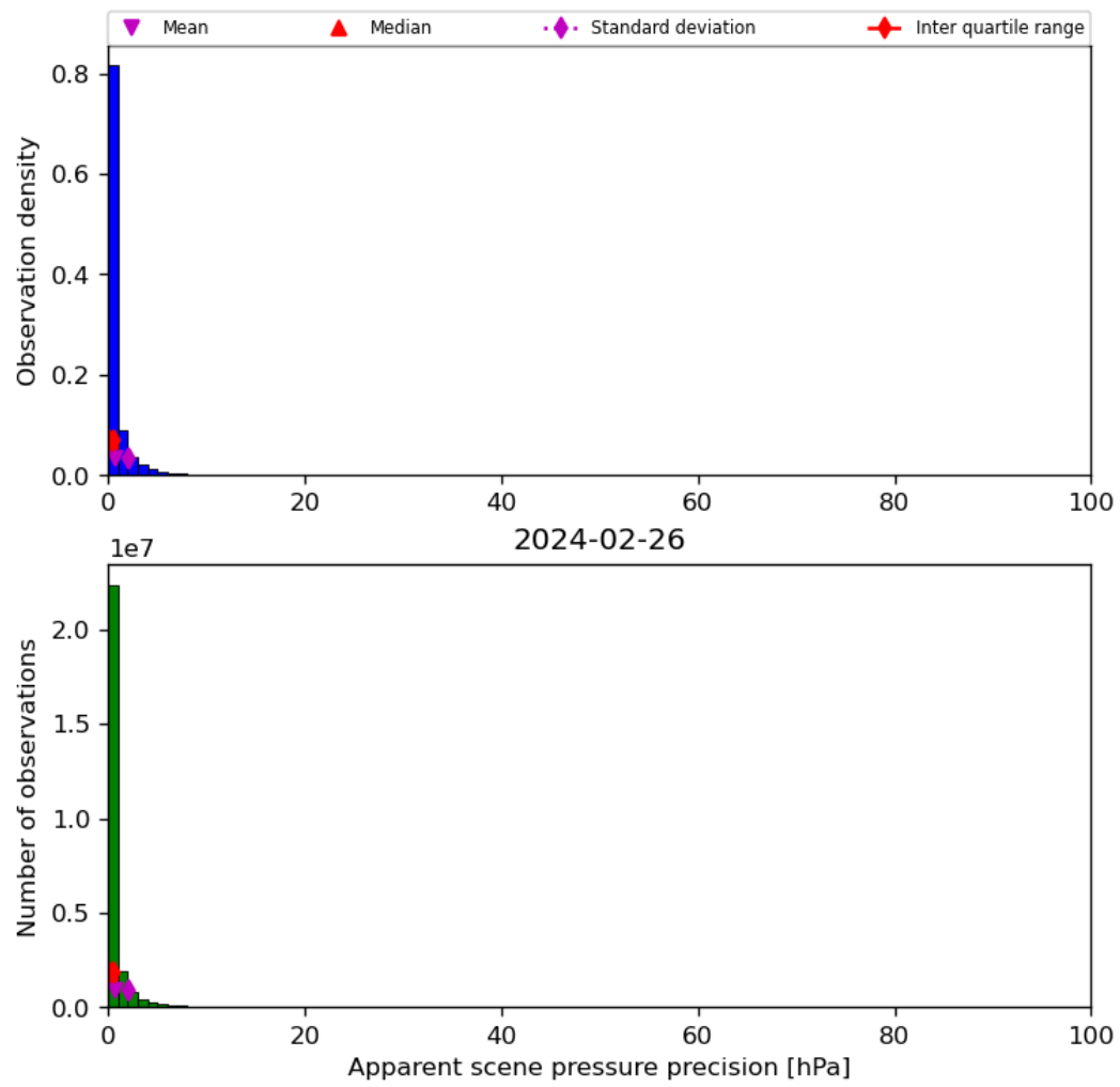
Figure 37: Histogram of “Apparent scene pressure precision” for 2024-02-25 to 2024-02-27
