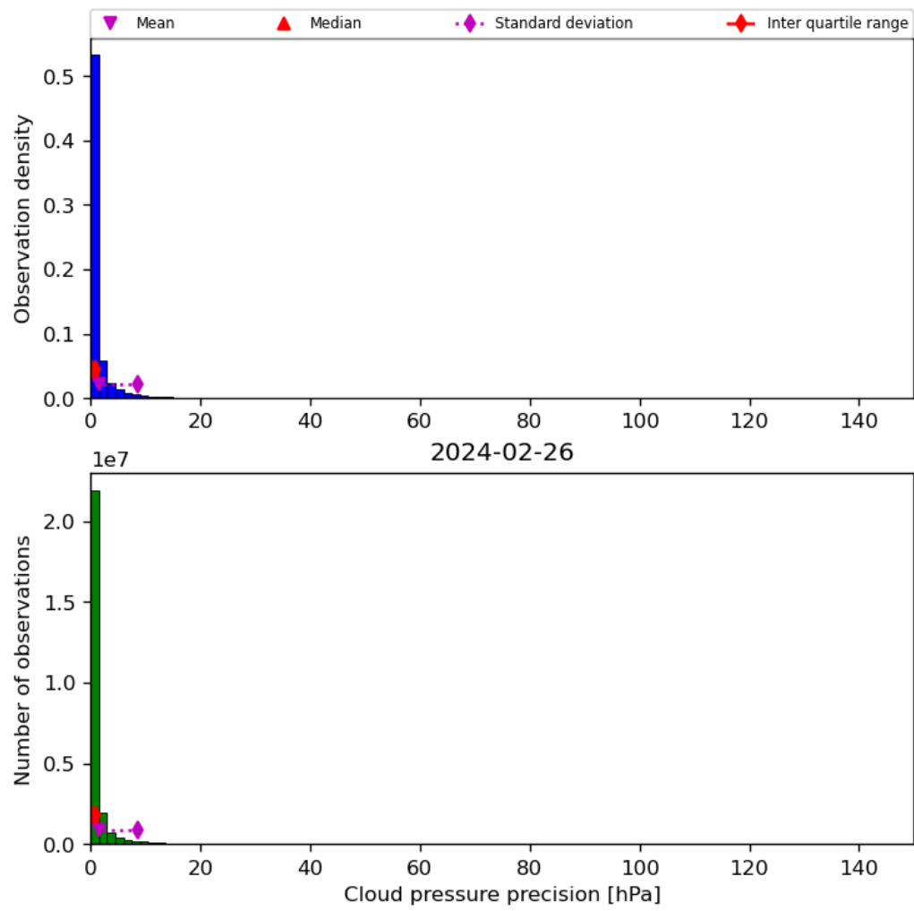
Figure 31: Histogram of “Cloud pressure precision” for 2024-02-25 to 2024-02-27
