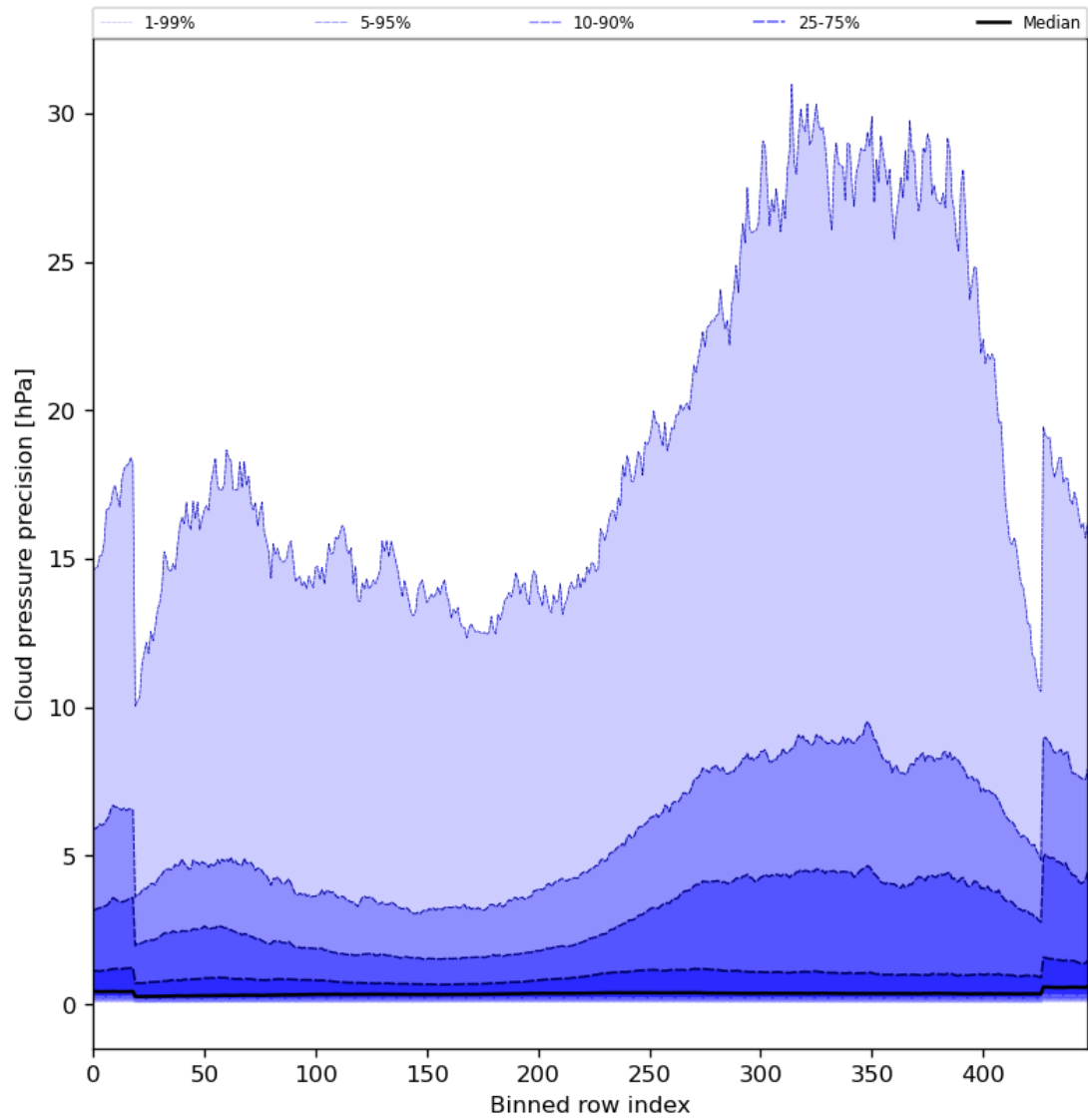
Figure 48: Along track statistics of “Cloud pressure precision” for 2024-02-25 to 2024-02-27
