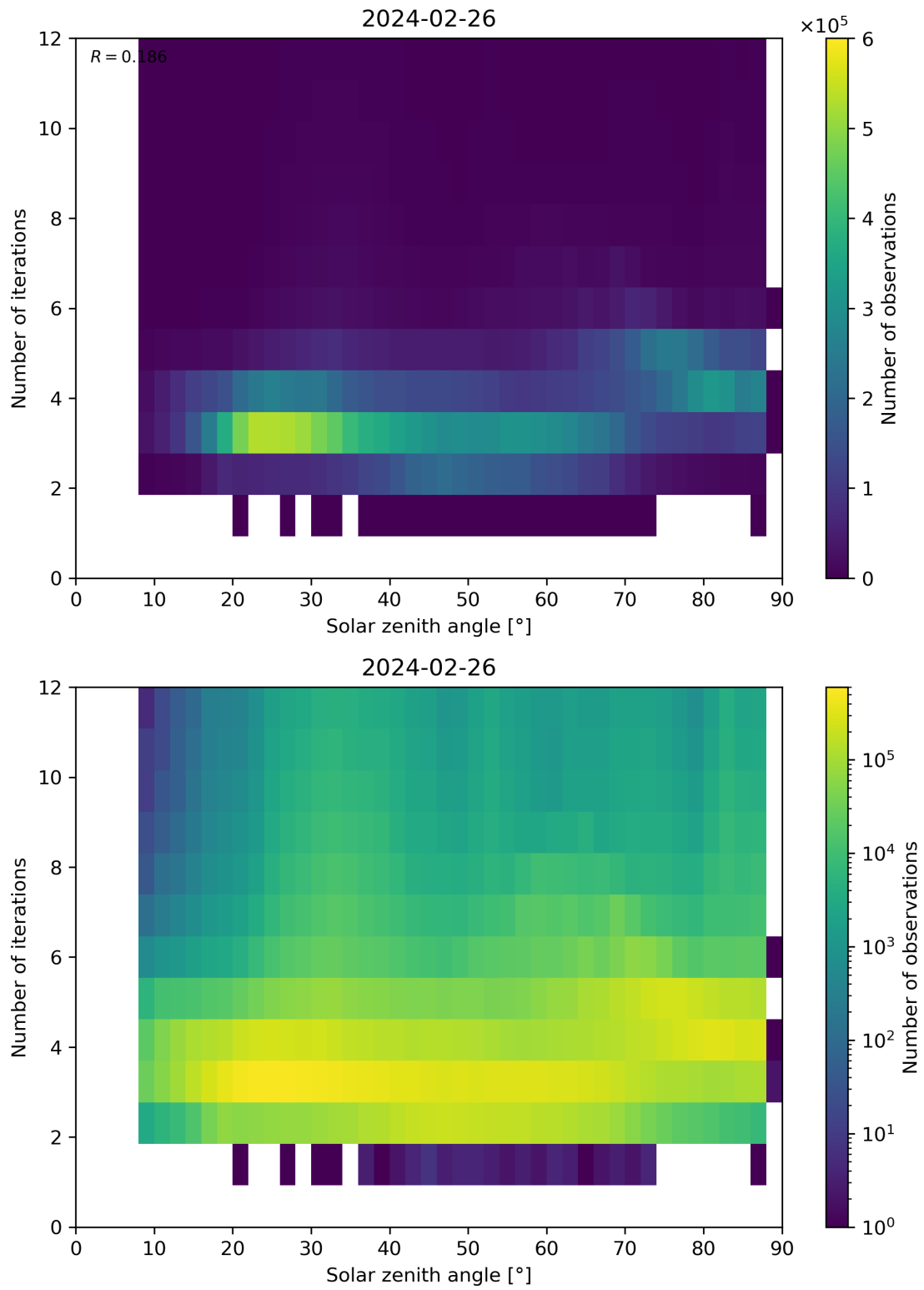
Figure 114: Scatter density plot of “Solar zenith angle” against “Number of iterations” for 2024-02-25 to 2024-02-27.
