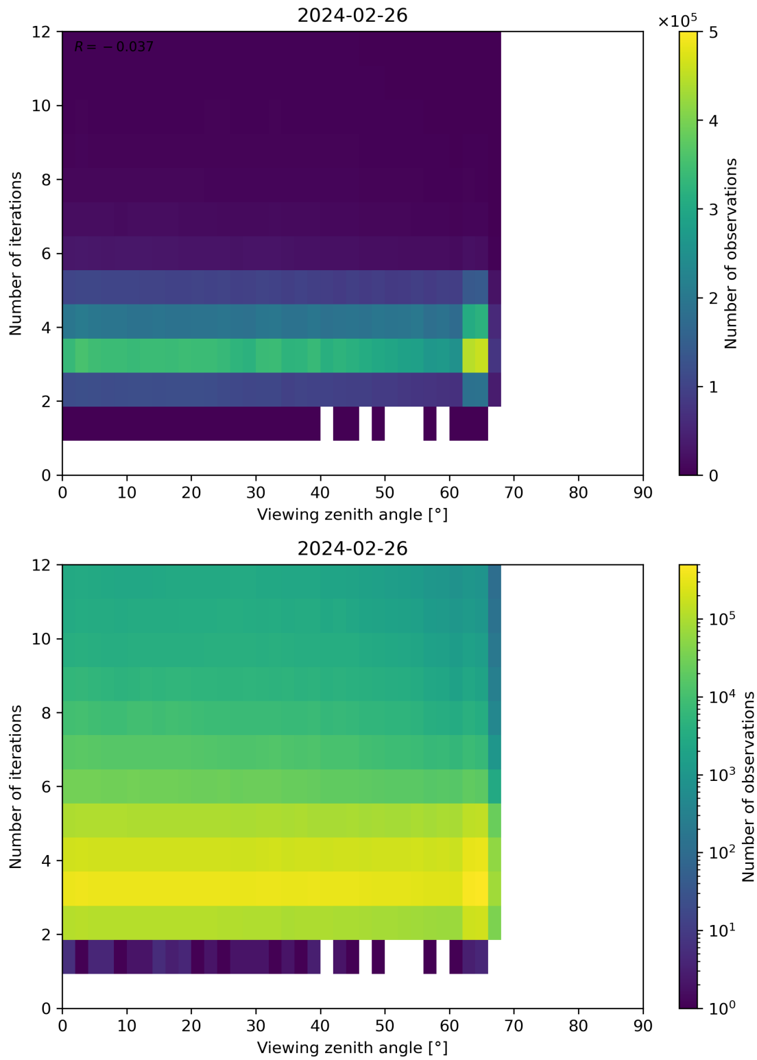
Figure 124: Scatter density plot of “Viewing zenith angle” against “Number of iterations” for 2024-02-25 to 2024-02-27.
