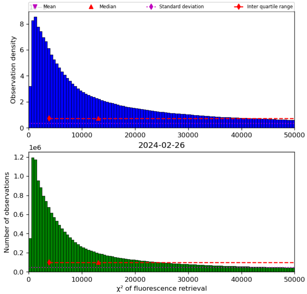
Figure 42: Histogram of “ \chi^2 of fluorescence retrieval” for 2024-02-25 to 2024-02-27
