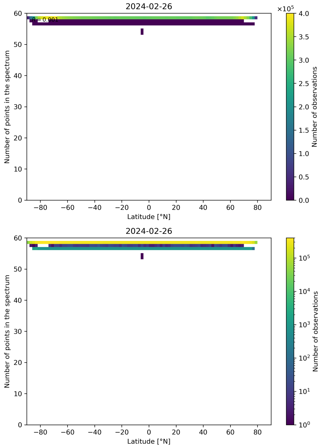
Figure 94: Scatter density plot of “Latitude” against “Number of points in the spectrum” for 2024-02-25 to 2024-02-27.
