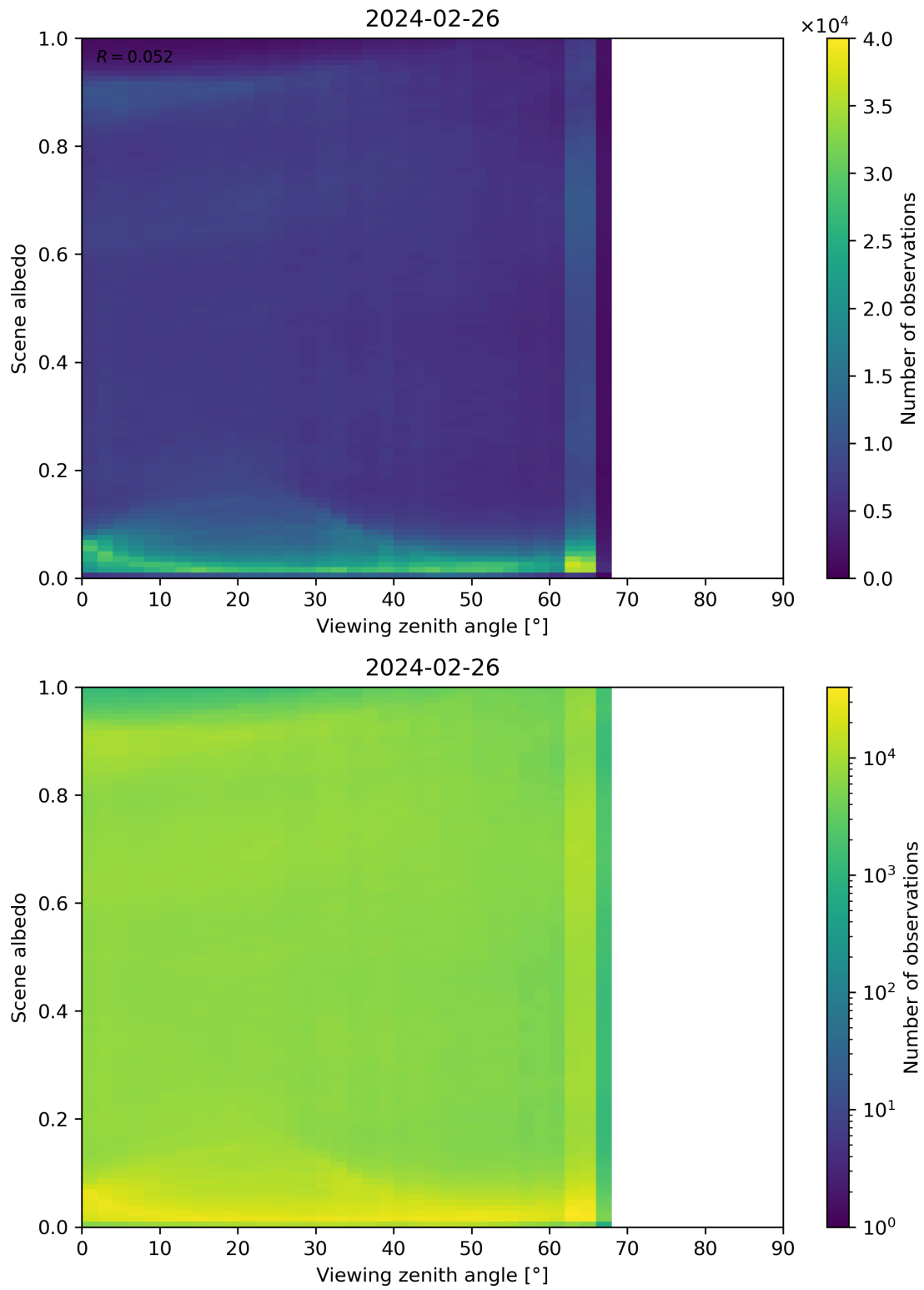
Figure 126: Scatter density plot of “Viewing zenith angle” against “Scene albedo” for 2024-02-25 to 2024-02-27.
