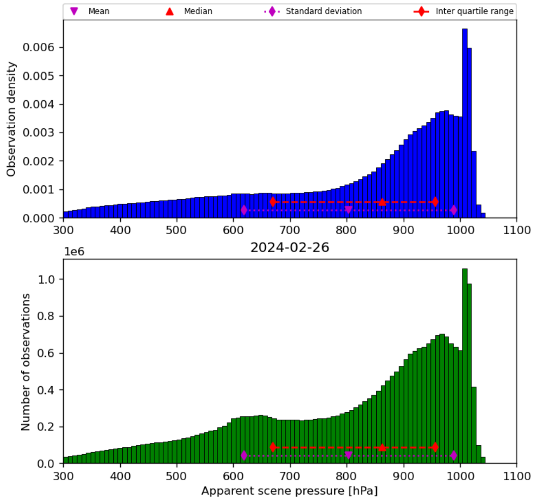
Figure 36: Histogram of “Apparent scene pressure” for 2024-02-25 to 2024-02-27
