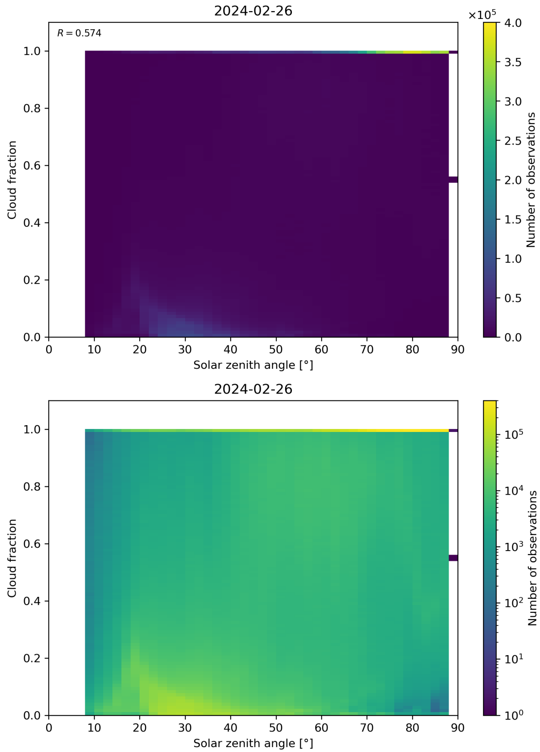
Figure 110: Scatter density plot of “Solar zenith angle” against “Cloud fraction” for 2024-02-25 to 2024-02-27.
