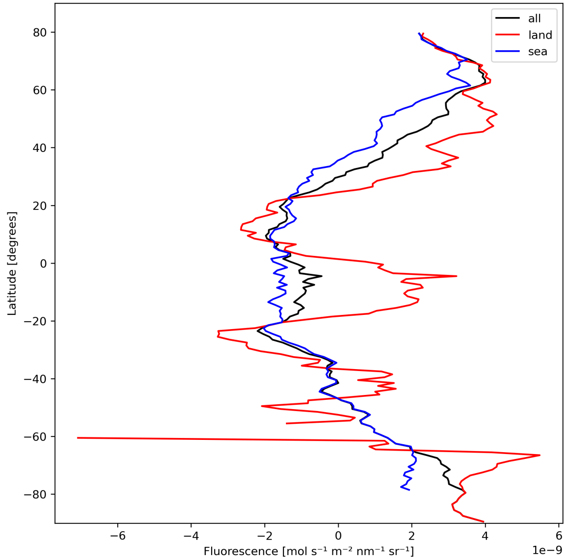
Figure 23: Zonal average of “Fluorescence” for 2024-02-25 to 2024-02-27.
