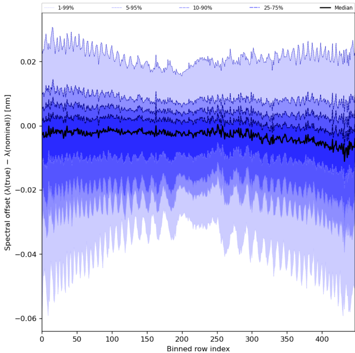
Figure 62: Along track statistics of “Spectral offset ( \lambda(\text{true}) - \lambda(\text{nominal}) )” for 2024-02-25 to 2024-02-27
