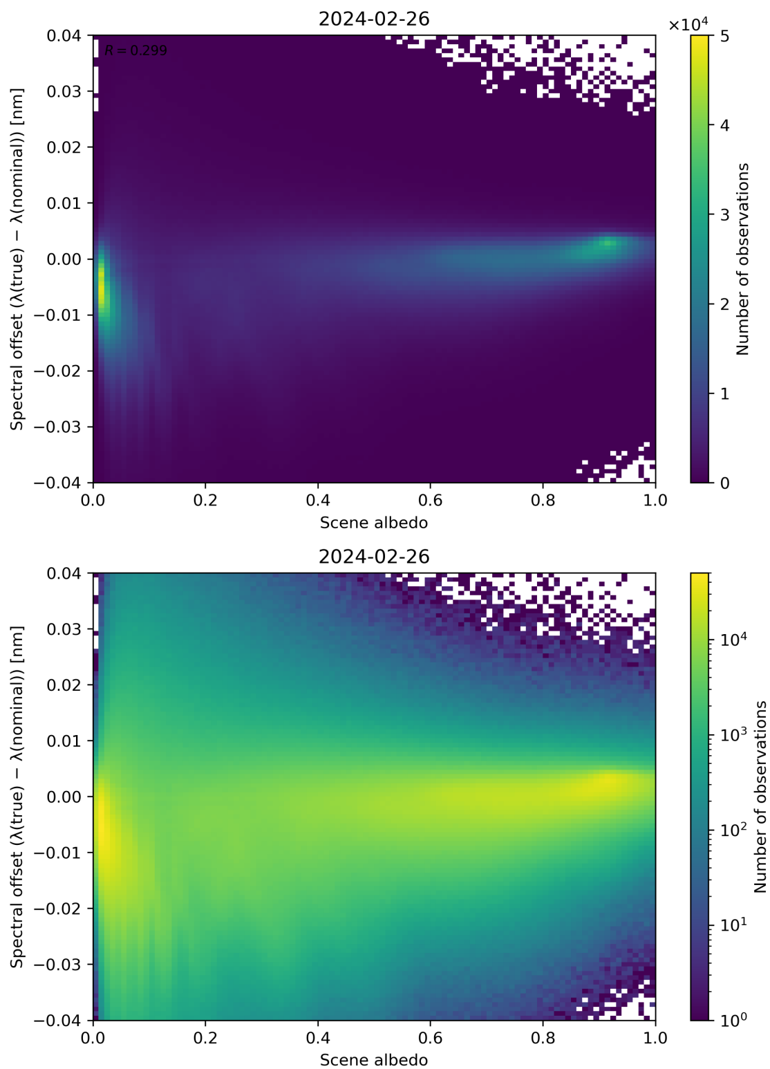
Figure 107: Scatter density plot of “Scene albedo” against “Spectral offset ( \lambda(\text{true}) - \lambda(\text{nominal}) )” for 2024-02-25 to 2024-02-27.
