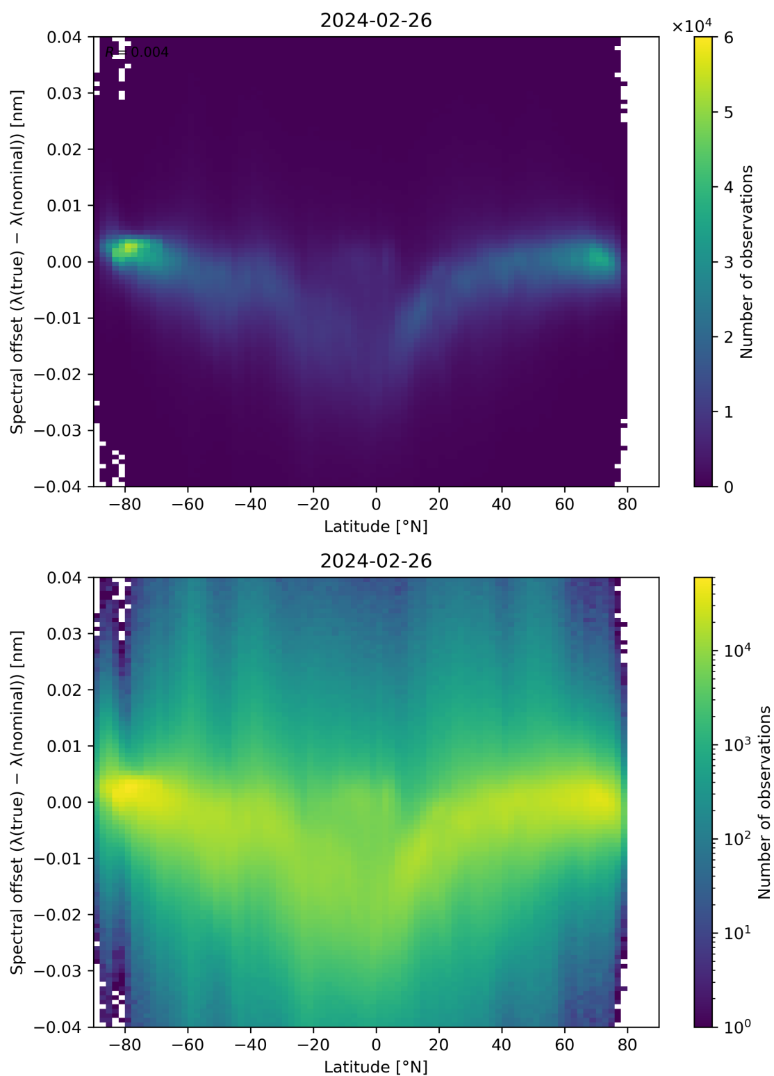
Figure 96: Scatter density plot of “Latitude” against “Spectral offset ( \lambda(\text{true}) - \lambda(\text{nominal}) )” for 2024-02-25 to 2024-02-27.
