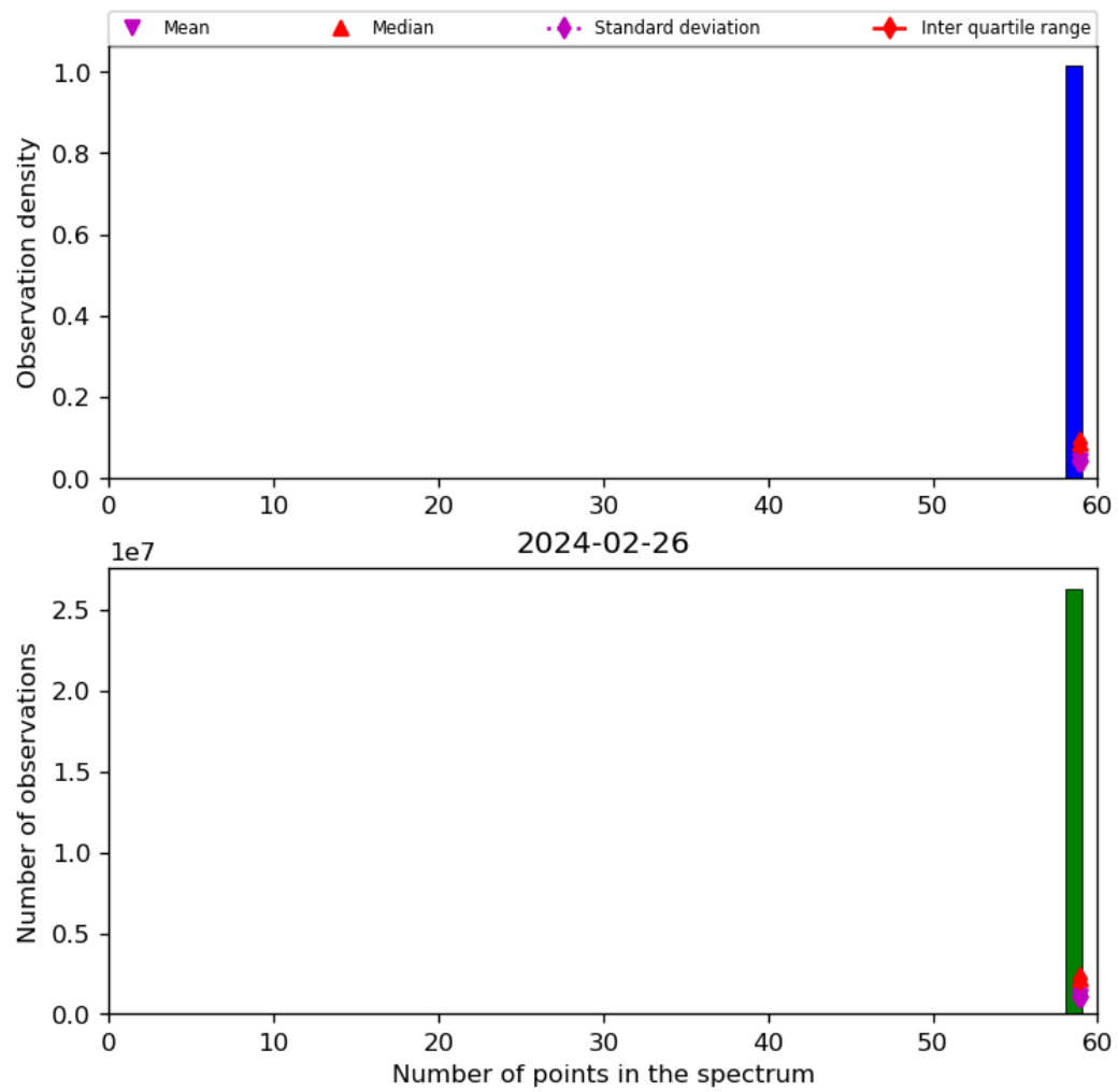
Figure 44: Histogram of “Number of points in the spectrum” for 2024-02-25 to 2024-02-27
