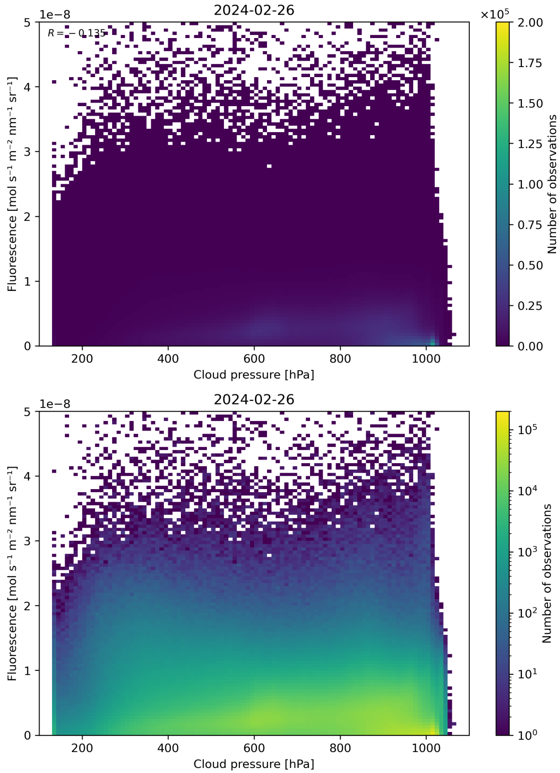
Figure 80: Scatter density plot of “Cloud pressure” against “Fluorescence” for 2024-02-25 to 2024-02-27.
