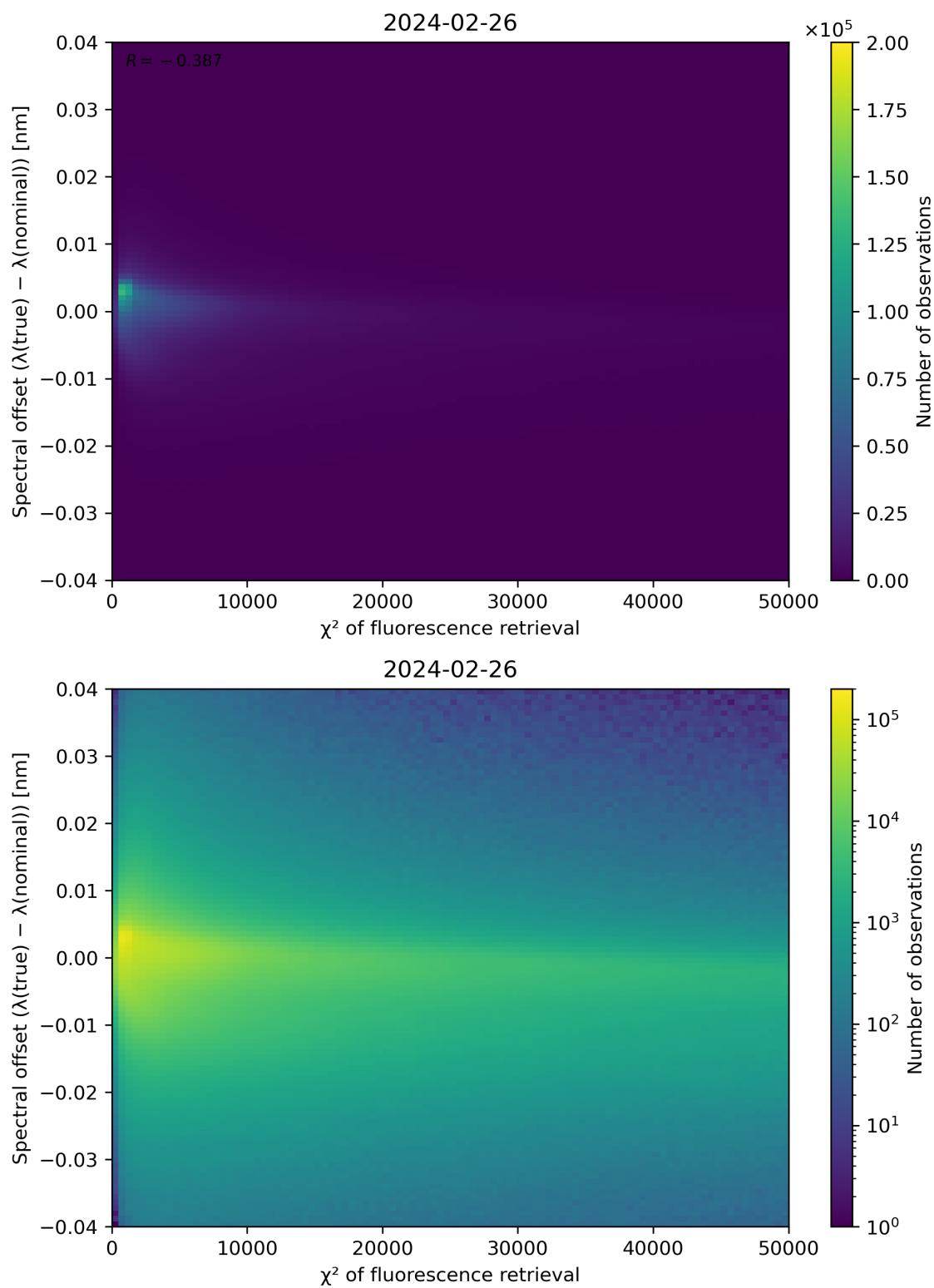
Figure 69: Scatter density plot of " \chi^2 of fluorescence retrieval" against "Spectral offset ( \lambda(\text{true}) - \lambda(\text{nominal}) )" for 2024-02-25 to 2024-02-27.
