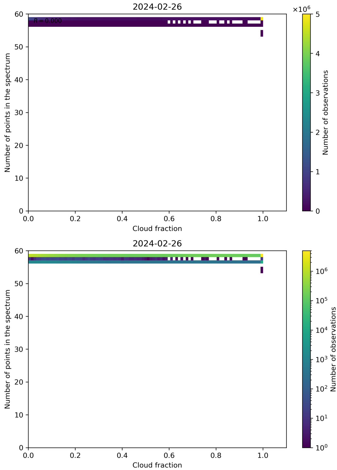
Figure 74: Scatter density plot of “Cloud fraction” against “Number of points in the spectrum” for 2024-02-25 to 2024-02-27.
