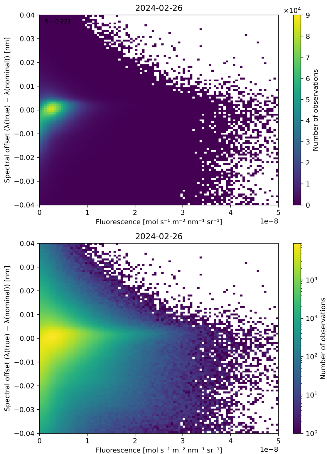
Figure 87: Scatter density plot of “Fluorescence” against “Spectral offset ( \lambda(\text{true}) - \lambda(\text{nominal}) )” for 2024-02-25 to 2024-02-27.
