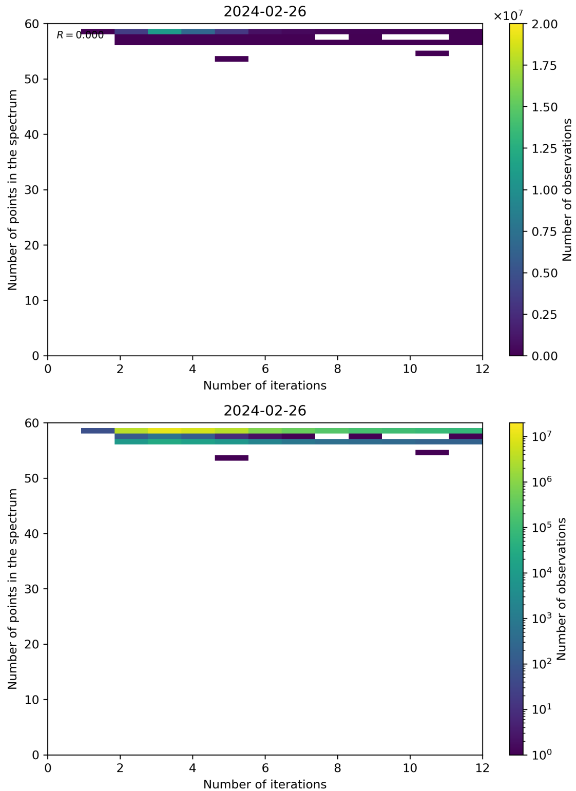
Figure 99: Scatter density plot of “Number of iterations” against “Number of points in the spectrum” for 2024-02-25 to 2024-02-27.
