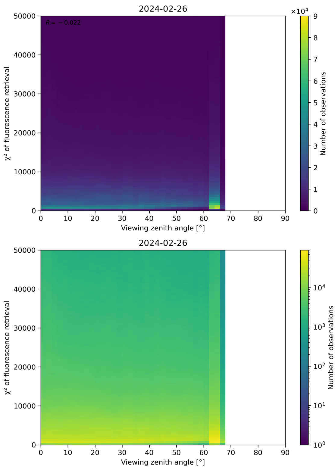
Figure 119: Scatter density plot of “Viewing zenith angle” against “ \chi^2 of fluorescence retrieval” for 2024-02-25 to 2024-02-27.
