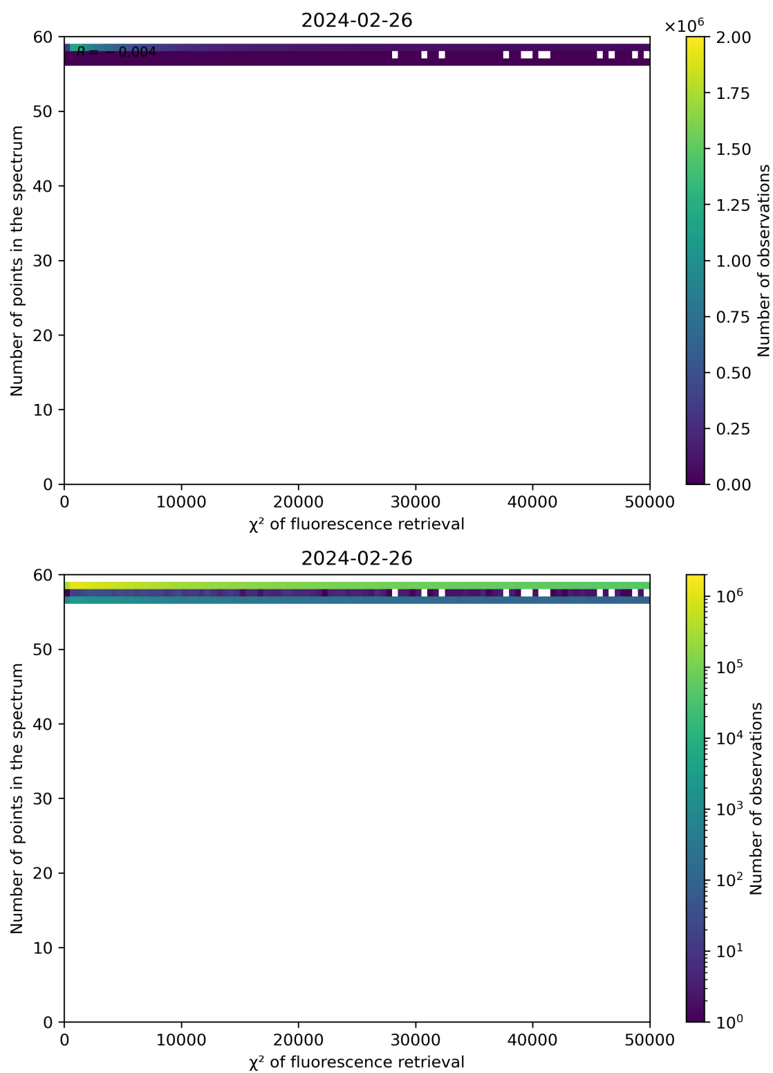
Figure 68: Scatter density plot of " \chi^2 of fluorescence retrieval" against "Number of points in the spectrum" for 2024-02-25 to 2024-02-27.
