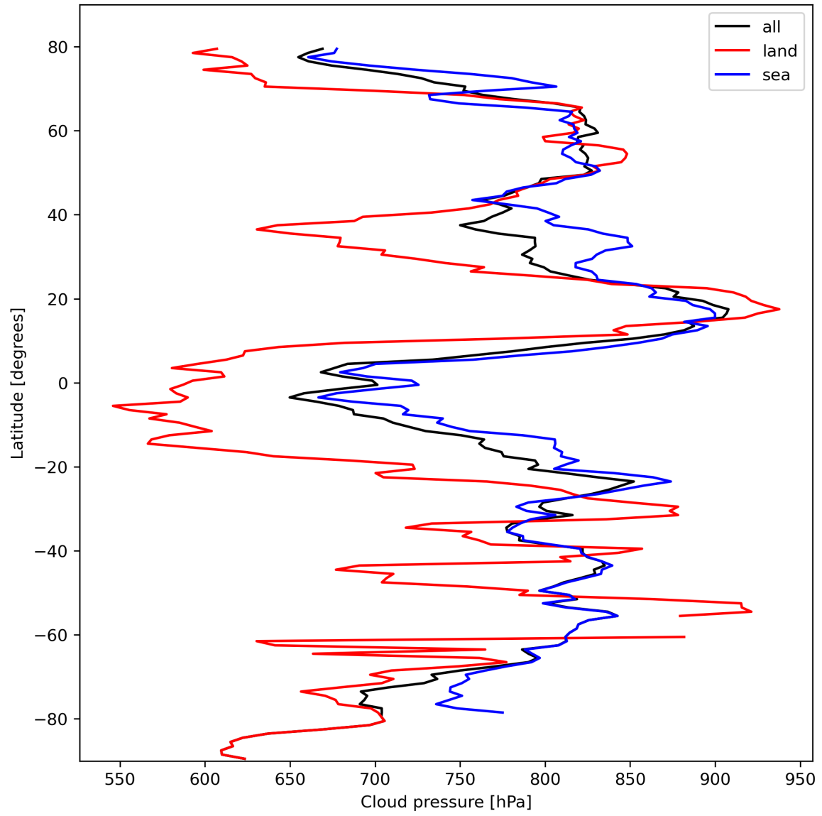
Figure 13: Zonal average of “Cloud pressure” for 2024-02-25 to 2024-02-27.
