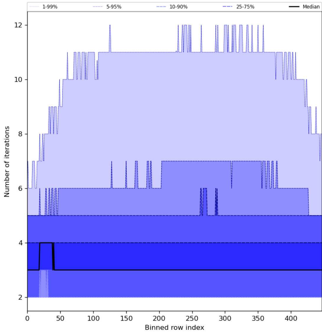
Figure 56: Along track statistics of “Number of iterations” for 2024-02-25 to 2024-02-27
