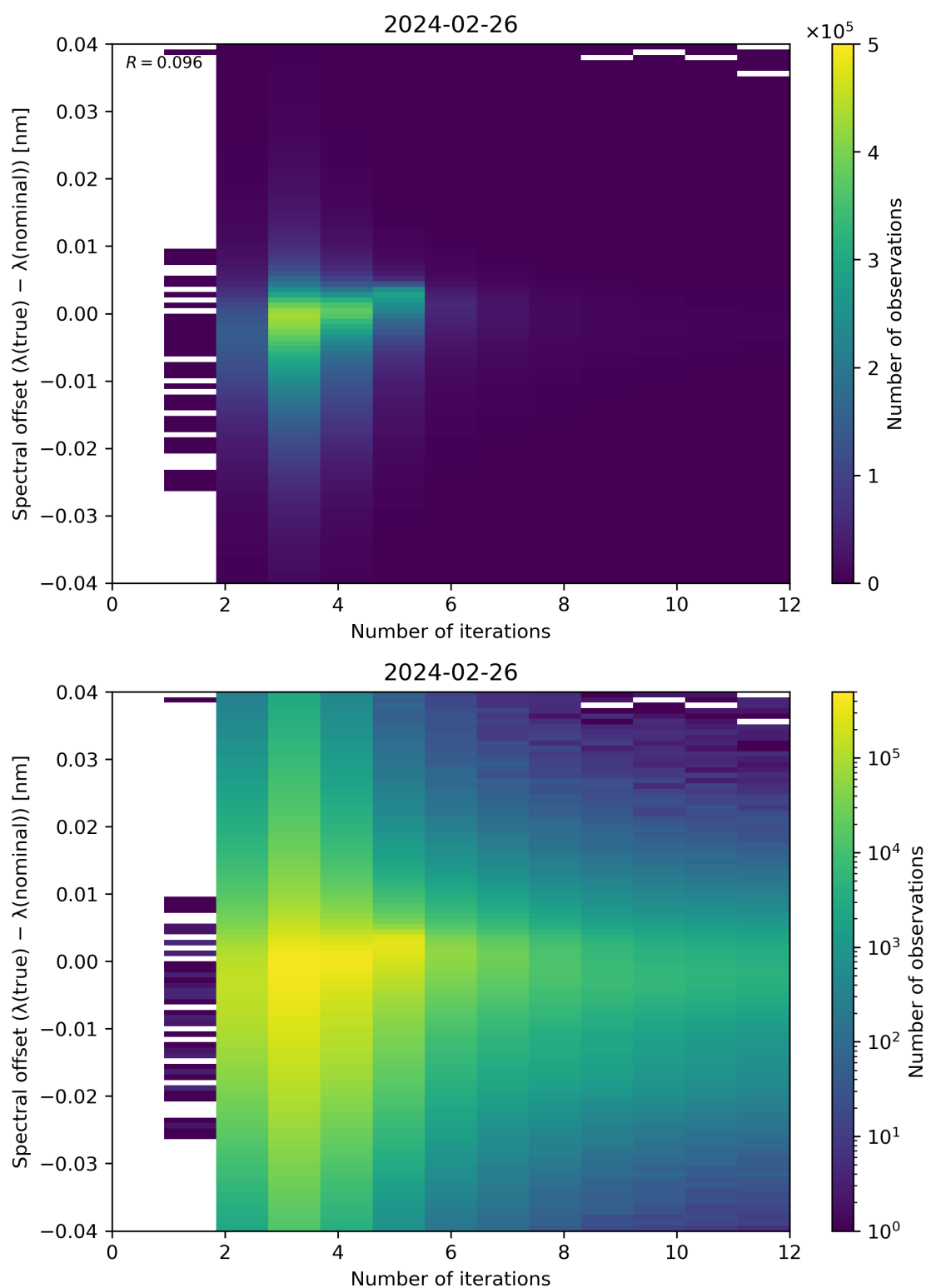
Figure 100: Scatter density plot of “Number of iterations” against “Spectral offset ( \lambda(\text{true}) - \lambda(\text{nominal}) )” for 2024-02-25 to 2024-02-27.
