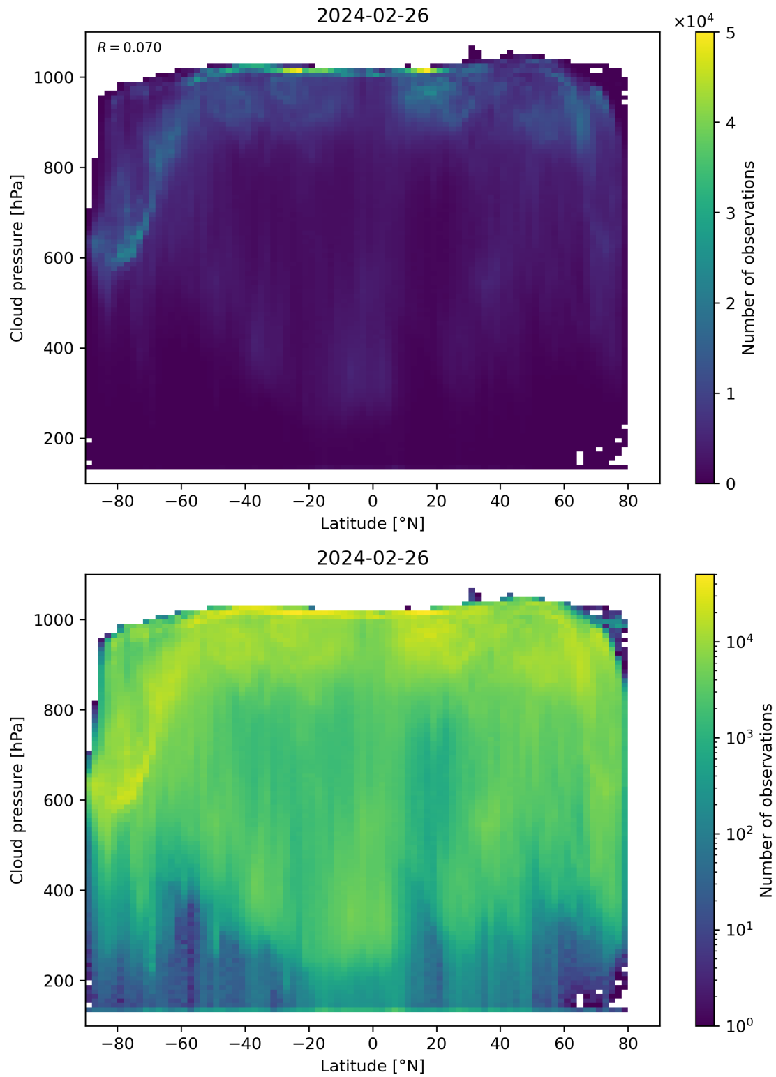
Figure 91: Scatter density plot of “Latitude” against “Cloud pressure” for 2024-02-25 to 2024-02-27.
