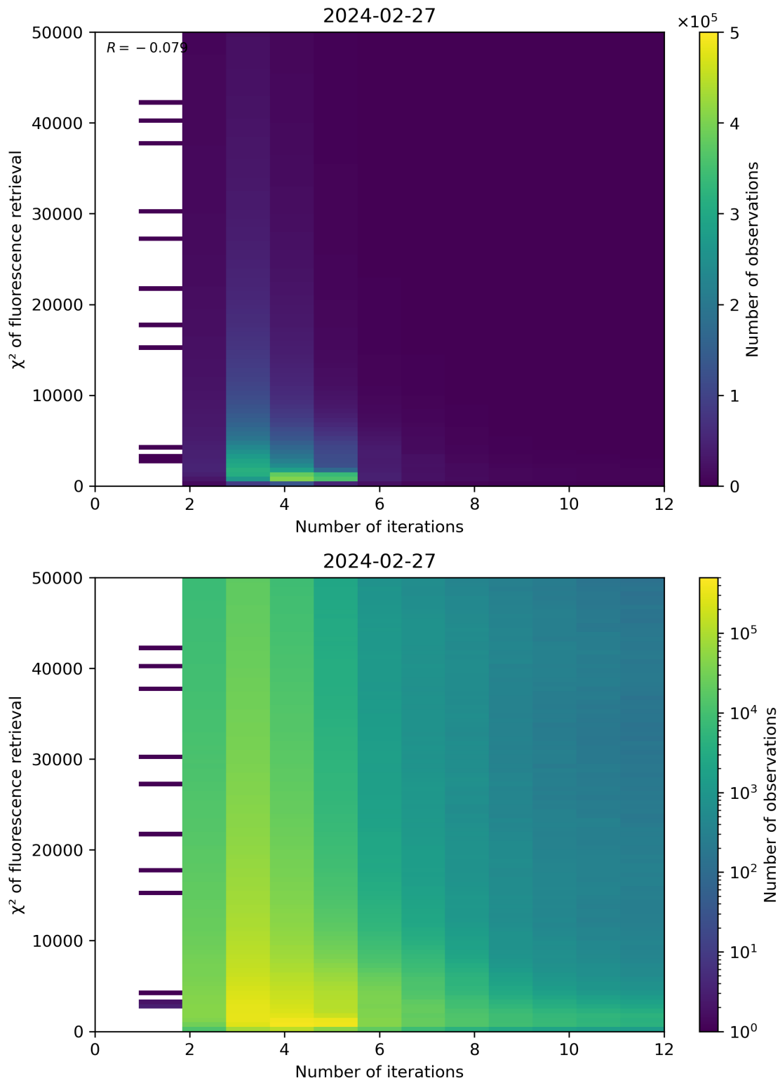
Figure 97: Scatter density plot of “Number of iterations” against “ \chi^2 of fluorescence retrieval” for 2024-02-27 to 2024-02-28.
