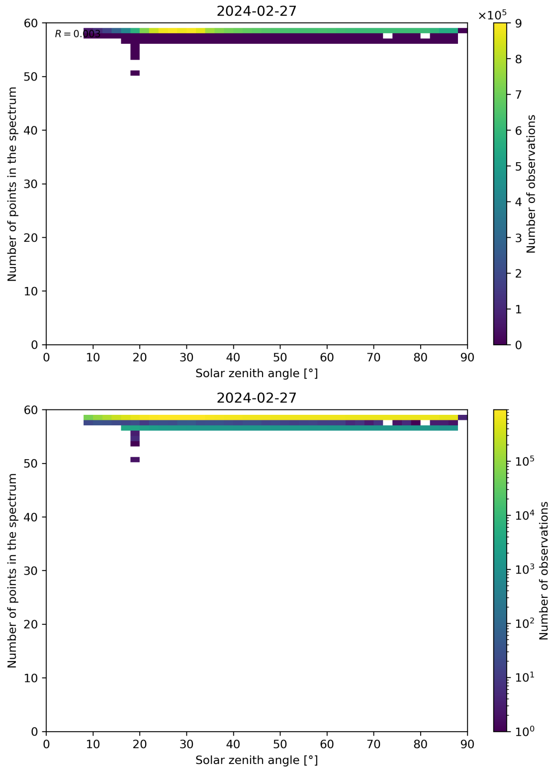
Figure 115: Scatter density plot of “Solar zenith angle” against “Number of points in the spectrum” for 2024-02-27 to 2024-02-28.
