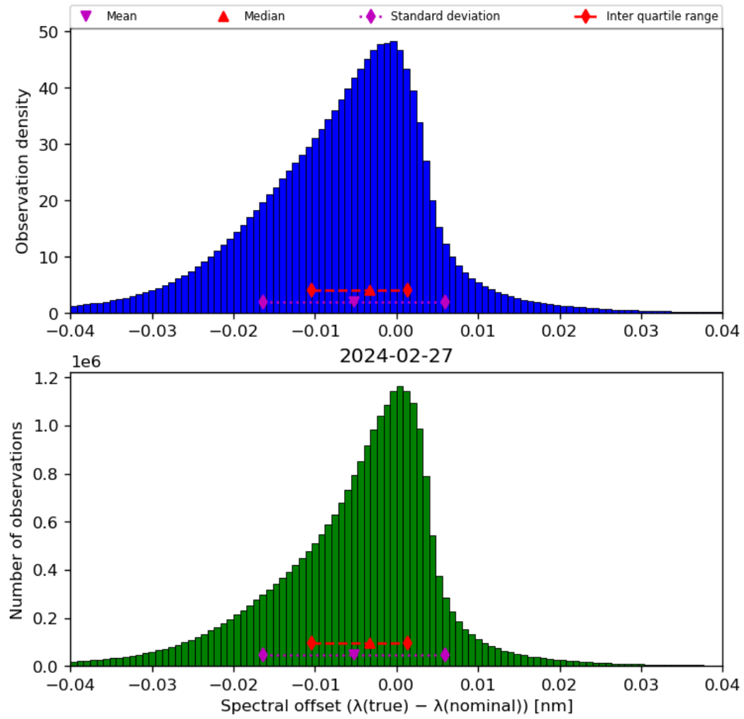
Figure 45: Histogram of “Spectral offset ( \lambda(\text{true}) - \lambda(\text{nominal}) )” for 2024-02-27 to 2024-02-28
