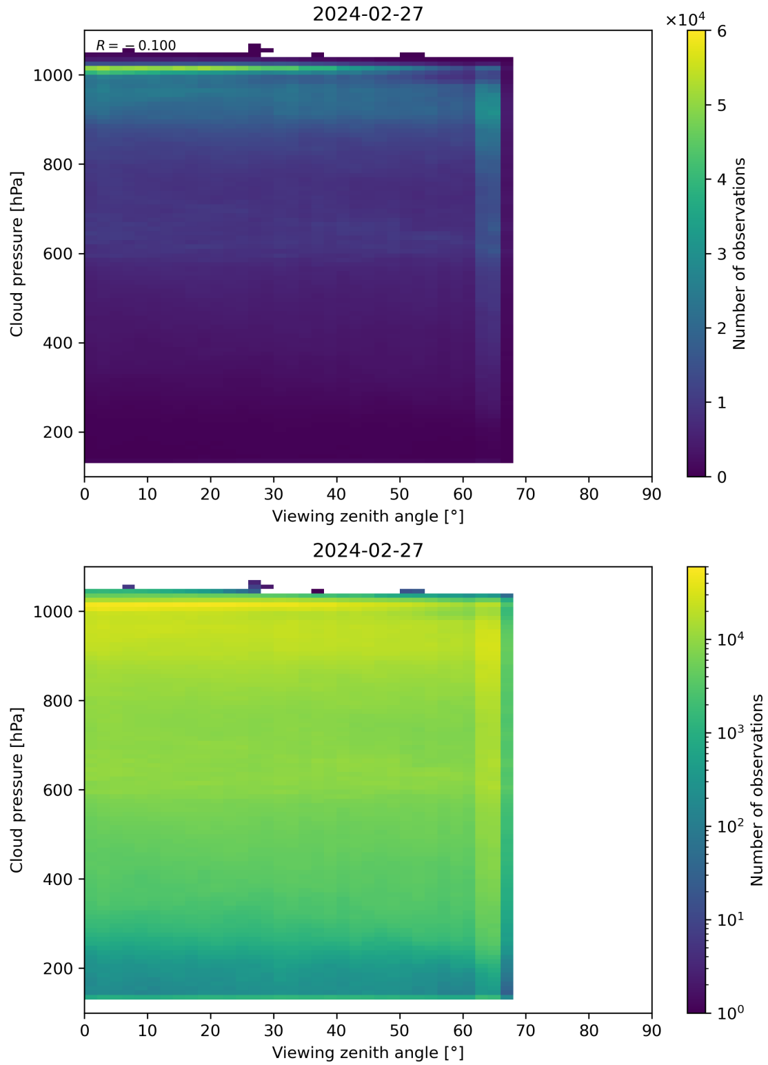
Figure 121: Scatter density plot of “Viewing zenith angle” against “Cloud pressure” for 2024-02-27 to 2024-02-28.
