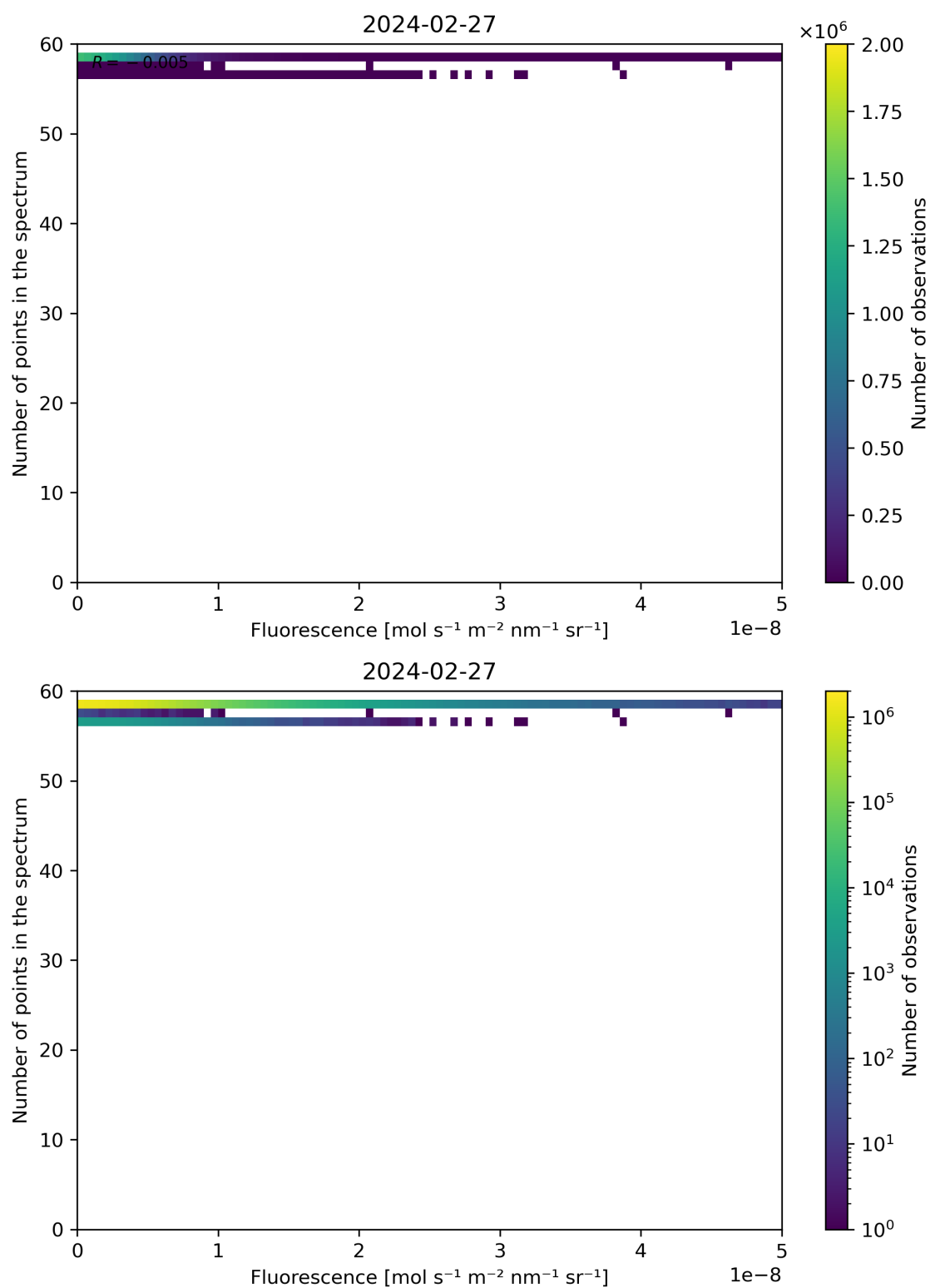
Figure 86: Scatter density plot of “Fluorescence” against “Number of points in the spectrum” for 2024-02-27 to 2024-02-28.
