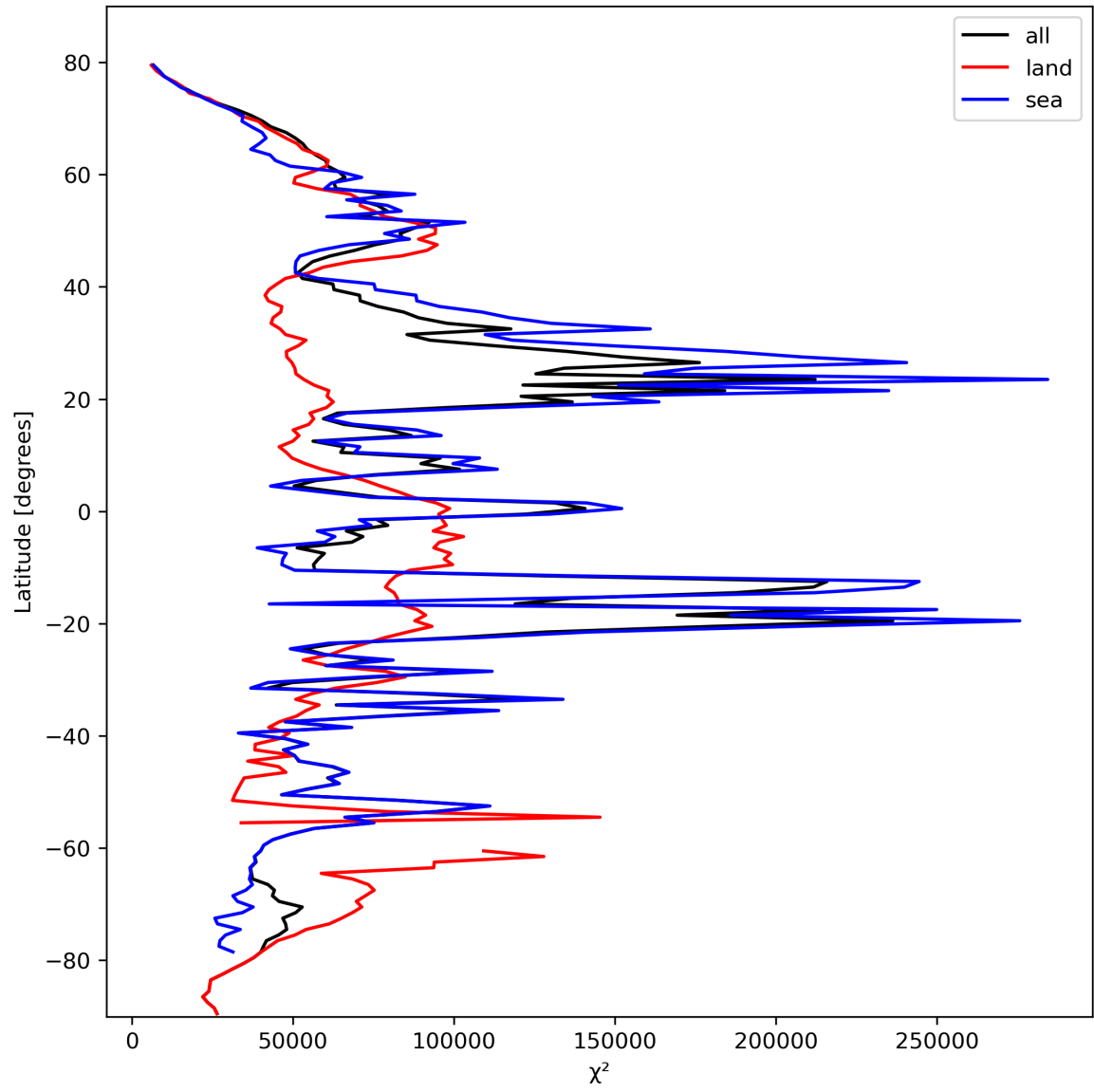
Figure 21: Zonal average of “ \chi^2 ” for 2024-02-27 to 2024-02-28.
