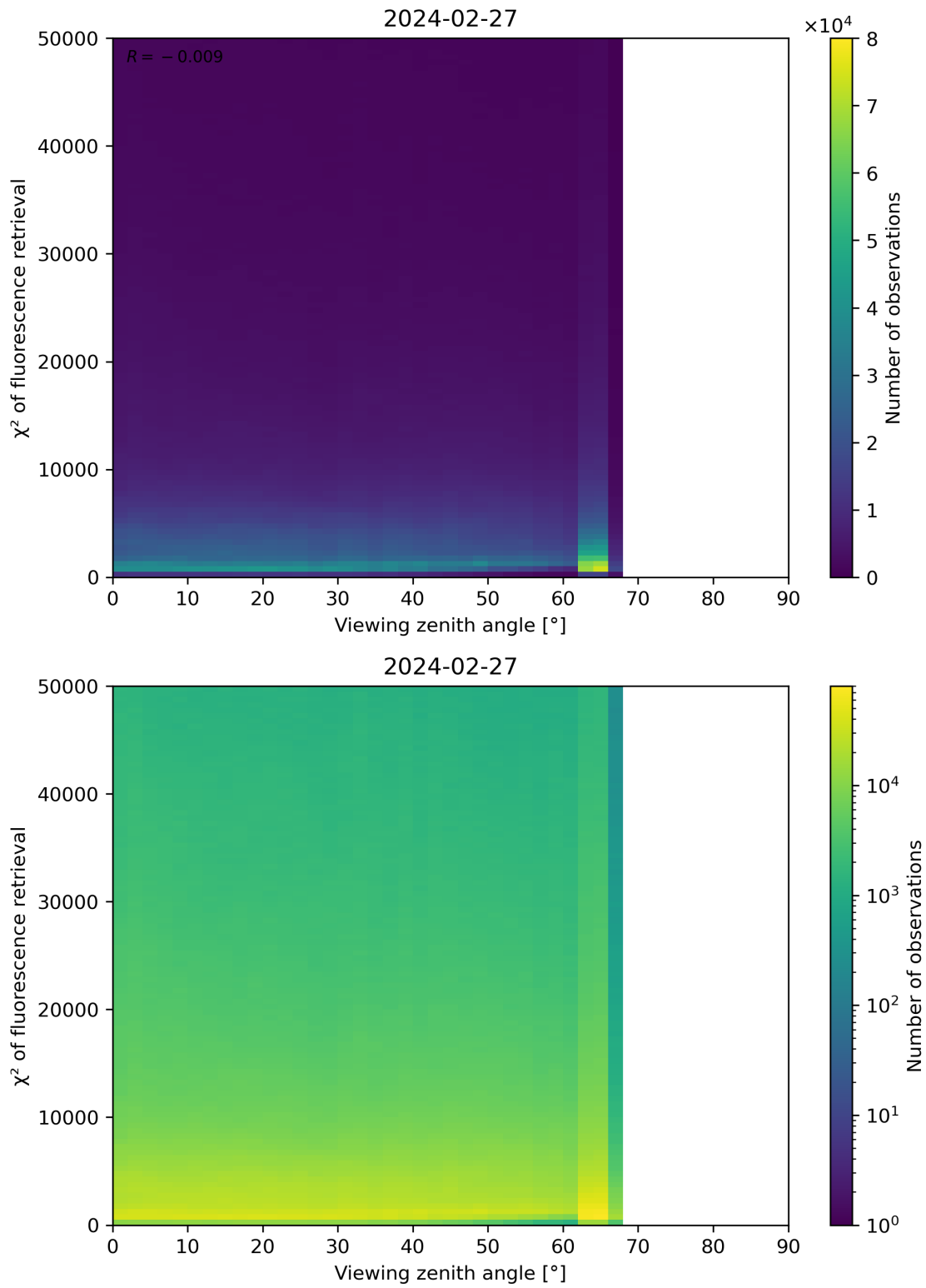
Figure 119: Scatter density plot of “Viewing zenith angle” against “ \chi^2 of fluorescence retrieval” for 2024-02-27 to 2024-02-28.
