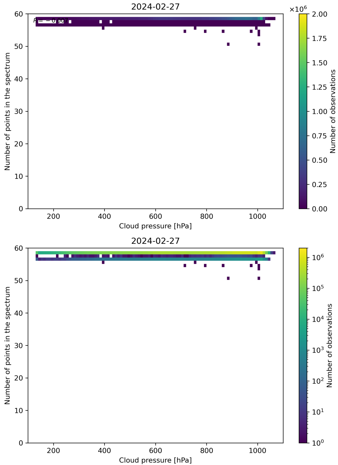
Figure 82: Scatter density plot of “Cloud pressure” against “Number of points in the spectrum” for 2024-02-27 to 2024-02-28.
