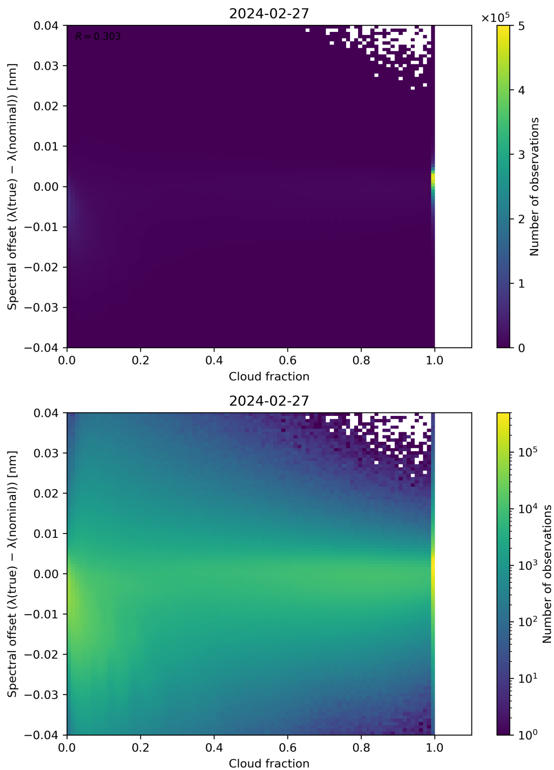
Figure 76: Scatter density plot of “Cloud fraction” against “Spectral offset ( \lambda(\text{true}) - \lambda(\text{nominal}) )” for 2024-02-27 to 2024-02-28.
