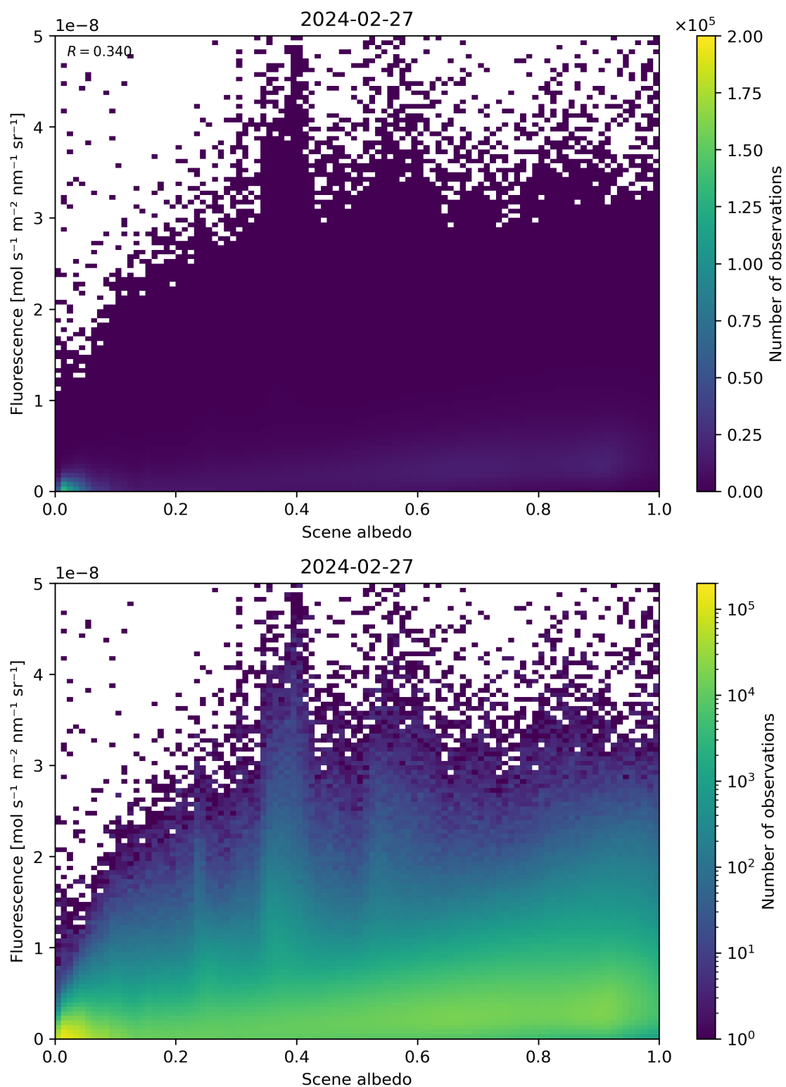
Figure 104: Scatter density plot of “Scene albedo” against “Fluorescence” for 2024-02-27 to 2024-02-28.
