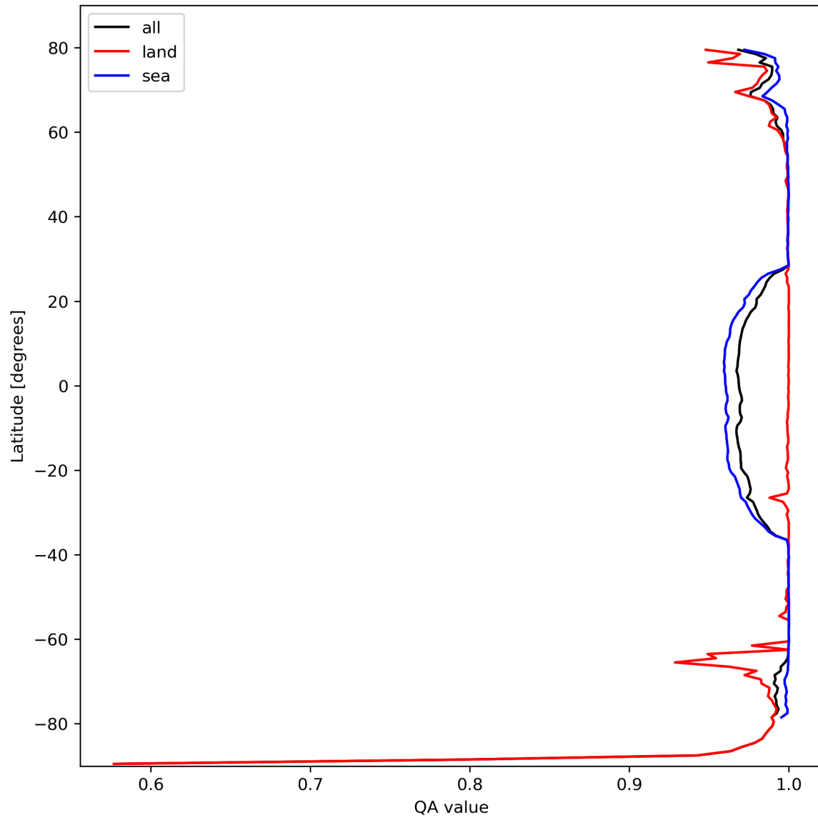
Figure 12: Zonal average of “QA value” for 2024-02-27 to 2024-02-28.
