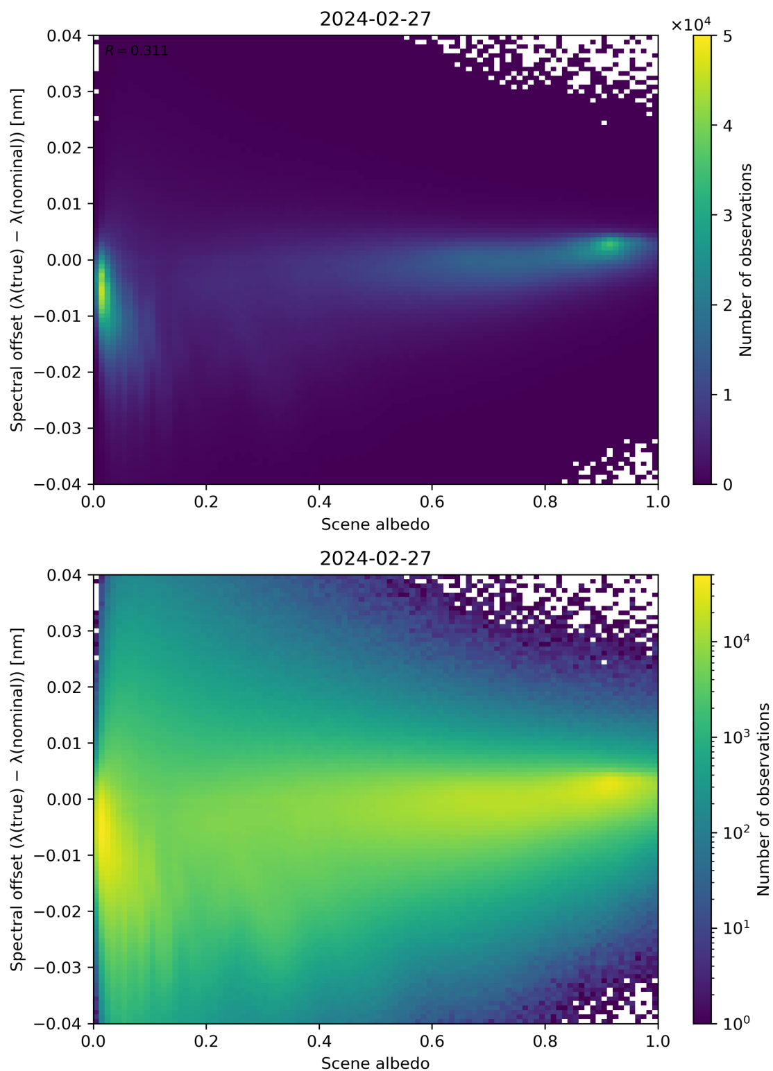
Figure 107: Scatter density plot of “Scene albedo” against “Spectral offset ( \lambda(\text{true}) - \lambda(\text{nominal}) )” for 2024-02-27 to 2024-02-28.
