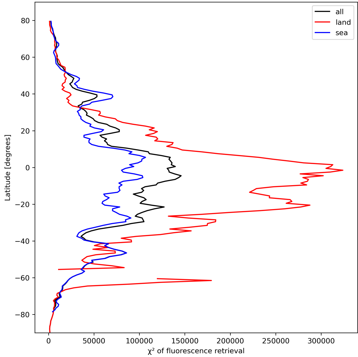
Figure 25: Zonal average of “ \chi^2 of fluorescence retrieval” for 2024-02-27 to 2024-02-28.
