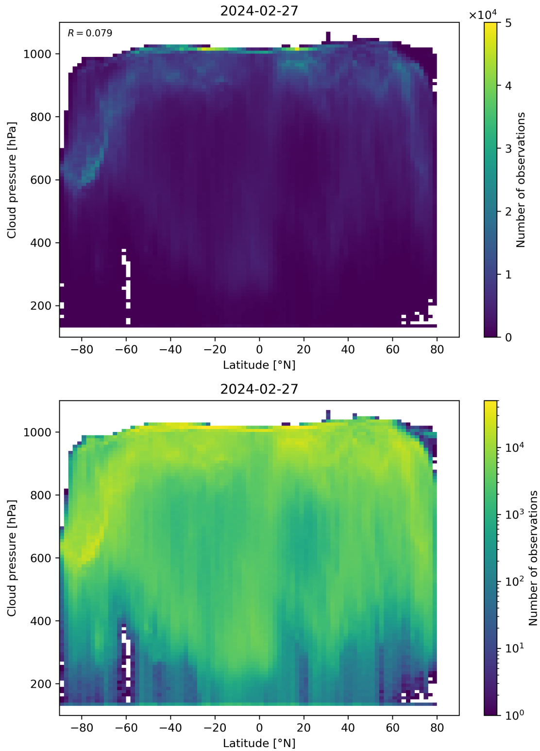
Figure 91: Scatter density plot of “Latitude” against “Cloud pressure” for 2024-02-27 to 2024-02-28.
