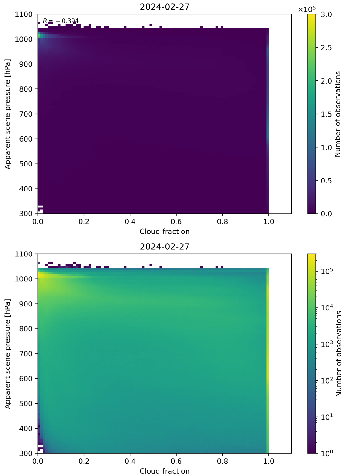
Figure 70: Scatter density plot of “Cloud fraction” against “Apparent scene pressure” for 2024-02-27 to 2024-02-28.
