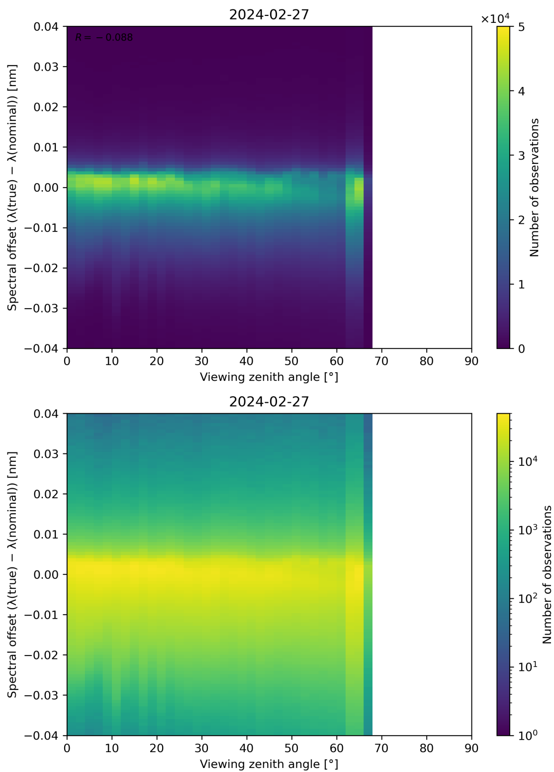
Figure 128: Scatter density plot of “Viewing zenith angle” against “Spectral offset ( \lambda(\text{true}) - \lambda(\text{nominal}) )” for 2024-02-27 to 2024-02-28.
