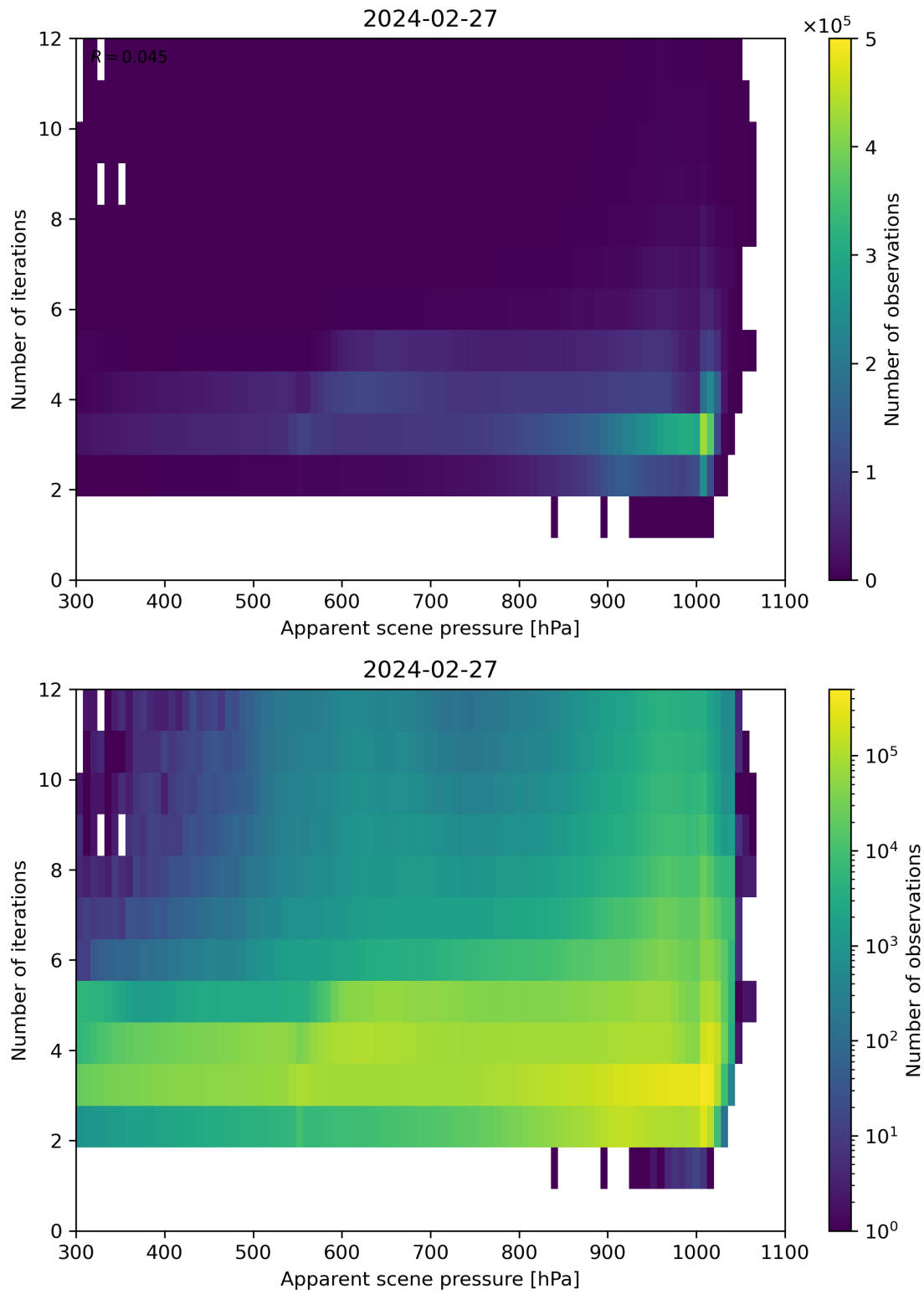
Figure 65: Scatter density plot of “Apparent scene pressure” against “Number of iterations” for 2024-02-27 to 2024-02-28.
