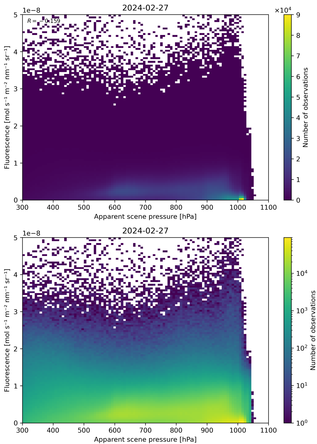
Figure 64: Scatter density plot of “Apparent scene pressure” against “Fluorescence” for 2024-02-27 to 2024-02-28.
