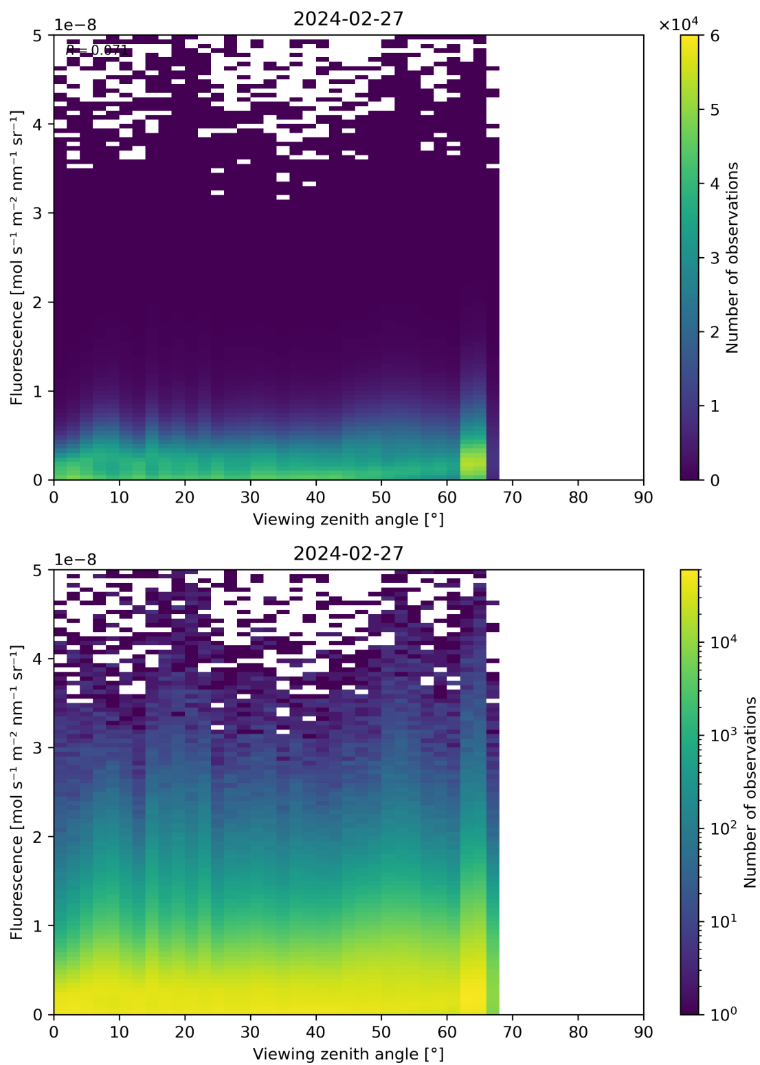
Figure 122: Scatter density plot of “Viewing zenith angle” against “Fluorescence” for 2024-02-27 to 2024-02-28.
