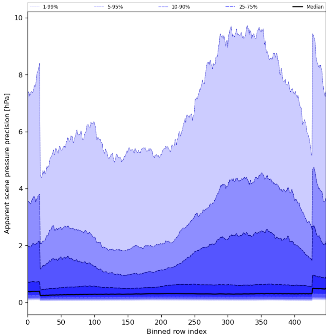
Figure 54: Along track statistics of “Apparent scene pressure precision” for 2024-02-27 to 2024-02-28
