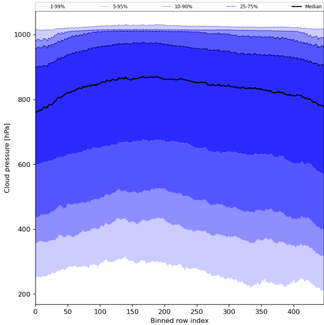
Figure 47: Along track statistics of “Cloud pressure” for 2024-02-27 to 2024-02-28
