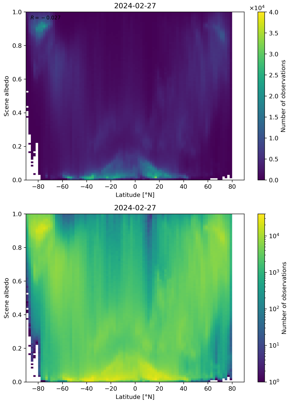
Figure 95: Scatter density plot of “Latitude” against “Scene albedo” for 2024-02-27 to 2024-02-28.
