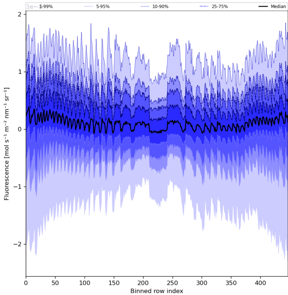
Figure 57: Along track statistics of “Fluorescence” for 2024-02-27 to 2024-02-28
