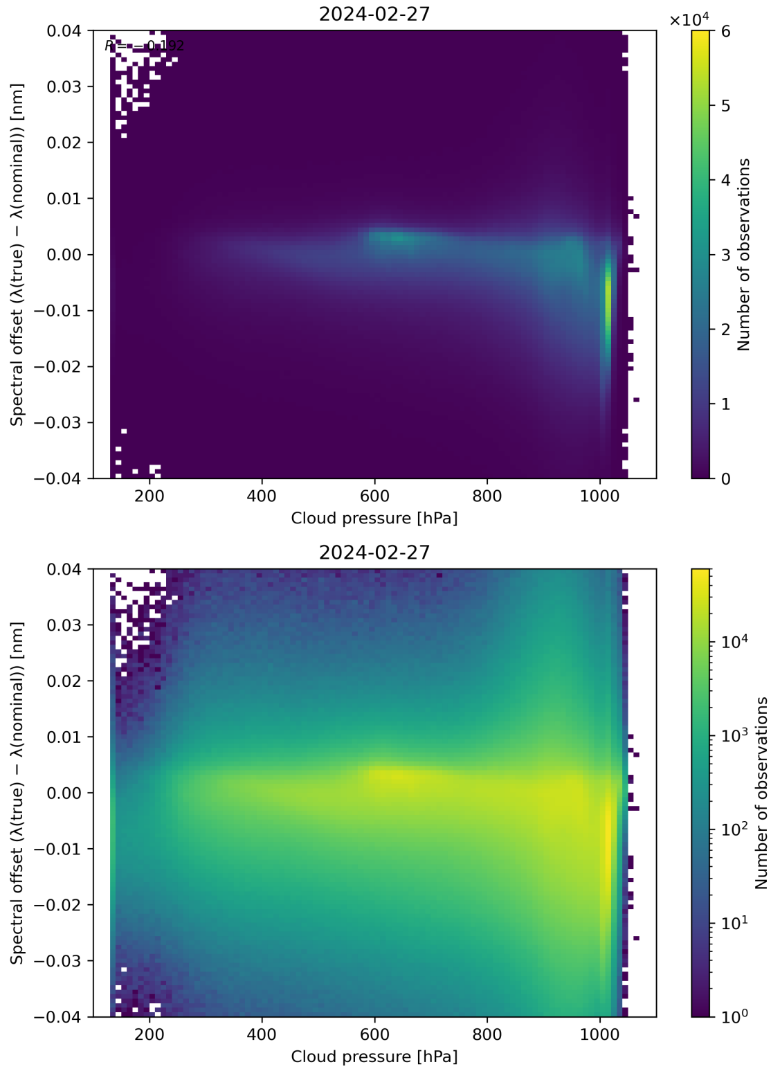
Figure 84: Scatter density plot of “Cloud pressure” against “Spectral offset ( \lambda(\text{true}) - \lambda(\text{nominal}) )” for 2024-02-27 to 2024-02-28.
