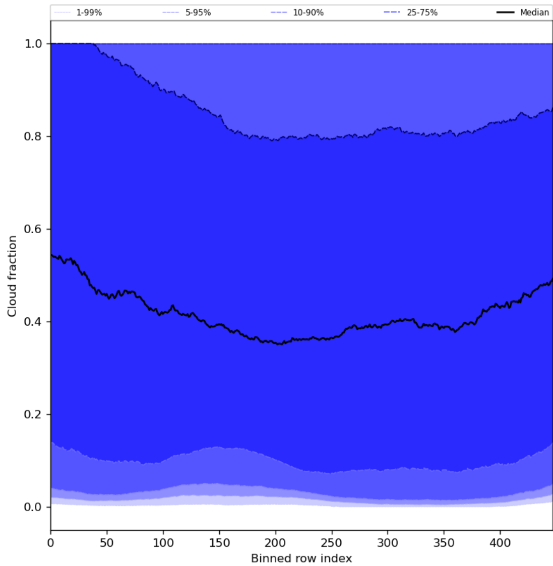
Figure 49: Along track statistics of “Cloud fraction” for 2024-02-27 to 2024-02-28
