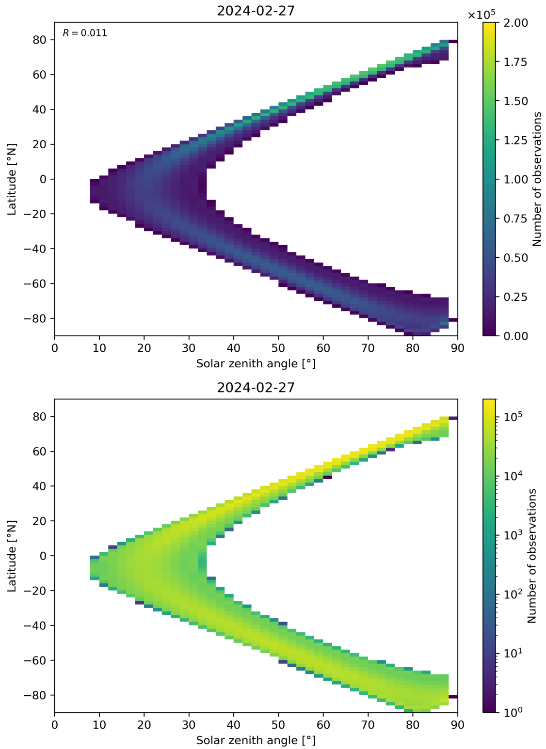
Figure 113: Scatter density plot of “Solar zenith angle” against “Latitude” for 2024-02-27 to 2024-02-28.
