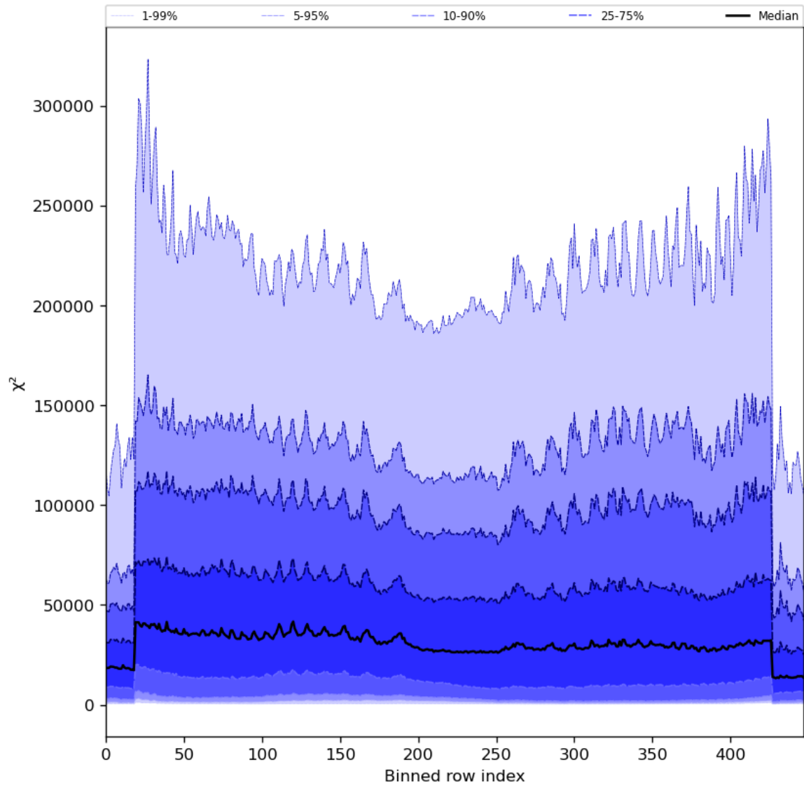
Figure 55: Along track statistics of “ \chi^2 ” for 2024-02-27 to 2024-02-28
