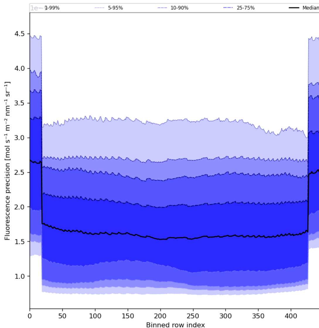
Figure 58: Along track statistics of “Fluorescence precision” for 2024-02-27 to 2024-02-28
