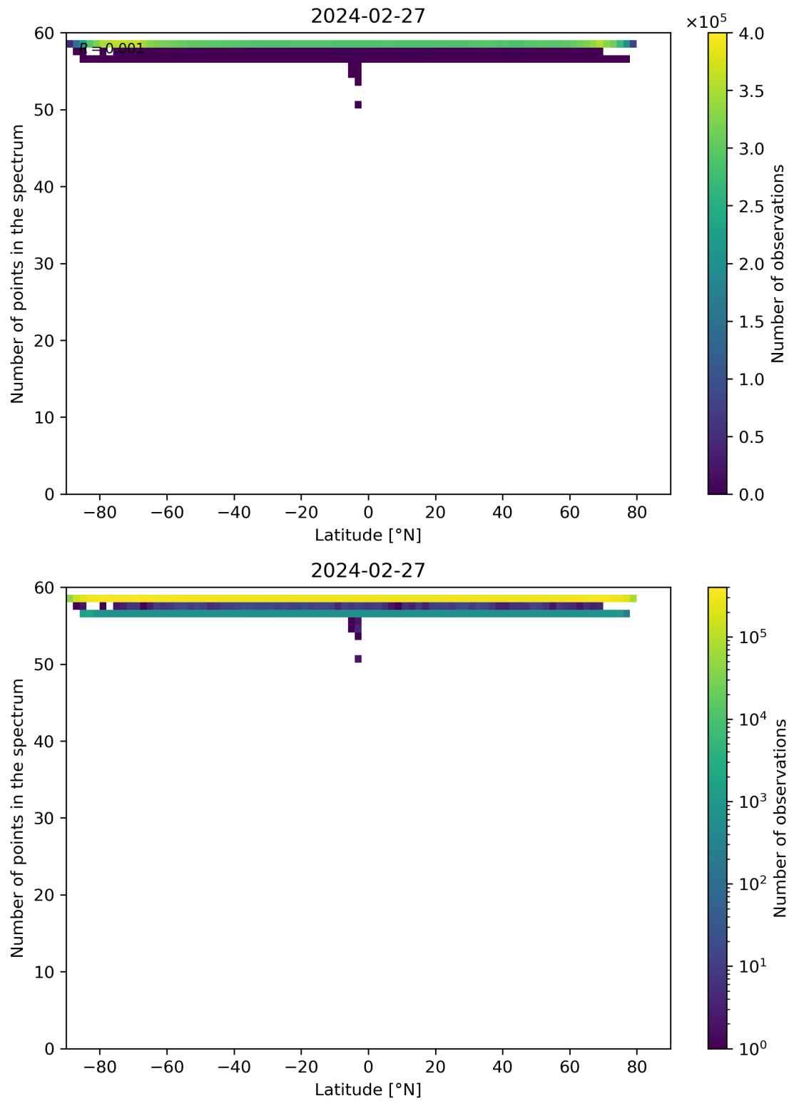
Figure 94: Scatter density plot of “Latitude” against “Number of points in the spectrum” for 2024-02-27 to 2024-02-28.
