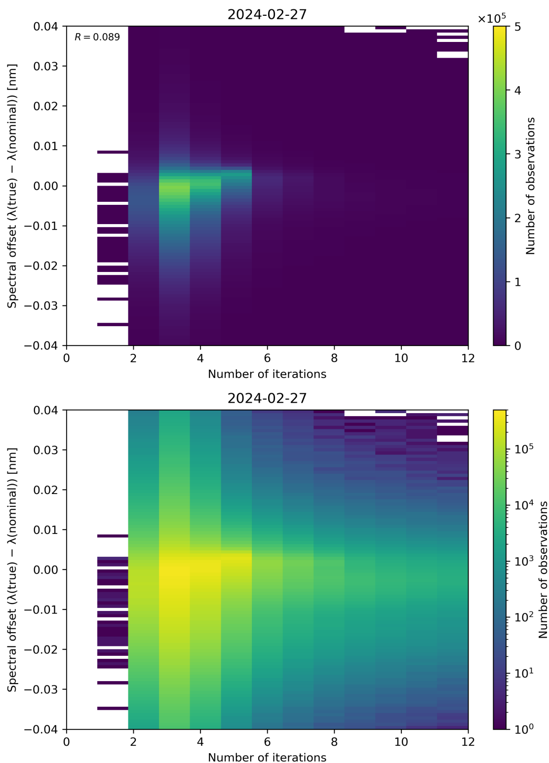
Figure 100: Scatter density plot of “Number of iterations” against “Spectral offset ( \lambda(\text{true}) - \lambda(\text{nominal}) )” for 2024-02-27 to 2024-02-28.
