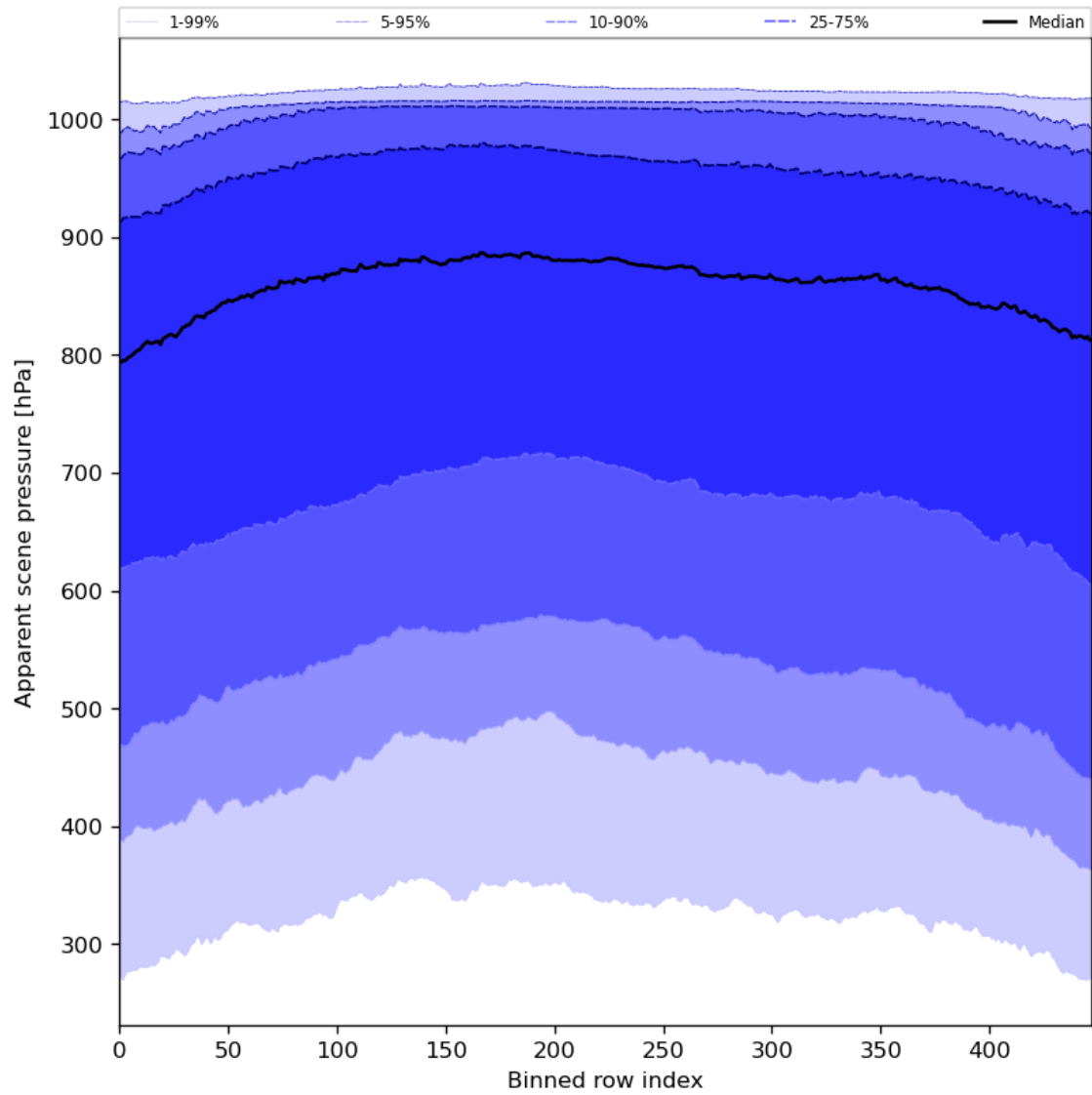
Figure 53: Along track statistics of “Apparent scene pressure” for 2024-02-27 to 2024-02-28
