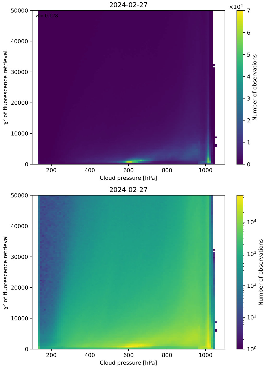
Figure 78: Scatter density plot of “Cloud pressure” against “ \chi^2 of fluorescence retrieval” for 2024-02-27 to 2024-02-28.
