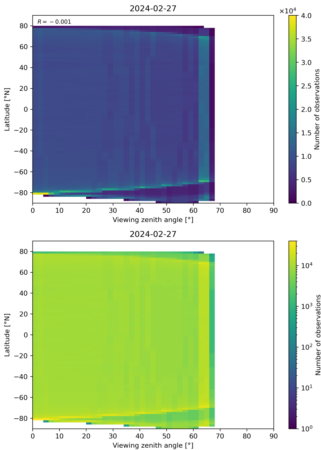
Figure 123: Scatter density plot of “Viewing zenith angle” against “Latitude” for 2024-02-27 to 2024-02-28.
