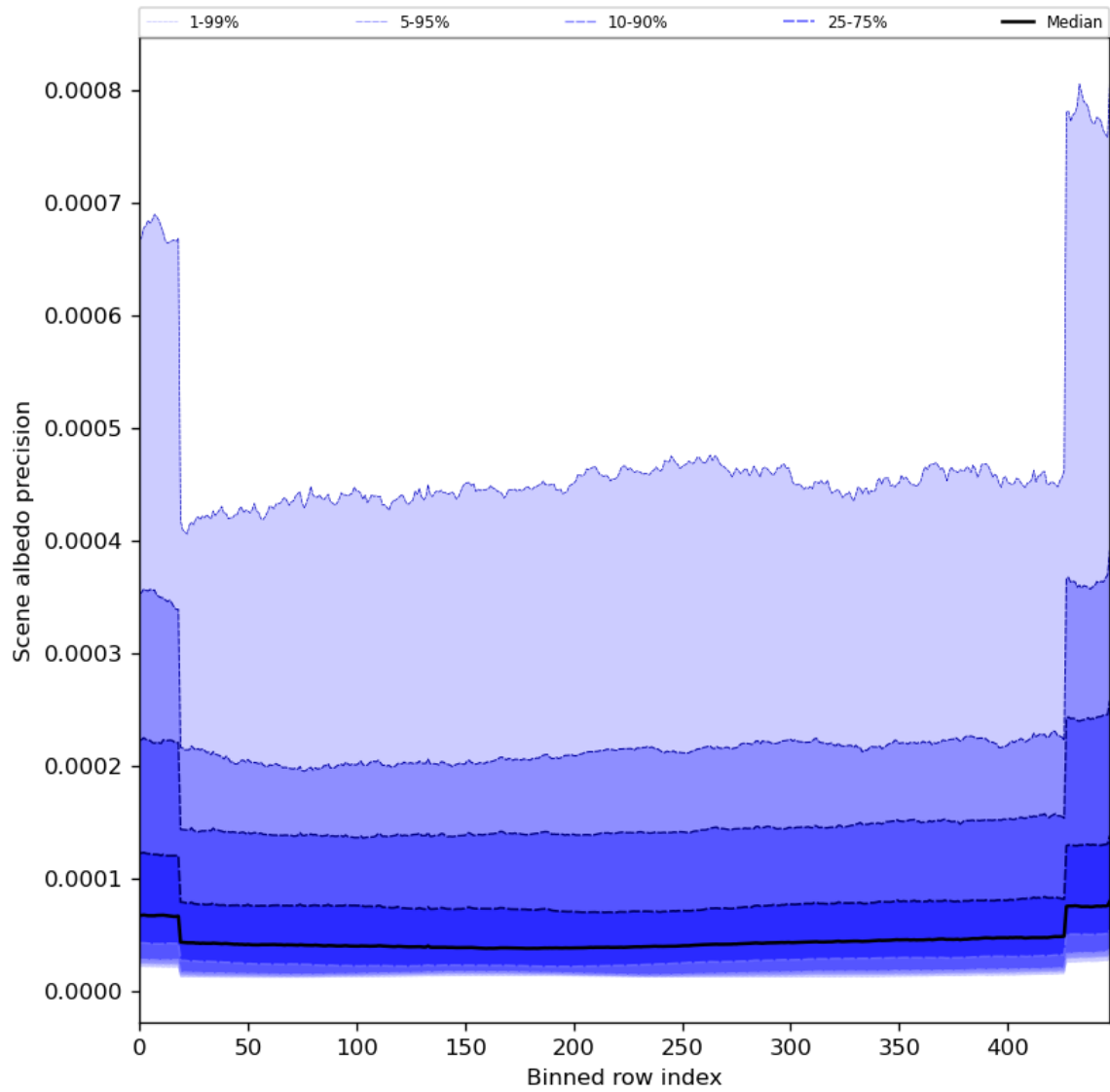
Figure 52: Along track statistics of “Scene albedo precision” for 2024-02-27 to 2024-02-28
