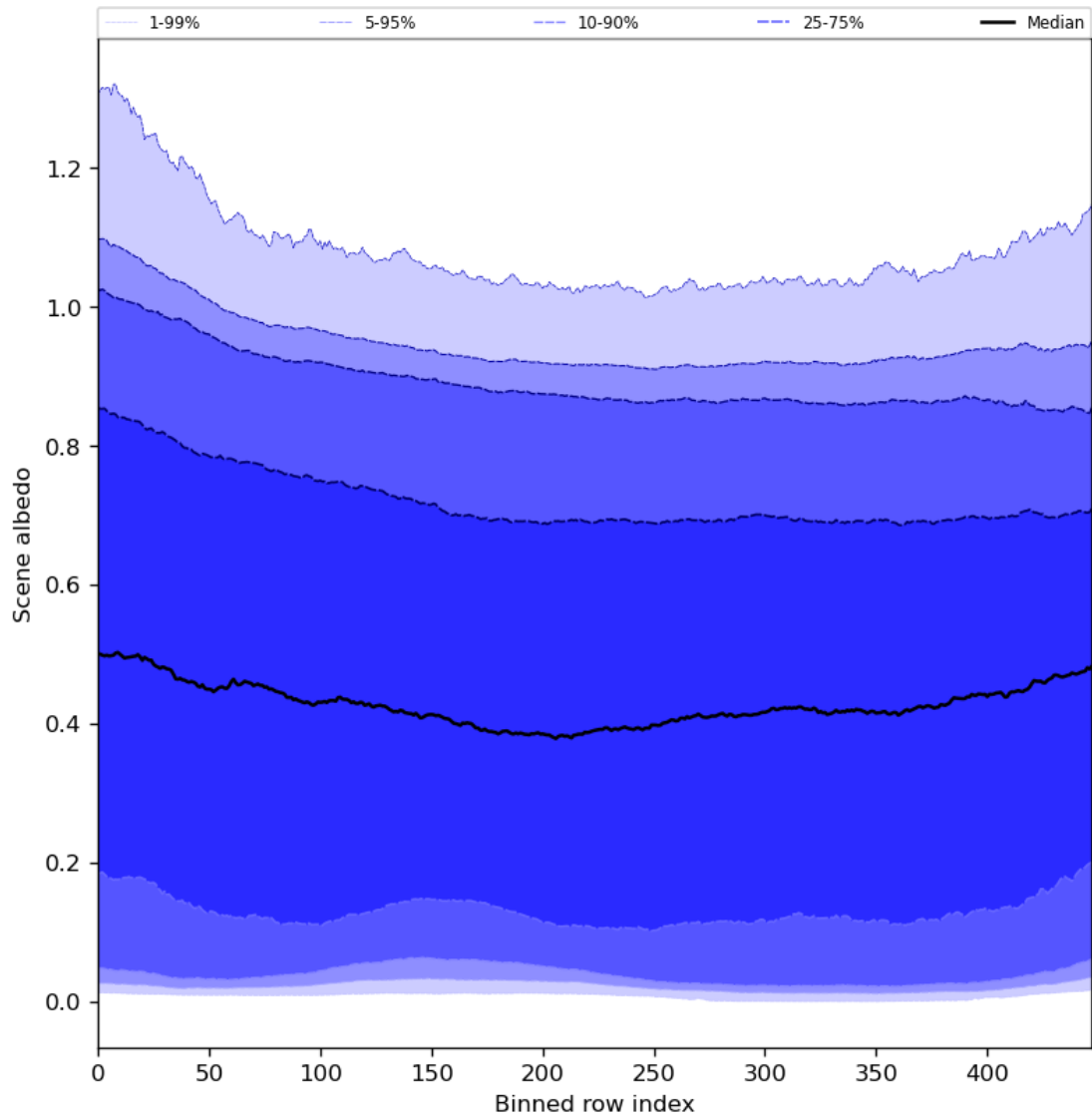
Figure 51: Along track statistics of “Scene albedo” for 2024-02-27 to 2024-02-28
