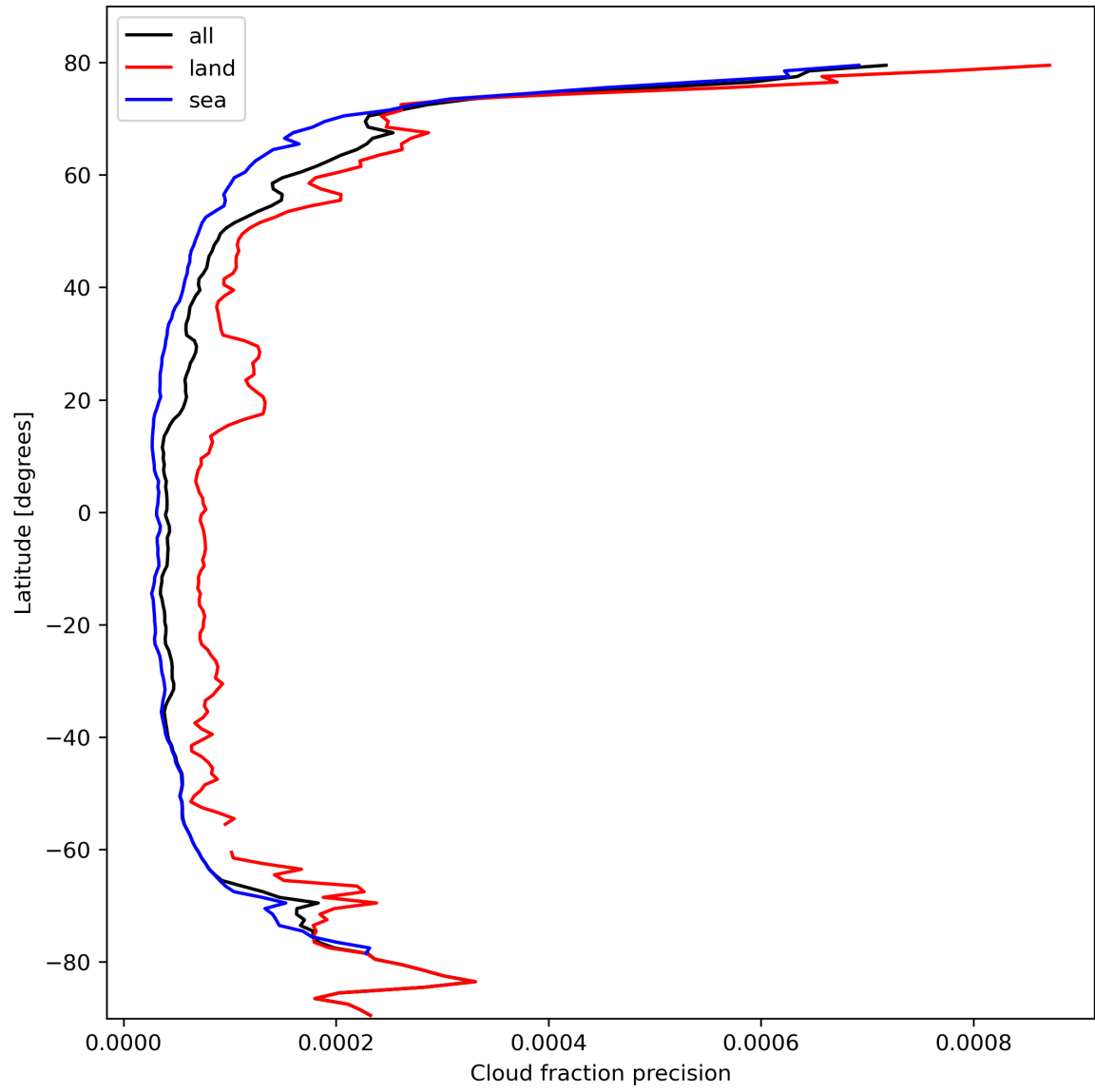
Figure 16: Zonal average of “Cloud fraction precision” for 2024-02-27 to 2024-02-28.
