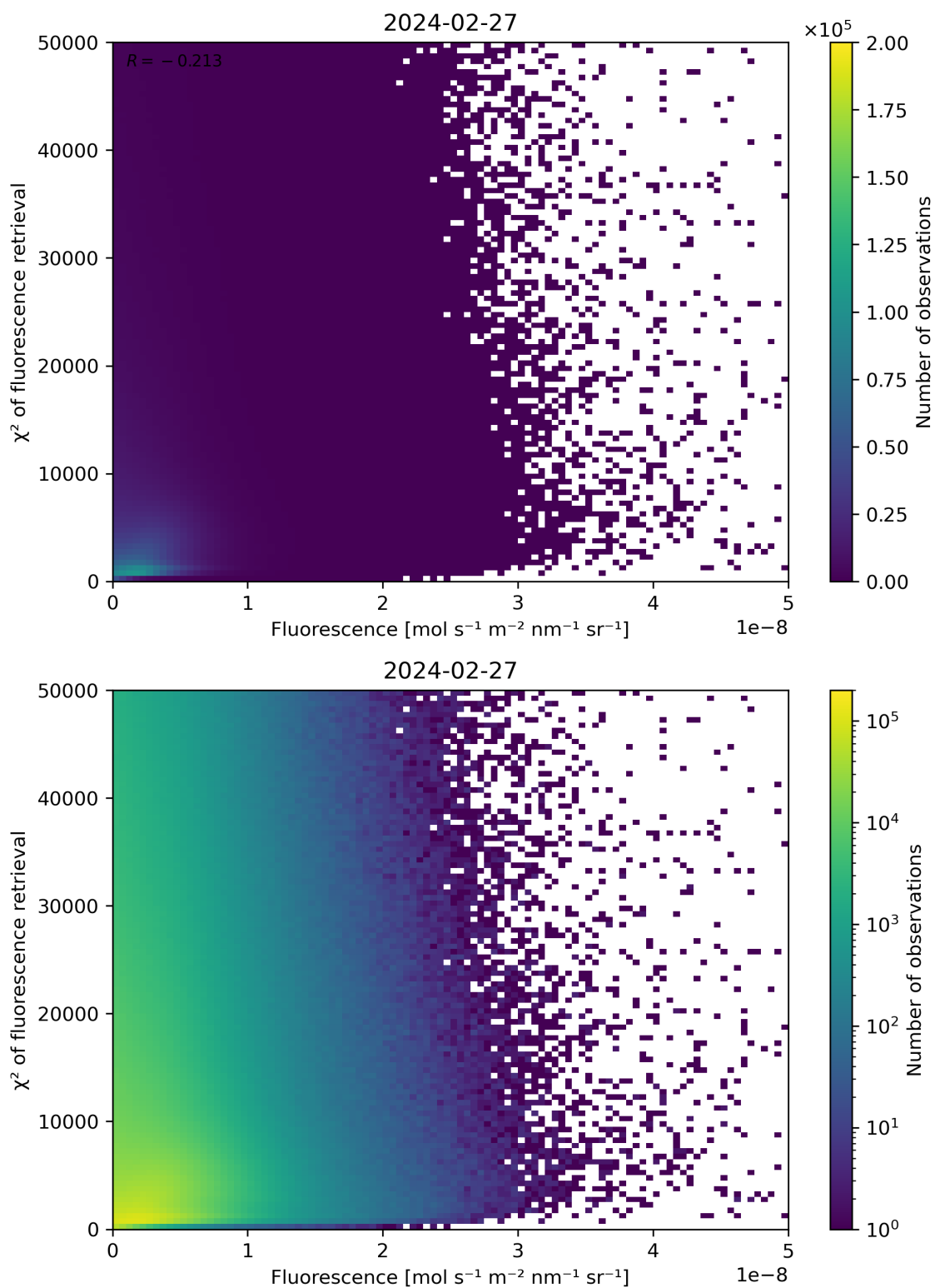
Figure 85: Scatter density plot of “Fluorescence” against “ \chi^2 of fluorescence retrieval” for 2024-02-27 to 2024-02-28.
