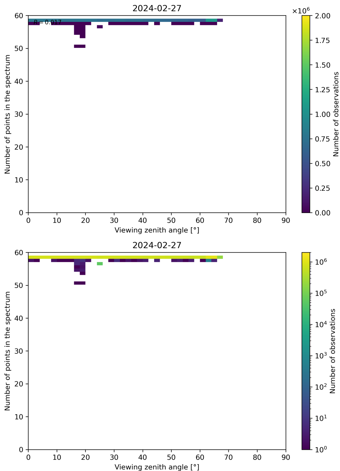
Figure 125: Scatter density plot of “Viewing zenith angle” against “Number of points in the spectrum” for 2024-02-27 to 2024-02-28.
