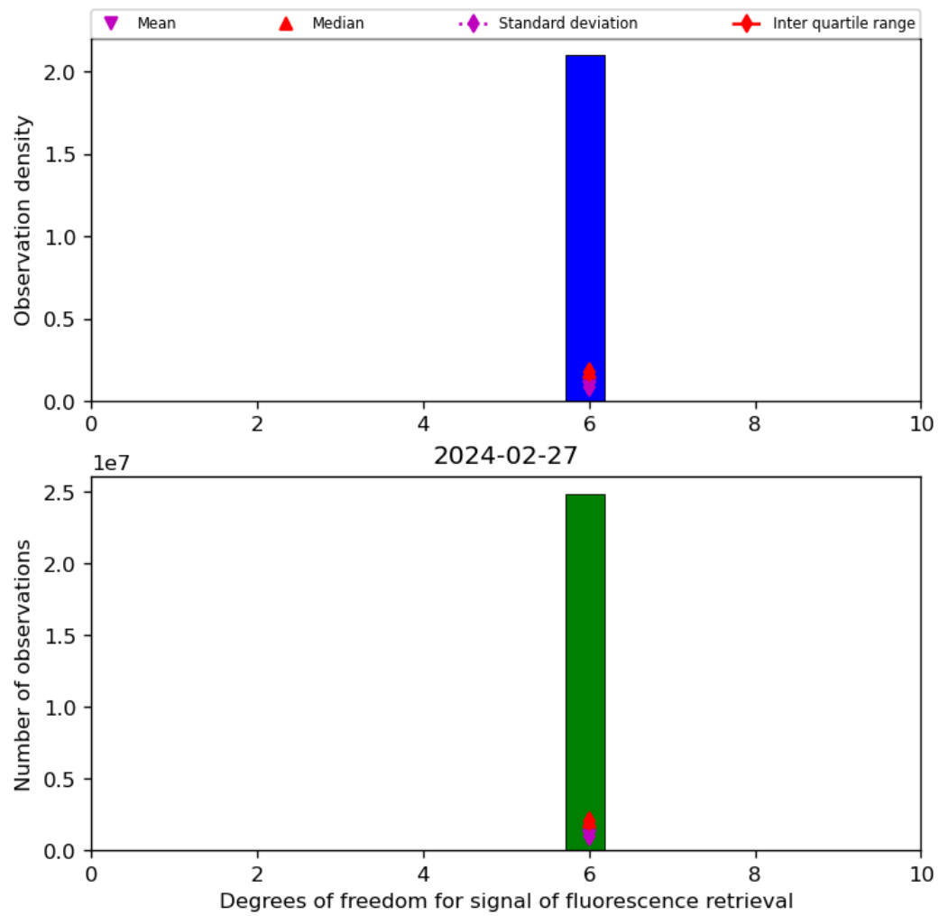
Figure 43: Histogram of “Degrees of freedom for signal of fluorescence retrieval” for 2024-02-27 to 2024-02-28
