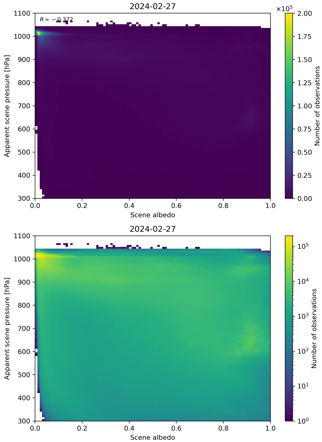
Figure 102: Scatter density plot of “Scene albedo” against “Apparent scene pressure” for 2024-02-27 to 2024-02-28.
