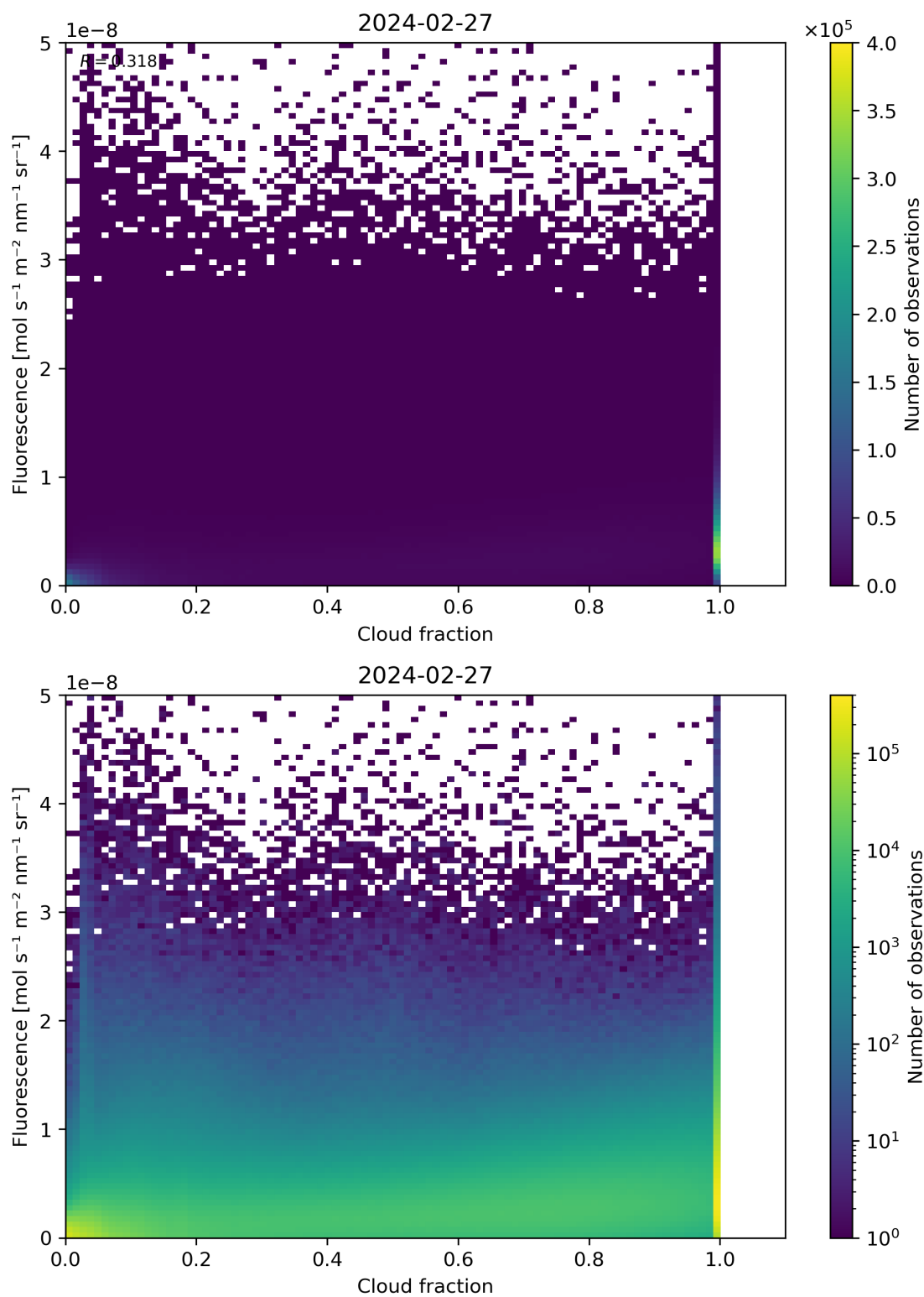
Figure 72: Scatter density plot of “Cloud fraction” against “Fluorescence” for 2024-02-27 to 2024-02-28.
