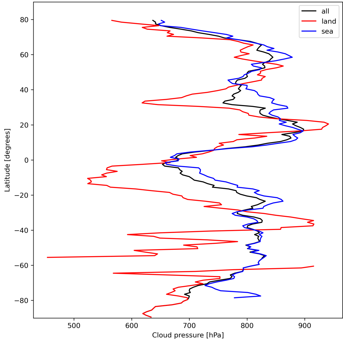
Figure 13: Zonal average of “Cloud pressure” for 2024-02-27 to 2024-02-28.
