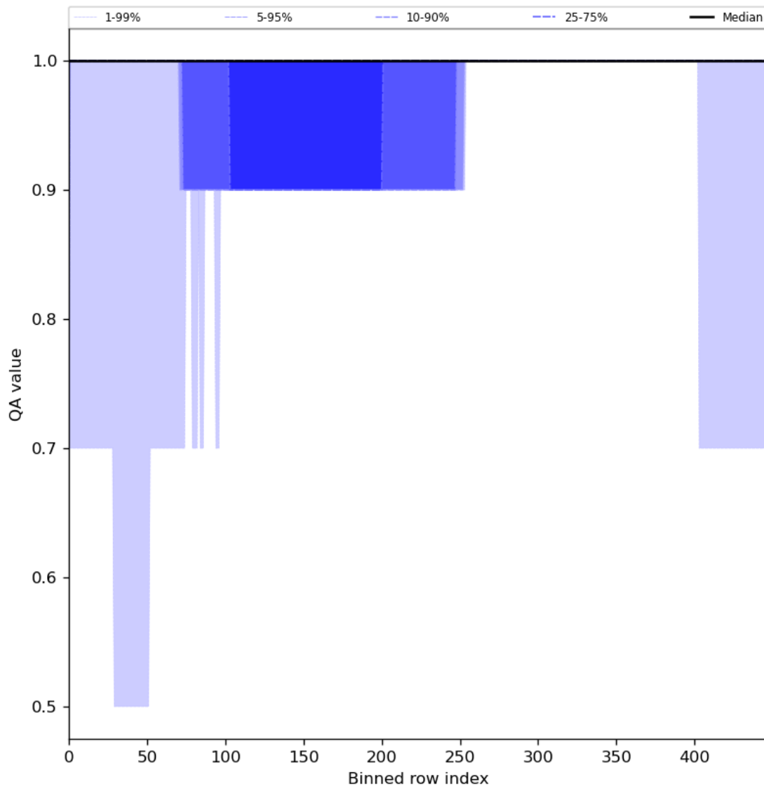
Figure 46: Along track statistics of "QA value" for 2024-02-27 to 2024-02-28
