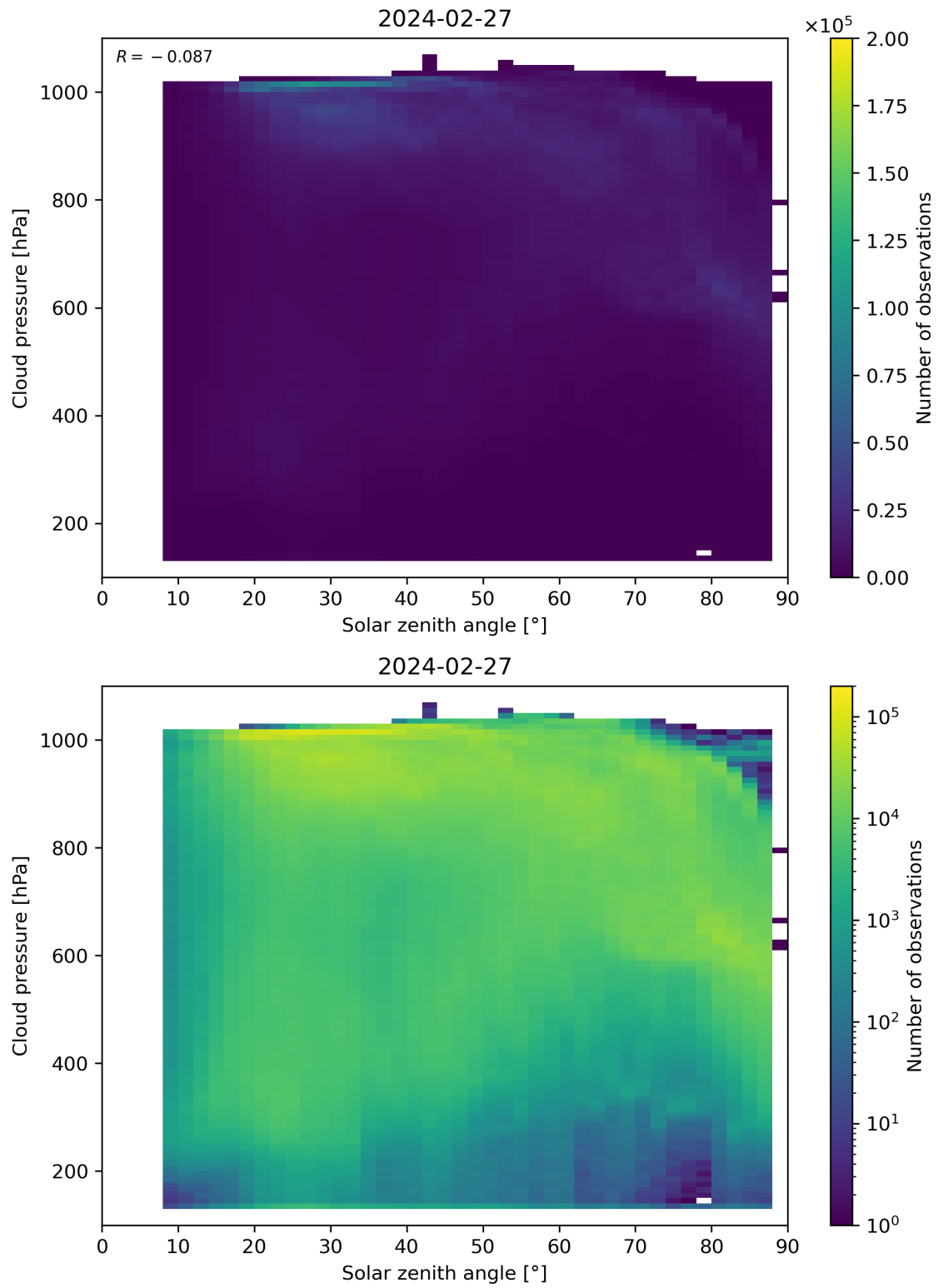
Figure 111: Scatter density plot of “Solar zenith angle” against “Cloud pressure” for 2024-02-27 to 2024-02-28.
