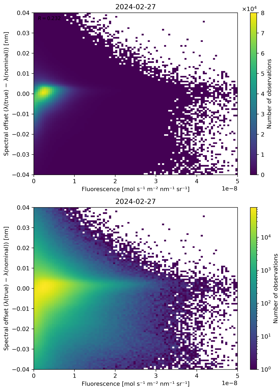
Figure 87: Scatter density plot of “Fluorescence” against “Spectral offset ( \lambda(\text{true}) - \lambda(\text{nominal}) )” for 2024-02-27 to 2024-02-28.
