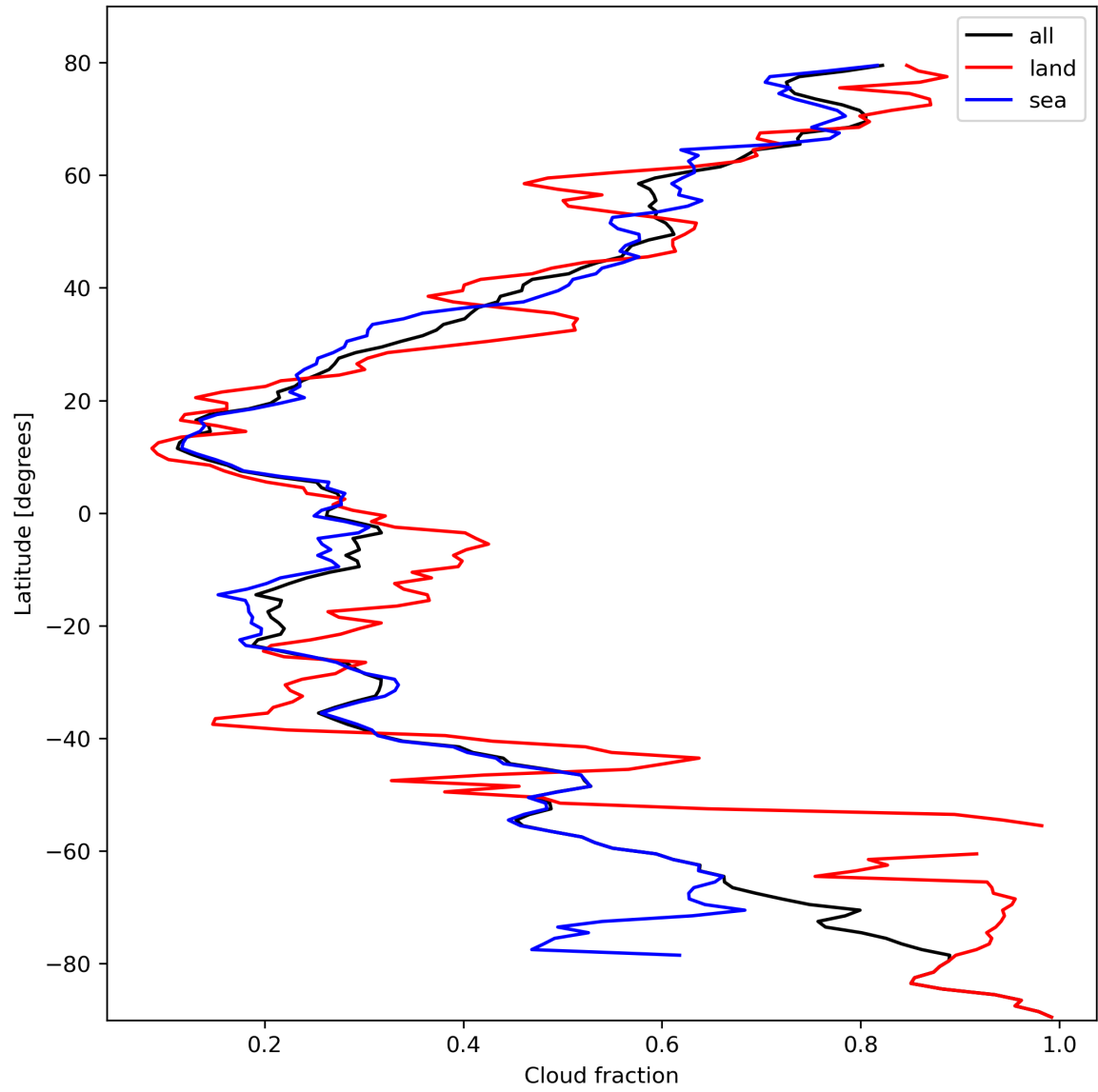
Figure 15: Zonal average of “Cloud fraction” for 2024-02-27 to 2024-02-28.
