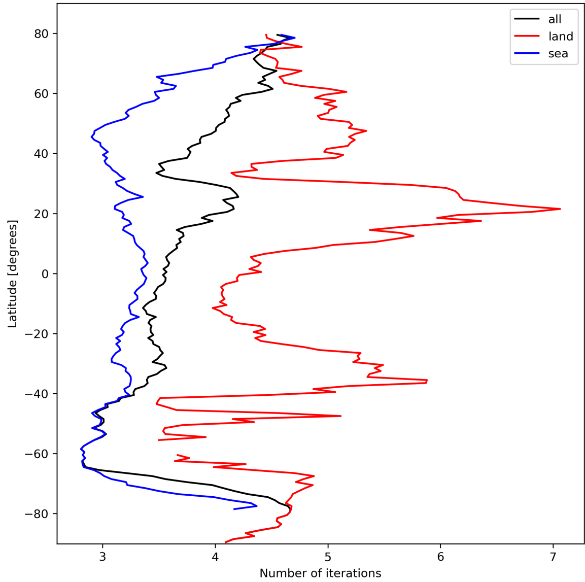
Figure 22: Zonal average of “Number of iterations” for 2024-02-27 to 2024-02-28.
