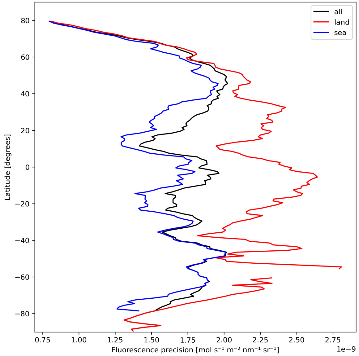
Figure 24: Zonal average of “Fluorescence precision” for 2024-02-27 to 2024-02-28.
