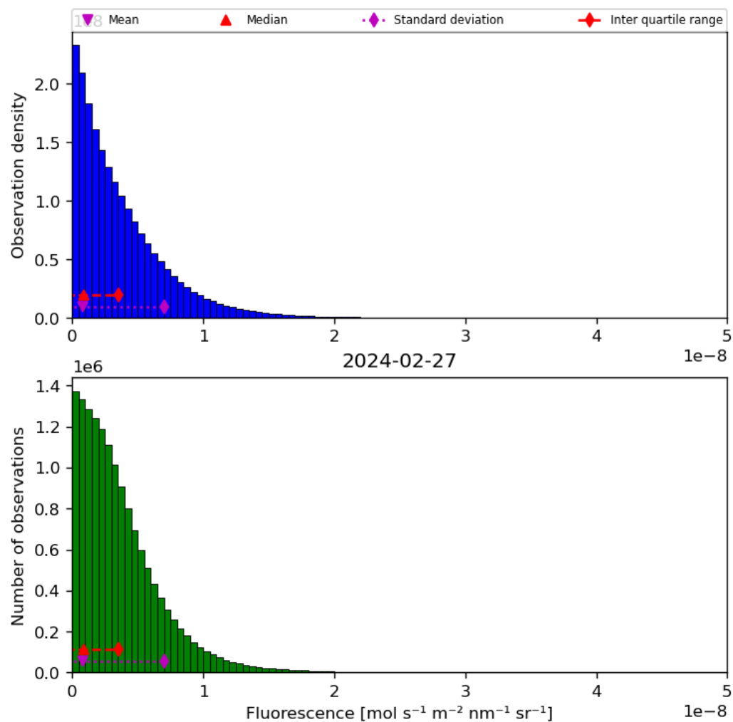
Figure 40: Histogram of “Fluorescence” for 2024-02-27 to 2024-02-28
