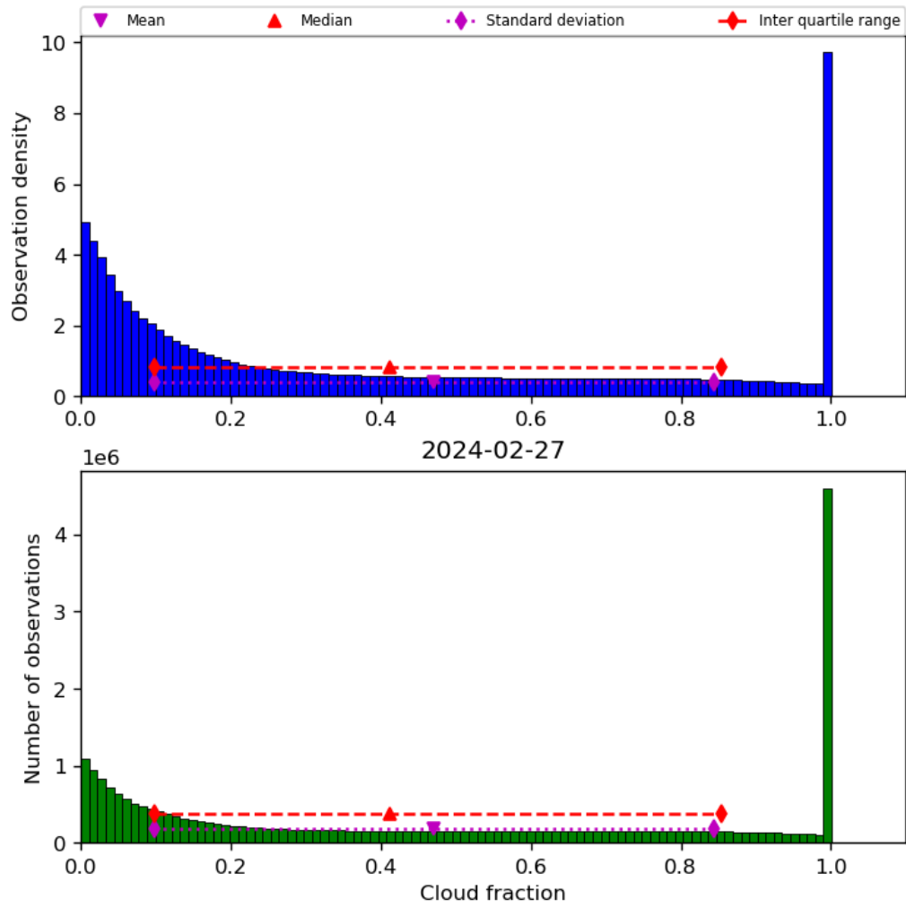
Figure 32: Histogram of “Cloud fraction” for 2024-02-27 to 2024-02-28
