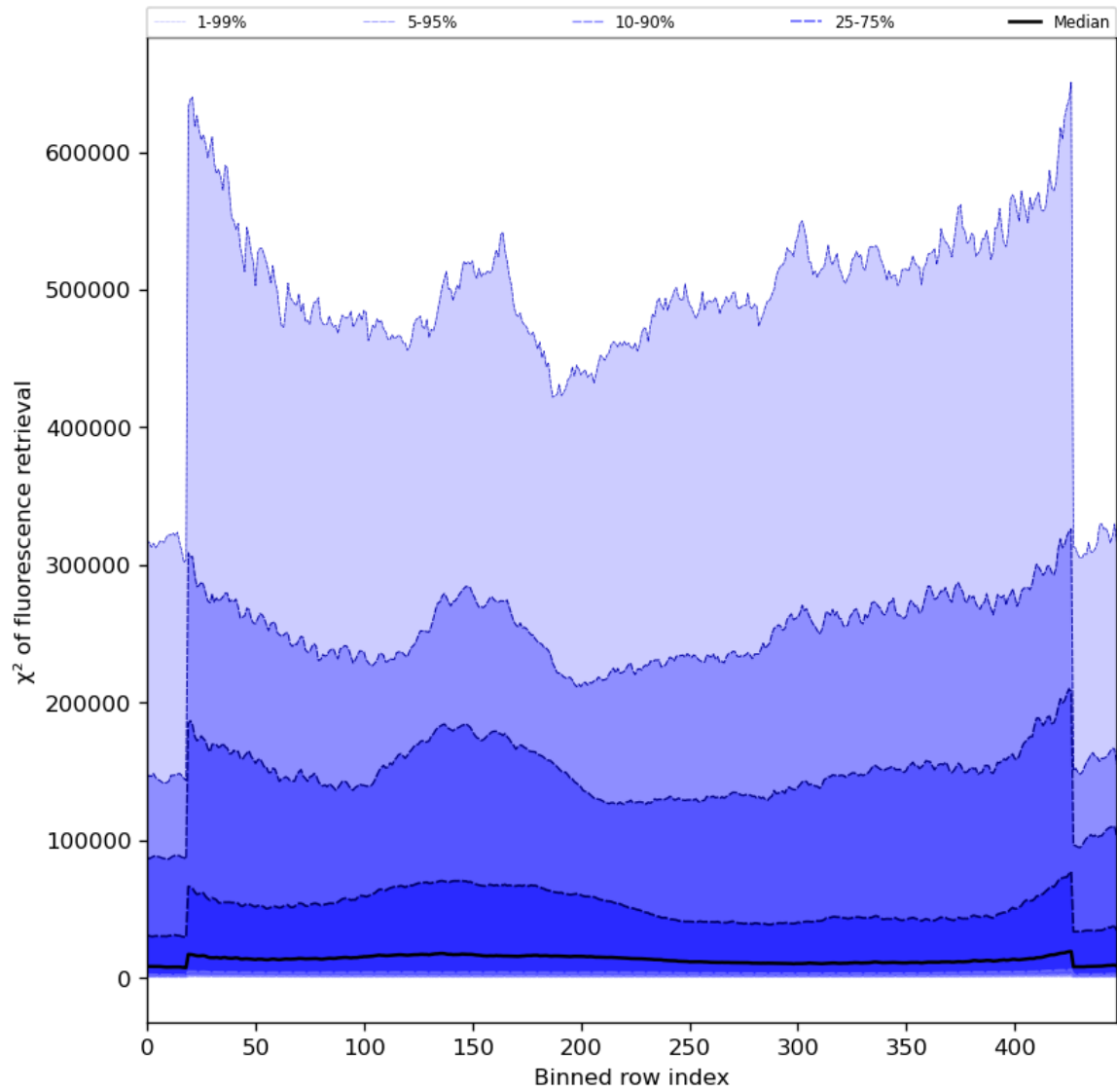
Figure 59: Along track statistics of " \chi^2 of fluorescence retrieval" for 2024-02-27 to 2024-02-28
