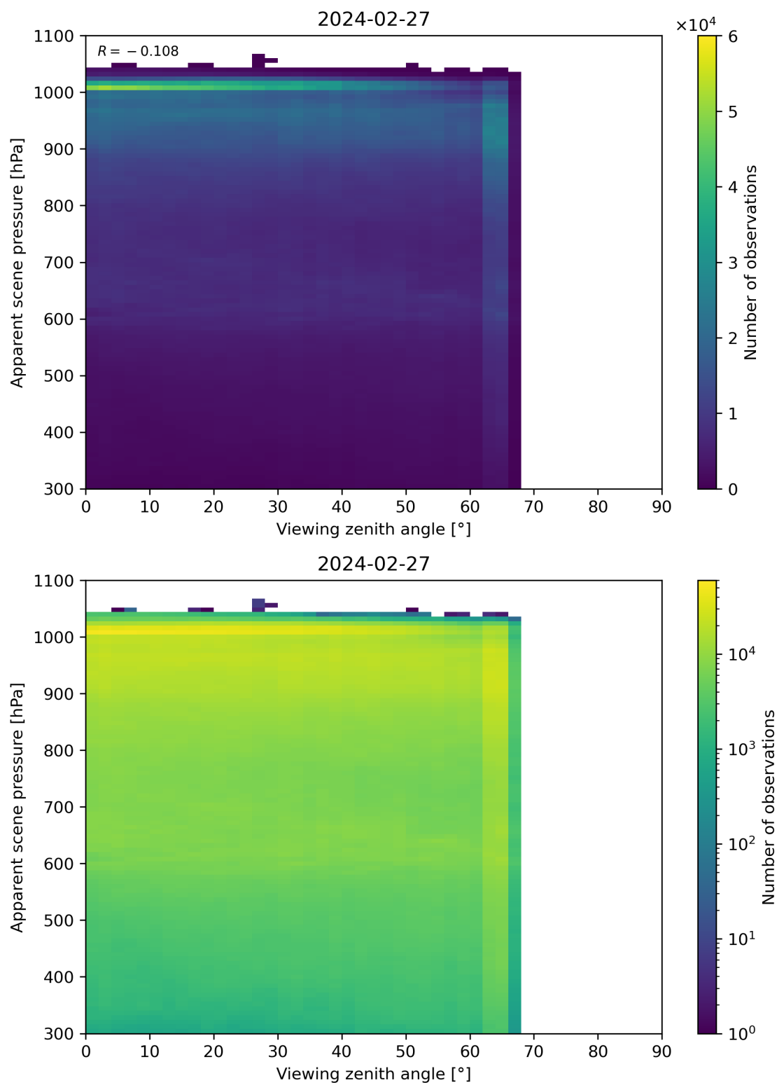
Figure 118: Scatter density plot of “Viewing zenith angle” against “Apparent scene pressure” for 2024-02-27 to 2024-02-28.
