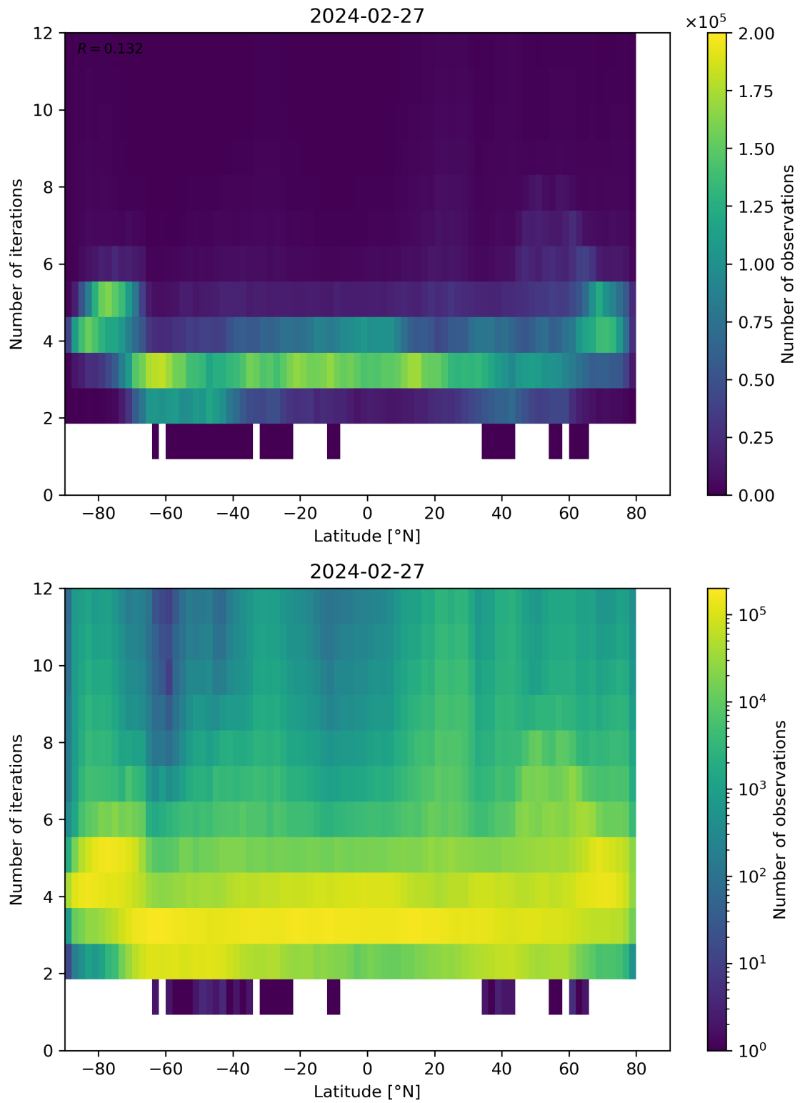
Figure 93: Scatter density plot of “Latitude” against “Number of iterations” for 2024-02-27 to 2024-02-28.
