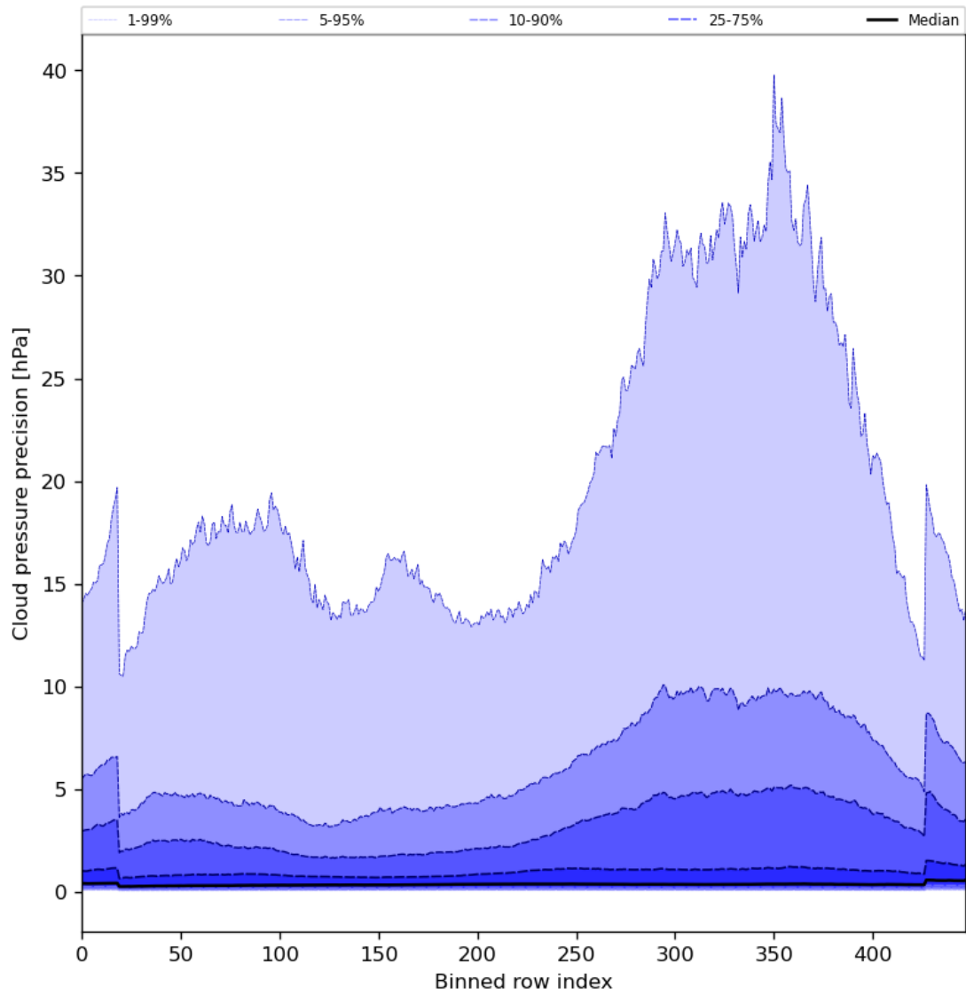
Figure 48: Along track statistics of “Cloud pressure precision” for 2024-02-27 to 2024-02-28
