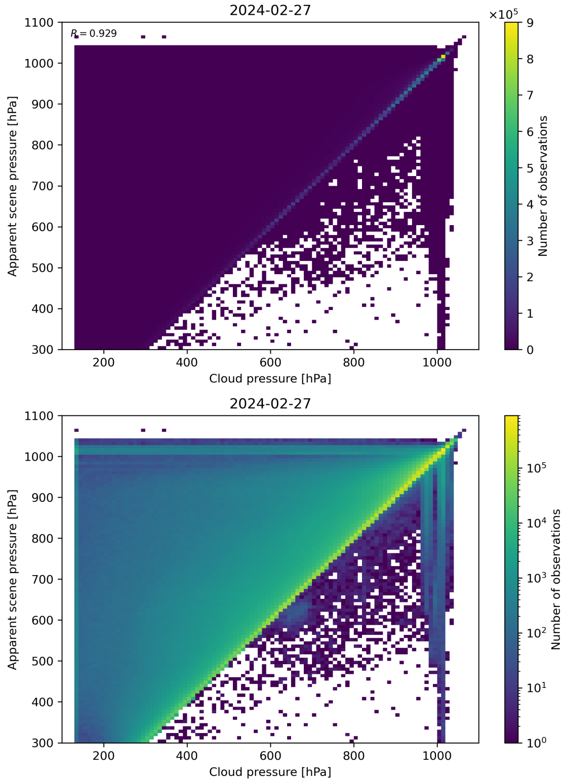
Figure 77: Scatter density plot of “Cloud pressure” against “Apparent scene pressure” for 2024-02-27 to 2024-02-28.
