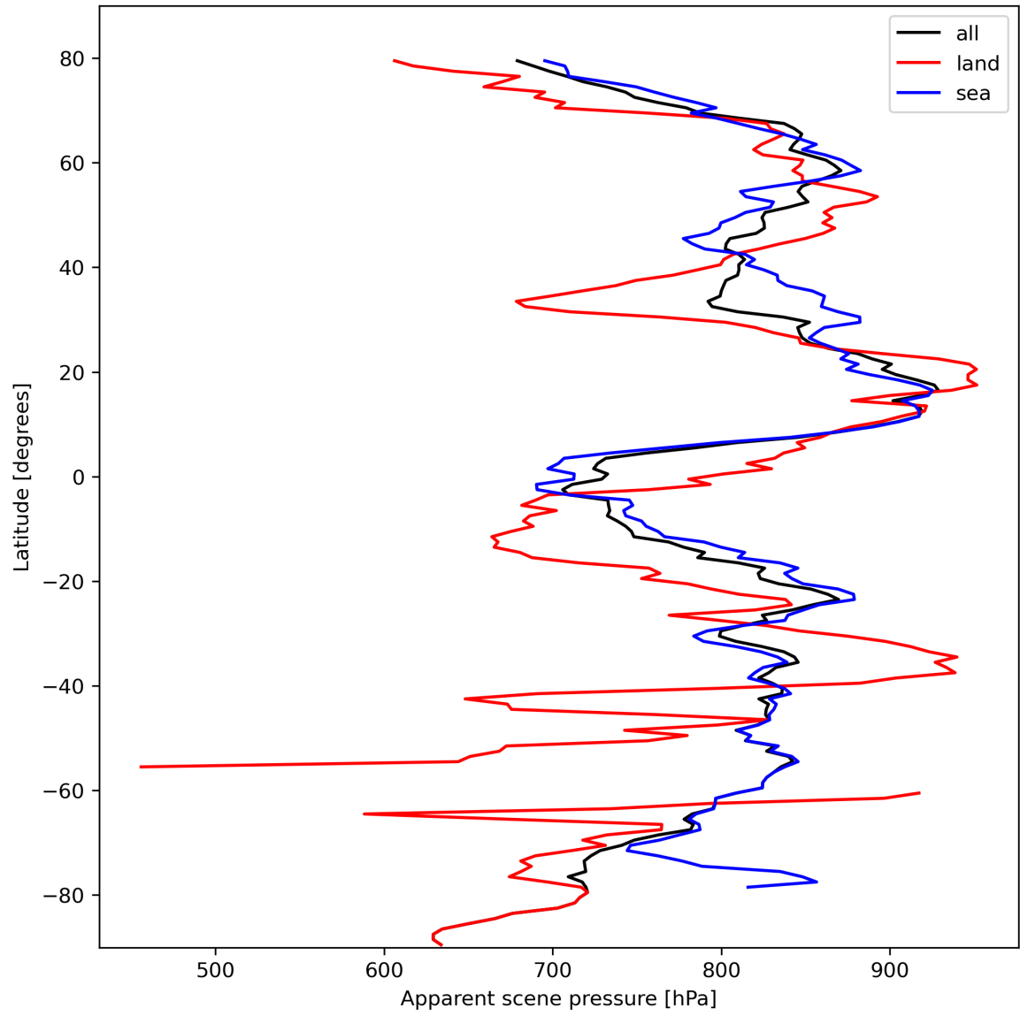
Figure 19: Zonal average of “Apparent scene pressure” for 2024-02-27 to 2024-02-28.
