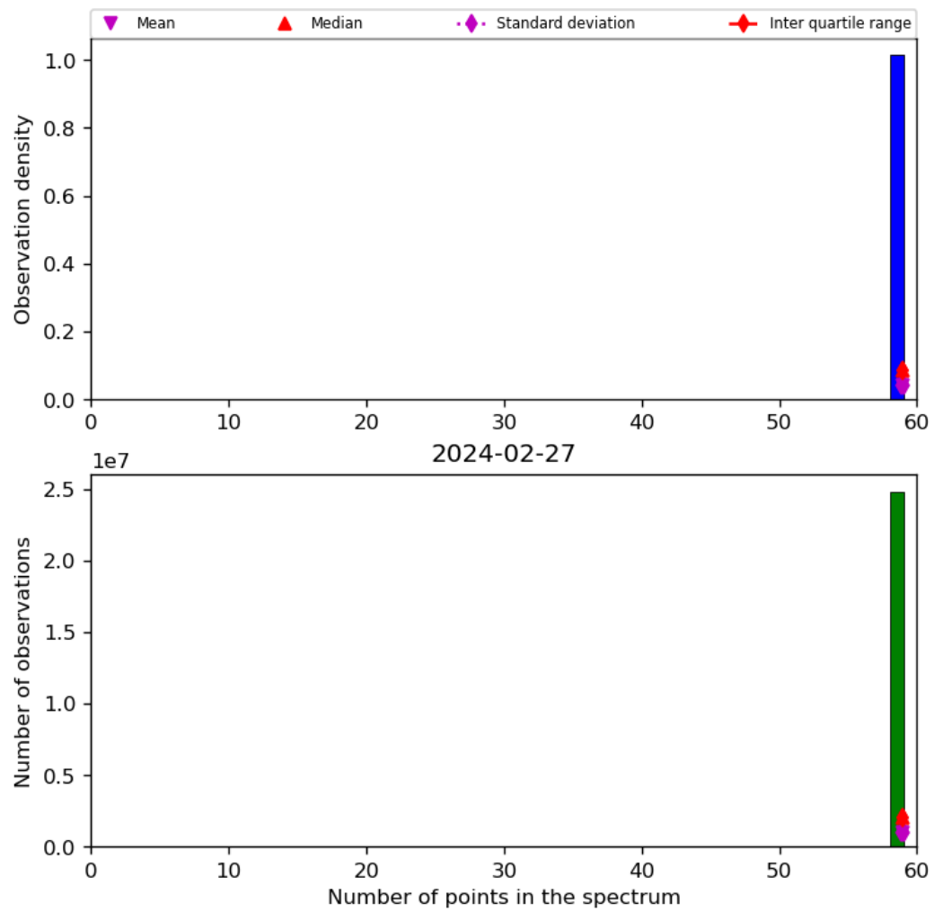
Figure 44: Histogram of “Number of points in the spectrum” for 2024-02-27 to 2024-02-28
