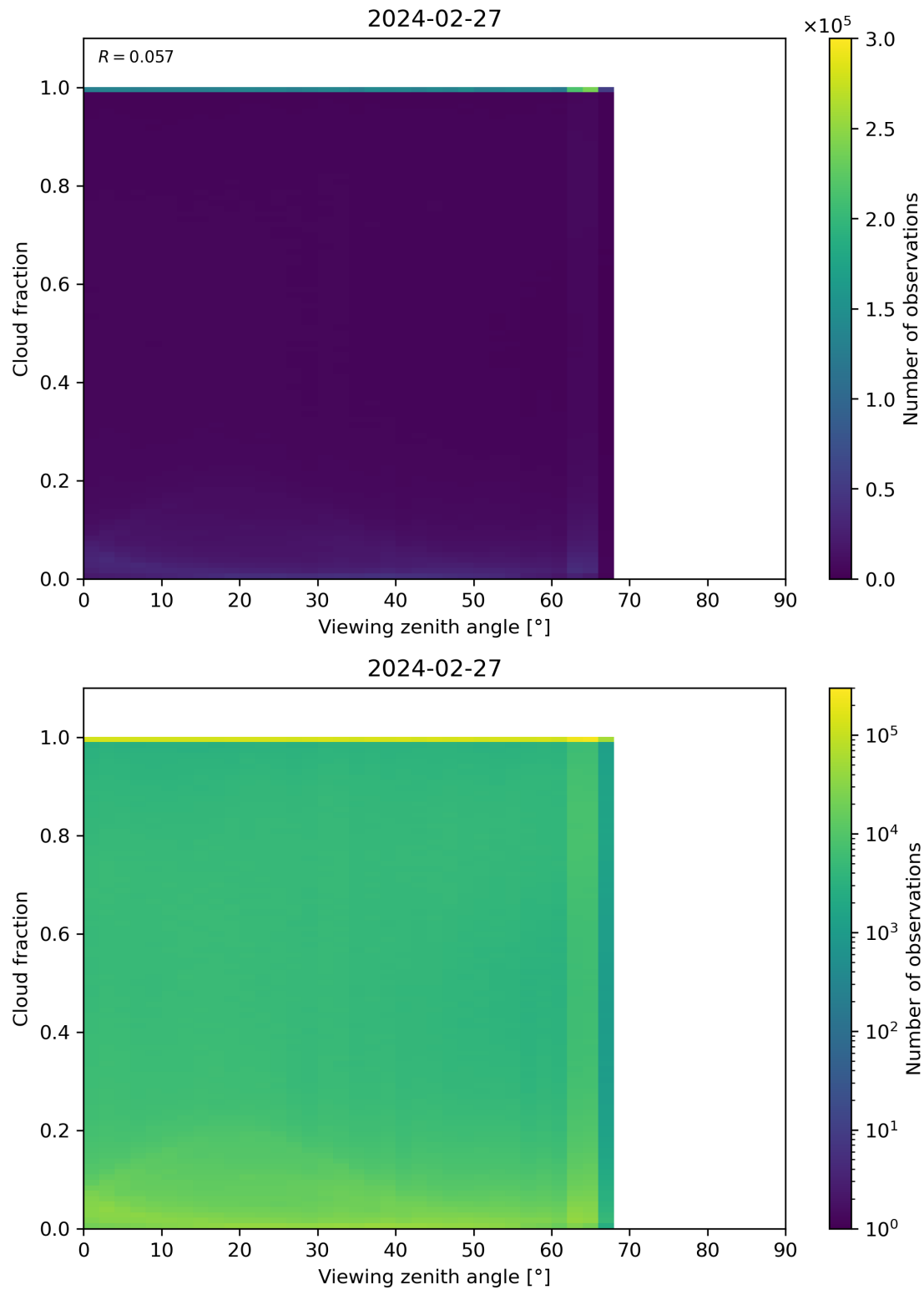
Figure 120: Scatter density plot of “Viewing zenith angle” against “Cloud fraction” for 2024-02-27 to 2024-02-28.
