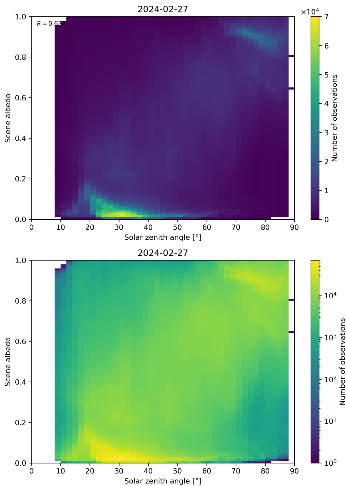
Figure 116: Scatter density plot of “Solar zenith angle” against “Scene albedo” for 2024-02-27 to 2024-02-28.
