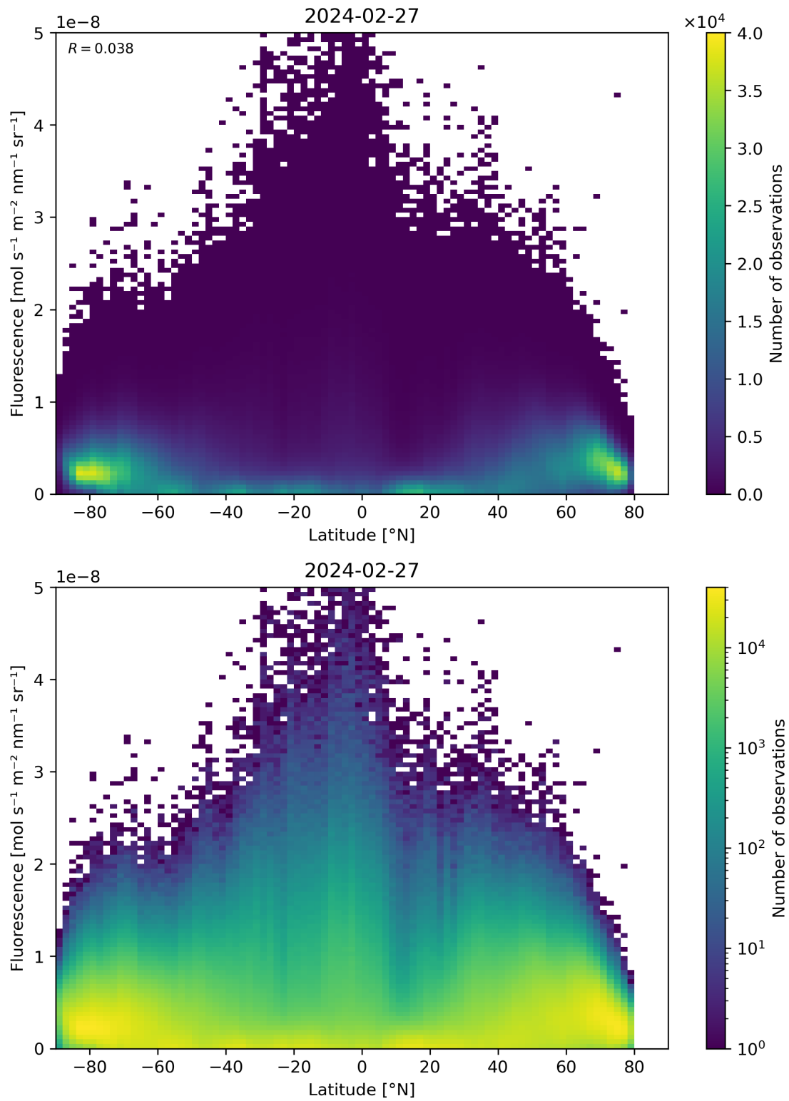
Figure 92: Scatter density plot of “Latitude” against “Fluorescence” for 2024-02-27 to 2024-02-28.
