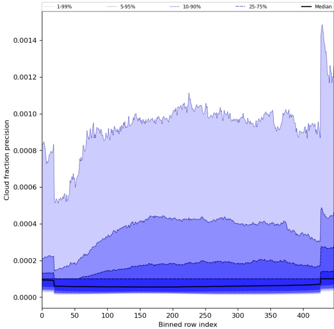
Figure 50: Along track statistics of “Cloud fraction precision” for 2024-02-27 to 2024-02-28
