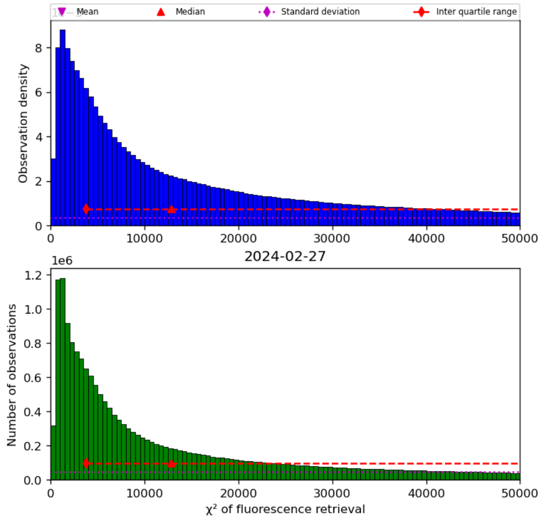
Figure 42: Histogram of “ \chi^2 of fluorescence retrieval” for 2024-02-27 to 2024-02-28
