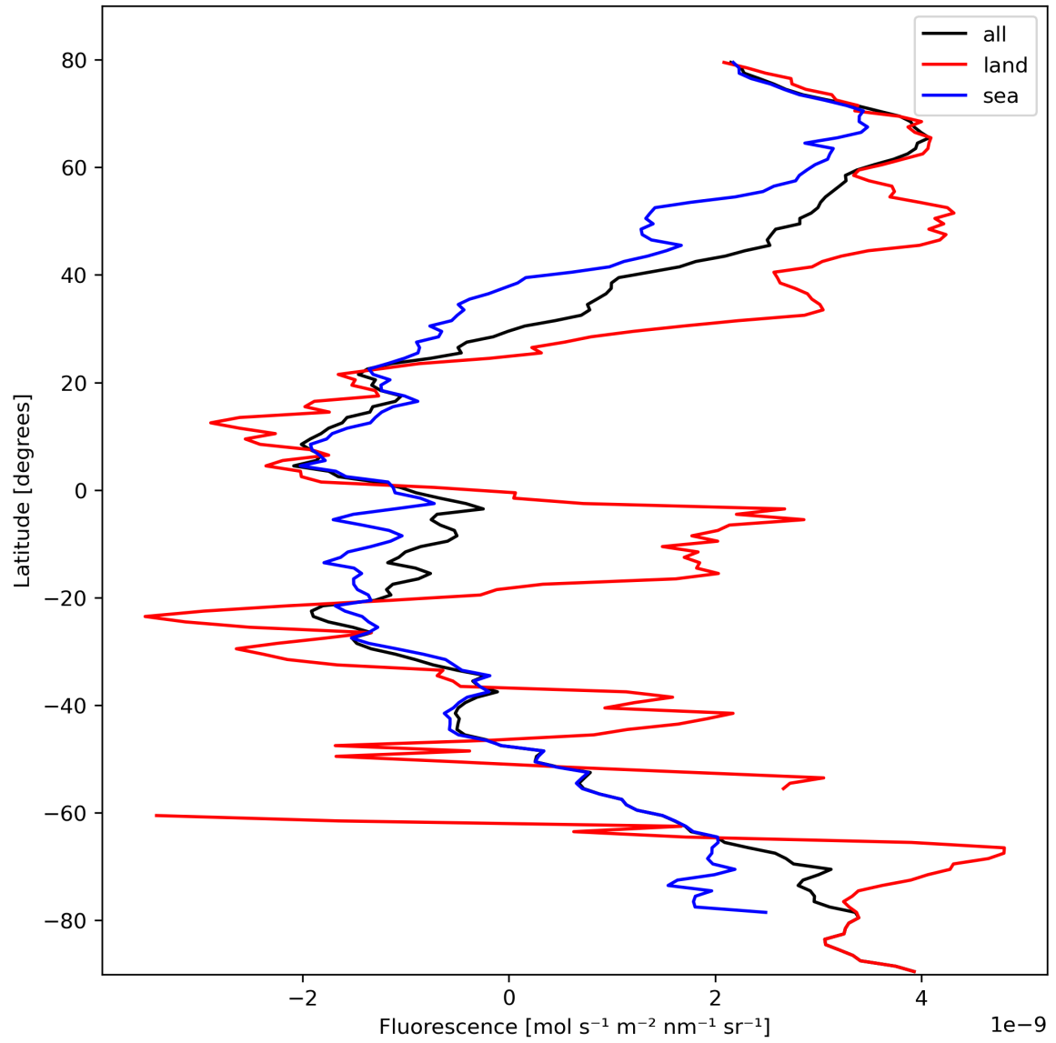
Figure 23: Zonal average of “Fluorescence” for 2024-02-27 to 2024-02-28.
