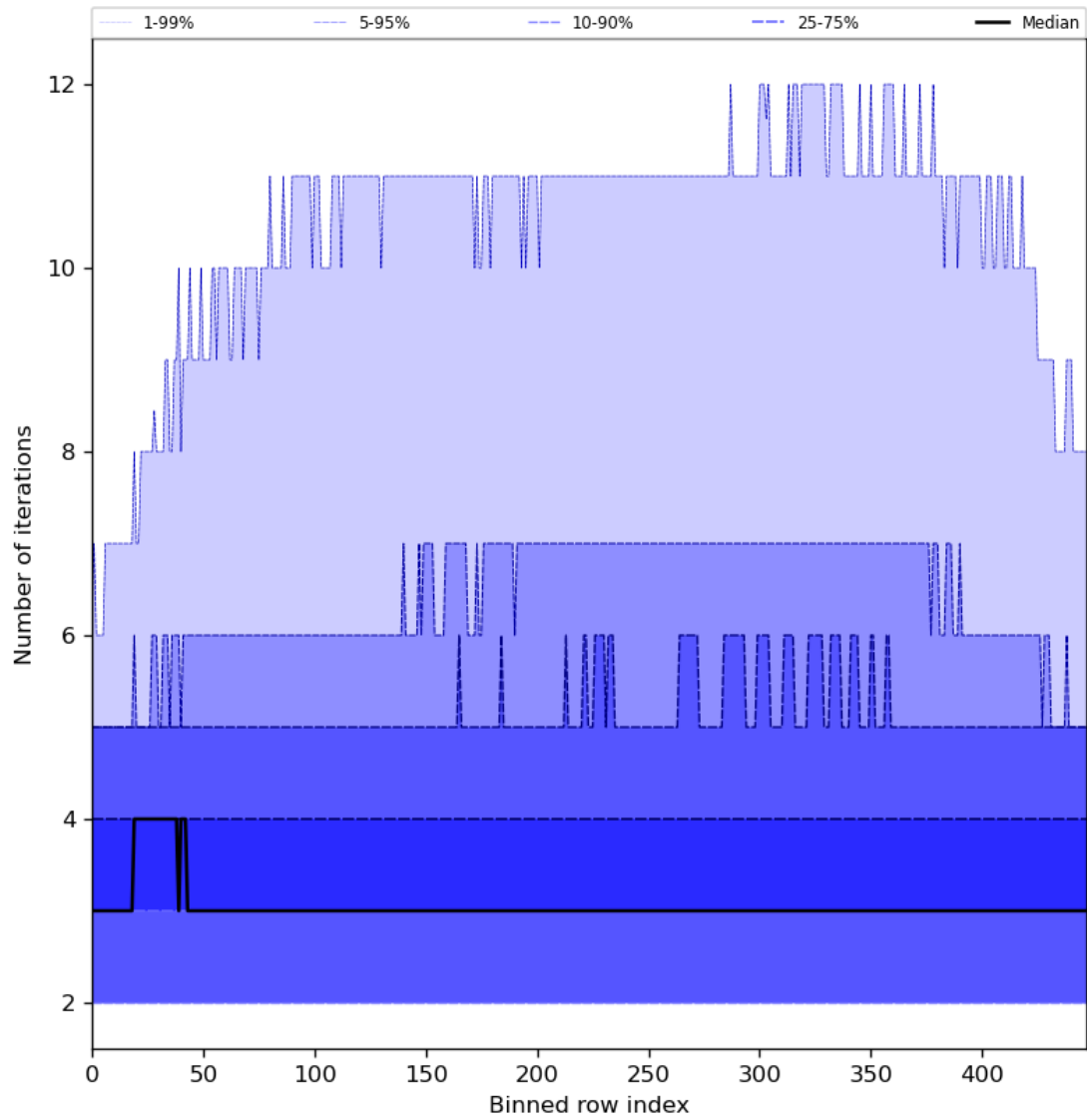
Figure 56: Along track statistics of “Number of iterations” for 2024-02-27 to 2024-02-28
