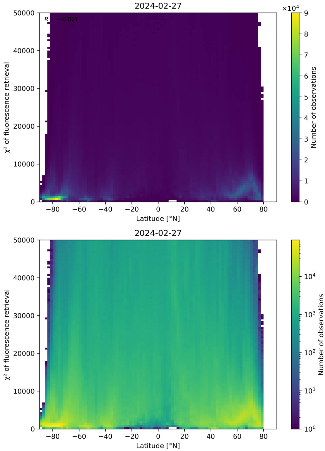
Figure 89: Scatter density plot of “Latitude” against “ \chi^2 of fluorescence retrieval” for 2024-02-27 to 2024-02-28.
