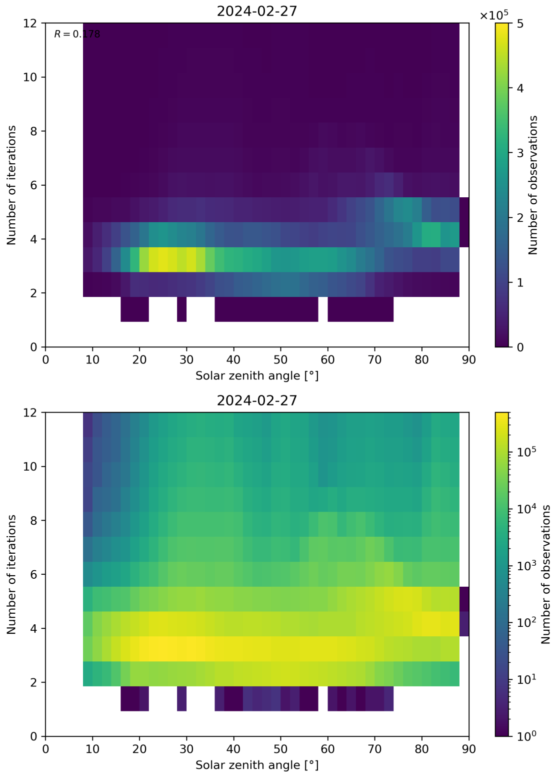
Figure 114: Scatter density plot of “Solar zenith angle” against “Number of iterations” for 2024-02-27 to 2024-02-28.
