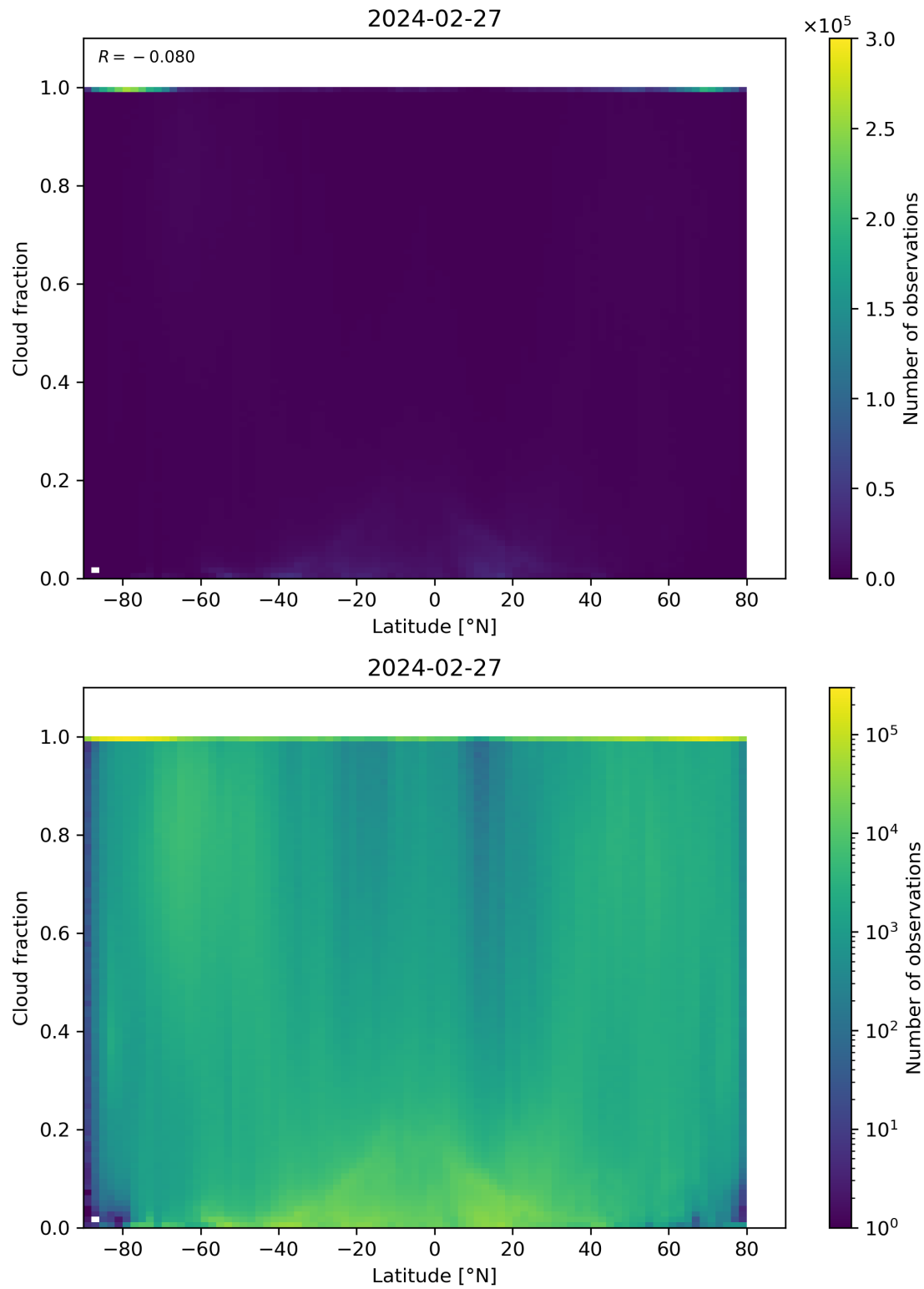
Figure 90: Scatter density plot of “Latitude” against “Cloud fraction” for 2024-02-27 to 2024-02-28.
