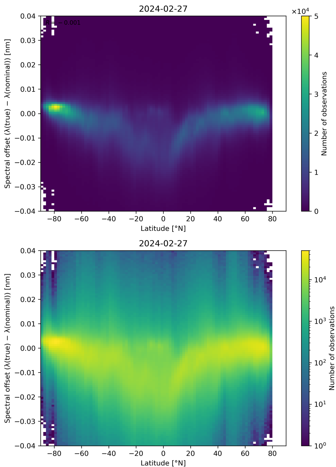
Figure 96: Scatter density plot of “Latitude” against “Spectral offset ( \lambda(\text{true}) - \lambda(\text{nominal}) )” for 2024-02-27 to 2024-02-28.
