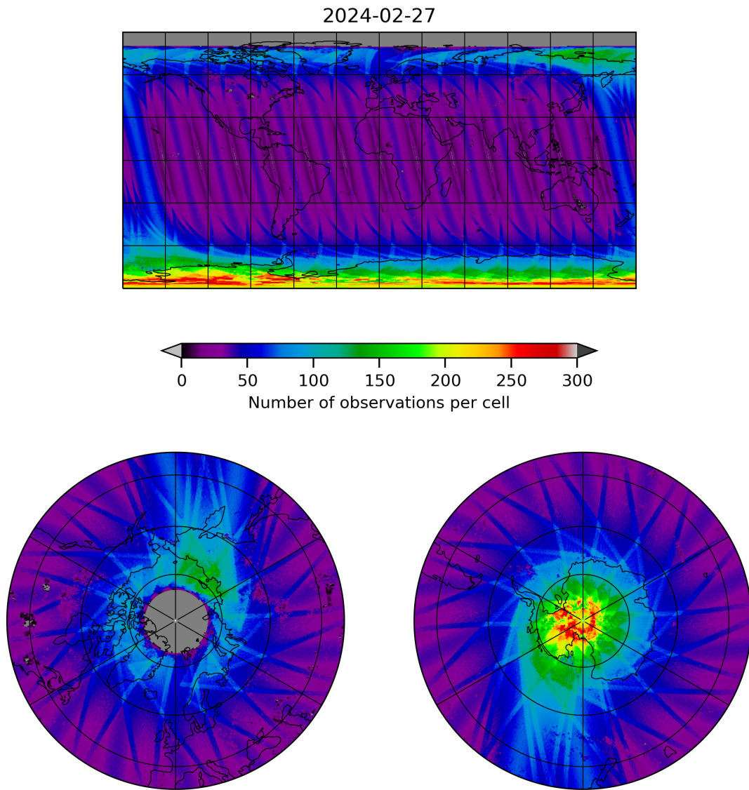
Figure 11: Map of the number of observations for 2024-02-27 to 2024-02-28
