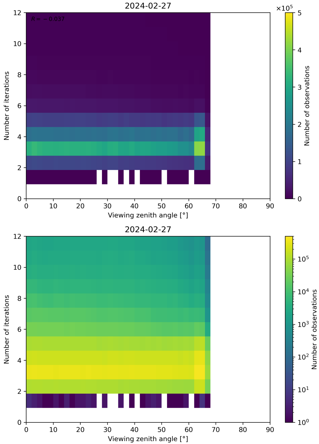
Figure 124: Scatter density plot of “Viewing zenith angle” against “Number of iterations” for 2024-02-27 to 2024-02-28.
