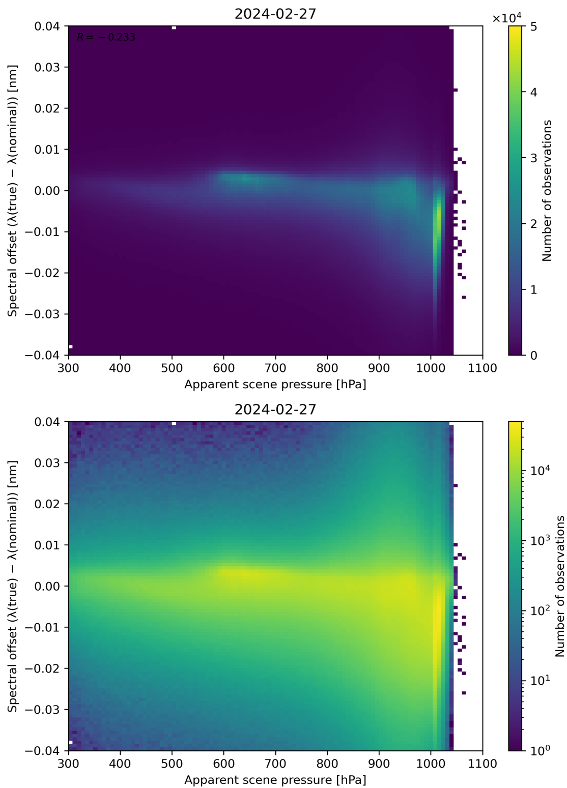
Figure 67: Scatter density plot of “Apparent scene pressure” against “Spectral offset ( \lambda(\text{true}) - \lambda(\text{nominal}) )” for 2024-02-27 to 2024-02-28.
