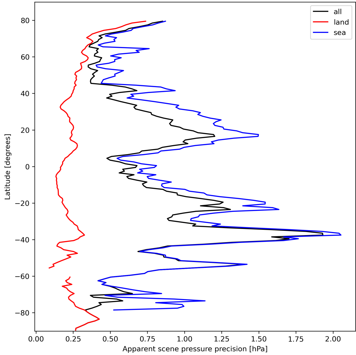
Figure 20: Zonal average of “Apparent scene pressure precision” for 2024-02-27 to 2024-02-28.
