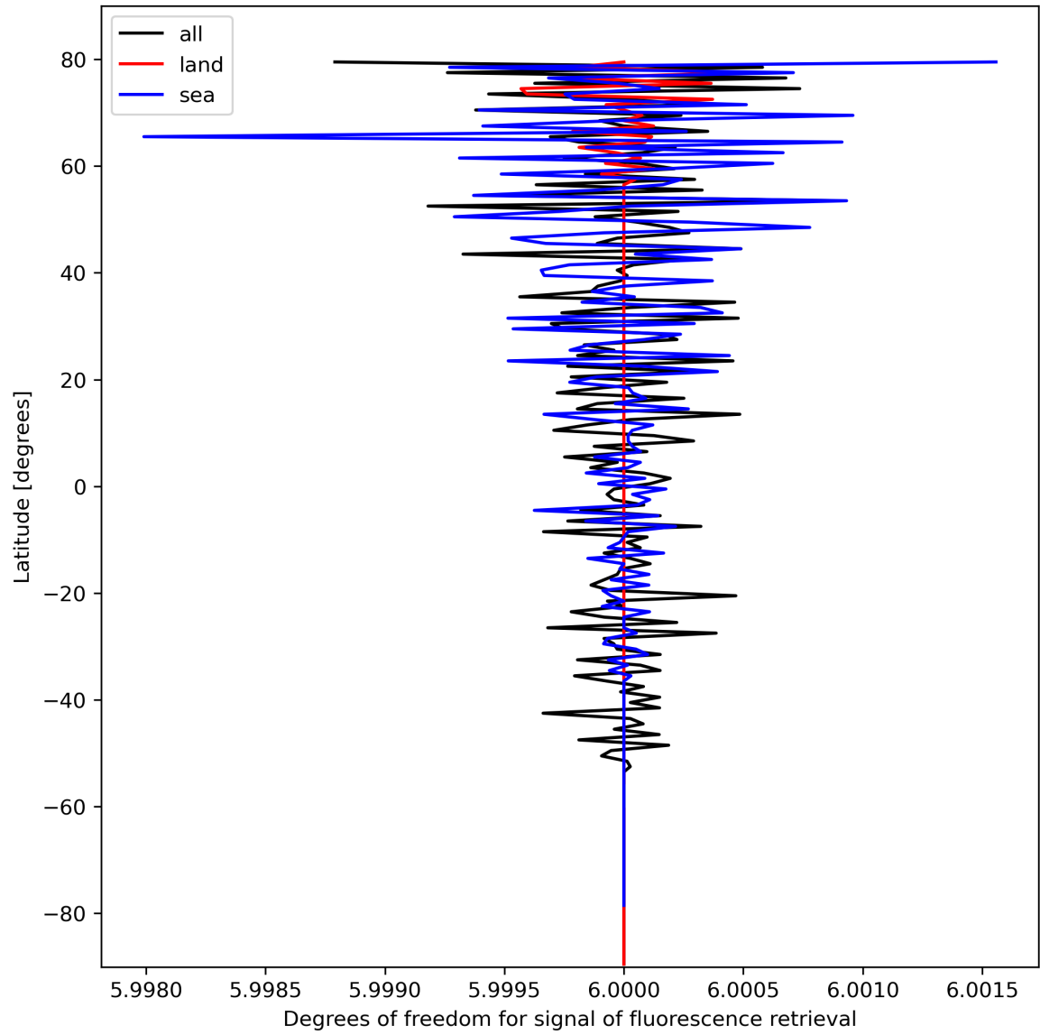
Figure 26: Zonal average of “Degrees of freedom for signal of fluorescence retrieval” for 2024-02-27 to 2024-02-28.
