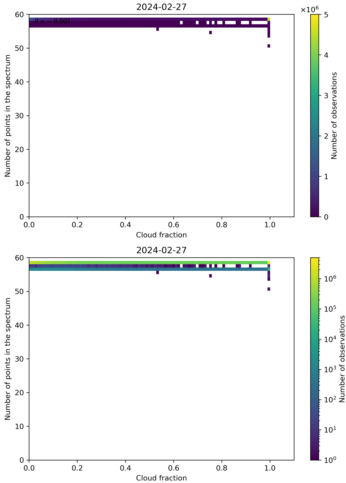
Figure 74: Scatter density plot of “Cloud fraction” against “Number of points in the spectrum” for 2024-02-27 to 2024-02-28.
