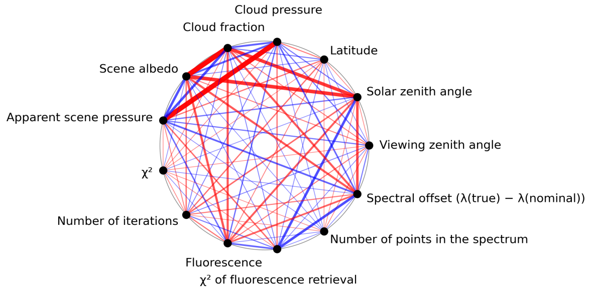
Figure 1: Map of correlation graph for 2024-02-27 to 2024-02-28.
