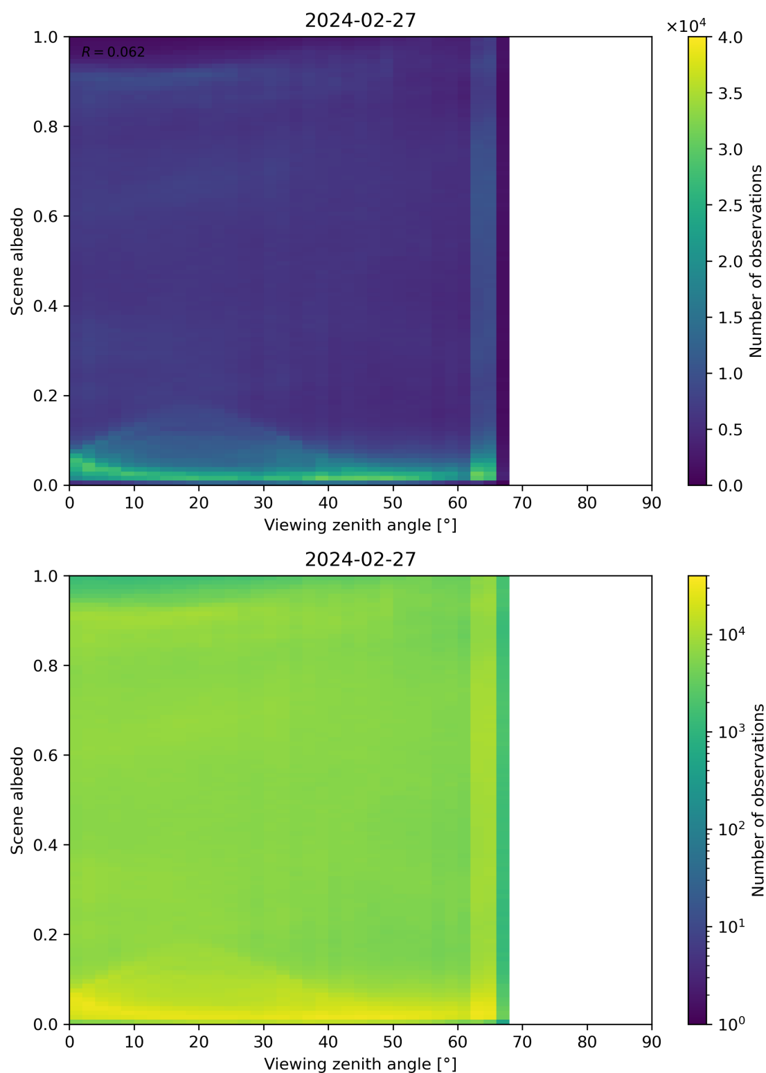
Figure 126: Scatter density plot of “Viewing zenith angle” against “Scene albedo” for 2024-02-27 to 2024-02-28.
