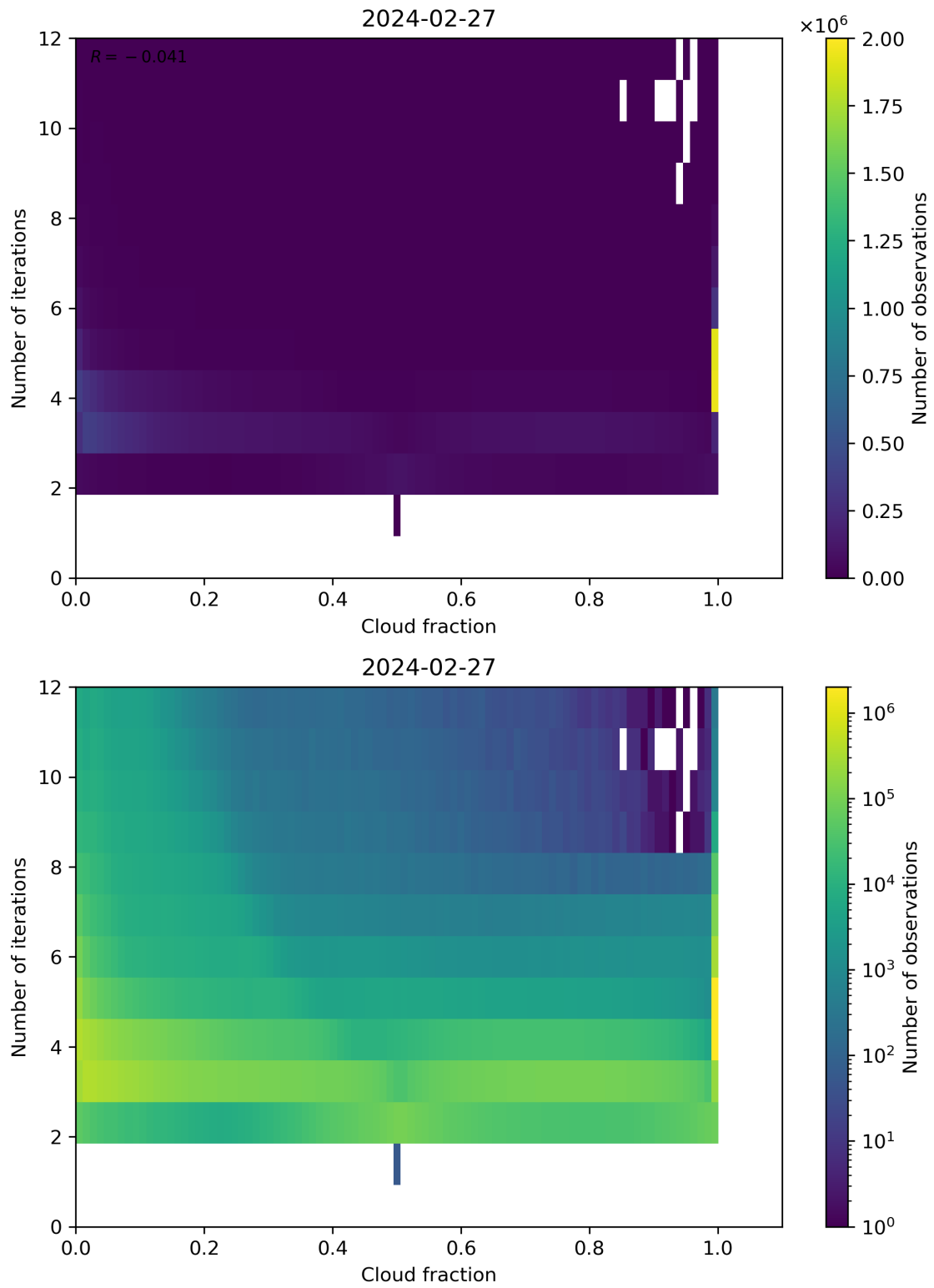
Figure 73: Scatter density plot of “Cloud fraction” against “Number of iterations” for 2024-02-27 to 2024-02-28.
