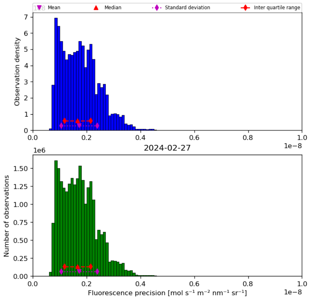
Figure 41: Histogram of “Fluorescence precision” for 2024-02-27 to 2024-02-28
