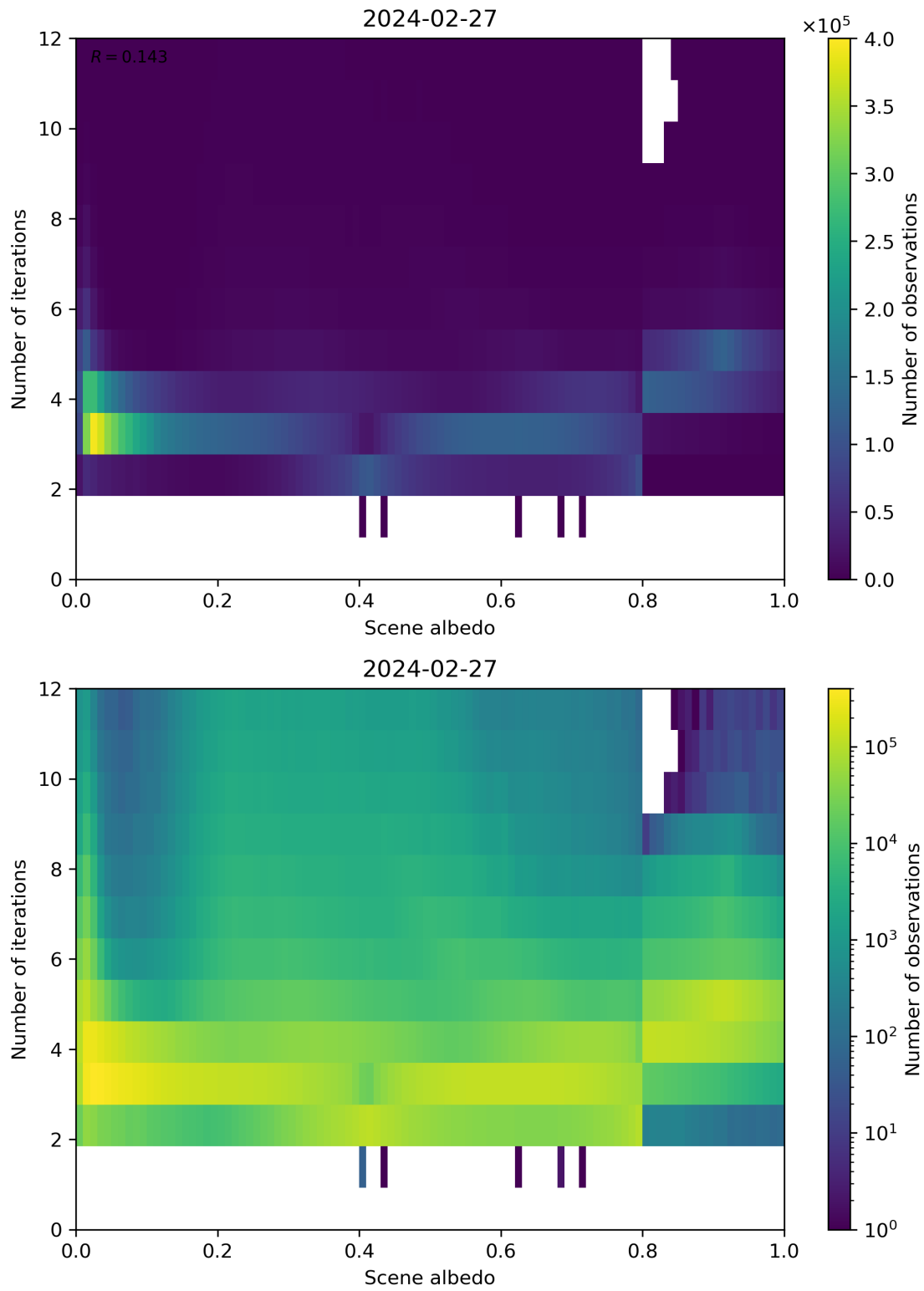
Figure 105: Scatter density plot of “Scene albedo” against “Number of iterations” for 2024-02-27 to 2024-02-28.
