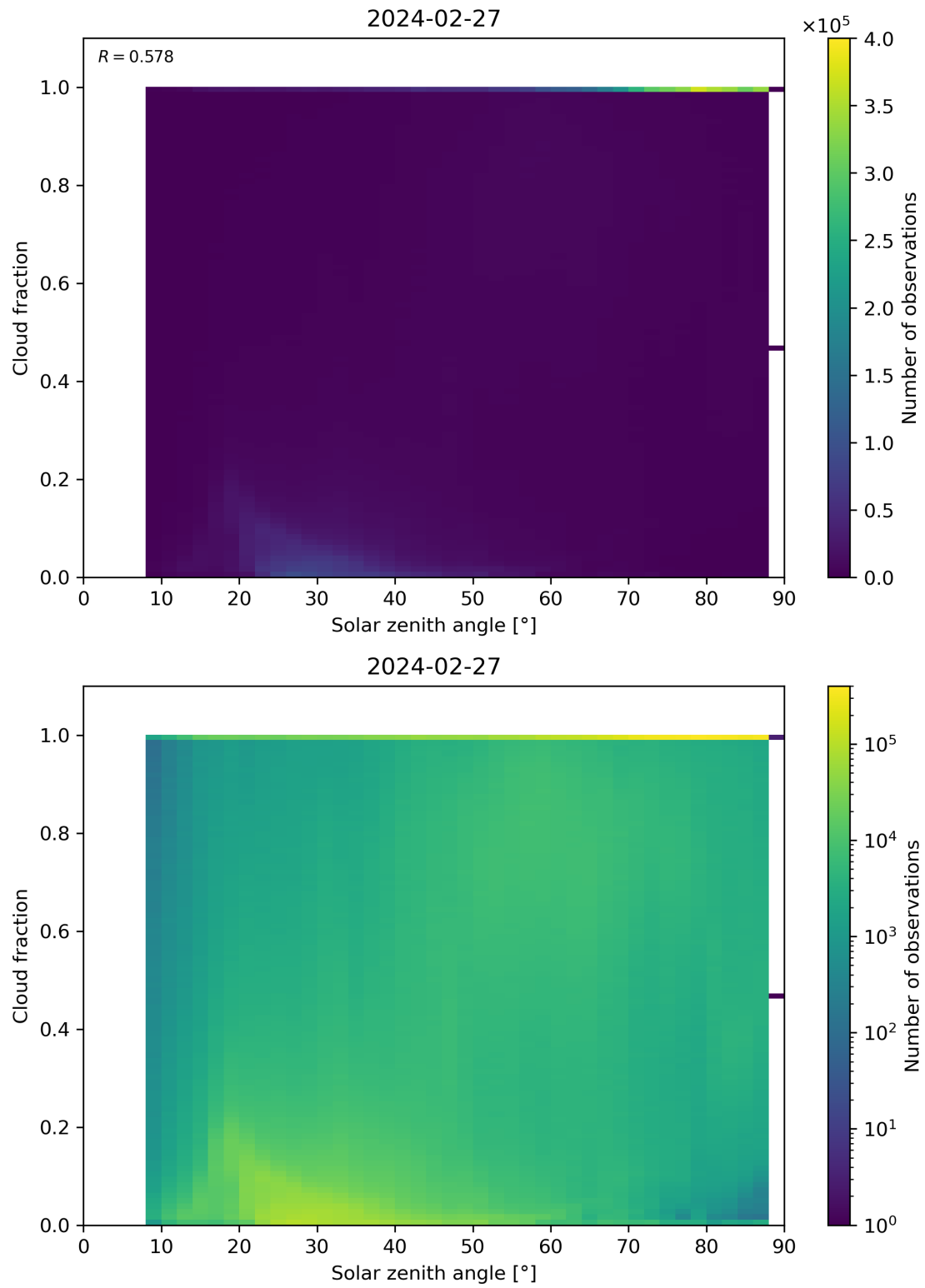
Figure 110: Scatter density plot of “Solar zenith angle” against “Cloud fraction” for 2024-02-27 to 2024-02-28.
