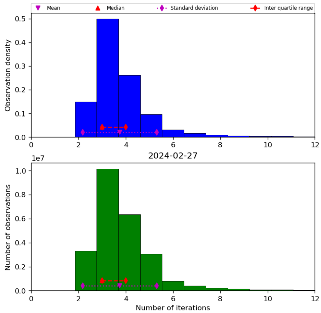
Figure 39: Histogram of “Number of iterations” for 2024-02-27 to 2024-02-28
