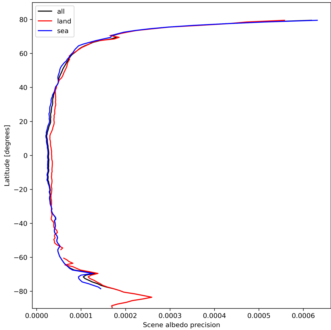
Figure 18: Zonal average of “Scene albedo precision” for 2024-02-27 to 2024-02-28.
