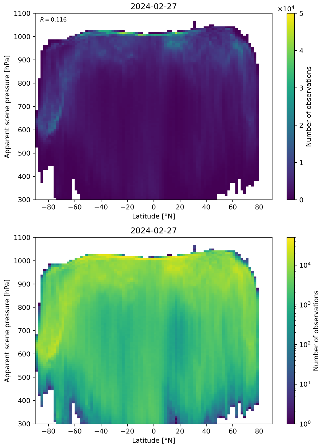
Figure 88: Scatter density plot of “Latitude” against “Apparent scene pressure” for 2024-02-27 to 2024-02-28.
