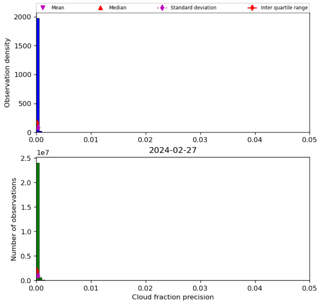
Figure 33: Histogram of “Cloud fraction precision” for 2024-02-27 to 2024-02-28
