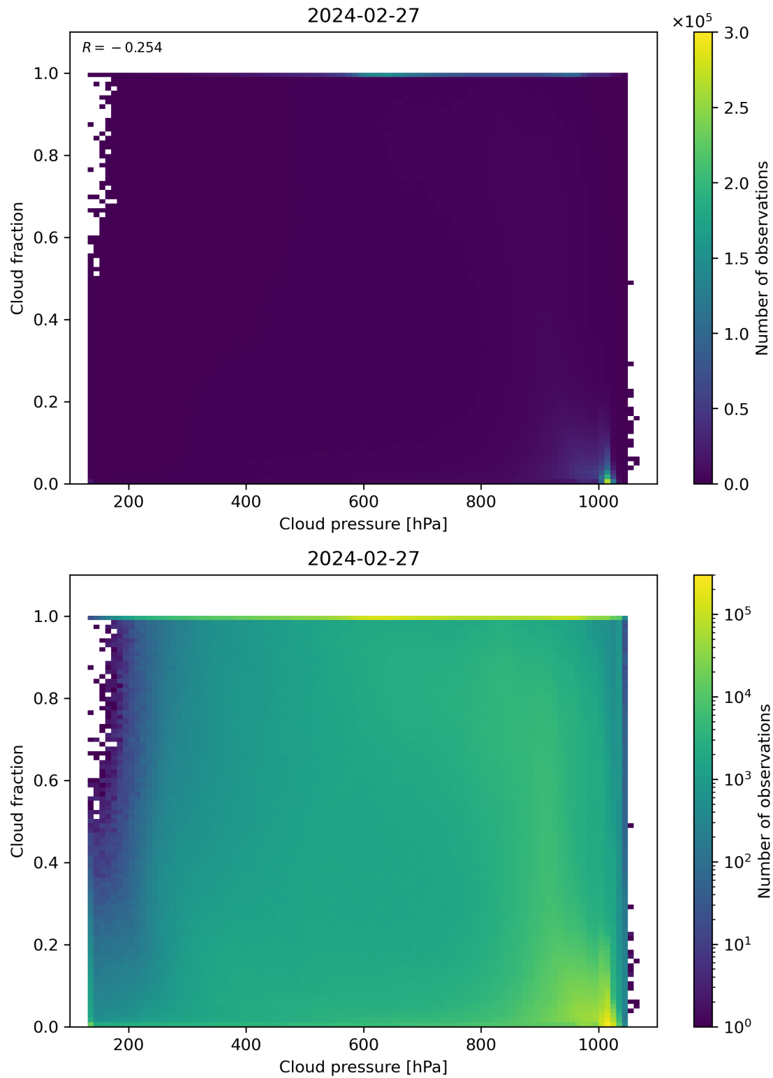
Figure 79: Scatter density plot of “Cloud pressure” against “Cloud fraction” for 2024-02-27 to 2024-02-28.
