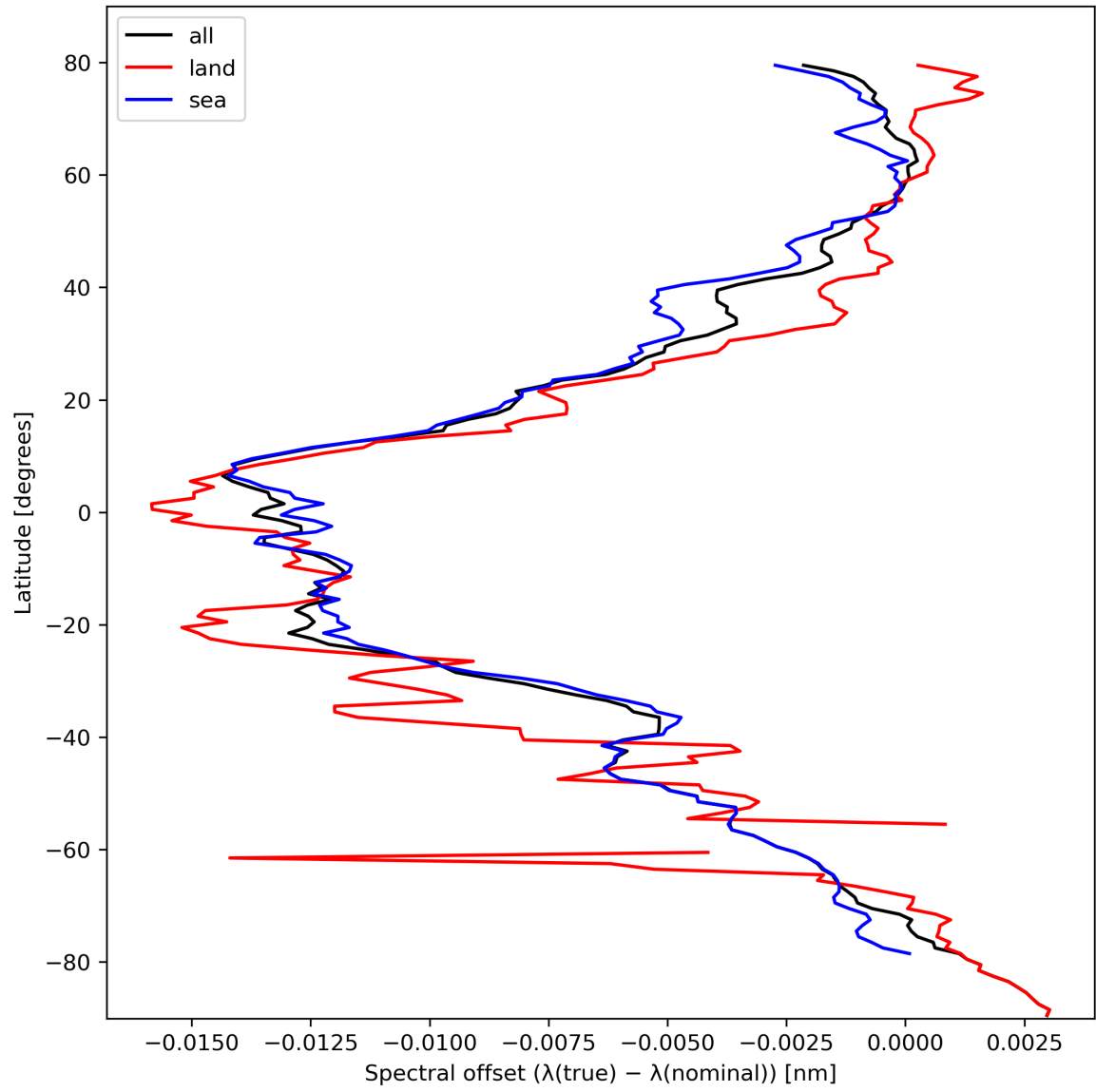
Figure 28: Zonal average of “Spectral offset ( \lambda(\text{true}) - \lambda(\text{nominal}) )” for 2024-02-27 to 2024-02-28.
