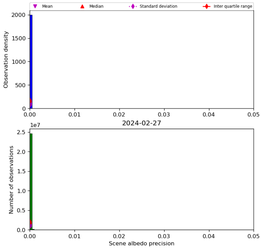
Figure 35: Histogram of “Scene albedo precision” for 2024-02-27 to 2024-02-28
