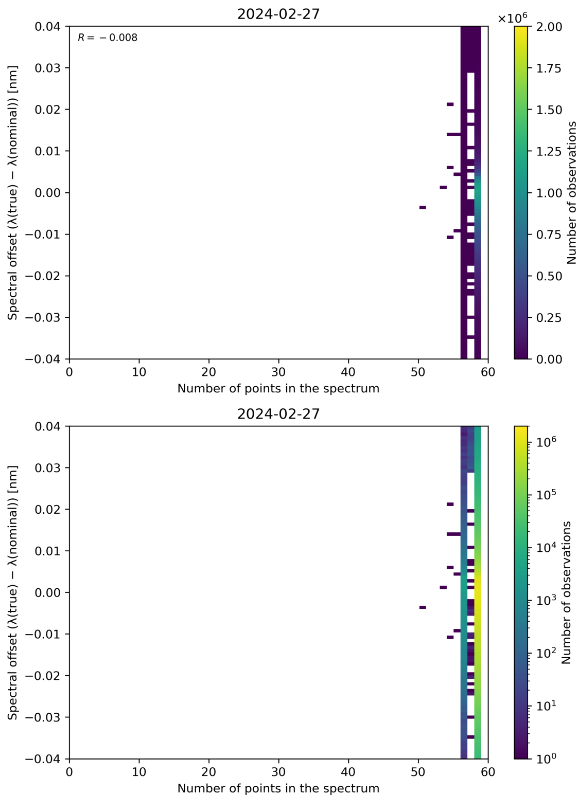
Figure 101: Scatter density plot of “Number of points in the spectrum” against “Spectral offset ( \lambda(\text{true}) - \lambda(\text{nominal}) )” for 2024-02-27 to 2024-02-28.
