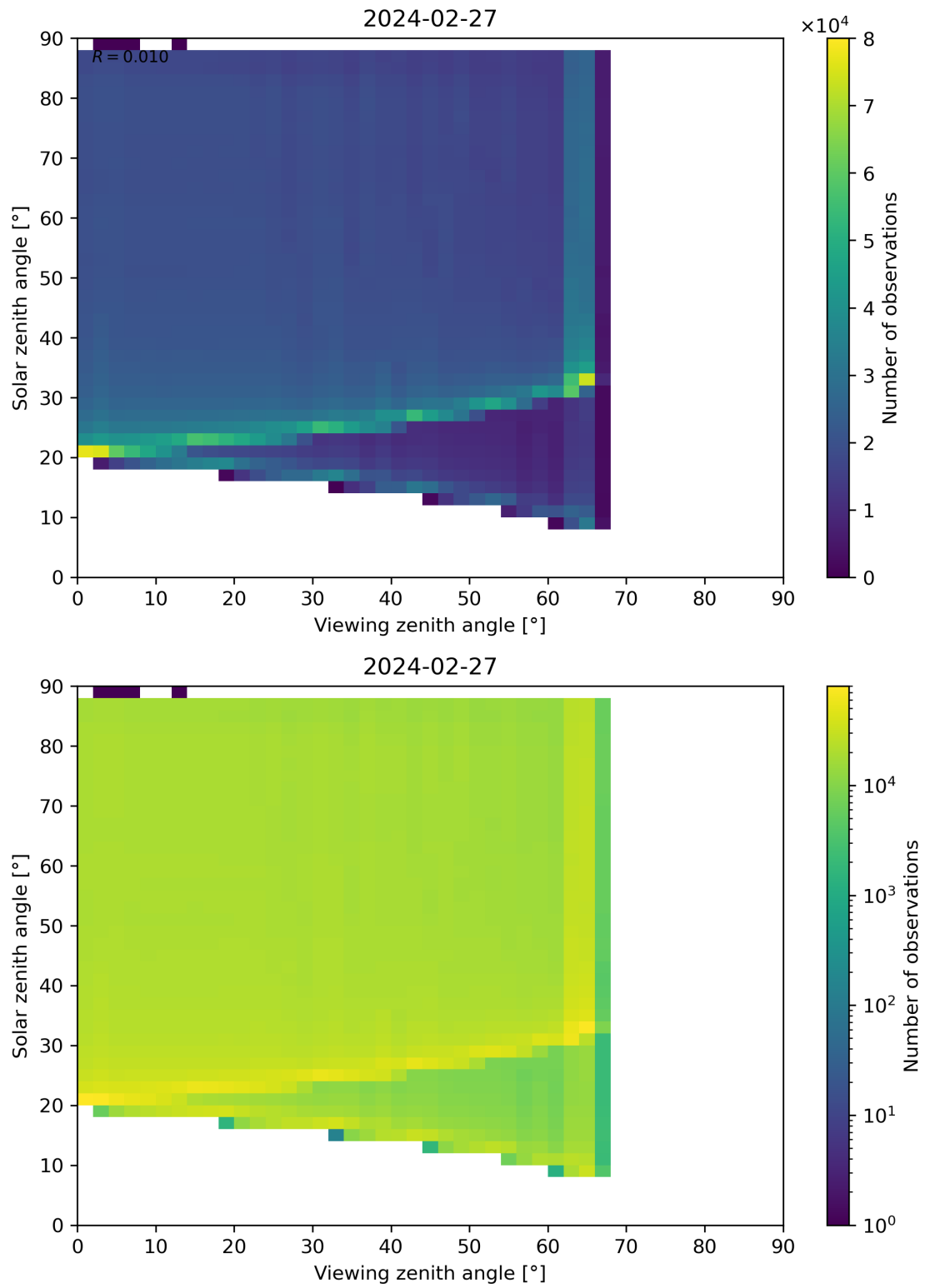
Figure 127: Scatter density plot of “Viewing zenith angle” against “Solar zenith angle” for 2024-02-27 to 2024-02-28.
