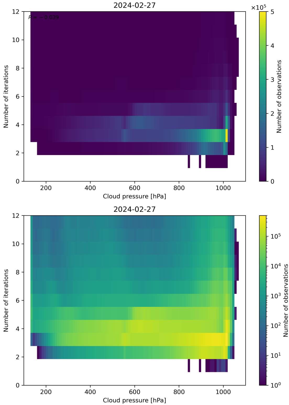
Figure 81: Scatter density plot of “Cloud pressure” against “Number of iterations” for 2024-02-27 to 2024-02-28.
