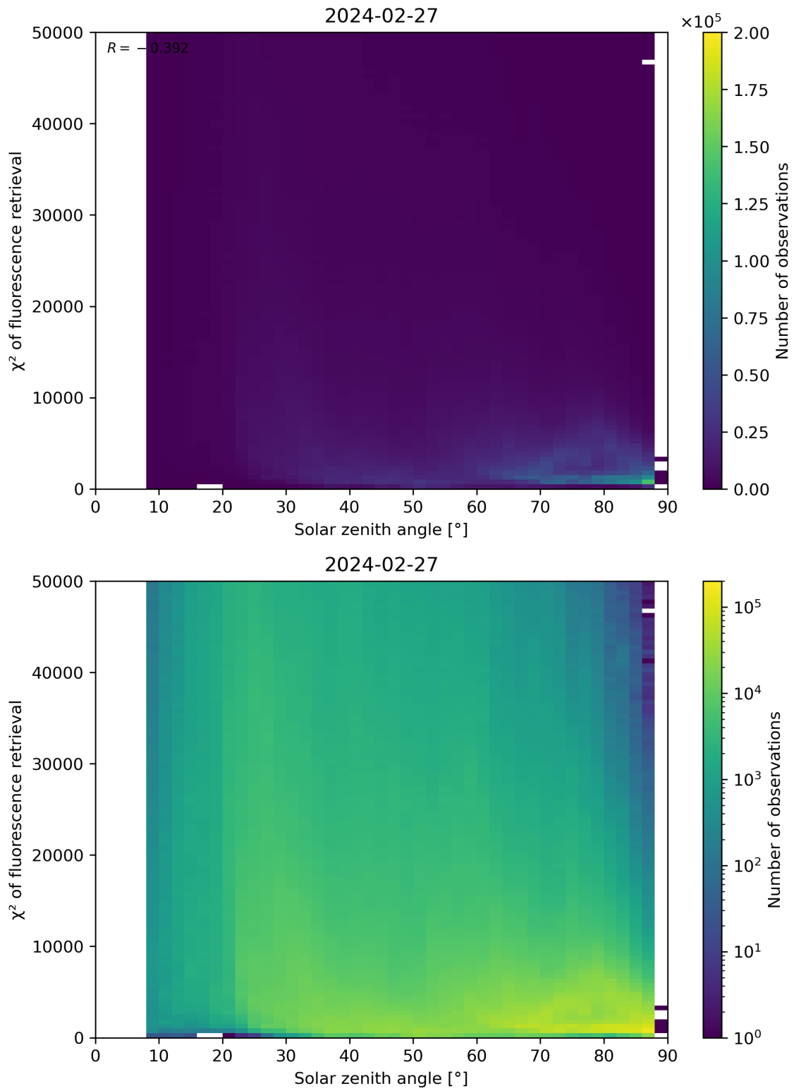
Figure 109: Scatter density plot of “Solar zenith angle” against “ \chi^2 of fluorescence retrieval” for 2024-02-27 to 2024-02-28.
