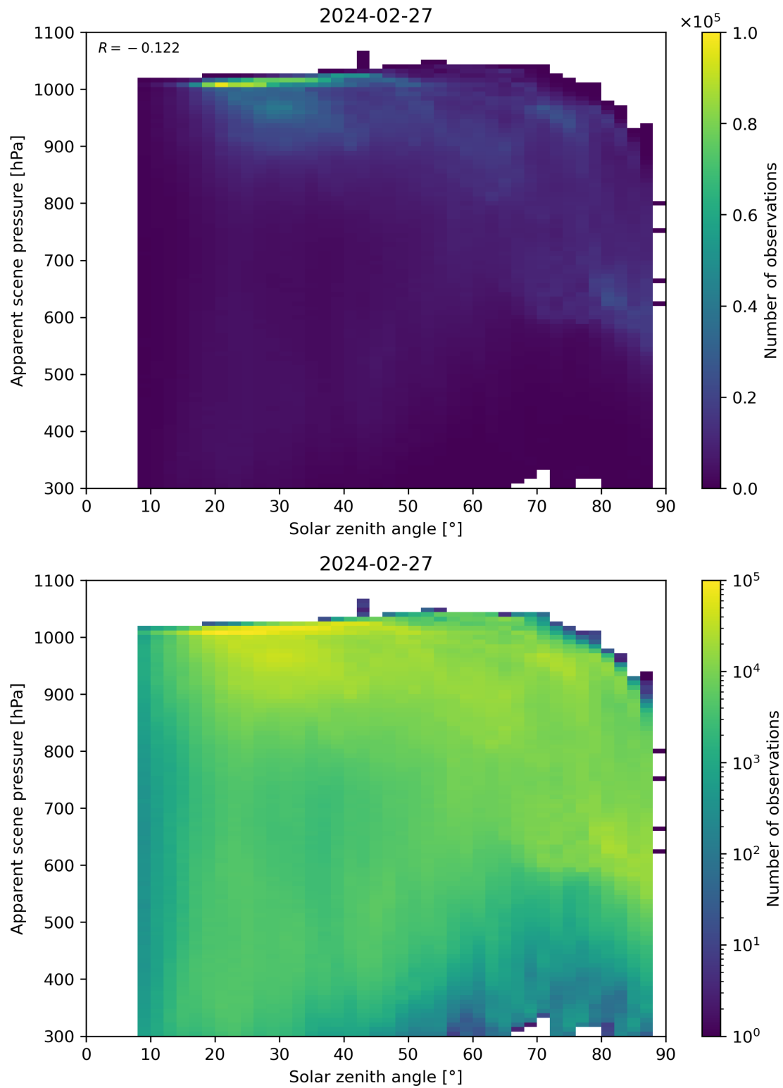
Figure 108: Scatter density plot of “Solar zenith angle” against “Apparent scene pressure” for 2024-02-27 to 2024-02-28.
