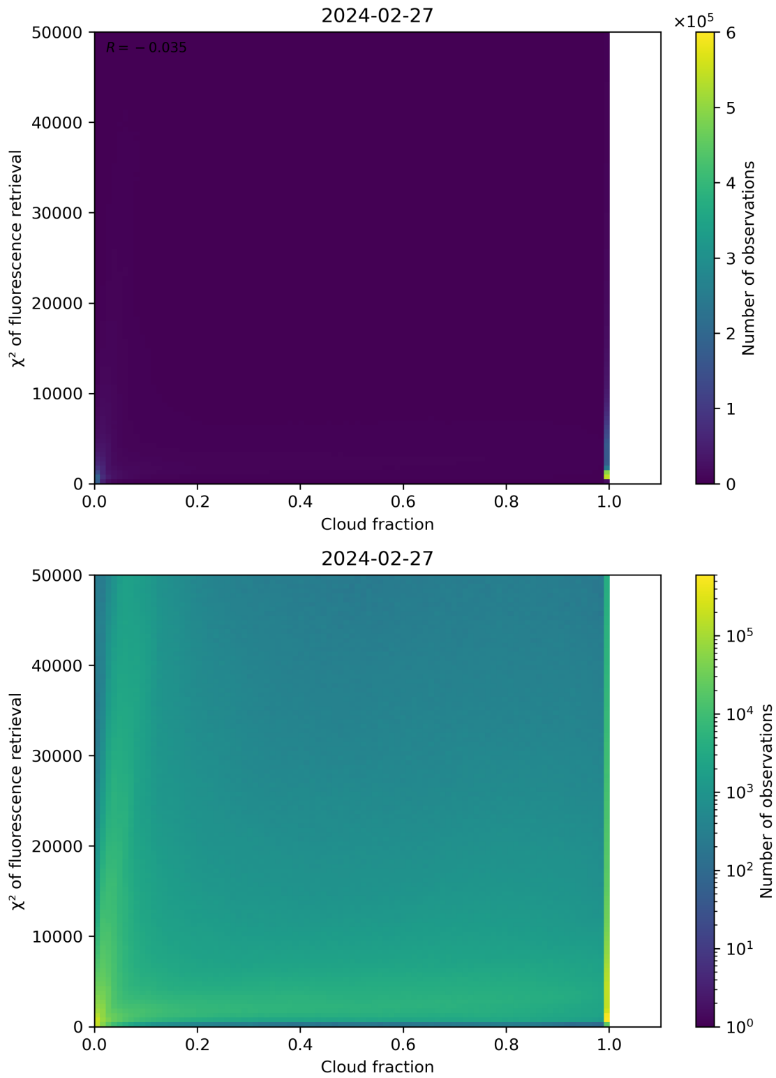
Figure 71: Scatter density plot of “Cloud fraction” against “ \chi^2 of fluorescence retrieval” for 2024-02-27 to 2024-02-28.
