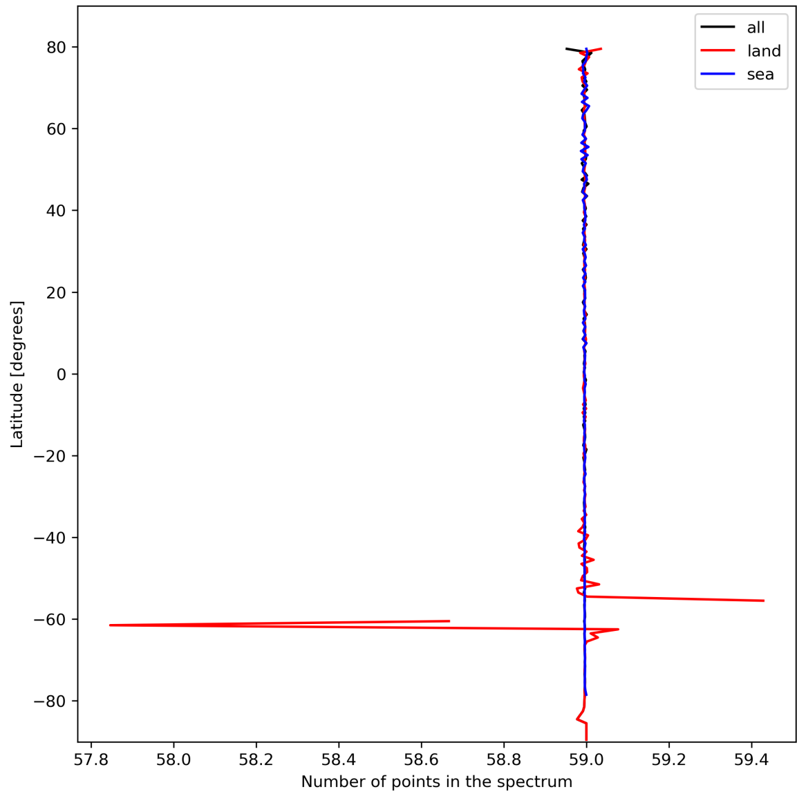
Figure 27: Zonal average of “Number of points in the spectrum” for 2024-02-27 to 2024-02-28.
