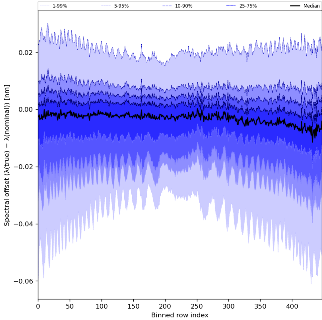
Figure 62: Along track statistics of “Spectral offset ( \lambda(\text{true}) - \lambda(\text{nominal}) )” for 2024-02-27 to 2024-02-28
