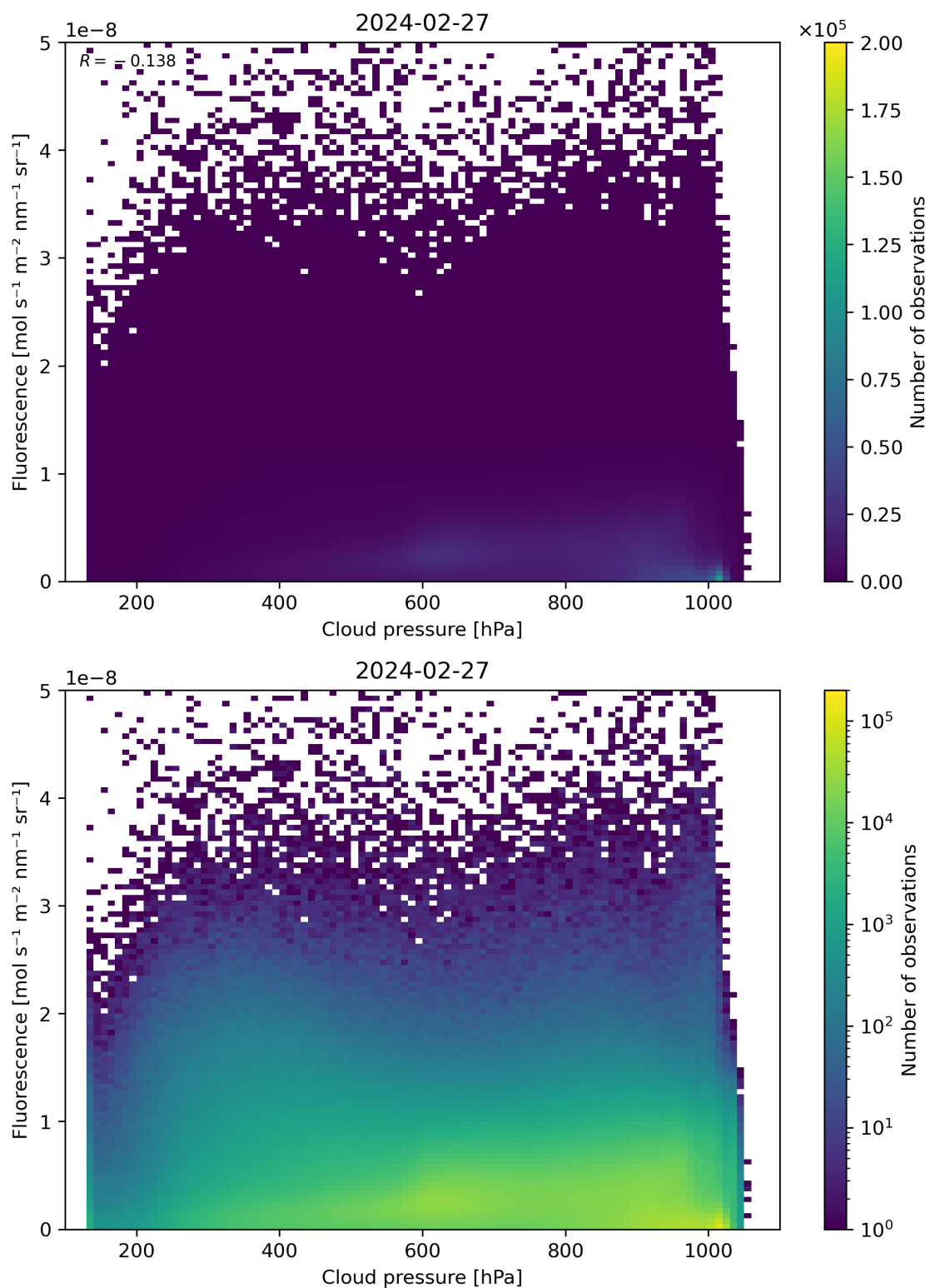
Figure 80: Scatter density plot of “Cloud pressure” against “Fluorescence” for 2024-02-27 to 2024-02-28.
