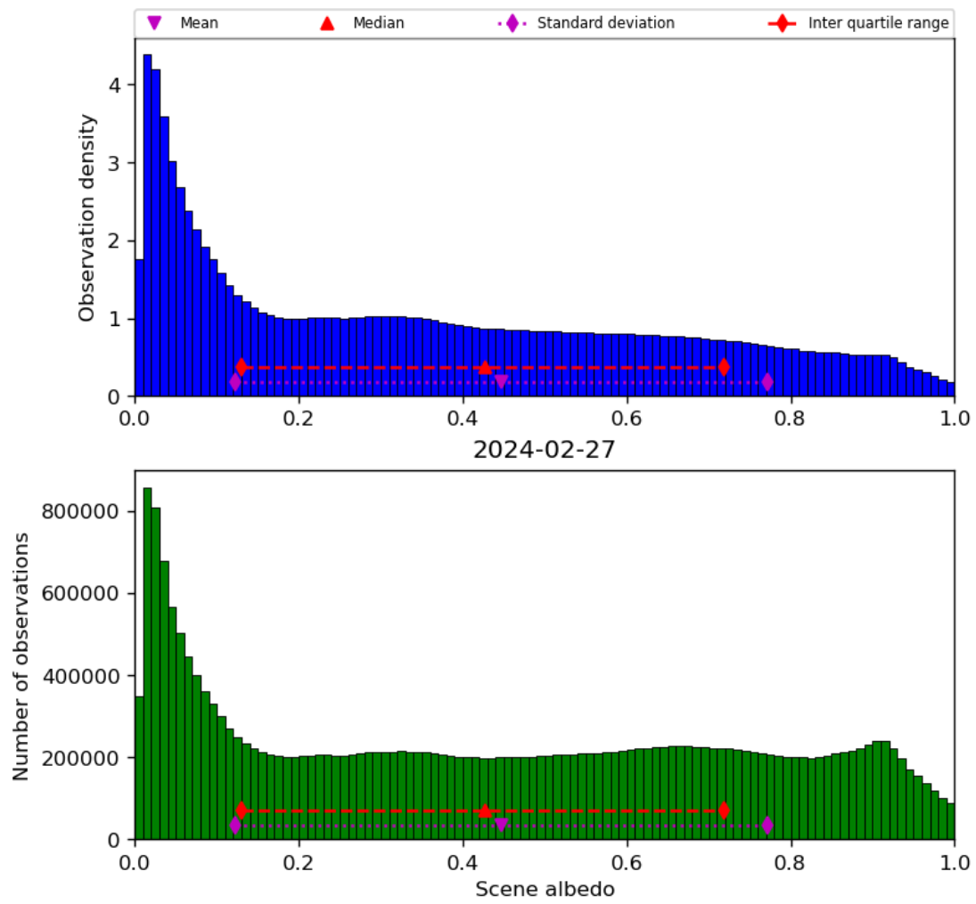
Figure 34: Histogram of “Scene albedo” for 2024-02-27 to 2024-02-28
