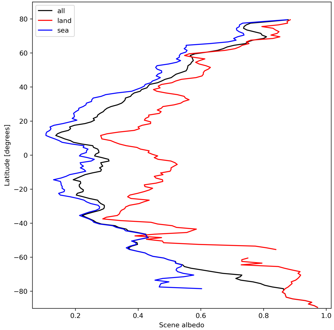
Figure 17: Zonal average of “Scene albedo” for 2024-02-27 to 2024-02-28.
