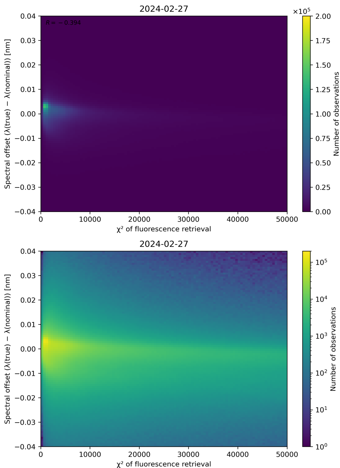
Figure 69: Scatter density plot of " \chi^2 of fluorescence retrieval" against "Spectral offset ( \lambda(\text{true}) - \lambda(\text{nominal}) )" for 2024-02-27 to 2024-02-28.
