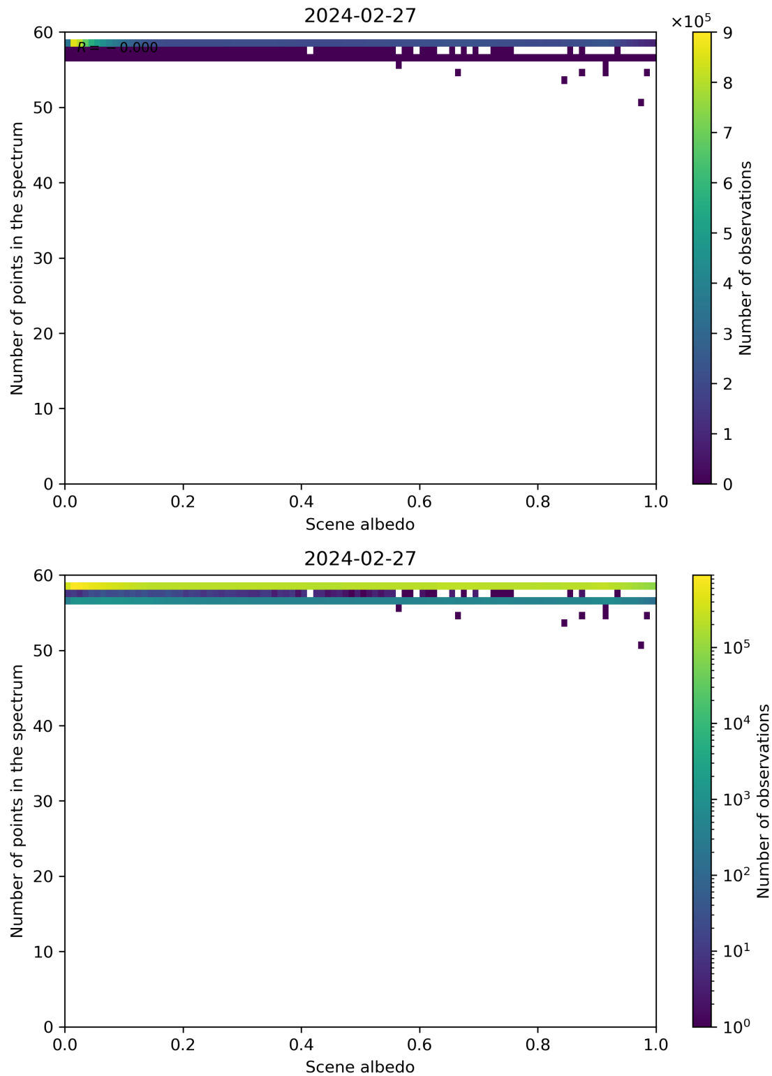
Figure 106: Scatter density plot of “Scene albedo” against “Number of points in the spectrum” for 2024-02-27 to 2024-02-28.
