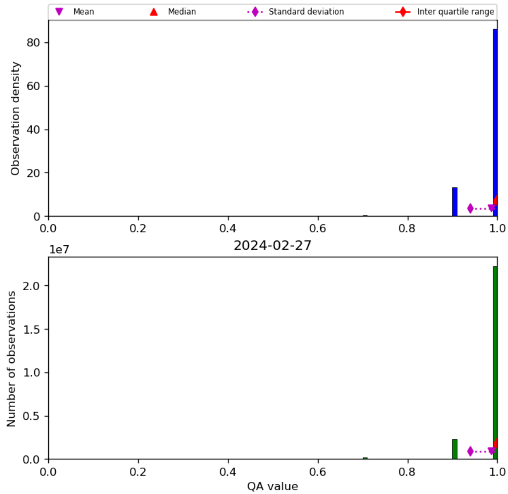
Figure 29: Histogram of “QA value” for 2024-02-27 to 2024-02-28
