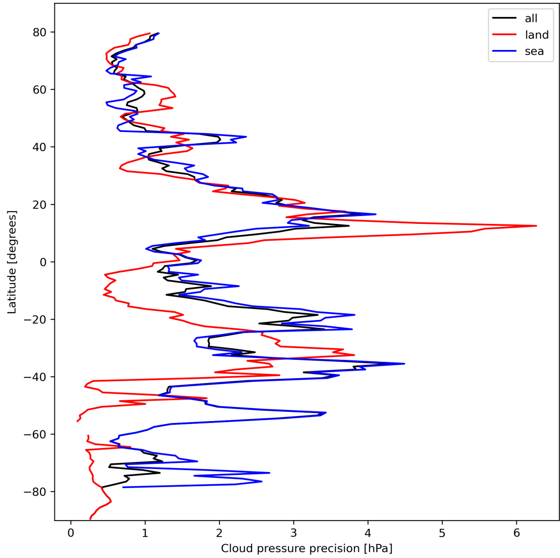
Figure 14: Zonal average of “Cloud pressure precision” for 2024-02-27 to 2024-02-28.
