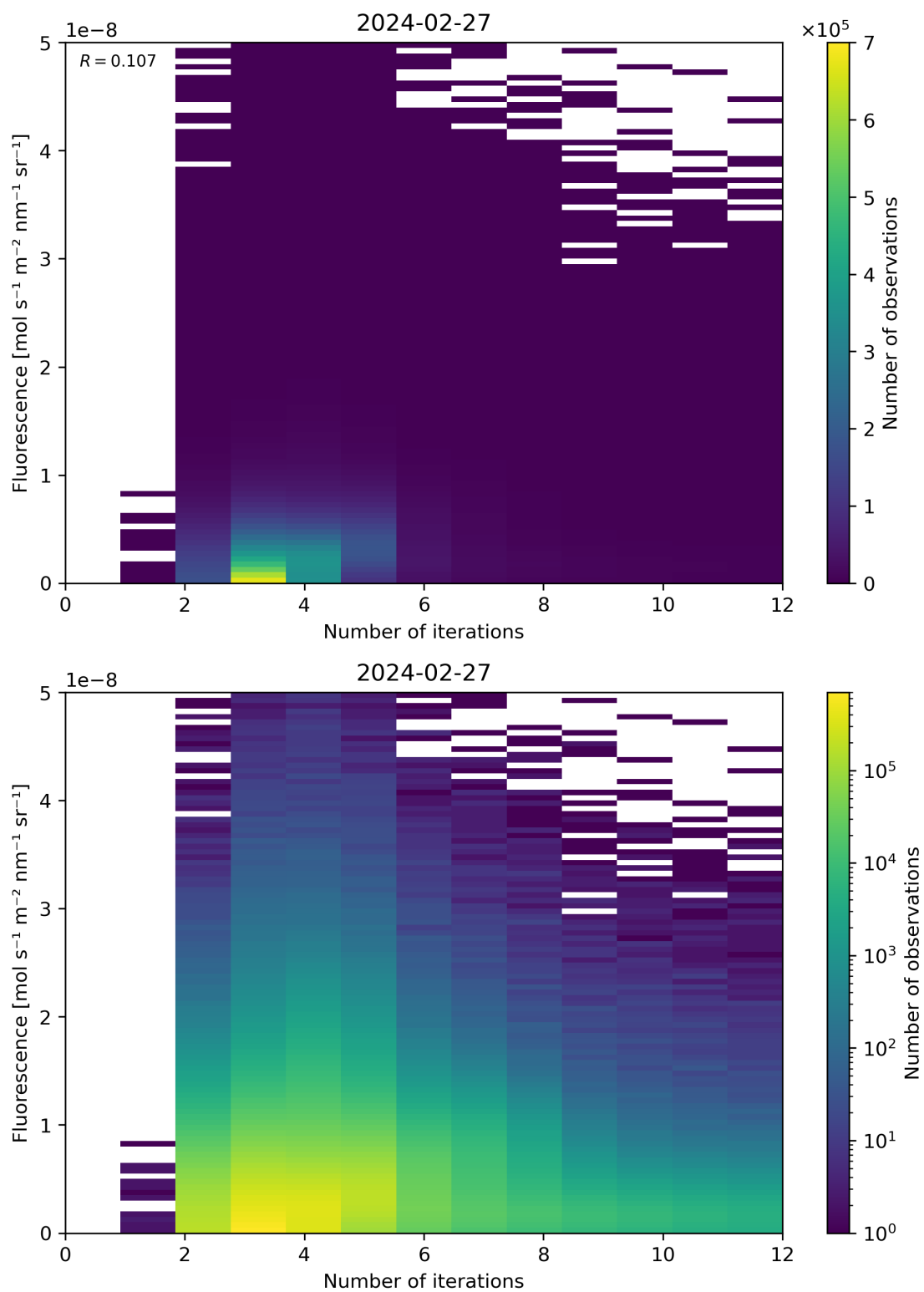
Figure 98: Scatter density plot of “Number of iterations” against “Fluorescence” for 2024-02-27 to 2024-02-28.
