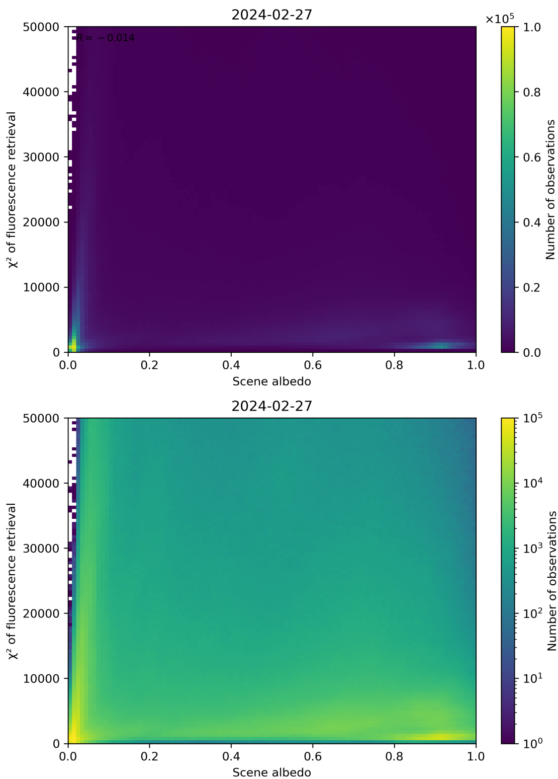
Figure 103: Scatter density plot of “Scene albedo” against “ \chi^2 of fluorescence retrieval” for 2024-02-27 to 2024-02-28.
