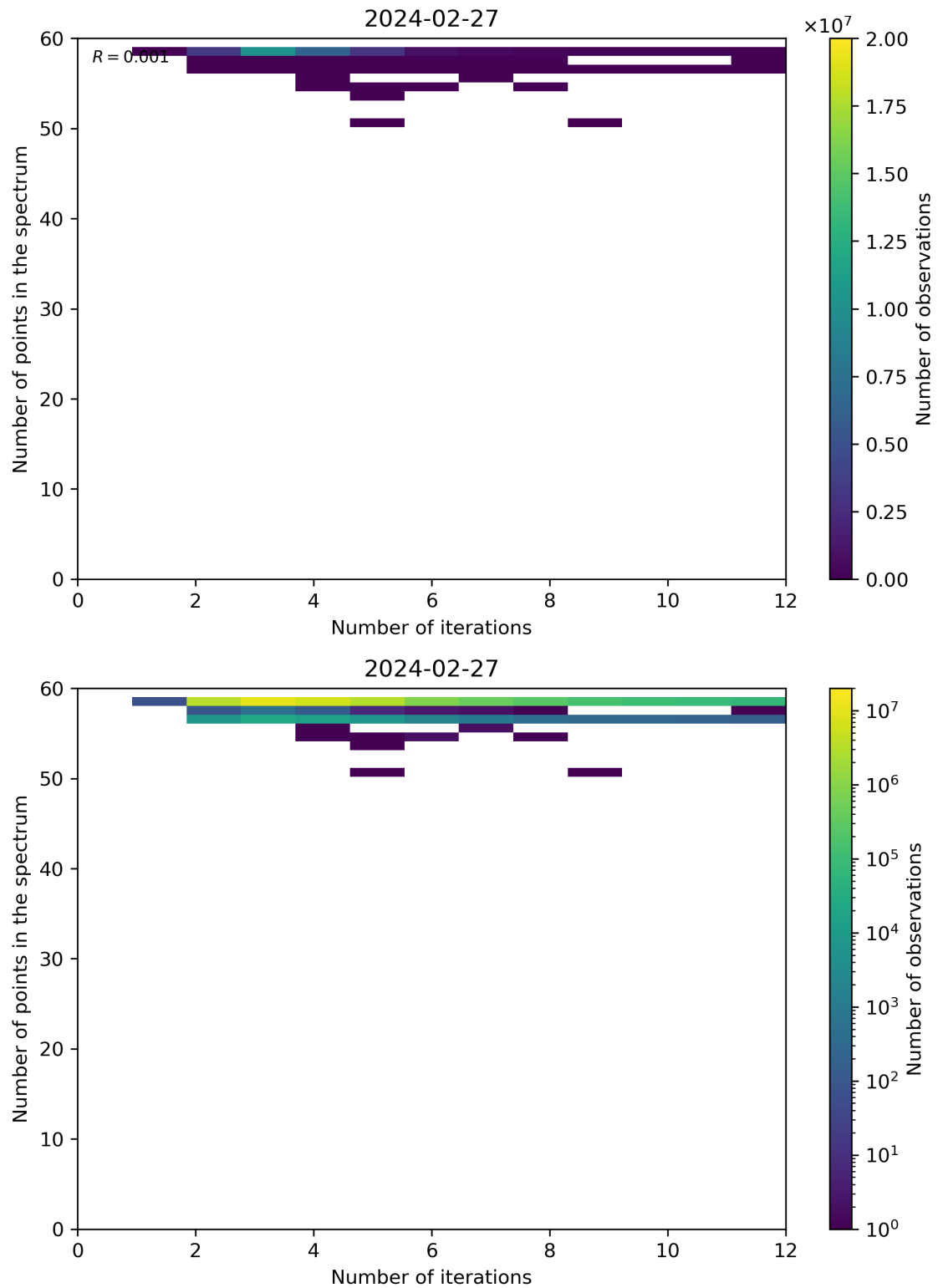
Figure 99: Scatter density plot of “Number of iterations” against “Number of points in the spectrum” for 2024-02-27 to 2024-02-28.
