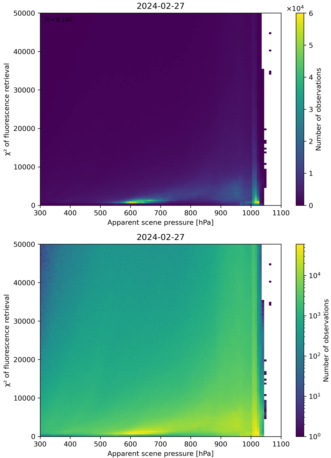
Figure 63: Scatter density plot of “Apparent scene pressure” against “ \chi^2 of fluorescence retrieval” for 2024-02-27 to 2024-02-28.
