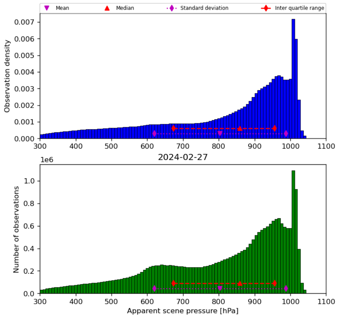
Figure 36: Histogram of “Apparent scene pressure” for 2024-02-27 to 2024-02-28
