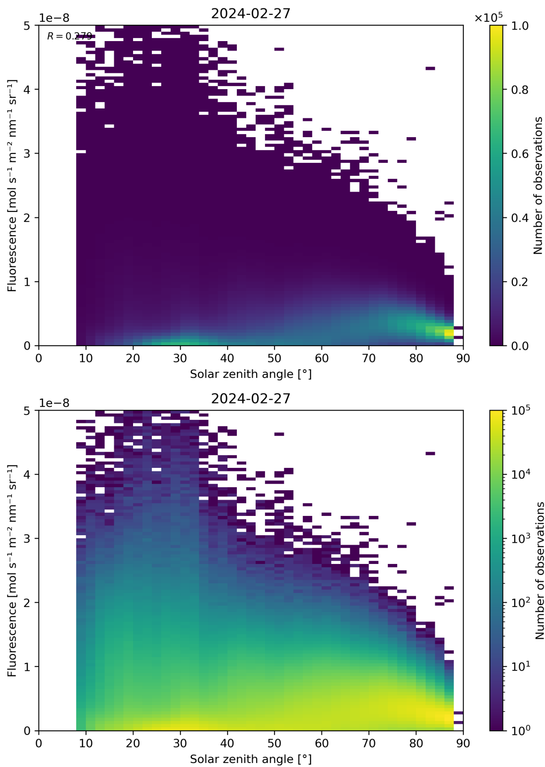
Figure 112: Scatter density plot of “Solar zenith angle” against “Fluorescence” for 2024-02-27 to 2024-02-28.
