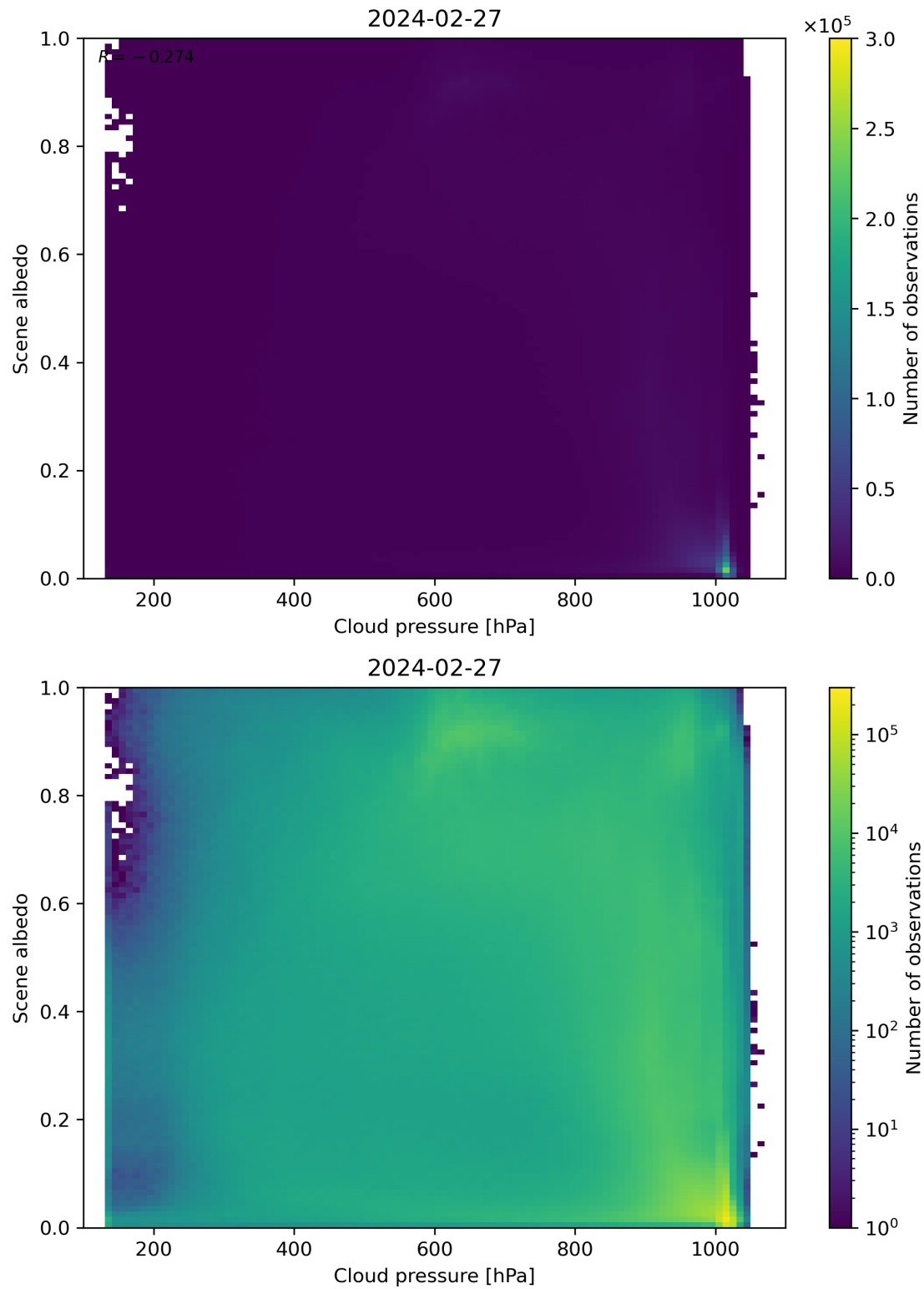
Figure 83: Scatter density plot of “Cloud pressure” against “Scene albedo” for 2024-02-27 to 2024-02-28.
