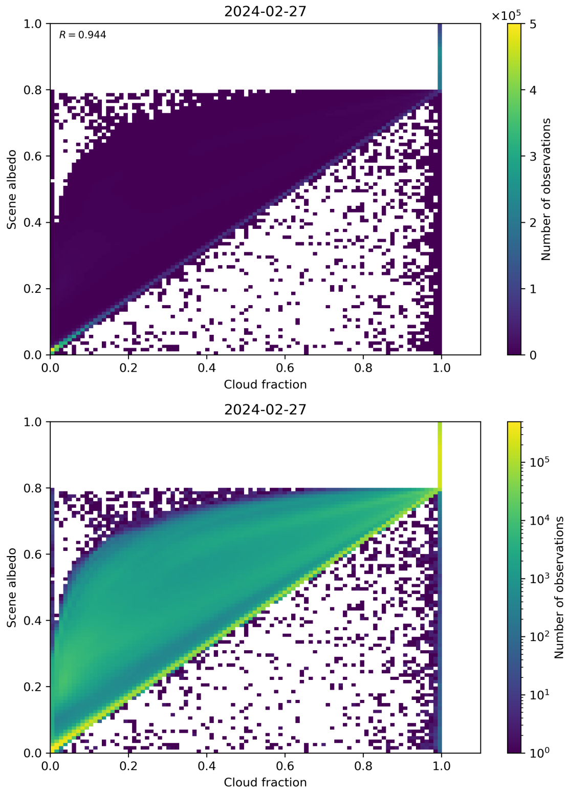
Figure 75: Scatter density plot of “Cloud fraction” against “Scene albedo” for 2024-02-27 to 2024-02-28.
