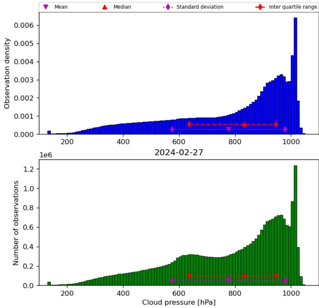
Figure 30: Histogram of “Cloud pressure” for 2024-02-27 to 2024-02-28
