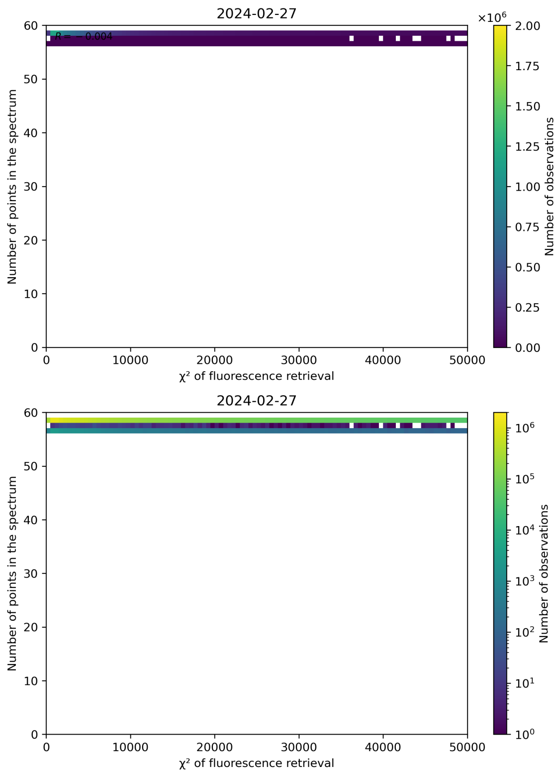
Figure 68: Scatter density plot of " \chi^2 of fluorescence retrieval" against "Number of points in the spectrum" for 2024-02-27 to 2024-02-28.
