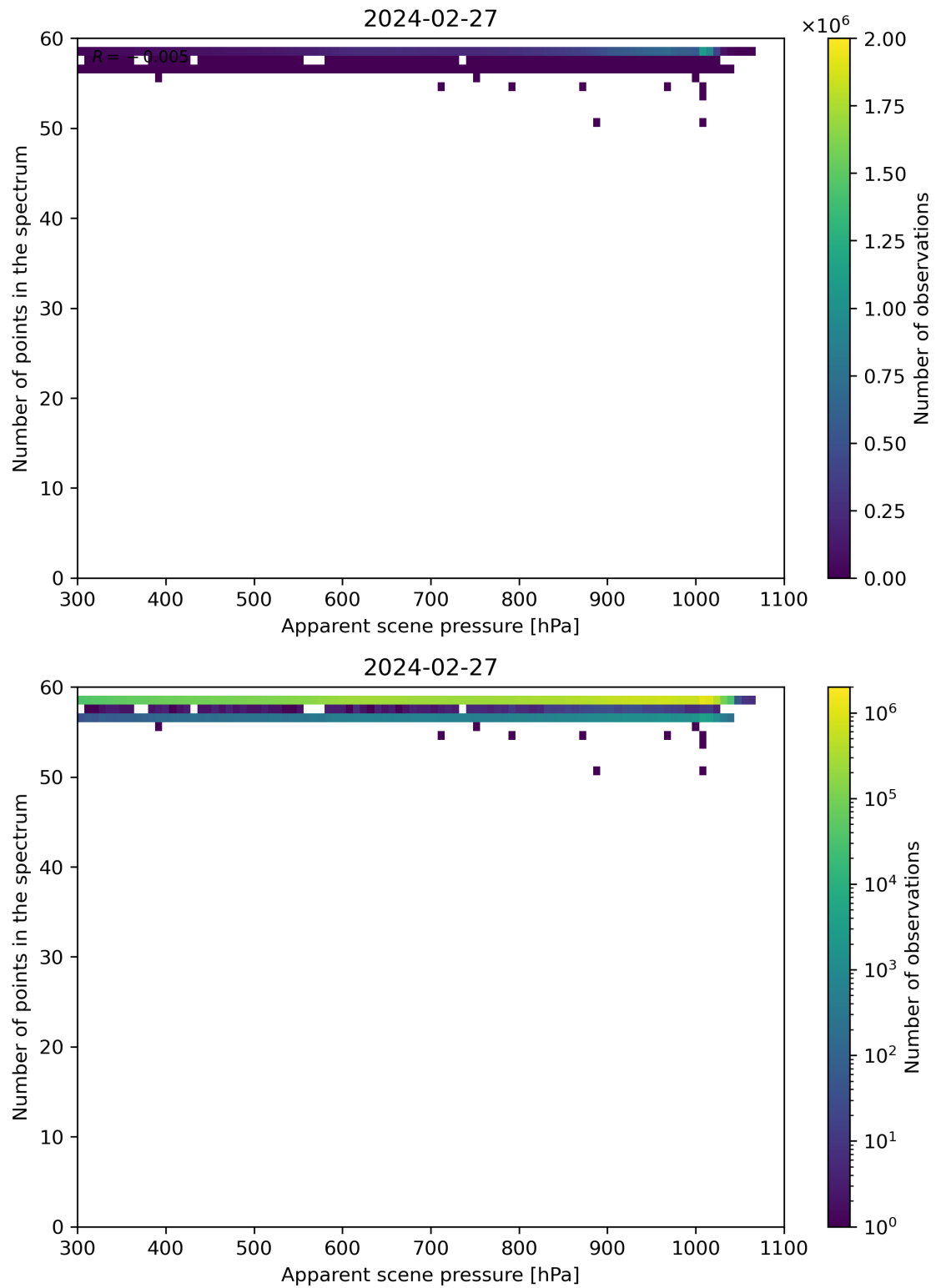
Figure 66: Scatter density plot of “Apparent scene pressure” against “Number of points in the spectrum” for 2024-02-27 to 2024-02-28.
