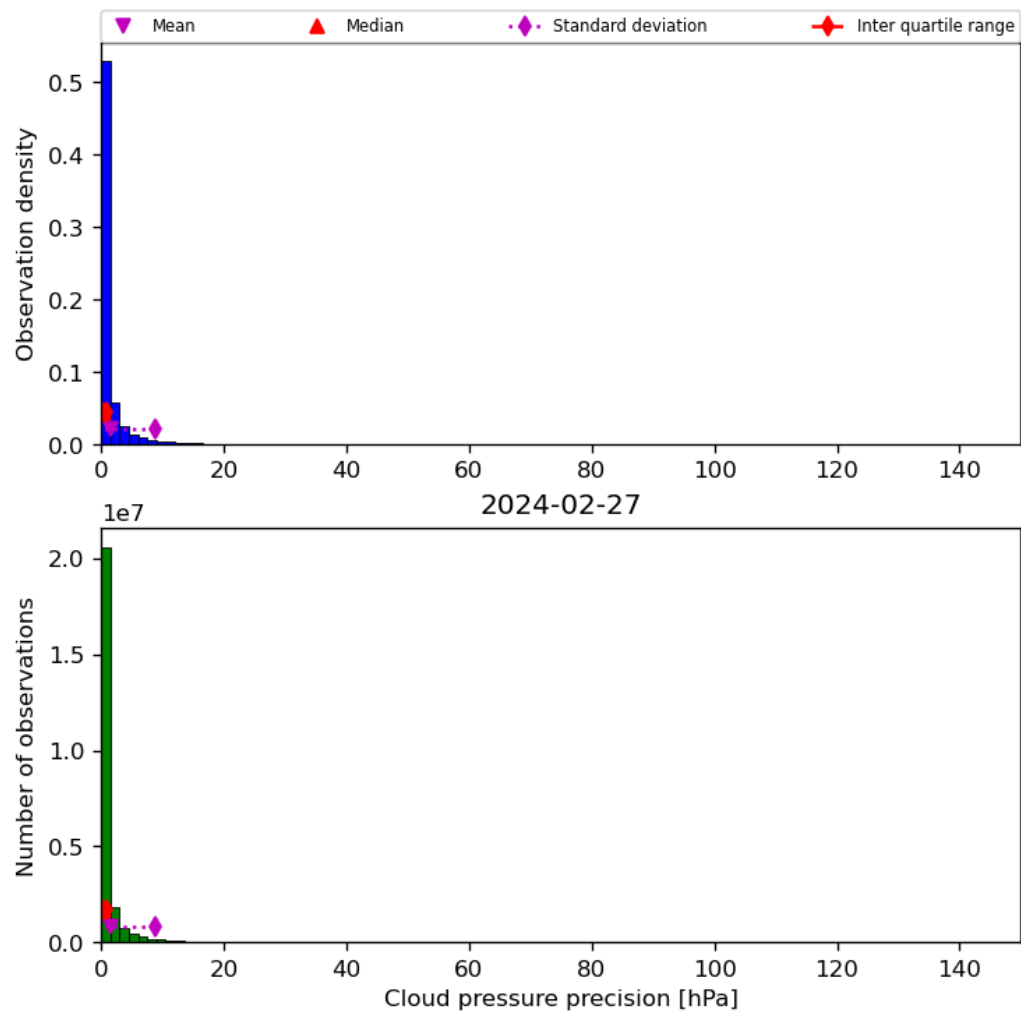
Figure 31: Histogram of “Cloud pressure precision” for 2024-02-27 to 2024-02-28
