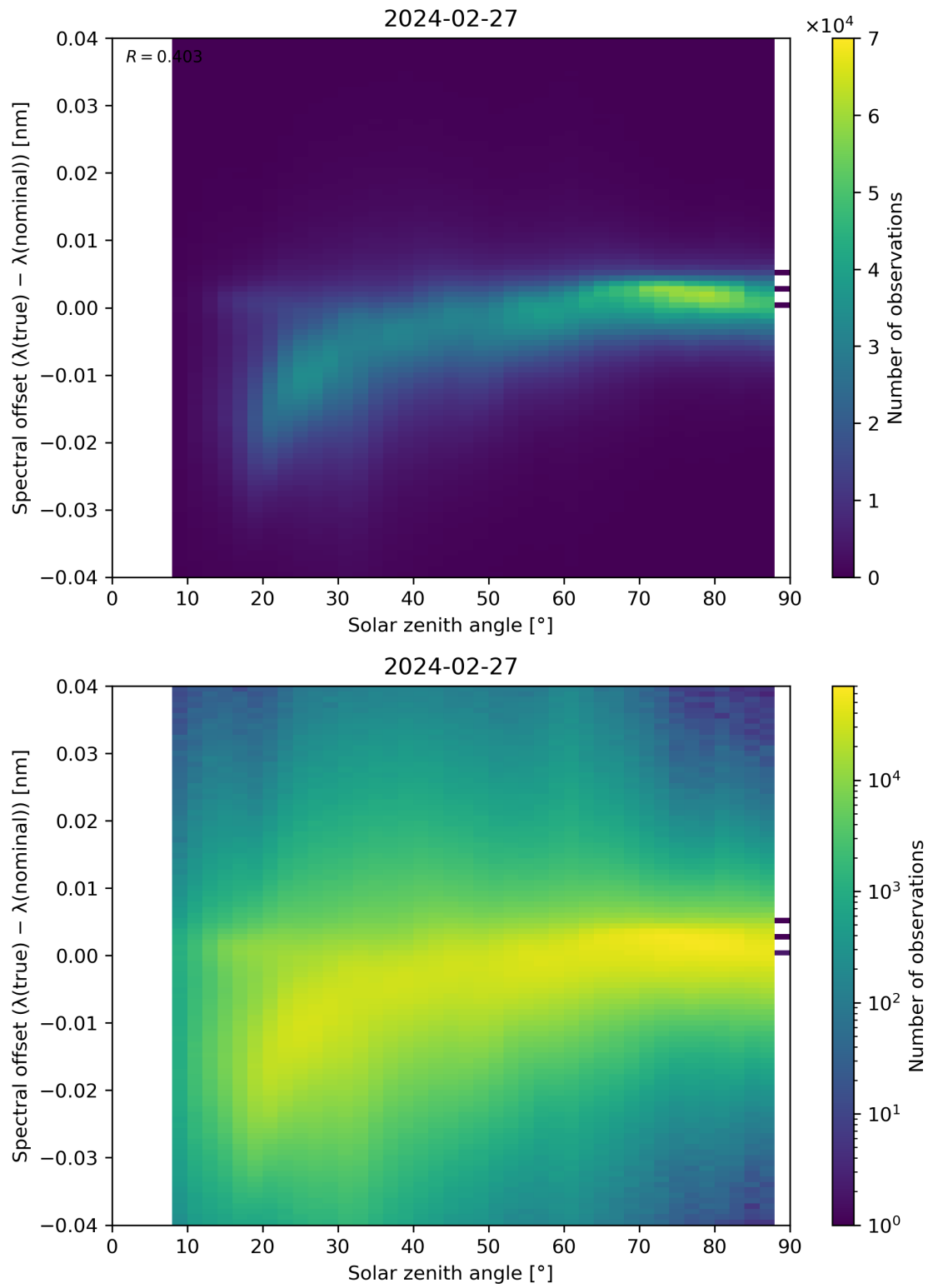
Figure 117: Scatter density plot of “Solar zenith angle” against “Spectral offset ( \lambda(\text{true}) - \lambda(\text{nominal}) )” for 2024-02-27 to 2024-02-28.
