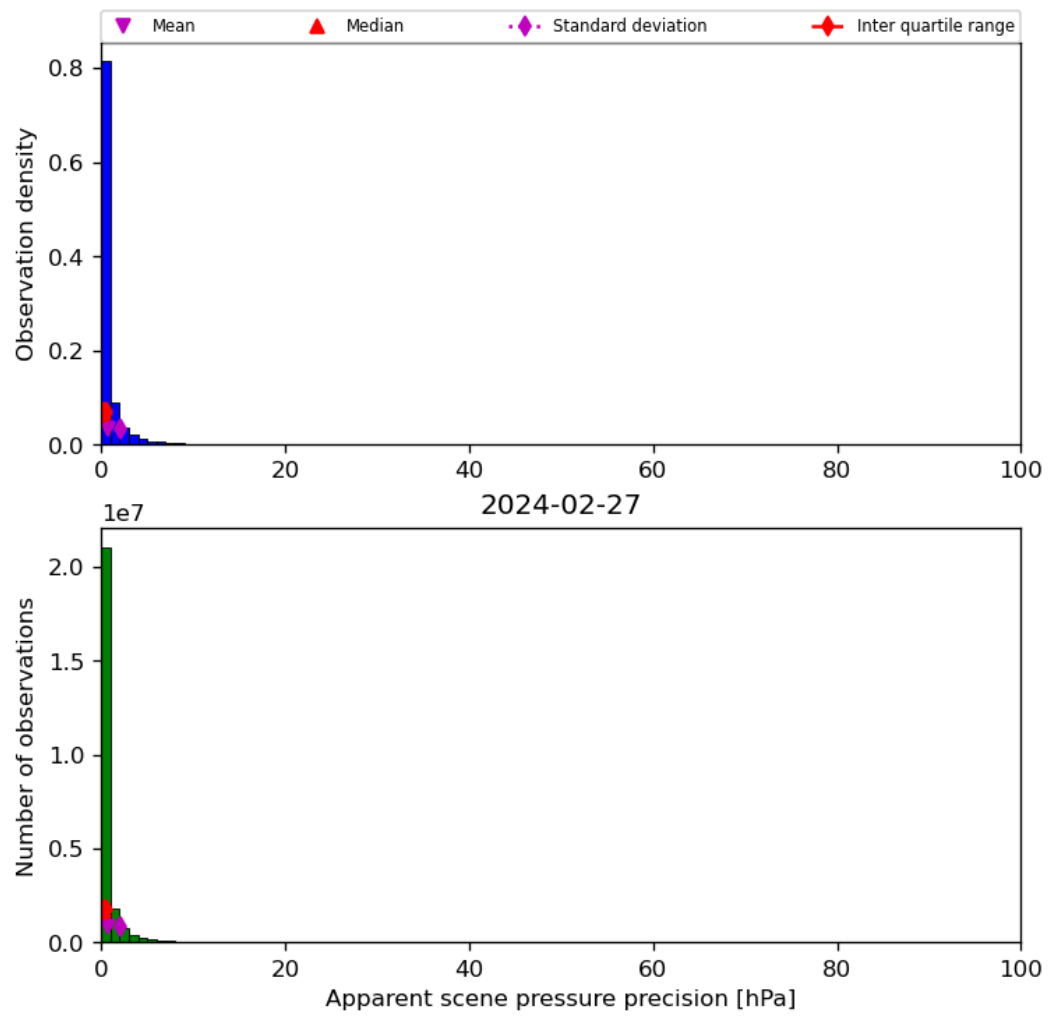
Figure 37: Histogram of “Apparent scene pressure precision” for 2024-02-27 to 2024-02-28
