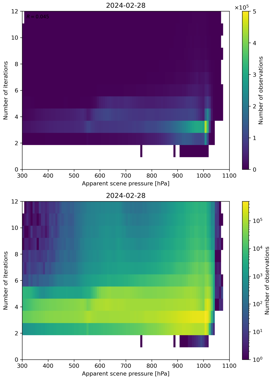
Figure 65: Scatter density plot of “Apparent scene pressure” against “Number of iterations” for 2024-02-27 to 2024-02-29.
