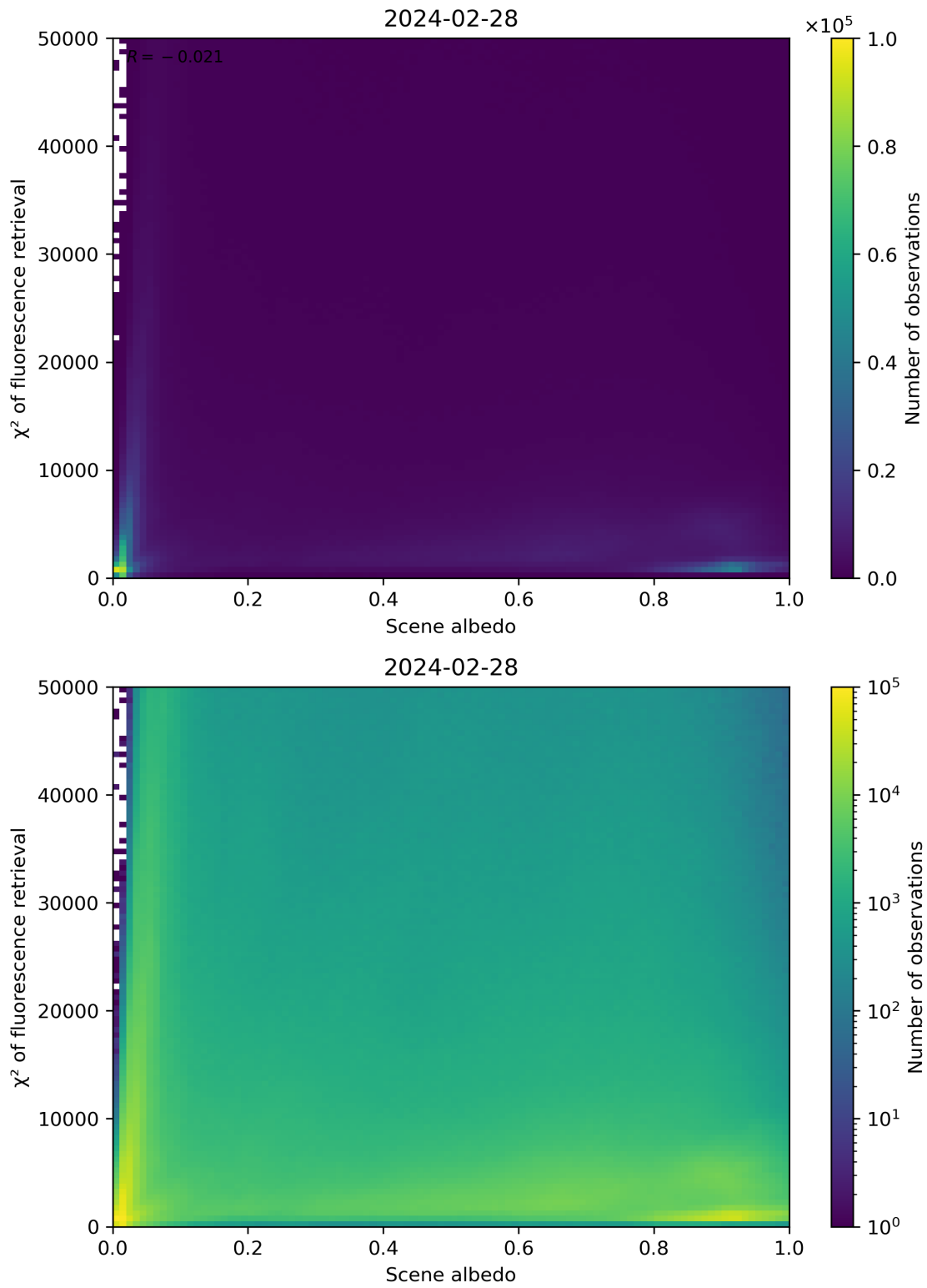
Figure 103: Scatter density plot of “Scene albedo” against “ \chi^2 of fluorescence retrieval” for 2024-02-27 to 2024-02-29.
