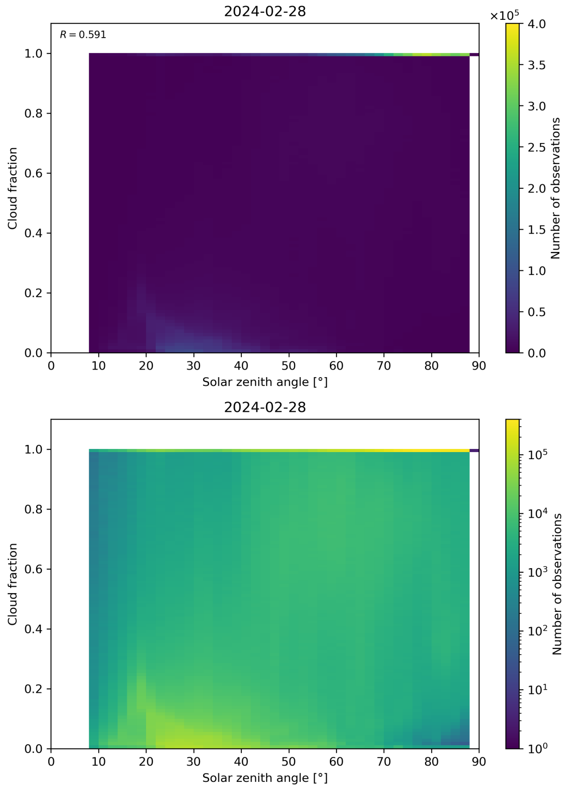
Figure 110: Scatter density plot of “Solar zenith angle” against “Cloud fraction” for 2024-02-27 to 2024-02-29.
