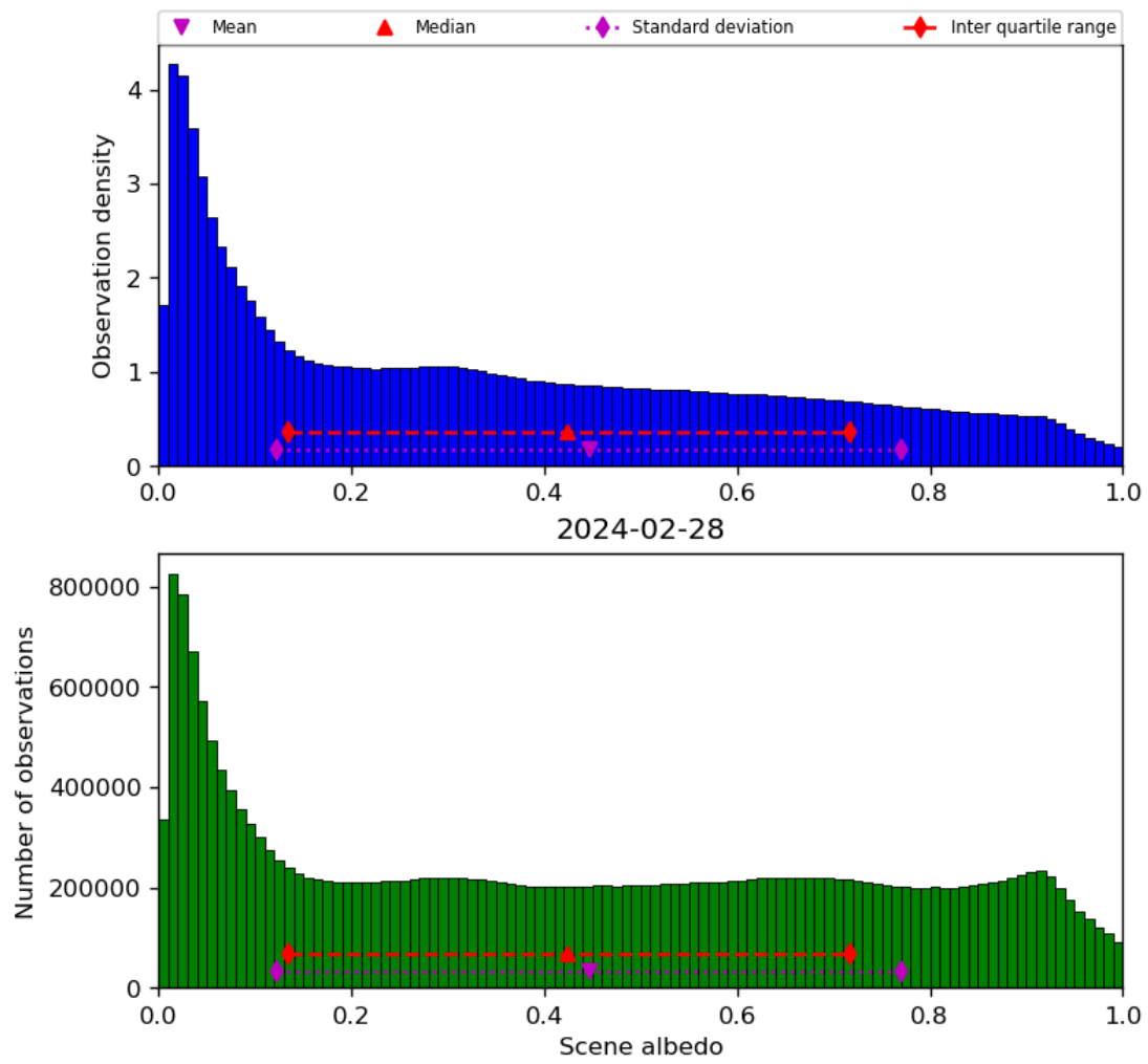
Figure 34: Histogram of “Scene albedo” for 2024-02-27 to 2024-02-29
