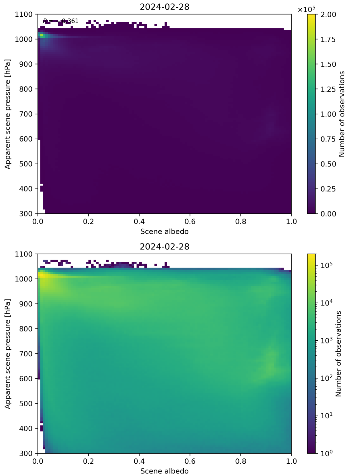
Figure 102: Scatter density plot of “Scene albedo” against “Apparent scene pressure” for 2024-02-27 to 2024-02-29.
