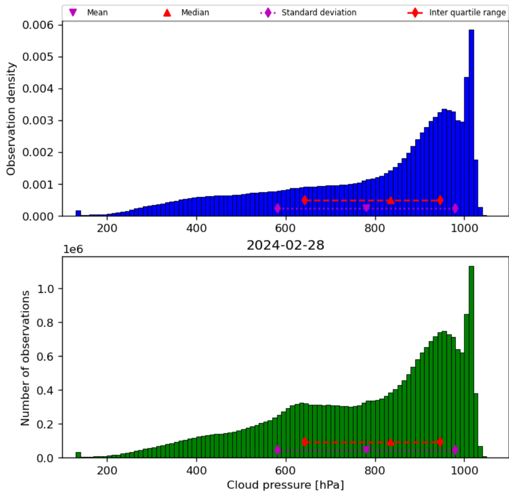
Figure 30: Histogram of “Cloud pressure” for 2024-02-27 to 2024-02-29
