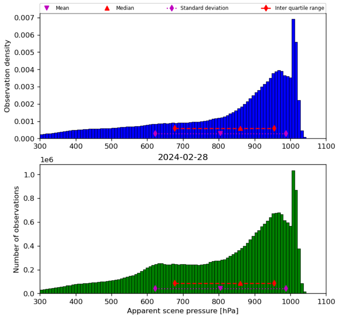
Figure 36: Histogram of “Apparent scene pressure” for 2024-02-27 to 2024-02-29
