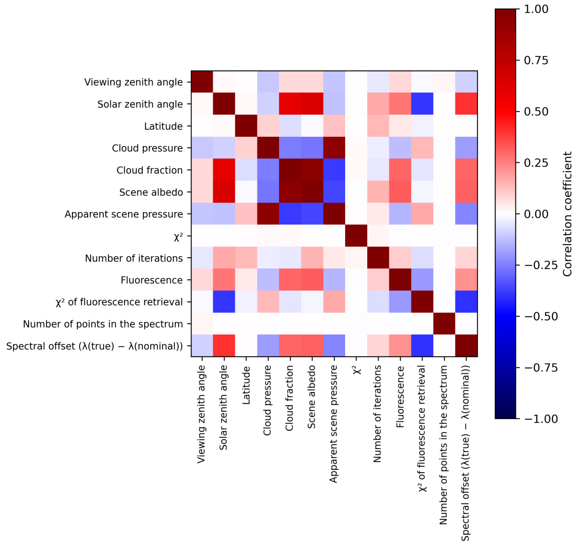
Figure 2: Map of correlation matrix for 2024-02-27 to 2024-02-29.
