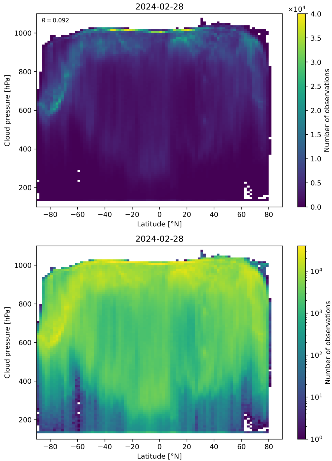
Figure 91: Scatter density plot of “Latitude” against “Cloud pressure” for 2024-02-27 to 2024-02-29.
