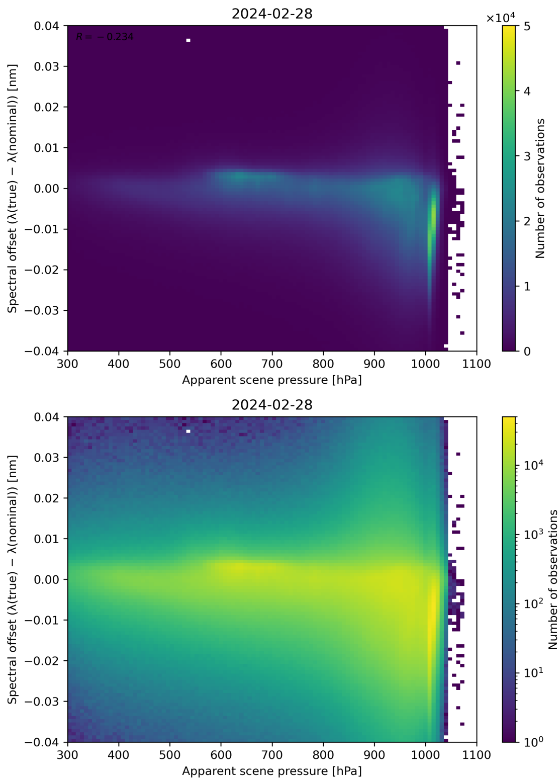
Figure 67: Scatter density plot of “Apparent scene pressure” against “Spectral offset ( \lambda(\text{true}) - \lambda(\text{nominal}) )” for 2024-02-27 to 2024-02-29.
