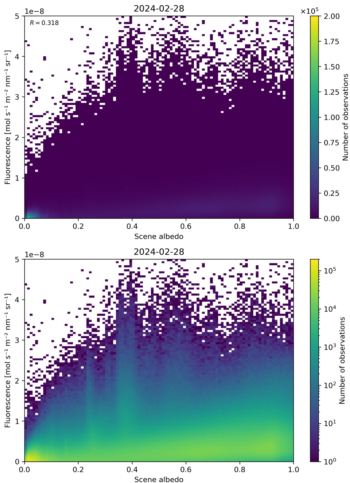
Figure 104: Scatter density plot of “Scene albedo” against “Fluorescence” for 2024-02-27 to 2024-02-29.
