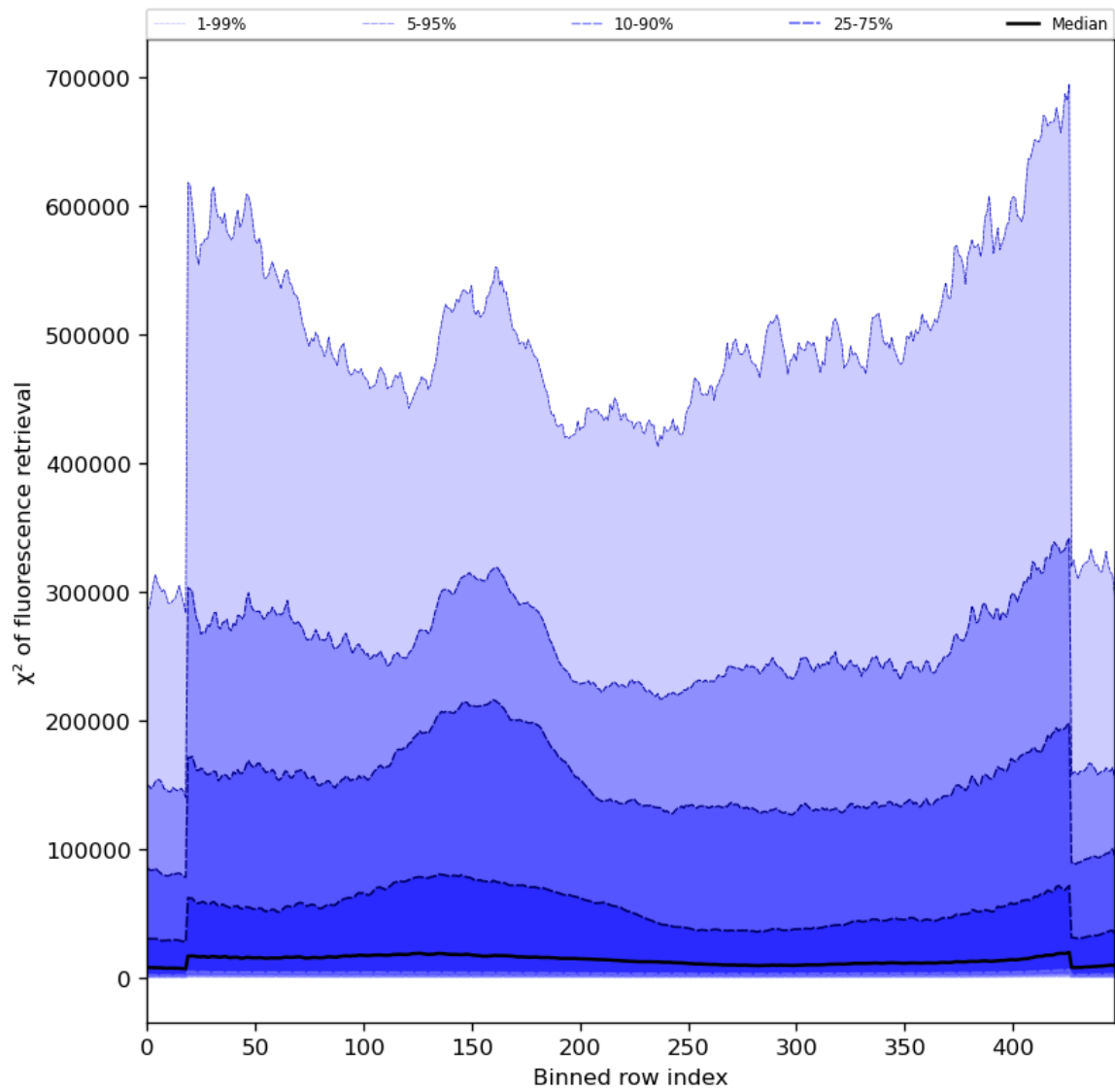
Figure 59: Along track statistics of “ \chi^2 of fluorescence retrieval” for 2024-02-27 to 2024-02-29
