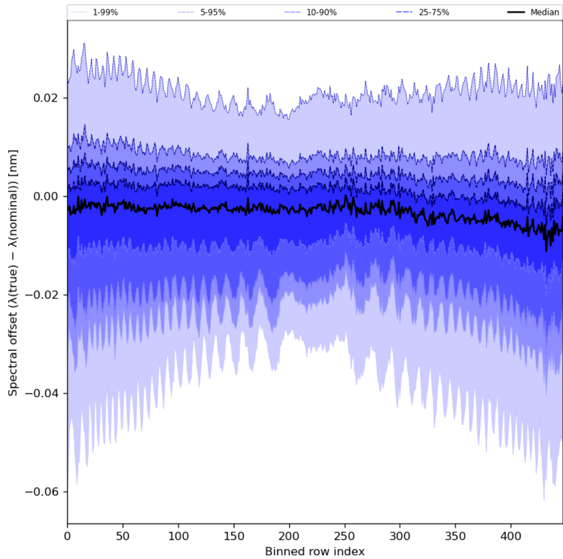
Figure 62: Along track statistics of “Spectral offset ( \lambda(\text{true}) - \lambda(\text{nominal}) )” for 2024-02-27 to 2024-02-29
