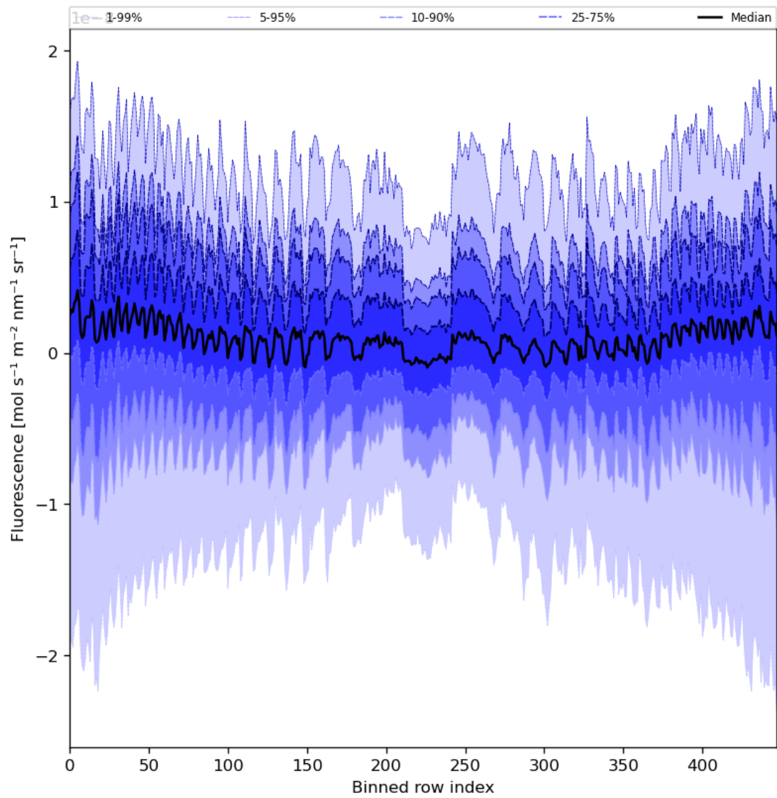
Figure 57: Along track statistics of “Fluorescence” for 2024-02-27 to 2024-02-29
