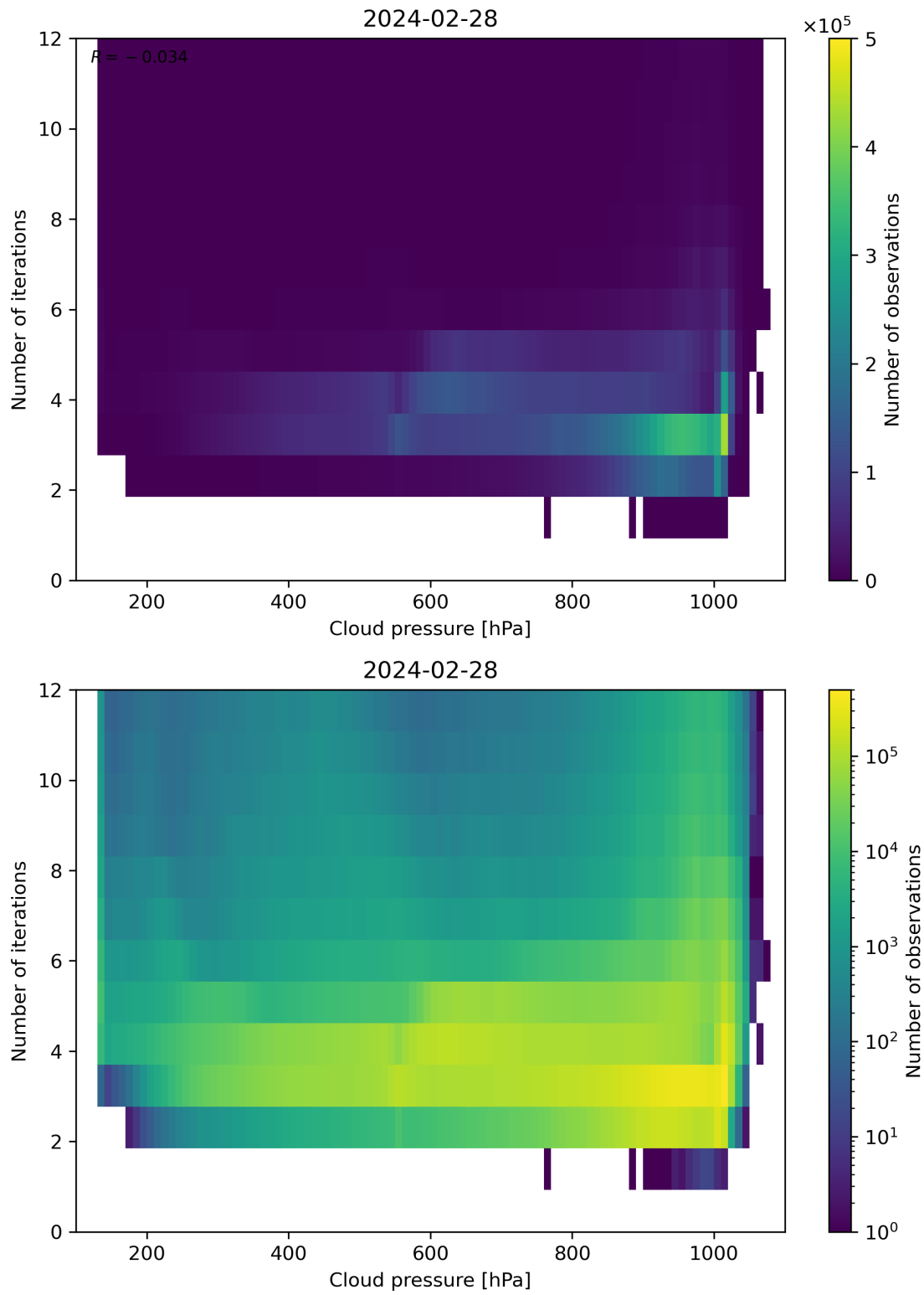
Figure 81: Scatter density plot of “Cloud pressure” against “Number of iterations” for 2024-02-27 to 2024-02-29.
