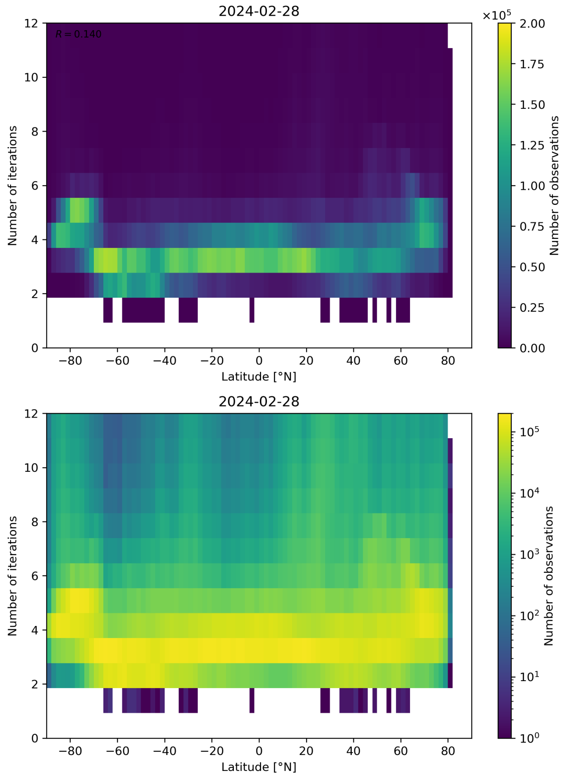
Figure 93: Scatter density plot of “Latitude” against “Number of iterations” for 2024-02-27 to 2024-02-29.
