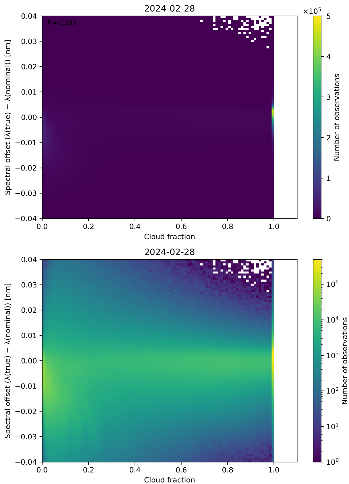
Figure 76: Scatter density plot of “Cloud fraction” against “Spectral offset ( \lambda(\text{true}) - \lambda(\text{nominal}) )” for 2024-02-27 to 2024-02-29.
