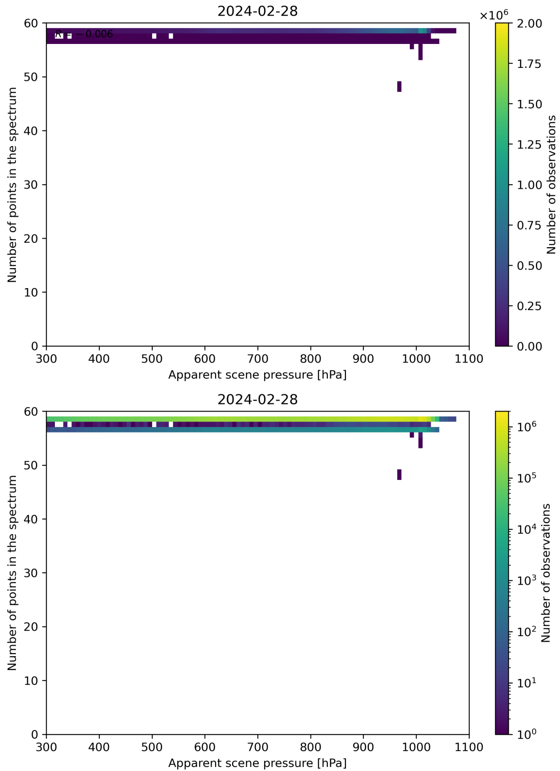
Figure 66: Scatter density plot of “Apparent scene pressure” against “Number of points in the spectrum” for 2024-02-27 to 2024-02-29.
