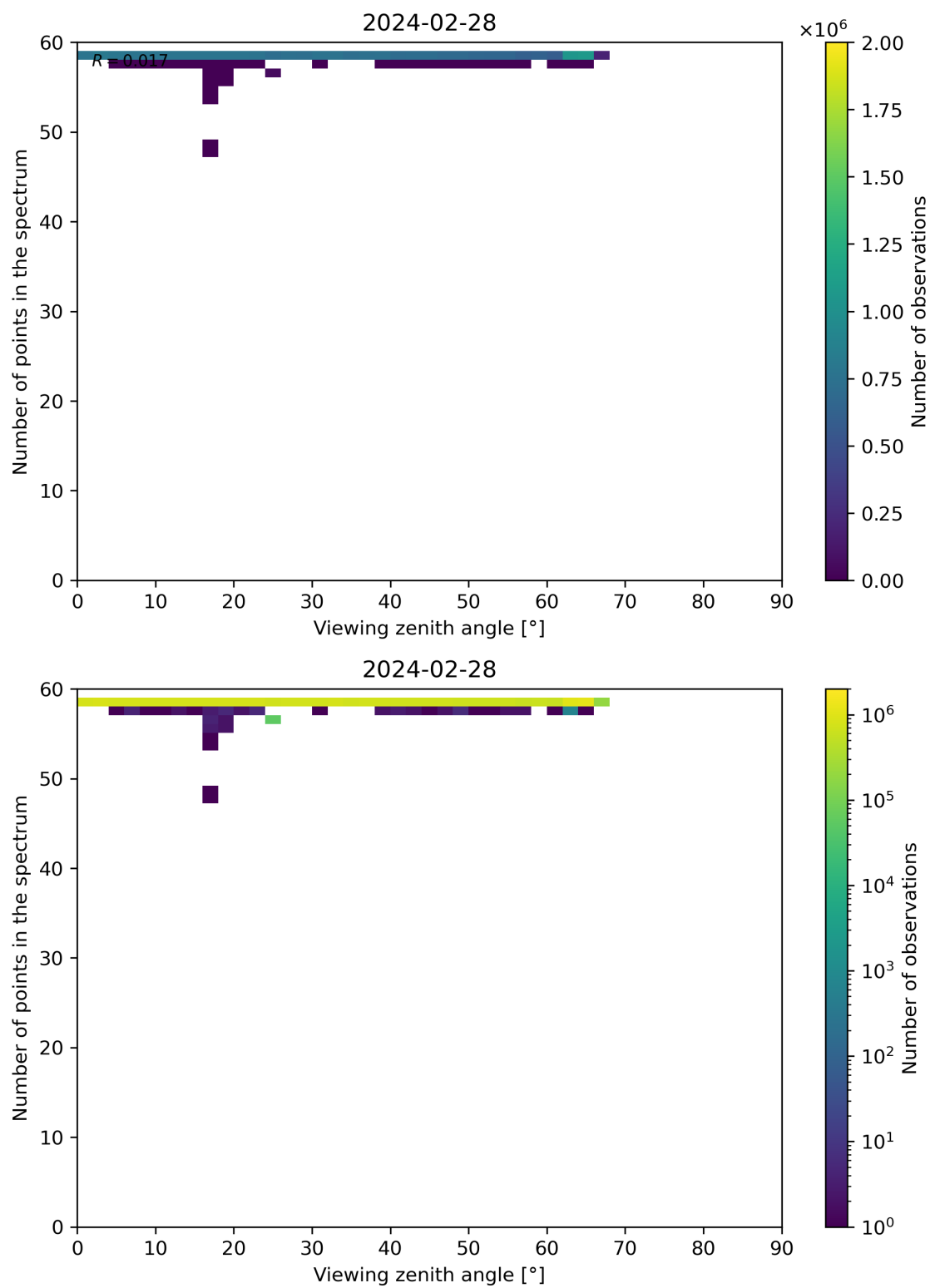
Figure 125: Scatter density plot of “Viewing zenith angle” against “Number of points in the spectrum” for 2024-02-27 to 2024-02-29.
