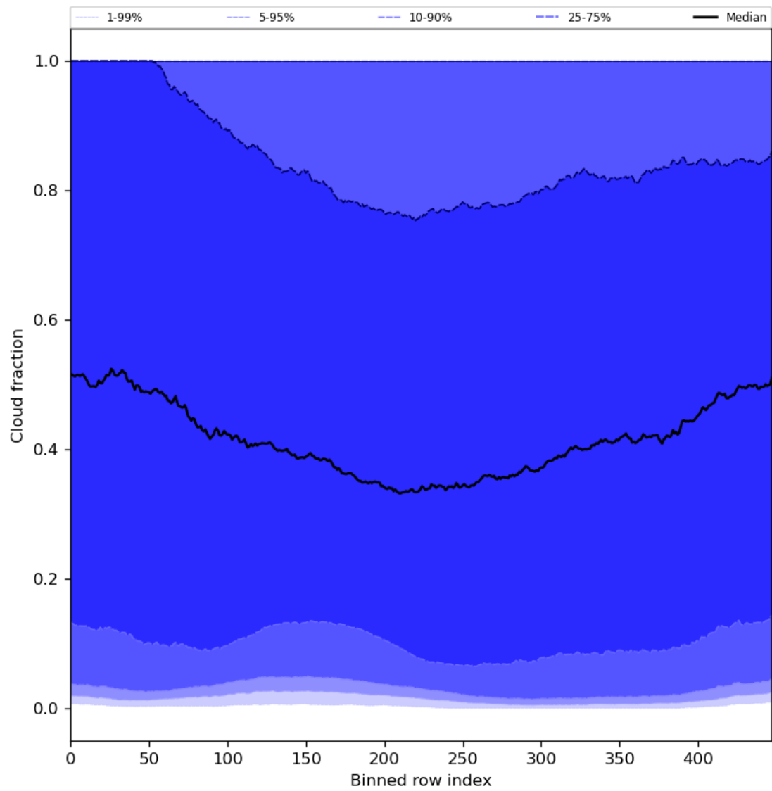
Figure 49: Along track statistics of “Cloud fraction” for 2024-02-27 to 2024-02-29
