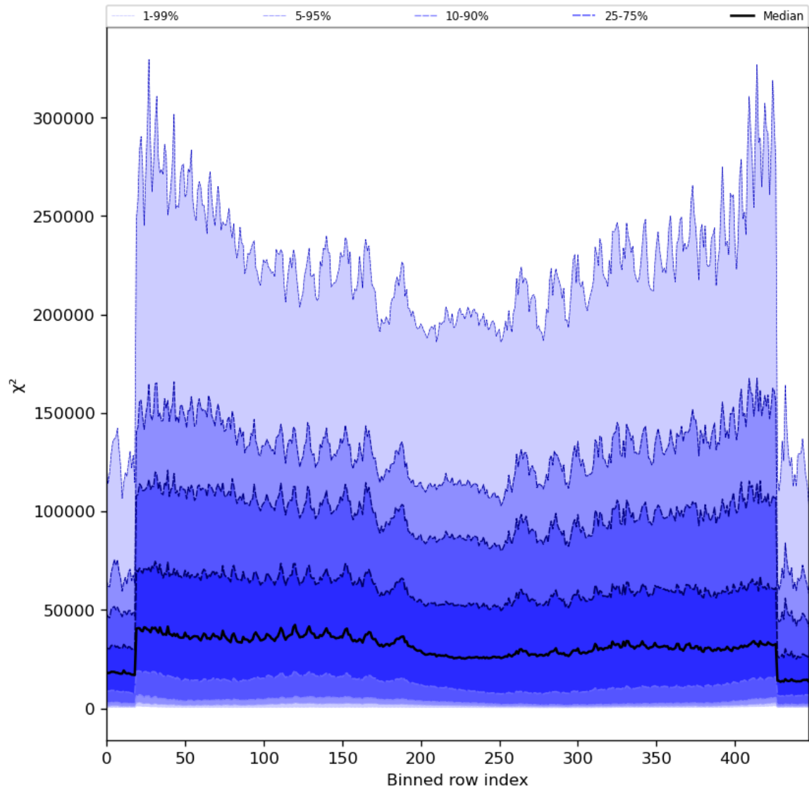
Figure 55: Along track statistics of “ \chi^2 ” for 2024-02-27 to 2024-02-29
