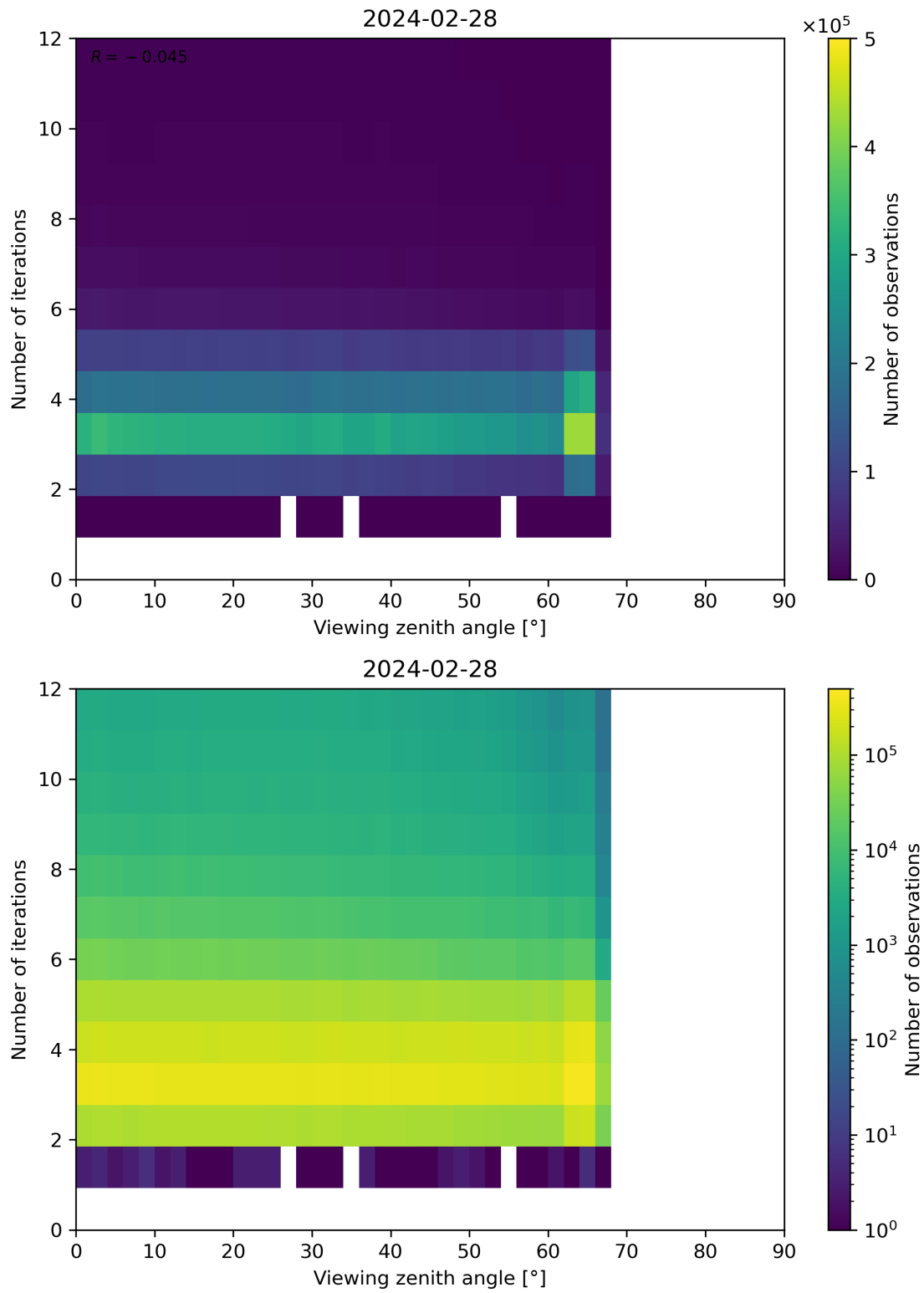
Figure 124: Scatter density plot of “Viewing zenith angle” against “Number of iterations” for 2024-02-27 to 2024-02-29.
