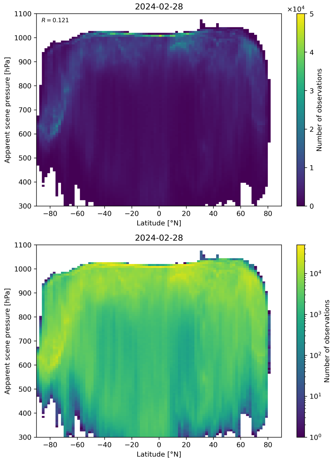
Figure 88: Scatter density plot of “Latitude” against “Apparent scene pressure” for 2024-02-27 to 2024-02-29.
