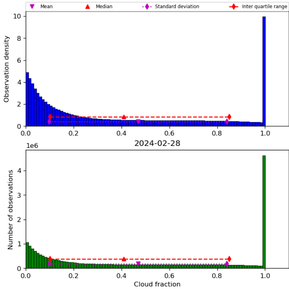
Figure 32: Histogram of “Cloud fraction” for 2024-02-27 to 2024-02-29
