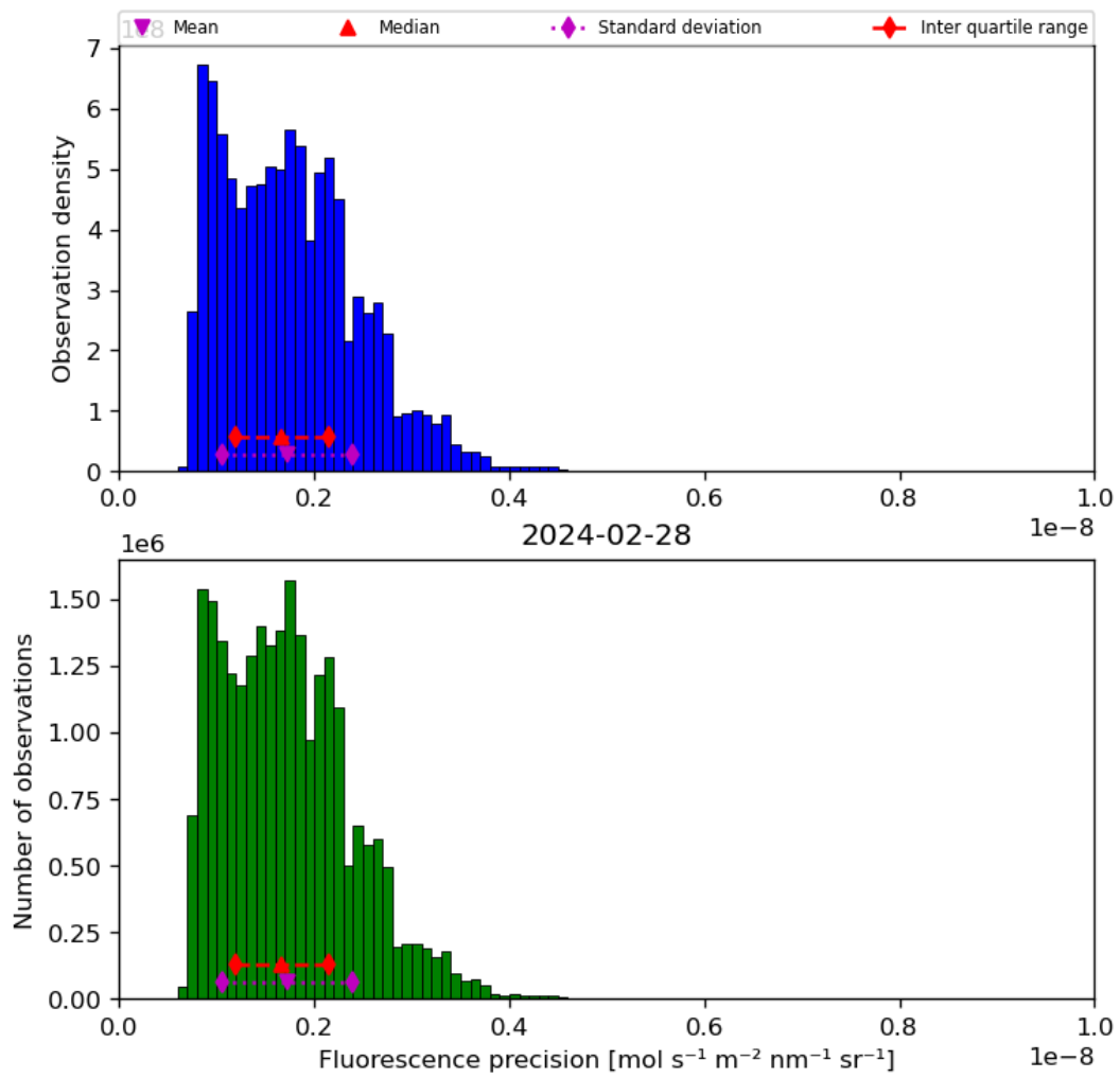
Figure 41: Histogram of “Fluorescence precision” for 2024-02-27 to 2024-02-29
