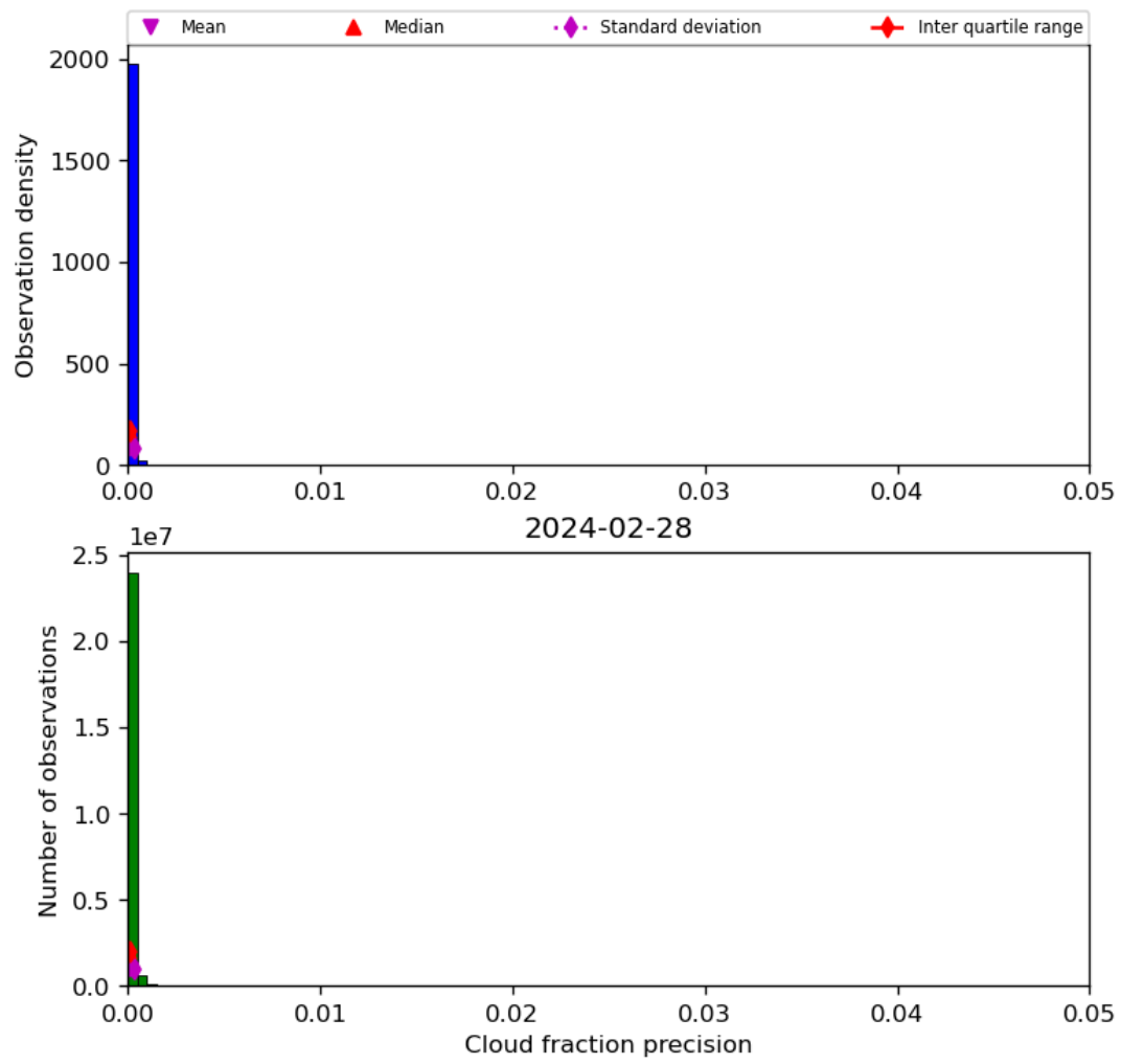
Figure 33: Histogram of “Cloud fraction precision” for 2024-02-27 to 2024-02-29
