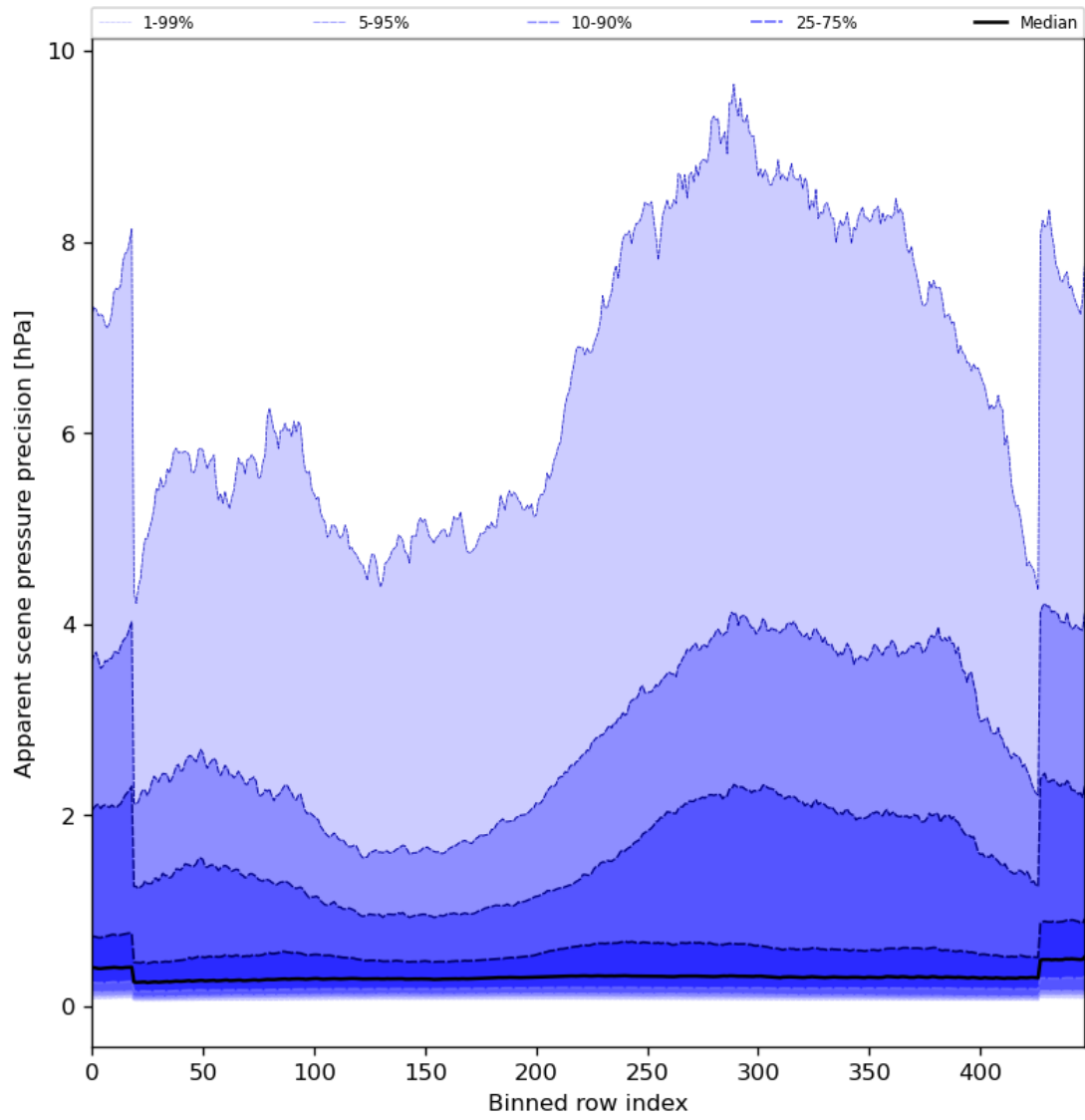
Figure 54: Along track statistics of “Apparent scene pressure precision” for 2024-02-27 to 2024-02-29
