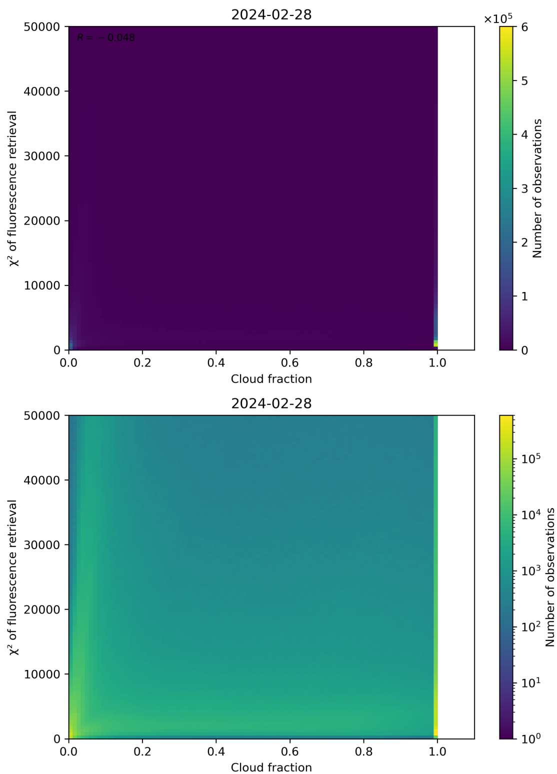
Figure 71: Scatter density plot of “Cloud fraction” against “ \chi^2 of fluorescence retrieval” for 2024-02-27 to 2024-02-29.
