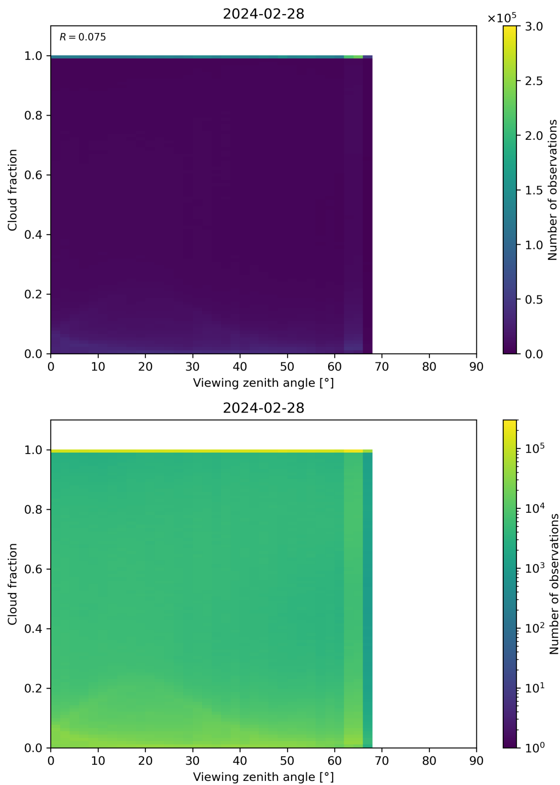
Figure 120: Scatter density plot of “Viewing zenith angle” against “Cloud fraction” for 2024-02-27 to 2024-02-29.
