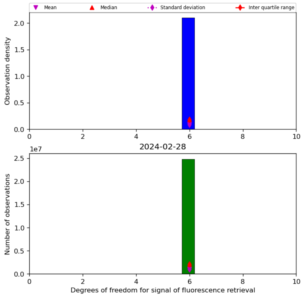
Figure 43: Histogram of “Degrees of freedom for signal of fluorescence retrieval” for 2024-02-27 to 2024-02-29
