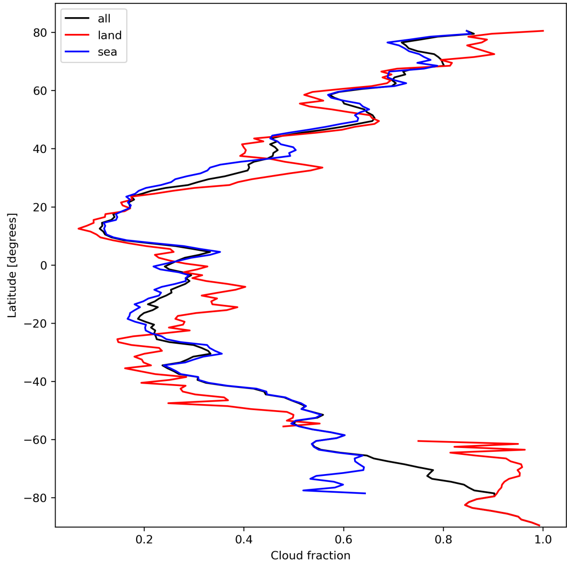
Figure 15: Zonal average of “Cloud fraction” for 2024-02-27 to 2024-02-29.
