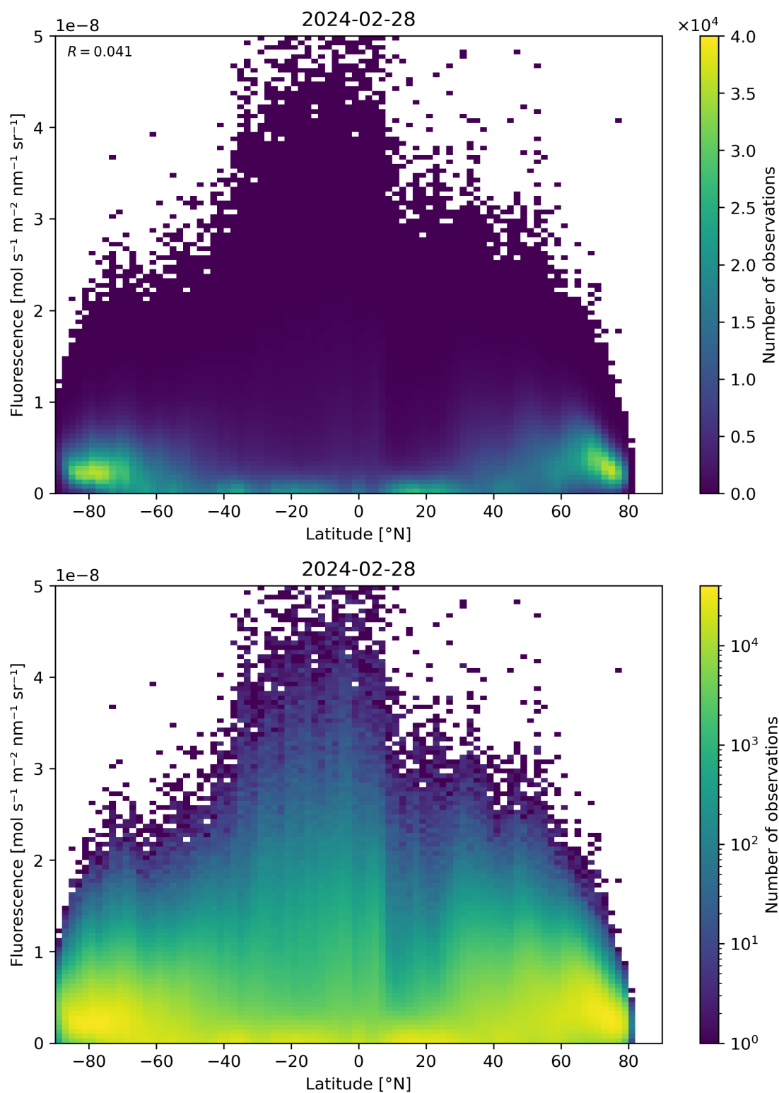
Figure 92: Scatter density plot of “Latitude” against “Fluorescence” for 2024-02-27 to 2024-02-29.
