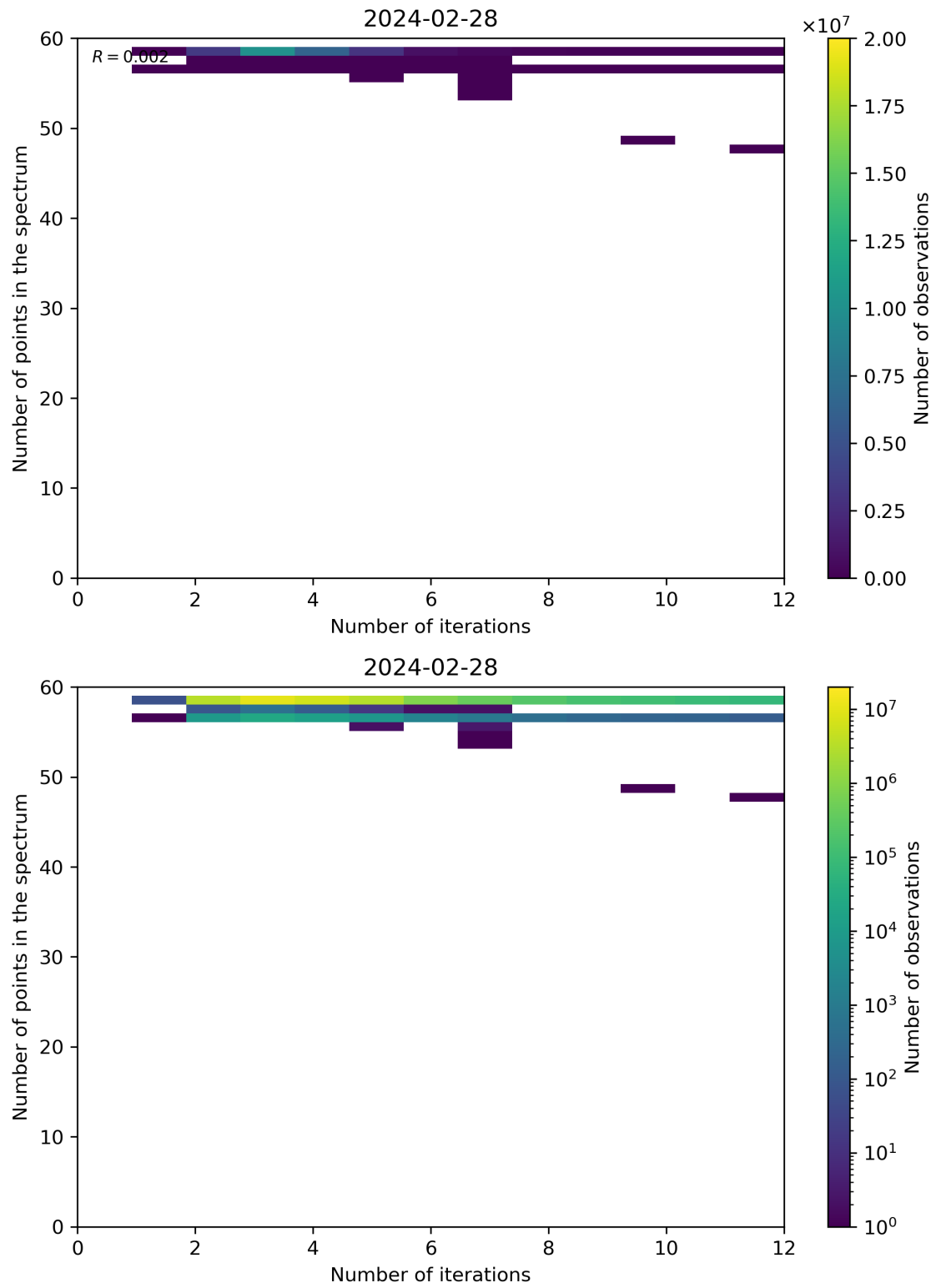
Figure 99: Scatter density plot of “Number of iterations” against “Number of points in the spectrum” for 2024-02-27 to 2024-02-29.
