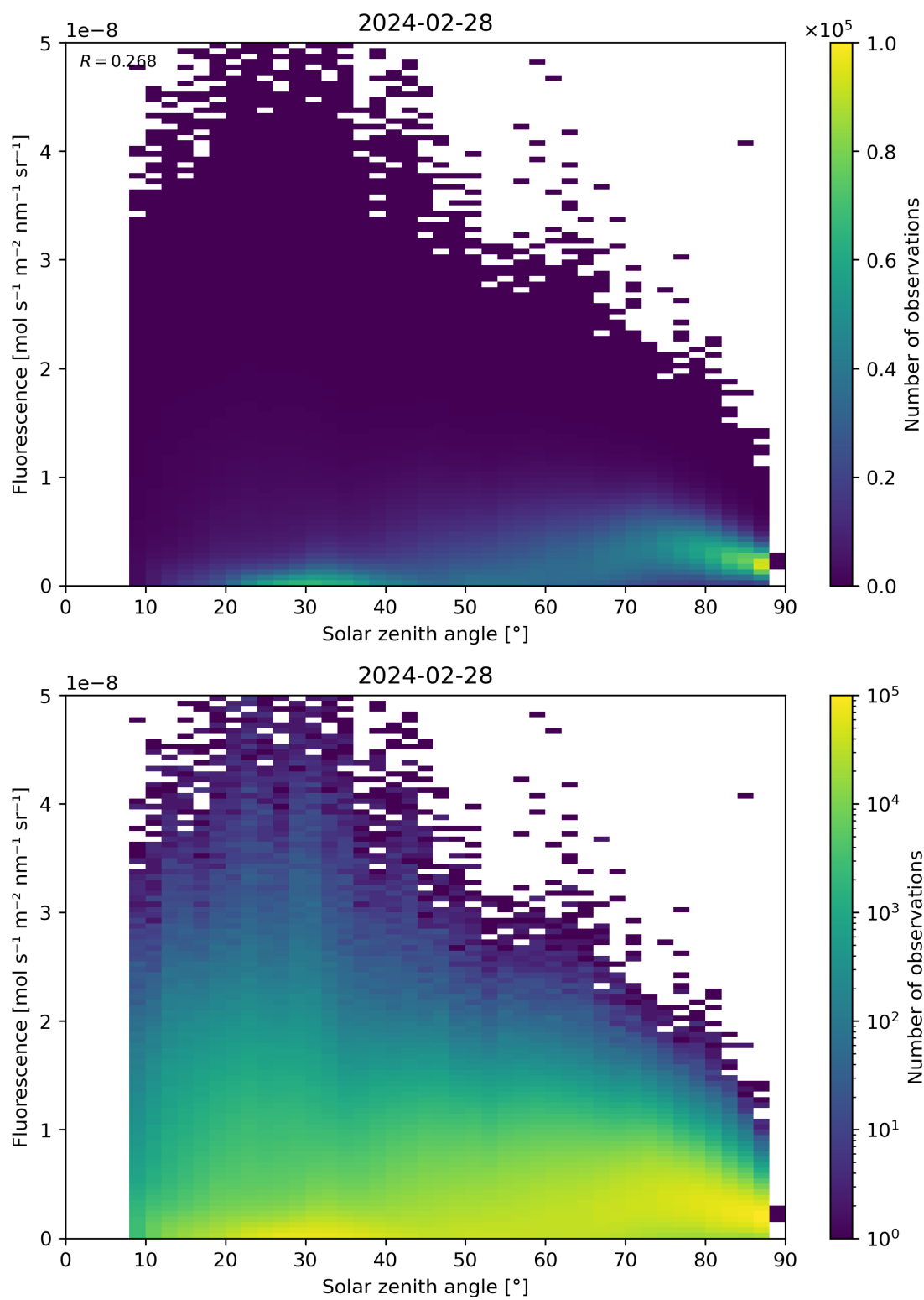
Figure 112: Scatter density plot of “Solar zenith angle” against “Fluorescence” for 2024-02-27 to 2024-02-29.
