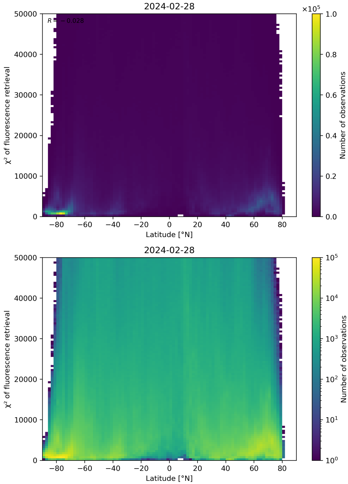
Figure 89: Scatter density plot of “Latitude” against “ \chi^2 of fluorescence retrieval” for 2024-02-27 to 2024-02-29.
