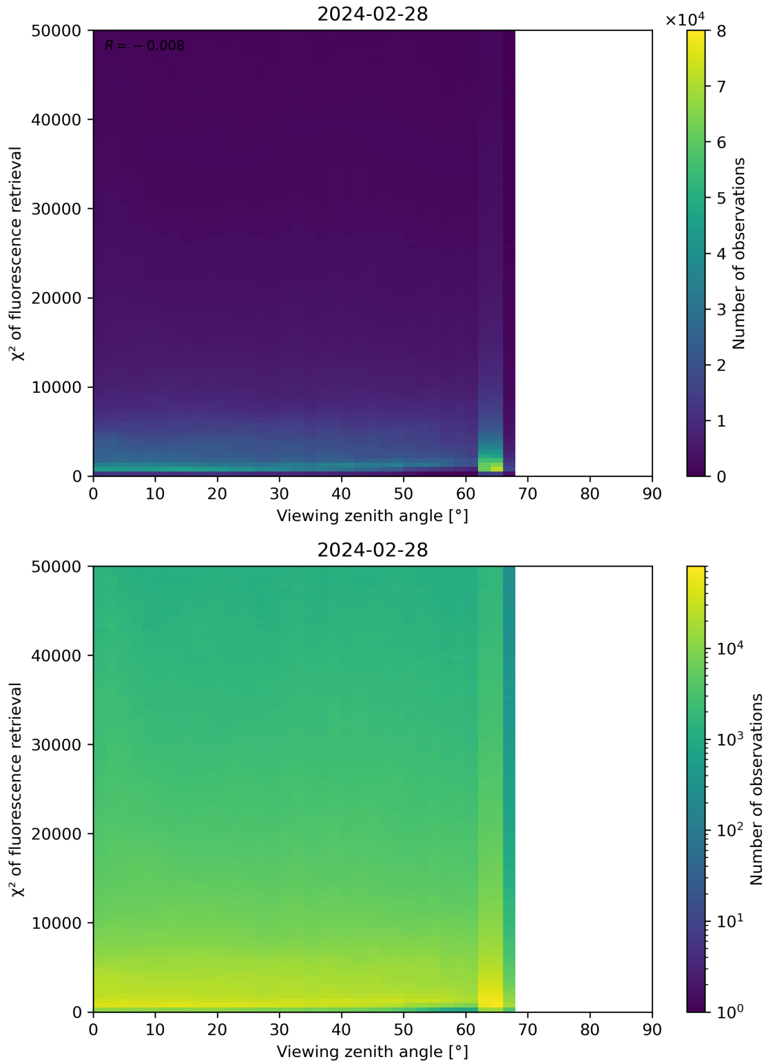
Figure 119: Scatter density plot of “Viewing zenith angle” against “ \chi^2 of fluorescence retrieval” for 2024-02-27 to 2024-02-29.
