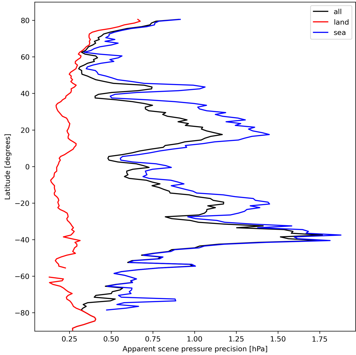
Figure 20: Zonal average of “Apparent scene pressure precision” for 2024-02-27 to 2024-02-29.
