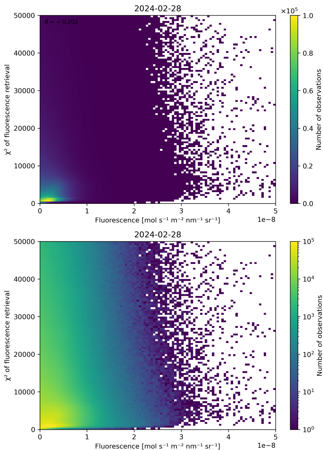
Figure 85: Scatter density plot of “Fluorescence” against “ \chi^2 of fluorescence retrieval” for 2024-02-27 to 2024-02-29.
