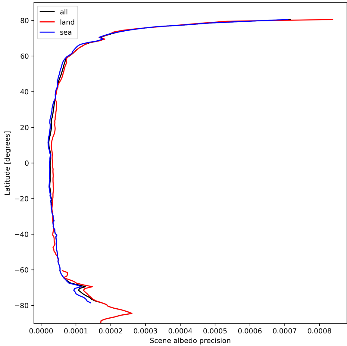
Figure 18: Zonal average of “Scene albedo precision” for 2024-02-27 to 2024-02-29.
