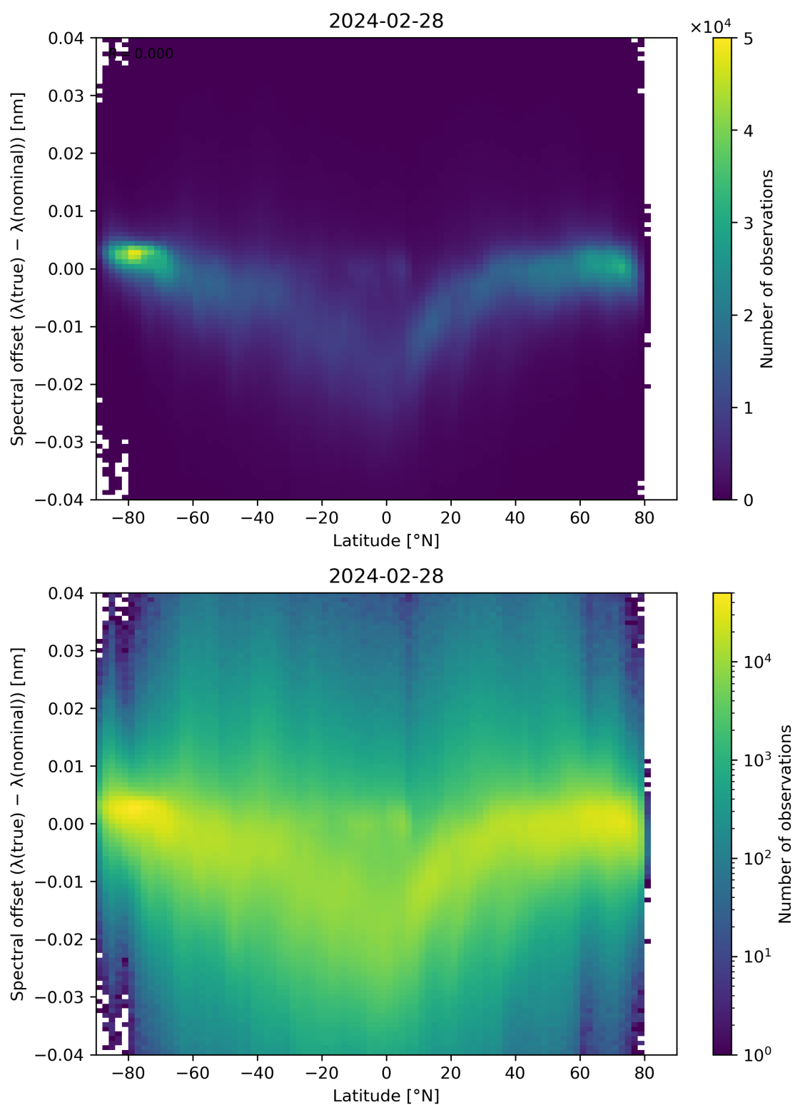
Figure 96: Scatter density plot of “Latitude” against “Spectral offset ( \lambda(\text{true}) - \lambda(\text{nominal}) )” for 2024-02-27 to 2024-02-29.
