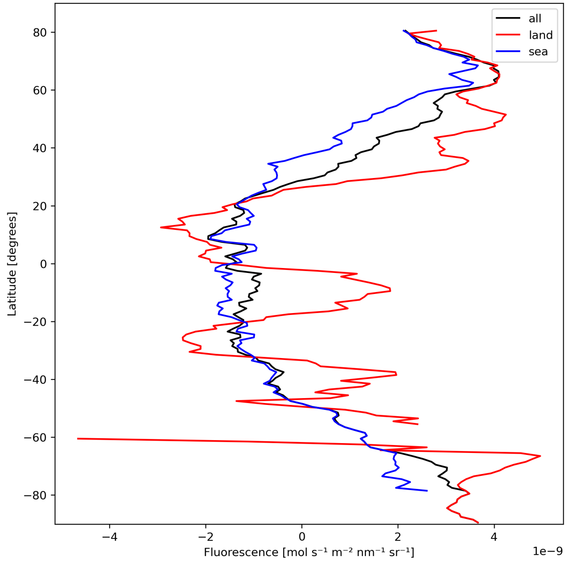
Figure 23: Zonal average of “Fluorescence” for 2024-02-27 to 2024-02-29.
