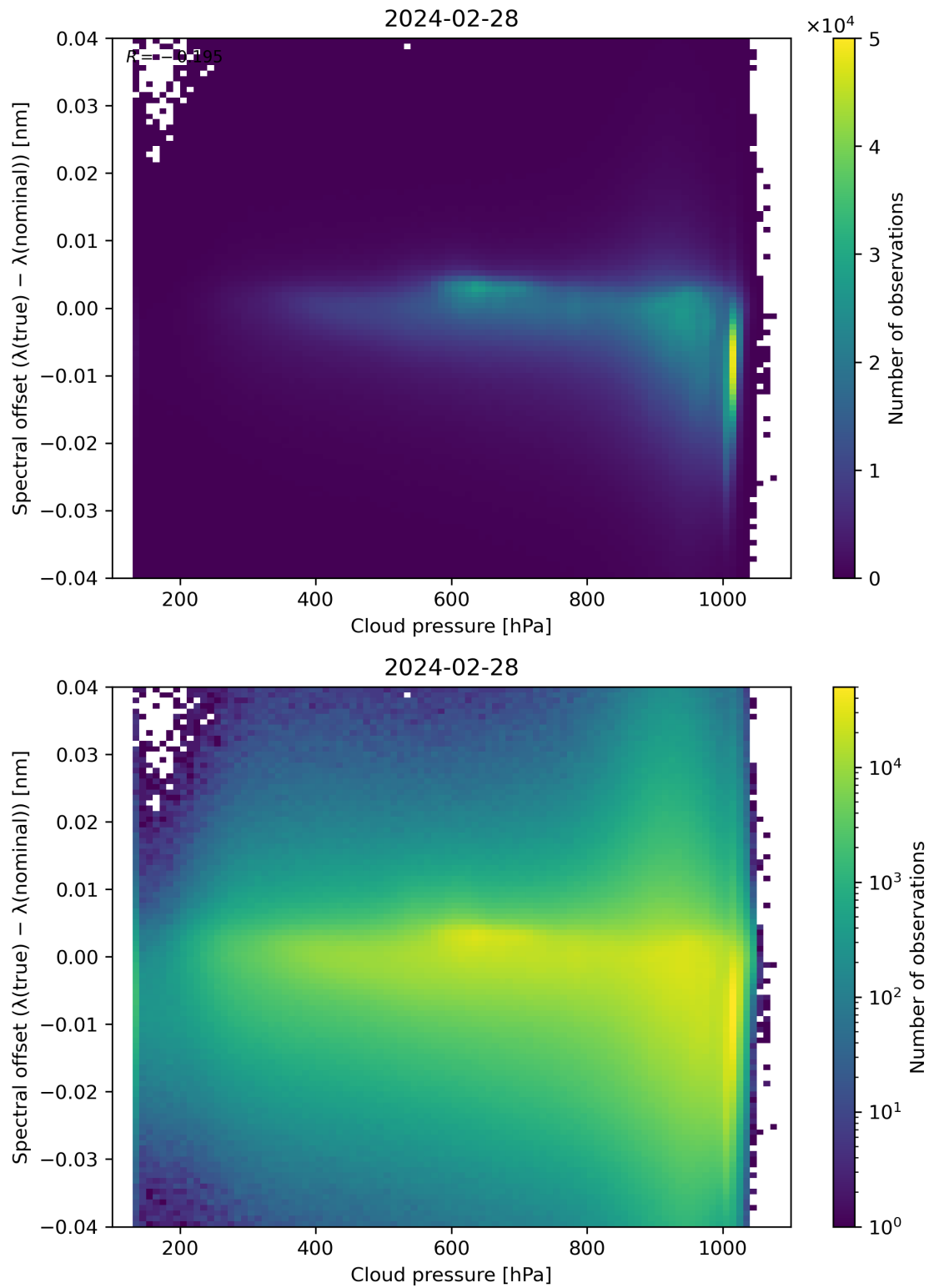
Figure 84: Scatter density plot of “Cloud pressure” against “Spectral offset ( \lambda(\text{true}) - \lambda(\text{nominal}) )” for 2024-02-27 to 2024-02-29.
