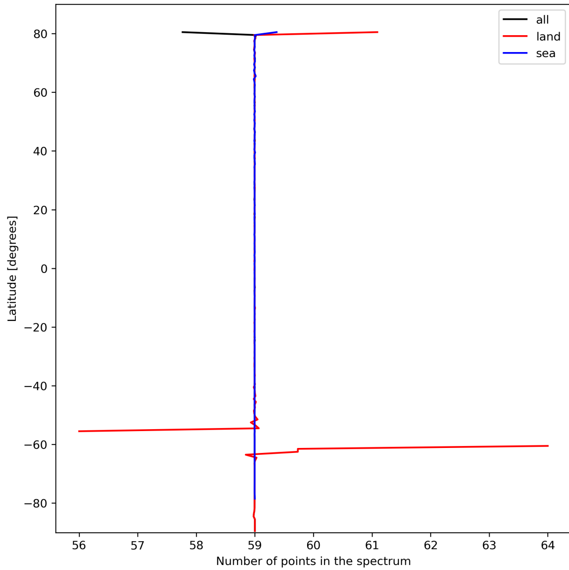
Figure 27: Zonal average of “Number of points in the spectrum” for 2024-02-27 to 2024-02-29.
