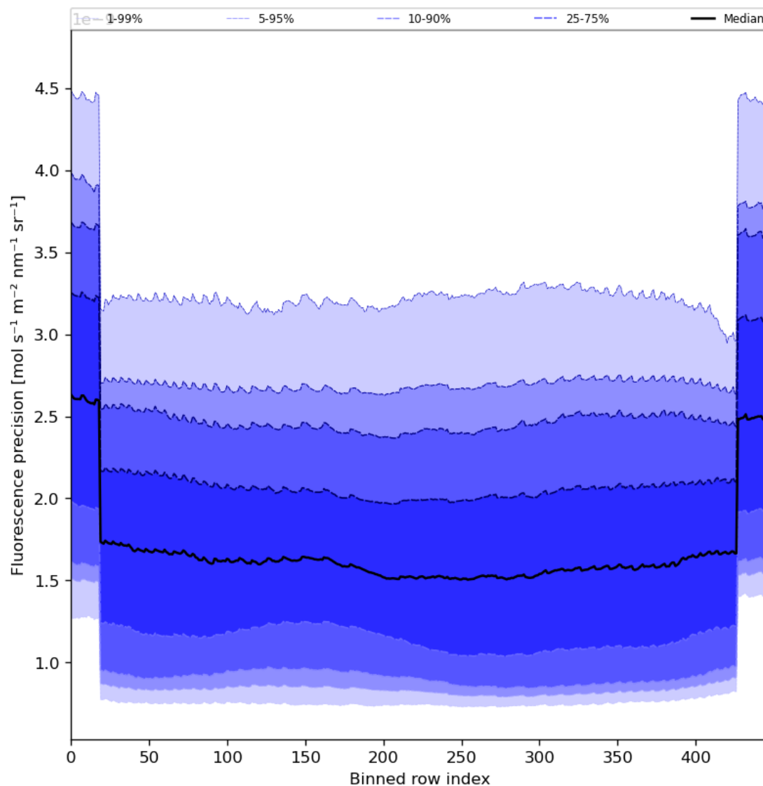
Figure 58: Along track statistics of “Fluorescence precision” for 2024-02-27 to 2024-02-29
