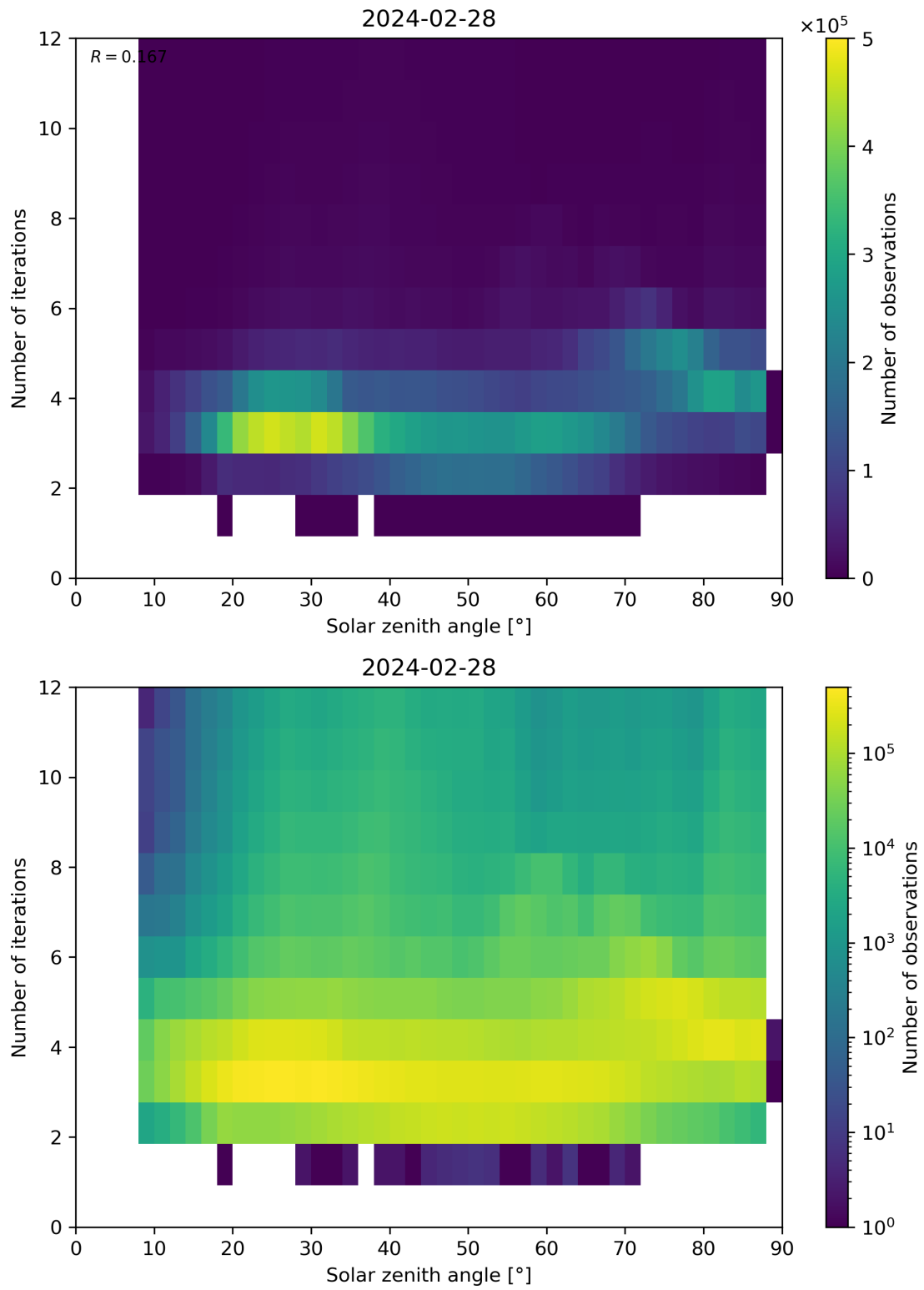
Figure 114: Scatter density plot of “Solar zenith angle” against “Number of iterations” for 2024-02-27 to 2024-02-29.
