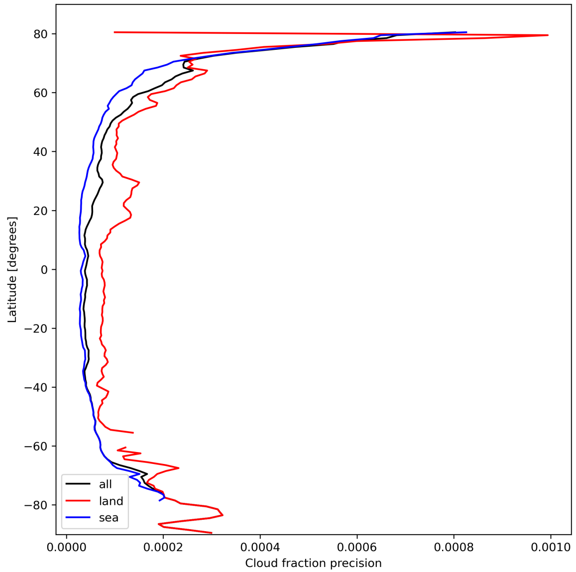
Figure 16: Zonal average of “Cloud fraction precision” for 2024-02-27 to 2024-02-29.
