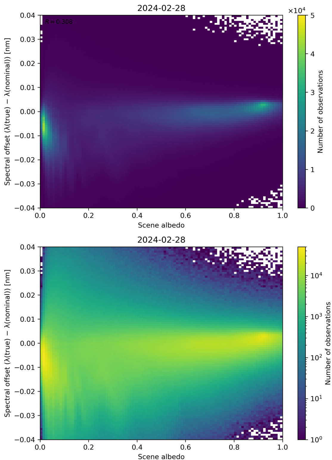
Figure 107: Scatter density plot of “Scene albedo” against “Spectral offset ( \lambda(\text{true}) - \lambda(\text{nominal}) )” for 2024-02-27 to 2024-02-29.
