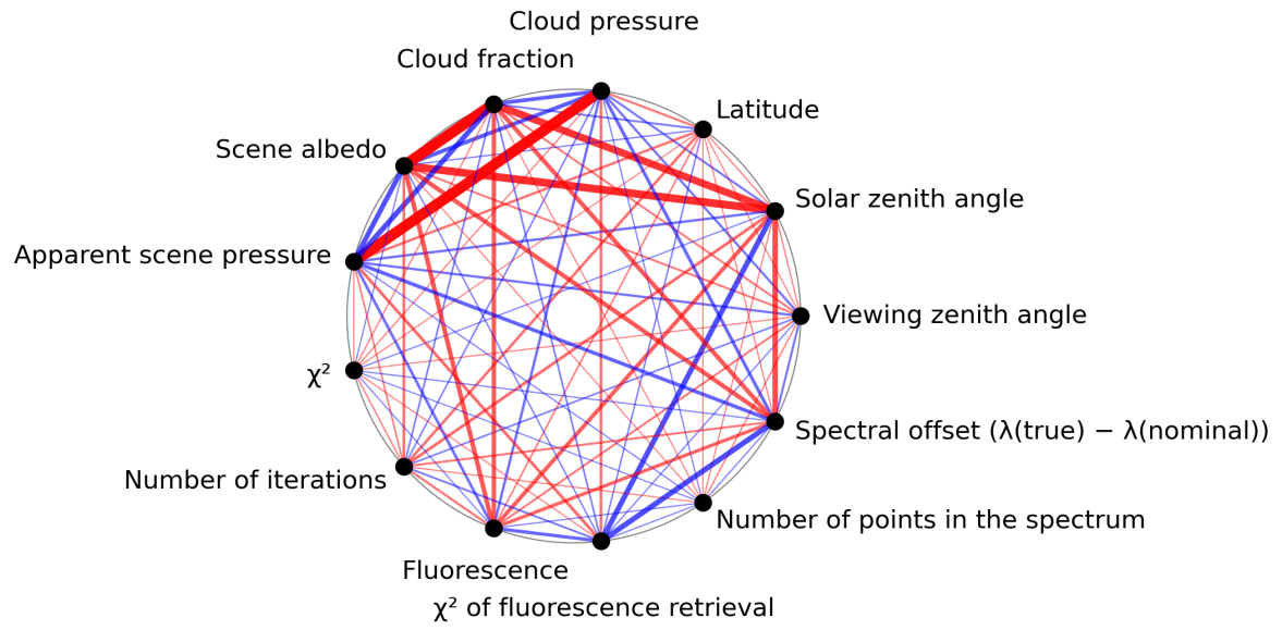
Figure 1: Map of correlation graph for 2024-02-27 to 2024-02-29.
