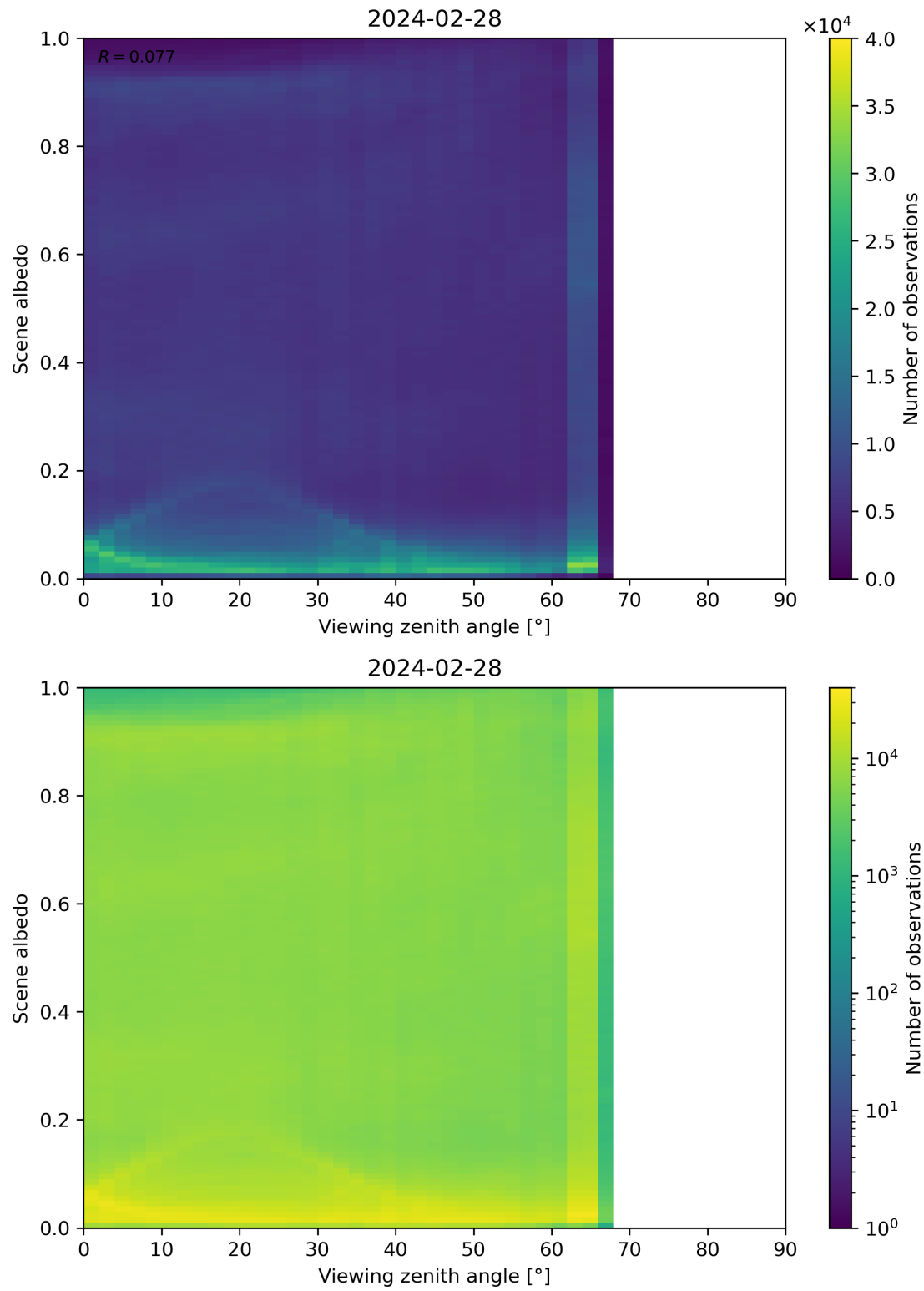
Figure 126: Scatter density plot of “Viewing zenith angle” against “Scene albedo” for 2024-02-27 to 2024-02-29.
