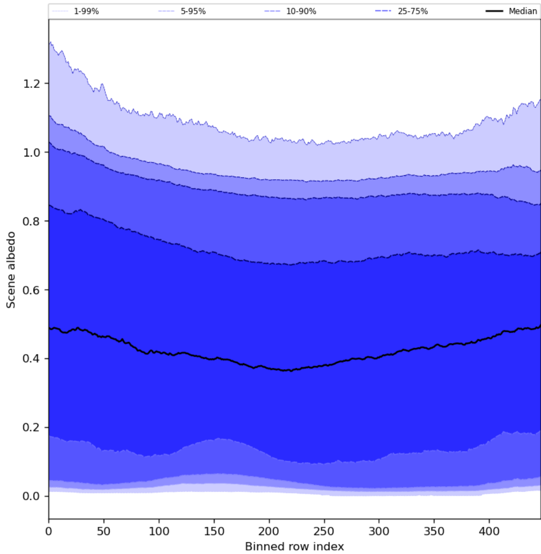
Figure 51: Along track statistics of “Scene albedo” for 2024-02-27 to 2024-02-29
