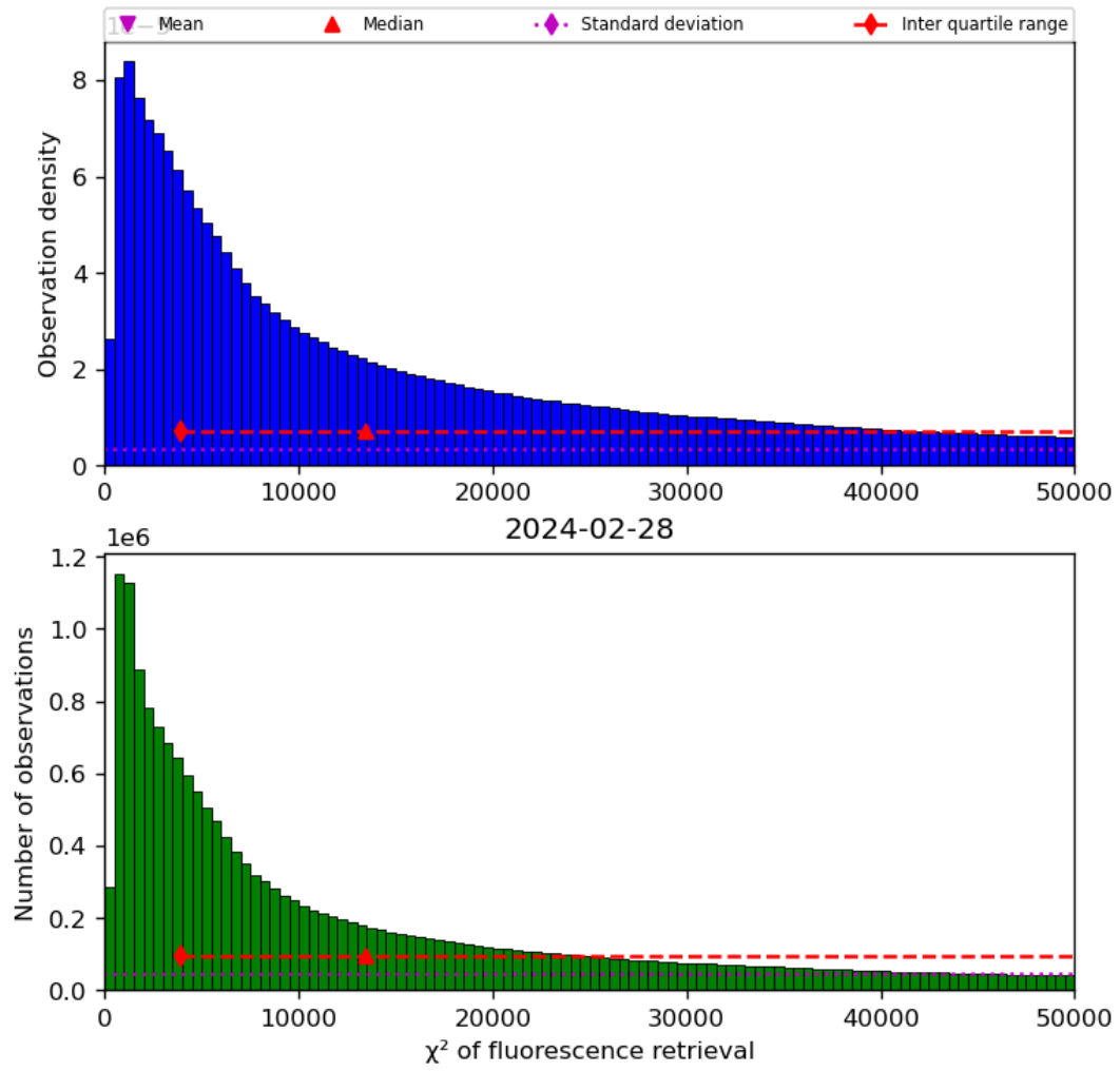
Figure 42: Histogram of “ \chi^2 of fluorescence retrieval” for 2024-02-27 to 2024-02-29
