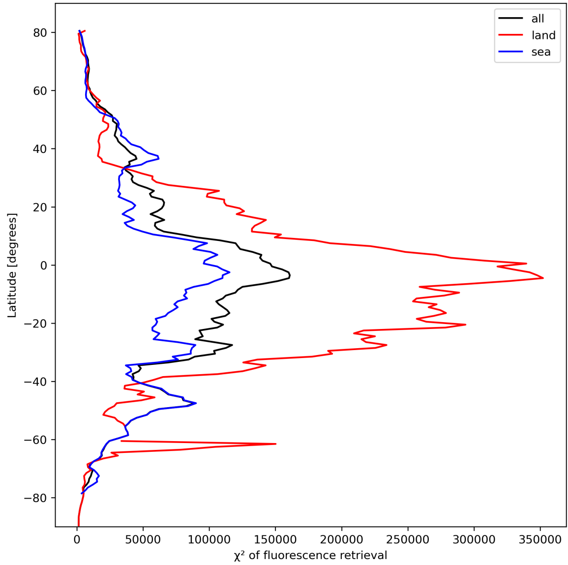
Figure 25: Zonal average of “ \chi^2 of fluorescence retrieval” for 2024-02-27 to 2024-02-29.
