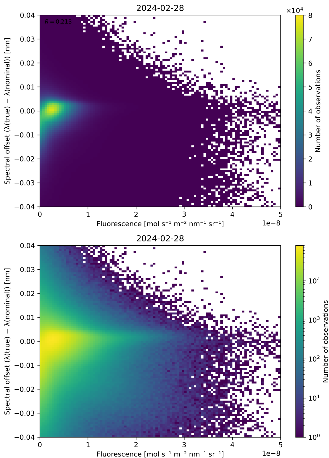
Figure 87: Scatter density plot of “Fluorescence” against “Spectral offset ( \lambda(\text{true}) - \lambda(\text{nominal}) )” for 2024-02-27 to 2024-02-29.
