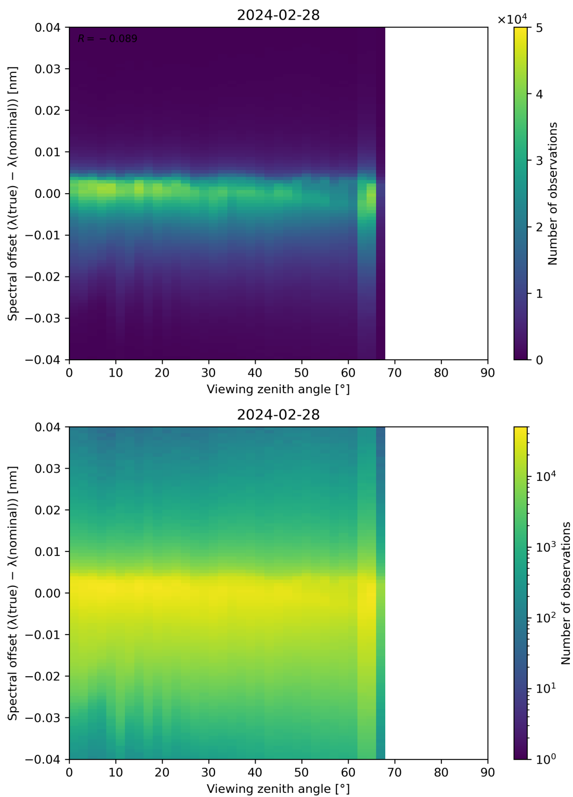
Figure 128: Scatter density plot of “Viewing zenith angle” against “Spectral offset ( \lambda(\text{true}) - \lambda(\text{nominal}) )” for 2024-02-27 to 2024-02-29.
