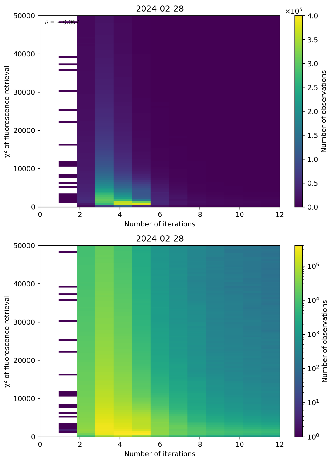
Figure 97: Scatter density plot of “Number of iterations” against “ \chi^2 of fluorescence retrieval” for 2024-02-27 to 2024-02-29.
