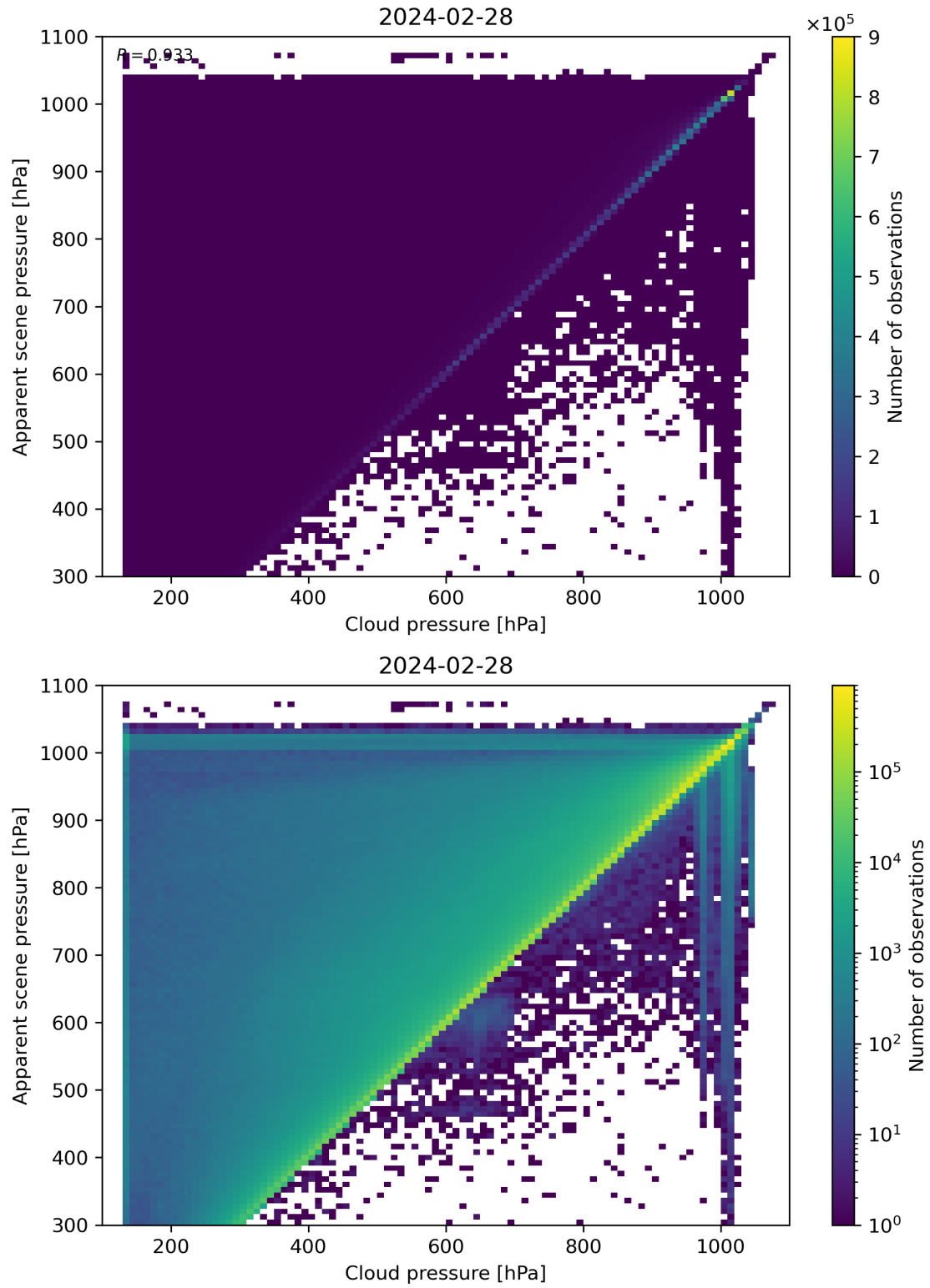
Figure 77: Scatter density plot of “Cloud pressure” against “Apparent scene pressure” for 2024-02-27 to 2024-02-29.
