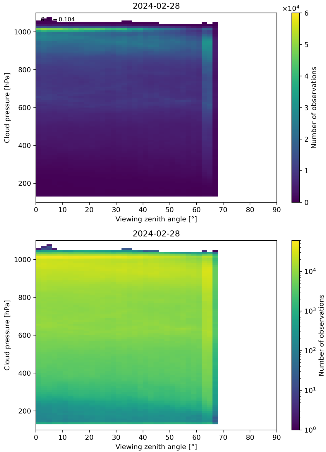
Figure 121: Scatter density plot of “Viewing zenith angle” against “Cloud pressure” for 2024-02-27 to 2024-02-29.
