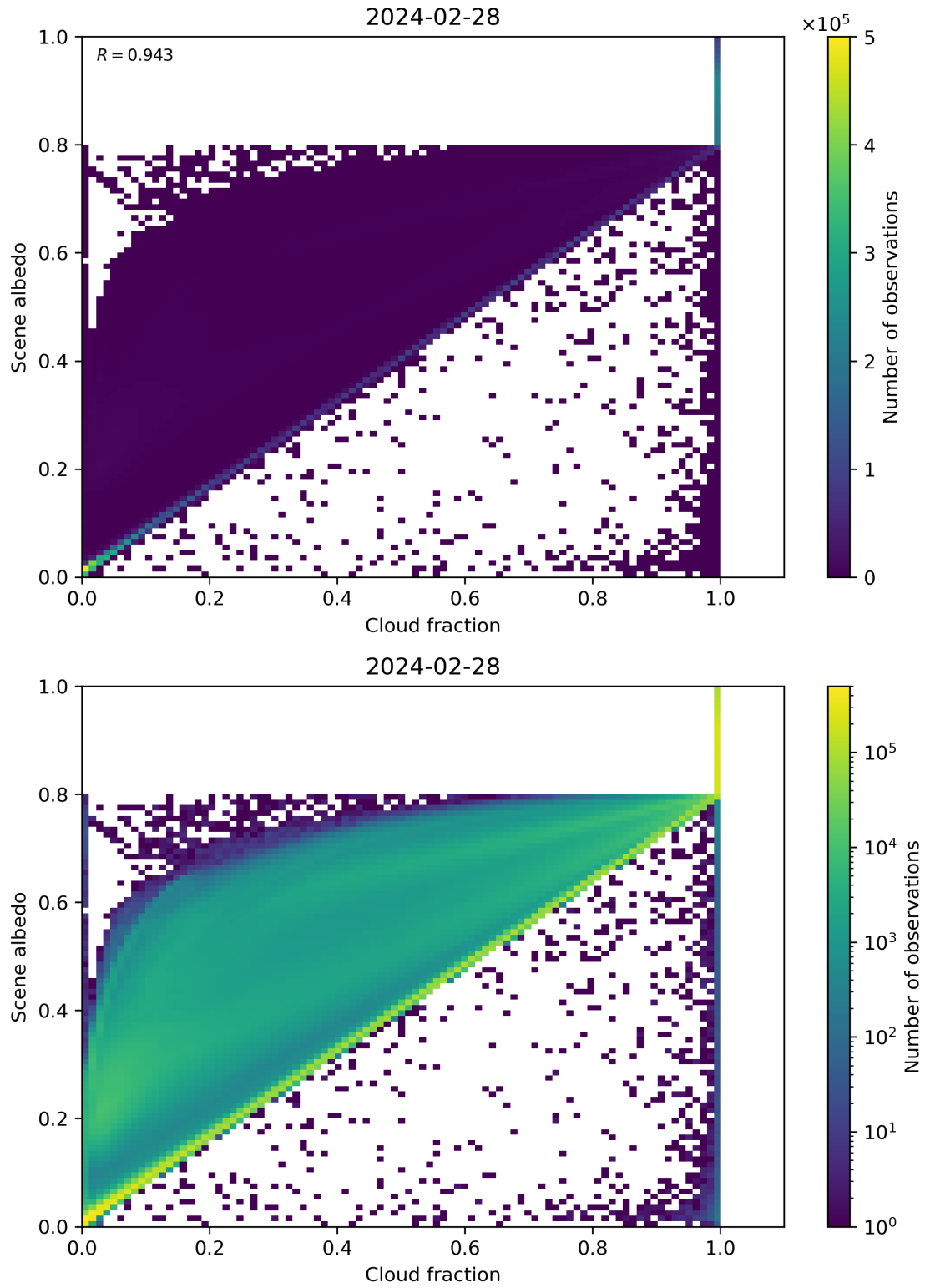
Figure 75: Scatter density plot of “Cloud fraction” against “Scene albedo” for 2024-02-27 to 2024-02-29.
