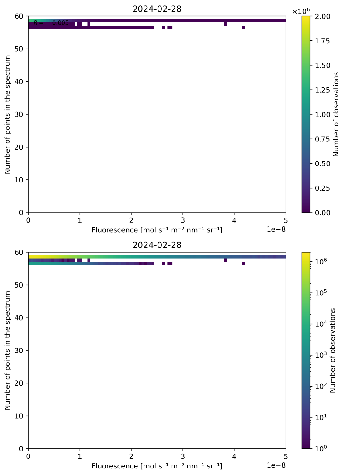
Figure 86: Scatter density plot of “Fluorescence” against “Number of points in the spectrum” for 2024-02-27 to 2024-02-29.
