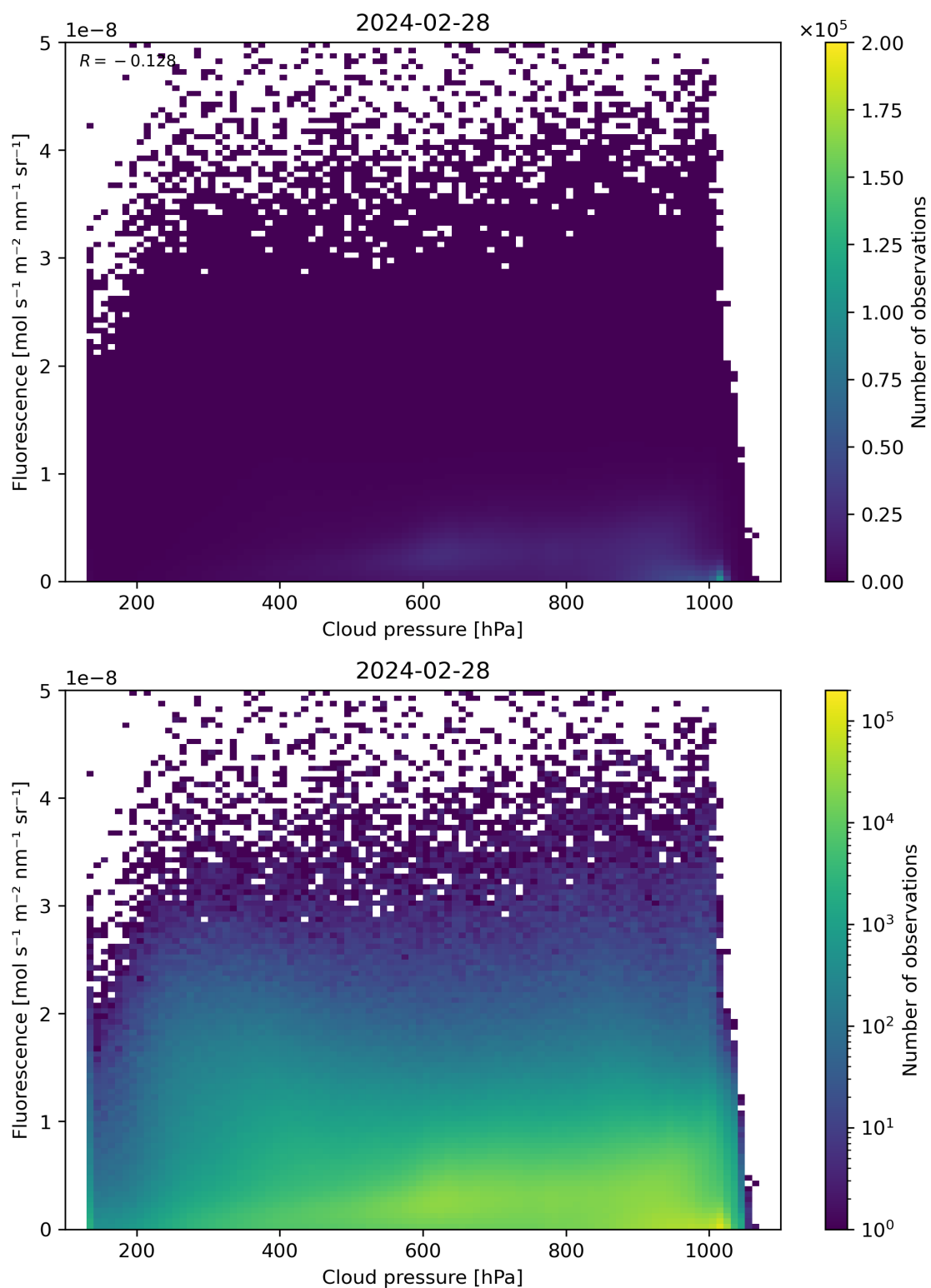
Figure 80: Scatter density plot of “Cloud pressure” against “Fluorescence” for 2024-02-27 to 2024-02-29.
