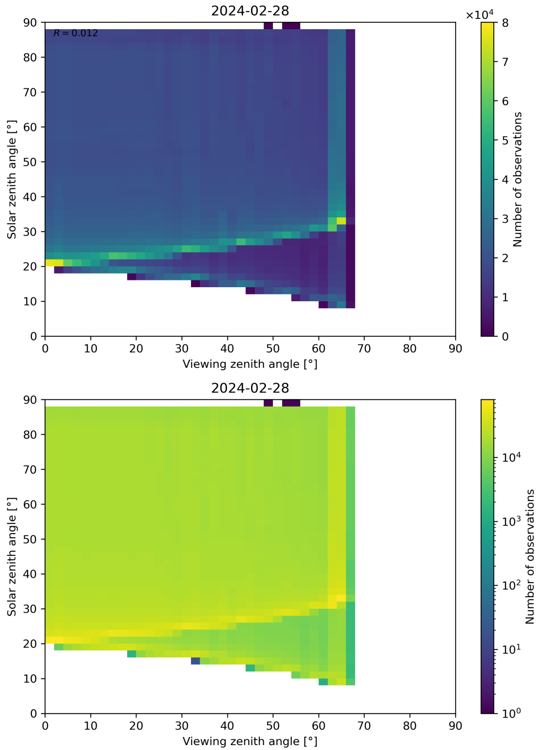
Figure 127: Scatter density plot of “Viewing zenith angle” against “Solar zenith angle” for 2024-02-27 to 2024-02-29.
