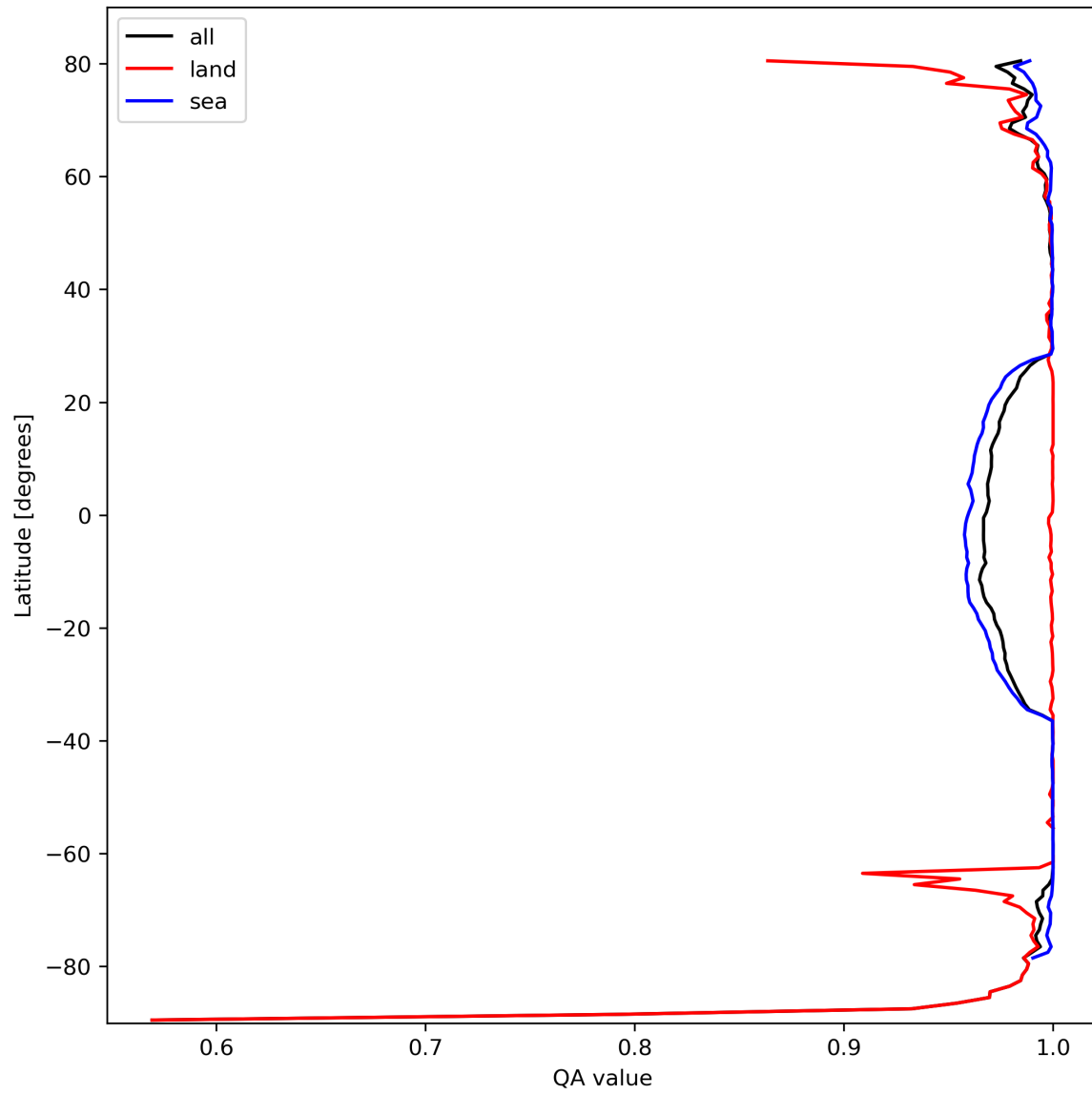
Figure 12: Zonal average of “QA value” for 2024-02-27 to 2024-02-29.
