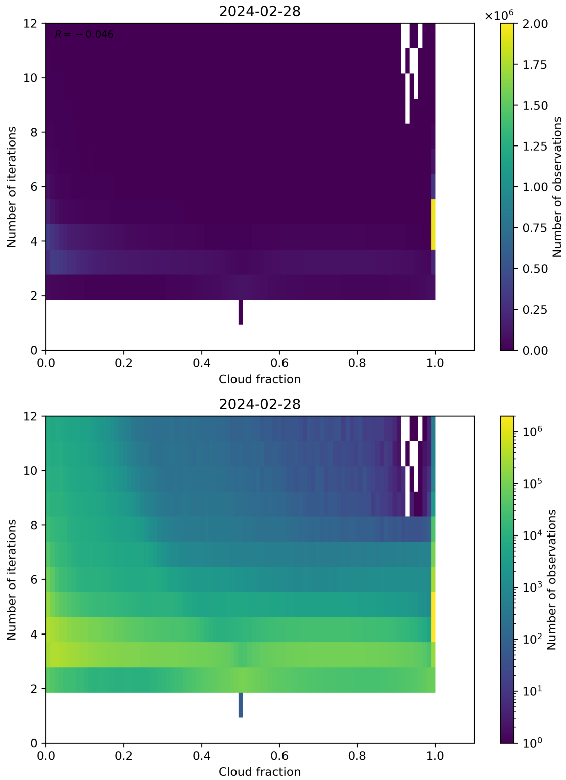
Figure 73: Scatter density plot of “Cloud fraction” against “Number of iterations” for 2024-02-27 to 2024-02-29.
