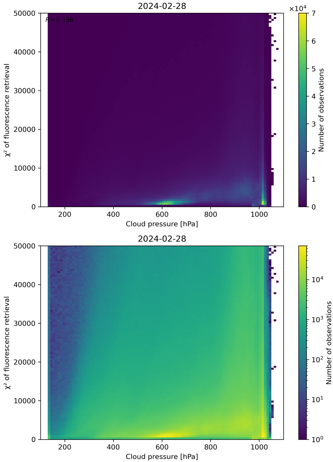
Figure 78: Scatter density plot of “Cloud pressure” against “ \chi^2 of fluorescence retrieval” for 2024-02-27 to 2024-02-29.
