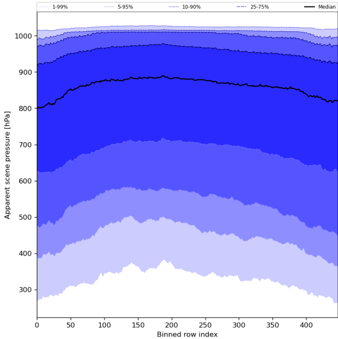
Figure 53: Along track statistics of “Apparent scene pressure” for 2024-02-27 to 2024-02-29
