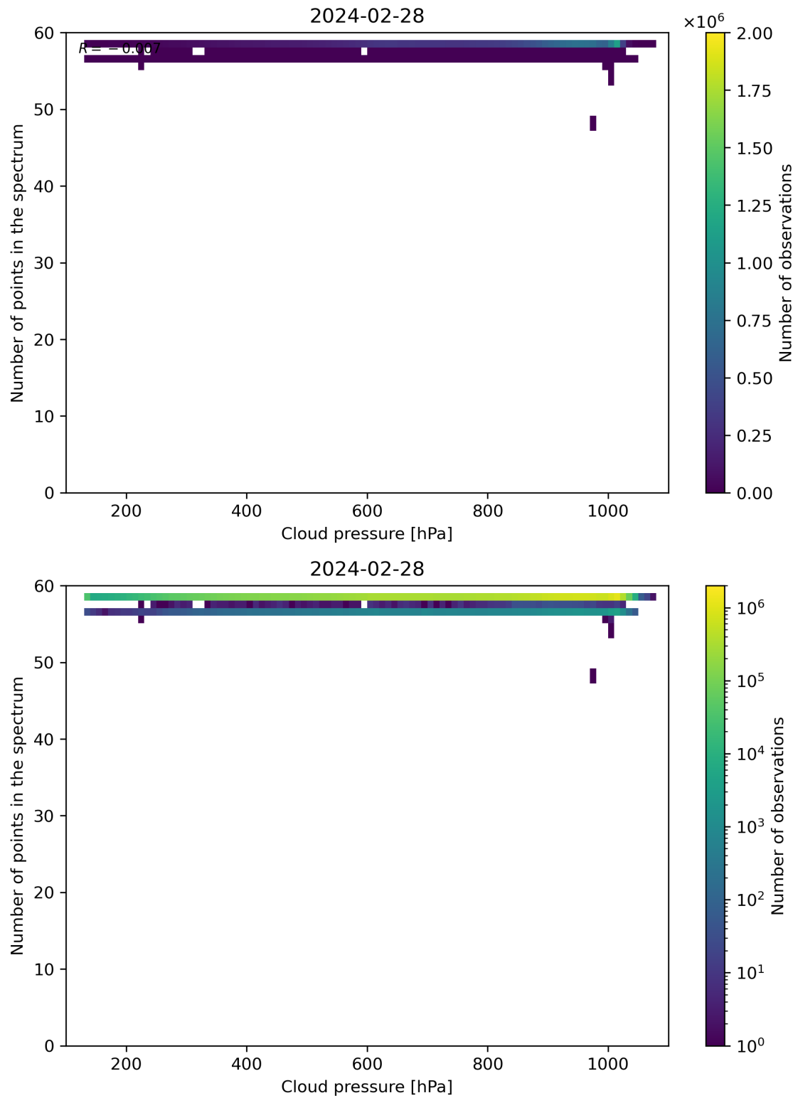
Figure 82: Scatter density plot of “Cloud pressure” against “Number of points in the spectrum” for 2024-02-27 to 2024-02-29.
