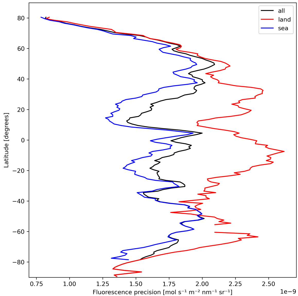
Figure 24: Zonal average of “Fluorescence precision” for 2024-02-27 to 2024-02-29.
