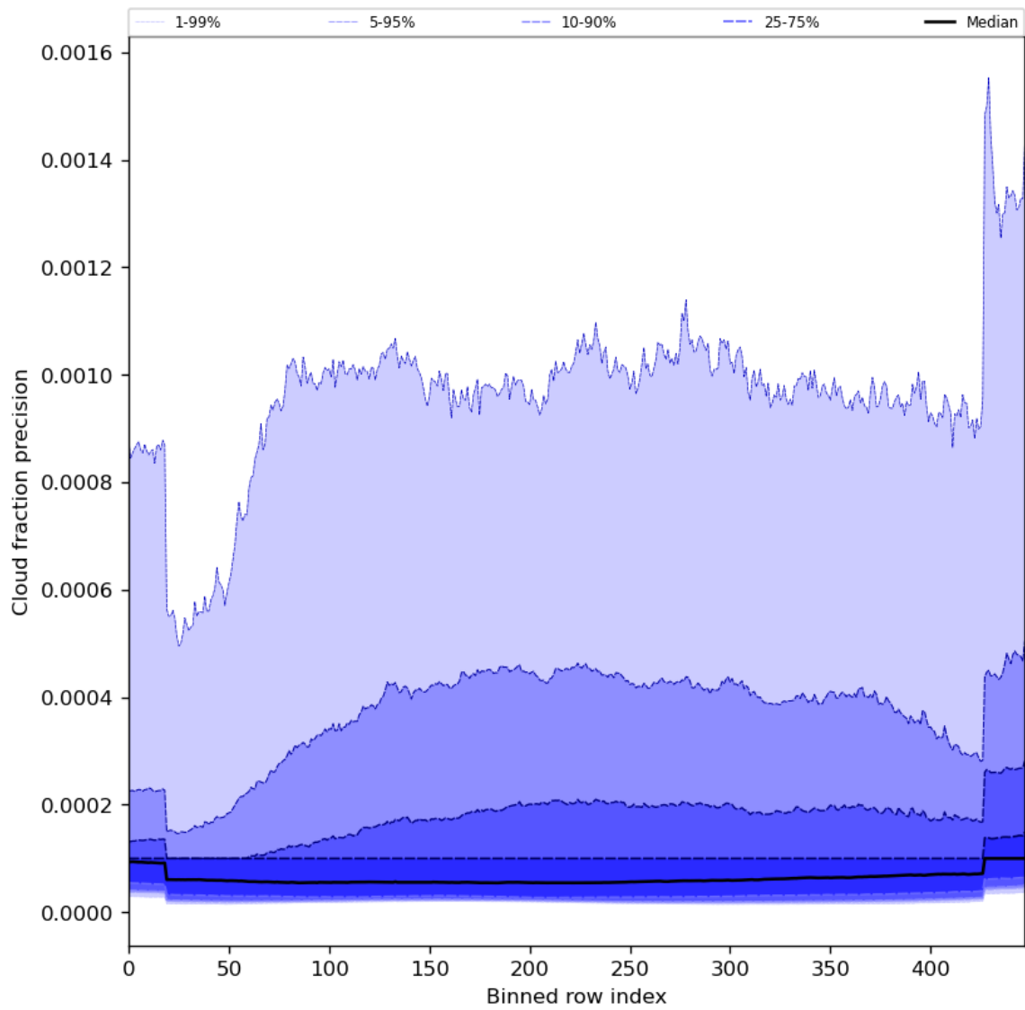
Figure 50: Along track statistics of “Cloud fraction precision” for 2024-02-27 to 2024-02-29
