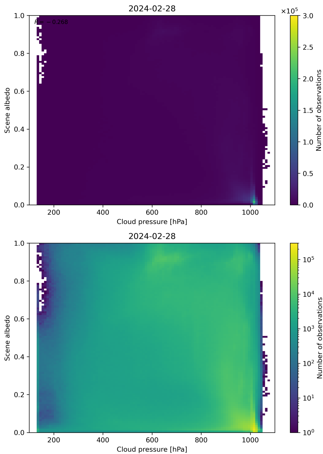
Figure 83: Scatter density plot of “Cloud pressure” against “Scene albedo” for 2024-02-27 to 2024-02-29.
