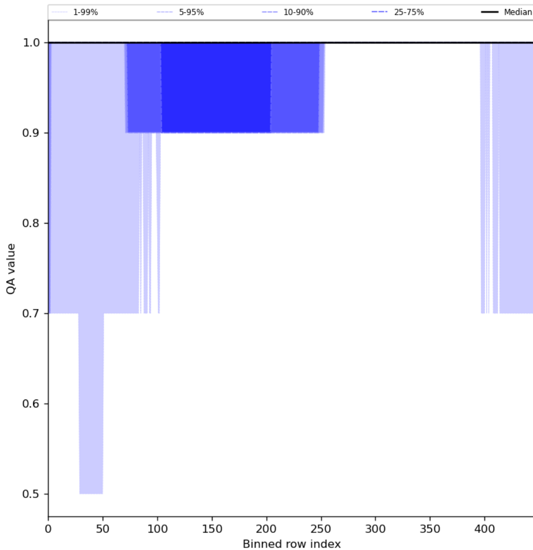
Figure 46: Along track statistics of “QA value” for 2024-02-27 to 2024-02-29
