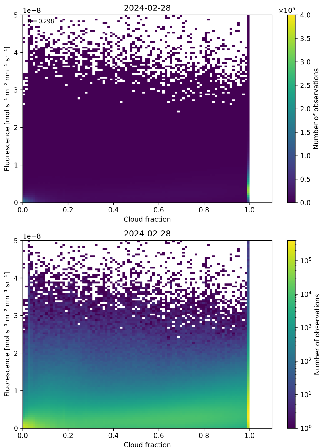
Figure 72: Scatter density plot of “Cloud fraction” against “Fluorescence” for 2024-02-27 to 2024-02-29.
