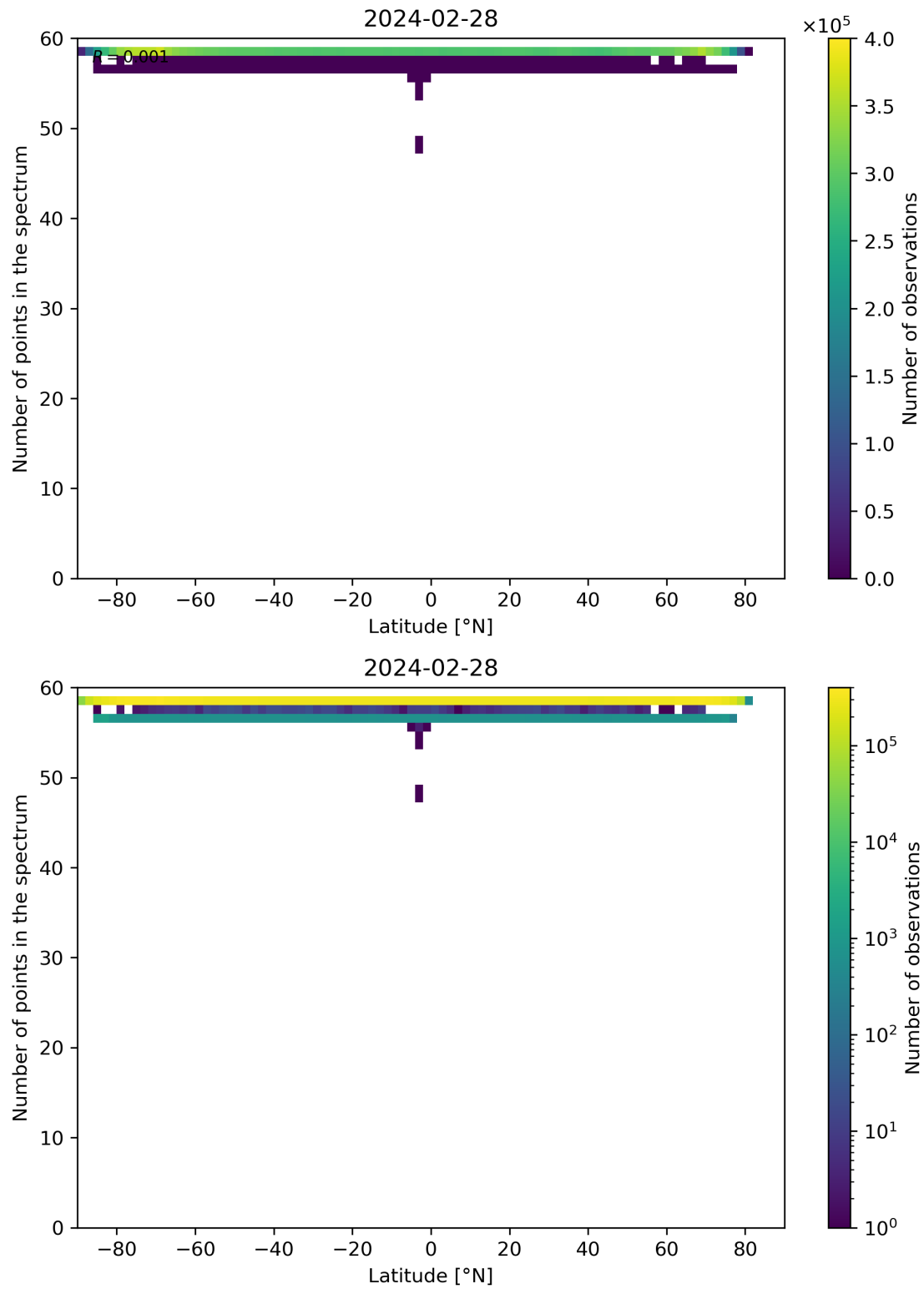
Figure 94: Scatter density plot of “Latitude” against “Number of points in the spectrum” for 2024-02-27 to 2024-02-29.
