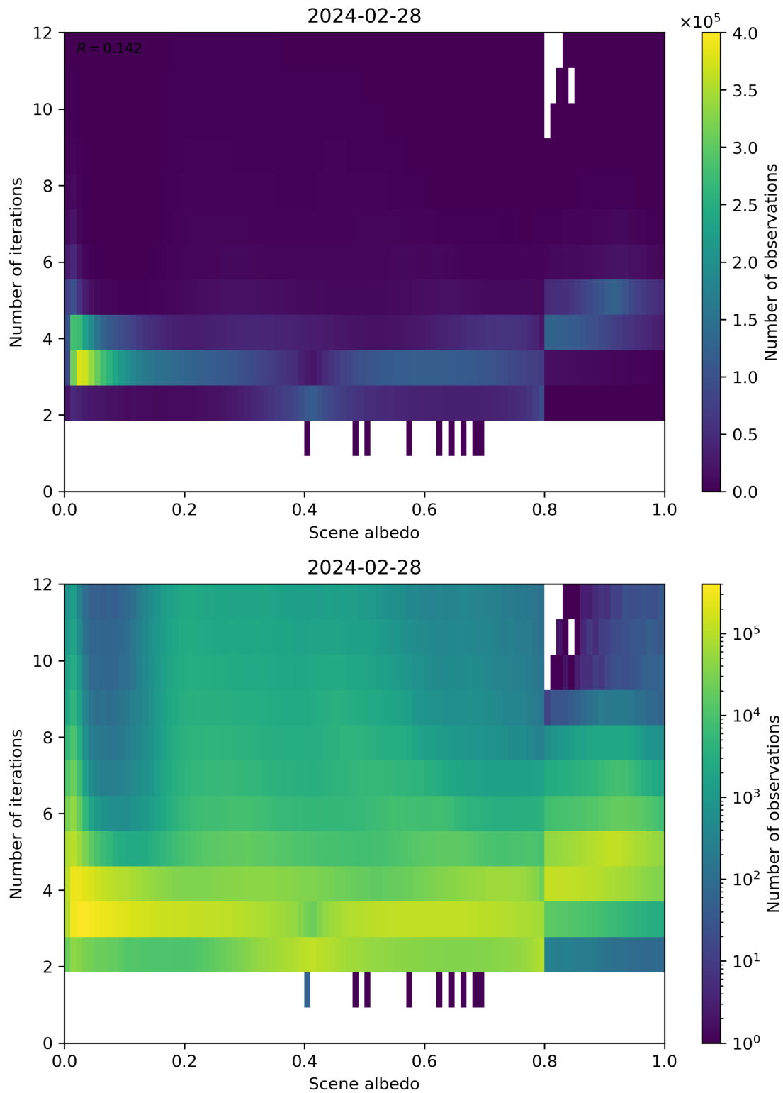
Figure 105: Scatter density plot of “Scene albedo” against “Number of iterations” for 2024-02-27 to 2024-02-29.
