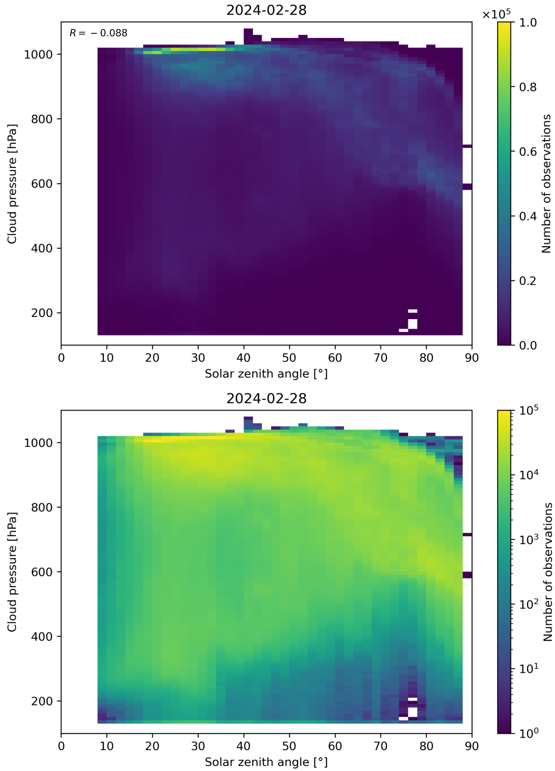
Figure 111: Scatter density plot of “Solar zenith angle” against “Cloud pressure” for 2024-02-27 to 2024-02-29.
