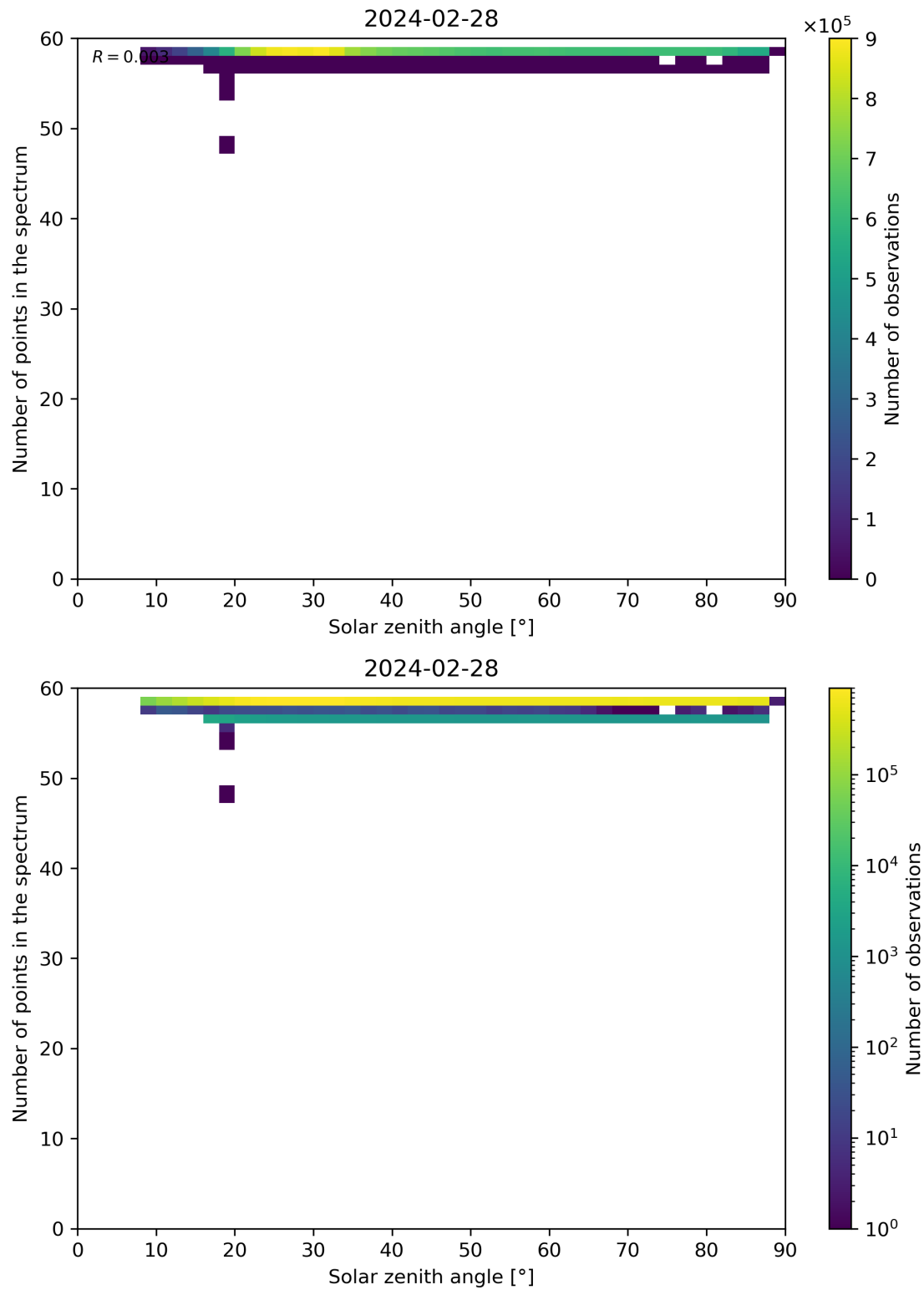
Figure 115: Scatter density plot of “Solar zenith angle” against “Number of points in the spectrum” for 2024-02-27 to 2024-02-29.
