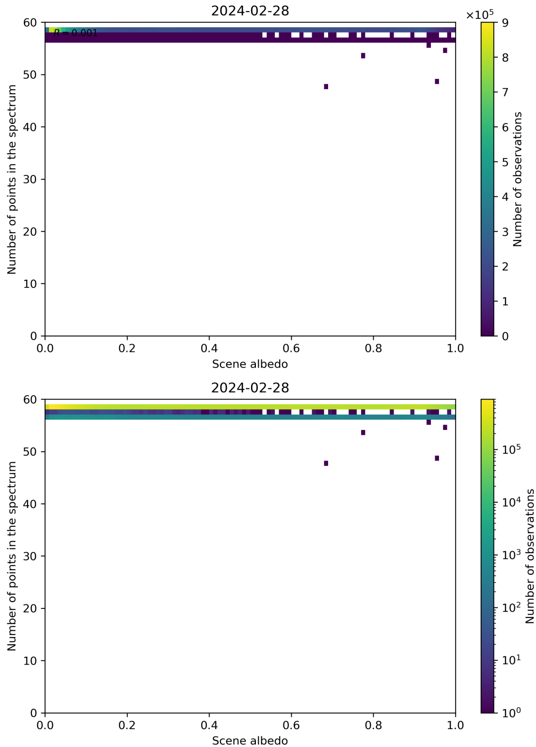
Figure 106: Scatter density plot of “Scene albedo” against “Number of points in the spectrum” for 2024-02-27 to 2024-02-29.
