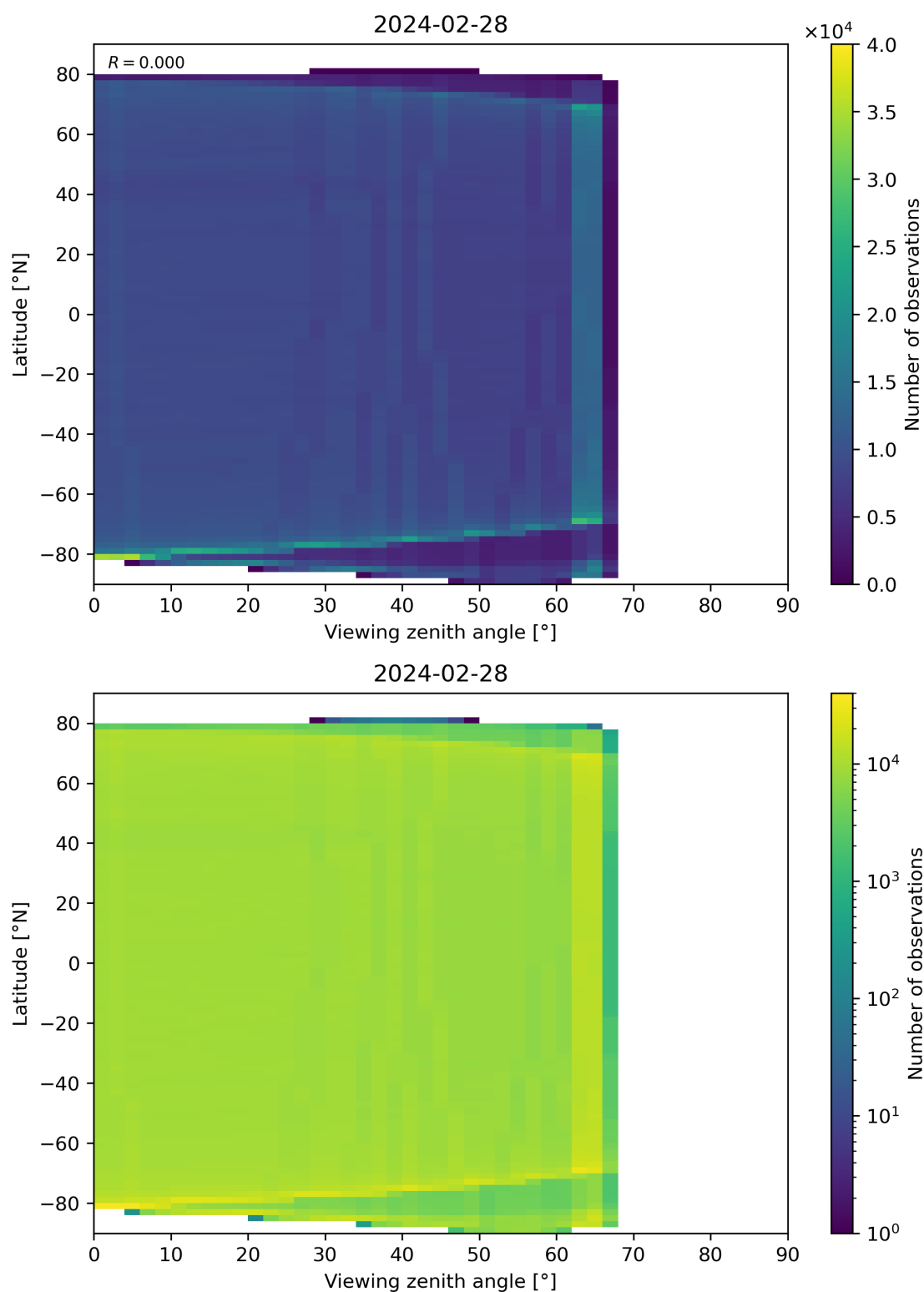
Figure 123: Scatter density plot of “Viewing zenith angle” against “Latitude” for 2024-02-27 to 2024-02-29.
