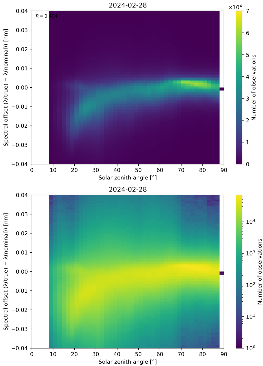
Figure 117: Scatter density plot of “Solar zenith angle” against “Spectral offset ( \lambda(\text{true}) - \lambda(\text{nominal}) )” for 2024-02-27 to 2024-02-29.
