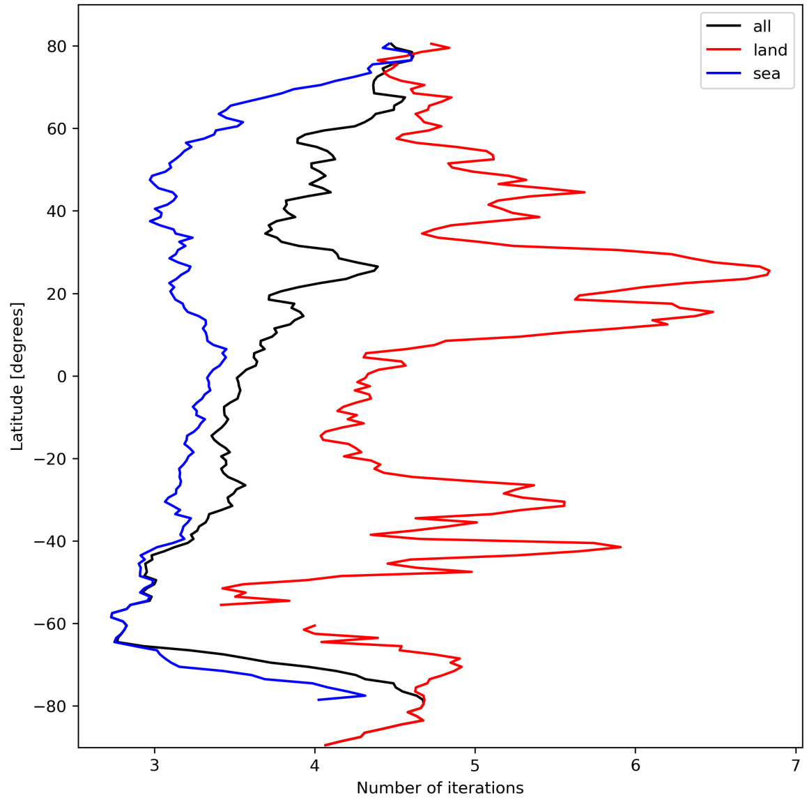
Figure 22: Zonal average of “Number of iterations” for 2024-02-27 to 2024-02-29.
