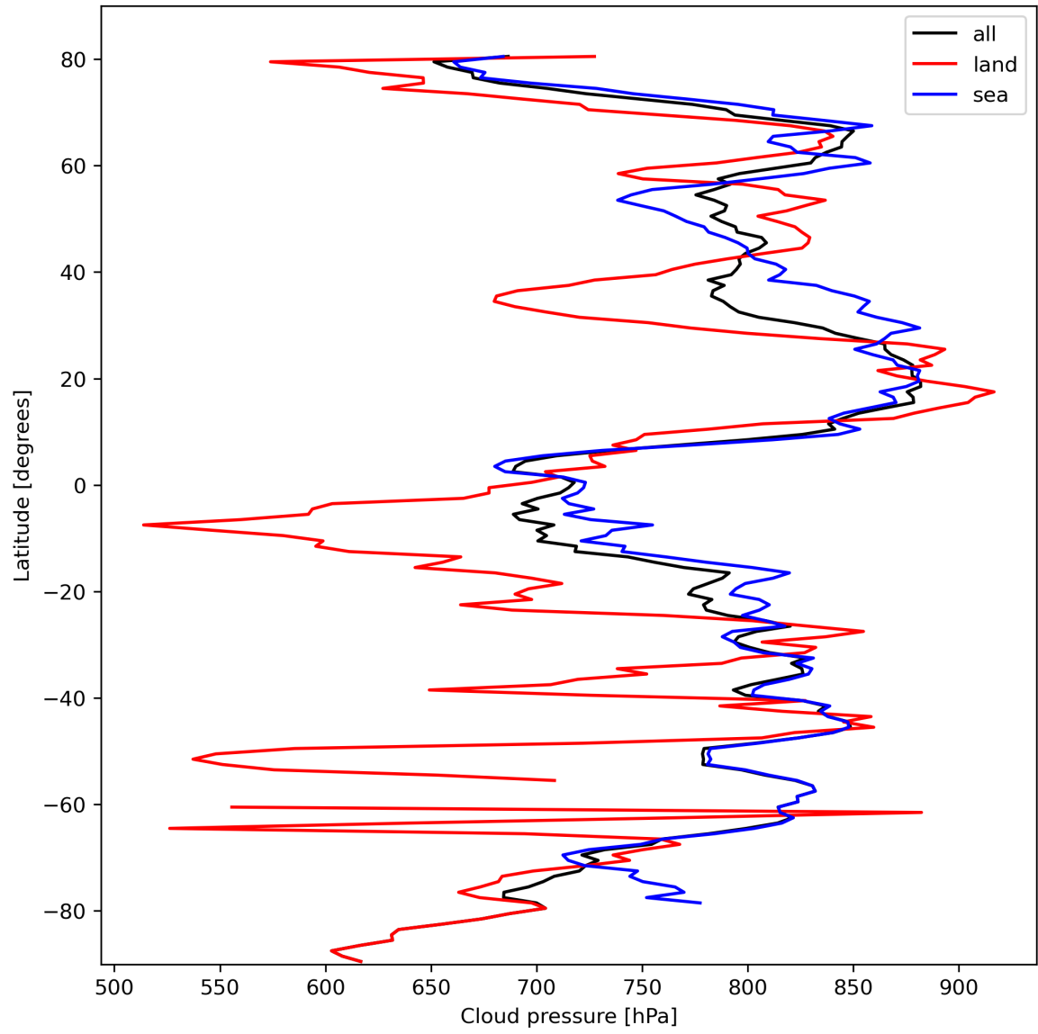
Figure 13: Zonal average of “Cloud pressure” for 2024-02-27 to 2024-02-29.
