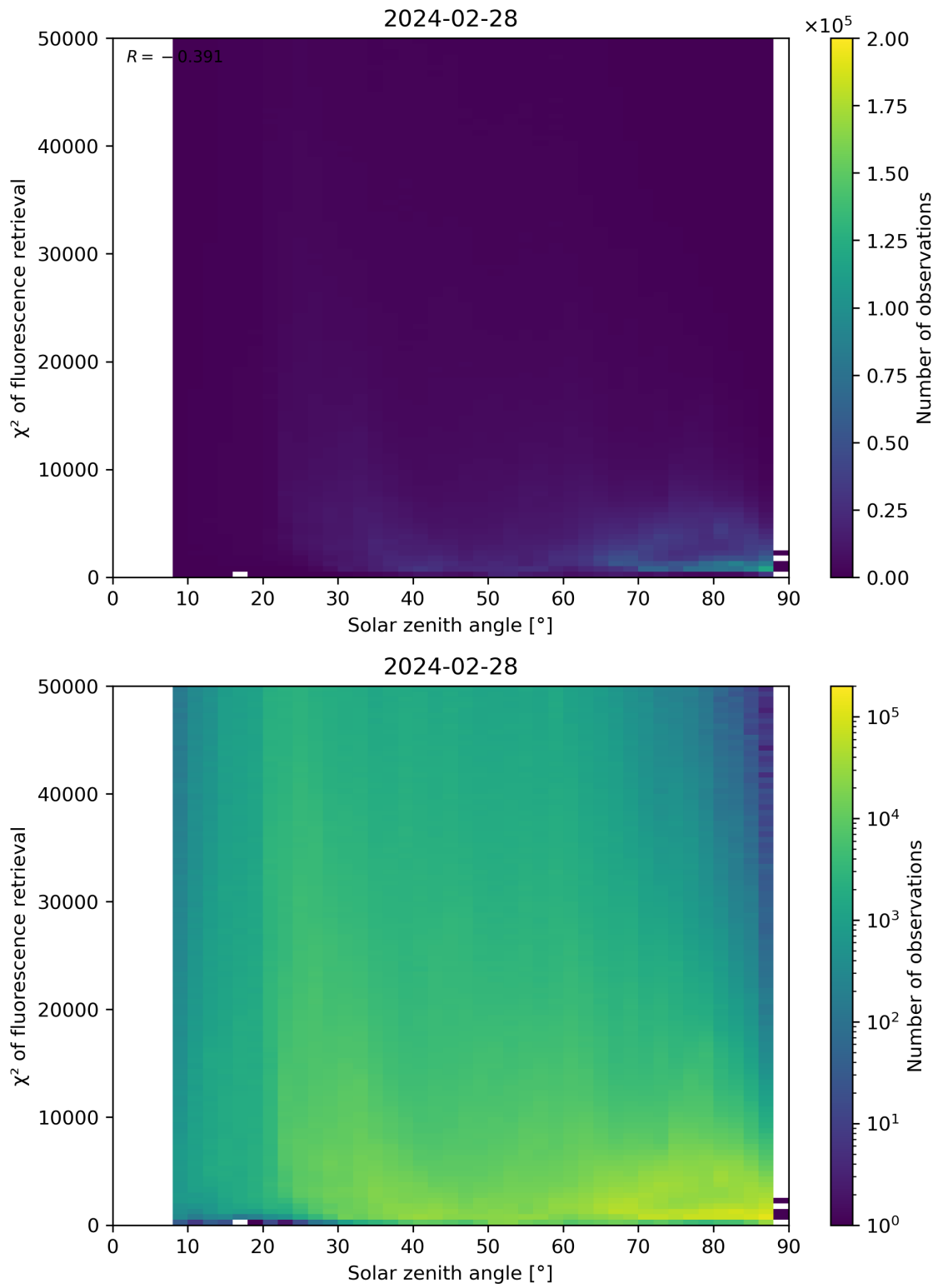
Figure 109: Scatter density plot of “Solar zenith angle” against “ \chi^2 of fluorescence retrieval” for 2024-02-27 to 2024-02-29.
