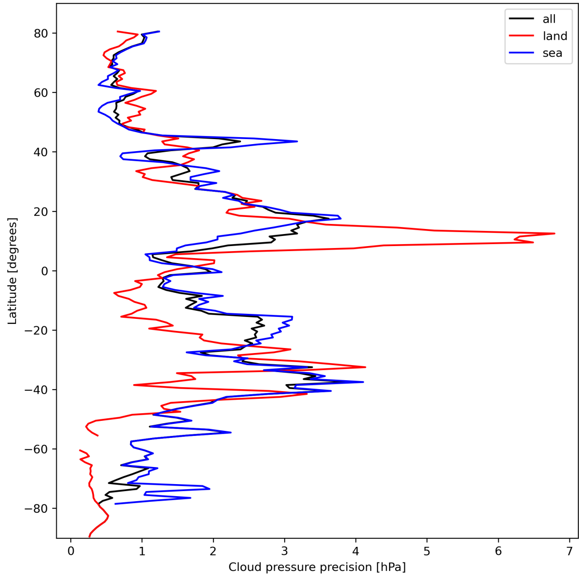
Figure 14: Zonal average of “Cloud pressure precision” for 2024-02-27 to 2024-02-29.
