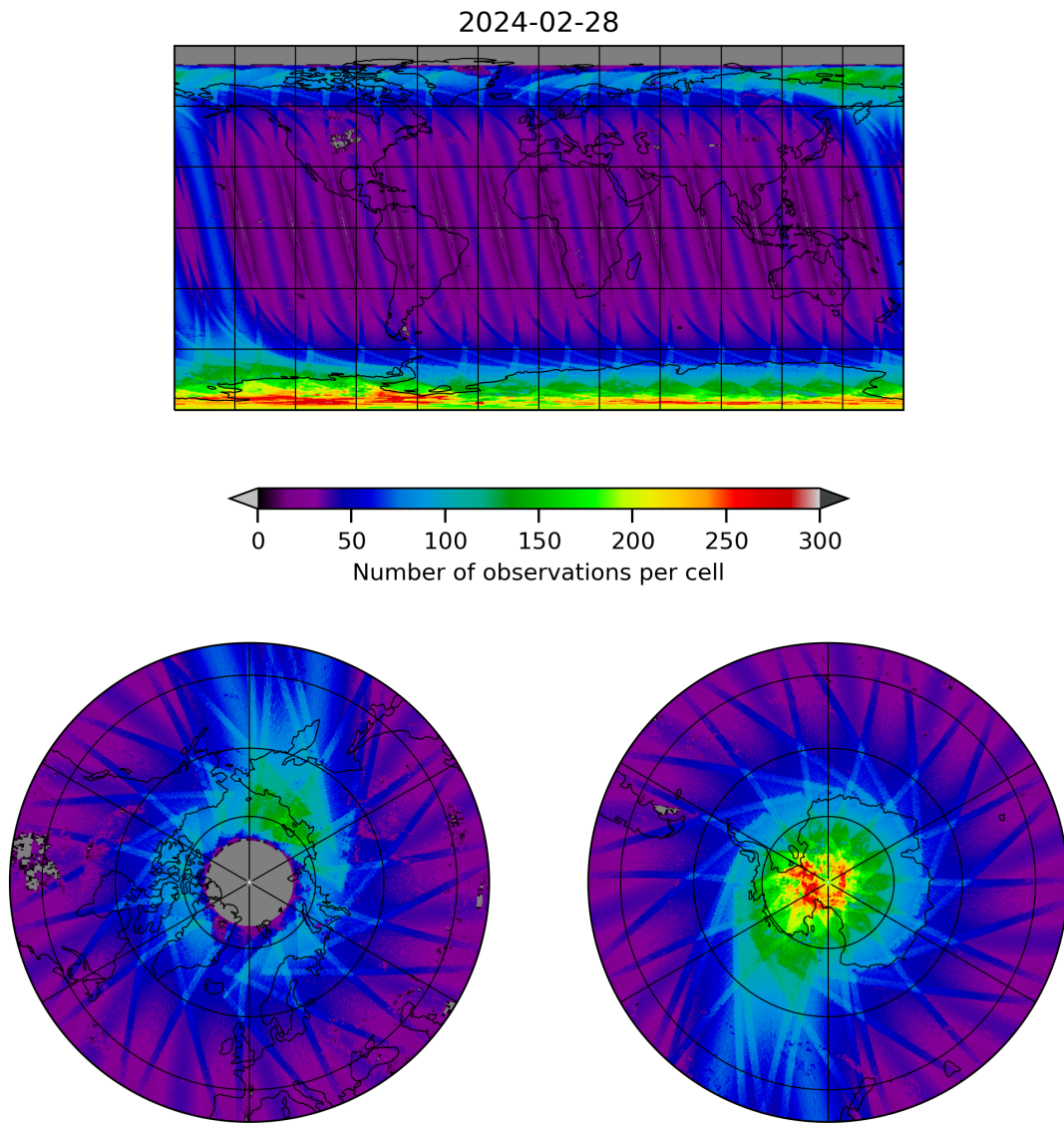
Figure 11: Map of the number of observations for 2024-02-27 to 2024-02-29
