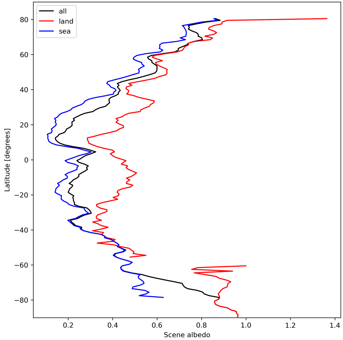
Figure 17: Zonal average of “Scene albedo” for 2024-02-27 to 2024-02-29.
