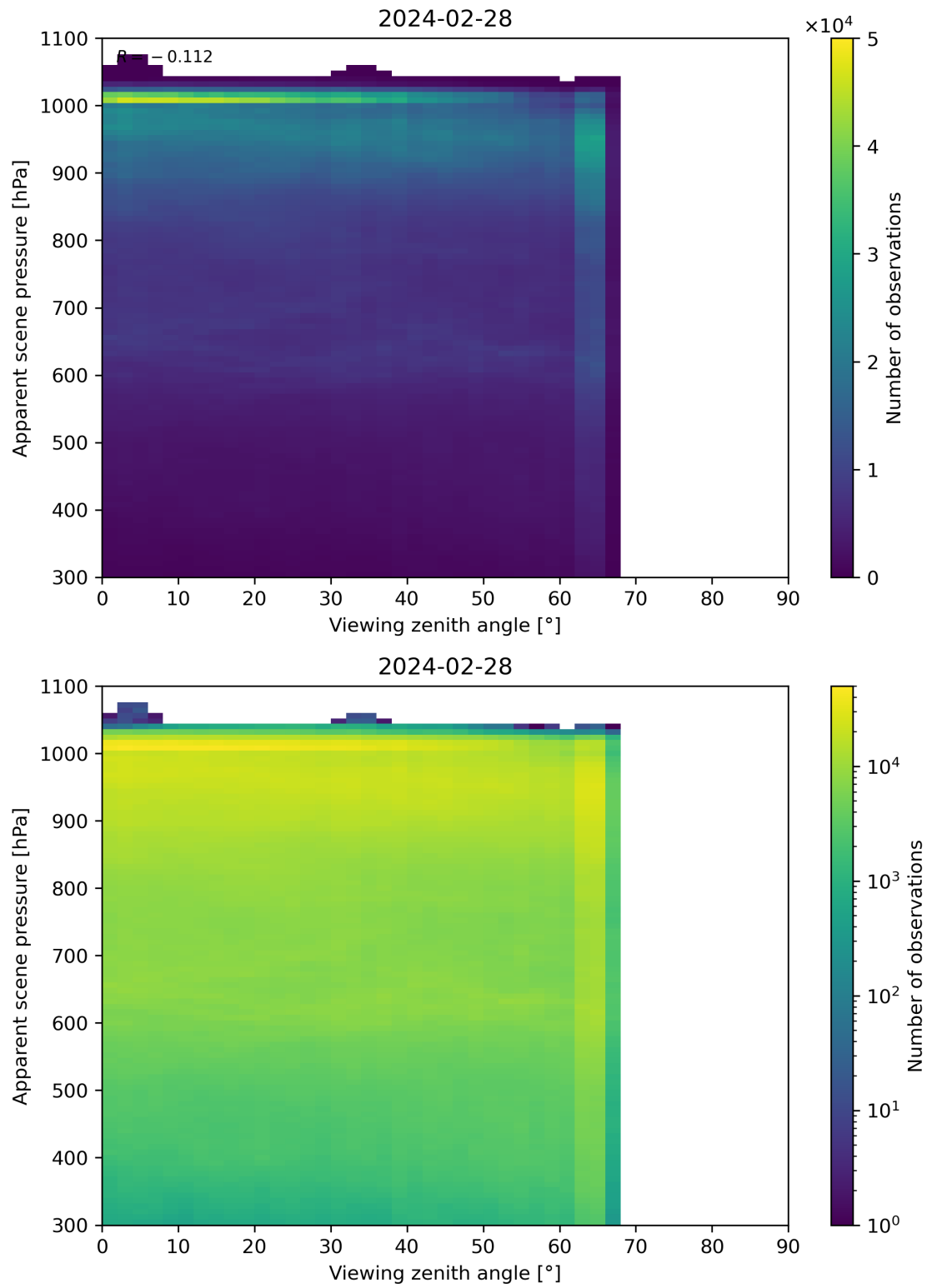
Figure 118: Scatter density plot of “Viewing zenith angle” against “Apparent scene pressure” for 2024-02-27 to 2024-02-29.
