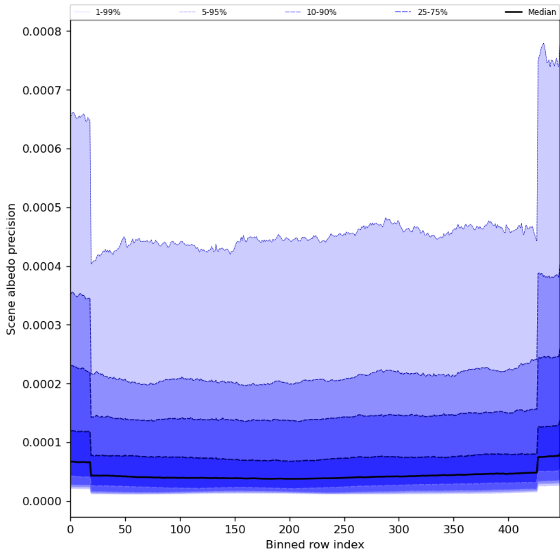
Figure 52: Along track statistics of “Scene albedo precision” for 2024-02-27 to 2024-02-29
