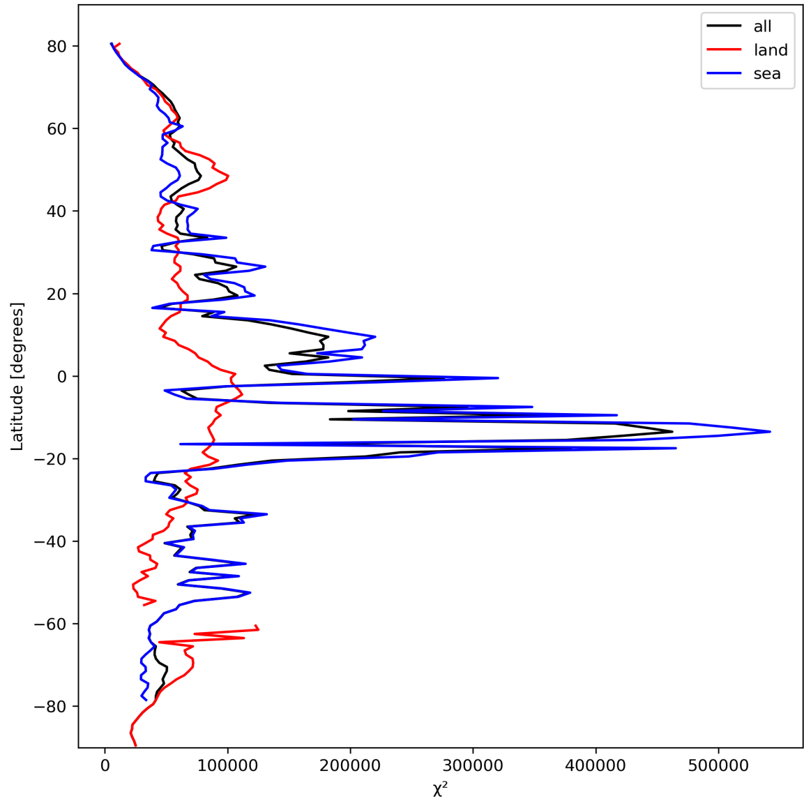
Figure 21: Zonal average of “ \chi^2 ” for 2024-02-27 to 2024-02-29.
