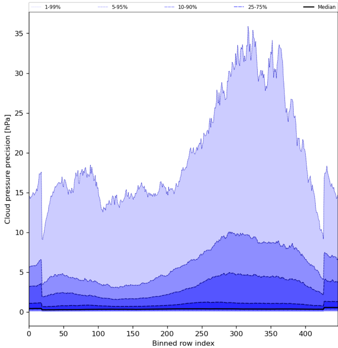
Figure 48: Along track statistics of “Cloud pressure precision” for 2024-02-27 to 2024-02-29
