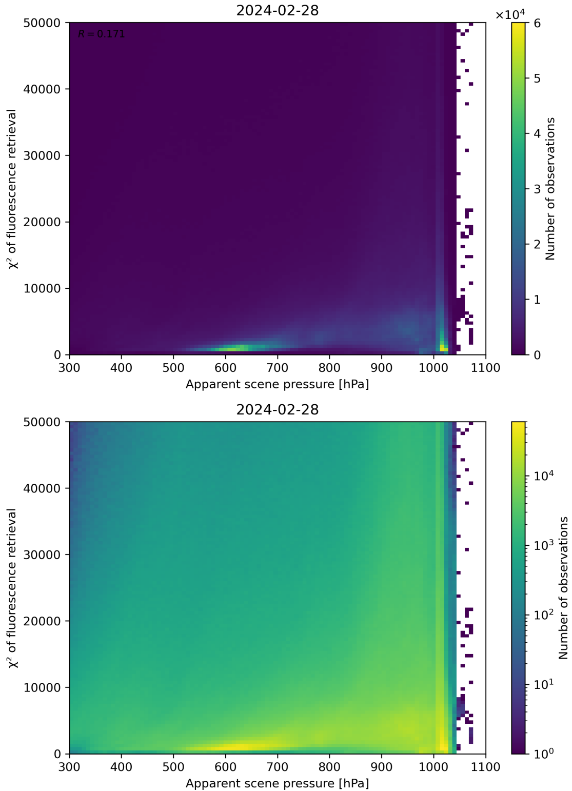
Figure 63: Scatter density plot of “Apparent scene pressure” against “ \chi^2 of fluorescence retrieval” for 2024-02-27 to 2024-02-29.
