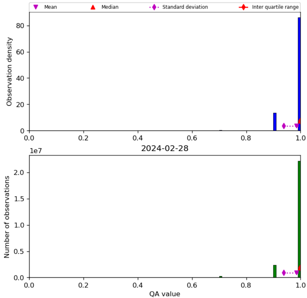
Figure 29: Histogram of “QA value” for 2024-02-27 to 2024-02-29
