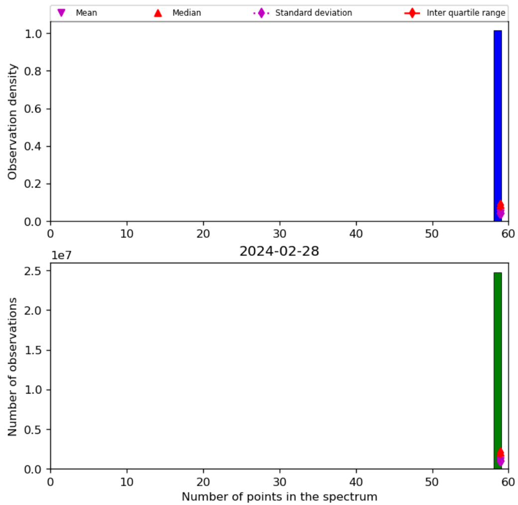
Figure 44: Histogram of “Number of points in the spectrum” for 2024-02-27 to 2024-02-29
