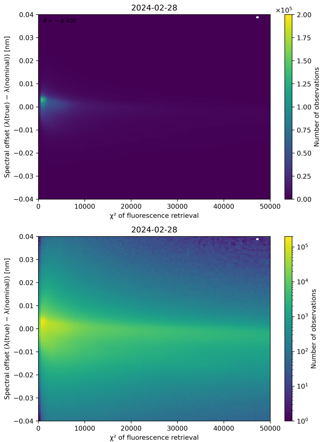
Figure 69: Scatter density plot of " \chi^2 of fluorescence retrieval" against "Spectral offset ( \lambda(\text{true}) - \lambda(\text{nominal})) " for 2024-02-27 to 2024-02-29.
