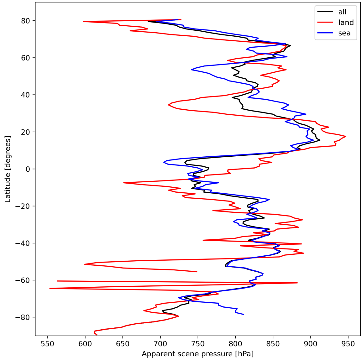
Figure 19: Zonal average of “Apparent scene pressure” for 2024-02-27 to 2024-02-29.
