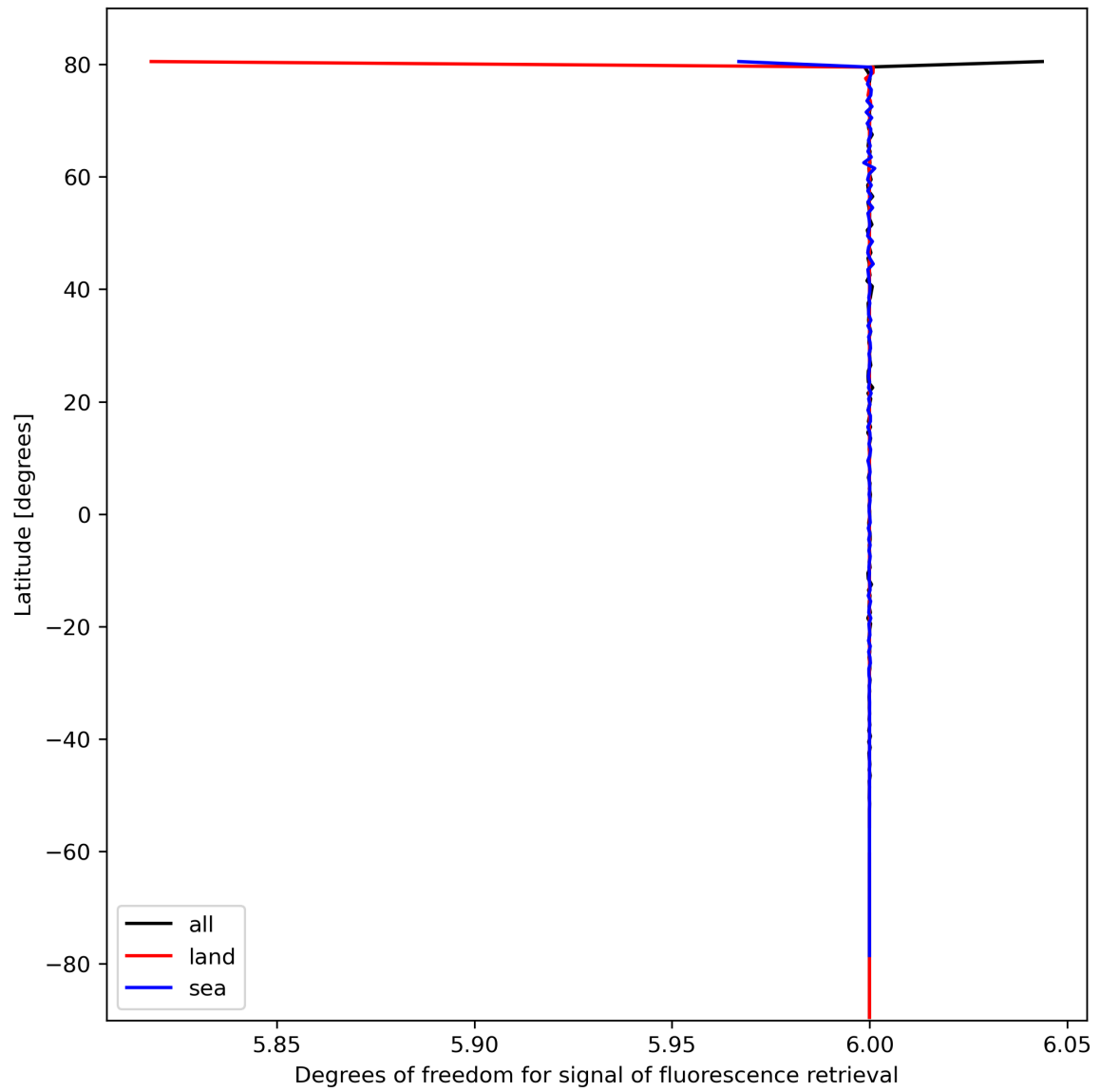
Figure 26: Zonal average of “Degrees of freedom for signal of fluorescence retrieval” for 2024-02-27 to 2024-02-29.
