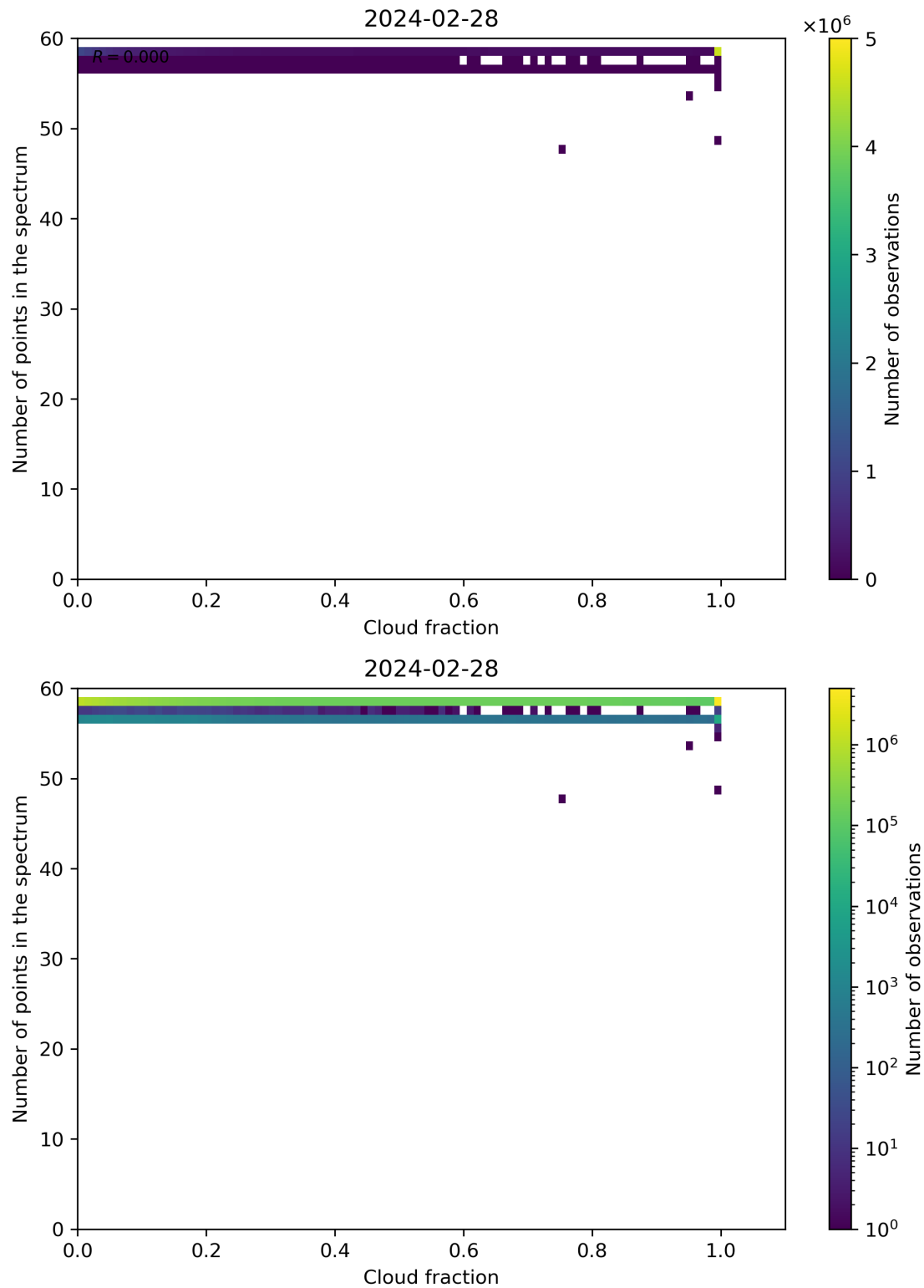
Figure 74: Scatter density plot of “Cloud fraction” against “Number of points in the spectrum” for 2024-02-27 to 2024-02-29.
