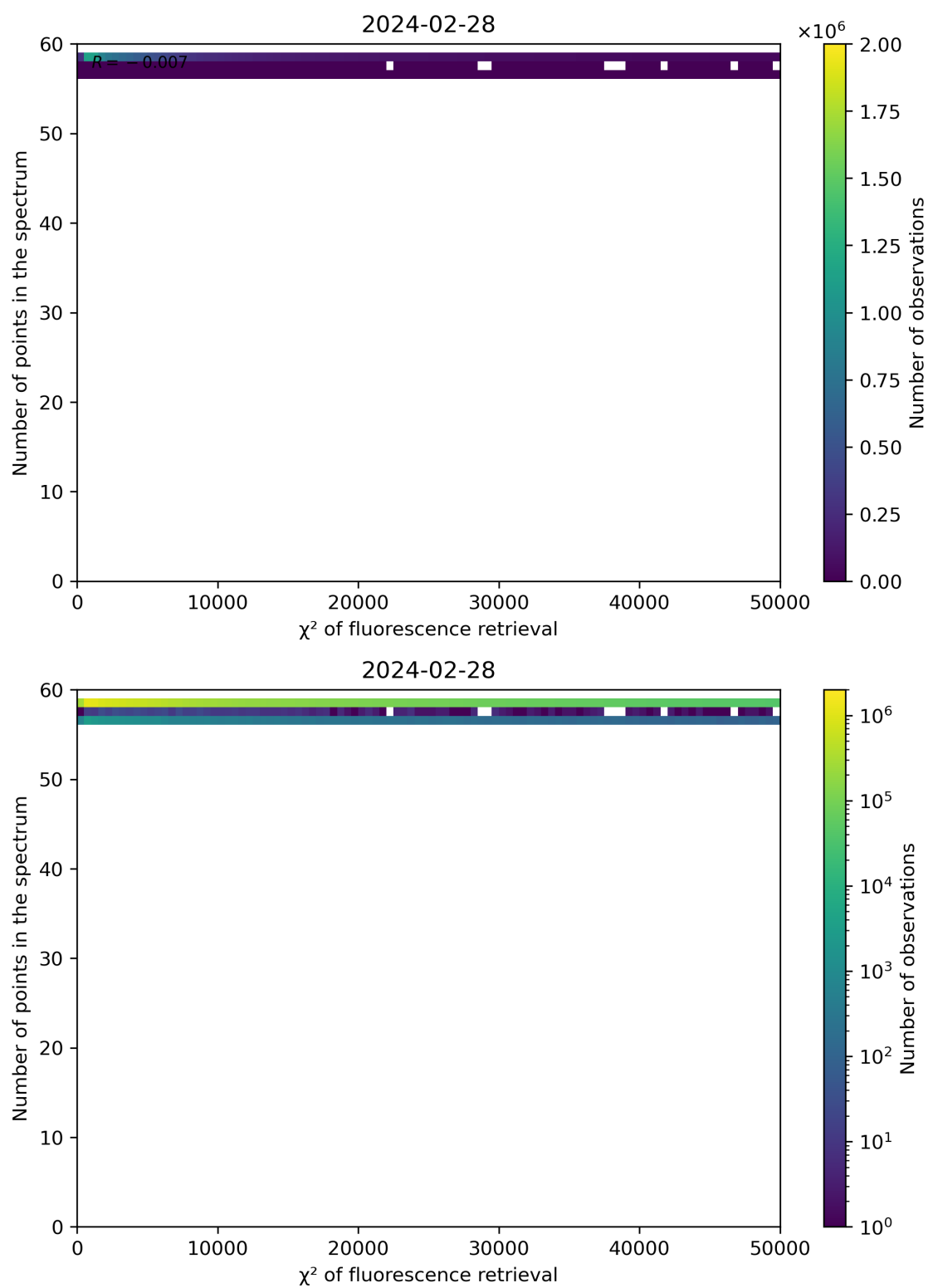
Figure 68: Scatter density plot of “ \chi^2 of fluorescence retrieval” against “Number of points in the spectrum” for 2024-02-27 to 2024-02-29.
