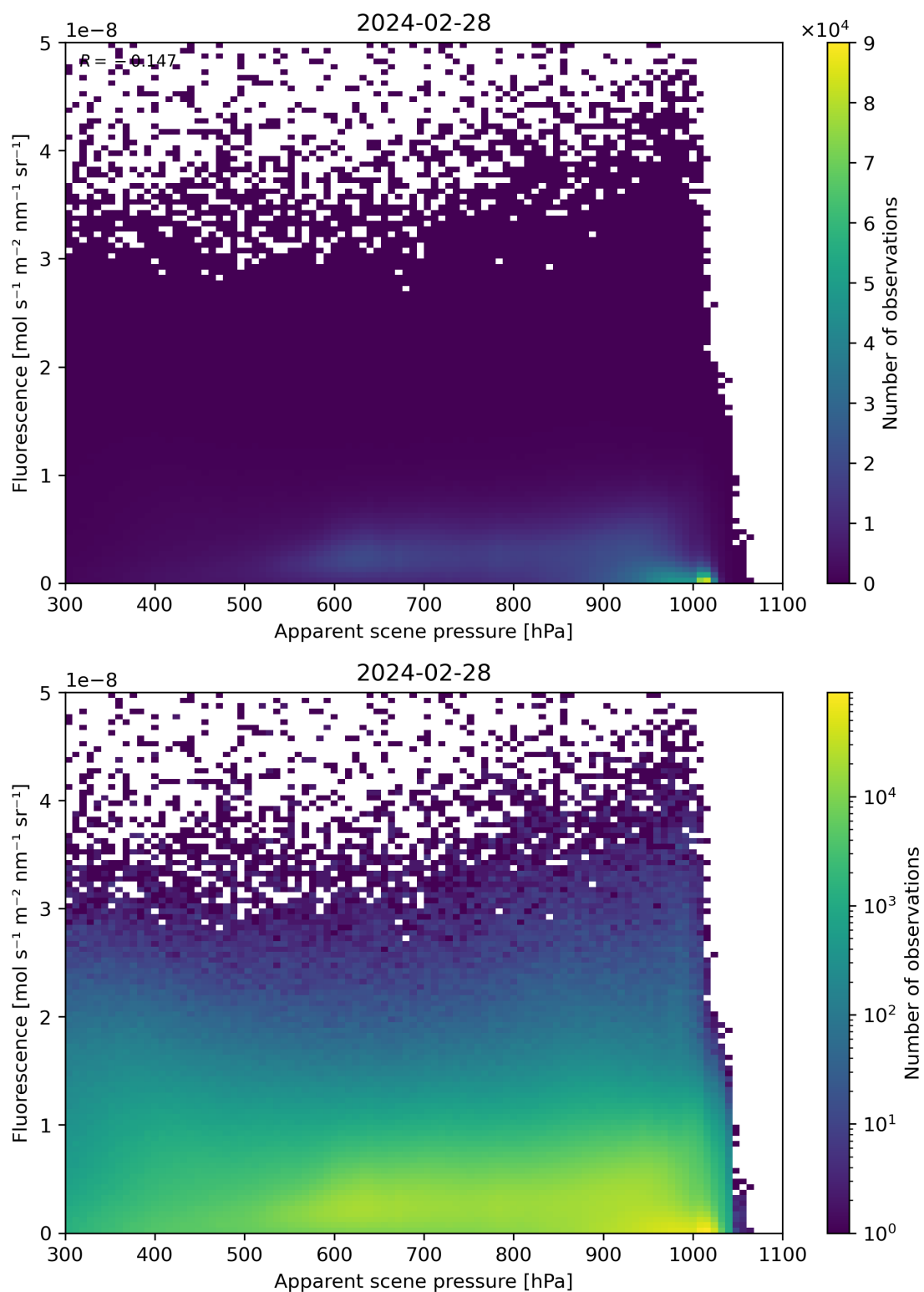
Figure 64: Scatter density plot of “Apparent scene pressure” against “Fluorescence” for 2024-02-27 to 2024-02-29.
