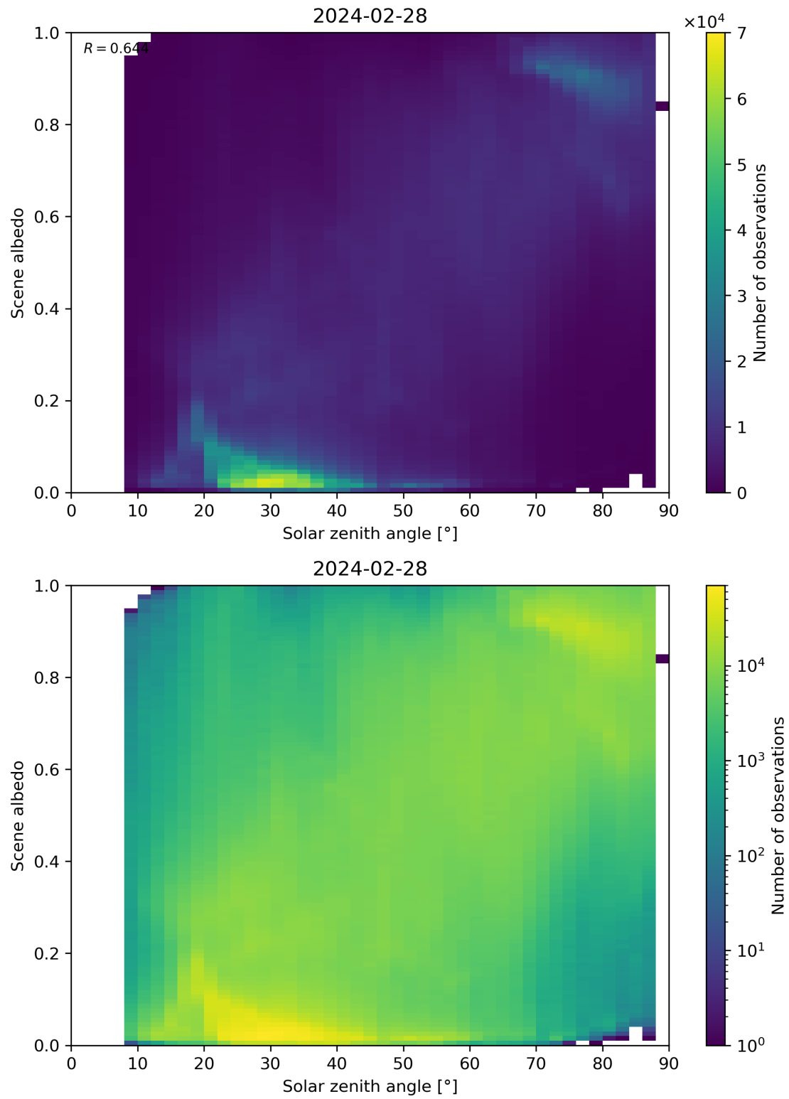
Figure 116: Scatter density plot of “Solar zenith angle” against “Scene albedo” for 2024-02-27 to 2024-02-29.
