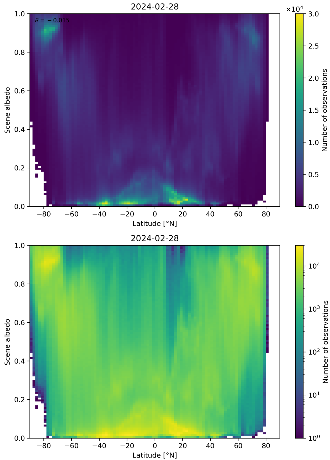
Figure 95: Scatter density plot of “Latitude” against “Scene albedo” for 2024-02-27 to 2024-02-29.
