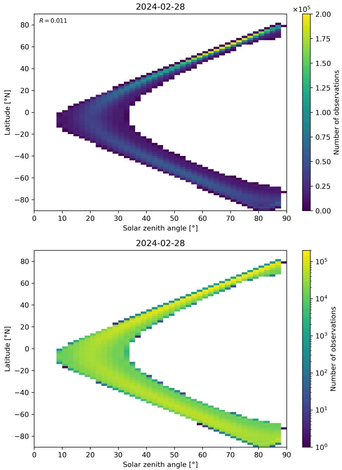
Figure 113: Scatter density plot of “Solar zenith angle” against “Latitude” for 2024-02-27 to 2024-02-29.
