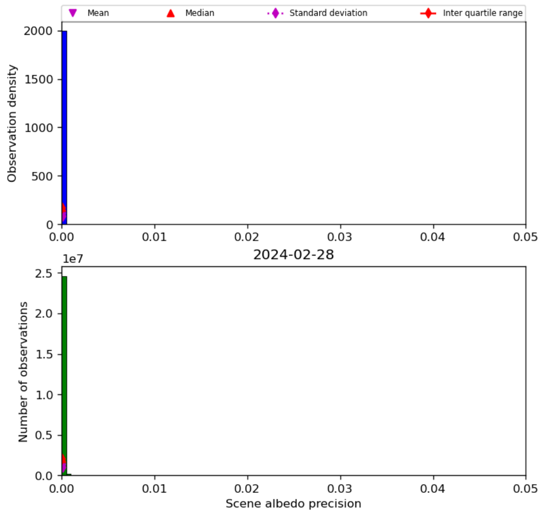
Figure 35: Histogram of “Scene albedo precision” for 2024-02-27 to 2024-02-29
