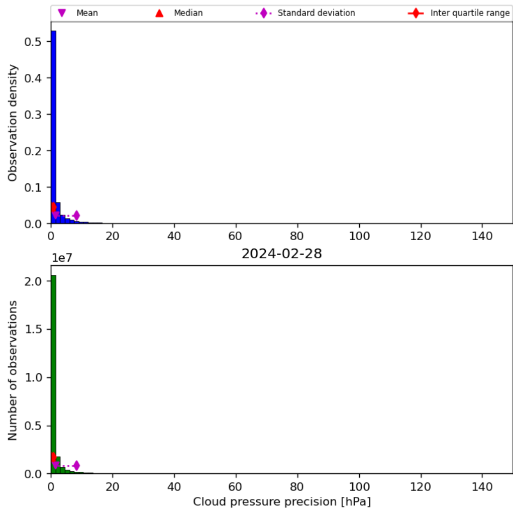
Figure 31: Histogram of “Cloud pressure precision” for 2024-02-27 to 2024-02-29
