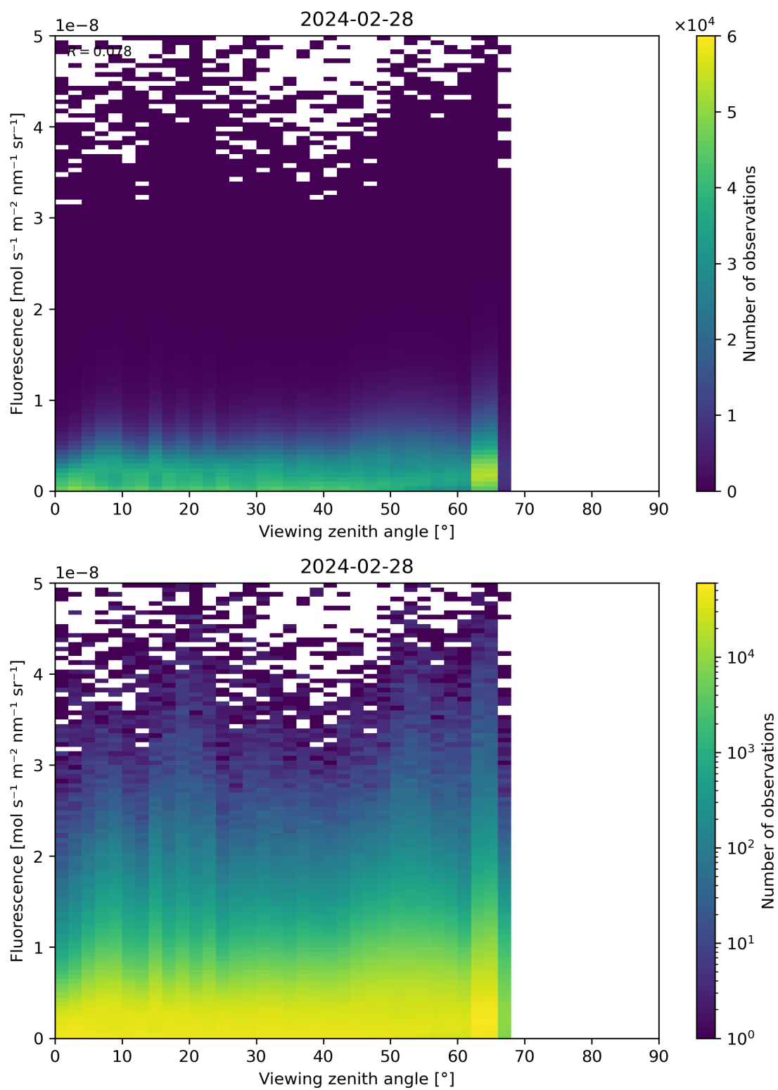
Figure 122: Scatter density plot of “Viewing zenith angle” against “Fluorescence” for 2024-02-27 to 2024-02-29.
