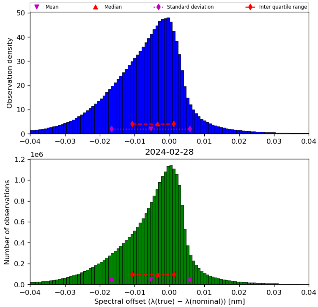
Figure 45: Histogram of “Spectral offset ( \lambda(\text{true}) - \lambda(\text{nominal}) )” for 2024-02-27 to 2024-02-29
