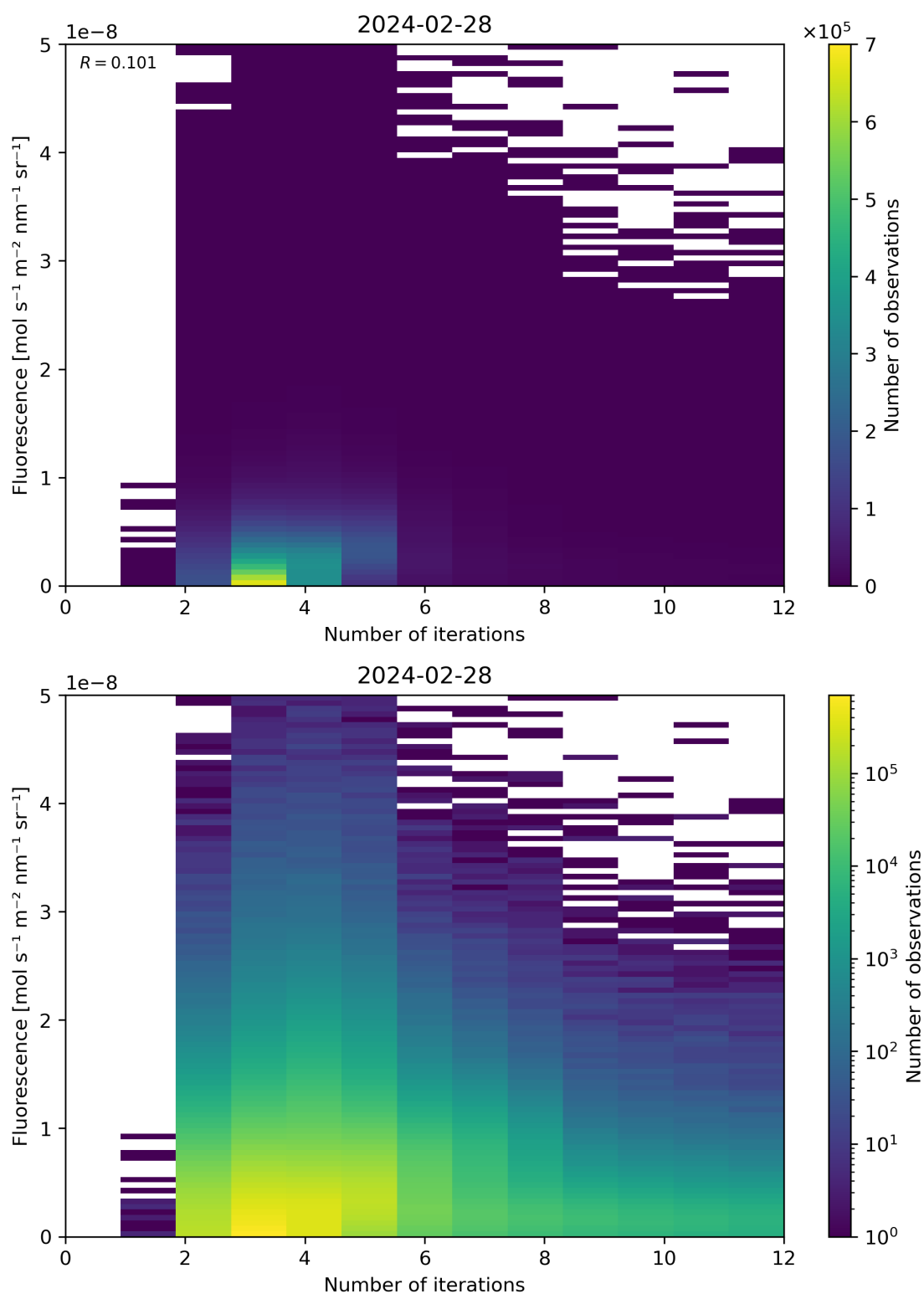
Figure 98: Scatter density plot of “Number of iterations” against “Fluorescence” for 2024-02-27 to 2024-02-29.
