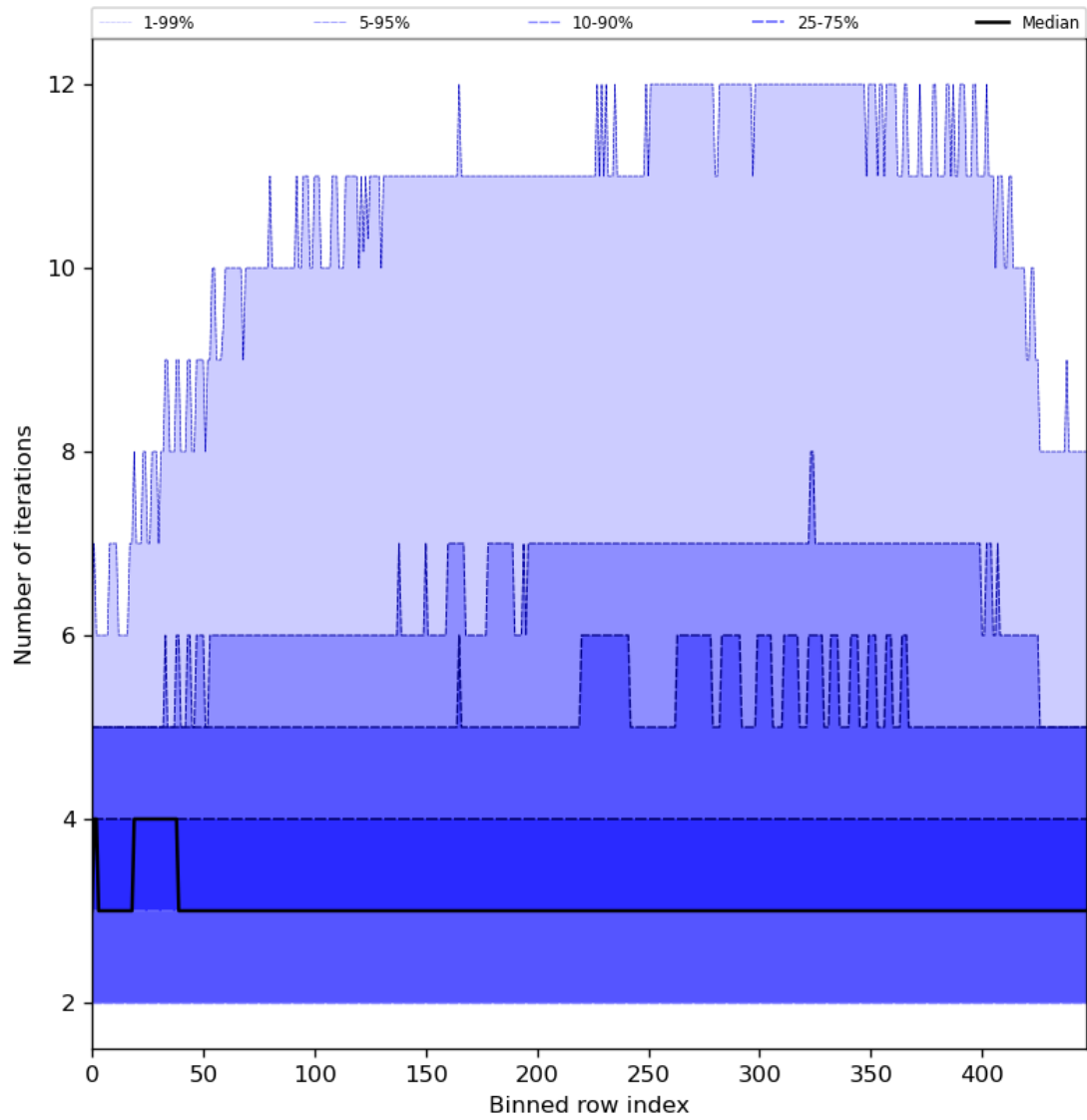
Figure 56: Along track statistics of “Number of iterations” for 2024-02-27 to 2024-02-29
