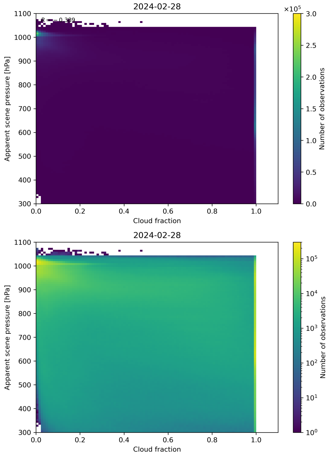
Figure 70: Scatter density plot of “Cloud fraction” against “Apparent scene pressure” for 2024-02-27 to 2024-02-29.
