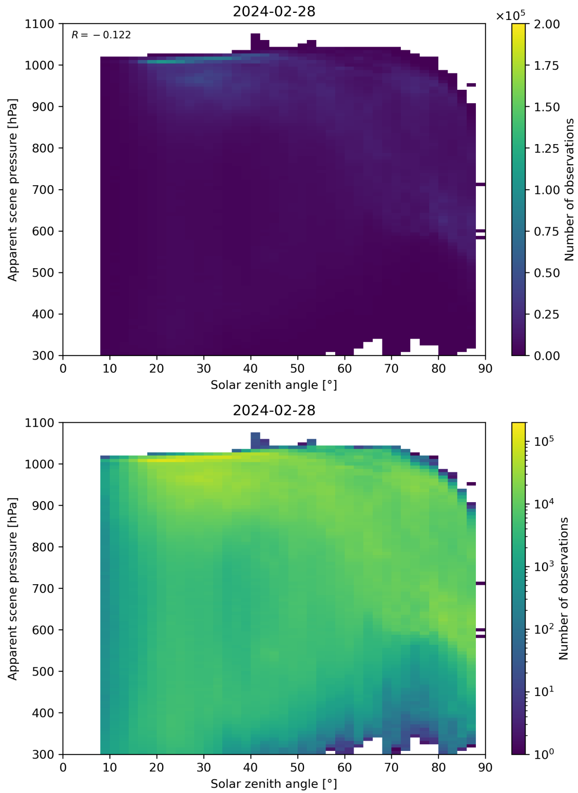
Figure 108: Scatter density plot of “Solar zenith angle” against “Apparent scene pressure” for 2024-02-27 to 2024-02-29.
