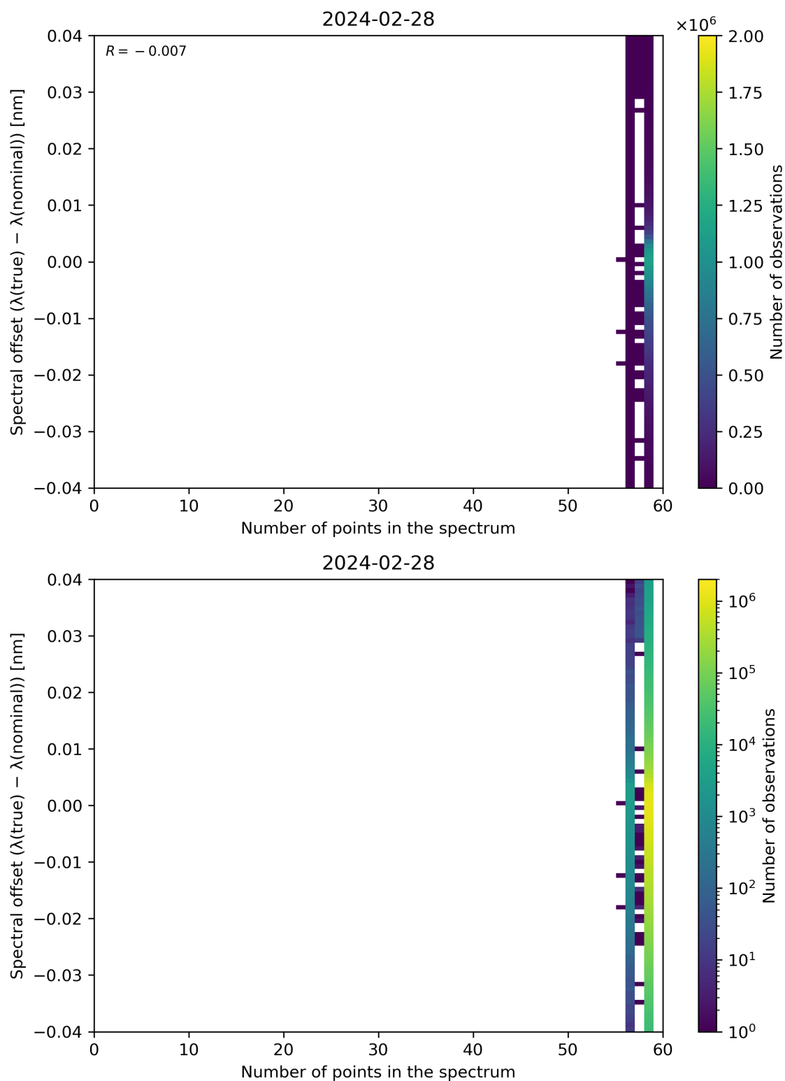
Figure 101: Scatter density plot of “Number of points in the spectrum” against “Spectral offset ( \lambda(\text{true}) - \lambda(\text{nominal}) )” for 2024-02-27 to 2024-02-29.
