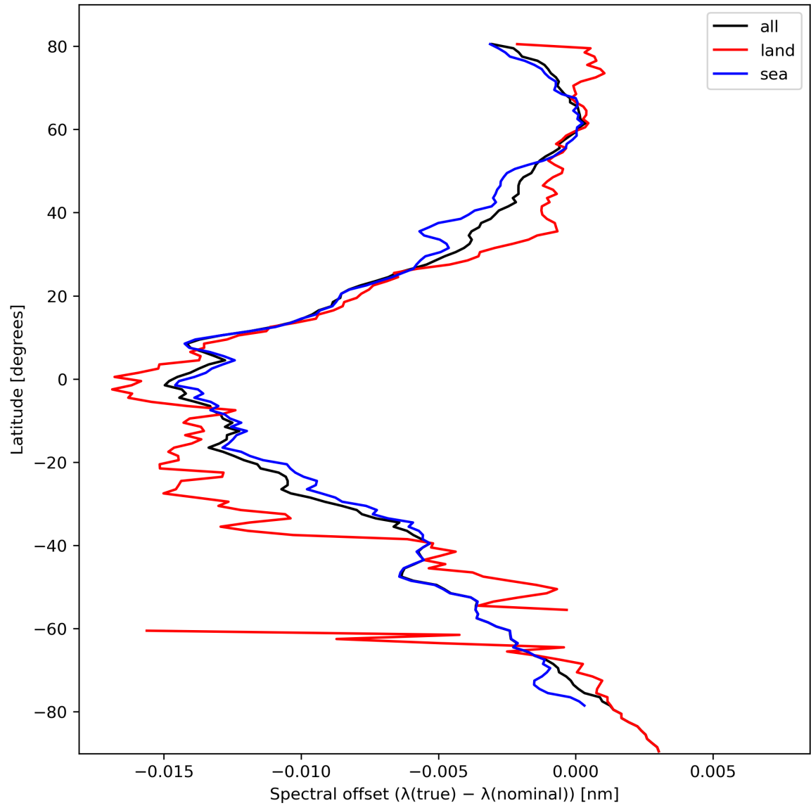
Figure 28: Zonal average of “Spectral offset ( \lambda(\text{true}) - \lambda(\text{nominal}) )” for 2024-02-27 to 2024-02-29.
