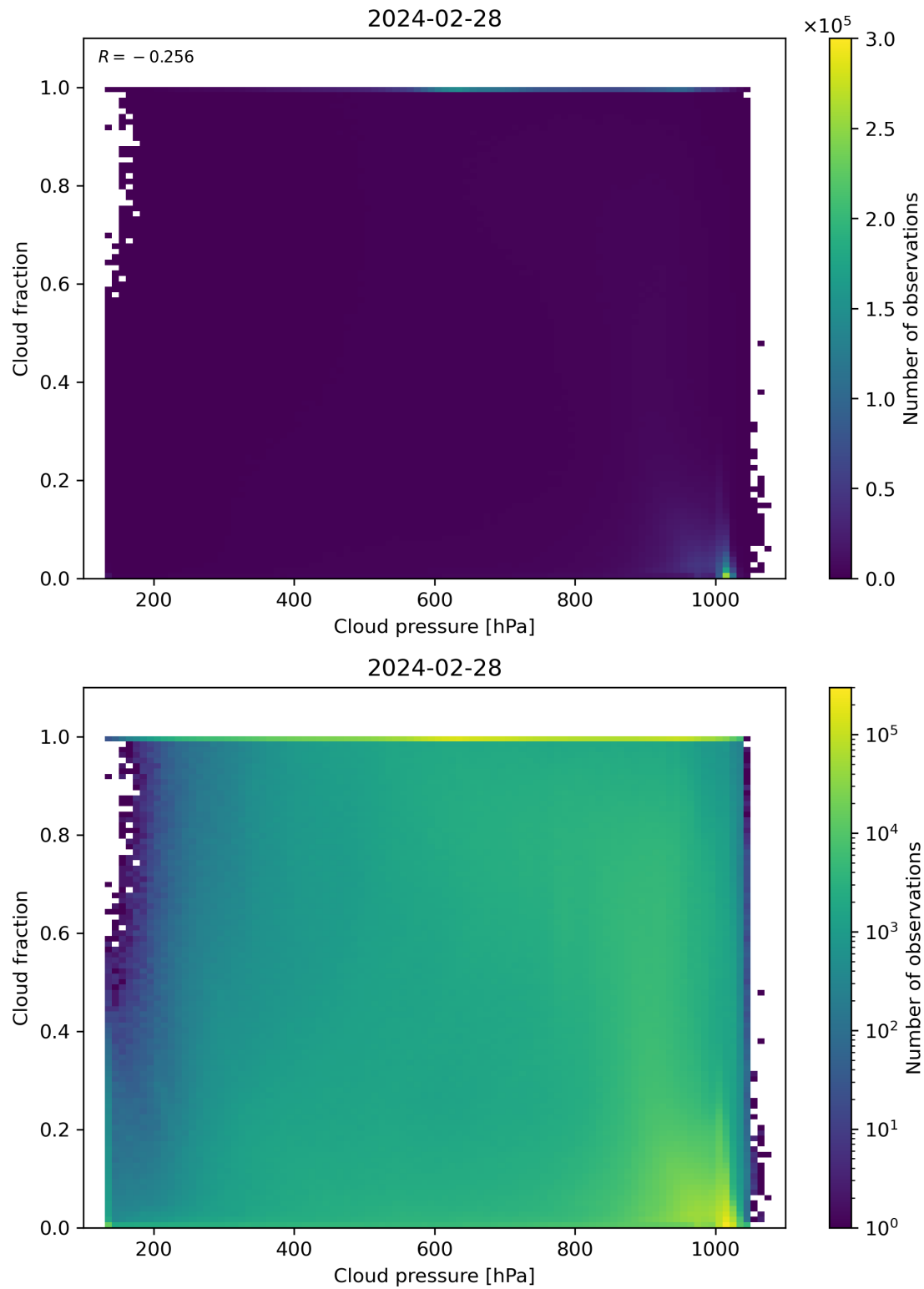
Figure 79: Scatter density plot of “Cloud pressure” against “Cloud fraction” for 2024-02-27 to 2024-02-29.
