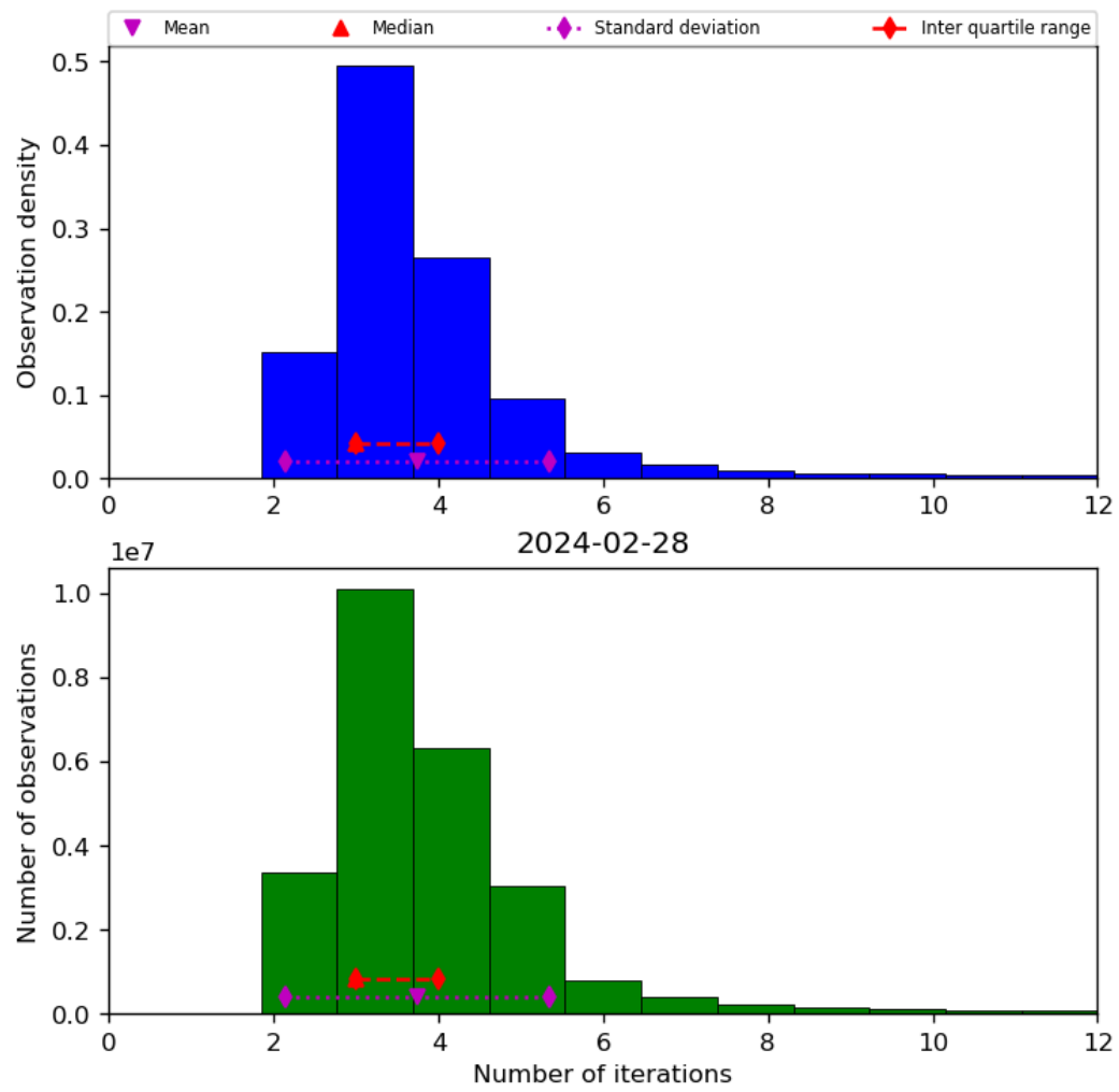
Figure 39: Histogram of “Number of iterations” for 2024-02-27 to 2024-02-29
