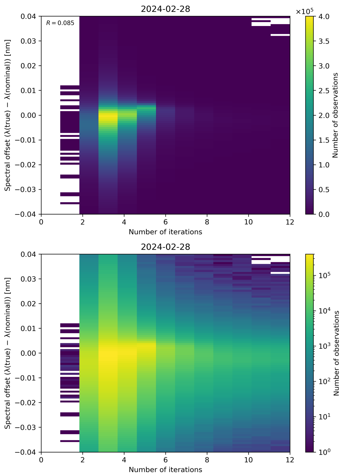
Figure 100: Scatter density plot of “Number of iterations” against “Spectral offset ( \lambda(\text{true}) - \lambda(\text{nominal}) )” for 2024-02-27 to 2024-02-29.
