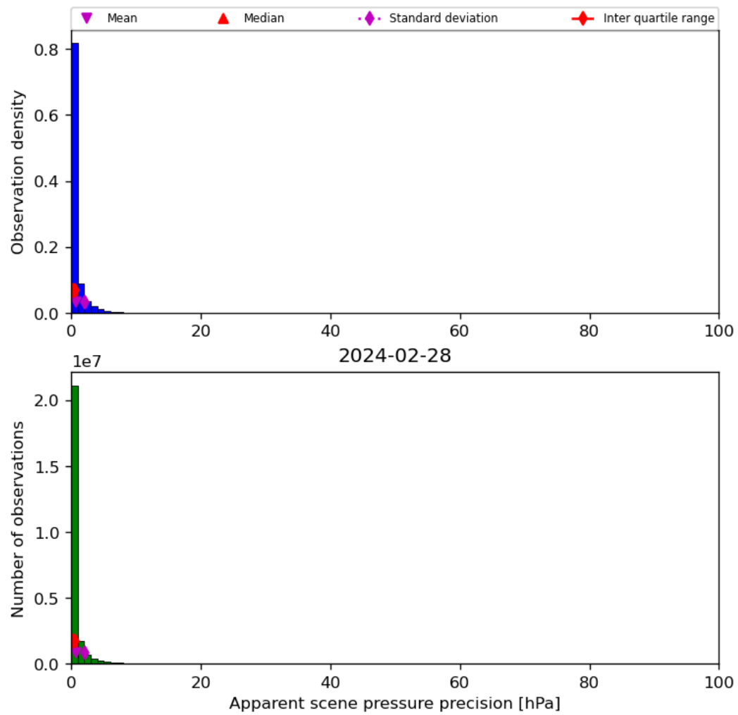
Figure 37: Histogram of “Apparent scene pressure precision” for 2024-02-27 to 2024-02-29
