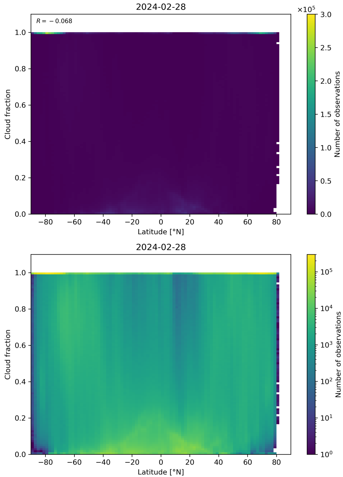
Figure 90: Scatter density plot of “Latitude” against “Cloud fraction” for 2024-02-27 to 2024-02-29.
