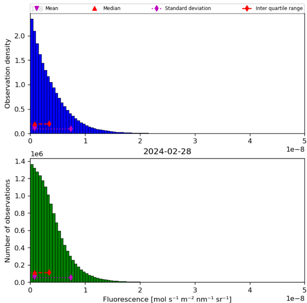
Figure 40: Histogram of “Fluorescence” for 2024-02-27 to 2024-02-29
