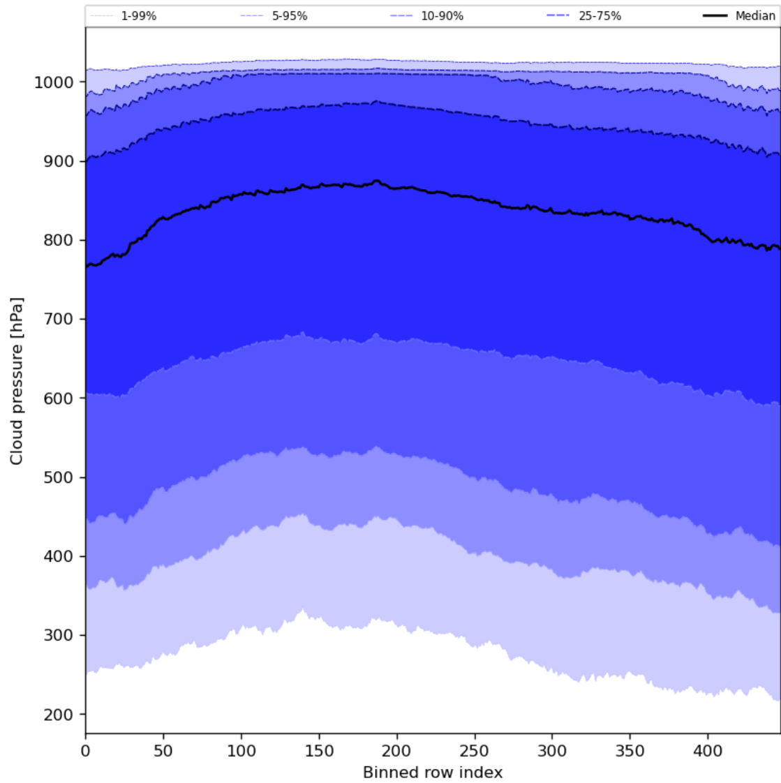
Figure 47: Along track statistics of “Cloud pressure” for 2024-02-27 to 2024-02-29
