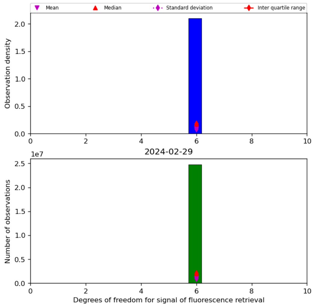
Figure 43: Histogram of “Degrees of freedom for signal of fluorescence retrieval” for 2024-02-28 to 2024-03-01
