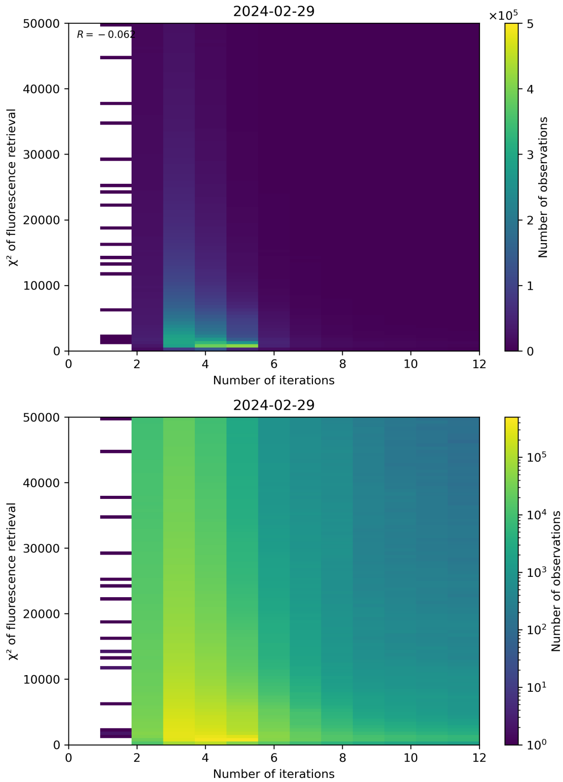
Figure 97: Scatter density plot of “Number of iterations” against “ \chi^2 of fluorescence retrieval” for 2024-02-28 to 2024-03-01.
