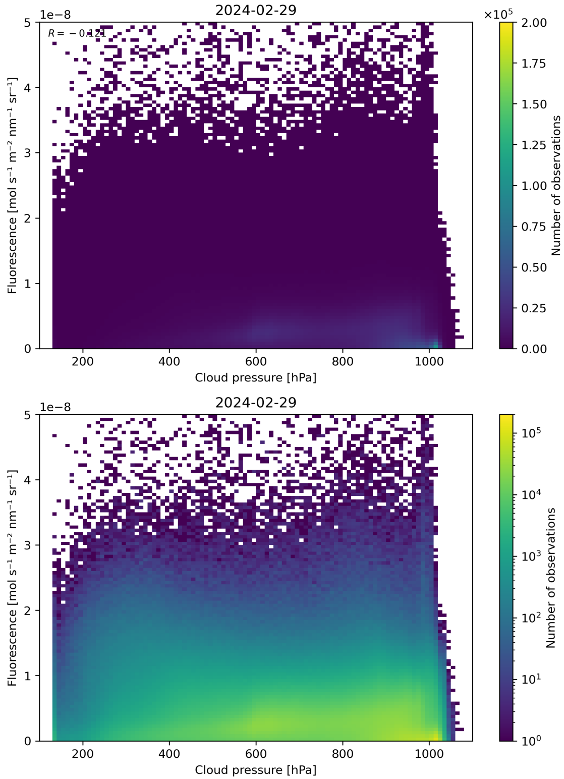
Figure 80: Scatter density plot of “Cloud pressure” against “Fluorescence” for 2024-02-28 to 2024-03-01.
