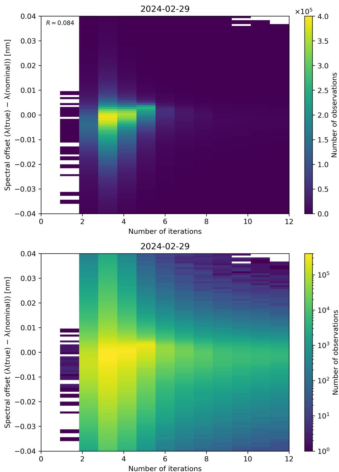
Figure 100: Scatter density plot of “Number of iterations” against “Spectral offset ( \lambda(\text{true}) - \lambda(\text{nominal}) )” for 2024-02-28 to 2024-03-01.
