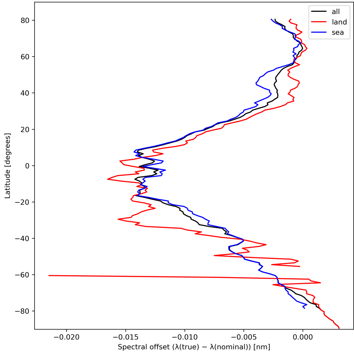
Figure 28: Zonal average of “Spectral offset ( \lambda(\text{true}) - \lambda(\text{nominal}) )” for 2024-02-28 to 2024-03-01.
