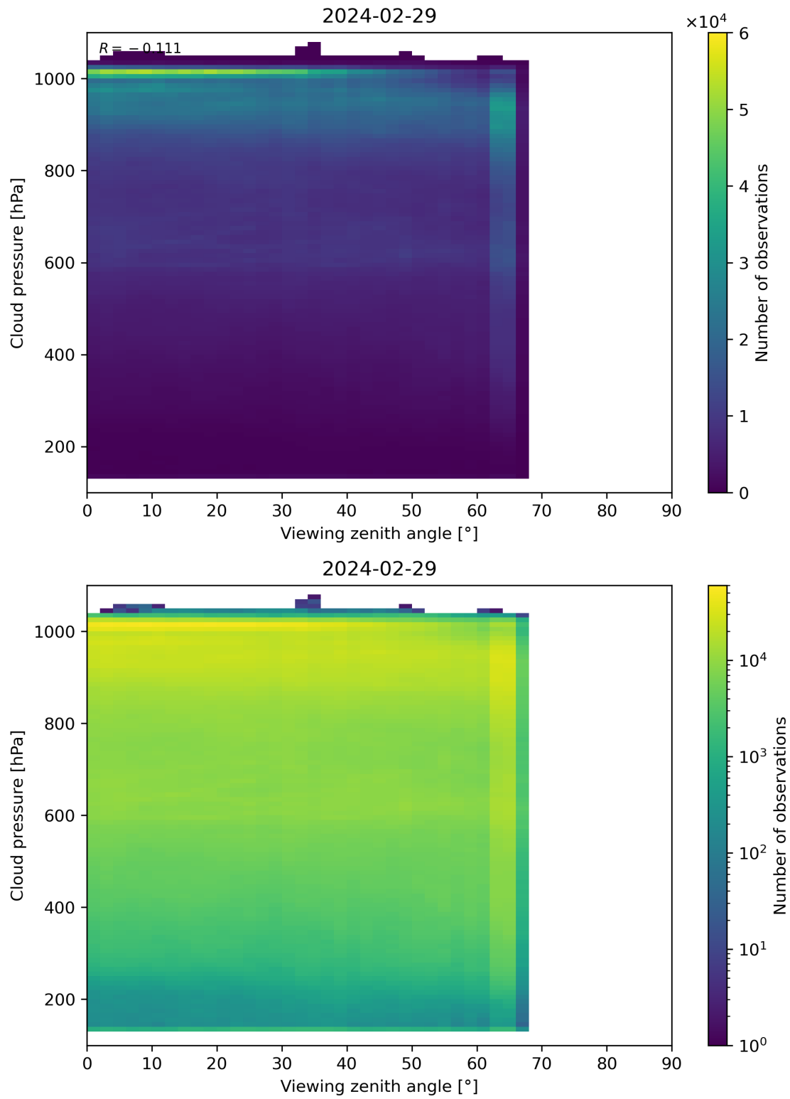
Figure 121: Scatter density plot of “Viewing zenith angle” against “Cloud pressure” for 2024-02-28 to 2024-03-01.
