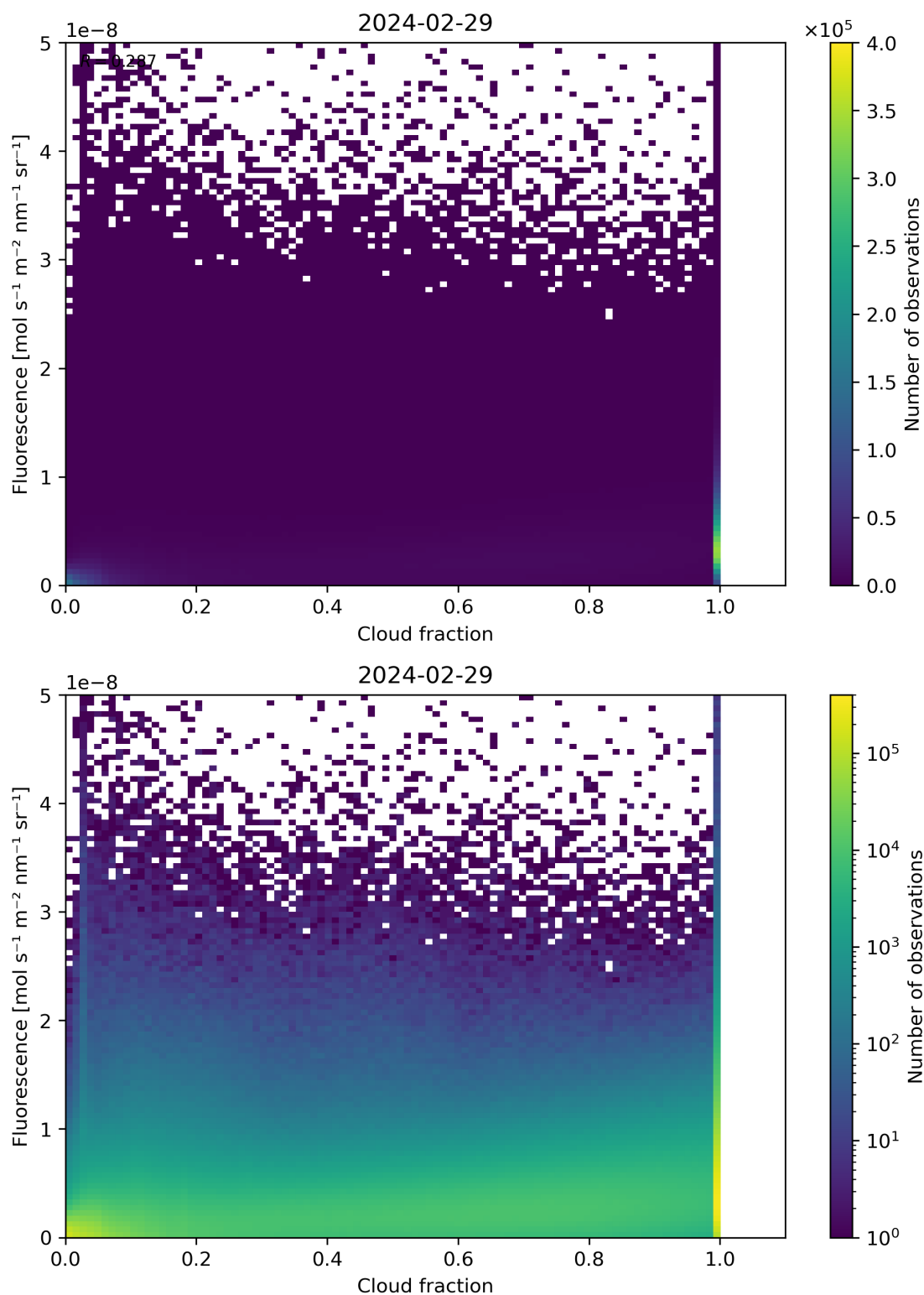
Figure 72: Scatter density plot of “Cloud fraction” against “Fluorescence” for 2024-02-28 to 2024-03-01.
