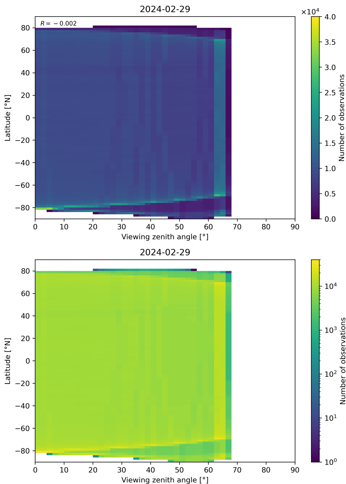
Figure 123: Scatter density plot of “Viewing zenith angle” against “Latitude” for 2024-02-28 to 2024-03-01.
