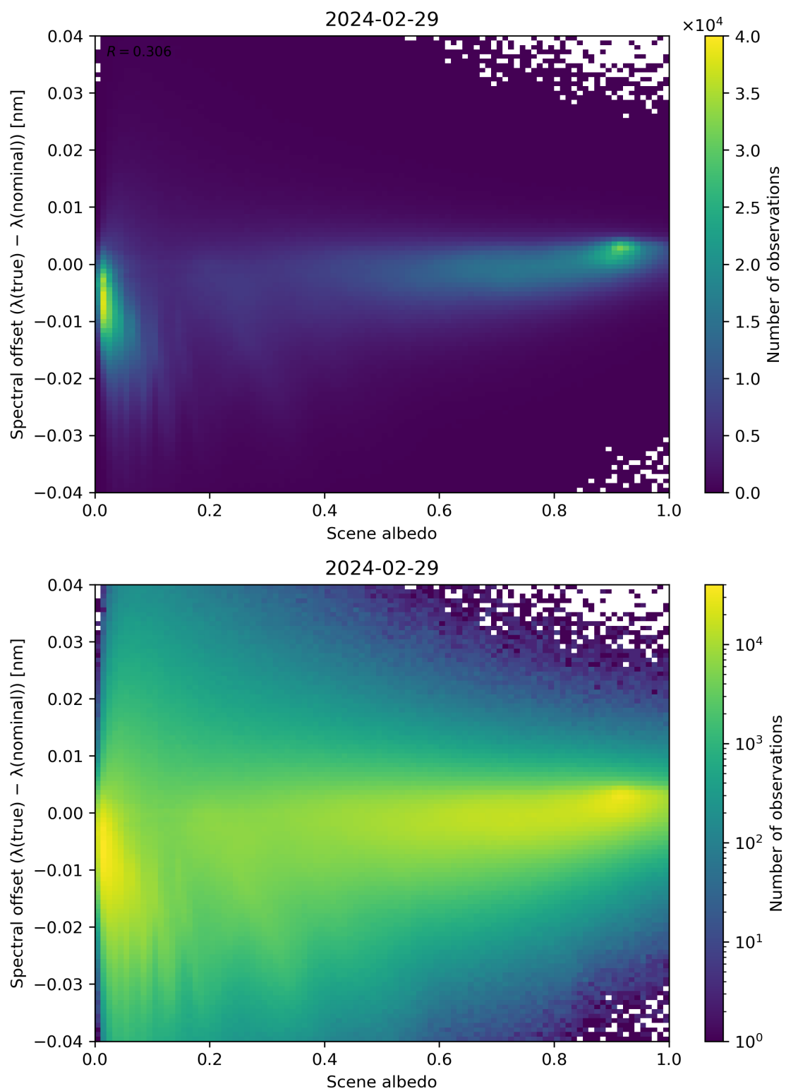
Figure 107: Scatter density plot of “Scene albedo” against “Spectral offset ( \lambda(\text{true}) - \lambda(\text{nominal}) )” for 2024-02-28 to 2024-03-01.
