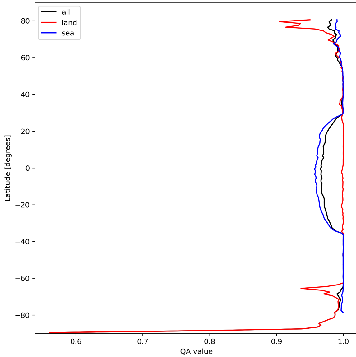
Figure 12: Zonal average of “QA value” for 2024-02-28 to 2024-03-01.
