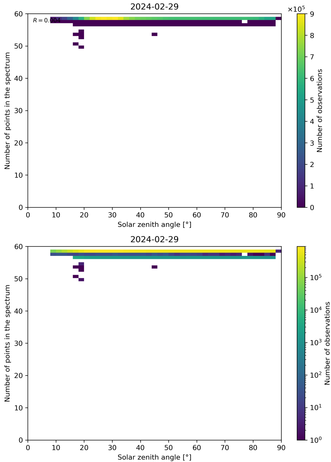
Figure 115: Scatter density plot of “Solar zenith angle” against “Number of points in the spectrum” for 2024-02-28 to 2024-03-01.
