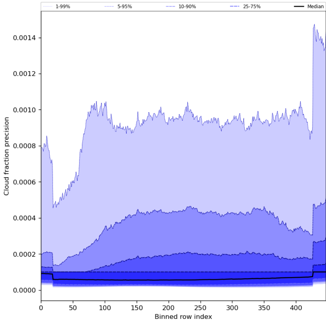
Figure 50: Along track statistics of “Cloud fraction precision” for 2024-02-28 to 2024-03-01
