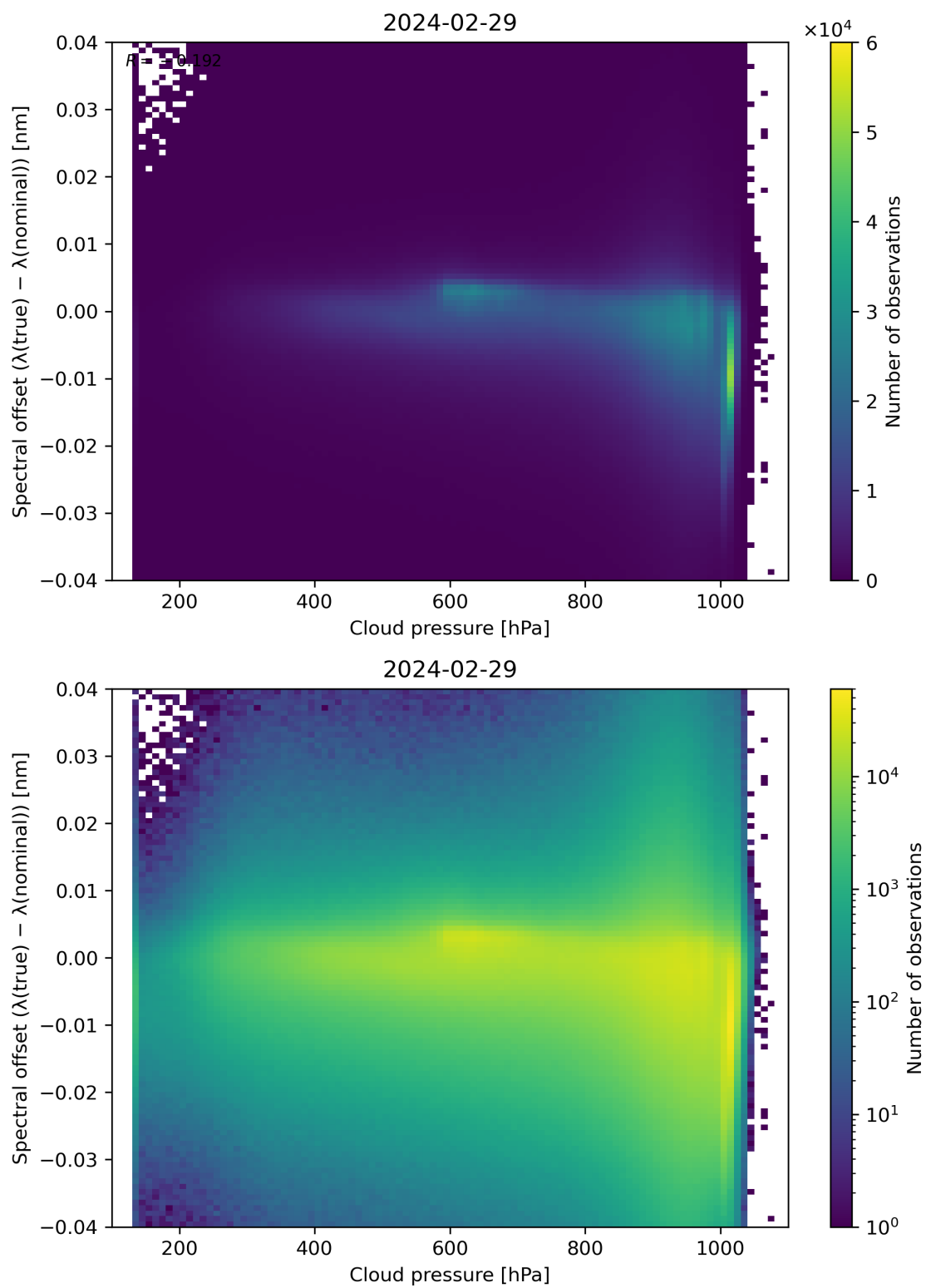
Figure 84: Scatter density plot of “Cloud pressure” against “Spectral offset ( \lambda(\text{true}) - \lambda(\text{nominal}) )” for 2024-02-28 to 2024-03-01.
