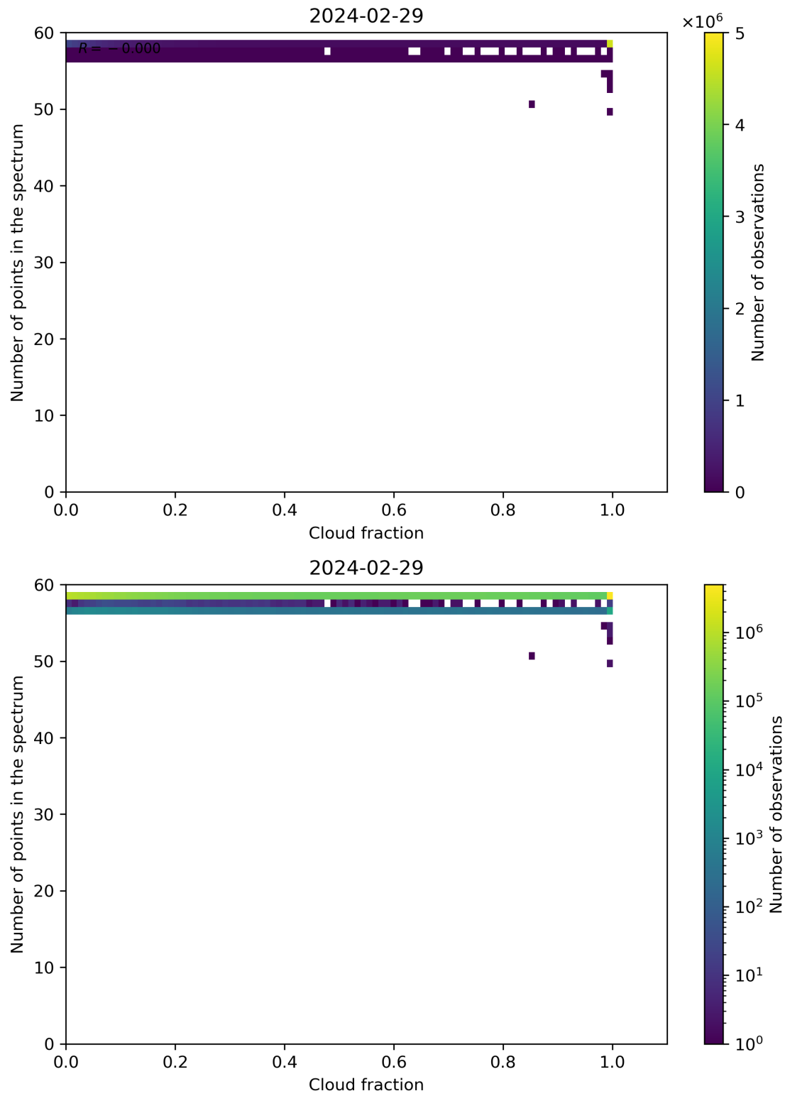
Figure 74: Scatter density plot of “Cloud fraction” against “Number of points in the spectrum” for 2024-02-28 to 2024-03-01.
