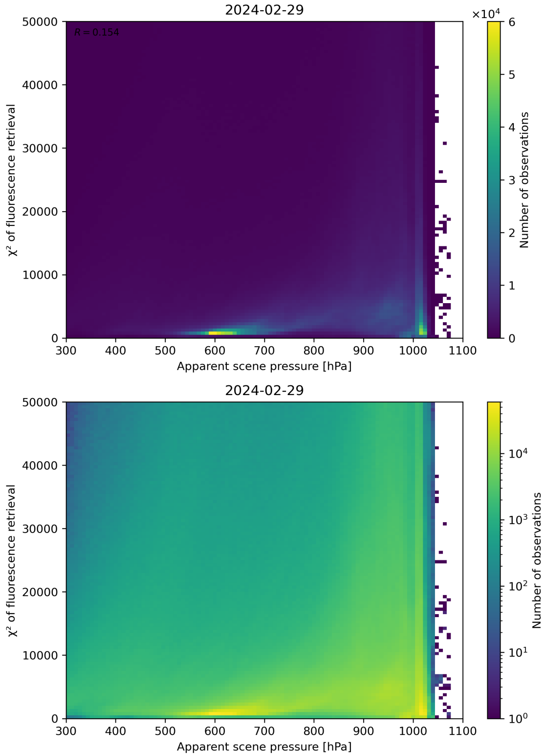
Figure 63: Scatter density plot of “Apparent scene pressure” against “ \chi^2 of fluorescence retrieval” for 2024-02-28 to 2024-03-01.
