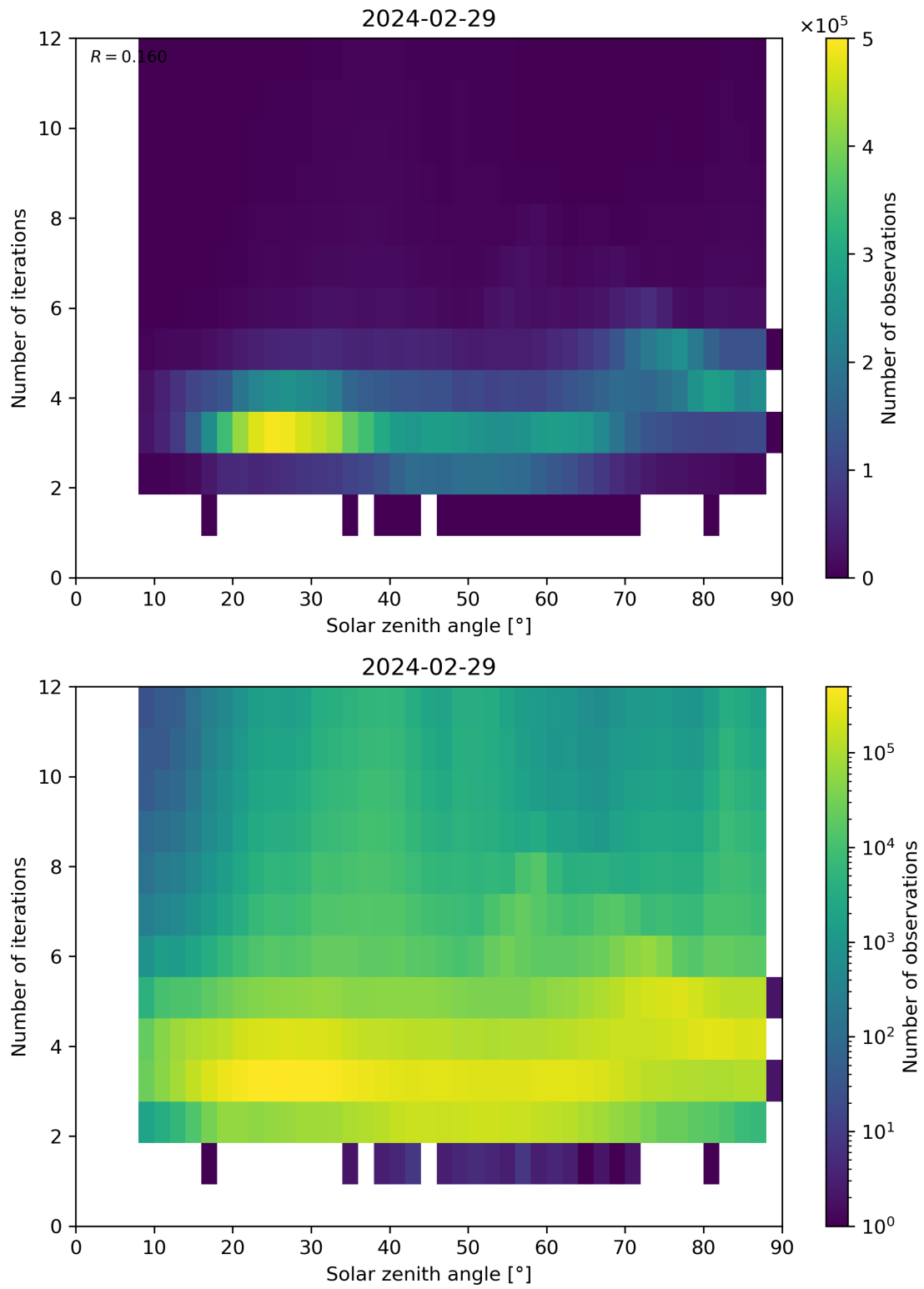
Figure 114: Scatter density plot of “Solar zenith angle” against “Number of iterations” for 2024-02-28 to 2024-03-01.
