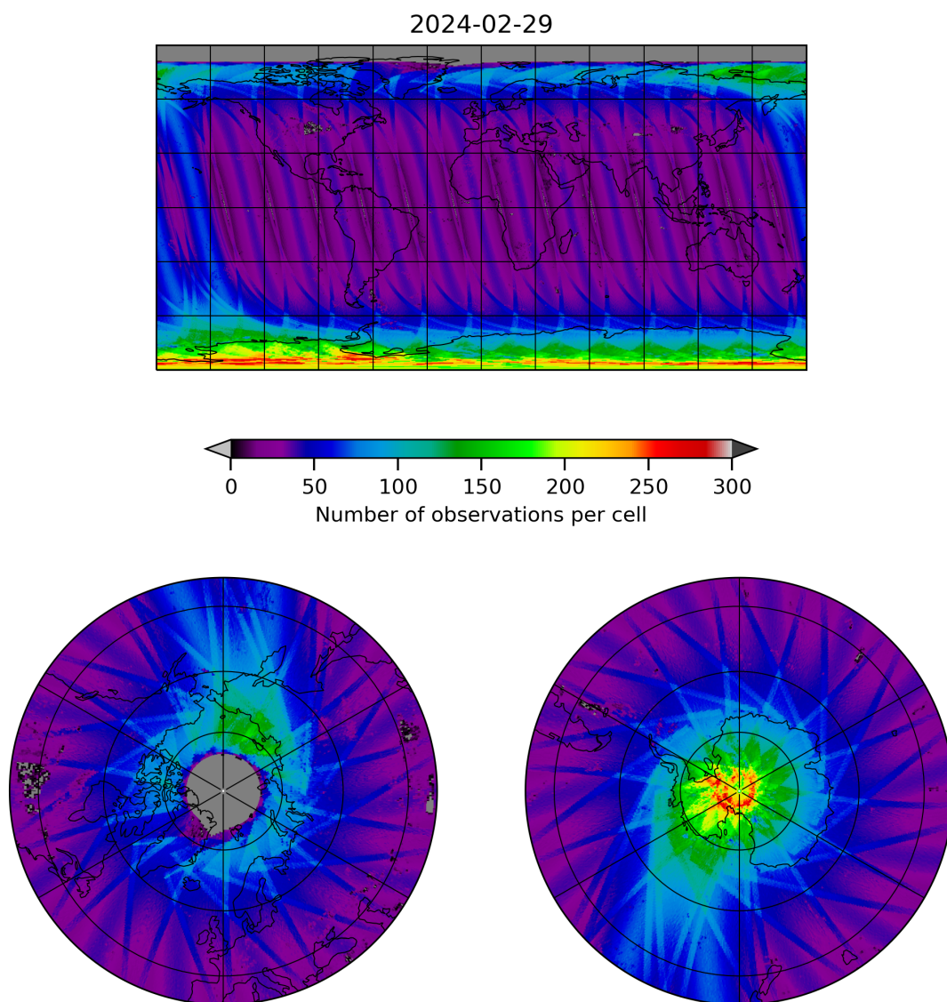
Figure 11: Map of the number of observations for 2024-02-28 to 2024-03-01
