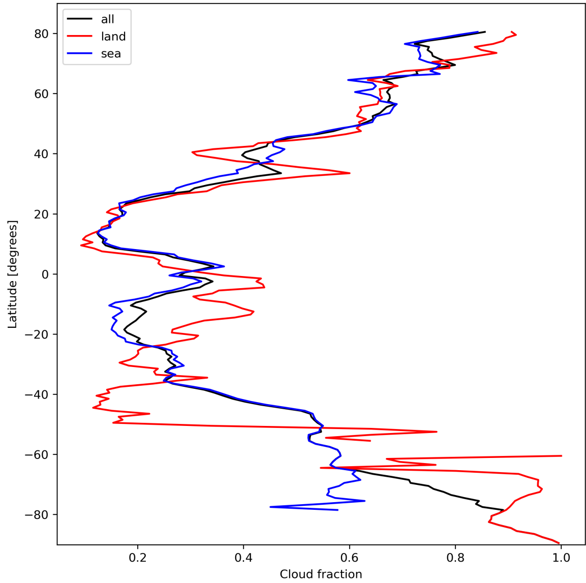
Figure 15: Zonal average of “Cloud fraction” for 2024-02-28 to 2024-03-01.
