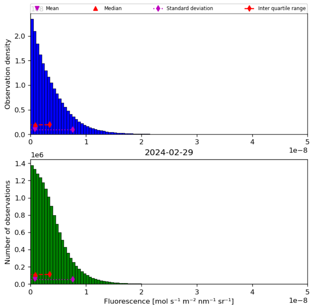
Figure 40: Histogram of “Fluorescence” for 2024-02-28 to 2024-03-01
