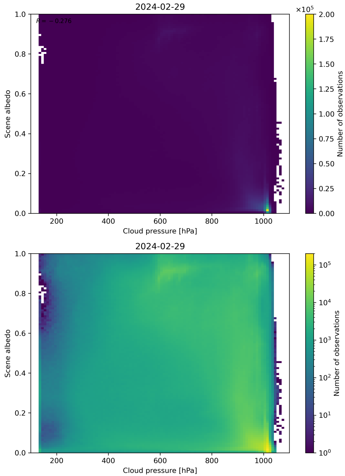
Figure 83: Scatter density plot of “Cloud pressure” against “Scene albedo” for 2024-02-28 to 2024-03-01.
