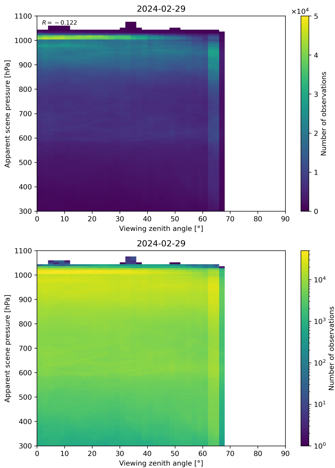
Figure 118: Scatter density plot of “Viewing zenith angle” against “Apparent scene pressure” for 2024-02-28 to 2024-03-01.
