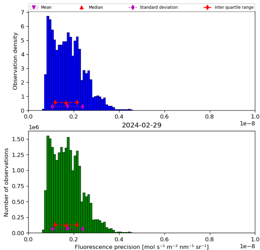
Figure 41: Histogram of “Fluorescence precision” for 2024-02-28 to 2024-03-01
