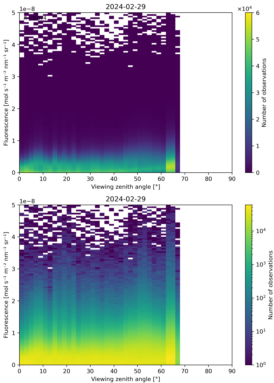
Figure 122: Scatter density plot of “Viewing zenith angle” against “Fluorescence” for 2024-02-28 to 2024-03-01.
