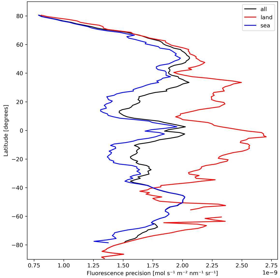
Figure 24: Zonal average of “Fluorescence precision” for 2024-02-28 to 2024-03-01.
