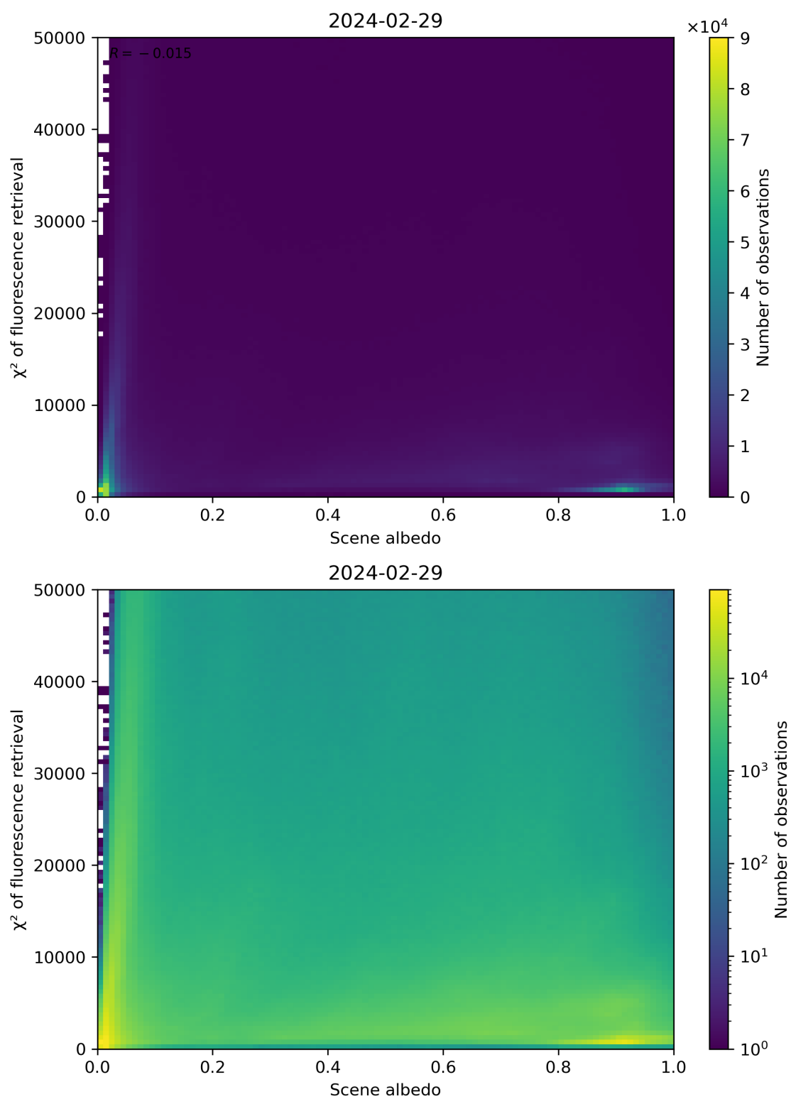
Figure 103: Scatter density plot of “Scene albedo” against “ \chi^2 of fluorescence retrieval” for 2024-02-28 to 2024-03-01.
