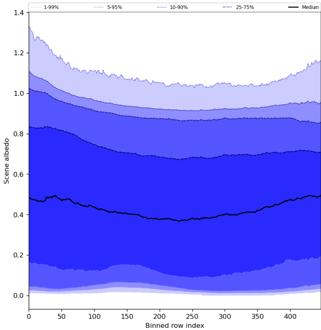
Figure 51: Along track statistics of “Scene albedo” for 2024-02-28 to 2024-03-01
