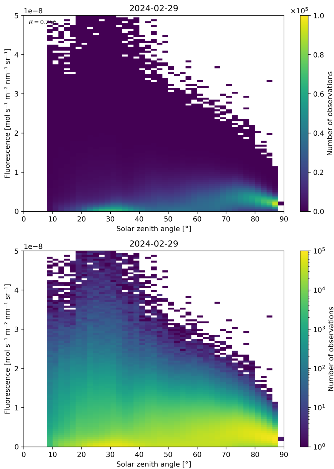
Figure 112: Scatter density plot of “Solar zenith angle” against “Fluorescence” for 2024-02-28 to 2024-03-01.
