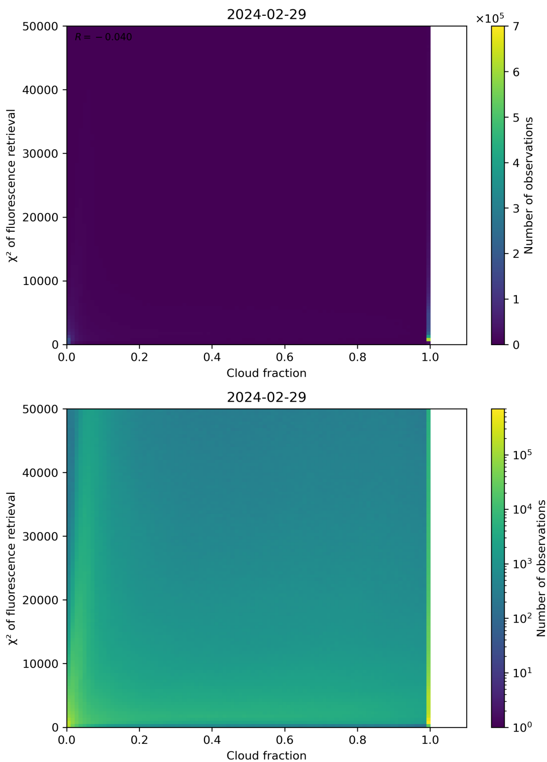
Figure 71: Scatter density plot of “Cloud fraction” against “ \chi^2 of fluorescence retrieval” for 2024-02-28 to 2024-03-01.
