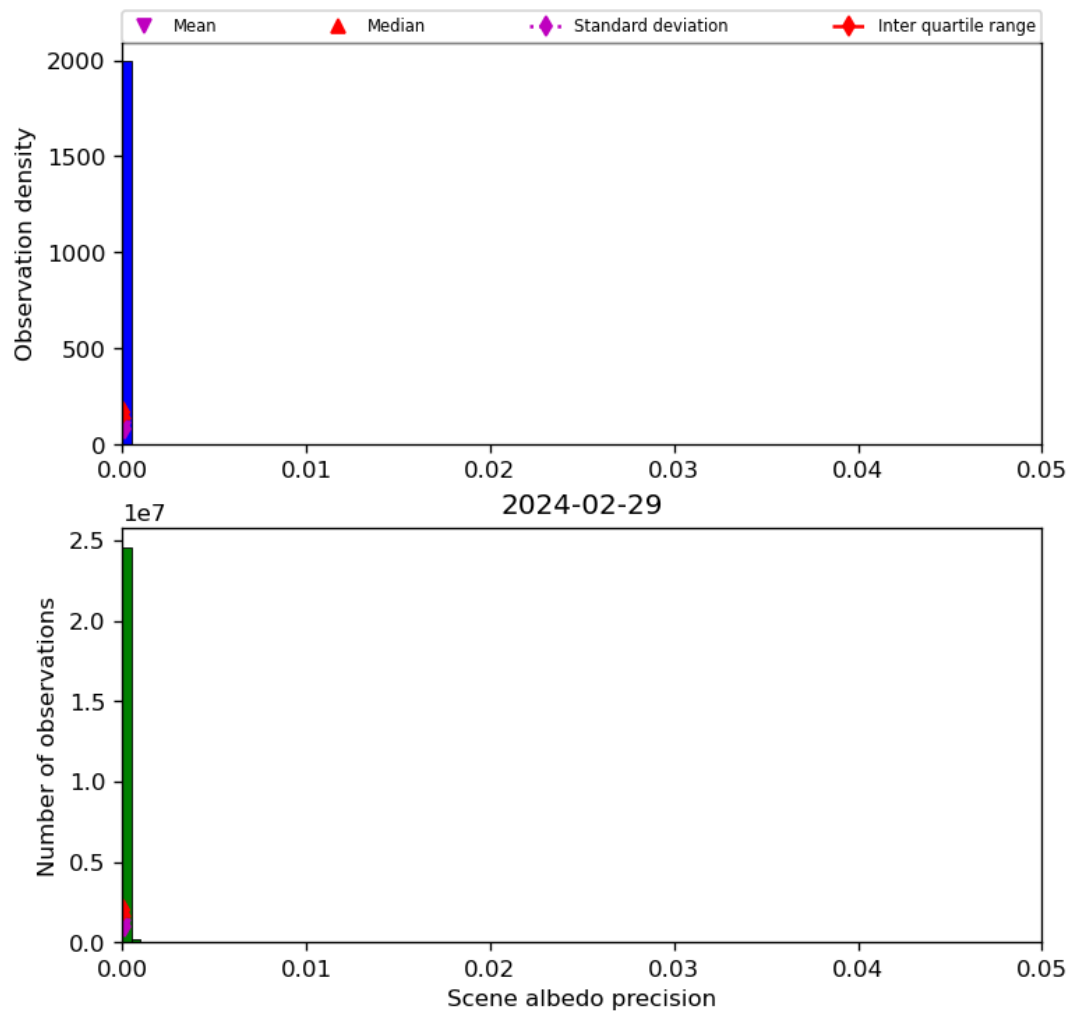
Figure 35: Histogram of “Scene albedo precision” for 2024-02-28 to 2024-03-01
