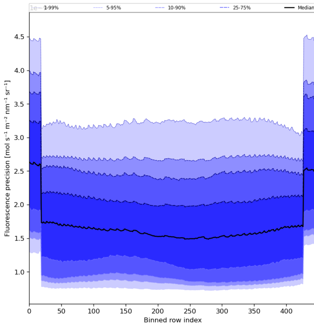
Figure 58: Along track statistics of “Fluorescence precision” for 2024-02-28 to 2024-03-01
