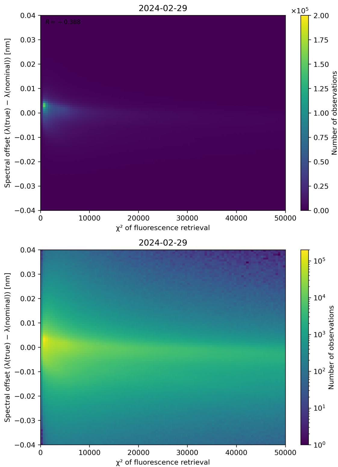
Figure 69: Scatter density plot of " \chi^2 of fluorescence retrieval" against "Spectral offset ( \lambda(\text{true}) - \lambda(\text{nominal})) " for 2024-02-28 to 2024-03-01.
