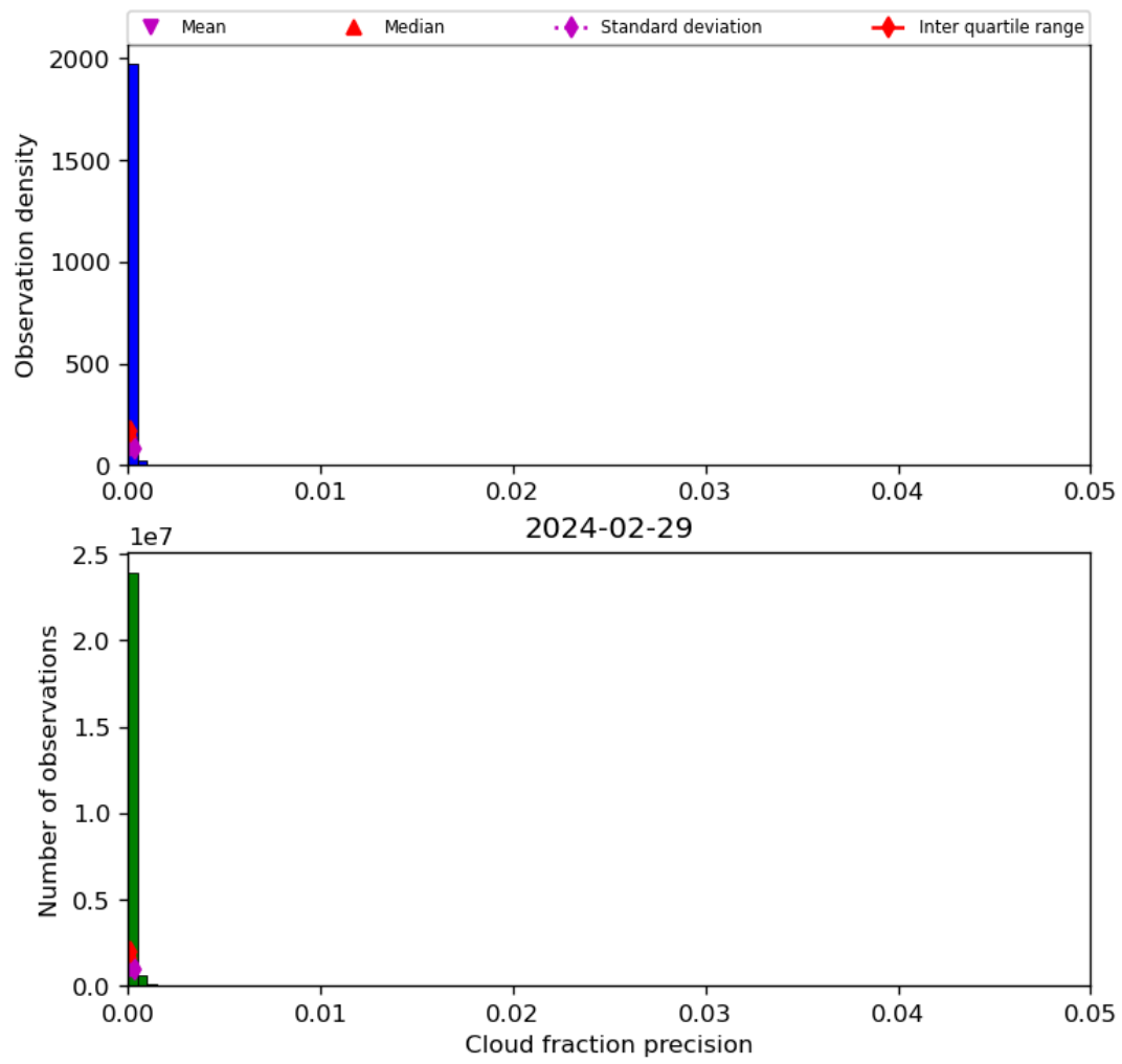
Figure 33: Histogram of “Cloud fraction precision” for 2024-02-28 to 2024-03-01
