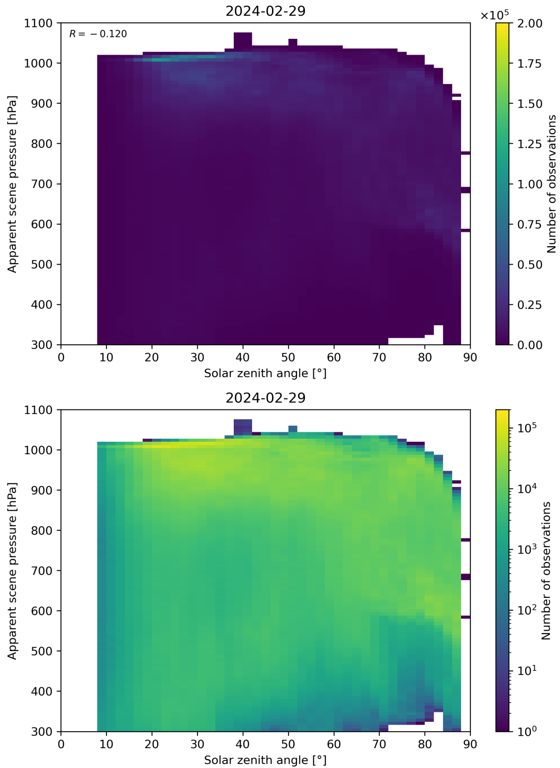
Figure 108: Scatter density plot of “Solar zenith angle” against “Apparent scene pressure” for 2024-02-28 to 2024-03-01.
