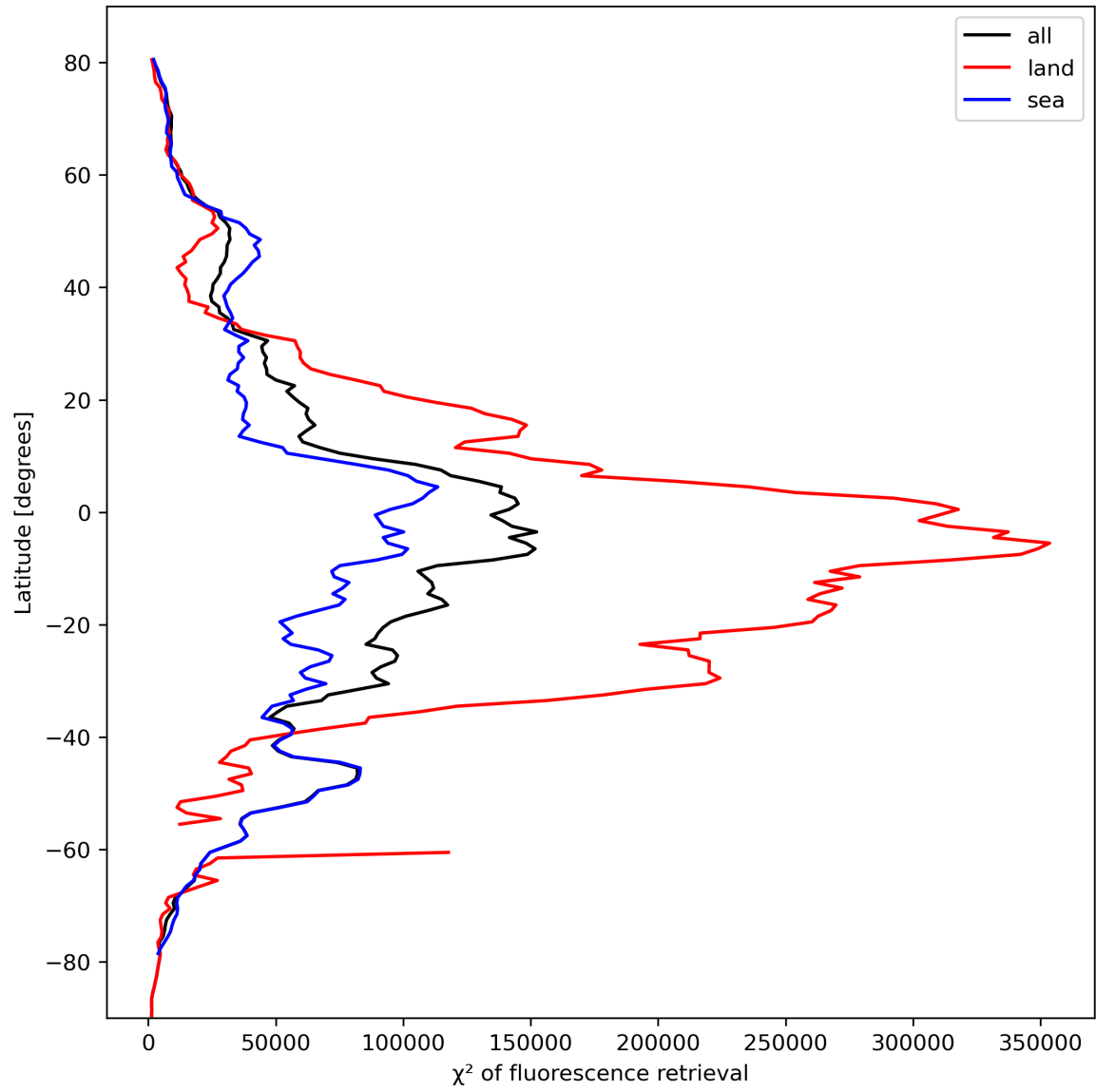
Figure 25: Zonal average of “ \chi^2 of fluorescence retrieval” for 2024-02-28 to 2024-03-01.
