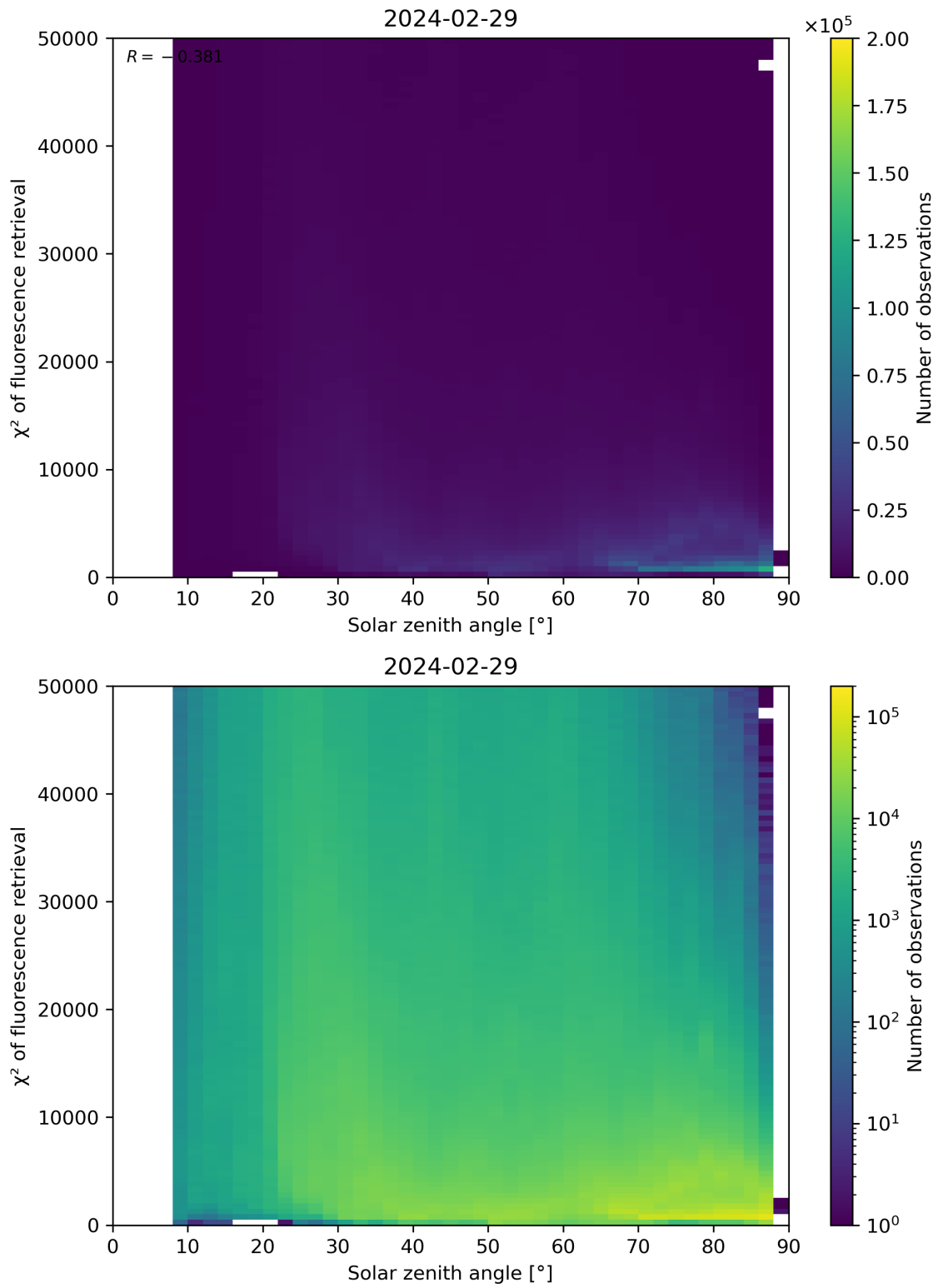
Figure 109: Scatter density plot of “Solar zenith angle” against “ \chi^2 of fluorescence retrieval” for 2024-02-28 to 2024-03-01.
