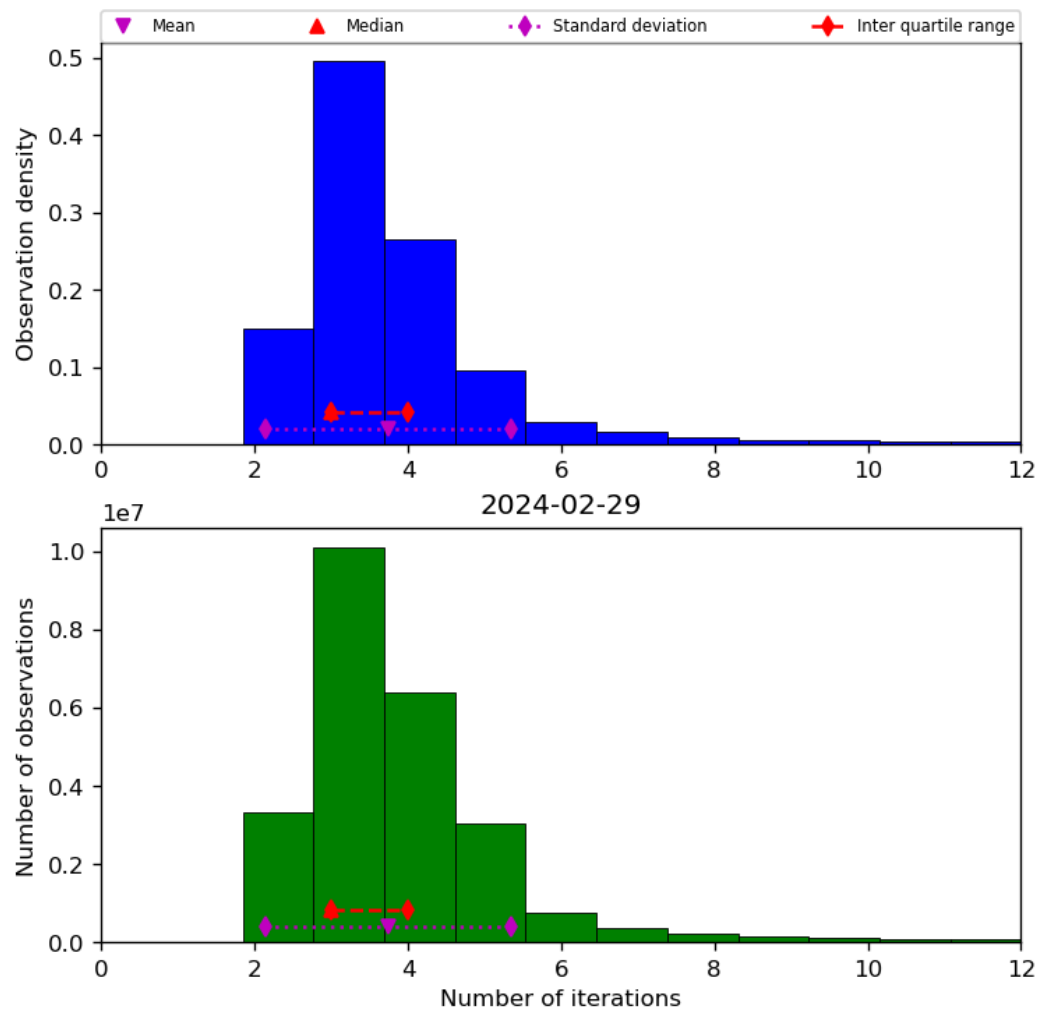
Figure 39: Histogram of “Number of iterations” for 2024-02-28 to 2024-03-01
