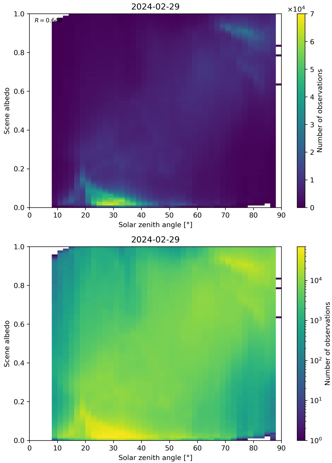
Figure 116: Scatter density plot of “Solar zenith angle” against “Scene albedo” for 2024-02-28 to 2024-03-01.
