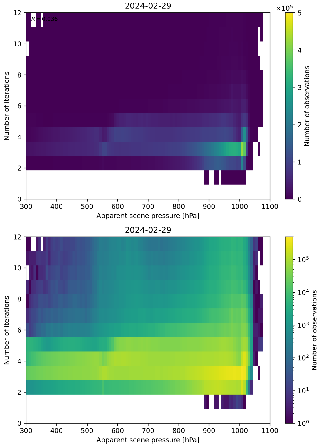
Figure 65: Scatter density plot of “Apparent scene pressure” against “Number of iterations” for 2024-02-28 to 2024-03-01.
