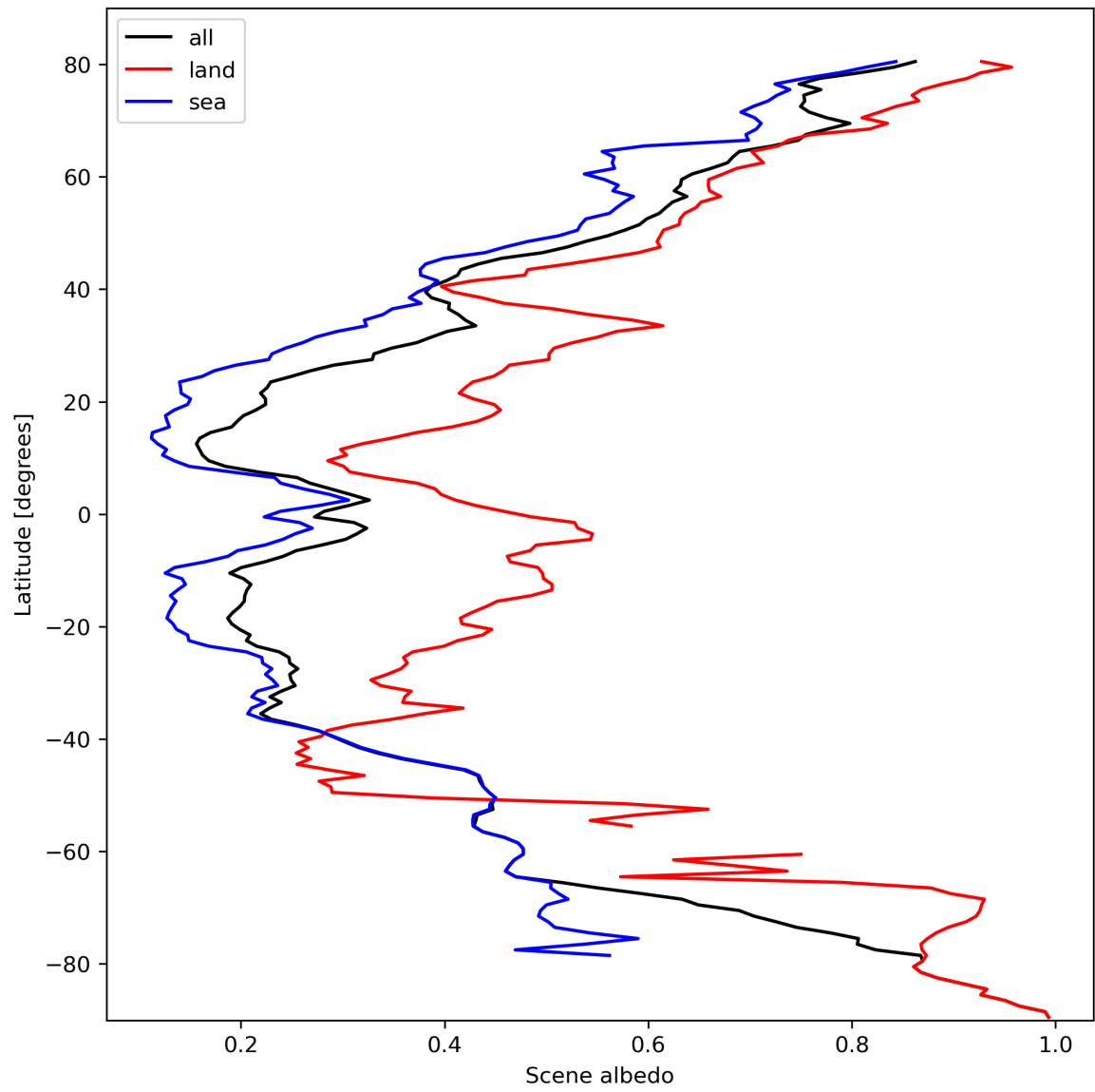
Figure 17: Zonal average of “Scene albedo” for 2024-02-28 to 2024-03-01.
