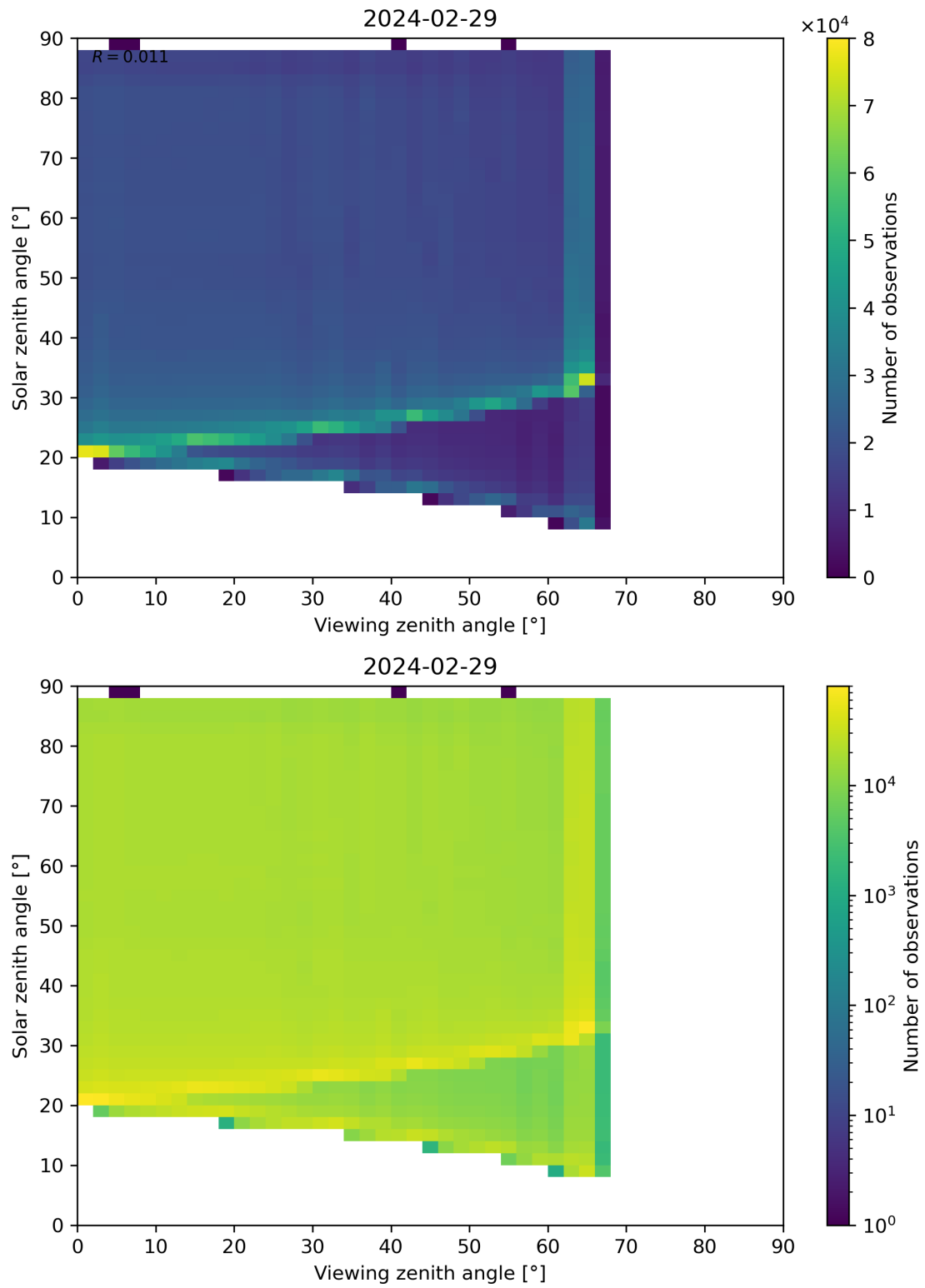
Figure 127: Scatter density plot of “Viewing zenith angle” against “Solar zenith angle” for 2024-02-28 to 2024-03-01.
