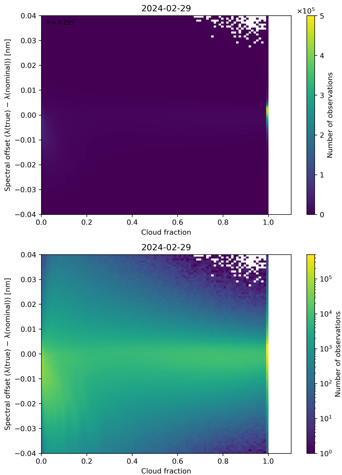
Figure 76: Scatter density plot of “Cloud fraction” against “Spectral offset ( \lambda(\text{true}) - \lambda(\text{nominal}) )” for 2024-02-28 to 2024-03-01.
