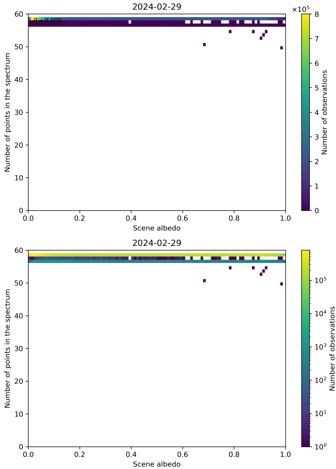
Figure 106: Scatter density plot of “Scene albedo” against “Number of points in the spectrum” for 2024-02-28 to 2024-03-01.
