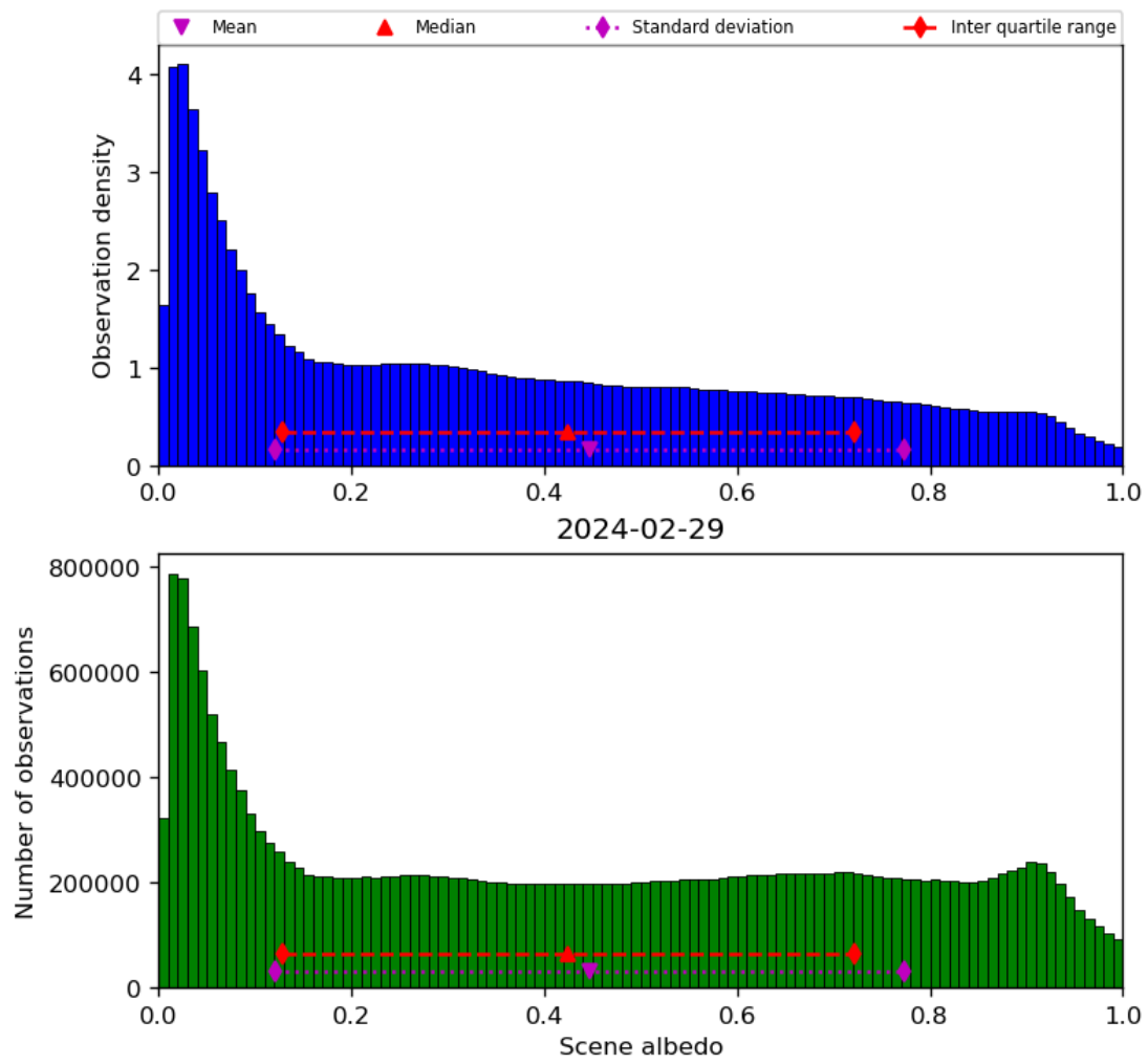
Figure 34: Histogram of “Scene albedo” for 2024-02-28 to 2024-03-01
