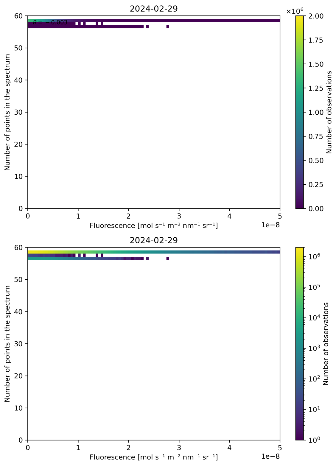
Figure 86: Scatter density plot of “Fluorescence” against “Number of points in the spectrum” for 2024-02-28 to 2024-03-01.
