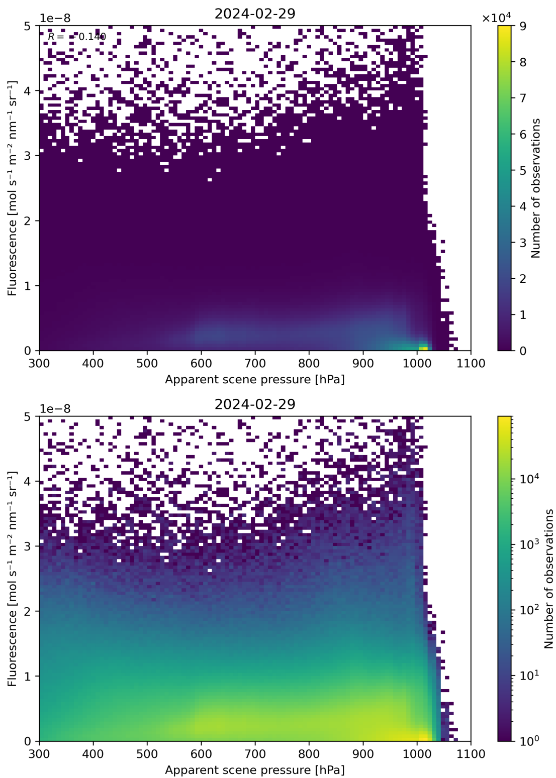
Figure 64: Scatter density plot of “Apparent scene pressure” against “Fluorescence” for 2024-02-28 to 2024-03-01.
