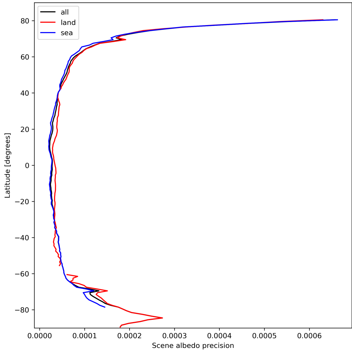
Figure 18: Zonal average of “Scene albedo precision” for 2024-02-28 to 2024-03-01.
