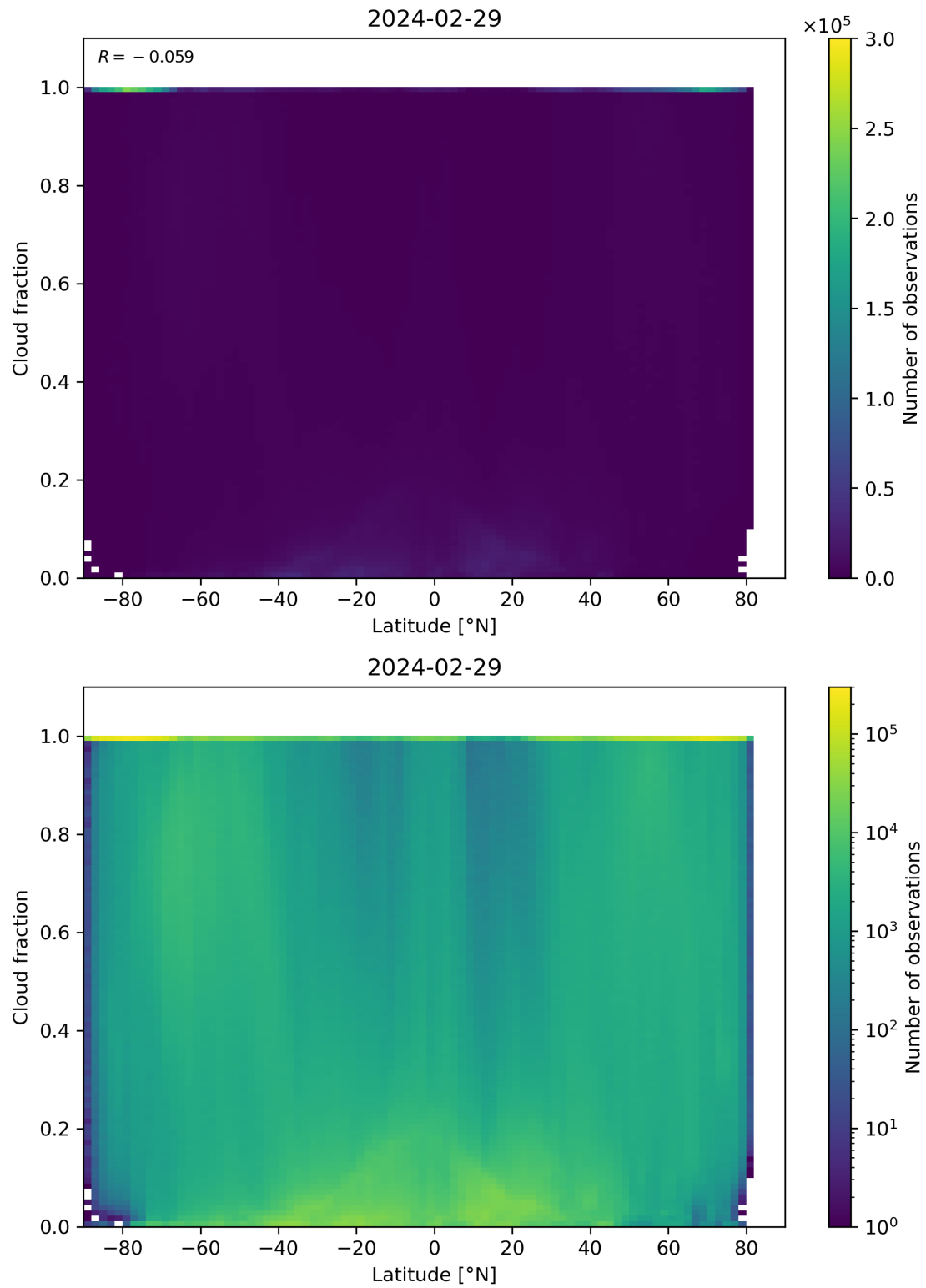
Figure 90: Scatter density plot of “Latitude” against “Cloud fraction” for 2024-02-28 to 2024-03-01.
