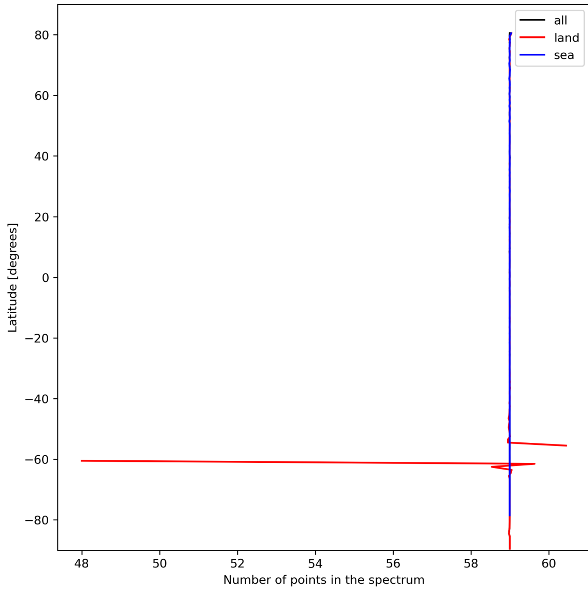
Figure 27: Zonal average of “Number of points in the spectrum” for 2024-02-28 to 2024-03-01.
