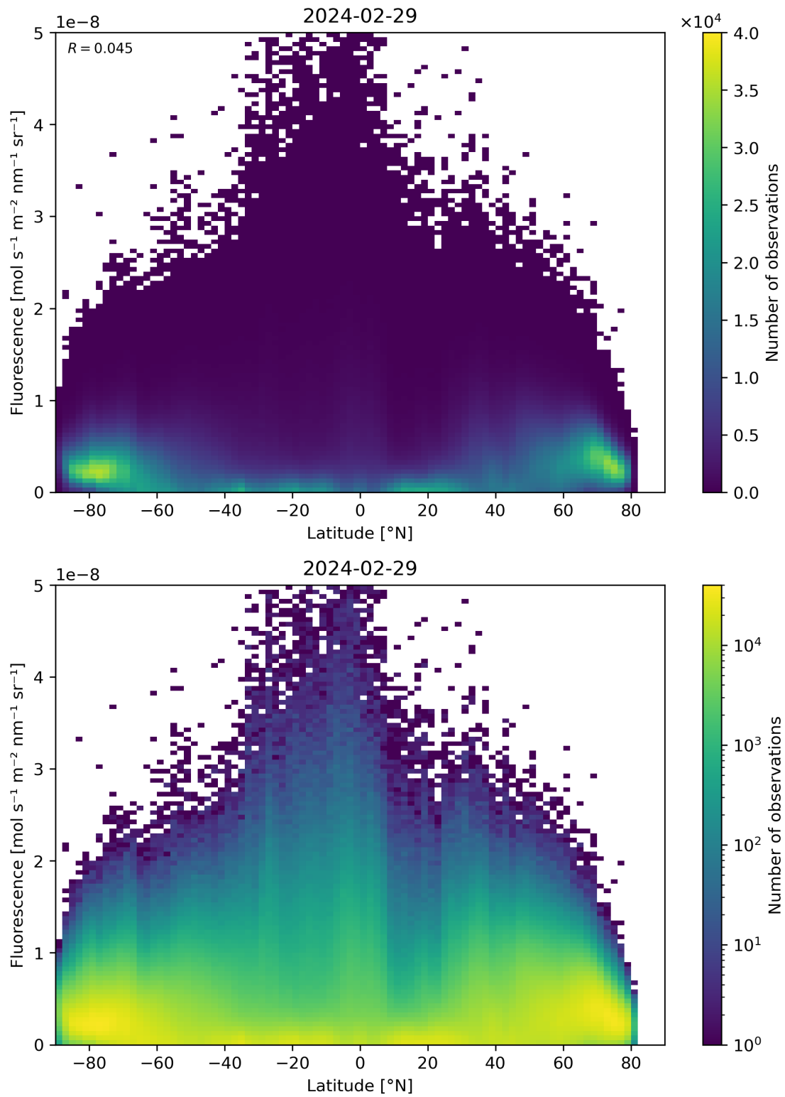
Figure 92: Scatter density plot of “Latitude” against “Fluorescence” for 2024-02-28 to 2024-03-01.
