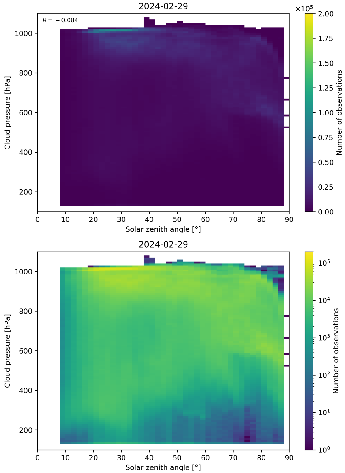
Figure 111: Scatter density plot of “Solar zenith angle” against “Cloud pressure” for 2024-02-28 to 2024-03-01.
