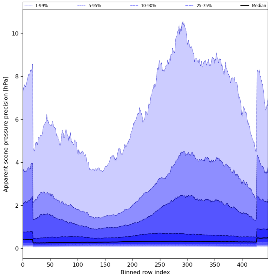
Figure 54: Along track statistics of “Apparent scene pressure precision” for 2024-02-28 to 2024-03-01
