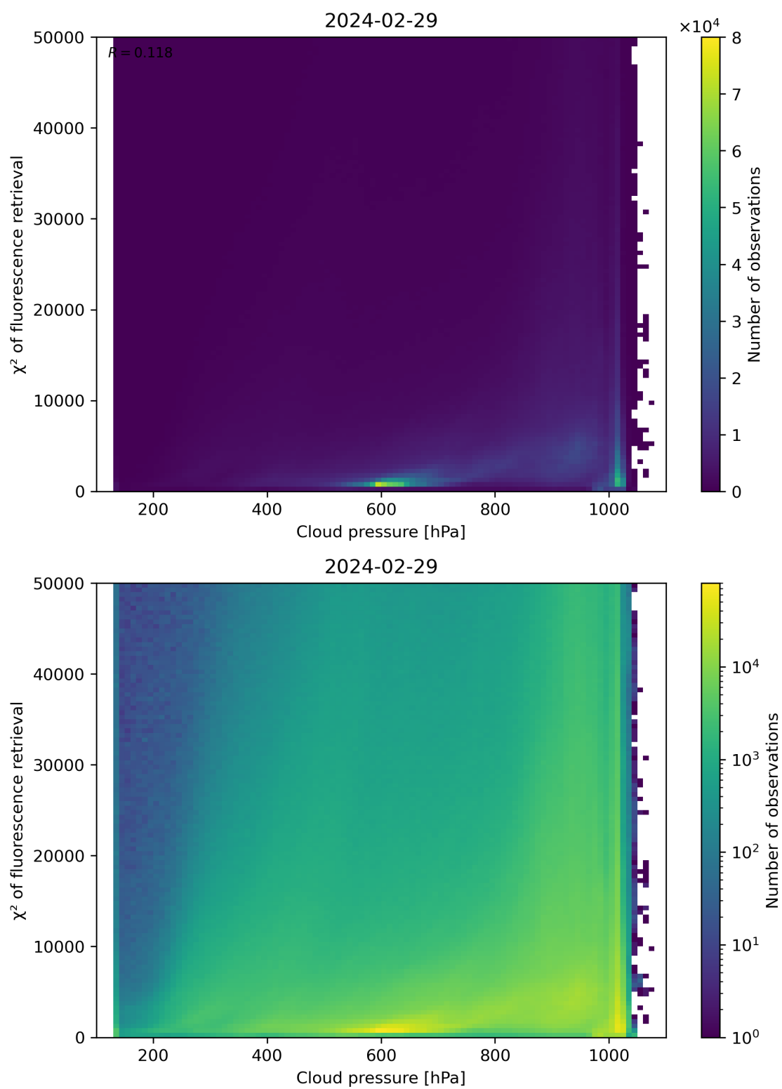
Figure 78: Scatter density plot of “Cloud pressure” against “ \chi^2 of fluorescence retrieval” for 2024-02-28 to 2024-03-01.
