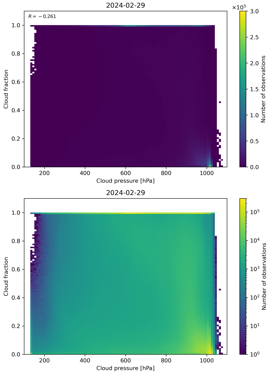
Figure 79: Scatter density plot of “Cloud pressure” against “Cloud fraction” for 2024-02-28 to 2024-03-01.
