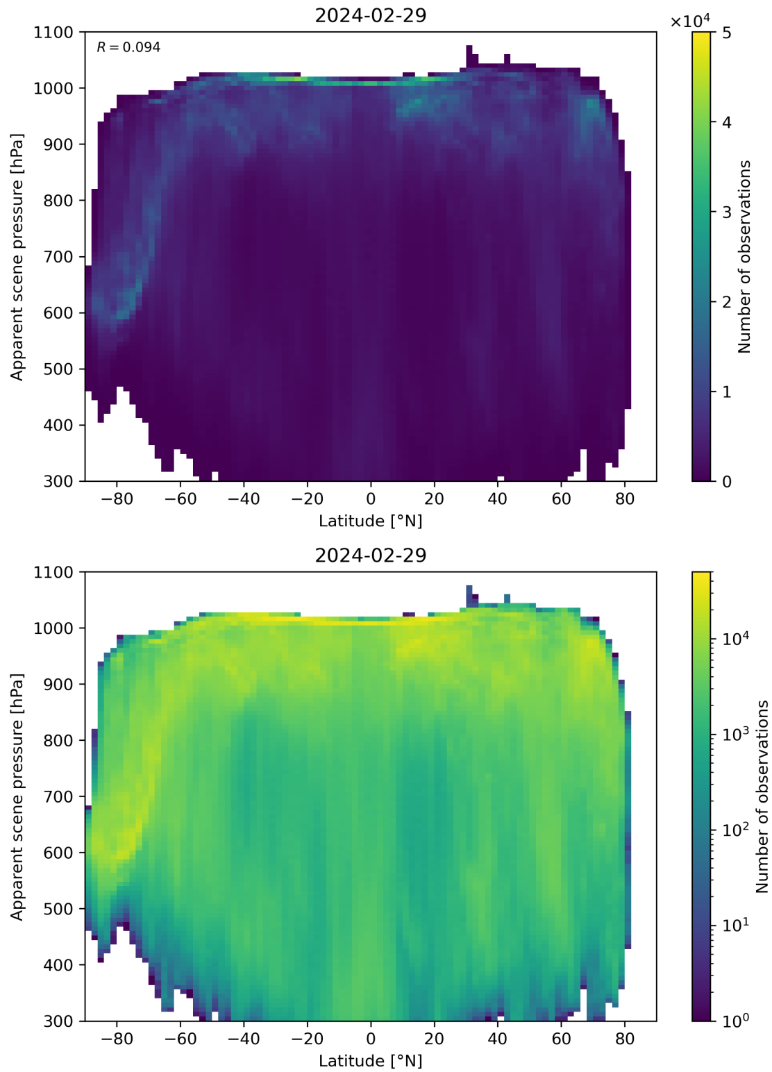
Figure 88: Scatter density plot of “Latitude” against “Apparent scene pressure” for 2024-02-28 to 2024-03-01.
