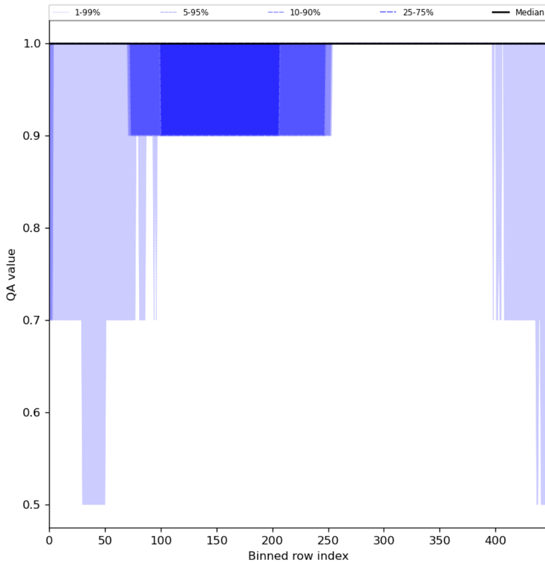
Figure 46: Along track statistics of "QA value" for 2024-02-28 to 2024-03-01
