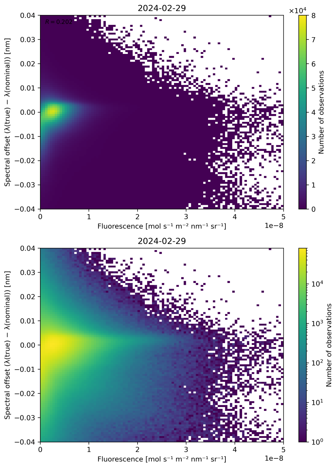
Figure 87: Scatter density plot of “Fluorescence” against “Spectral offset ( \lambda(\text{true}) - \lambda(\text{nominal}) )” for 2024-02-28 to 2024-03-01.
