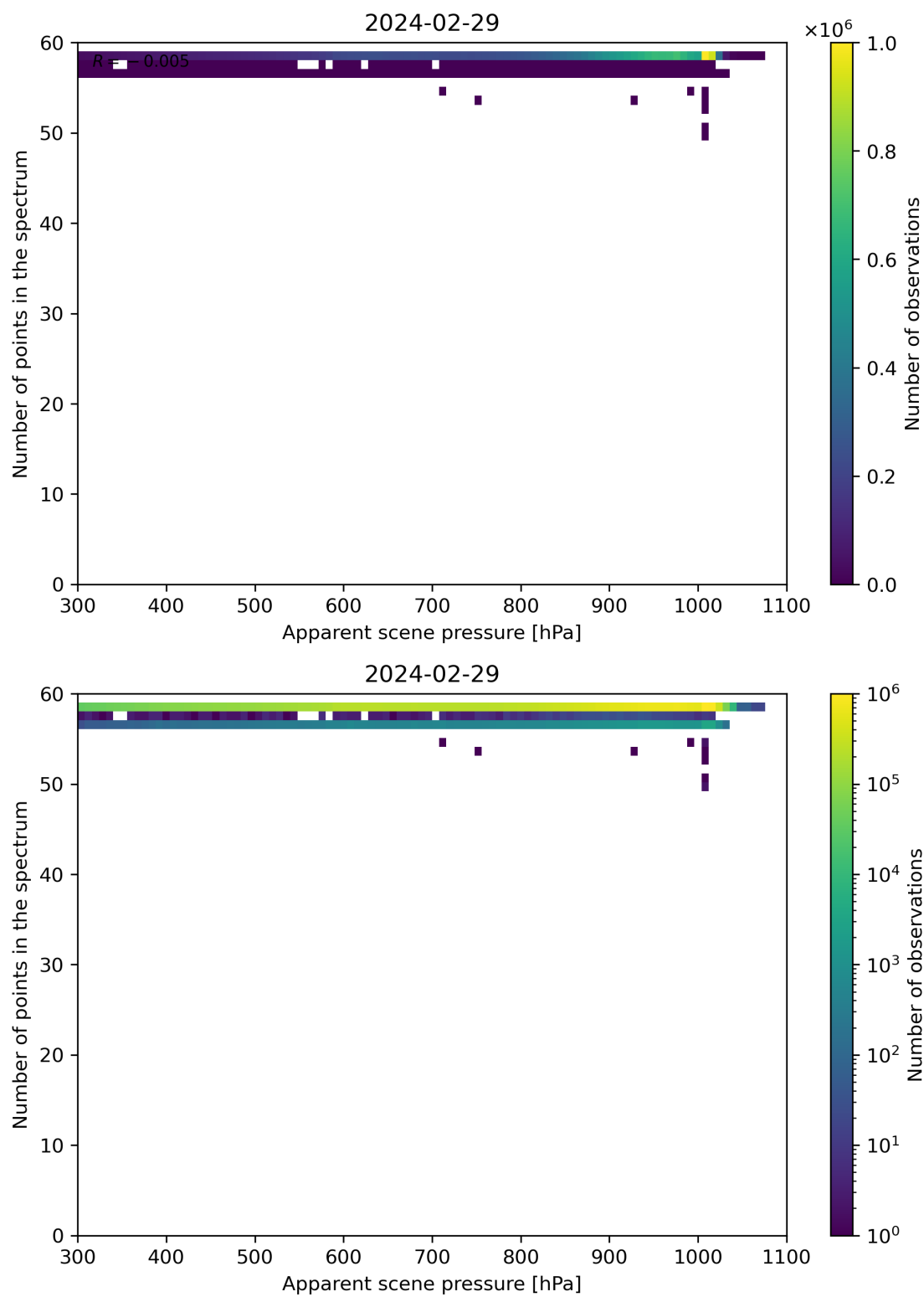
Figure 66: Scatter density plot of “Apparent scene pressure” against “Number of points in the spectrum” for 2024-02-28 to 2024-03-01.
