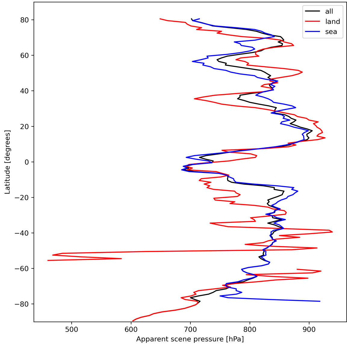
Figure 19: Zonal average of “Apparent scene pressure” for 2024-02-28 to 2024-03-01.
