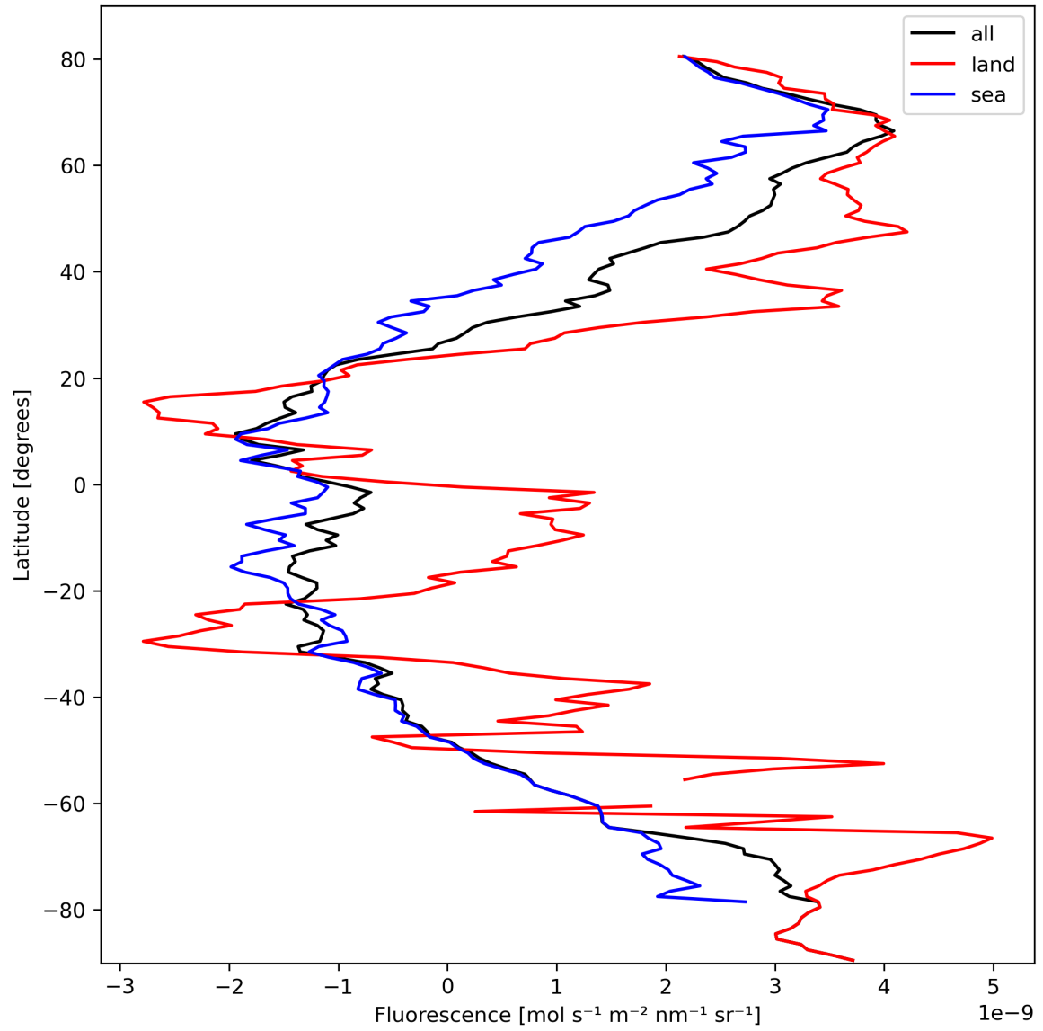
Figure 23: Zonal average of “Fluorescence” for 2024-02-28 to 2024-03-01.
