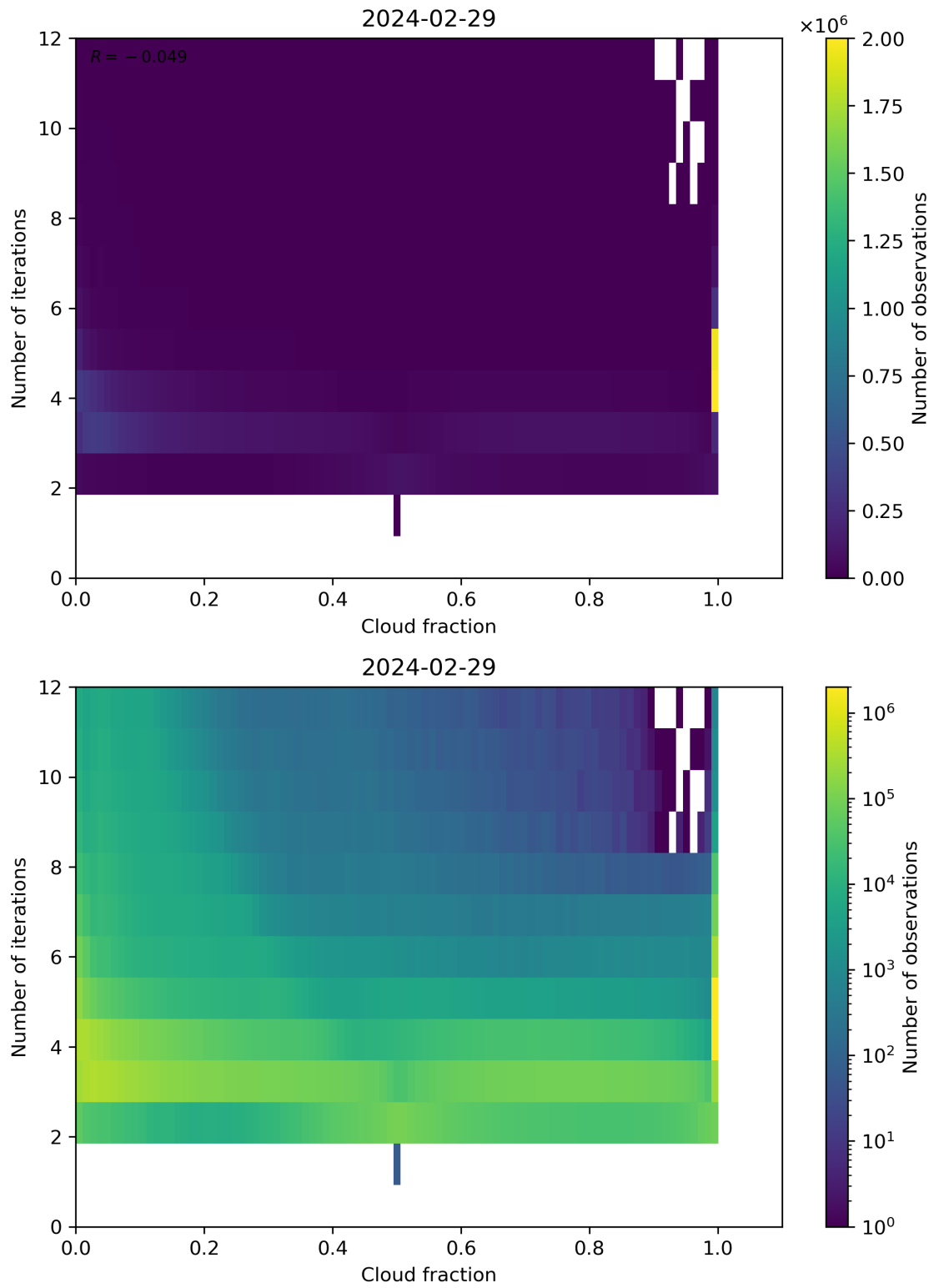
Figure 73: Scatter density plot of “Cloud fraction” against “Number of iterations” for 2024-02-28 to 2024-03-01.
