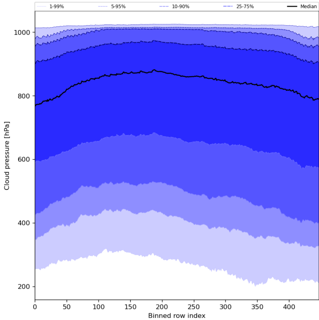
Figure 47: Along track statistics of “Cloud pressure” for 2024-02-28 to 2024-03-01
