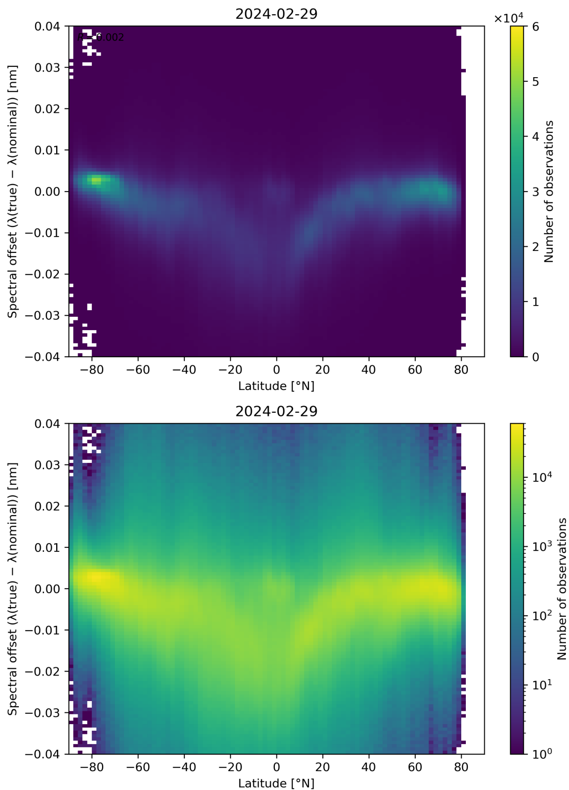
Figure 96: Scatter density plot of “Latitude” against “Spectral offset ( \lambda(\text{true}) - \lambda(\text{nominal}) )” for 2024-02-28 to 2024-03-01.
