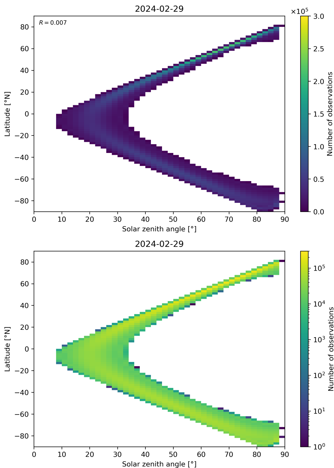
Figure 113: Scatter density plot of “Solar zenith angle” against “Latitude” for 2024-02-28 to 2024-03-01.
