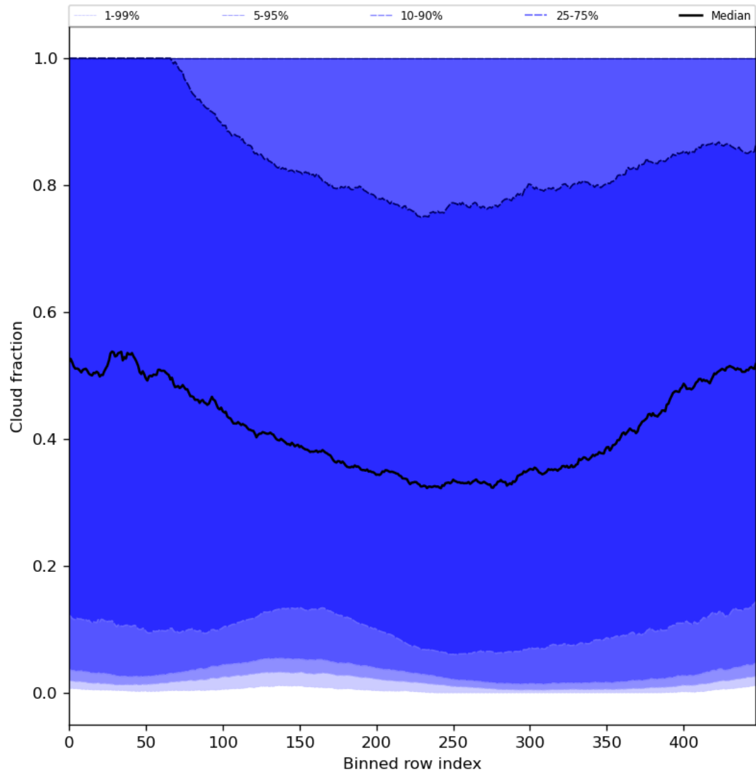
Figure 49: Along track statistics of “Cloud fraction” for 2024-02-28 to 2024-03-01
