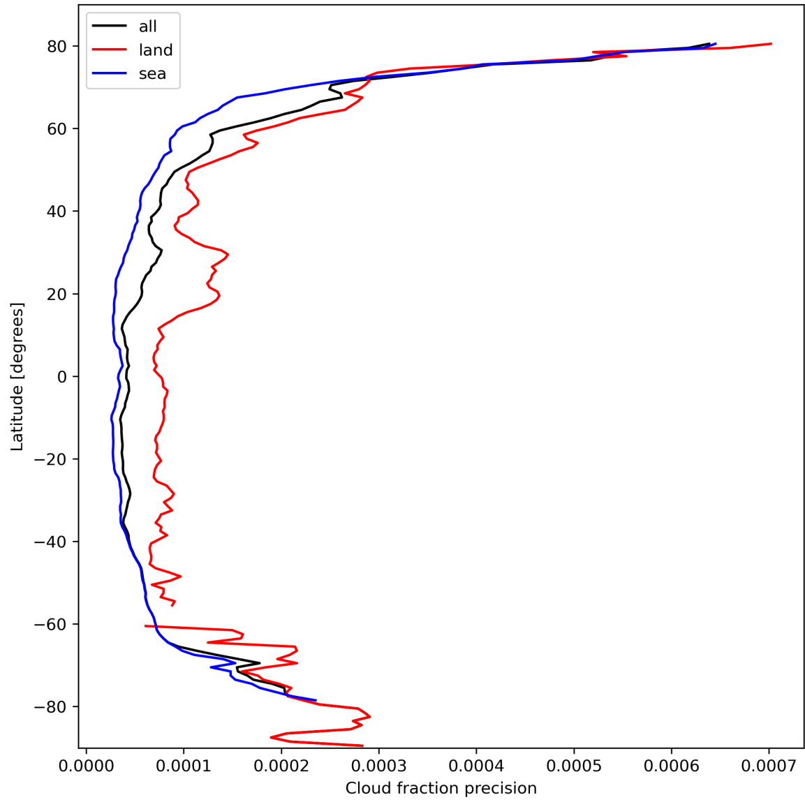
Figure 16: Zonal average of “Cloud fraction precision” for 2024-02-28 to 2024-03-01.
