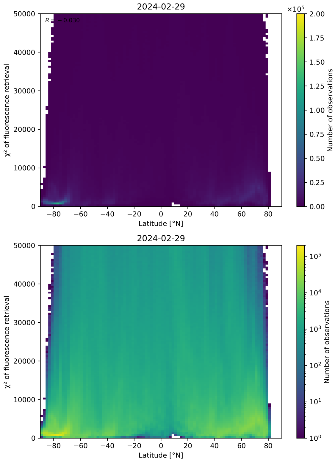
Figure 89: Scatter density plot of “Latitude” against “ \chi^2 of fluorescence retrieval” for 2024-02-28 to 2024-03-01.
