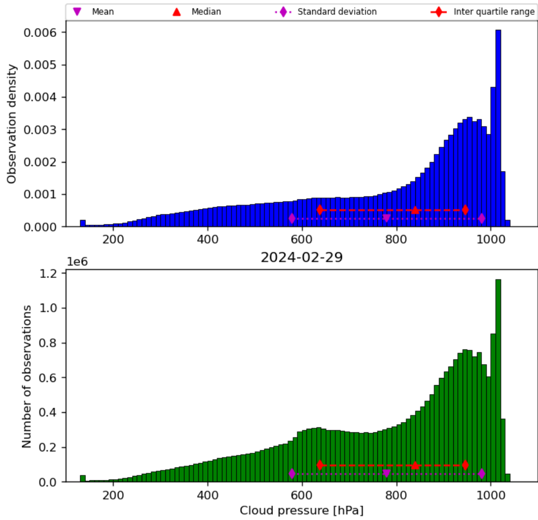
Figure 30: Histogram of “Cloud pressure” for 2024-02-28 to 2024-03-01
