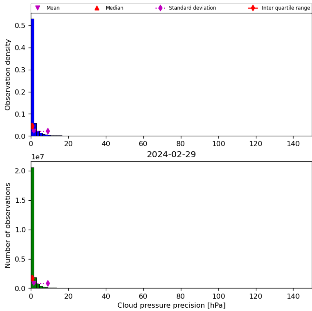
Figure 31: Histogram of “Cloud pressure precision” for 2024-02-28 to 2024-03-01
