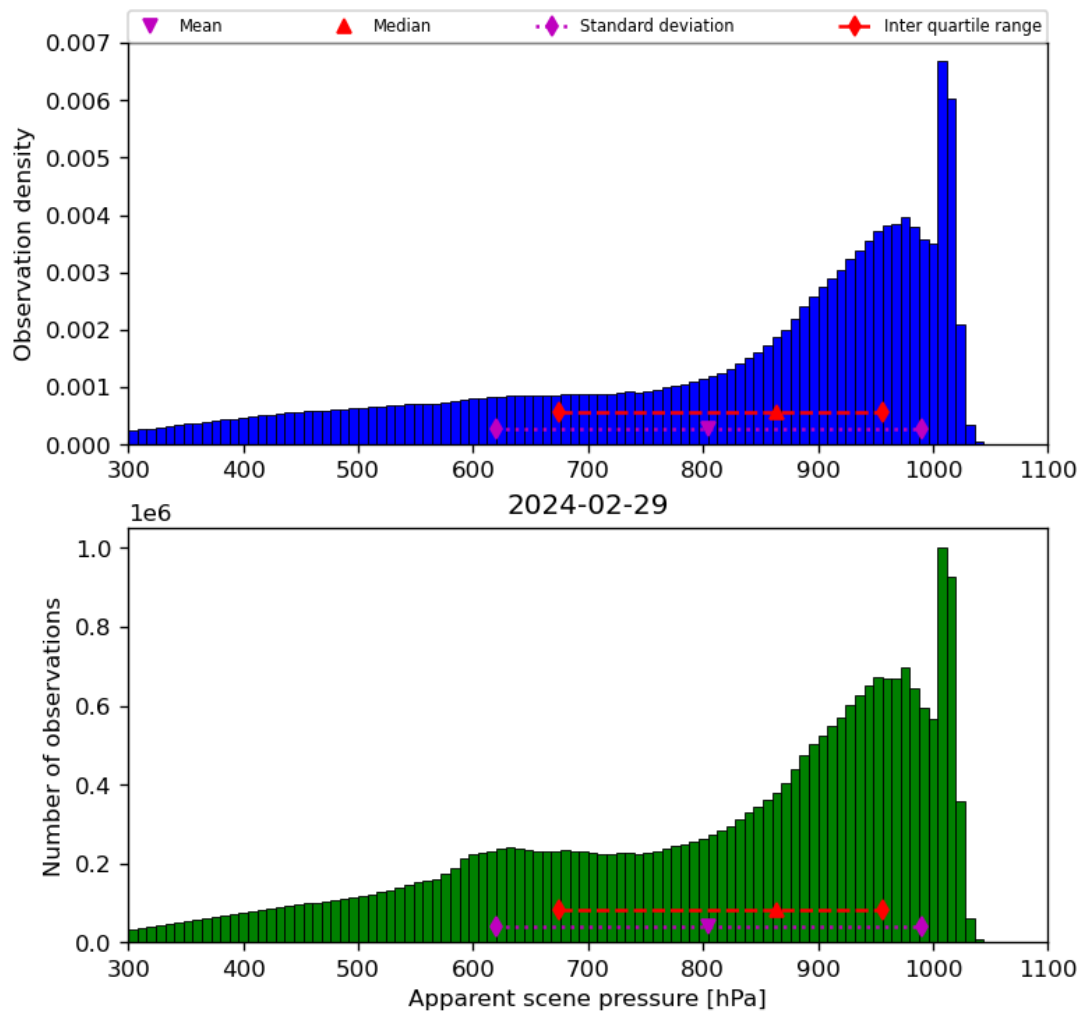
Figure 36: Histogram of “Apparent scene pressure” for 2024-02-28 to 2024-03-01
