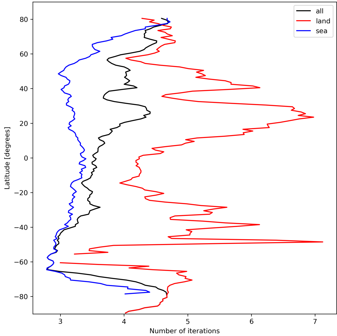
Figure 22: Zonal average of “Number of iterations” for 2024-02-28 to 2024-03-01.
