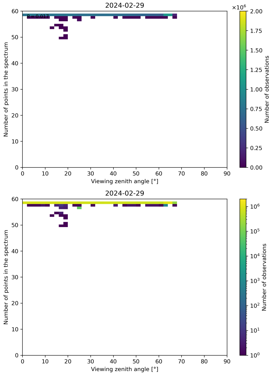
Figure 125: Scatter density plot of “Viewing zenith angle” against “Number of points in the spectrum” for 2024-02-28 to 2024-03-01.
