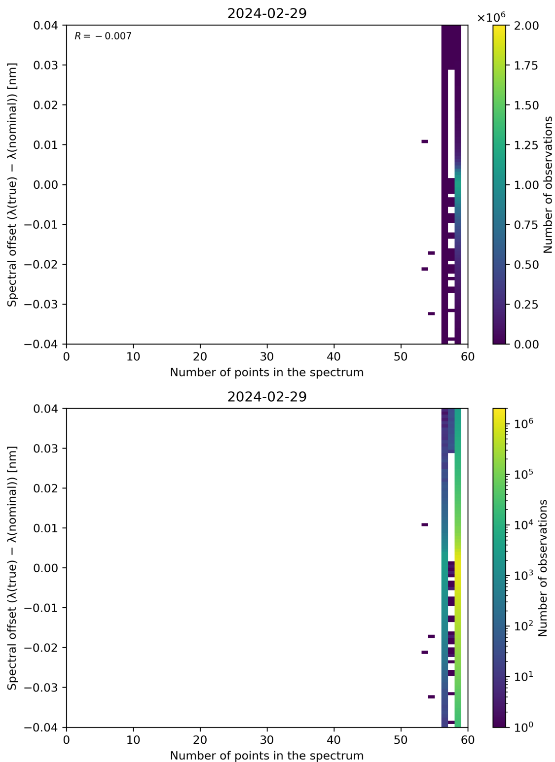
Figure 101: Scatter density plot of “Number of points in the spectrum” against “Spectral offset ( \lambda(\text{true}) - \lambda(\text{nominal}) )” for 2024-02-28 to 2024-03-01.
