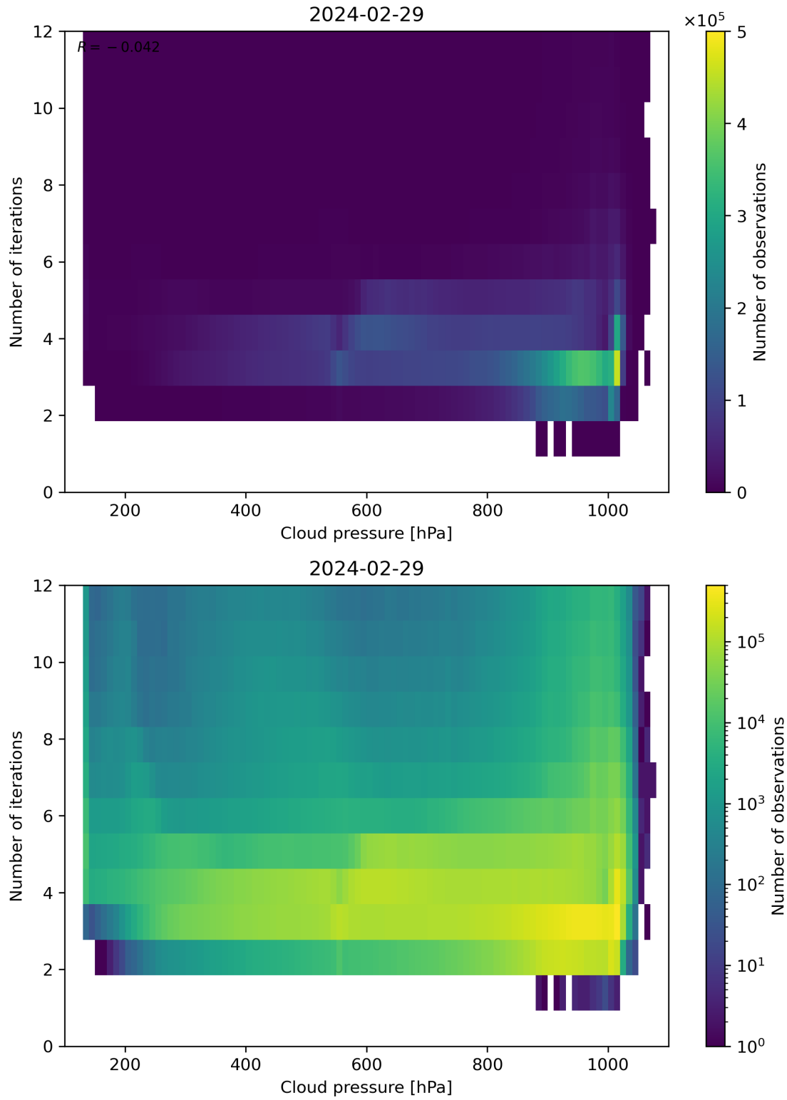
Figure 81: Scatter density plot of “Cloud pressure” against “Number of iterations” for 2024-02-28 to 2024-03-01.
