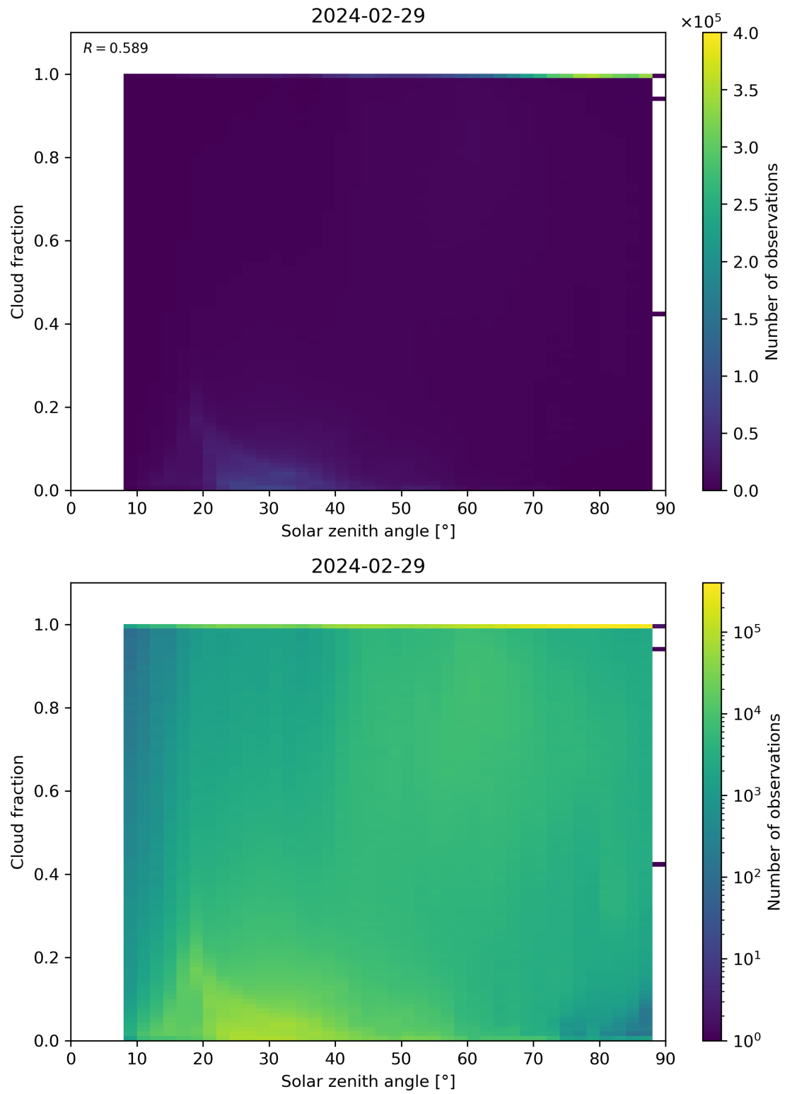
Figure 110: Scatter density plot of “Solar zenith angle” against “Cloud fraction” for 2024-02-28 to 2024-03-01.
