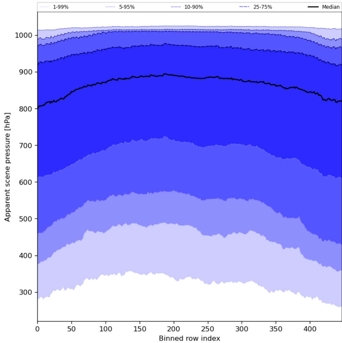
Figure 53: Along track statistics of “Apparent scene pressure” for 2024-02-28 to 2024-03-01
