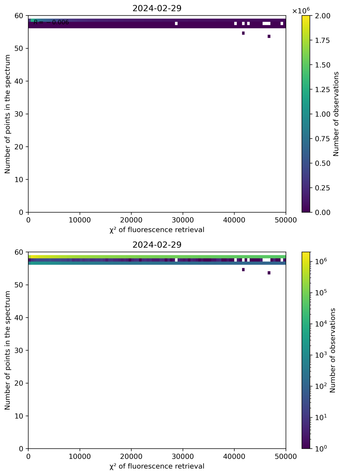
Figure 68: Scatter density plot of “ \chi^2 of fluorescence retrieval” against “Number of points in the spectrum” for 2024-02-28 to 2024-03-01.
