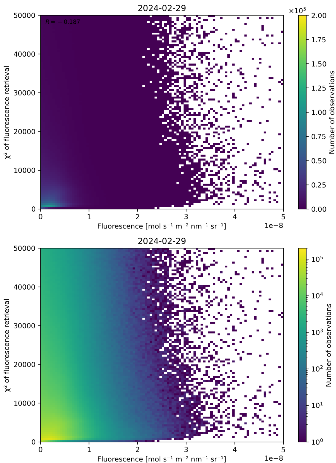
Figure 85: Scatter density plot of “Fluorescence” against “ \chi^2 of fluorescence retrieval” for 2024-02-28 to 2024-03-01.
