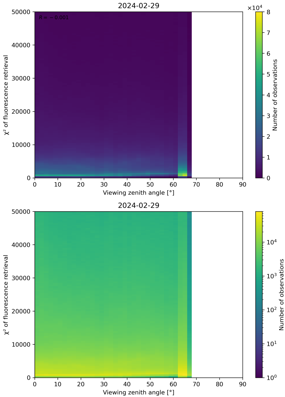
Figure 119: Scatter density plot of “Viewing zenith angle” against “ \chi^2 of fluorescence retrieval” for 2024-02-28 to 2024-03-01.
