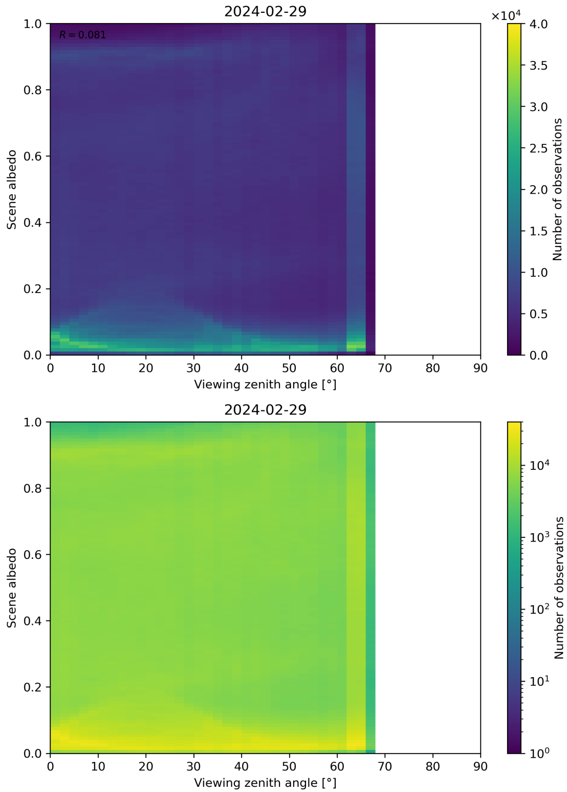
Figure 126: Scatter density plot of “Viewing zenith angle” against “Scene albedo” for 2024-02-28 to 2024-03-01.
