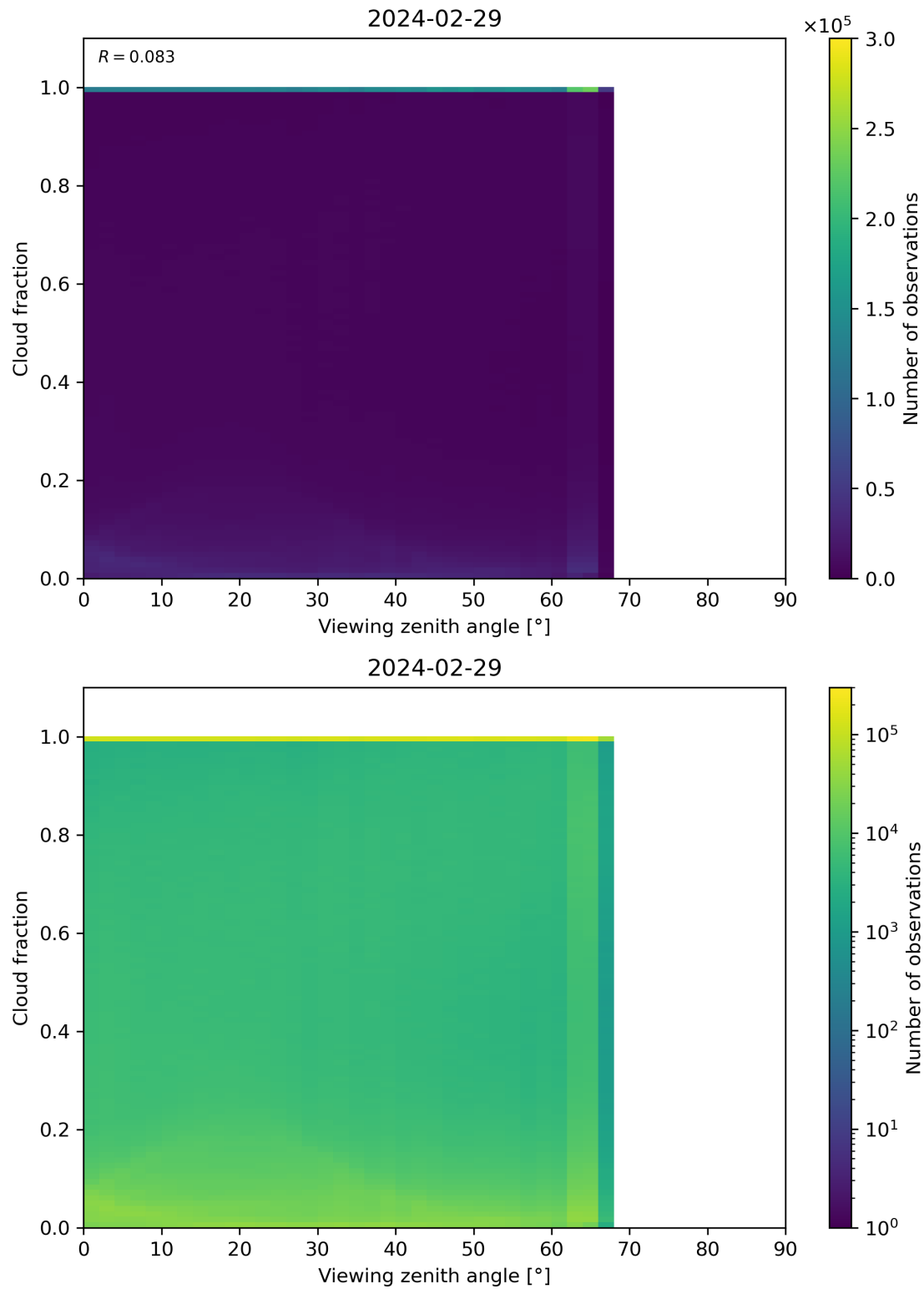
Figure 120: Scatter density plot of “Viewing zenith angle” against “Cloud fraction” for 2024-02-28 to 2024-03-01.
