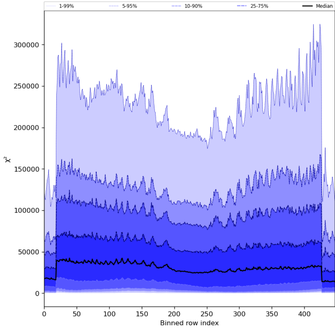
Figure 55: Along track statistics of “ \chi^2 ” for 2024-02-28 to 2024-03-01
