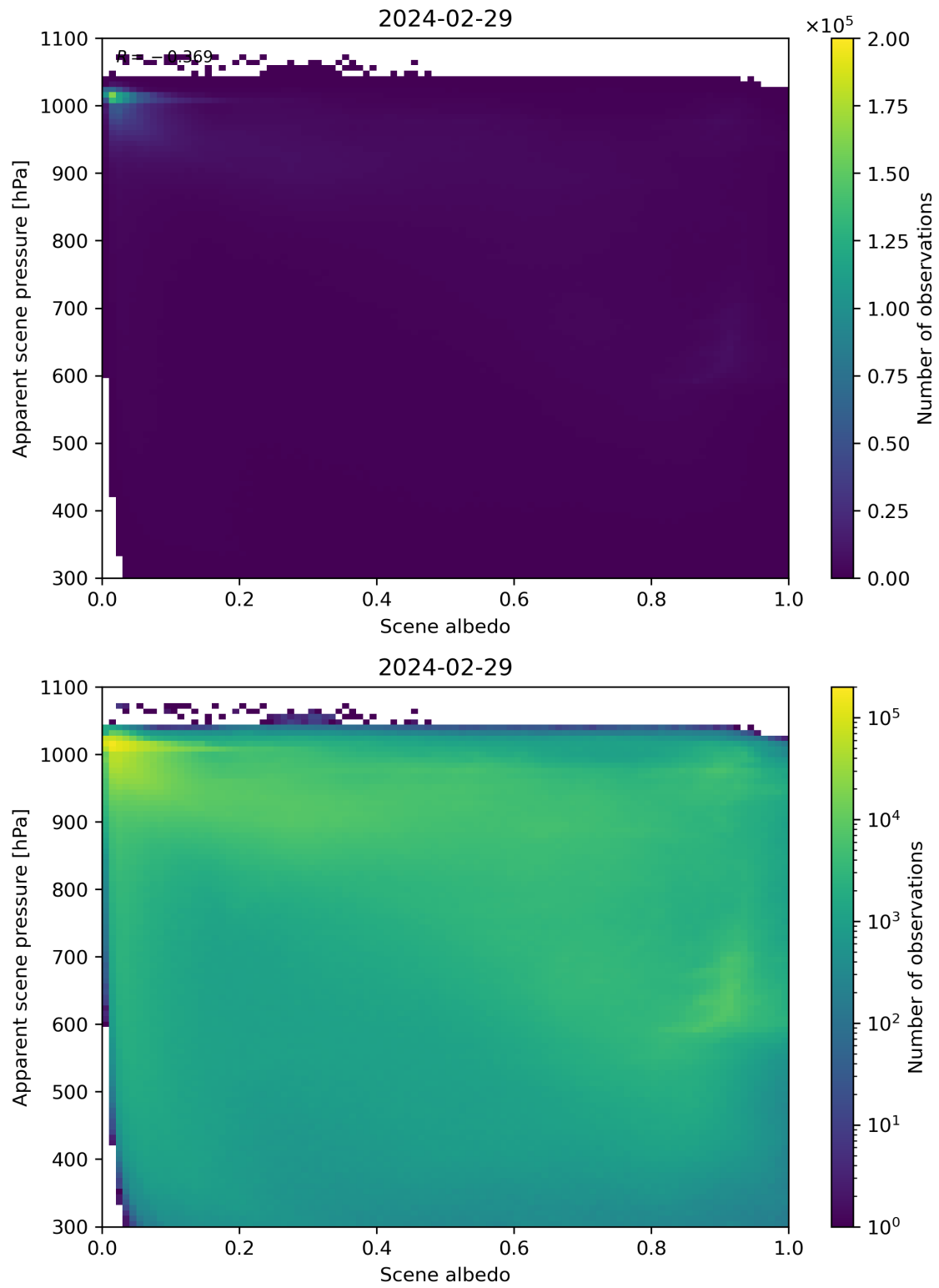
Figure 102: Scatter density plot of “Scene albedo” against “Apparent scene pressure” for 2024-02-28 to 2024-03-01.
