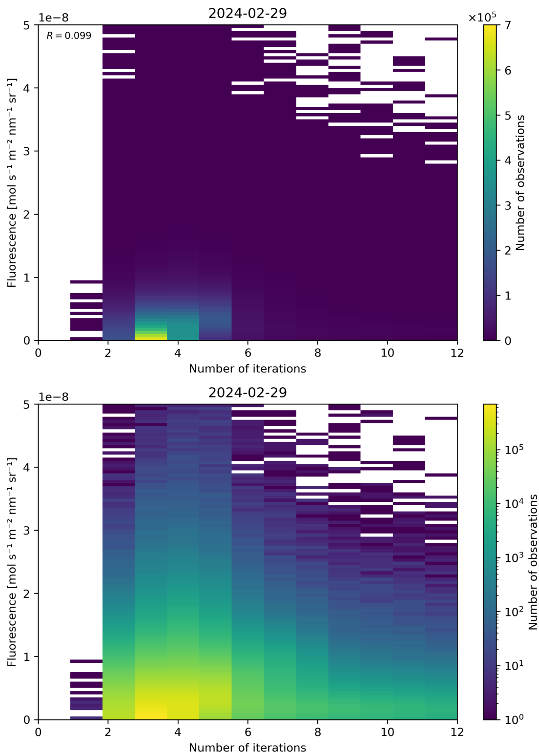
Figure 98: Scatter density plot of “Number of iterations” against “Fluorescence” for 2024-02-28 to 2024-03-01.
