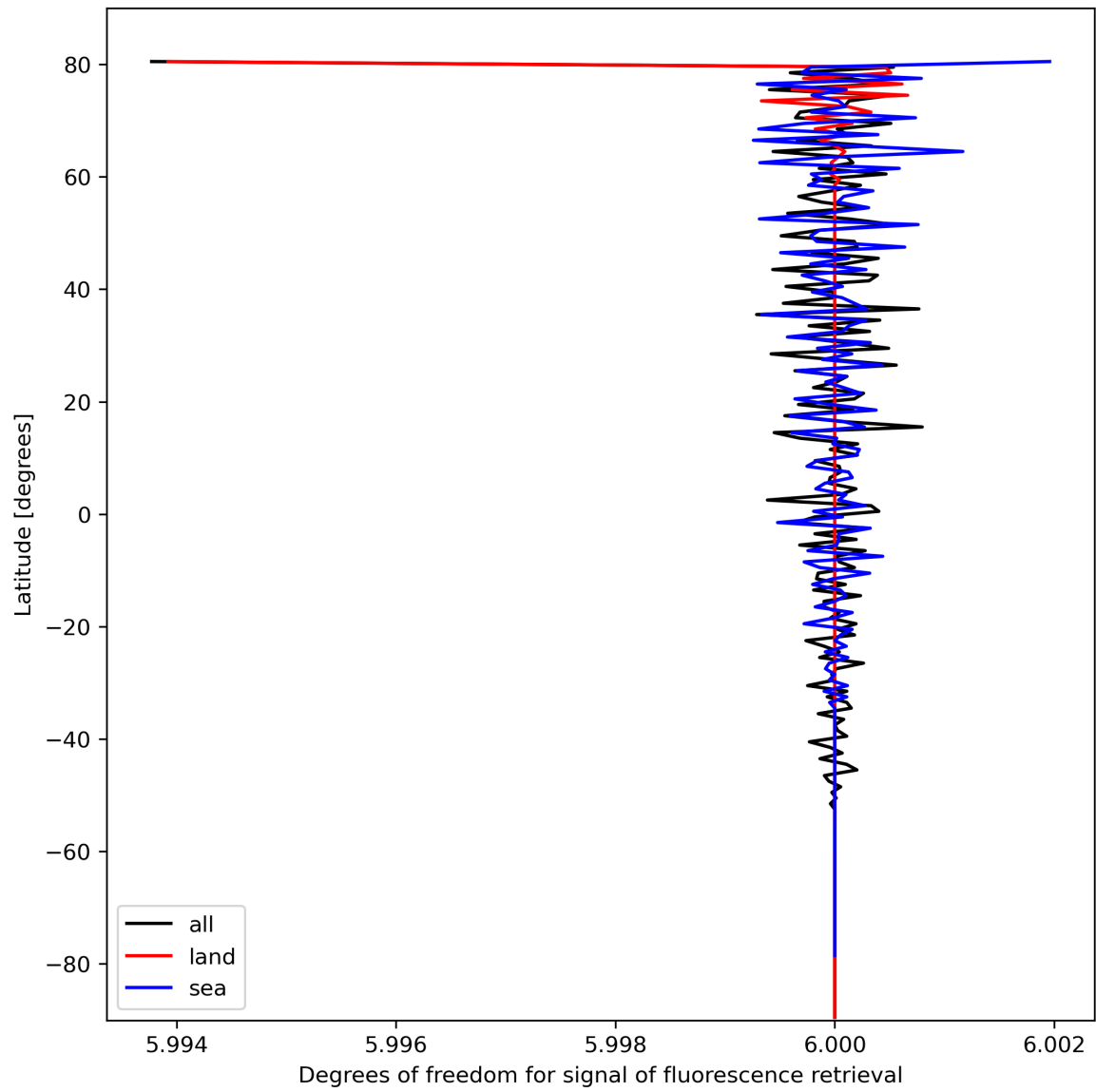
Figure 26: Zonal average of “Degrees of freedom for signal of fluorescence retrieval” for 2024-02-28 to 2024-03-01.
