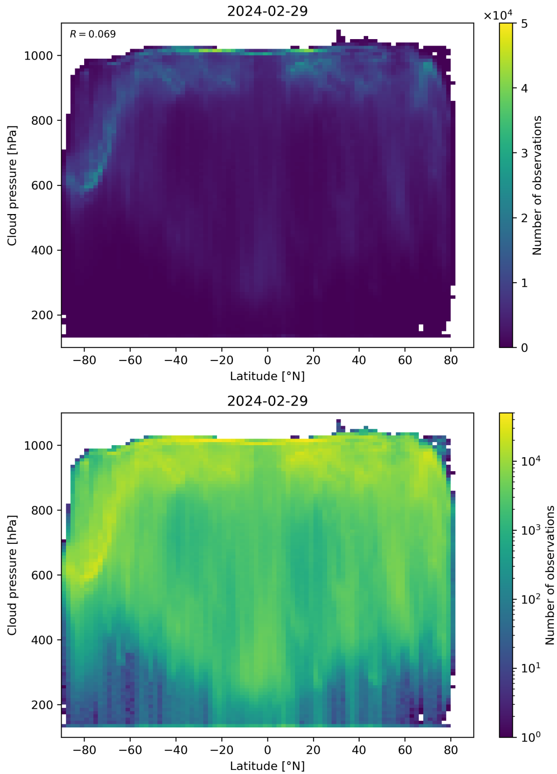
Figure 91: Scatter density plot of “Latitude” against “Cloud pressure” for 2024-02-28 to 2024-03-01.
