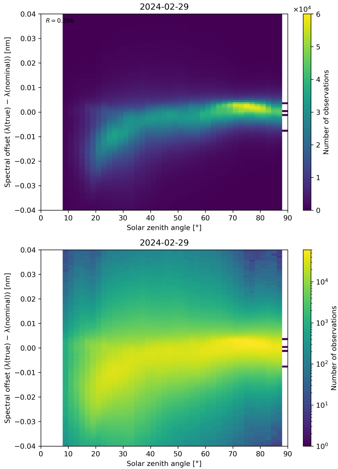
Figure 117: Scatter density plot of “Solar zenith angle” against “Spectral offset ( \lambda(\text{true}) - \lambda(\text{nominal}) )” for 2024-02-28 to 2024-03-01.
