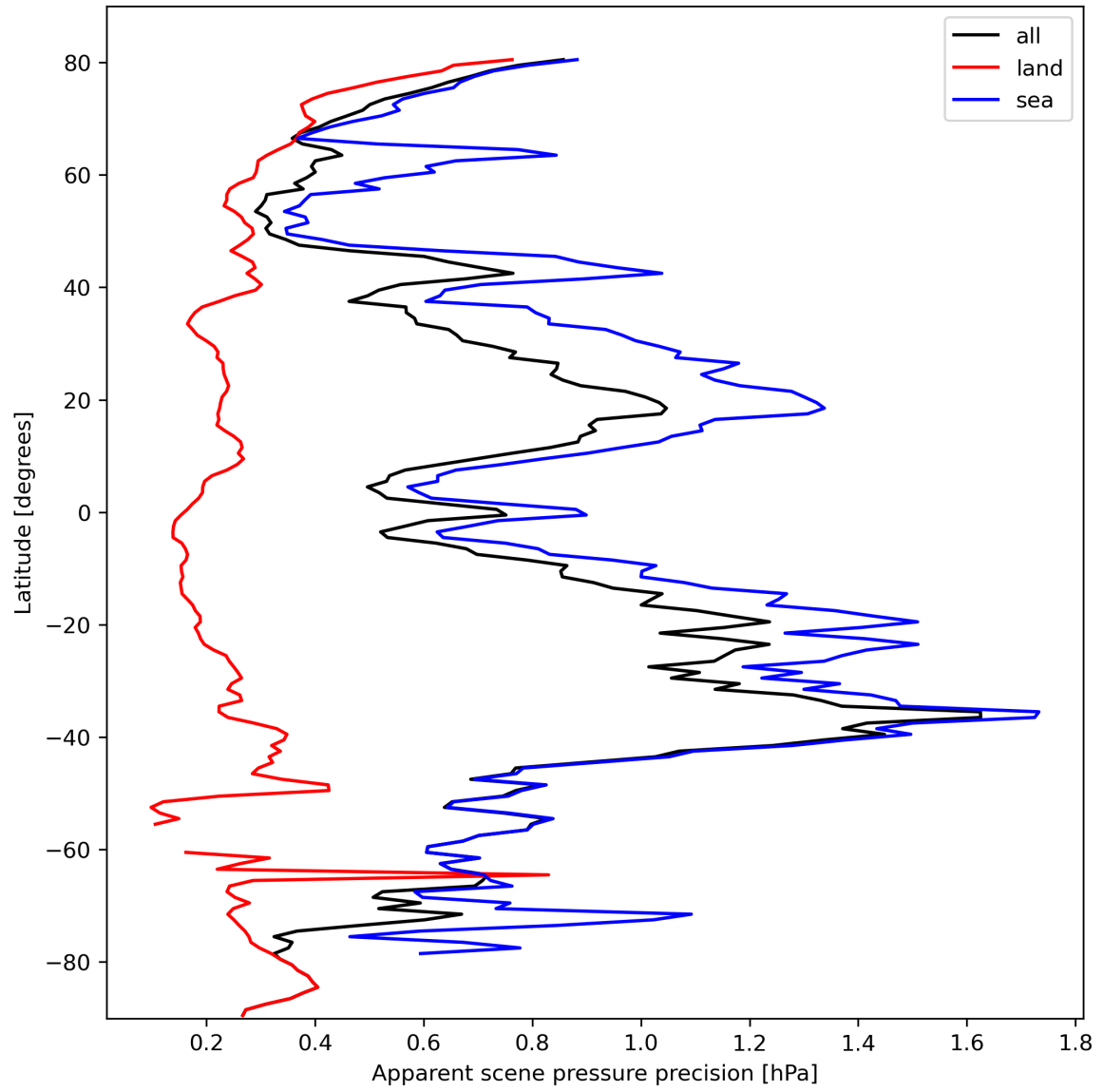
Figure 20: Zonal average of “Apparent scene pressure precision” for 2024-02-28 to 2024-03-01.
