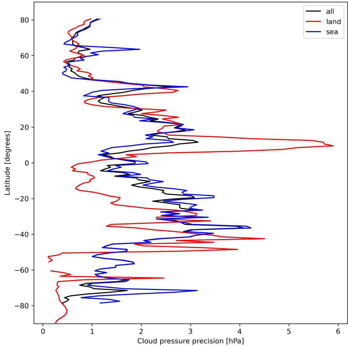
Figure 14: Zonal average of “Cloud pressure precision” for 2024-02-28 to 2024-03-01.
