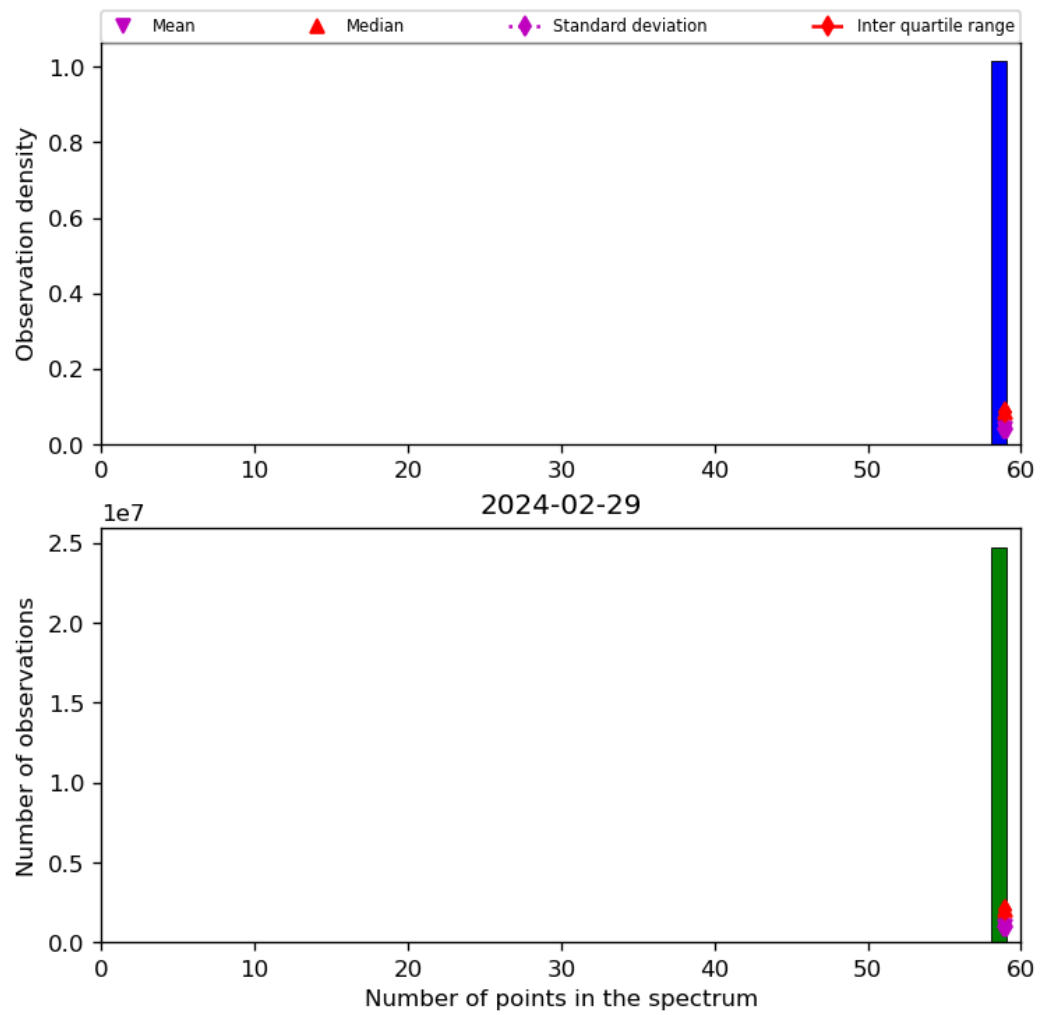
Figure 44: Histogram of “Number of points in the spectrum” for 2024-02-28 to 2024-03-01
