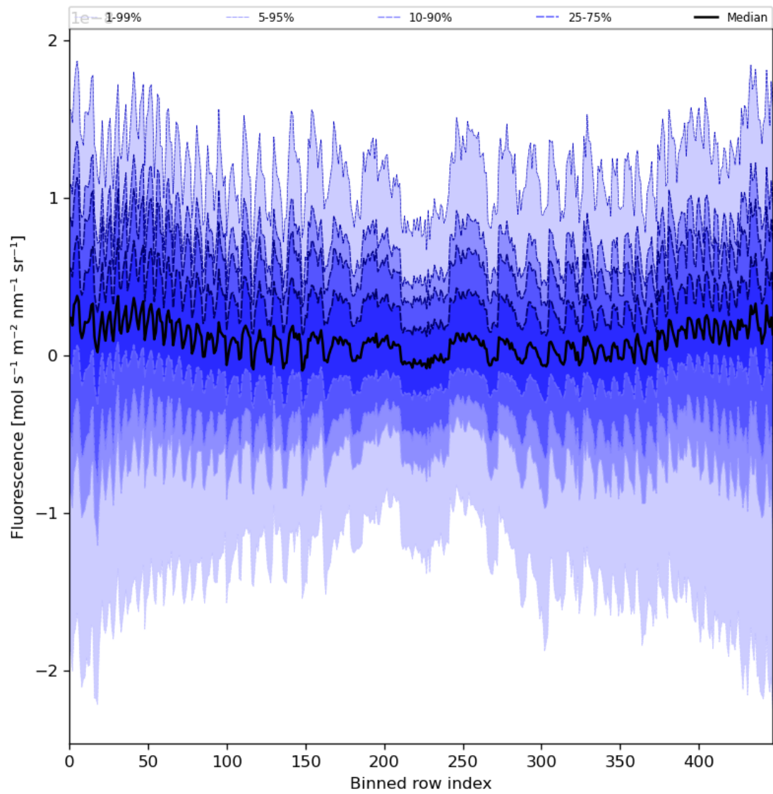
Figure 57: Along track statistics of “Fluorescence” for 2024-02-28 to 2024-03-01
