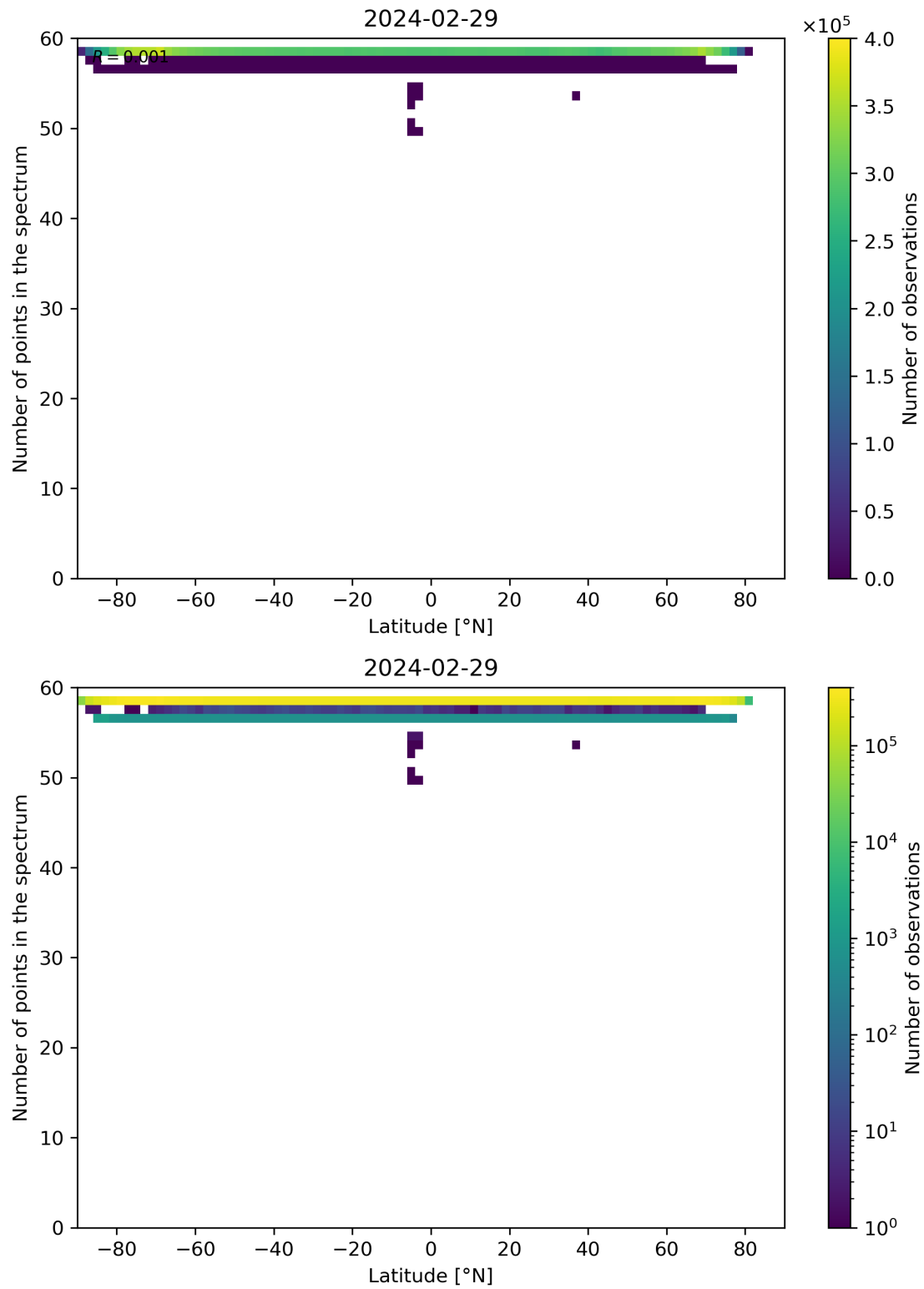
Figure 94: Scatter density plot of “Latitude” against “Number of points in the spectrum” for 2024-02-28 to 2024-03-01.
