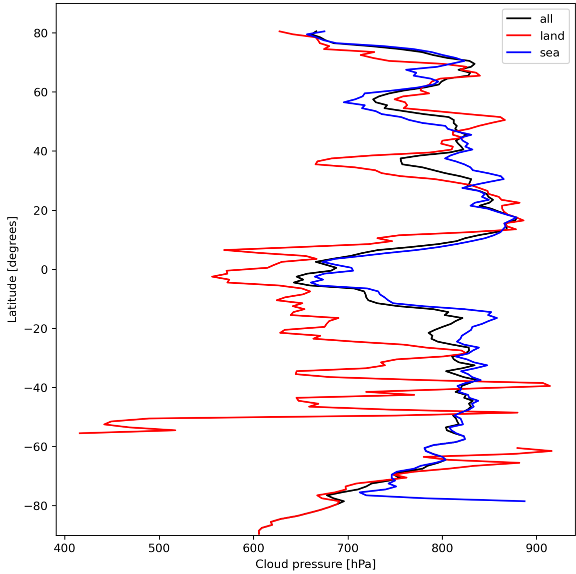
Figure 13: Zonal average of “Cloud pressure” for 2024-02-28 to 2024-03-01.
