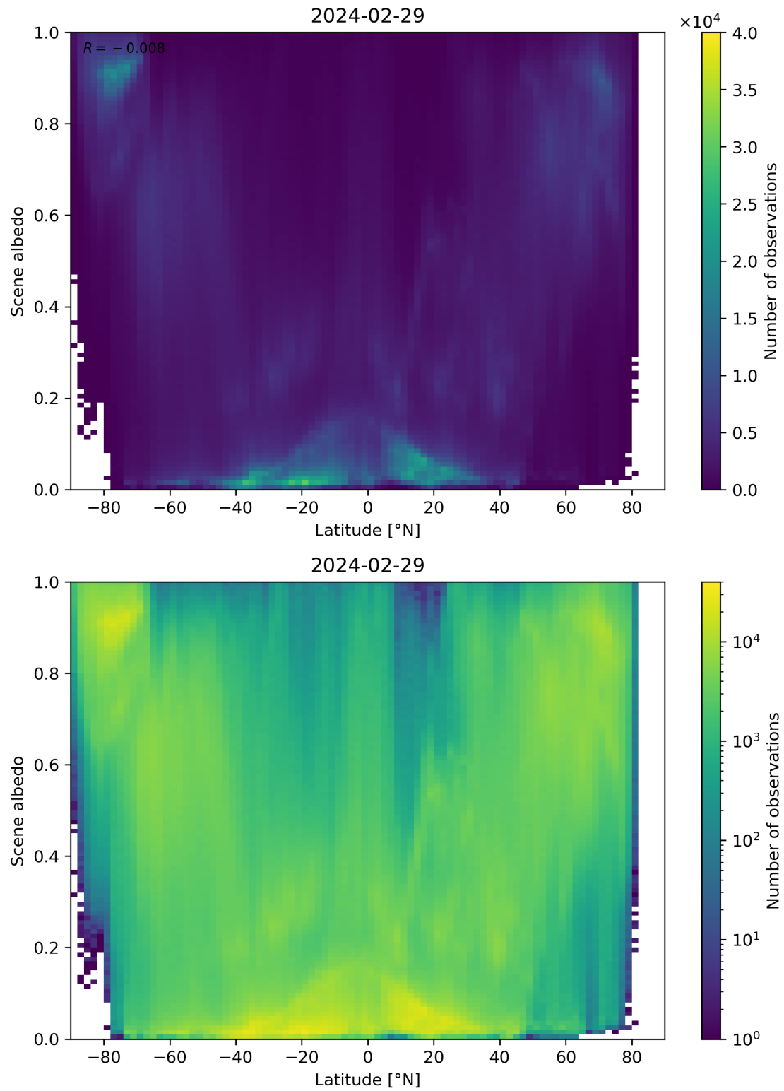
Figure 95: Scatter density plot of “Latitude” against “Scene albedo” for 2024-02-28 to 2024-03-01.
