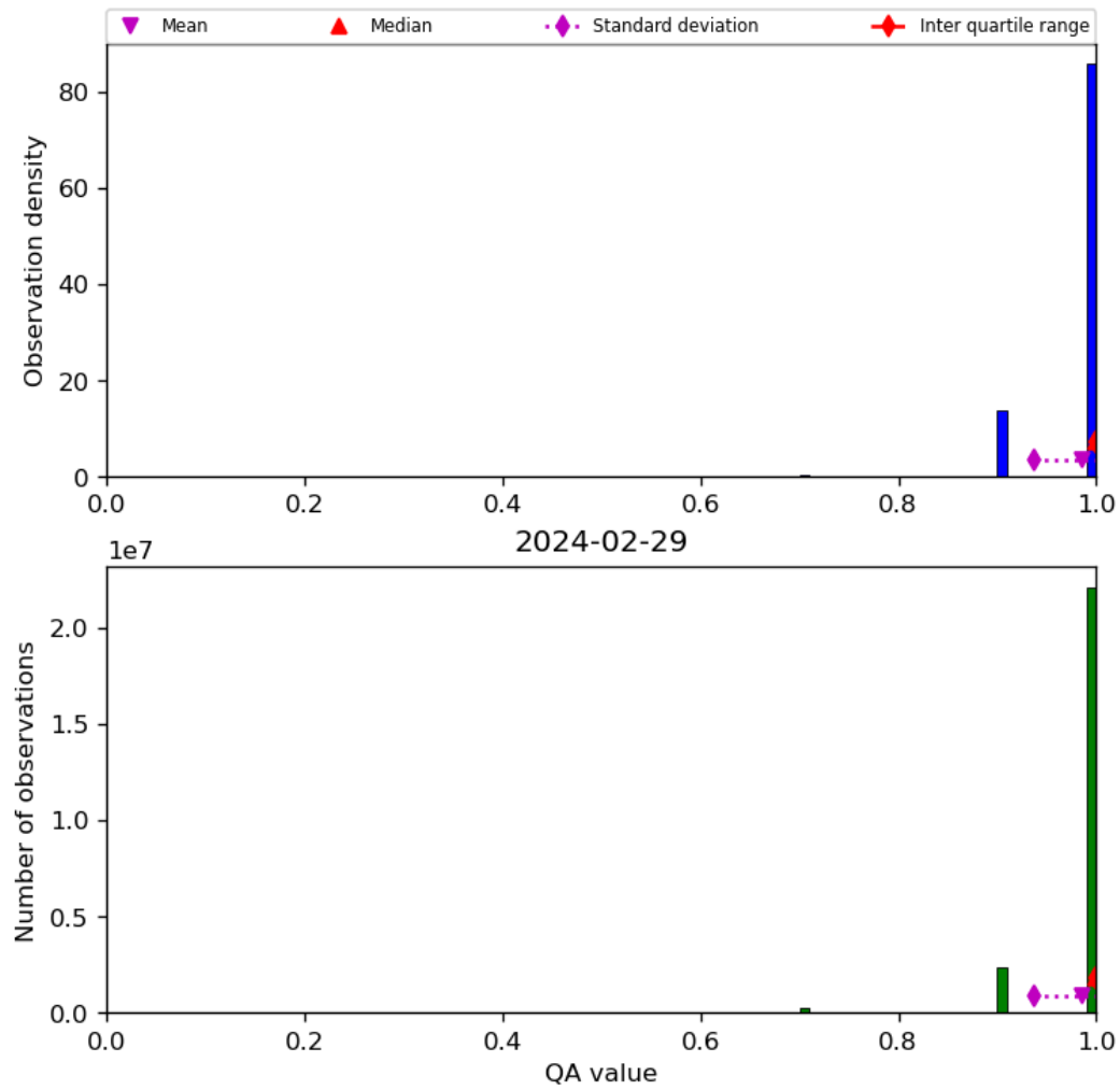
Figure 29: Histogram of “QA value” for 2024-02-28 to 2024-03-01
