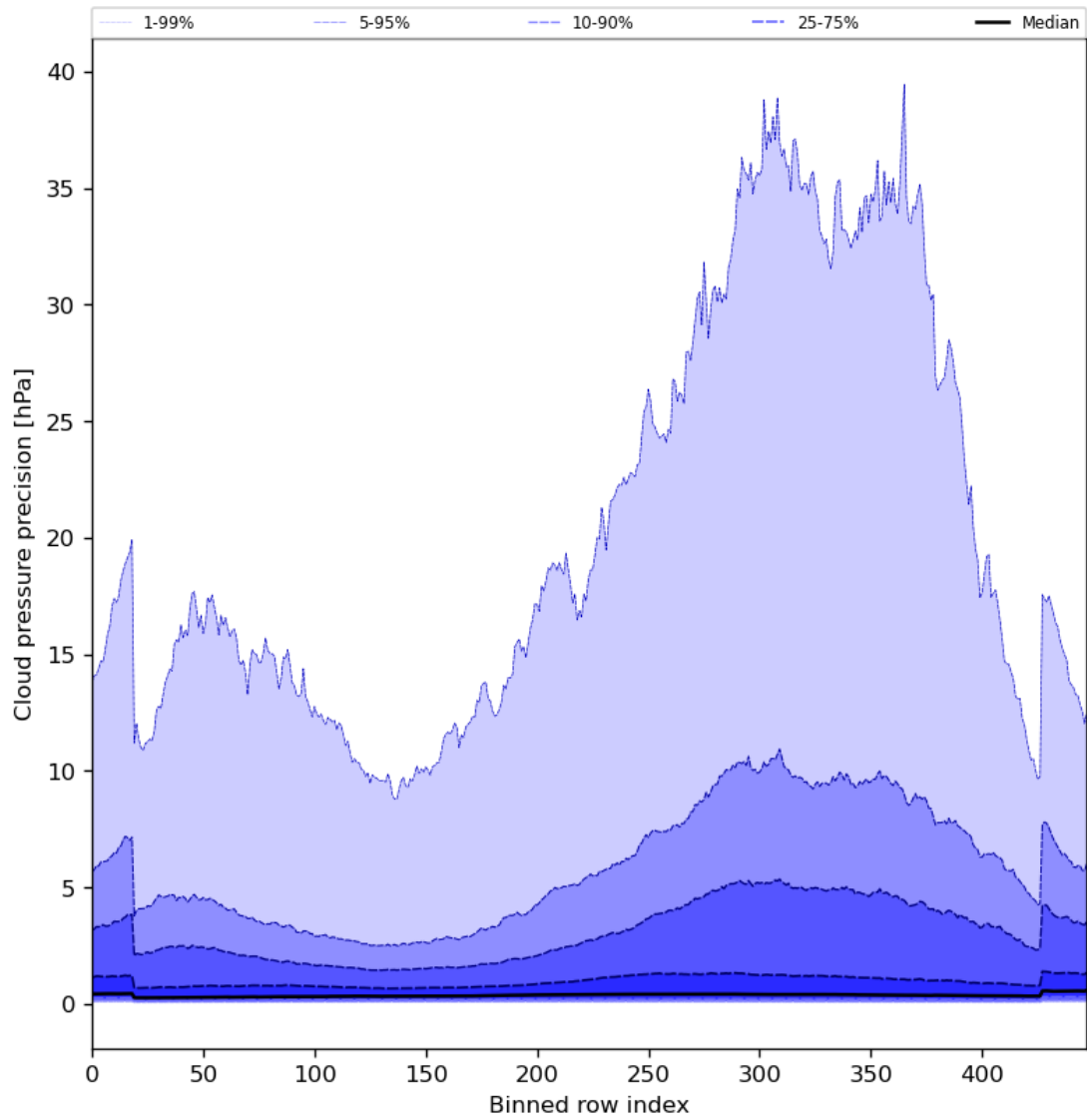
Figure 48: Along track statistics of “Cloud pressure precision” for 2024-02-28 to 2024-03-01
