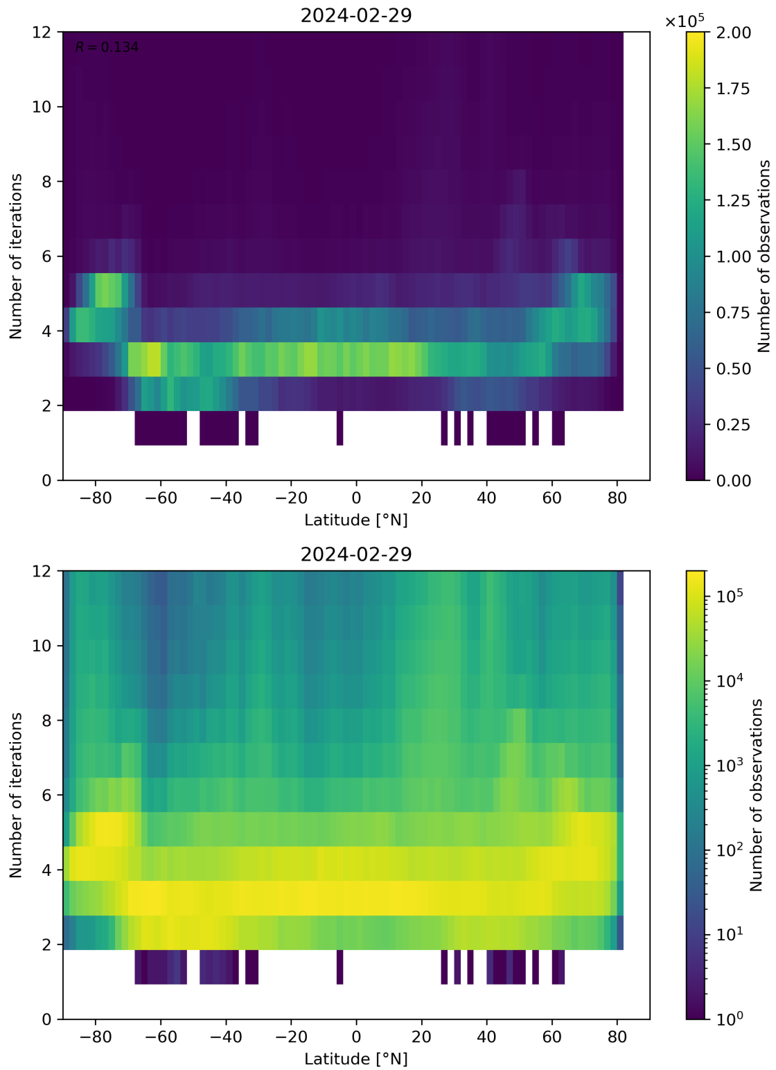
Figure 93: Scatter density plot of “Latitude” against “Number of iterations” for 2024-02-28 to 2024-03-01.
