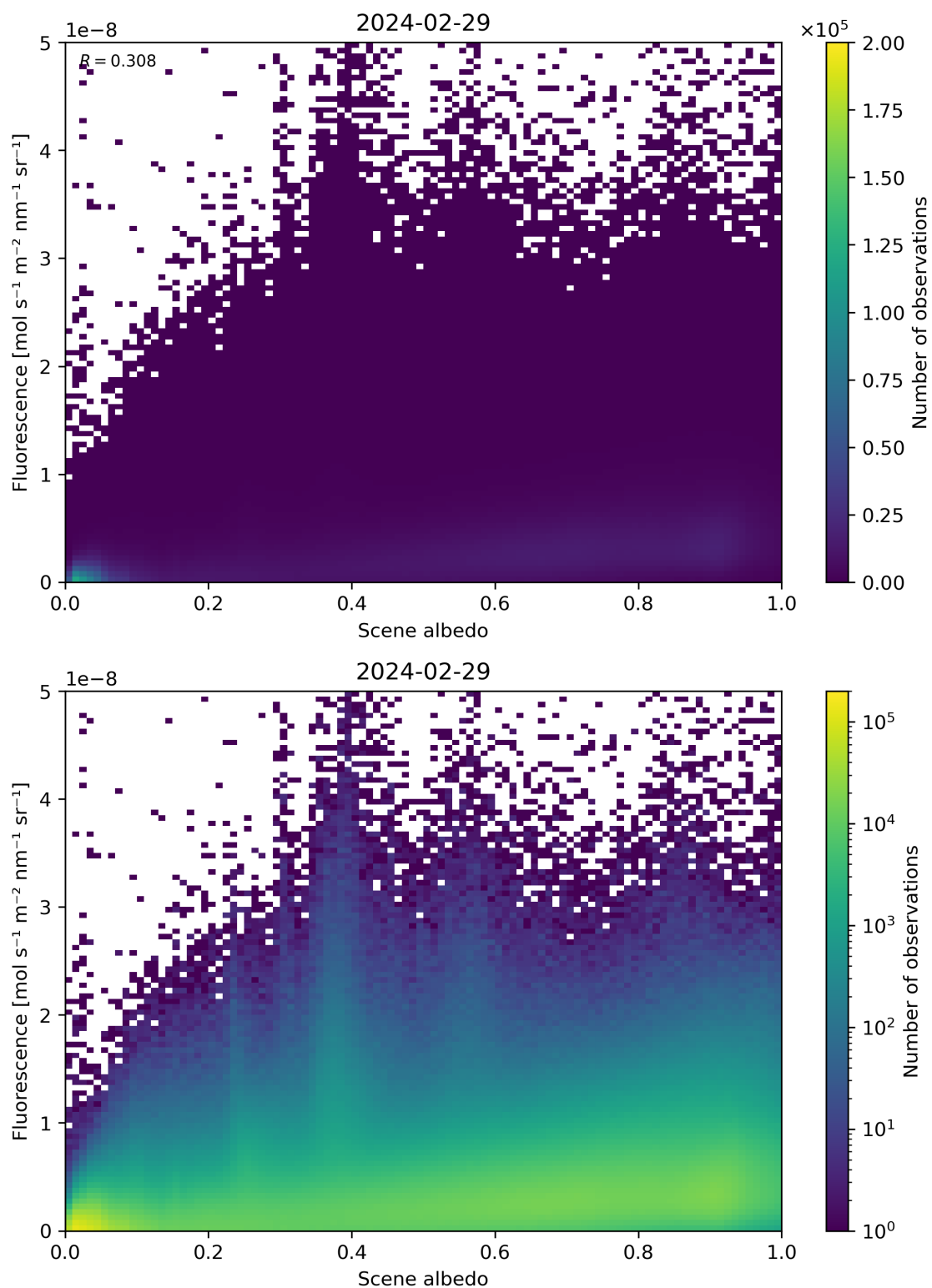
Figure 104: Scatter density plot of “Scene albedo” against “Fluorescence” for 2024-02-28 to 2024-03-01.
