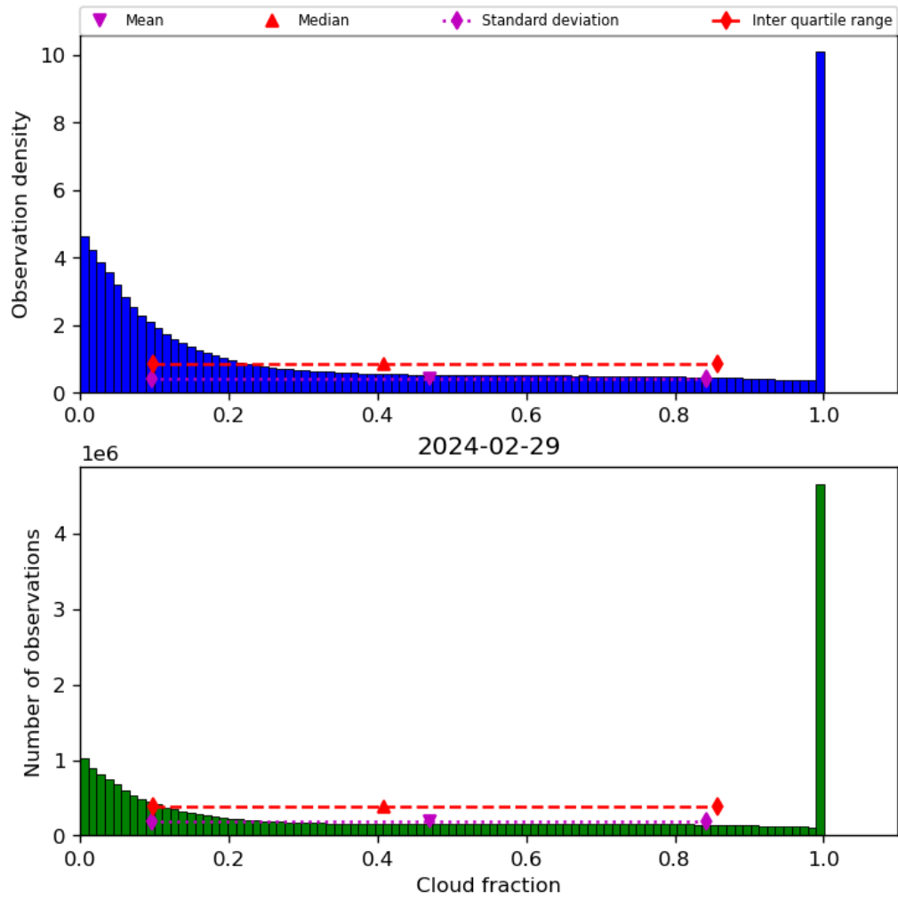
Figure 32: Histogram of “Cloud fraction” for 2024-02-28 to 2024-03-01
