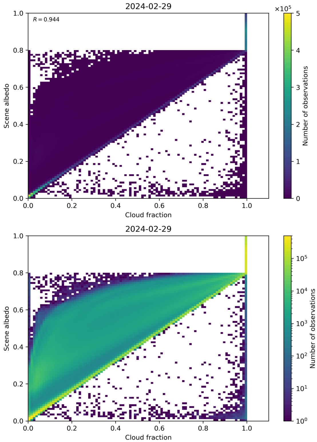
Figure 75: Scatter density plot of “Cloud fraction” against “Scene albedo” for 2024-02-28 to 2024-03-01.
