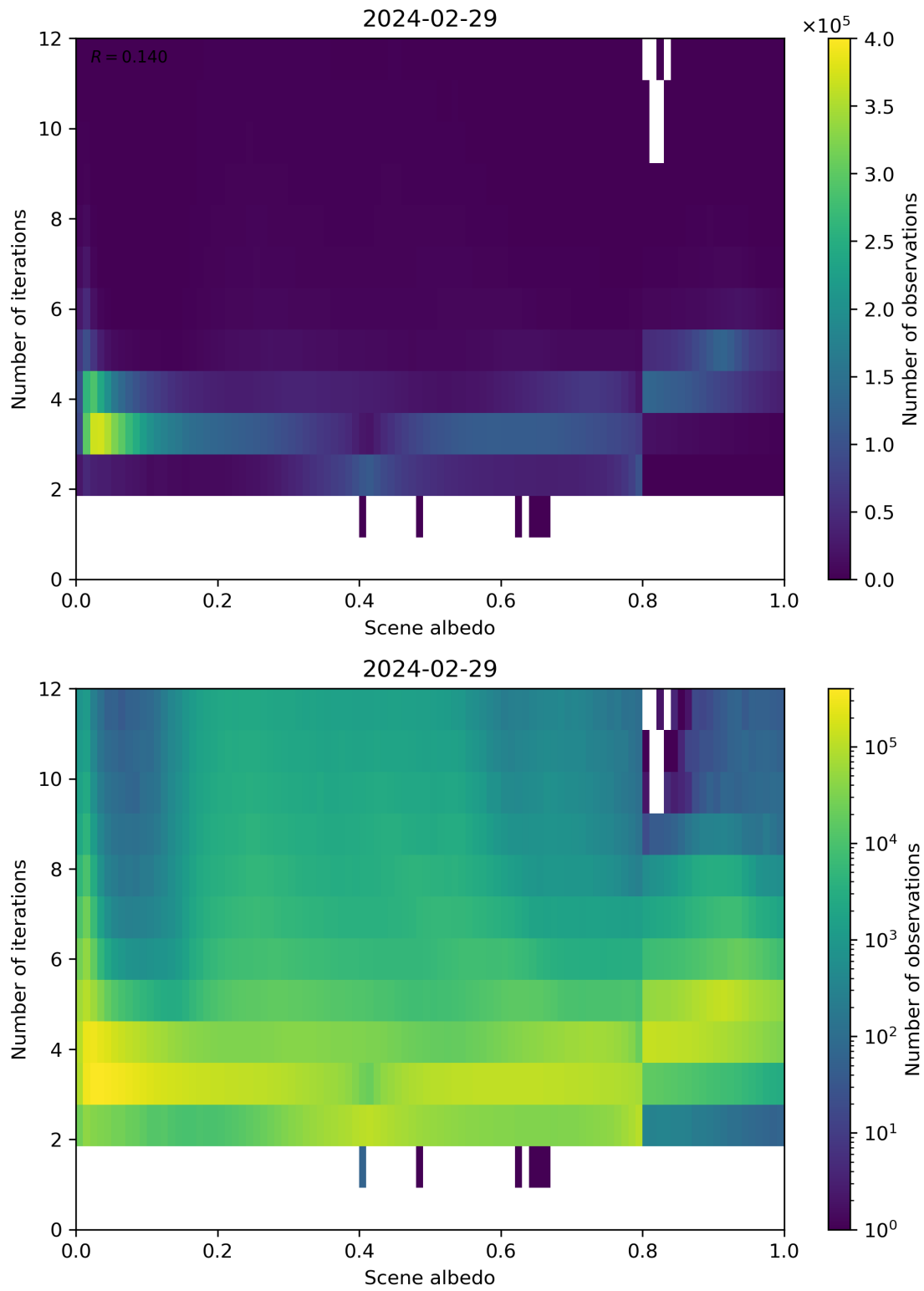
Figure 105: Scatter density plot of “Scene albedo” against “Number of iterations” for 2024-02-28 to 2024-03-01.
