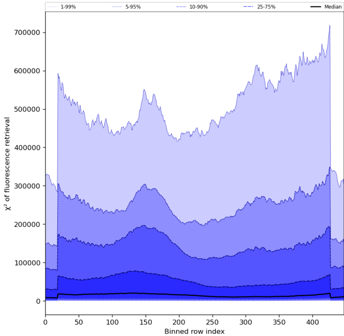
Figure 59: Along track statistics of “ \chi^2 of fluorescence retrieval” for 2024-02-28 to 2024-03-01
