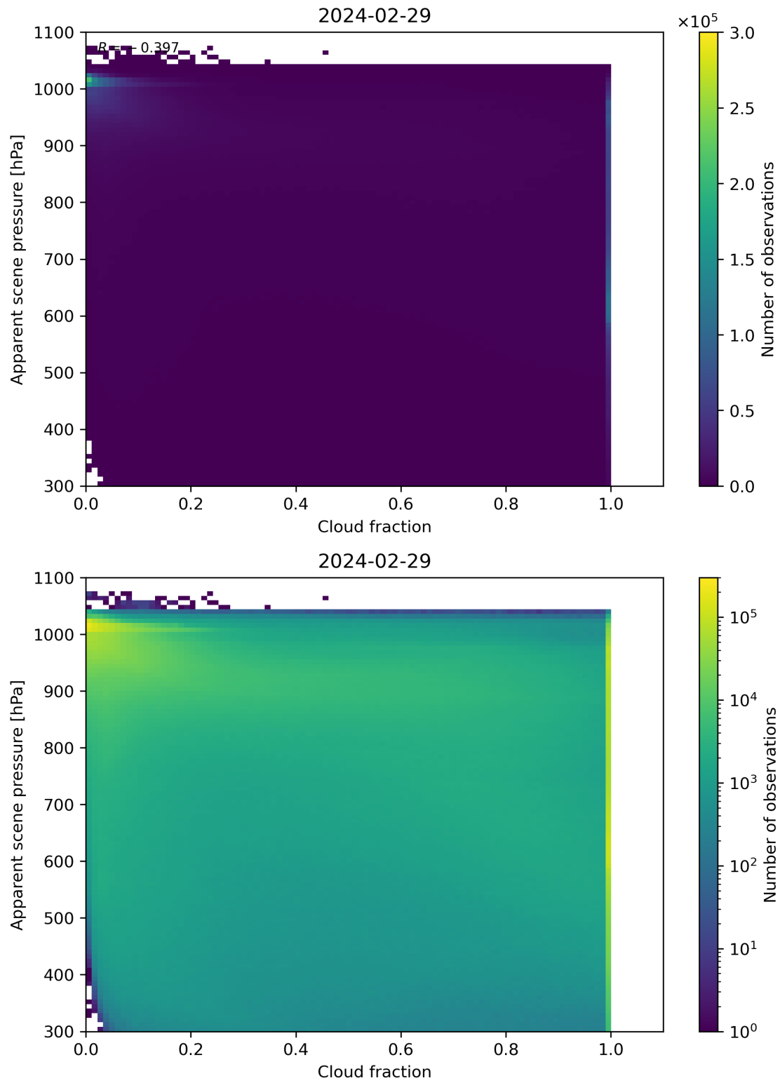
Figure 70: Scatter density plot of “Cloud fraction” against “Apparent scene pressure” for 2024-02-28 to 2024-03-01.
