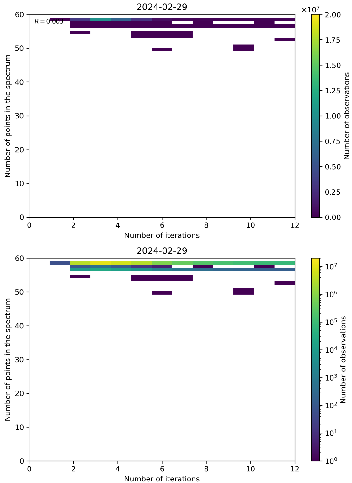
Figure 99: Scatter density plot of “Number of iterations” against “Number of points in the spectrum” for 2024-02-28 to 2024-03-01.
