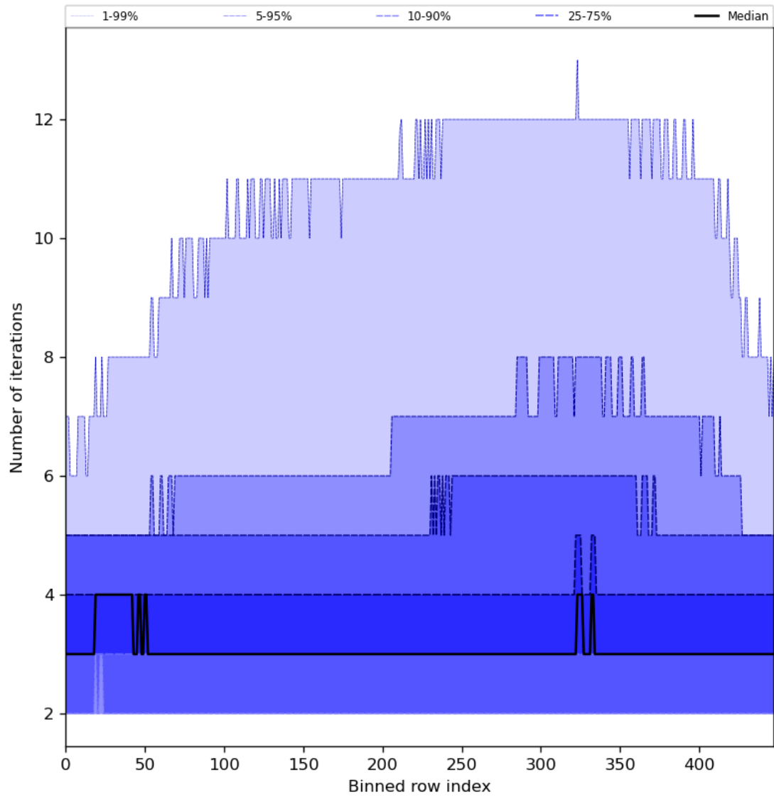
Figure 56: Along track statistics of “Number of iterations” for 2024-02-28 to 2024-03-01
