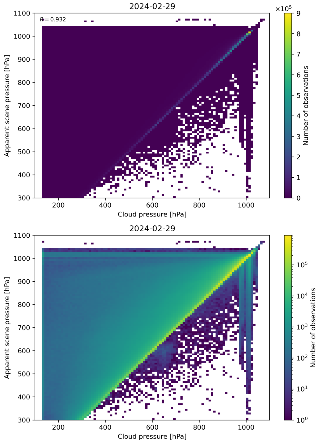
Figure 77: Scatter density plot of “Cloud pressure” against “Apparent scene pressure” for 2024-02-28 to 2024-03-01.
