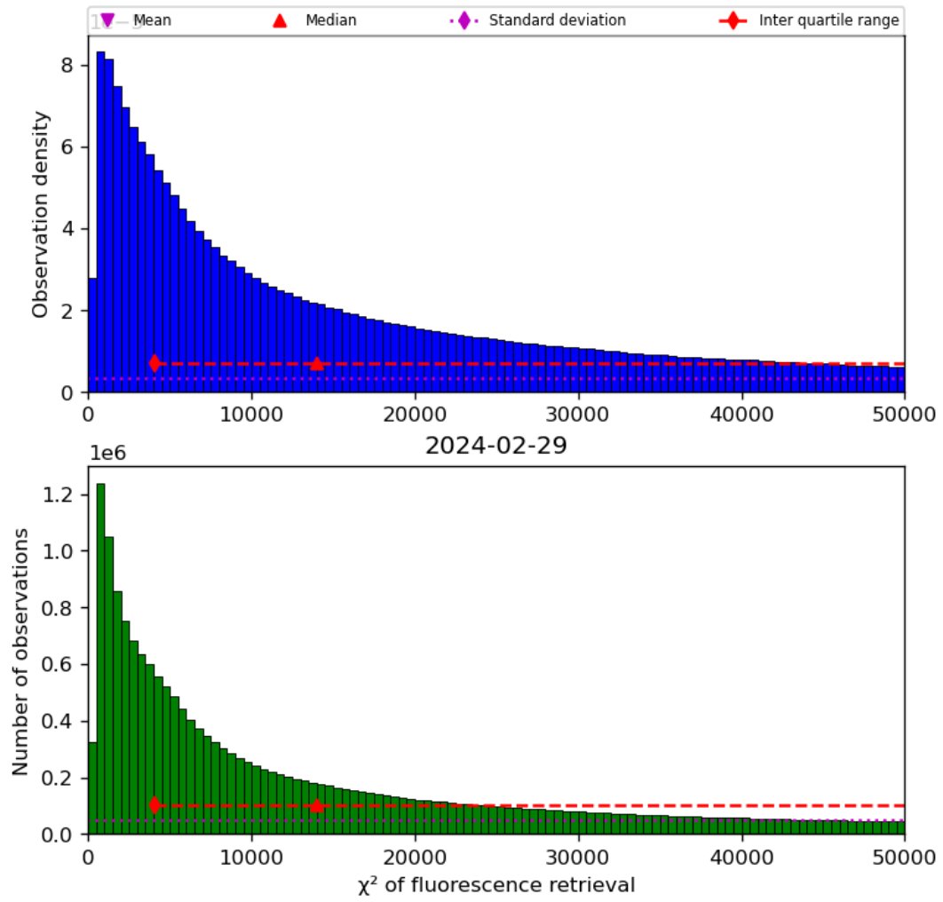
Figure 42: Histogram of “ \chi^2 of fluorescence retrieval” for 2024-02-28 to 2024-03-01
