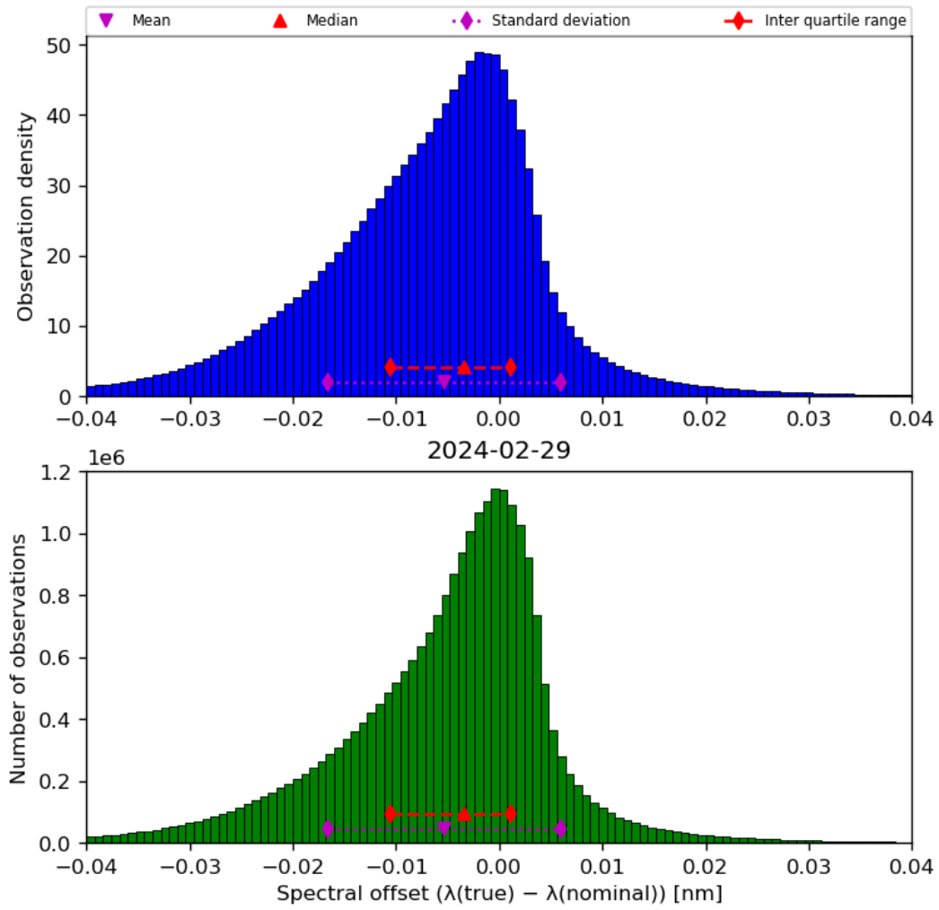
Figure 45: Histogram of “Spectral offset ( \lambda(\text{true}) - \lambda(\text{nominal}) )” for 2024-02-28 to 2024-03-01
