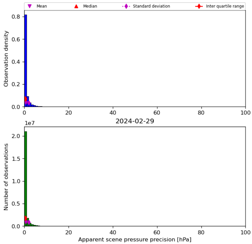
Figure 37: Histogram of “Apparent scene pressure precision” for 2024-02-28 to 2024-03-01
