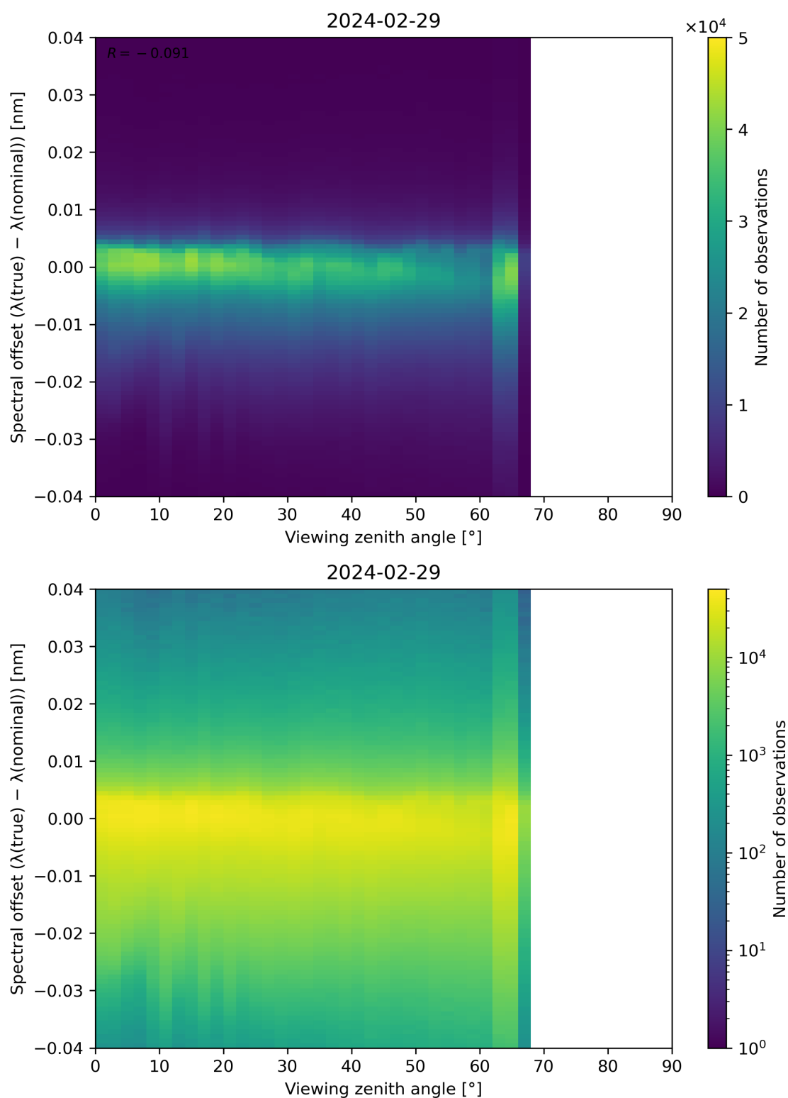
Figure 128: Scatter density plot of “Viewing zenith angle” against “Spectral offset ( \lambda(\text{true}) - \lambda(\text{nominal}) )” for 2024-02-28 to 2024-03-01.
