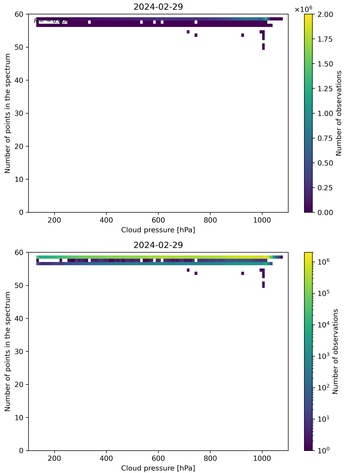
Figure 82: Scatter density plot of “Cloud pressure” against “Number of points in the spectrum” for 2024-02-28 to 2024-03-01.
