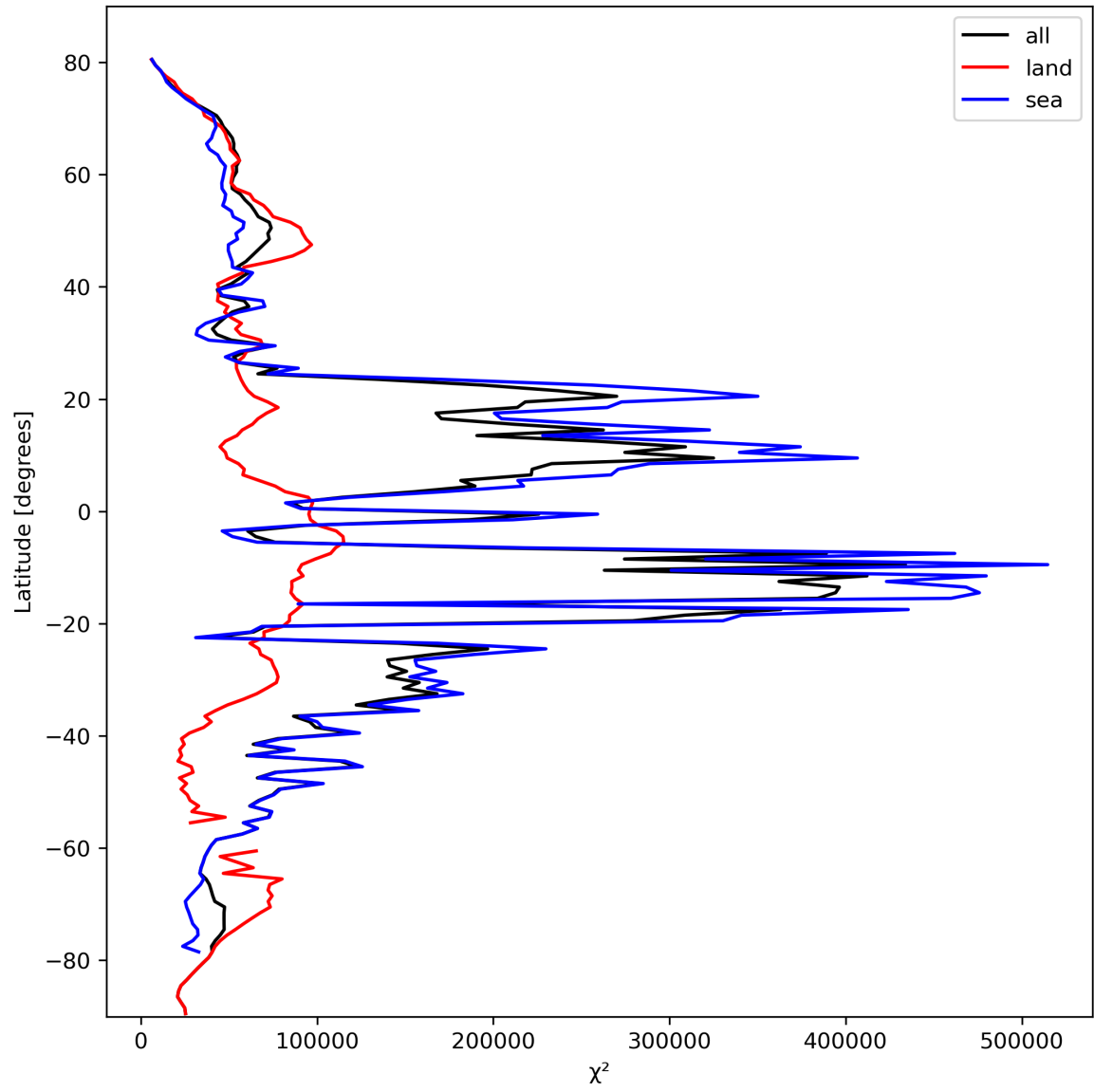
Figure 21: Zonal average of “ \chi^2 ” for 2024-02-28 to 2024-03-01.
