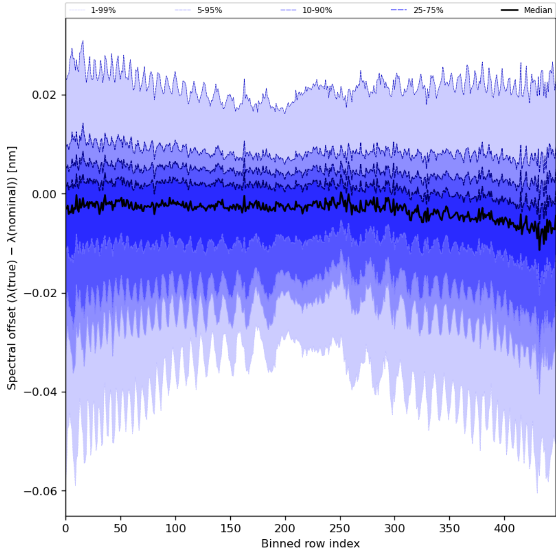
Figure 62: Along track statistics of “Spectral offset ( \lambda(\text{true}) - \lambda(\text{nominal}) )” for 2024-02-28 to 2024-03-01
