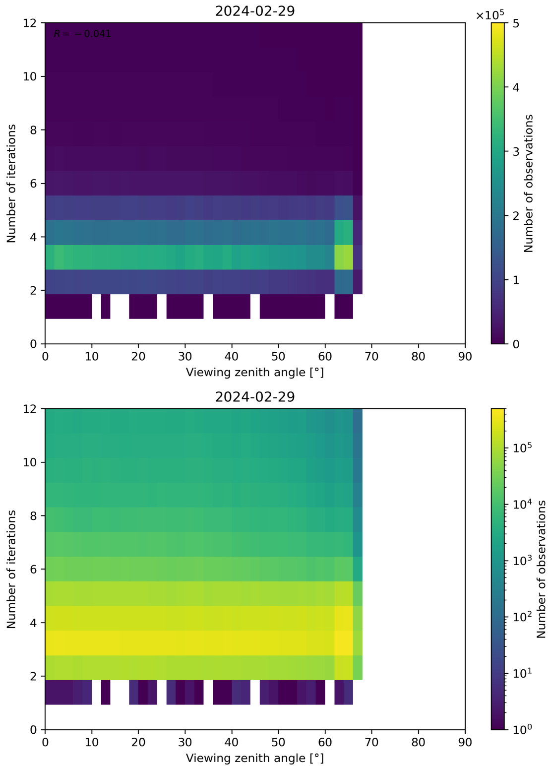
Figure 124: Scatter density plot of “Viewing zenith angle” against “Number of iterations” for 2024-02-28 to 2024-03-01.
