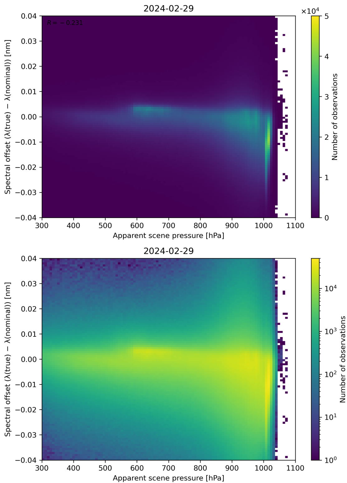
Figure 67: Scatter density plot of “Apparent scene pressure” against “Spectral offset ( \lambda(\text{true}) - \lambda(\text{nominal}) )” for 2024-02-28 to 2024-03-01.
