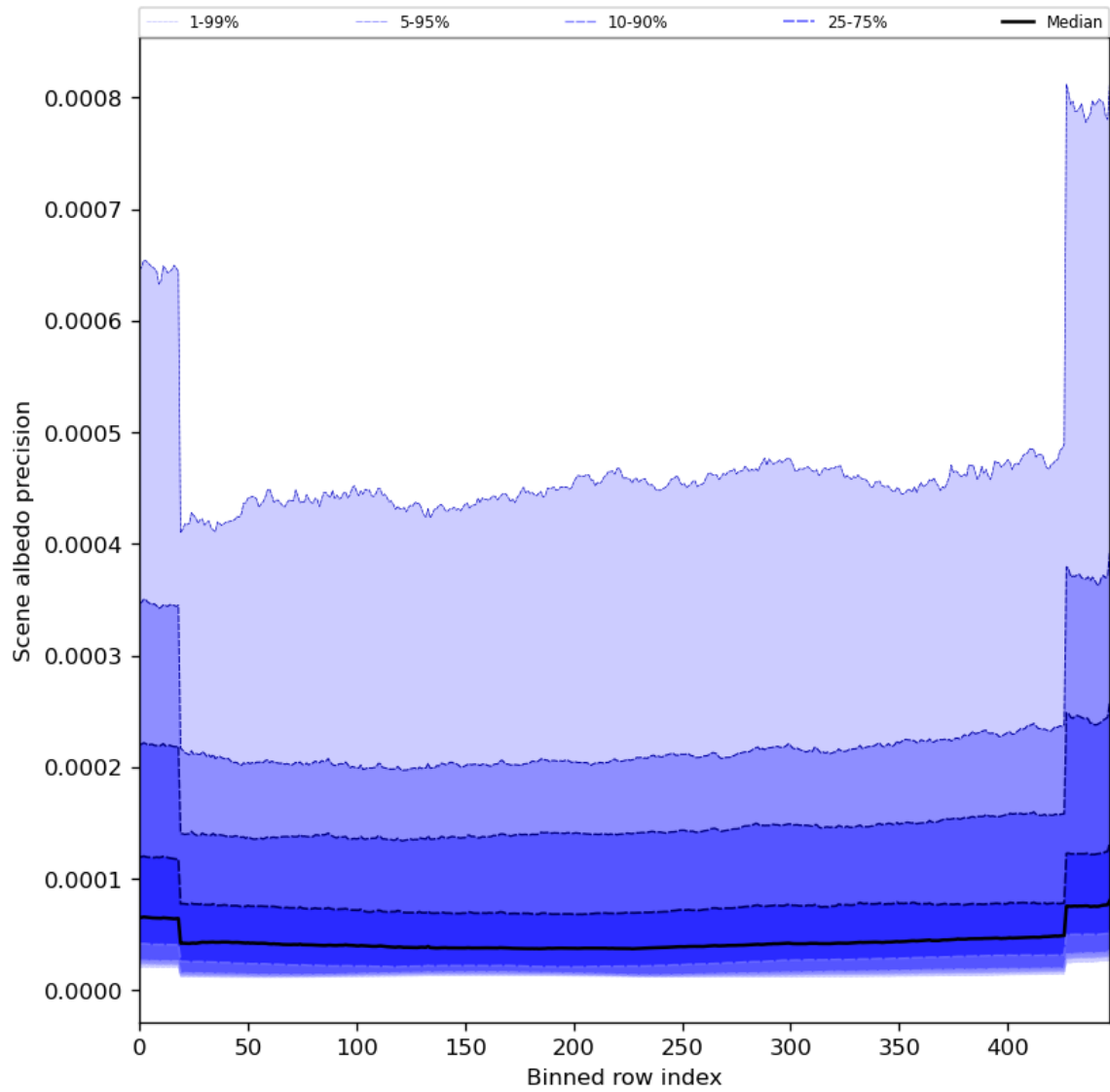
Figure 52: Along track statistics of “Scene albedo precision” for 2024-02-28 to 2024-03-01
